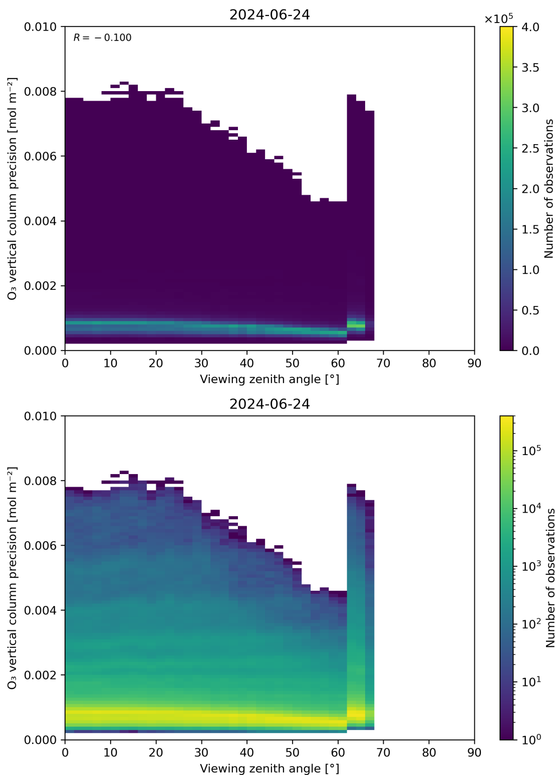
Figure 53: Scatter density plot of “Viewing zenith angle” against “O 3 vertical column precision” for 2024-06-24 to 2024-06-25.
