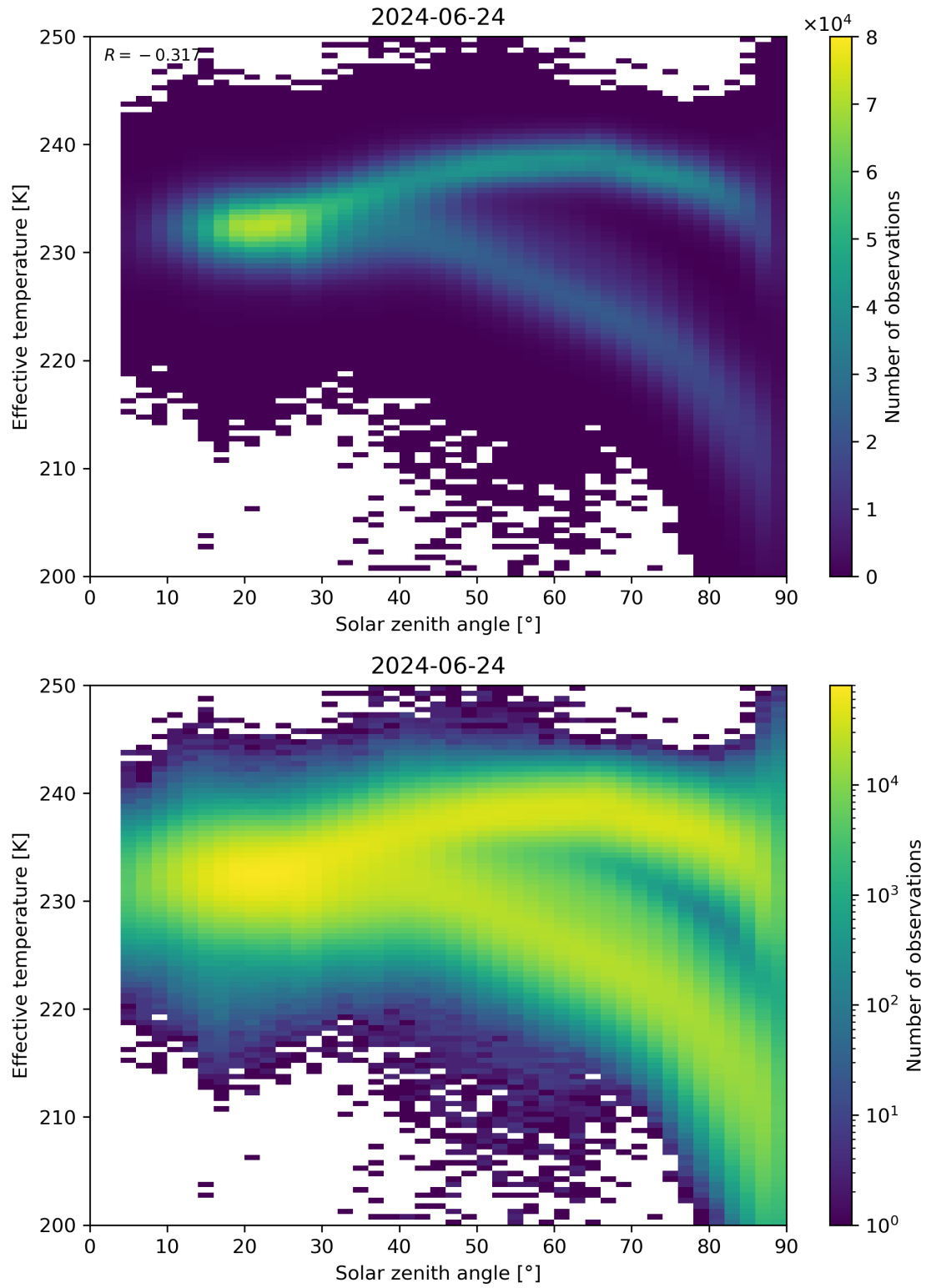
Figure 45: Scatter density plot of “Solar zenith angle” against “Effective temperature” for 2024-06-24 to 2024-06-25.
