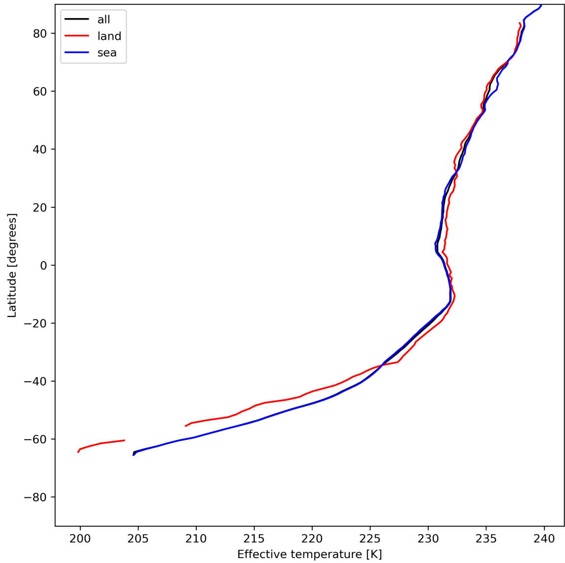
Figure 17: Zonal average of “Effective temperature” for 2024-06-24 to 2024-06-25.
