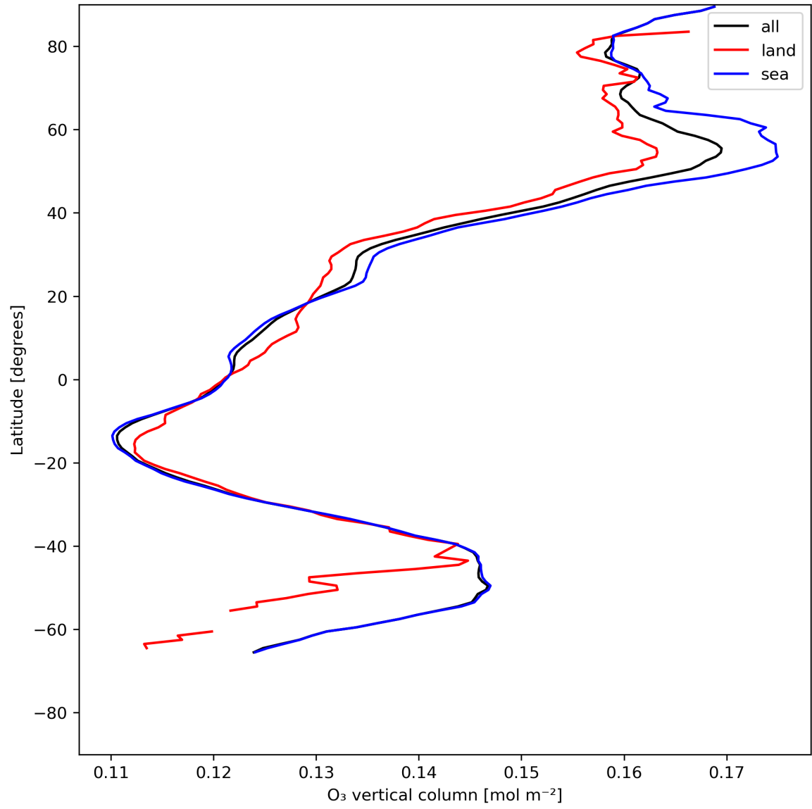
Figure 14: Zonal average of “O 3 vertical column” for 2024-06-24 to 2024-06-25.
