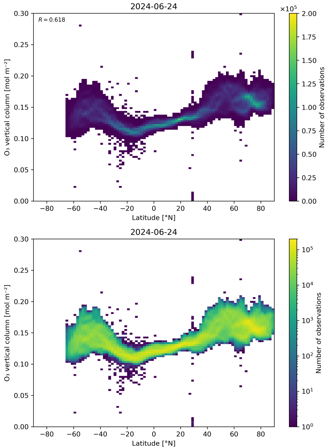
Figure 36: Scatter density plot of “Latitude” against “O 3 vertical column” for 2024-06-24 to 2024-06-25.
