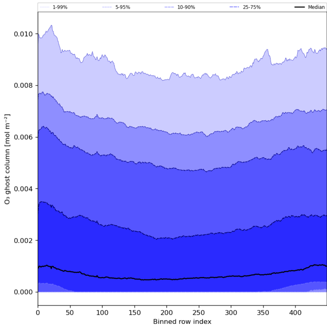
Figure 32: Along track statistics of “O 3 ghost column” for 2024-06-24 to 2024-06-25
