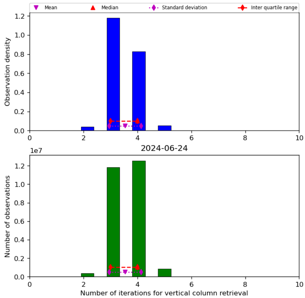
Figure 26: Histogram of “Number of iterations for vertical column retrieval” for 2024-06-24 to 2024-06-25
