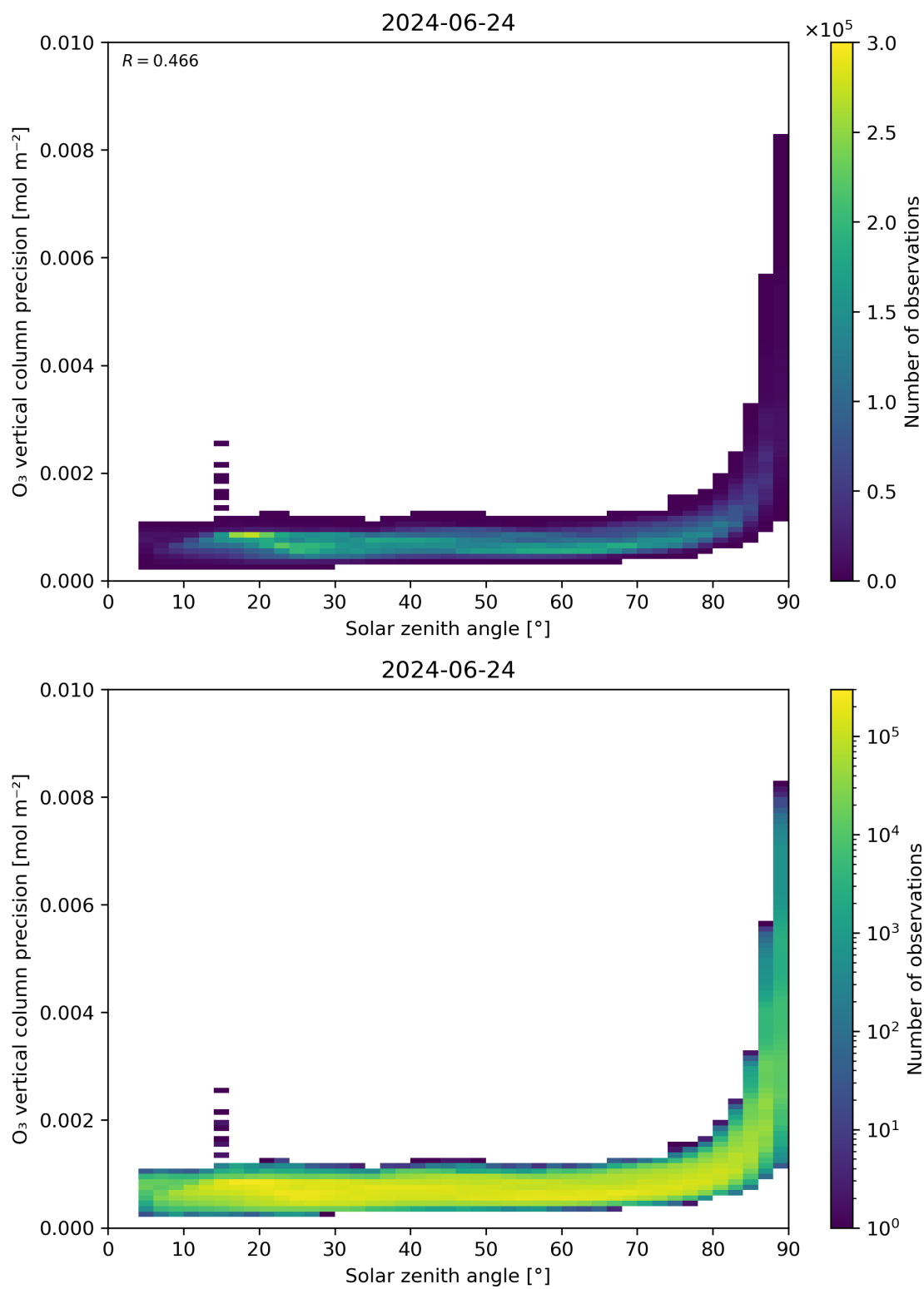
Figure 48: Scatter density plot of “Solar zenith angle” against “O 3 vertical column precision” for 2024-06-24 to 2024-06-25.
