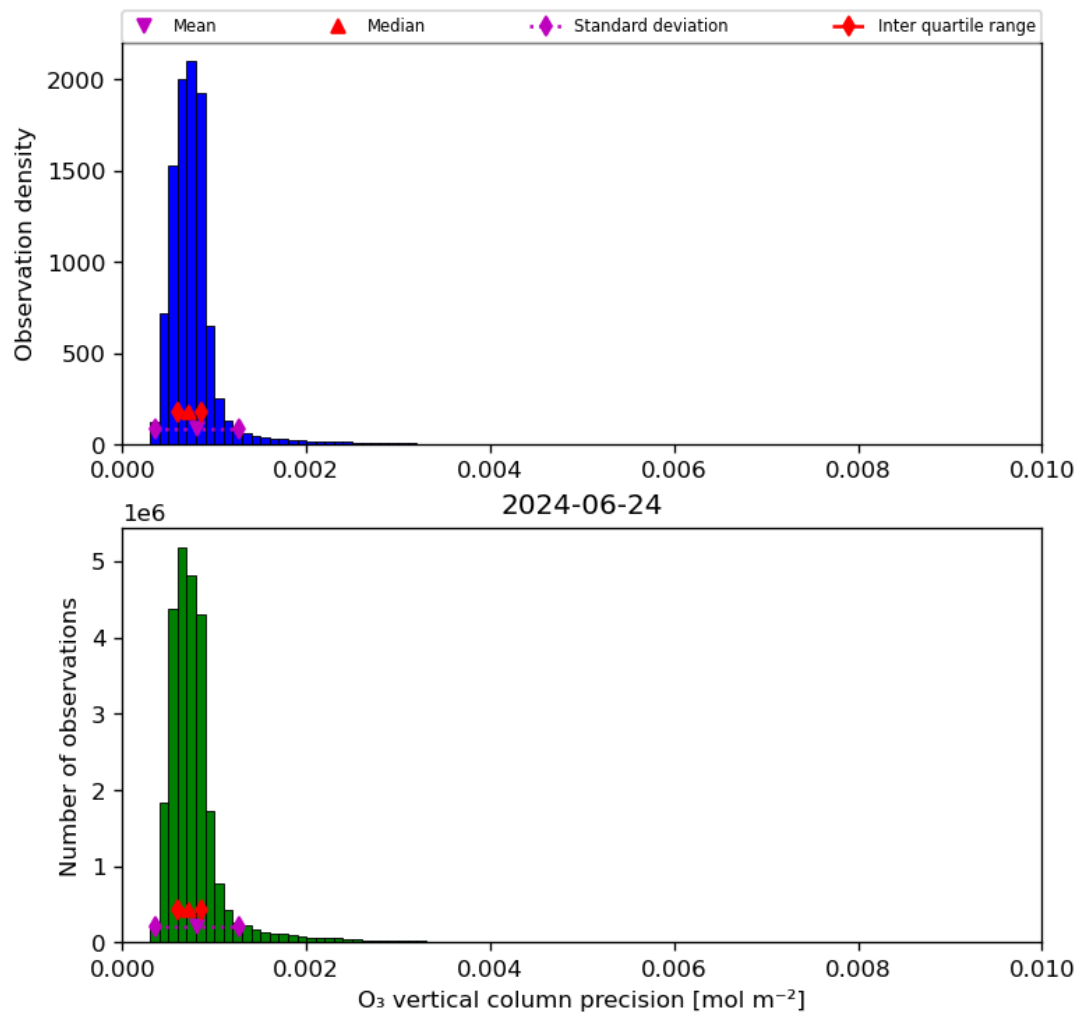
Figure 22: Histogram of “O 3 vertical column precision” for 2024-06-24 to 2024-06-25
