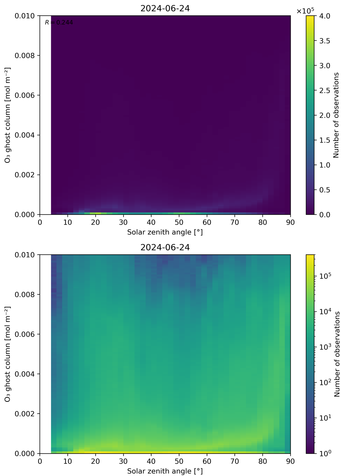
Figure 46: Scatter density plot of “Solar zenith angle” against “O 3 ghost column” for 2024-06-24 to 2024-06-25.
