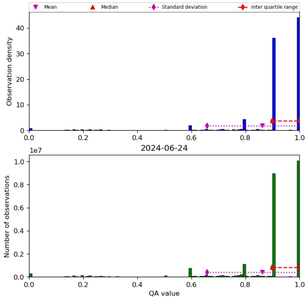
Figure 20: Histogram of “QA value” for 2024-06-24 to 2024-06-25
