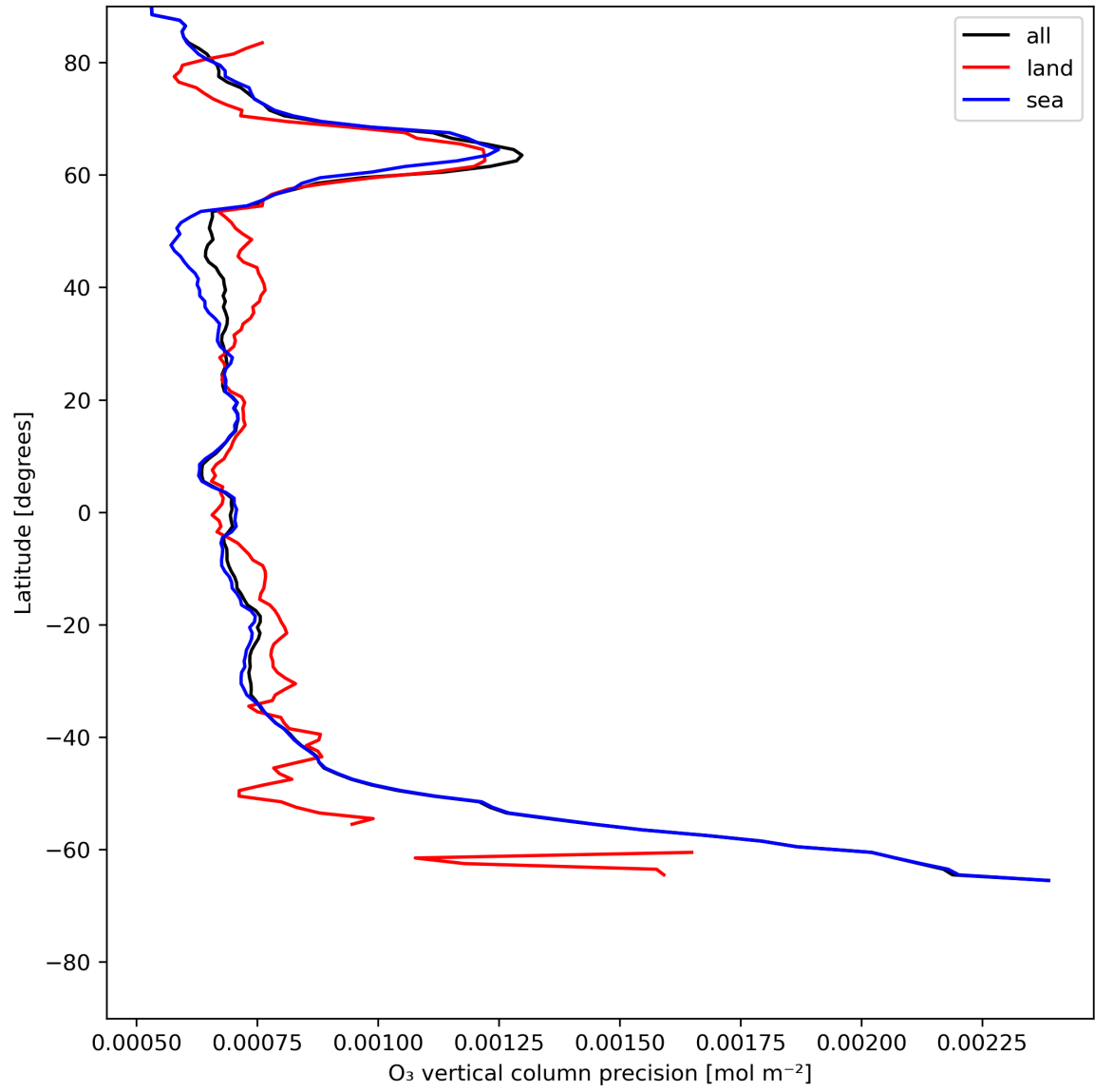
Figure 15: Zonal average of “O 3 vertical column precision” for 2024-06-24 to 2024-06-25.
