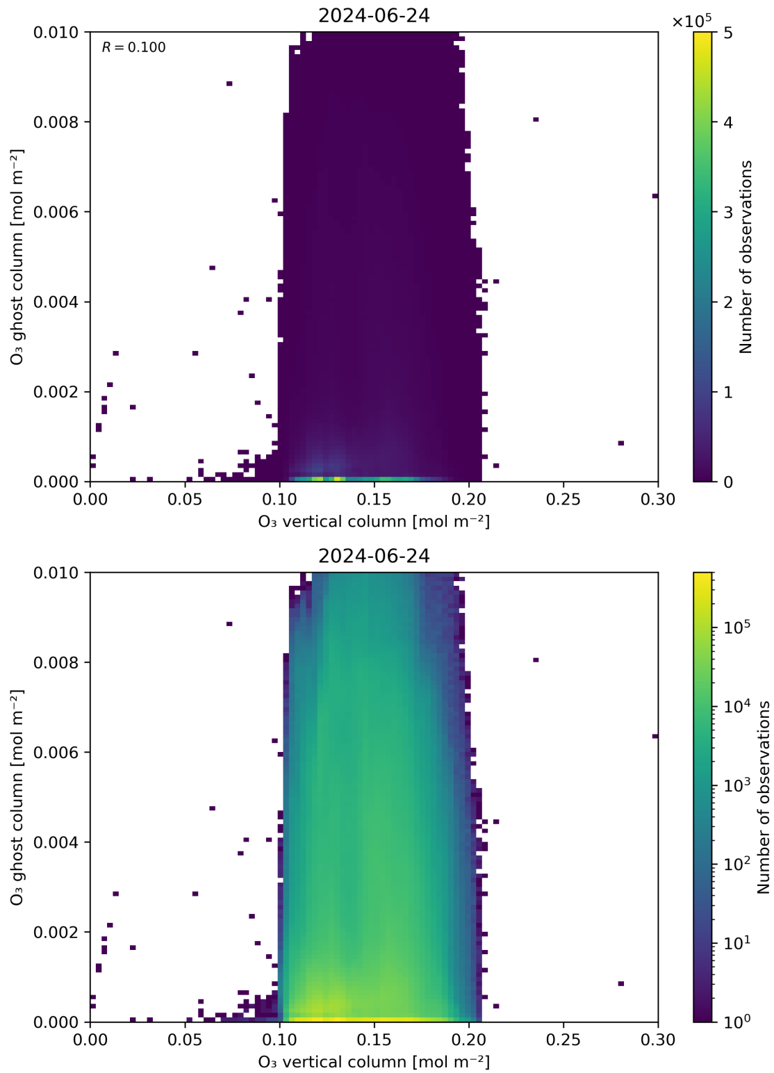
Figure 40: Scatter density plot of “O 3 vertical column” against “O 3 ghost column” for 2024-06-24 to 2024-06-25.
