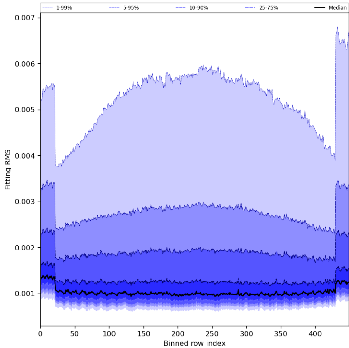
Figure 30: Along track statistics of “Fitting RMS” for 2024-06-24 to 2024-06-25
