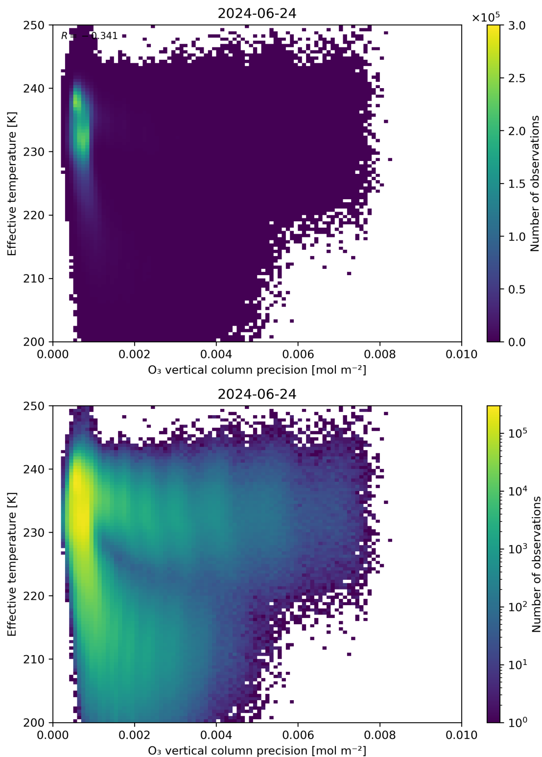
Figure 42: Scatter density plot of “O 3 vertical column precision” against “Effective temperature” for 2024-06-24 to 2024-06-25.
