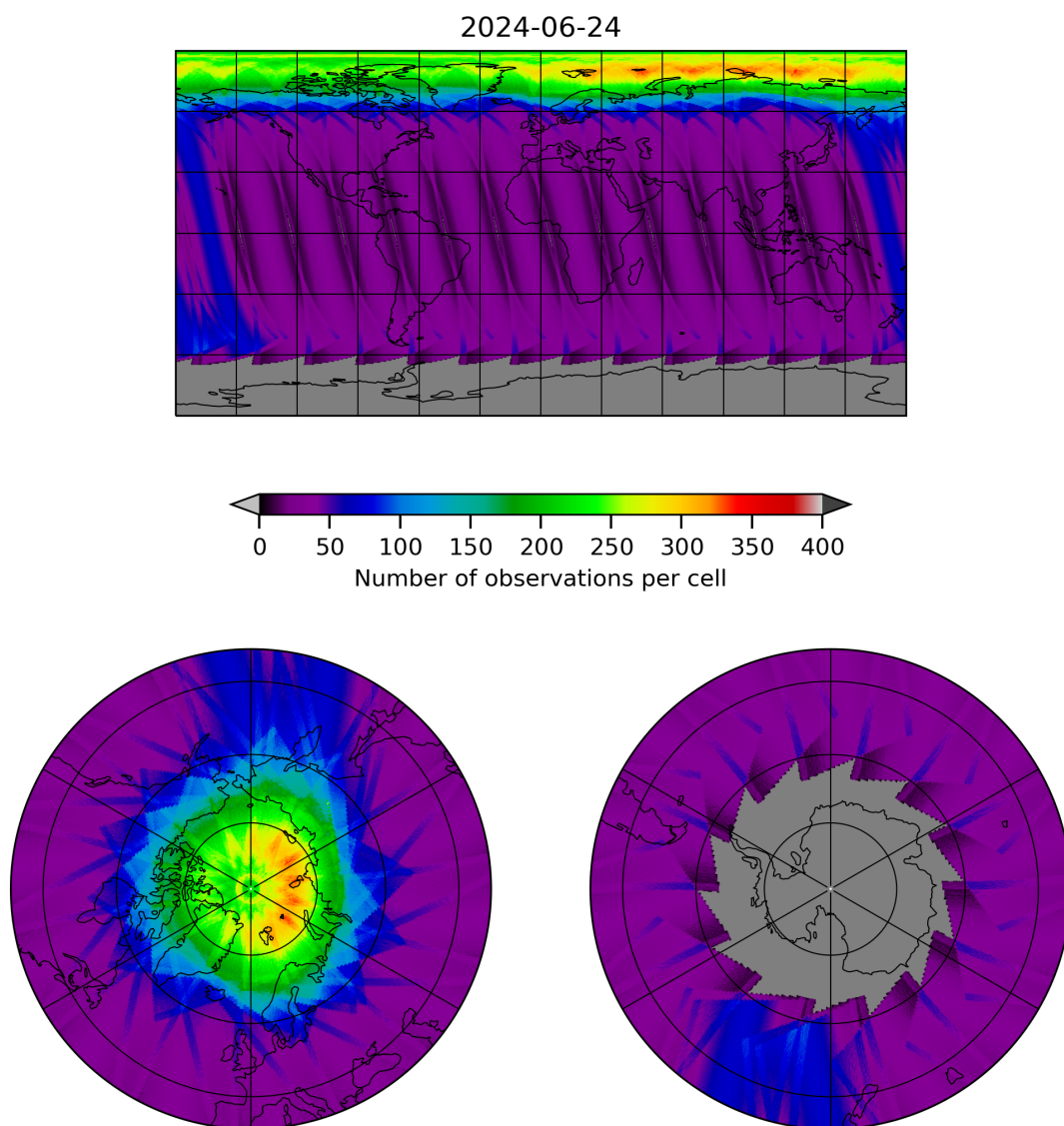
Figure 12: Map of the number of observations for 2024-06-24 to 2024-06-25
