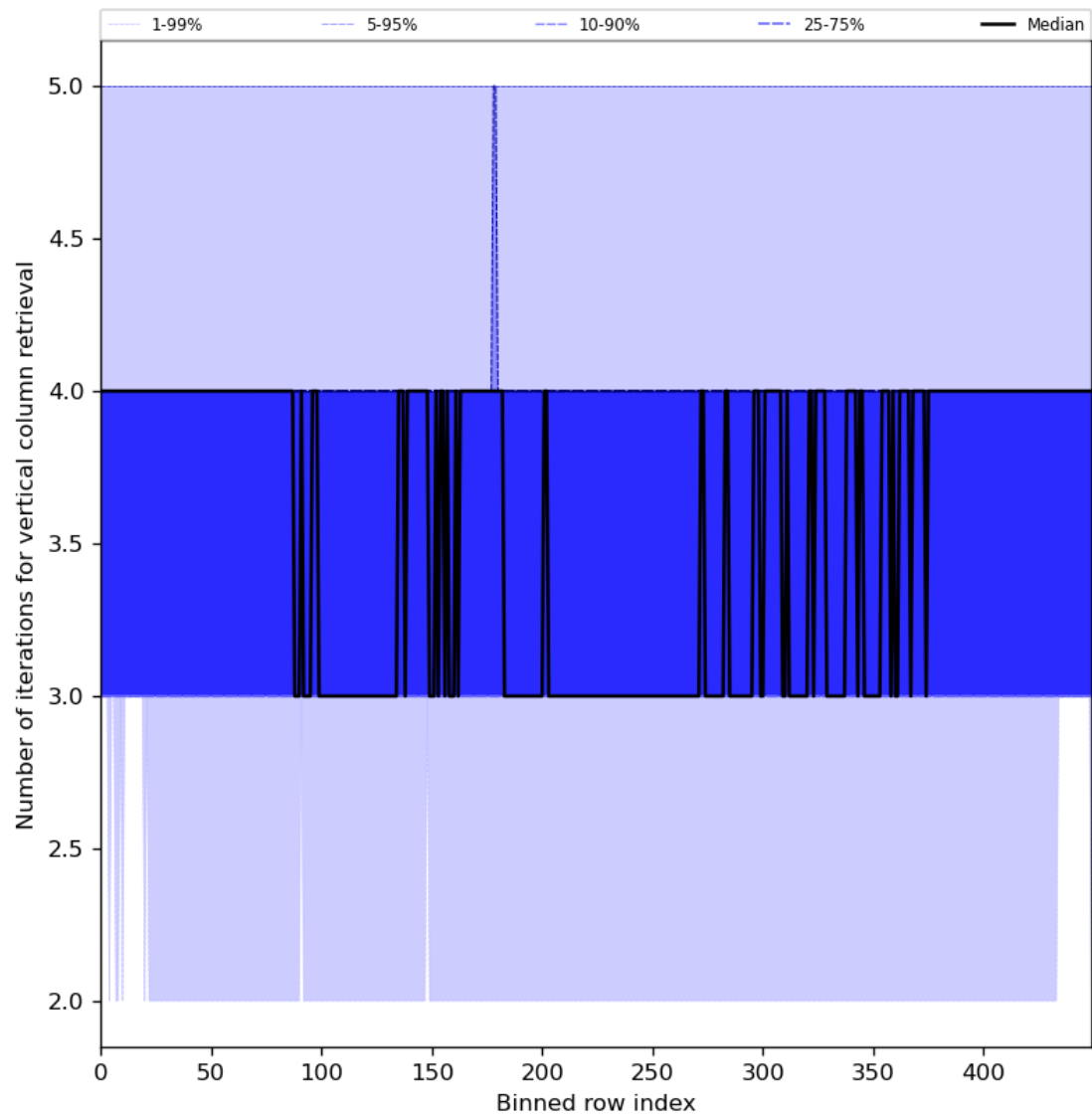
Figure 33: Along track statistics of “Number of iterations for vertical column retrieval” for 2024-06-24 to 2024-06-25
