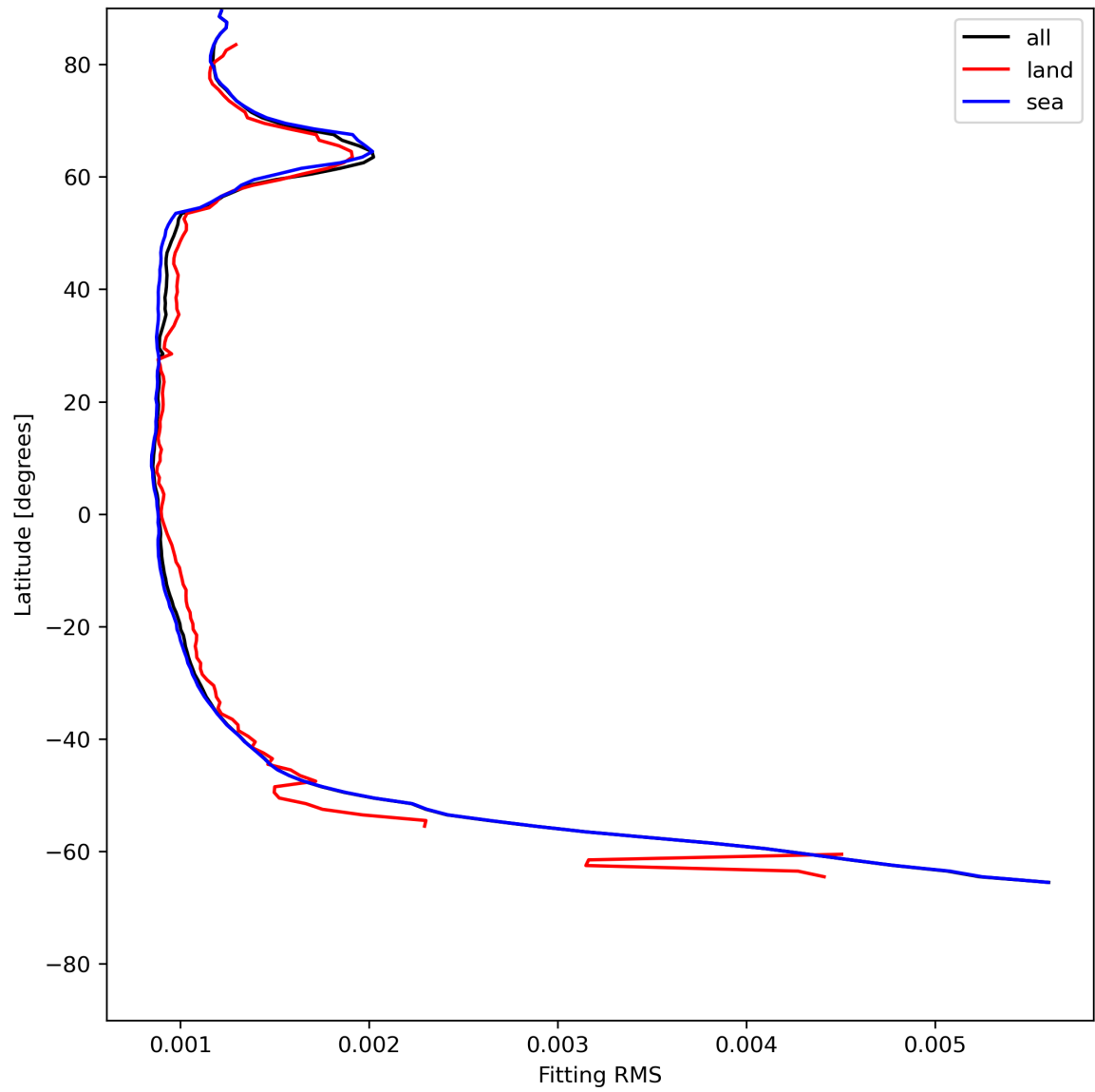
Figure 16: Zonal average of “Fitting RMS” for 2024-06-24 to 2024-06-25.
