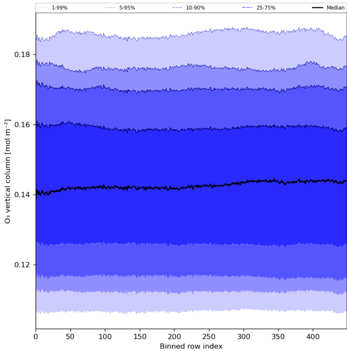
Figure 28: Along track statistics of “O 3 vertical column” for 2024-06-24 to 2024-06-25
