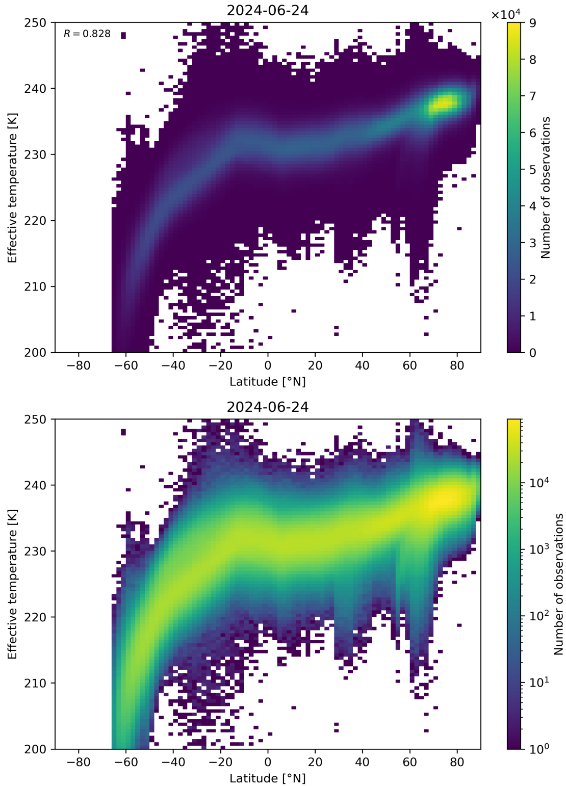
Figure 34: Scatter density plot of “Latitude” against “Effective temperature” for 2024-06-24 to 2024-06-25.
