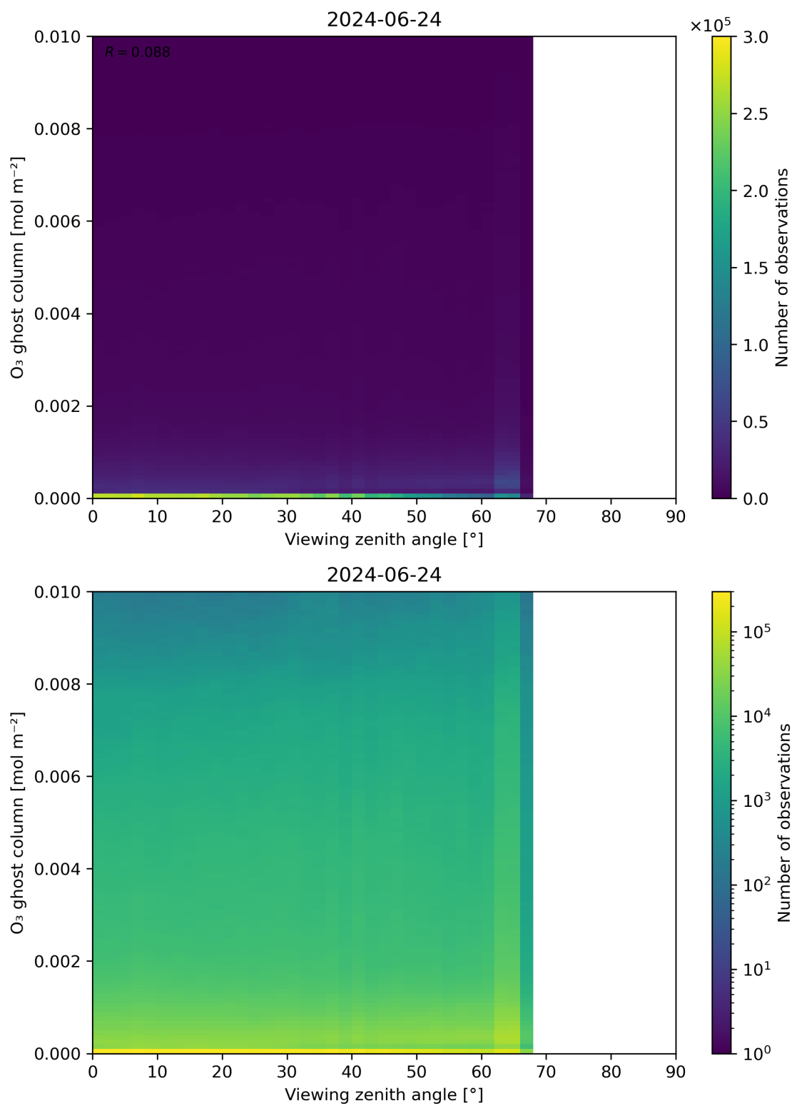
Figure 51: Scatter density plot of “Viewing zenith angle” against “O 3 ghost column” for 2024-06-24 to 2024-06-25.
