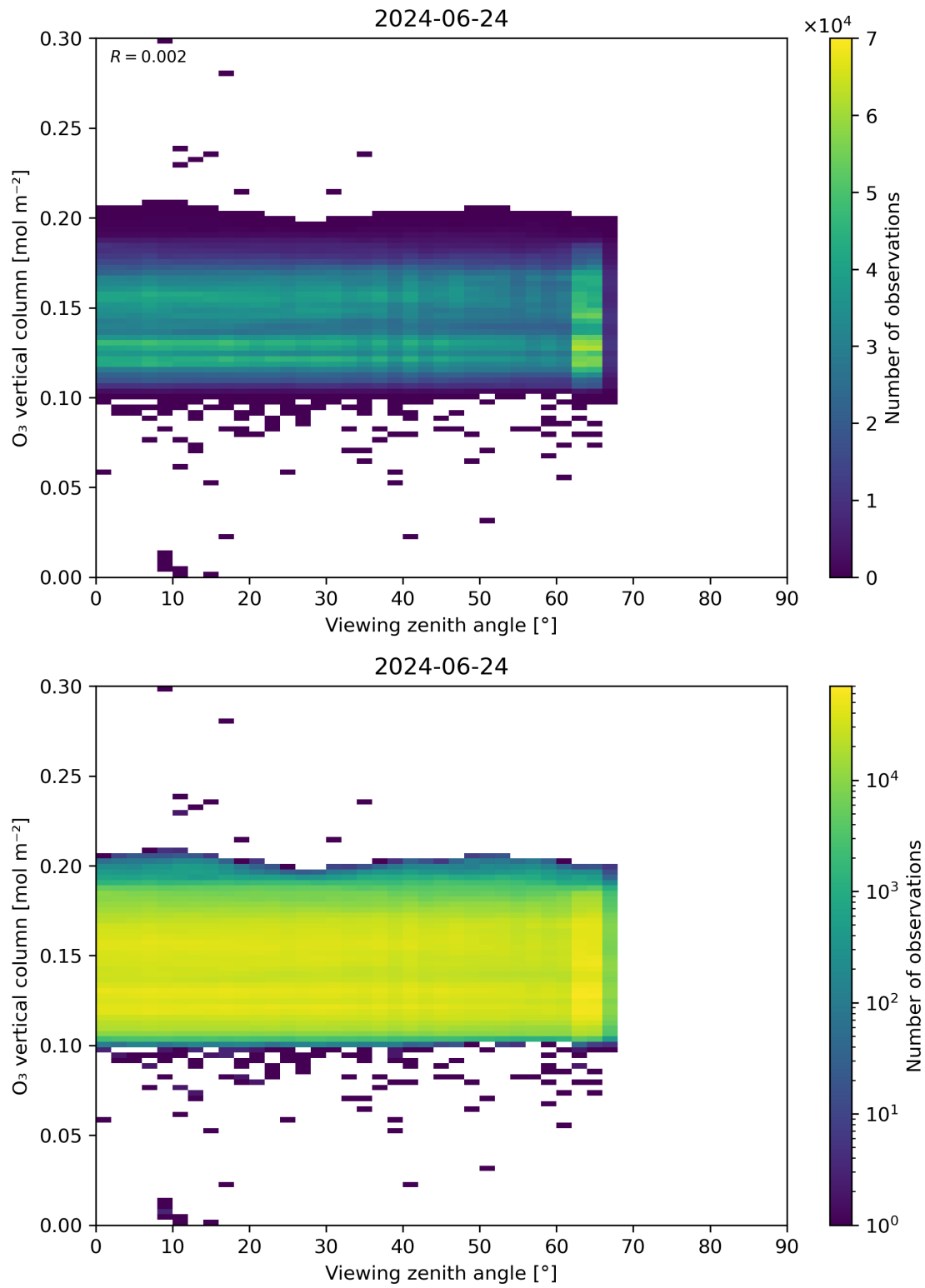
Figure 52: Scatter density plot of “Viewing zenith angle” against “O 3 vertical column” for 2024-06-24 to 2024-06-25.
