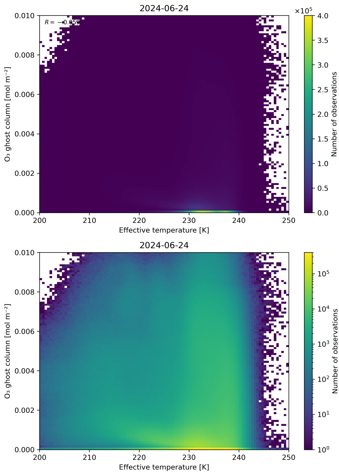
Figure 38: Scatter density plot of “Effective temperature” against “O 3 ghost column” for 2024-06-24 to 2024-06-25.
