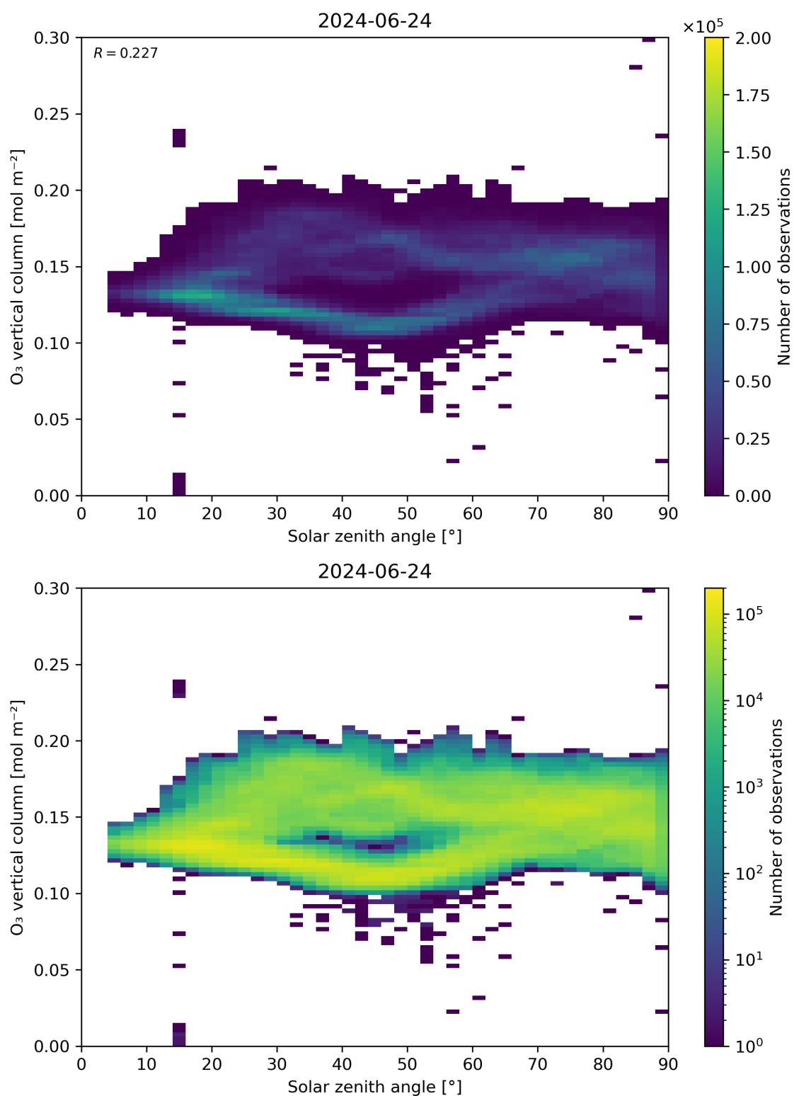
Figure 47: Scatter density plot of “Solar zenith angle” against “O 3 vertical column” for 2024-06-24 to 2024-06-25.
