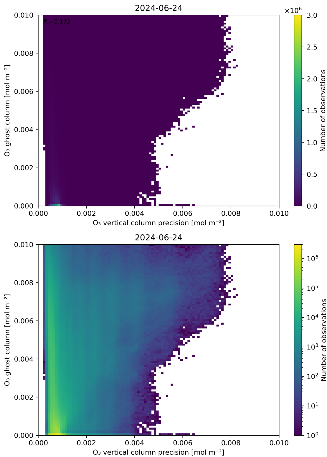
Figure 43: Scatter density plot of “ \text{O}_3 vertical column precision” against “ \text{O}_3 ghost column” for 2024-06-24 to 2024-06-25.
