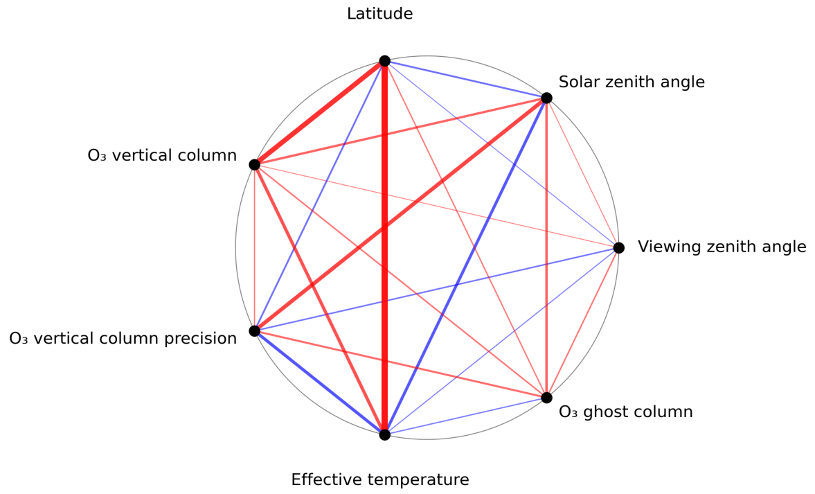
Figure 1: Map of correlation graph for 2024-06-24 to 2024-06-25.
