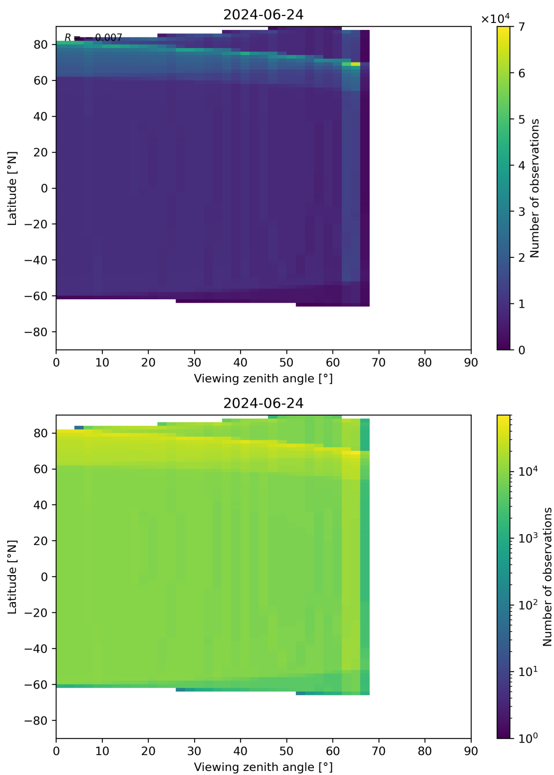
Figure 49: Scatter density plot of “Viewing zenith angle” against “Latitude” for 2024-06-24 to 2024-06-25.
