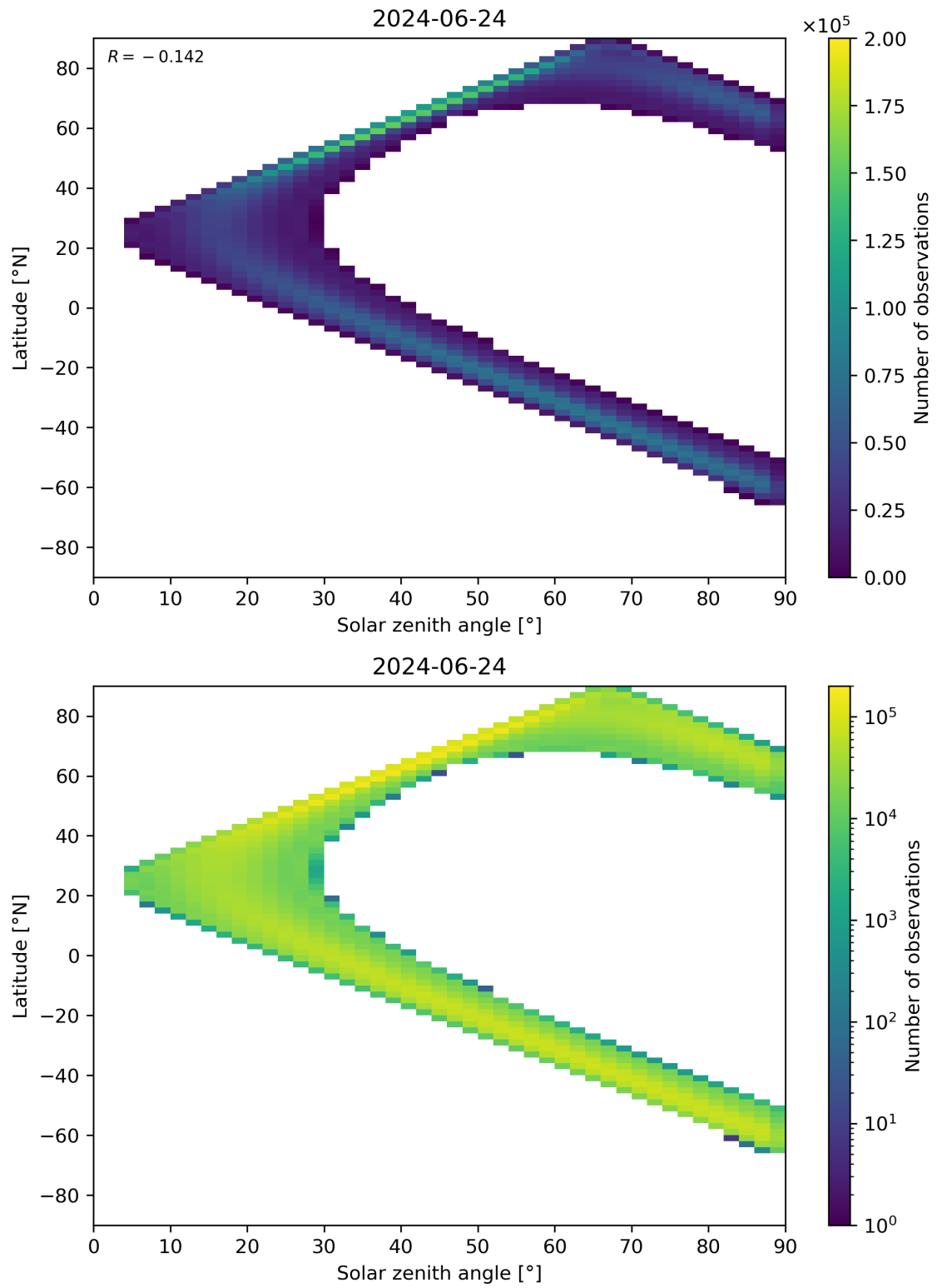
Figure 44: Scatter density plot of “Solar zenith angle” against “Latitude” for 2024-06-24 to 2024-06-25.
