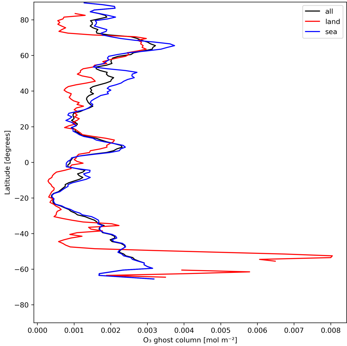
Figure 18: Zonal average of "O 3 ghost column" for 2024-06-24 to 2024-06-25.
