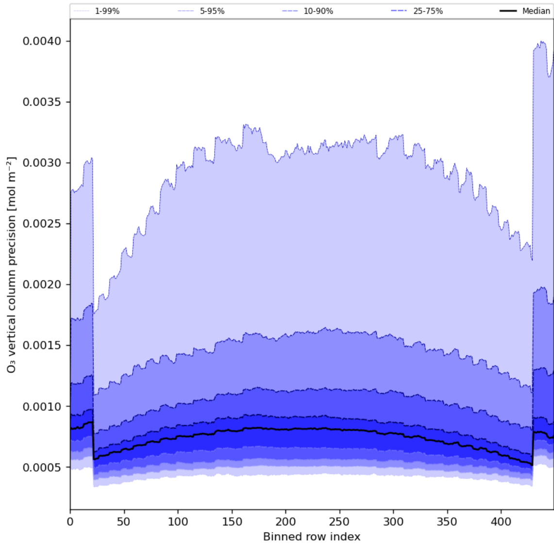
Figure 29: Along track statistics of “O 3 vertical column precision” for 2024-06-24 to 2024-06-25
