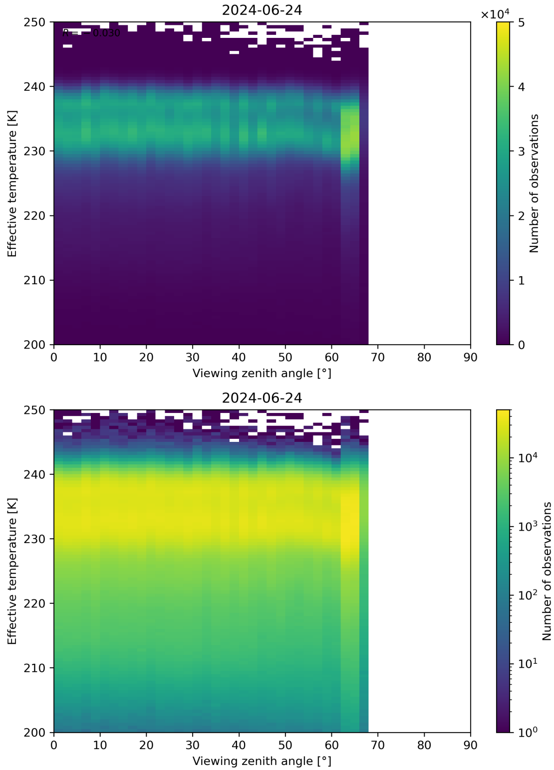
Figure 50: Scatter density plot of “Viewing zenith angle” against “Effective temperature” for 2024-06-24 to 2024-06-25.
