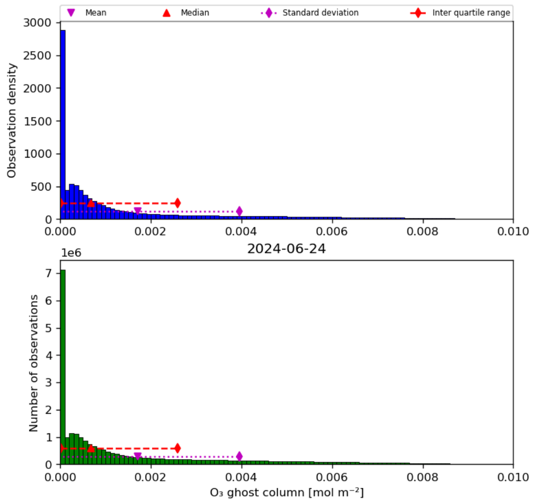
Figure 25: Histogram of “O 3 ghost column” for 2024-06-24 to 2024-06-25
