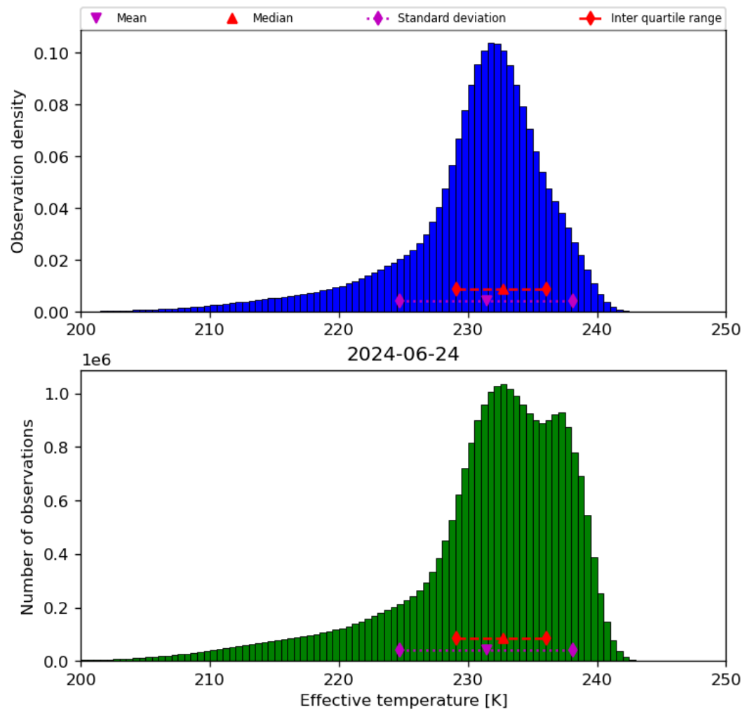
Figure 24: Histogram of “Effective temperature” for 2024-06-24 to 2024-06-25
