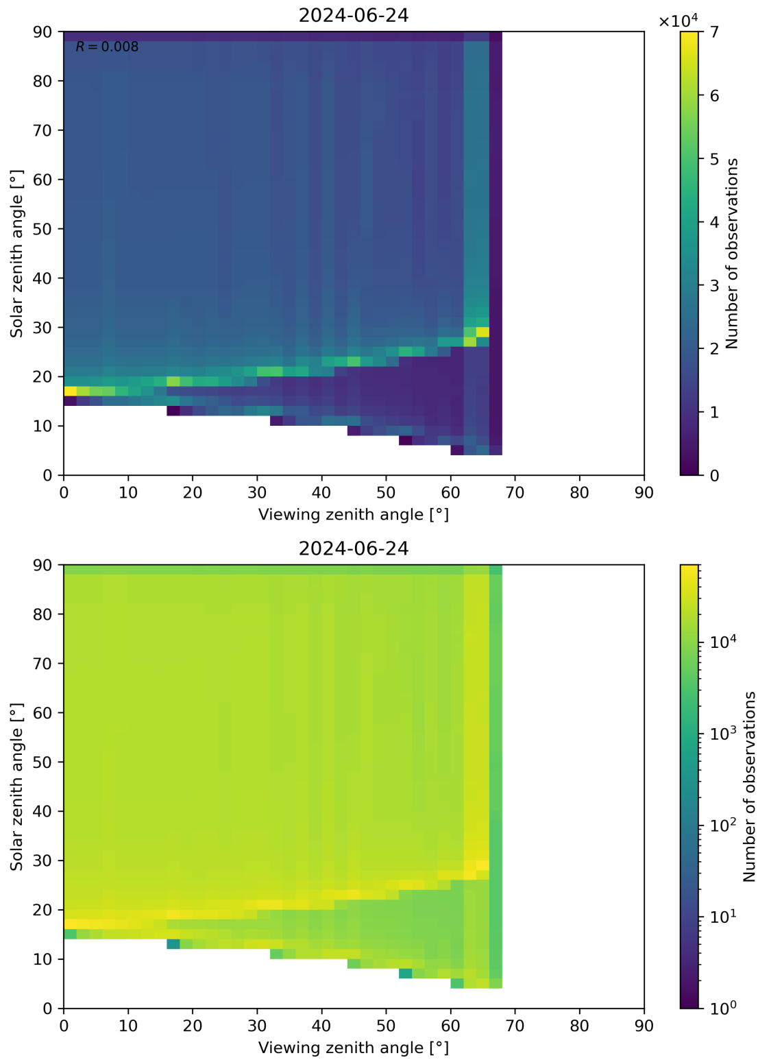
Figure 54: Scatter density plot of “Viewing zenith angle” against “Solar zenith angle” for 2024-06-24 to 2024-06-25.
