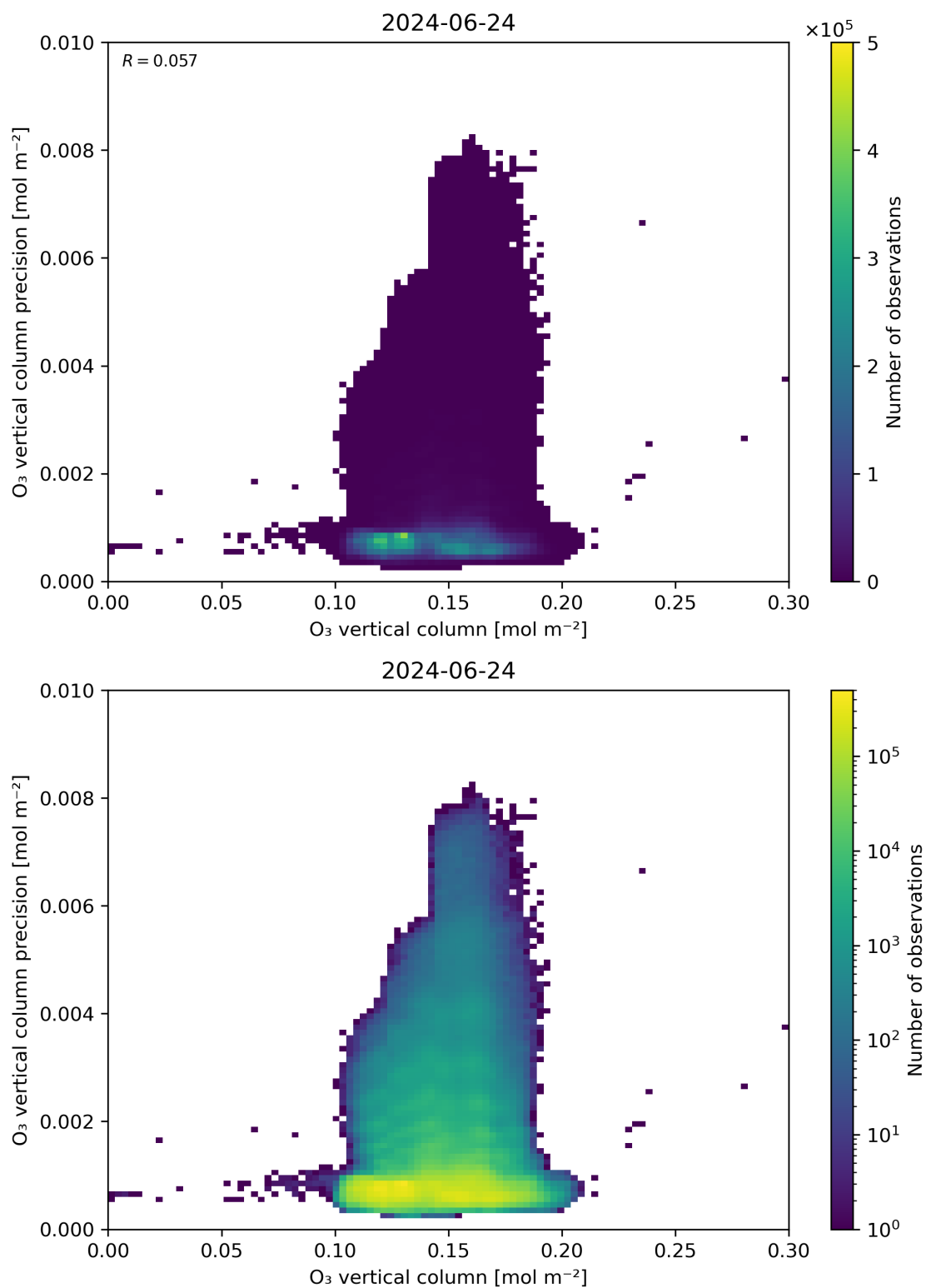
Figure 41: Scatter density plot of “O 3 vertical column” against “O 3 vertical column precision” for 2024-06-24 to 2024-06-25.
