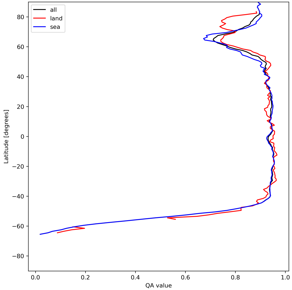
Figure 13: Zonal average of “QA value” for 2024-06-24 to 2024-06-25.
