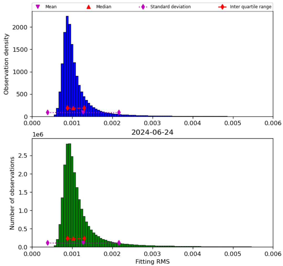
Figure 23: Histogram of “Fitting RMS” for 2024-06-24 to 2024-06-25
