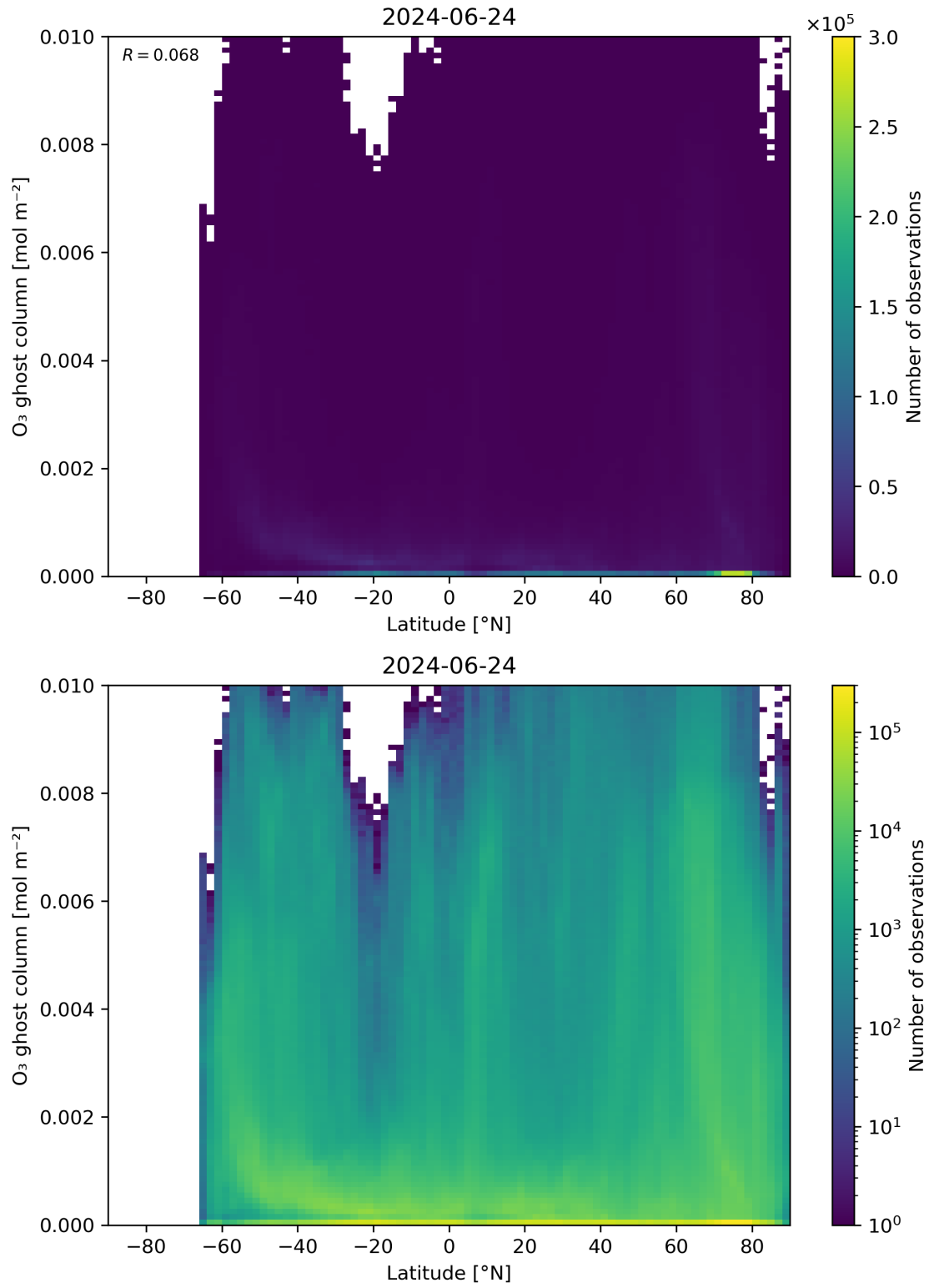
Figure 35: Scatter density plot of “Latitude” against “O 3 ghost column” for 2024-06-24 to 2024-06-25.
