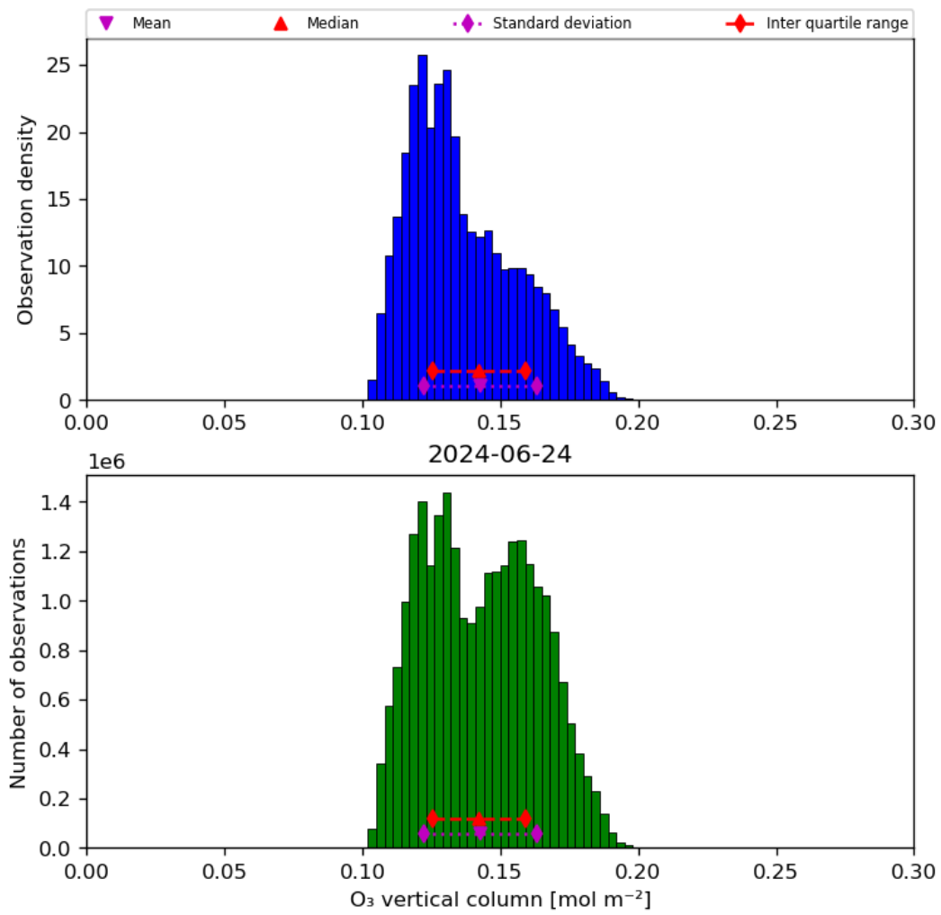
Figure 21: Histogram of “O 3 vertical column” for 2024-06-24 to 2024-06-25
