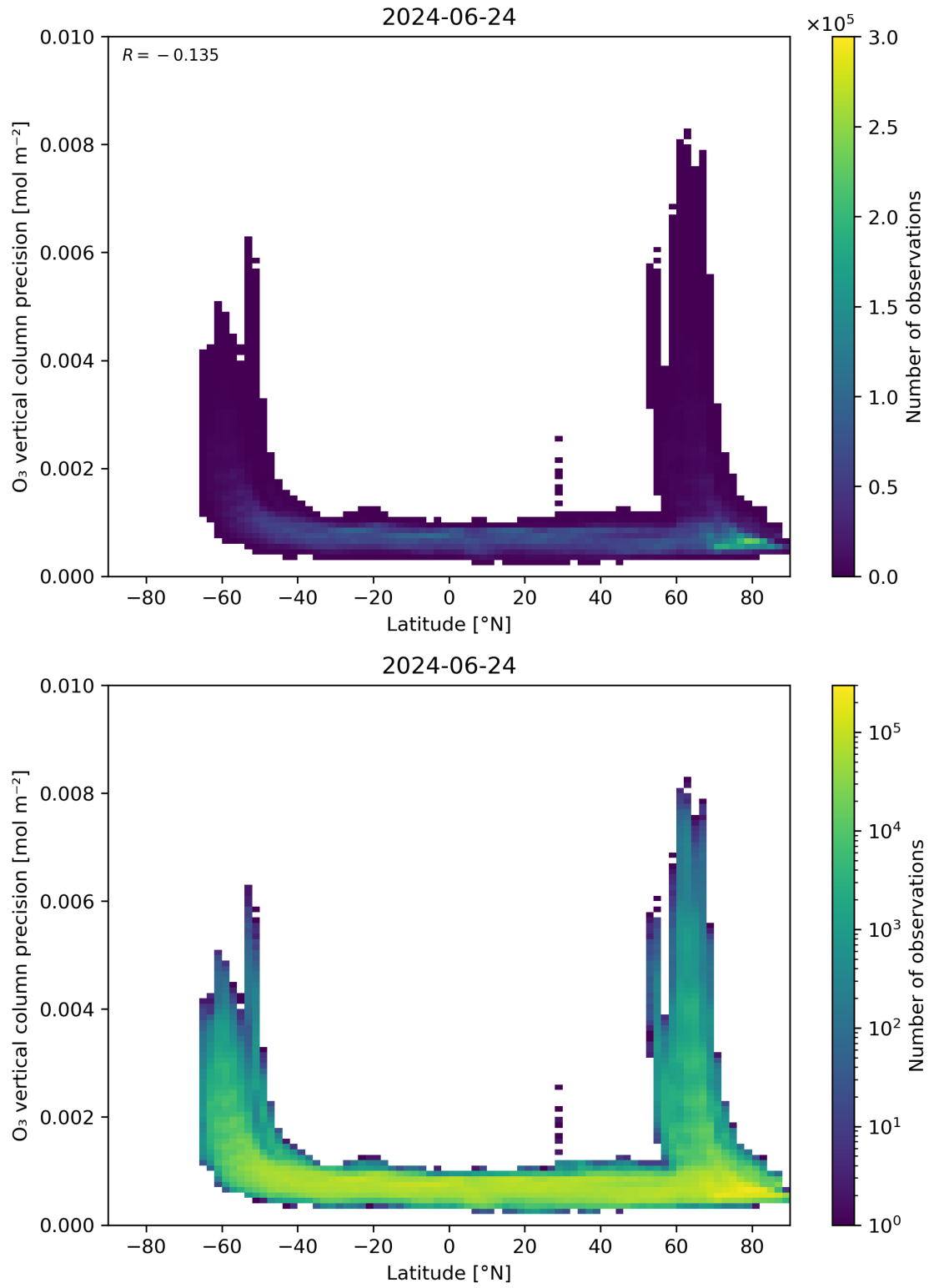
Figure 37: Scatter density plot of “Latitude” against “O 3 vertical column precision” for 2024-06-24 to 2024-06-25.
