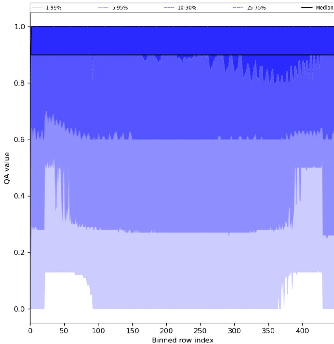
Figure 27: Along track statistics of “QA value” for 2024-06-24 to 2024-06-25
