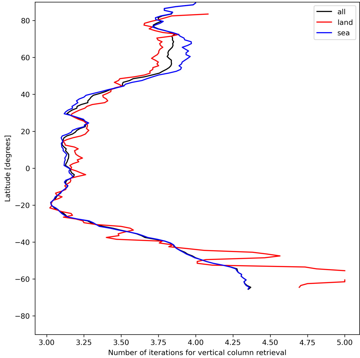
Figure 19: Zonal average of “Number of iterations for vertical column retrieval” for 2024-06-24 to 2024-06-25.
