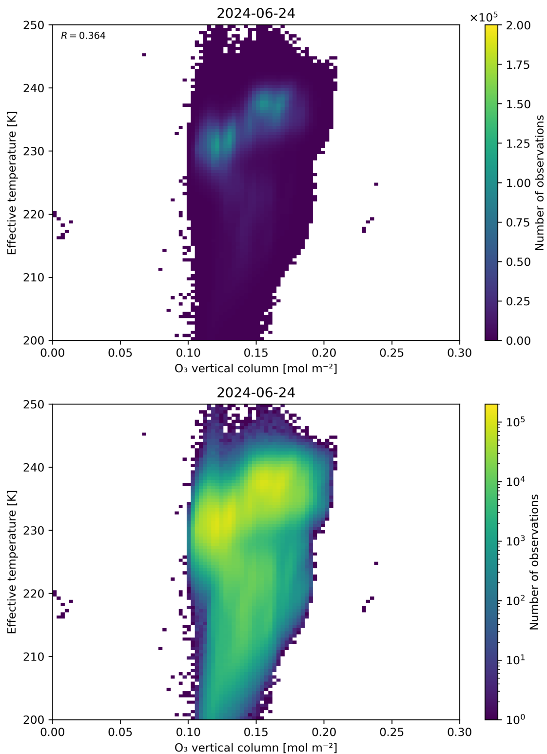
Figure 39: Scatter density plot of “O 3 vertical column” against “Effective temperature” for 2024-06-24 to 2024-06-25.
