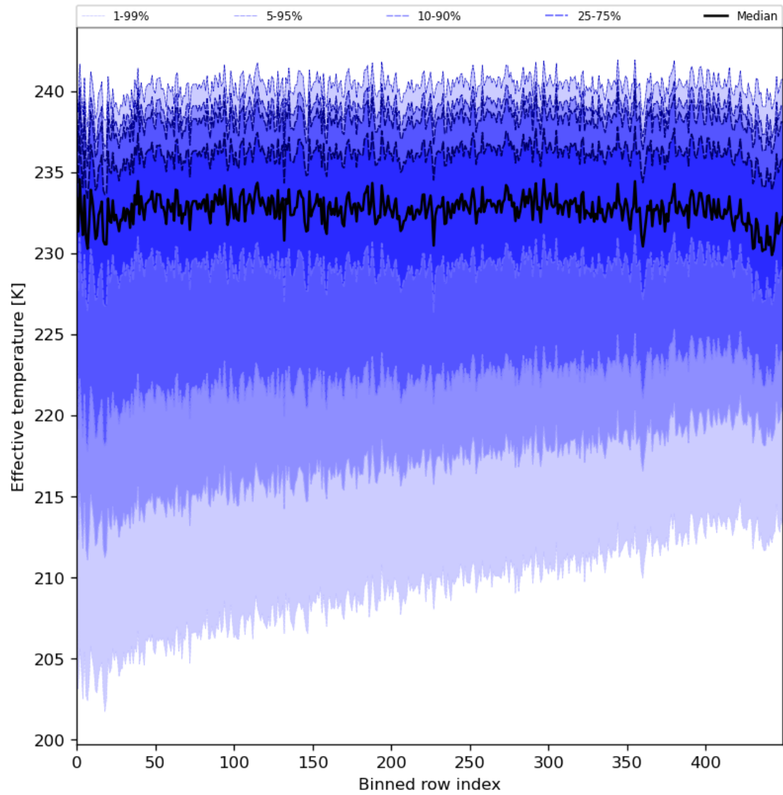
Figure 31: Along track statistics of “Effective temperature” for 2024-06-24 to 2024-06-25
