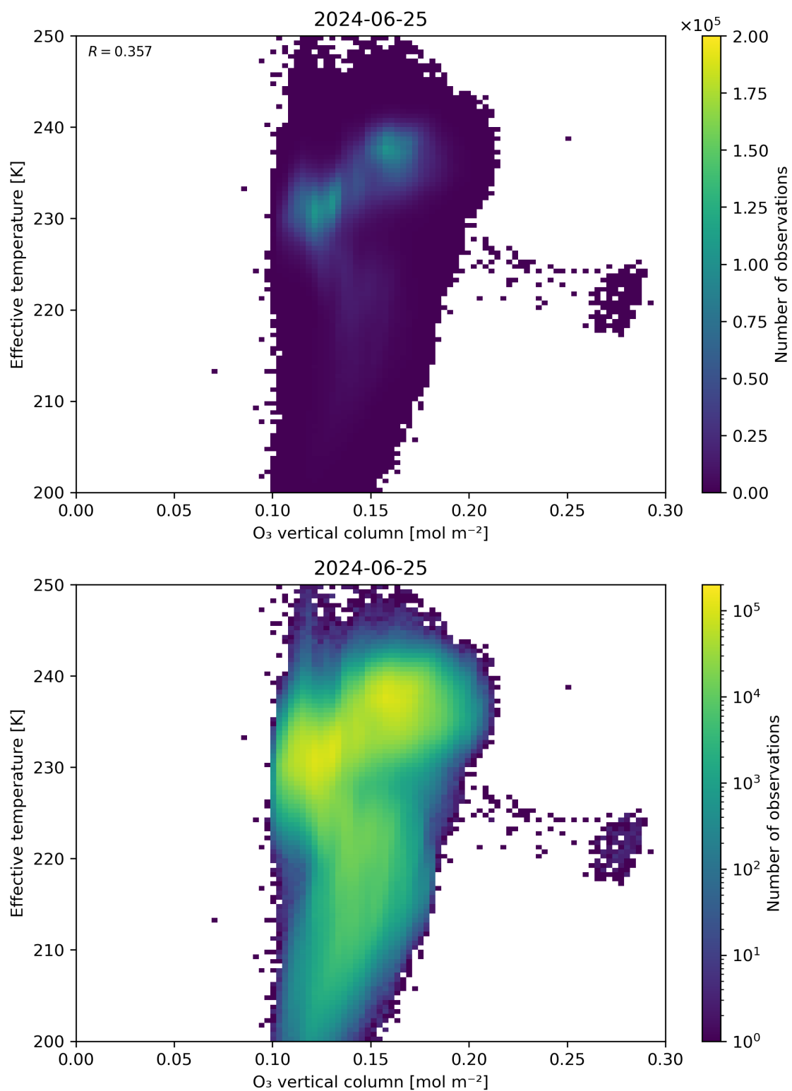
Figure 39: Scatter density plot of “O 3 vertical column” against “Effective temperature” for 2024-06-24 to 2024-06-26.
