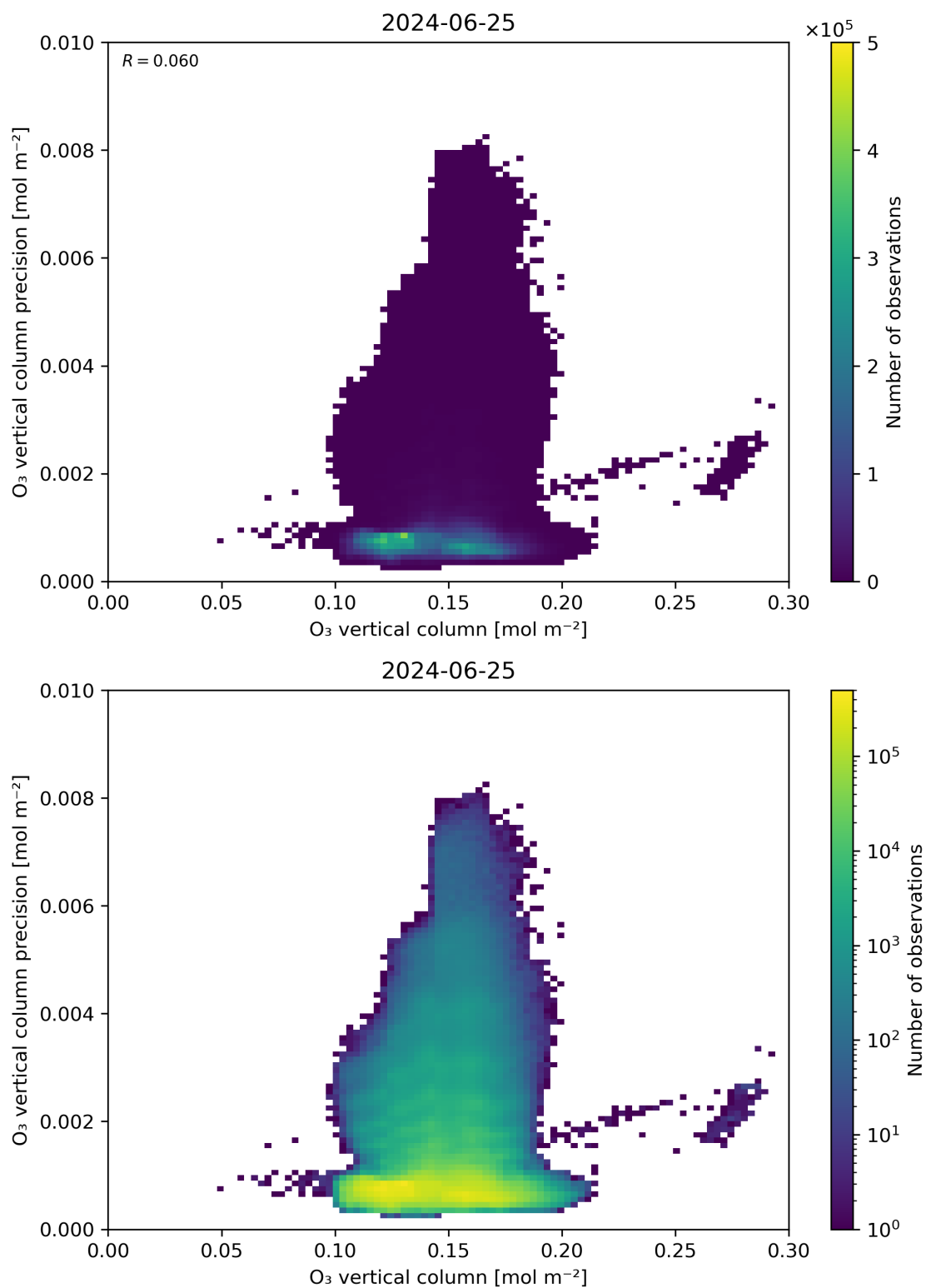
Figure 41: Scatter density plot of “O 3 vertical column” against “O 3 vertical column precision” for 2024-06-24 to 2024-06-26.
