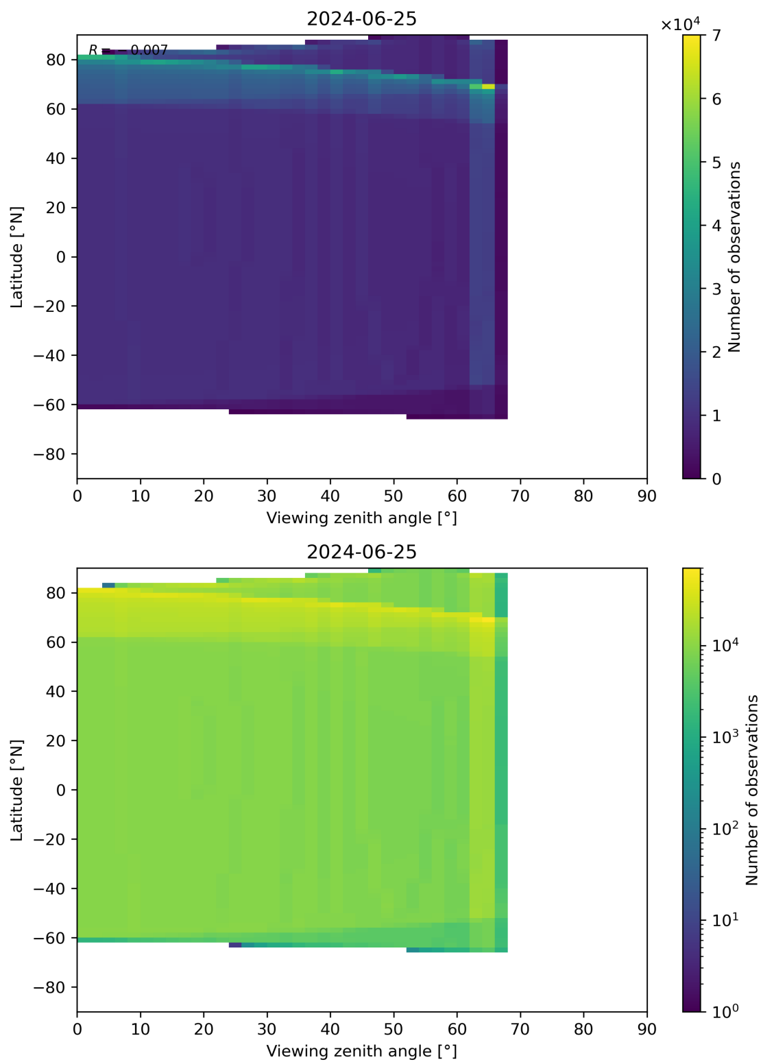
Figure 49: Scatter density plot of “Viewing zenith angle” against “Latitude” for 2024-06-24 to 2024-06-26.
