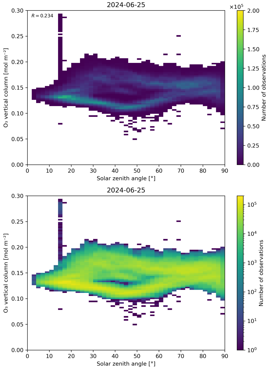
Figure 47: Scatter density plot of “Solar zenith angle” against “O 3 vertical column” for 2024-06-24 to 2024-06-26.
