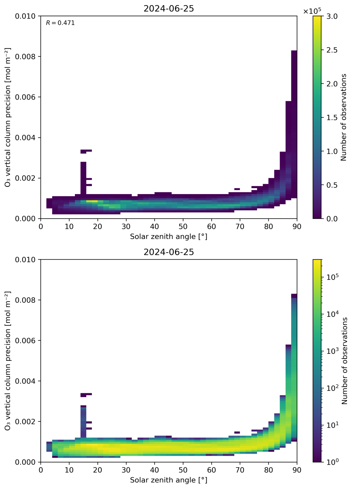
Figure 48: Scatter density plot of “Solar zenith angle” against “O 3 vertical column precision” for 2024-06-24 to 2024-06-26.
