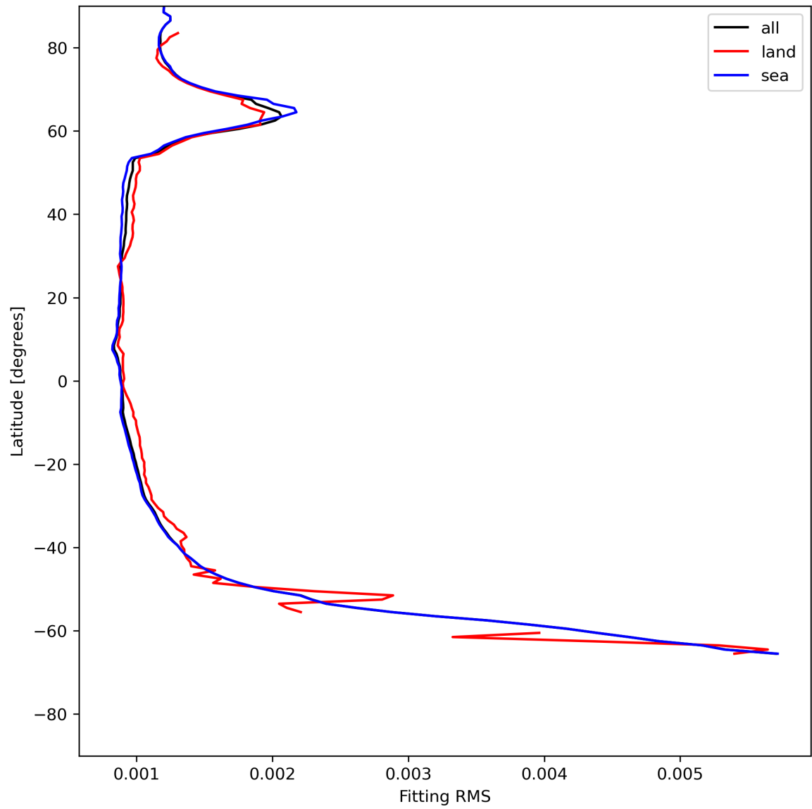
Figure 16: Zonal average of “Fitting RMS” for 2024-06-24 to 2024-06-26.
