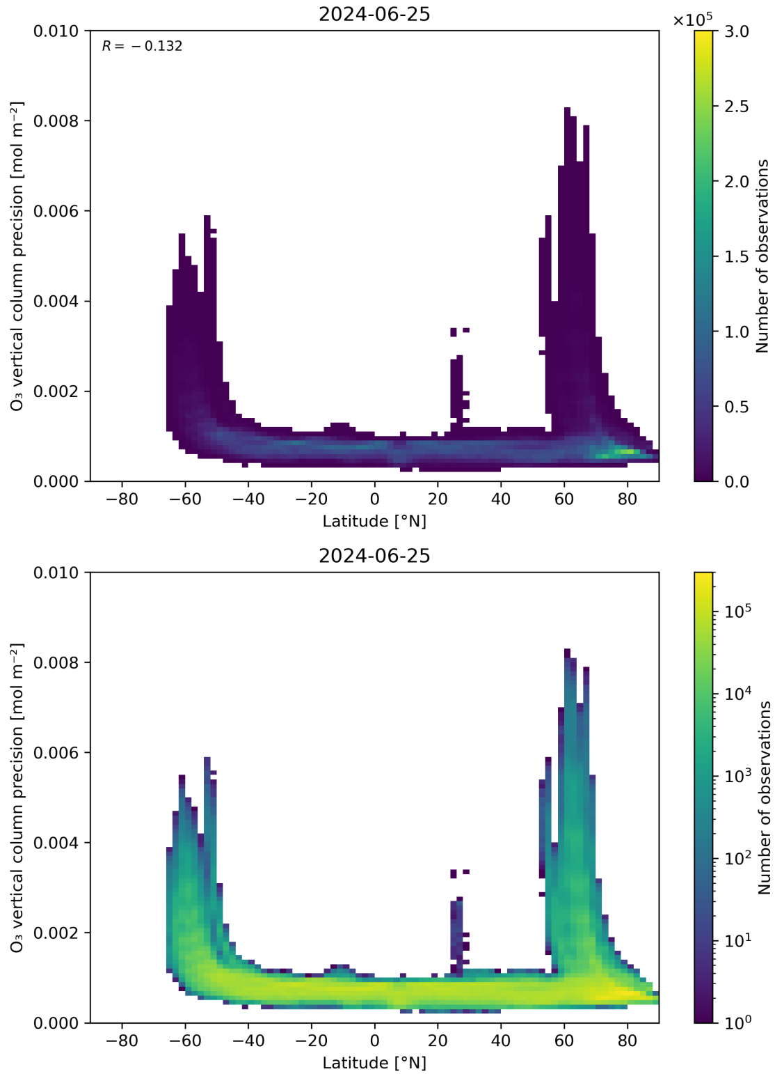
Figure 37: Scatter density plot of “Latitude” against “O 3 vertical column precision” for 2024-06-24 to 2024-06-26.
