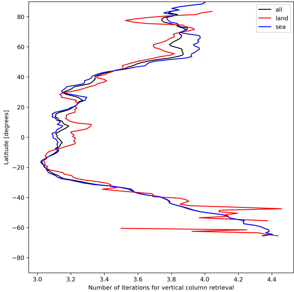
Figure 19: Zonal average of “Number of iterations for vertical column retrieval” for 2024-06-24 to 2024-06-26.
