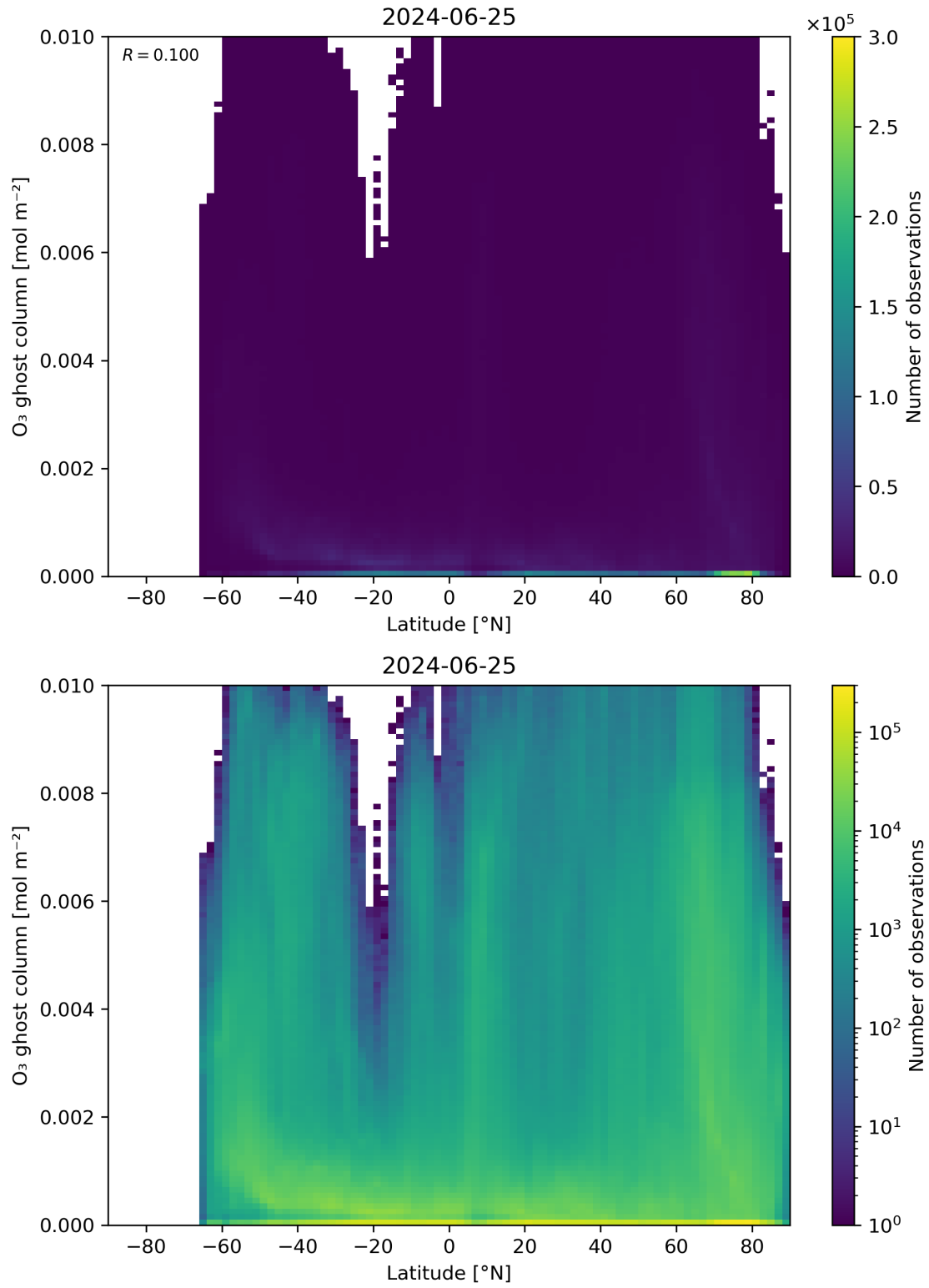
Figure 35: Scatter density plot of “Latitude” against “O 3 ghost column” for 2024-06-24 to 2024-06-26.
