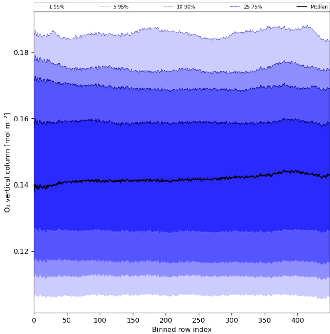
Figure 28: Along track statistics of “O 3 vertical column” for 2024-06-24 to 2024-06-26
