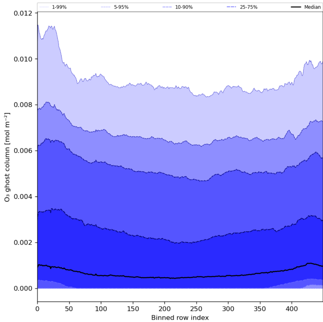
Figure 32: Along track statistics of “O 3 ghost column” for 2024-06-24 to 2024-06-26
