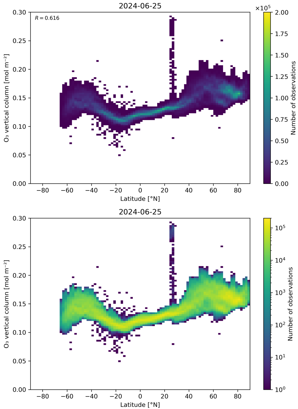
Figure 36: Scatter density plot of “Latitude” against “O 3 vertical column” for 2024-06-24 to 2024-06-26.
