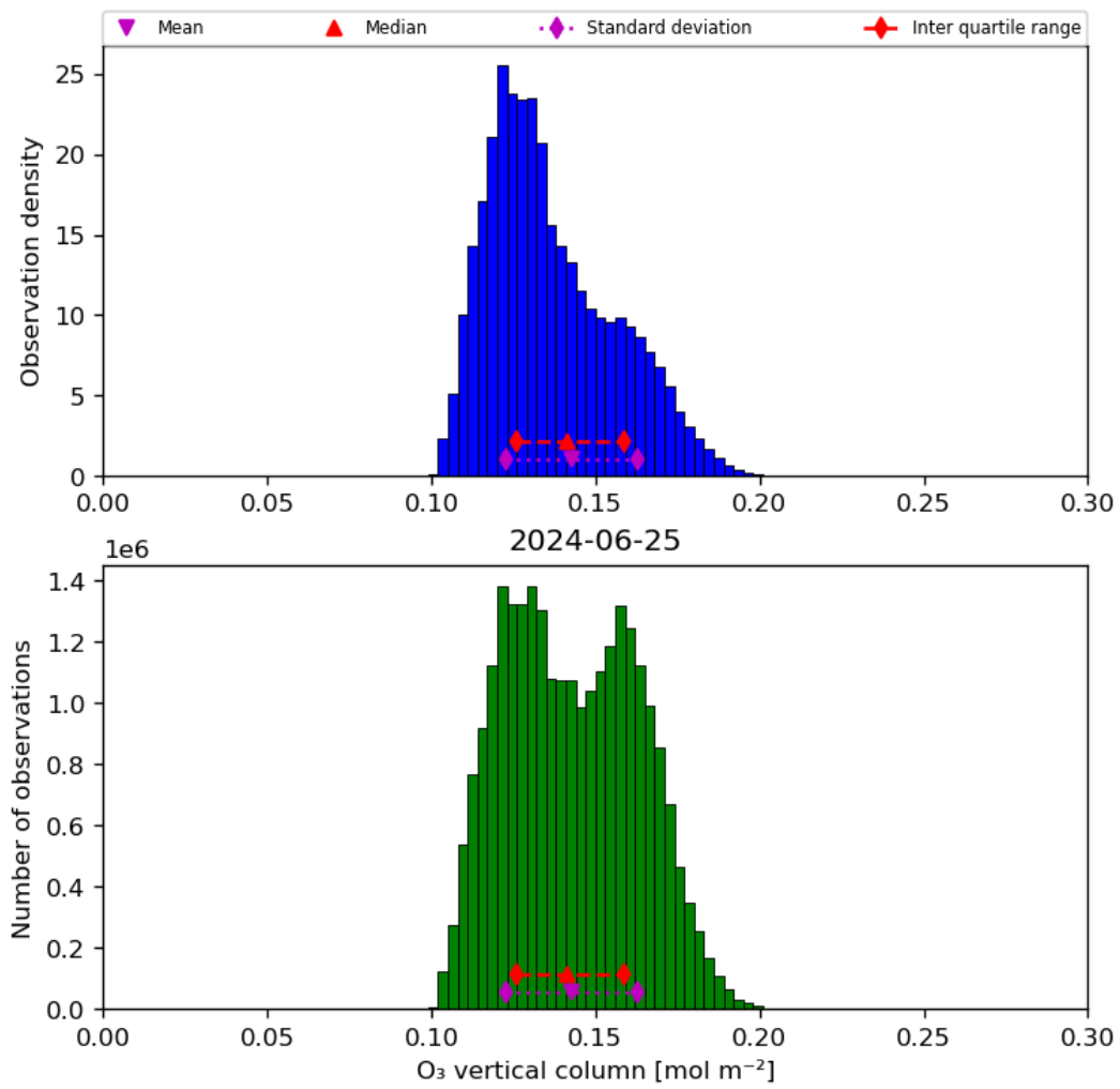
Figure 21: Histogram of “O 3 vertical column” for 2024-06-24 to 2024-06-26
