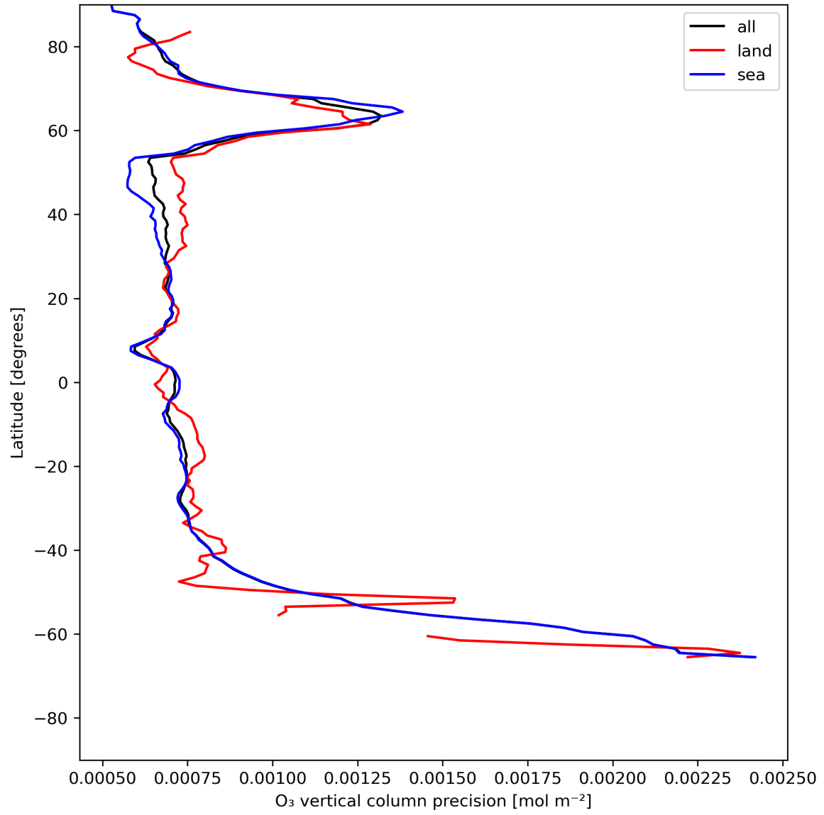
Figure 15: Zonal average of “O 3 vertical column precision” for 2024-06-24 to 2024-06-26.
