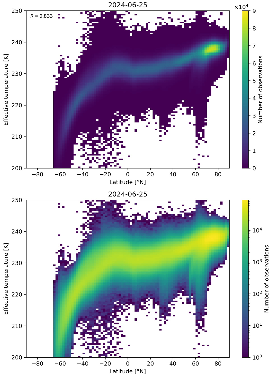
Figure 34: Scatter density plot of “Latitude” against “Effective temperature” for 2024-06-24 to 2024-06-26.
