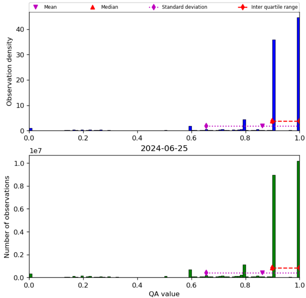
Figure 20: Histogram of “QA value” for 2024-06-24 to 2024-06-26
