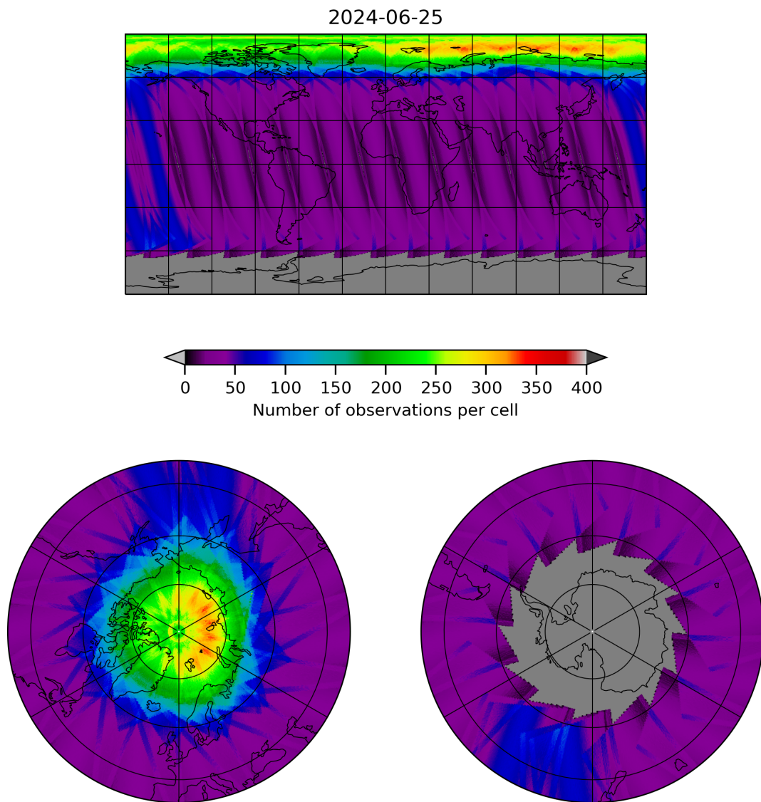
Figure 12: Map of the number of observations for 2024-06-24 to 2024-06-26
