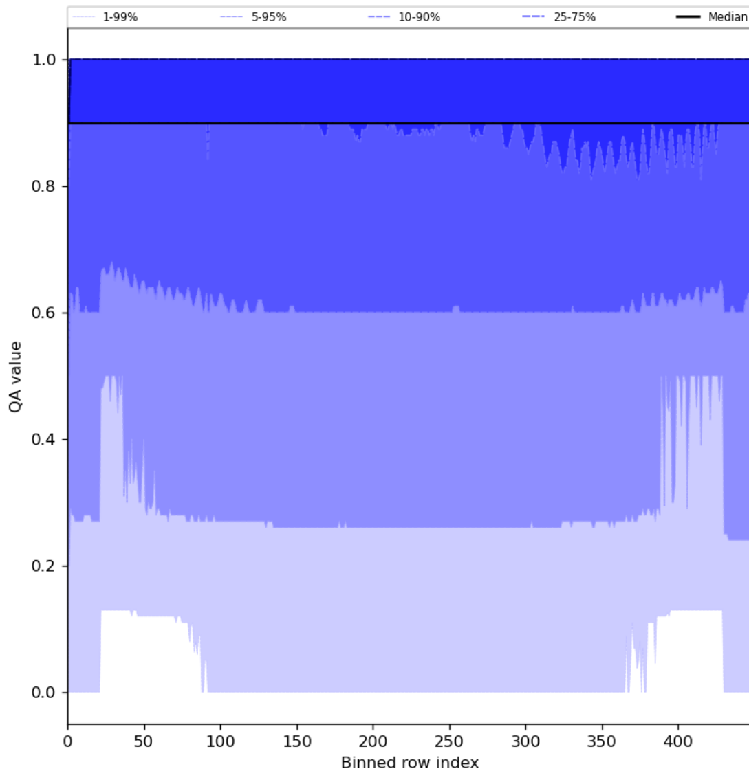
Figure 27: Along track statistics of “QA value” for 2024-06-24 to 2024-06-26
