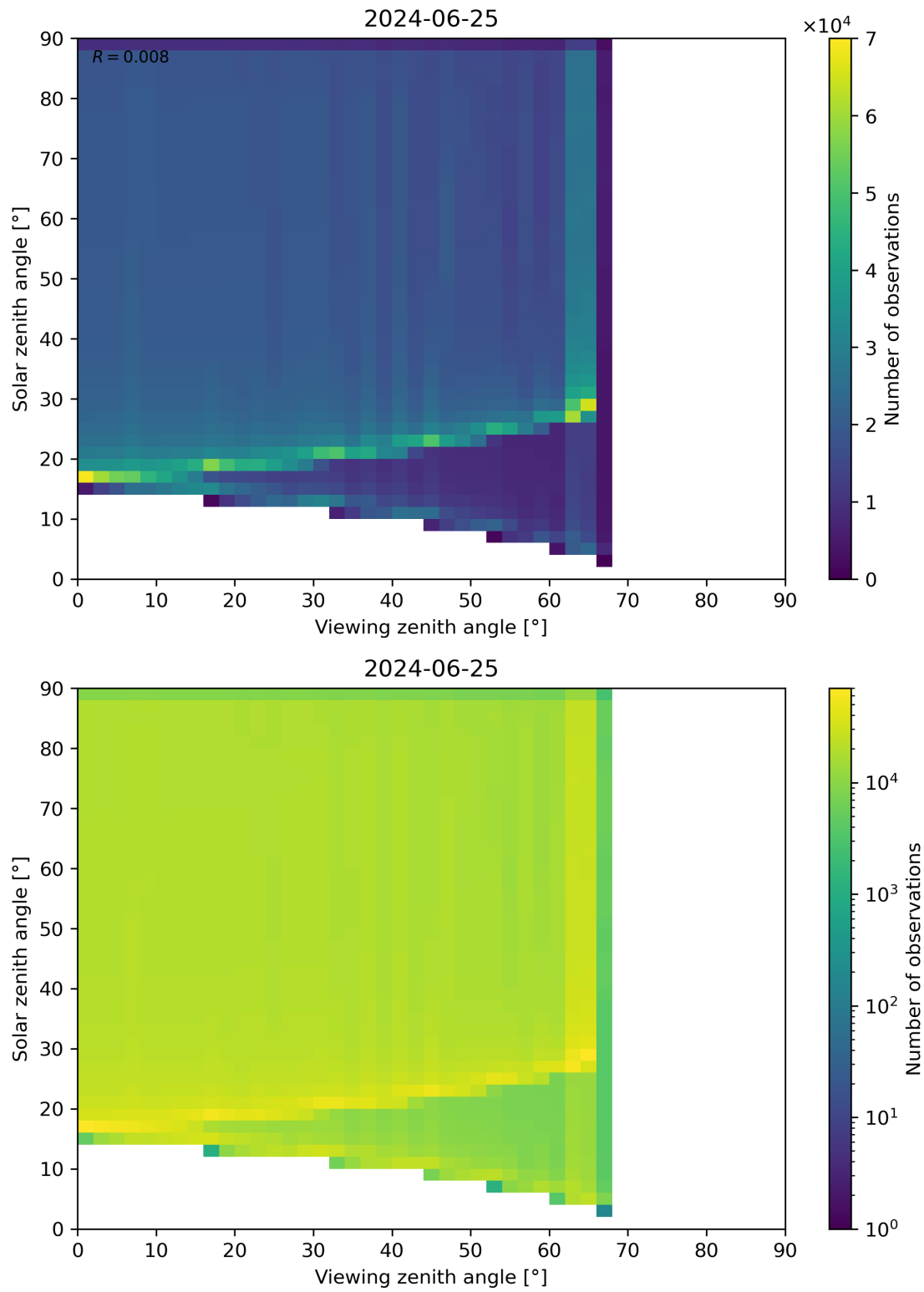
Figure 54: Scatter density plot of “Viewing zenith angle” against “Solar zenith angle” for 2024-06-24 to 2024-06-26.
