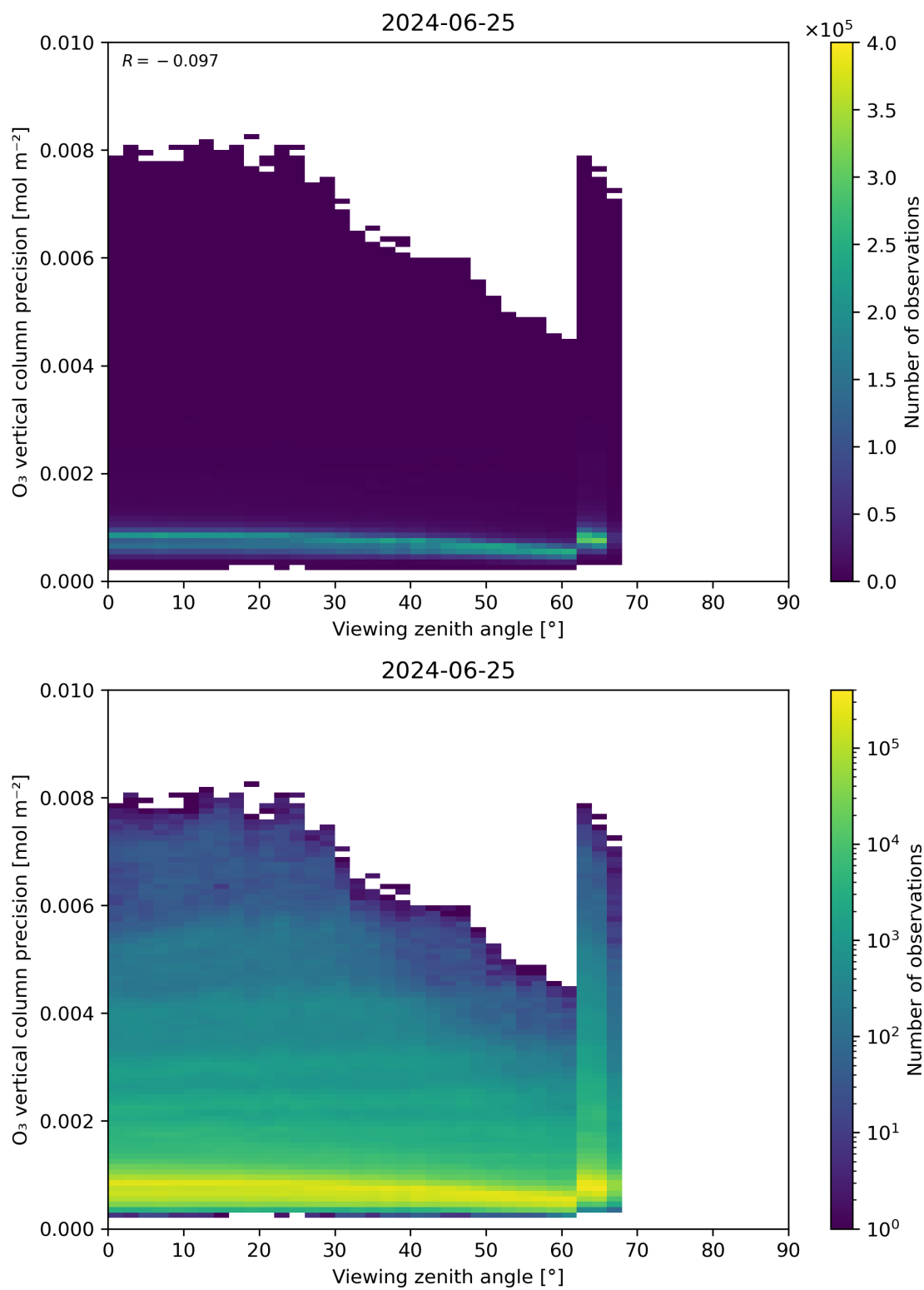
Figure 53: Scatter density plot of “Viewing zenith angle” against “O 3 vertical column precision” for 2024-06-24 to 2024-06-26.
