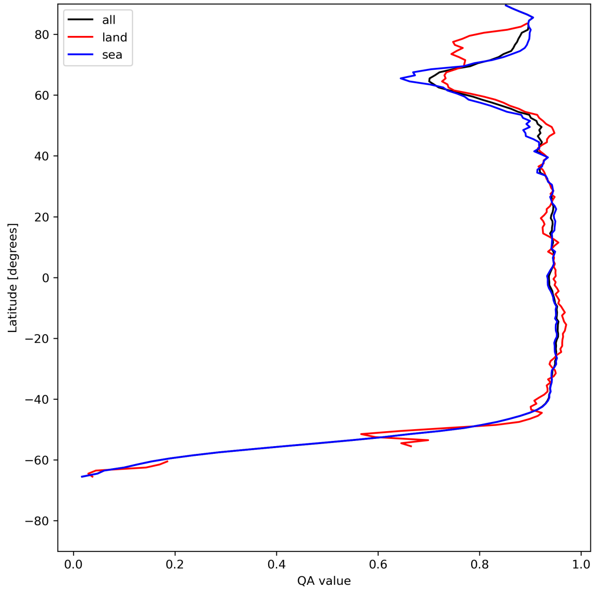
Figure 13: Zonal average of “QA value” for 2024-06-24 to 2024-06-26.
