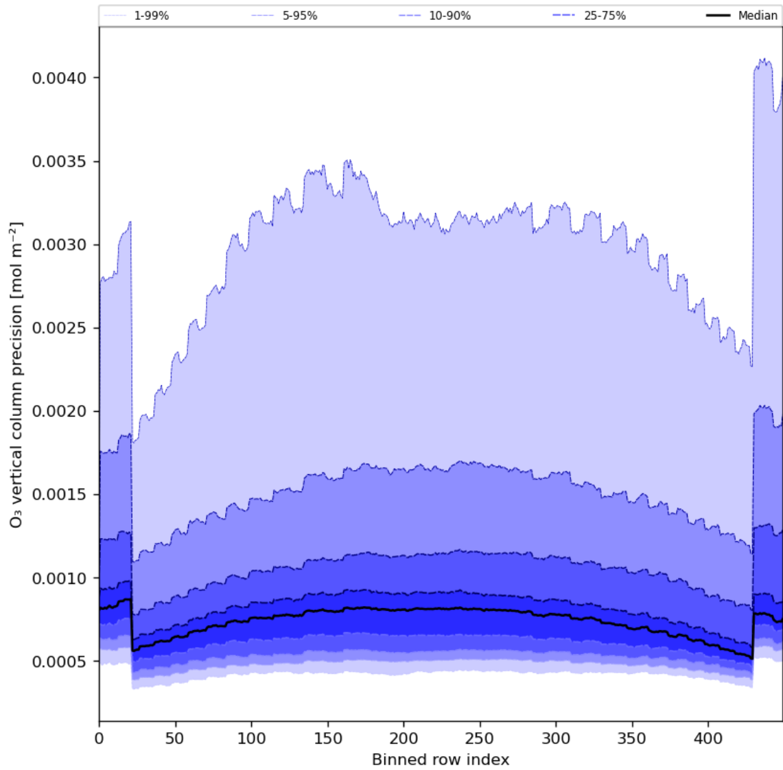
Figure 29: Along track statistics of “O 3 vertical column precision” for 2024-06-24 to 2024-06-26
