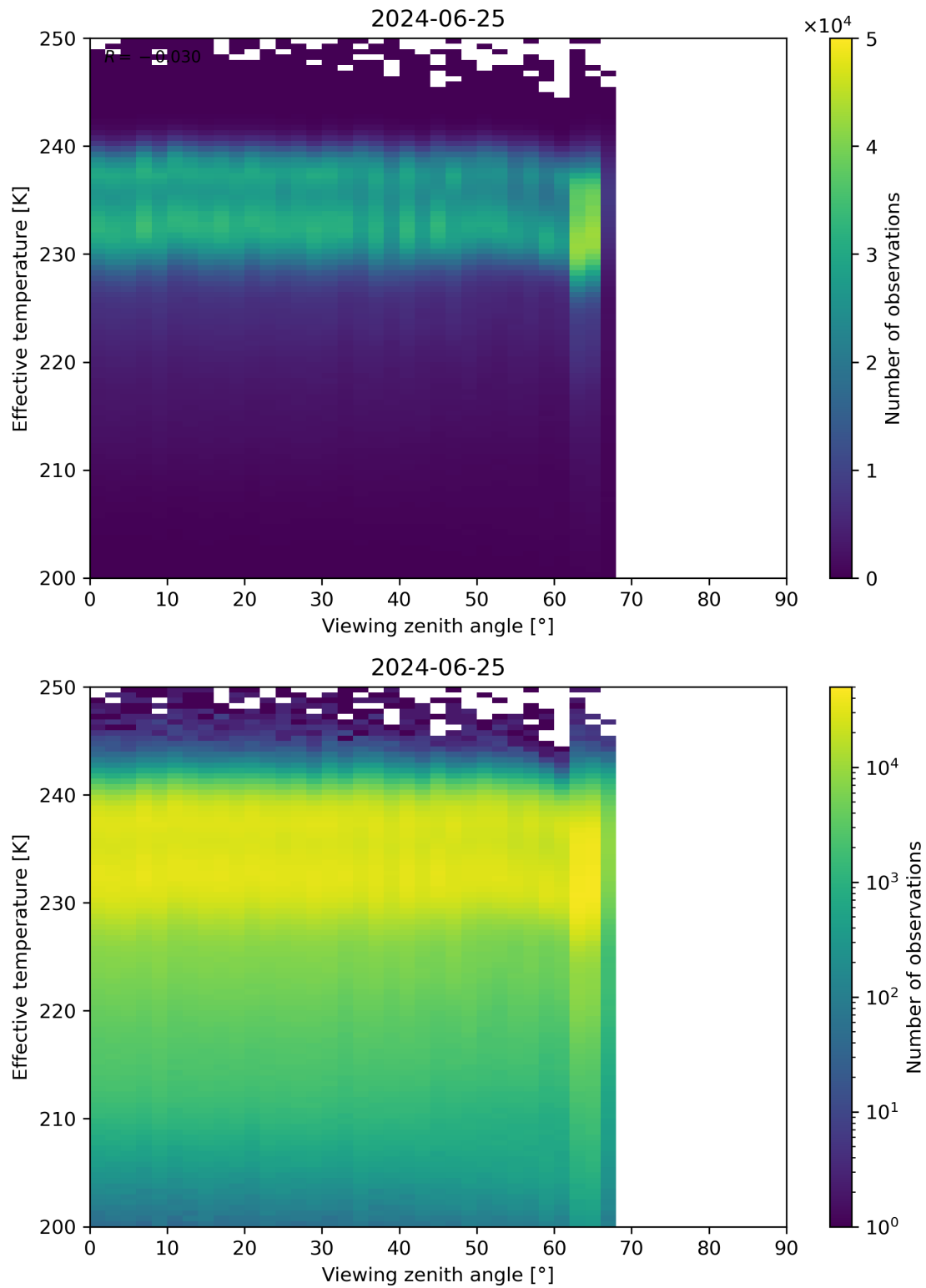
Figure 50: Scatter density plot of “Viewing zenith angle” against “Effective temperature” for 2024-06-24 to 2024-06-26.
