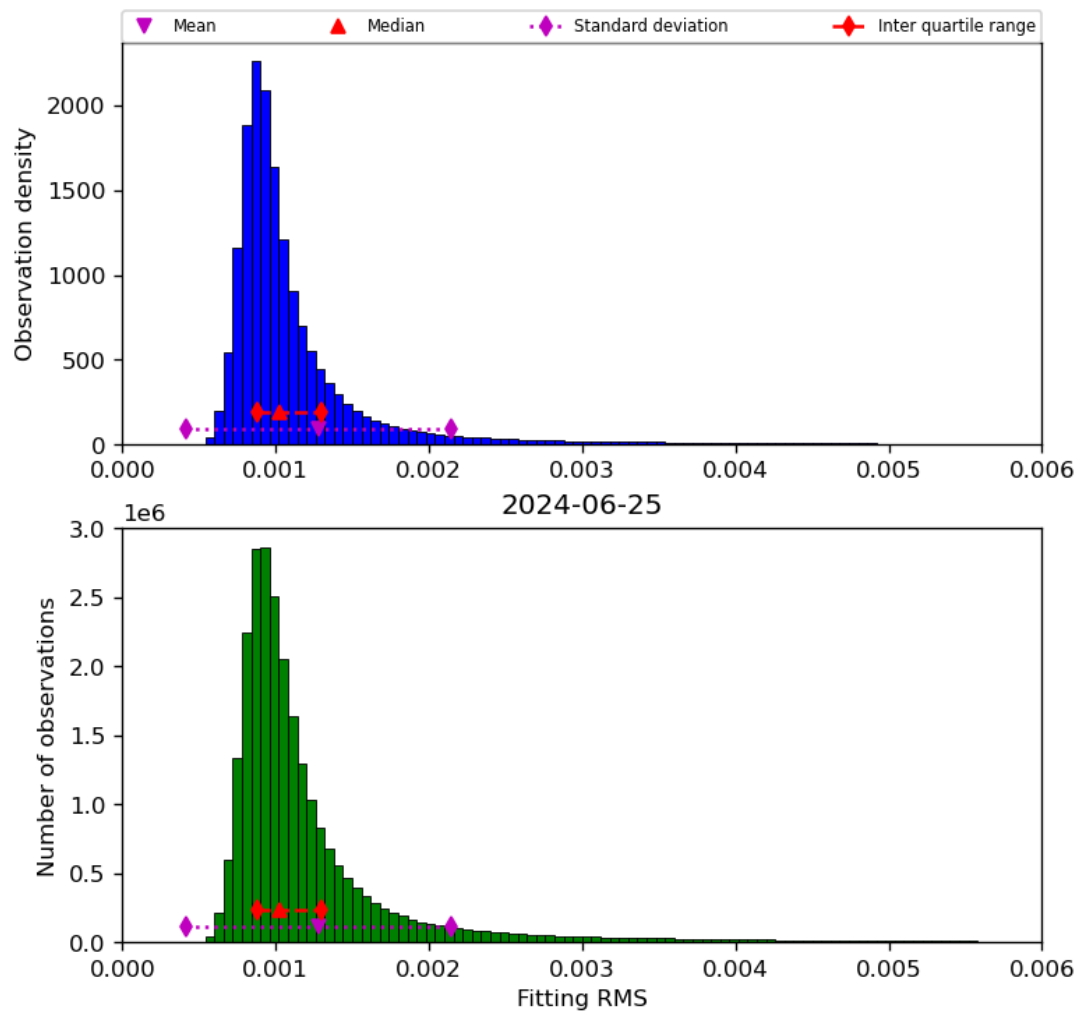
Figure 23: Histogram of “Fitting RMS” for 2024-06-24 to 2024-06-26
