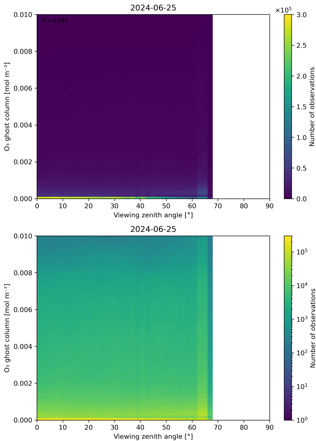
Figure 51: Scatter density plot of “Viewing zenith angle” against “O 3 ghost column” for 2024-06-24 to 2024-06-26.
