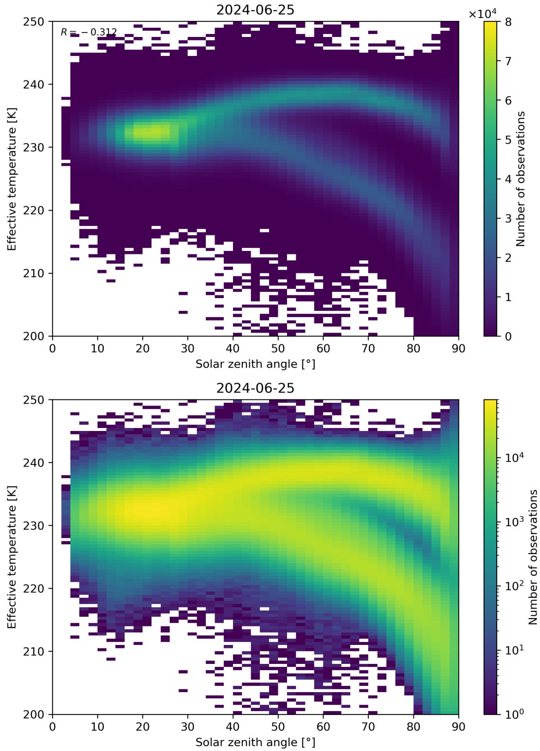
Figure 45: Scatter density plot of “Solar zenith angle” against “Effective temperature” for 2024-06-24 to 2024-06-26.
