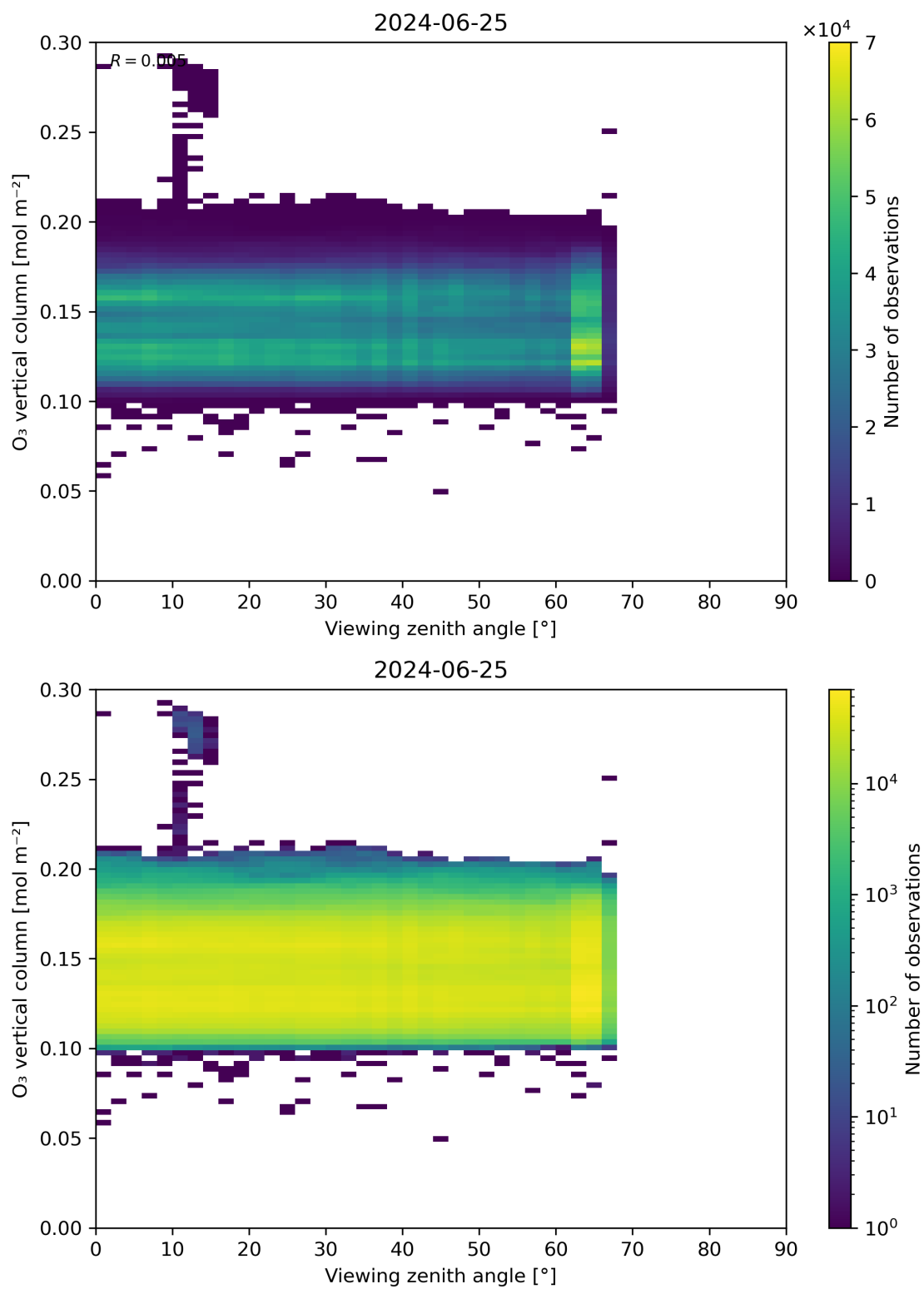
Figure 52: Scatter density plot of “Viewing zenith angle” against “O 3 vertical column” for 2024-06-24 to 2024-06-26.
