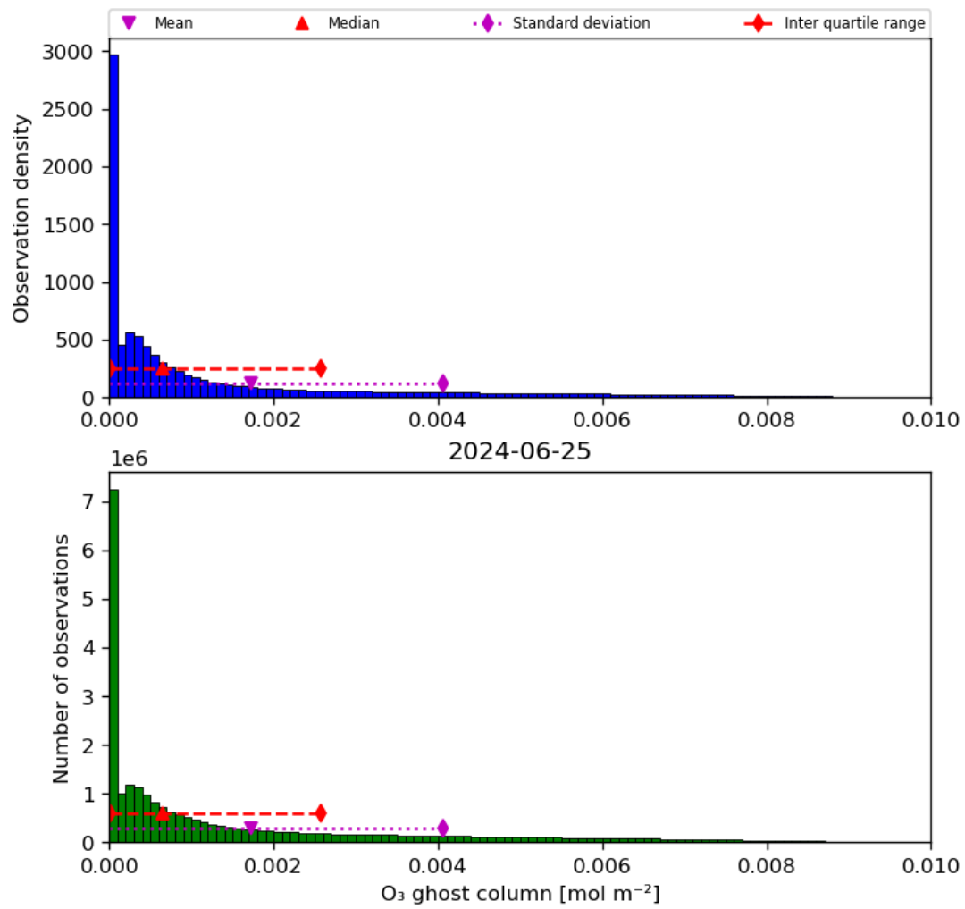
Figure 25: Histogram of “O 3 ghost column” for 2024-06-24 to 2024-06-26
