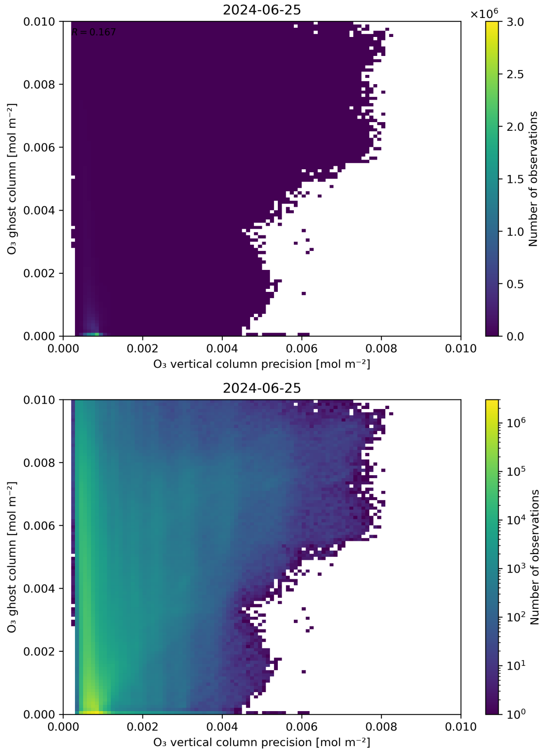
Figure 43: Scatter density plot of “ \text{O}_3 vertical column precision” against “ \text{O}_3 ghost column” for 2024-06-24 to 2024-06-26.
