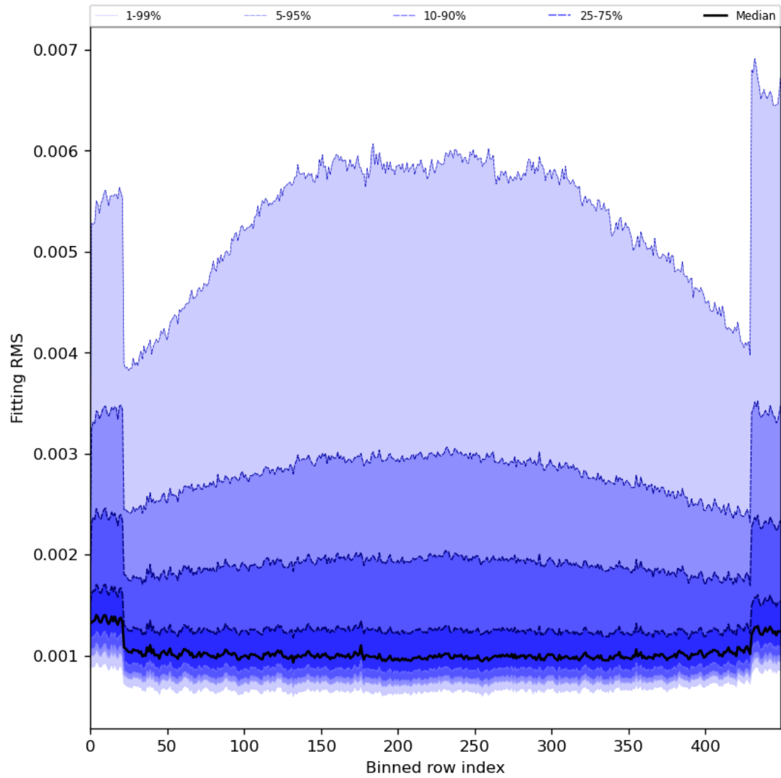
Figure 30: Along track statistics of “Fitting RMS” for 2024-06-24 to 2024-06-26
