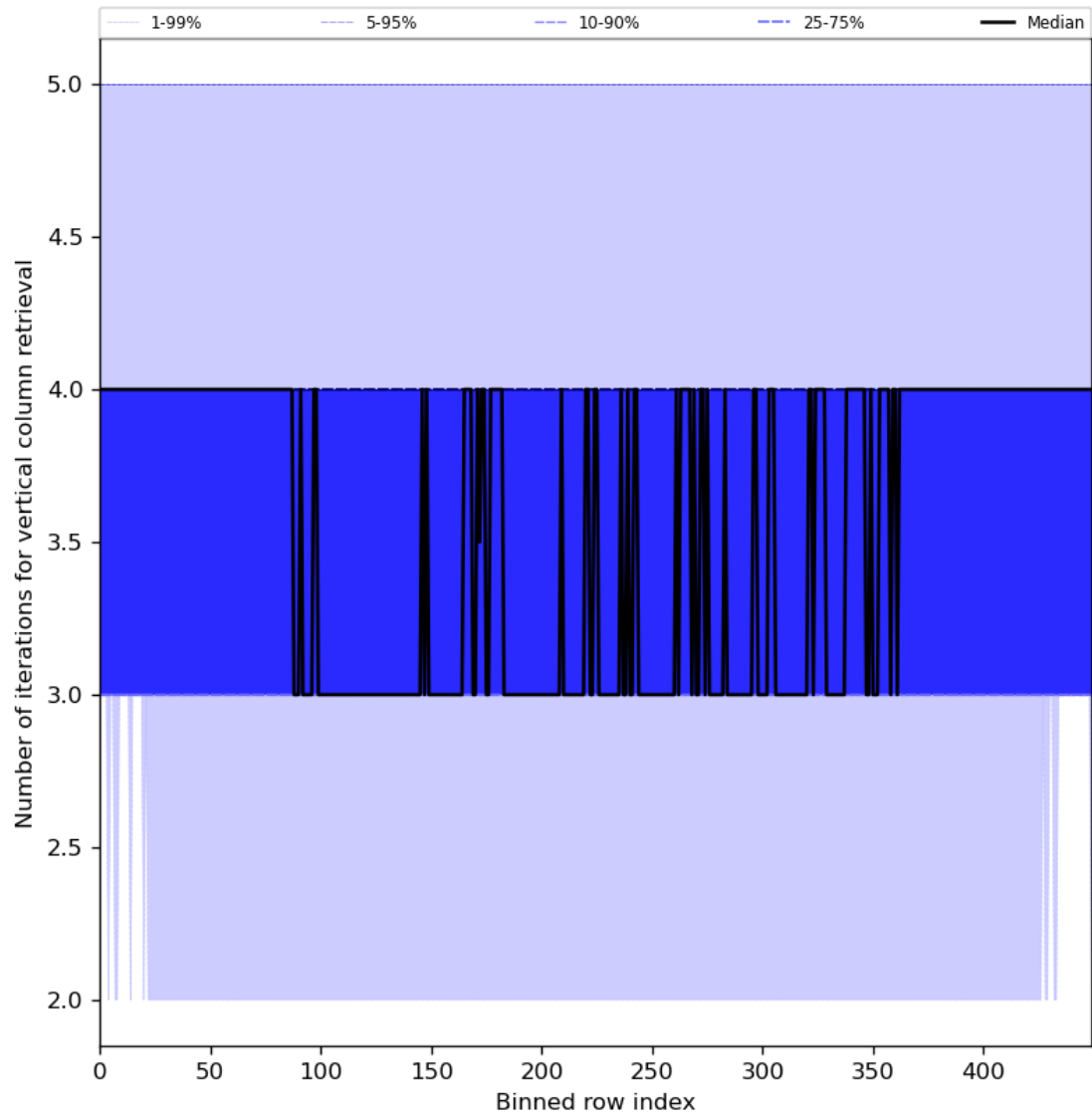
Figure 33: Along track statistics of “Number of iterations for vertical column retrieval” for 2024-06-24 to 2024-06-26
