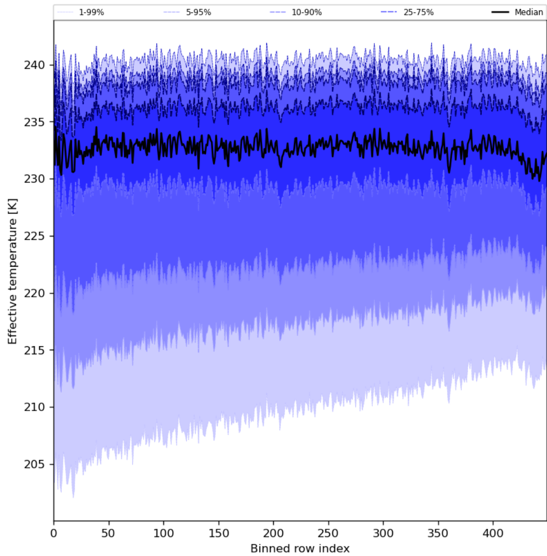
Figure 31: Along track statistics of "Effective temperature" for 2024-06-24 to 2024-06-26
