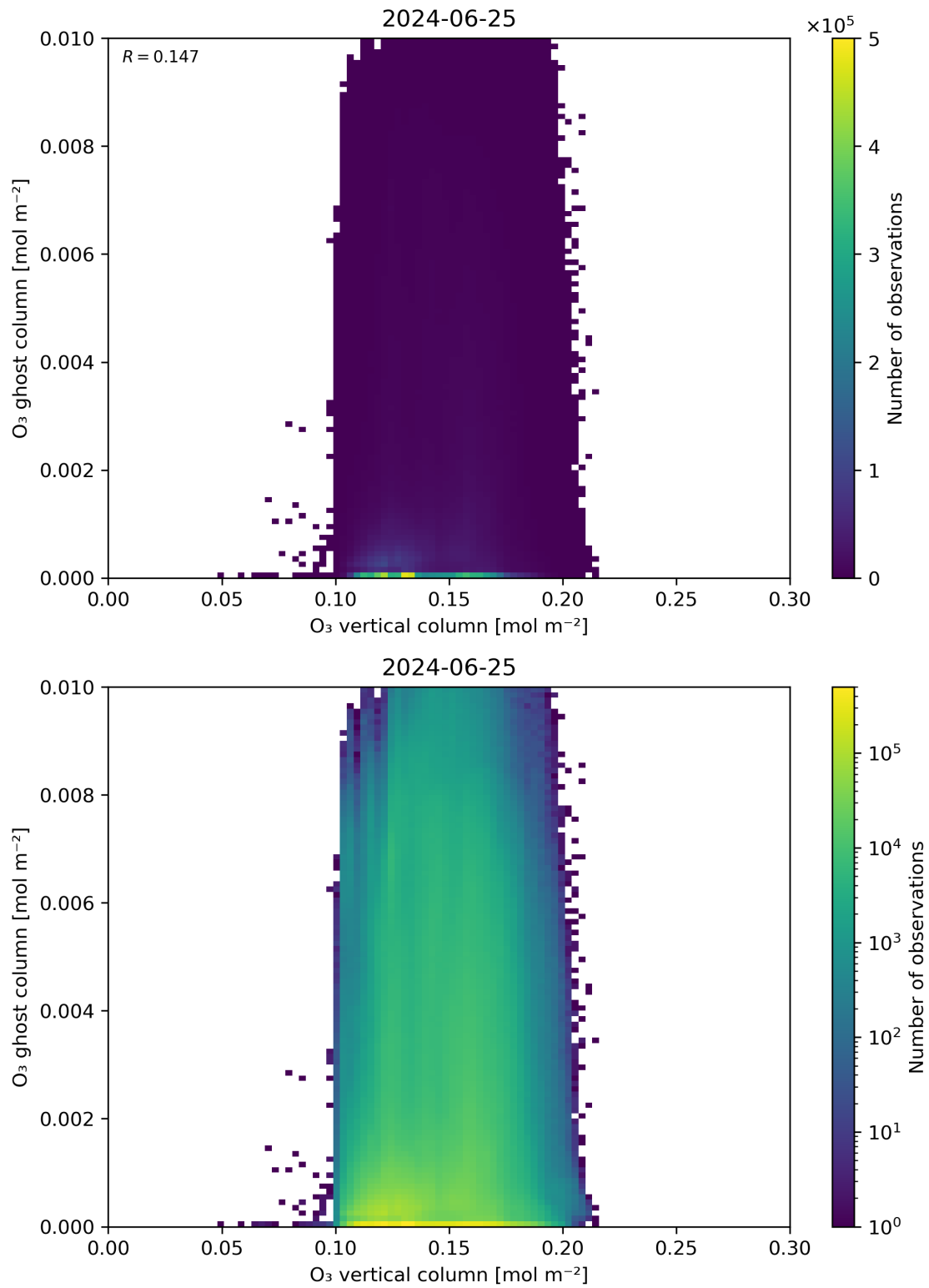
Figure 40: Scatter density plot of “O 3 vertical column” against “O 3 ghost column” for 2024-06-24 to 2024-06-26.
