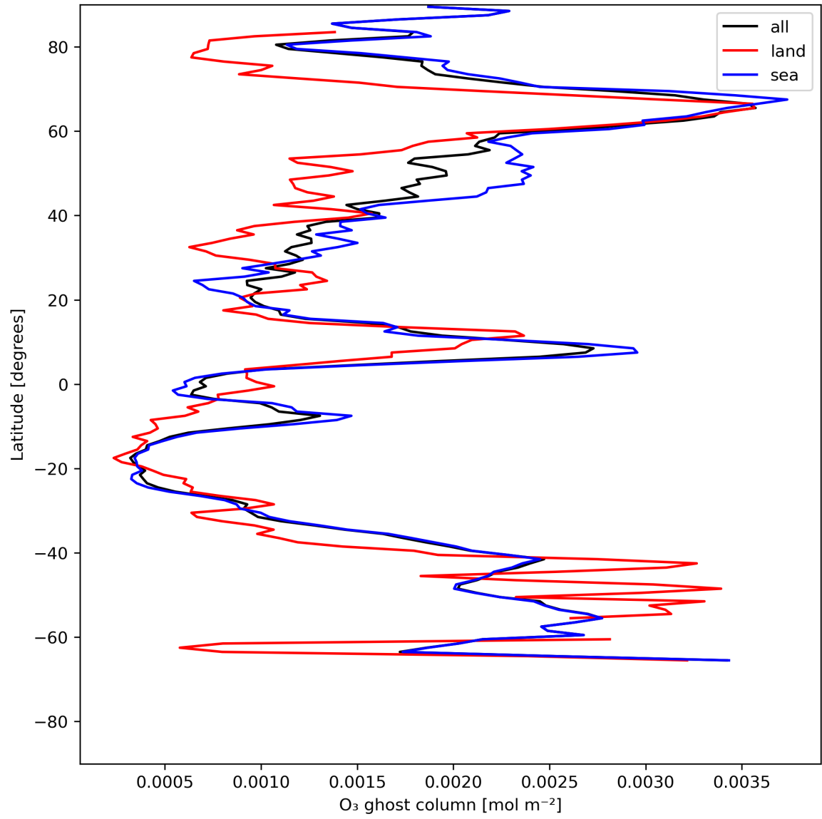
Figure 18: Zonal average of "O 3 ghost column" for 2024-06-24 to 2024-06-26.
