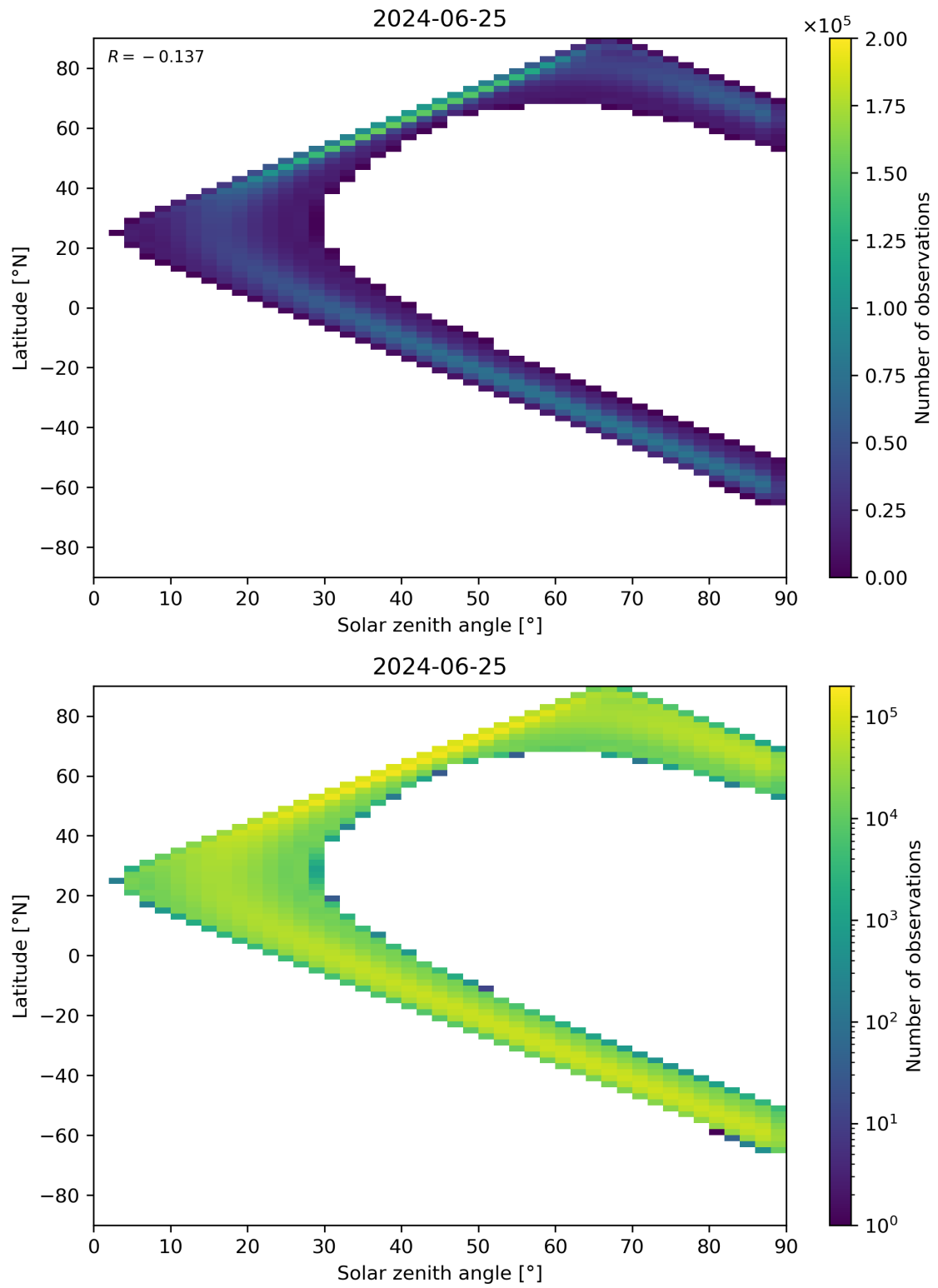
Figure 44: Scatter density plot of “Solar zenith angle” against “Latitude” for 2024-06-24 to 2024-06-26.
