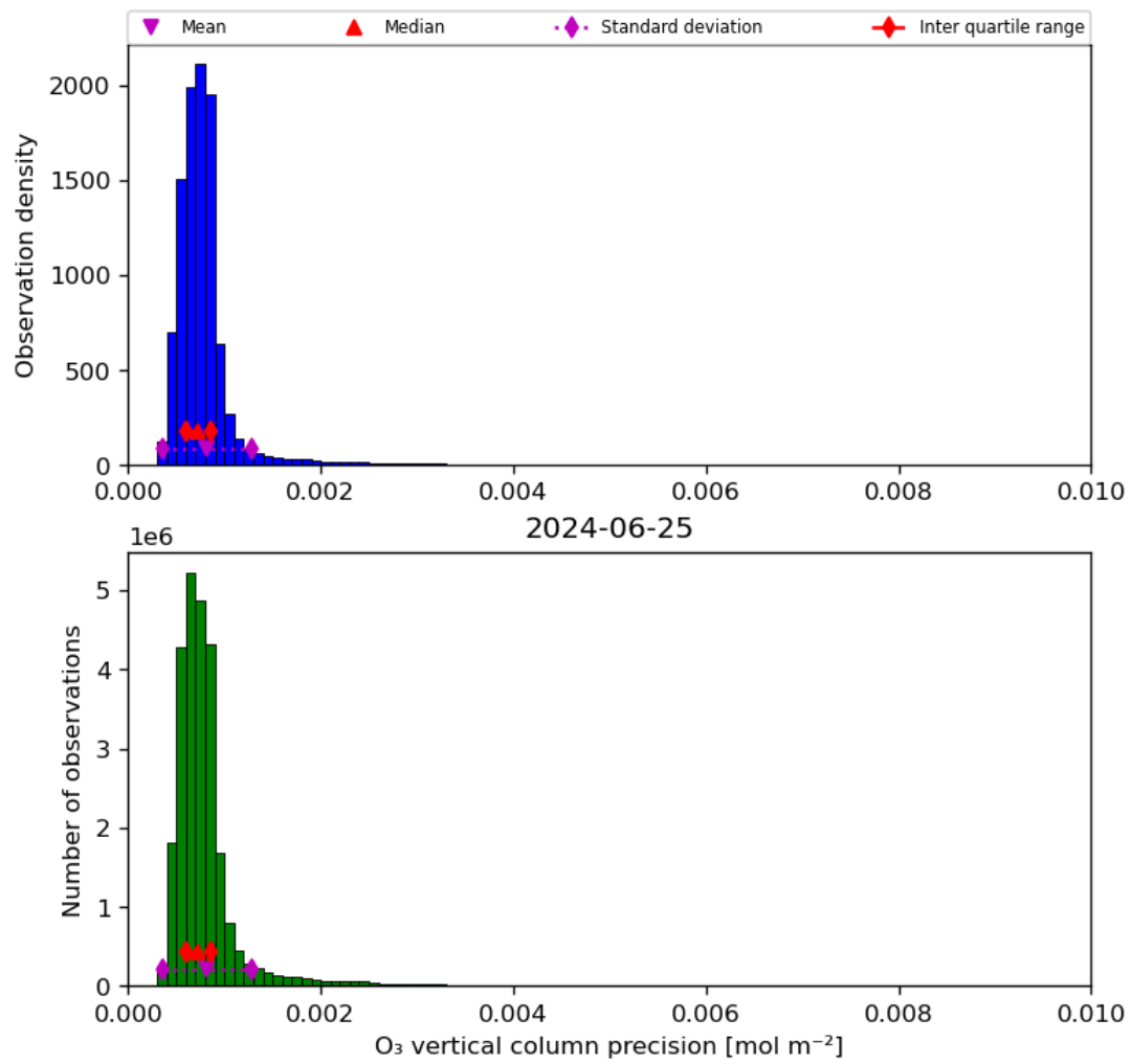
Figure 22: Histogram of “O 3 vertical column precision” for 2024-06-24 to 2024-06-26
