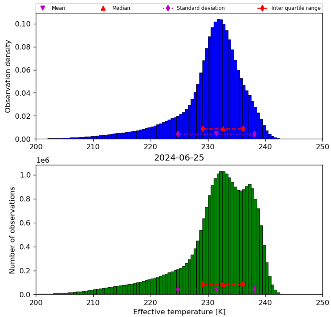
Figure 24: Histogram of “Effective temperature” for 2024-06-24 to 2024-06-26
