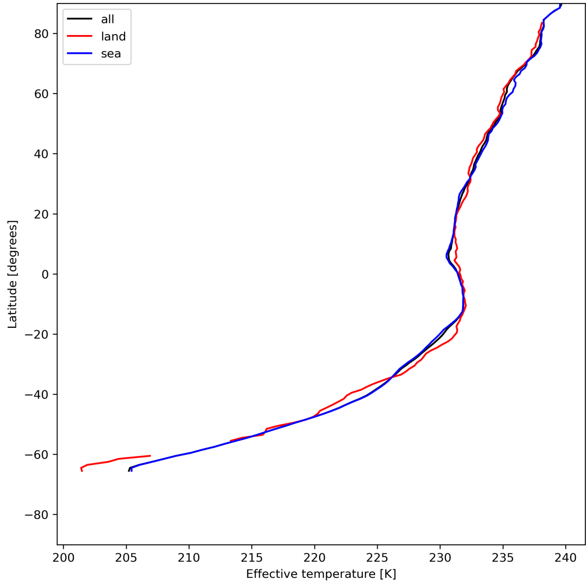
Figure 17: Zonal average of "Effective temperature" for 2024-06-24 to 2024-06-26.
