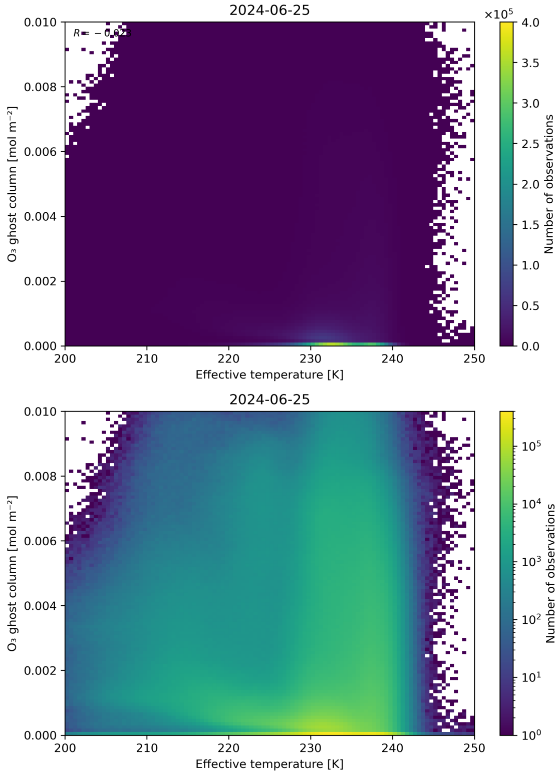
Figure 38: Scatter density plot of “Effective temperature” against “O 3 ghost column” for 2024-06-24 to 2024-06-26.
