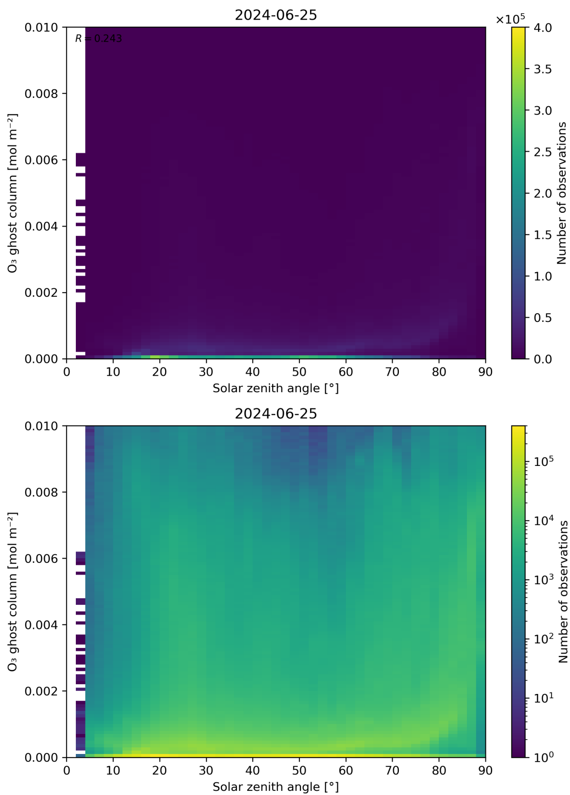
Figure 46: Scatter density plot of “Solar zenith angle” against “O 3 ghost column” for 2024-06-24 to 2024-06-26.
