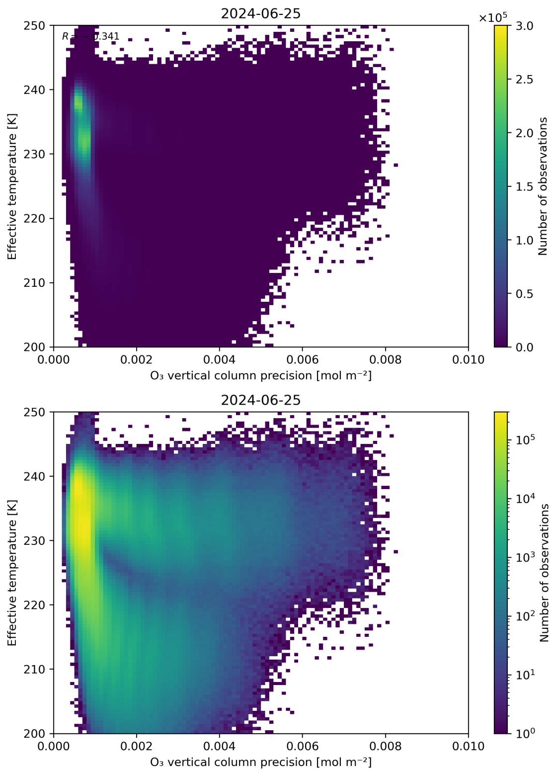
Figure 42: Scatter density plot of “O 3 vertical column precision” against “Effective temperature” for 2024-06-24 to 2024-06-26.
