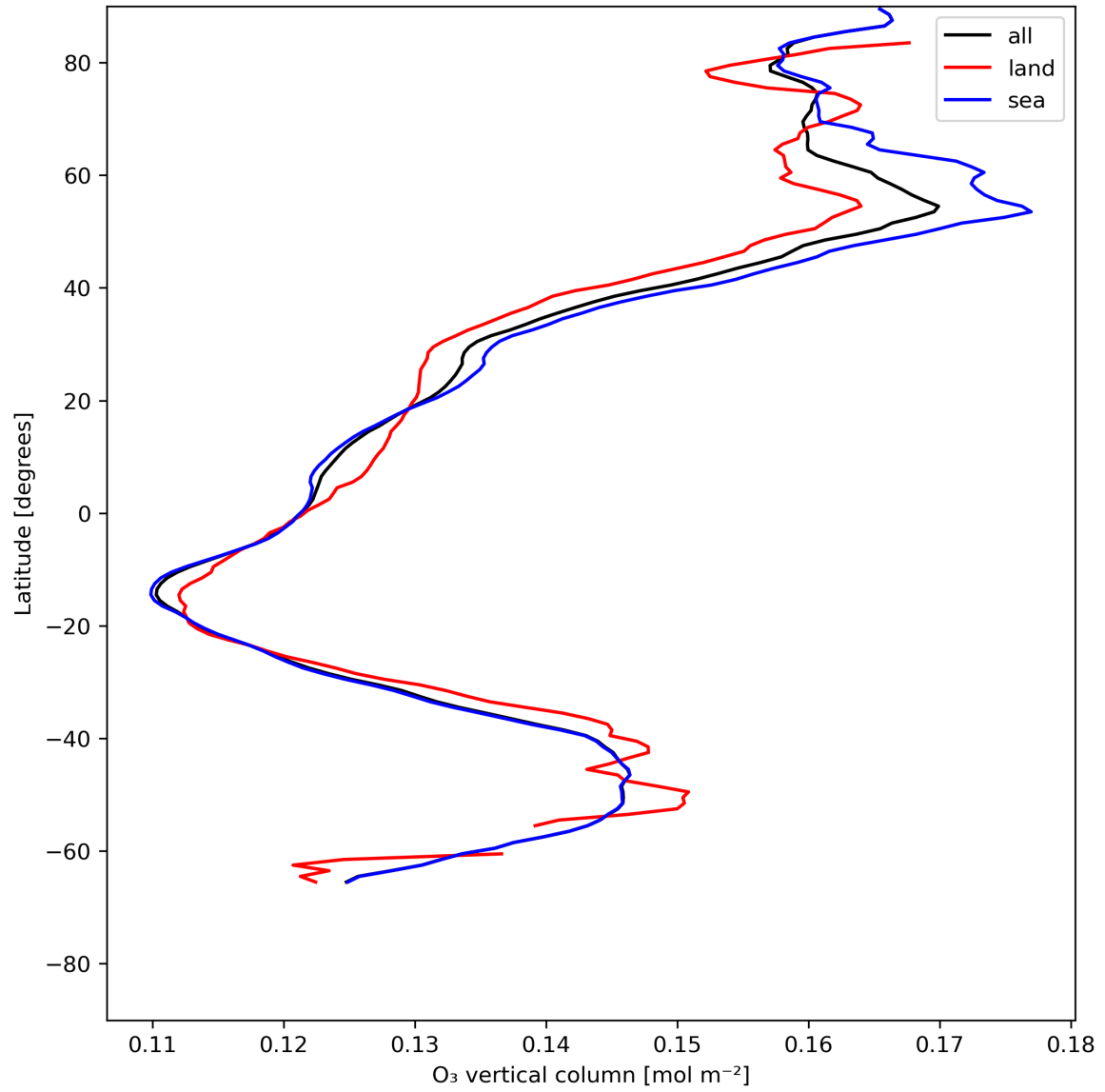
Figure 14: Zonal average of “O 3 vertical column” for 2024-06-24 to 2024-06-26.
