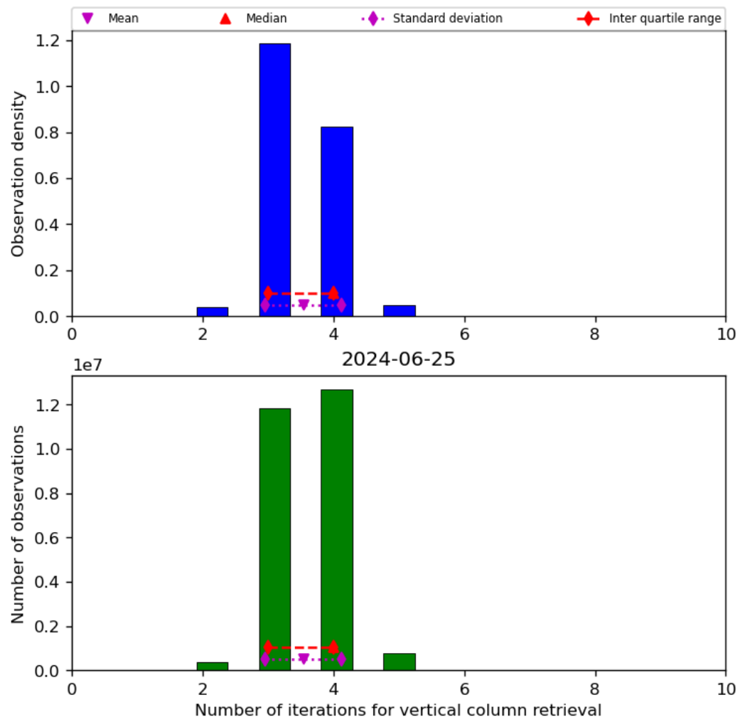
Figure 26: Histogram of “Number of iterations for vertical column retrieval” for 2024-06-24 to 2024-06-26
