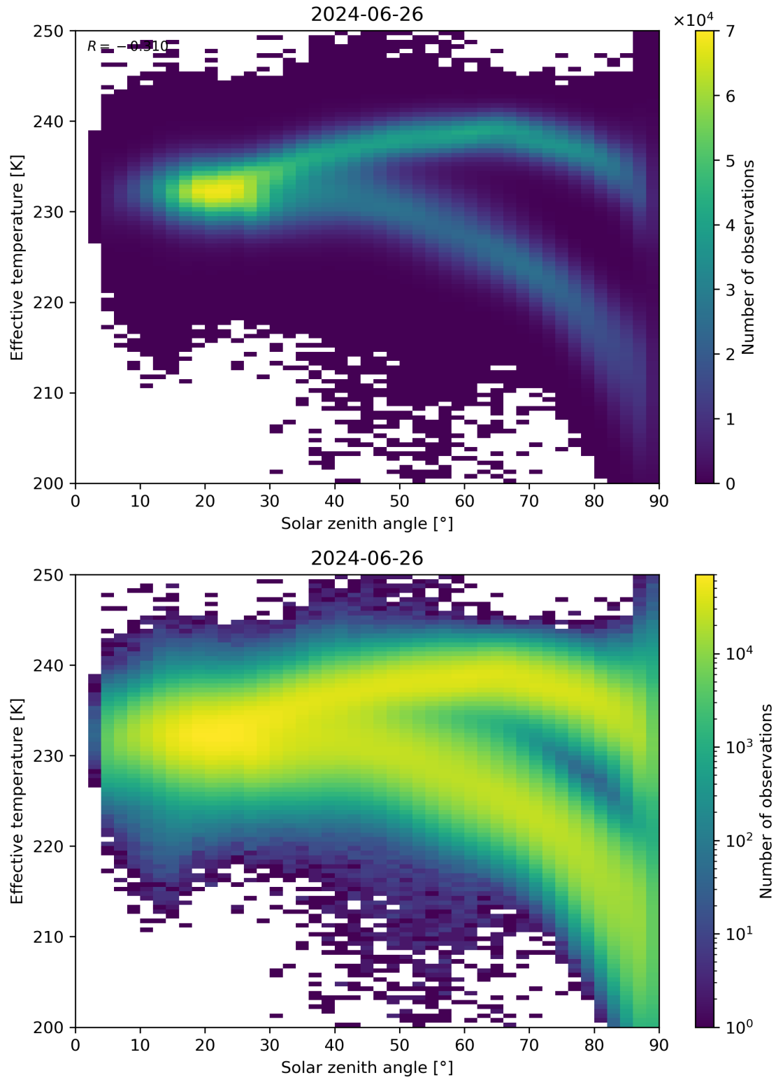
Figure 45: Scatter density plot of “Solar zenith angle” against “Effective temperature” for 2024-06-25 to 2024-06-27.
