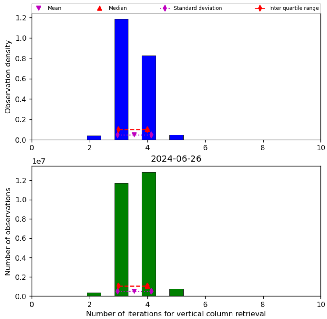
Figure 26: Histogram of “Number of iterations for vertical column retrieval” for 2024-06-25 to 2024-06-27
