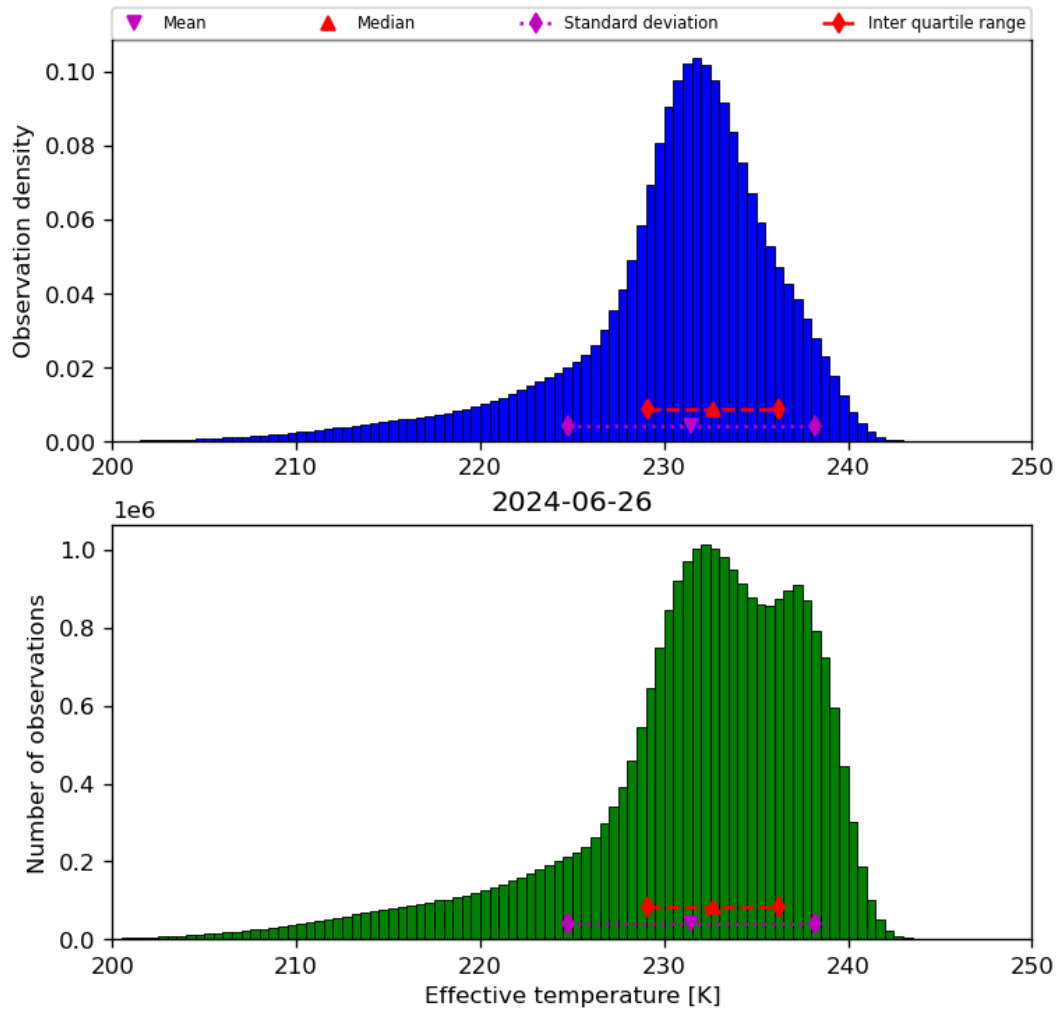
Figure 24: Histogram of “Effective temperature” for 2024-06-25 to 2024-06-27
