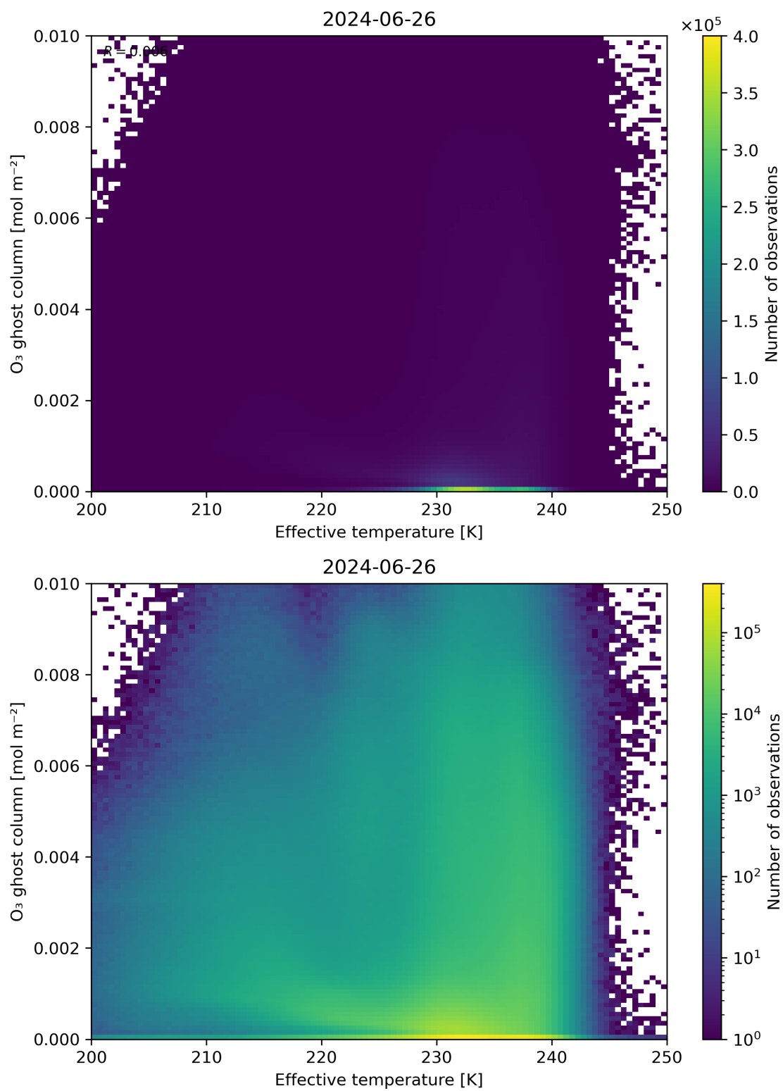
Figure 38: Scatter density plot of “Effective temperature” against “O 3 ghost column” for 2024-06-25 to 2024-06-27.
