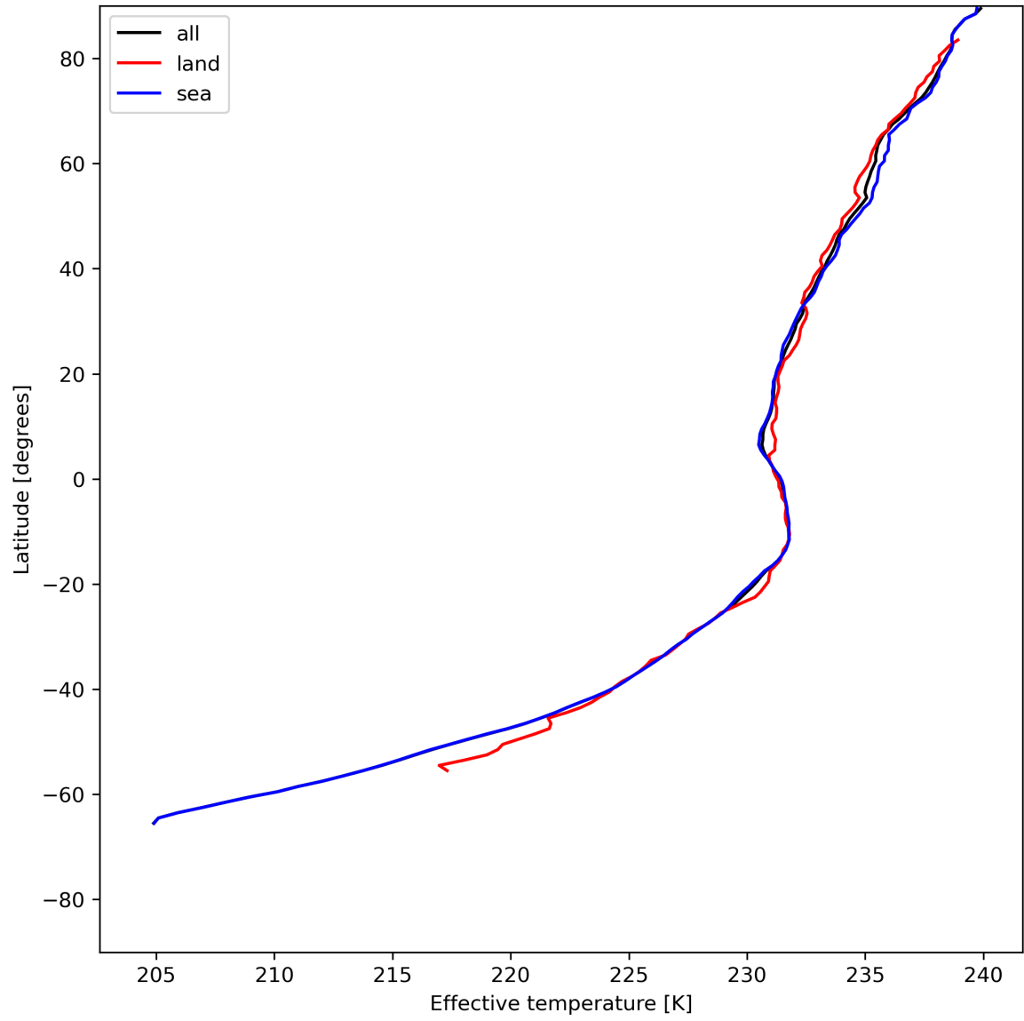
Figure 17: Zonal average of "Effective temperature" for 2024-06-25 to 2024-06-27.
