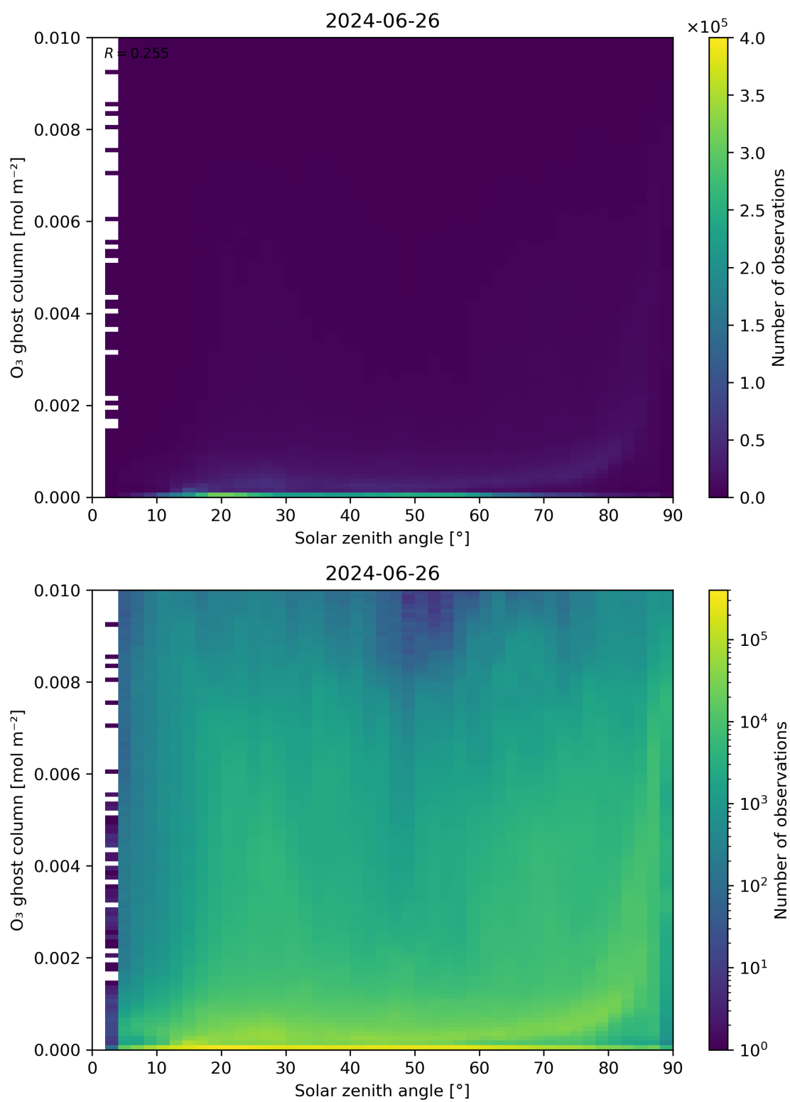
Figure 46: Scatter density plot of “Solar zenith angle” against “O 3 ghost column” for 2024-06-25 to 2024-06-27.
