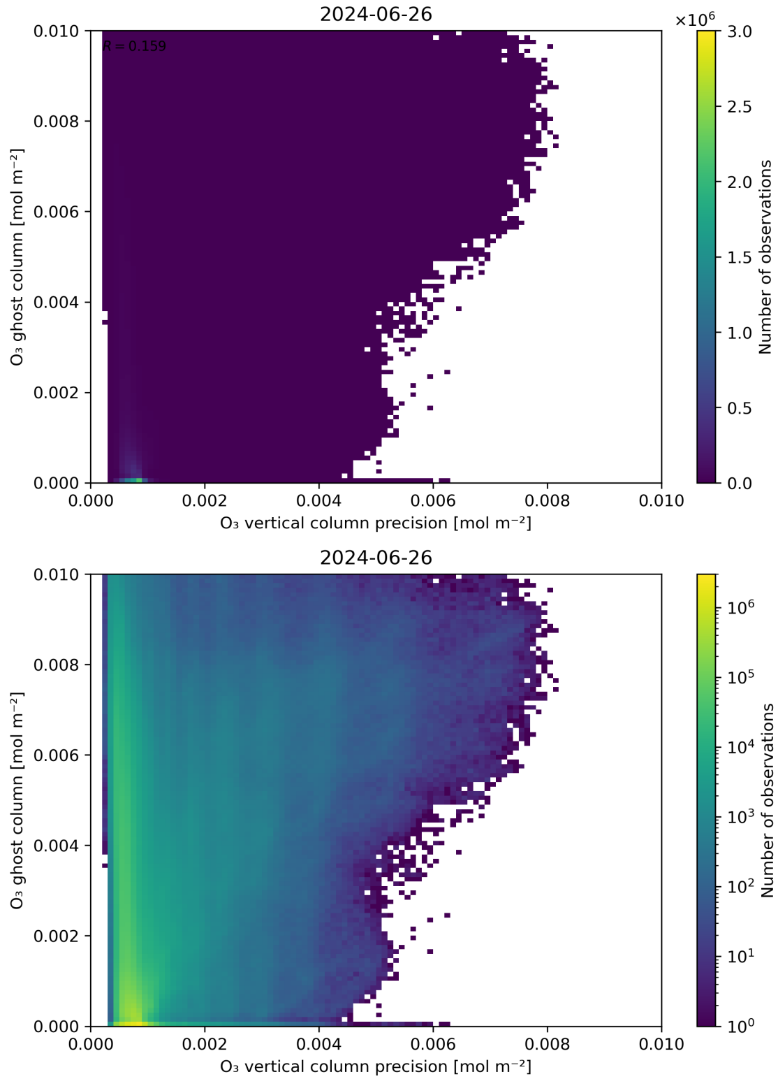
Figure 43: Scatter density plot of “ \text{O}_3 vertical column precision” against “ \text{O}_3 ghost column” for 2024-06-25 to 2024-06-27.
