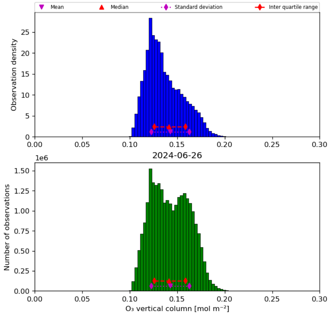
Figure 21: Histogram of “O 3 vertical column” for 2024-06-25 to 2024-06-27
