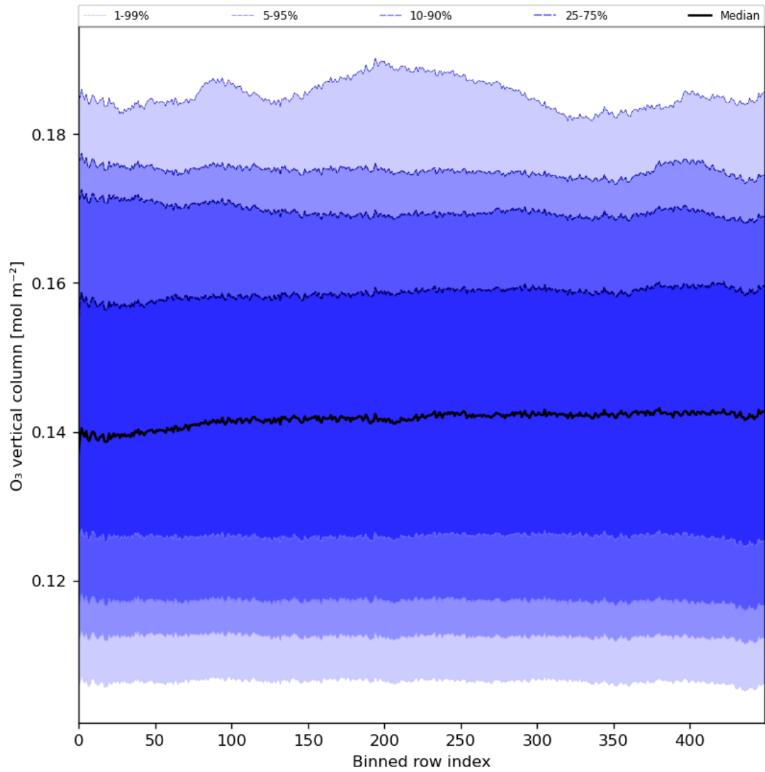
Figure 28: Along track statistics of “O 3 vertical column” for 2024-06-25 to 2024-06-27
