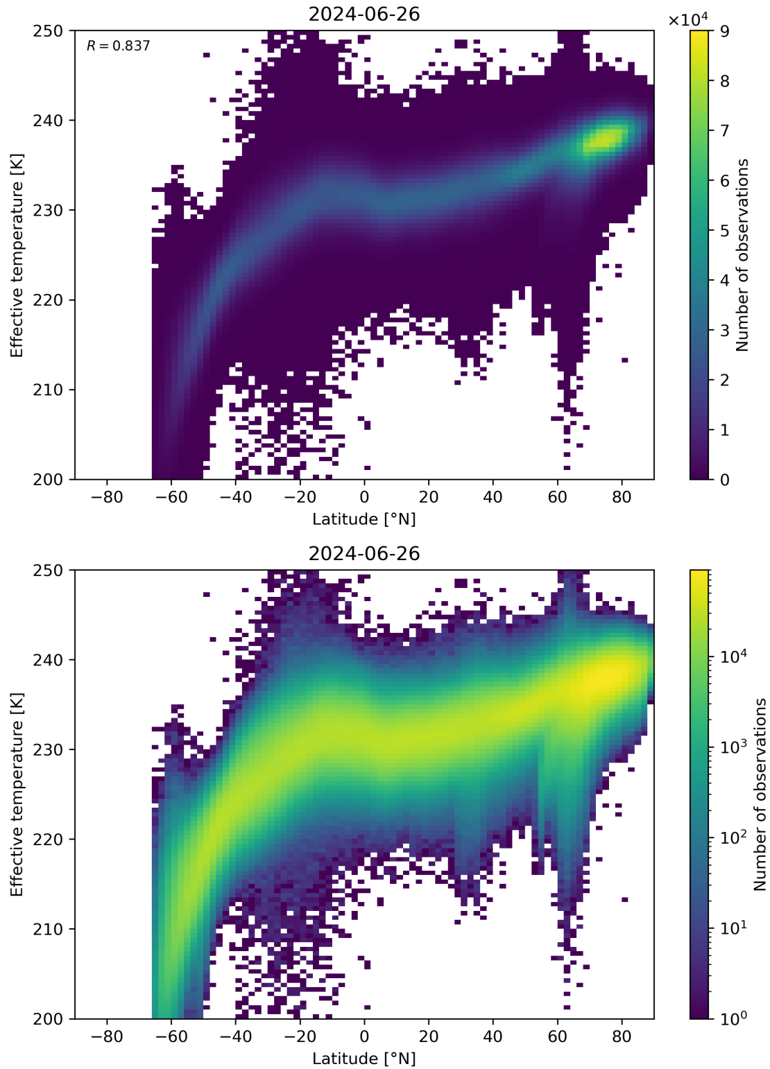
Figure 34: Scatter density plot of “Latitude” against “Effective temperature” for 2024-06-25 to 2024-06-27.
