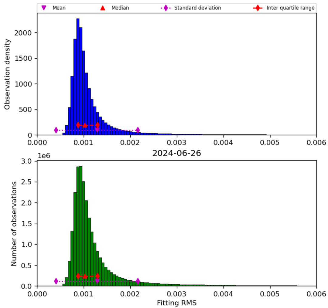
Figure 23: Histogram of “Fitting RMS” for 2024-06-25 to 2024-06-27
