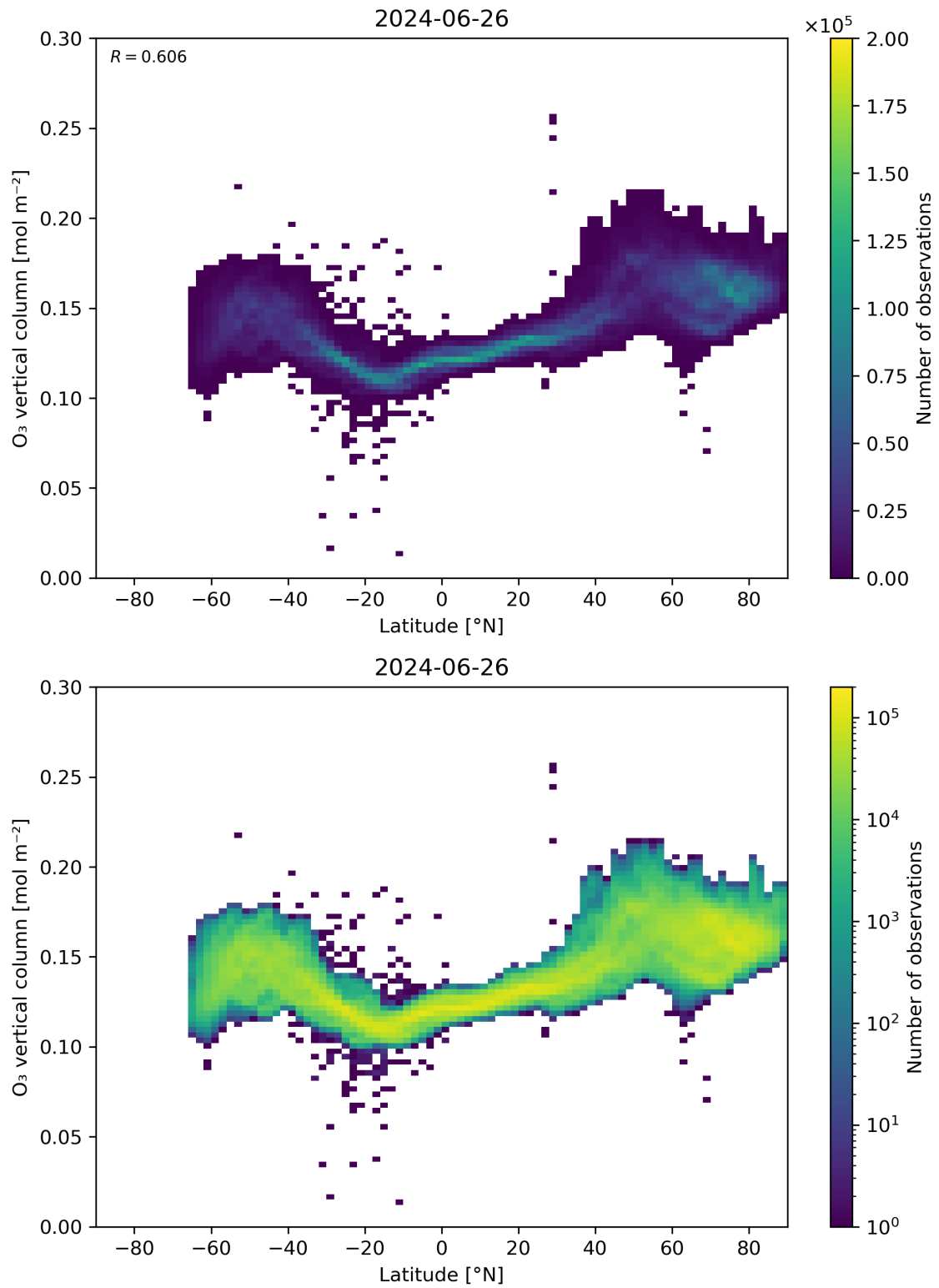
Figure 36: Scatter density plot of “Latitude” against “O 3 vertical column” for 2024-06-25 to 2024-06-27.
