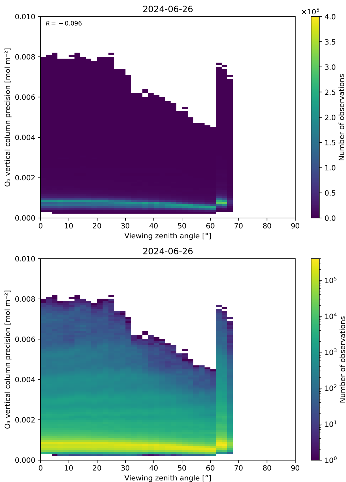
Figure 53: Scatter density plot of “Viewing zenith angle” against “O 3 vertical column precision” for 2024-06-25 to 2024-06-27.
