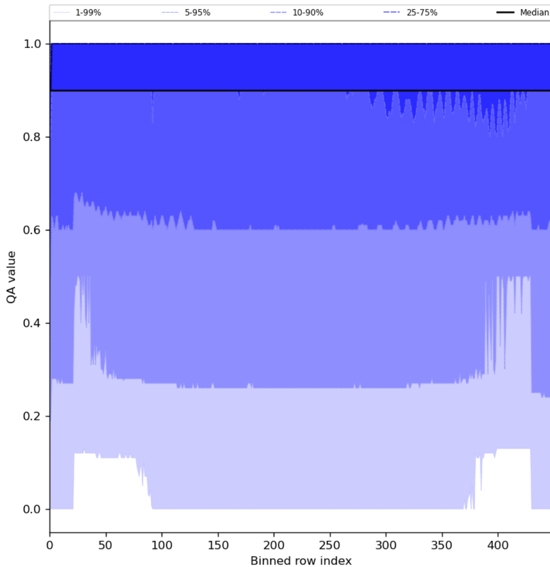
Figure 27: Along track statistics of “QA value” for 2024-06-25 to 2024-06-27
