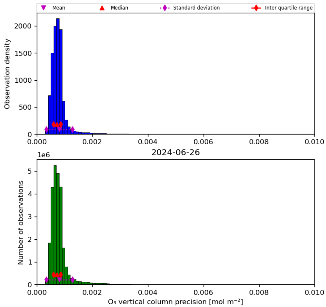
Figure 22: Histogram of “O 3 vertical column precision” for 2024-06-25 to 2024-06-27
