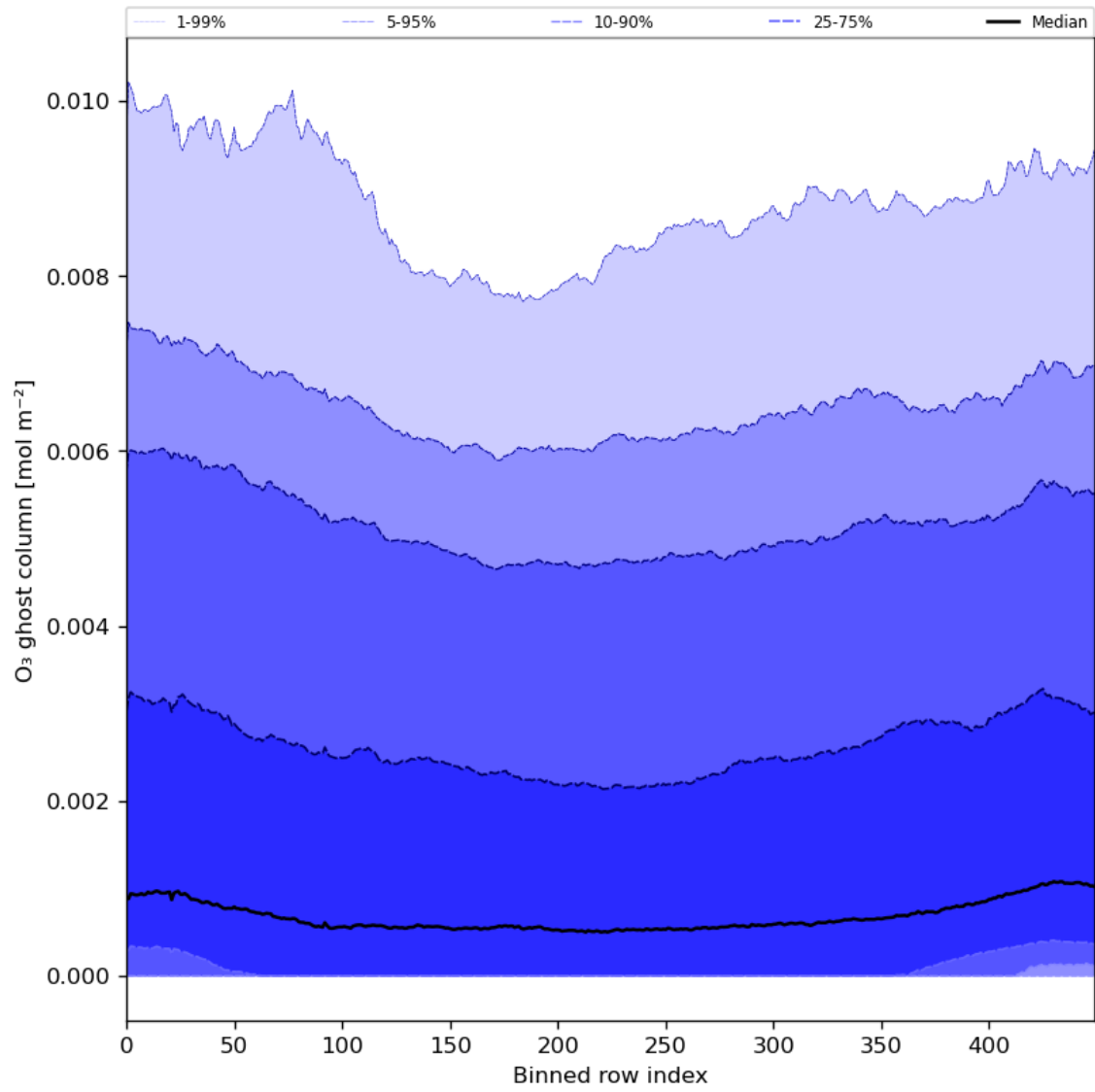
Figure 32: Along track statistics of “O 3 ghost column” for 2024-06-25 to 2024-06-27
