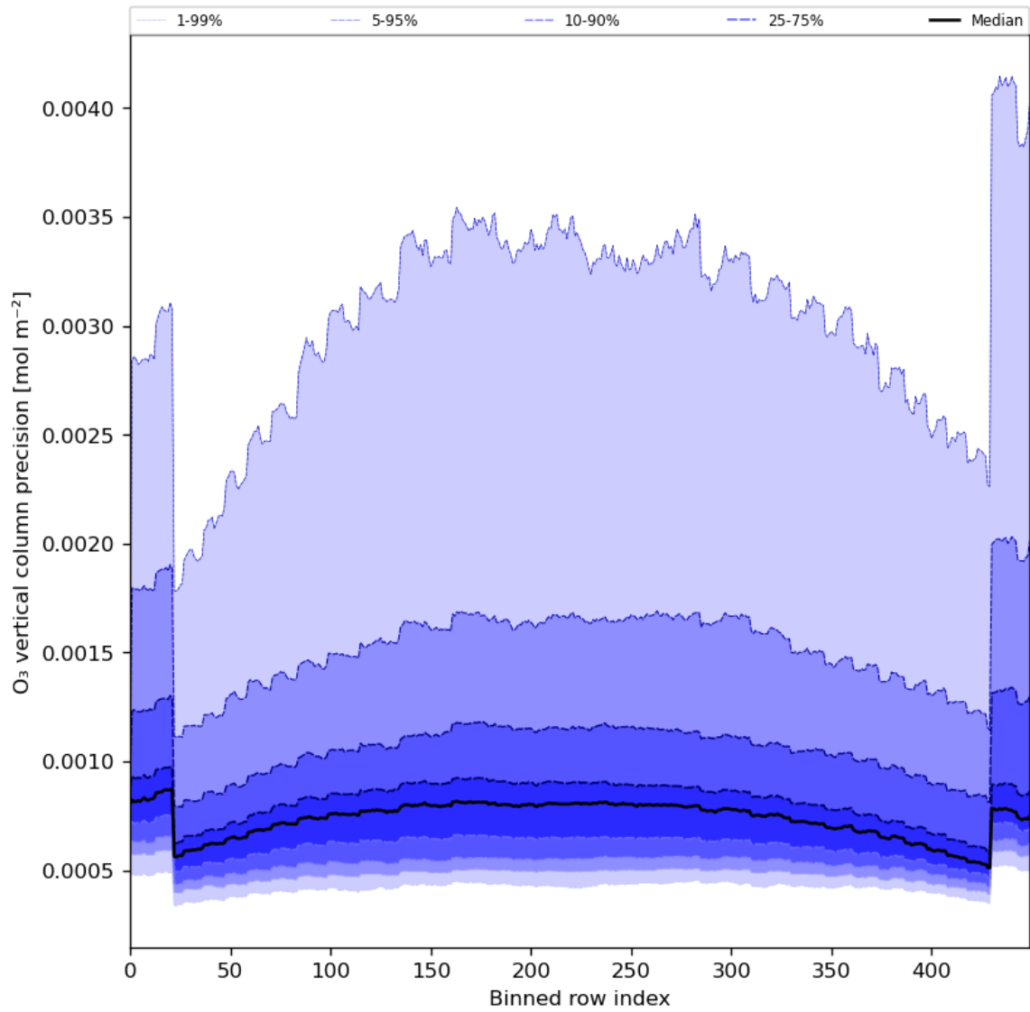
Figure 29: Along track statistics of “O 3 vertical column precision” for 2024-06-25 to 2024-06-27
