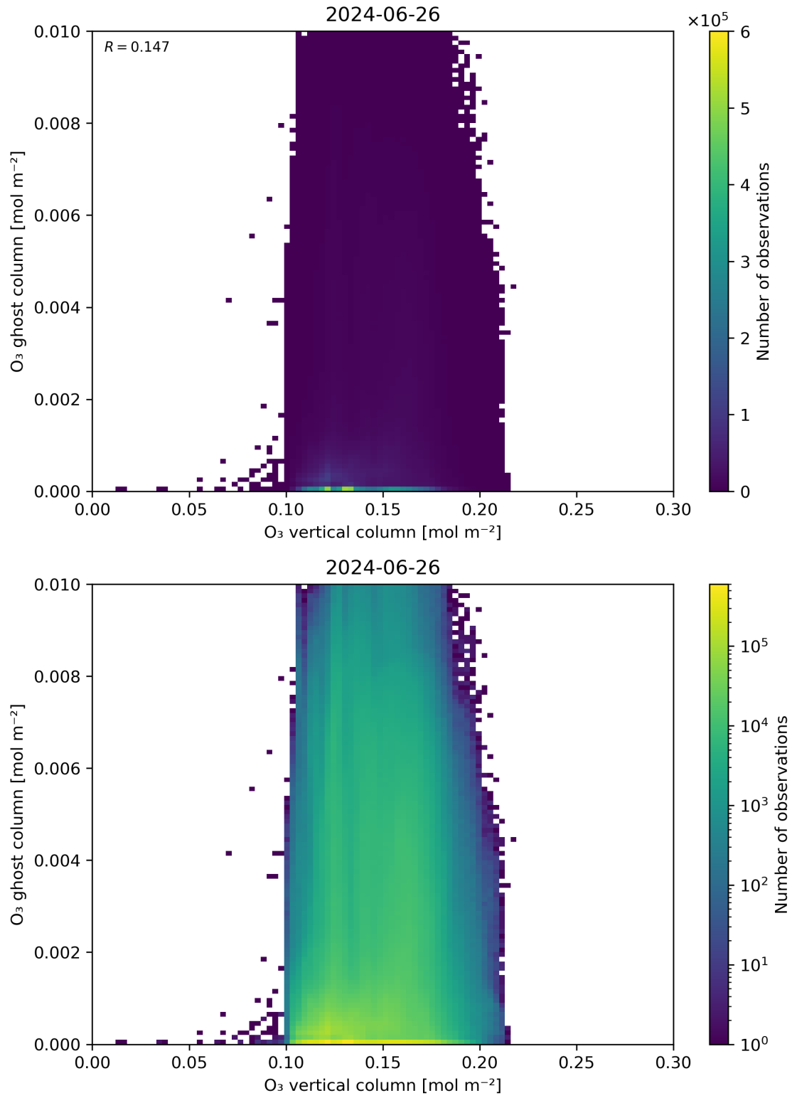
Figure 40: Scatter density plot of “O 3 vertical column” against “O 3 ghost column” for 2024-06-25 to 2024-06-27.
