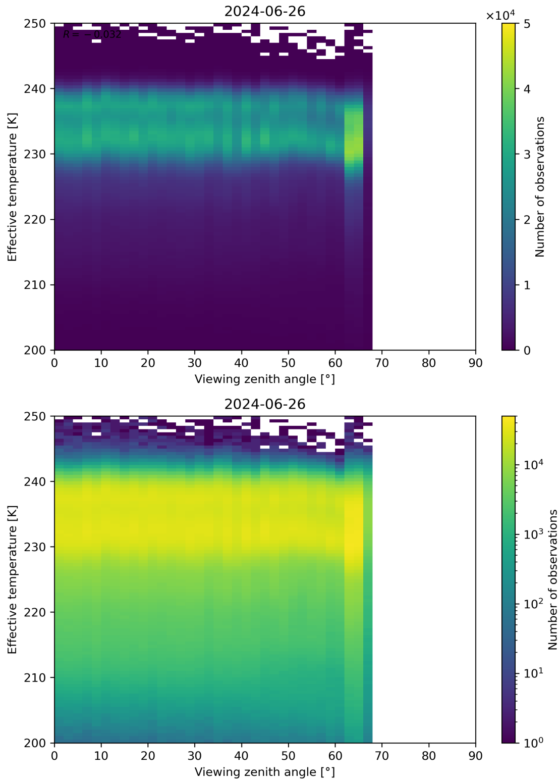
Figure 50: Scatter density plot of “Viewing zenith angle” against “Effective temperature” for 2024-06-25 to 2024-06-27.
