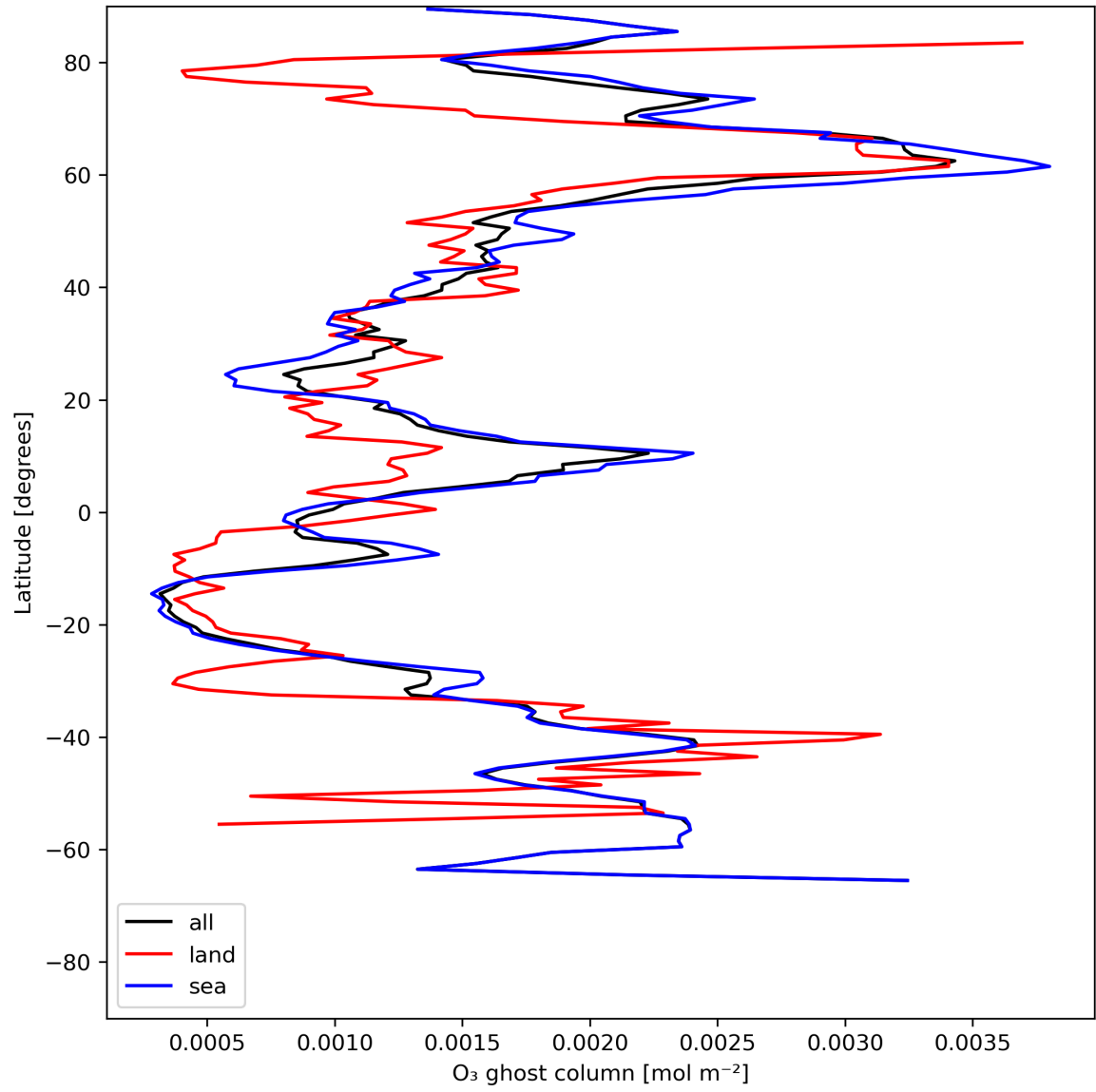
Figure 18: Zonal average of “O 3 ghost column” for 2024-06-25 to 2024-06-27.
