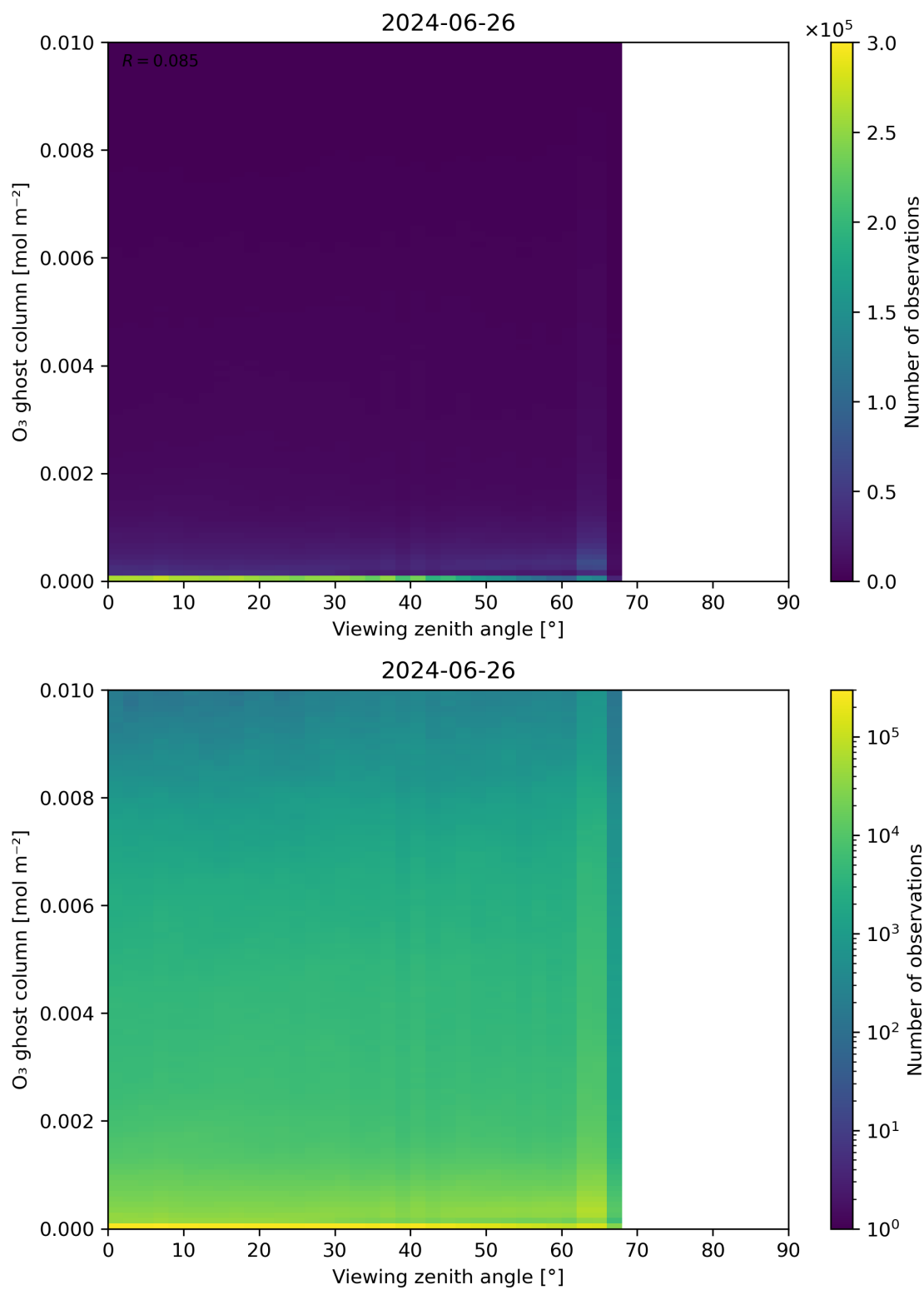
Figure 51: Scatter density plot of “Viewing zenith angle” against “O 3 ghost column” for 2024-06-25 to 2024-06-27.
