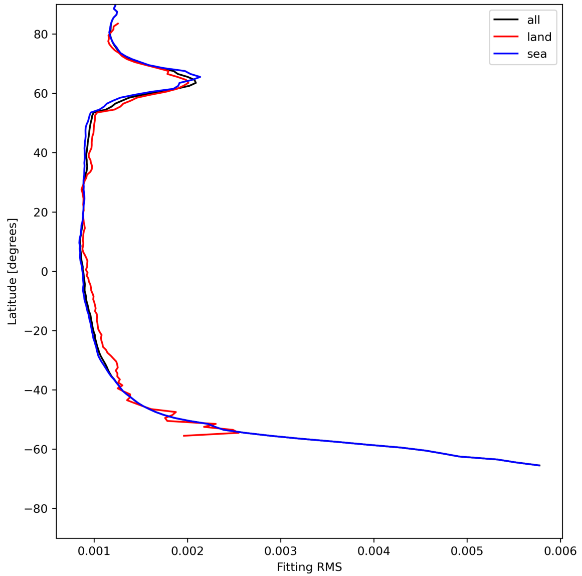
Figure 16: Zonal average of “Fitting RMS” for 2024-06-25 to 2024-06-27.
