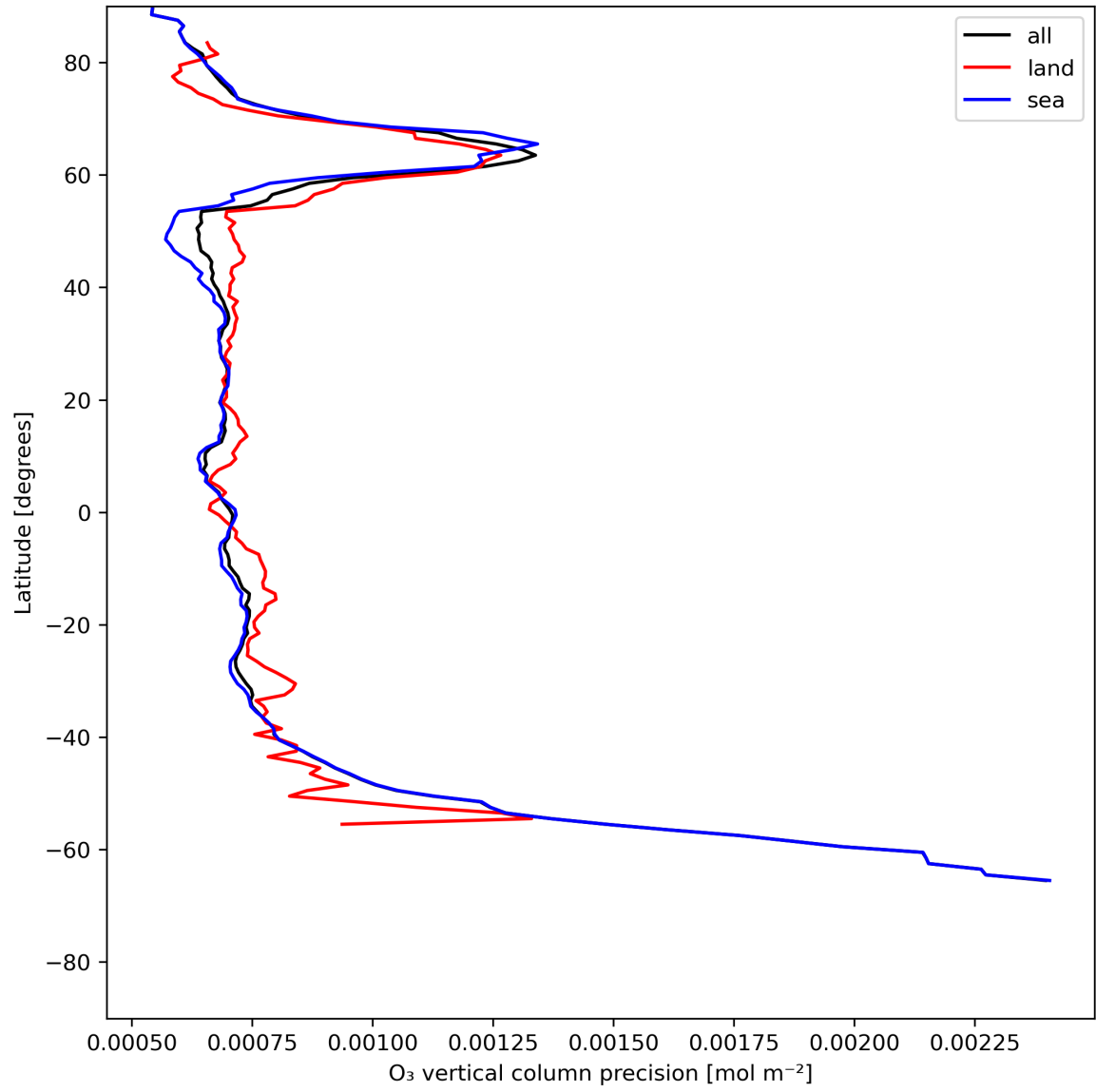
Figure 15: Zonal average of “O 3 vertical column precision” for 2024-06-25 to 2024-06-27.
