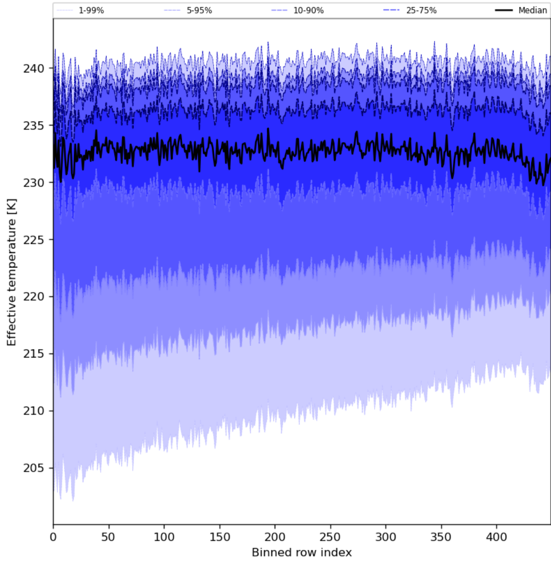
Figure 31: Along track statistics of “Effective temperature” for 2024-06-25 to 2024-06-27
