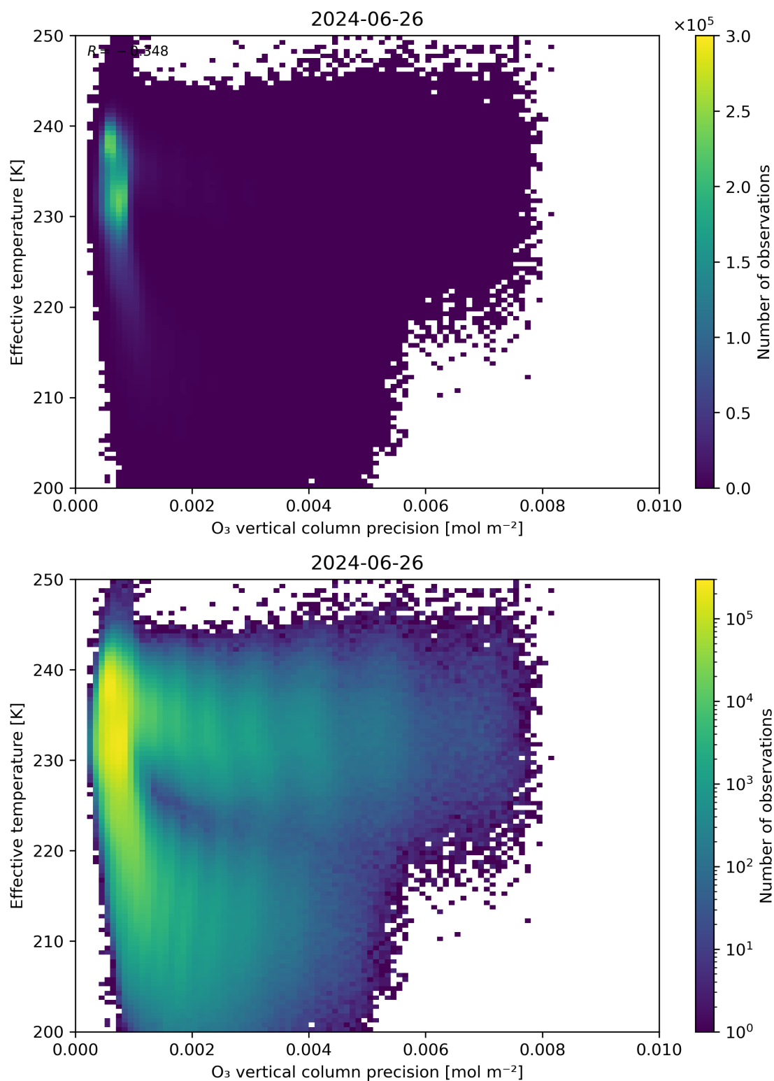
Figure 42: Scatter density plot of “O 3 vertical column precision” against “Effective temperature” for 2024-06-25 to 2024-06-27.
