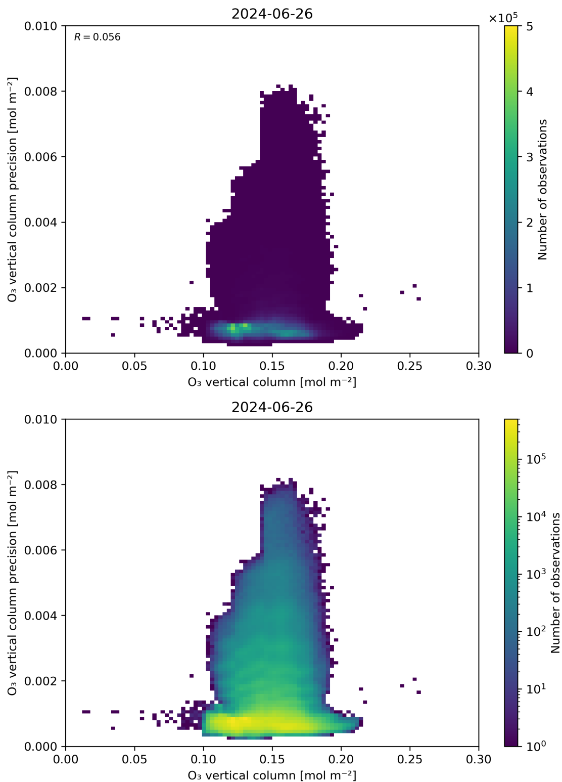
Figure 41: Scatter density plot of “O 3 vertical column” against “O 3 vertical column precision” for 2024-06-25 to 2024-06-27.
