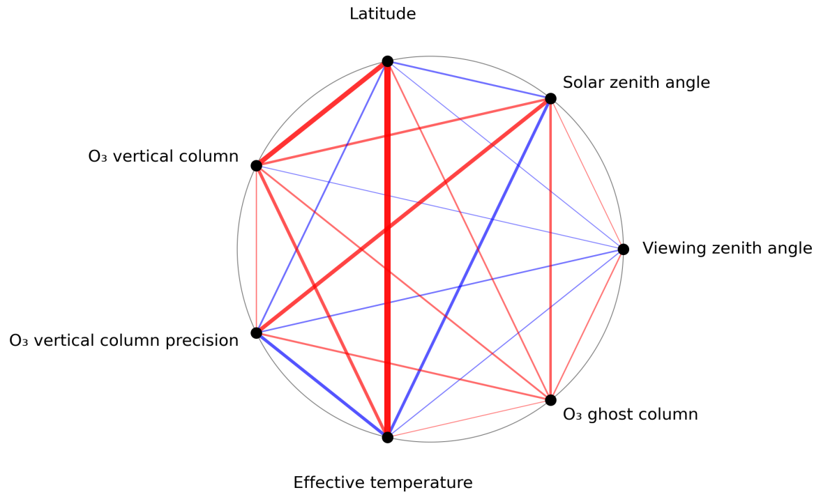
Figure 1: Map of correlation graph for 2024-06-25 to 2024-06-27.
