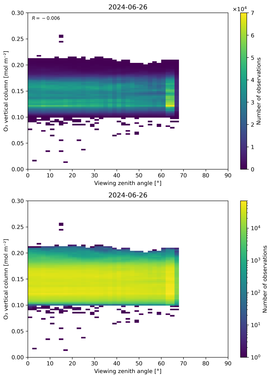
Figure 52: Scatter density plot of “Viewing zenith angle” against “O 3 vertical column” for 2024-06-25 to 2024-06-27.
