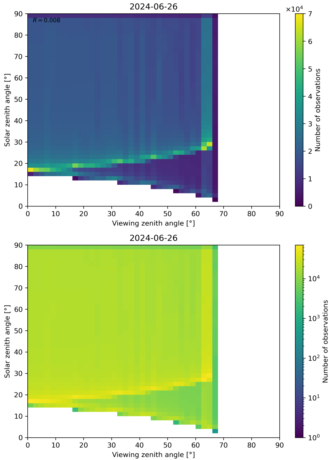
Figure 54: Scatter density plot of “Viewing zenith angle” against “Solar zenith angle” for 2024-06-25 to 2024-06-27.
