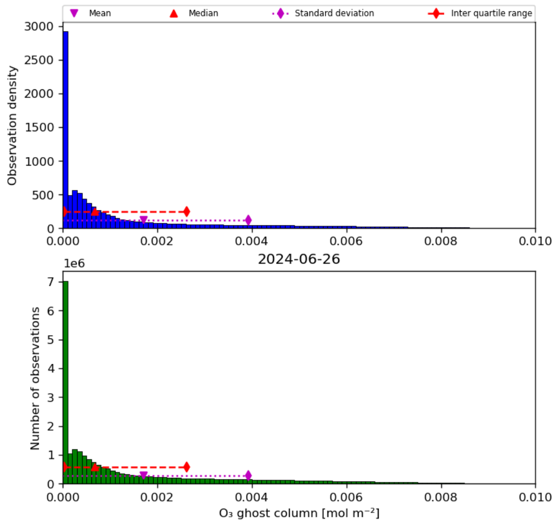
Figure 25: Histogram of “O 3 ghost column” for 2024-06-25 to 2024-06-27
