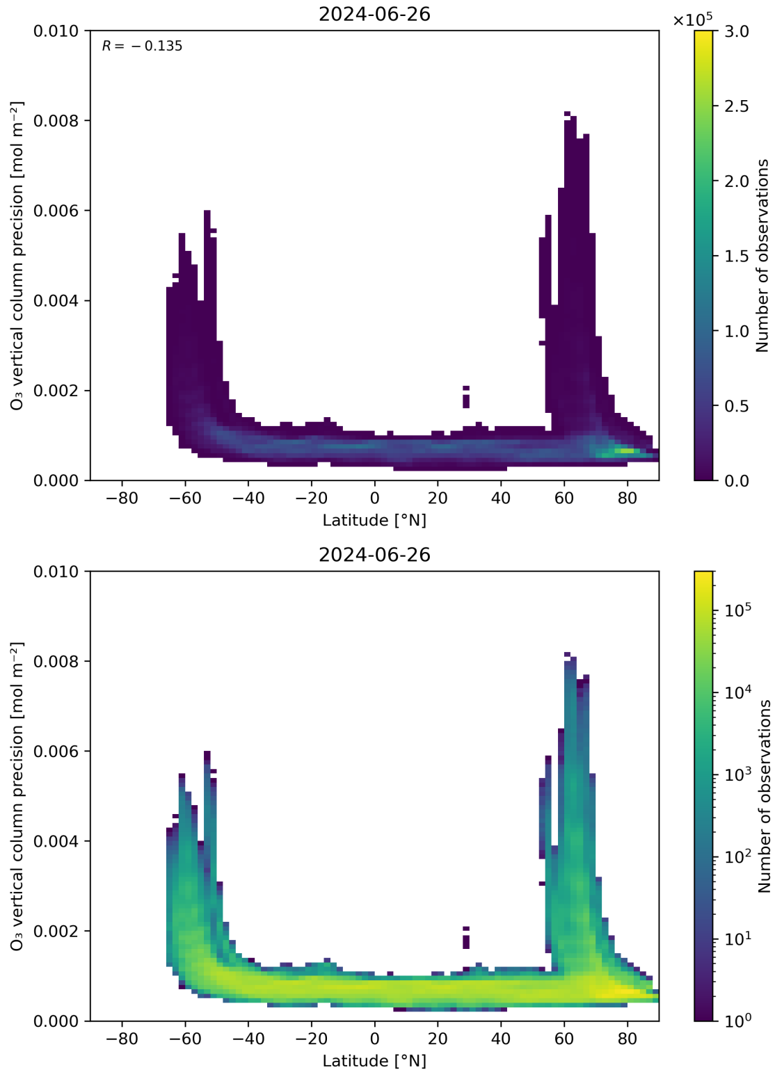
Figure 37: Scatter density plot of “Latitude” against “O 3 vertical column precision” for 2024-06-25 to 2024-06-27.
