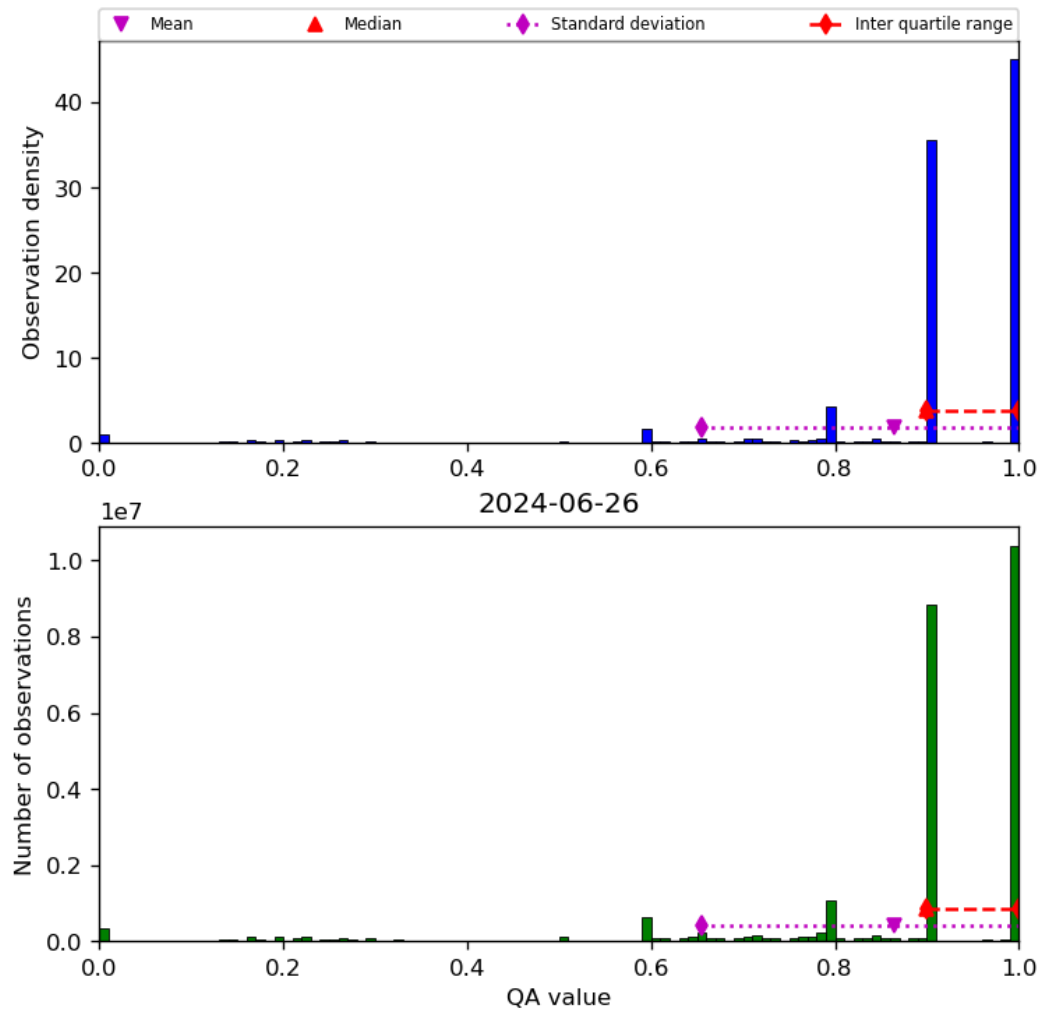
Figure 20: Histogram of “QA value” for 2024-06-25 to 2024-06-27
