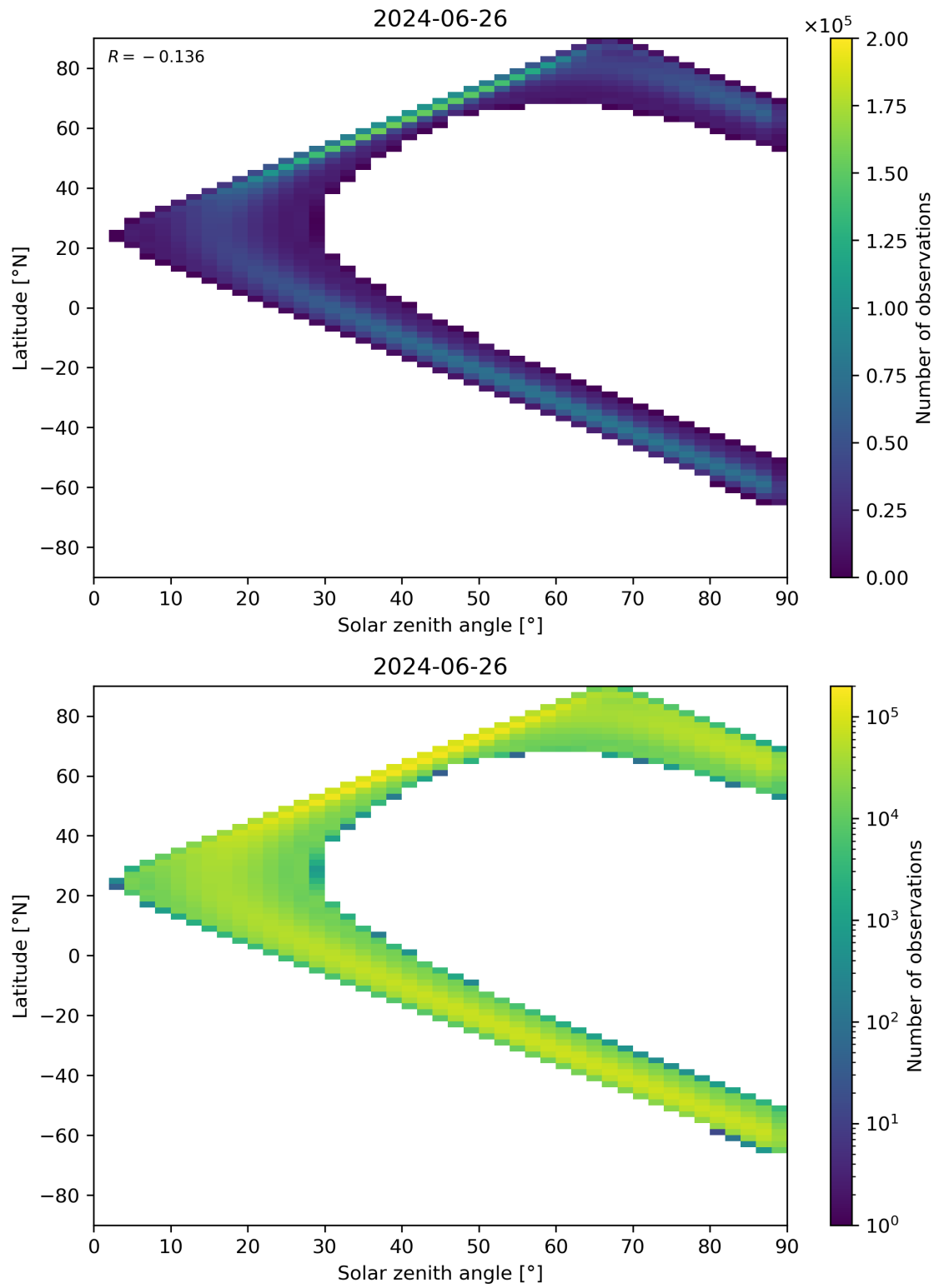
Figure 44: Scatter density plot of “Solar zenith angle” against “Latitude” for 2024-06-25 to 2024-06-27.
