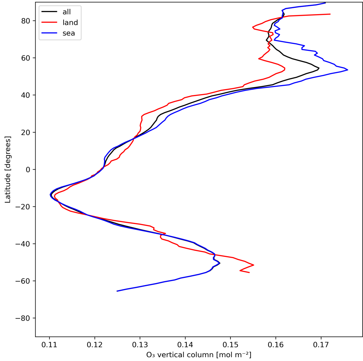
Figure 14: Zonal average of “O 3 vertical column” for 2024-06-25 to 2024-06-27.
