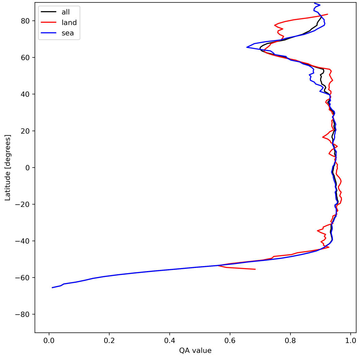
Figure 13: Zonal average of “QA value” for 2024-06-25 to 2024-06-27.
