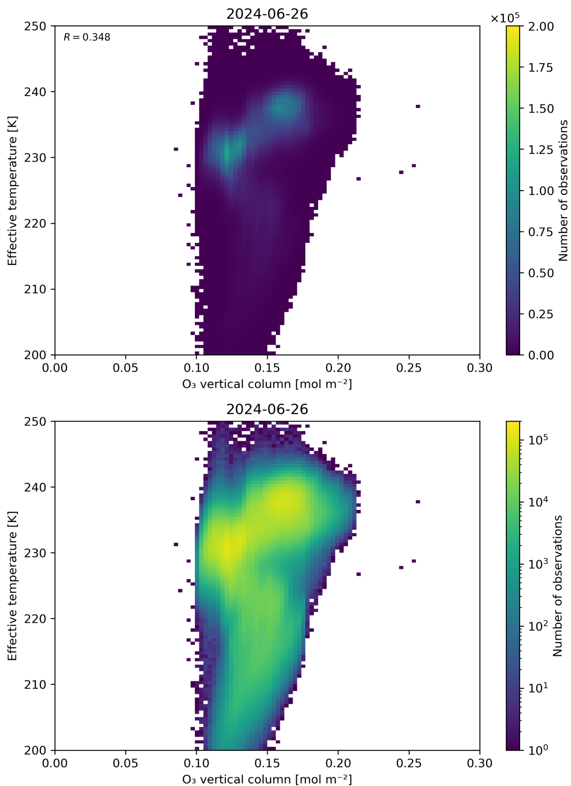
Figure 39: Scatter density plot of “O 3 vertical column” against “Effective temperature” for 2024-06-25 to 2024-06-27.
