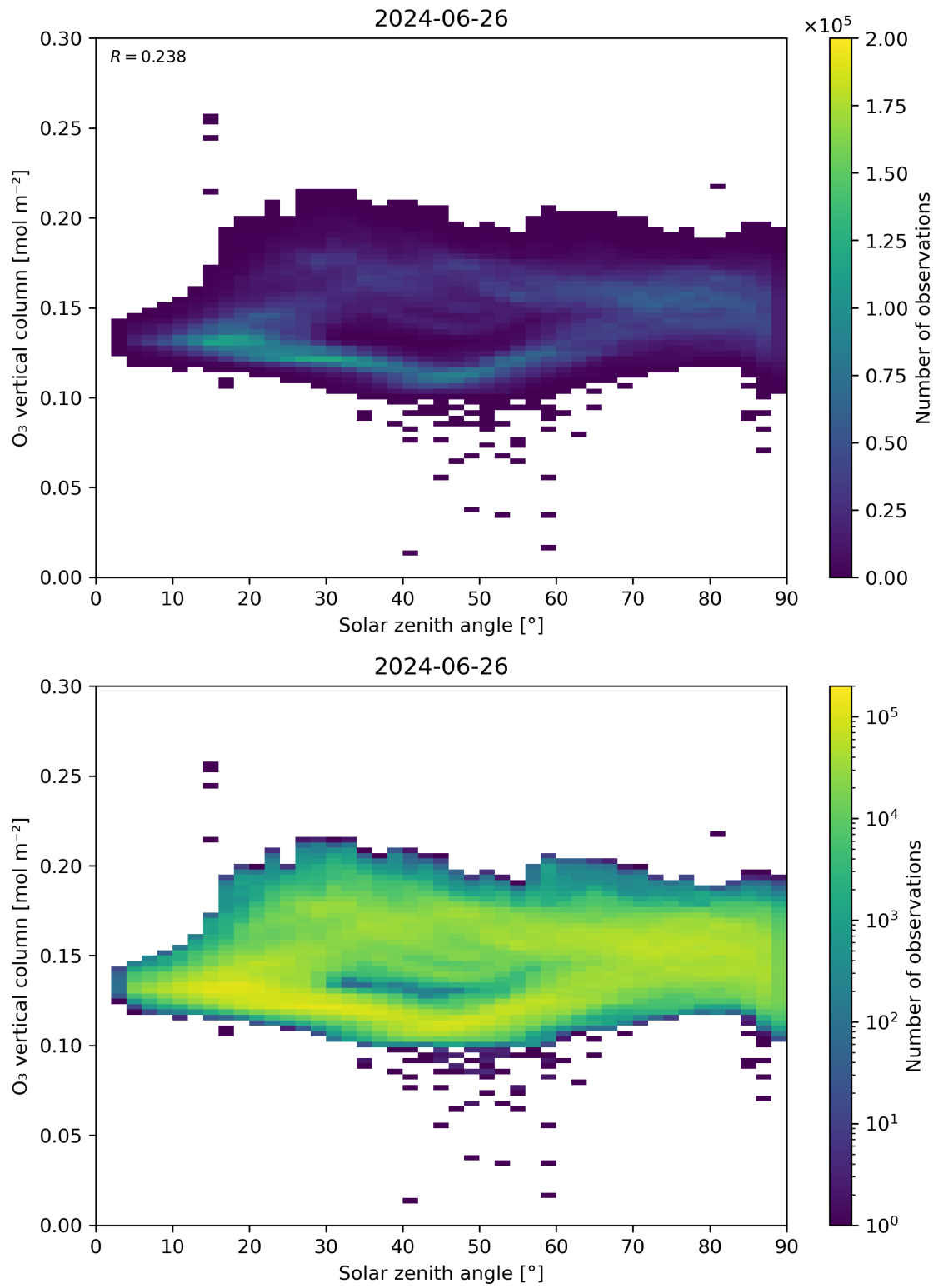
Figure 47: Scatter density plot of “Solar zenith angle” against “O 3 vertical column” for 2024-06-25 to 2024-06-27.
