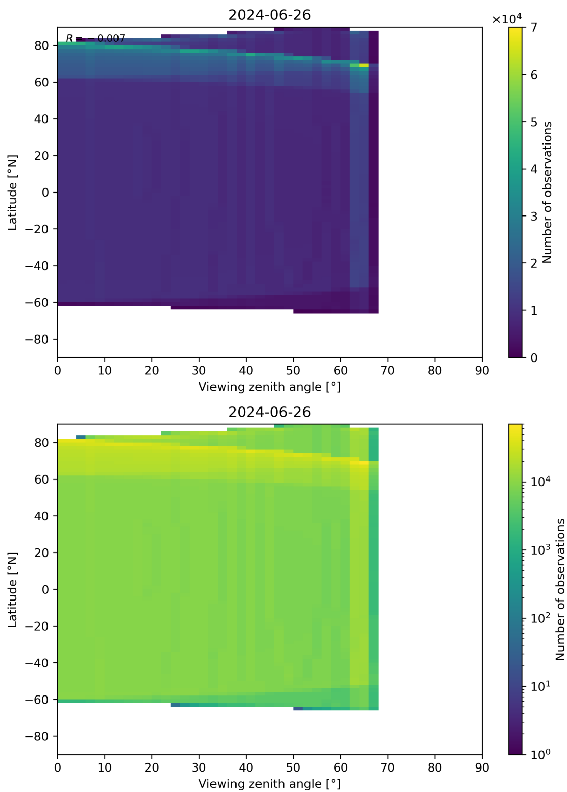
Figure 49: Scatter density plot of “Viewing zenith angle” against “Latitude” for 2024-06-25 to 2024-06-27.
