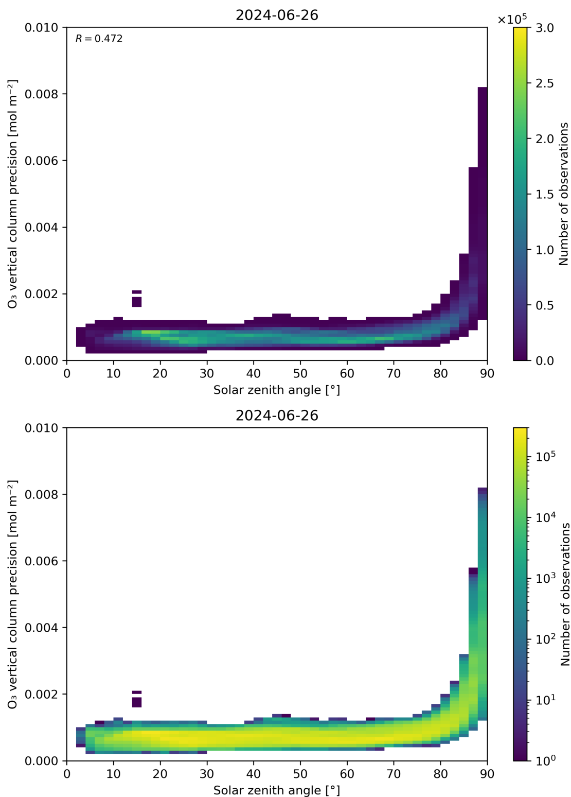
Figure 48: Scatter density plot of “Solar zenith angle” against “O 3 vertical column precision” for 2024-06-25 to 2024-06-27.
