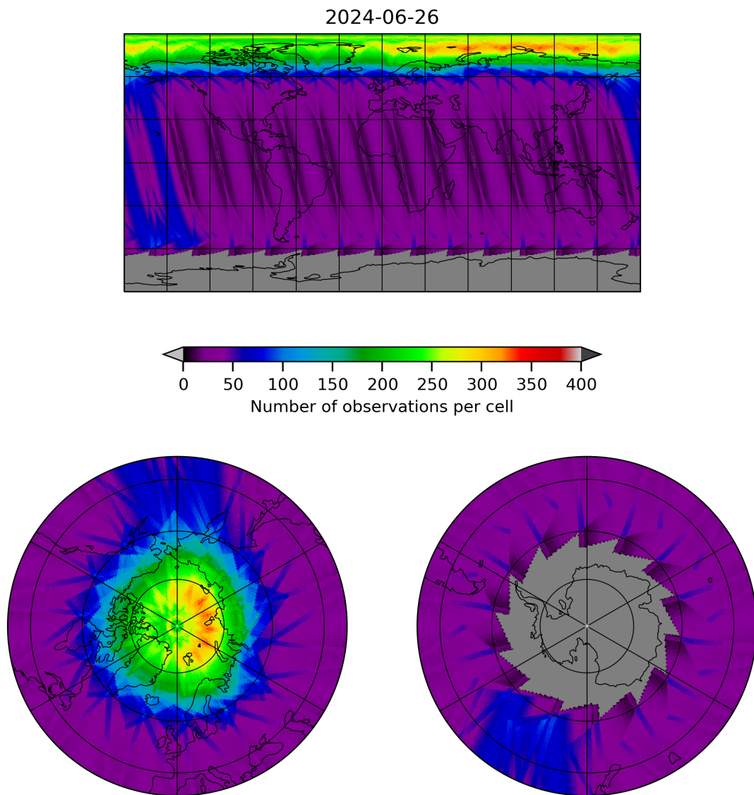
Figure 12: Map of the number of observations for 2024-06-25 to 2024-06-27
