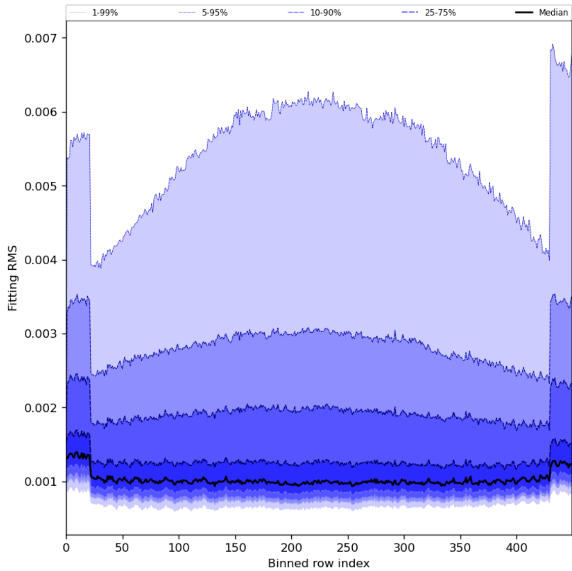
Figure 30: Along track statistics of “Fitting RMS” for 2024-06-25 to 2024-06-27
