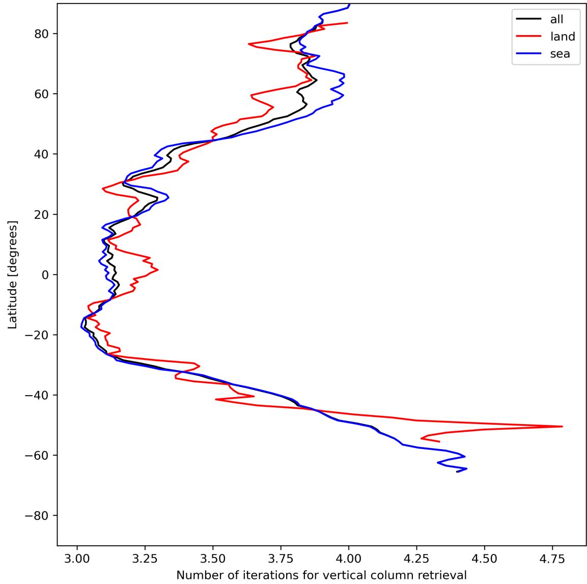
Figure 19: Zonal average of “Number of iterations for vertical column retrieval” for 2024-06-25 to 2024-06-27.
