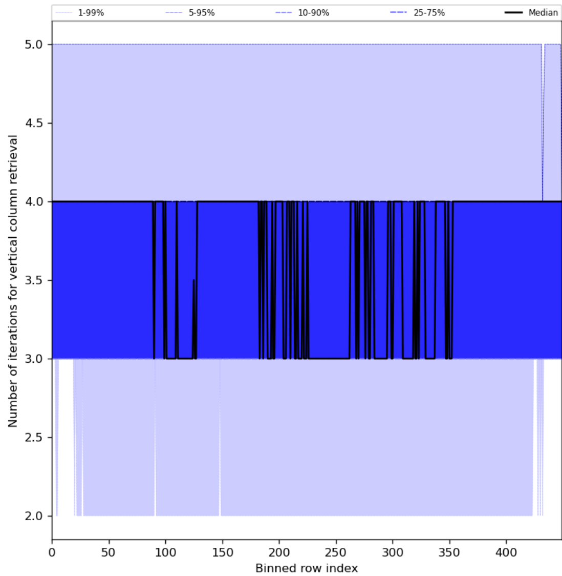
Figure 33: Along track statistics of “Number of iterations for vertical column retrieval” for 2024-06-25 to 2024-06-27
