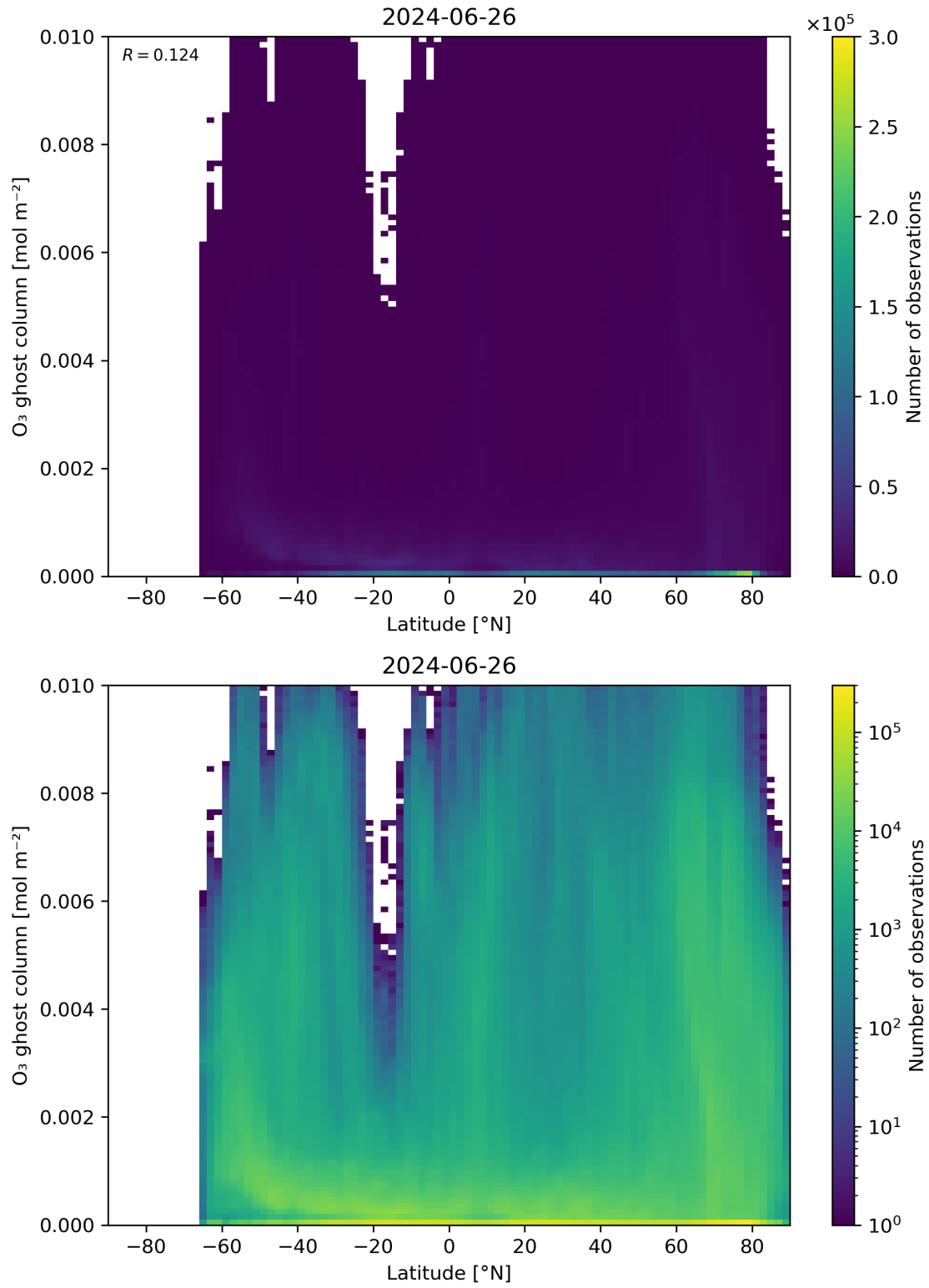
Figure 35: Scatter density plot of “Latitude” against “O 3 ghost column” for 2024-06-25 to 2024-06-27.
