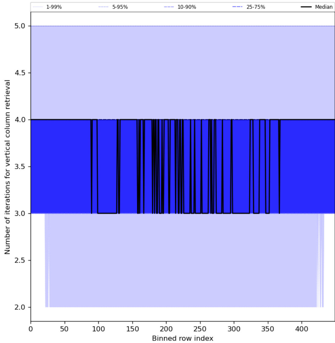
Figure 33: Along track statistics of “Number of iterations for vertical column retrieval” for 2024-06-26 to 2024-06-28
