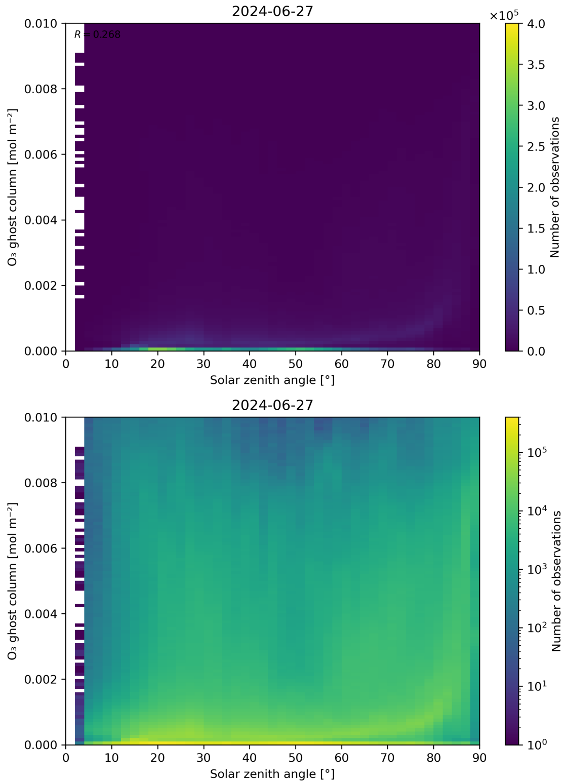
Figure 46: Scatter density plot of “Solar zenith angle” against “O 3 ghost column” for 2024-06-26 to 2024-06-28.
