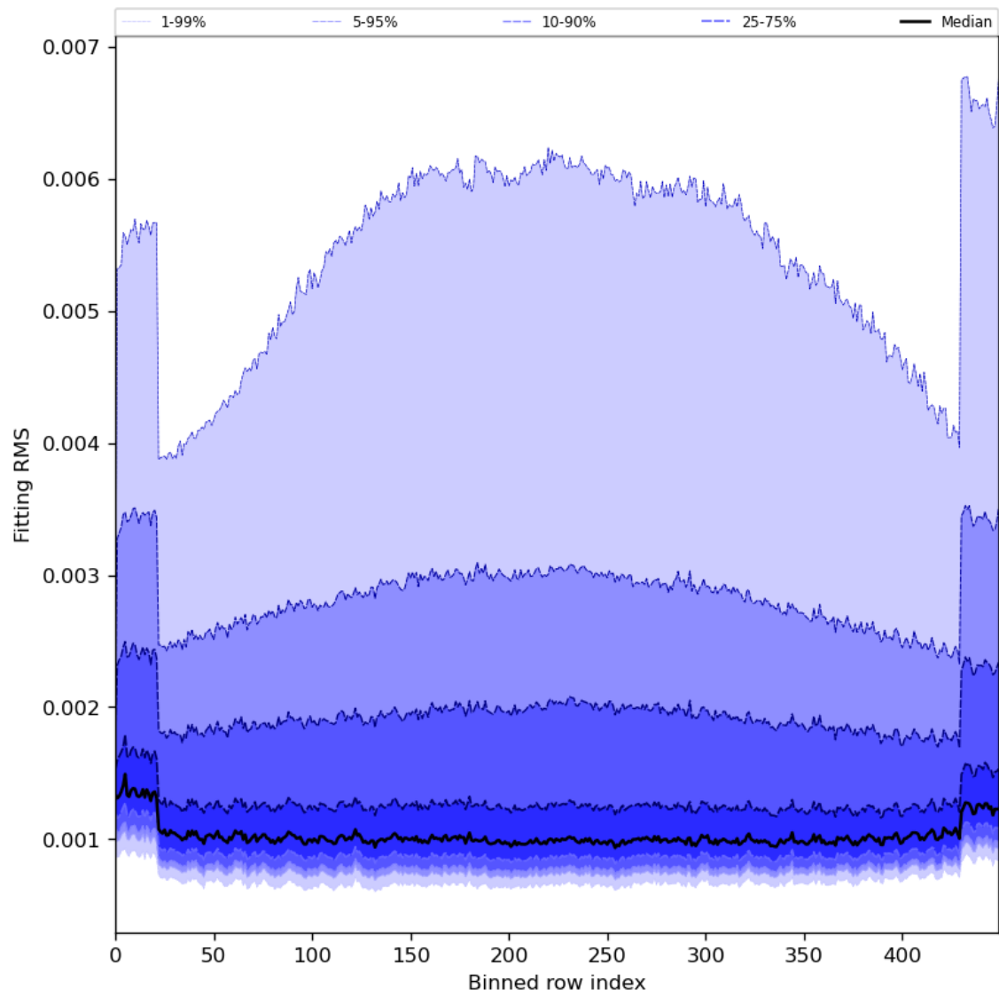
Figure 30: Along track statistics of “Fitting RMS” for 2024-06-26 to 2024-06-28
