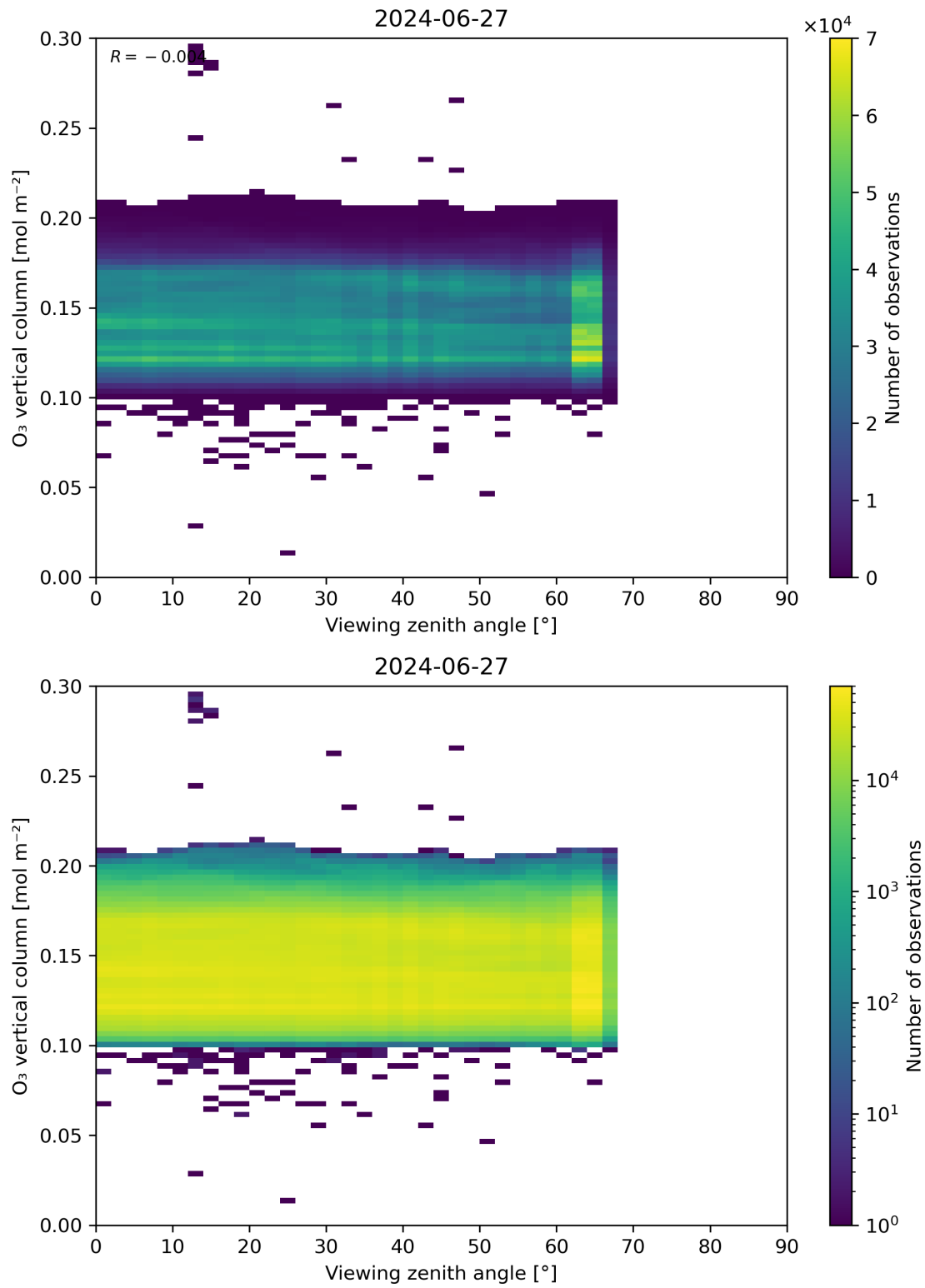
Figure 52: Scatter density plot of “Viewing zenith angle” against “O 3 vertical column” for 2024-06-26 to 2024-06-28.
