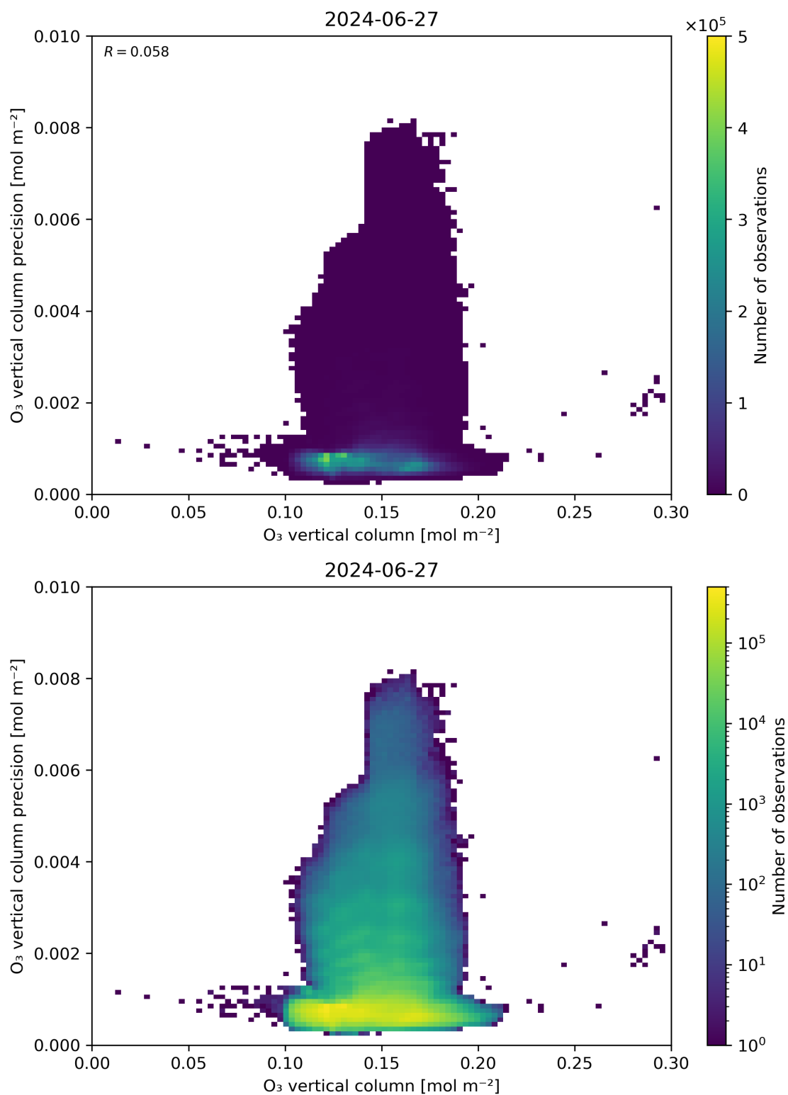
Figure 41: Scatter density plot of “O 3 vertical column” against “O 3 vertical column precision” for 2024-06-26 to 2024-06-28.
