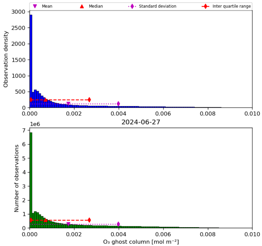
Figure 25: Histogram of “O 3 ghost column” for 2024-06-26 to 2024-06-28
