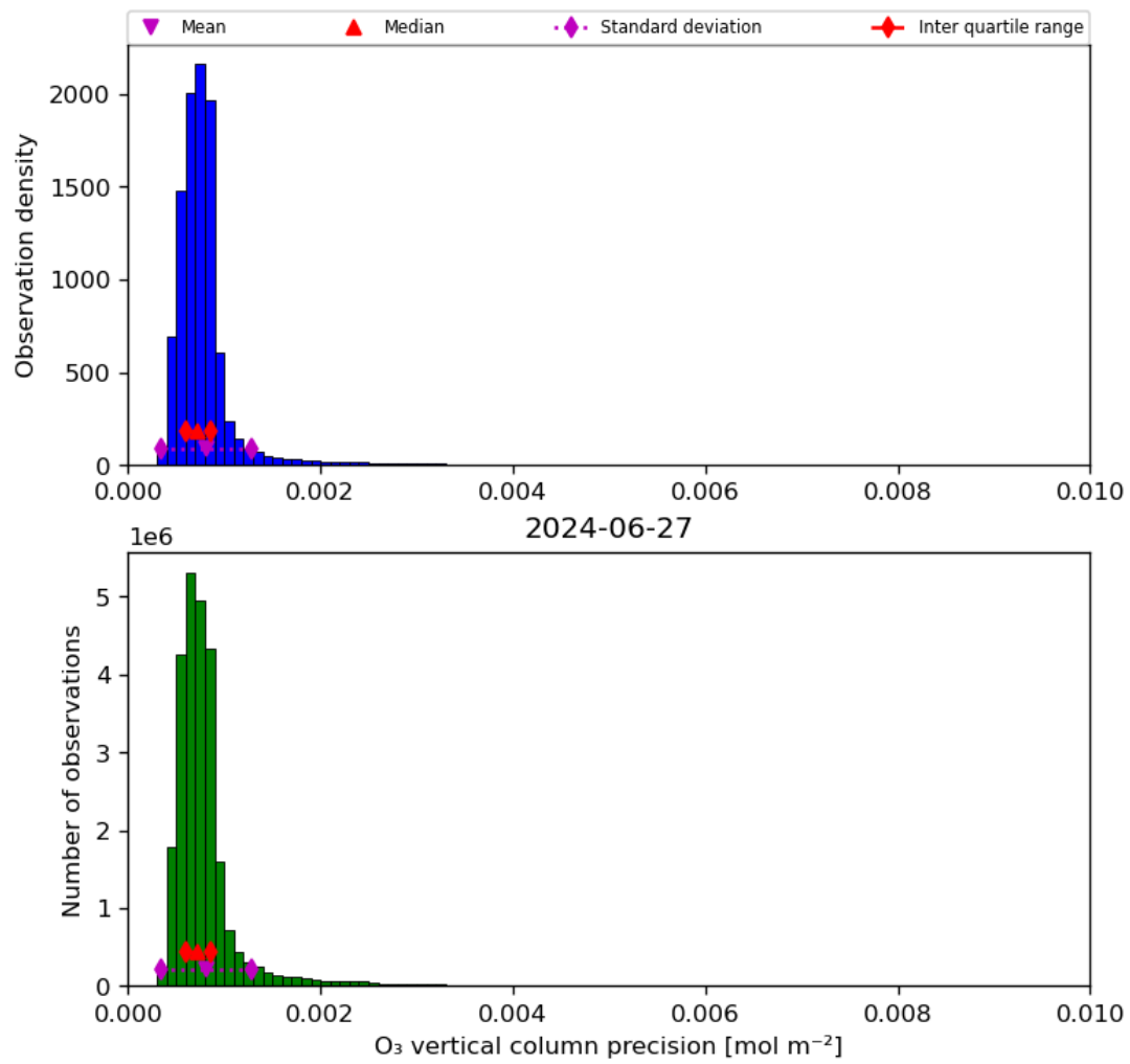
Figure 22: Histogram of “O 3 vertical column precision” for 2024-06-26 to 2024-06-28
