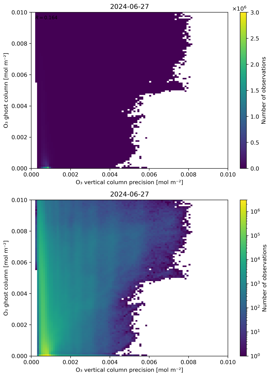
Figure 43: Scatter density plot of “ \text{O}_3 vertical column precision” against “ \text{O}_3 ghost column” for 2024-06-26 to 2024-06-28.
