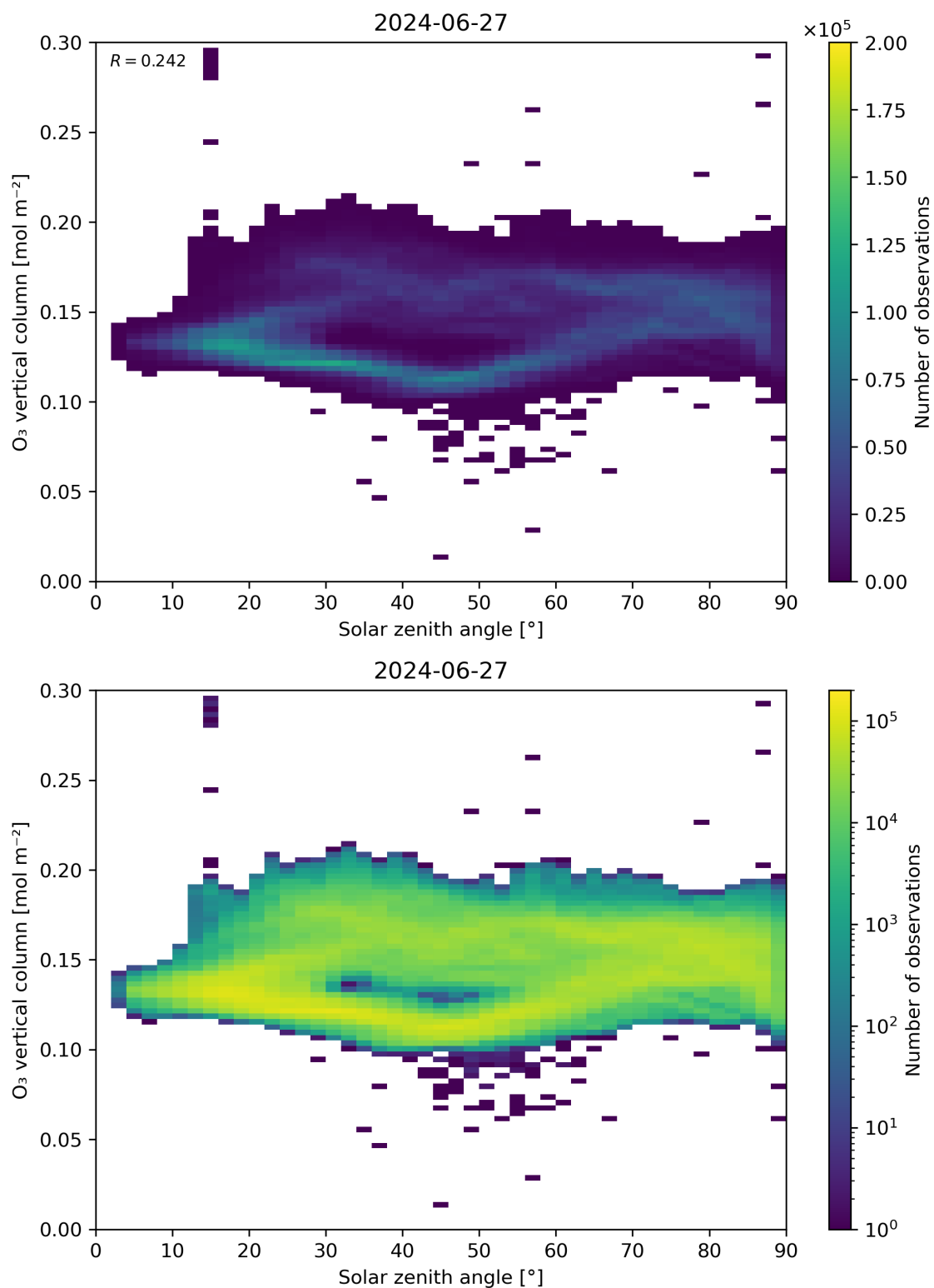
Figure 47: Scatter density plot of “Solar zenith angle” against “O 3 vertical column” for 2024-06-26 to 2024-06-28.
