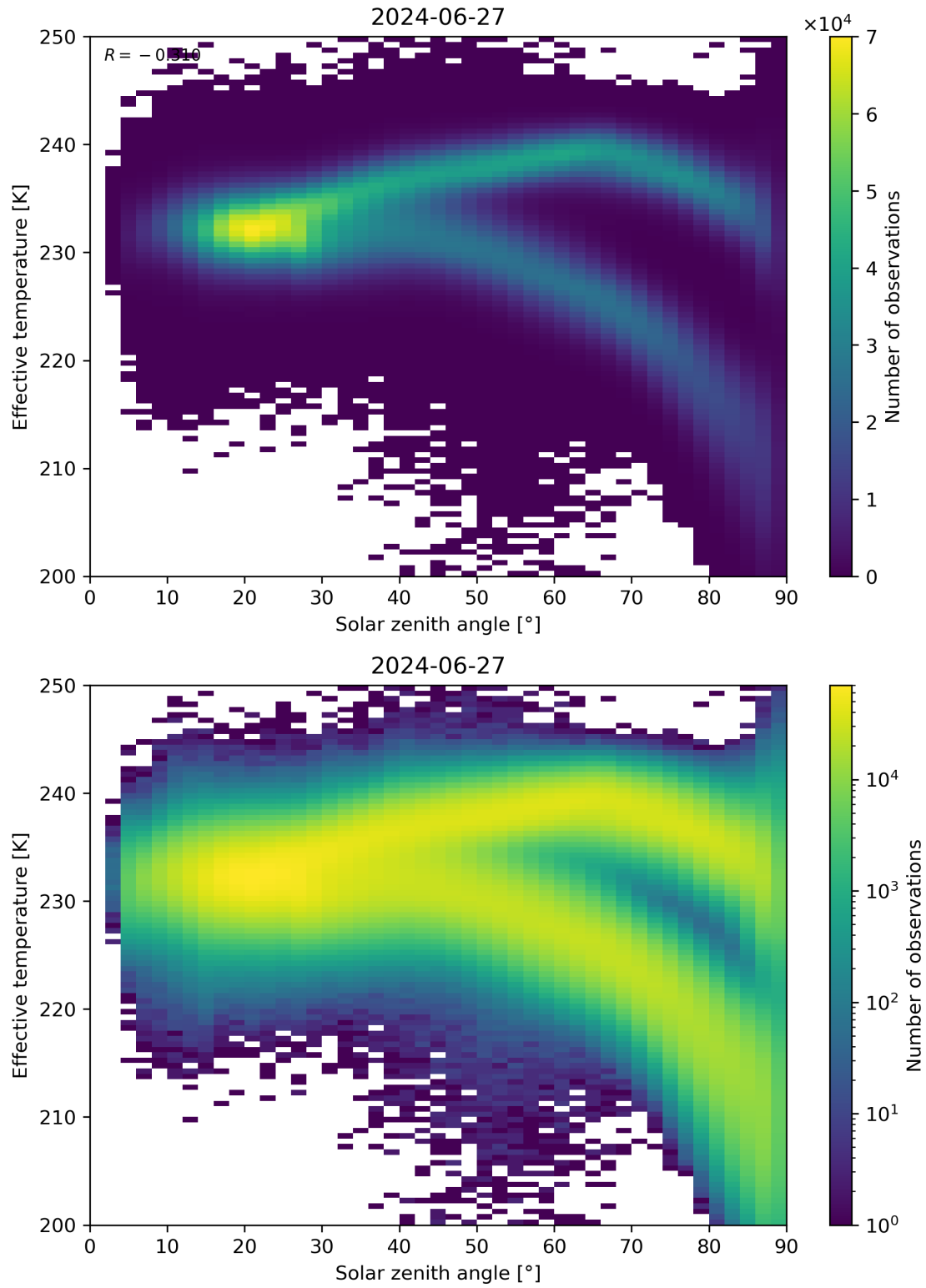
Figure 45: Scatter density plot of “Solar zenith angle” against “Effective temperature” for 2024-06-26 to 2024-06-28.
