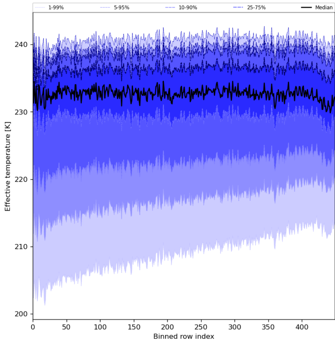
Figure 31: Along track statistics of “Effective temperature” for 2024-06-26 to 2024-06-28
