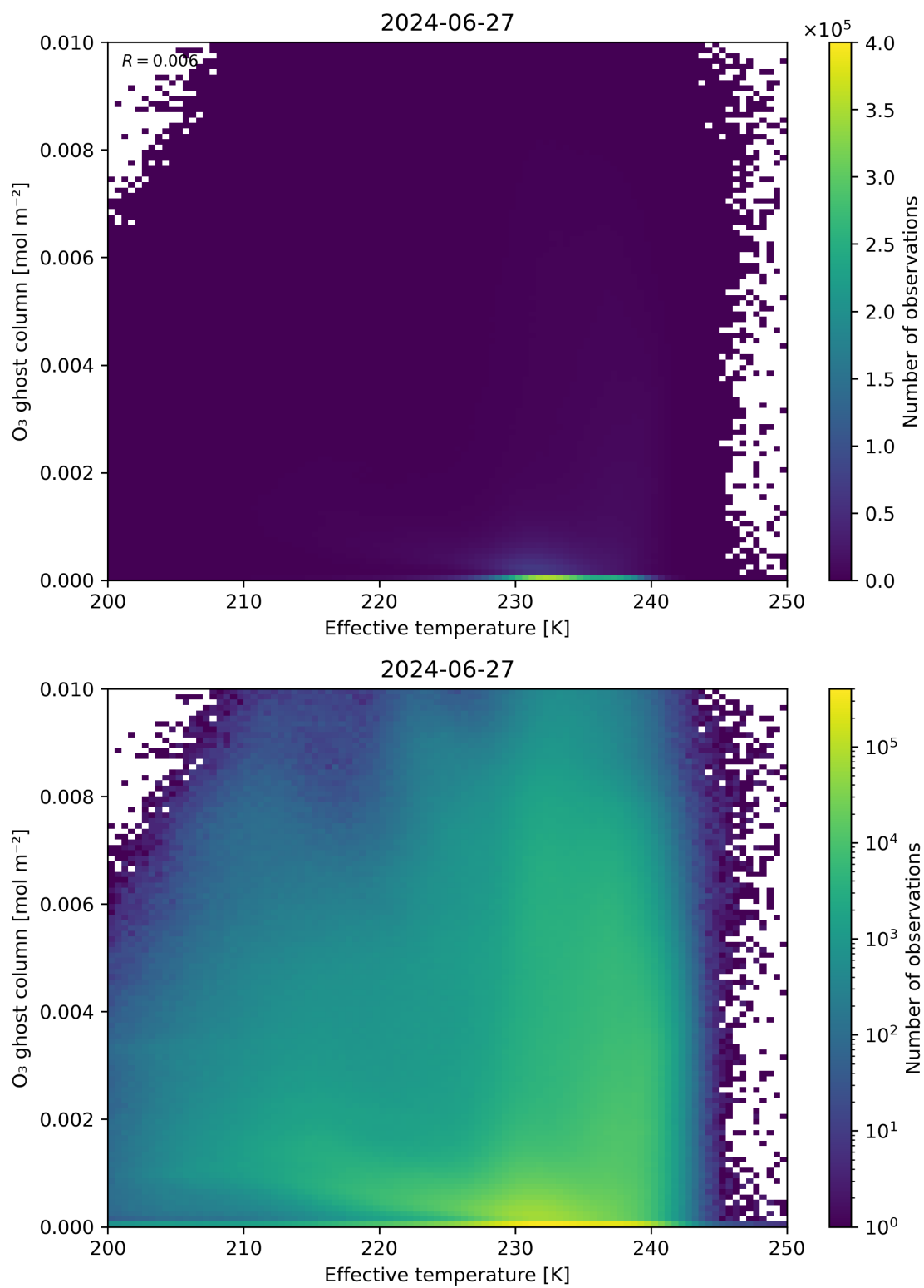
Figure 38: Scatter density plot of “Effective temperature” against “O 3 ghost column” for 2024-06-26 to 2024-06-28.
