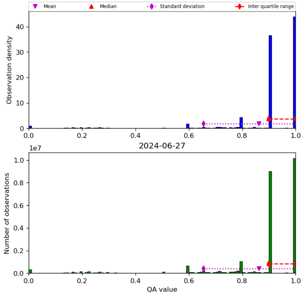
Figure 20: Histogram of “QA value” for 2024-06-26 to 2024-06-28
