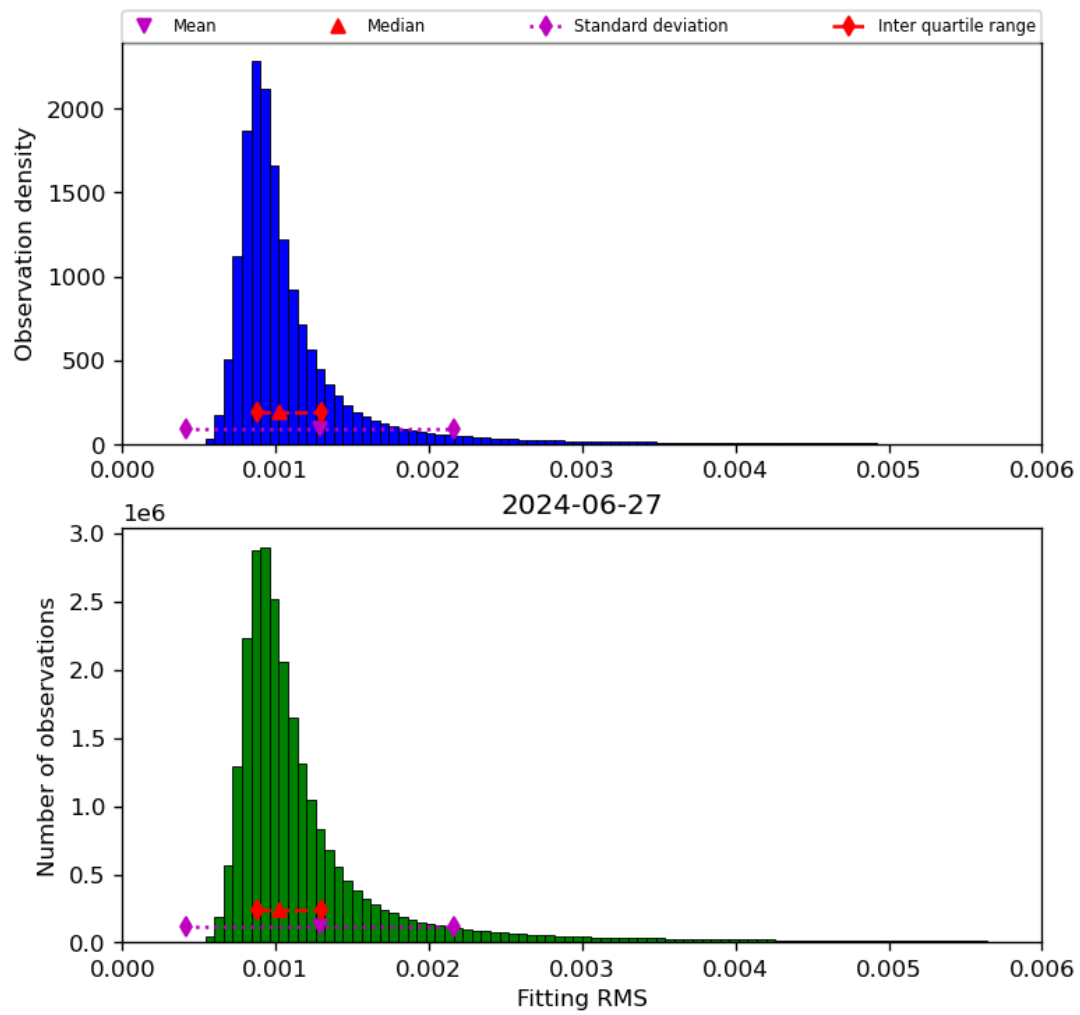
Figure 23: Histogram of “Fitting RMS” for 2024-06-26 to 2024-06-28
