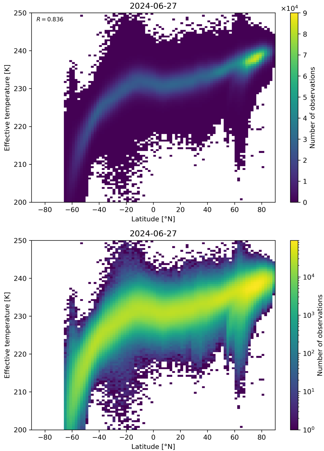
Figure 34: Scatter density plot of “Latitude” against “Effective temperature” for 2024-06-26 to 2024-06-28.
