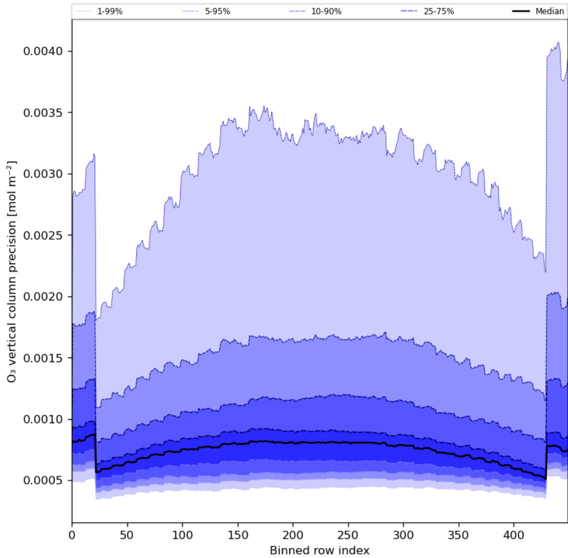
Figure 29: Along track statistics of “O 3 vertical column precision” for 2024-06-26 to 2024-06-28
