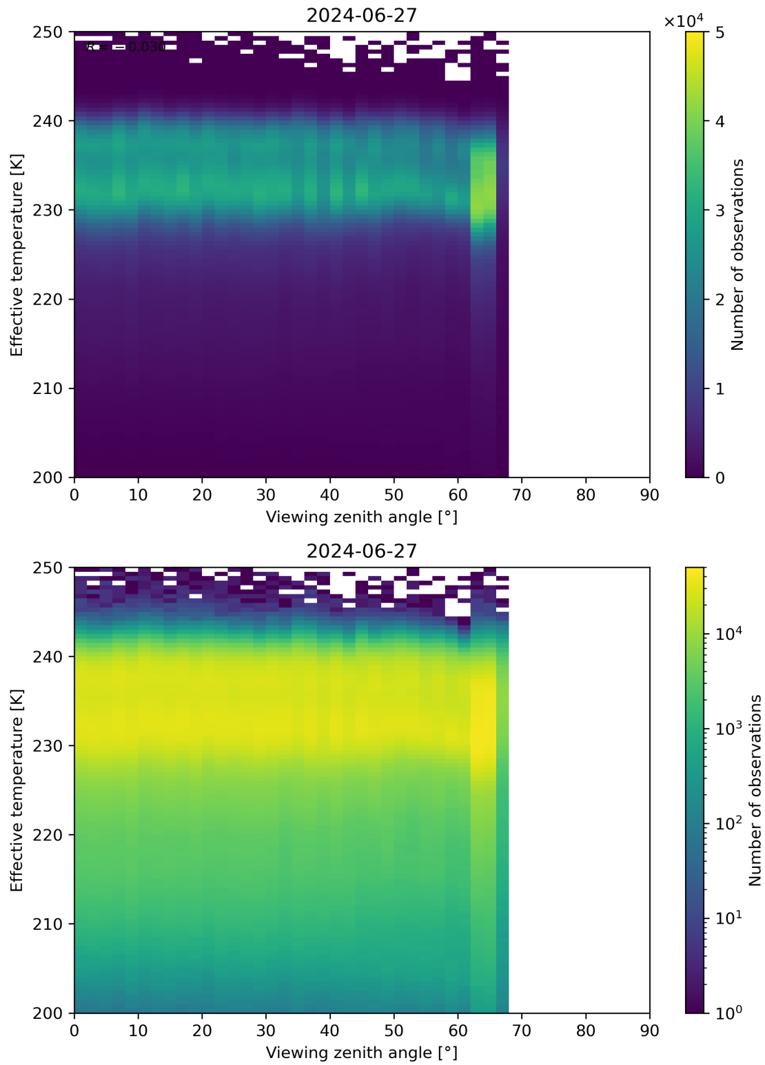
Figure 50: Scatter density plot of “Viewing zenith angle” against “Effective temperature” for 2024-06-26 to 2024-06-28.
