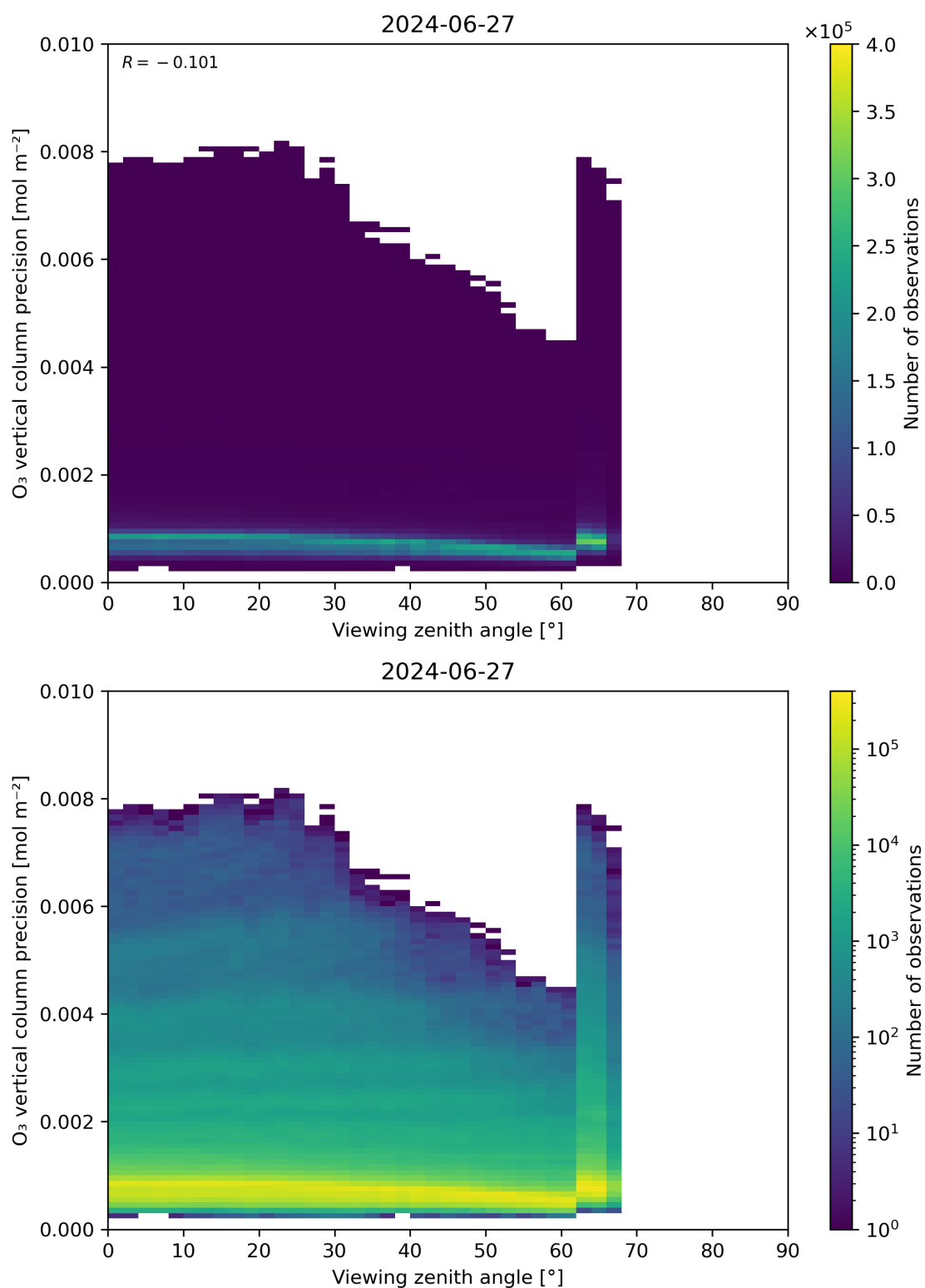
Figure 53: Scatter density plot of “Viewing zenith angle” against “O 3 vertical column precision” for 2024-06-26 to 2024-06-28.
