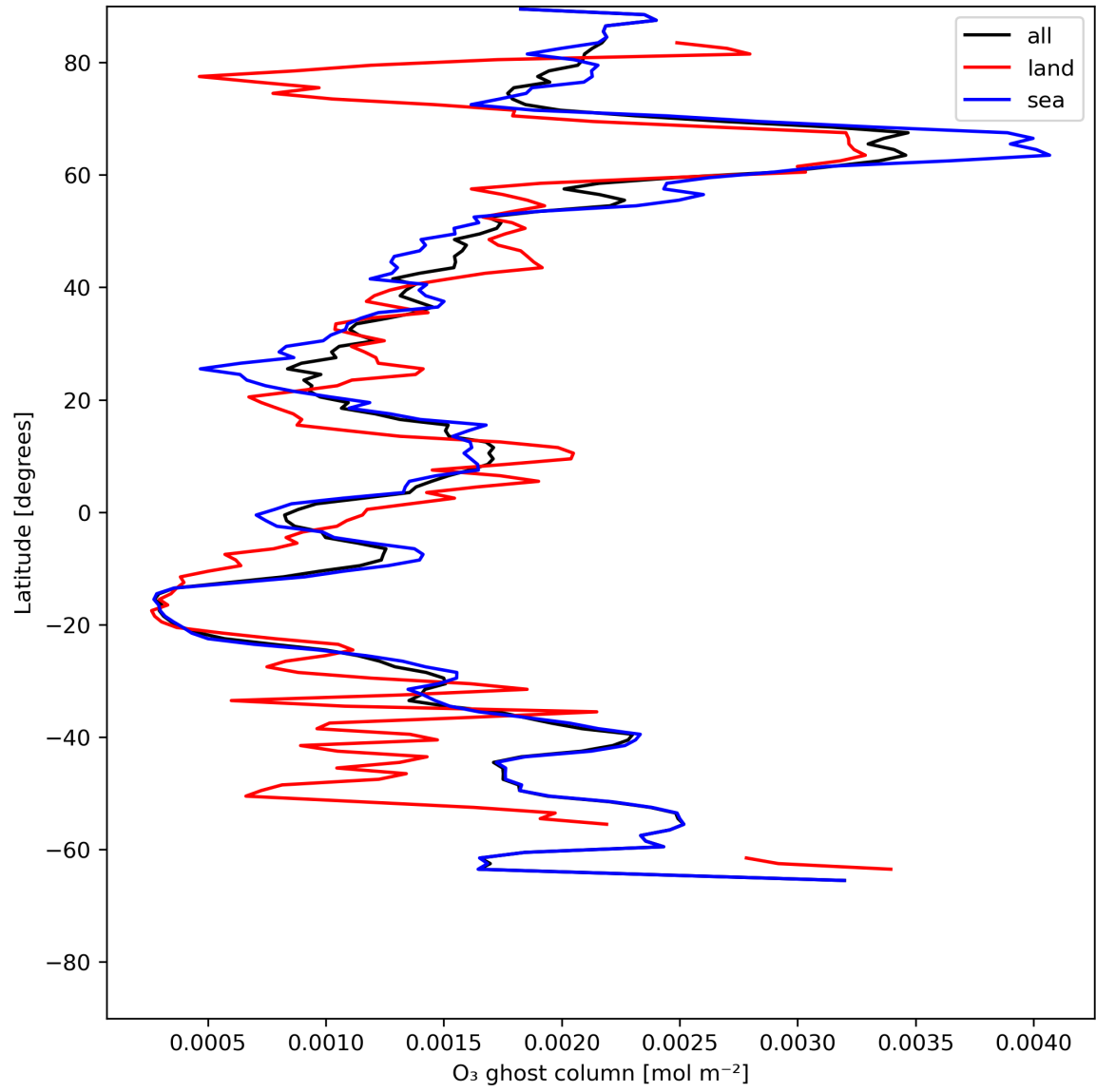
Figure 18: Zonal average of “O 3 ghost column” for 2024-06-26 to 2024-06-28.
