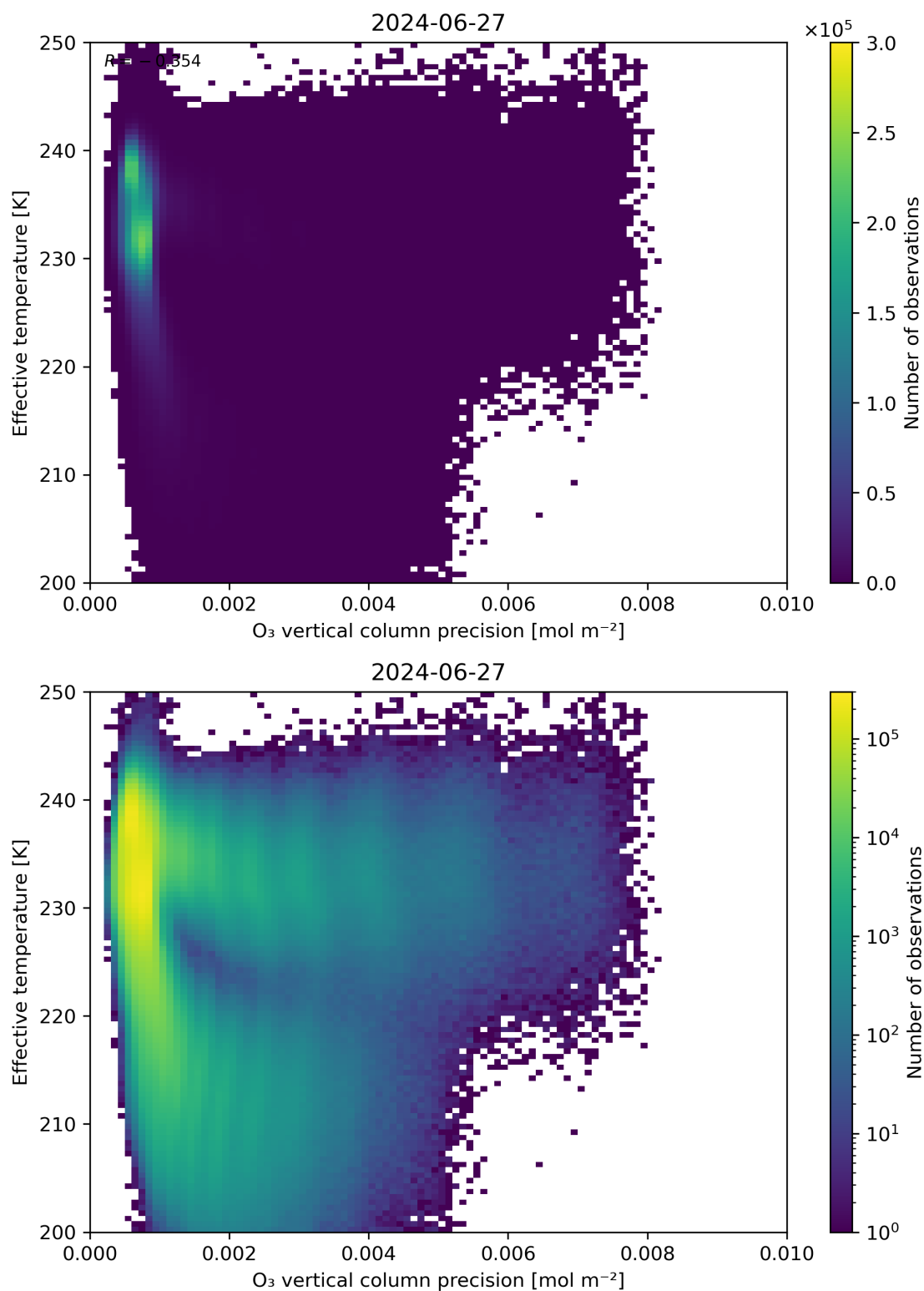
Figure 42: Scatter density plot of “O 3 vertical column precision” against “Effective temperature” for 2024-06-26 to 2024-06-28.
