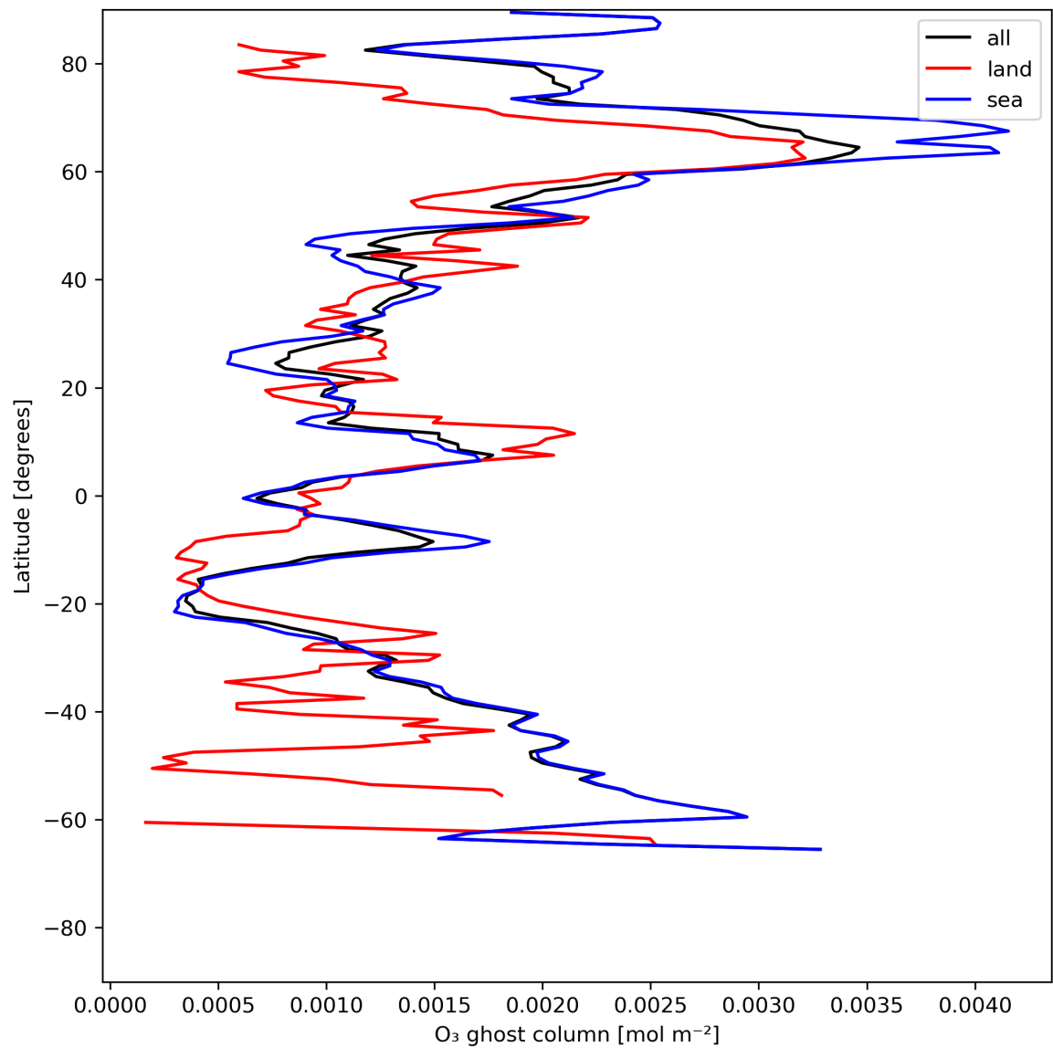
Figure 18: Zonal average of "O 3 ghost column" for 2024-06-27 to 2024-06-29.
