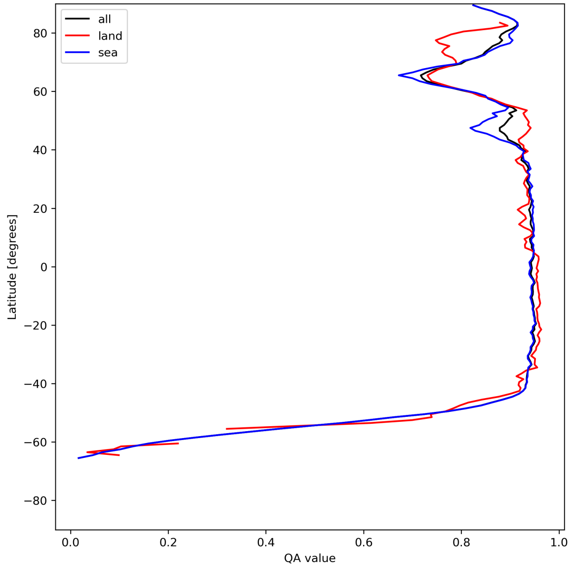
Figure 13: Zonal average of “QA value” for 2024-06-27 to 2024-06-29.
