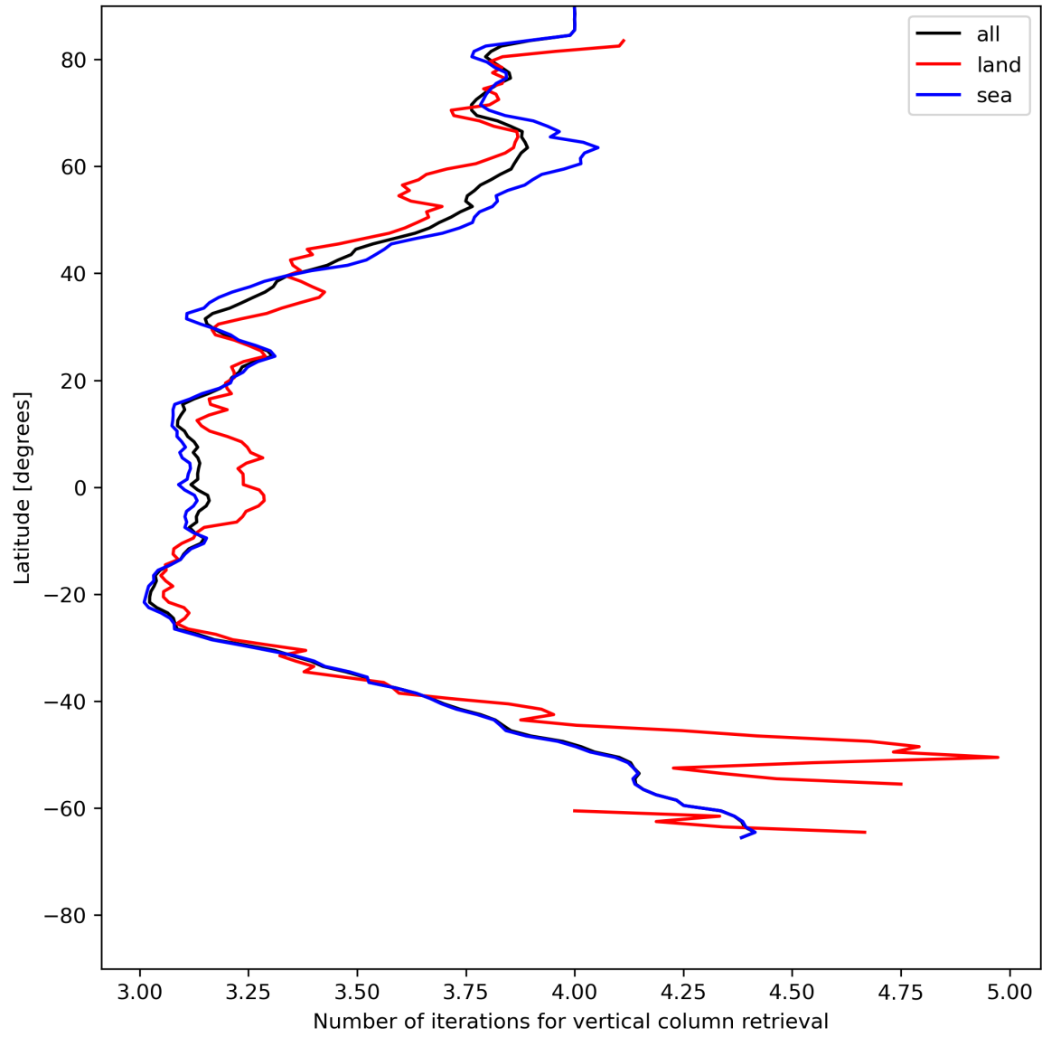
Figure 19: Zonal average of “Number of iterations for vertical column retrieval” for 2024-06-27 to 2024-06-29.
