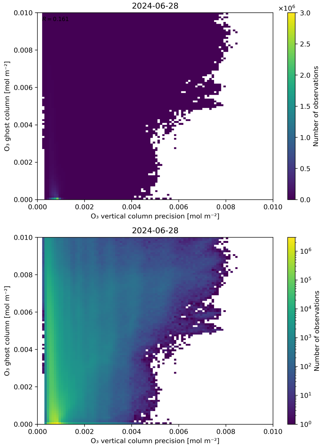
Figure 43: Scatter density plot of “ \text{O}_3 vertical column precision” against “ \text{O}_3 ghost column” for 2024-06-27 to 2024-06-29.
