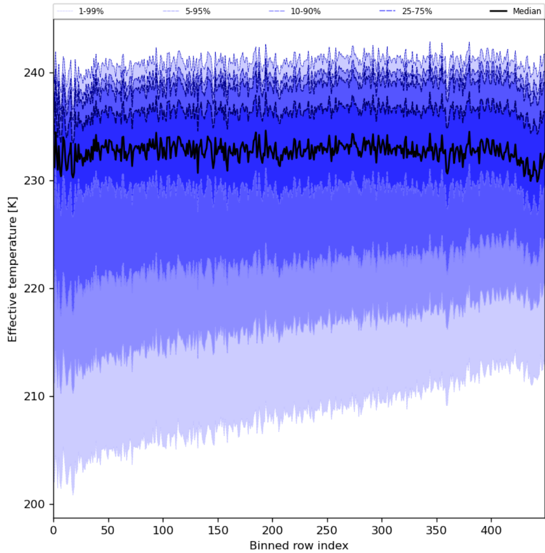
Figure 31: Along track statistics of “Effective temperature” for 2024-06-27 to 2024-06-29
