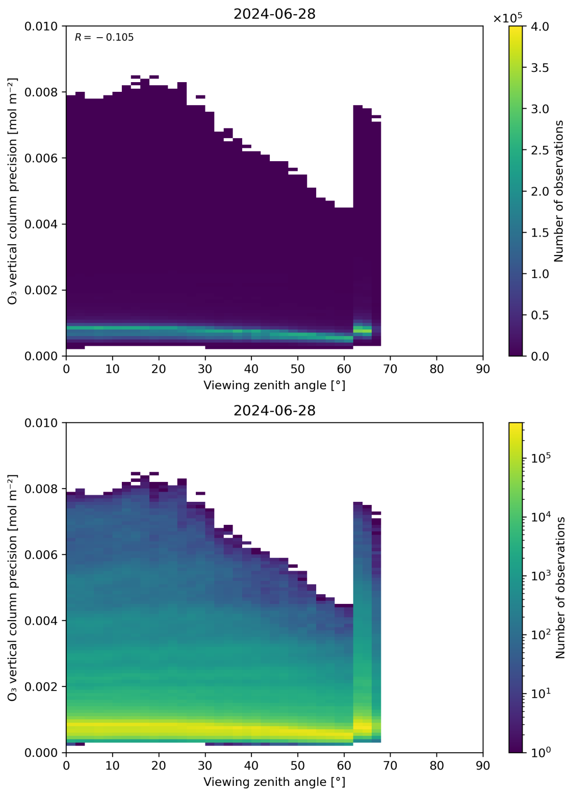
Figure 53: Scatter density plot of “Viewing zenith angle” against “O 3 vertical column precision” for 2024-06-27 to 2024-06-29.
