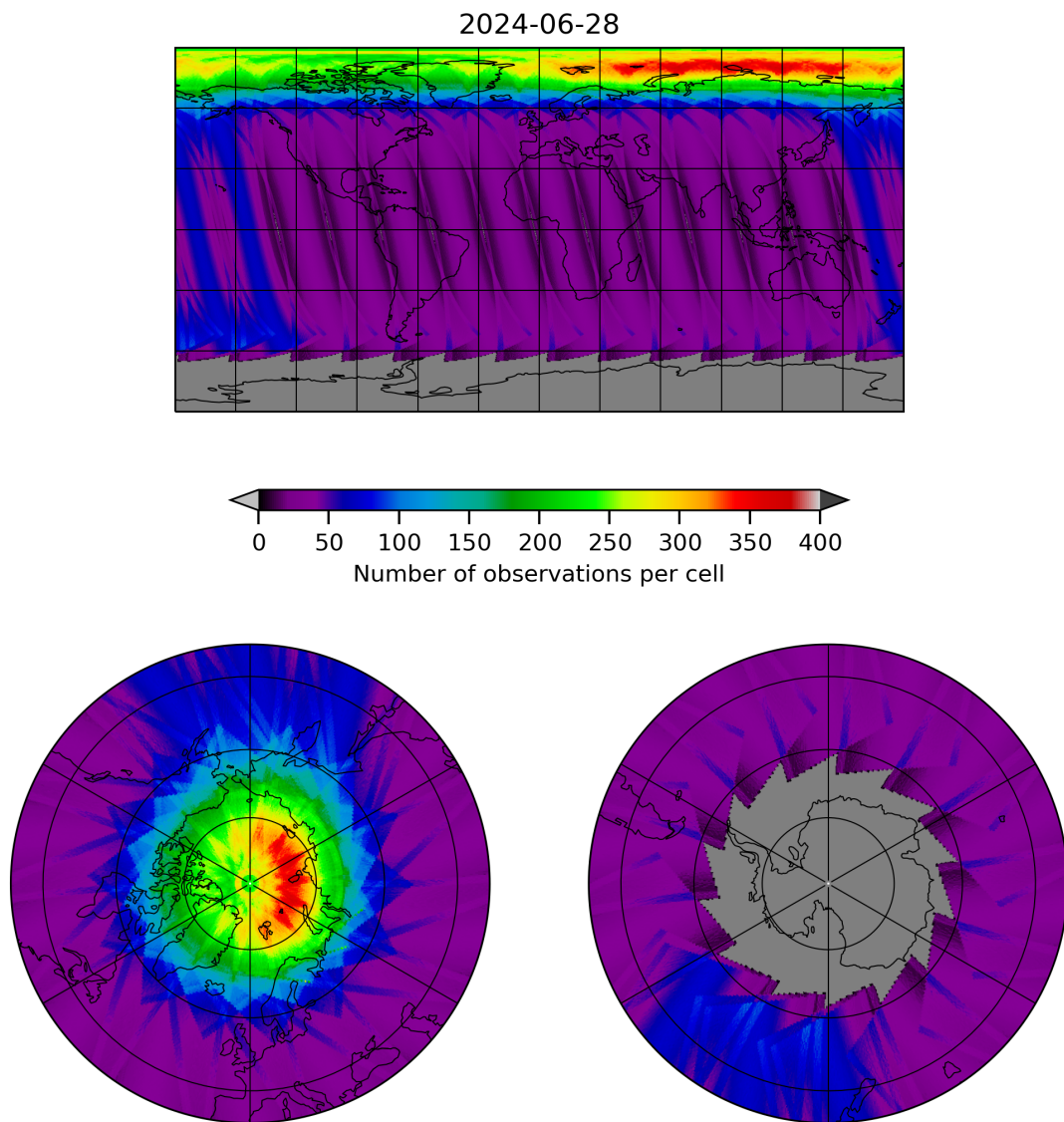
Figure 12: Map of the number of observations for 2024-06-27 to 2024-06-29
