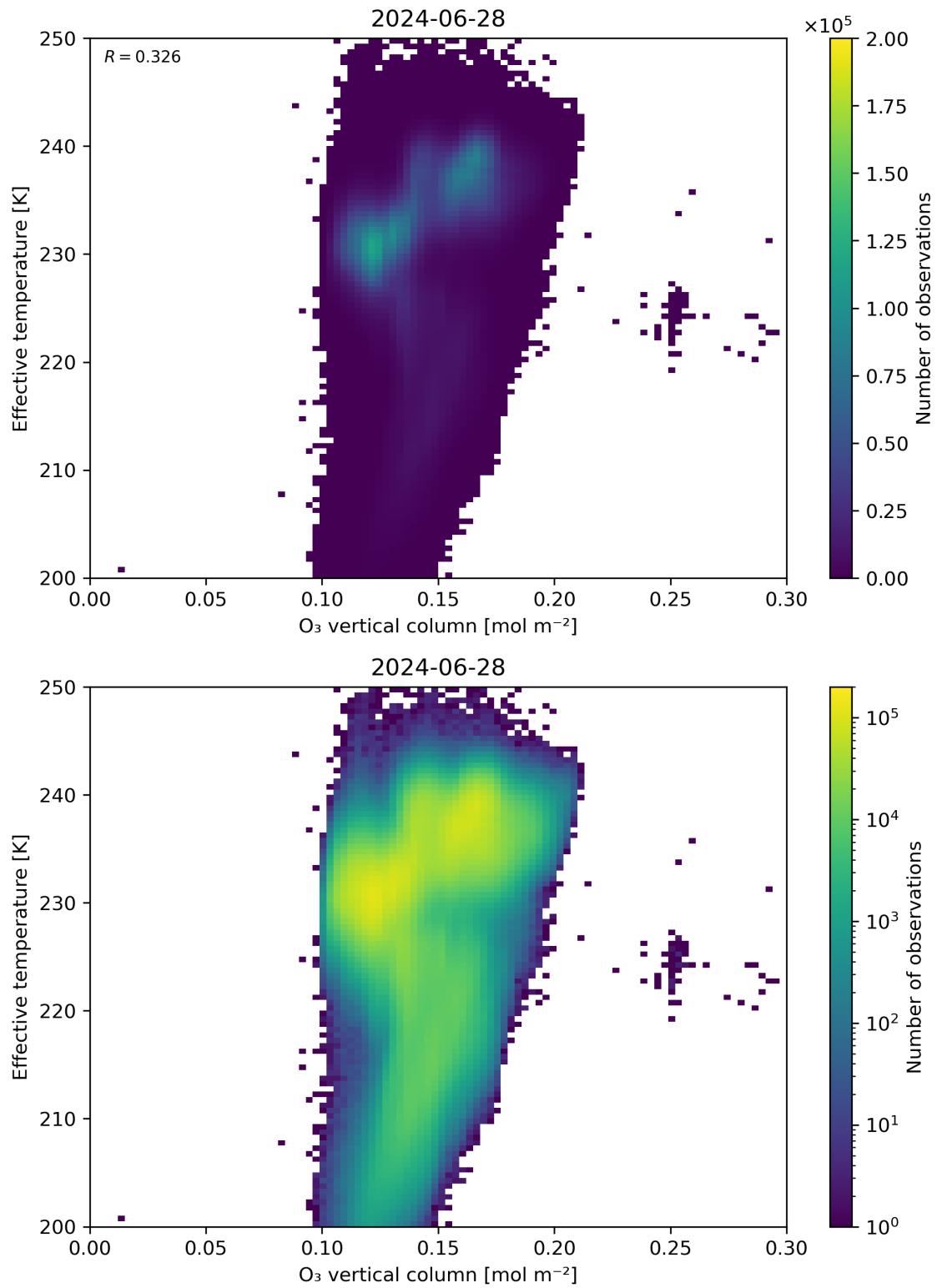
Figure 39: Scatter density plot of “O 3 vertical column” against “Effective temperature” for 2024-06-27 to 2024-06-29.
