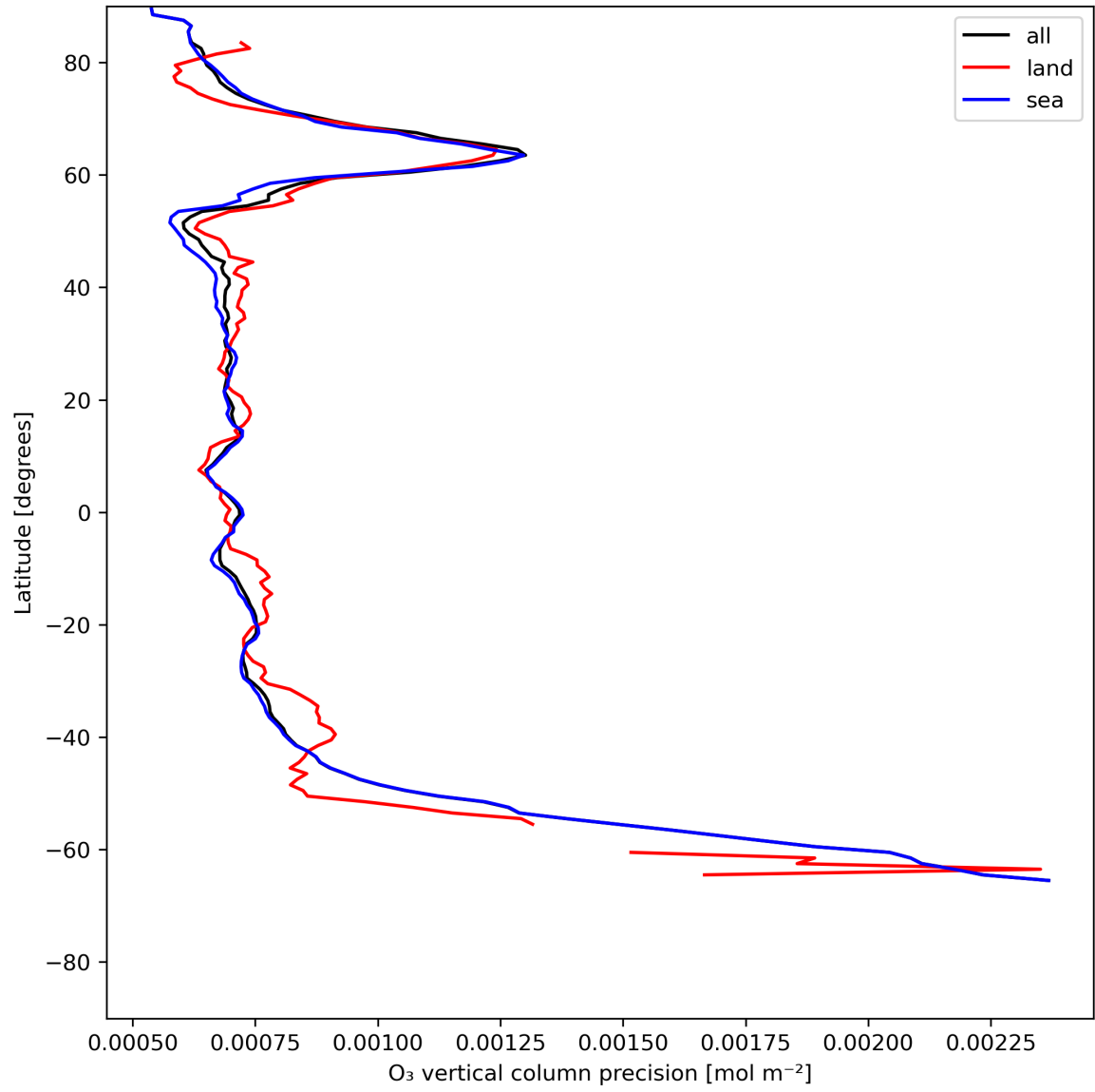
Figure 15: Zonal average of “O 3 vertical column precision” for 2024-06-27 to 2024-06-29.
