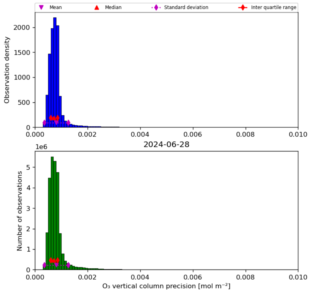
Figure 22: Histogram of “O 3 vertical column precision” for 2024-06-27 to 2024-06-29
