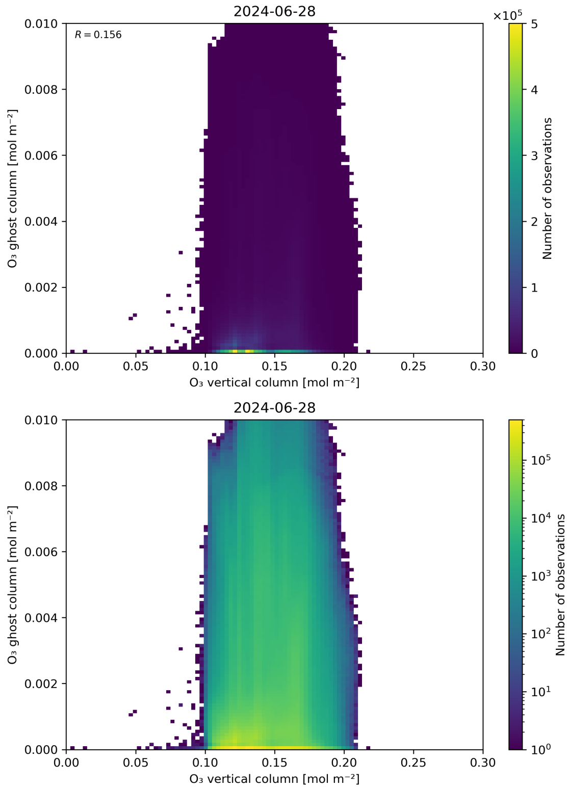
Figure 40: Scatter density plot of “O 3 vertical column” against “O 3 ghost column” for 2024-06-27 to 2024-06-29.
