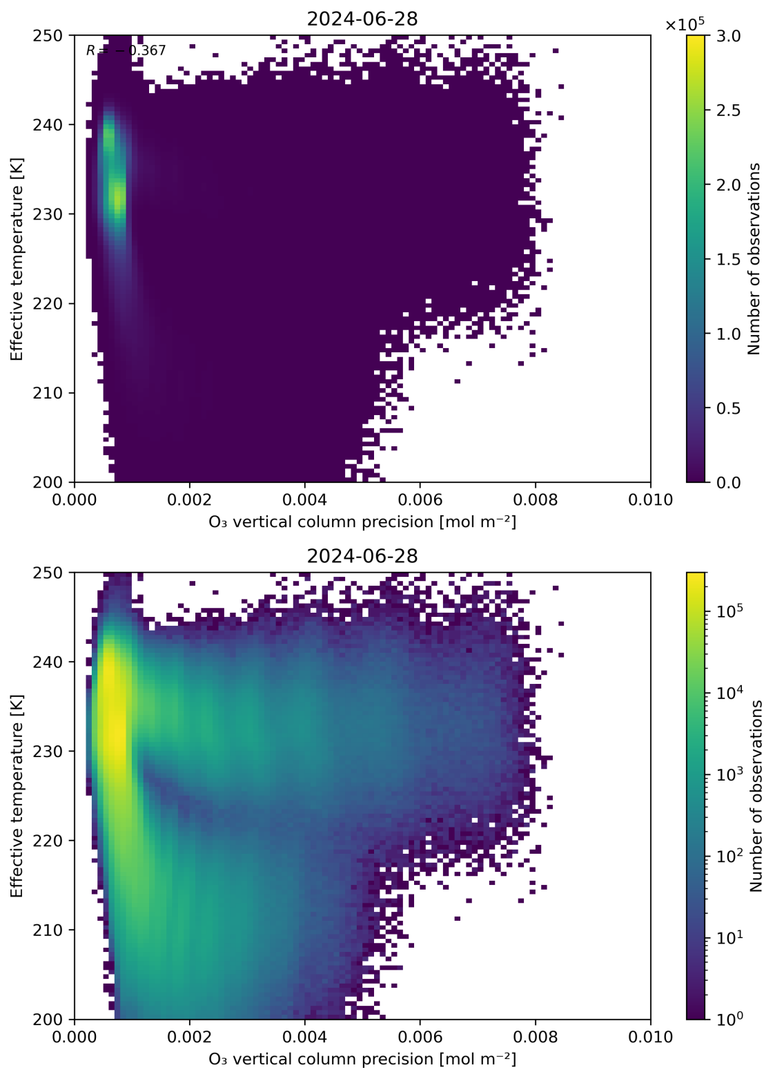
Figure 42: Scatter density plot of “O 3 vertical column precision” against “Effective temperature” for 2024-06-27 to 2024-06-29.
