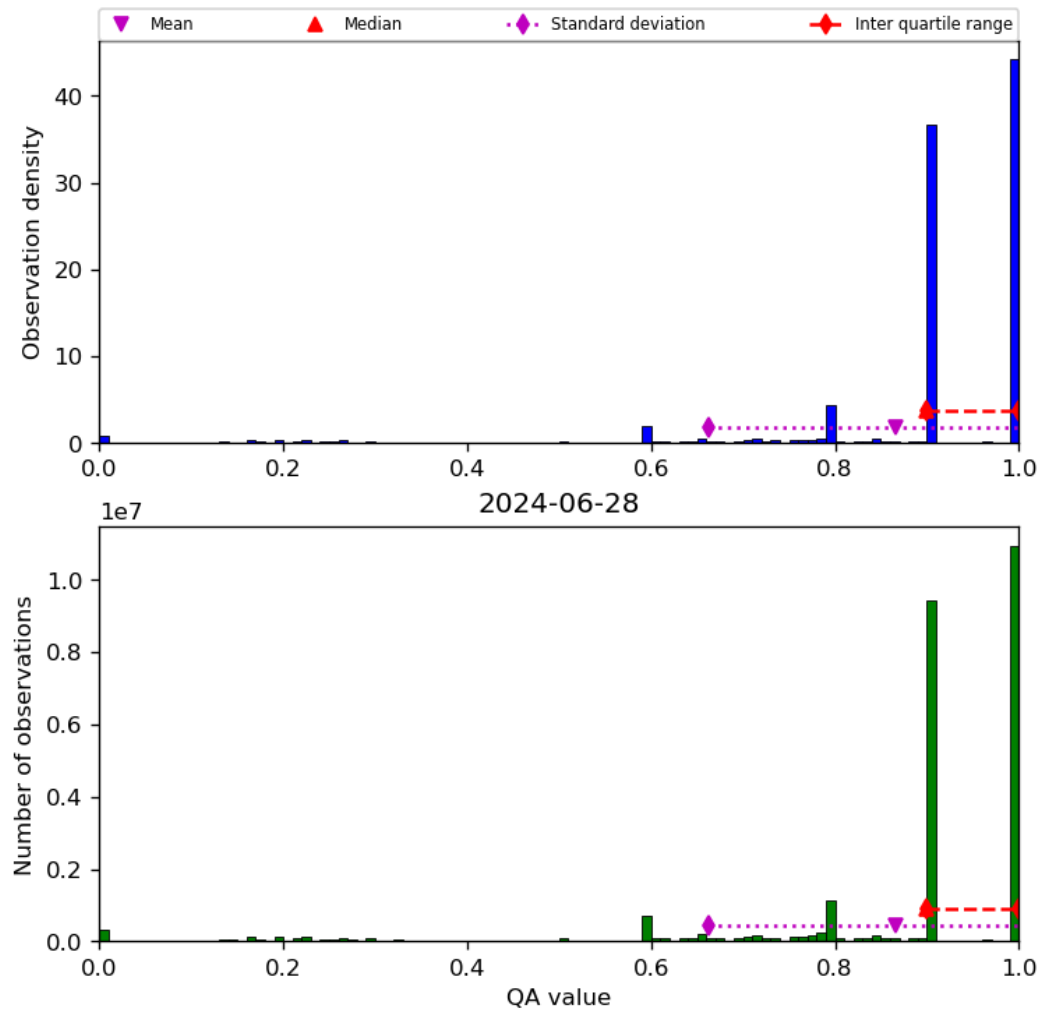
Figure 20: Histogram of “QA value” for 2024-06-27 to 2024-06-29
