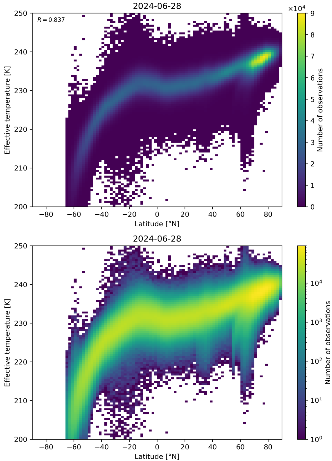
Figure 34: Scatter density plot of “Latitude” against “Effective temperature” for 2024-06-27 to 2024-06-29.
