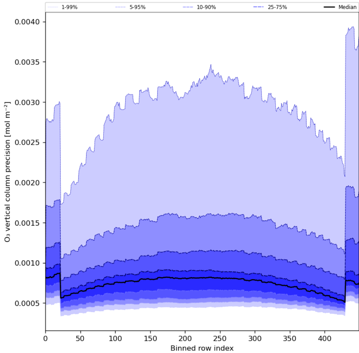
Figure 29: Along track statistics of “O 3 vertical column precision” for 2024-06-27 to 2024-06-29
