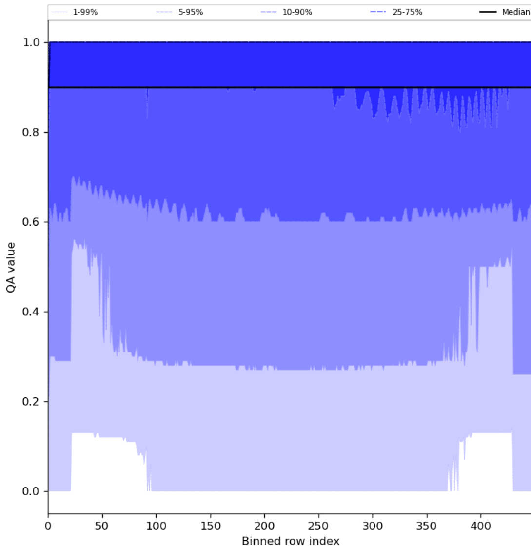
Figure 27: Along track statistics of “QA value” for 2024-06-27 to 2024-06-29
