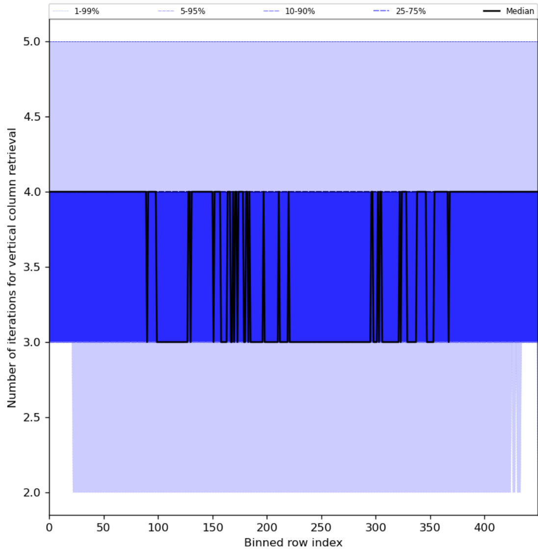
Figure 33: Along track statistics of “Number of iterations for vertical column retrieval” for 2024-06-27 to 2024-06-29
