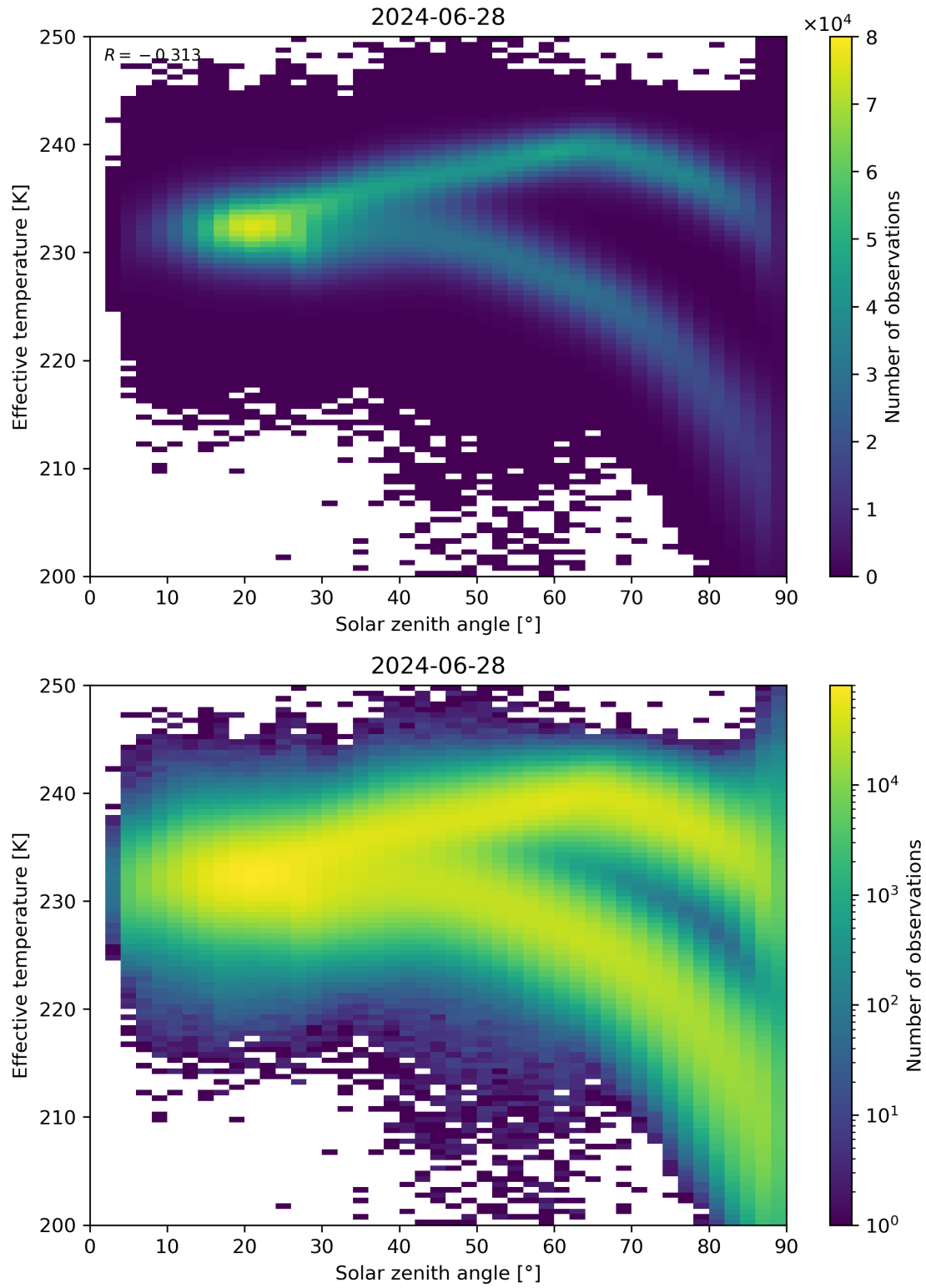
Figure 45: Scatter density plot of “Solar zenith angle” against “Effective temperature” for 2024-06-27 to 2024-06-29.
