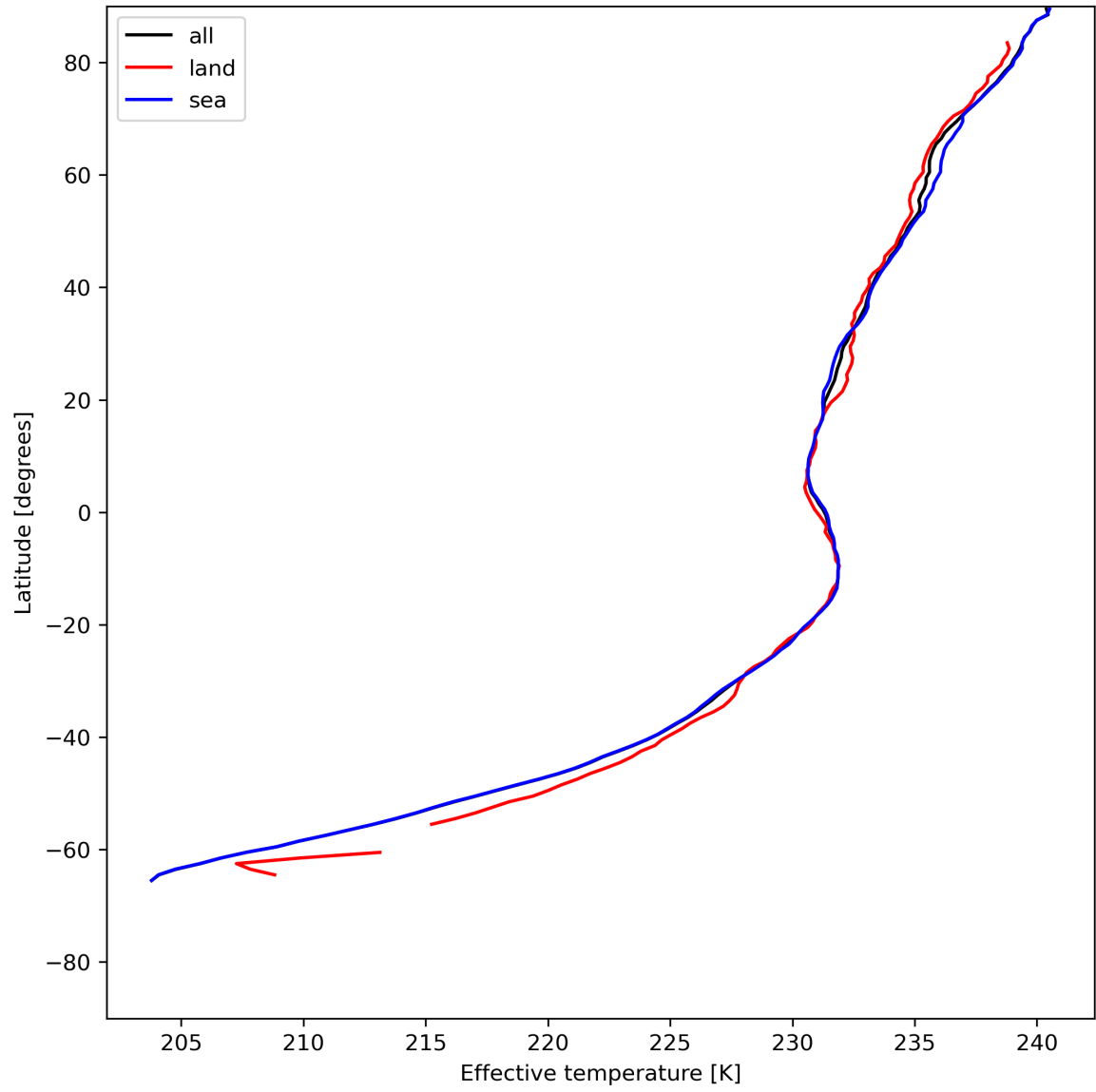
Figure 17: Zonal average of "Effective temperature" for 2024-06-27 to 2024-06-29.
