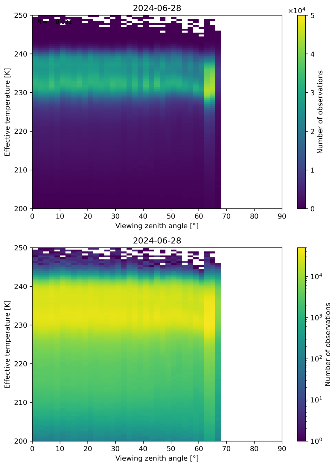
Figure 50: Scatter density plot of “Viewing zenith angle” against “Effective temperature” for 2024-06-27 to 2024-06-29.
