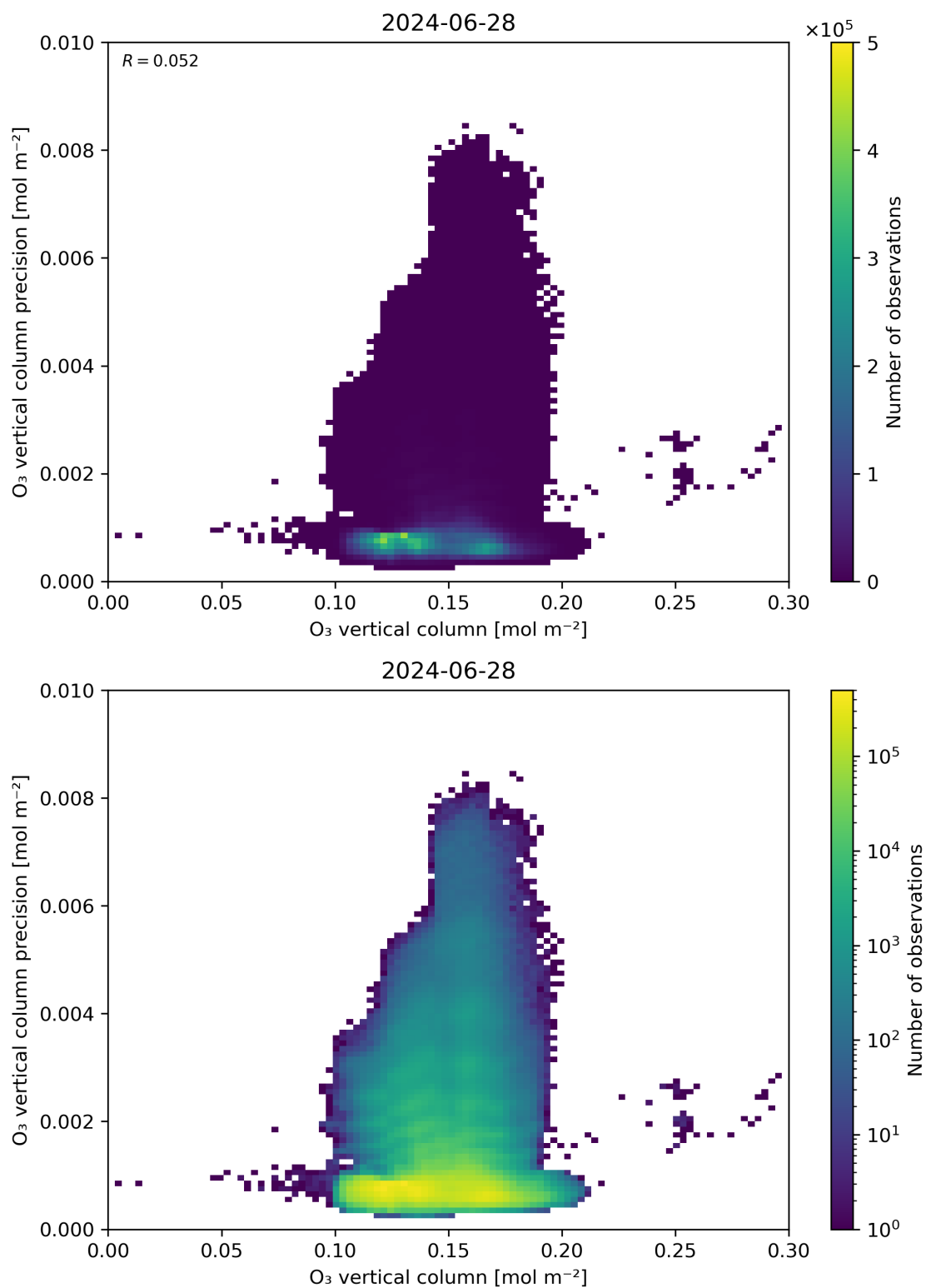
Figure 41: Scatter density plot of “O 3 vertical column” against “O 3 vertical column precision” for 2024-06-27 to 2024-06-29.
