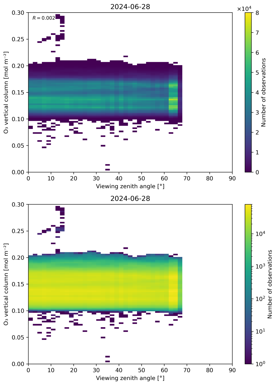
Figure 52: Scatter density plot of “Viewing zenith angle” against “O 3 vertical column” for 2024-06-27 to 2024-06-29.
