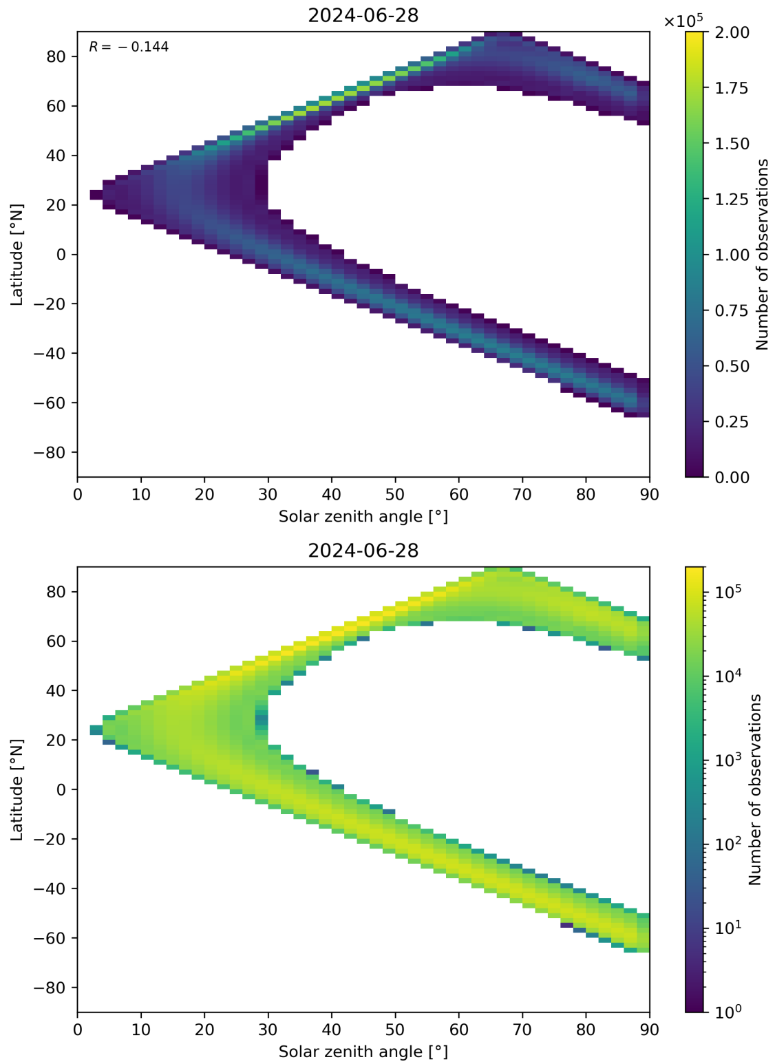
Figure 44: Scatter density plot of “Solar zenith angle” against “Latitude” for 2024-06-27 to 2024-06-29.
