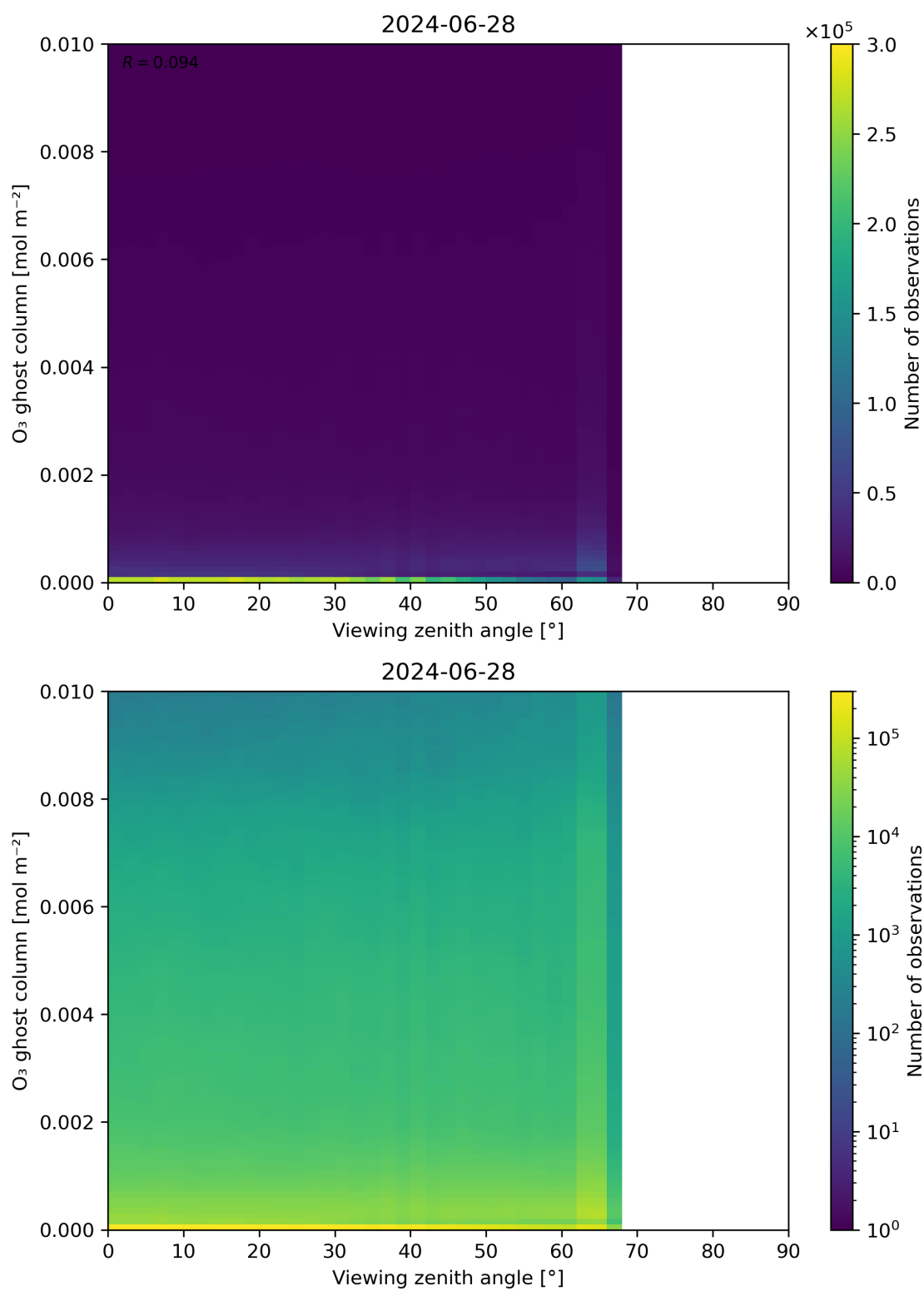
Figure 51: Scatter density plot of “Viewing zenith angle” against “O 3 ghost column” for 2024-06-27 to 2024-06-29.
