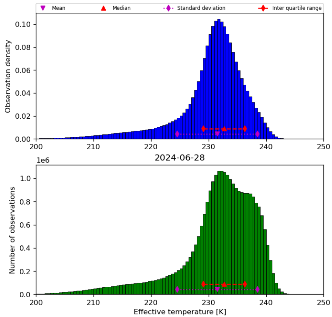
Figure 24: Histogram of “Effective temperature” for 2024-06-27 to 2024-06-29
