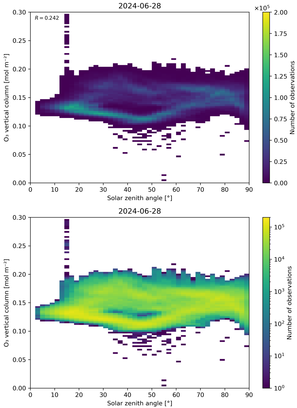
Figure 47: Scatter density plot of “Solar zenith angle” against “O 3 vertical column” for 2024-06-27 to 2024-06-29.
