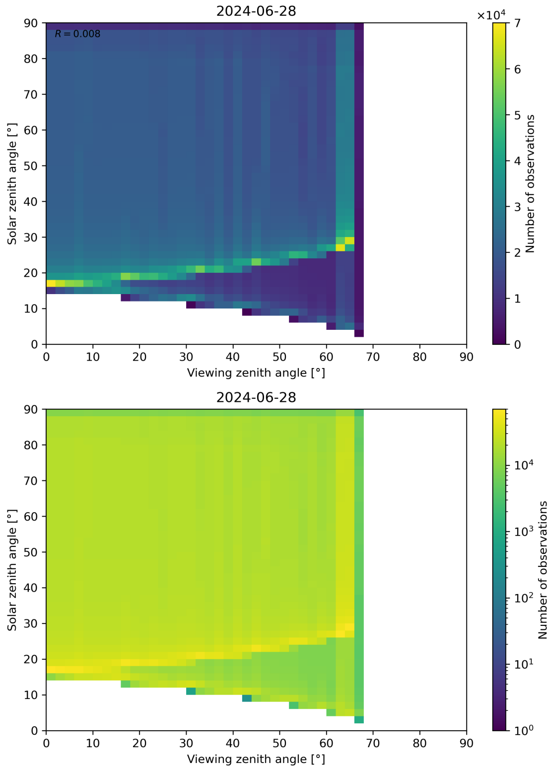
Figure 54: Scatter density plot of “Viewing zenith angle” against “Solar zenith angle” for 2024-06-27 to 2024-06-29.
