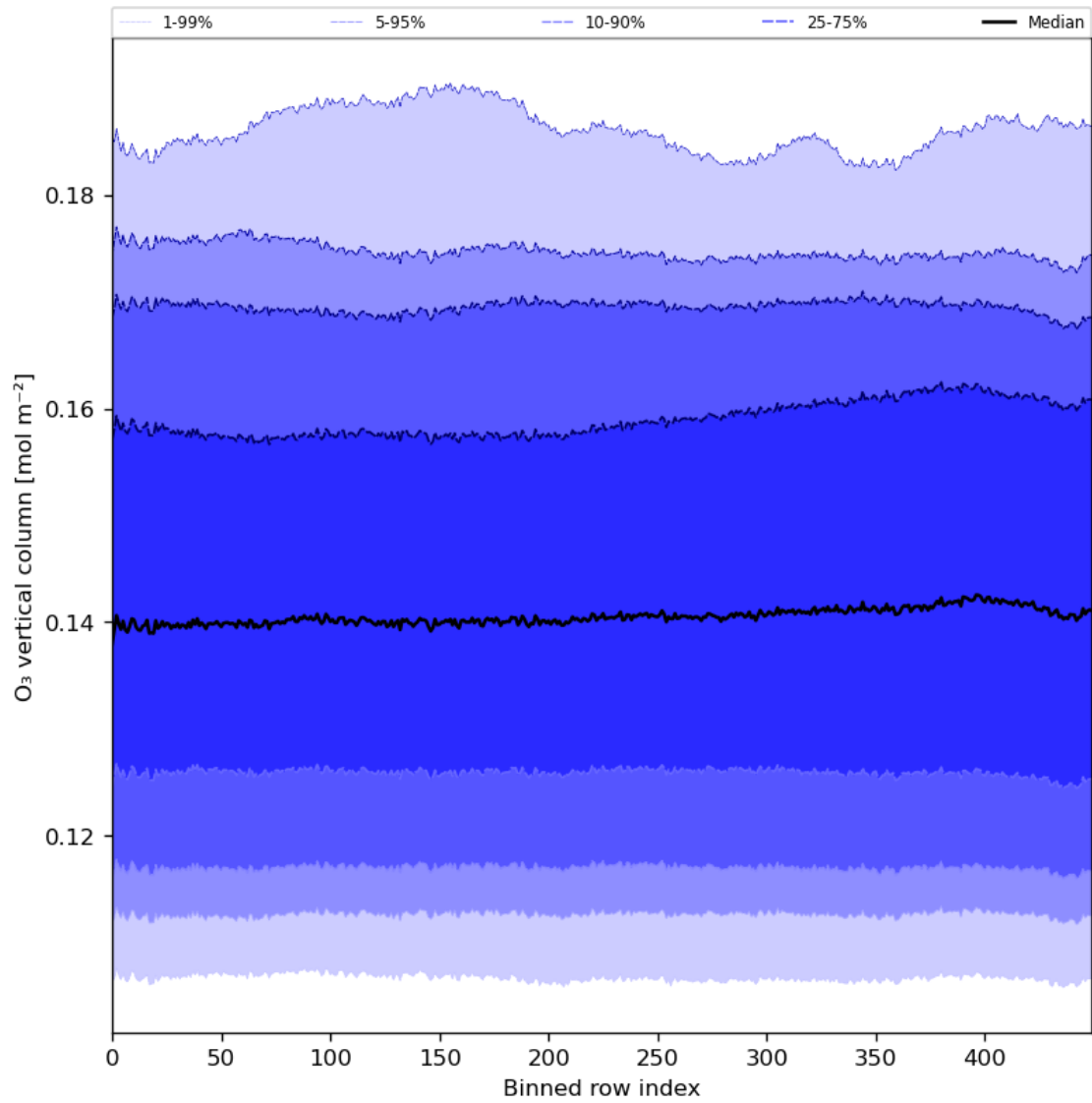
Figure 28: Along track statistics of “O 3 vertical column” for 2024-06-27 to 2024-06-29
