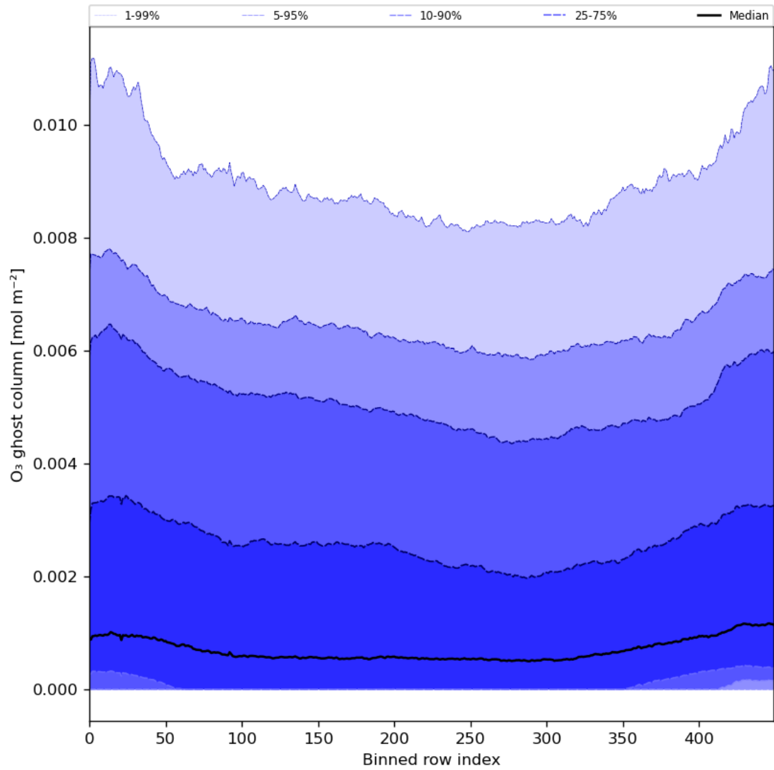
Figure 32: Along track statistics of “O 3 ghost column” for 2024-06-27 to 2024-06-29
