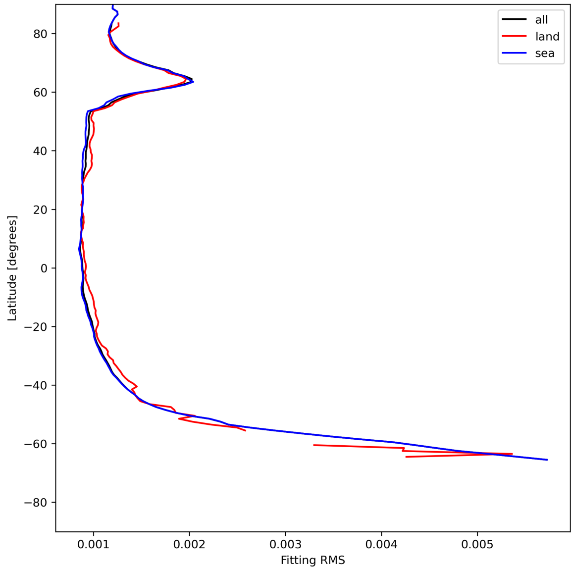
Figure 16: Zonal average of “Fitting RMS” for 2024-06-27 to 2024-06-29.
