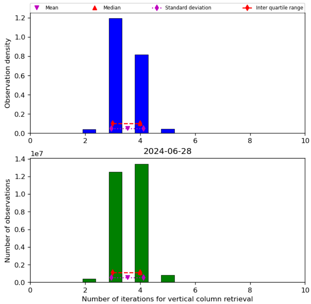
Figure 26: Histogram of “Number of iterations for vertical column retrieval” for 2024-06-27 to 2024-06-29
