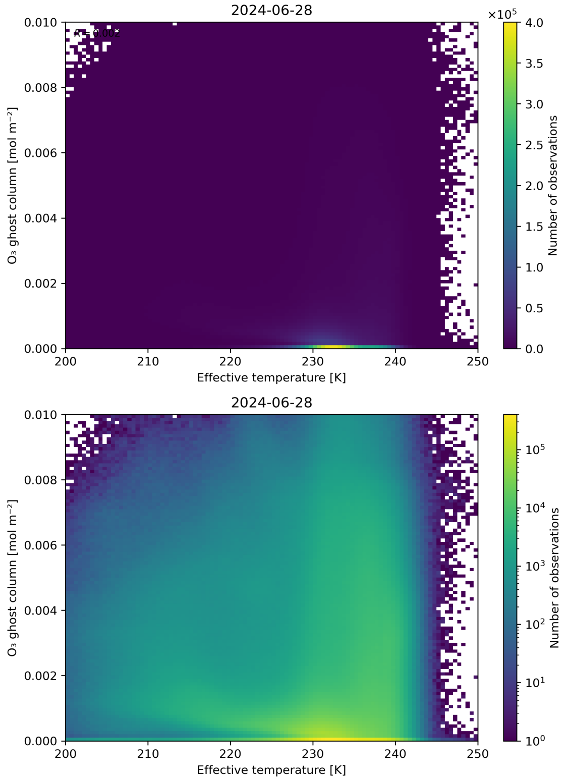
Figure 38: Scatter density plot of “Effective temperature” against “O 3 ghost column” for 2024-06-27 to 2024-06-29.
