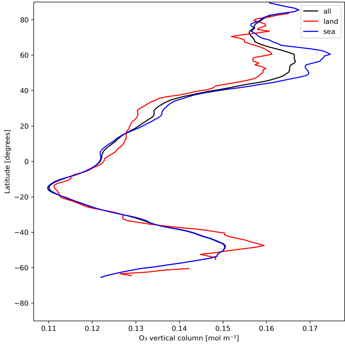
Figure 14: Zonal average of “O 3 vertical column” for 2024-06-27 to 2024-06-29.
