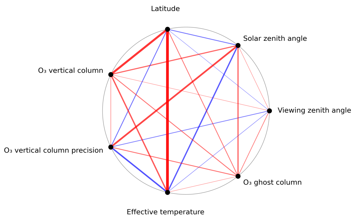
Figure 1: Map of correlation graph for 2024-06-27 to 2024-06-29.
