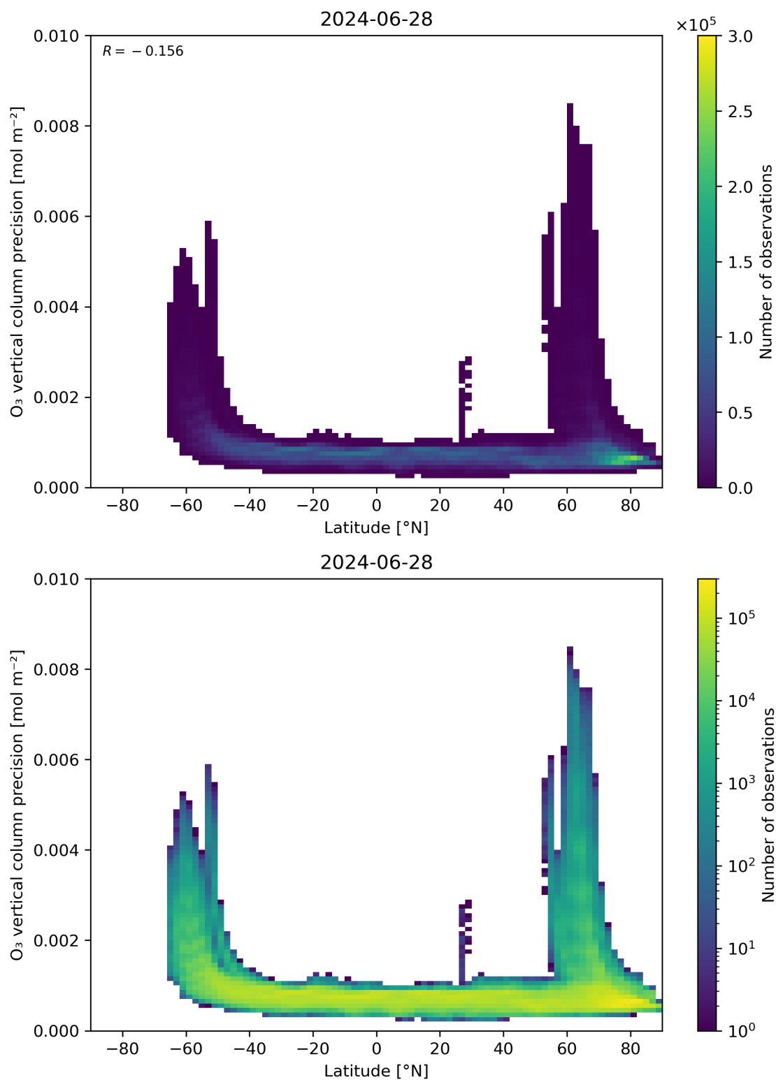
Figure 37: Scatter density plot of “Latitude” against “O 3 vertical column precision” for 2024-06-27 to 2024-06-29.
