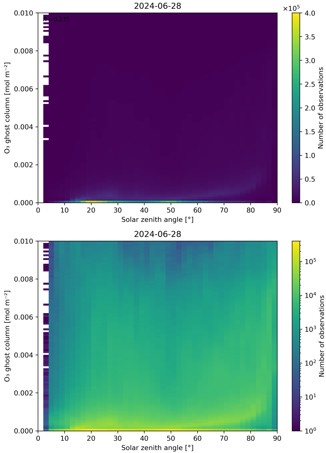
Figure 46: Scatter density plot of “Solar zenith angle” against “O 3 ghost column” for 2024-06-27 to 2024-06-29.
