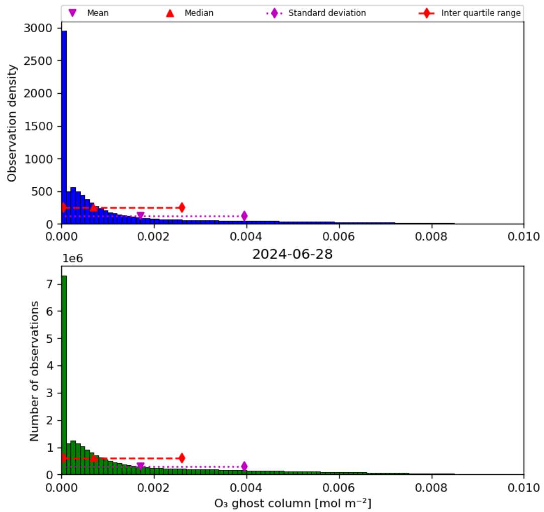
Figure 25: Histogram of “O 3 ghost column” for 2024-06-27 to 2024-06-29
