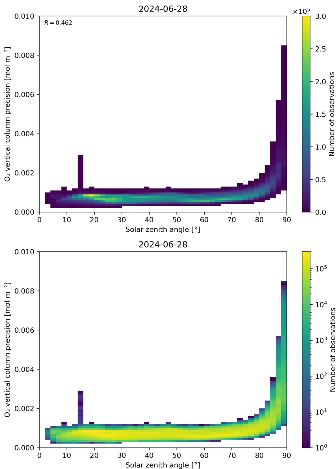
Figure 48: Scatter density plot of “Solar zenith angle” against “O 3 vertical column precision” for 2024-06-27 to 2024-06-29.
