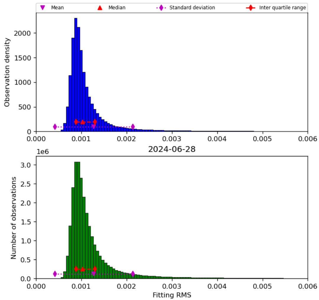
Figure 23: Histogram of “Fitting RMS” for 2024-06-27 to 2024-06-29
