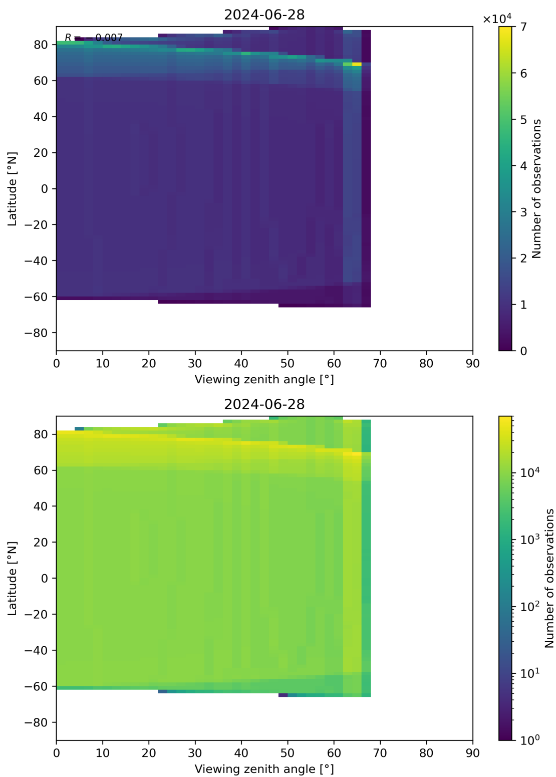
Figure 49: Scatter density plot of “Viewing zenith angle” against “Latitude” for 2024-06-27 to 2024-06-29.
