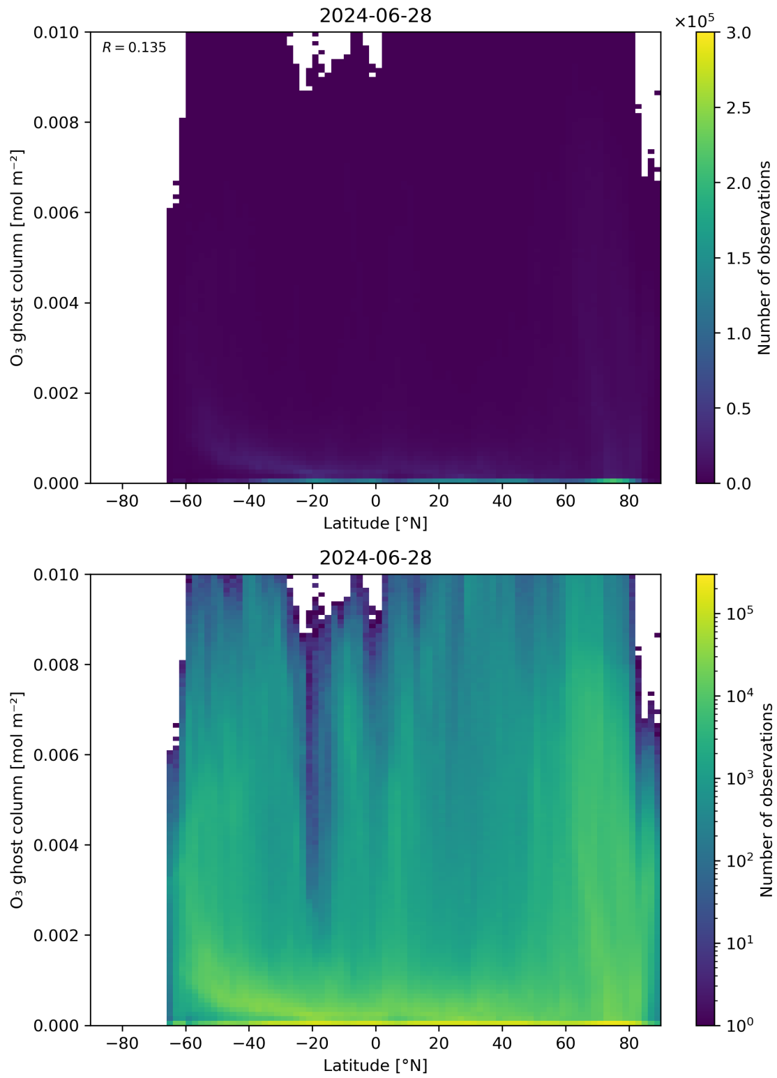
Figure 35: Scatter density plot of “Latitude” against “O 3 ghost column” for 2024-06-27 to 2024-06-29.
