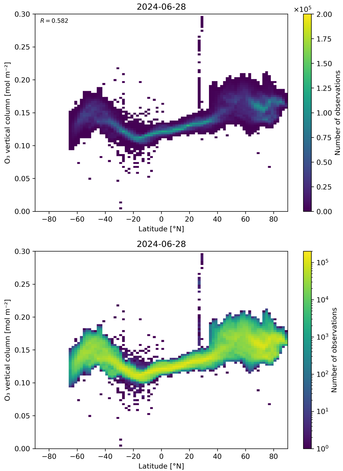
Figure 36: Scatter density plot of “Latitude” against “O 3 vertical column” for 2024-06-27 to 2024-06-29.
