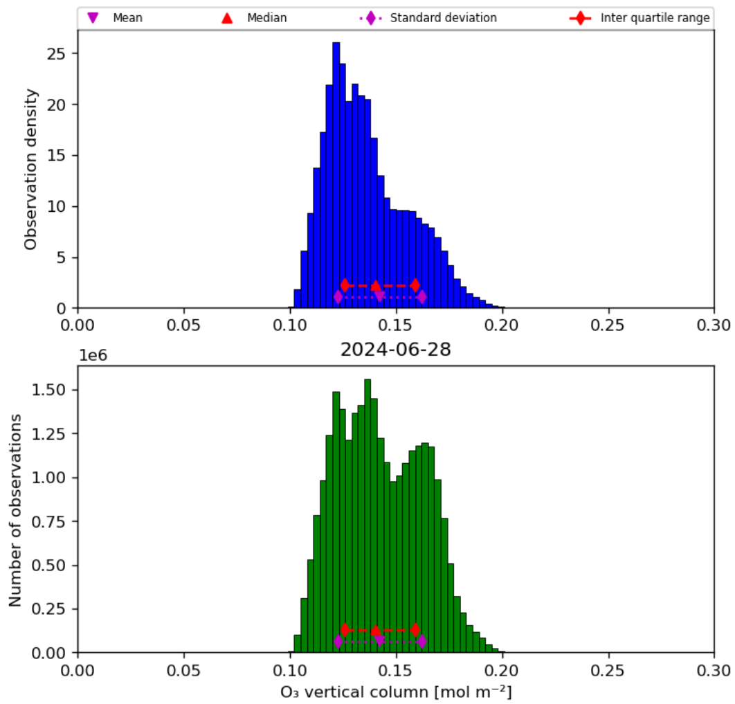
Figure 21: Histogram of “O 3 vertical column” for 2024-06-27 to 2024-06-29
