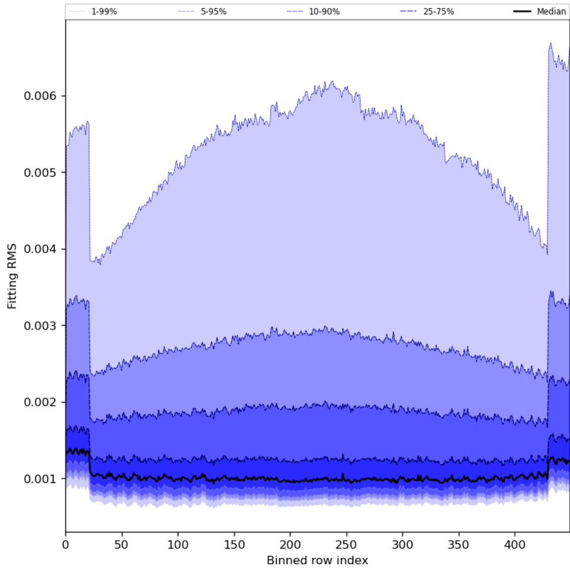
Figure 30: Along track statistics of “Fitting RMS” for 2024-06-27 to 2024-06-29
