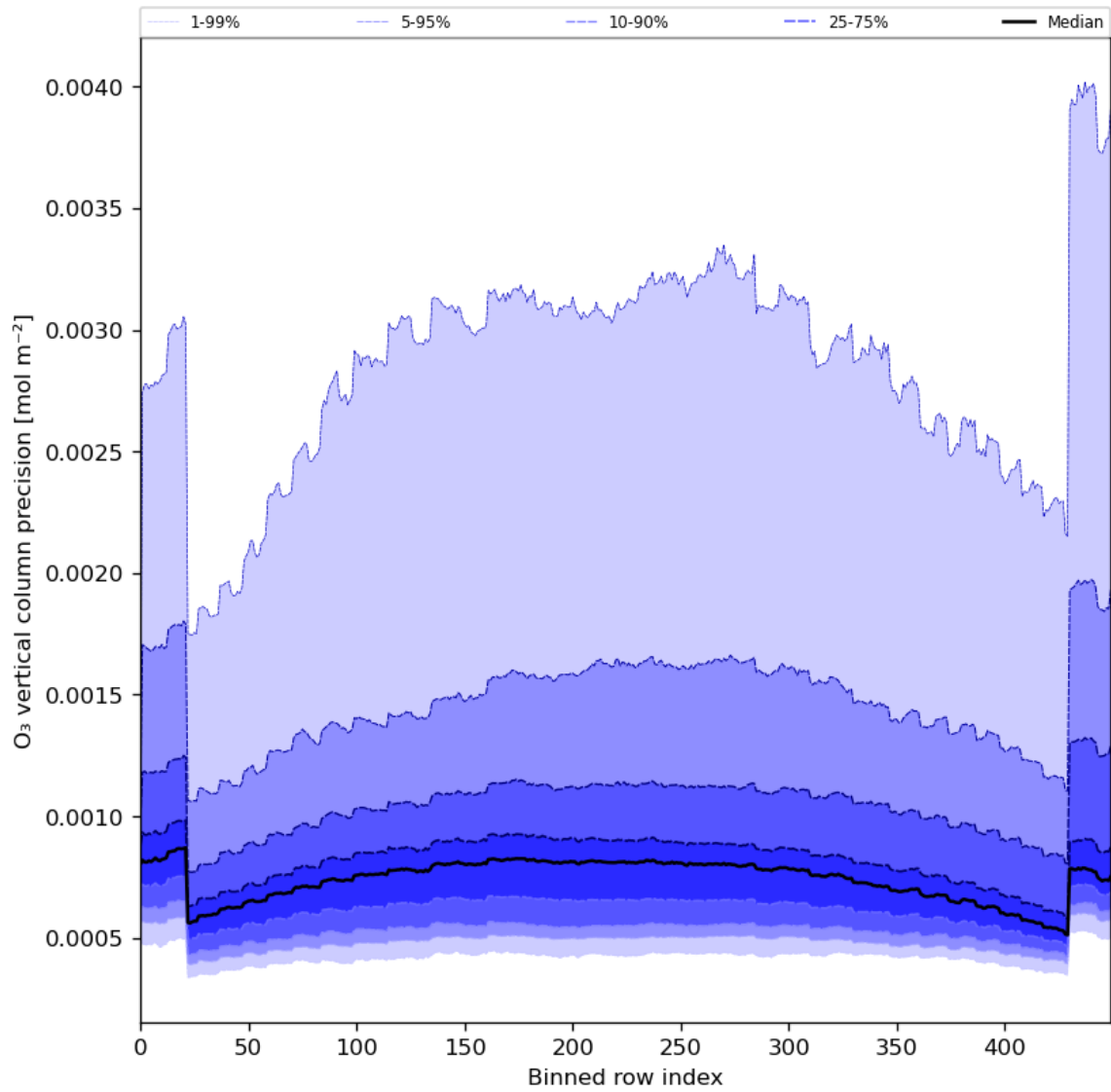
Figure 29: Along track statistics of “O 3 vertical column precision” for 2024-06-29 to 2024-06-30
