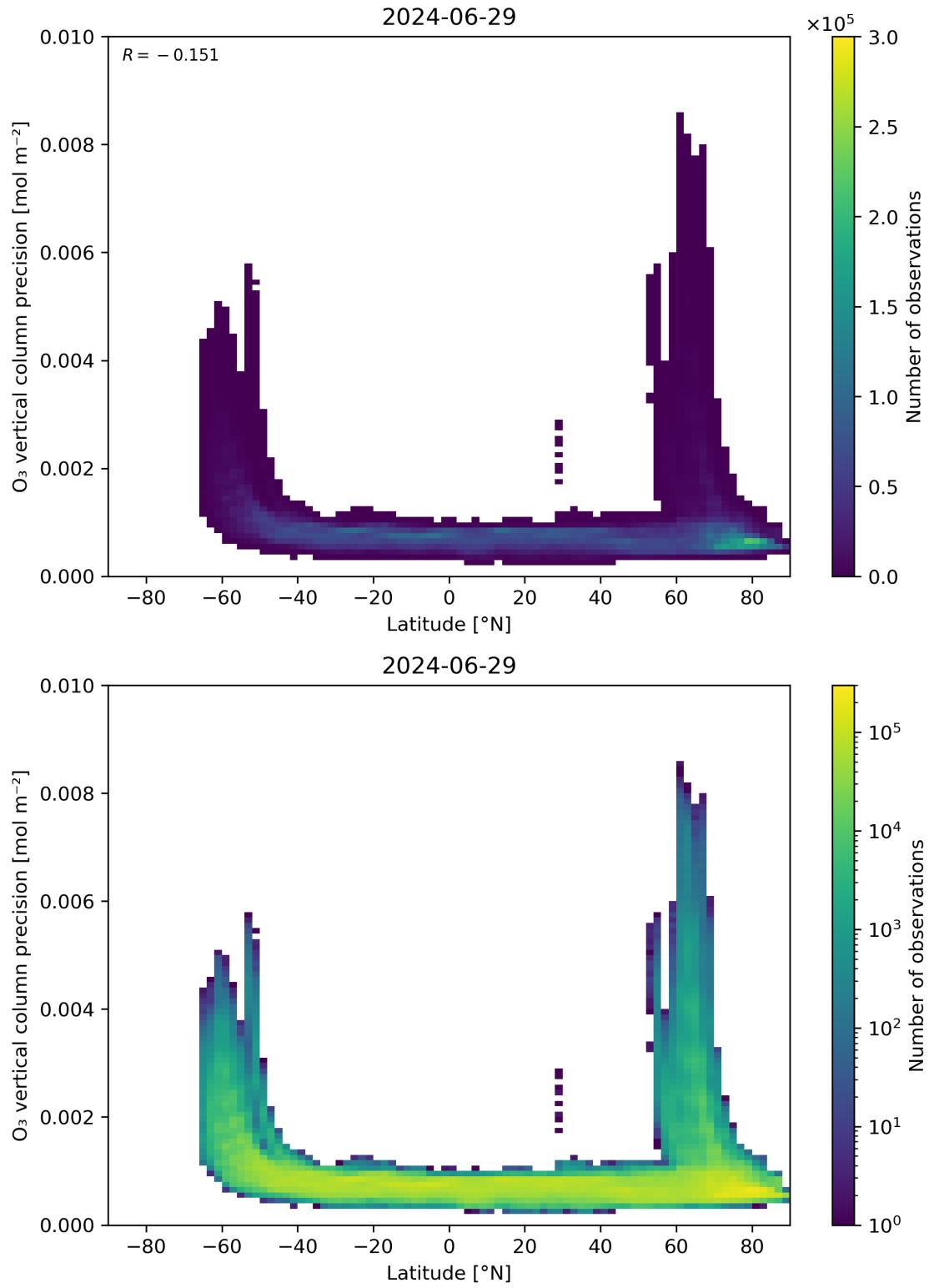
Figure 37: Scatter density plot of “Latitude” against “O 3 vertical column precision” for 2024-06-29 to 2024-06-30.
