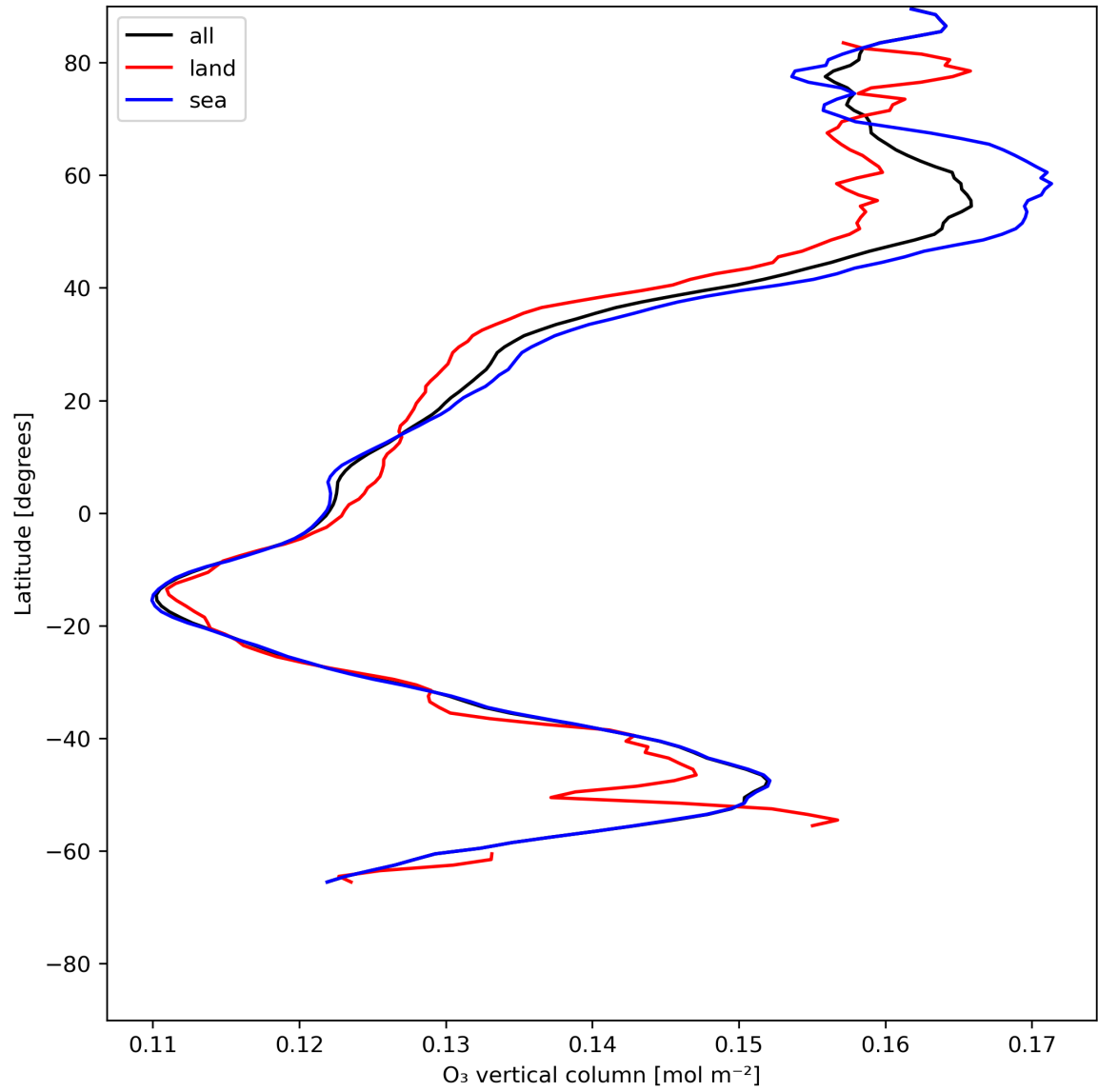
Figure 14: Zonal average of “O 3 vertical column” for 2024-06-29 to 2024-06-30.
