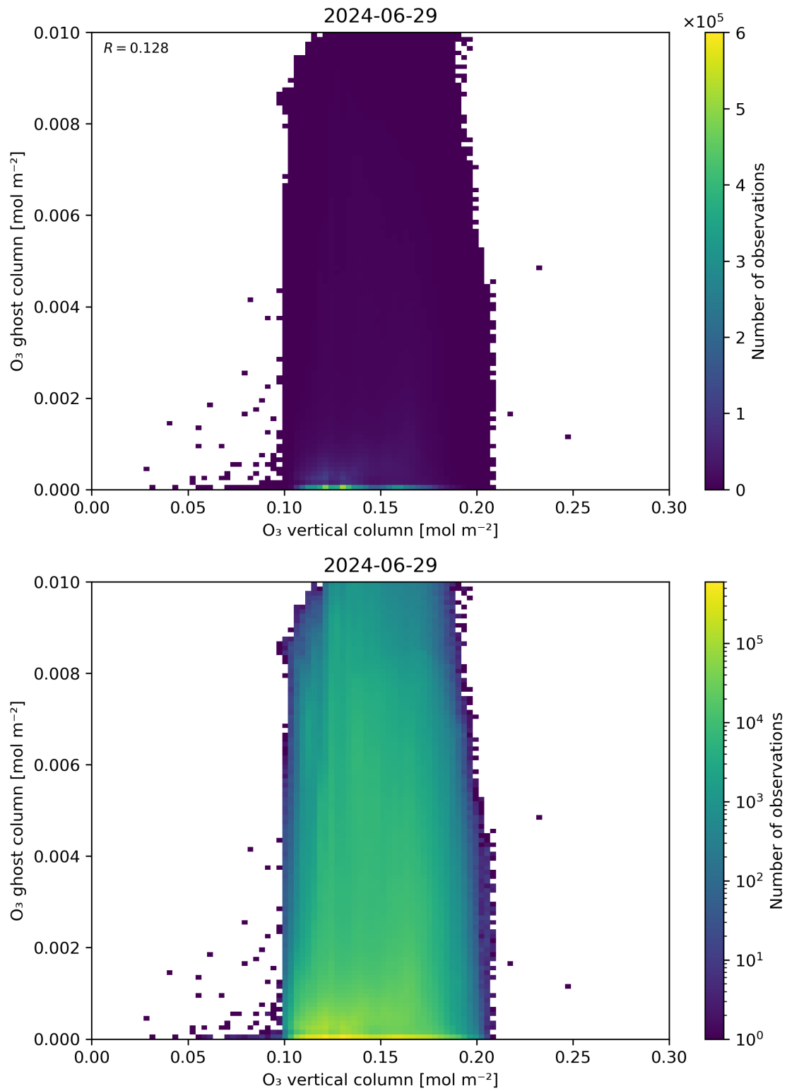
Figure 40: Scatter density plot of “O 3 vertical column” against “O 3 ghost column” for 2024-06-29 to 2024-06-30.
