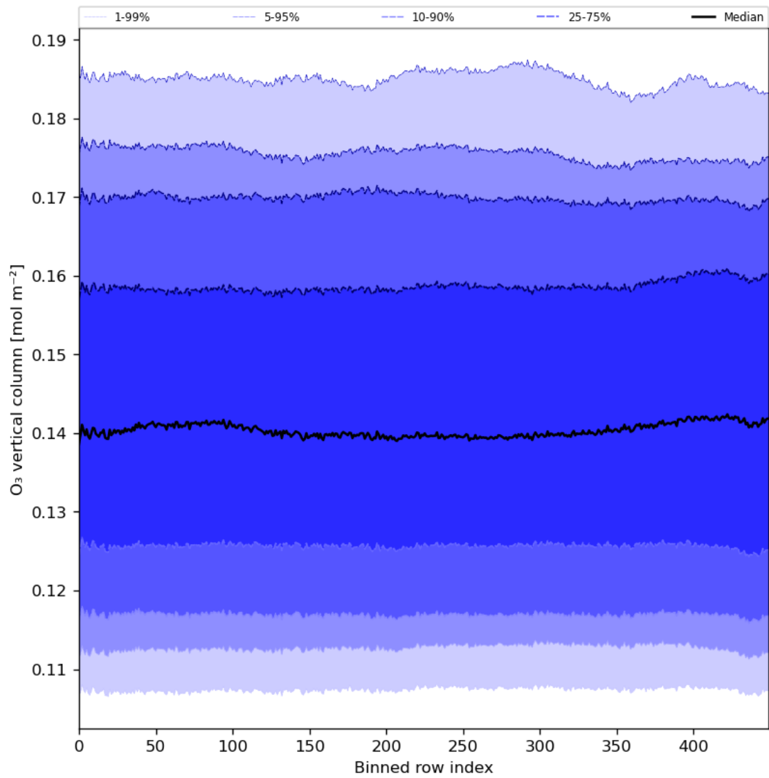
Figure 28: Along track statistics of “O 3 vertical column” for 2024-06-29 to 2024-06-30
