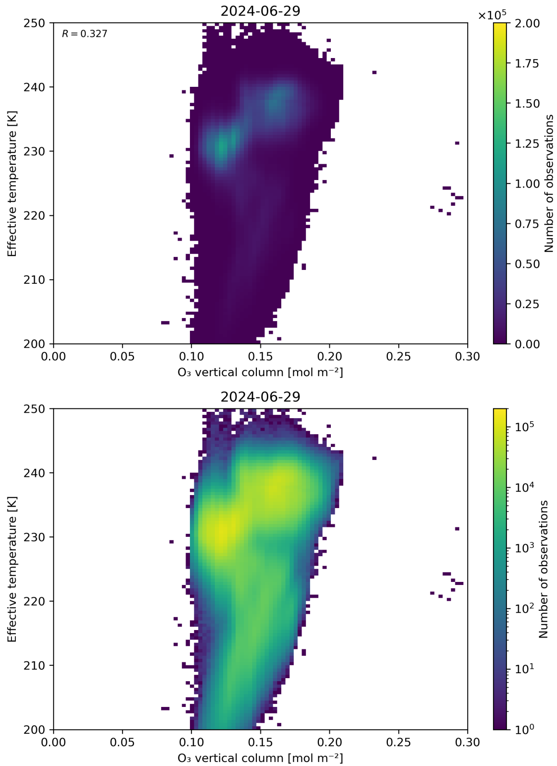
Figure 39: Scatter density plot of “O 3 vertical column” against “Effective temperature” for 2024-06-29 to 2024-06-30.
