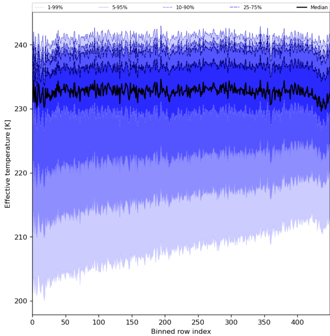
Figure 31: Along track statistics of “Effective temperature” for 2024-06-29 to 2024-06-30
