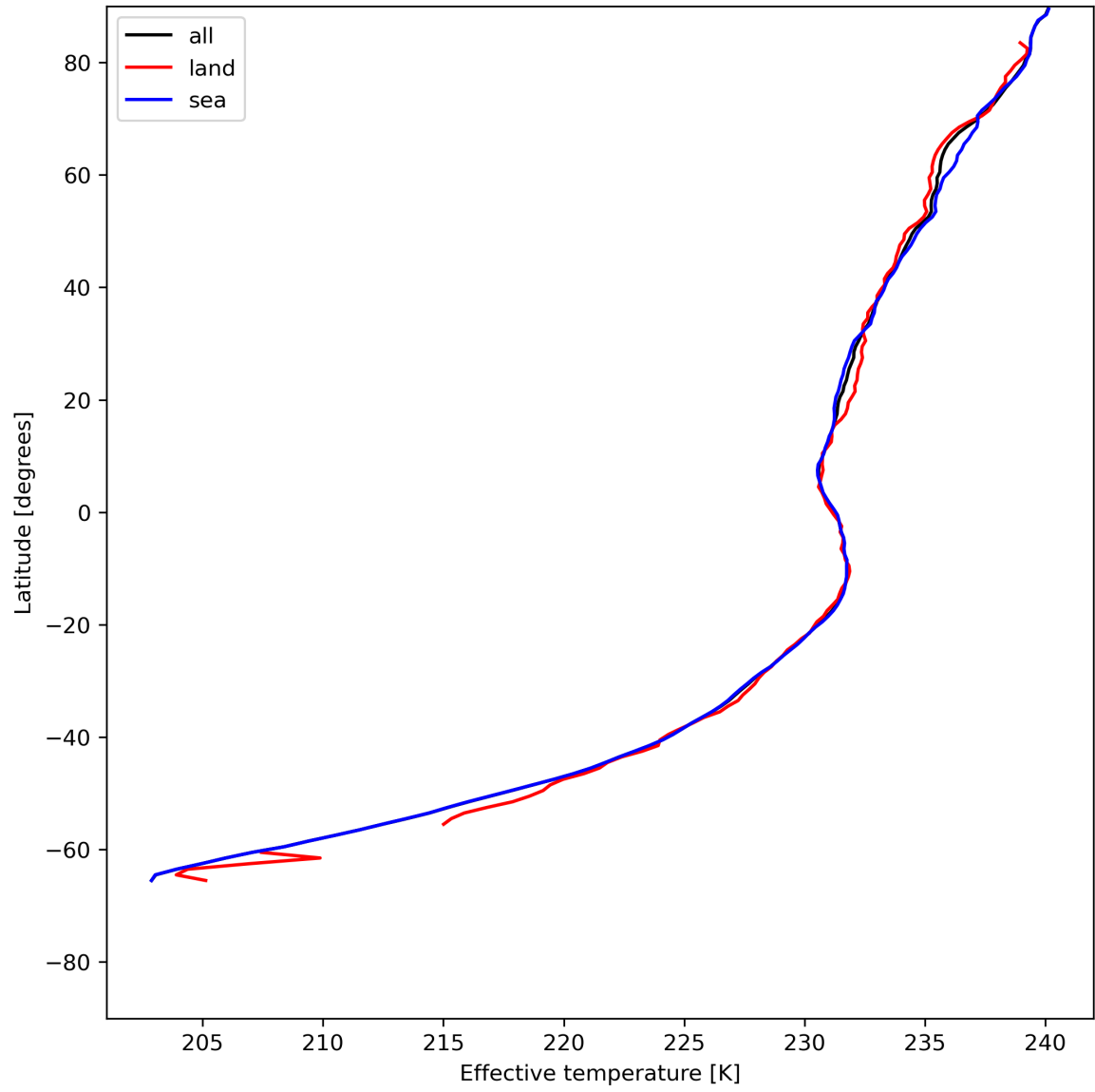
Figure 17: Zonal average of "Effective temperature" for 2024-06-29 to 2024-06-30.
