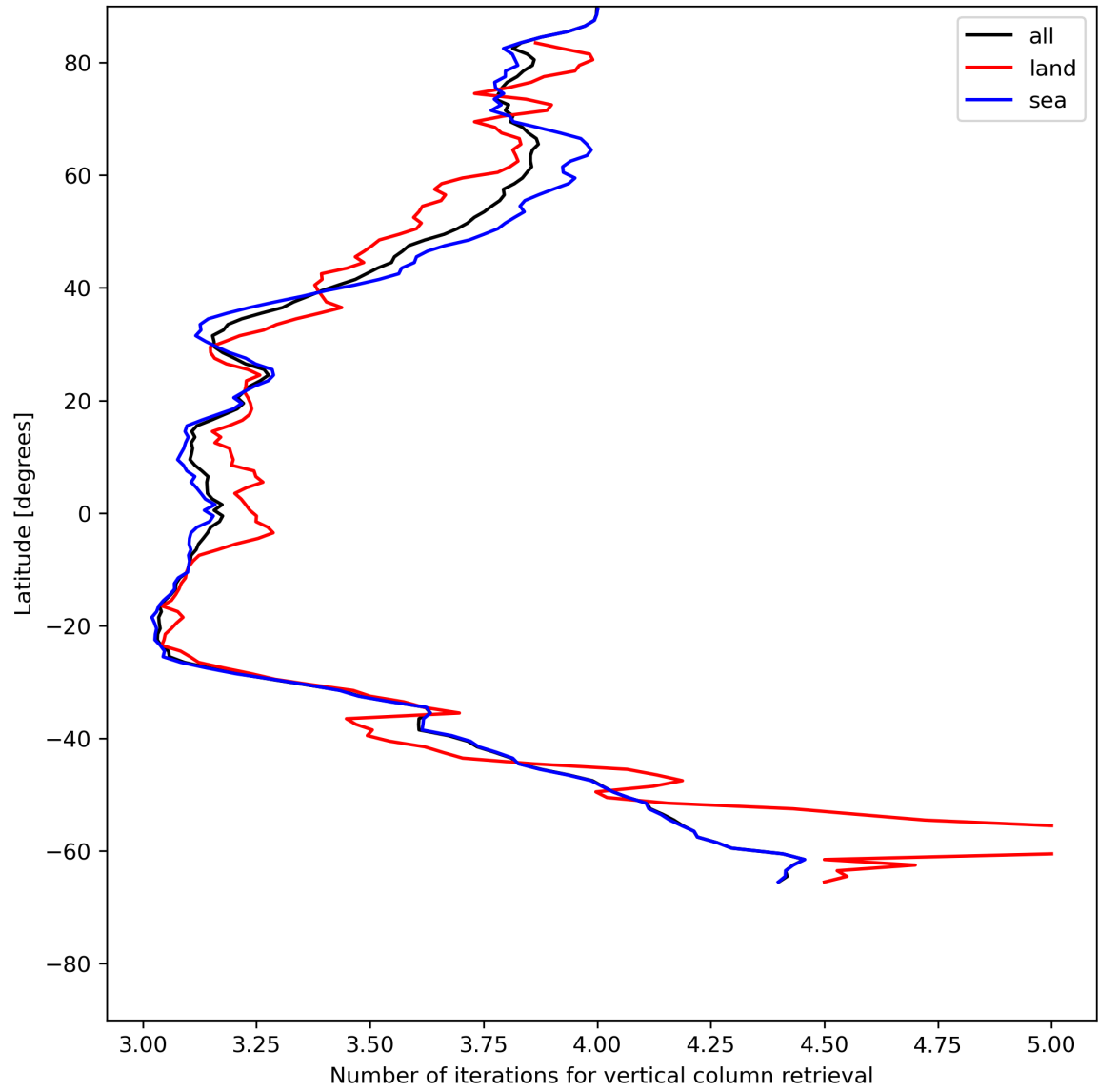
Figure 19: Zonal average of “Number of iterations for vertical column retrieval” for 2024-06-29 to 2024-06-30.
