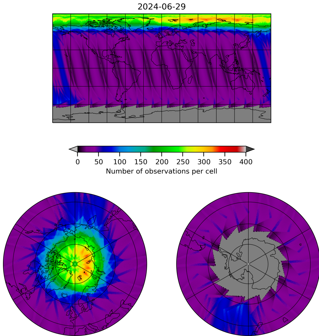
Figure 12: Map of the number of observations for 2024-06-29 to 2024-06-30
