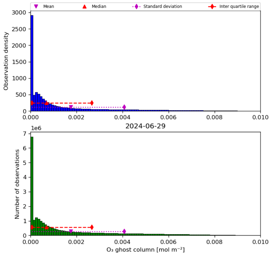
Figure 25: Histogram of “O 3 ghost column” for 2024-06-29 to 2024-06-30
