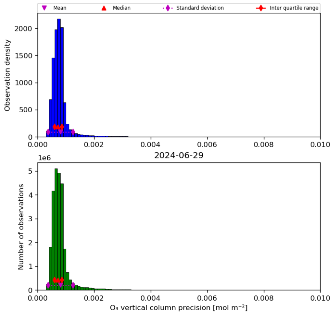
Figure 22: Histogram of “O 3 vertical column precision” for 2024-06-29 to 2024-06-30
