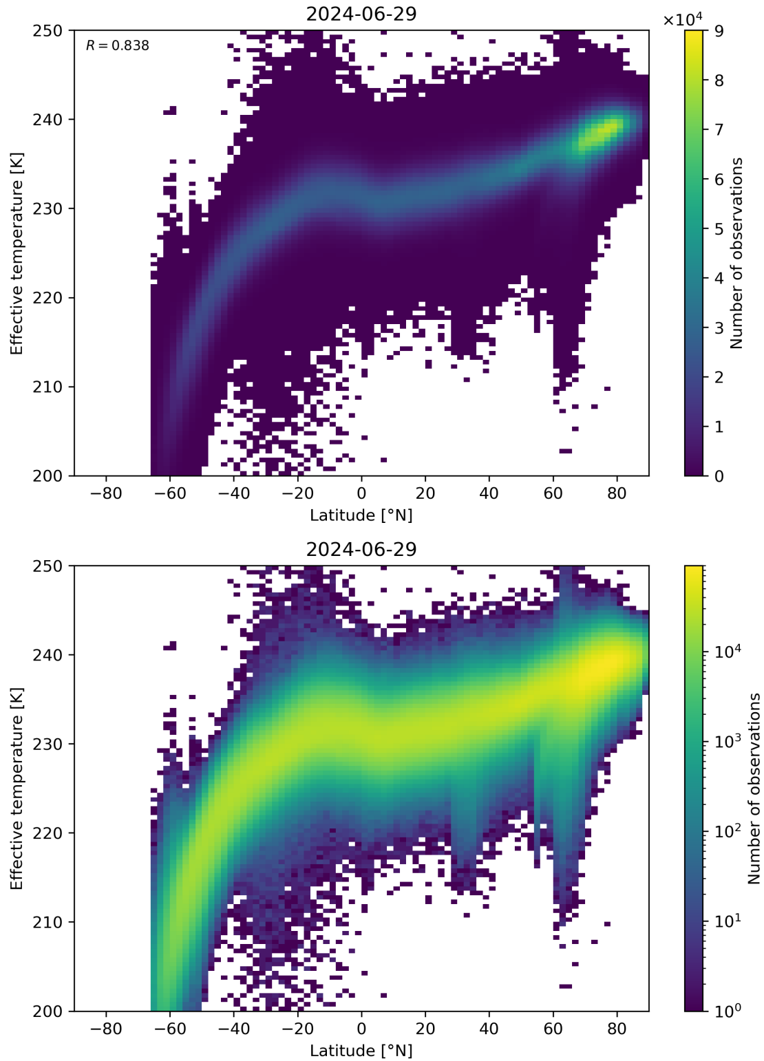
Figure 34: Scatter density plot of “Latitude” against “Effective temperature” for 2024-06-29 to 2024-06-30.
