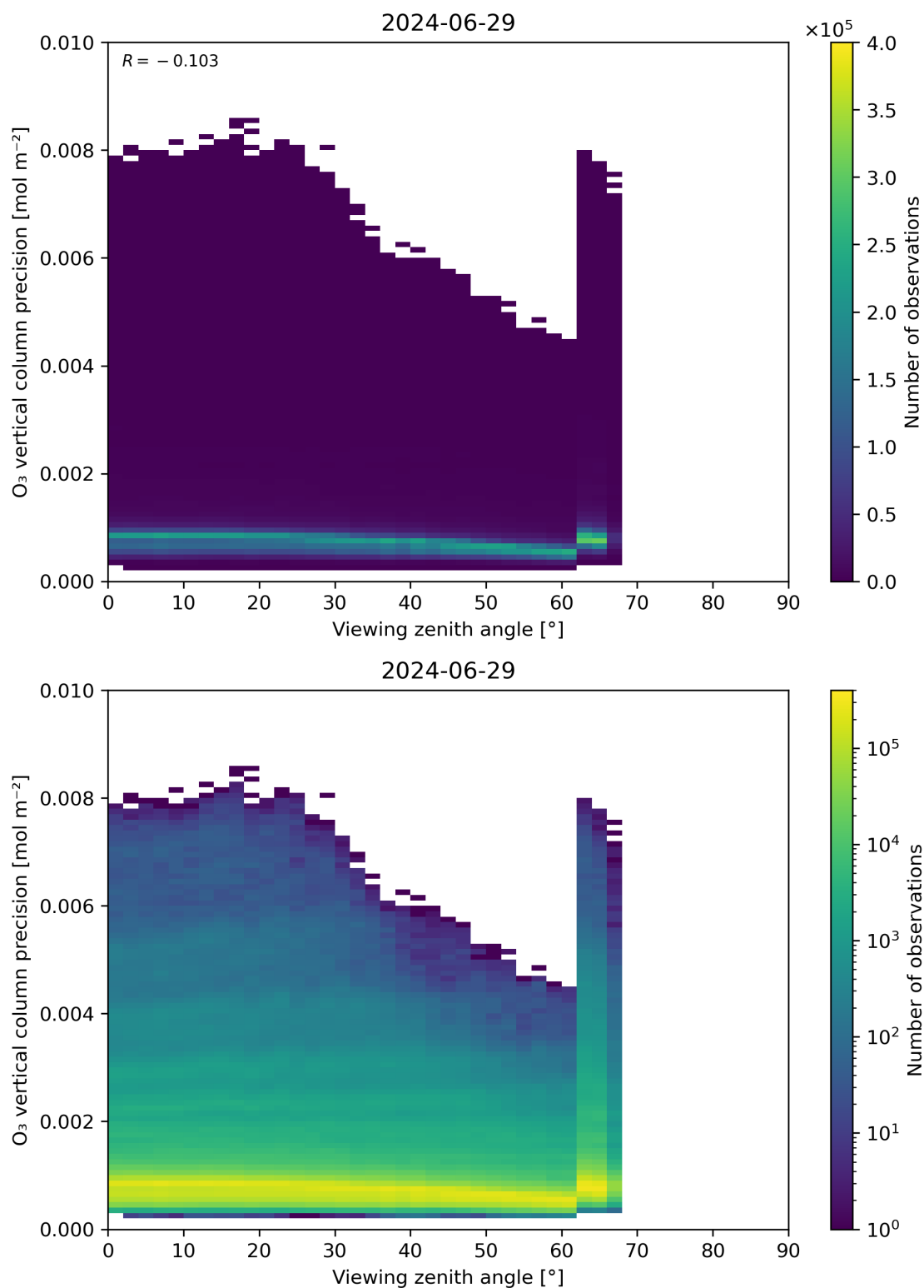
Figure 53: Scatter density plot of “Viewing zenith angle” against “O 3 vertical column precision” for 2024-06-29 to 2024-06-30.
