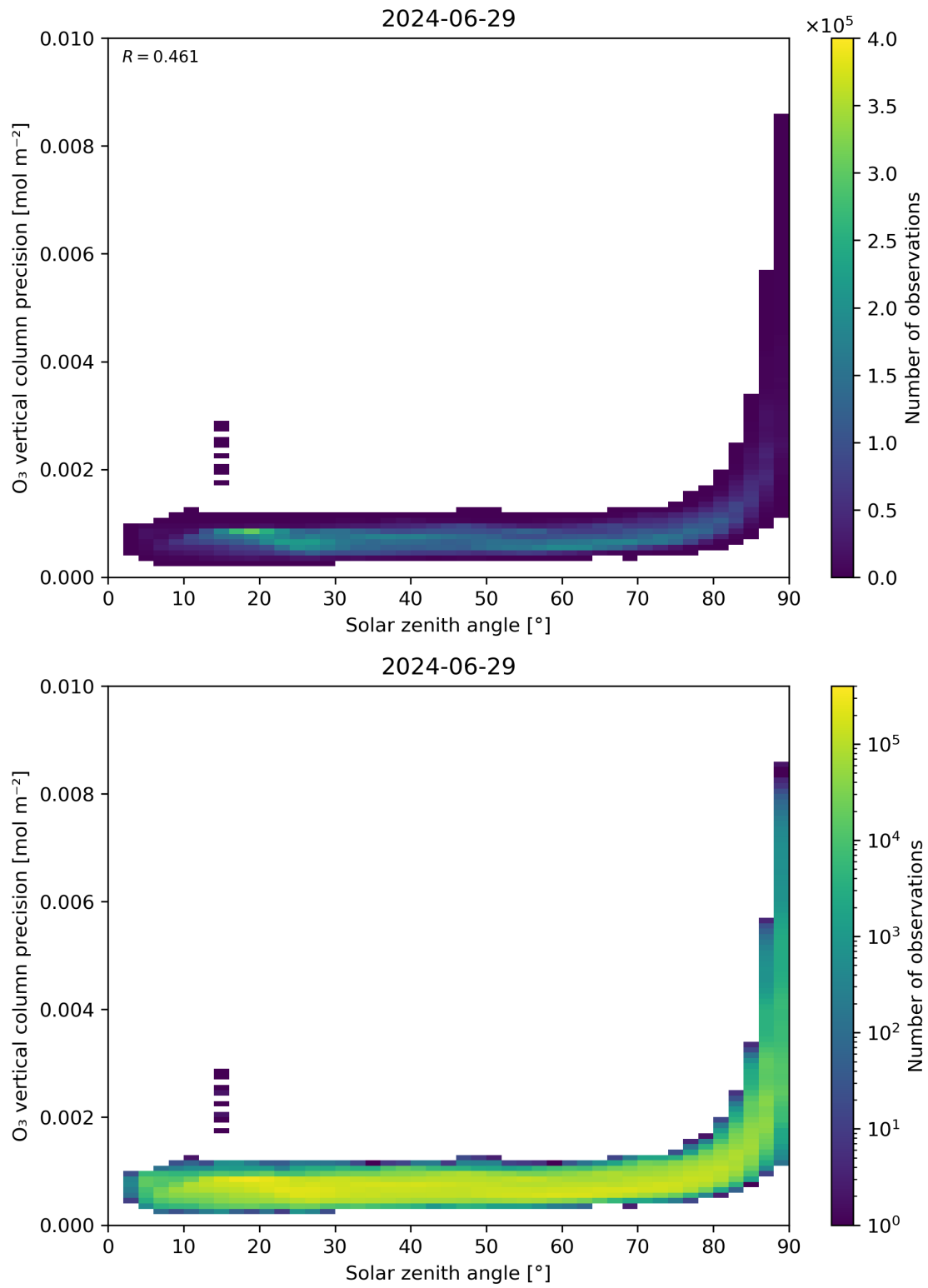
Figure 48: Scatter density plot of “Solar zenith angle” against “O 3 vertical column precision” for 2024-06-29 to 2024-06-30.
