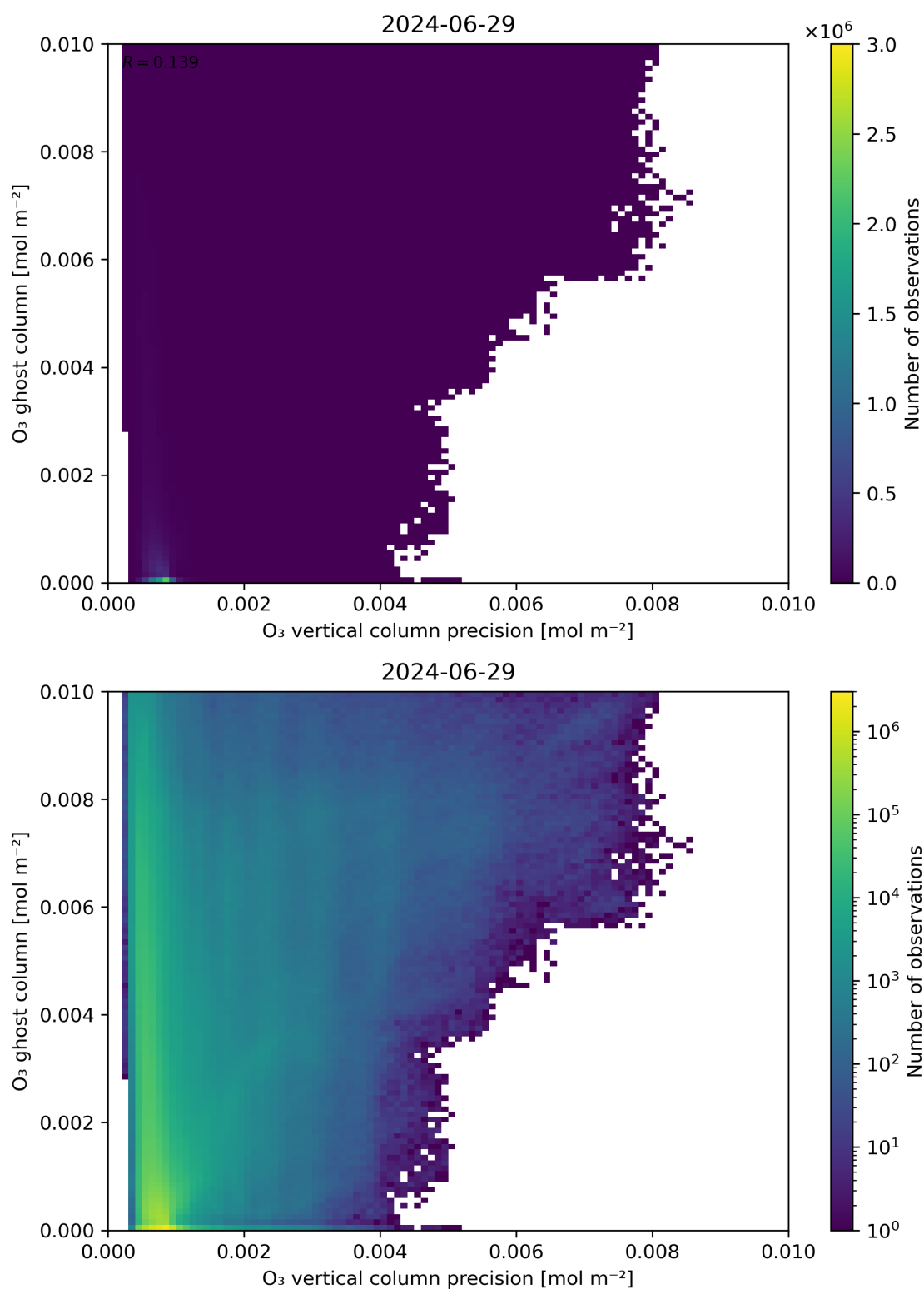
Figure 43: Scatter density plot of “ \text{O}_3 vertical column precision” against “ \text{O}_3 ghost column” for 2024-06-29 to 2024-06-30.
