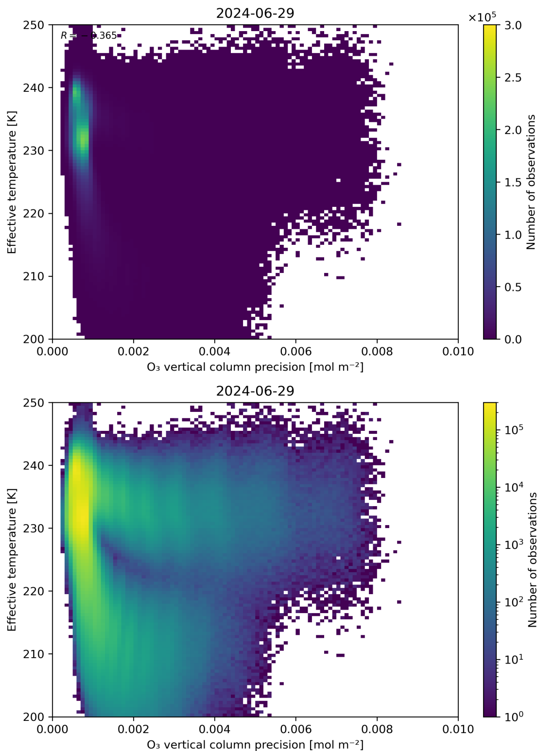
Figure 42: Scatter density plot of “O 3 vertical column precision” against “Effective temperature” for 2024-06-29 to 2024-06-30.
