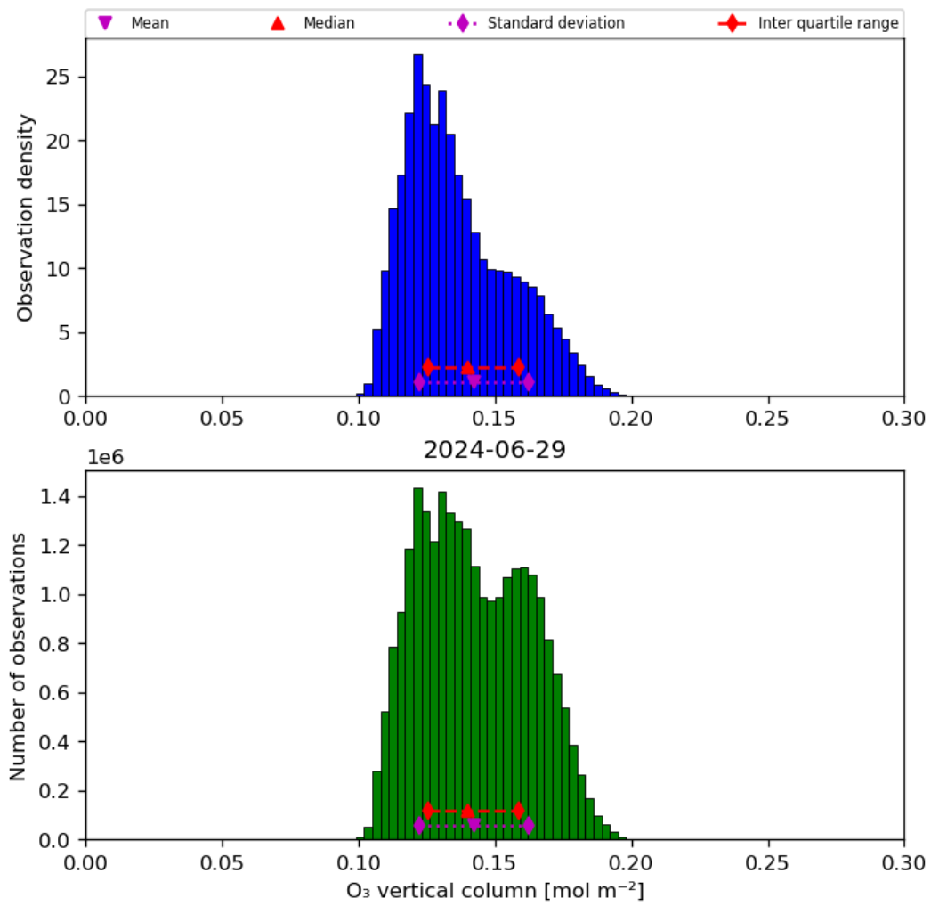
Figure 21: Histogram of “O 3 vertical column” for 2024-06-29 to 2024-06-30
