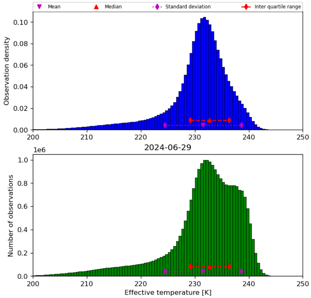
Figure 24: Histogram of “Effective temperature” for 2024-06-29 to 2024-06-30
