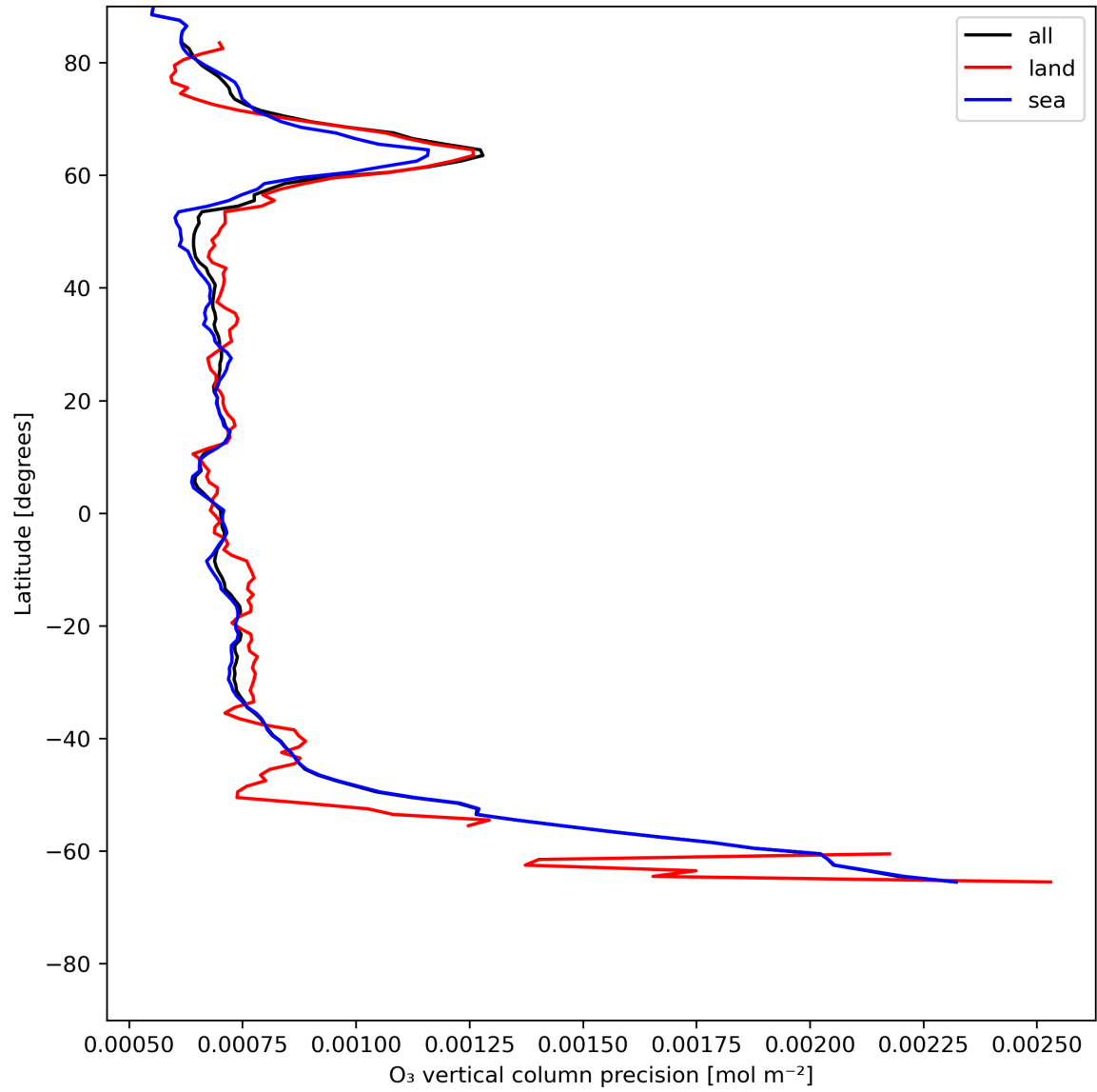
Figure 15: Zonal average of “O 3 vertical column precision” for 2024-06-29 to 2024-06-30.
