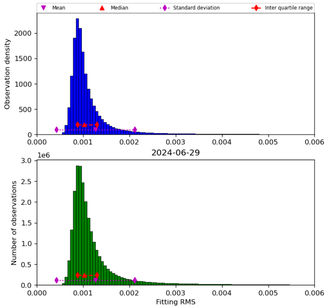
Figure 23: Histogram of “Fitting RMS” for 2024-06-29 to 2024-06-30
