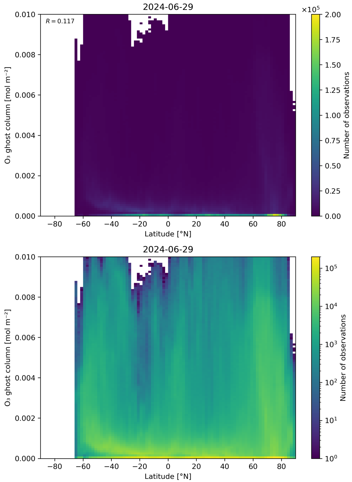
Figure 35: Scatter density plot of “Latitude” against “O 3 ghost column” for 2024-06-29 to 2024-06-30.
