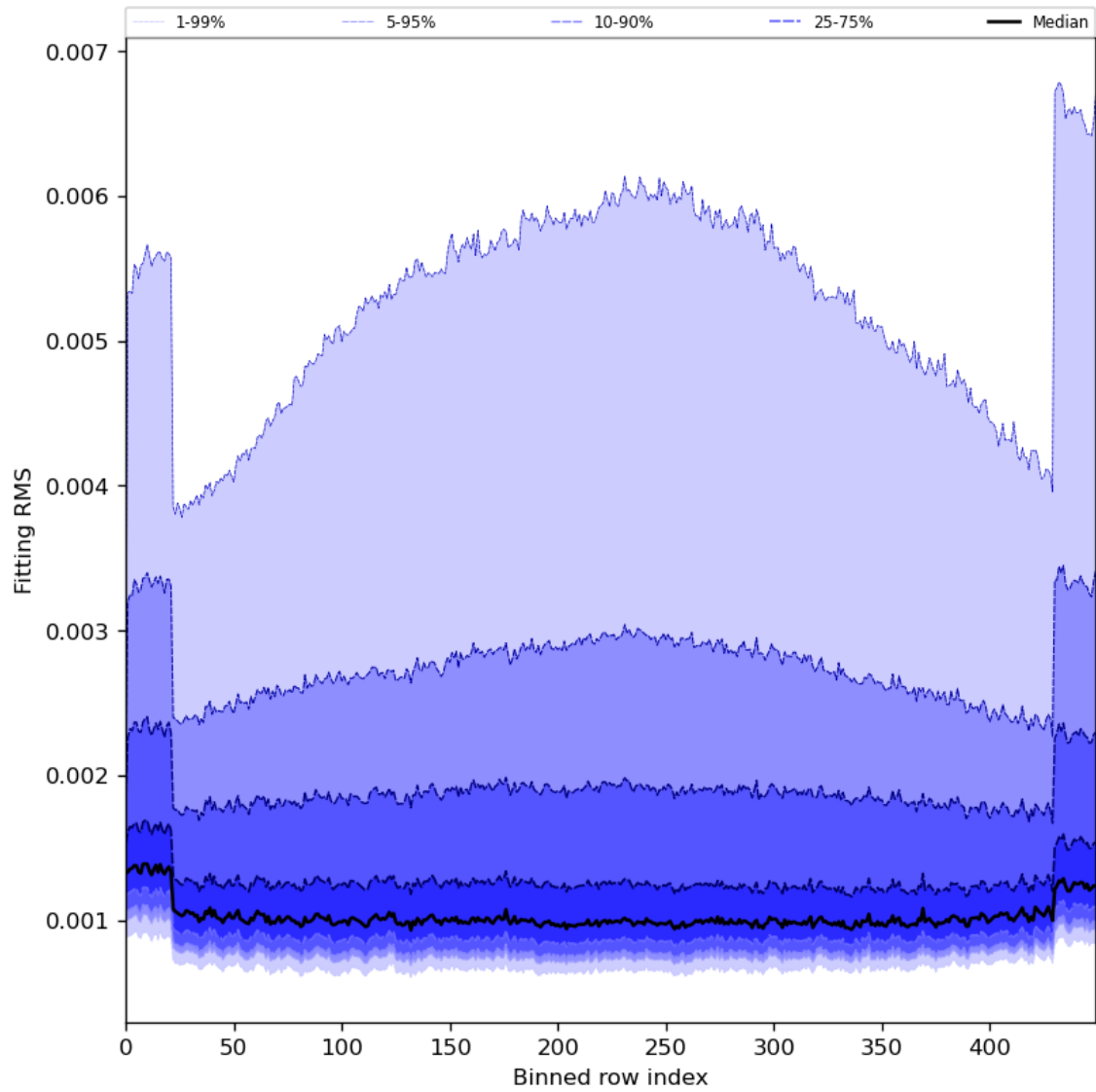
Figure 30: Along track statistics of “Fitting RMS” for 2024-06-29 to 2024-06-30
