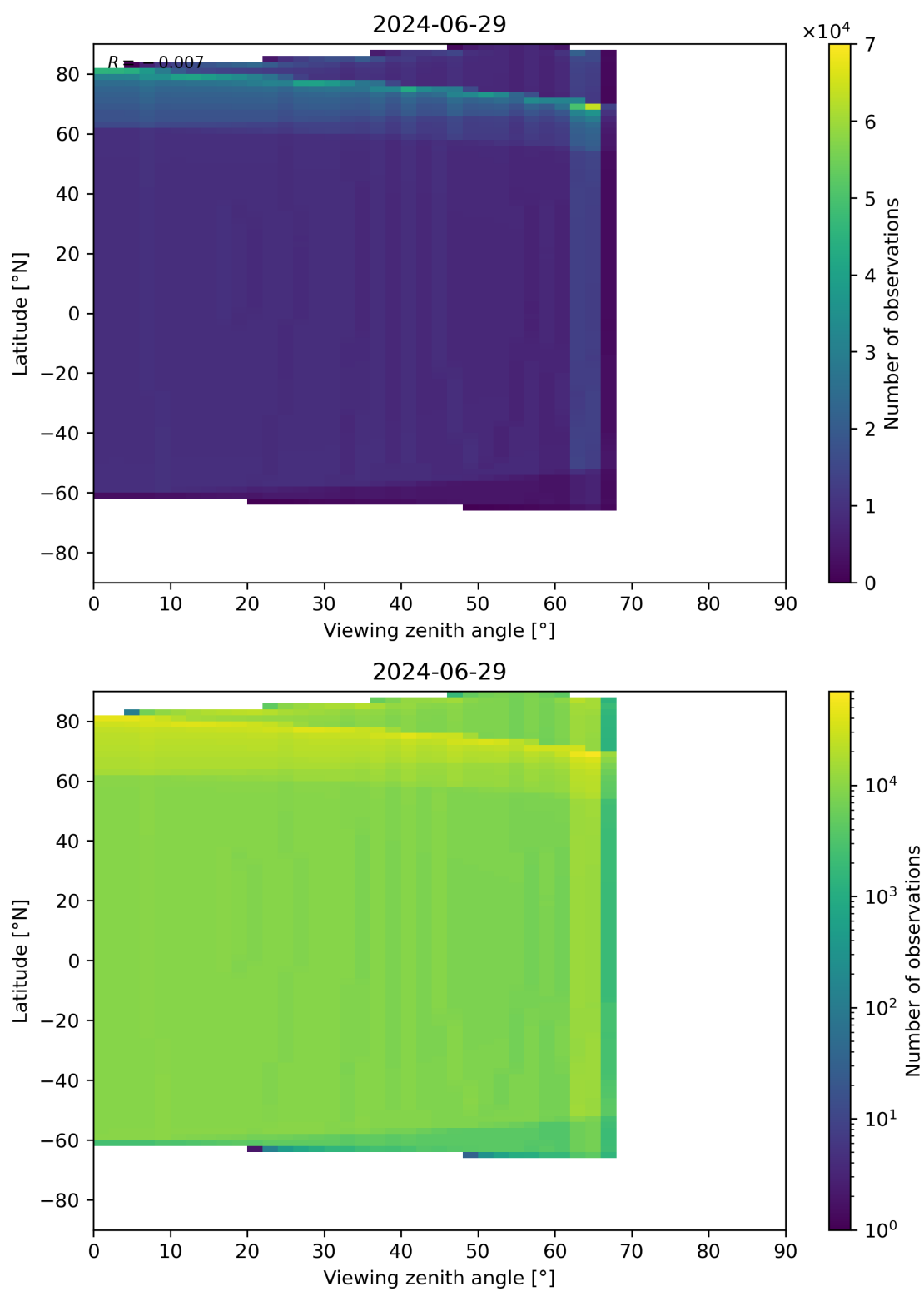
Figure 49: Scatter density plot of “Viewing zenith angle” against “Latitude” for 2024-06-29 to 2024-06-30.
