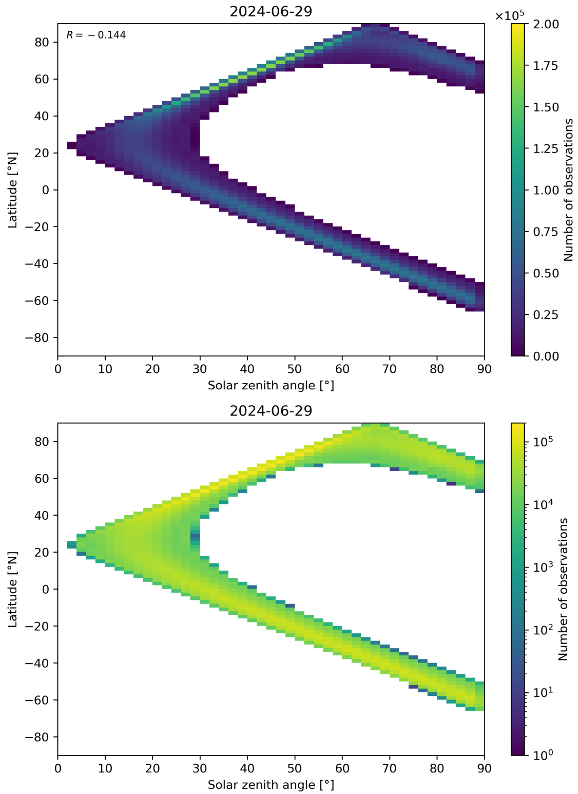
Figure 44: Scatter density plot of “Solar zenith angle” against “Latitude” for 2024-06-29 to 2024-06-30.
