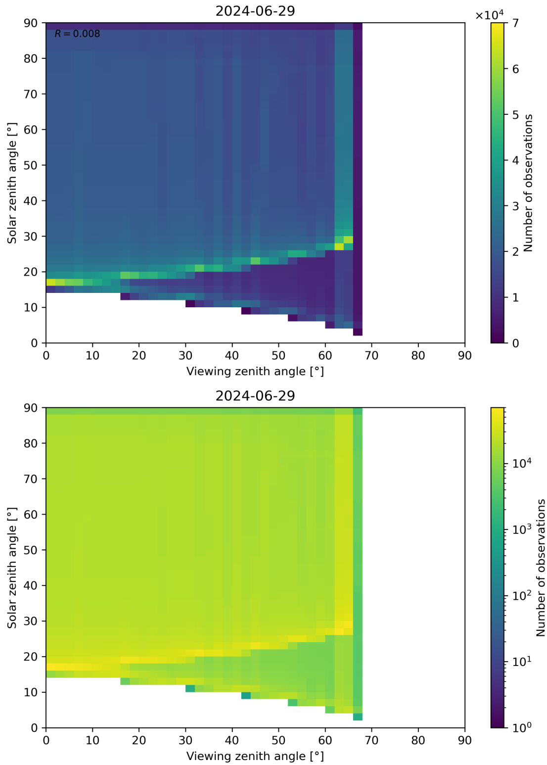
Figure 54: Scatter density plot of “Viewing zenith angle” against “Solar zenith angle” for 2024-06-29 to 2024-06-30.
