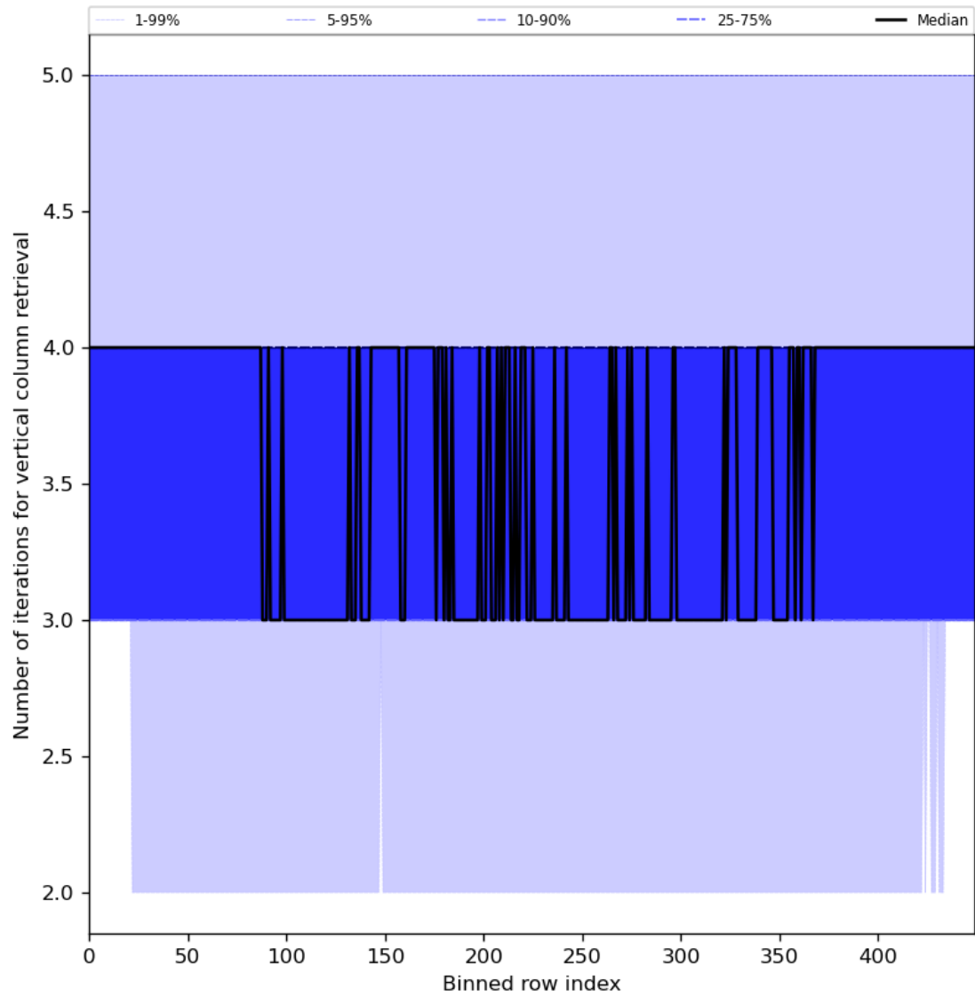
Figure 33: Along track statistics of “Number of iterations for vertical column retrieval” for 2024-06-29 to 2024-06-30
