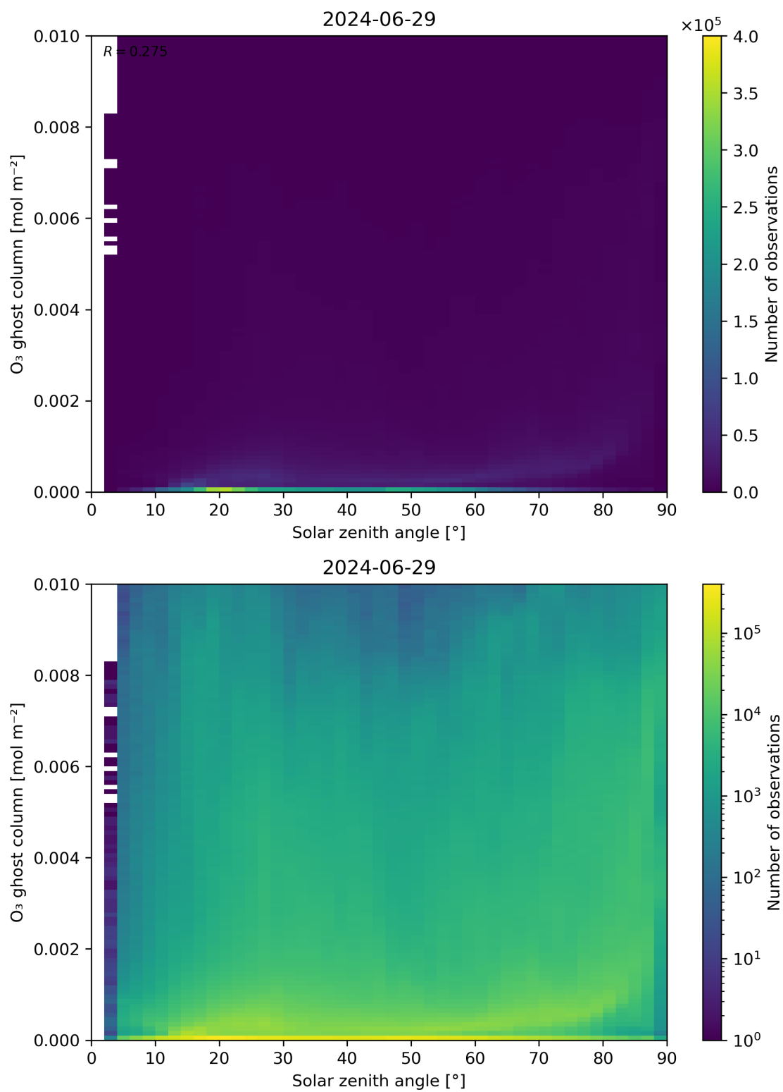
Figure 46: Scatter density plot of “Solar zenith angle” against “O 3 ghost column” for 2024-06-29 to 2024-06-30.
