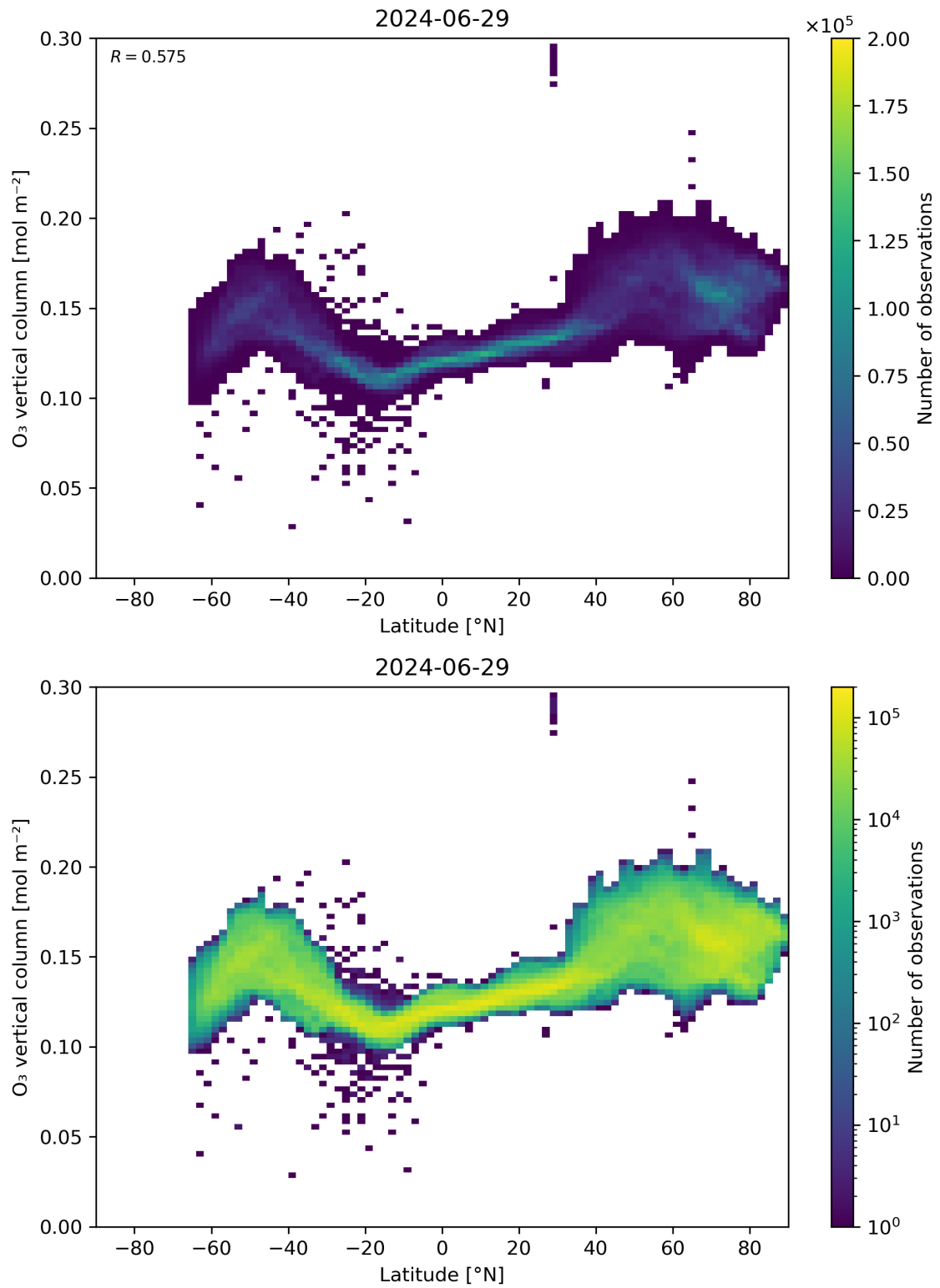
Figure 36: Scatter density plot of “Latitude” against “O 3 vertical column” for 2024-06-29 to 2024-06-30.
