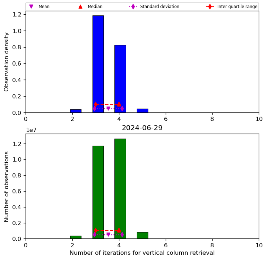
Figure 26: Histogram of “Number of iterations for vertical column retrieval” for 2024-06-29 to 2024-06-30
