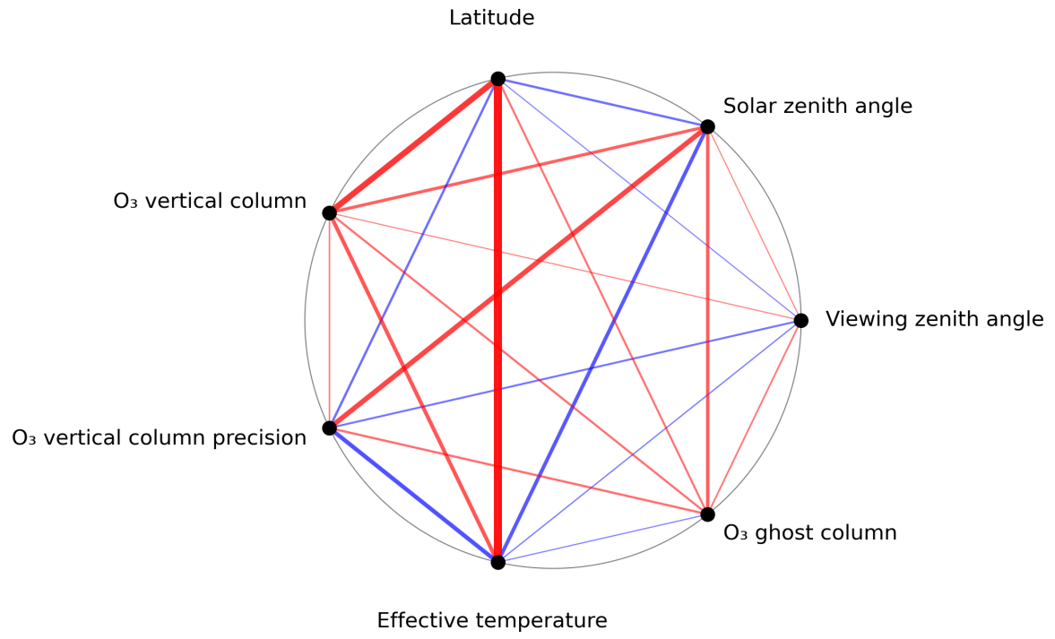
Figure 1: Map of correlation graph for 2024-06-29 to 2024-06-30.
