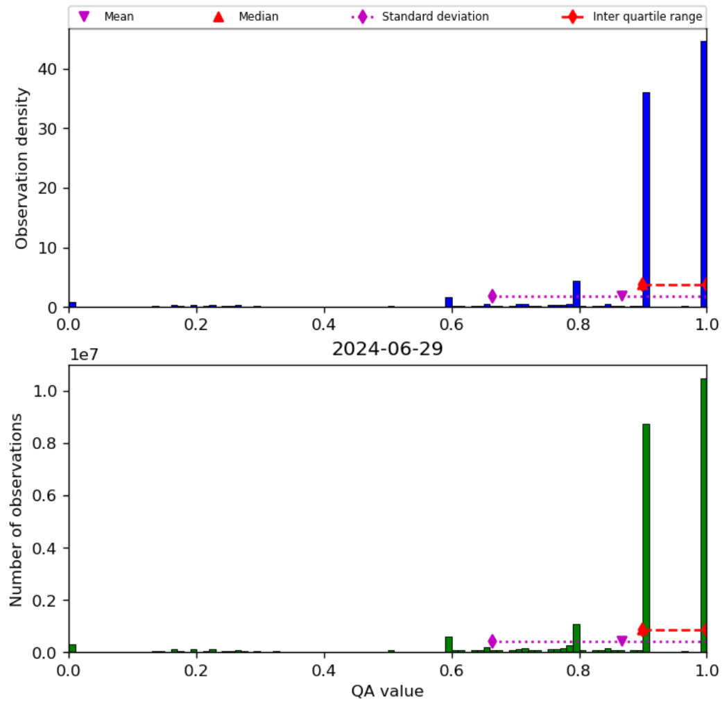
Figure 20: Histogram of “QA value” for 2024-06-29 to 2024-06-30
