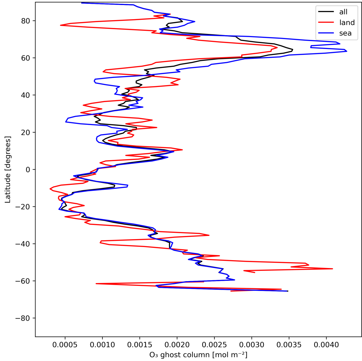
Figure 18: Zonal average of “O 3 ghost column” for 2024-06-29 to 2024-06-30.
