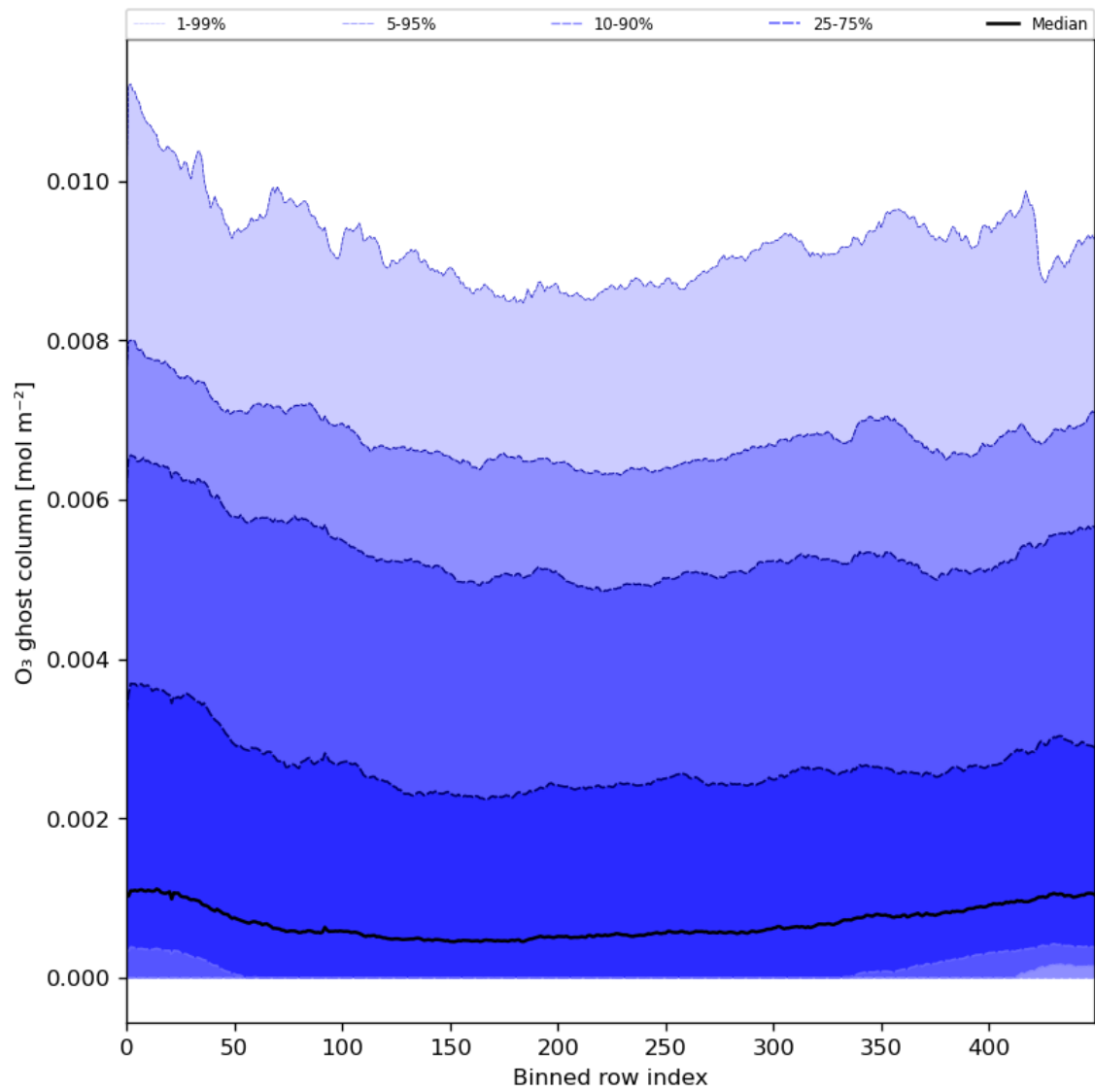
Figure 32: Along track statistics of “O 3 ghost column” for 2024-06-29 to 2024-06-30
