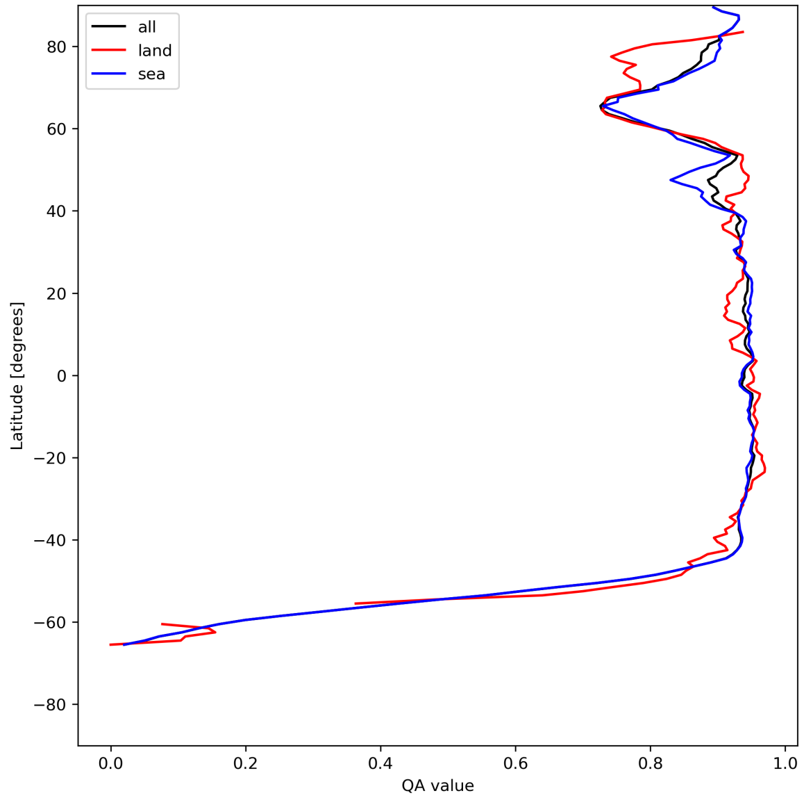
Figure 13: Zonal average of “QA value” for 2024-06-29 to 2024-06-30.
