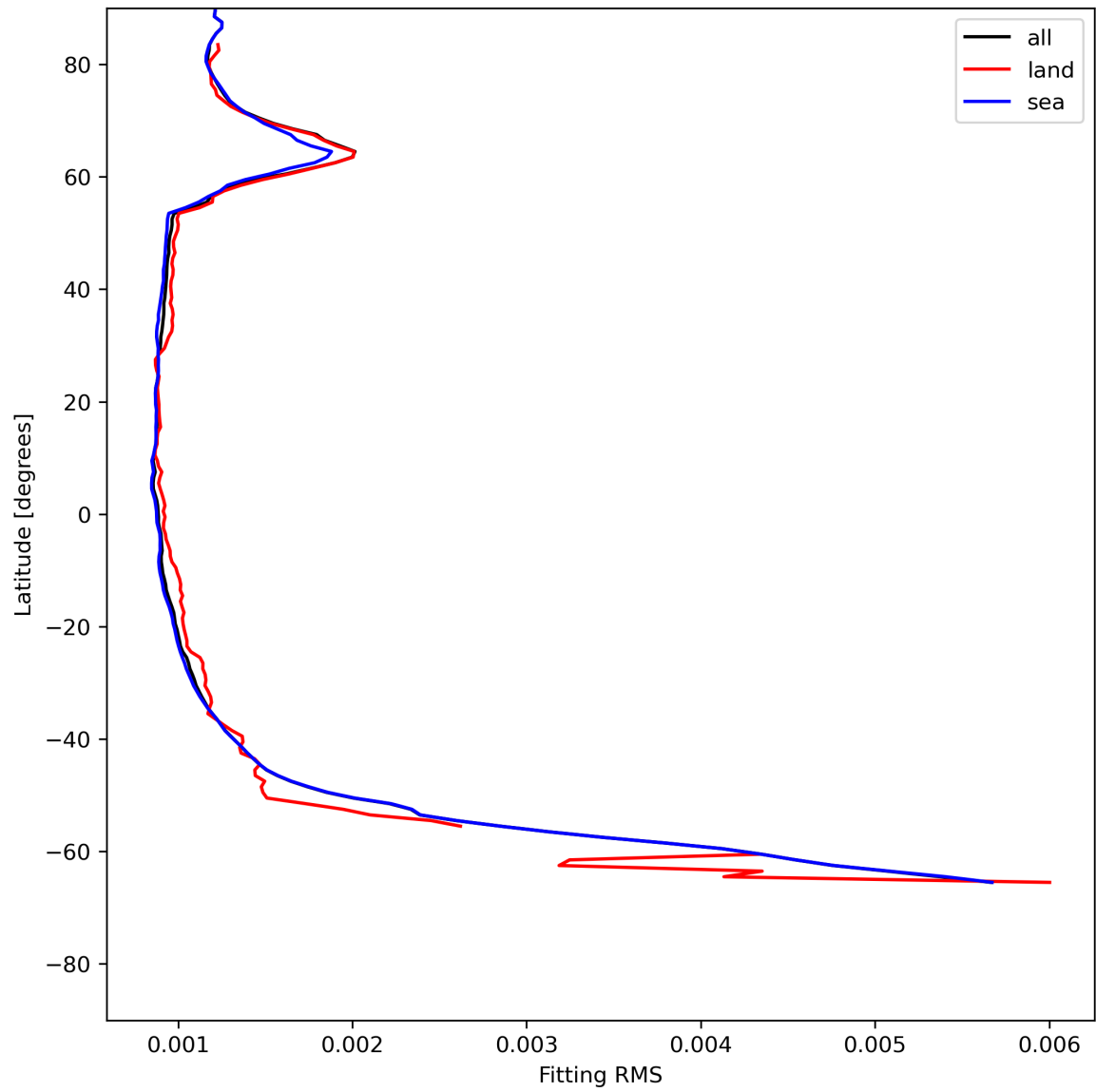
Figure 16: Zonal average of “Fitting RMS” for 2024-06-29 to 2024-06-30.
