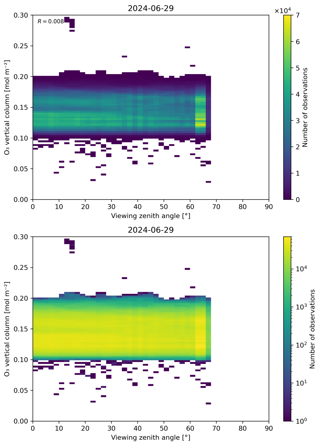
Figure 52: Scatter density plot of “Viewing zenith angle” against “O 3 vertical column” for 2024-06-29 to 2024-06-30.
