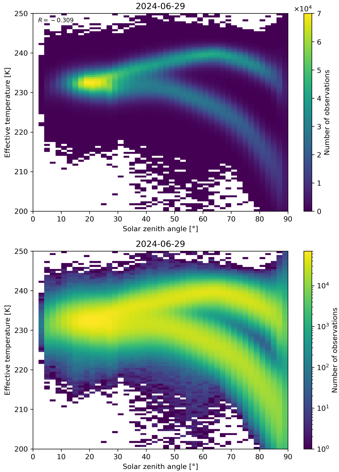
Figure 45: Scatter density plot of “Solar zenith angle” against “Effective temperature” for 2024-06-29 to 2024-06-30.
