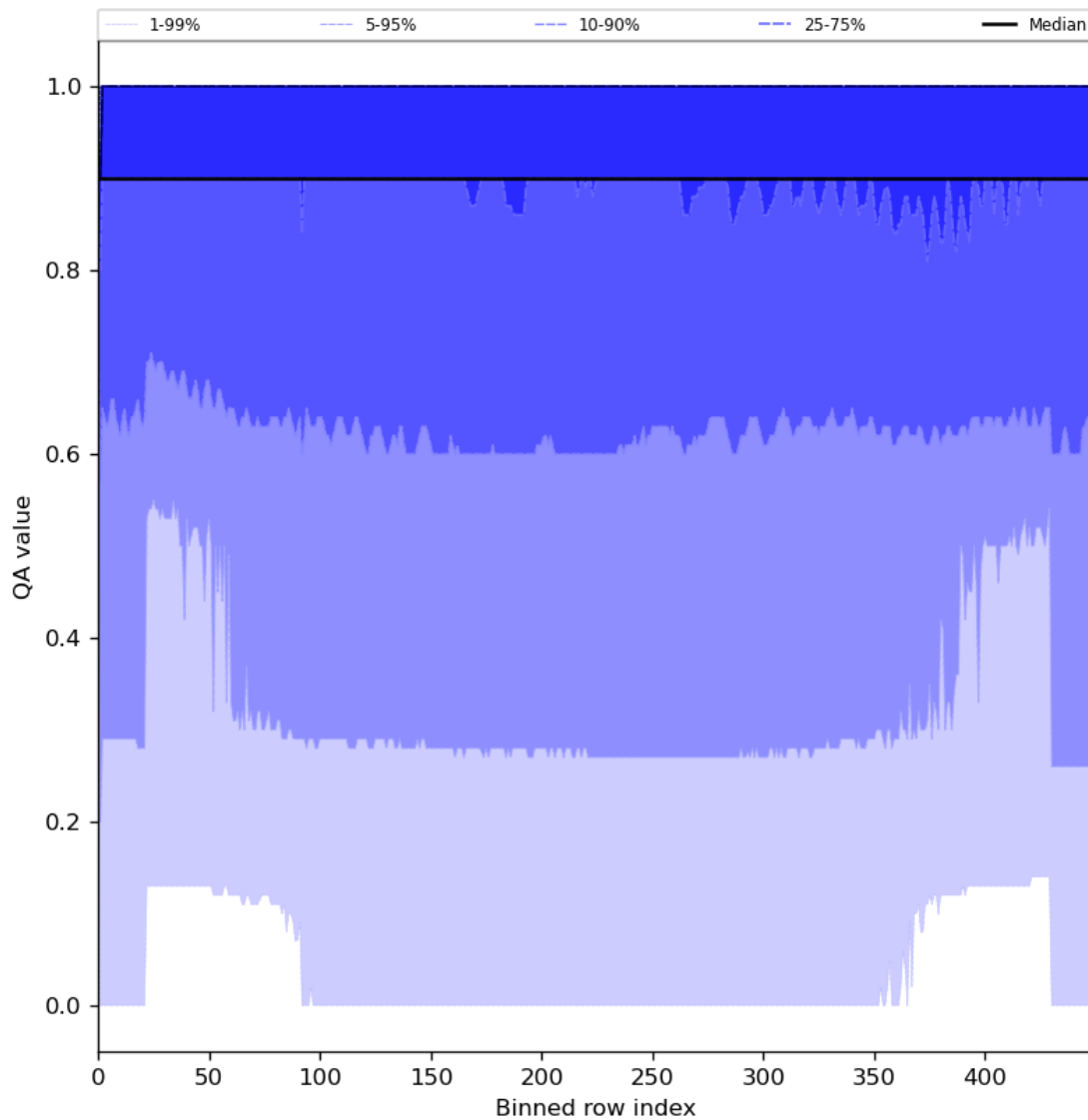
Figure 27: Along track statistics of “QA value” for 2024-06-29 to 2024-06-30
