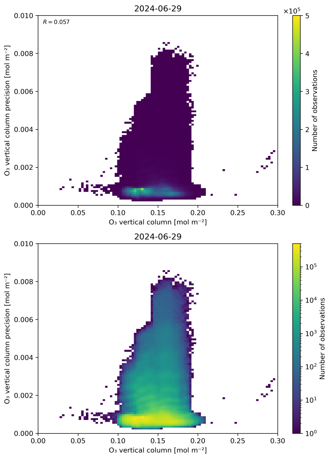
Figure 41: Scatter density plot of “O 3 vertical column” against “O 3 vertical column precision” for 2024-06-29 to 2024-06-30.
