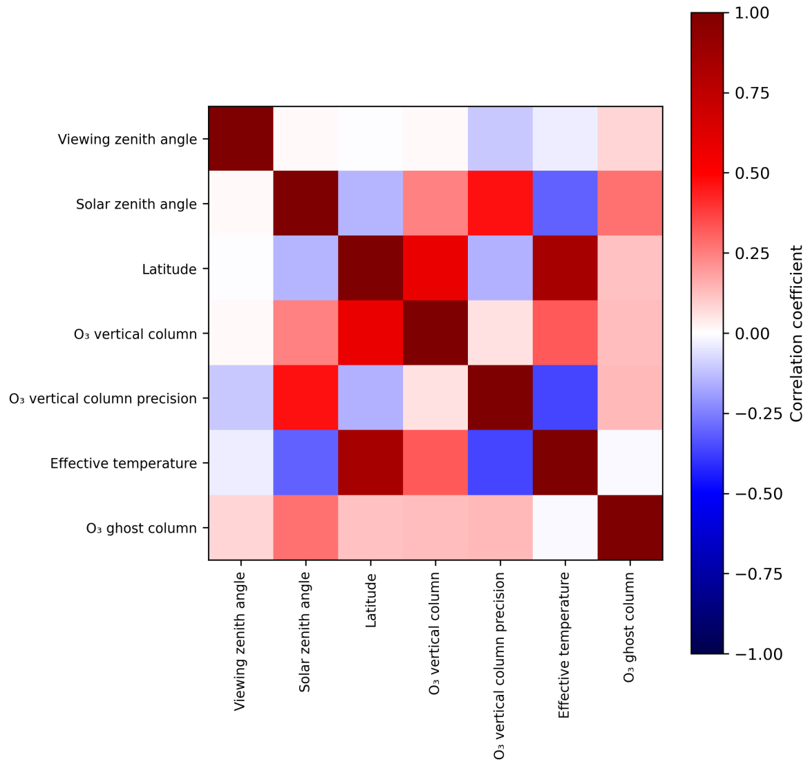
Figure 2: Map of correlation matrix for 2024-06-29 to 2024-06-30.
