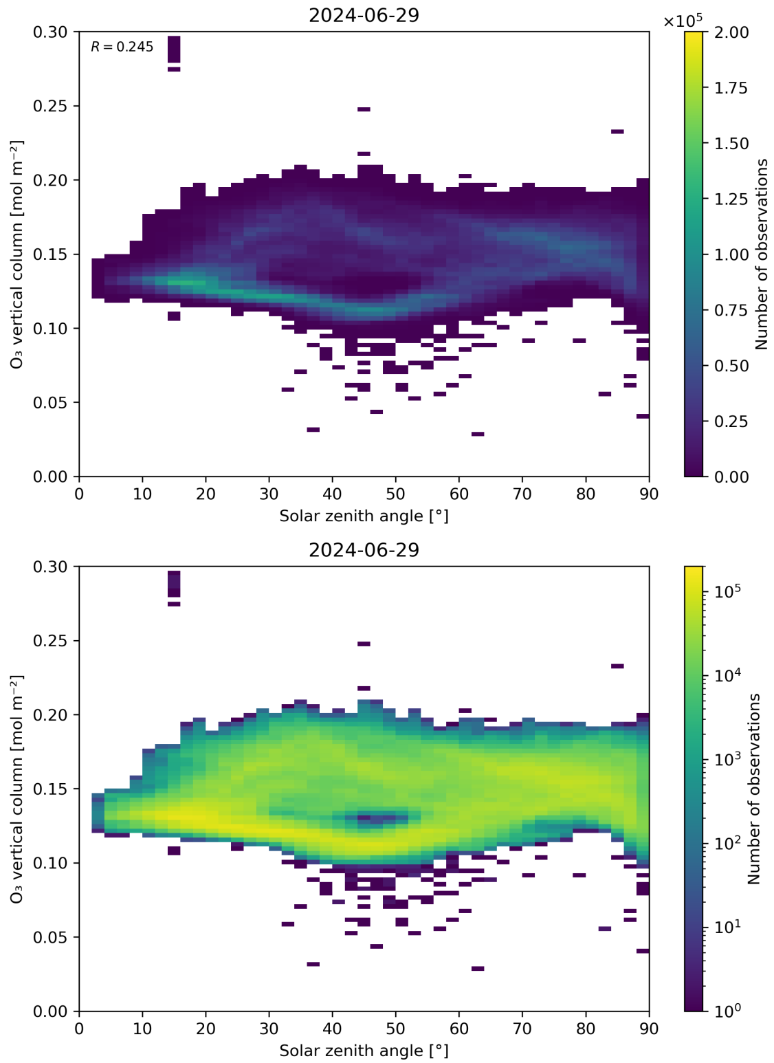
Figure 47: Scatter density plot of “Solar zenith angle” against “O 3 vertical column” for 2024-06-29 to 2024-06-30.
