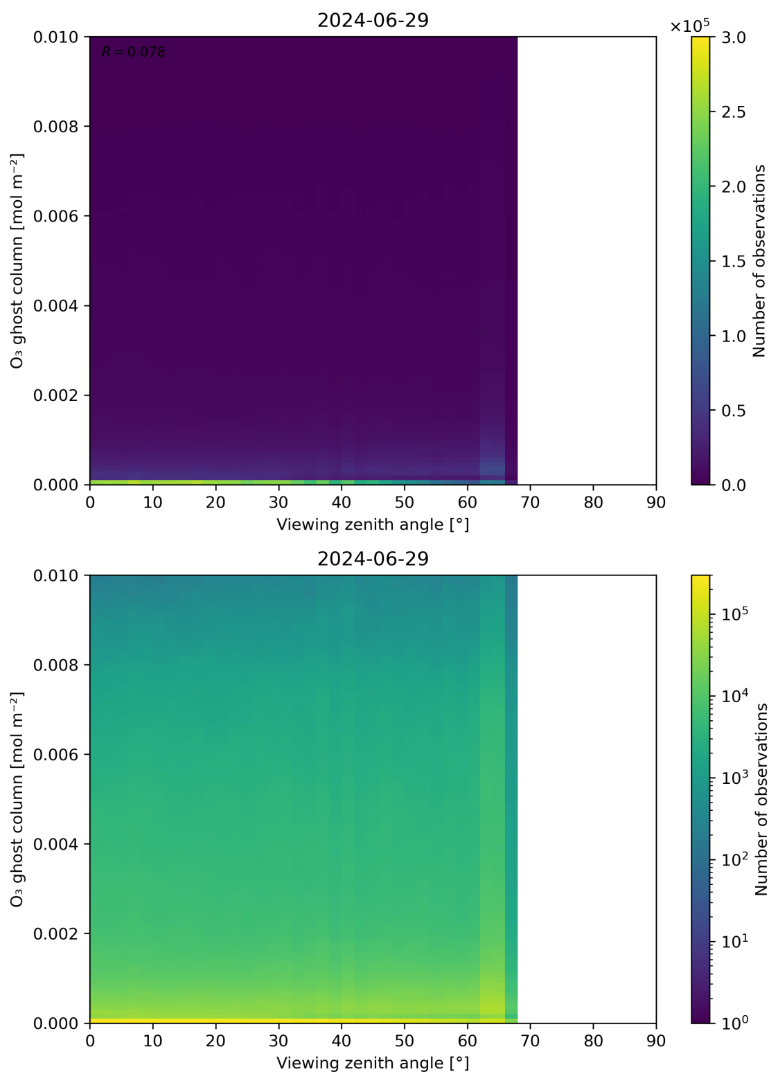
Figure 51: Scatter density plot of “Viewing zenith angle” against “O 3 ghost column” for 2024-06-29 to 2024-06-30.
