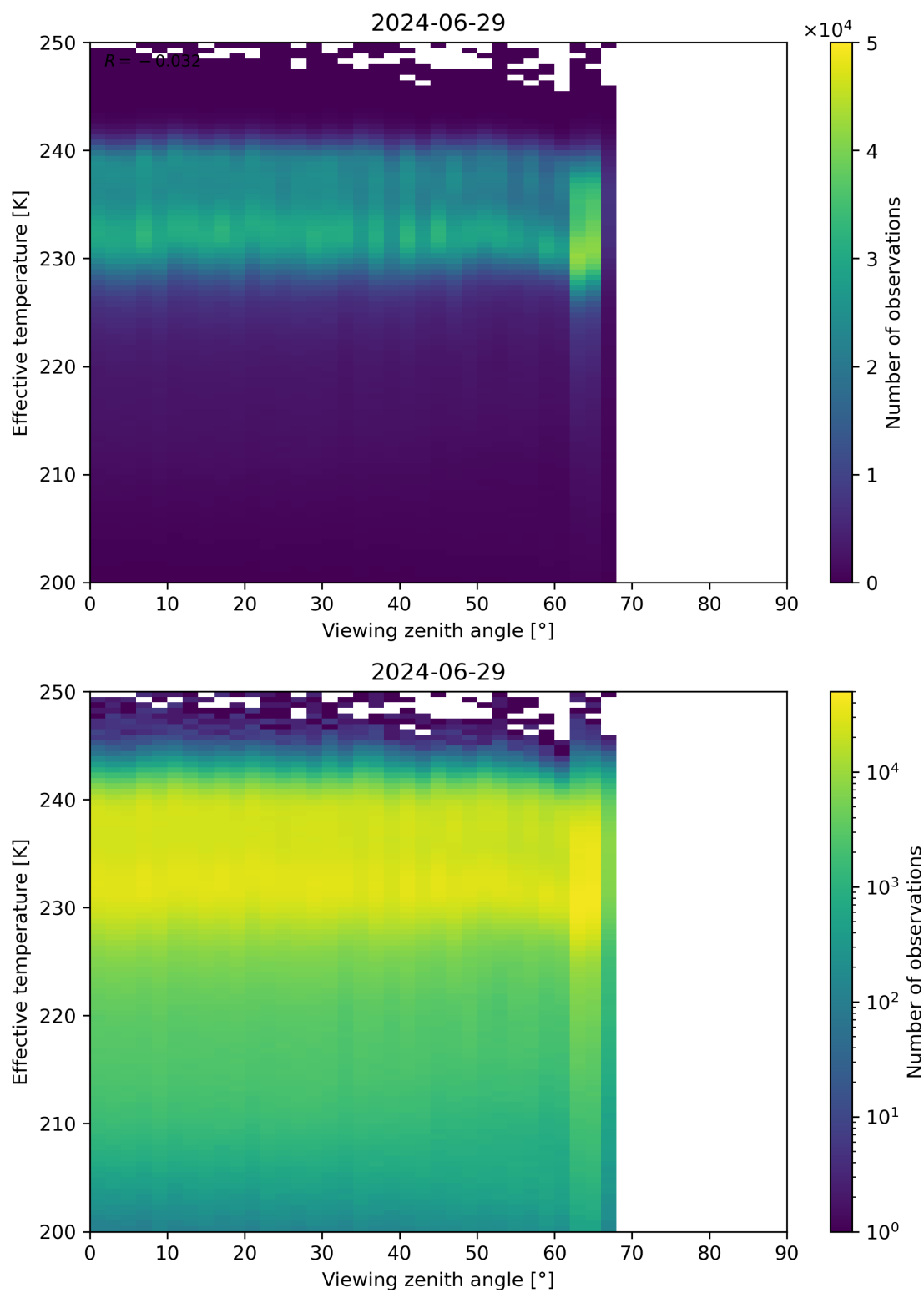
Figure 50: Scatter density plot of “Viewing zenith angle” against “Effective temperature” for 2024-06-29 to 2024-06-30.
