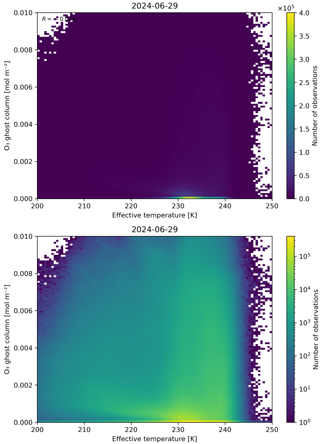
Figure 38: Scatter density plot of “Effective temperature” against “O 3 ghost column” for 2024-06-29 to 2024-06-30.
