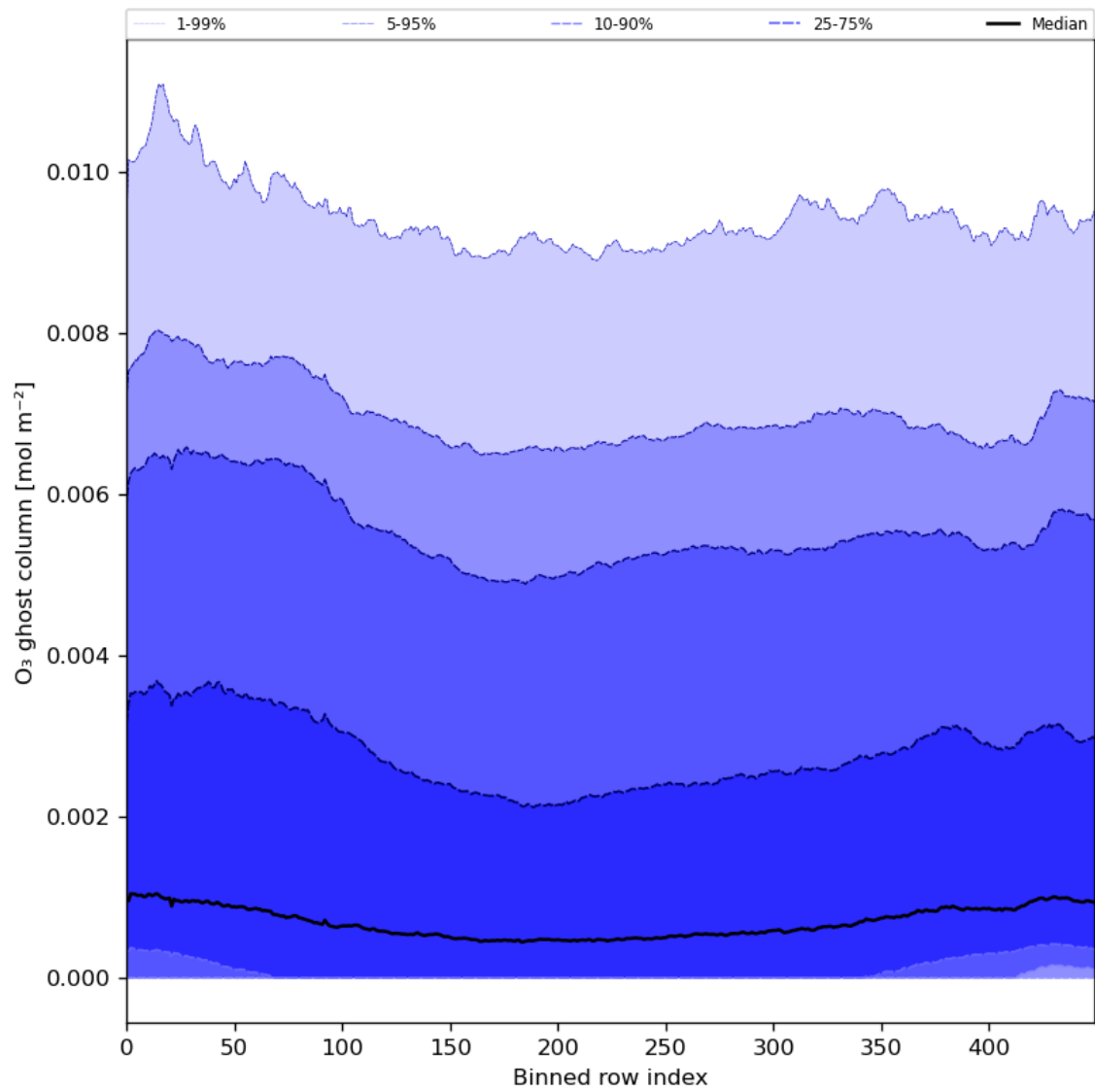
Figure 32: Along track statistics of “O 3 ghost column” for 2024-06-29 to 2024-07-01
