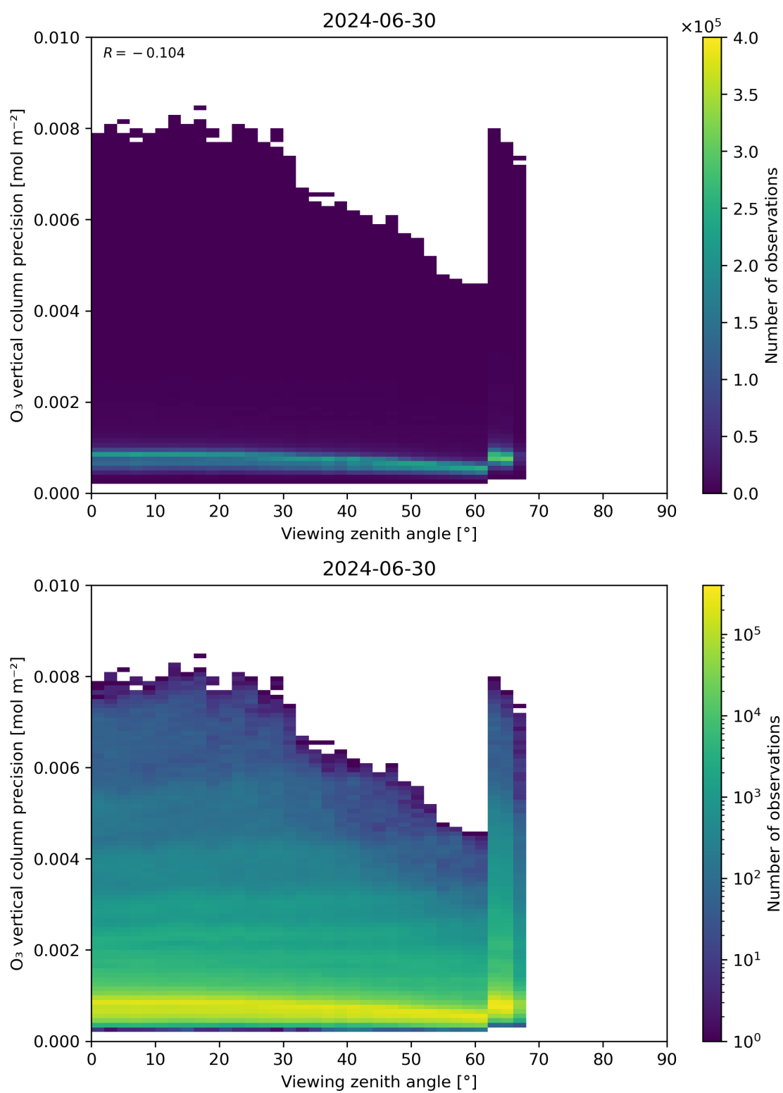
Figure 53: Scatter density plot of “Viewing zenith angle” against “O 3 vertical column precision” for 2024-06-29 to 2024-07-01.
