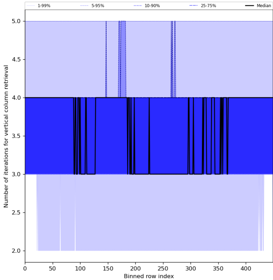
Figure 33: Along track statistics of “Number of iterations for vertical column retrieval” for 2024-06-29 to 2024-07-01
