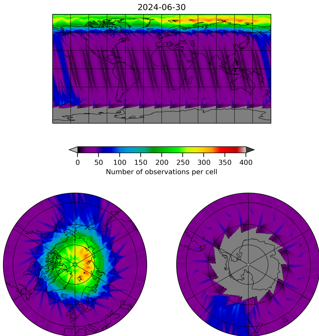
Figure 12: Map of the number of observations for 2024-06-29 to 2024-07-01
