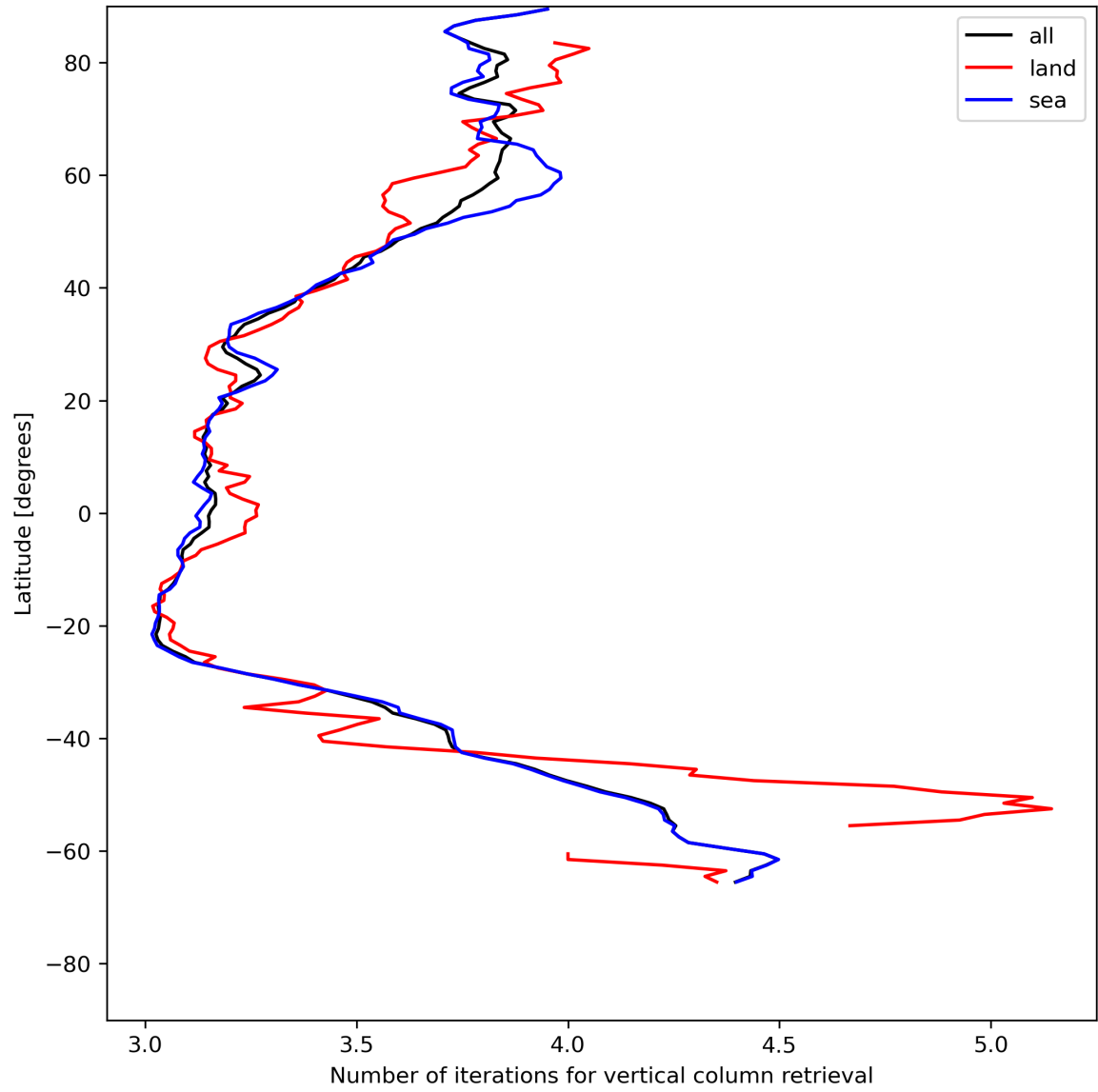
Figure 19: Zonal average of “Number of iterations for vertical column retrieval” for 2024-06-29 to 2024-07-01.
