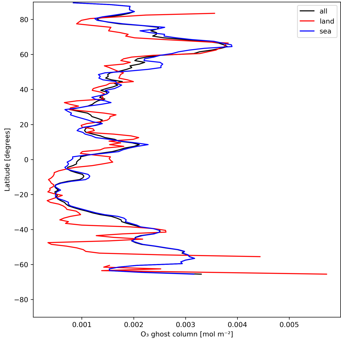
Figure 18: Zonal average of “O 3 ghost column” for 2024-06-29 to 2024-07-01.
