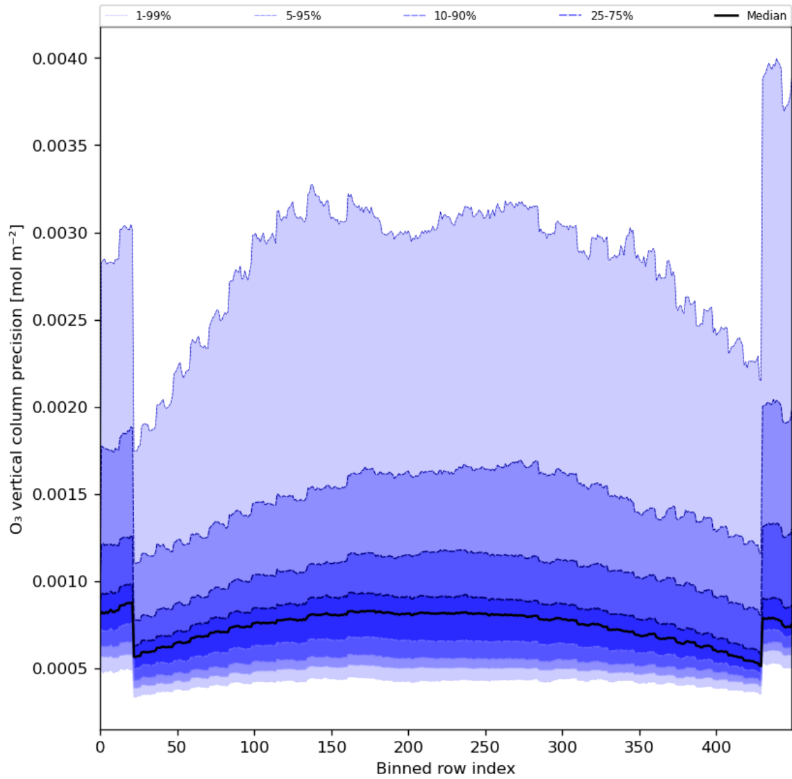
Figure 29: Along track statistics of “O 3 vertical column precision” for 2024-06-29 to 2024-07-01
