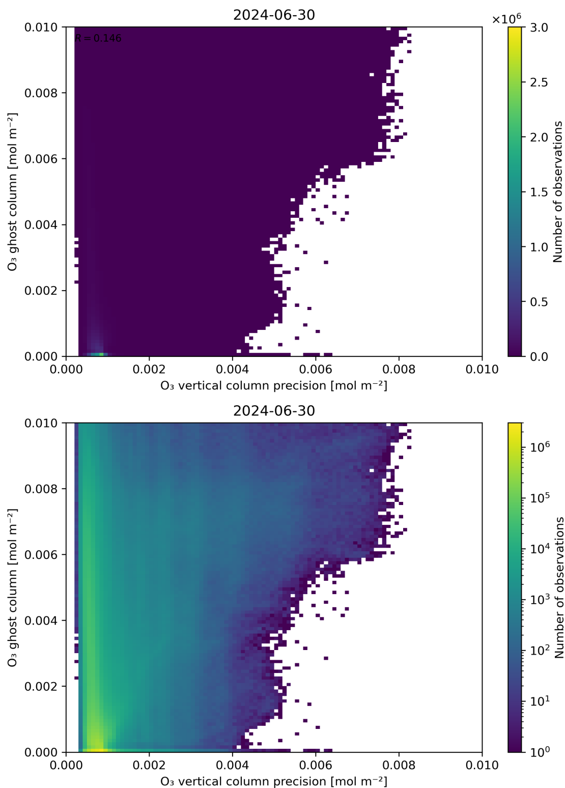
Figure 43: Scatter density plot of “ \text{O}_3 vertical column precision” against “ \text{O}_3 ghost column” for 2024-06-29 to 2024-07-01.
