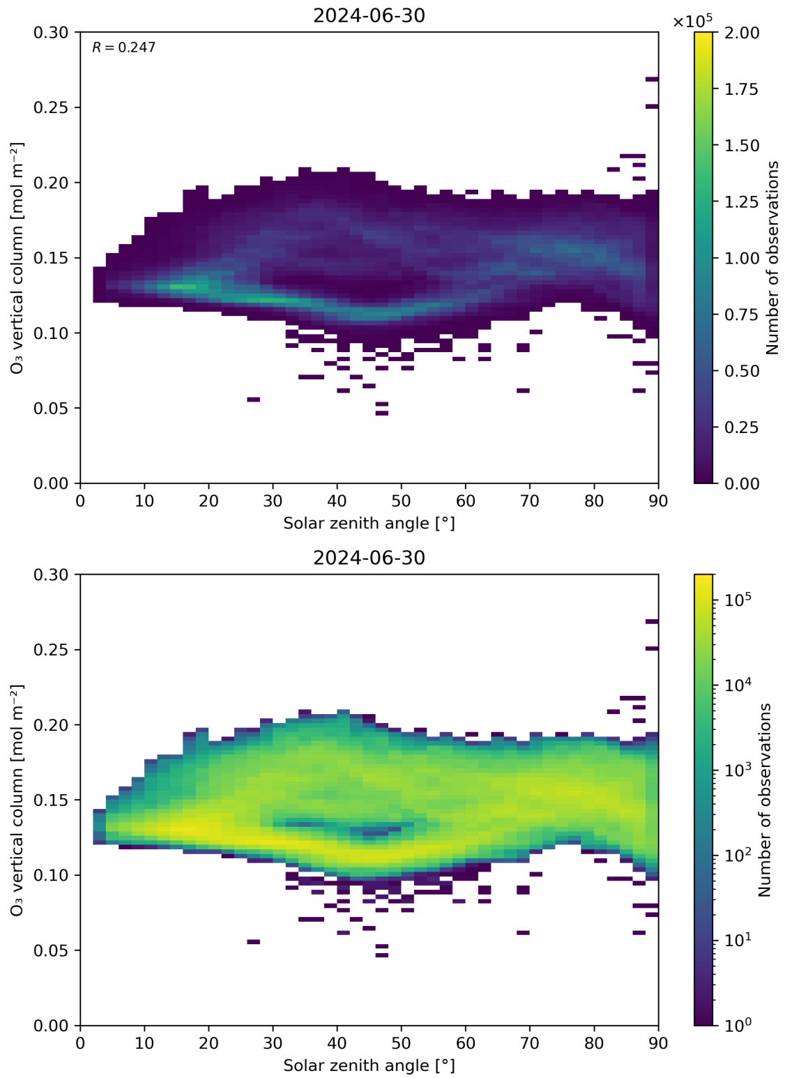
Figure 47: Scatter density plot of “Solar zenith angle” against “O 3 vertical column” for 2024-06-29 to 2024-07-01.
