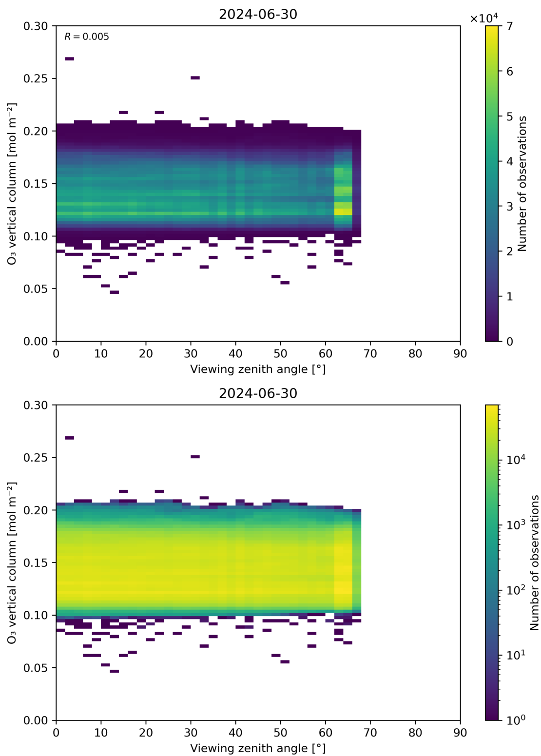
Figure 52: Scatter density plot of “Viewing zenith angle” against “O 3 vertical column” for 2024-06-29 to 2024-07-01.
