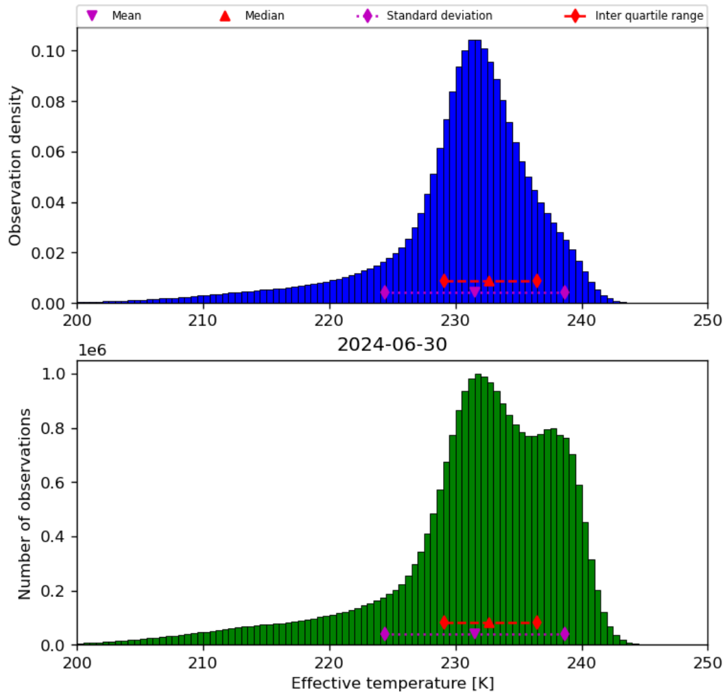
Figure 24: Histogram of “Effective temperature” for 2024-06-29 to 2024-07-01
