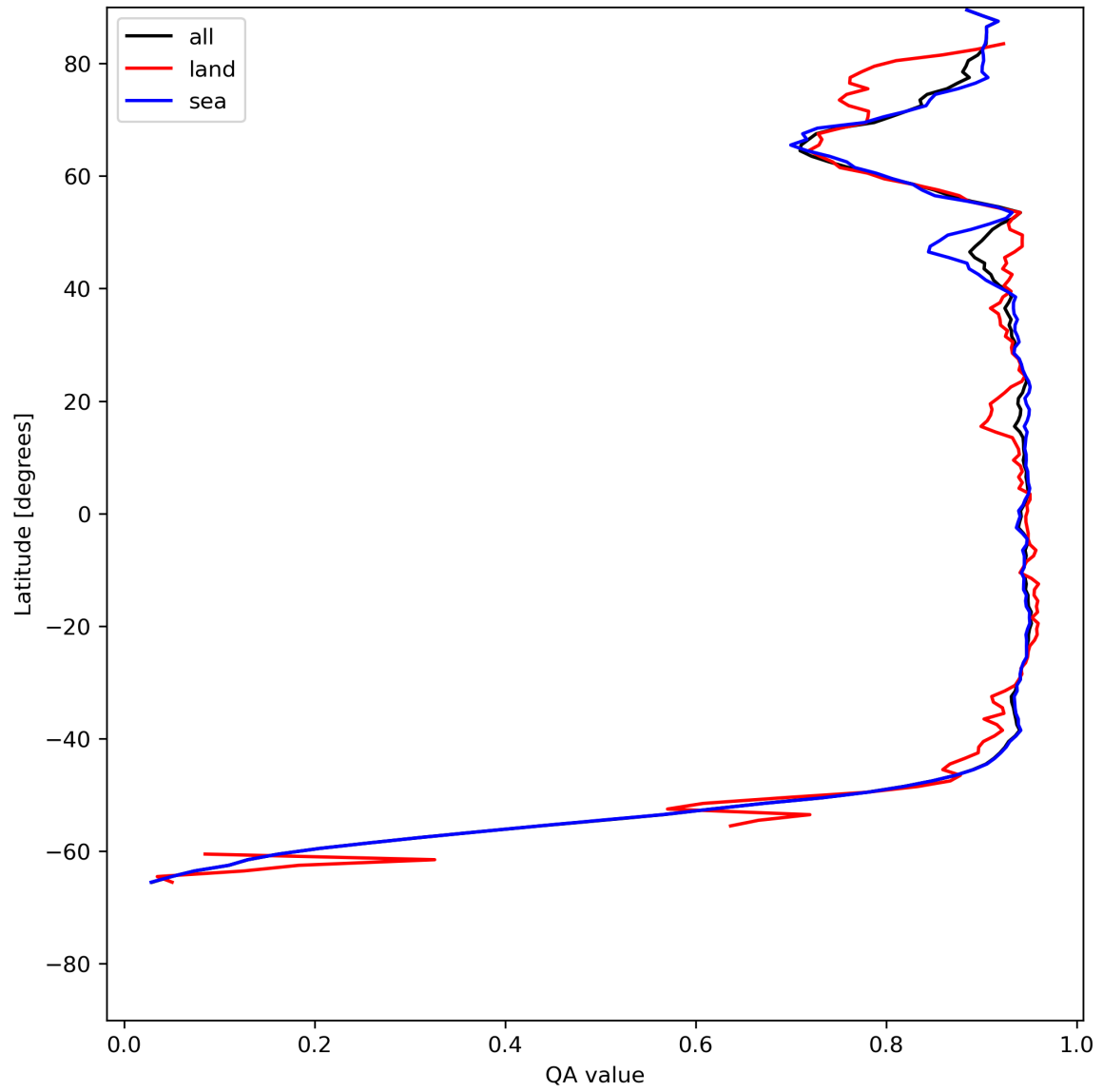
Figure 13: Zonal average of “QA value” for 2024-06-29 to 2024-07-01.
