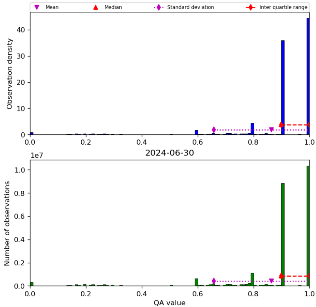
Figure 20: Histogram of “QA value” for 2024-06-29 to 2024-07-01
