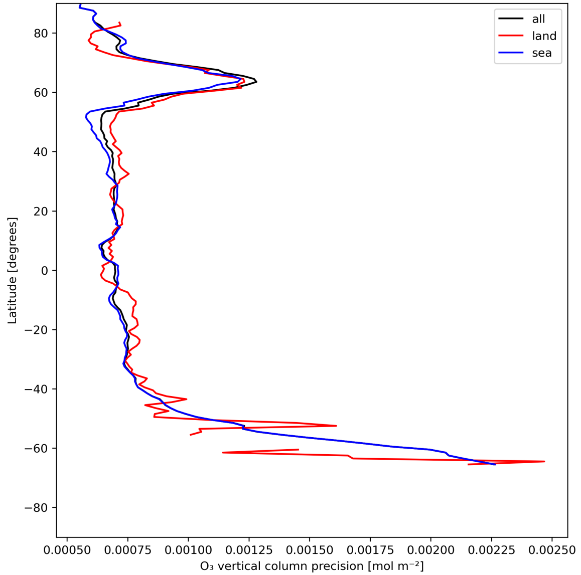
Figure 15: Zonal average of “O 3 vertical column precision” for 2024-06-29 to 2024-07-01.
