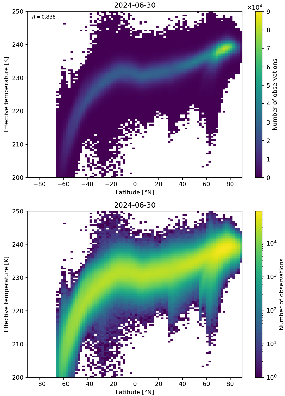
Figure 34: Scatter density plot of “Latitude” against “Effective temperature” for 2024-06-29 to 2024-07-01.
