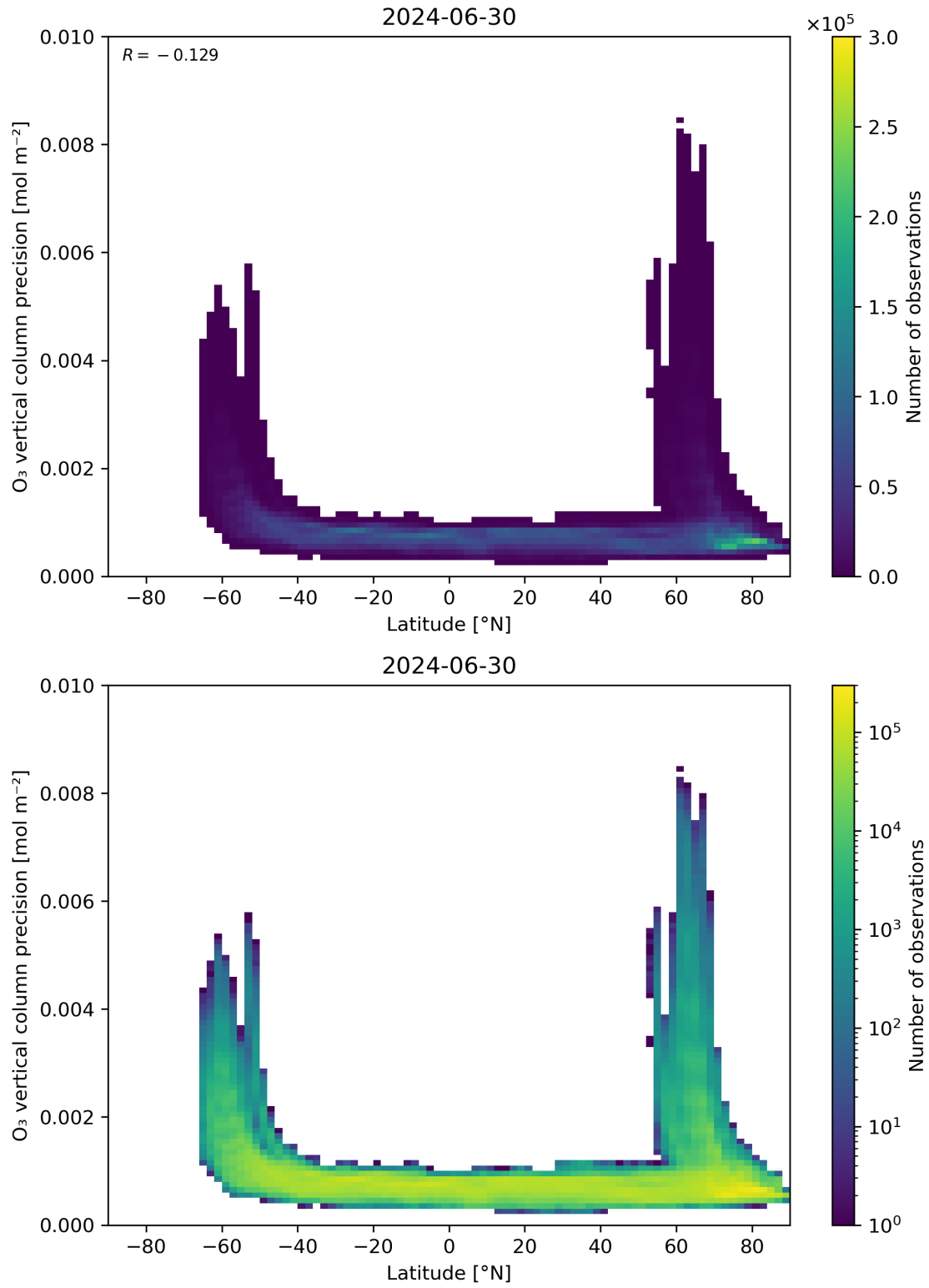
Figure 37: Scatter density plot of “Latitude” against “O 3 vertical column precision” for 2024-06-29 to 2024-07-01.
