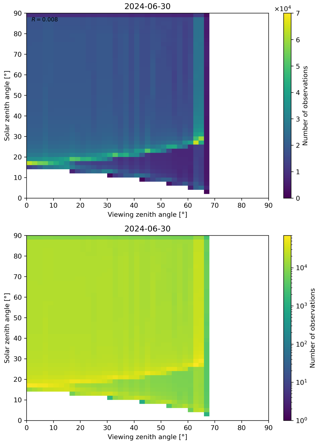
Figure 54: Scatter density plot of “Viewing zenith angle” against “Solar zenith angle” for 2024-06-29 to 2024-07-01.
