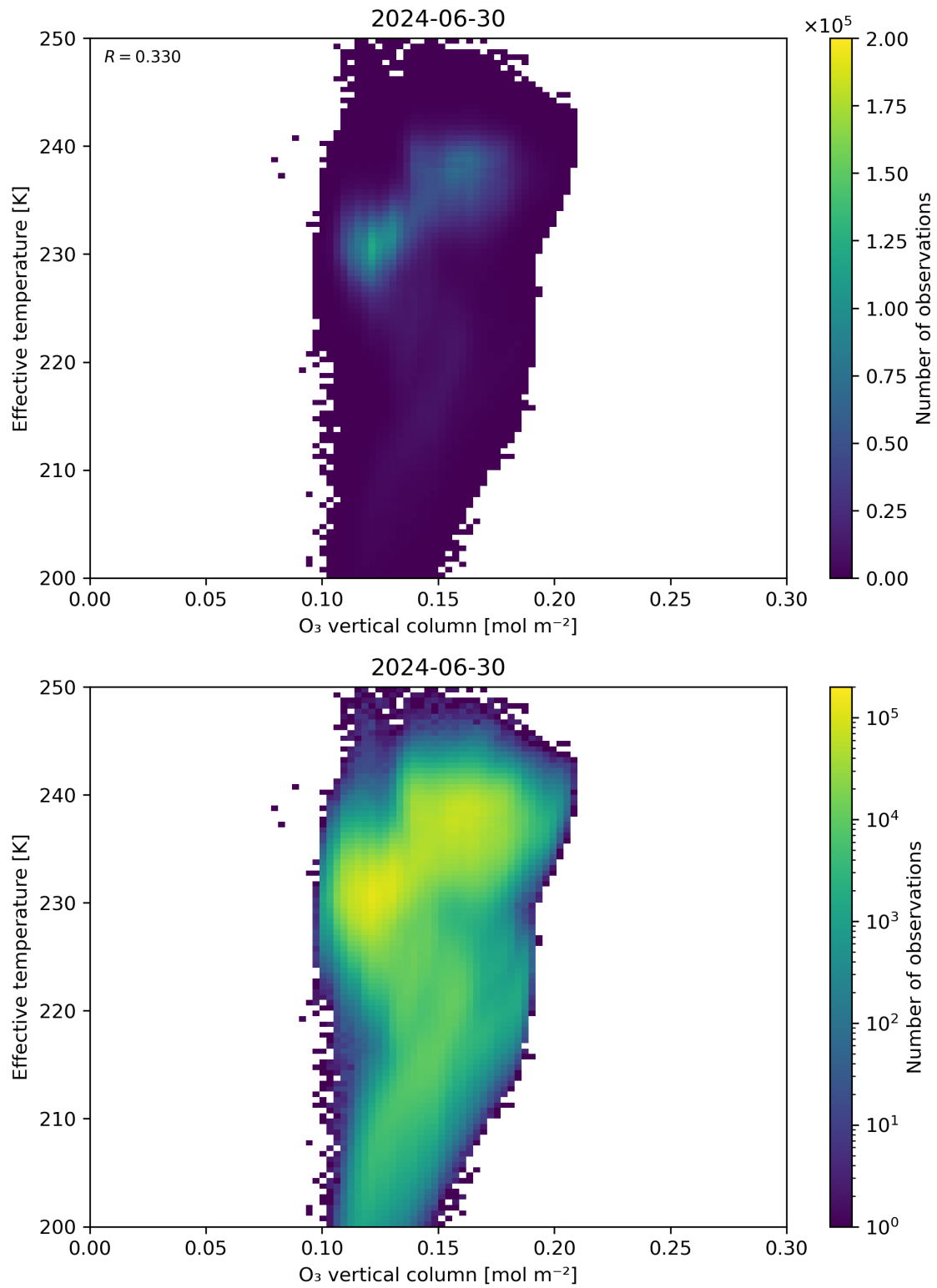
Figure 39: Scatter density plot of “O 3 vertical column” against “Effective temperature” for 2024-06-29 to 2024-07-01.
