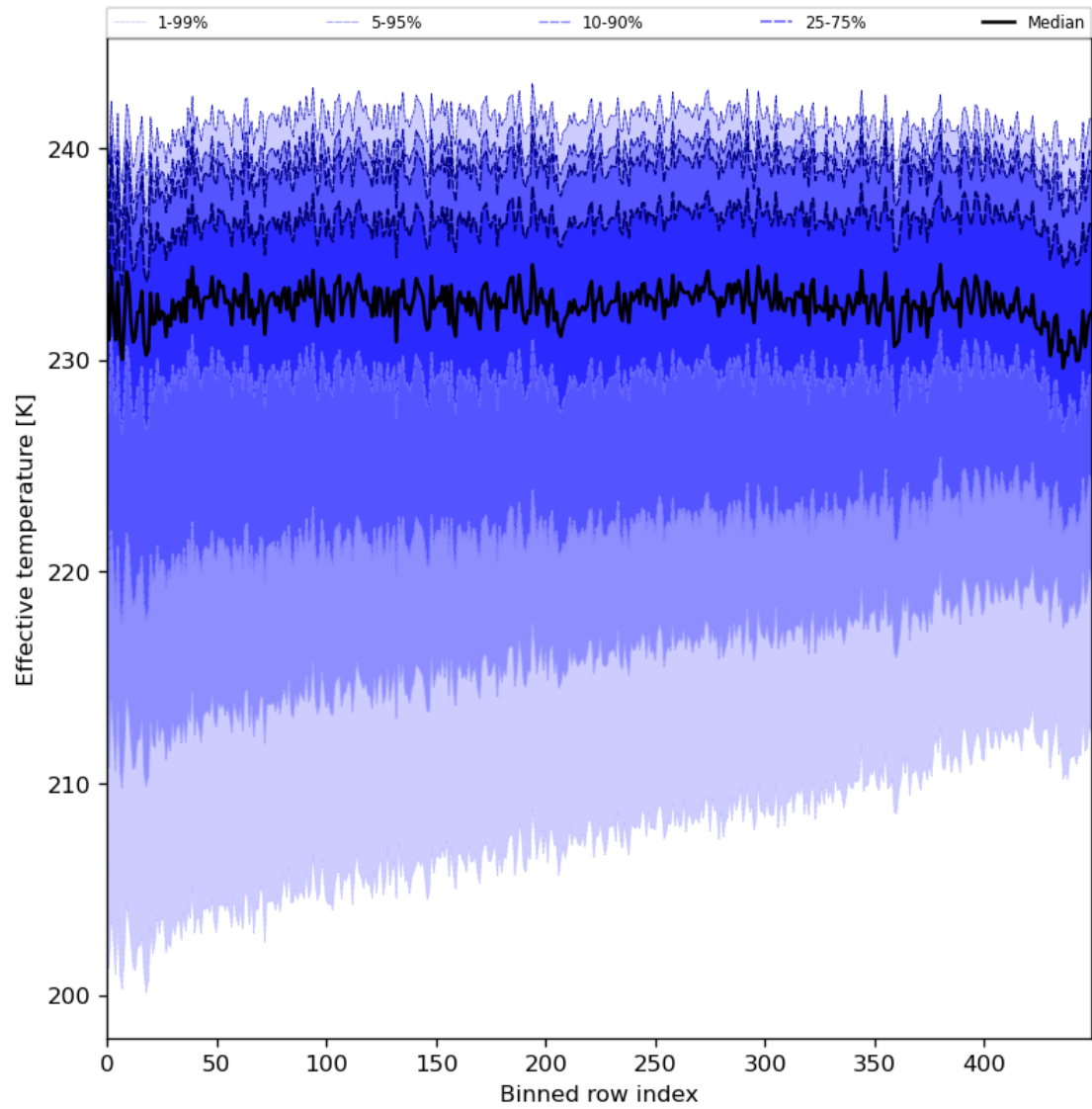
Figure 31: Along track statistics of “Effective temperature” for 2024-06-29 to 2024-07-01
