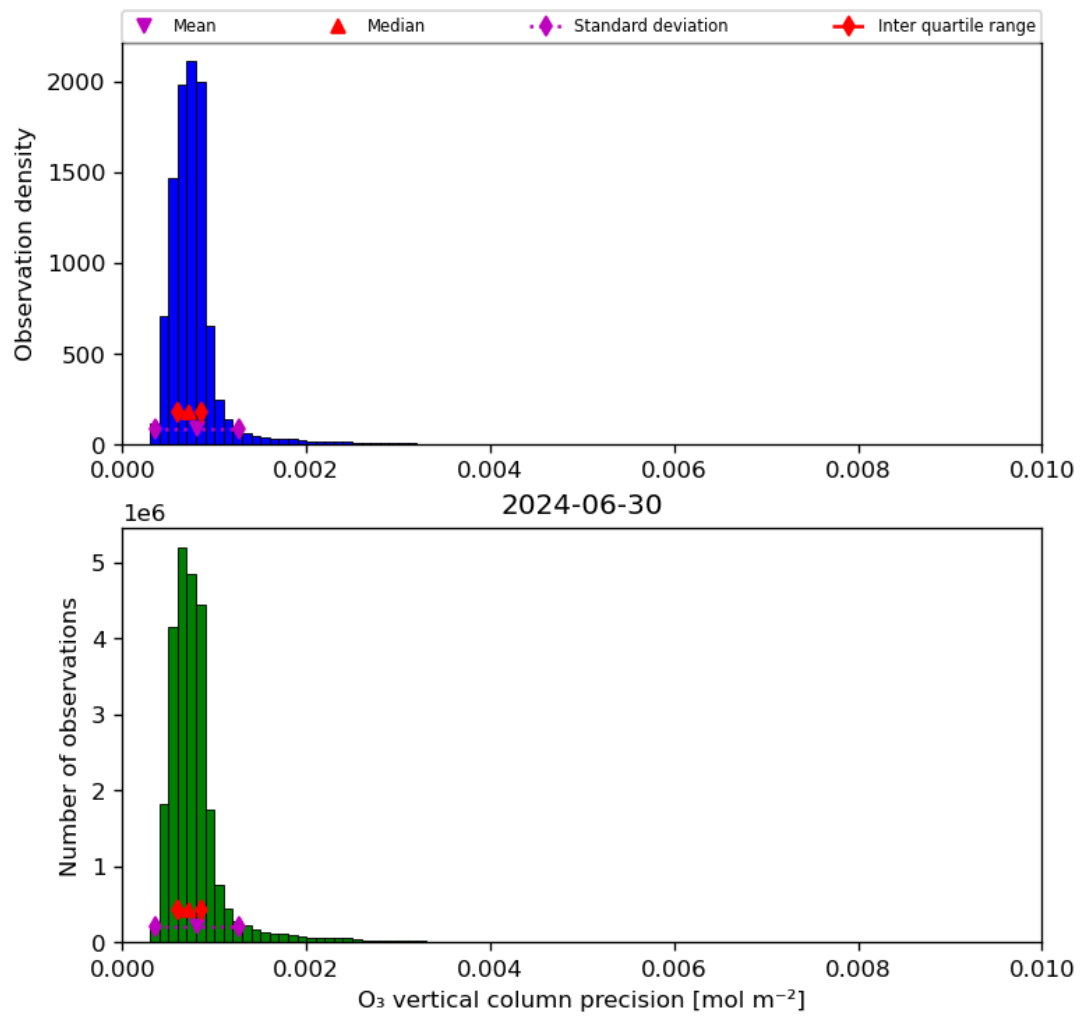
Figure 22: Histogram of “O 3 vertical column precision” for 2024-06-29 to 2024-07-01
