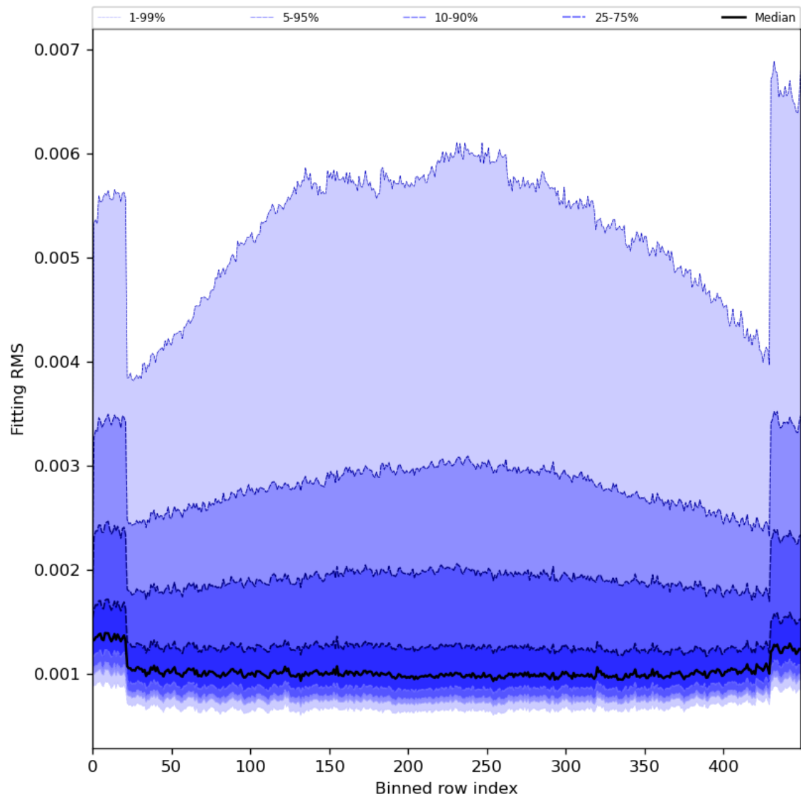
Figure 30: Along track statistics of “Fitting RMS” for 2024-06-29 to 2024-07-01
