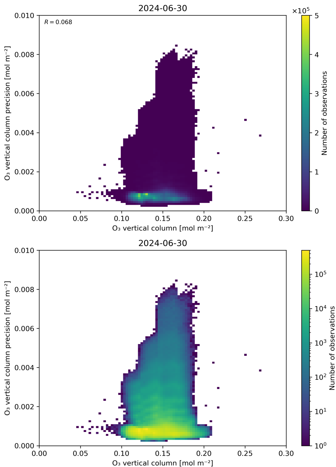
Figure 41: Scatter density plot of “O 3 vertical column” against “O 3 vertical column precision” for 2024-06-29 to 2024-07-01.
