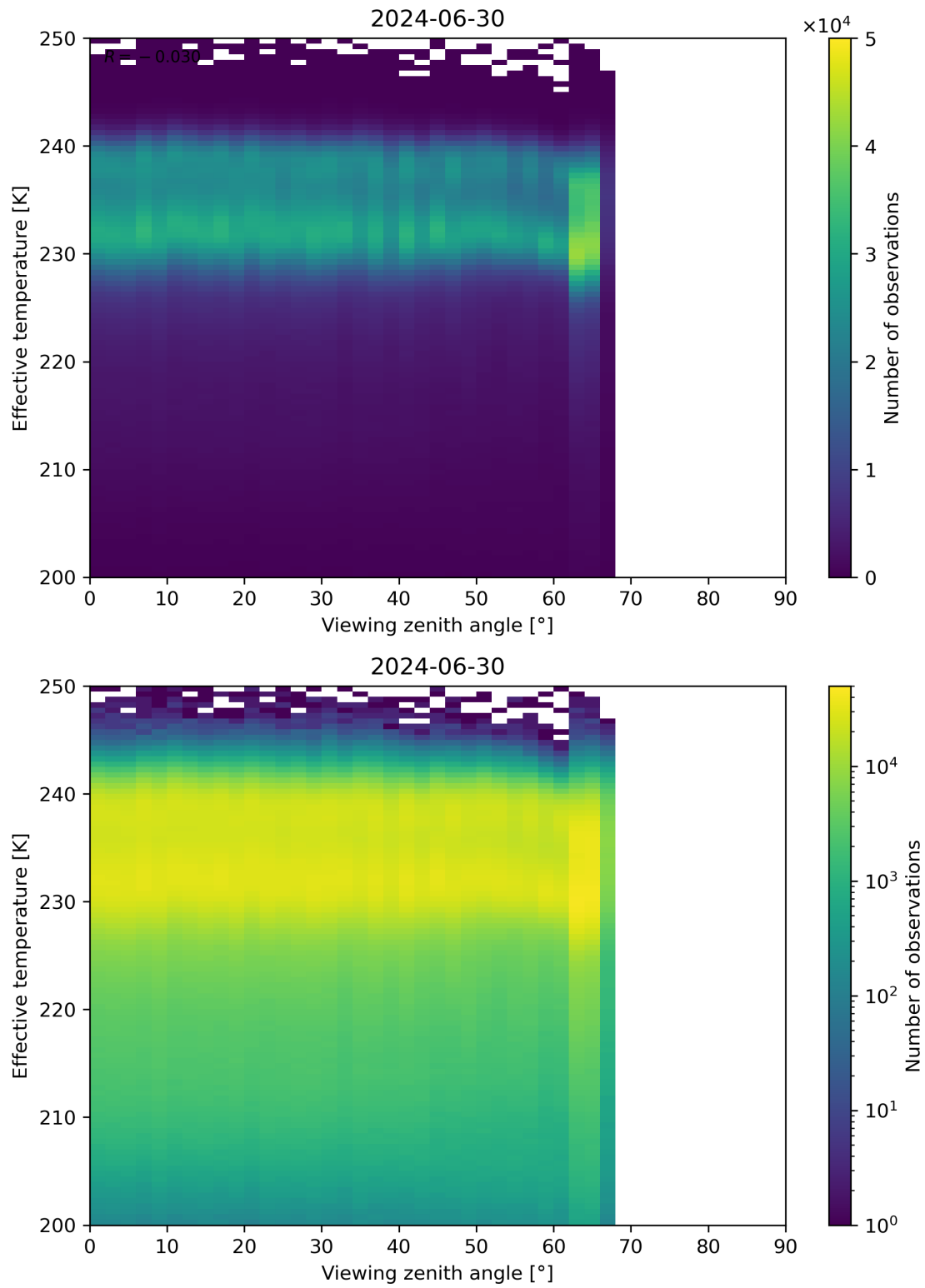
Figure 50: Scatter density plot of “Viewing zenith angle” against “Effective temperature” for 2024-06-29 to 2024-07-01.
