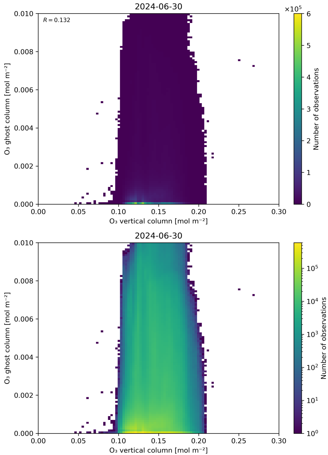
Figure 40: Scatter density plot of “O 3 vertical column” against “O 3 ghost column” for 2024-06-29 to 2024-07-01.
