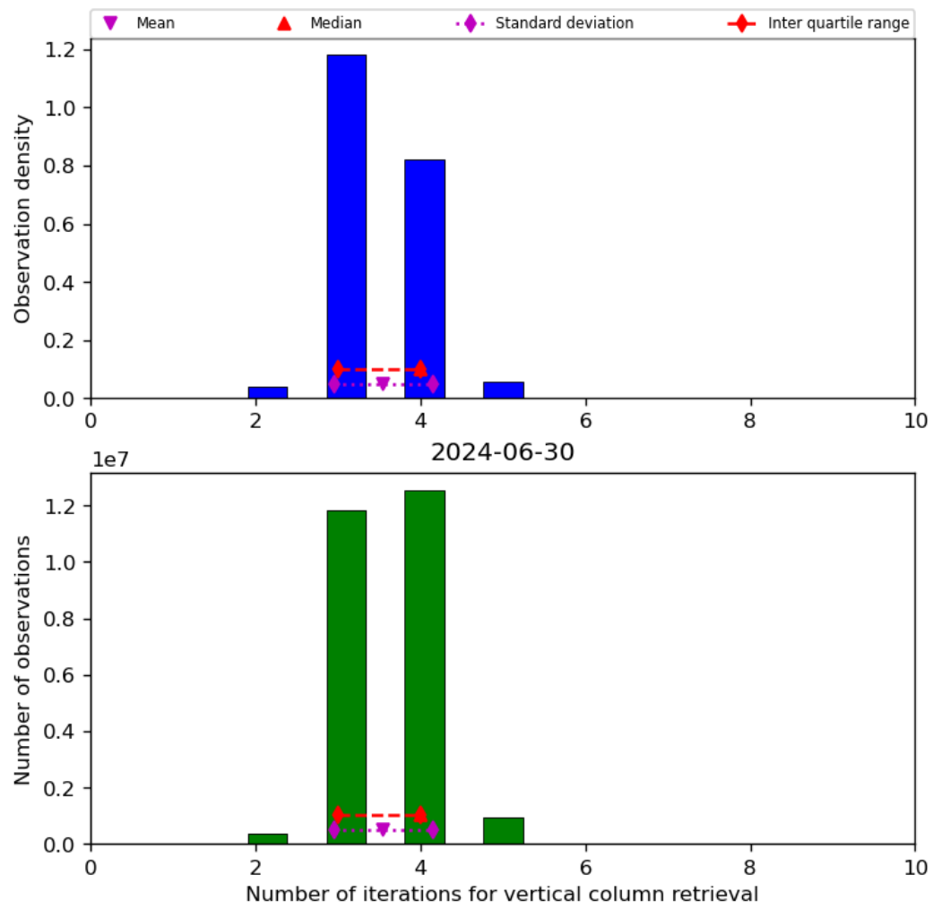
Figure 26: Histogram of “Number of iterations for vertical column retrieval” for 2024-06-29 to 2024-07-01
