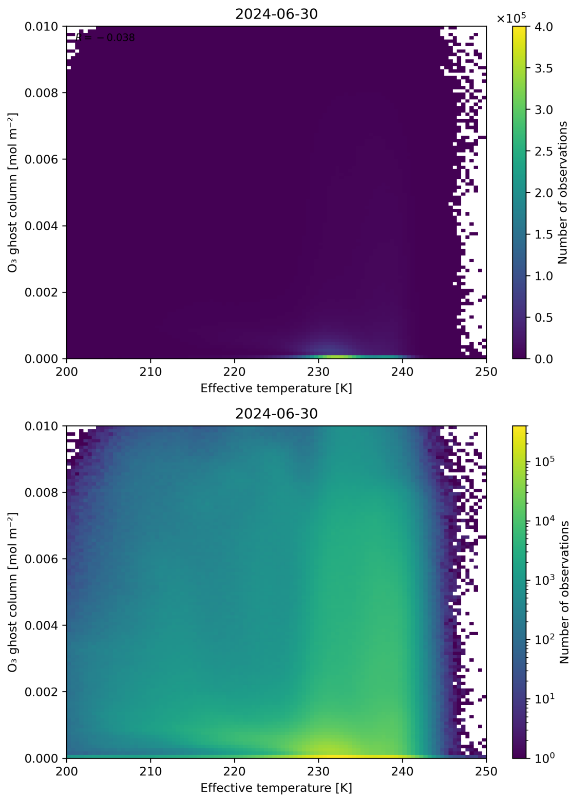
Figure 38: Scatter density plot of “Effective temperature” against “O 3 ghost column” for 2024-06-29 to 2024-07-01.
