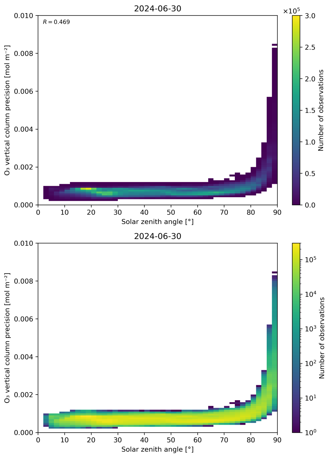
Figure 48: Scatter density plot of “Solar zenith angle” against “O 3 vertical column precision” for 2024-06-29 to 2024-07-01.
