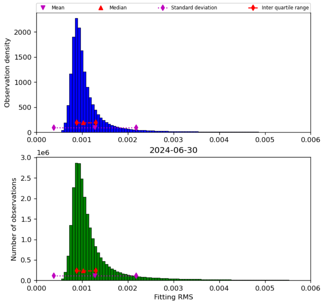
Figure 23: Histogram of “Fitting RMS” for 2024-06-29 to 2024-07-01
