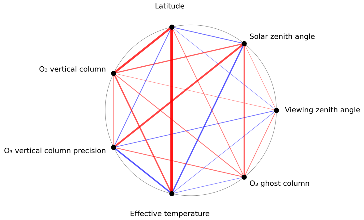
Figure 1: Map of correlation graph for 2024-06-29 to 2024-07-01.
