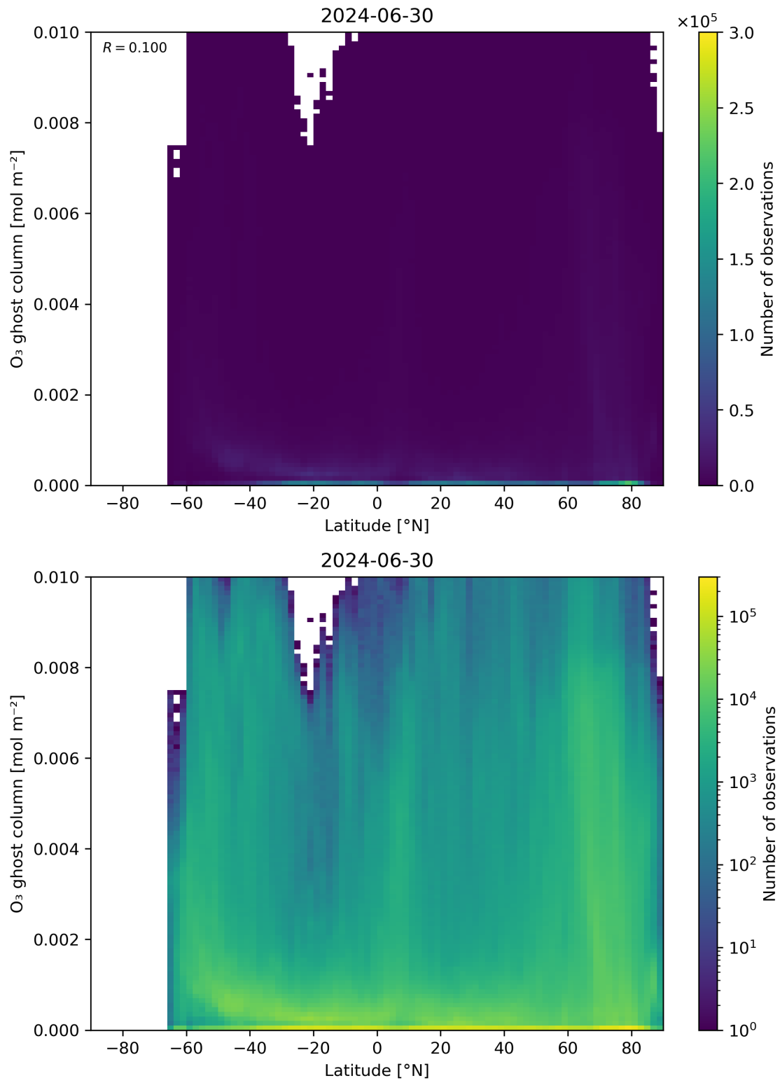
Figure 35: Scatter density plot of “Latitude” against “O 3 ghost column” for 2024-06-29 to 2024-07-01.
