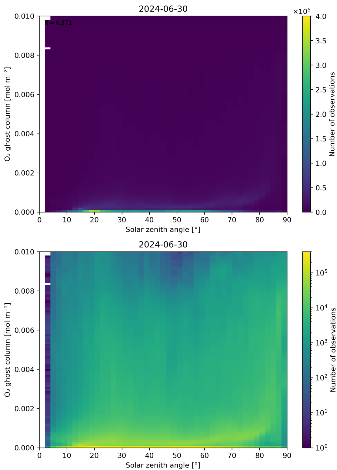
Figure 46: Scatter density plot of “Solar zenith angle” against “O 3 ghost column” for 2024-06-29 to 2024-07-01.
