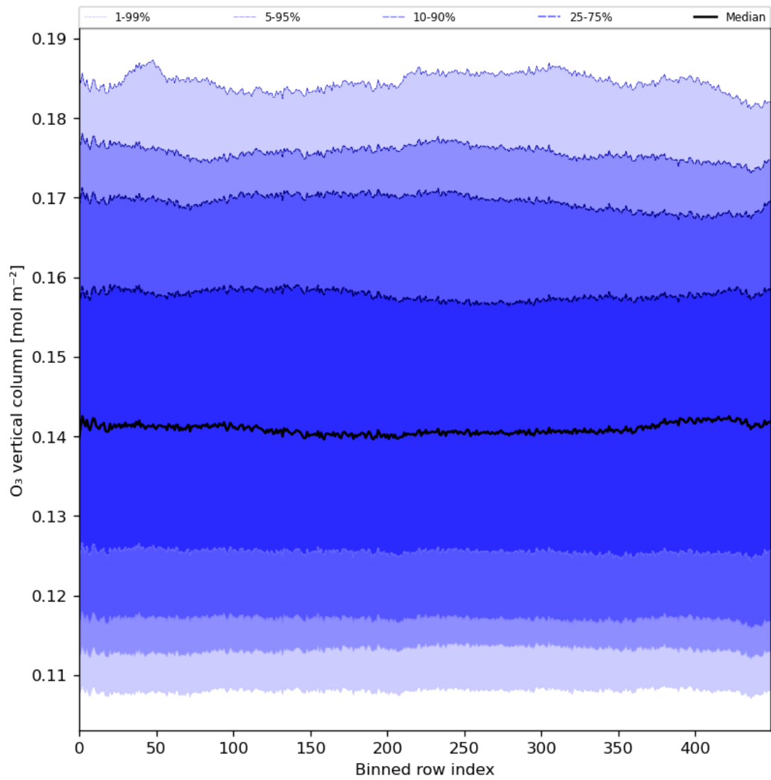
Figure 28: Along track statistics of “O 3 vertical column” for 2024-06-29 to 2024-07-01
