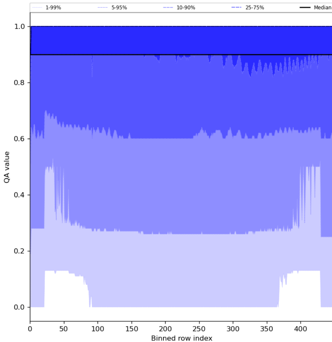
Figure 27: Along track statistics of “QA value” for 2024-06-29 to 2024-07-01
