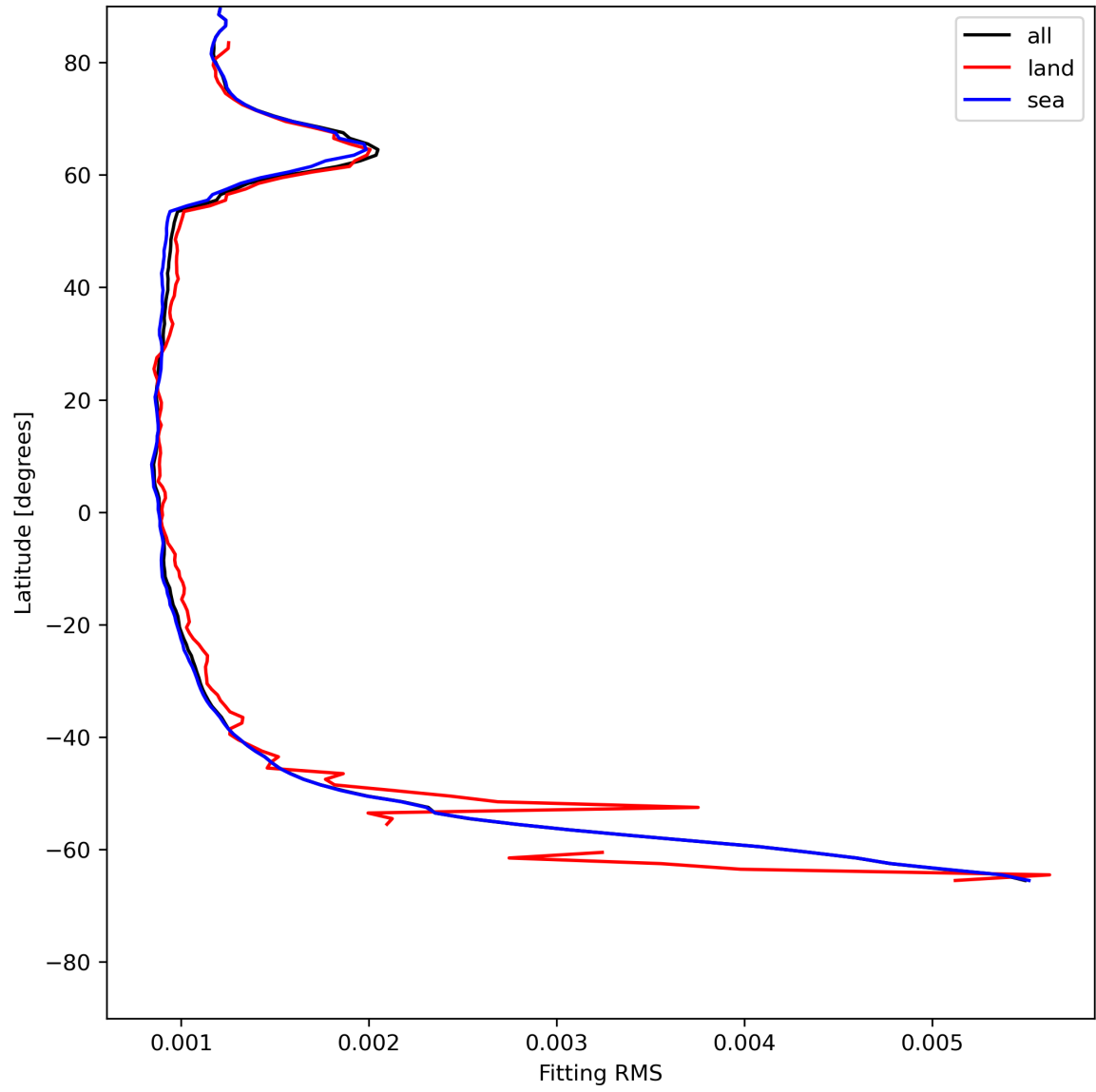
Figure 16: Zonal average of “Fitting RMS” for 2024-06-29 to 2024-07-01.
