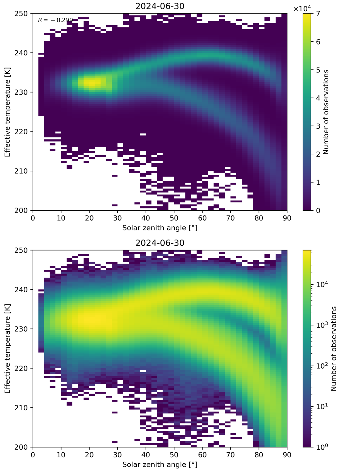
Figure 45: Scatter density plot of “Solar zenith angle” against “Effective temperature” for 2024-06-29 to 2024-07-01.
