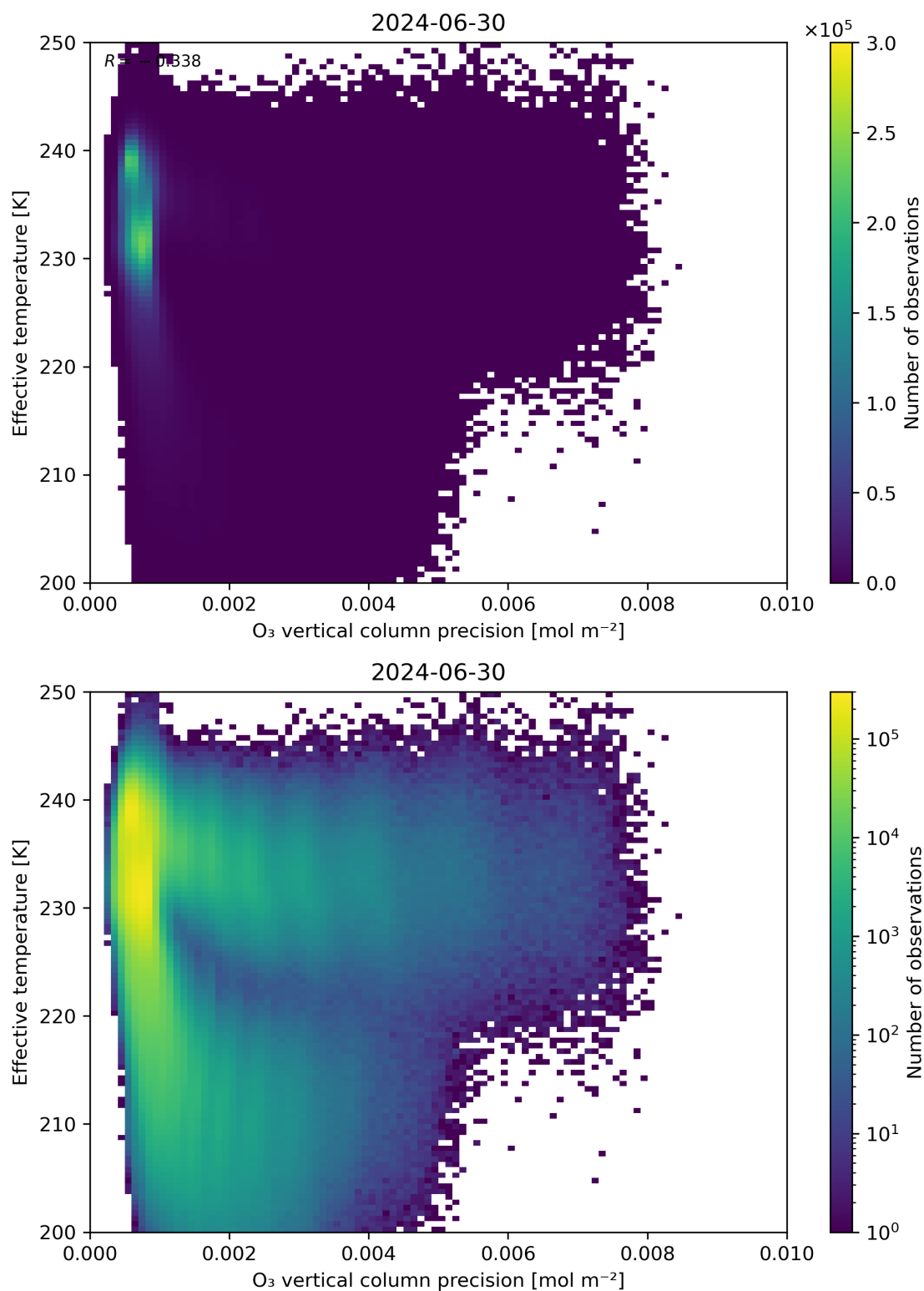
Figure 42: Scatter density plot of “O 3 vertical column precision” against “Effective temperature” for 2024-06-29 to 2024-07-01.
