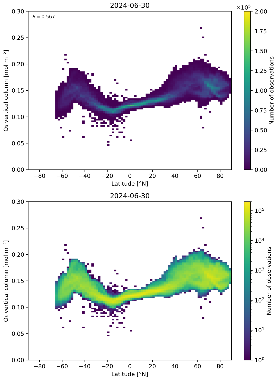
Figure 36: Scatter density plot of “Latitude” against “O 3 vertical column” for 2024-06-29 to 2024-07-01.
