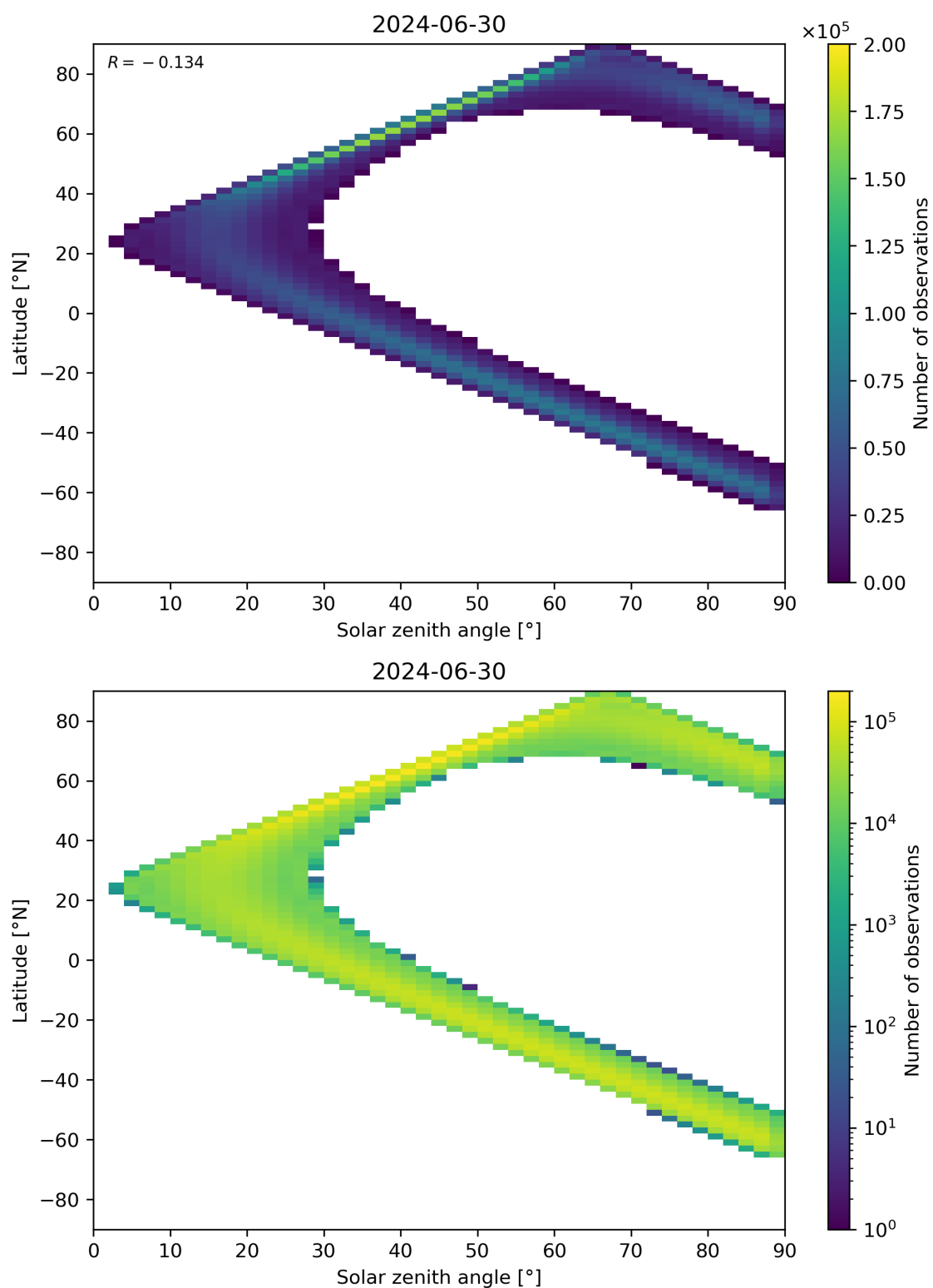
Figure 44: Scatter density plot of “Solar zenith angle” against “Latitude” for 2024-06-29 to 2024-07-01.
