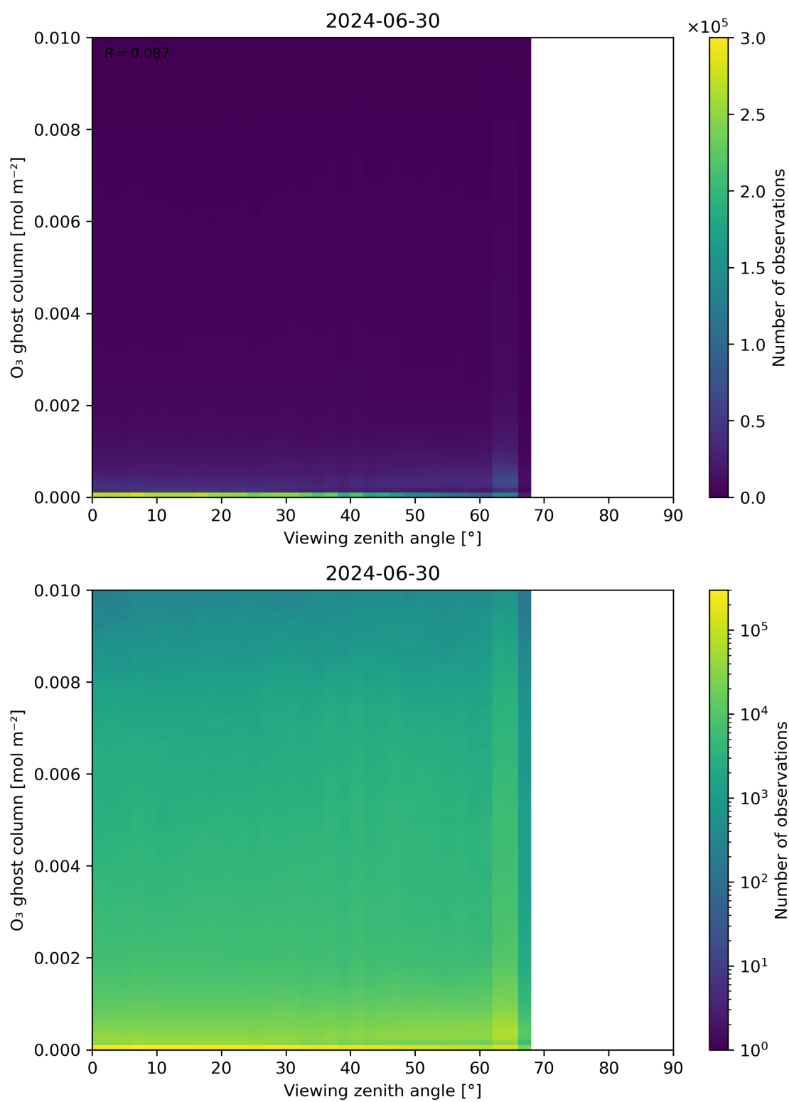
Figure 51: Scatter density plot of “Viewing zenith angle” against “O 3 ghost column” for 2024-06-29 to 2024-07-01.
