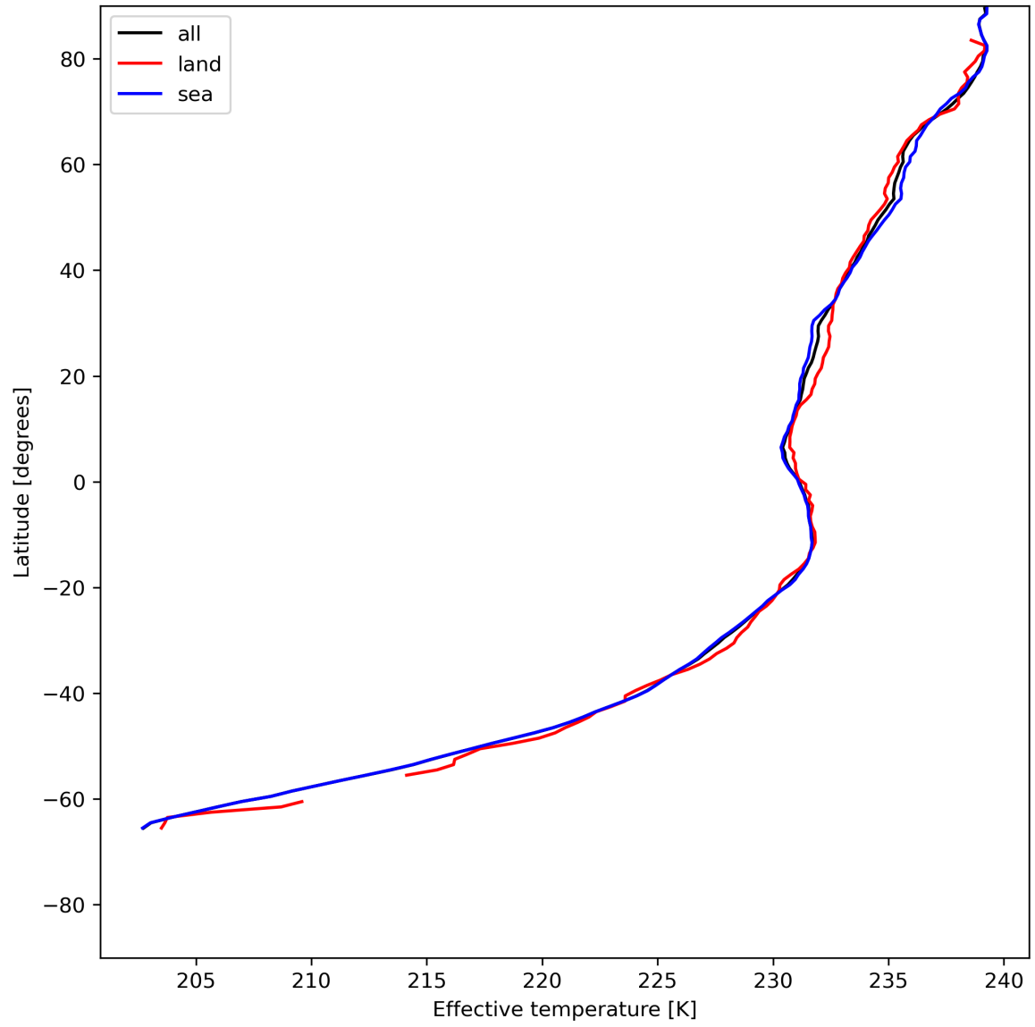
Figure 17: Zonal average of “Effective temperature” for 2024-06-29 to 2024-07-01.
