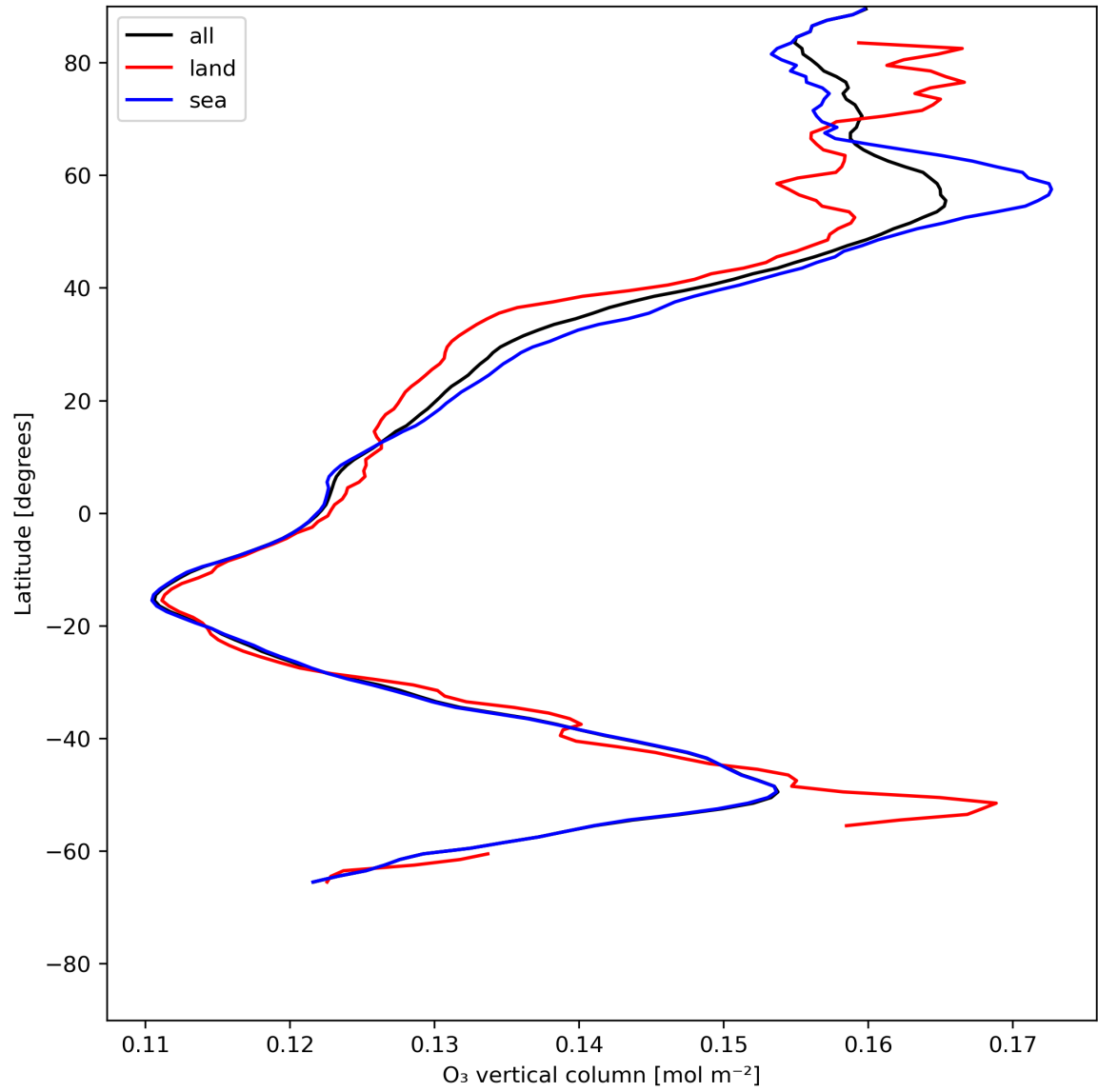
Figure 14: Zonal average of “O 3 vertical column” for 2024-06-29 to 2024-07-01.
