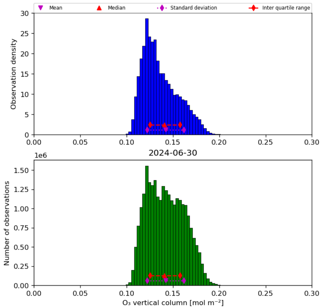
Figure 21: Histogram of “O 3 vertical column” for 2024-06-29 to 2024-07-01
