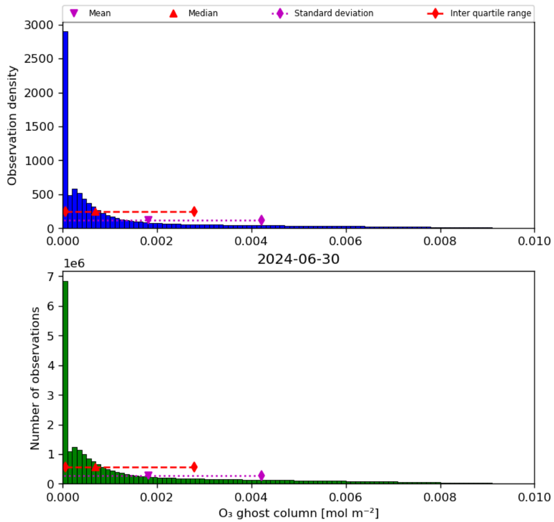
Figure 25: Histogram of “O 3 ghost column” for 2024-06-29 to 2024-07-01
