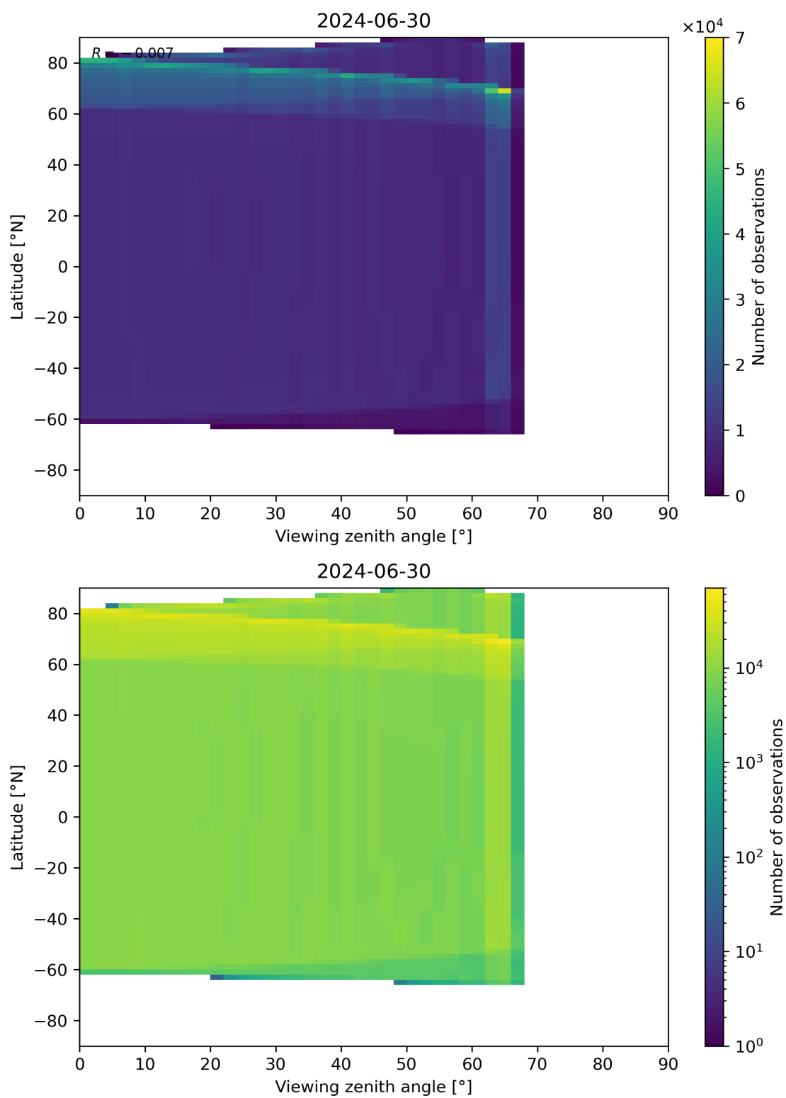
Figure 49: Scatter density plot of “Viewing zenith angle” against “Latitude” for 2024-06-29 to 2024-07-01.
