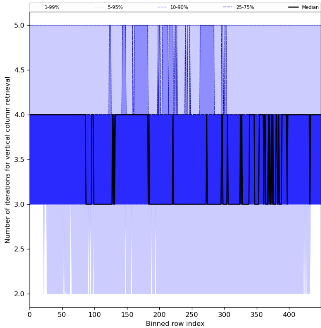
Figure 33: Along track statistics of “Number of iterations for vertical column retrieval” for 2024-06-30 to 2024-07-02
