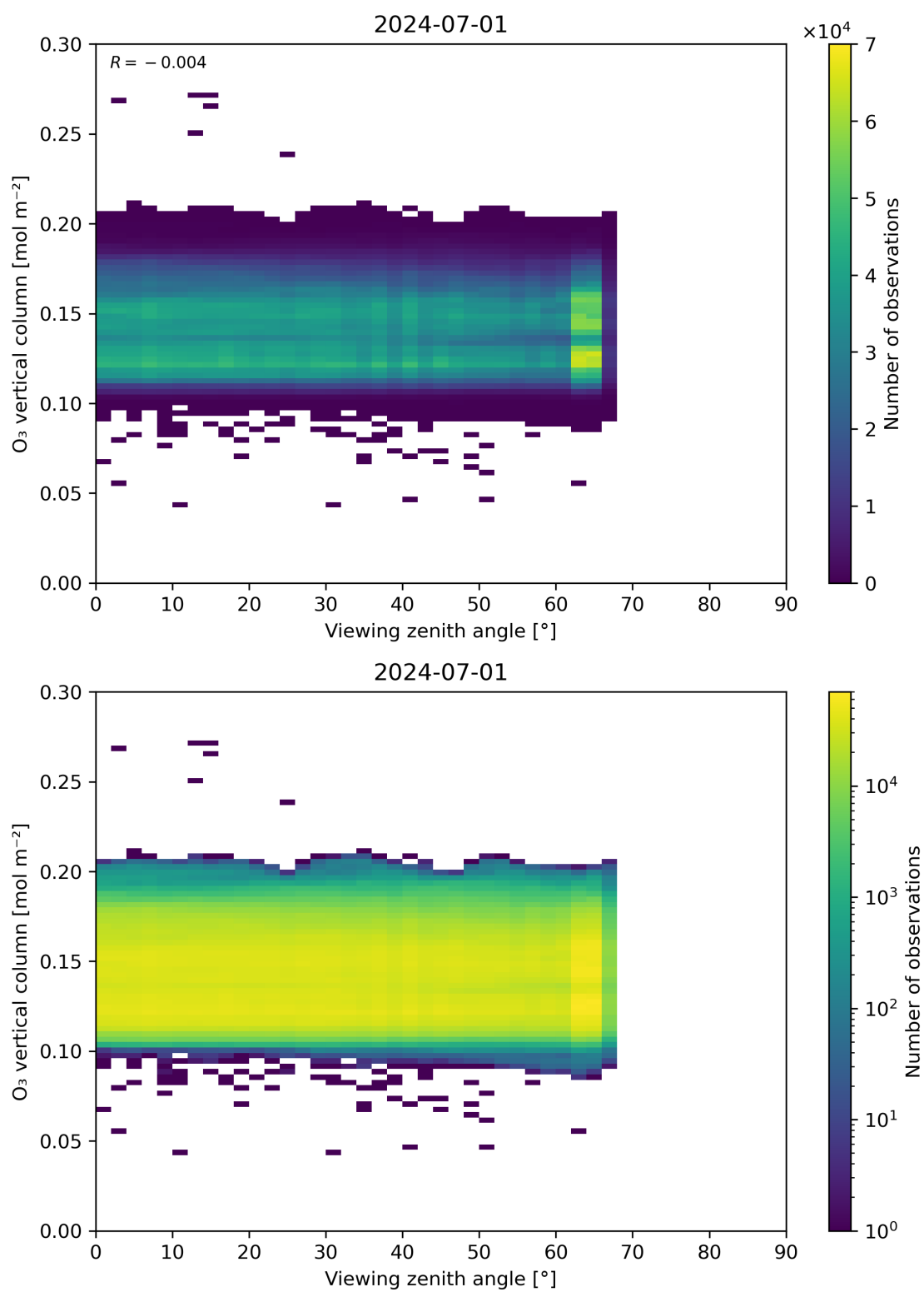
Figure 52: Scatter density plot of “Viewing zenith angle” against “O 3 vertical column” for 2024-06-30 to 2024-07-02.
