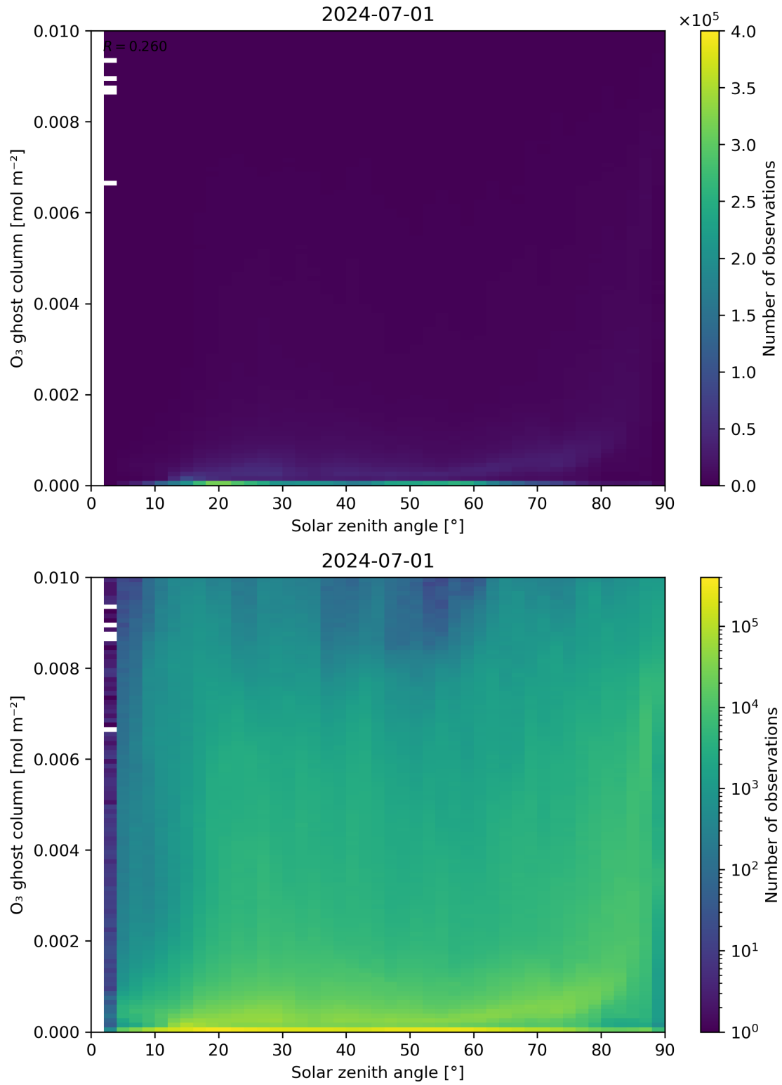
Figure 46: Scatter density plot of “Solar zenith angle” against “O 3 ghost column” for 2024-06-30 to 2024-07-02.
