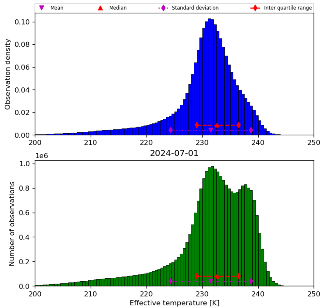
Figure 24: Histogram of “Effective temperature” for 2024-06-30 to 2024-07-02
