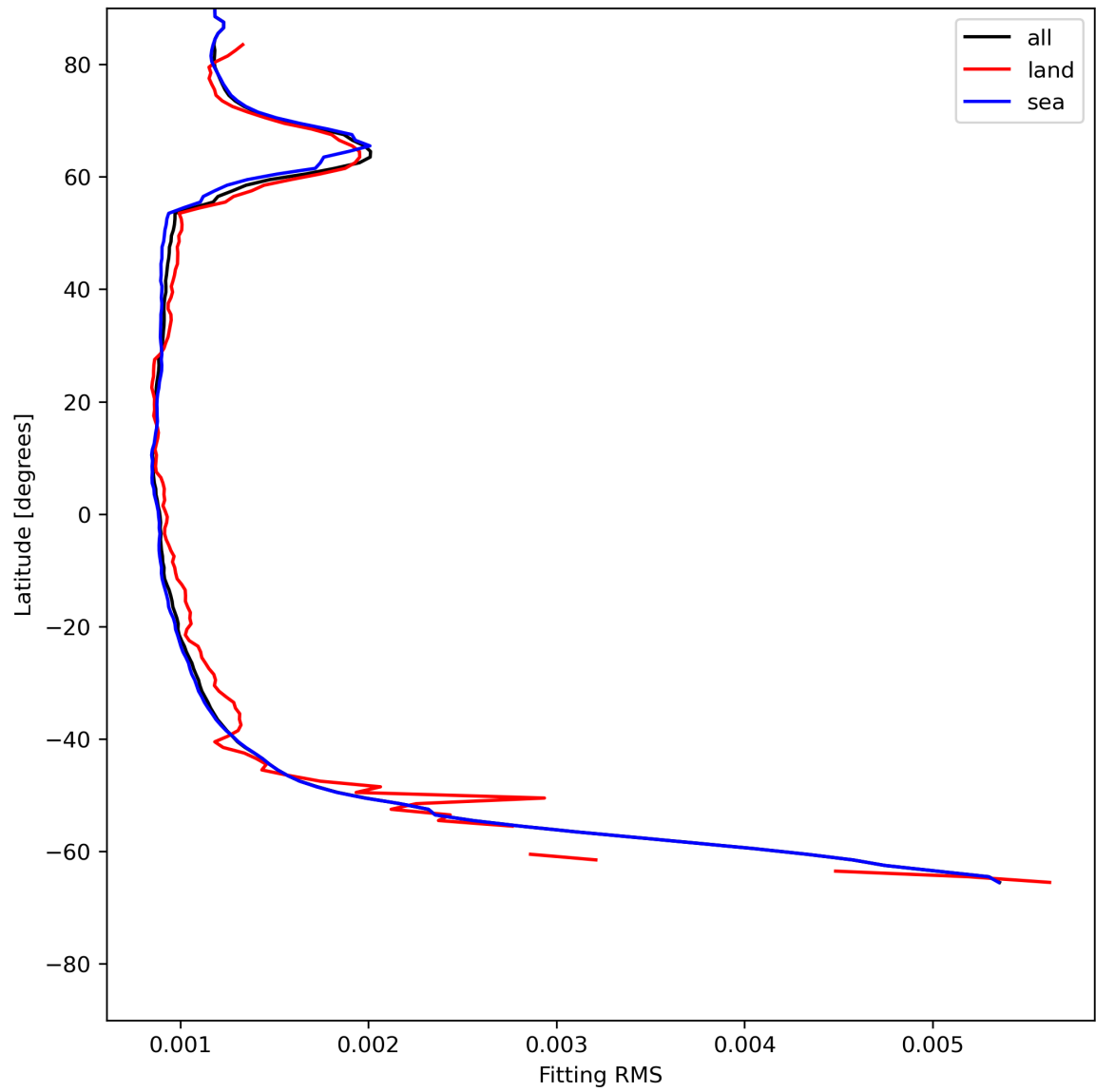
Figure 16: Zonal average of “Fitting RMS” for 2024-06-30 to 2024-07-02.
