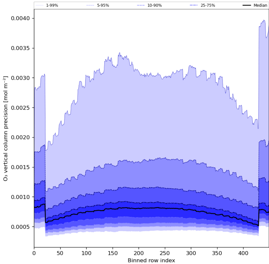
Figure 29: Along track statistics of “O 3 vertical column precision” for 2024-06-30 to 2024-07-02
