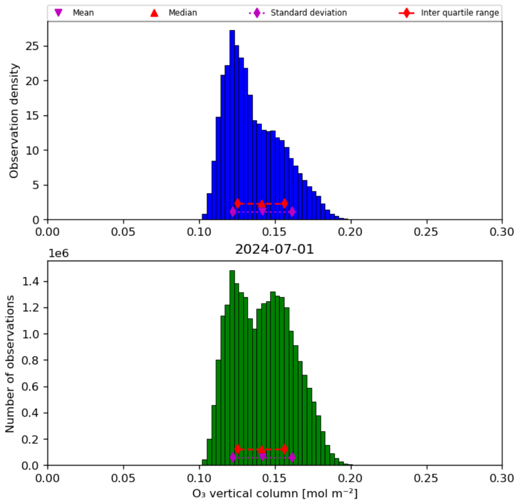
Figure 21: Histogram of “O 3 vertical column” for 2024-06-30 to 2024-07-02
