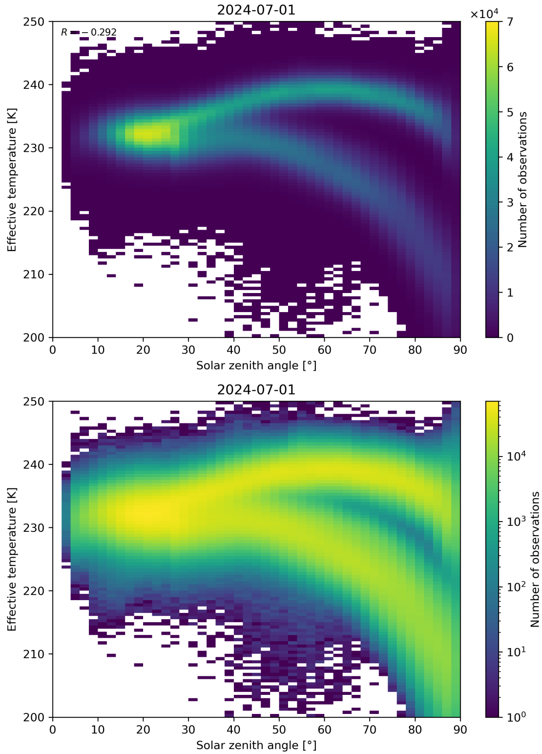
Figure 45: Scatter density plot of “Solar zenith angle” against “Effective temperature” for 2024-06-30 to 2024-07-02.
