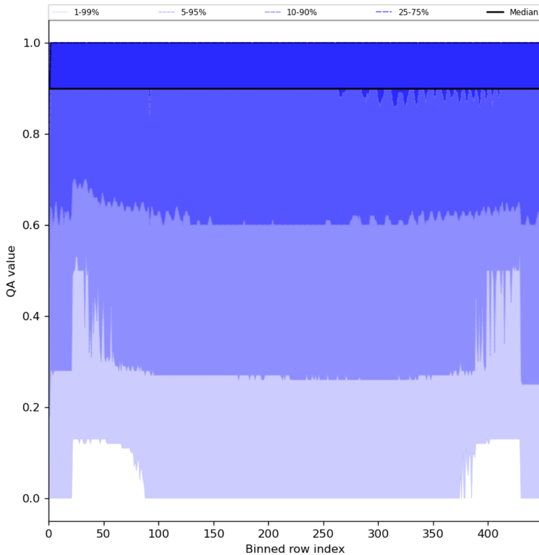
Figure 27: Along track statistics of “QA value” for 2024-06-30 to 2024-07-02
