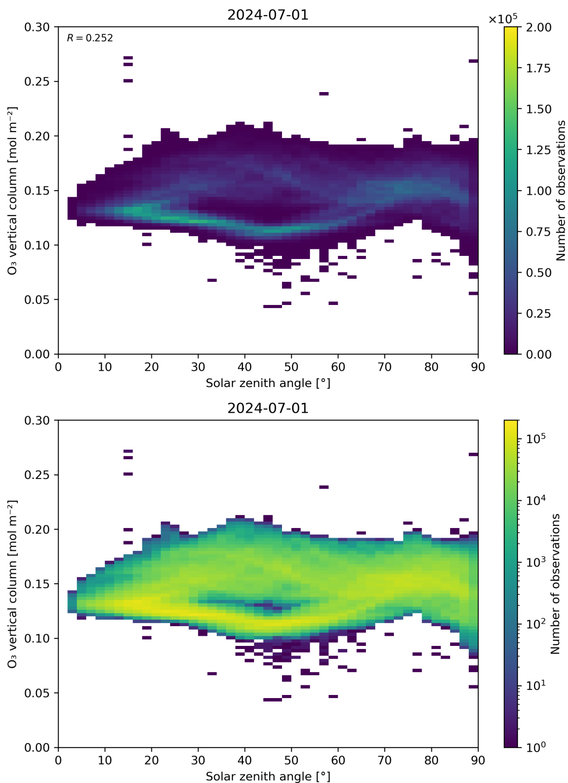
Figure 47: Scatter density plot of “Solar zenith angle” against “O 3 vertical column” for 2024-06-30 to 2024-07-02.
