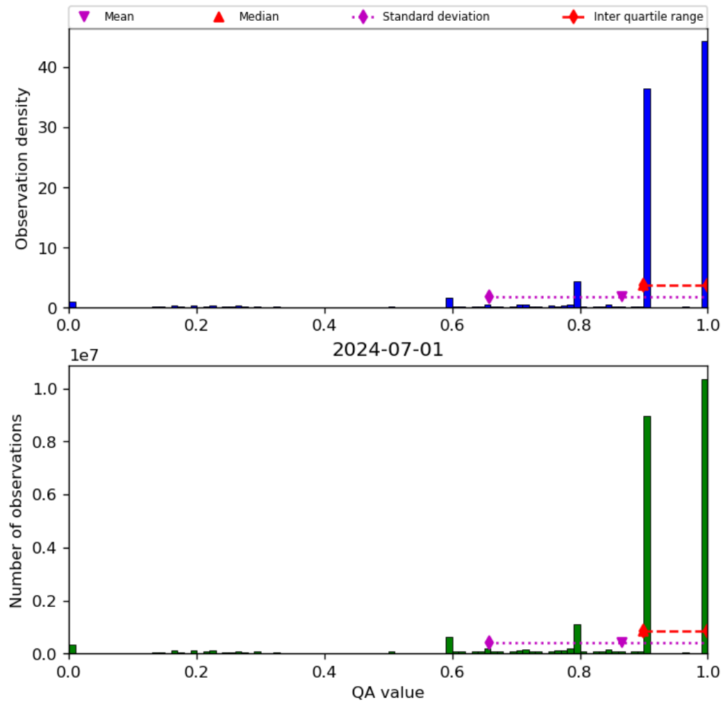
Figure 20: Histogram of “QA value” for 2024-06-30 to 2024-07-02
