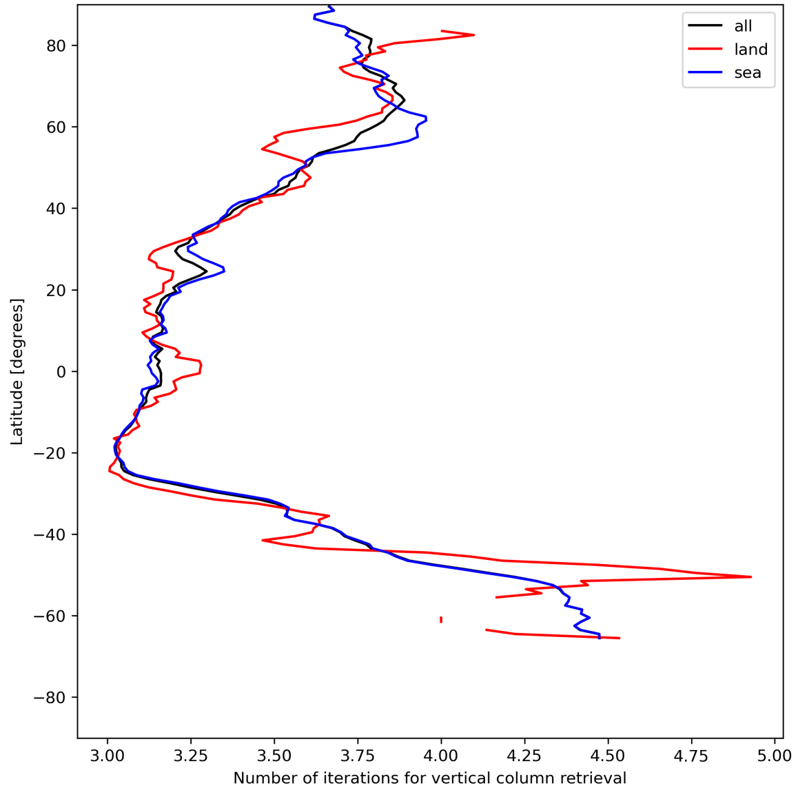
Figure 19: Zonal average of “Number of iterations for vertical column retrieval” for 2024-06-30 to 2024-07-02.
