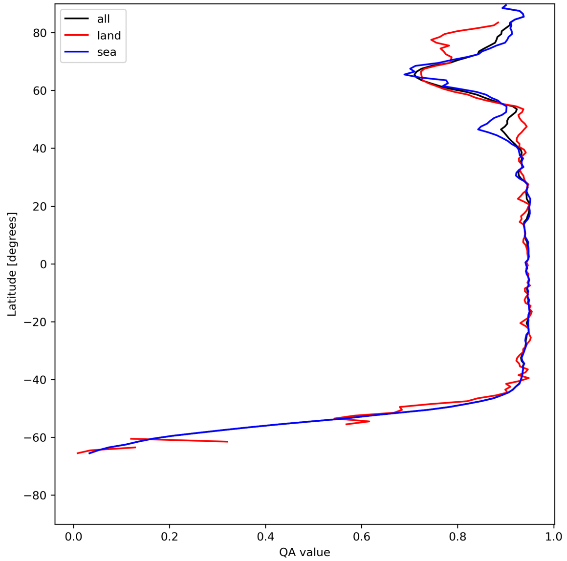
Figure 13: Zonal average of “QA value” for 2024-06-30 to 2024-07-02.
