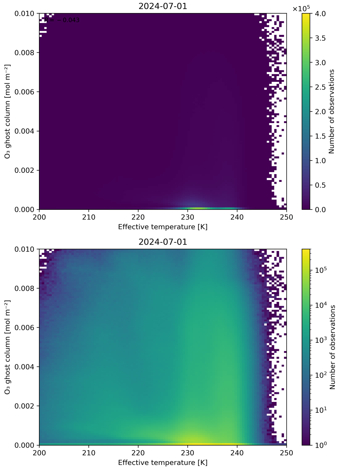
Figure 38: Scatter density plot of “Effective temperature” against “O 3 ghost column” for 2024-06-30 to 2024-07-02.
