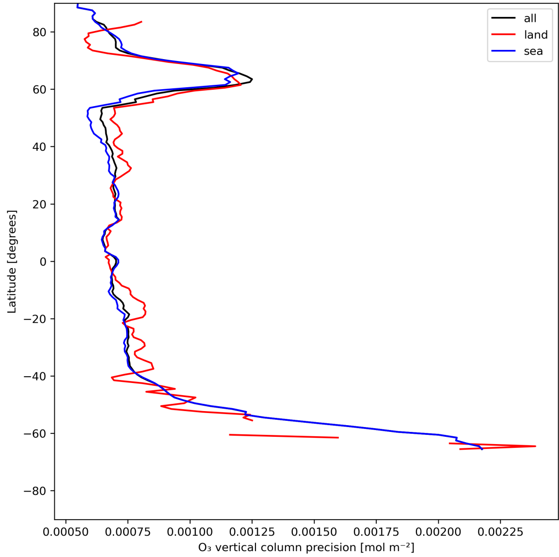
Figure 15: Zonal average of “O 3 vertical column precision” for 2024-06-30 to 2024-07-02.
