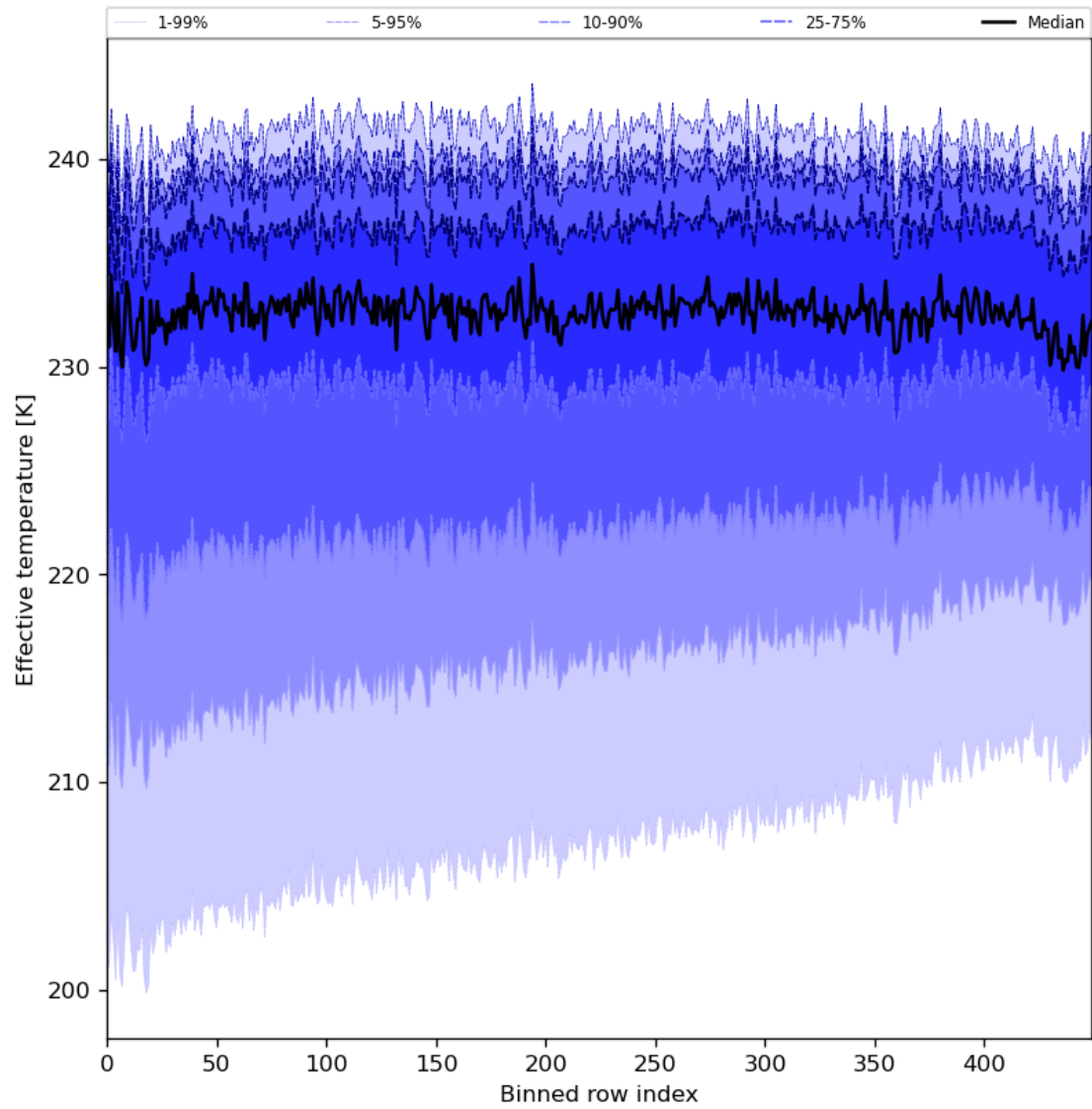
Figure 31: Along track statistics of “Effective temperature” for 2024-06-30 to 2024-07-02
