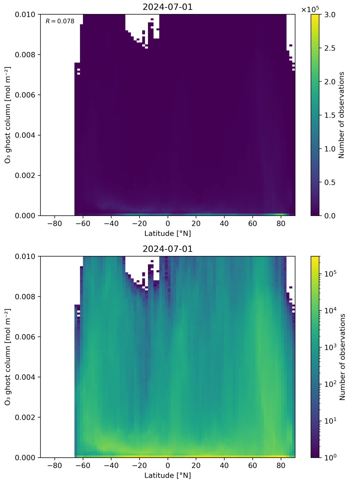
Figure 35: Scatter density plot of “Latitude” against “O 3 ghost column” for 2024-06-30 to 2024-07-02.
