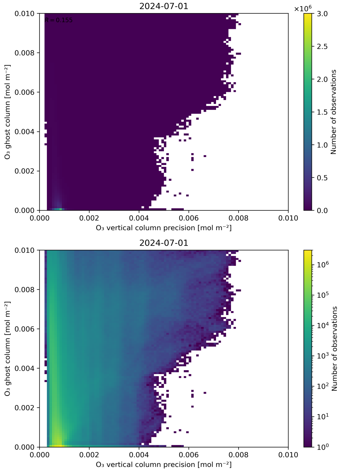
Figure 43: Scatter density plot of “ O_3 vertical column precision” against “ O_3 ghost column” for 2024-06-30 to 2024-07-02.
