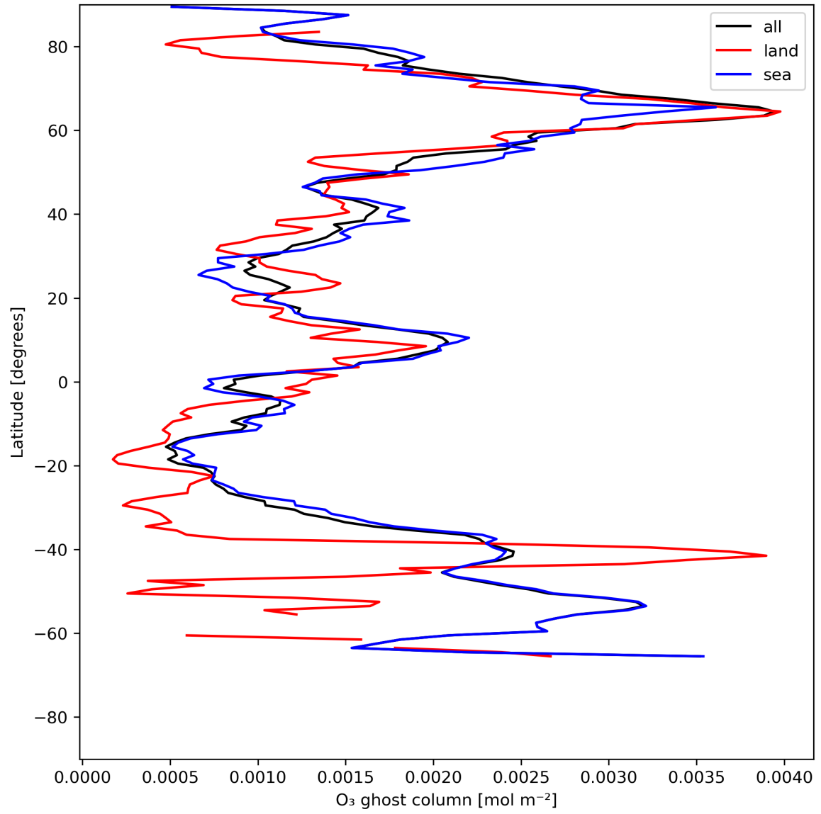
Figure 18: Zonal average of “O 3 ghost column” for 2024-06-30 to 2024-07-02.
