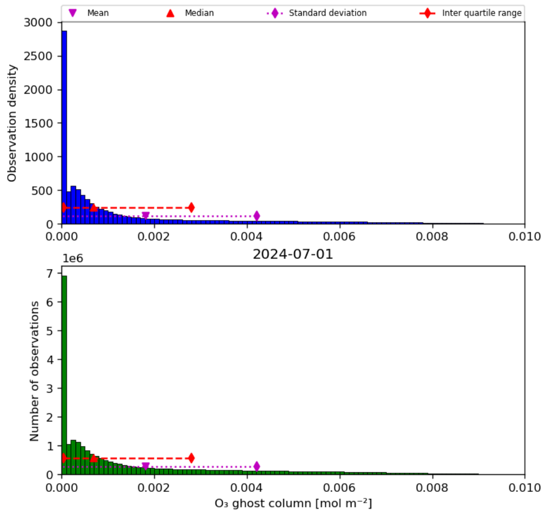
Figure 25: Histogram of “O 3 ghost column” for 2024-06-30 to 2024-07-02
