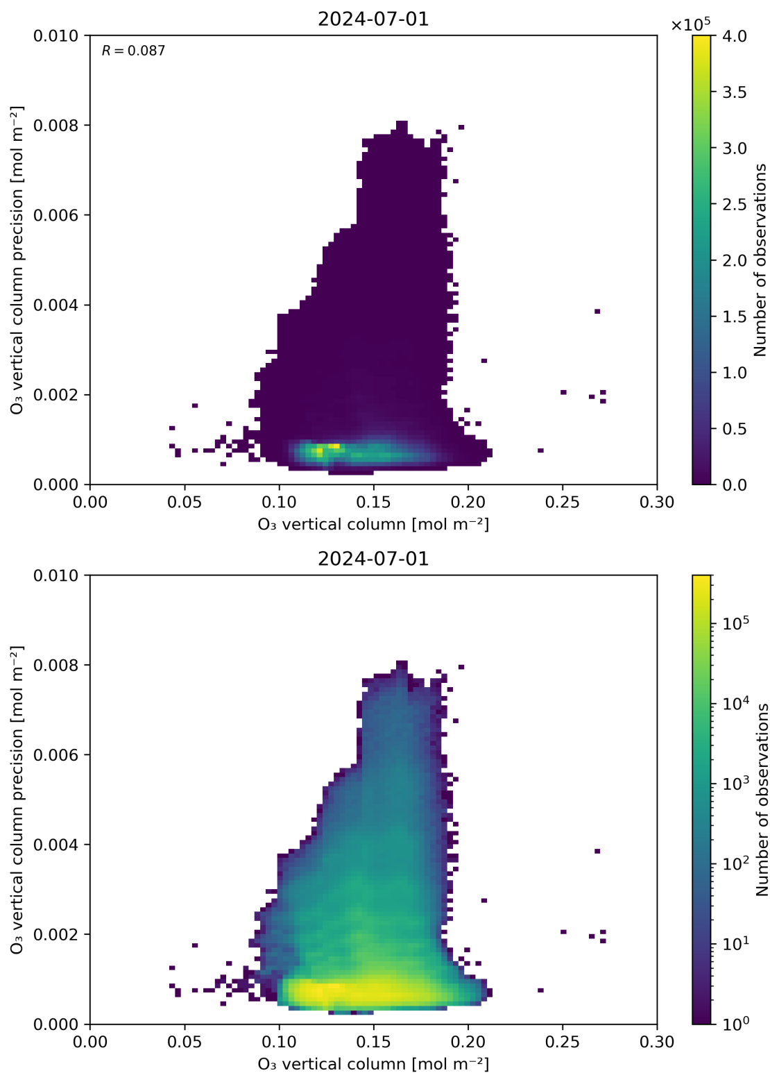
Figure 41: Scatter density plot of “O 3 vertical column” against “O 3 vertical column precision” for 2024-06-30 to 2024-07-02.
