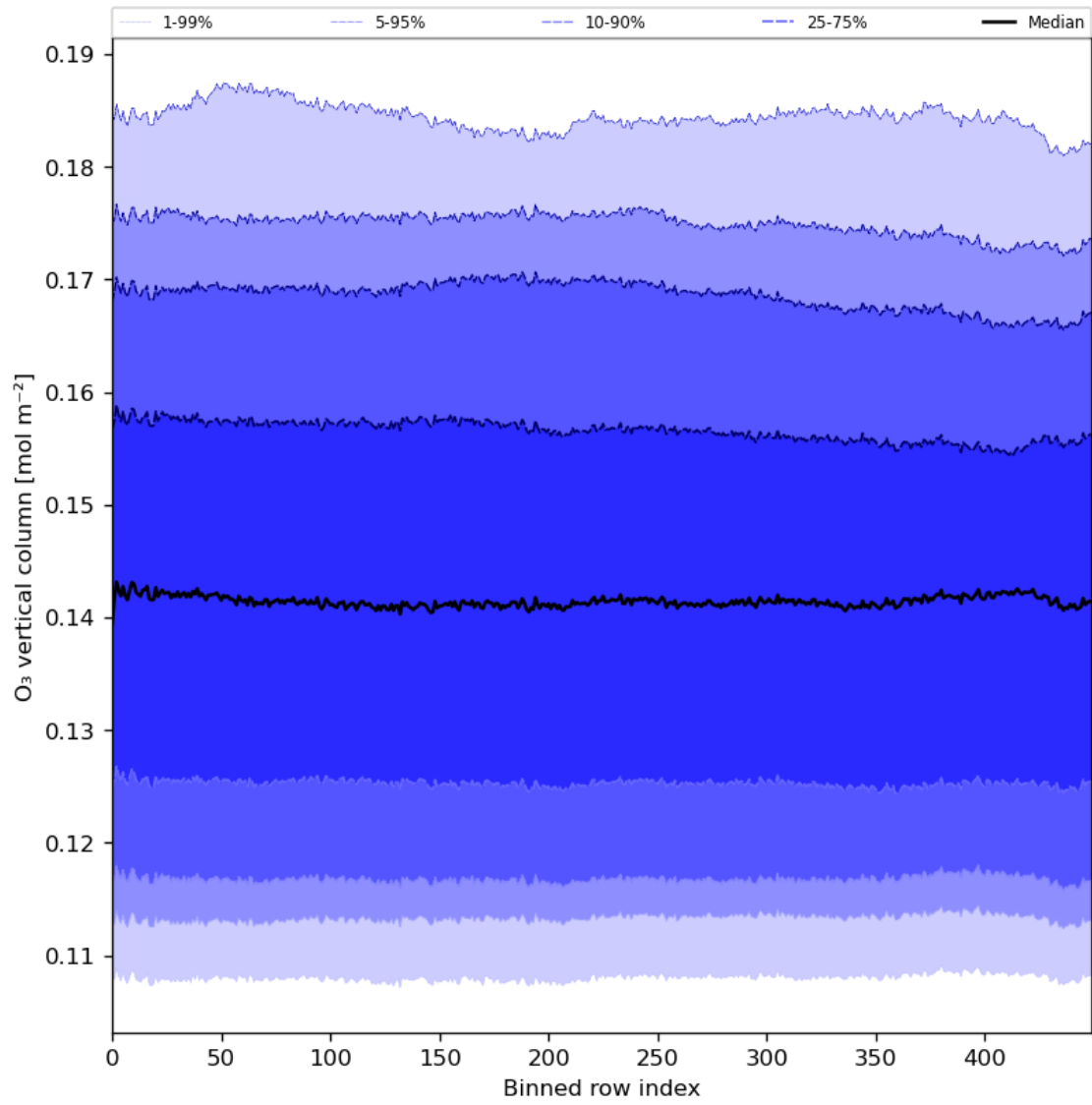
Figure 28: Along track statistics of “O 3 vertical column” for 2024-06-30 to 2024-07-02
