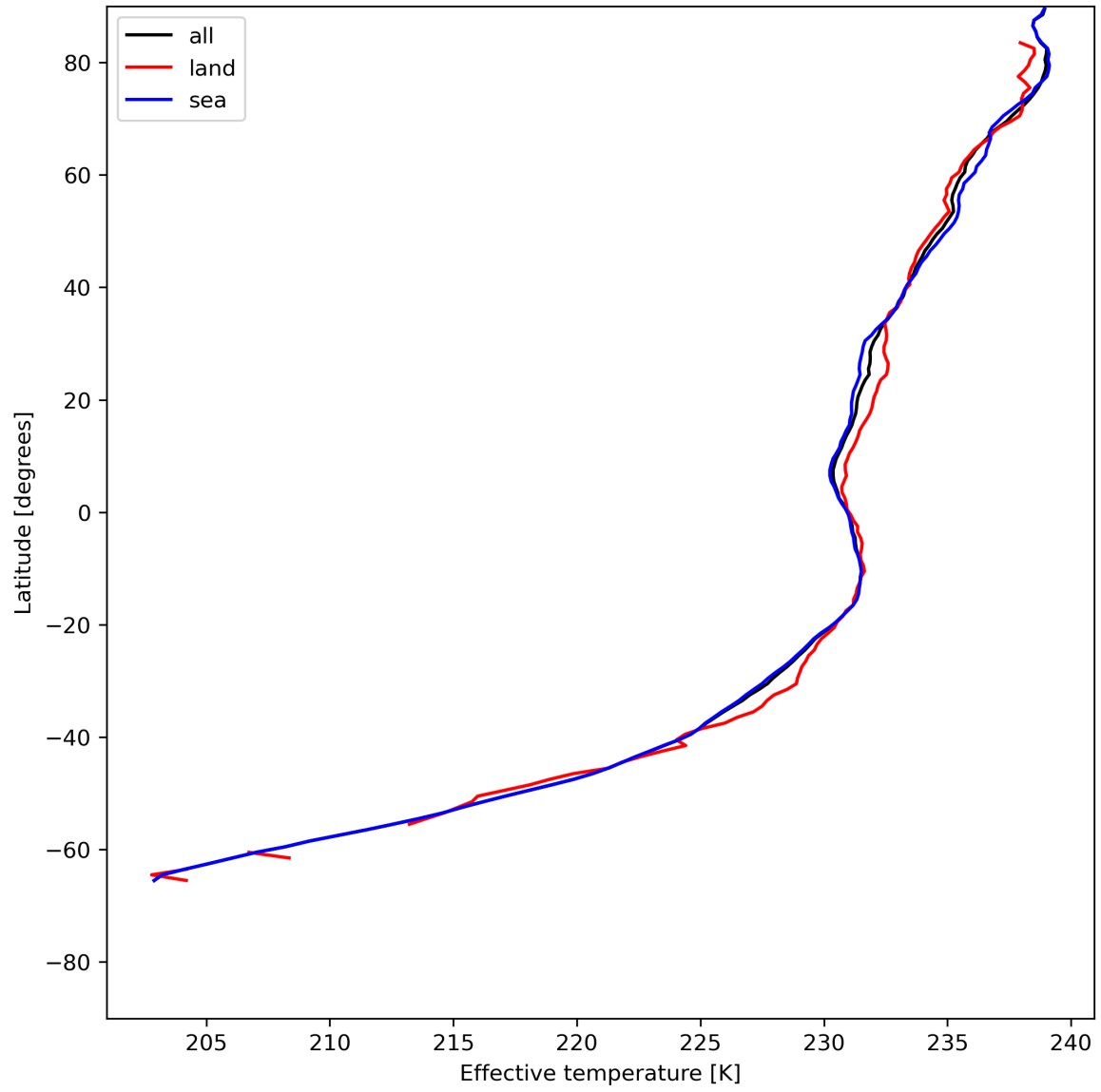
Figure 17: Zonal average of “Effective temperature” for 2024-06-30 to 2024-07-02.
