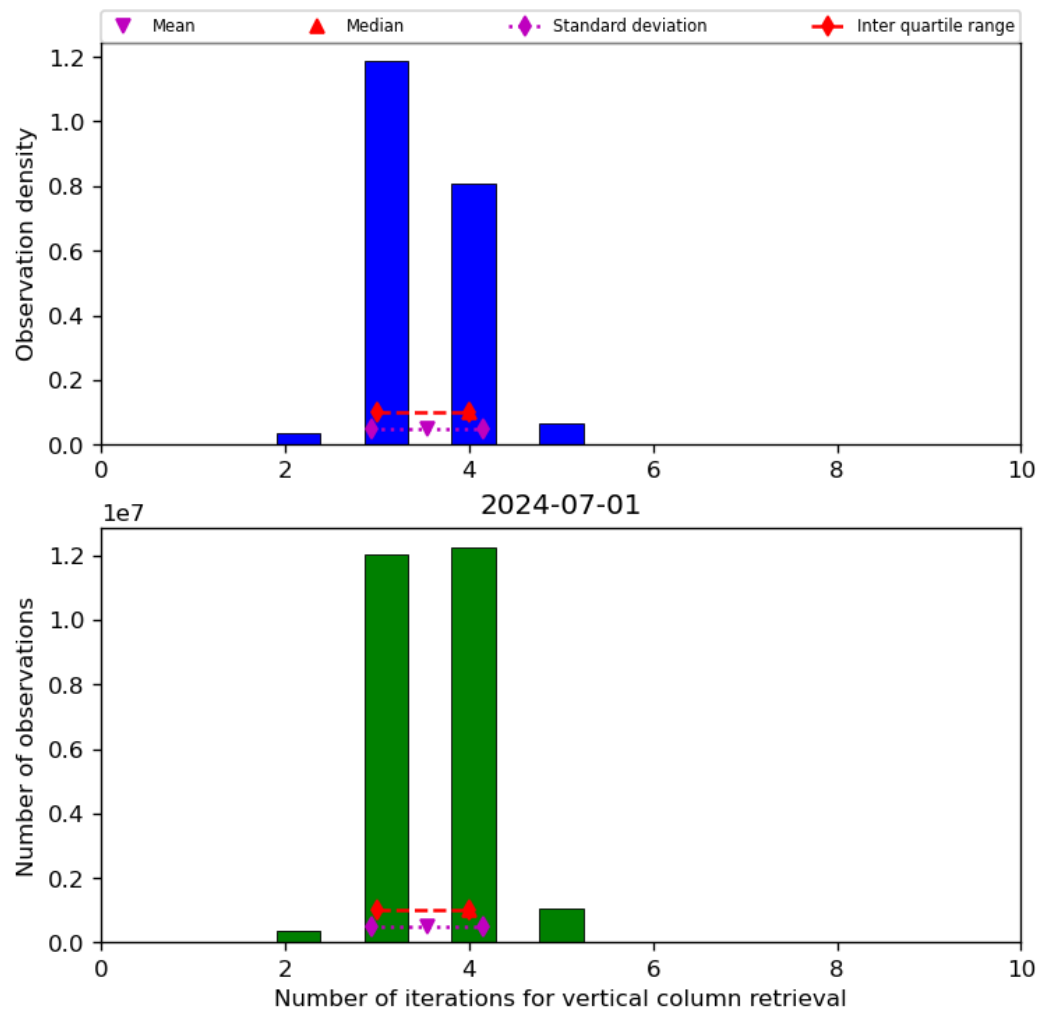
Figure 26: Histogram of “Number of iterations for vertical column retrieval” for 2024-06-30 to 2024-07-02
