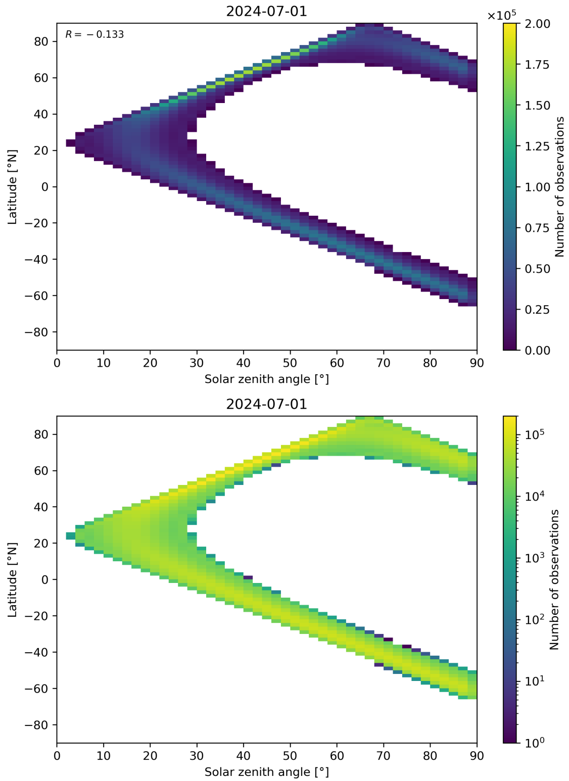
Figure 44: Scatter density plot of “Solar zenith angle” against “Latitude” for 2024-06-30 to 2024-07-02.
