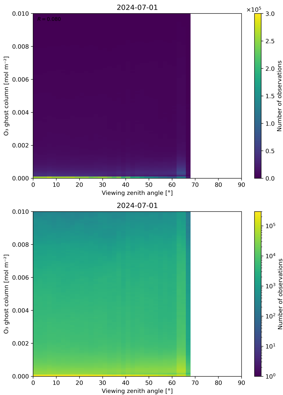
Figure 51: Scatter density plot of “Viewing zenith angle” against “O 3 ghost column” for 2024-06-30 to 2024-07-02.
