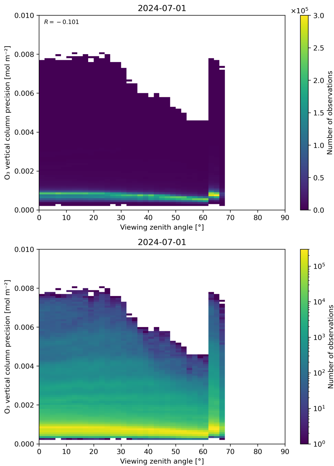
Figure 53: Scatter density plot of “Viewing zenith angle” against “O 3 vertical column precision” for 2024-06-30 to 2024-07-02.
