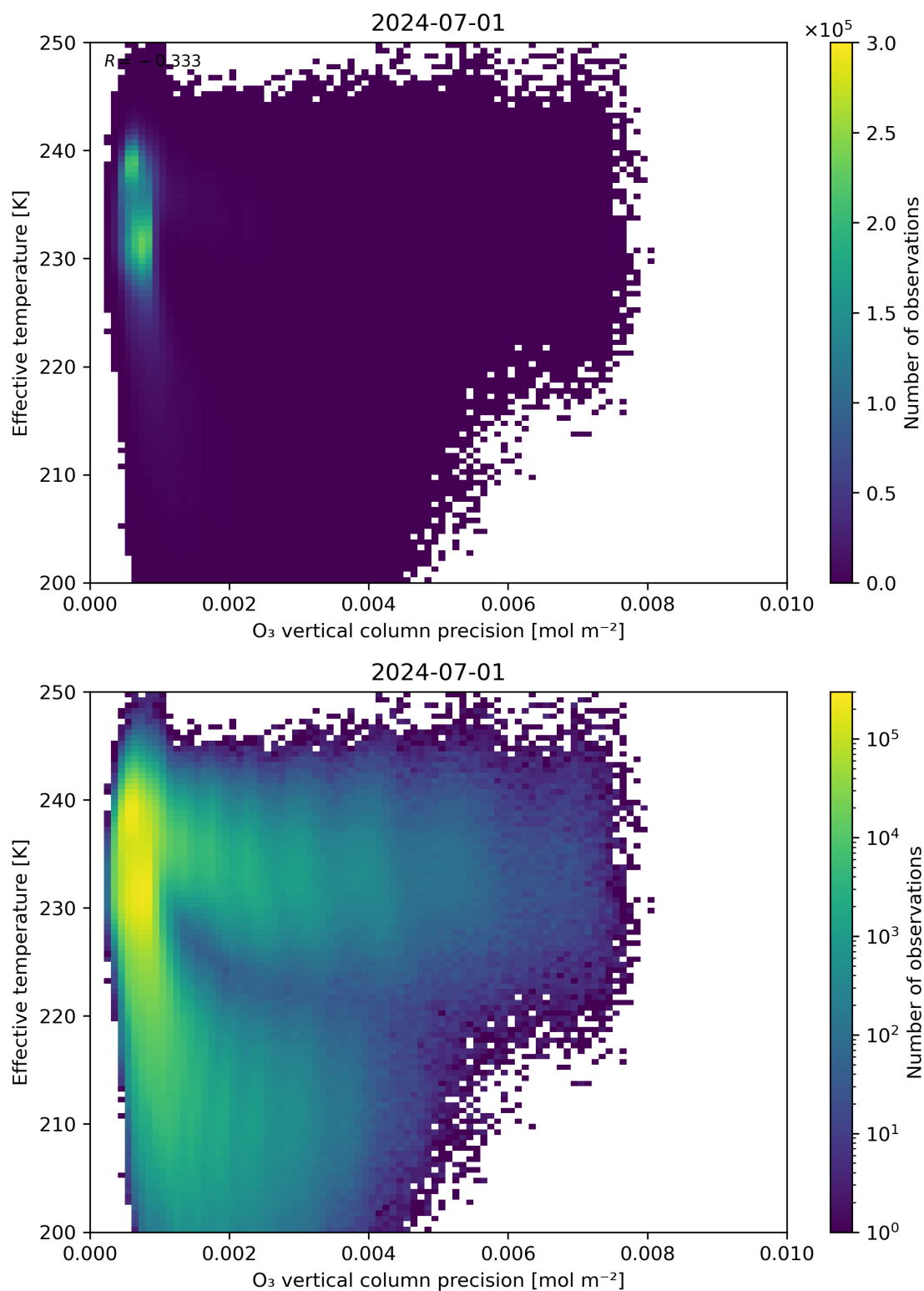
Figure 42: Scatter density plot of “O 3 vertical column precision” against “Effective temperature” for 2024-06-30 to 2024-07-02.
