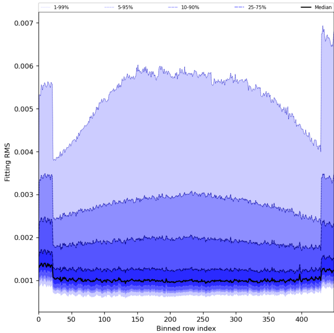
Figure 30: Along track statistics of “Fitting RMS” for 2024-06-30 to 2024-07-02
