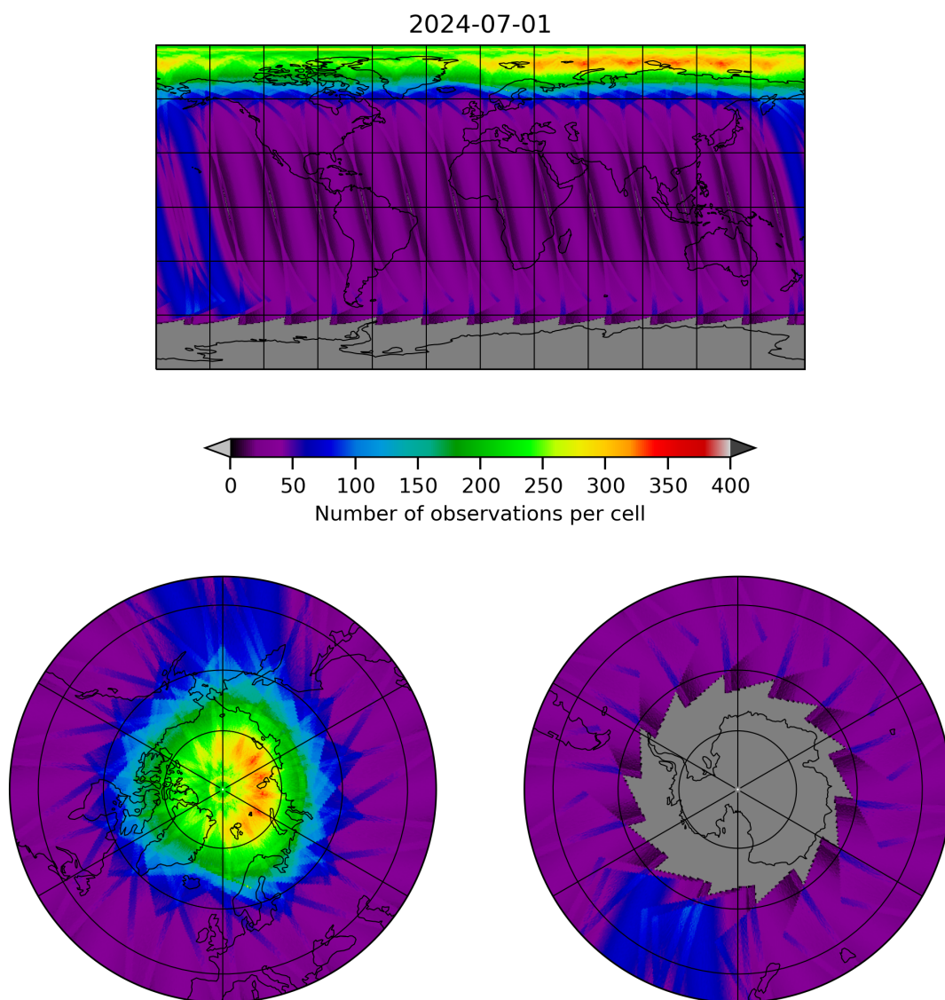
Figure 12: Map of the number of observations for 2024-06-30 to 2024-07-02
