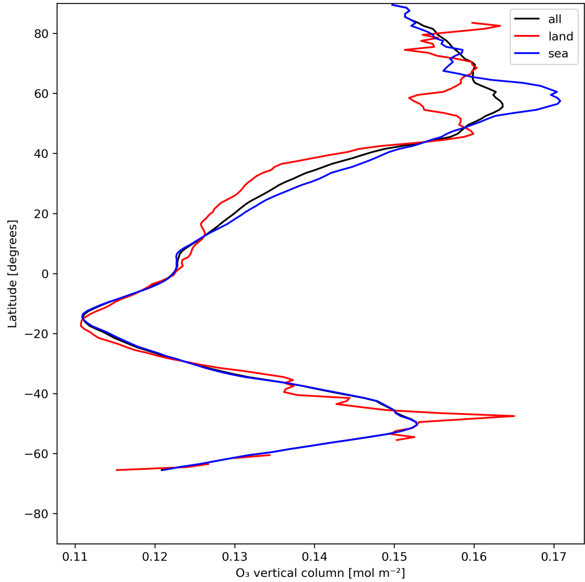
Figure 14: Zonal average of “O 3 vertical column” for 2024-06-30 to 2024-07-02.
