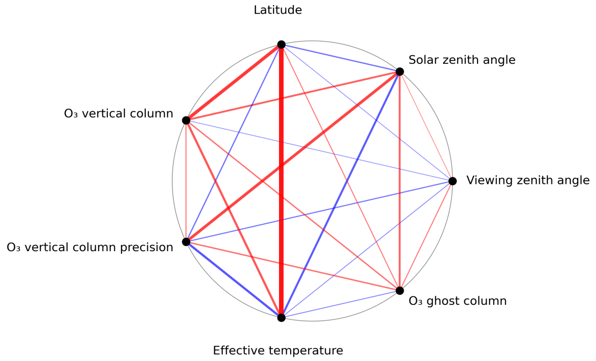
Figure 1: Map of correlation graph for 2024-06-30 to 2024-07-02.
