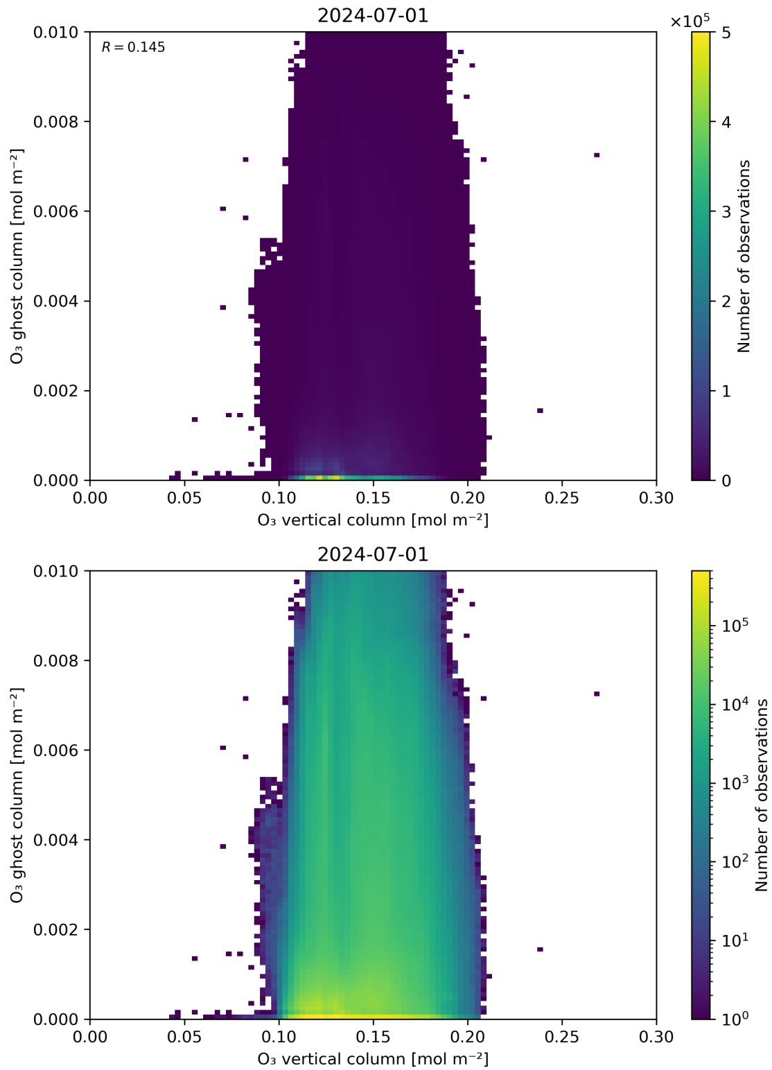
Figure 40: Scatter density plot of “O 3 vertical column” against “O 3 ghost column” for 2024-06-30 to 2024-07-02.
