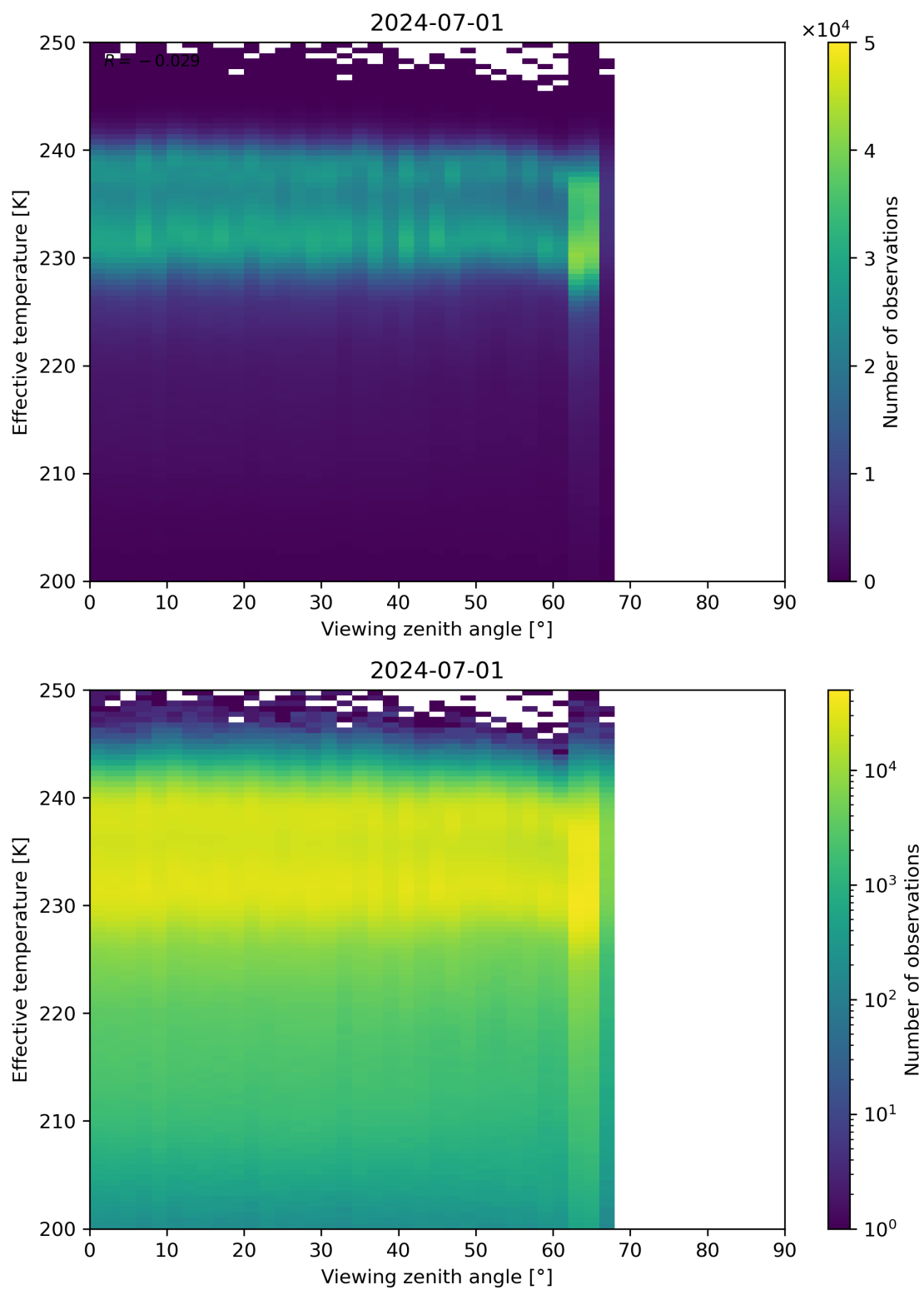
Figure 50: Scatter density plot of “Viewing zenith angle” against “Effective temperature” for 2024-06-30 to 2024-07-02.
