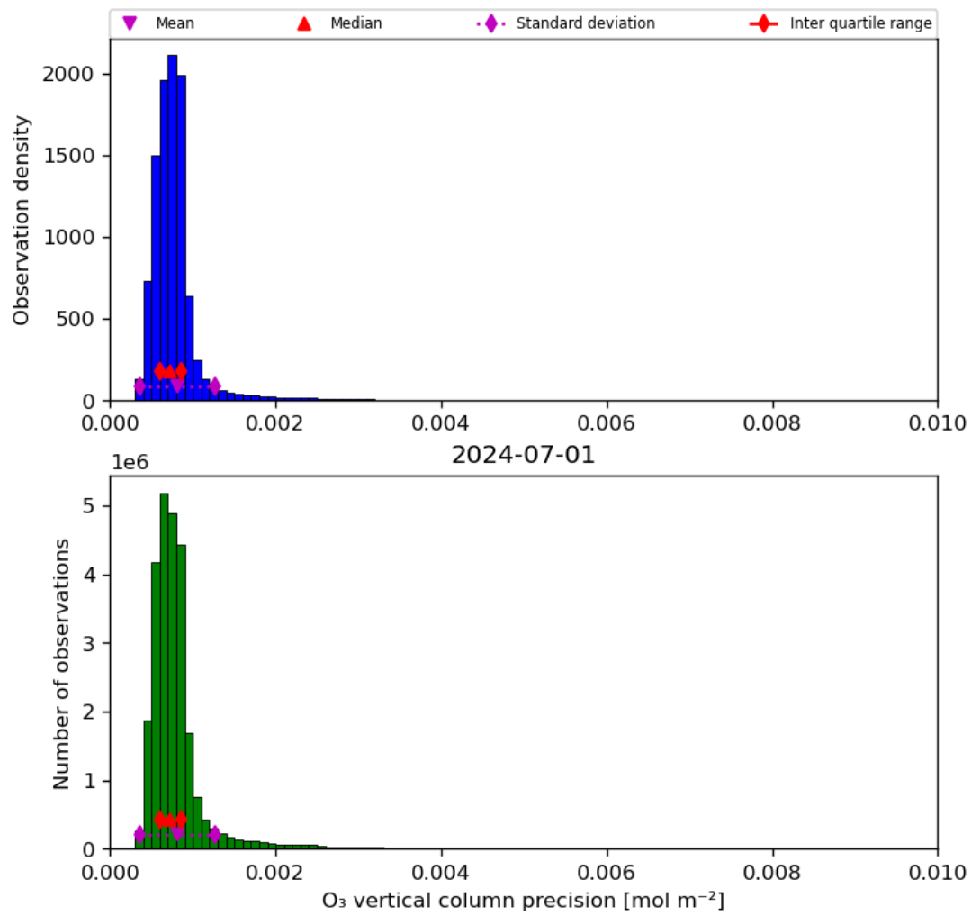
Figure 22: Histogram of “O 3 vertical column precision” for 2024-06-30 to 2024-07-02
