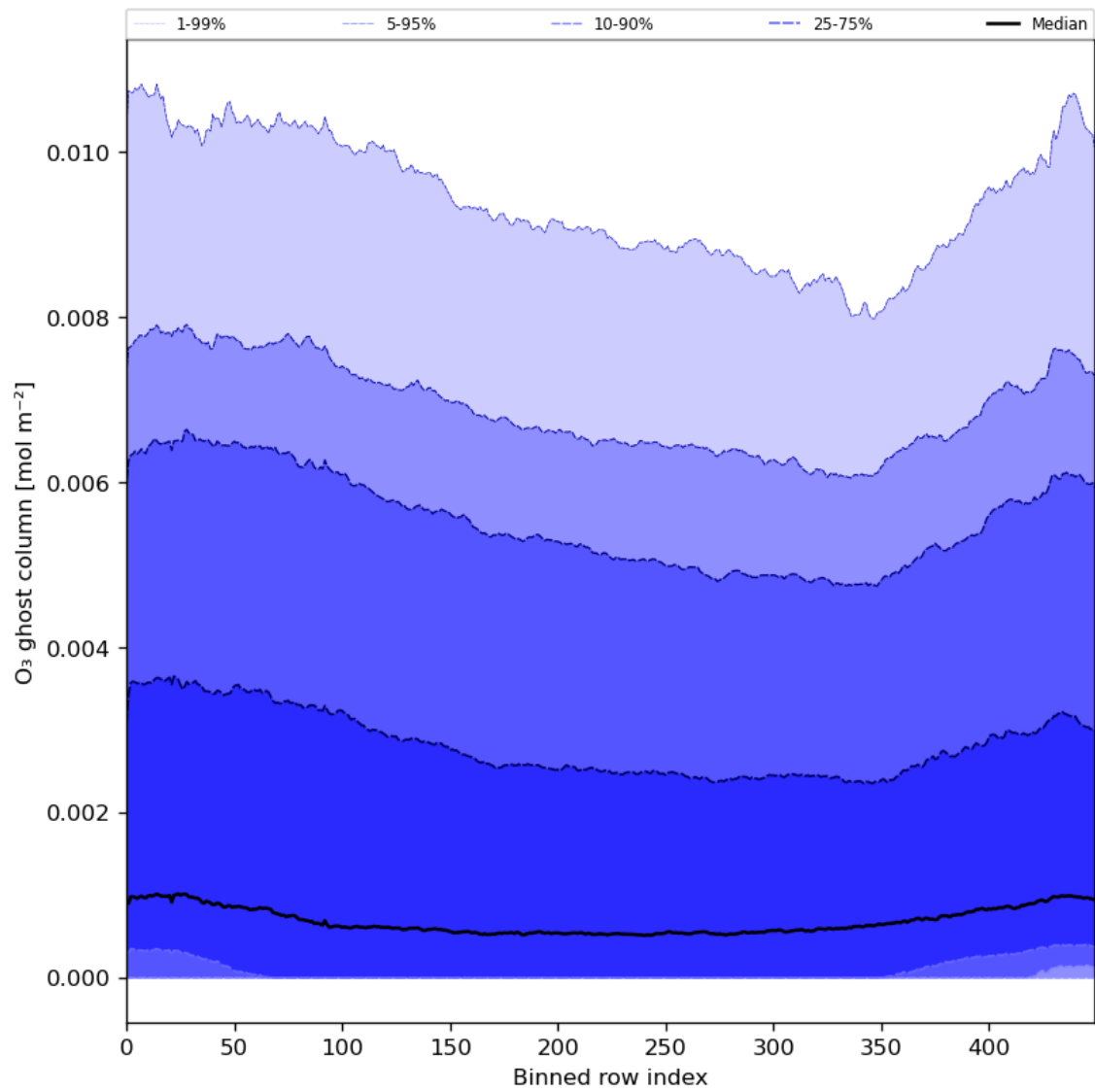
Figure 32: Along track statistics of “O 3 ghost column” for 2024-06-30 to 2024-07-02
