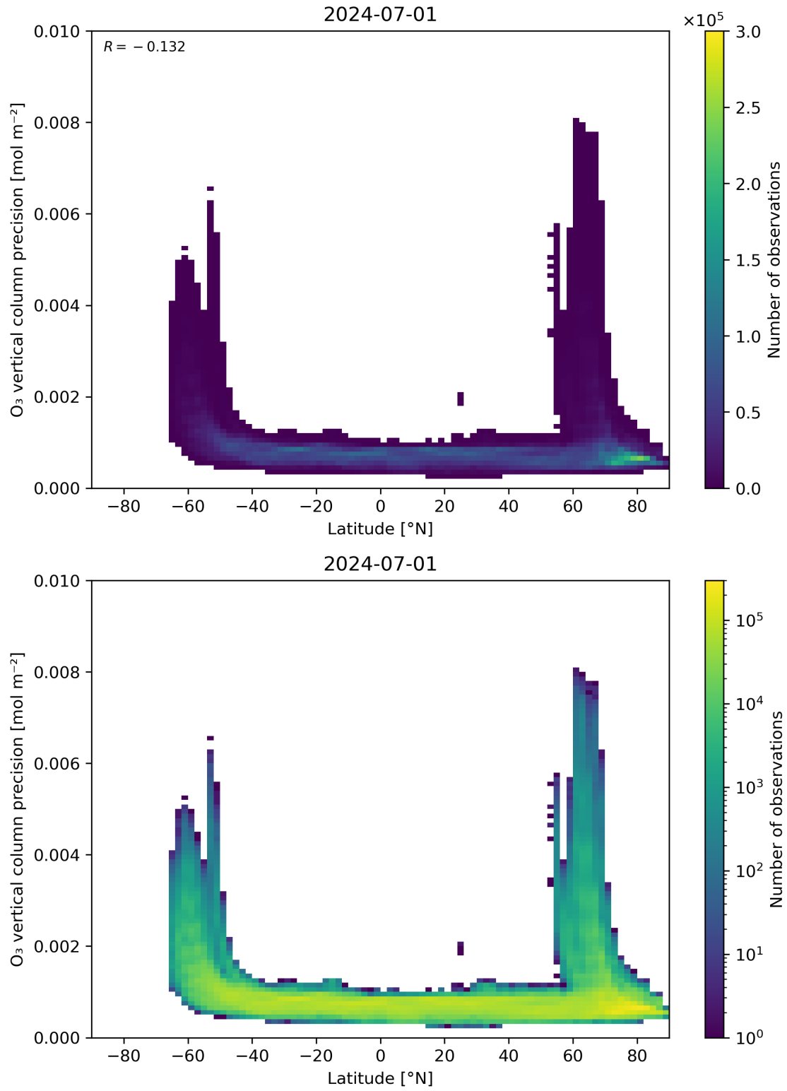
Figure 37: Scatter density plot of “Latitude” against “O 3 vertical column precision” for 2024-06-30 to 2024-07-02.
