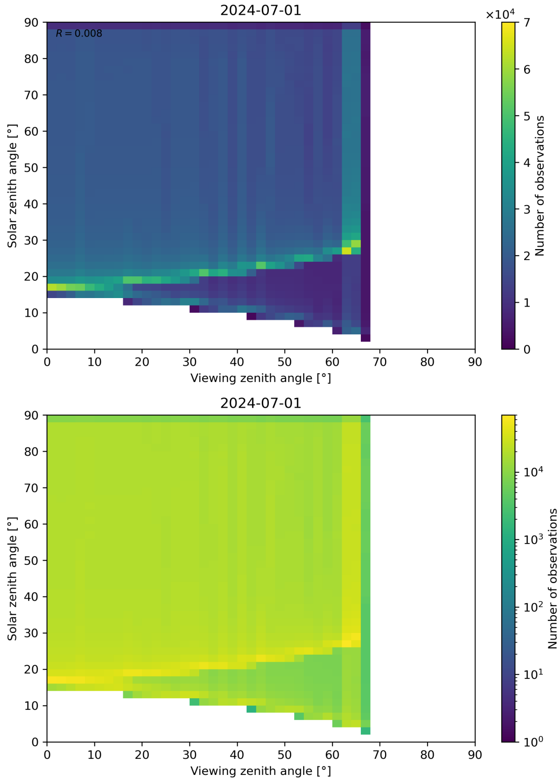
Figure 54: Scatter density plot of “Viewing zenith angle” against “Solar zenith angle” for 2024-06-30 to 2024-07-02.
