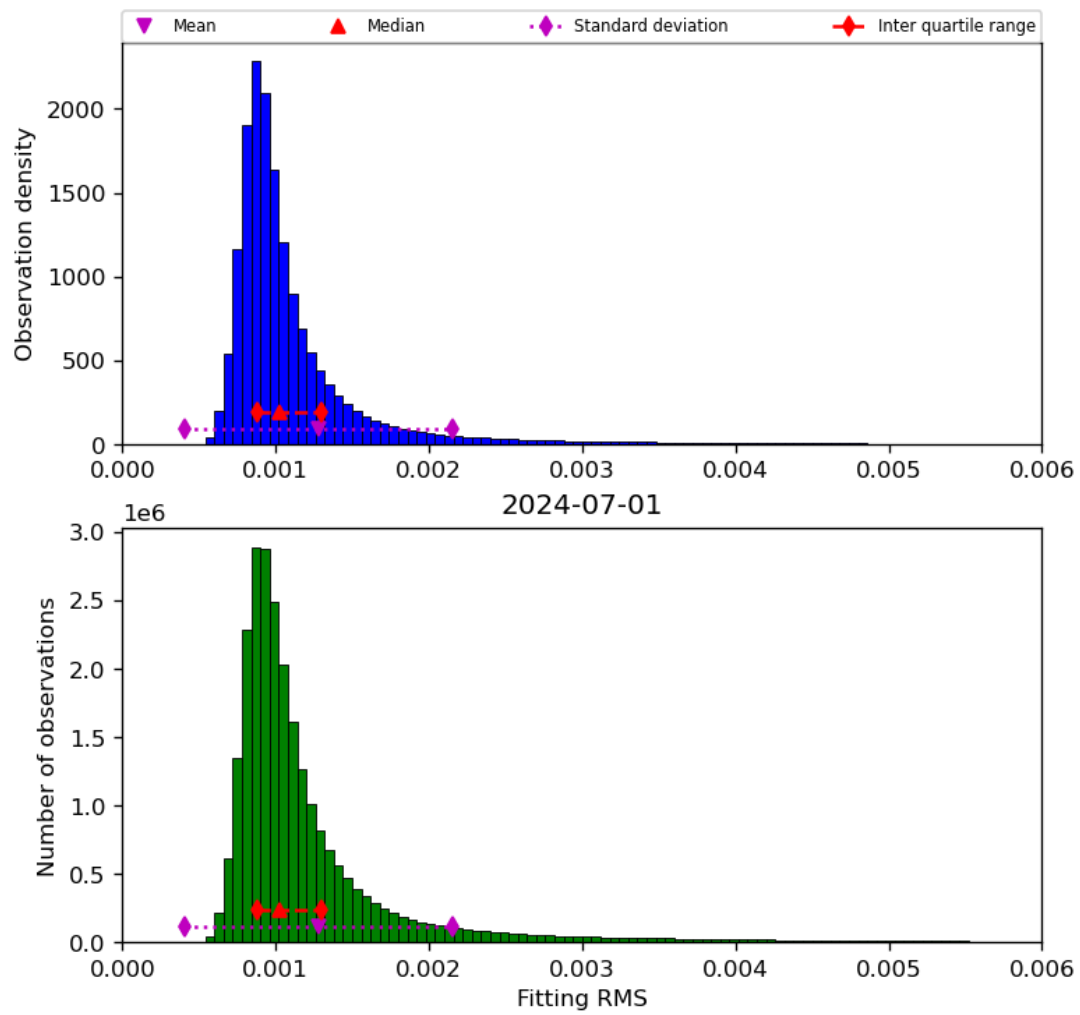
Figure 23: Histogram of “Fitting RMS” for 2024-06-30 to 2024-07-02
