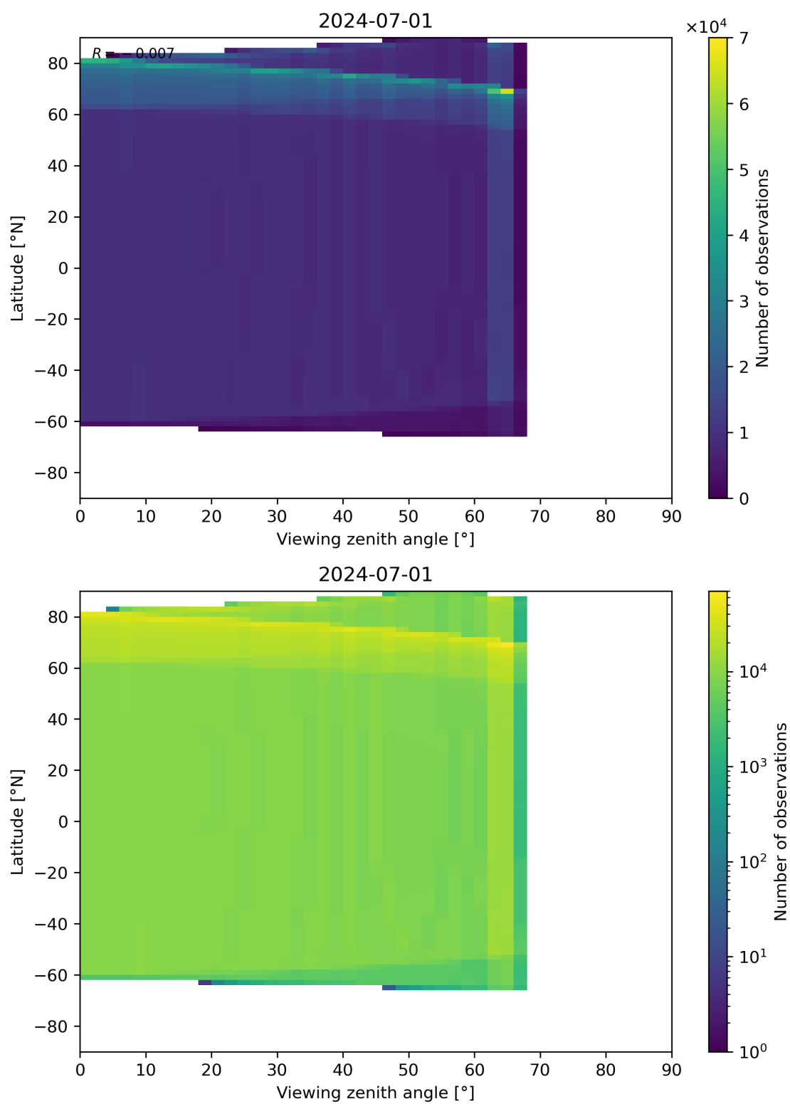
Figure 49: Scatter density plot of “Viewing zenith angle” against “Latitude” for 2024-06-30 to 2024-07-02.
