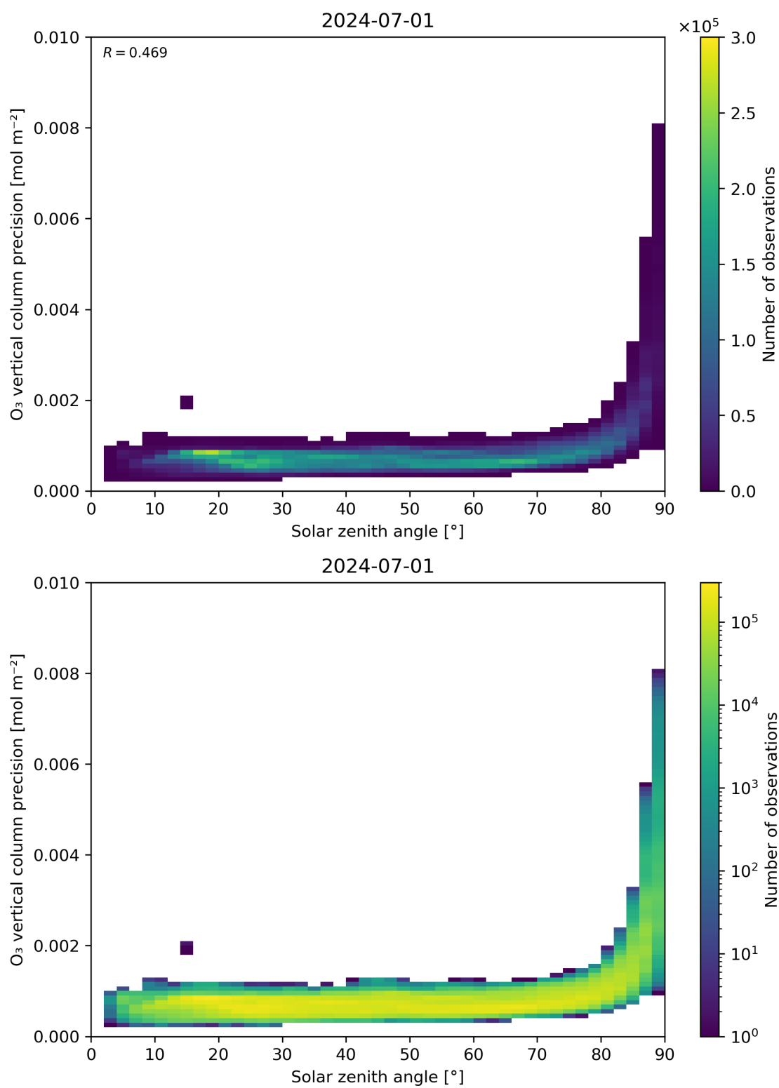
Figure 48: Scatter density plot of “Solar zenith angle” against “O 3 vertical column precision” for 2024-06-30 to 2024-07-02.
