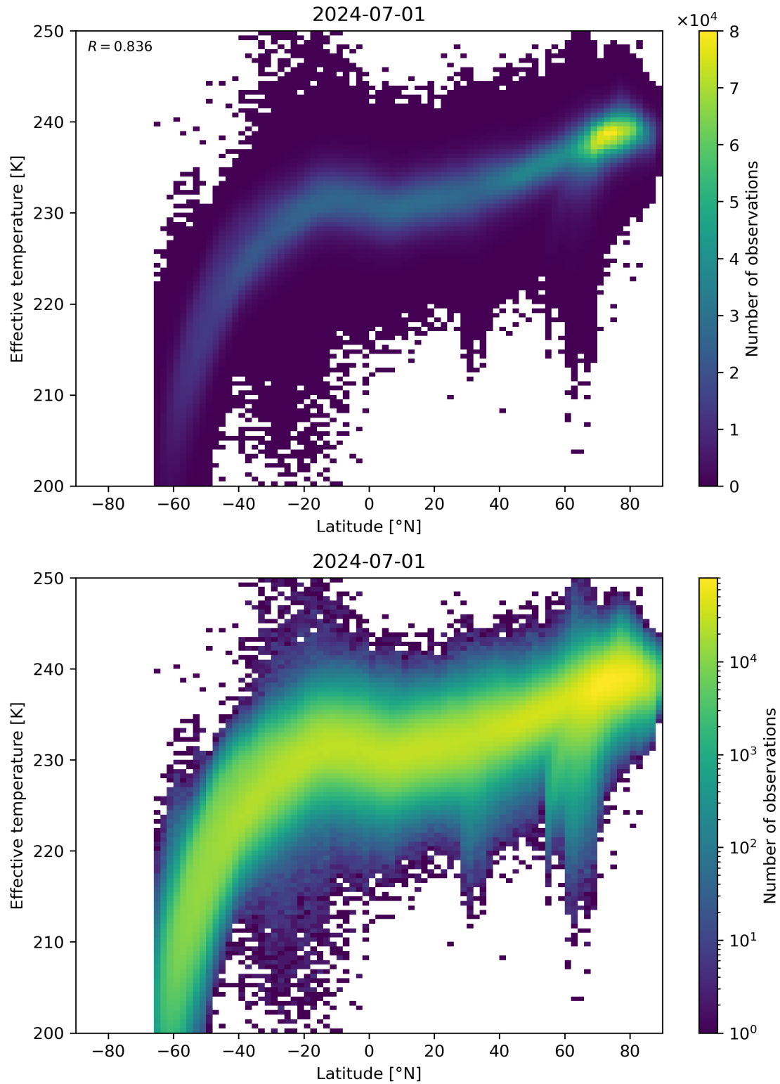
Figure 34: Scatter density plot of “Latitude” against “Effective temperature” for 2024-06-30 to 2024-07-02.
