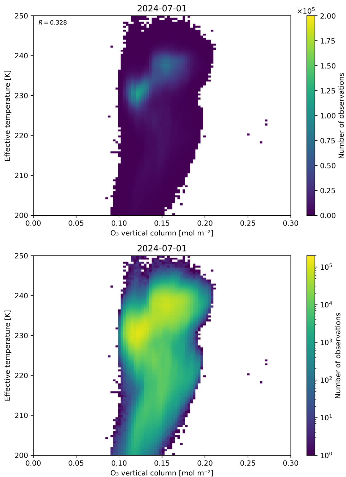
Figure 39: Scatter density plot of “O 3 vertical column” against “Effective temperature” for 2024-06-30 to 2024-07-02.
