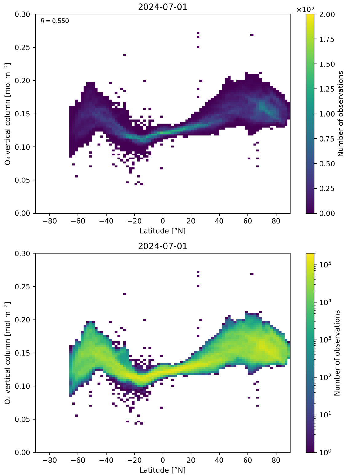
Figure 36: Scatter density plot of “Latitude” against “O 3 vertical column” for 2024-06-30 to 2024-07-02.
