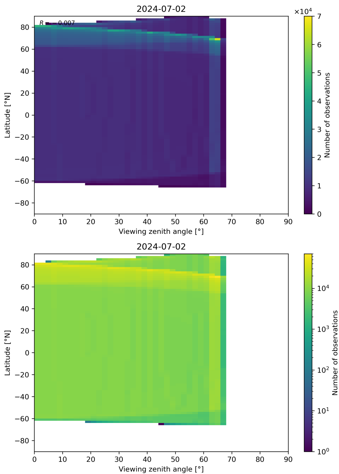
Figure 49: Scatter density plot of “Viewing zenith angle” against “Latitude” for 2024-07-01 to 2024-07-03.
