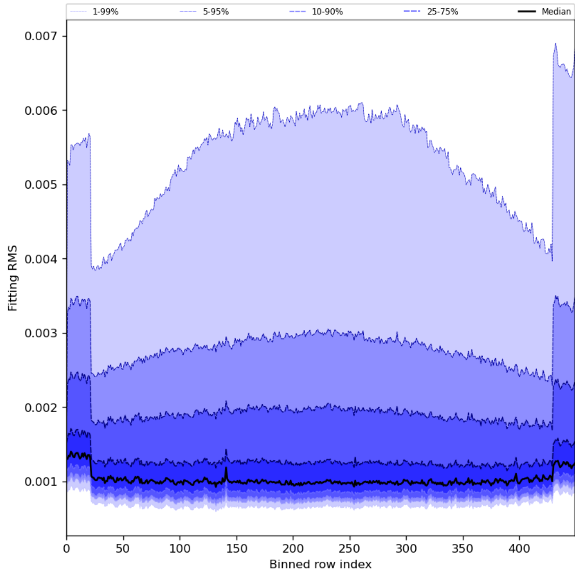
Figure 30: Along track statistics of “Fitting RMS” for 2024-07-01 to 2024-07-03
