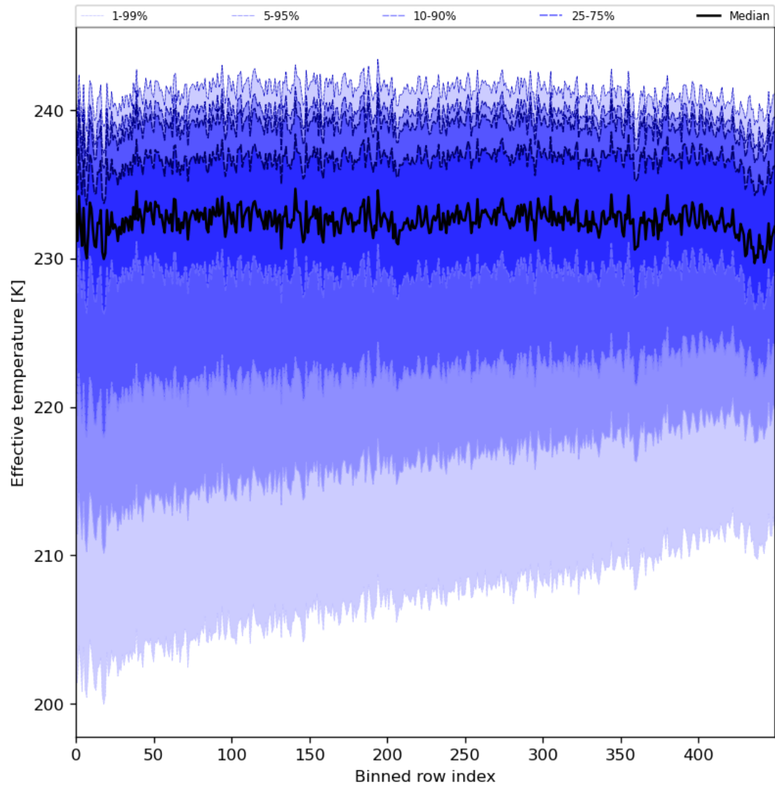
Figure 31: Along track statistics of “Effective temperature” for 2024-07-01 to 2024-07-03
