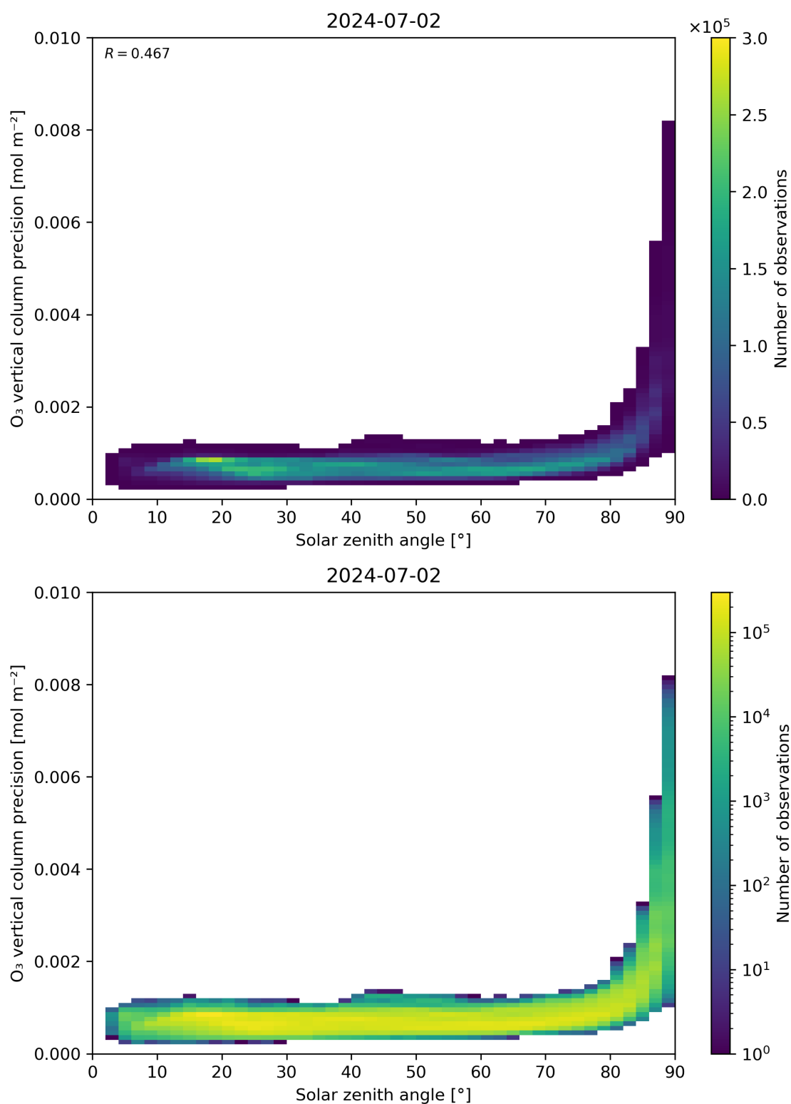
Figure 48: Scatter density plot of “Solar zenith angle” against “O 3 vertical column precision” for 2024-07-01 to 2024-07-03.
