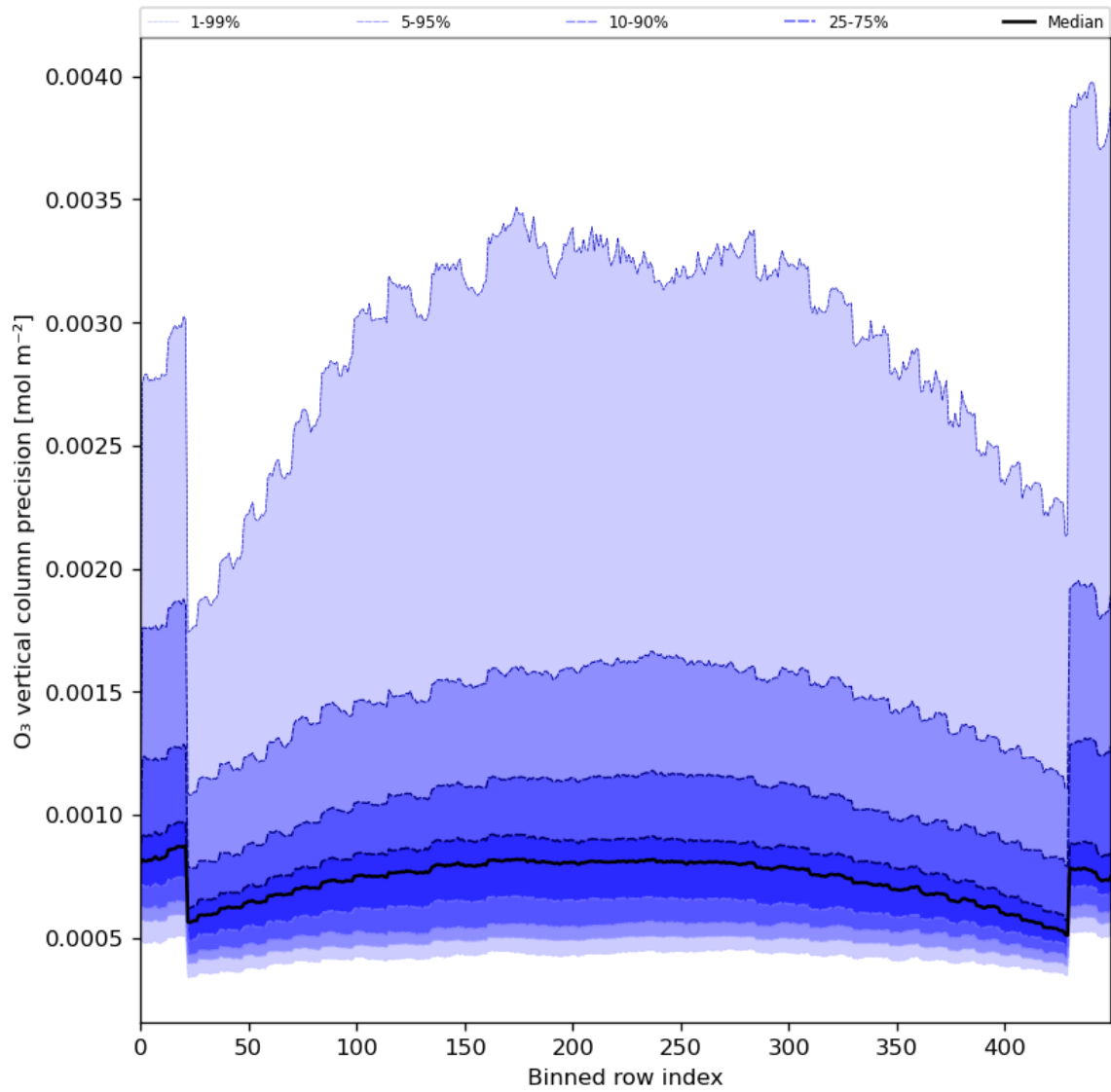
Figure 29: Along track statistics of “O 3 vertical column precision” for 2024-07-01 to 2024-07-03
