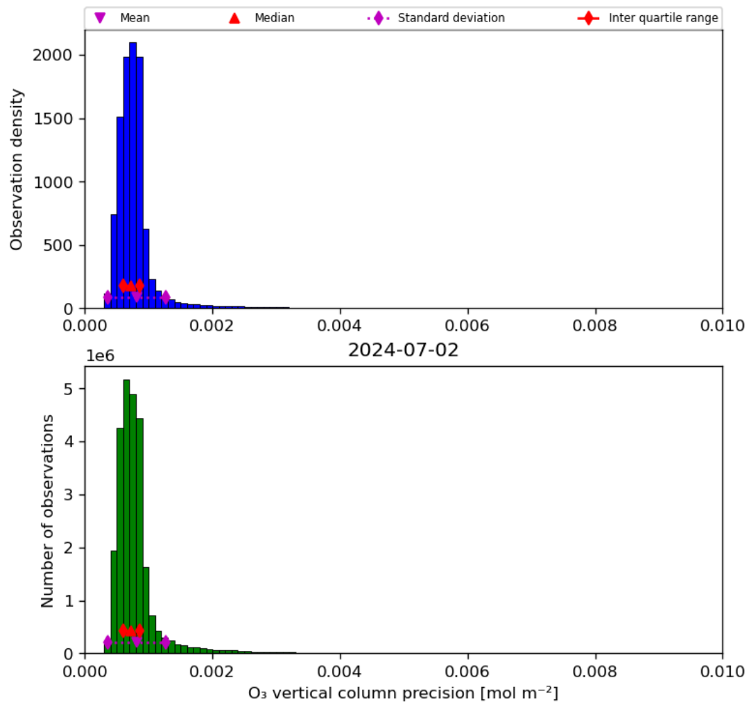
Figure 22: Histogram of “O 3 vertical column precision” for 2024-07-01 to 2024-07-03
