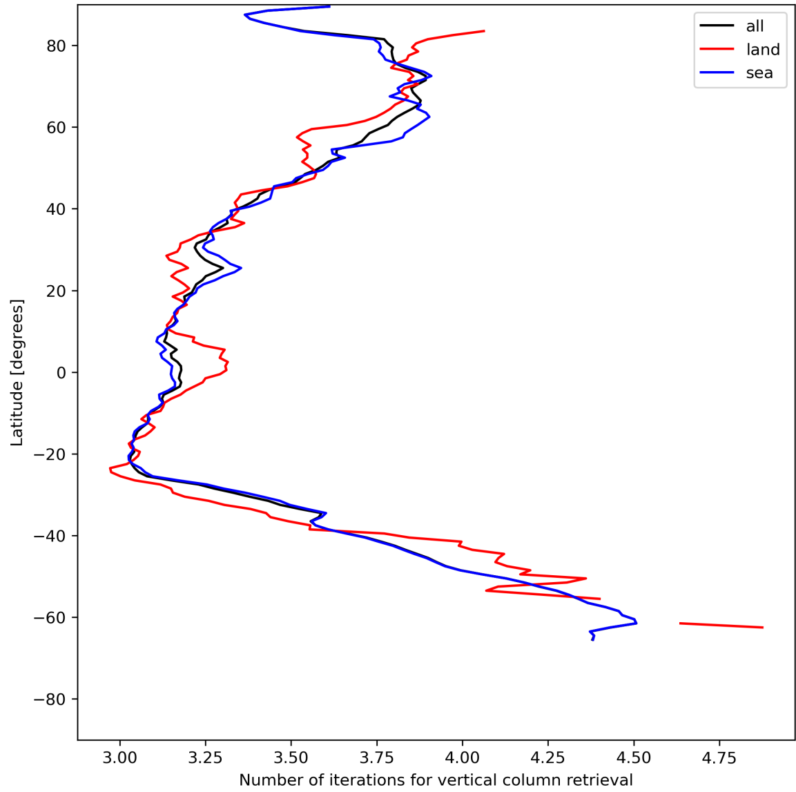
Figure 19: Zonal average of “Number of iterations for vertical column retrieval” for 2024-07-01 to 2024-07-03.
