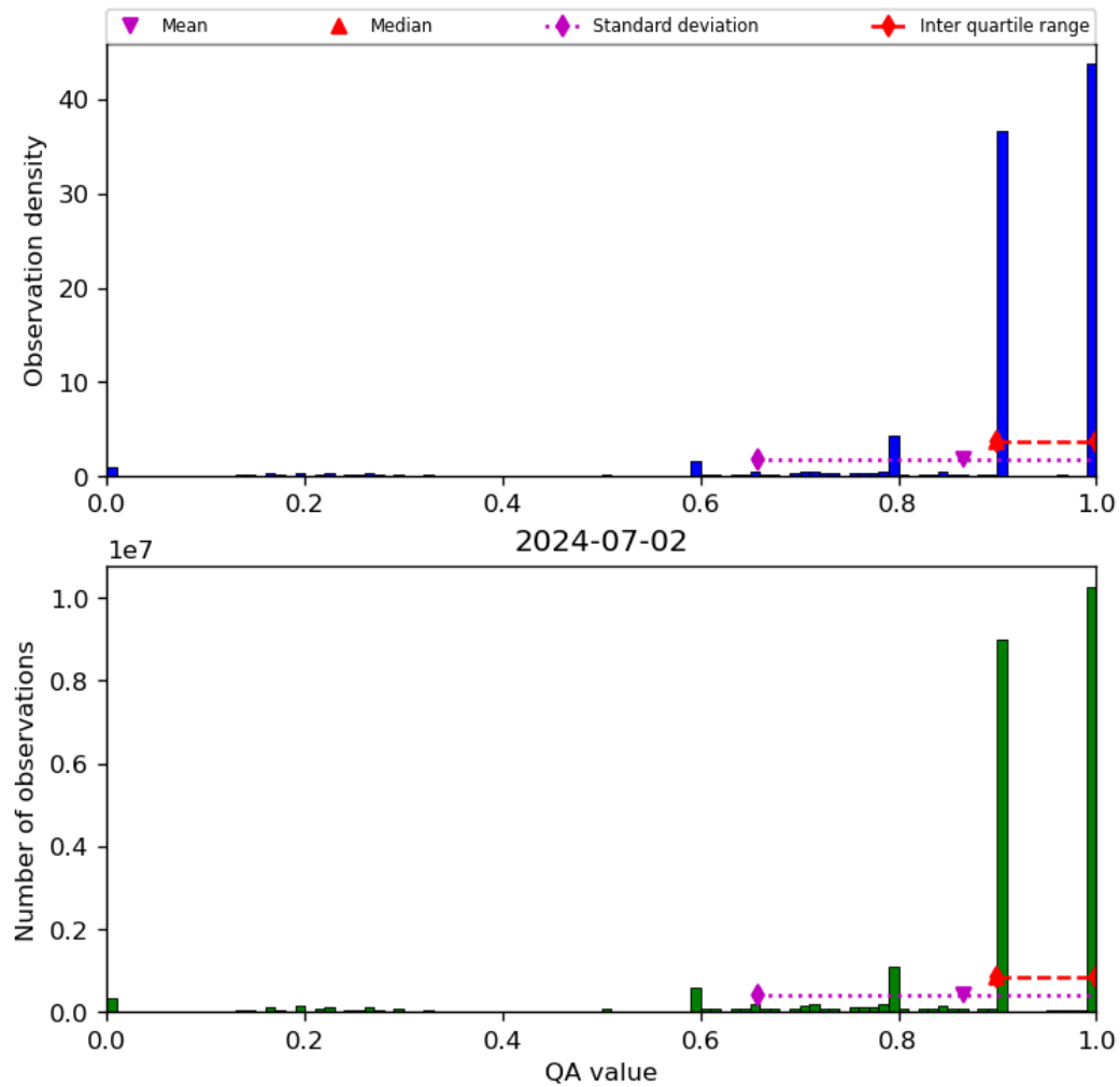
Figure 20: Histogram of “QA value” for 2024-07-01 to 2024-07-03
