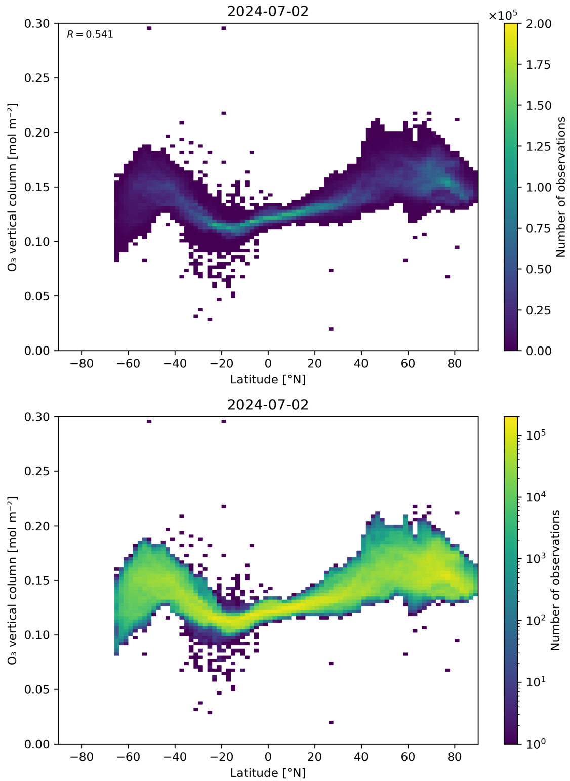
Figure 36: Scatter density plot of “Latitude” against “O 3 vertical column” for 2024-07-01 to 2024-07-03.
