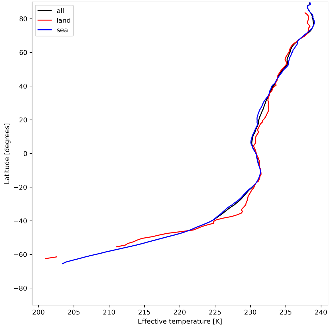
Figure 17: Zonal average of “Effective temperature” for 2024-07-01 to 2024-07-03.
