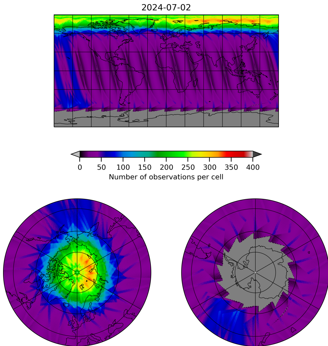
Figure 12: Map of the number of observations for 2024-07-01 to 2024-07-03
