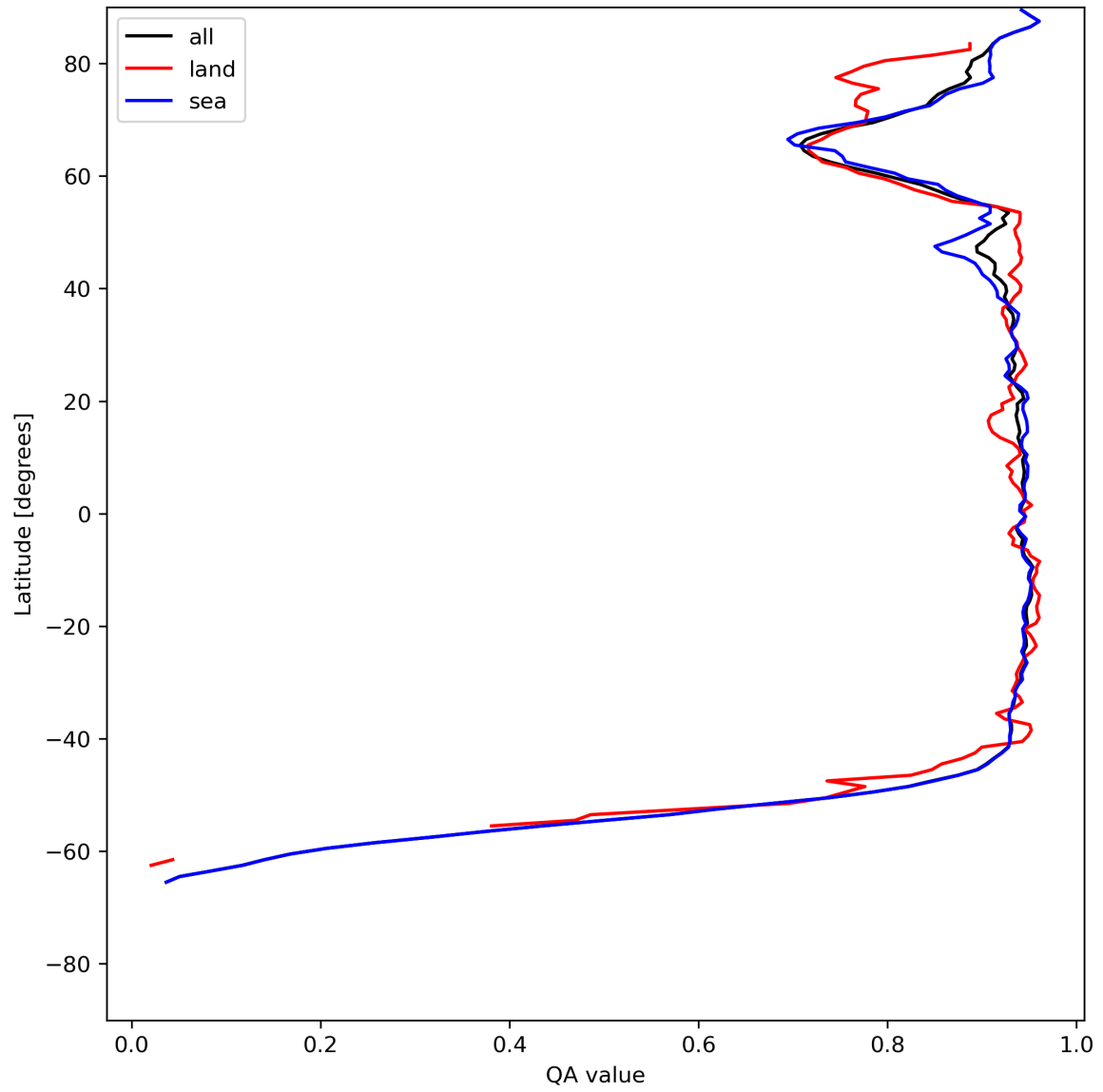
Figure 13: Zonal average of “QA value” for 2024-07-01 to 2024-07-03.
