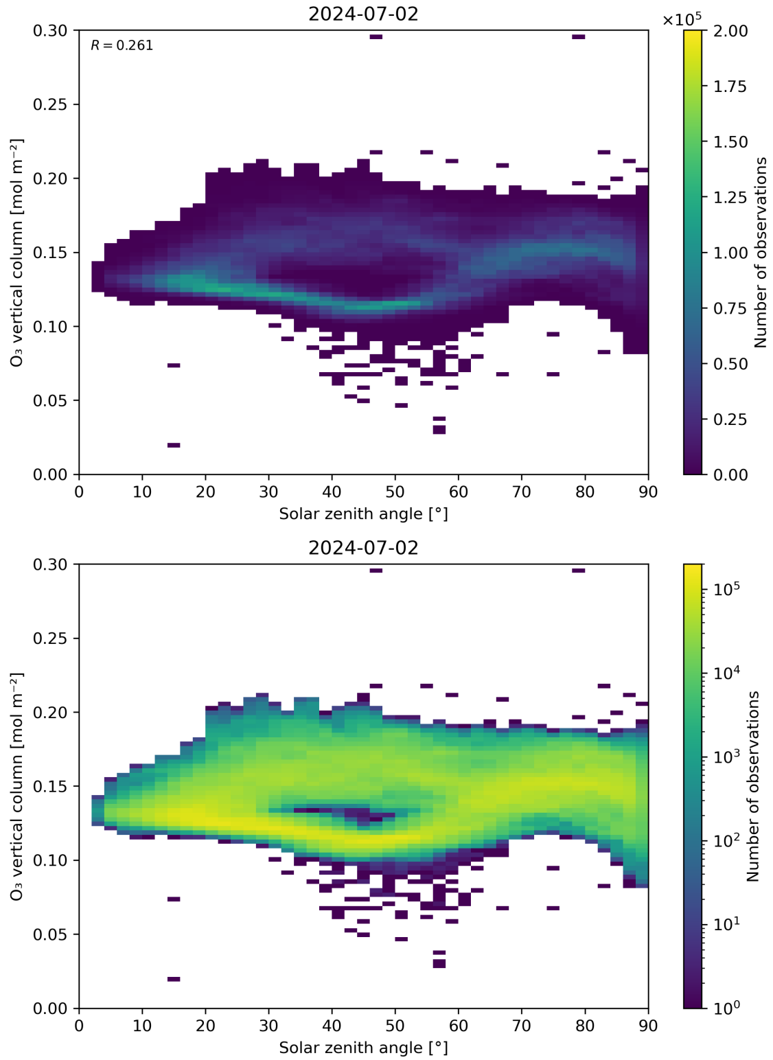
Figure 47: Scatter density plot of “Solar zenith angle” against “O 3 vertical column” for 2024-07-01 to 2024-07-03.
