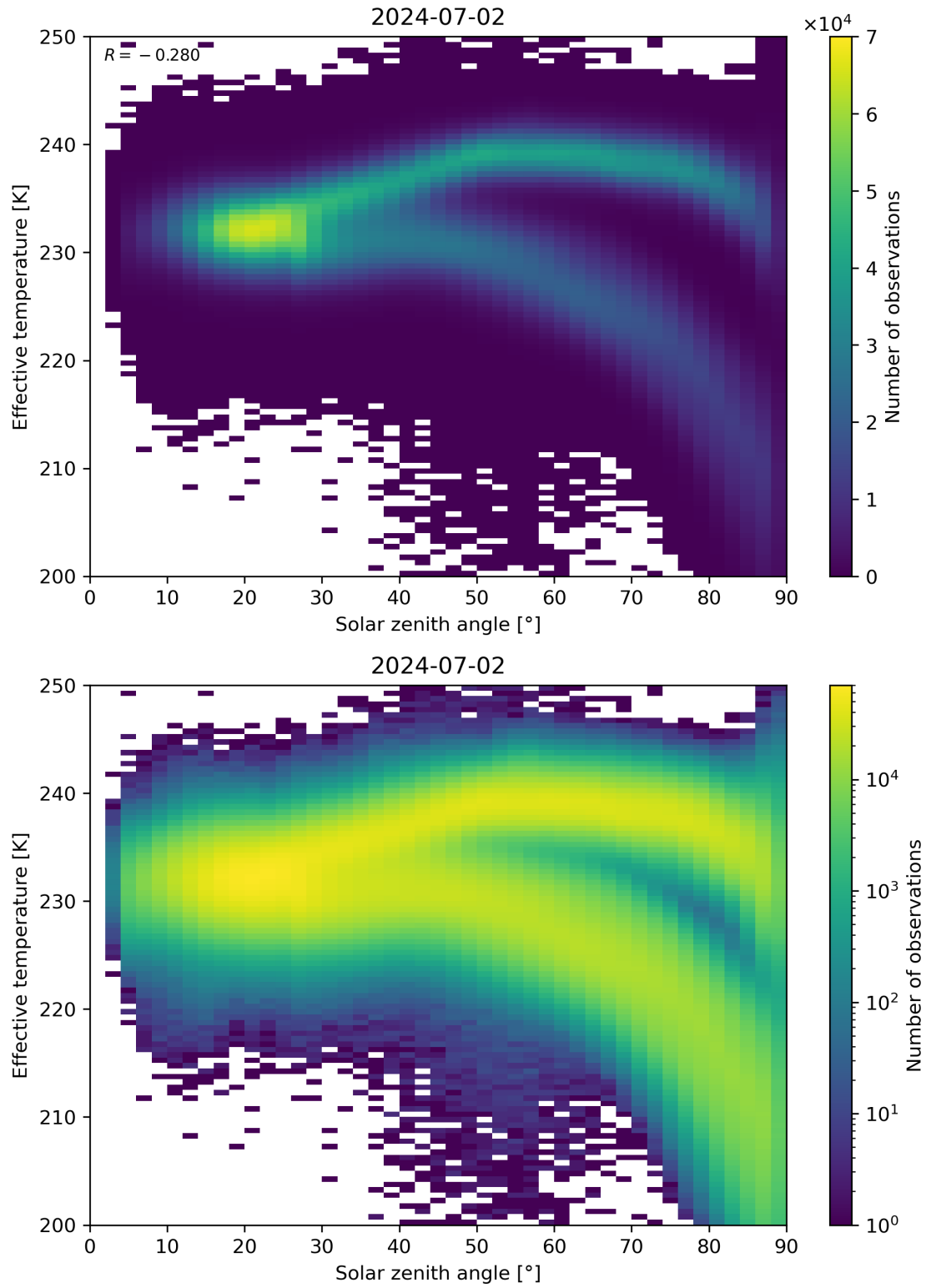
Figure 45: Scatter density plot of “Solar zenith angle” against “Effective temperature” for 2024-07-01 to 2024-07-03.
