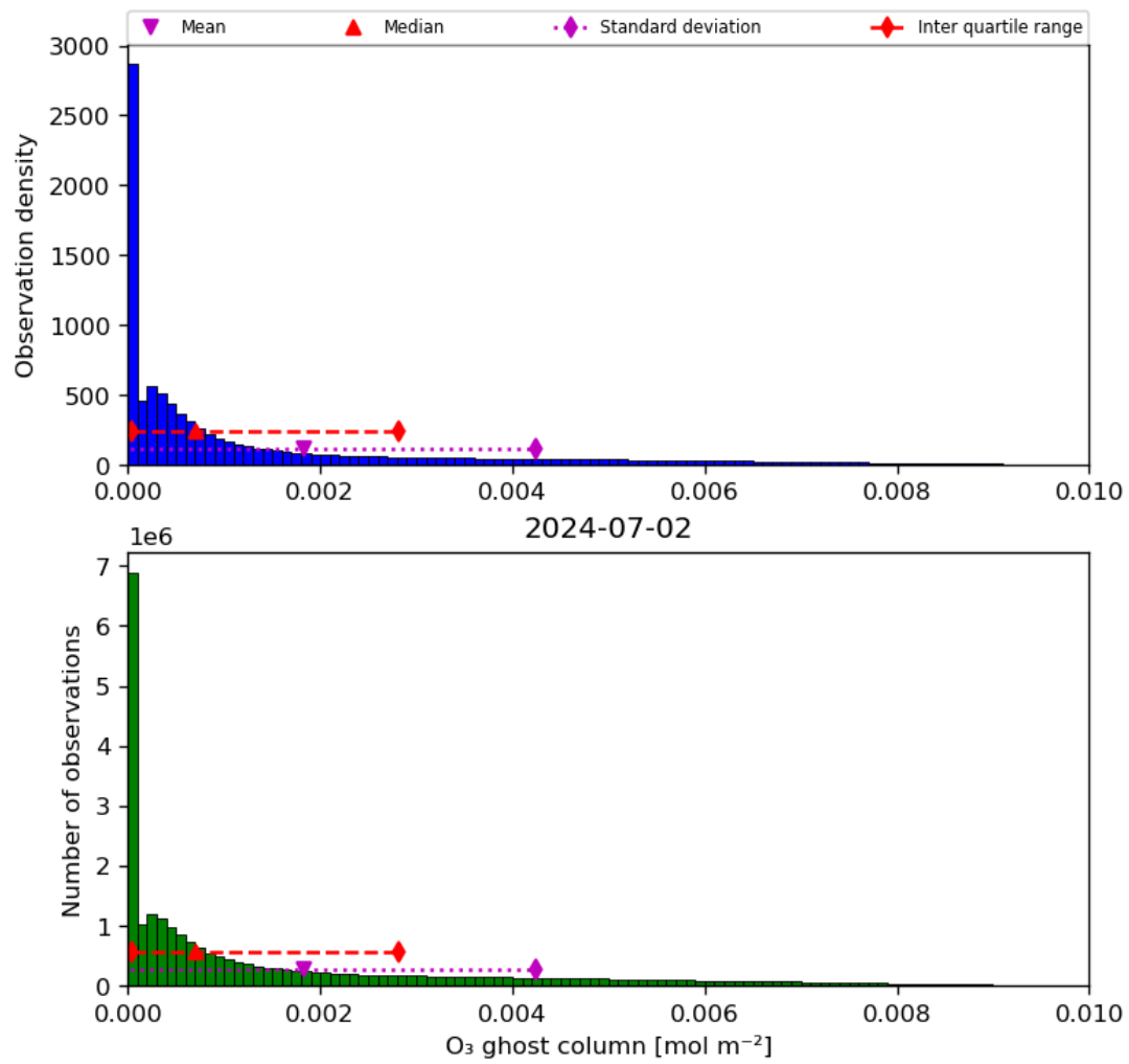
Figure 25: Histogram of "O 3 ghost column" for 2024-07-01 to 2024-07-03
