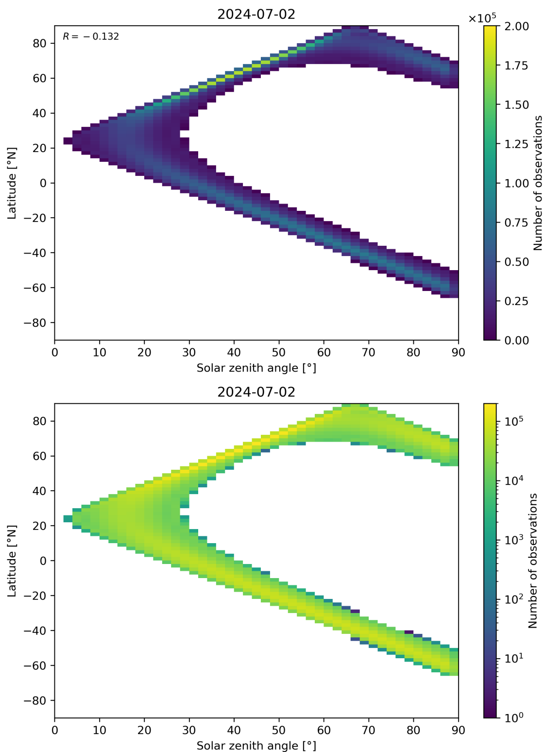
Figure 44: Scatter density plot of “Solar zenith angle” against “Latitude” for 2024-07-01 to 2024-07-03.
