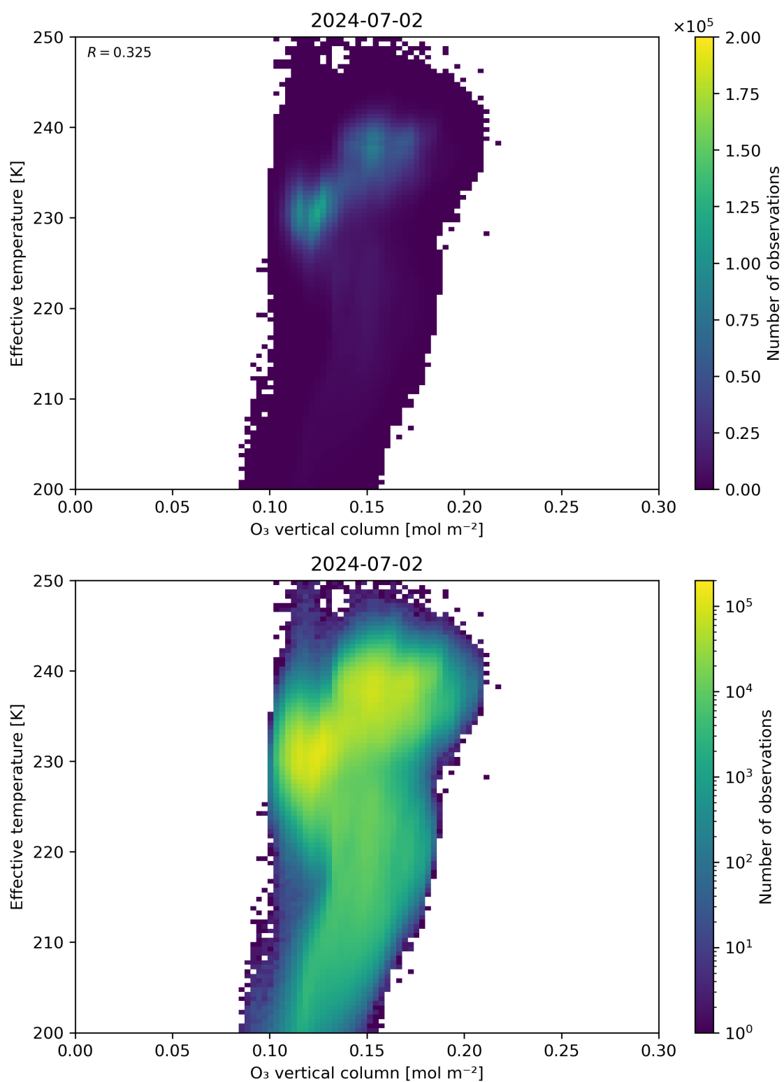
Figure 39: Scatter density plot of “O 3 vertical column” against “Effective temperature” for 2024-07-01 to 2024-07-03.
