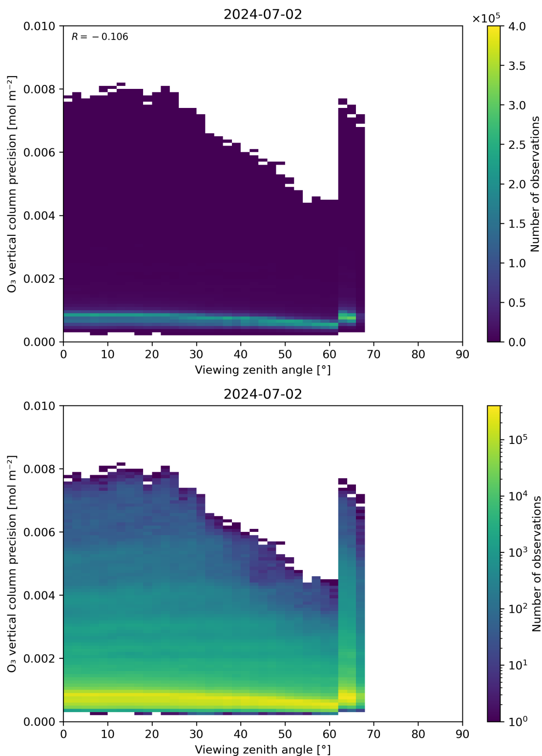
Figure 53: Scatter density plot of “Viewing zenith angle” against “O 3 vertical column precision” for 2024-07-01 to 2024-07-03.
