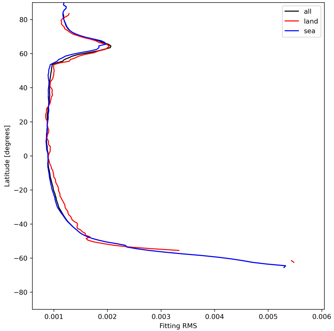
Figure 16: Zonal average of “Fitting RMS” for 2024-07-01 to 2024-07-03.
