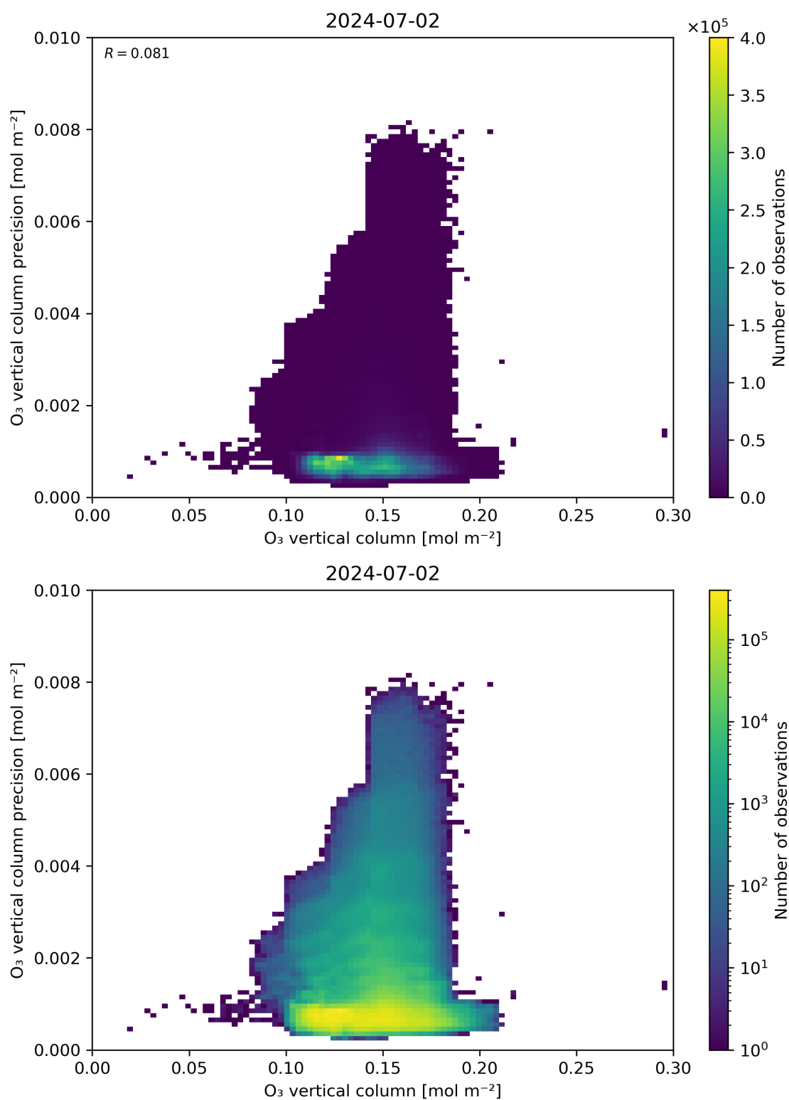
Figure 41: Scatter density plot of “O 3 vertical column” against “O 3 vertical column precision” for 2024-07-01 to 2024-07-03.
