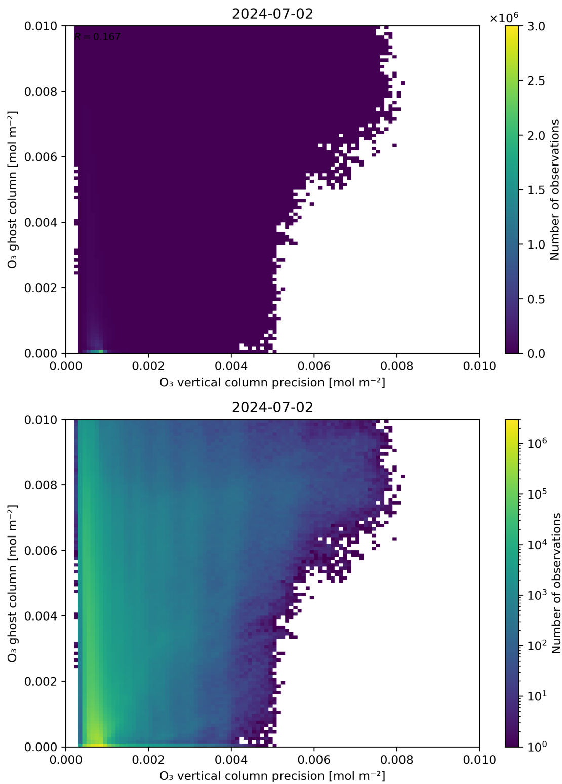
Figure 43: Scatter density plot of “ \text{O}_3 vertical column precision” against “ \text{O}_3 ghost column” for 2024-07-01 to 2024-07-03.
