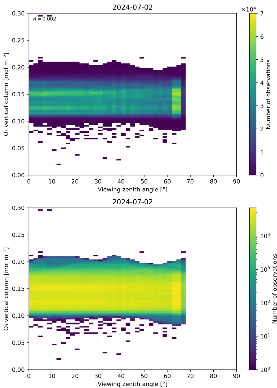
Figure 52: Scatter density plot of “Viewing zenith angle” against “O 3 vertical column” for 2024-07-01 to 2024-07-03.
