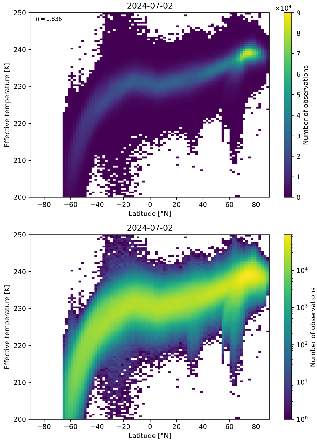
Figure 34: Scatter density plot of “Latitude” against “Effective temperature” for 2024-07-01 to 2024-07-03.
