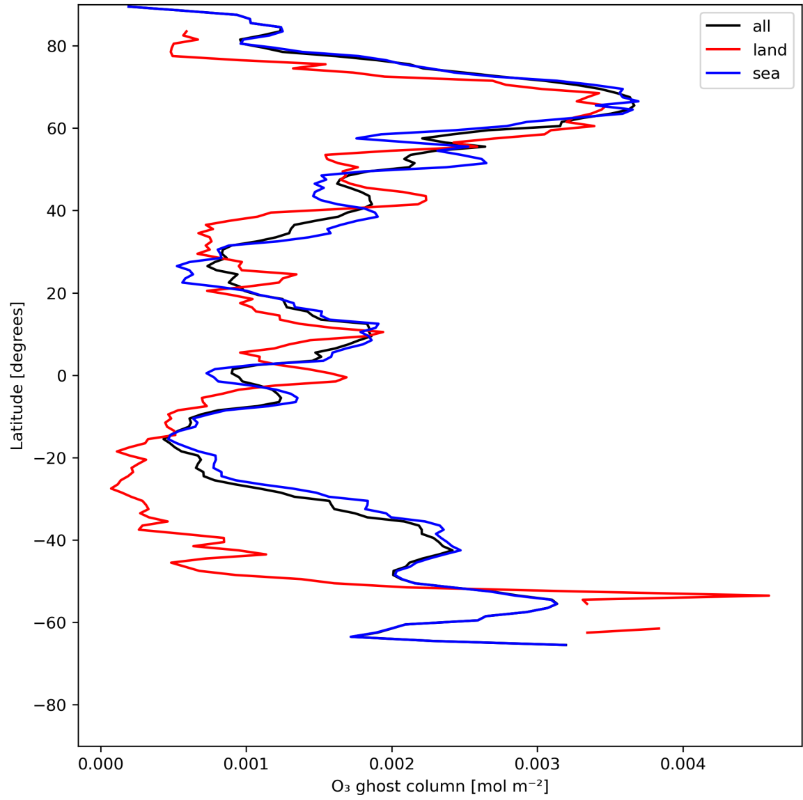
Figure 18: Zonal average of "O 3 ghost column" for 2024-07-01 to 2024-07-03.
