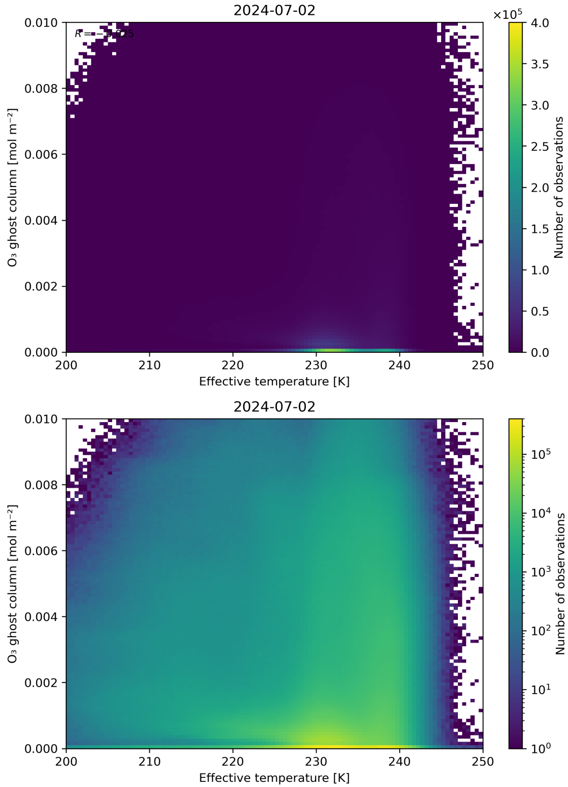
Figure 38: Scatter density plot of “Effective temperature” against “O 3 ghost column” for 2024-07-01 to 2024-07-03.
