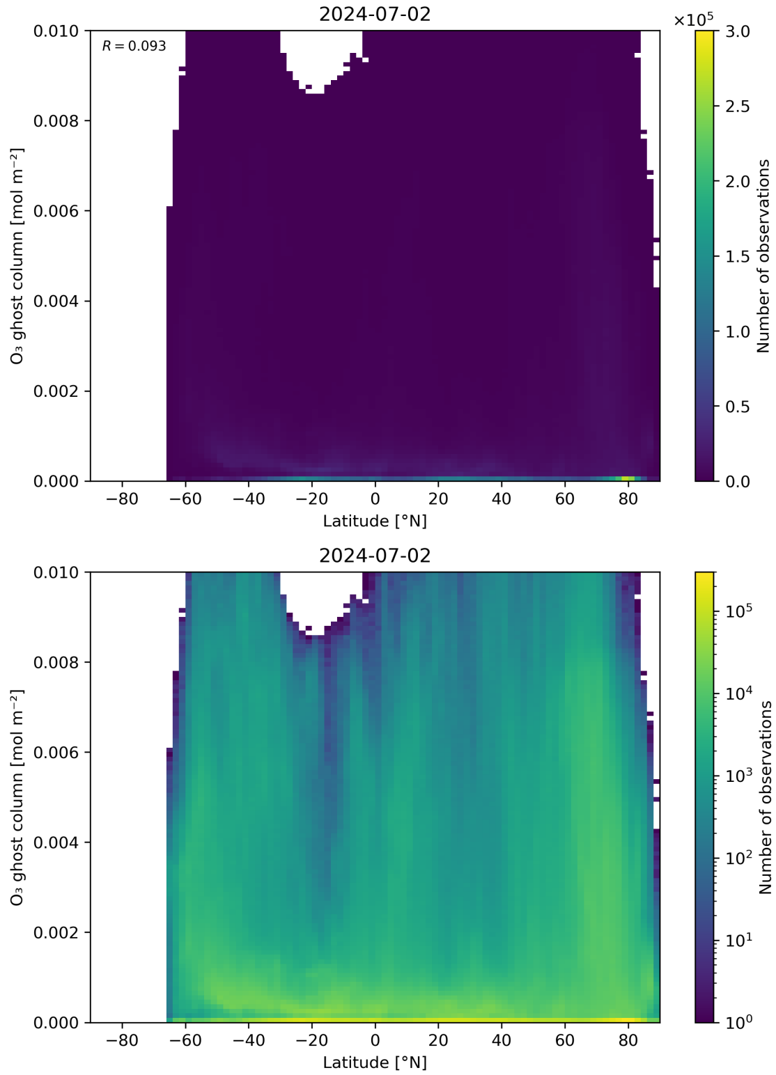
Figure 35: Scatter density plot of “Latitude” against “O 3 ghost column” for 2024-07-01 to 2024-07-03.
