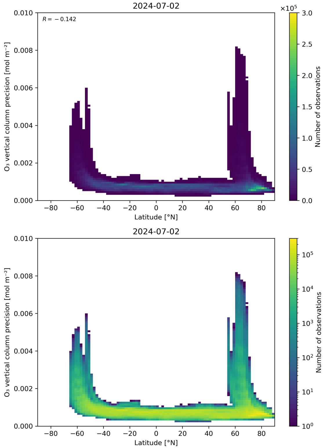
Figure 37: Scatter density plot of “Latitude” against “O 3 vertical column precision” for 2024-07-01 to 2024-07-03.
