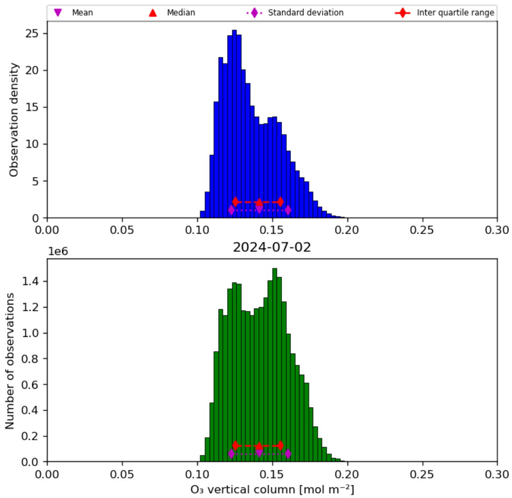
Figure 21: Histogram of “O 3 vertical column” for 2024-07-01 to 2024-07-03
