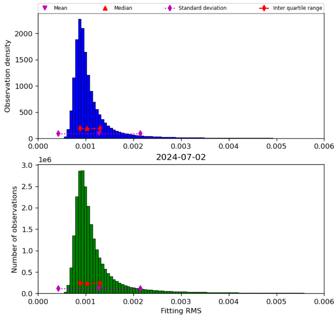
Figure 23: Histogram of “Fitting RMS” for 2024-07-01 to 2024-07-03
