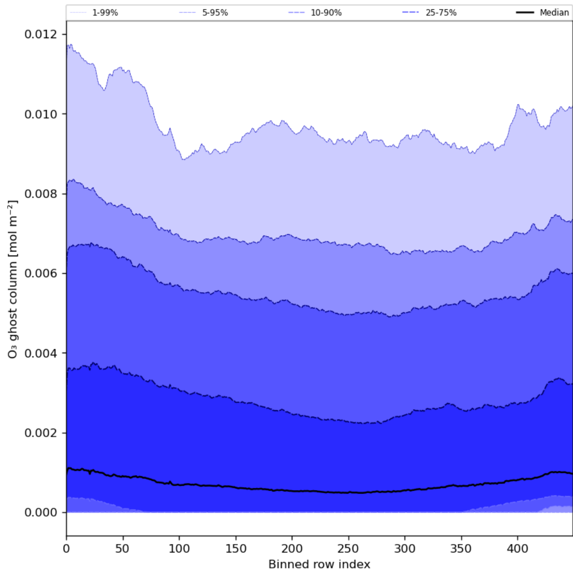
Figure 32: Along track statistics of “O 3 ghost column” for 2024-07-01 to 2024-07-03
