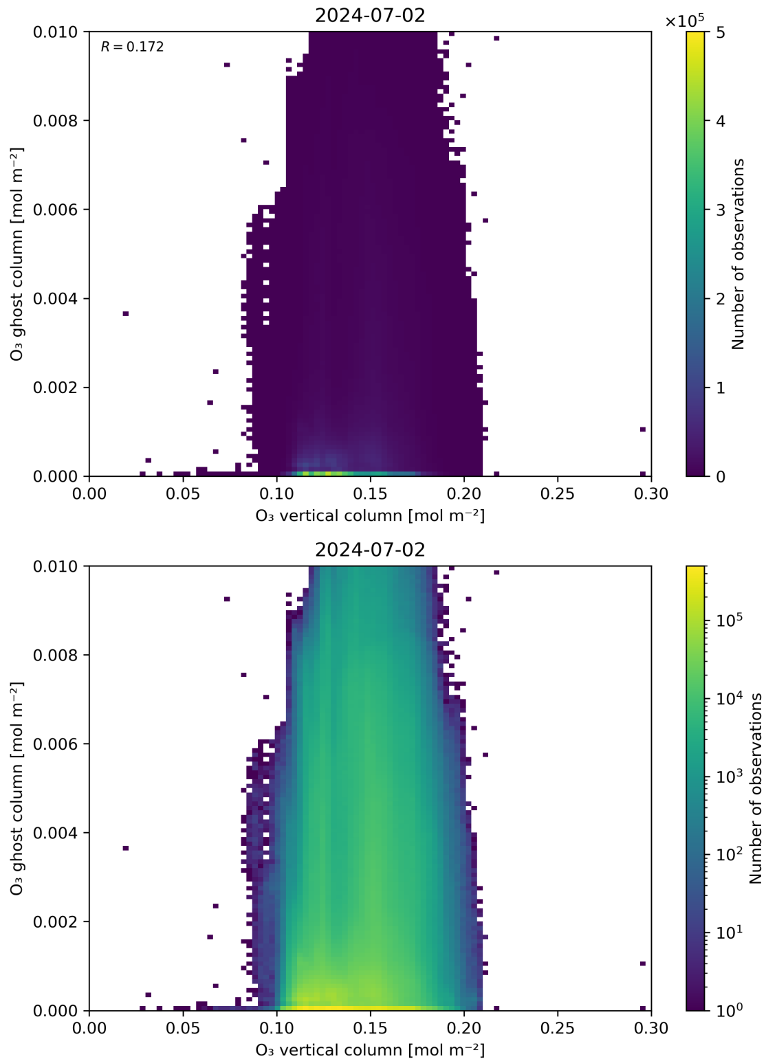
Figure 40: Scatter density plot of “O 3 vertical column” against “O 3 ghost column” for 2024-07-01 to 2024-07-03.
