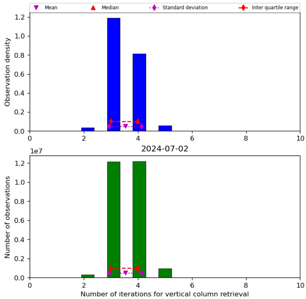
Figure 26: Histogram of “Number of iterations for vertical column retrieval” for 2024-07-01 to 2024-07-03
