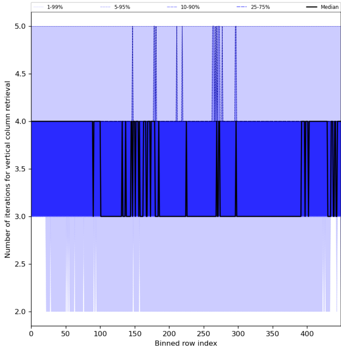
Figure 33: Along track statistics of “Number of iterations for vertical column retrieval” for 2024-07-01 to 2024-07-03
