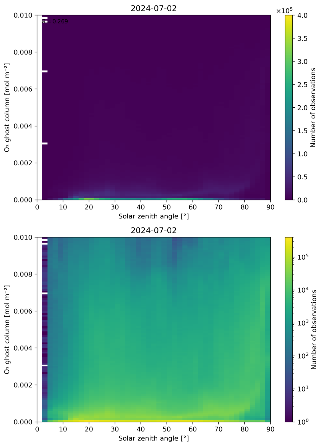
Figure 46: Scatter density plot of “Solar zenith angle” against “O 3 ghost column” for 2024-07-01 to 2024-07-03.
