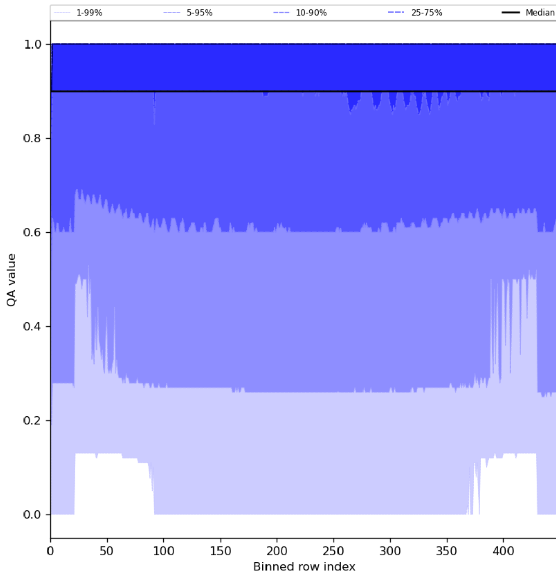
Figure 27: Along track statistics of “QA value” for 2024-07-01 to 2024-07-03
