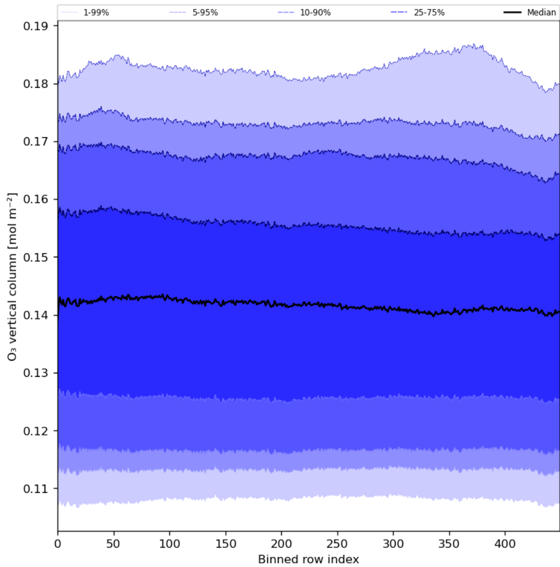
Figure 28: Along track statistics of “O 3 vertical column” for 2024-07-01 to 2024-07-03
