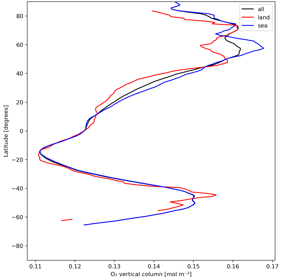
Figure 14: Zonal average of “O 3 vertical column” for 2024-07-01 to 2024-07-03.
