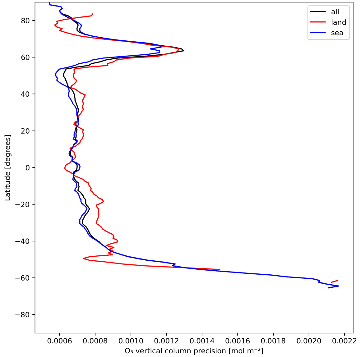
Figure 15: Zonal average of “O 3 vertical column precision” for 2024-07-01 to 2024-07-03.
