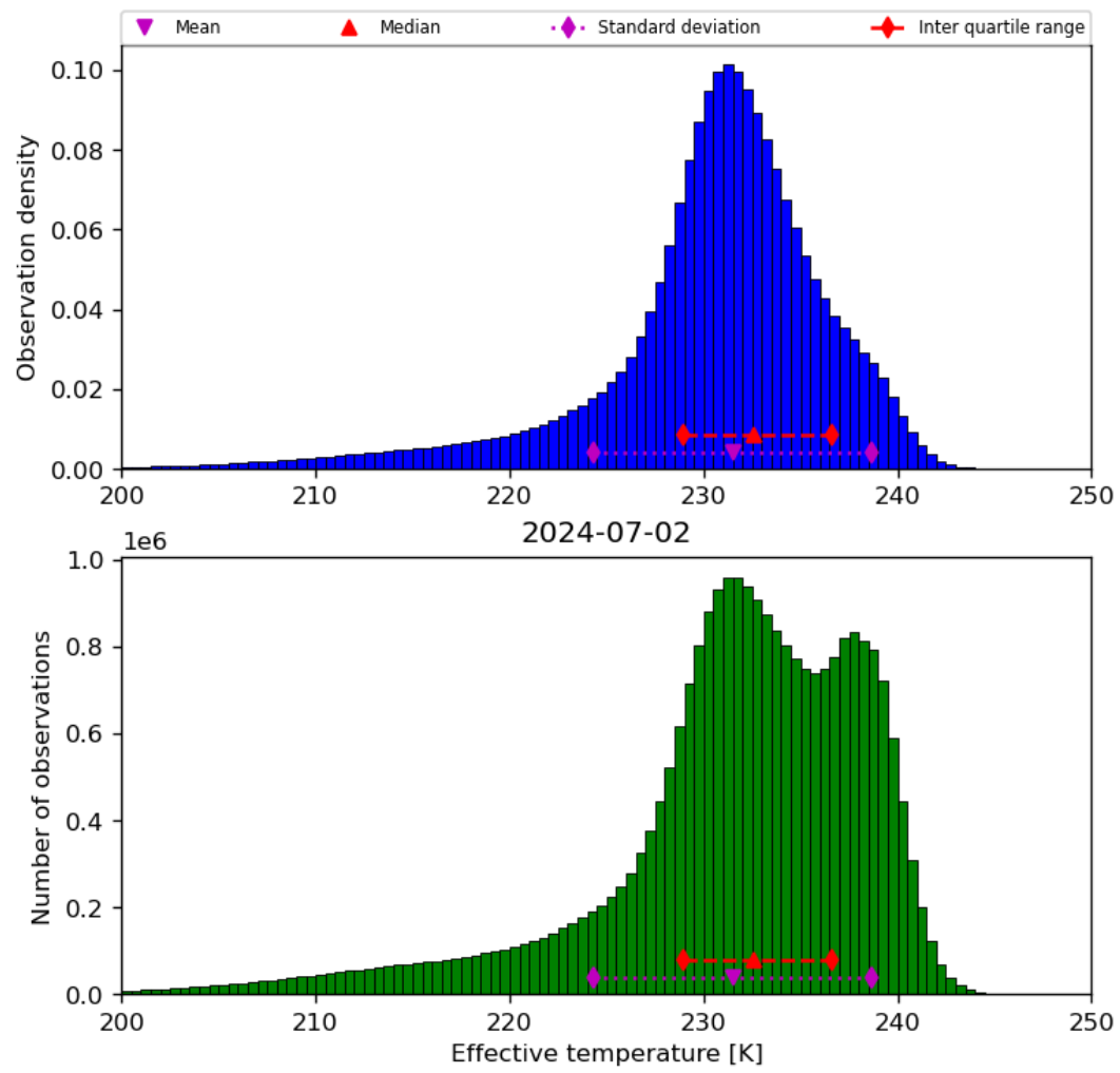
Figure 24: Histogram of “Effective temperature” for 2024-07-01 to 2024-07-03
