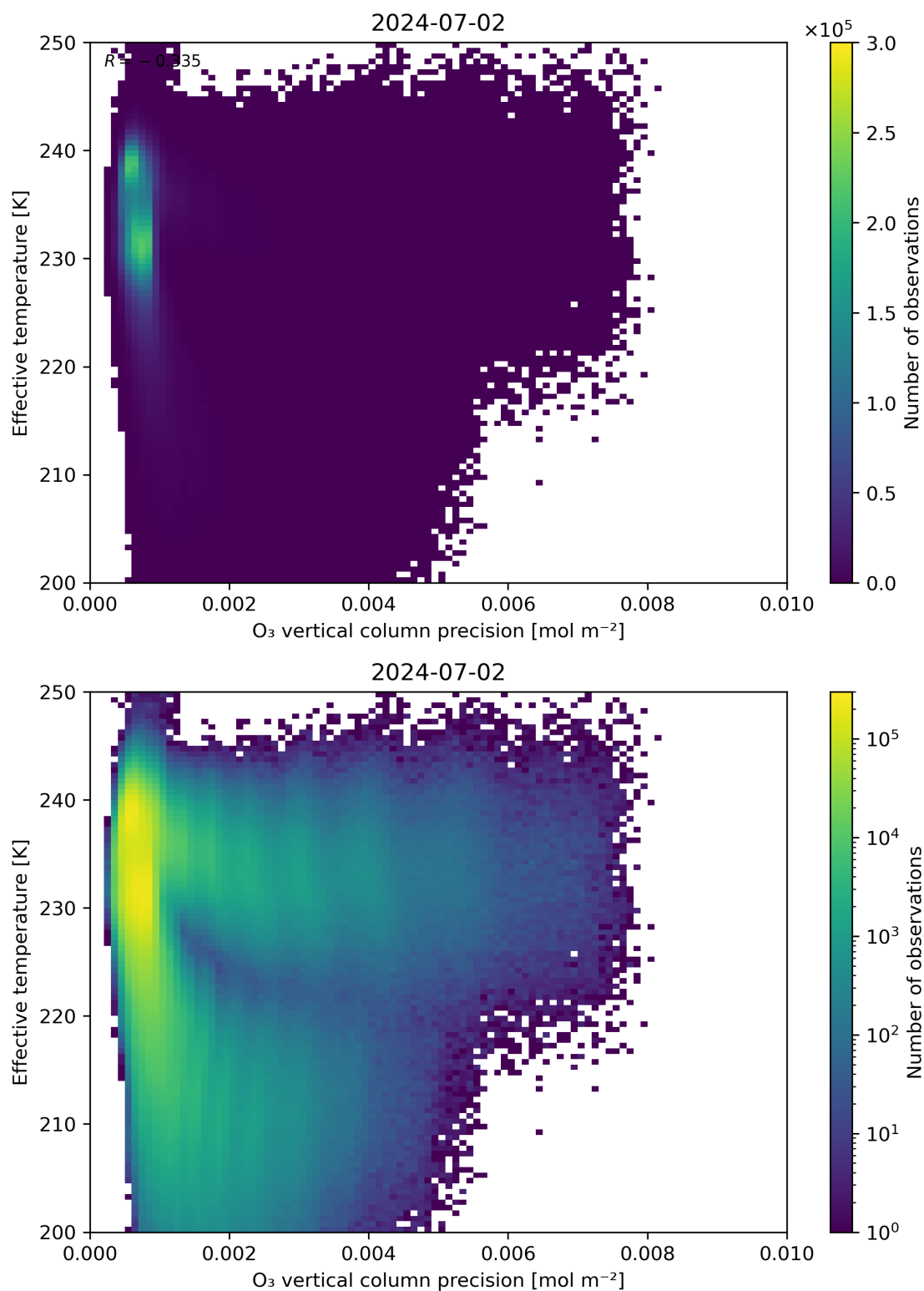
Figure 42: Scatter density plot of “O 3 vertical column precision” against “Effective temperature” for 2024-07-01 to 2024-07-03.
