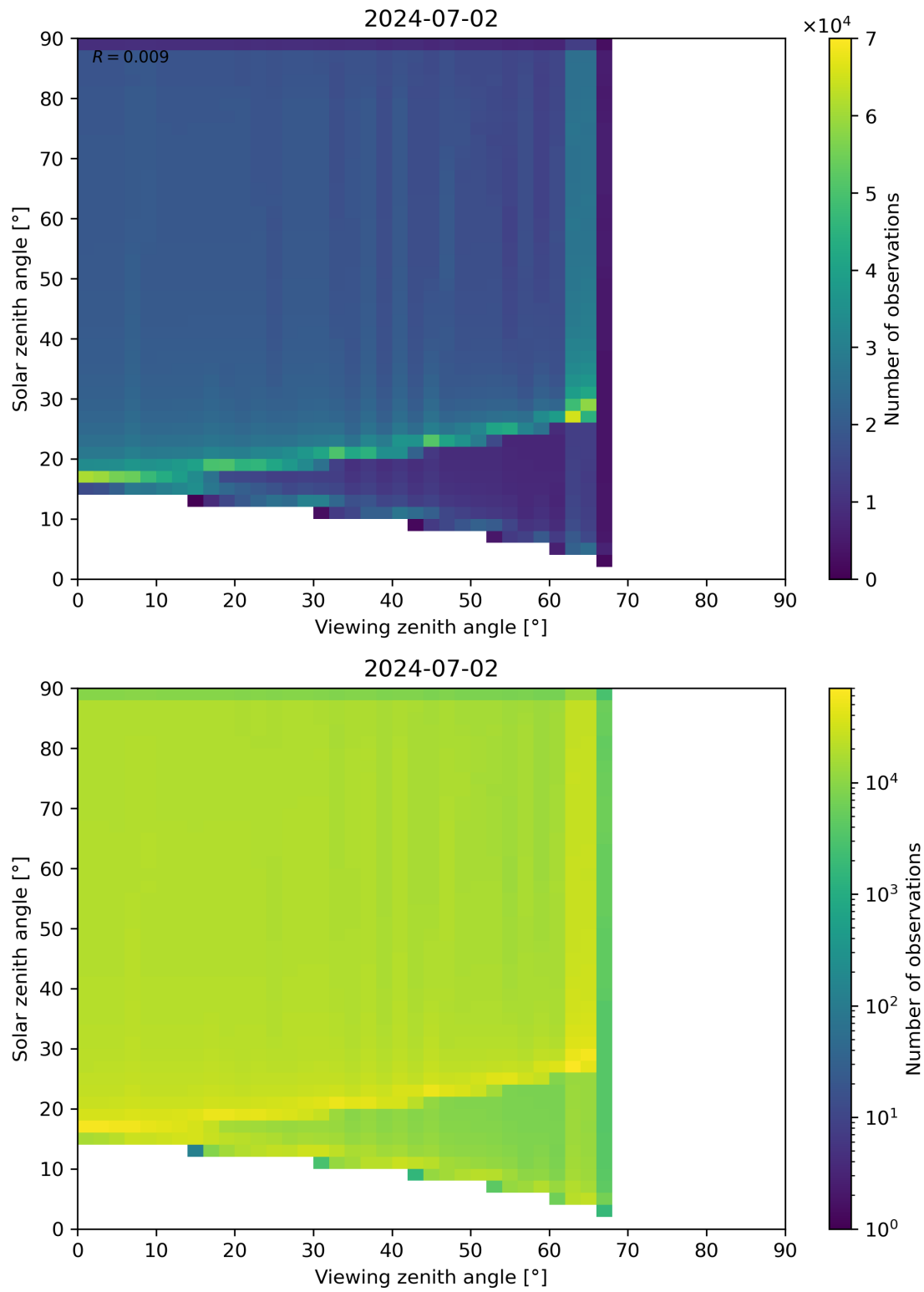
Figure 54: Scatter density plot of “Viewing zenith angle” against “Solar zenith angle” for 2024-07-01 to 2024-07-03.
