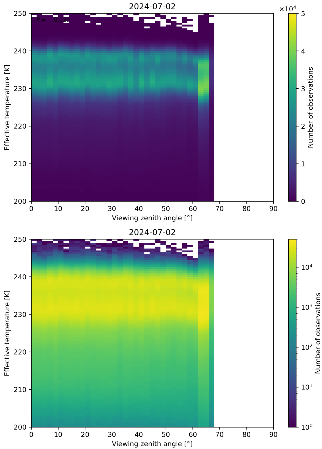
Figure 50: Scatter density plot of “Viewing zenith angle” against “Effective temperature” for 2024-07-01 to 2024-07-03.
