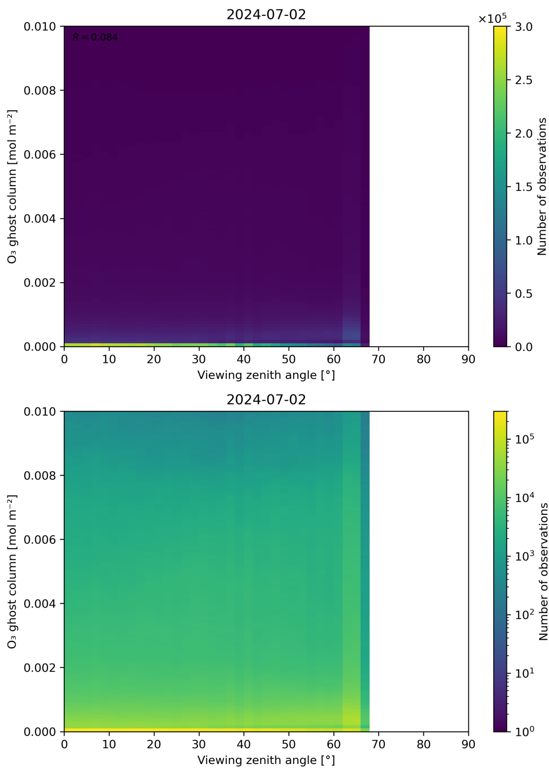
Figure 51: Scatter density plot of “Viewing zenith angle” against “O 3 ghost column” for 2024-07-01 to 2024-07-03.
