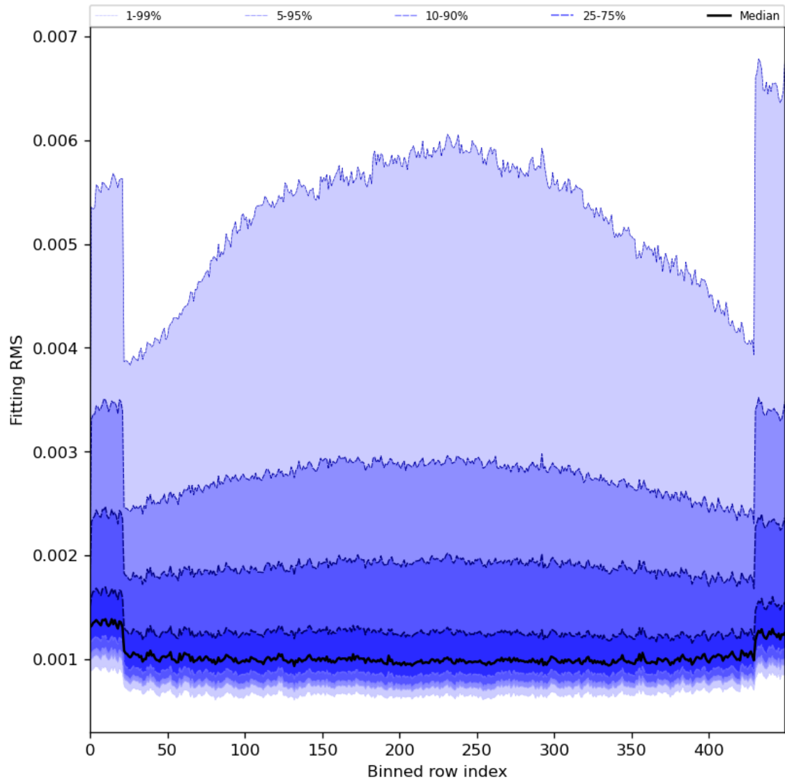
Figure 30: Along track statistics of “Fitting RMS” for 2024-07-03 to 2024-07-05
