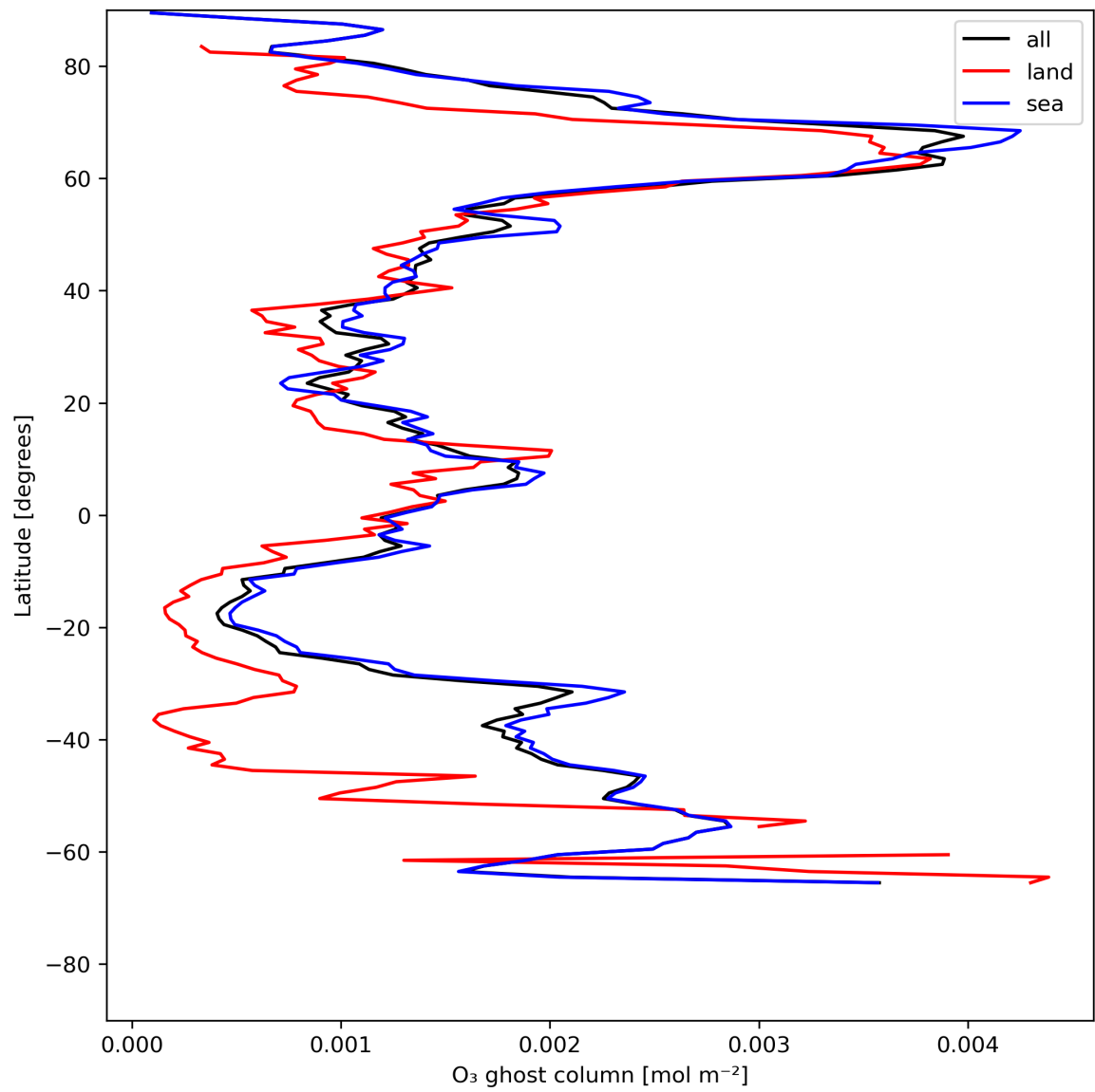
Figure 18: Zonal average of “O 3 ghost column” for 2024-07-03 to 2024-07-05.
