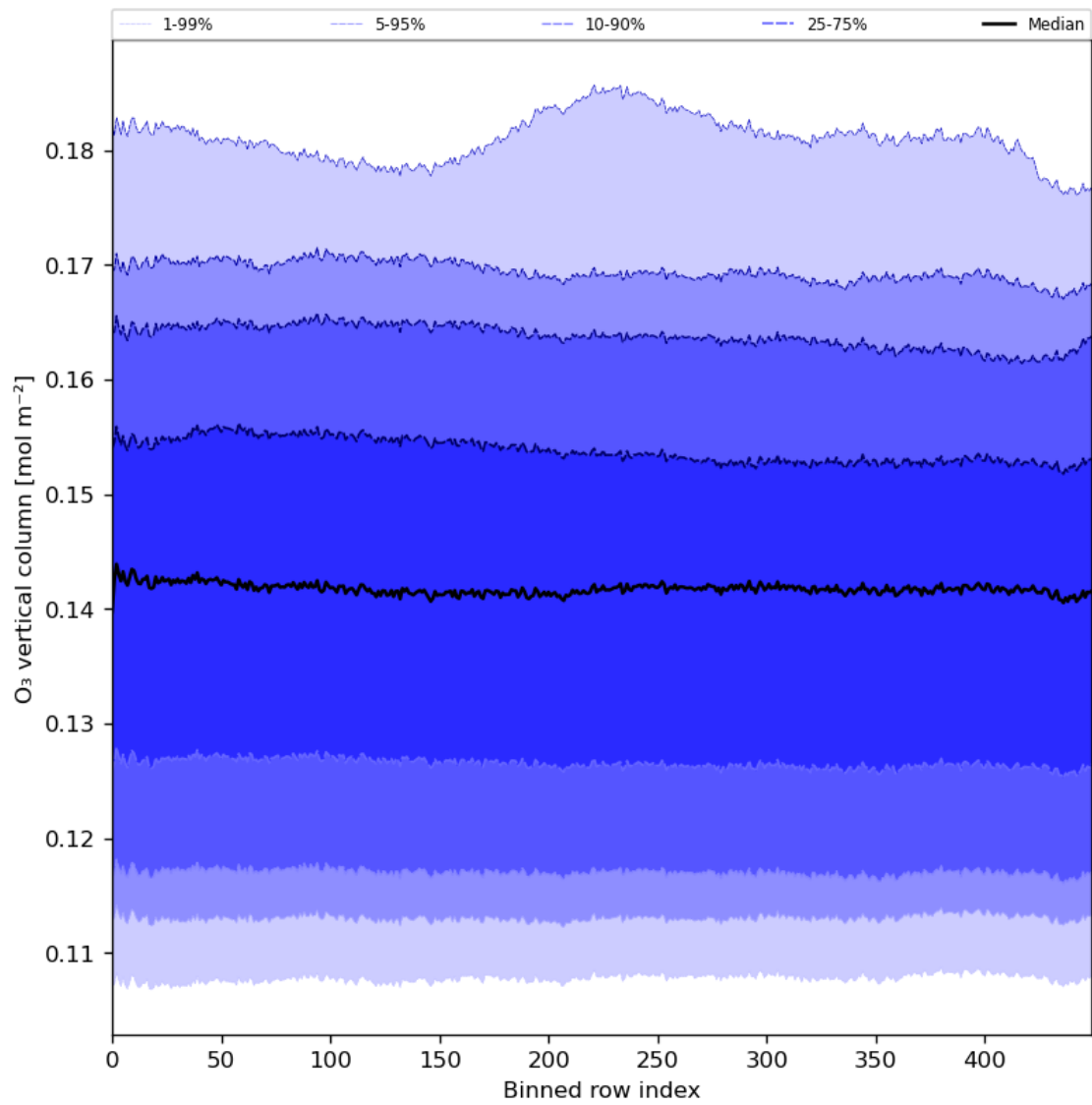
Figure 28: Along track statistics of “O 3 vertical column” for 2024-07-03 to 2024-07-05
