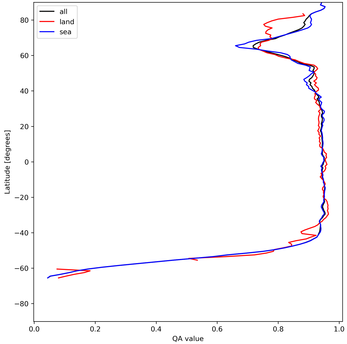
Figure 13: Zonal average of “QA value” for 2024-07-03 to 2024-07-05.
