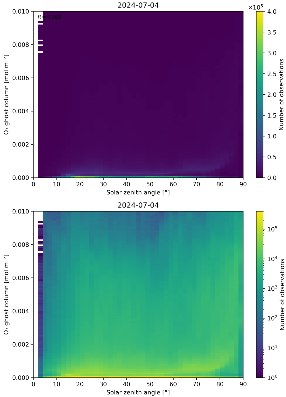
Figure 46: Scatter density plot of “Solar zenith angle” against “O 3 ghost column” for 2024-07-03 to 2024-07-05.
