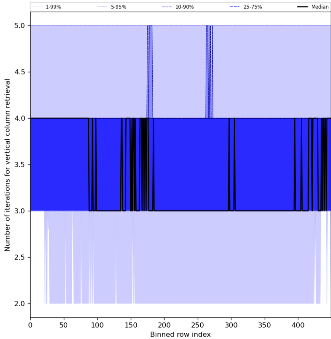
Figure 33: Along track statistics of “Number of iterations for vertical column retrieval” for 2024-07-03 to 2024-07-05
