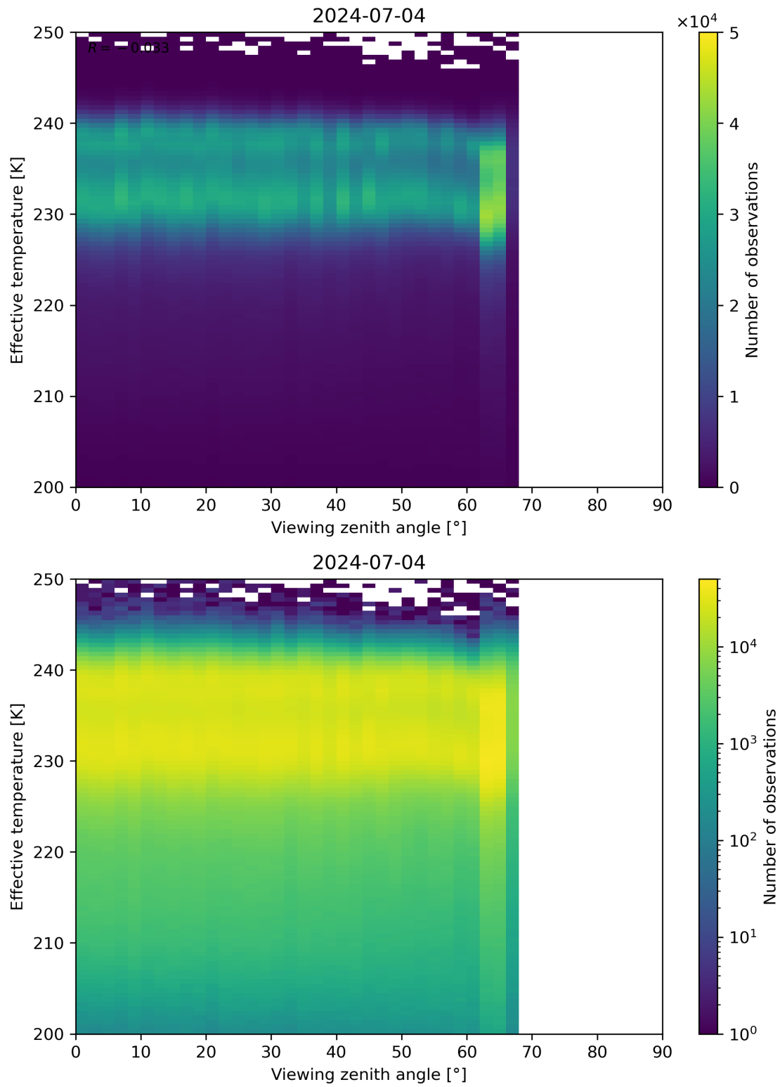
Figure 50: Scatter density plot of “Viewing zenith angle” against “Effective temperature” for 2024-07-03 to 2024-07-05.
