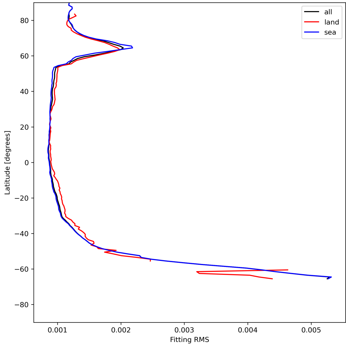
Figure 16: Zonal average of “Fitting RMS” for 2024-07-03 to 2024-07-05.
