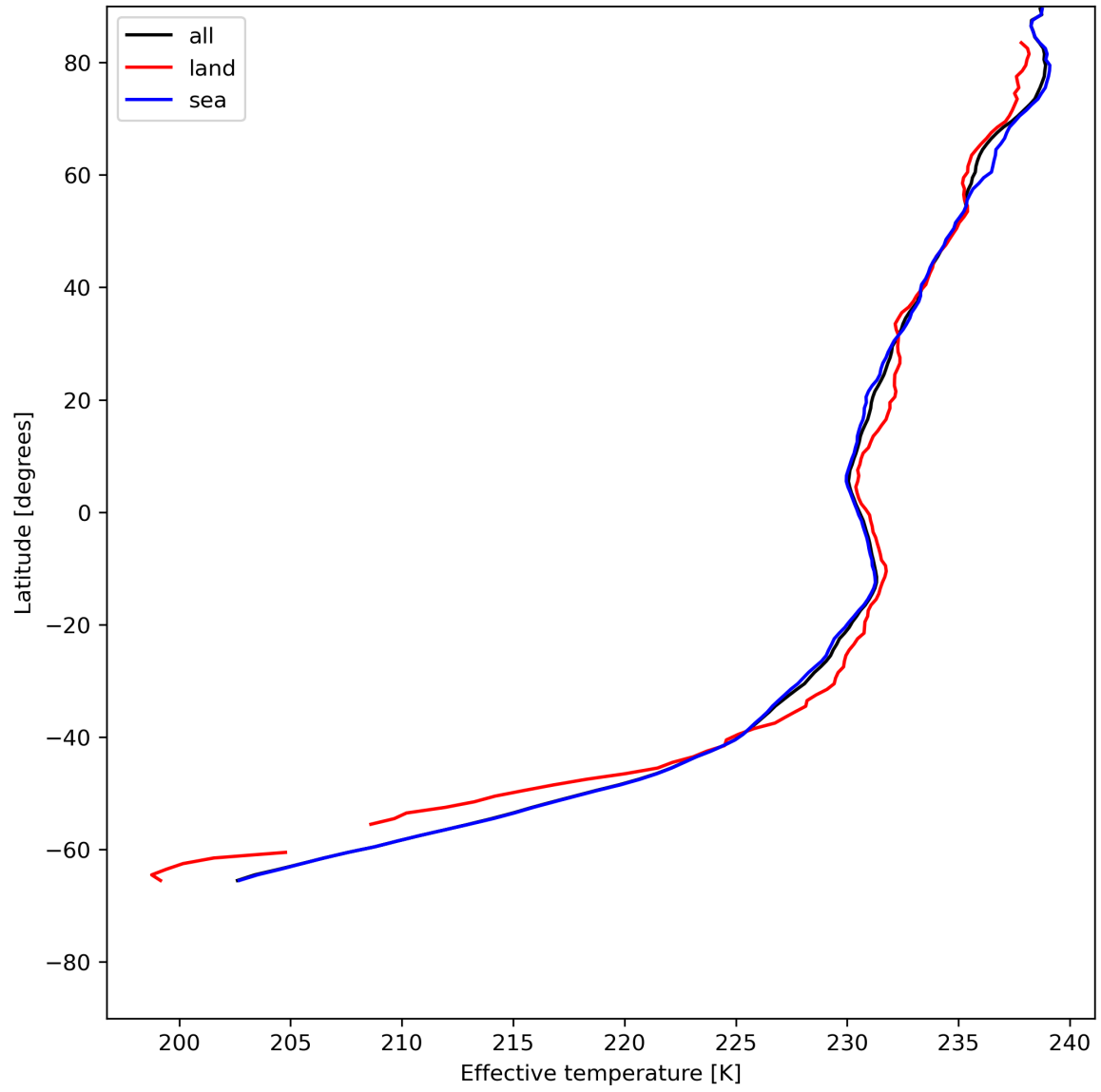
Figure 17: Zonal average of “Effective temperature” for 2024-07-03 to 2024-07-05.
