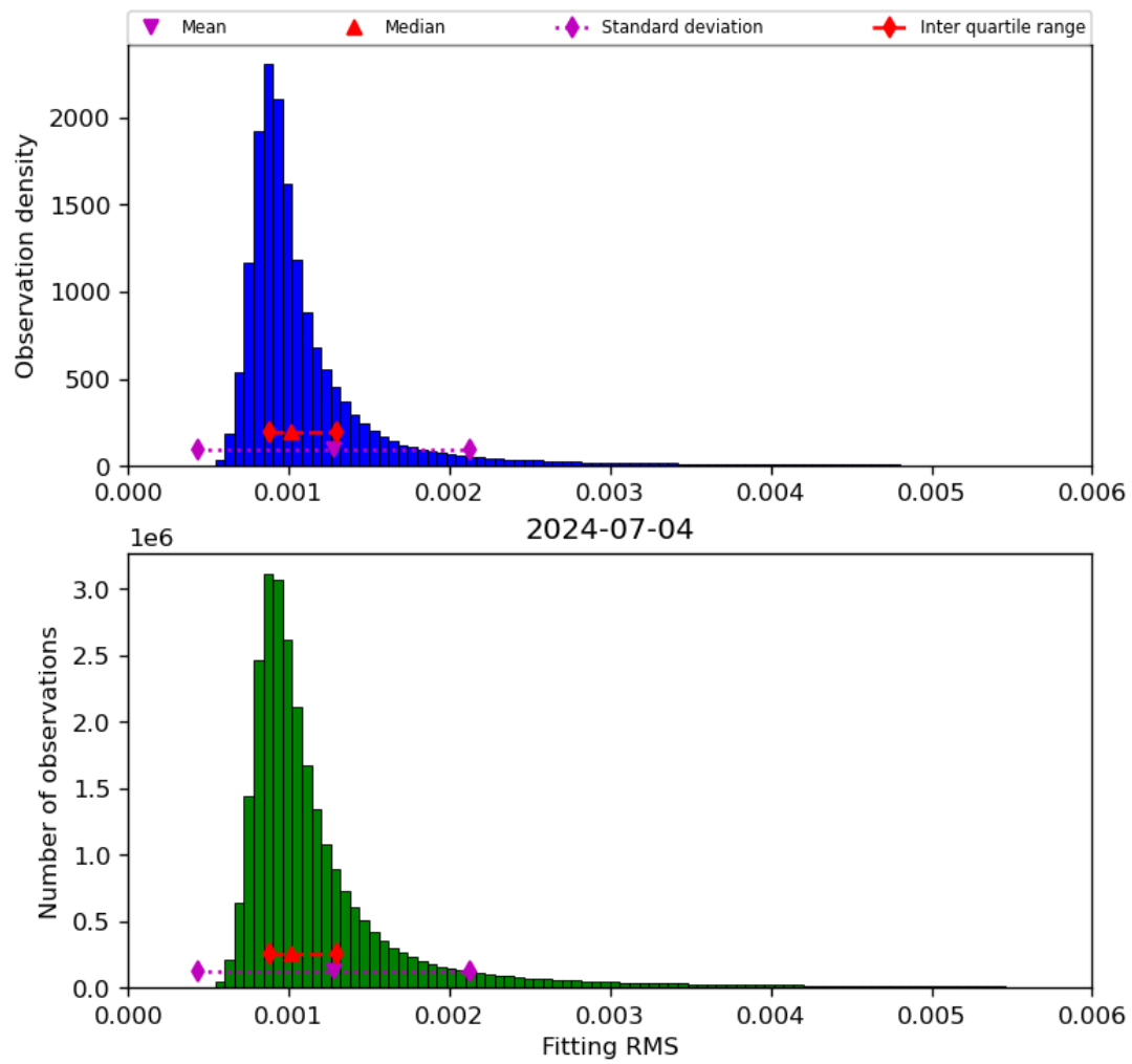
Figure 23: Histogram of “Fitting RMS” for 2024-07-03 to 2024-07-05
