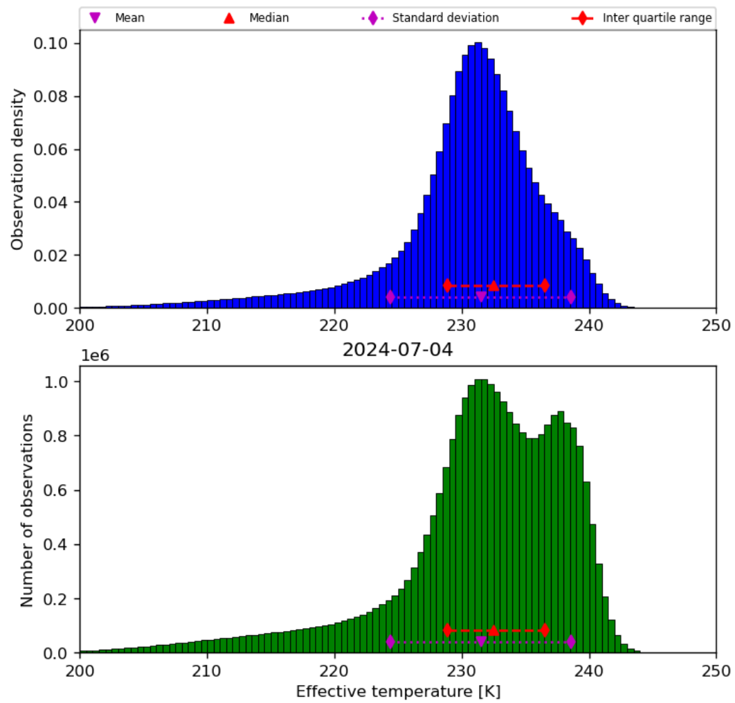
Figure 24: Histogram of “Effective temperature” for 2024-07-03 to 2024-07-05
