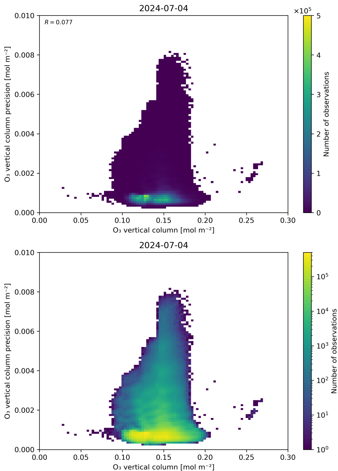
Figure 41: Scatter density plot of "O 3 vertical column" against "O 3 vertical column precision" for 2024-07-03 to 2024-07-05.
