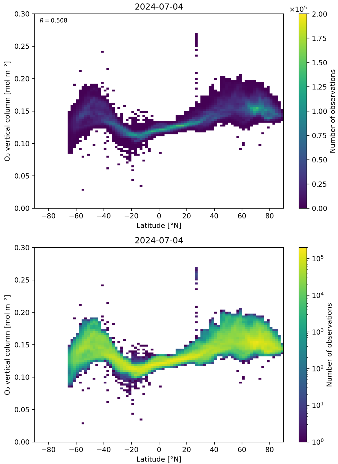
Figure 36: Scatter density plot of “Latitude” against “O 3 vertical column” for 2024-07-03 to 2024-07-05.
