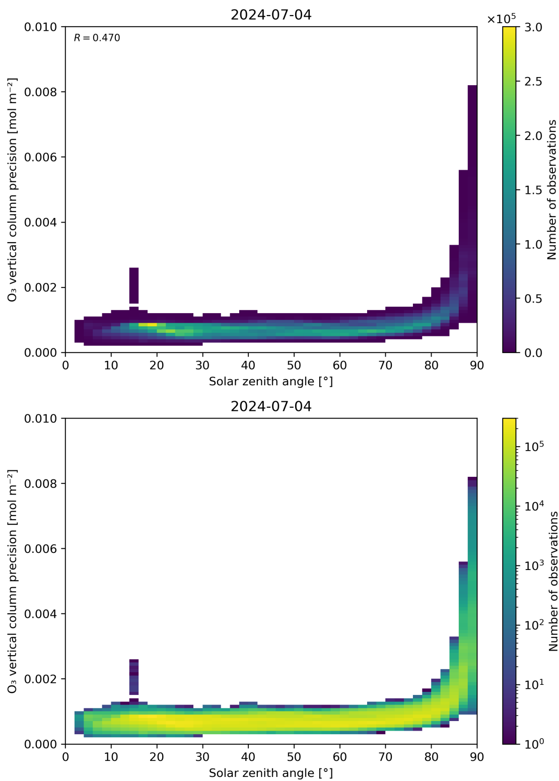
Figure 48: Scatter density plot of “Solar zenith angle” against “O 3 vertical column precision” for 2024-07-03 to 2024-07-05.
