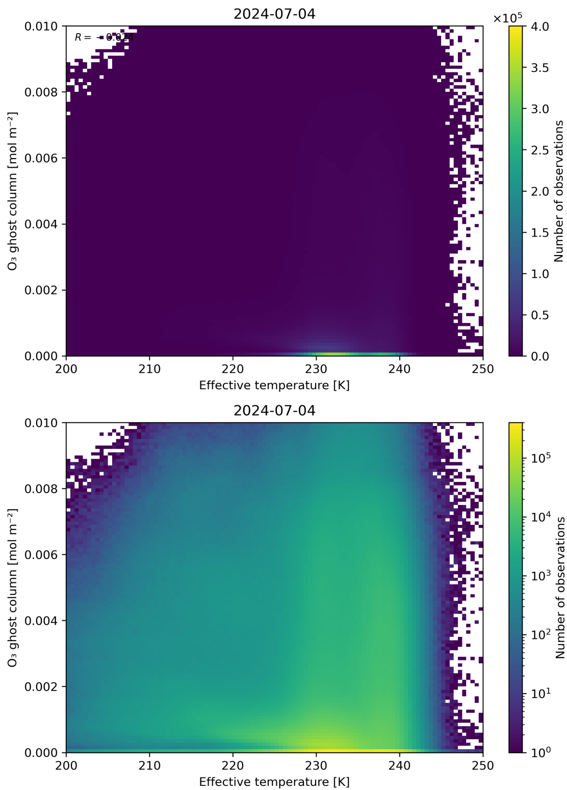
Figure 38: Scatter density plot of “Effective temperature” against “O 3 ghost column” for 2024-07-03 to 2024-07-05.
