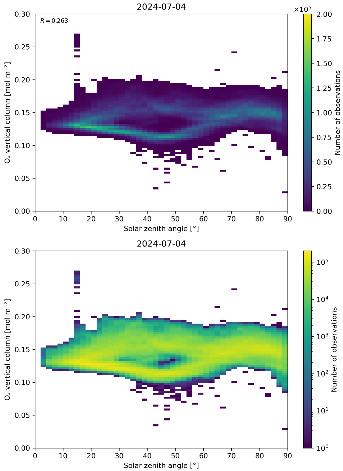
Figure 47: Scatter density plot of “Solar zenith angle” against “O 3 vertical column” for 2024-07-03 to 2024-07-05.
