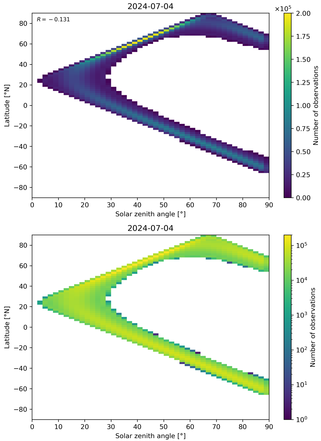
Figure 44: Scatter density plot of “Solar zenith angle” against “Latitude” for 2024-07-03 to 2024-07-05.
