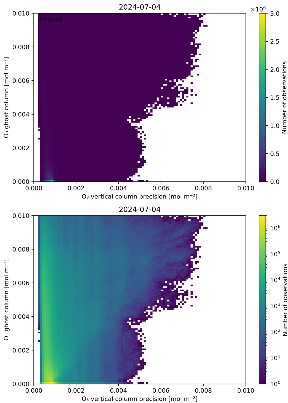
Figure 43: Scatter density plot of “ \text{O}_3 vertical column precision” against “ \text{O}_3 ghost column” for 2024-07-03 to 2024-07-05.
