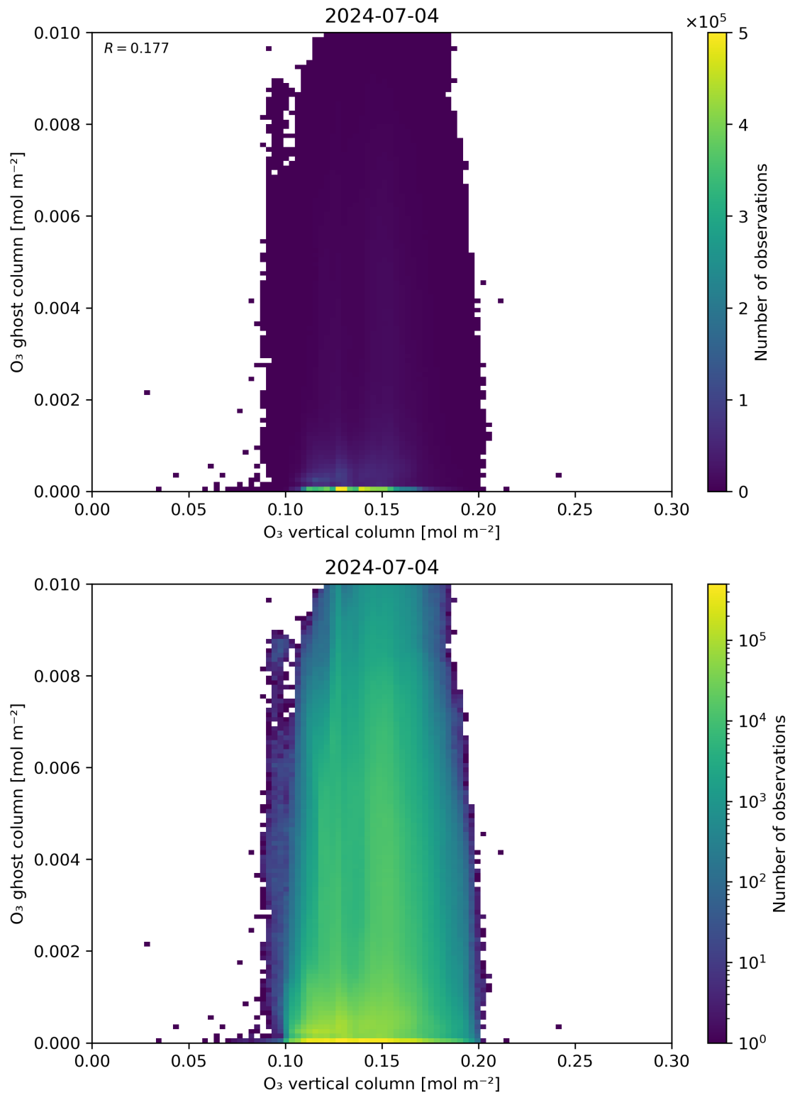
Figure 40: Scatter density plot of “O 3 vertical column” against “O 3 ghost column” for 2024-07-03 to 2024-07-05.
