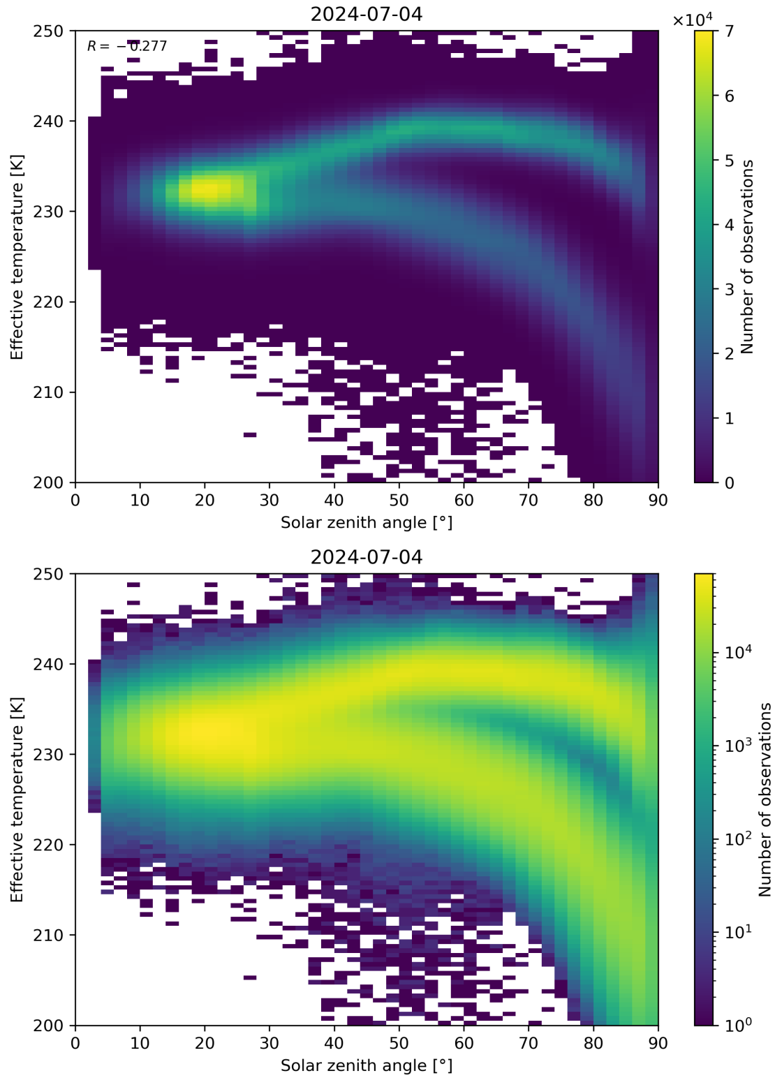
Figure 45: Scatter density plot of “Solar zenith angle” against “Effective temperature” for 2024-07-03 to 2024-07-05.
