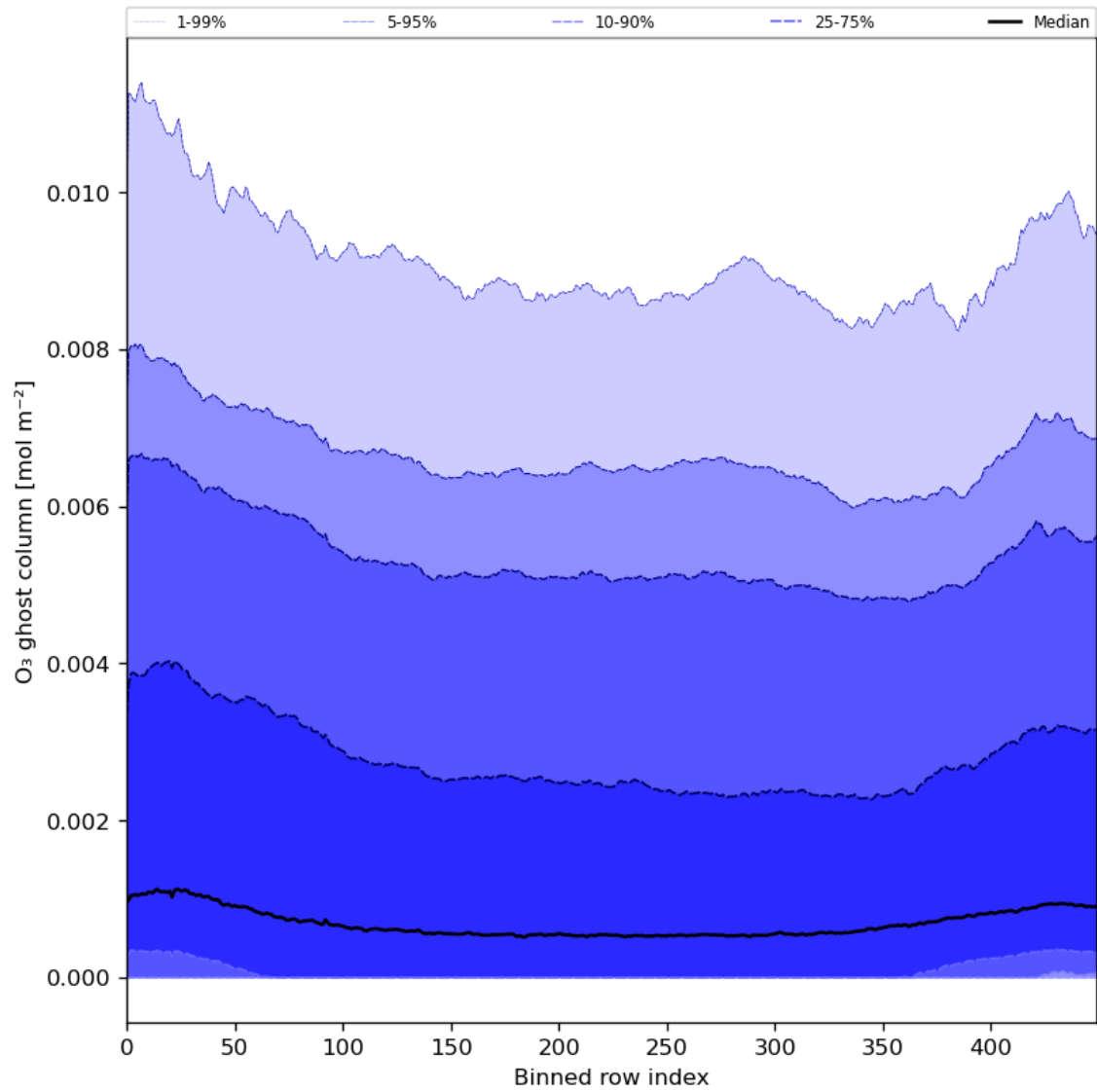
Figure 32: Along track statistics of "O 3 ghost column" for 2024-07-03 to 2024-07-05
