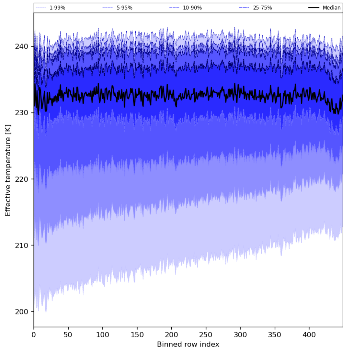
Figure 31: Along track statistics of “Effective temperature” for 2024-07-03 to 2024-07-05
