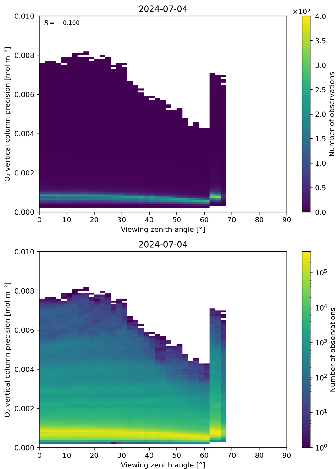
Figure 53: Scatter density plot of “Viewing zenith angle” against “O 3 vertical column precision” for 2024-07-03 to 2024-07-05.
