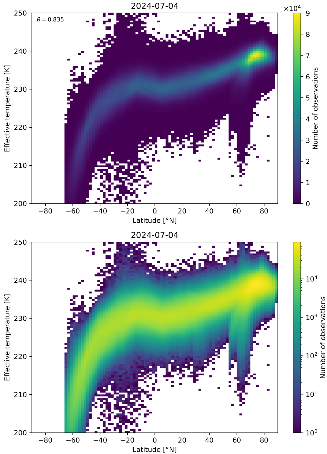
Figure 34: Scatter density plot of “Latitude” against “Effective temperature” for 2024-07-03 to 2024-07-05.
