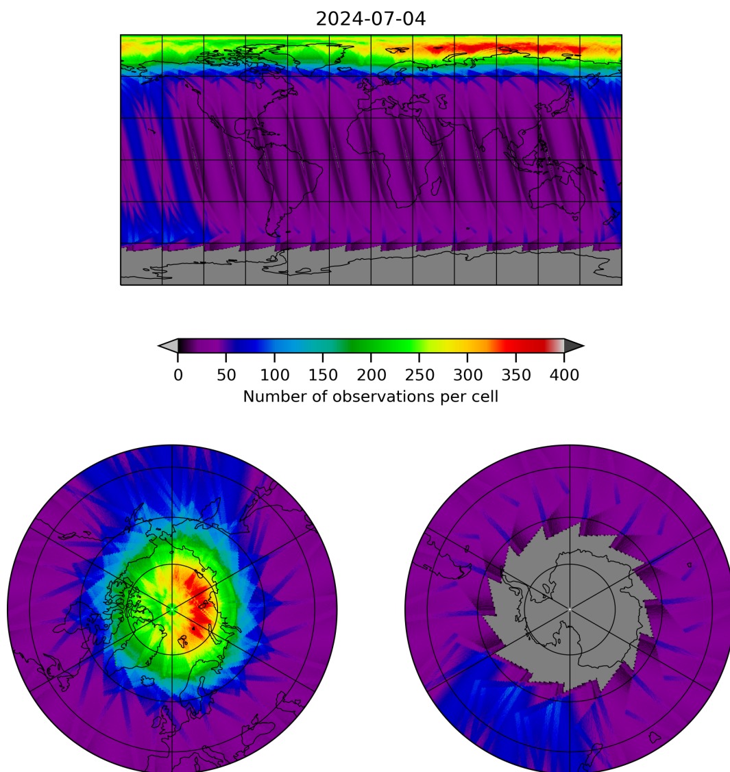
Figure 12: Map of the number of observations for 2024-07-03 to 2024-07-05
