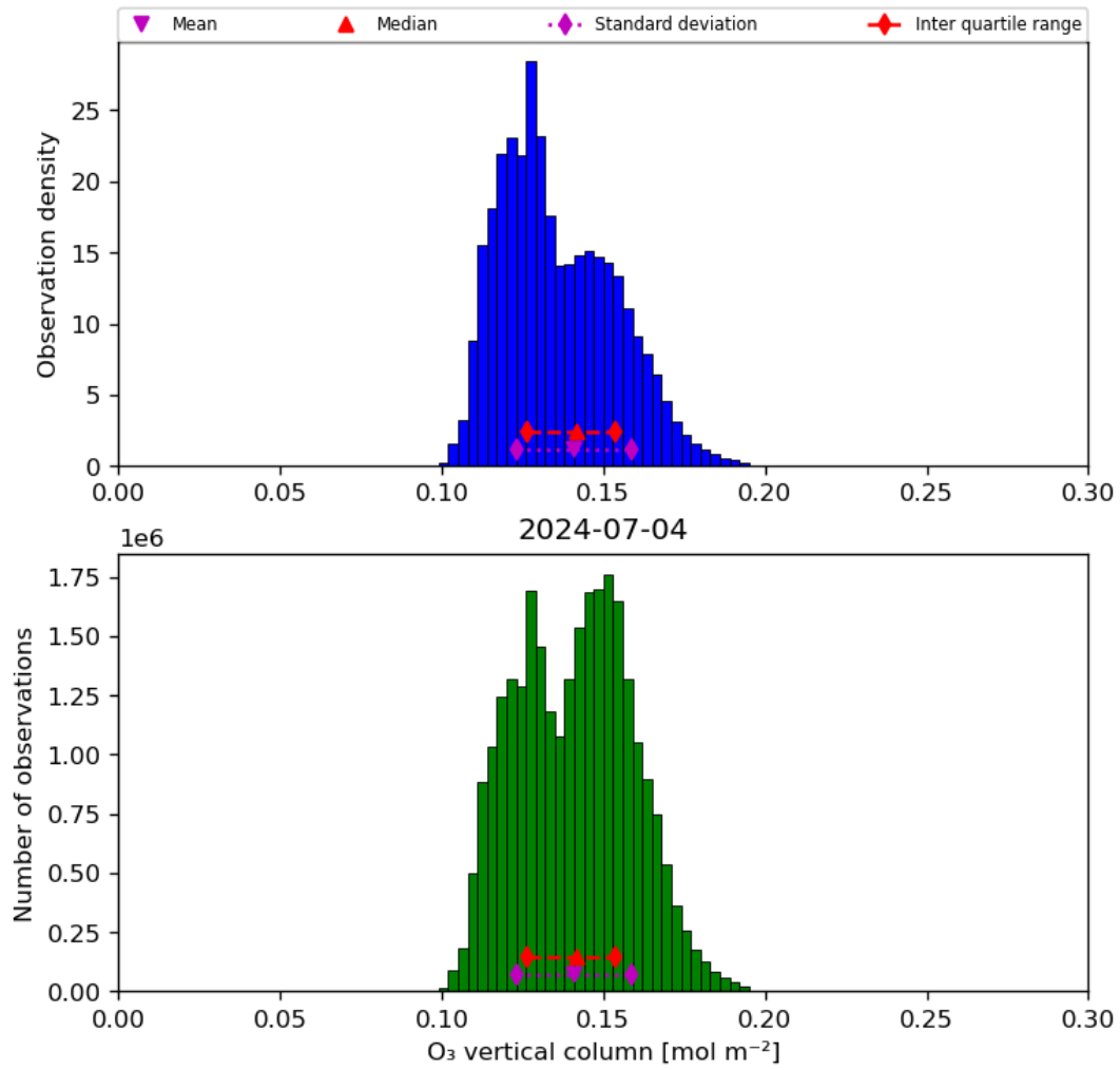
Figure 21: Histogram of “O 3 vertical column” for 2024-07-03 to 2024-07-05
