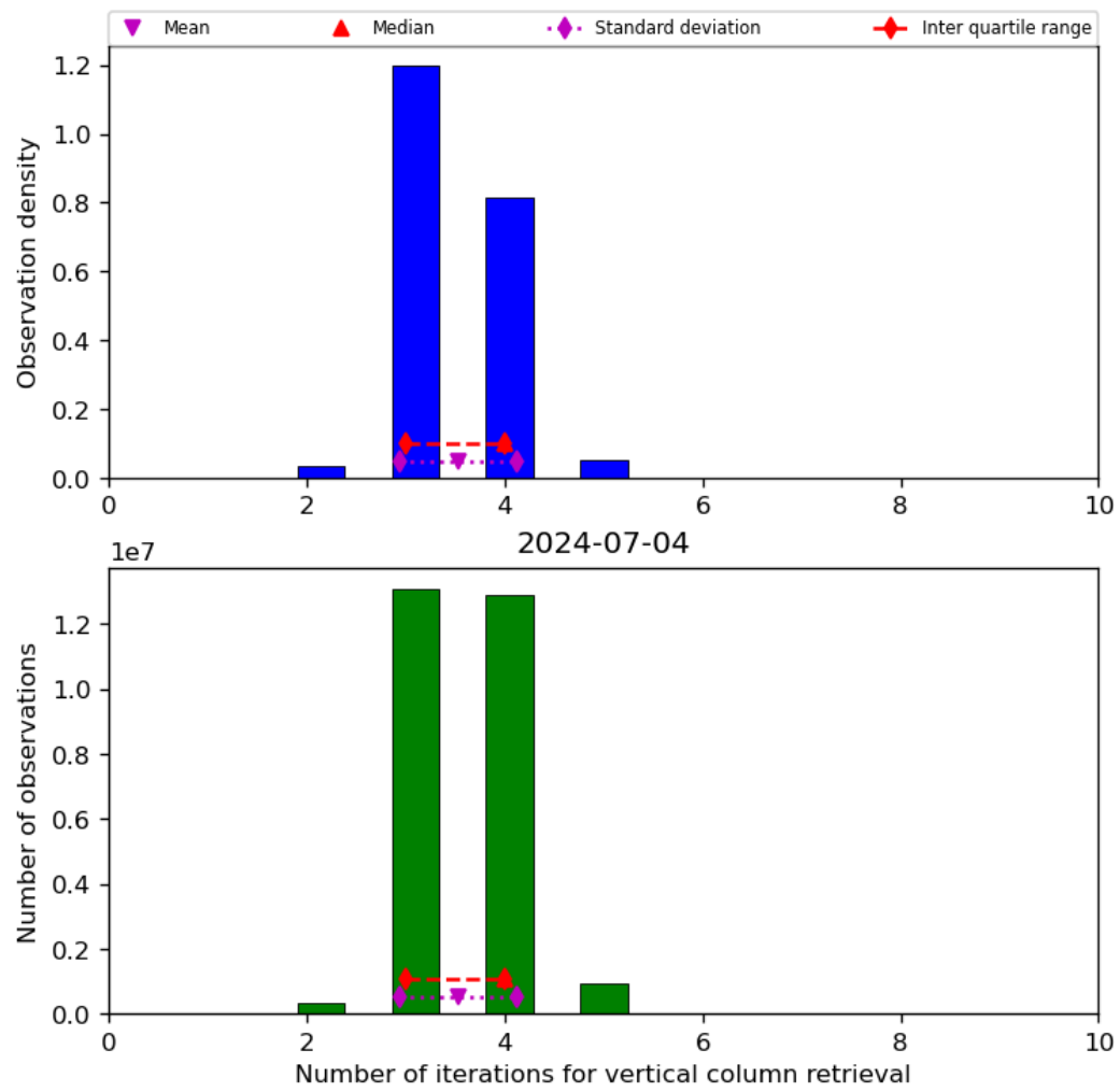
Figure 26: Histogram of “Number of iterations for vertical column retrieval” for 2024-07-03 to 2024-07-05
