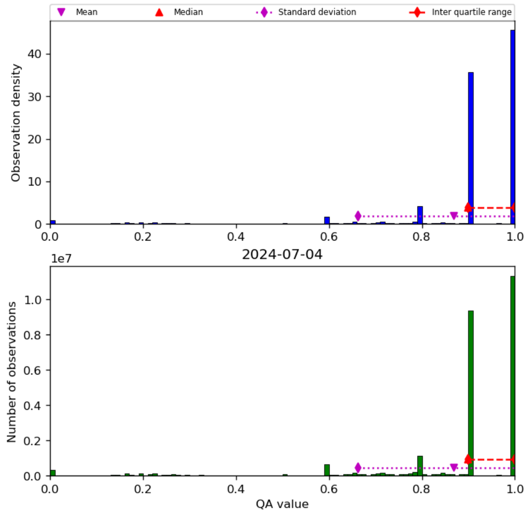
Figure 20: Histogram of “QA value” for 2024-07-03 to 2024-07-05
