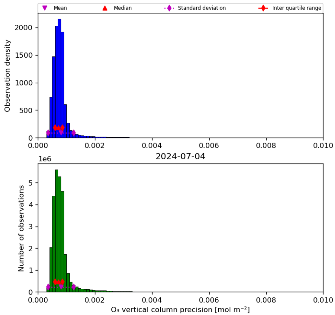
Figure 22: Histogram of “O 3 vertical column precision” for 2024-07-03 to 2024-07-05
