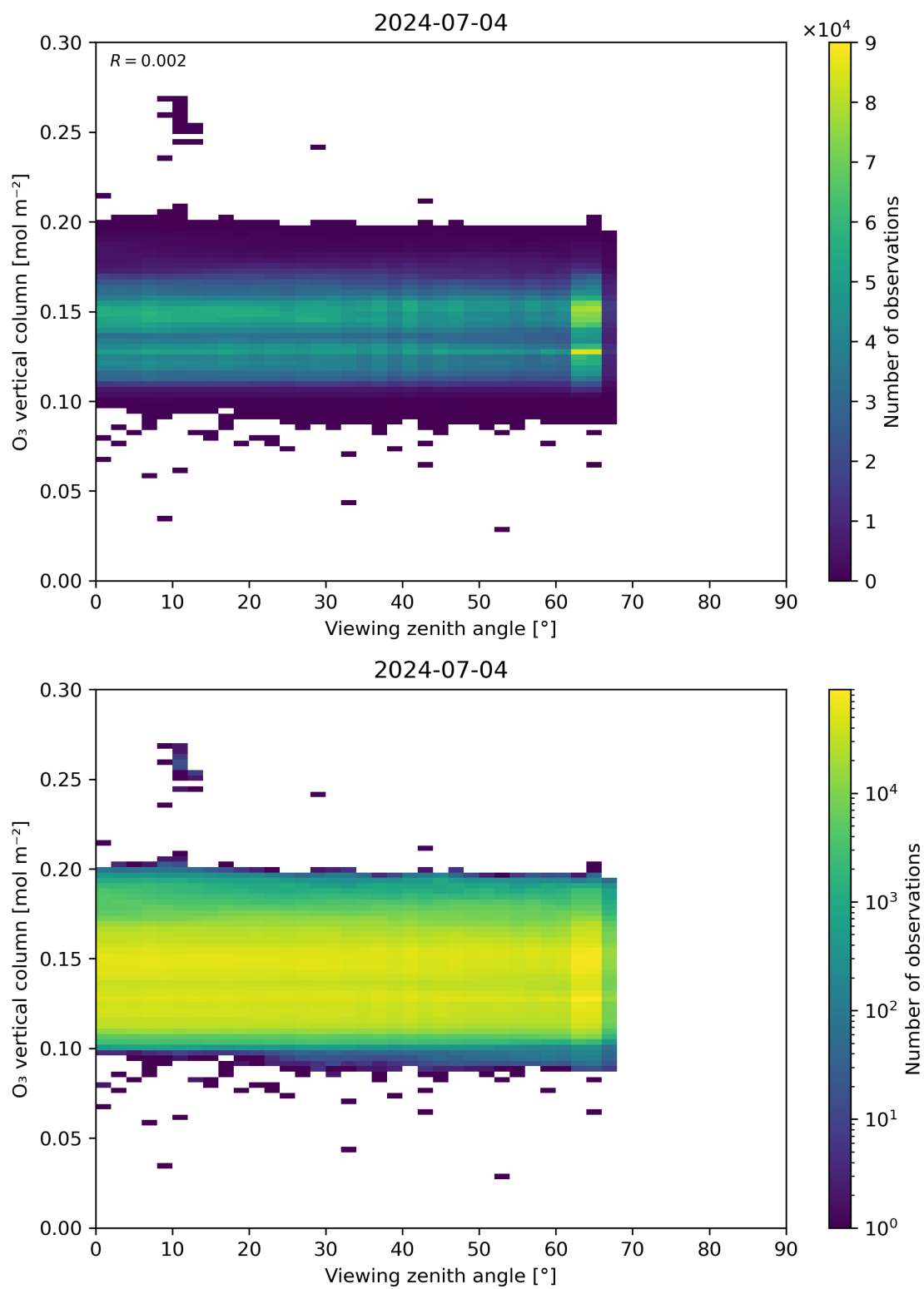
Figure 52: Scatter density plot of “Viewing zenith angle” against “O 3 vertical column” for 2024-07-03 to 2024-07-05.
