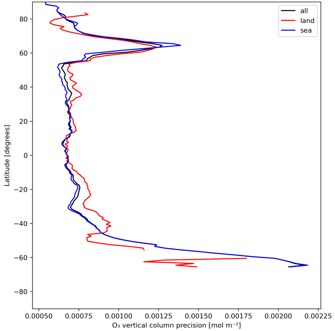
Figure 15: Zonal average of "O 3 vertical column precision" for 2024-07-03 to 2024-07-05.
