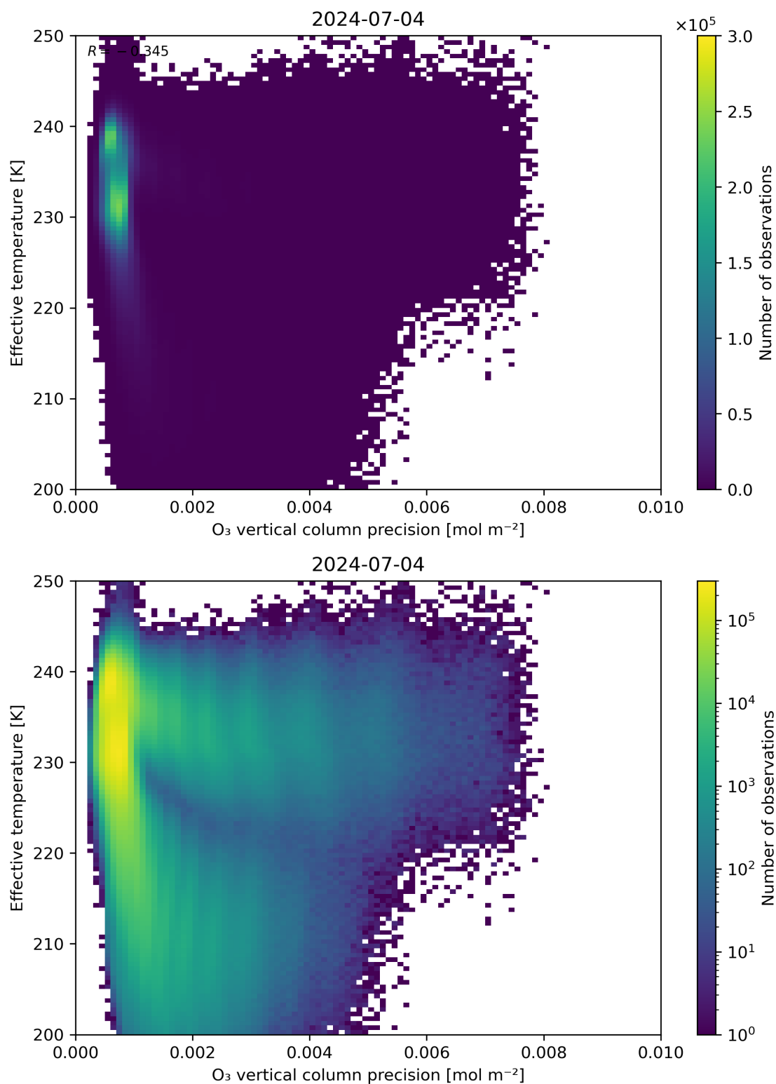
Figure 42: Scatter density plot of “O 3 vertical column precision” against “Effective temperature” for 2024-07-03 to 2024-07-05.
