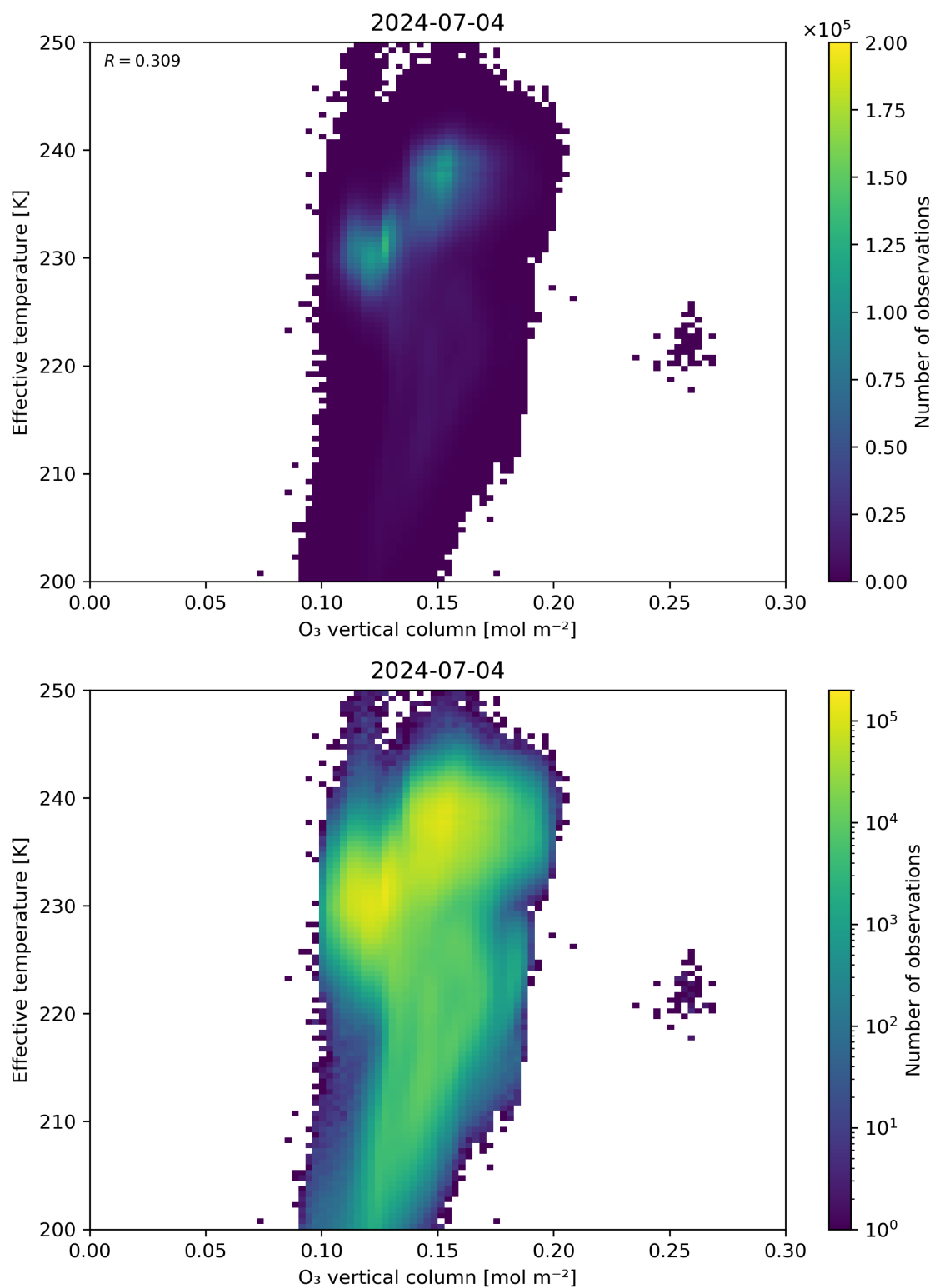
Figure 39: Scatter density plot of “O 3 vertical column” against “Effective temperature” for 2024-07-03 to 2024-07-05.
