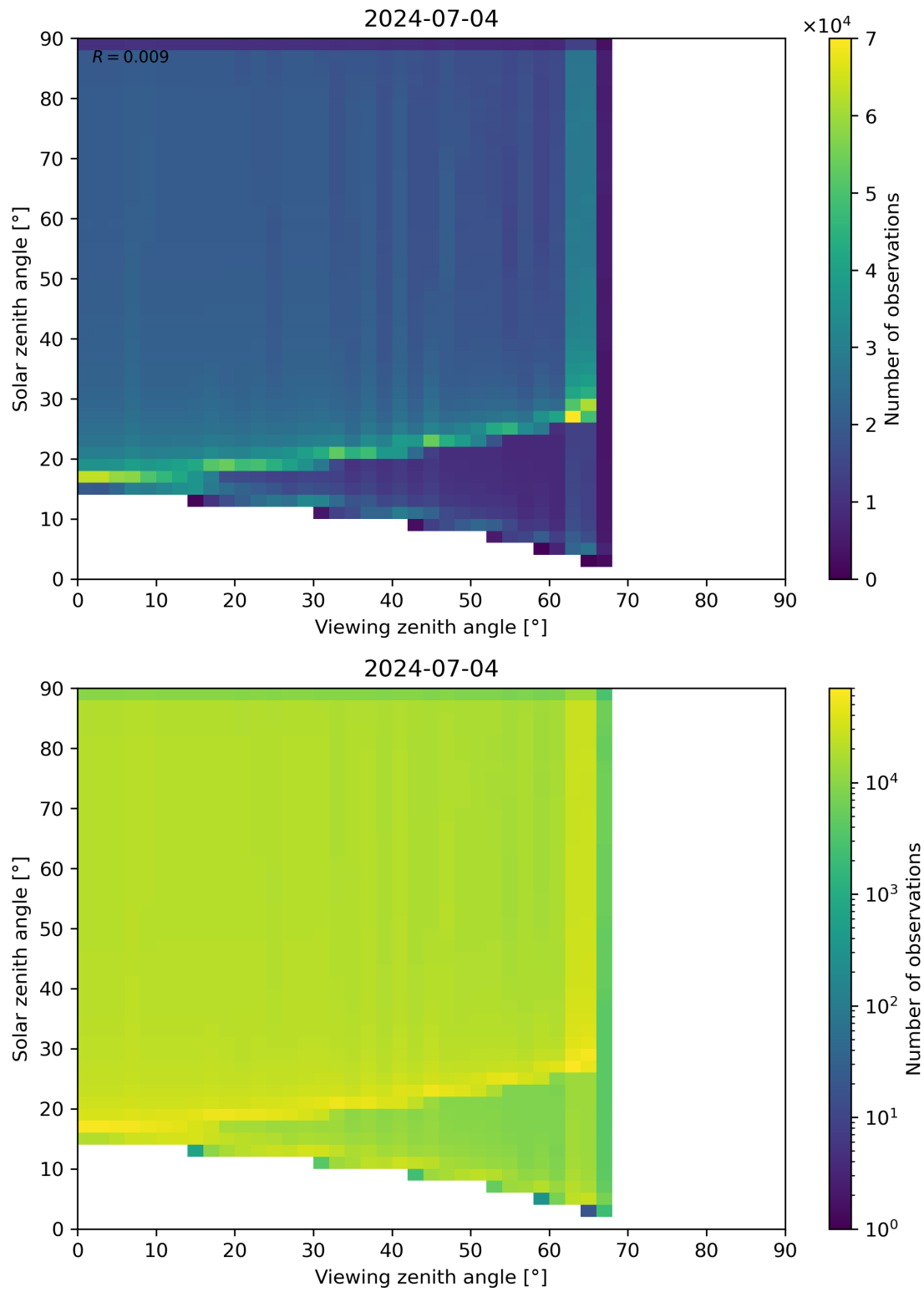
Figure 54: Scatter density plot of “Viewing zenith angle” against “Solar zenith angle” for 2024-07-03 to 2024-07-05.
