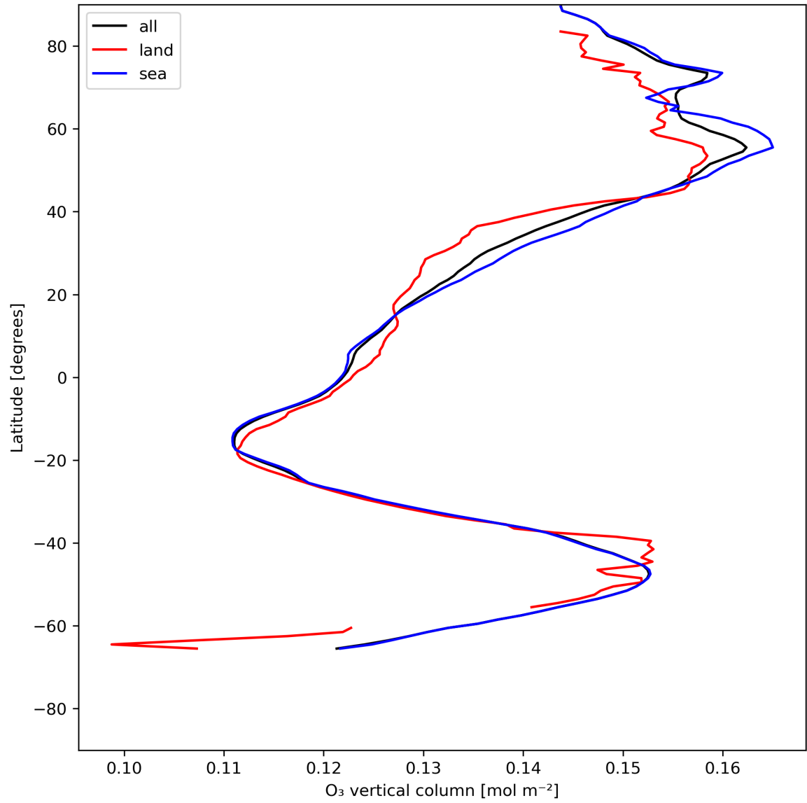
Figure 14: Zonal average of “O 3 vertical column” for 2024-07-03 to 2024-07-05.
