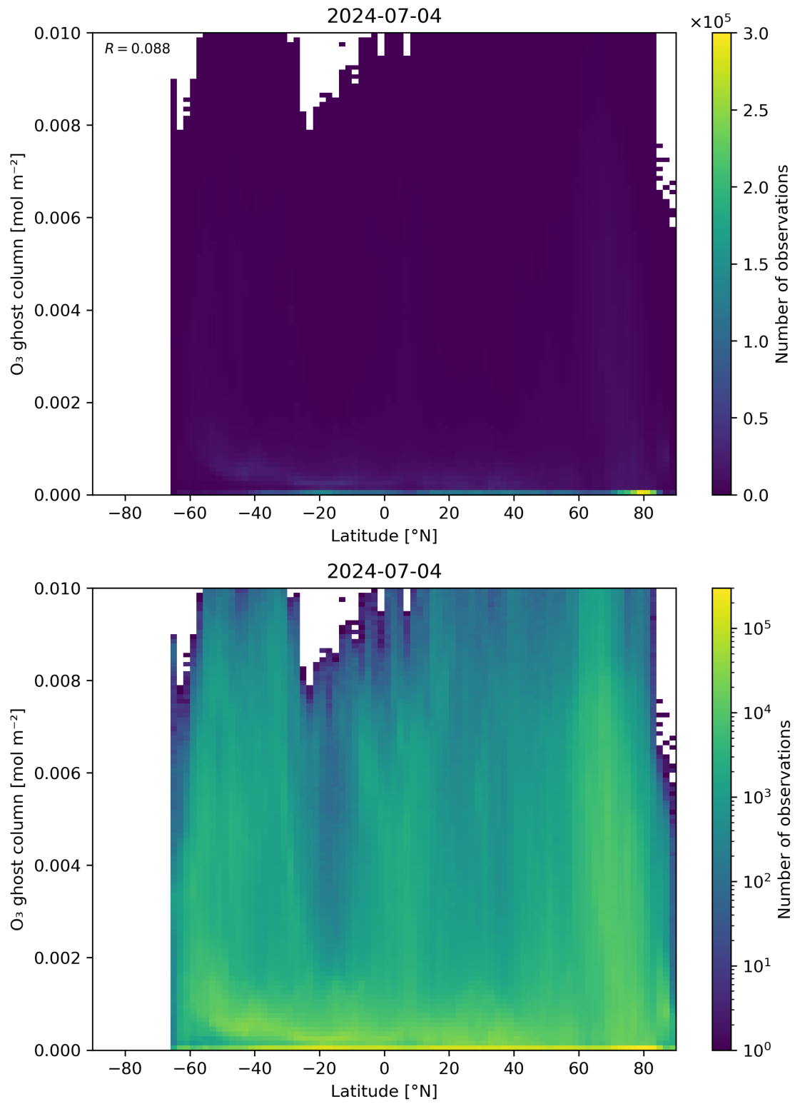
Figure 35: Scatter density plot of “Latitude” against “O 3 ghost column” for 2024-07-03 to 2024-07-05.
