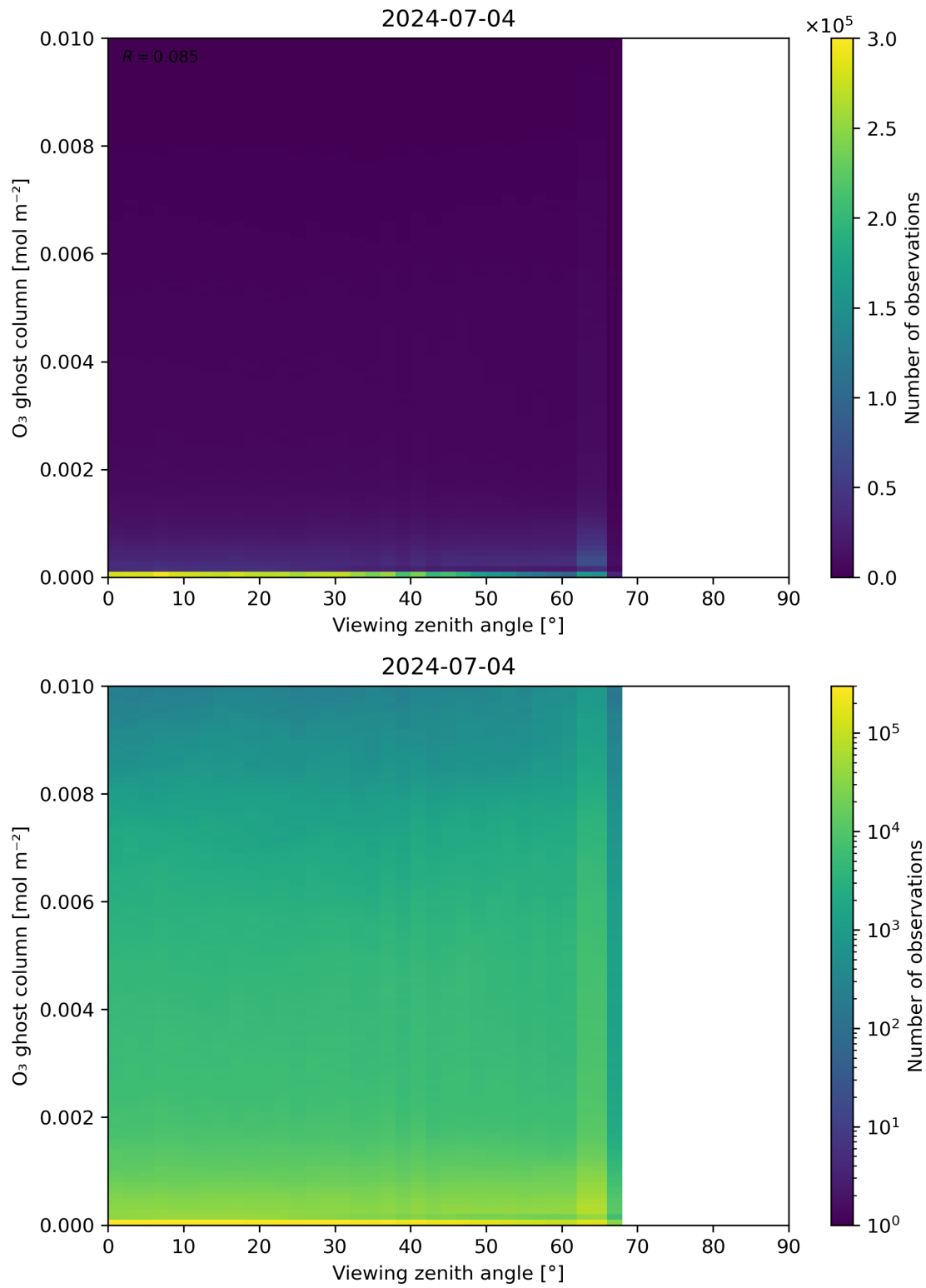
Figure 51: Scatter density plot of “Viewing zenith angle” against “O 3 ghost column” for 2024-07-03 to 2024-07-05.
