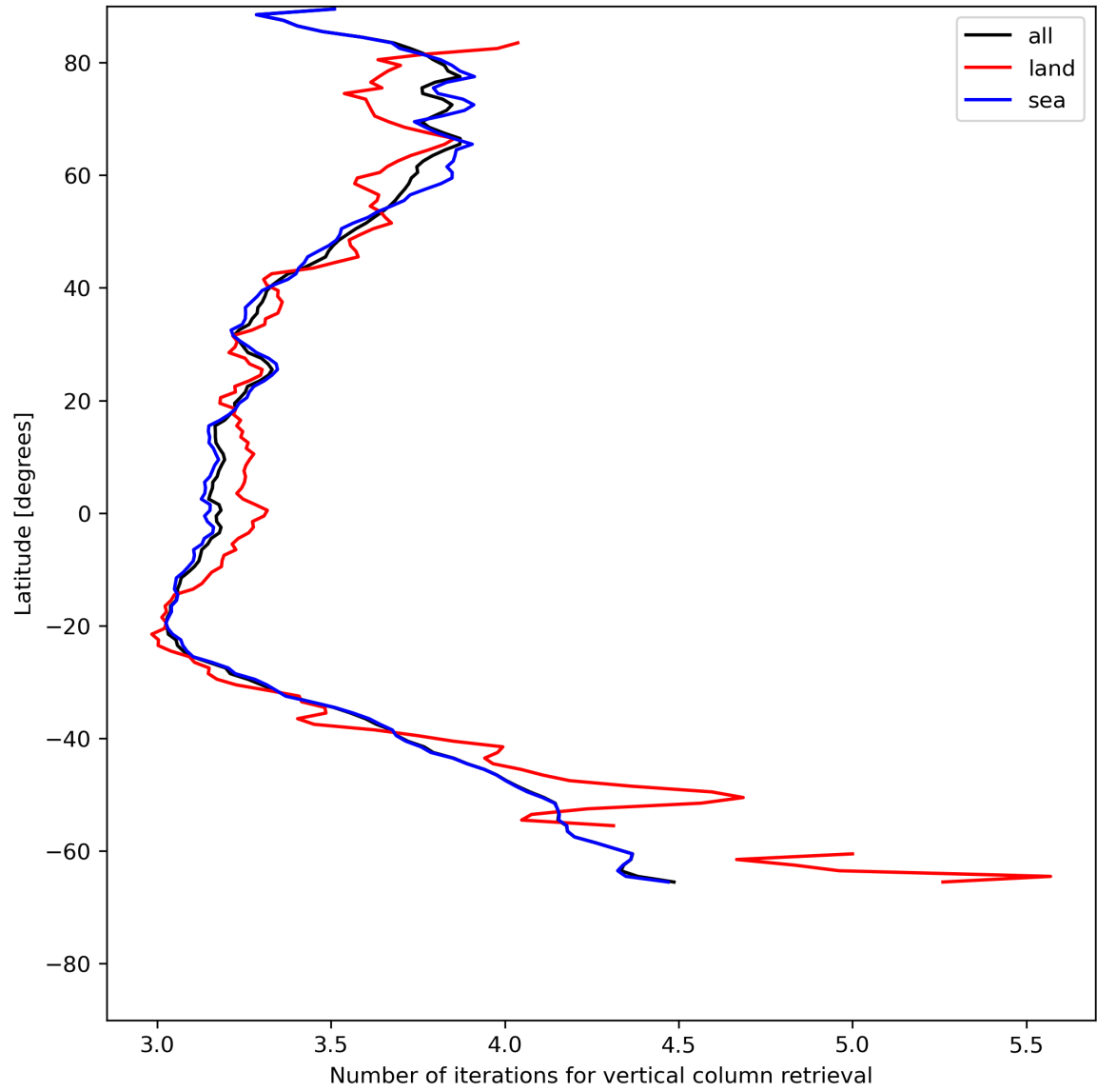
Figure 19: Zonal average of “Number of iterations for vertical column retrieval” for 2024-07-03 to 2024-07-05.
