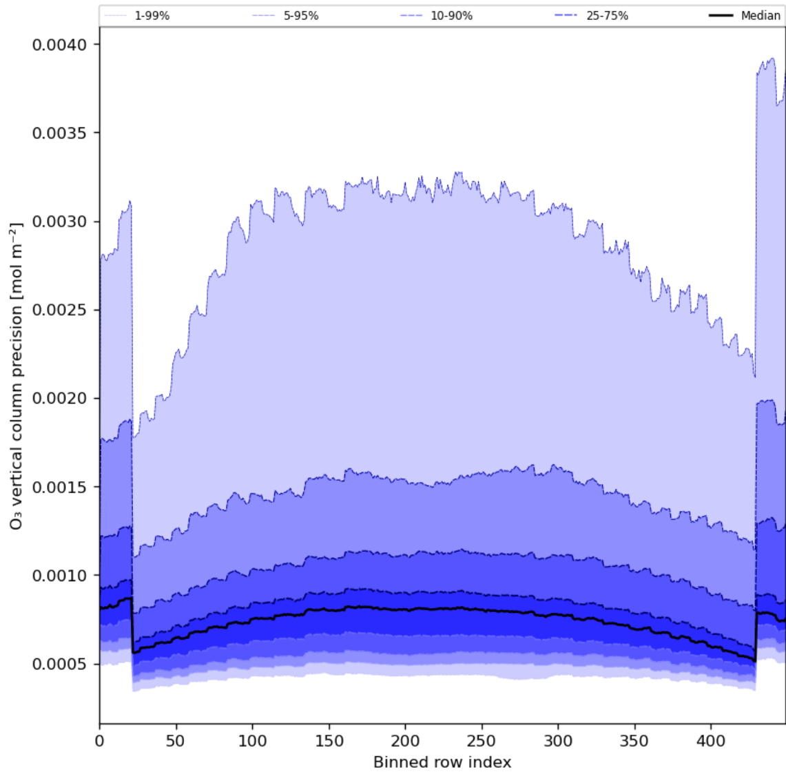
Figure 29: Along track statistics of “O 3 vertical column precision” for 2024-07-03 to 2024-07-05
