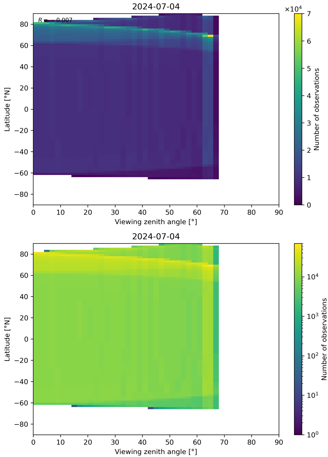
Figure 49: Scatter density plot of “Viewing zenith angle” against “Latitude” for 2024-07-03 to 2024-07-05.
