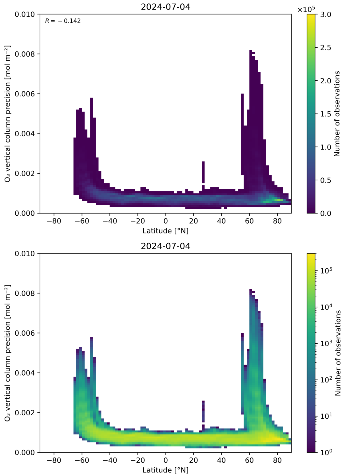
Figure 37: Scatter density plot of “Latitude” against “O 3 vertical column precision” for 2024-07-03 to 2024-07-05.
