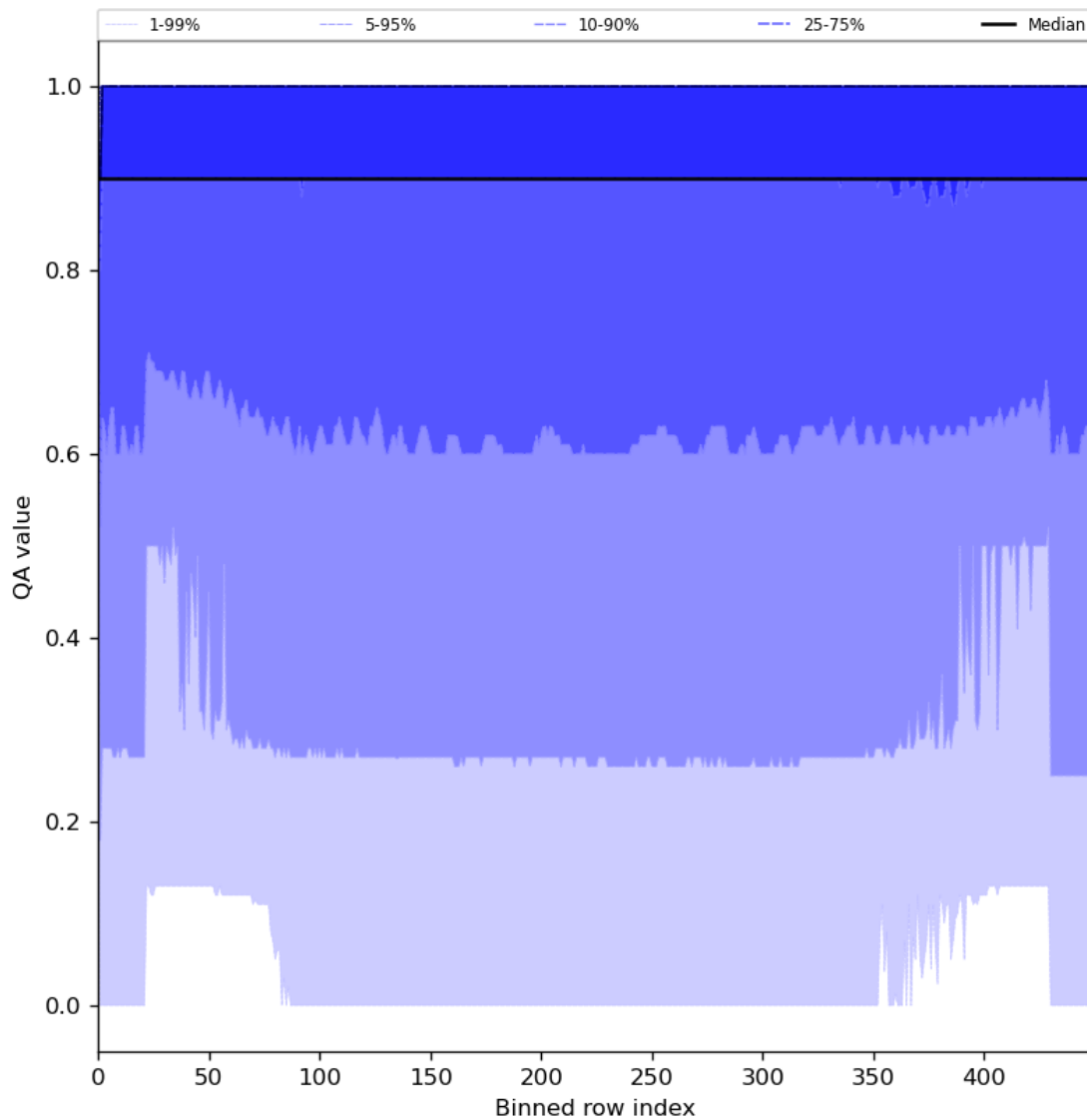
Figure 27: Along track statistics of “QA value” for 2024-07-03 to 2024-07-05
