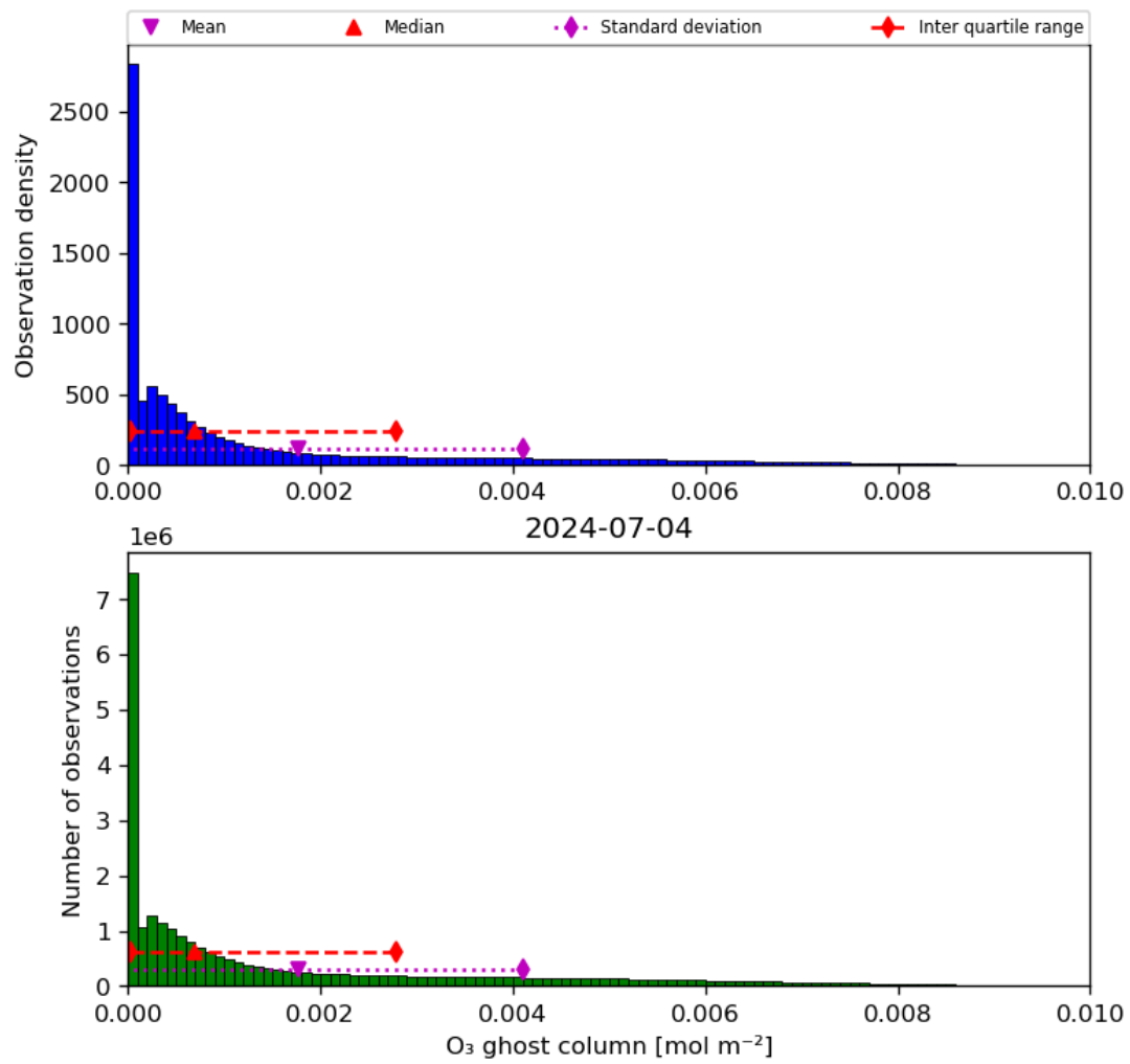
Figure 25: Histogram of "O 3 ghost column" for 2024-07-03 to 2024-07-05
