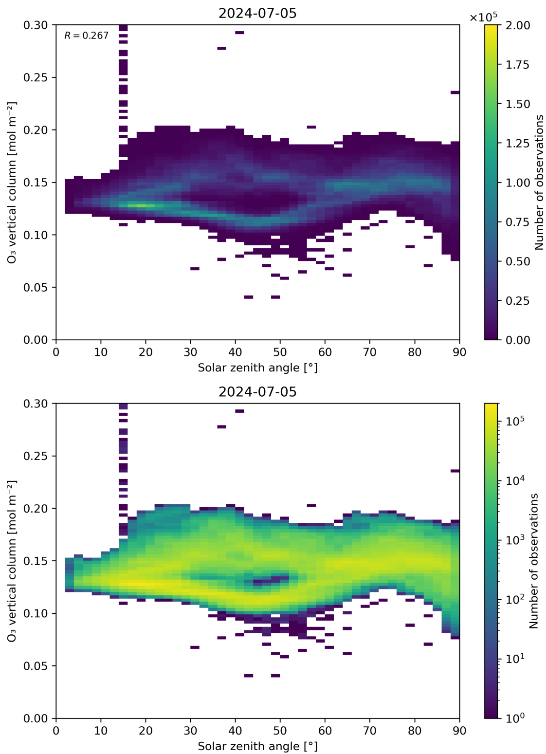
Figure 47: Scatter density plot of “Solar zenith angle” against “O 3 vertical column” for 2024-07-05 to 2024-07-06.
