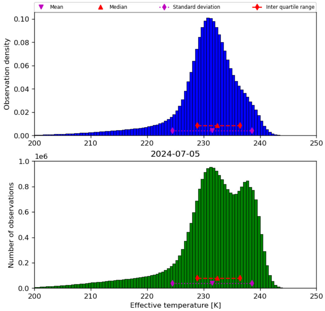
Figure 24: Histogram of “Effective temperature” for 2024-07-05 to 2024-07-06
