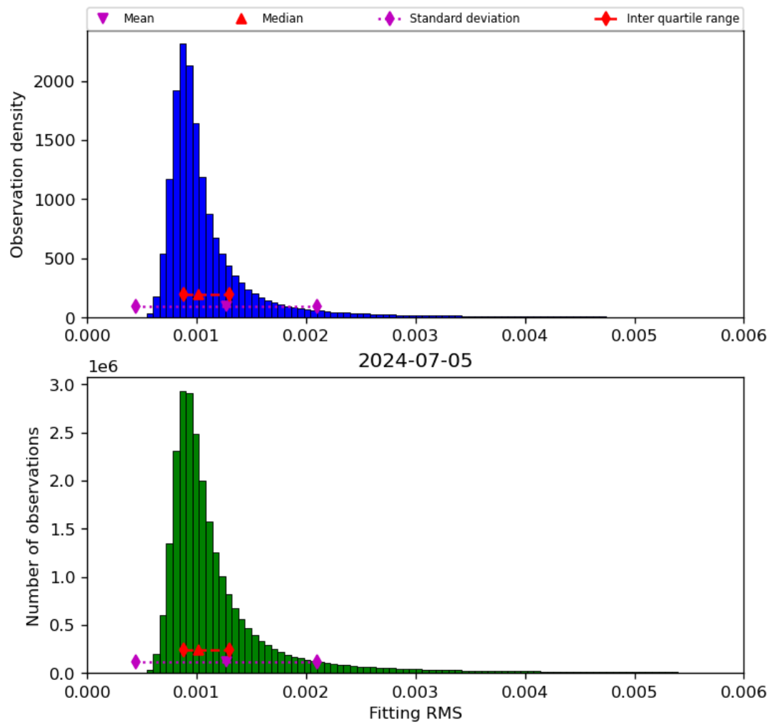
Figure 23: Histogram of “Fitting RMS” for 2024-07-05 to 2024-07-06
