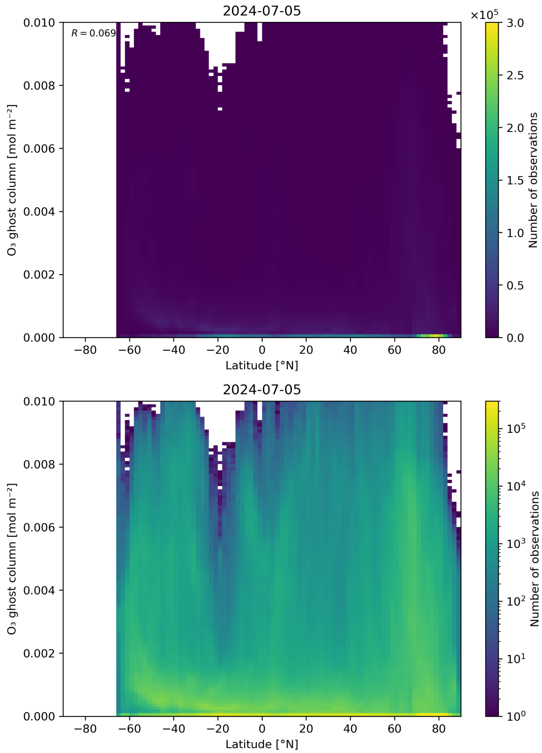
Figure 35: Scatter density plot of “Latitude” against “O 3 ghost column” for 2024-07-05 to 2024-07-06.
