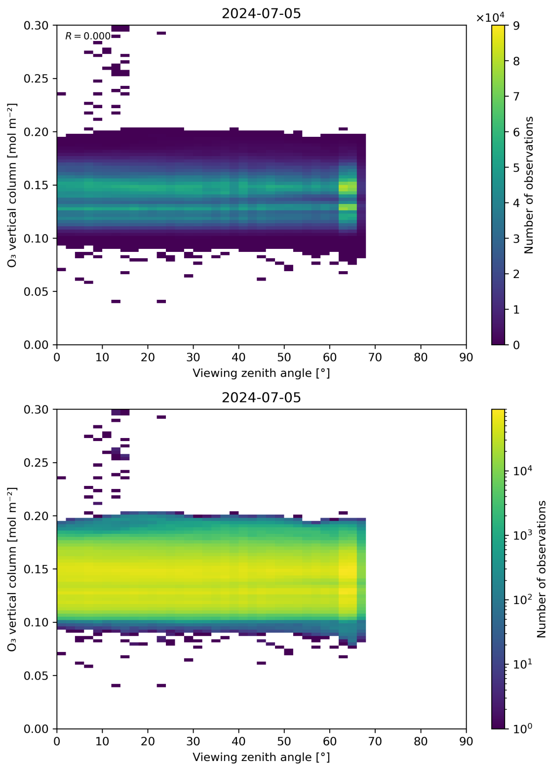
Figure 52: Scatter density plot of “Viewing zenith angle” against “O 3 vertical column” for 2024-07-05 to 2024-07-06.
