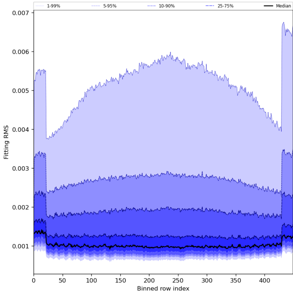
Figure 30: Along track statistics of “Fitting RMS” for 2024-07-05 to 2024-07-06
