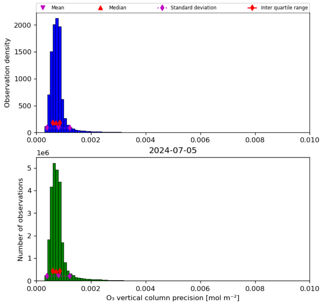
Figure 22: Histogram of “O 3 vertical column precision” for 2024-07-05 to 2024-07-06
