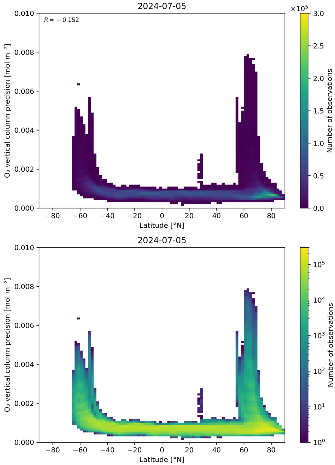
Figure 37: Scatter density plot of “Latitude” against “O 3 vertical column precision” for 2024-07-05 to 2024-07-06.
