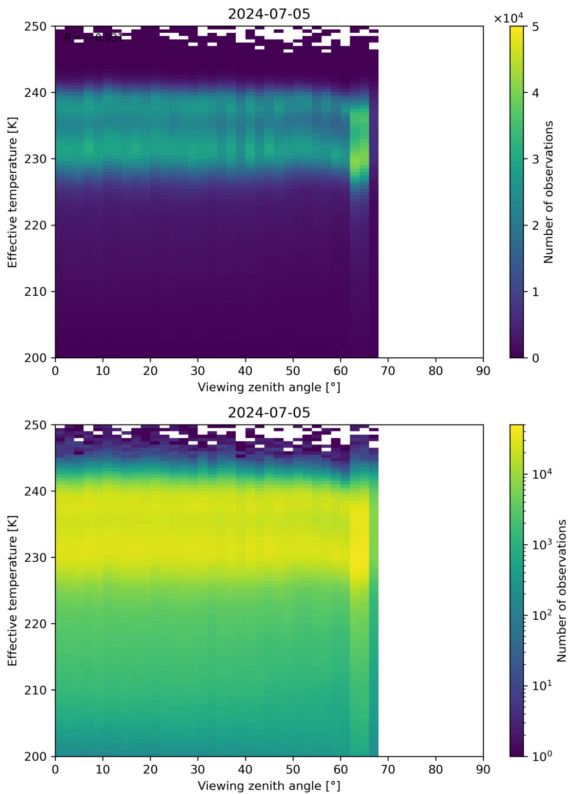
Figure 50: Scatter density plot of “Viewing zenith angle” against “Effective temperature” for 2024-07-05 to 2024-07-06.
