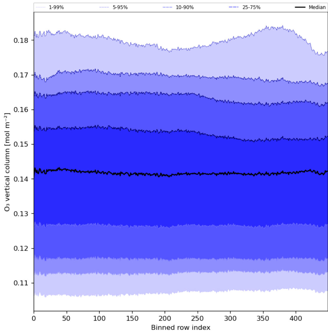
Figure 28: Along track statistics of “O 3 vertical column” for 2024-07-05 to 2024-07-06
