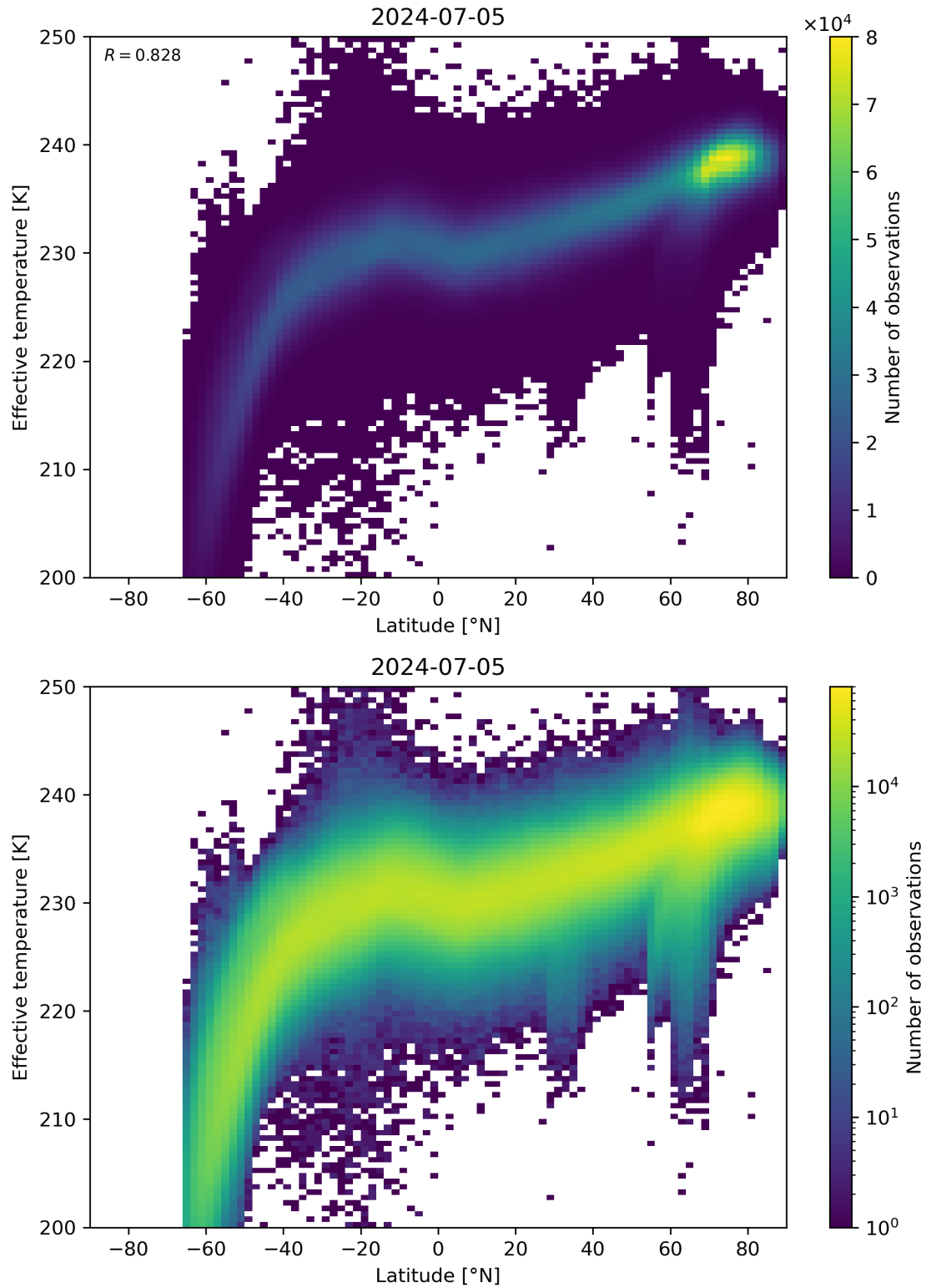
Figure 34: Scatter density plot of “Latitude” against “Effective temperature” for 2024-07-05 to 2024-07-06.
