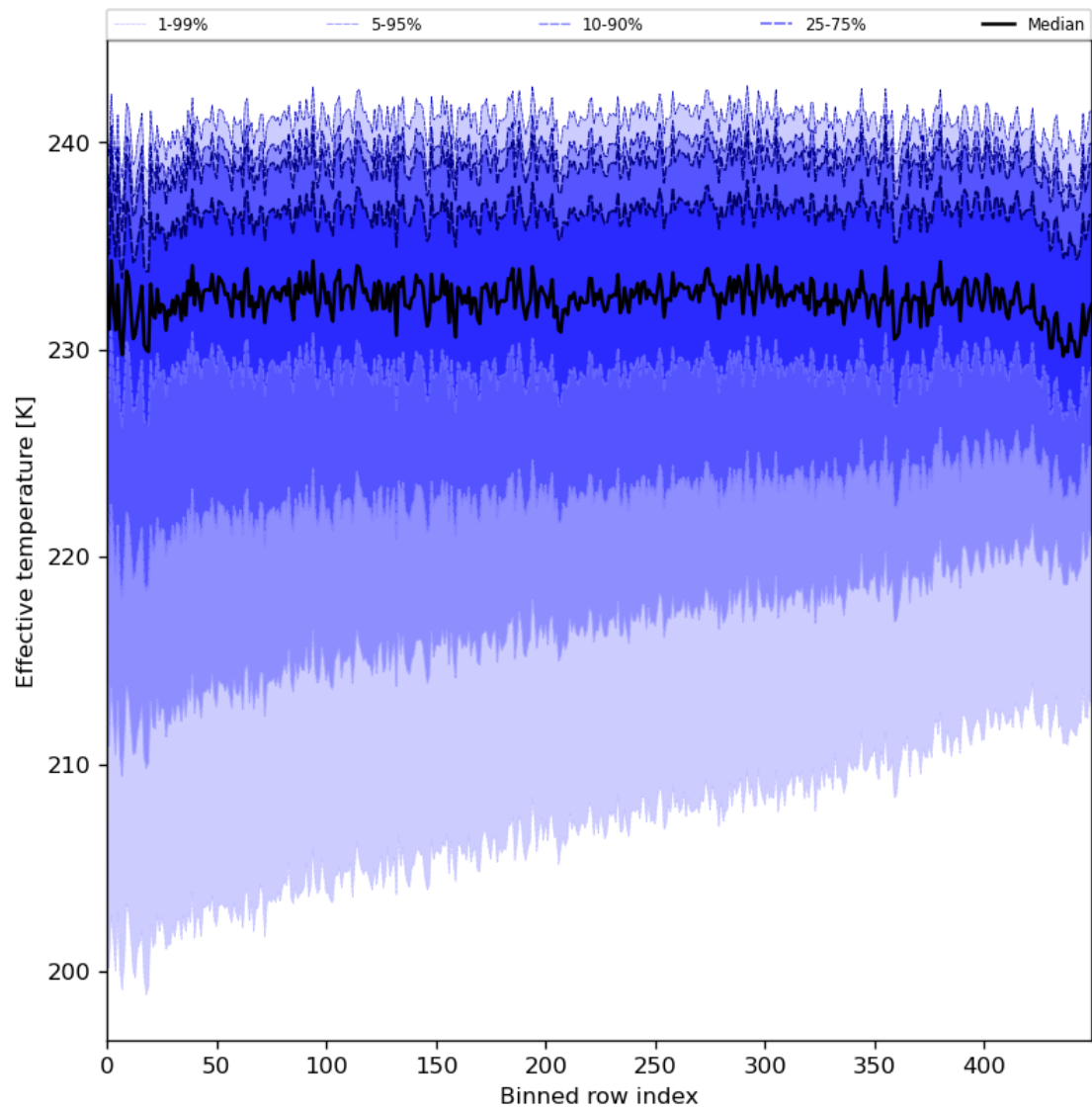
Figure 31: Along track statistics of “Effective temperature” for 2024-07-05 to 2024-07-06
