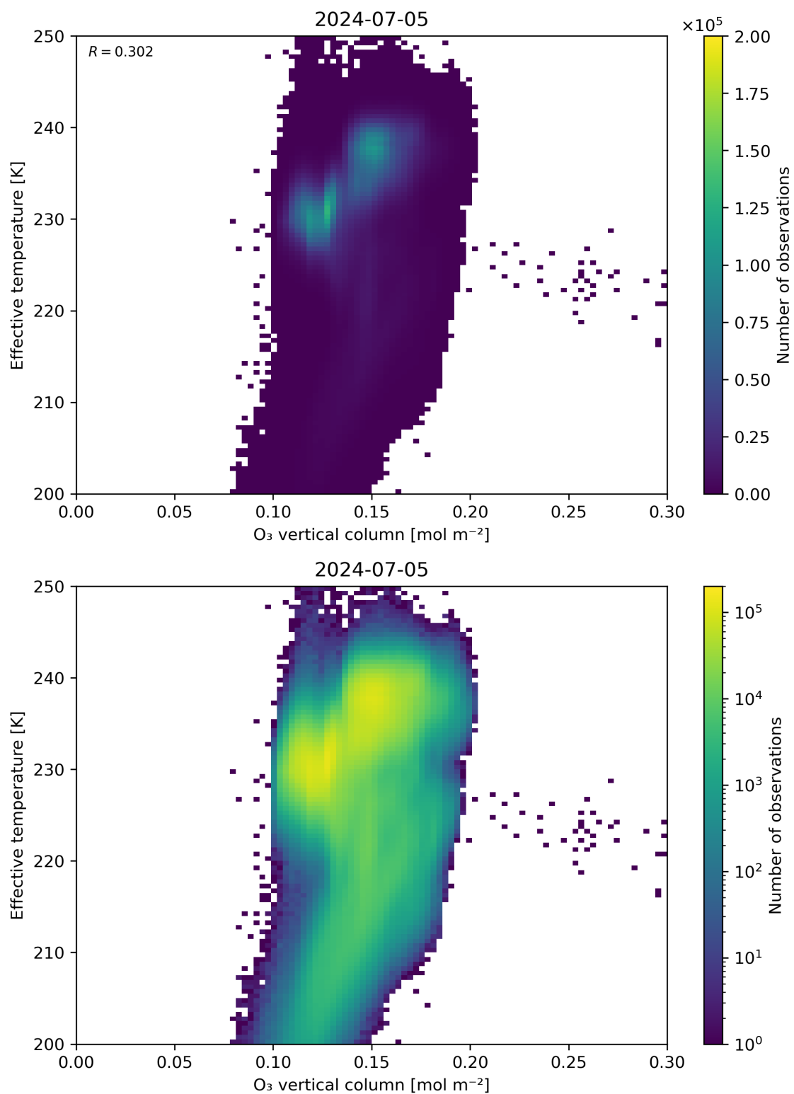
Figure 39: Scatter density plot of “O 3 vertical column” against “Effective temperature” for 2024-07-05 to 2024-07-06.
