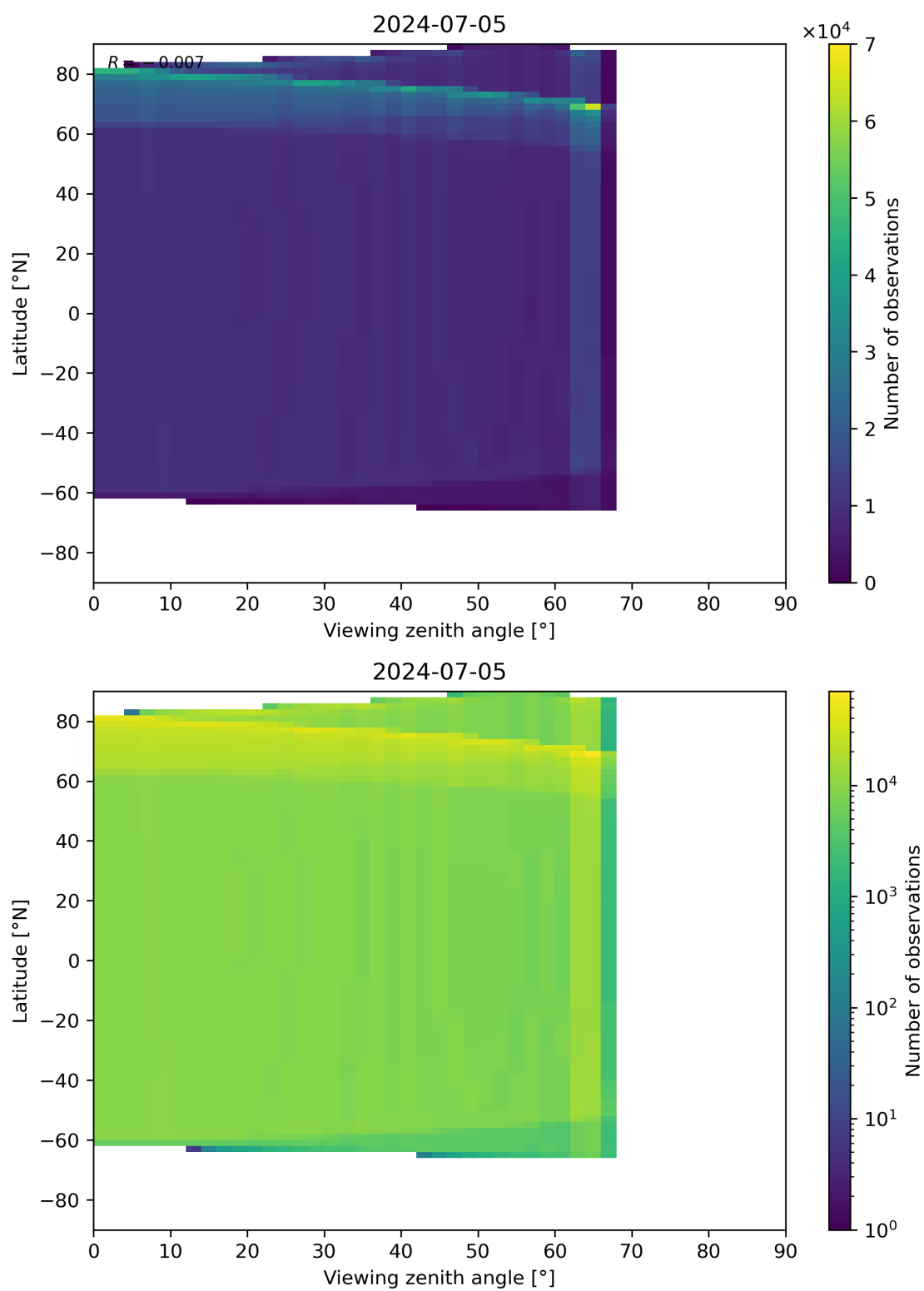
Figure 49: Scatter density plot of “Viewing zenith angle” against “Latitude” for 2024-07-05 to 2024-07-06.
