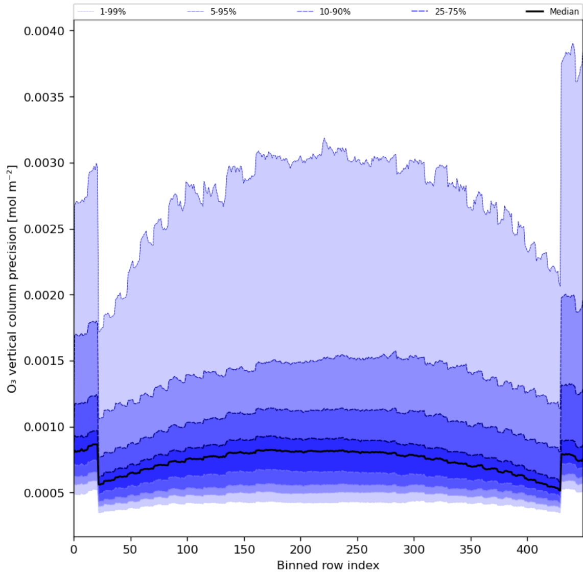
Figure 29: Along track statistics of “O 3 vertical column precision” for 2024-07-05 to 2024-07-06
