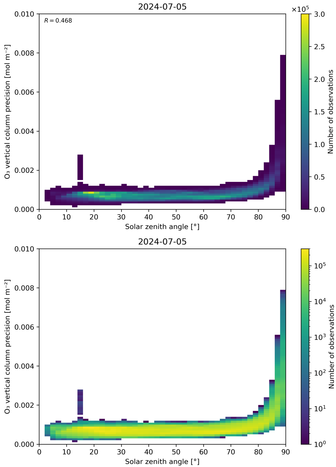
Figure 48: Scatter density plot of “Solar zenith angle” against “O 3 vertical column precision” for 2024-07-05 to 2024-07-06.
