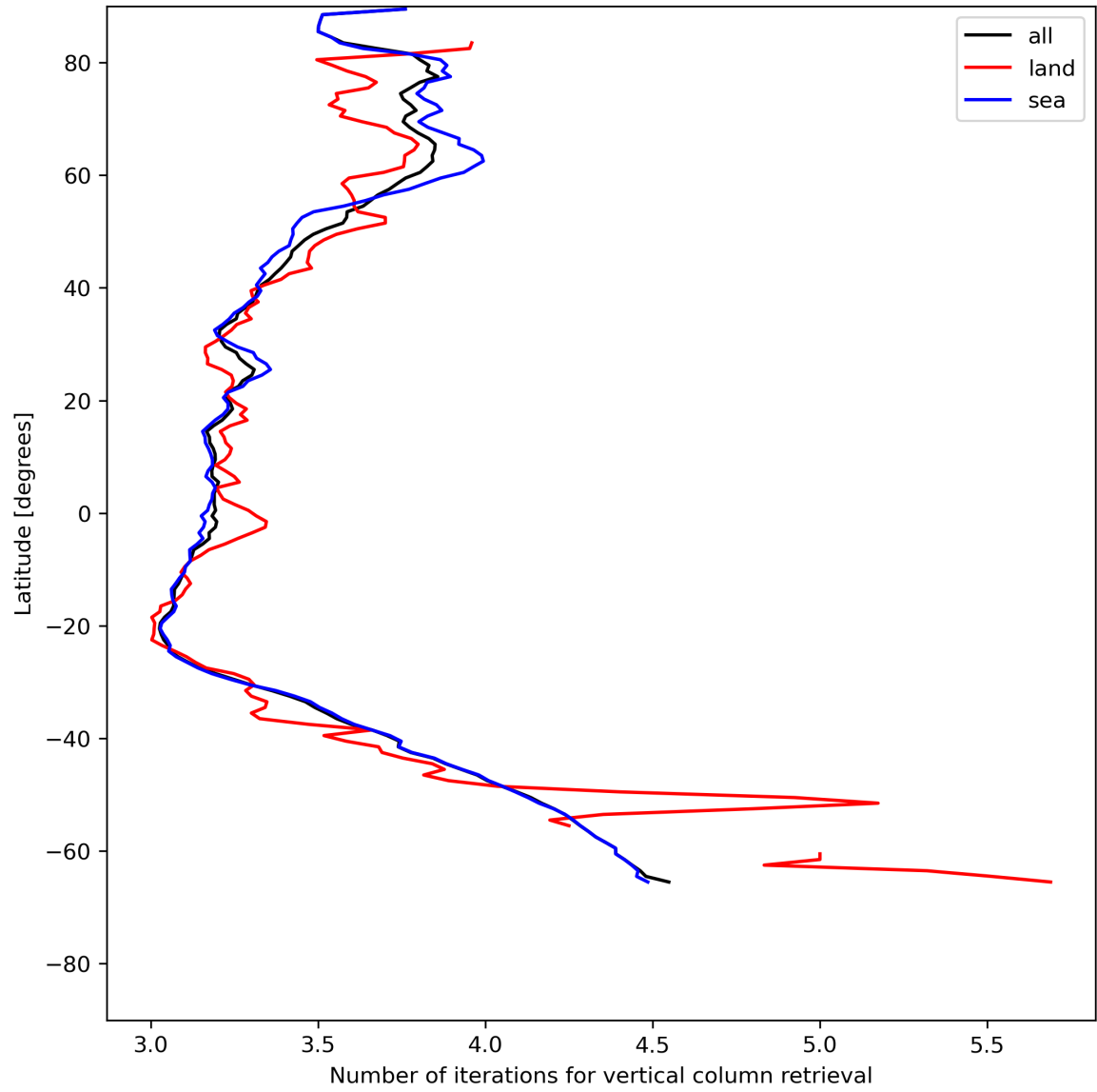
Figure 19: Zonal average of “Number of iterations for vertical column retrieval” for 2024-07-05 to 2024-07-06.
