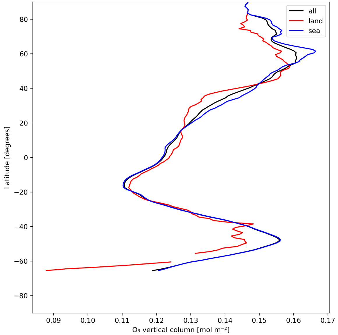
Figure 14: Zonal average of “O 3 vertical column” for 2024-07-05 to 2024-07-06.
