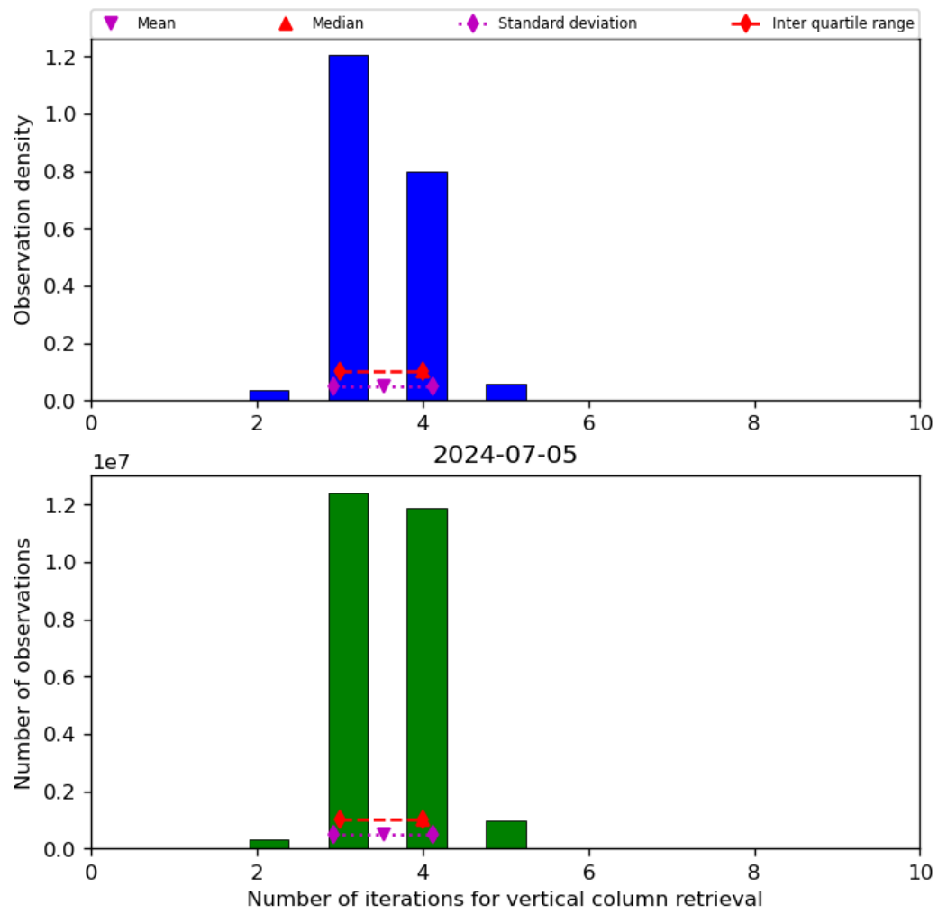
Figure 26: Histogram of “Number of iterations for vertical column retrieval” for 2024-07-05 to 2024-07-06
