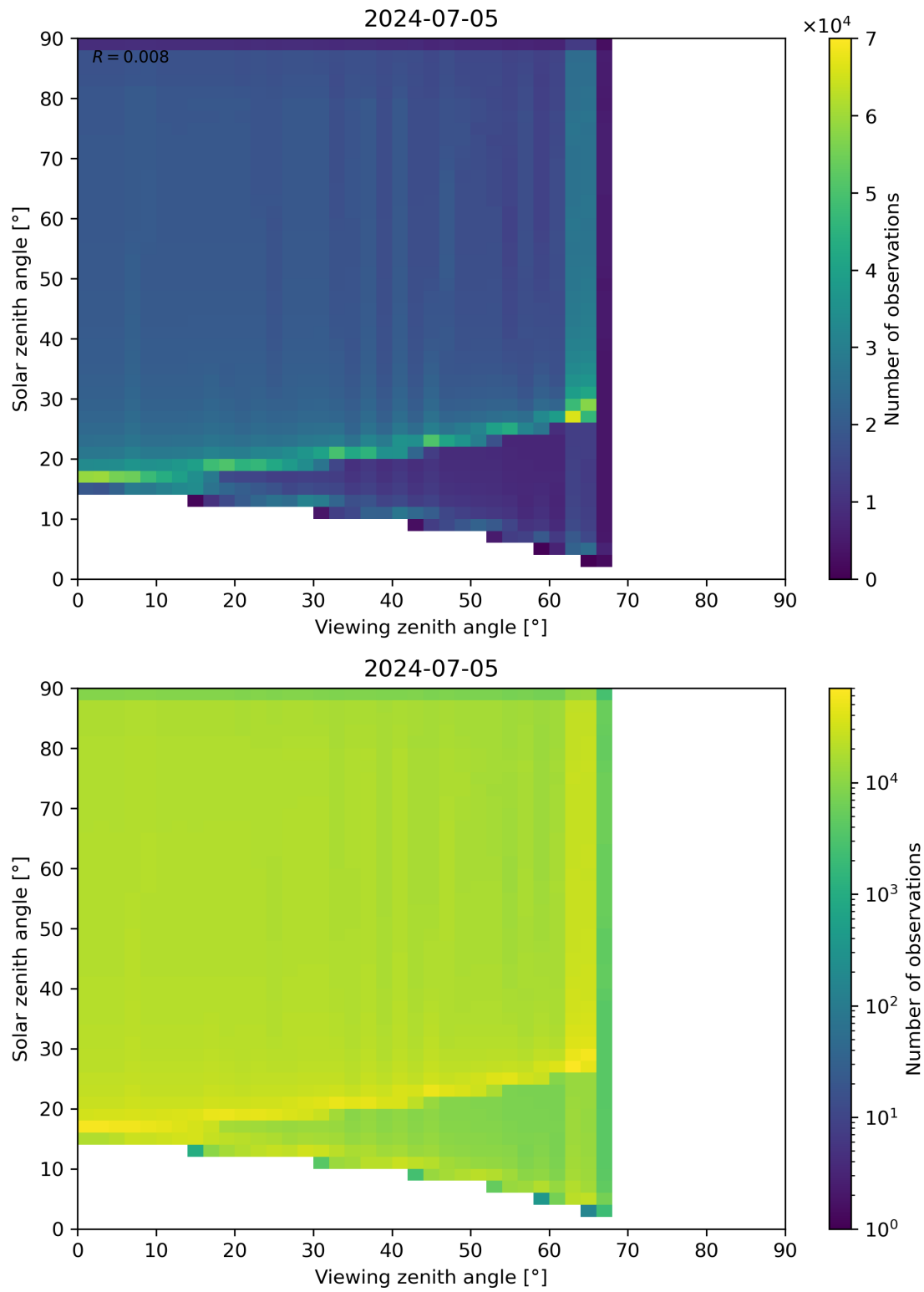
Figure 54: Scatter density plot of “Viewing zenith angle” against “Solar zenith angle” for 2024-07-05 to 2024-07-06.
