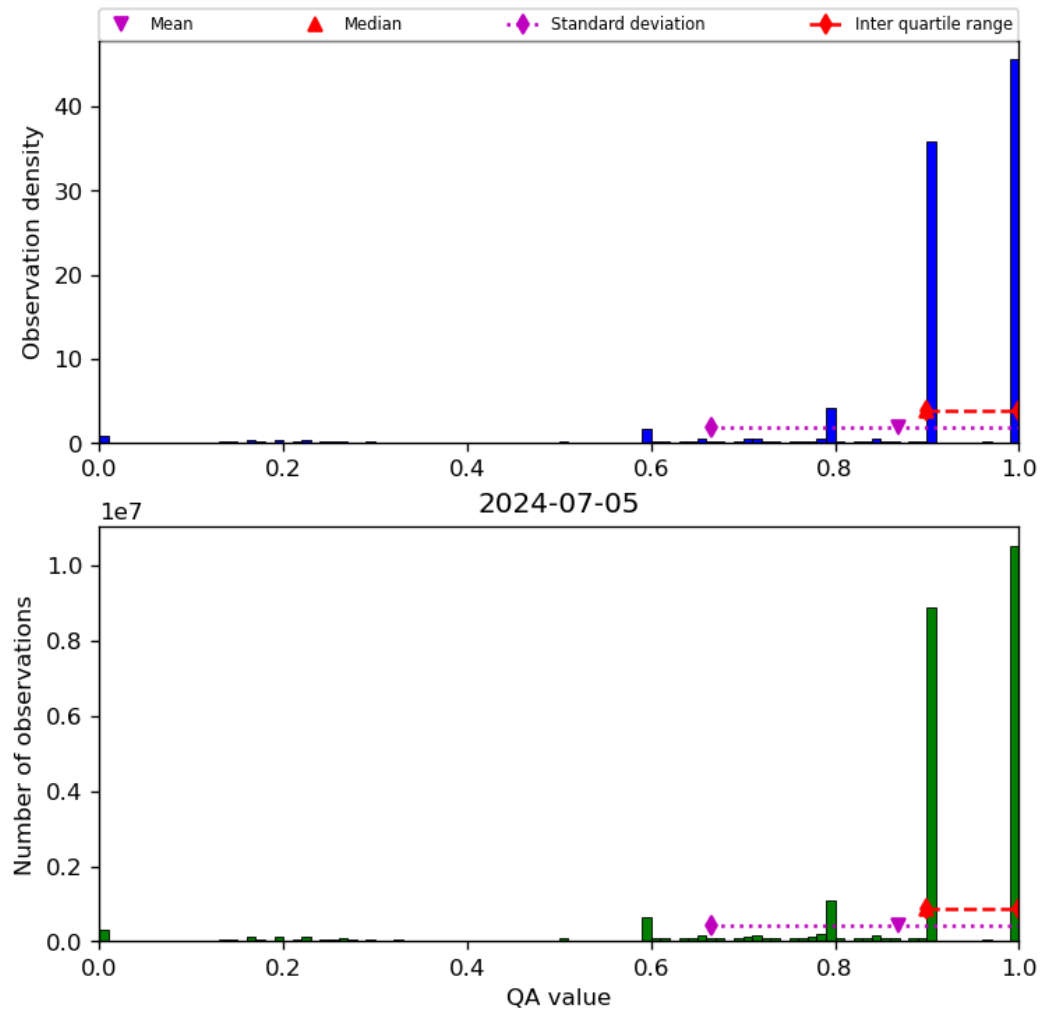
Figure 20: Histogram of “QA value” for 2024-07-05 to 2024-07-06
