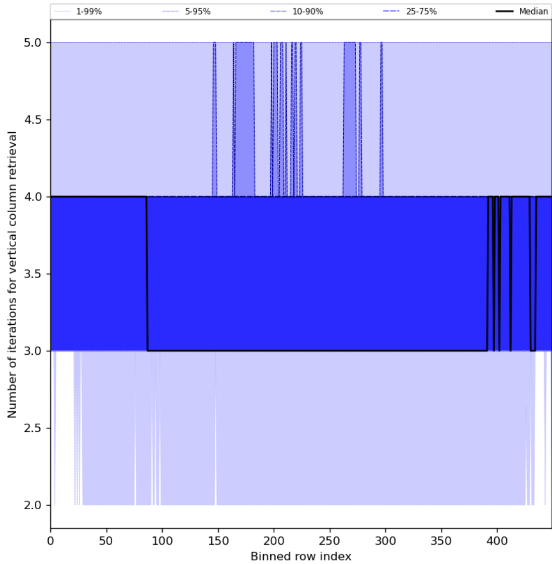
Figure 33: Along track statistics of “Number of iterations for vertical column retrieval” for 2024-07-05 to 2024-07-06
