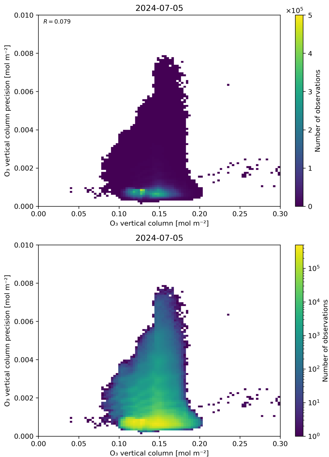
Figure 41: Scatter density plot of “O 3 vertical column” against “O 3 vertical column precision” for 2024-07-05 to 2024-07-06.
