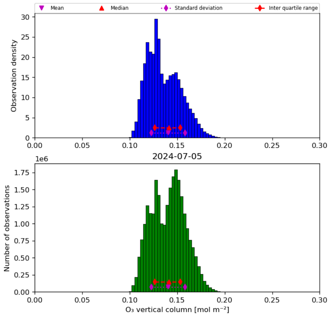
Figure 21: Histogram of “O 3 vertical column” for 2024-07-05 to 2024-07-06
