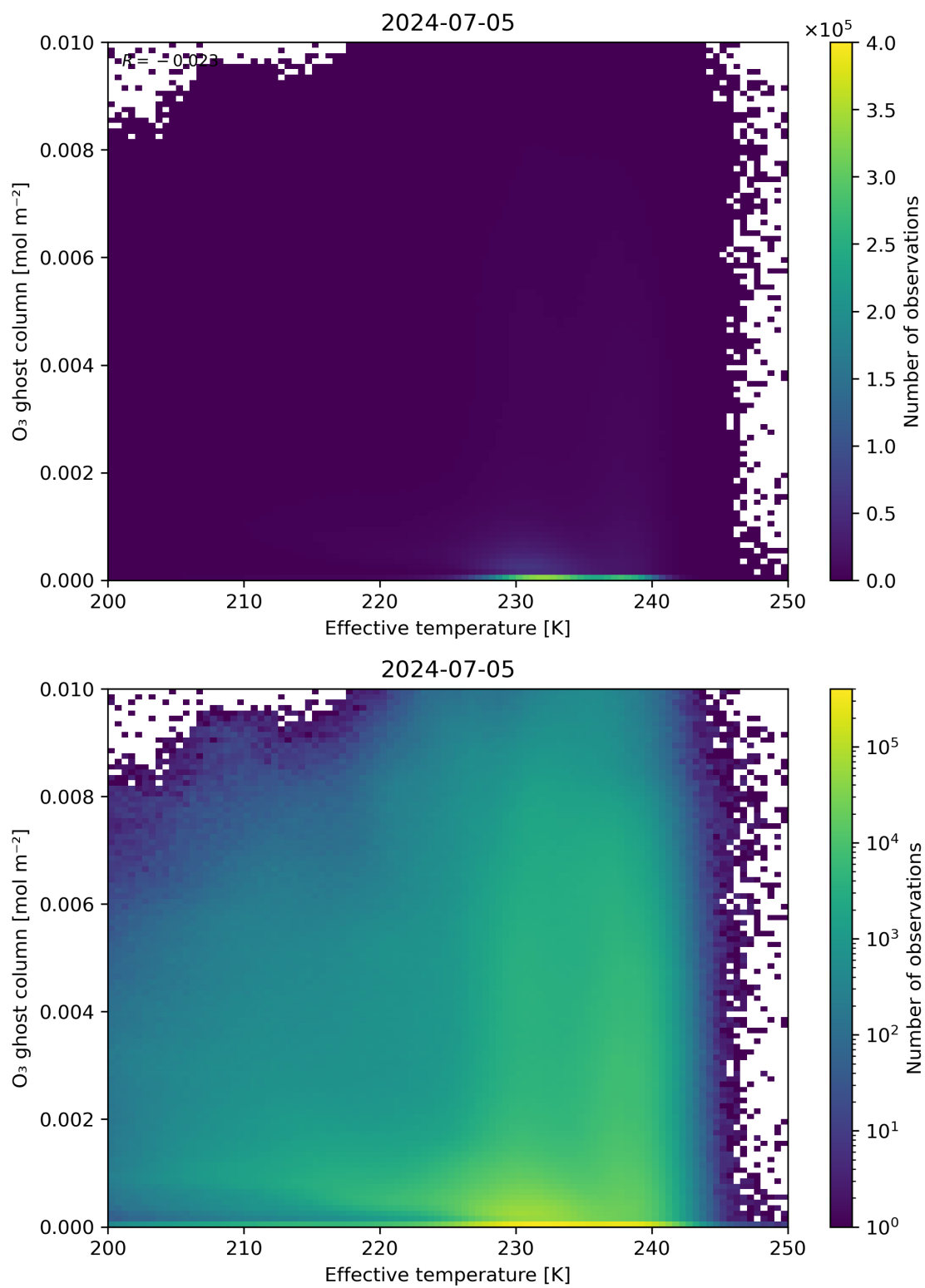
Figure 38: Scatter density plot of “Effective temperature” against “O 3 ghost column” for 2024-07-05 to 2024-07-06.
