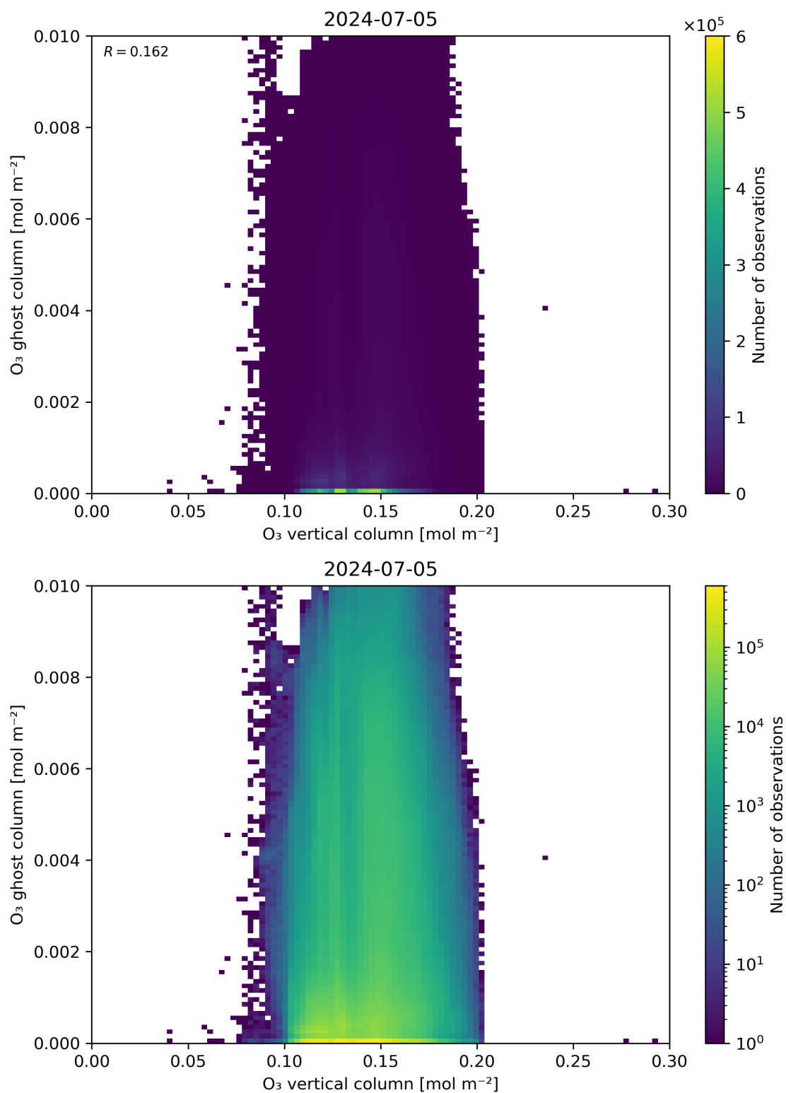
Figure 40: Scatter density plot of “O 3 vertical column” against “O 3 ghost column” for 2024-07-05 to 2024-07-06.
