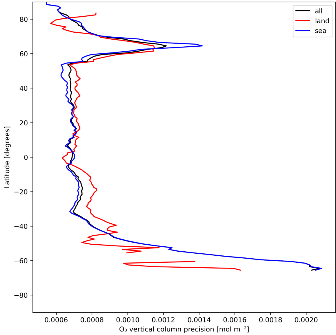
Figure 15: Zonal average of “O 3 vertical column precision” for 2024-07-05 to 2024-07-06.
