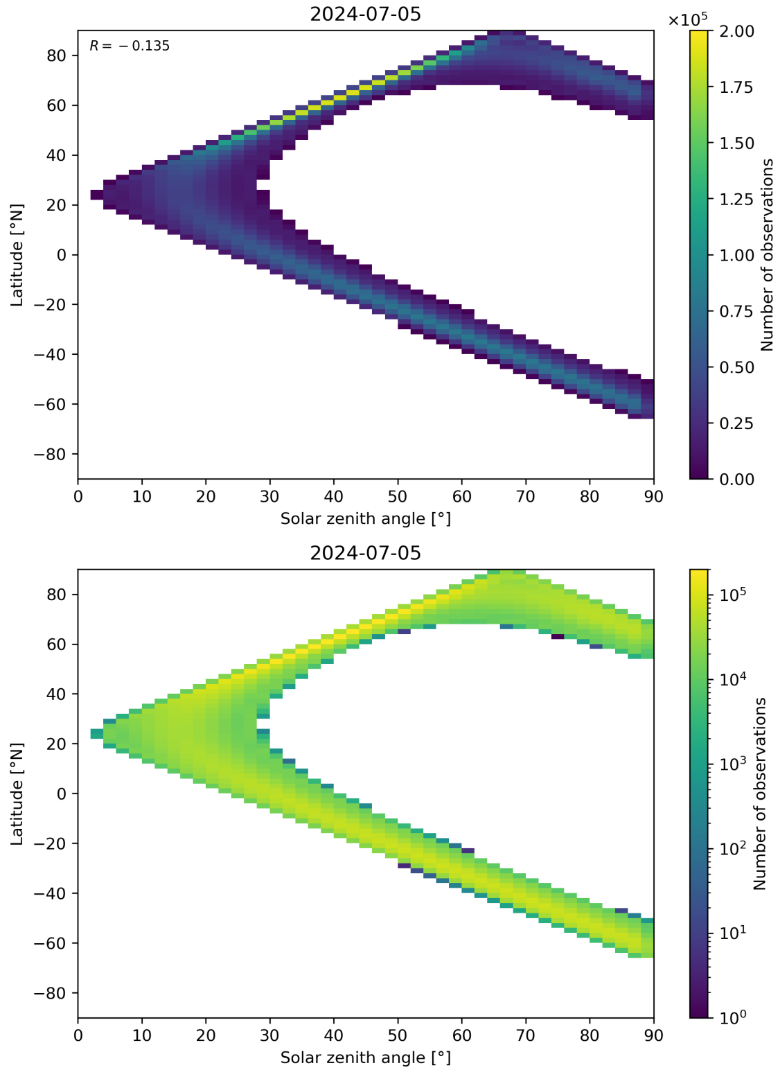
Figure 44: Scatter density plot of “Solar zenith angle” against “Latitude” for 2024-07-05 to 2024-07-06.
