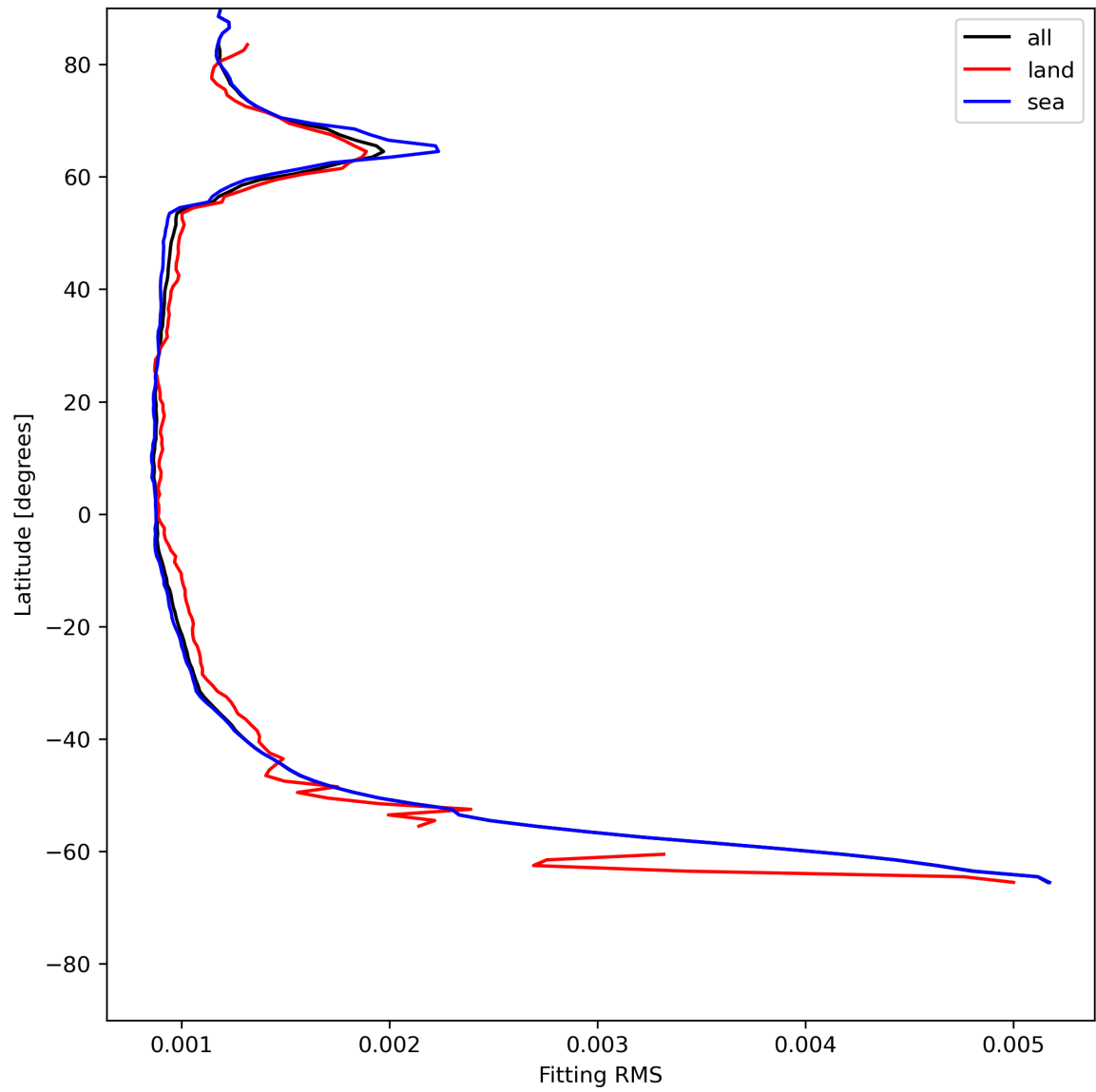
Figure 16: Zonal average of “Fitting RMS” for 2024-07-05 to 2024-07-06.
