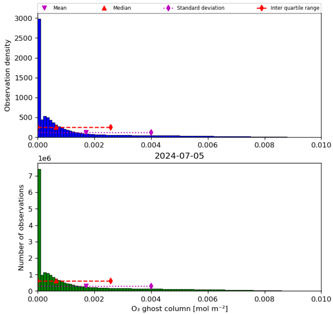
Figure 25: Histogram of “O 3 ghost column” for 2024-07-05 to 2024-07-06
