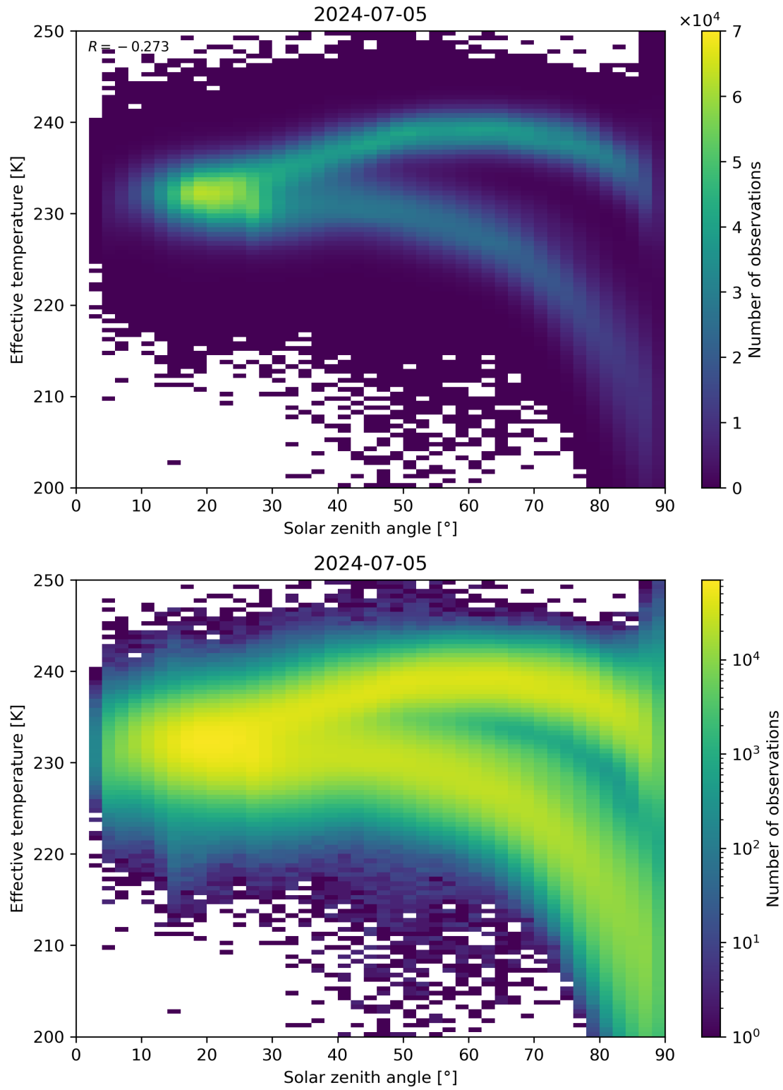
Figure 45: Scatter density plot of “Solar zenith angle” against “Effective temperature” for 2024-07-05 to 2024-07-06.
