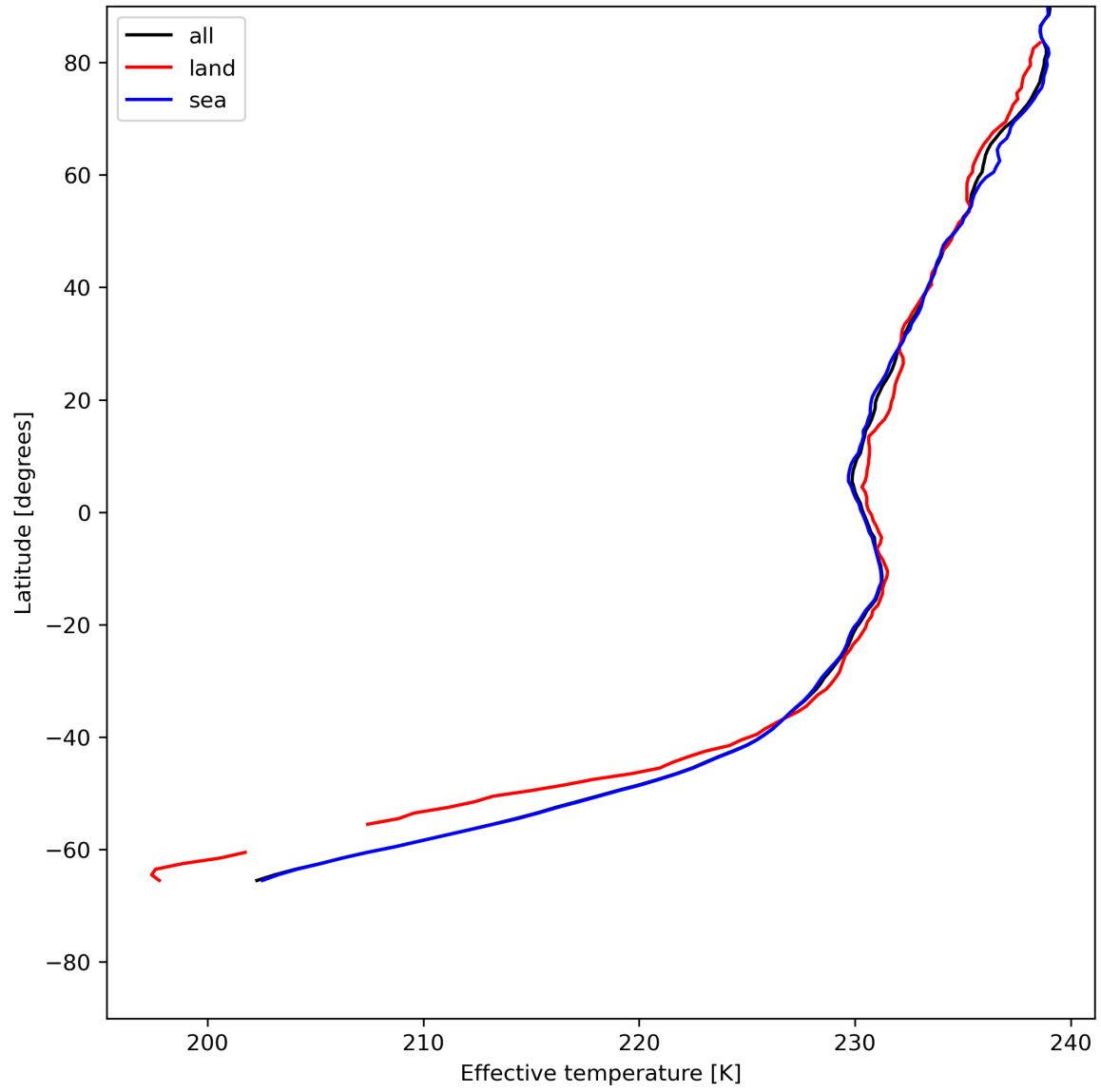
Figure 17: Zonal average of “Effective temperature” for 2024-07-05 to 2024-07-06.
