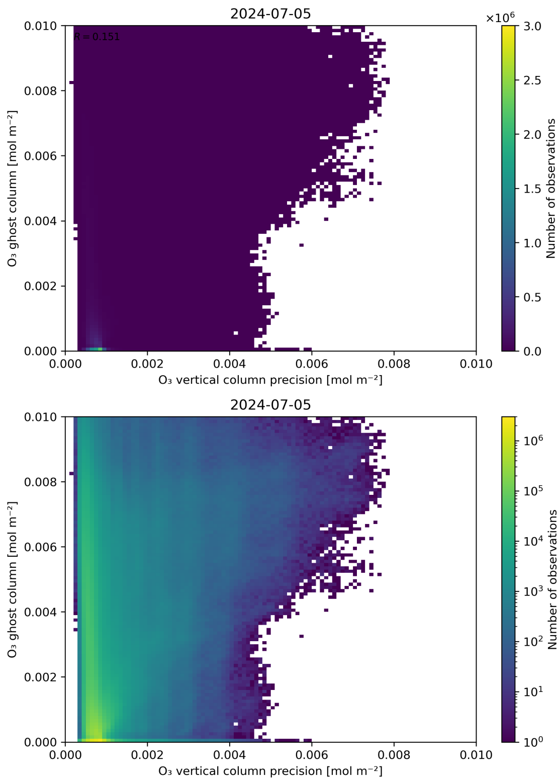
Figure 43: Scatter density plot of “ \text{O}_3 vertical column precision” against “ \text{O}_3 ghost column” for 2024-07-05 to 2024-07-06.
