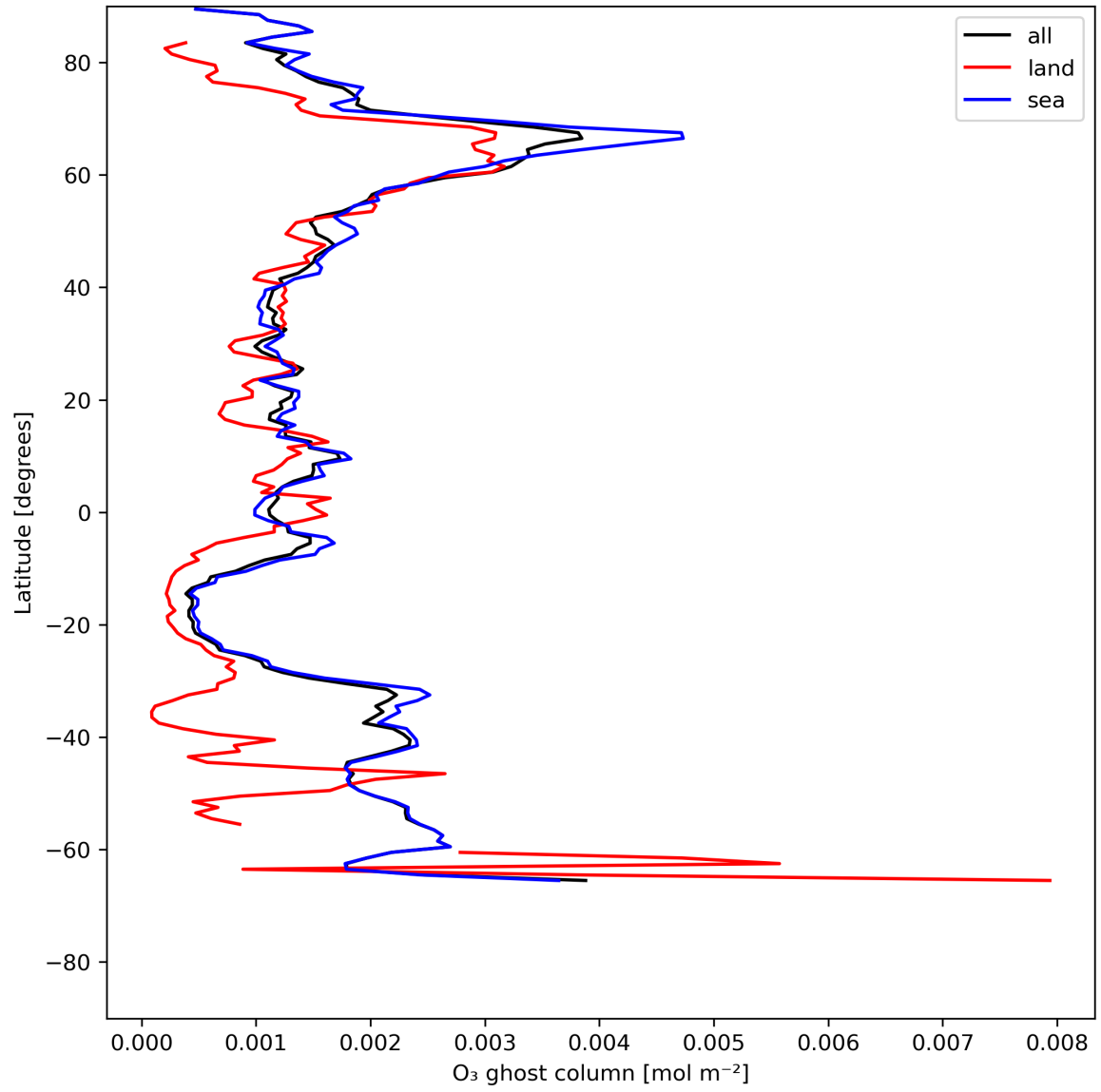
Figure 18: Zonal average of “O 3 ghost column” for 2024-07-05 to 2024-07-06.
