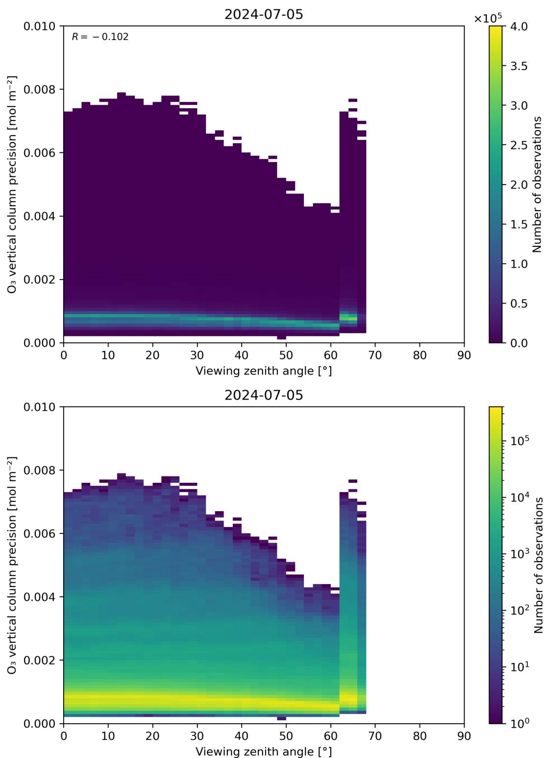
Figure 53: Scatter density plot of “Viewing zenith angle” against “O 3 vertical column precision” for 2024-07-05 to 2024-07-06.
