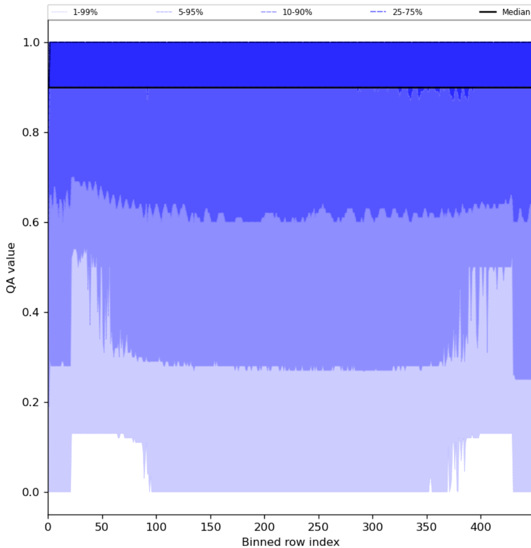
Figure 27: Along track statistics of “QA value” for 2024-07-05 to 2024-07-06
