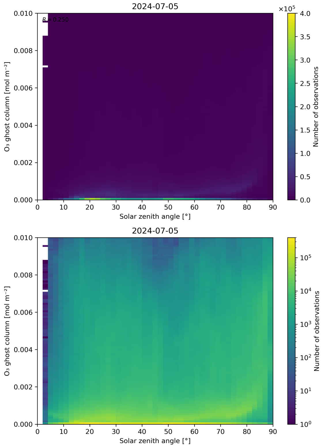
Figure 46: Scatter density plot of “Solar zenith angle” against “O 3 ghost column” for 2024-07-05 to 2024-07-06.
