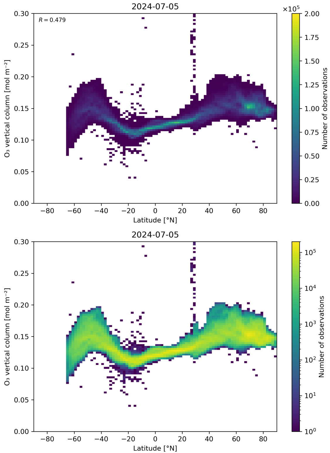
Figure 36: Scatter density plot of “Latitude” against “O 3 vertical column” for 2024-07-05 to 2024-07-06.
