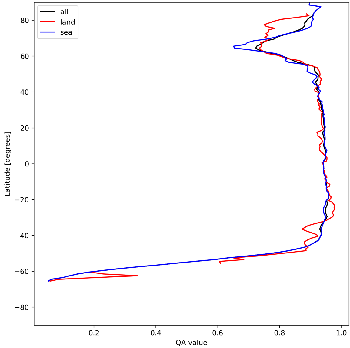
Figure 13: Zonal average of “QA value” for 2024-07-05 to 2024-07-06.
