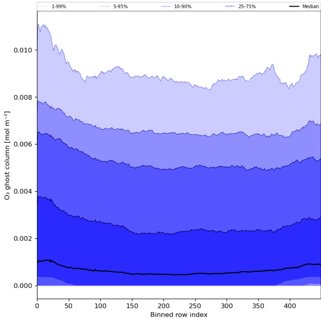
Figure 32: Along track statistics of “O 3 ghost column” for 2024-07-05 to 2024-07-06
