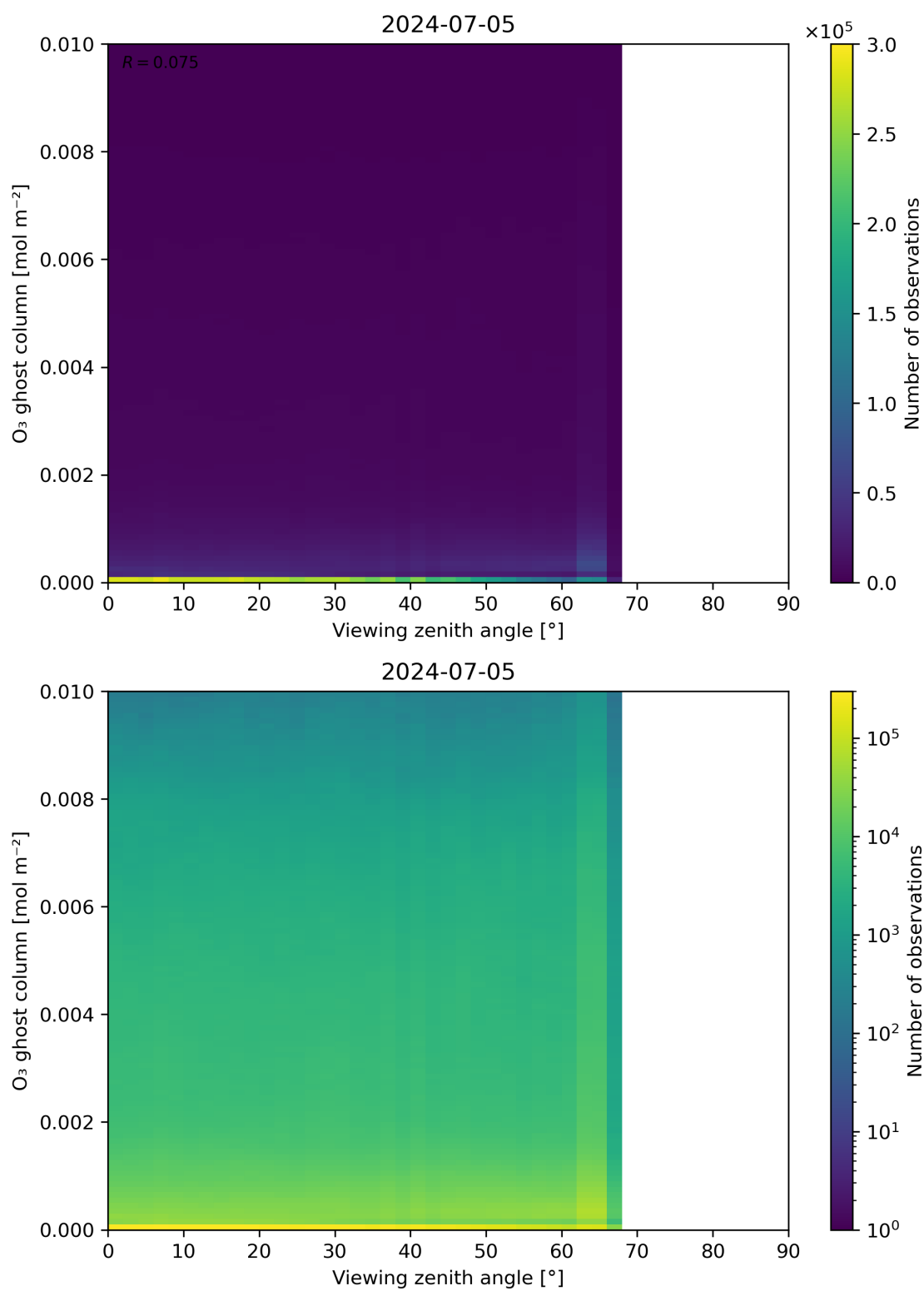
Figure 51: Scatter density plot of “Viewing zenith angle” against “O 3 ghost column” for 2024-07-05 to 2024-07-06.
