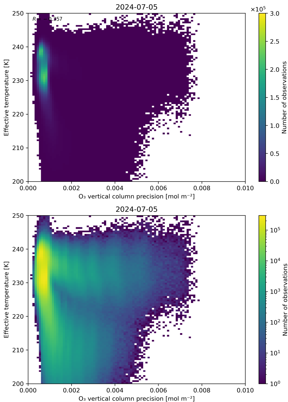
Figure 42: Scatter density plot of “O 3 vertical column precision” against “Effective temperature” for 2024-07-05 to 2024-07-06.
