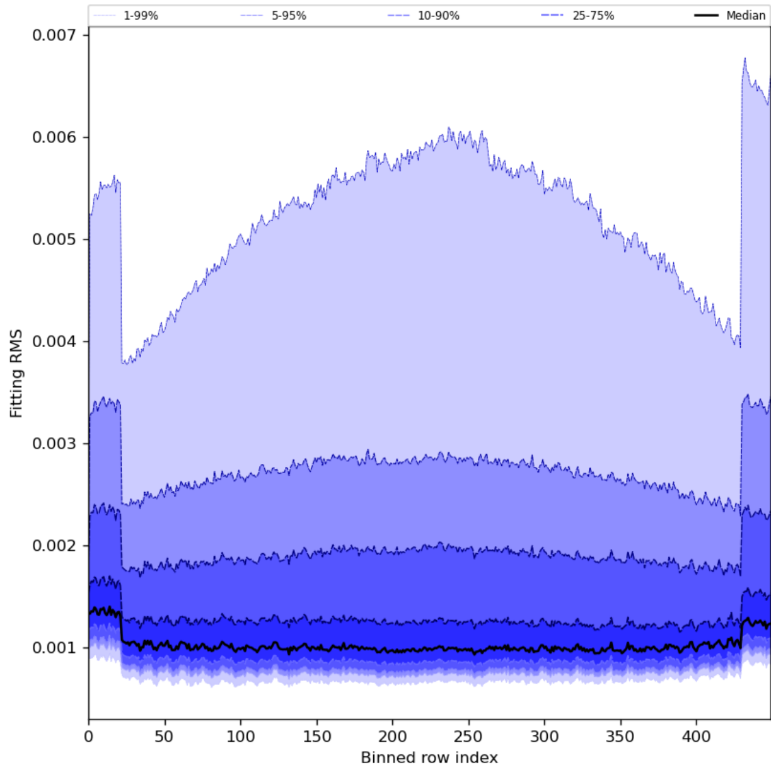
Figure 30: Along track statistics of “Fitting RMS” for 2024-07-05 to 2024-07-07
