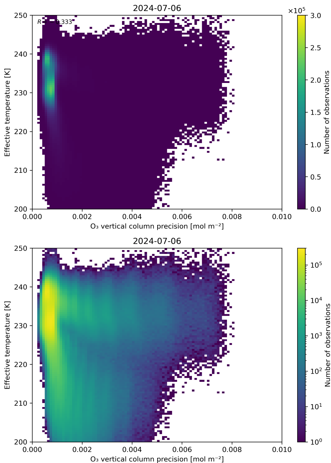
Figure 42: Scatter density plot of “O 3 vertical column precision” against “Effective temperature” for 2024-07-05 to 2024-07-07.
