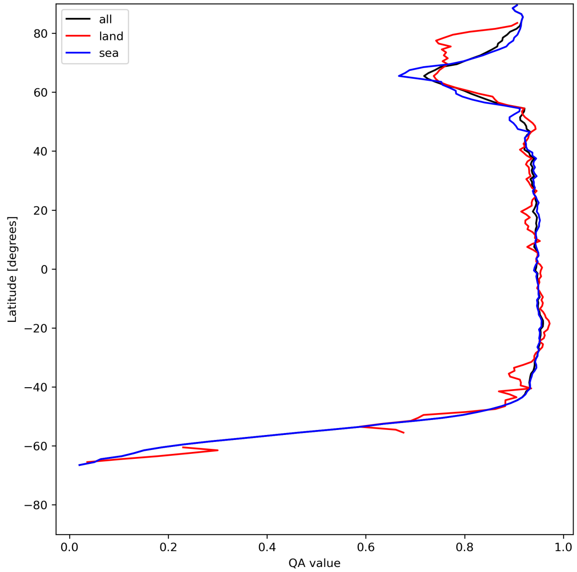
Figure 13: Zonal average of “QA value” for 2024-07-05 to 2024-07-07.
