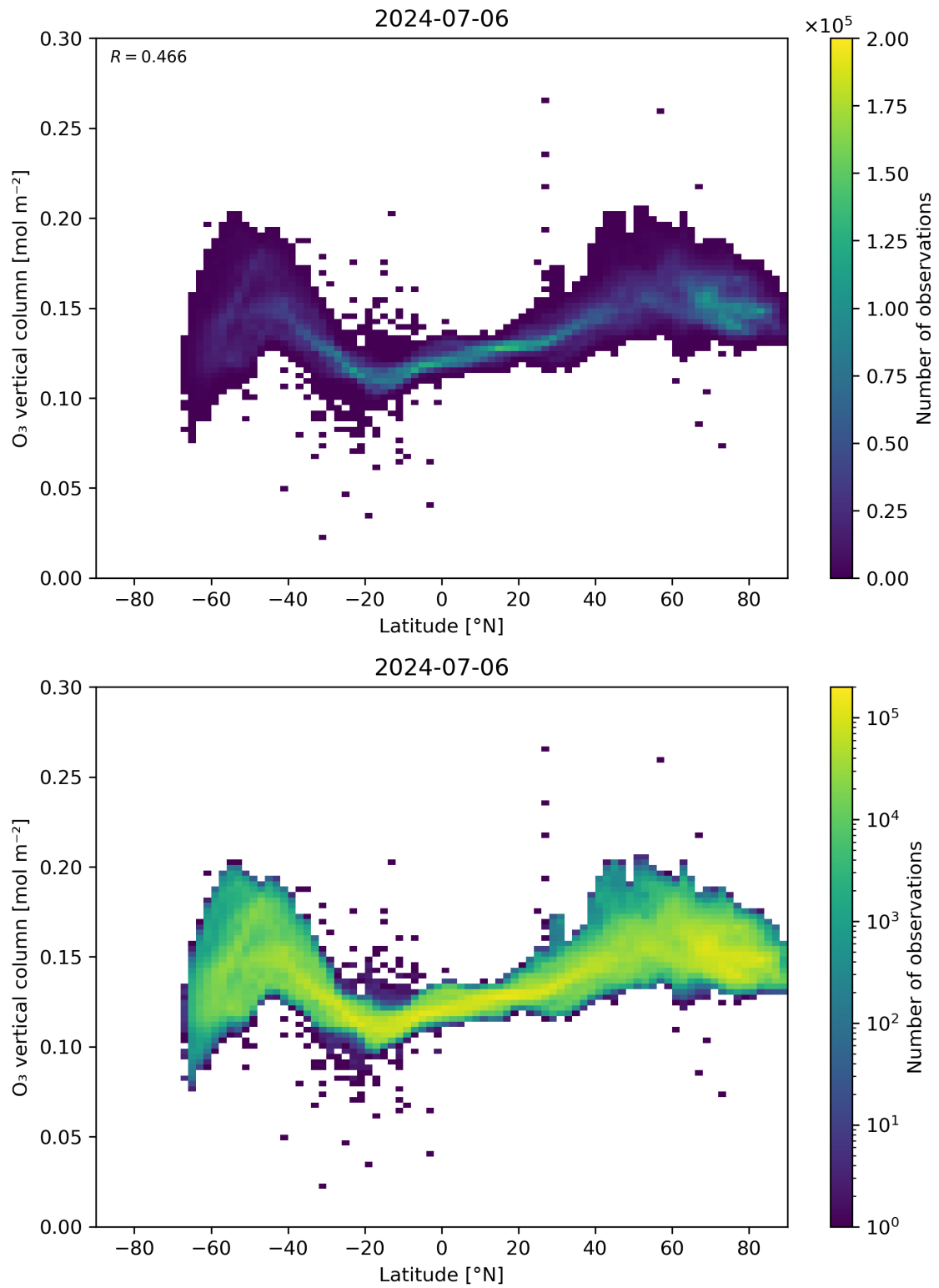
Figure 36: Scatter density plot of “Latitude” against “O 3 vertical column” for 2024-07-05 to 2024-07-07.
