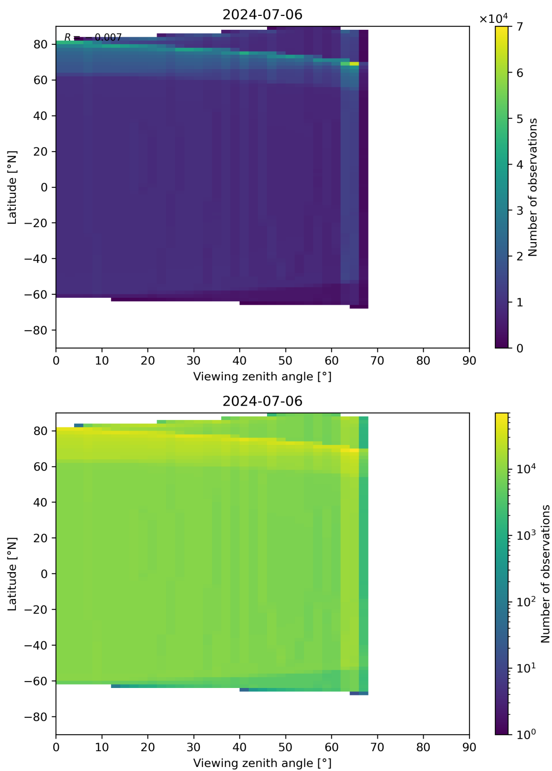
Figure 49: Scatter density plot of “Viewing zenith angle” against “Latitude” for 2024-07-05 to 2024-07-07.
