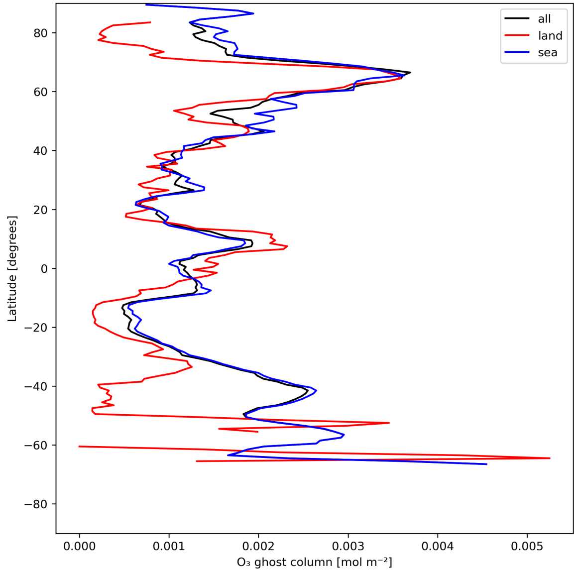
Figure 18: Zonal average of "O 3 ghost column" for 2024-07-05 to 2024-07-07.
