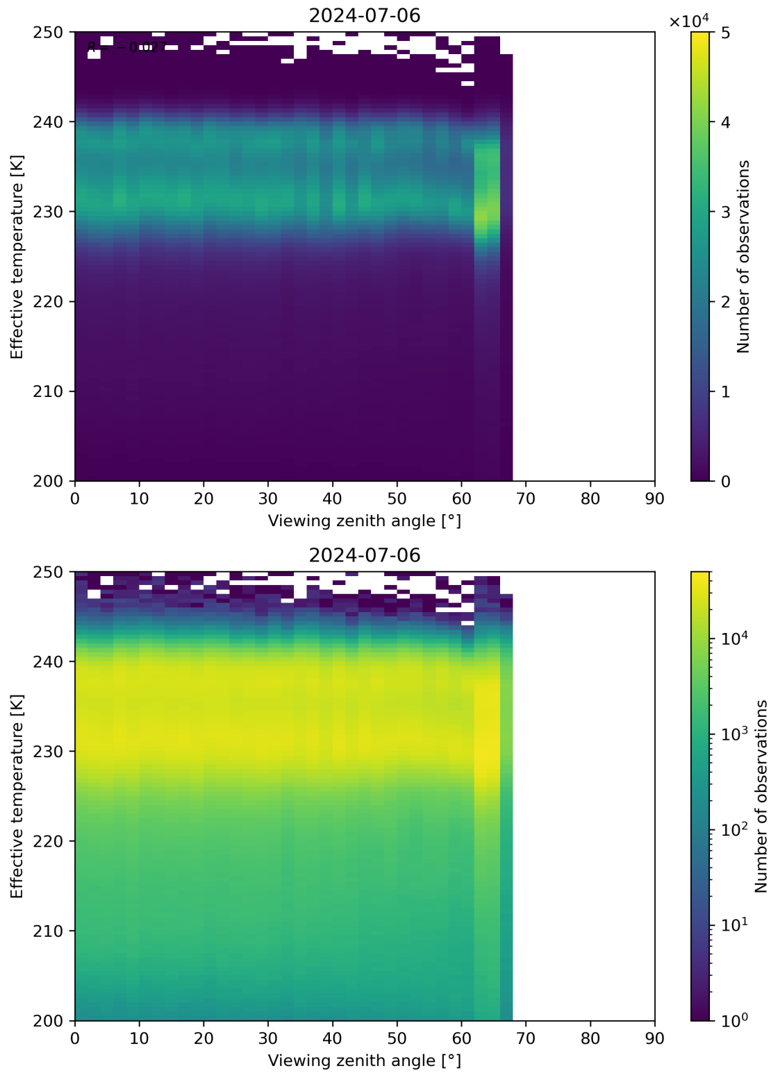
Figure 50: Scatter density plot of “Viewing zenith angle” against “Effective temperature” for 2024-07-05 to 2024-07-07.
