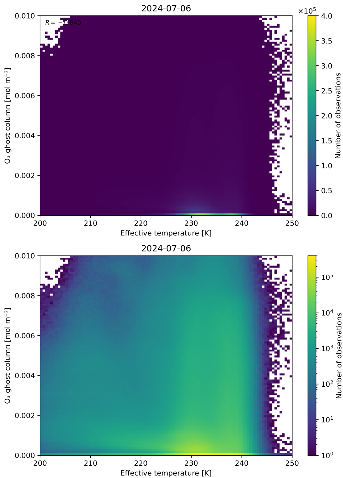
Figure 38: Scatter density plot of “Effective temperature” against “O 3 ghost column” for 2024-07-05 to 2024-07-07.
