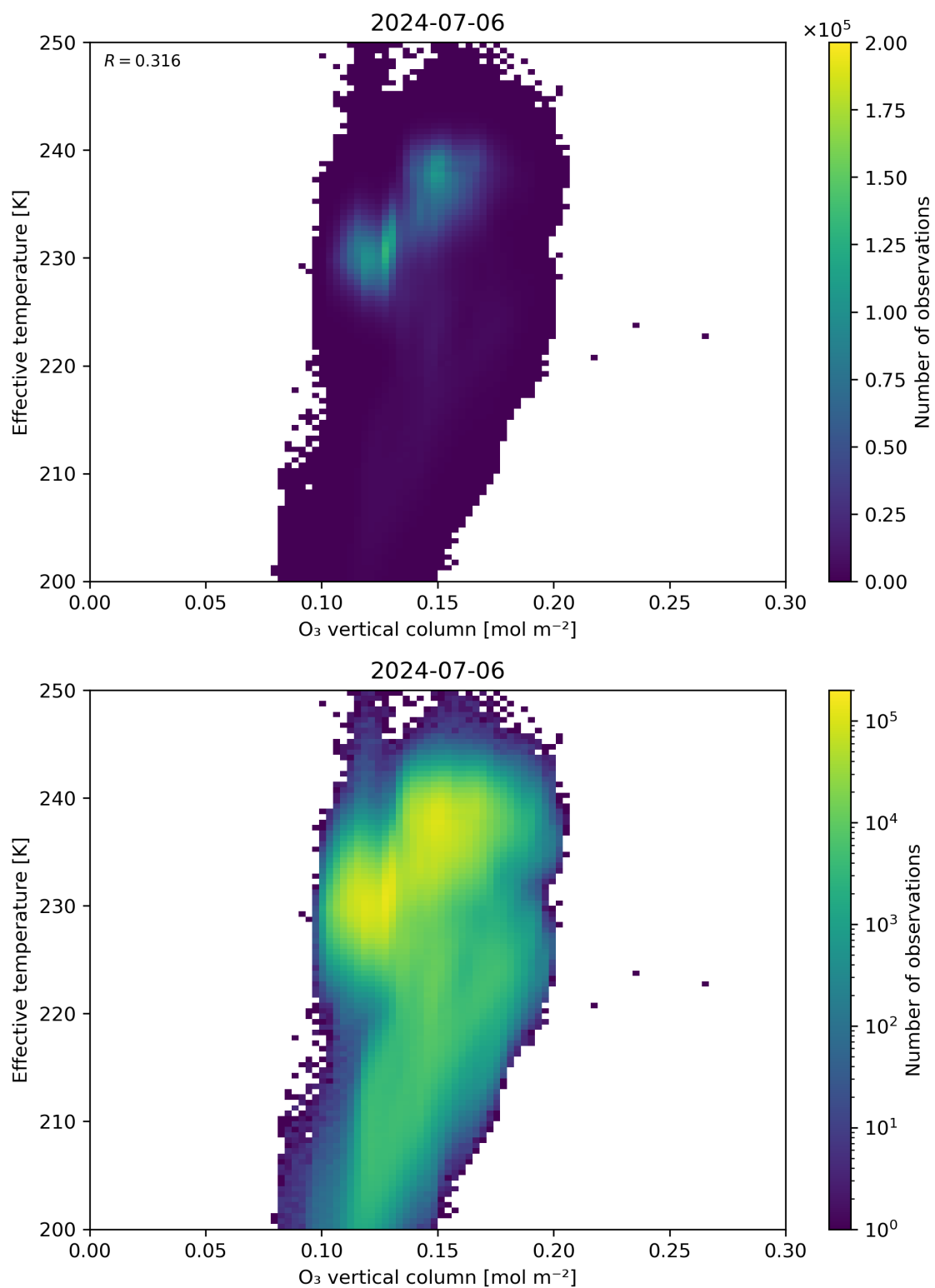
Figure 39: Scatter density plot of “O 3 vertical column” against “Effective temperature” for 2024-07-05 to 2024-07-07.
