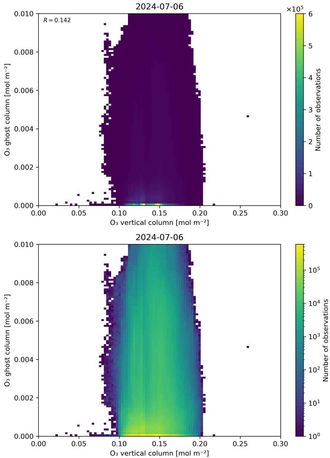
Figure 40: Scatter density plot of “O 3 vertical column” against “O 3 ghost column” for 2024-07-05 to 2024-07-07.
