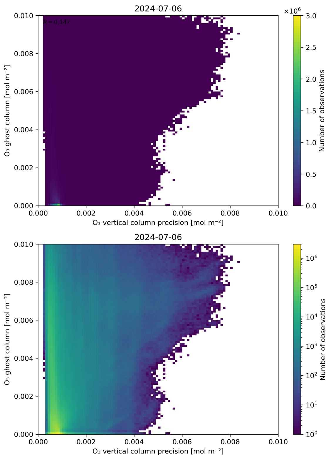
Figure 43: Scatter density plot of “ \text{O}_3 vertical column precision” against “ \text{O}_3 ghost column” for 2024-07-05 to 2024-07-07.
