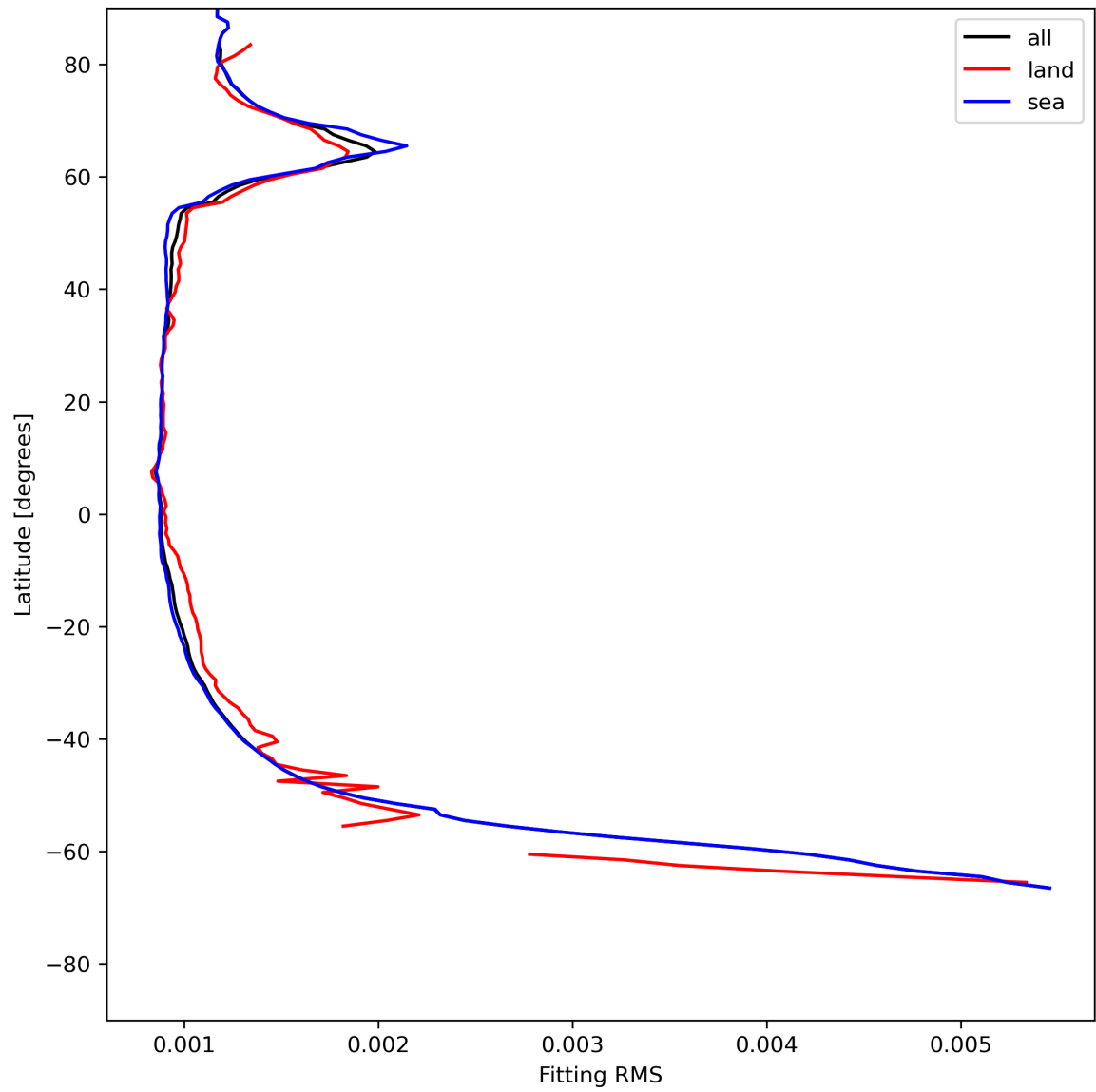
Figure 16: Zonal average of “Fitting RMS” for 2024-07-05 to 2024-07-07.
