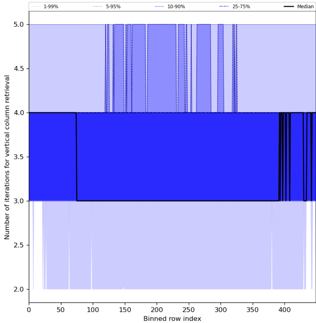
Figure 33: Along track statistics of “Number of iterations for vertical column retrieval” for 2024-07-05 to 2024-07-07
