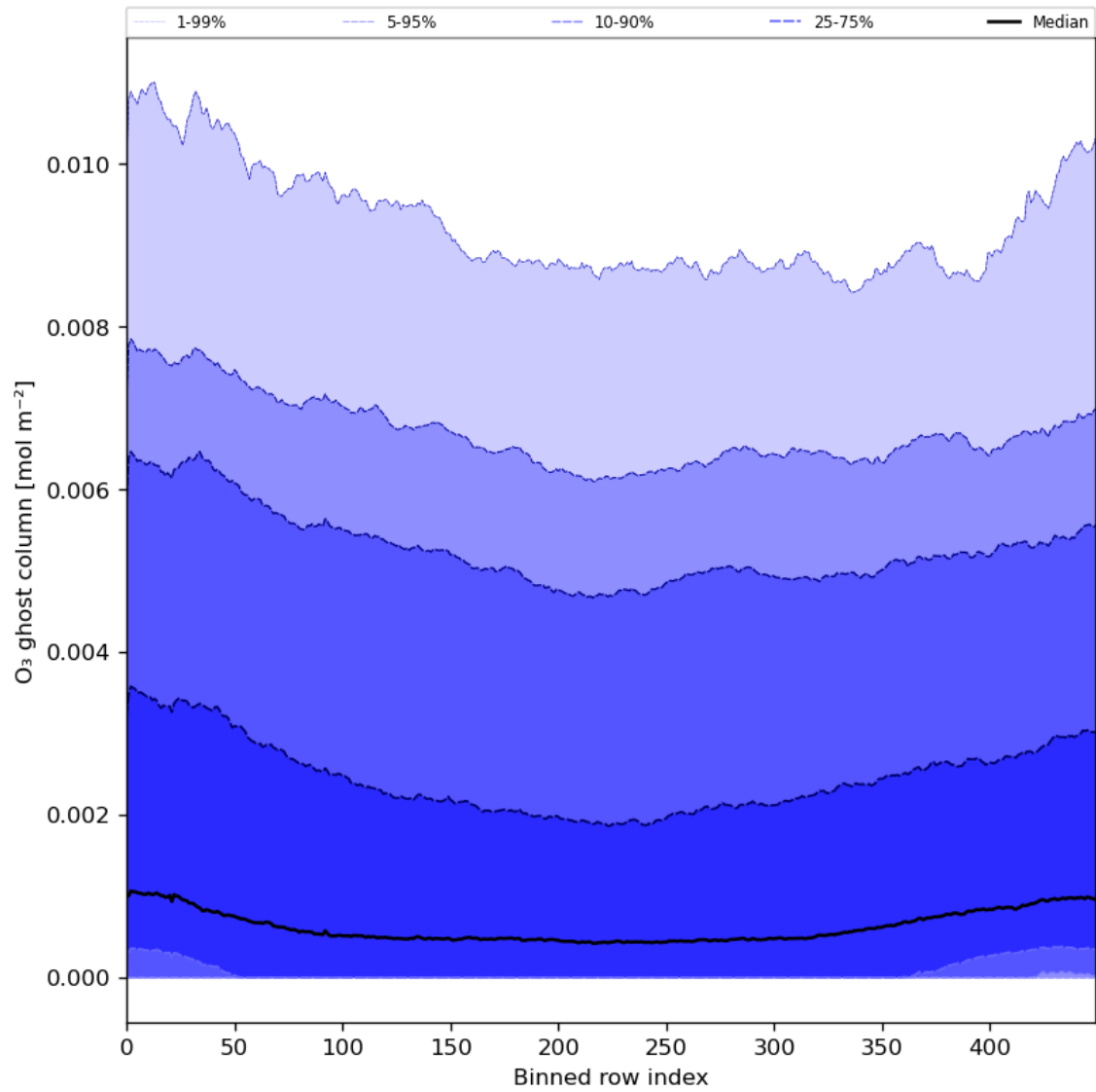
Figure 32: Along track statistics of “O 3 ghost column” for 2024-07-05 to 2024-07-07
