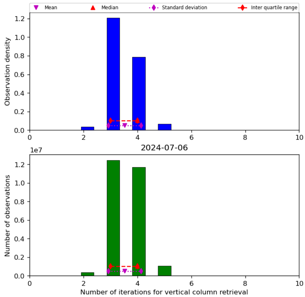
Figure 26: Histogram of “Number of iterations for vertical column retrieval” for 2024-07-05 to 2024-07-07
