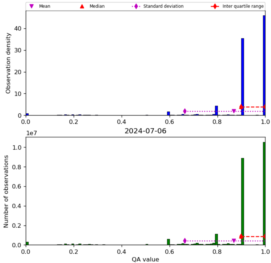
Figure 20: Histogram of “QA value” for 2024-07-05 to 2024-07-07
