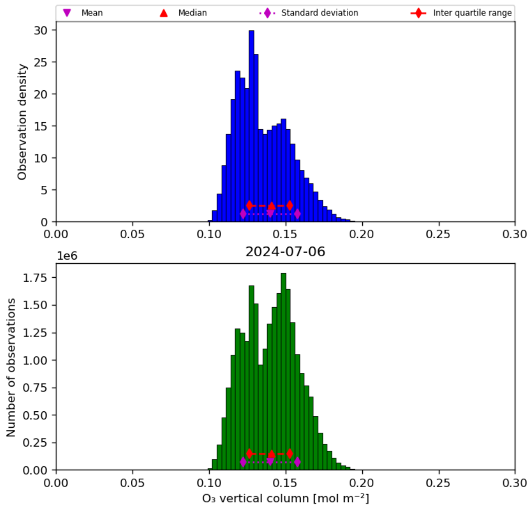
Figure 21: Histogram of “O 3 vertical column” for 2024-07-05 to 2024-07-07
