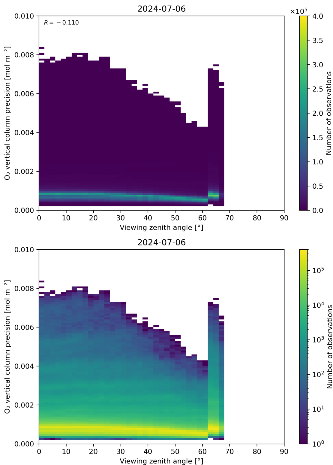
Figure 53: Scatter density plot of “Viewing zenith angle” against “O 3 vertical column precision” for 2024-07-05 to 2024-07-07.
