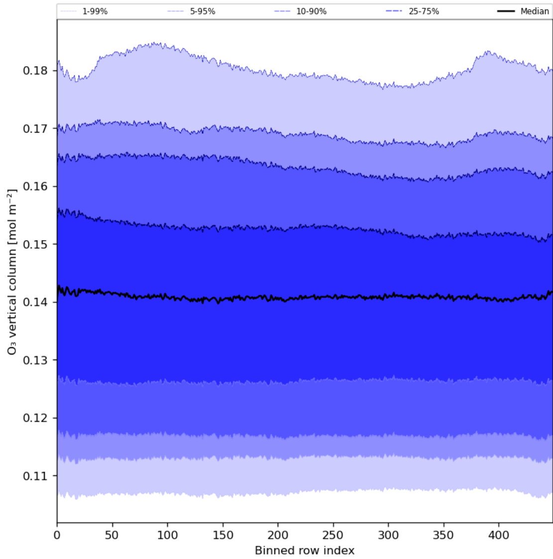
Figure 28: Along track statistics of “O 3 vertical column” for 2024-07-05 to 2024-07-07
