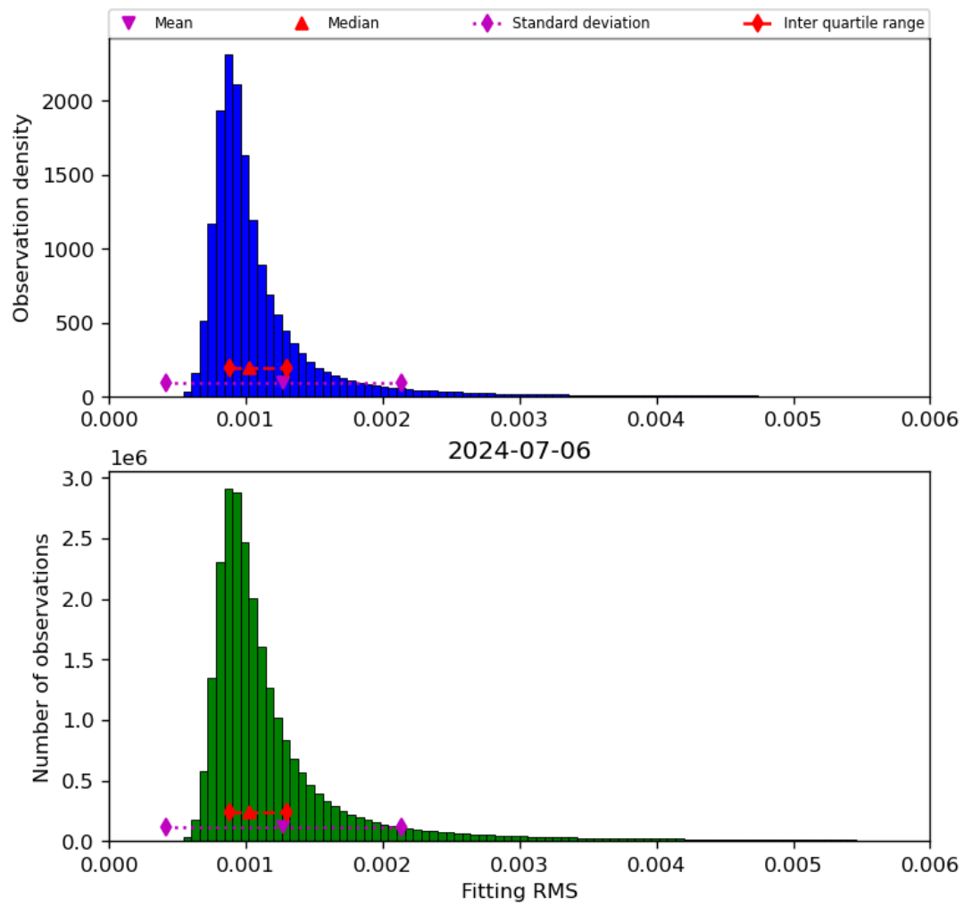
Figure 23: Histogram of “Fitting RMS” for 2024-07-05 to 2024-07-07
