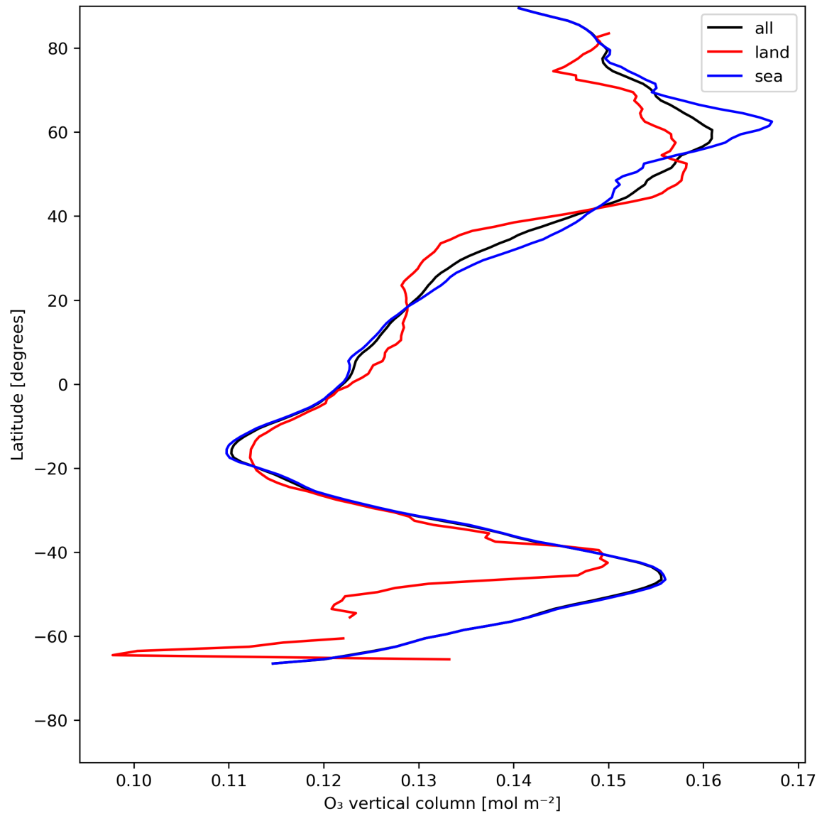
Figure 14: Zonal average of “O 3 vertical column” for 2024-07-05 to 2024-07-07.
