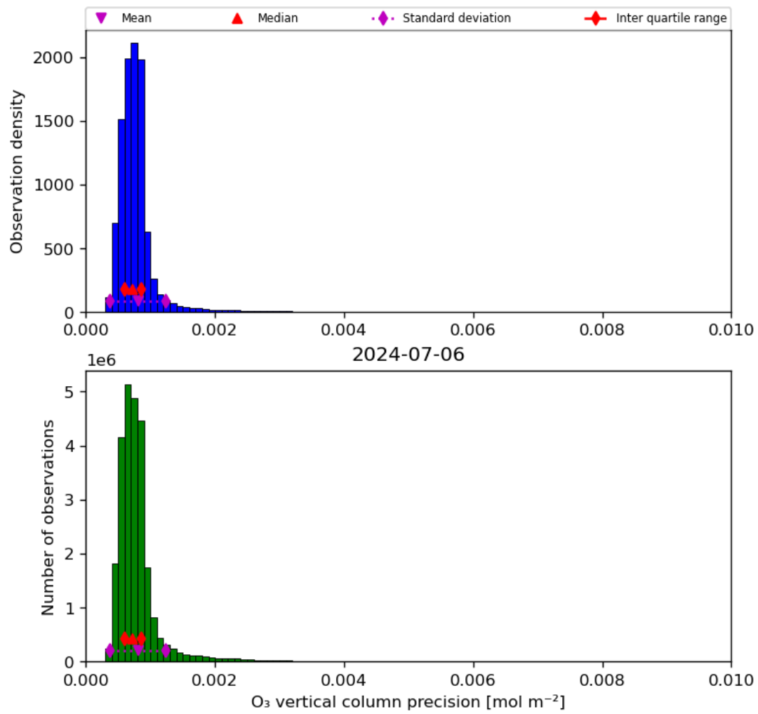
Figure 22: Histogram of “O 3 vertical column precision” for 2024-07-05 to 2024-07-07
