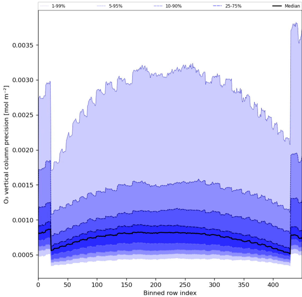
Figure 29: Along track statistics of “O 3 vertical column precision” for 2024-07-05 to 2024-07-07
