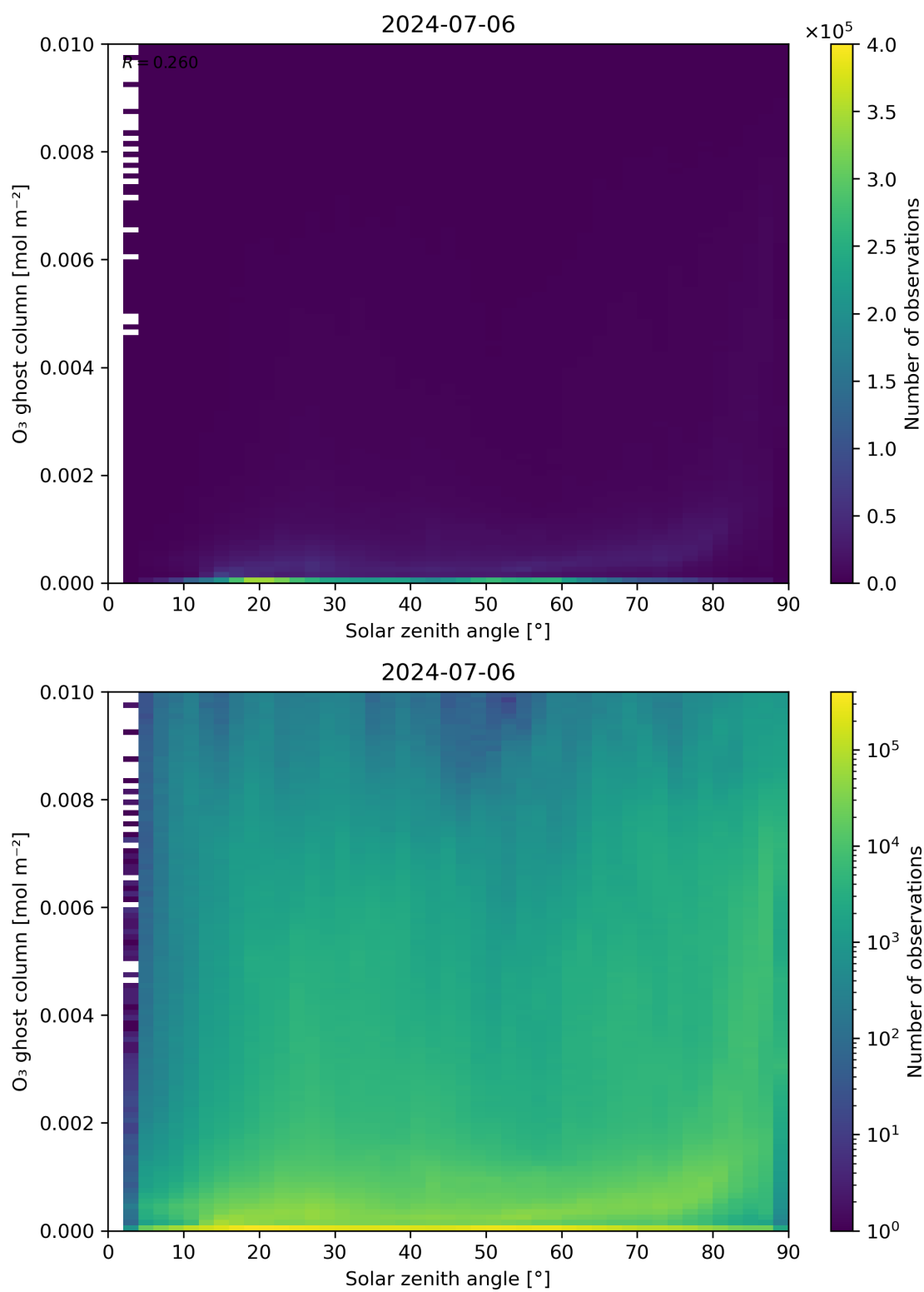
Figure 46: Scatter density plot of “Solar zenith angle” against “O 3 ghost column” for 2024-07-05 to 2024-07-07.
