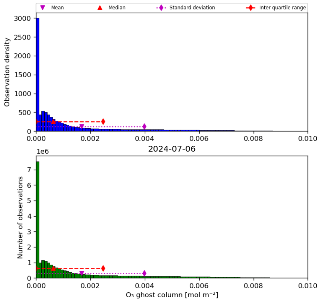
Figure 25: Histogram of “O 3 ghost column” for 2024-07-05 to 2024-07-07
