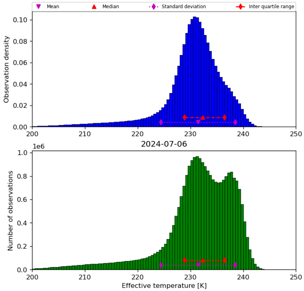
Figure 24: Histogram of “Effective temperature” for 2024-07-05 to 2024-07-07
