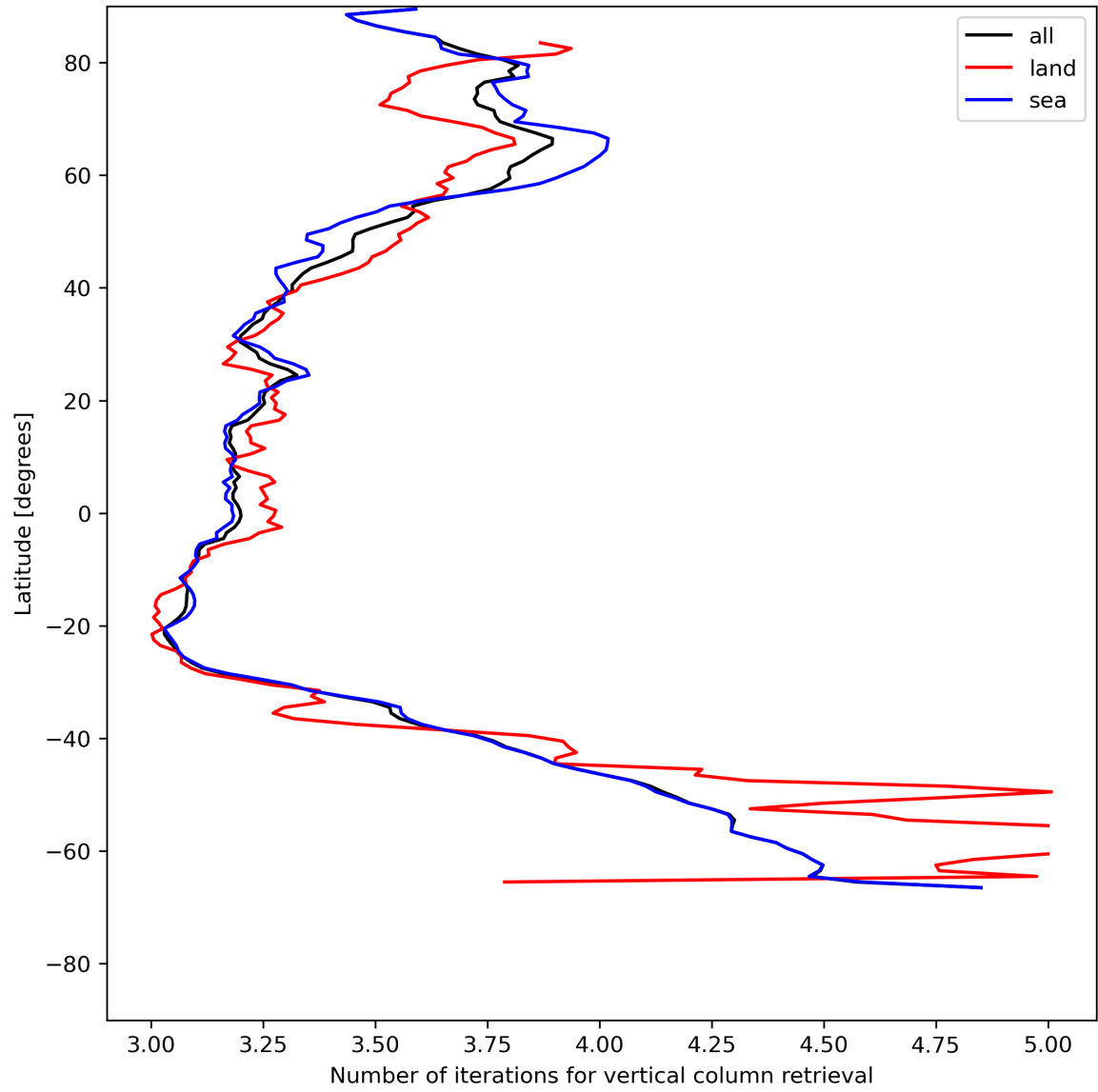
Figure 19: Zonal average of “Number of iterations for vertical column retrieval” for 2024-07-05 to 2024-07-07.
