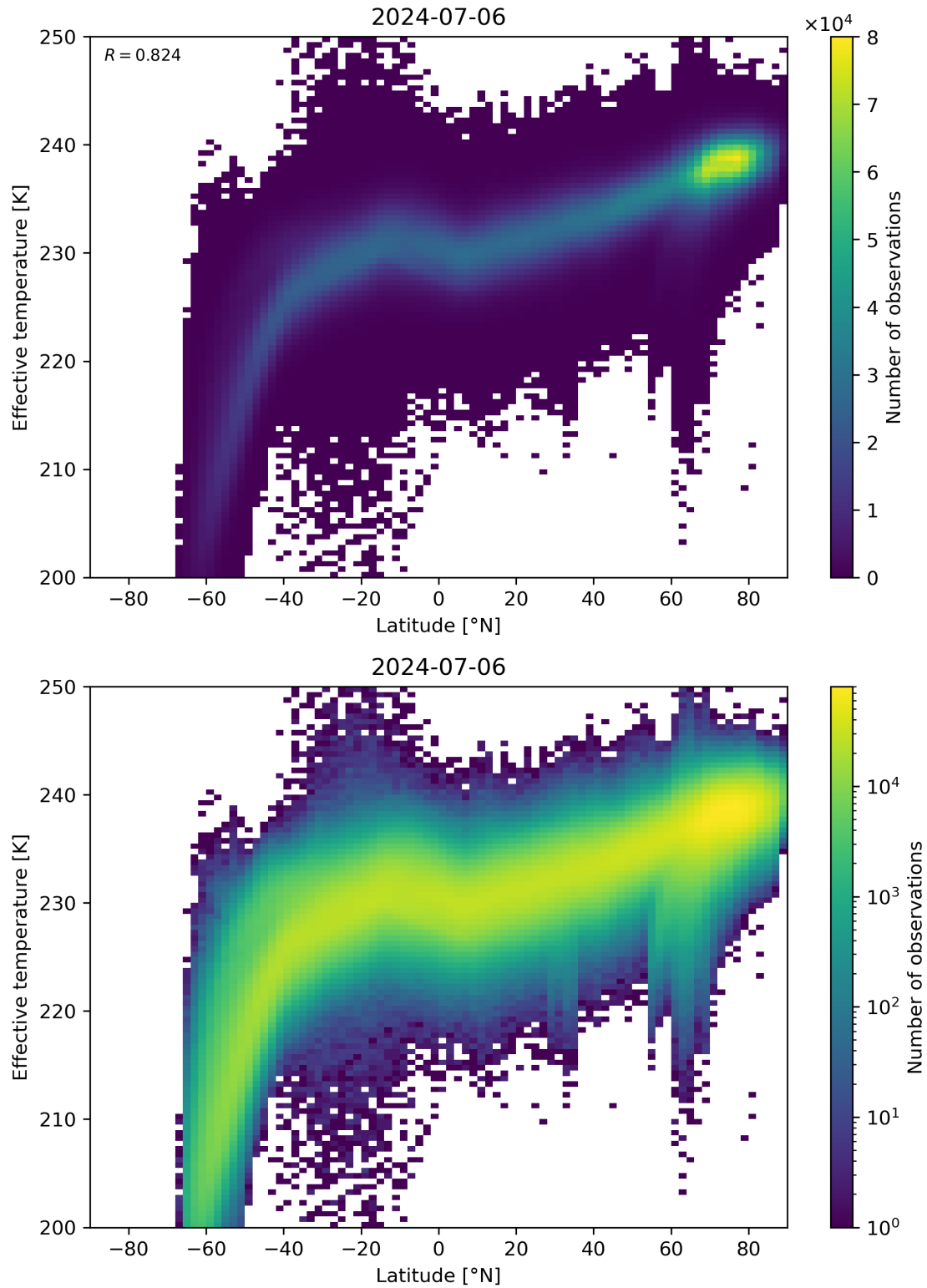
Figure 34: Scatter density plot of “Latitude” against “Effective temperature” for 2024-07-05 to 2024-07-07.
