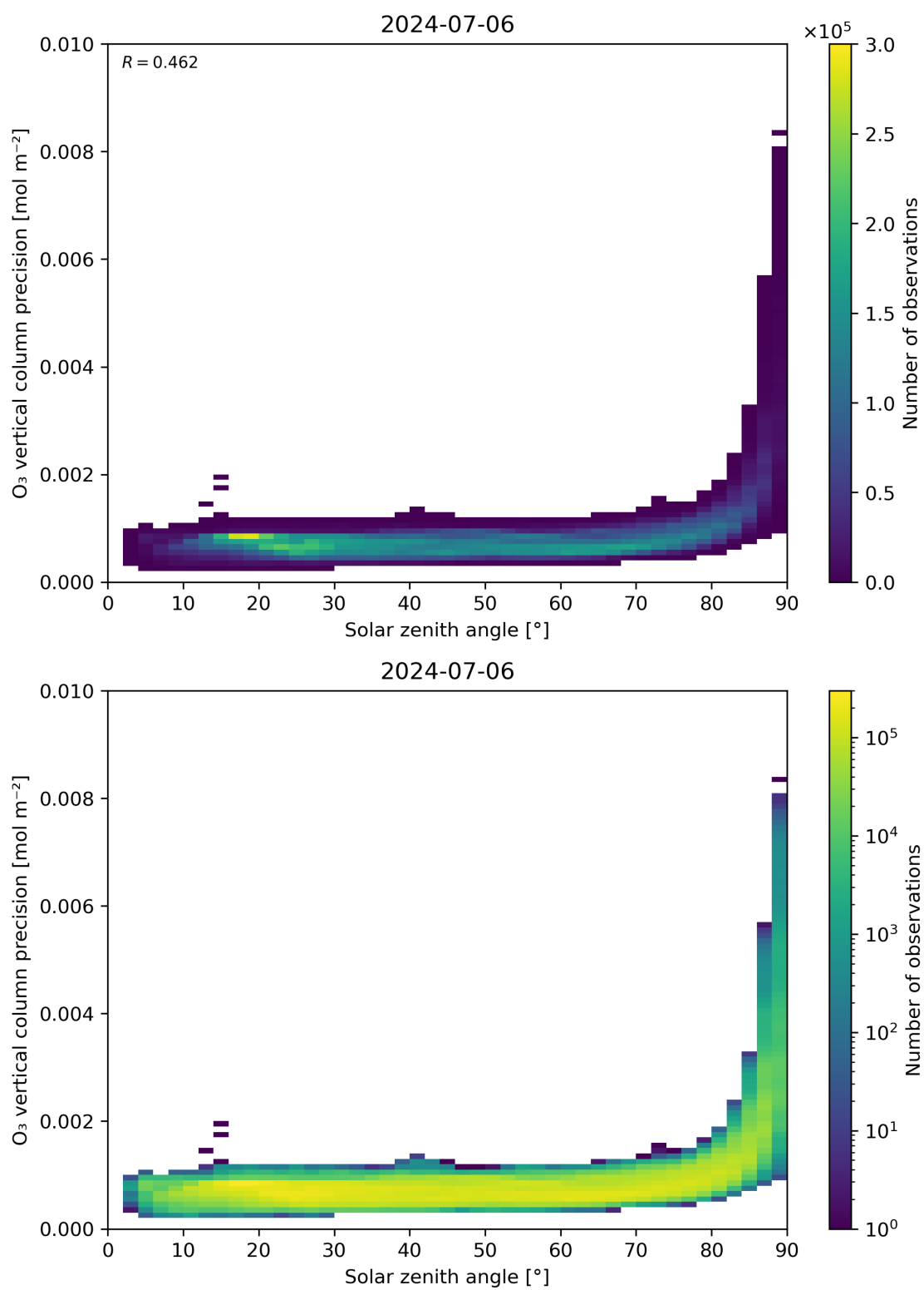
Figure 48: Scatter density plot of “Solar zenith angle” against “O 3 vertical column precision” for 2024-07-05 to 2024-07-07.
