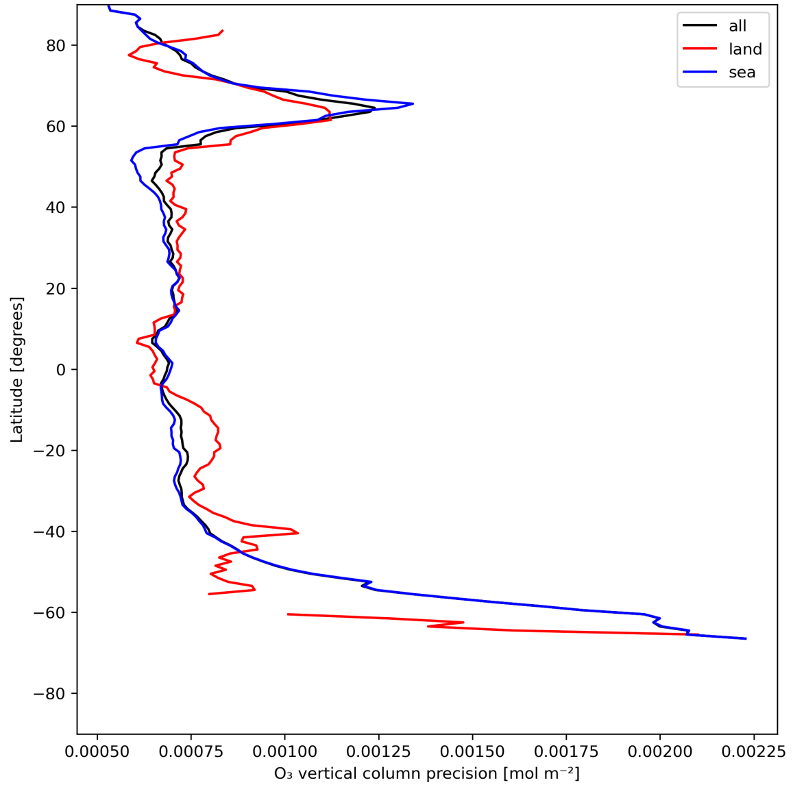
Figure 15: Zonal average of “O 3 vertical column precision” for 2024-07-05 to 2024-07-07.
