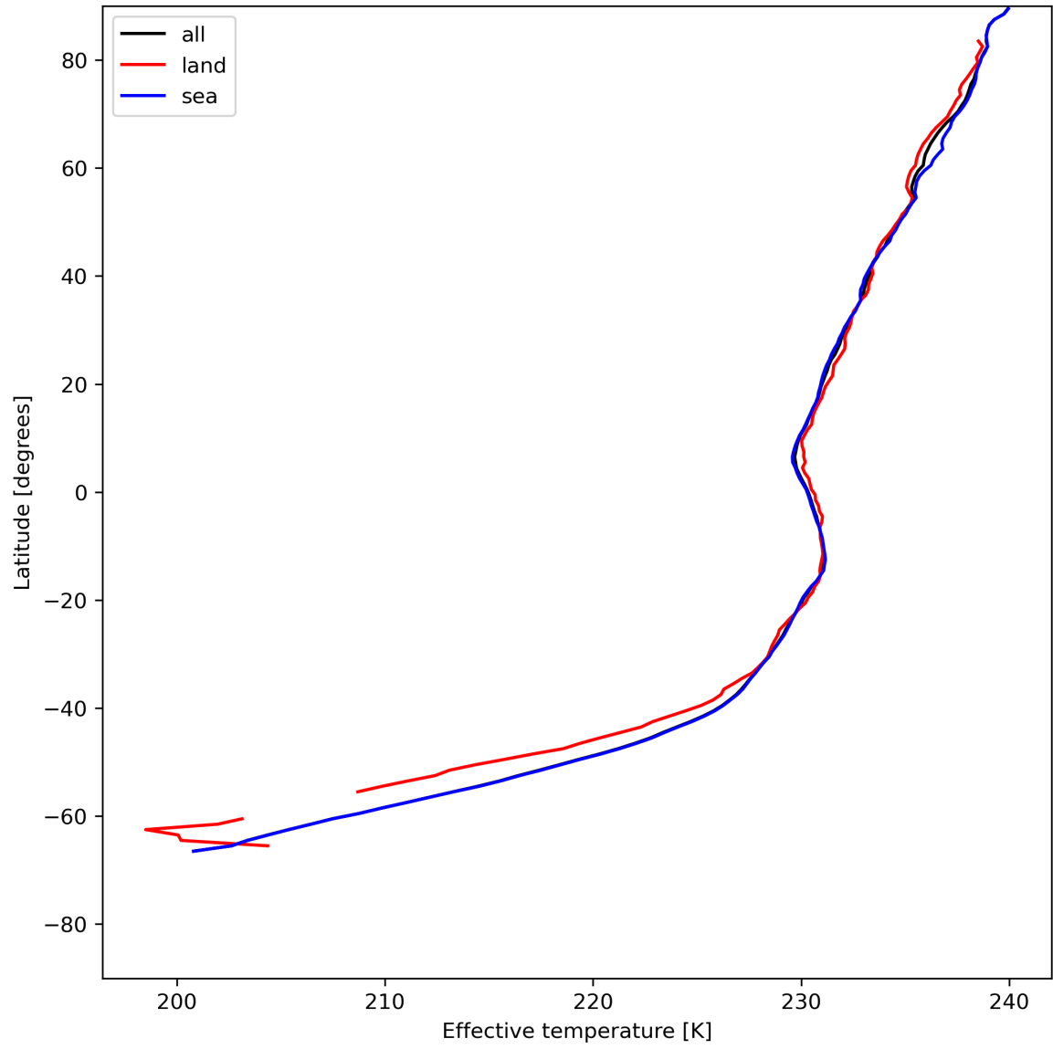
Figure 17: Zonal average of “Effective temperature” for 2024-07-05 to 2024-07-07.
