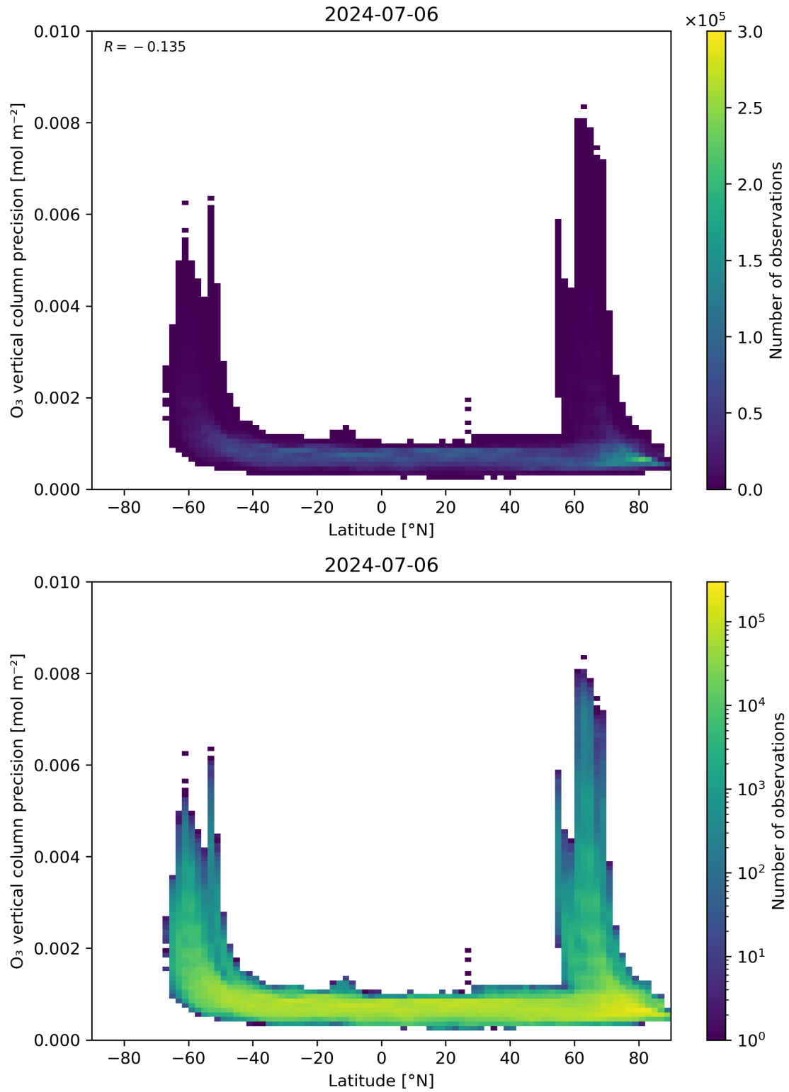
Figure 37: Scatter density plot of “Latitude” against “O 3 vertical column precision” for 2024-07-05 to 2024-07-07.
