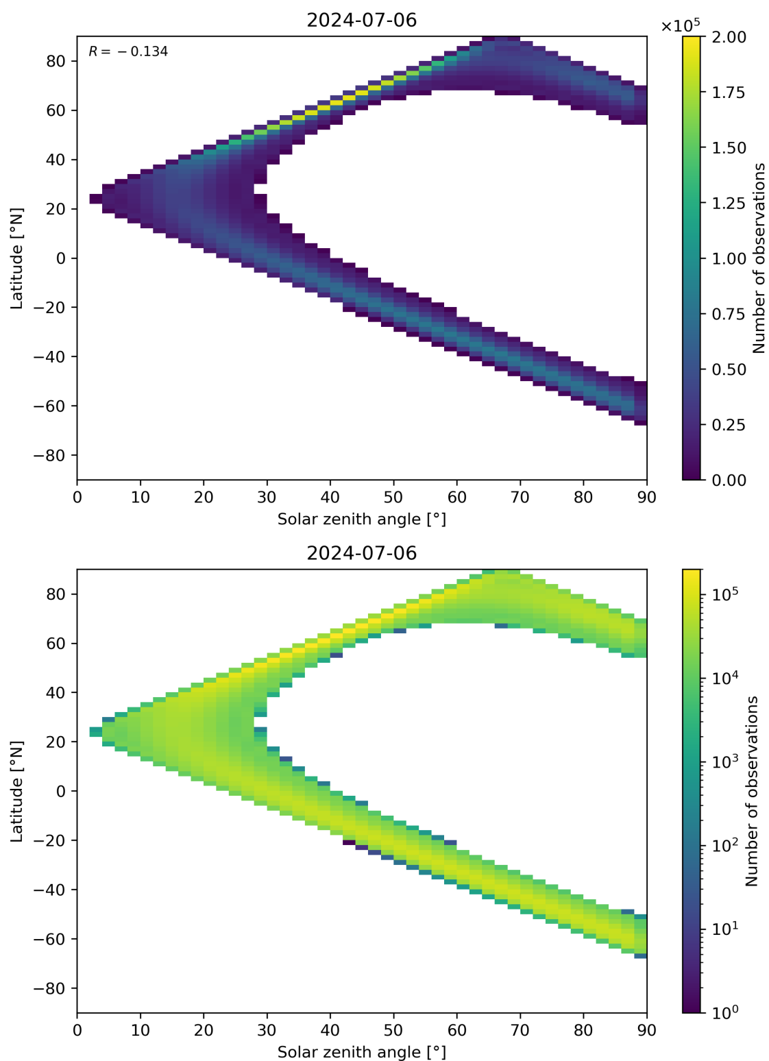
Figure 44: Scatter density plot of “Solar zenith angle” against “Latitude” for 2024-07-05 to 2024-07-07.
