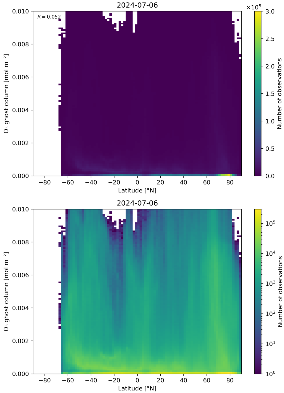
Figure 35: Scatter density plot of “Latitude” against “O 3 ghost column” for 2024-07-05 to 2024-07-07.
