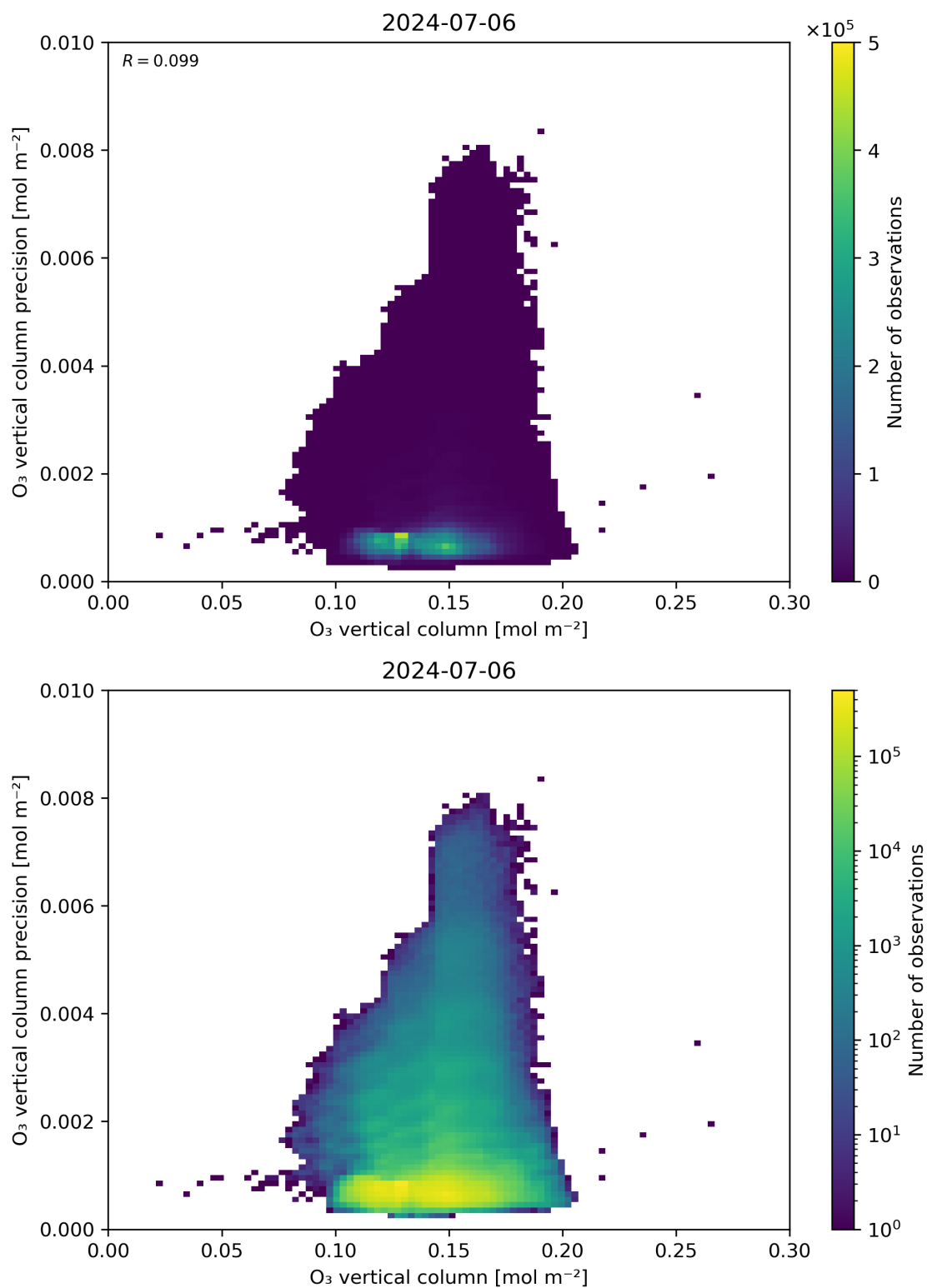
Figure 41: Scatter density plot of “O 3 vertical column” against “O 3 vertical column precision” for 2024-07-05 to 2024-07-07.
