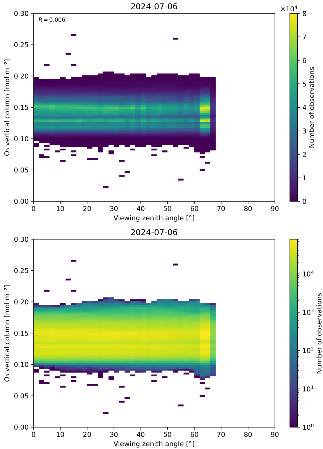
Figure 52: Scatter density plot of “Viewing zenith angle” against “O 3 vertical column” for 2024-07-05 to 2024-07-07.
