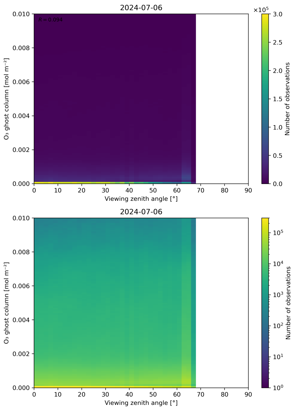
Figure 51: Scatter density plot of “Viewing zenith angle” against “O 3 ghost column” for 2024-07-05 to 2024-07-07.
