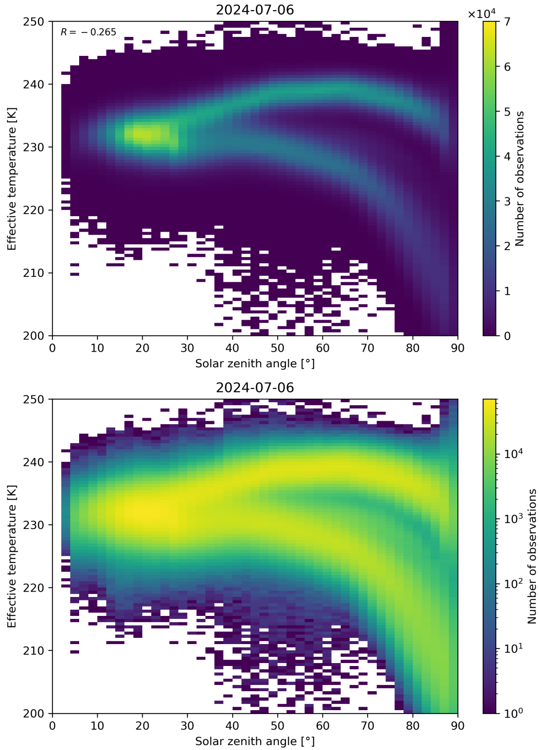
Figure 45: Scatter density plot of “Solar zenith angle” against “Effective temperature” for 2024-07-05 to 2024-07-07.
