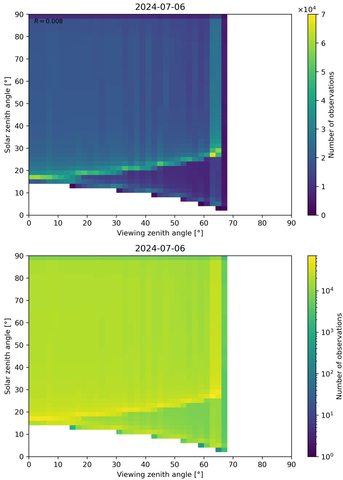
Figure 54: Scatter density plot of “Viewing zenith angle” against “Solar zenith angle” for 2024-07-05 to 2024-07-07.
