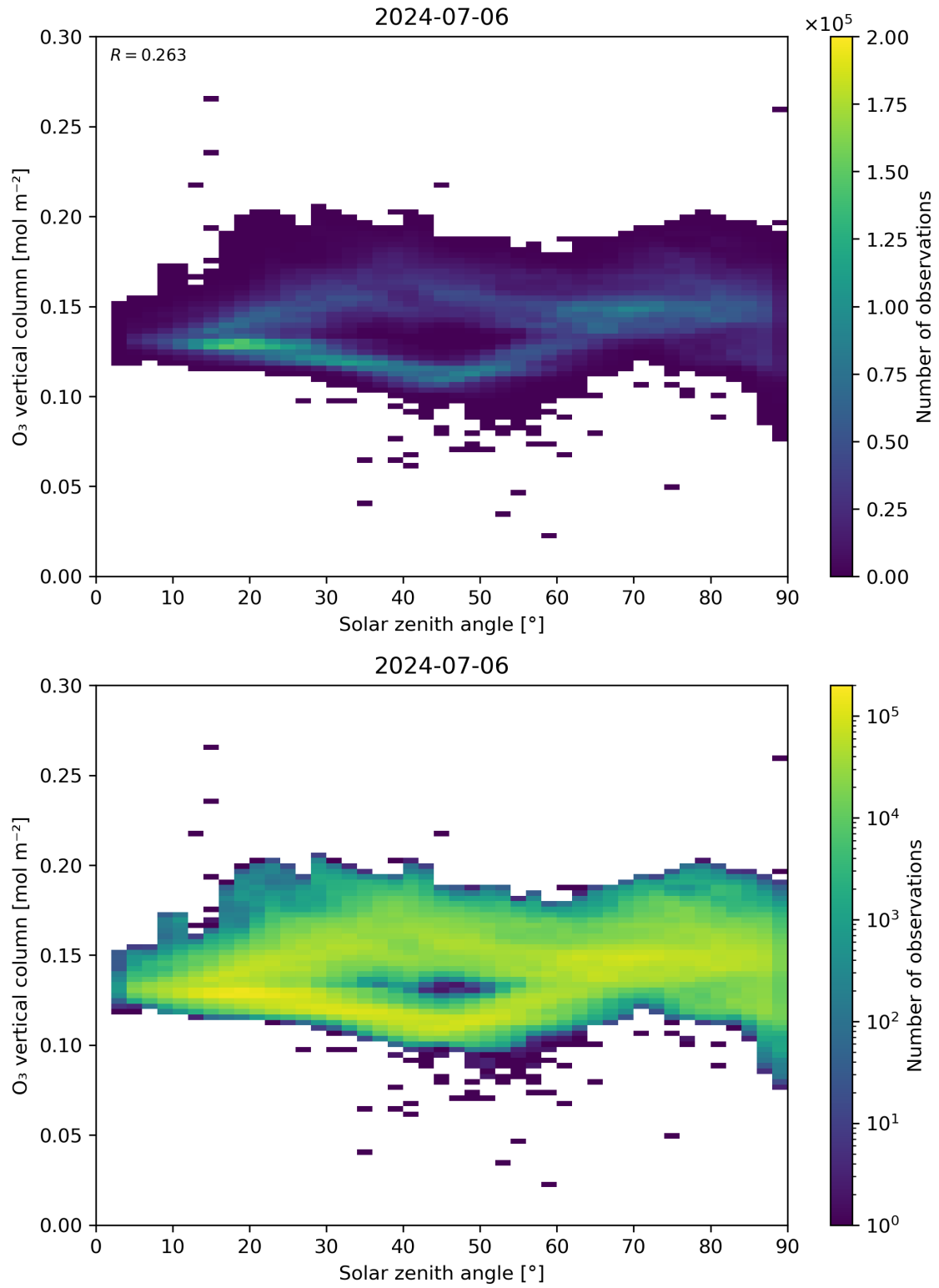
Figure 47: Scatter density plot of “Solar zenith angle” against “O 3 vertical column” for 2024-07-05 to 2024-07-07.
