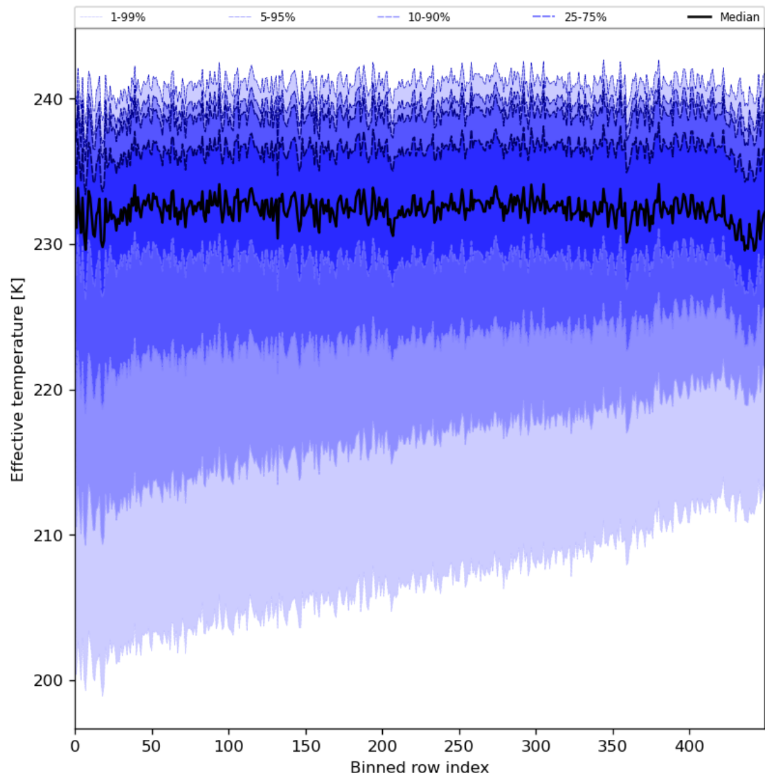
Figure 31: Along track statistics of “Effective temperature” for 2024-07-05 to 2024-07-07
