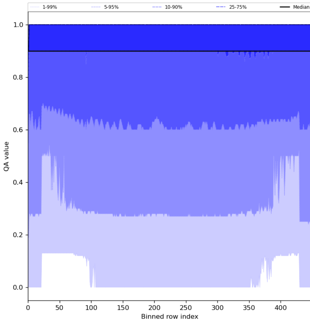
Figure 27: Along track statistics of “QA value” for 2024-07-05 to 2024-07-07
