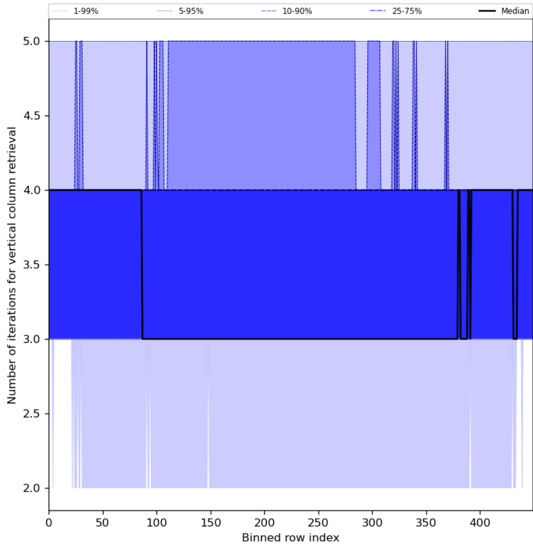
Figure 33: Along track statistics of “Number of iterations for vertical column retrieval” for 2024-07-07 to 2024-07-09
