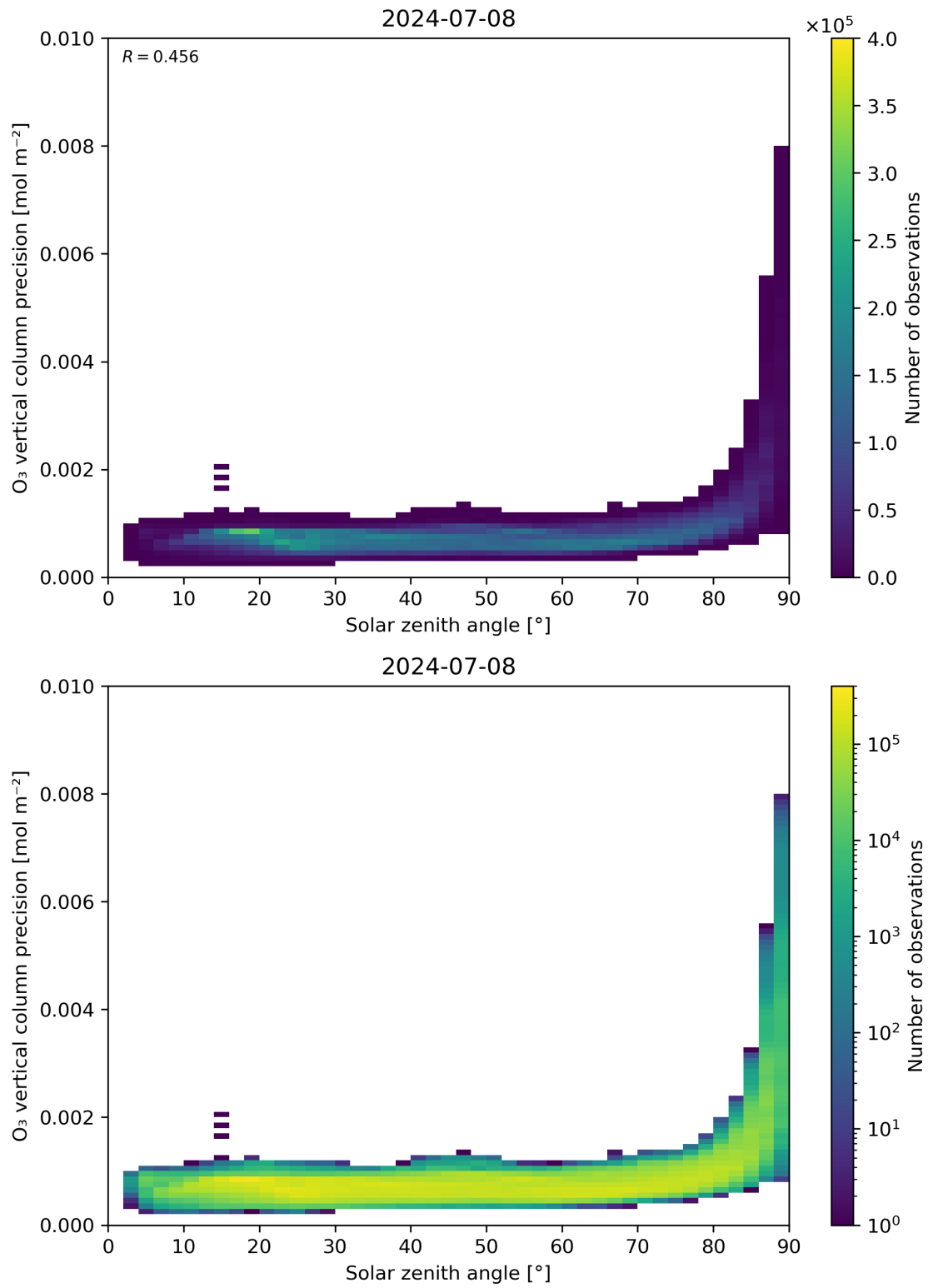
Figure 48: Scatter density plot of “Solar zenith angle” against “O 3 vertical column precision” for 2024-07-07 to 2024-07-09.
