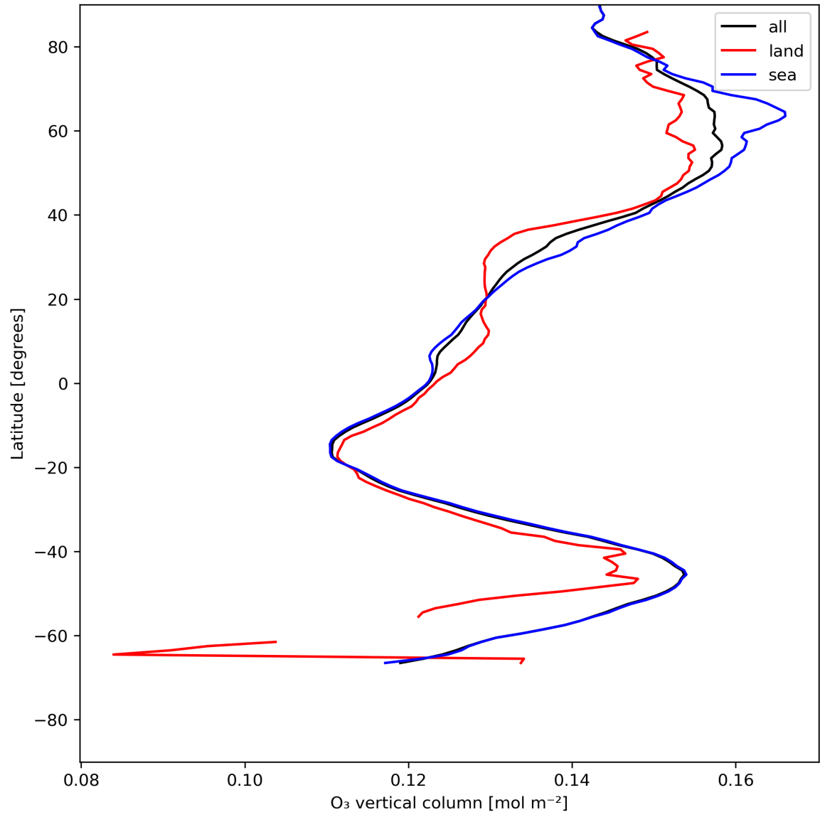
Figure 14: Zonal average of “O 3 vertical column” for 2024-07-07 to 2024-07-09.
