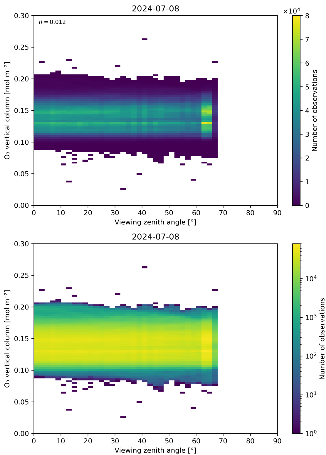
Figure 52: Scatter density plot of “Viewing zenith angle” against “O 3 vertical column” for 2024-07-07 to 2024-07-09.
