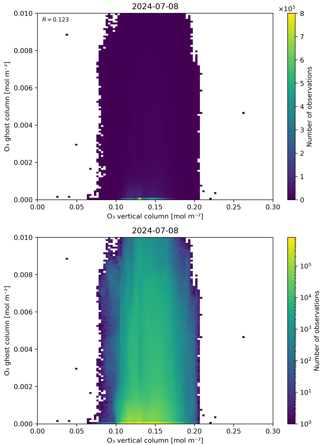
Figure 40: Scatter density plot of “O 3 vertical column” against “O 3 ghost column” for 2024-07-07 to 2024-07-09.
