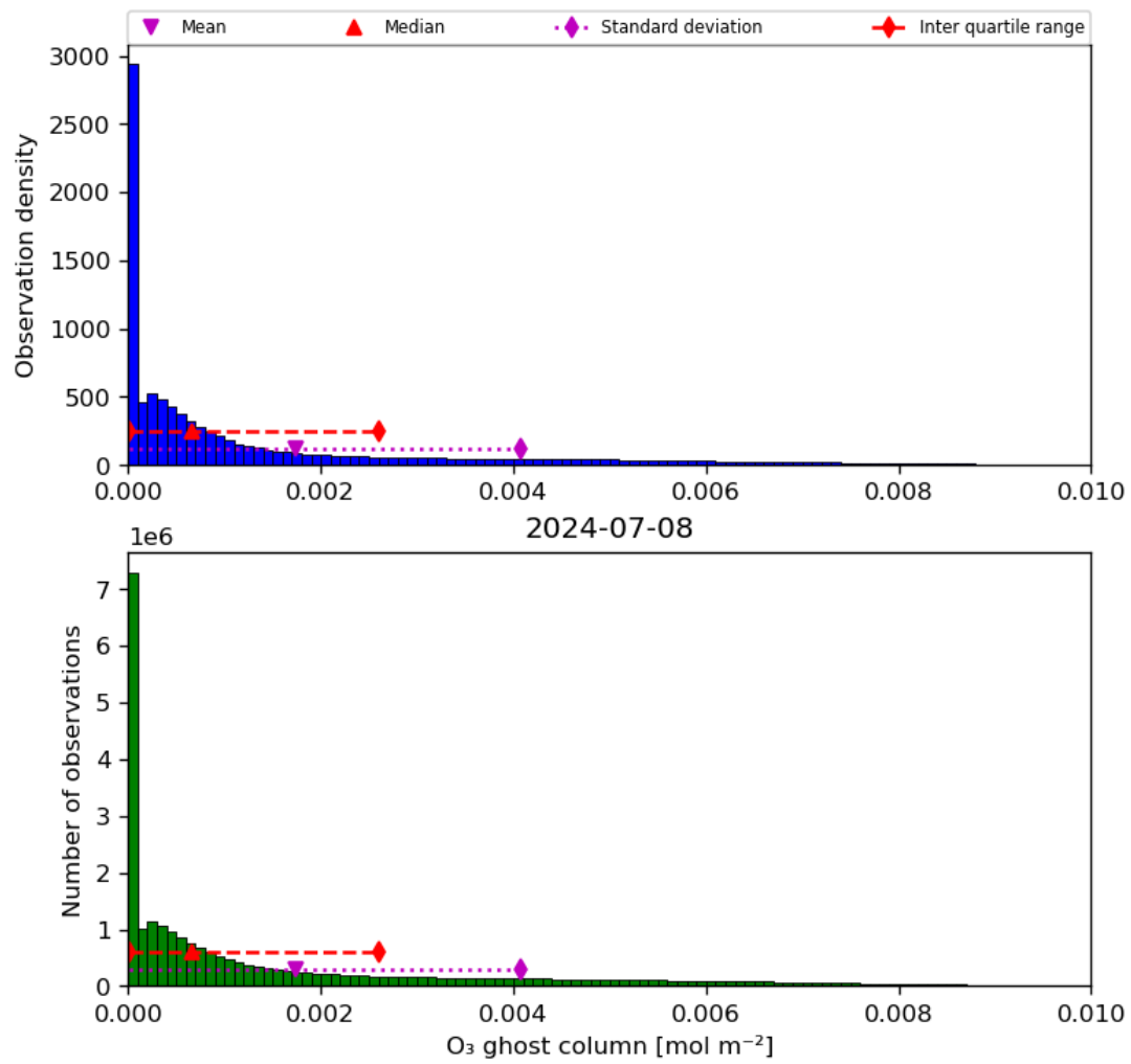
Figure 25: Histogram of “O 3 ghost column” for 2024-07-07 to 2024-07-09
