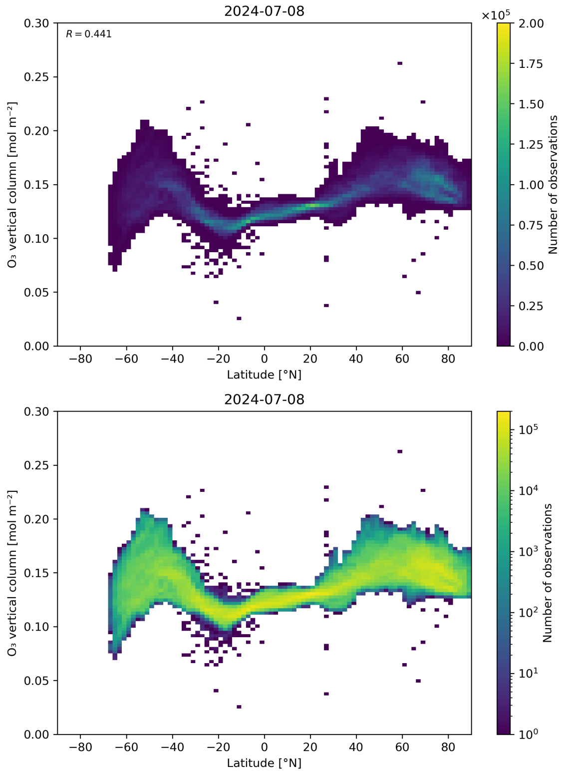
Figure 36: Scatter density plot of “Latitude” against “O 3 vertical column” for 2024-07-07 to 2024-07-09.
