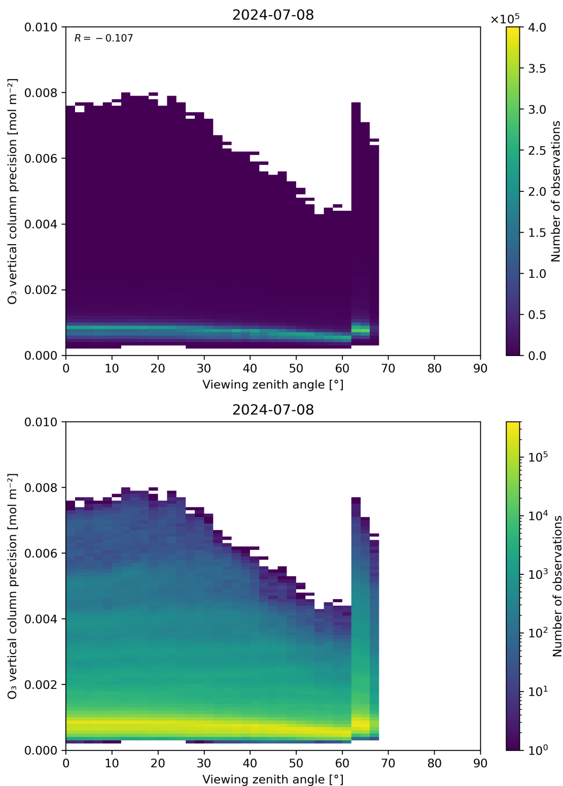
Figure 53: Scatter density plot of “Viewing zenith angle” against “O 3 vertical column precision” for 2024-07-07 to 2024-07-09.
