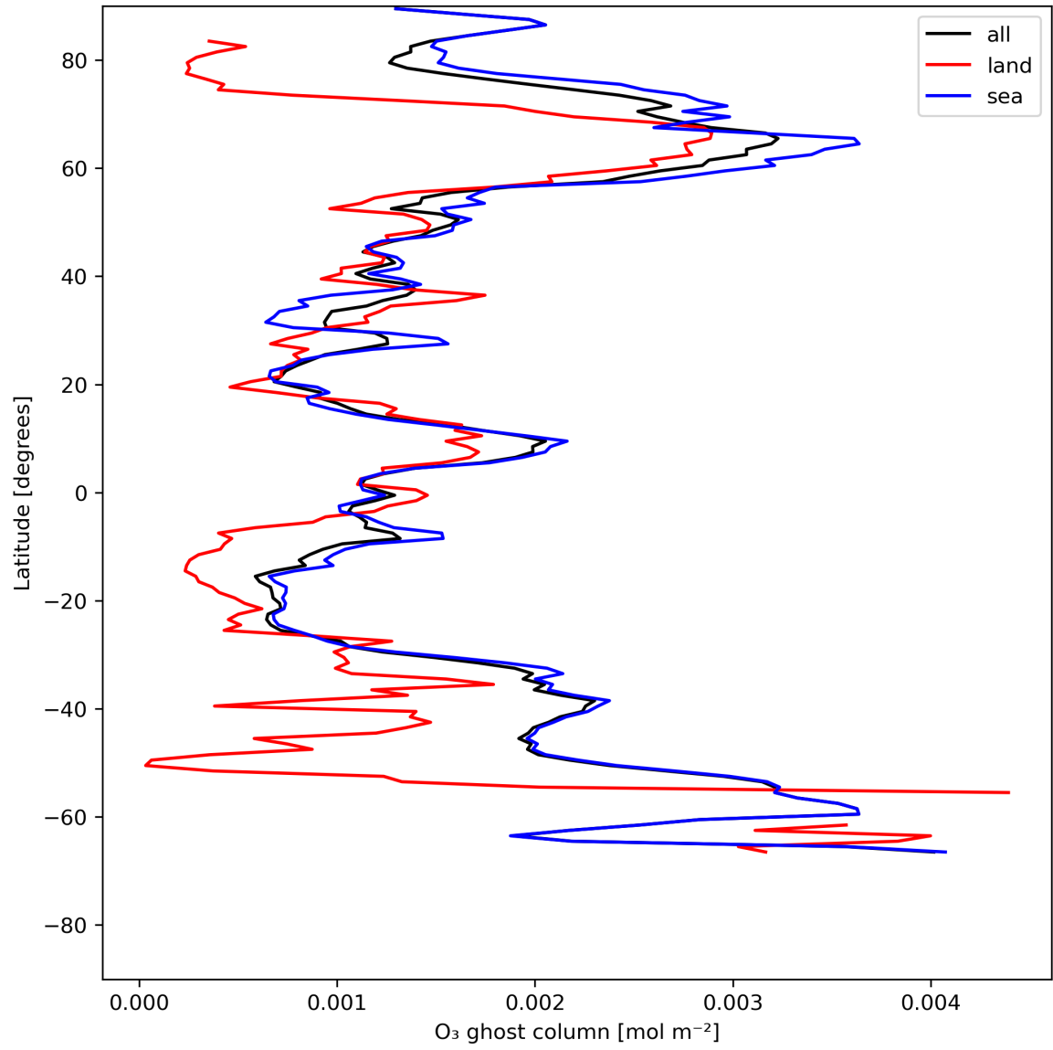
Figure 18: Zonal average of "O 3 ghost column" for 2024-07-07 to 2024-07-09.
