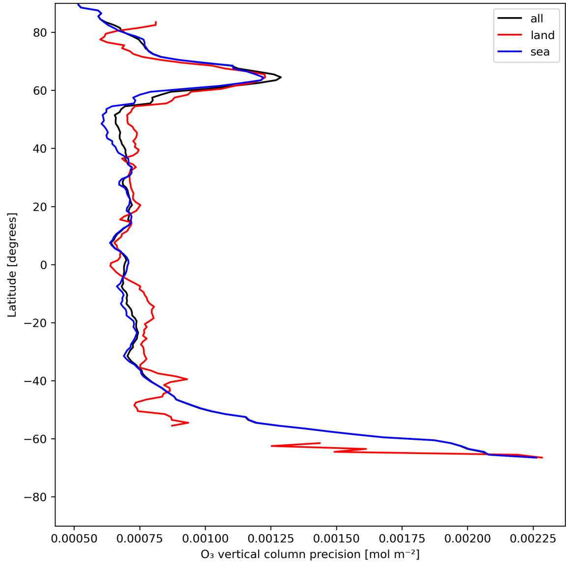
Figure 15: Zonal average of “O 3 vertical column precision” for 2024-07-07 to 2024-07-09.
