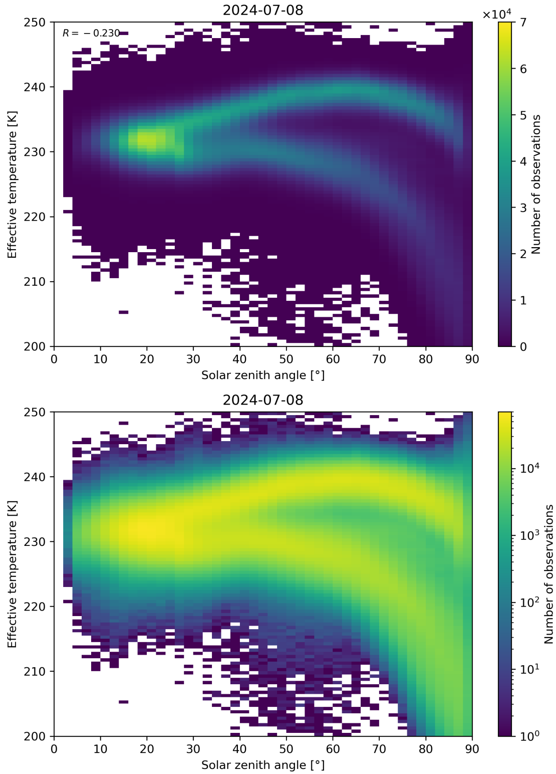
Figure 45: Scatter density plot of “Solar zenith angle” against “Effective temperature” for 2024-07-07 to 2024-07-09.
