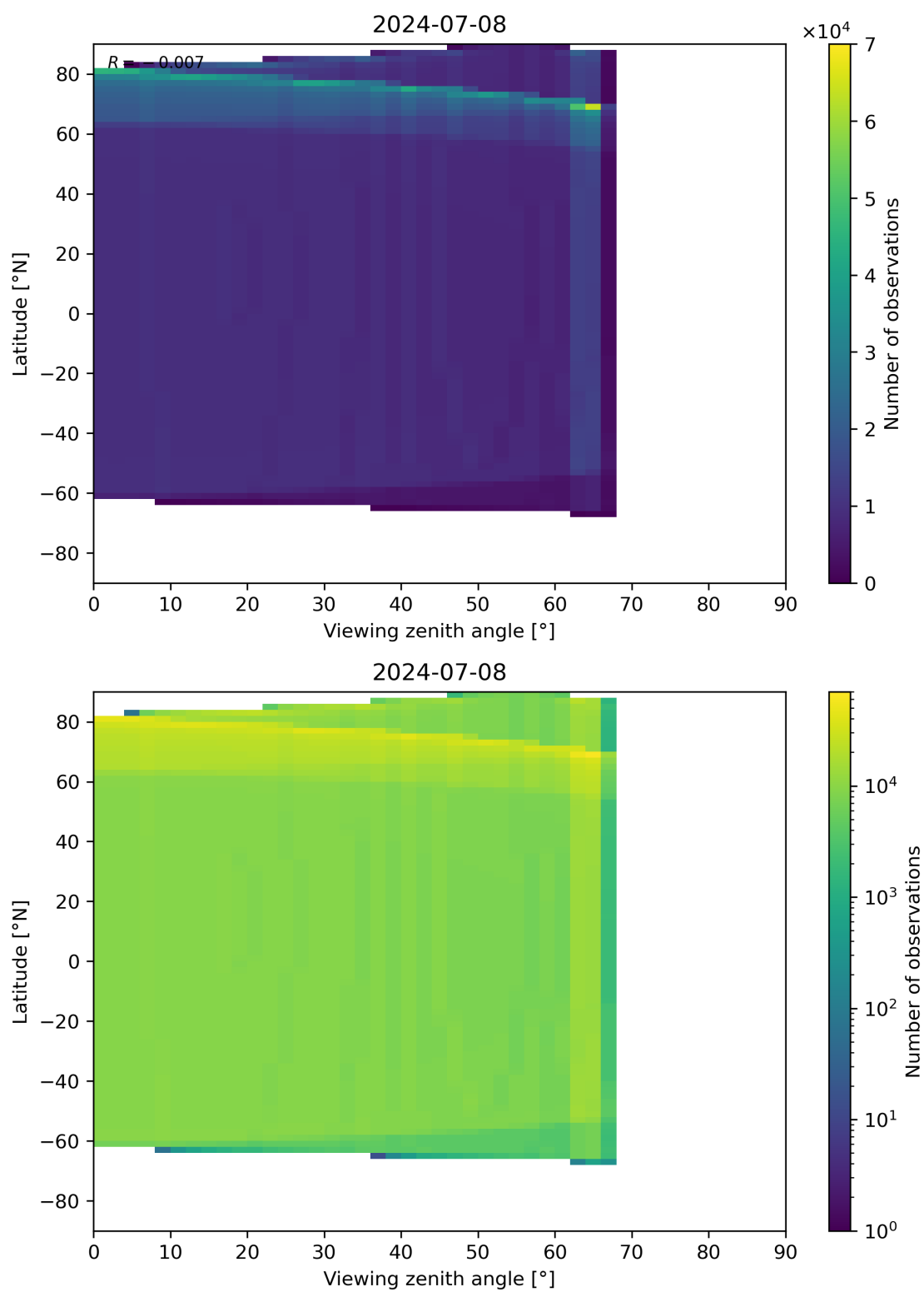
Figure 49: Scatter density plot of “Viewing zenith angle” against “Latitude” for 2024-07-07 to 2024-07-09.
