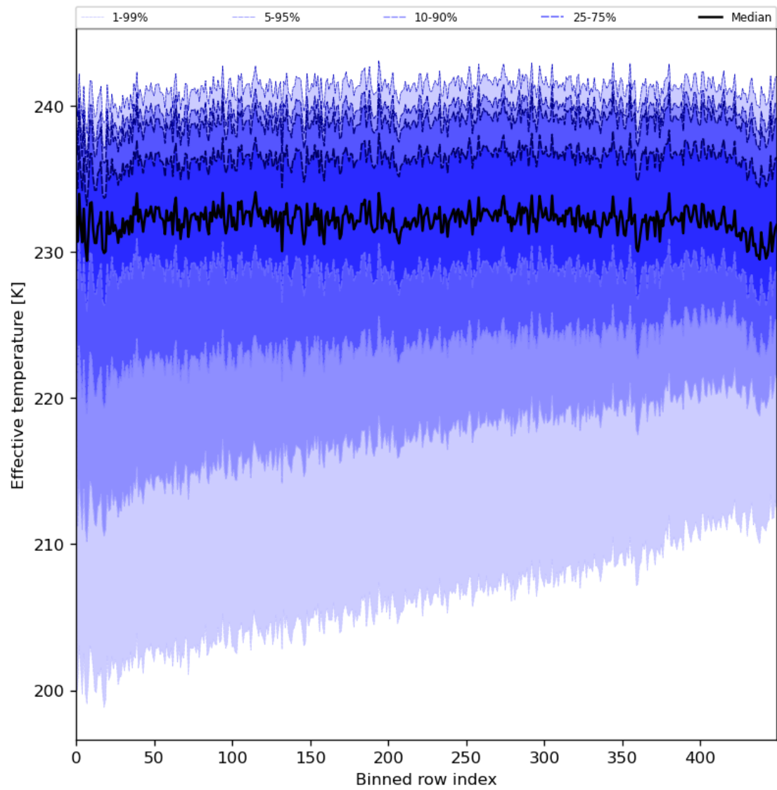
Figure 31: Along track statistics of “Effective temperature” for 2024-07-07 to 2024-07-09
