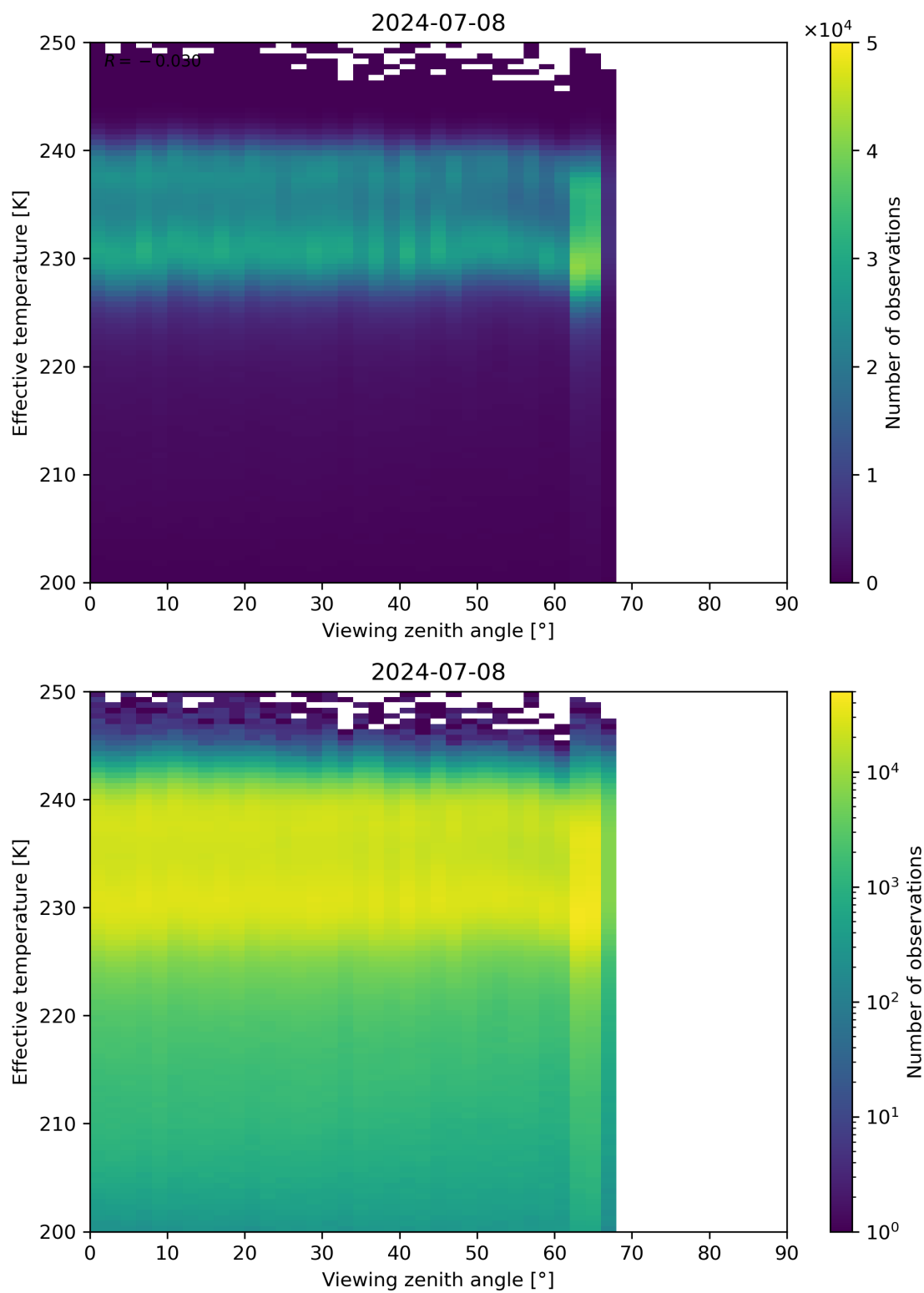
Figure 50: Scatter density plot of “Viewing zenith angle” against “Effective temperature” for 2024-07-07 to 2024-07-09.
