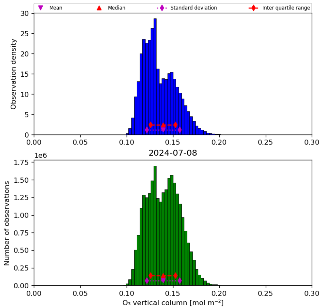
Figure 21: Histogram of “O 3 vertical column” for 2024-07-07 to 2024-07-09
