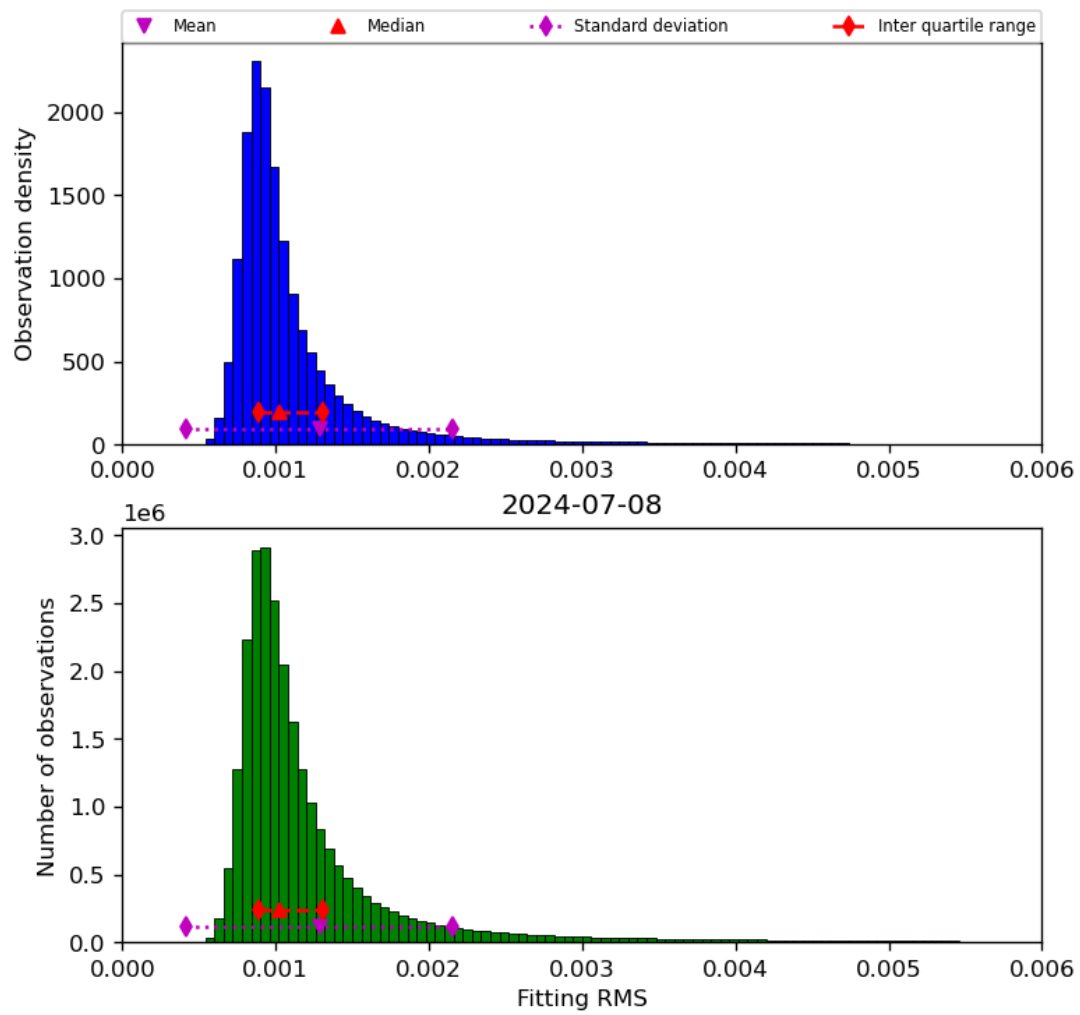
Figure 23: Histogram of “Fitting RMS” for 2024-07-07 to 2024-07-09
