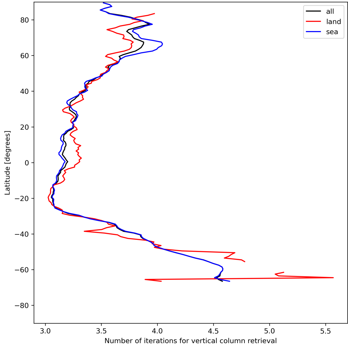
Figure 19: Zonal average of “Number of iterations for vertical column retrieval” for 2024-07-07 to 2024-07-09.
