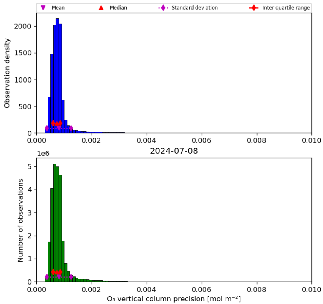
Figure 22: Histogram of “O 3 vertical column precision” for 2024-07-07 to 2024-07-09
