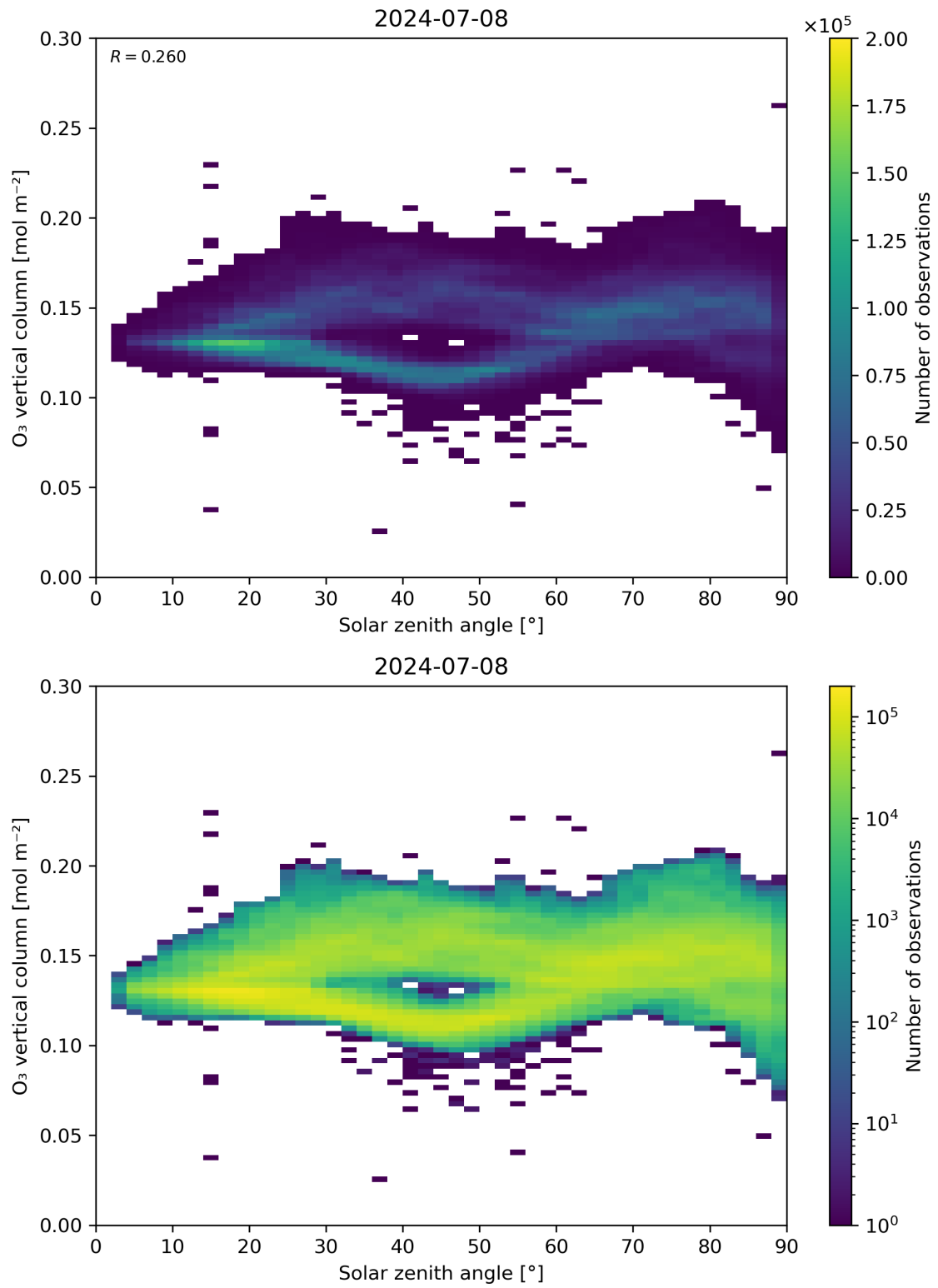
Figure 47: Scatter density plot of “Solar zenith angle” against “O 3 vertical column” for 2024-07-07 to 2024-07-09.
