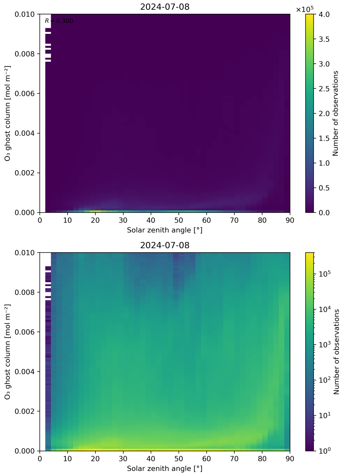
Figure 46: Scatter density plot of “Solar zenith angle” against “O 3 ghost column” for 2024-07-07 to 2024-07-09.
