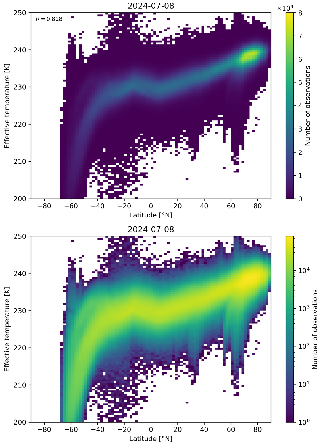
Figure 34: Scatter density plot of “Latitude” against “Effective temperature” for 2024-07-07 to 2024-07-09.
