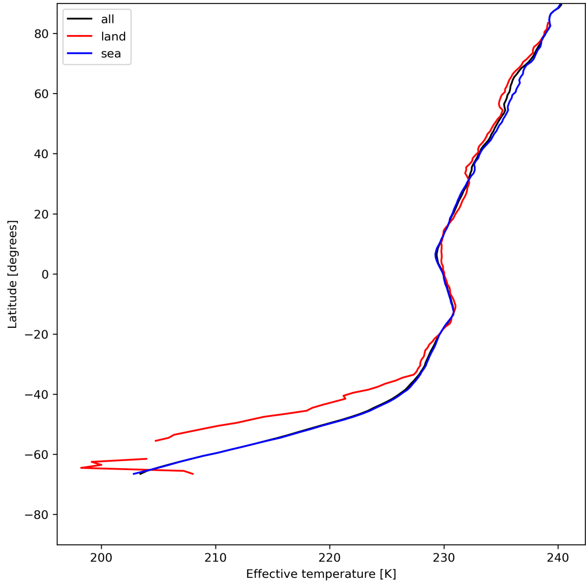
Figure 17: Zonal average of "Effective temperature" for 2024-07-07 to 2024-07-09.
