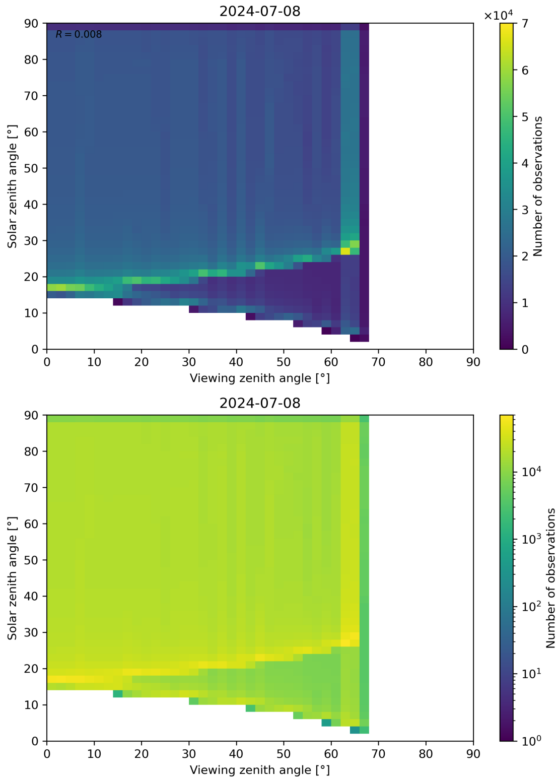
Figure 54: Scatter density plot of “Viewing zenith angle” against “Solar zenith angle” for 2024-07-07 to 2024-07-09.
