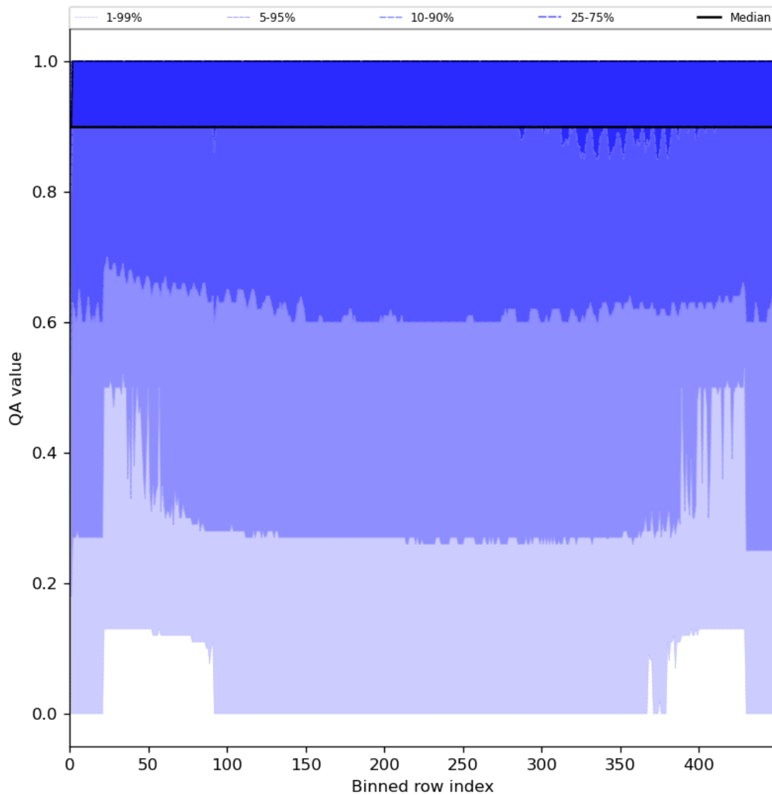
Figure 27: Along track statistics of “QA value” for 2024-07-07 to 2024-07-09
