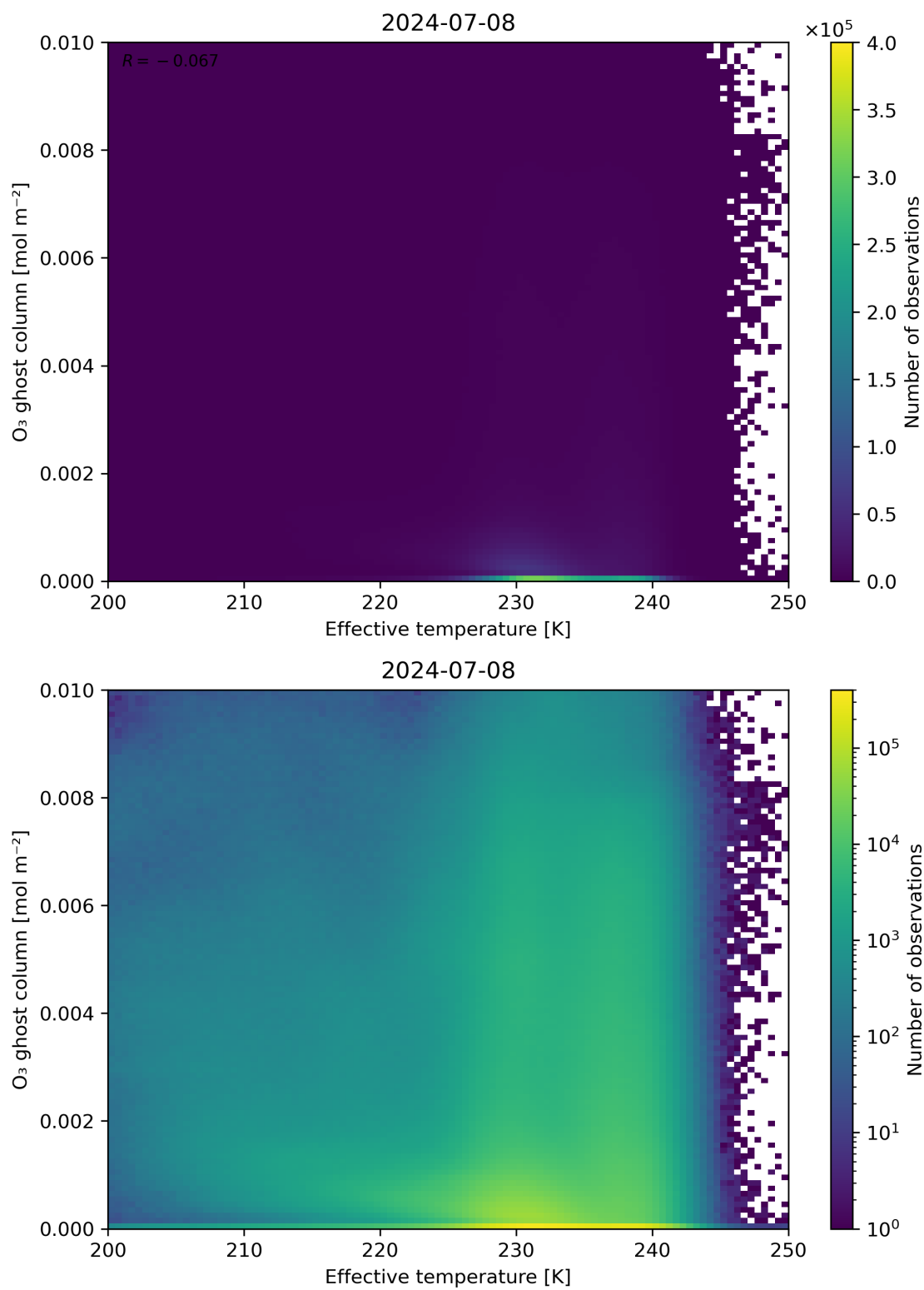
Figure 38: Scatter density plot of “Effective temperature” against “O 3 ghost column” for 2024-07-07 to 2024-07-09.
