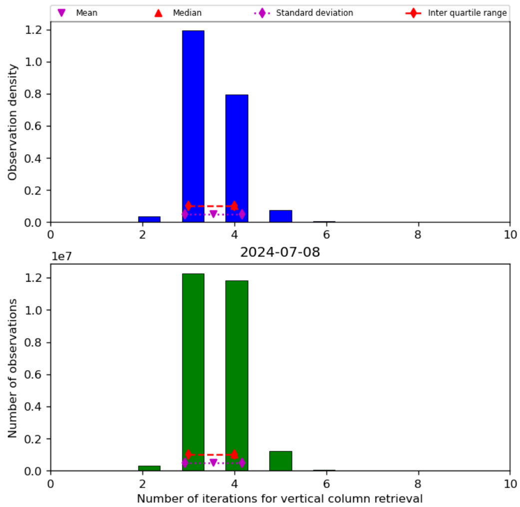
Figure 26: Histogram of “Number of iterations for vertical column retrieval” for 2024-07-07 to 2024-07-09
