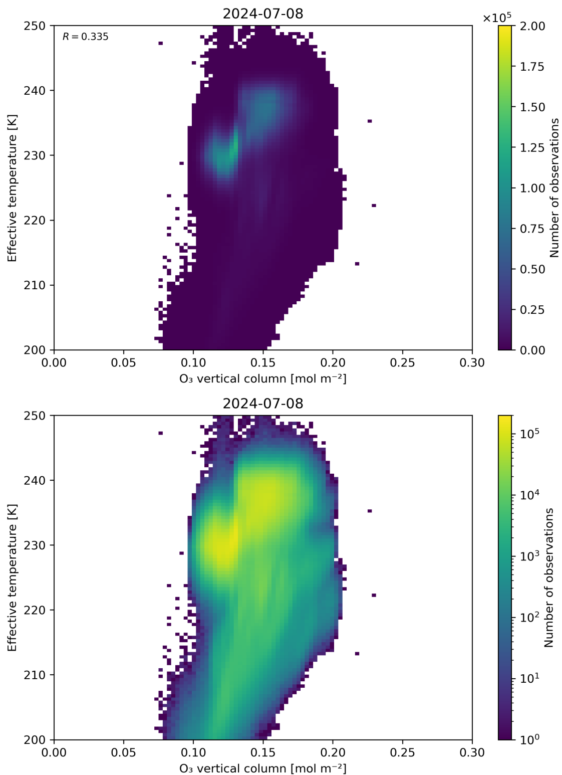
Figure 39: Scatter density plot of “O 3 vertical column” against “Effective temperature” for 2024-07-07 to 2024-07-09.
