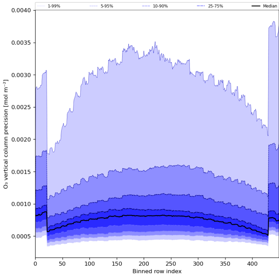
Figure 29: Along track statistics of “O 3 vertical column precision” for 2024-07-07 to 2024-07-09
