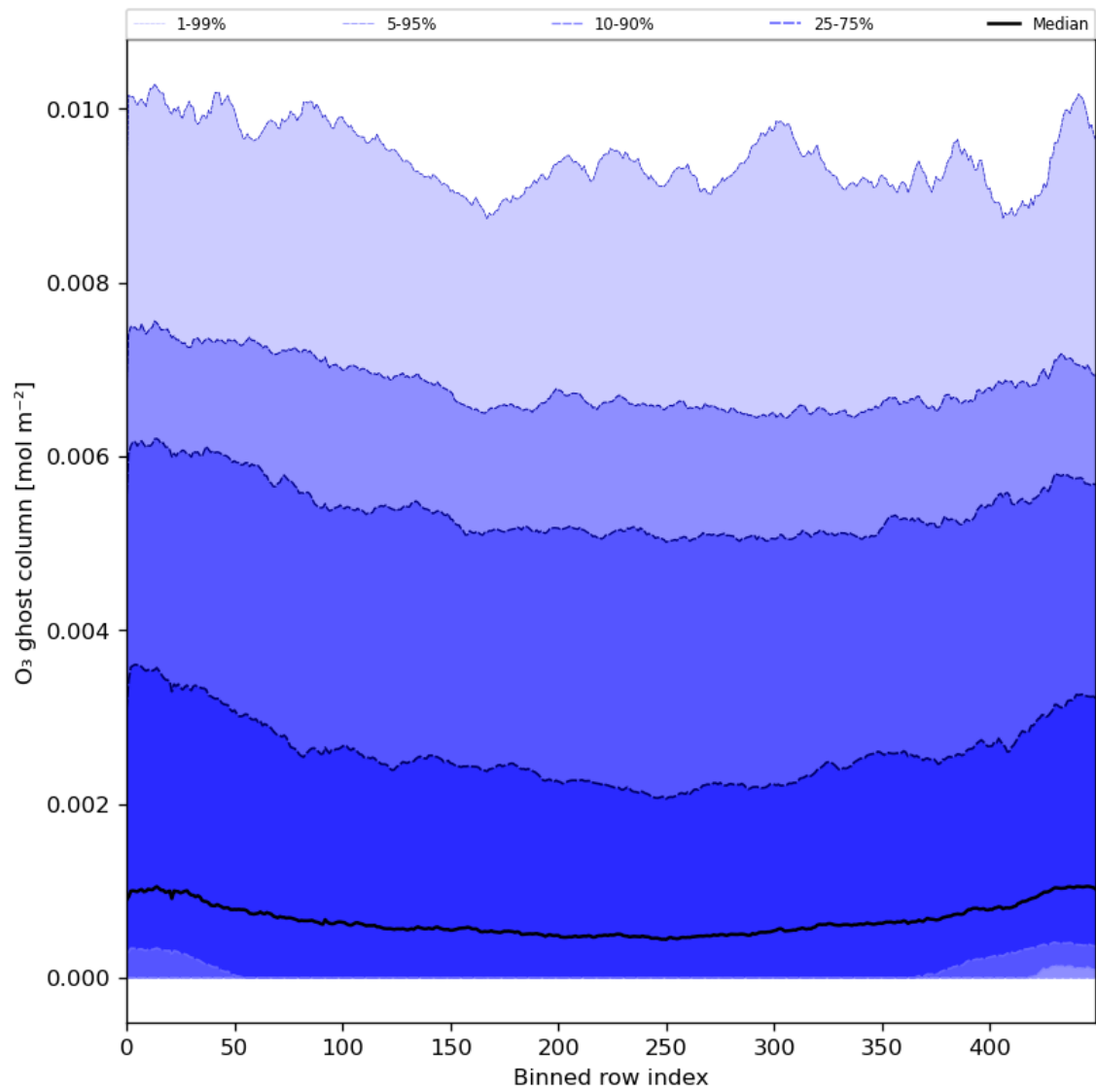
Figure 32: Along track statistics of “O 3 ghost column” for 2024-07-07 to 2024-07-09
