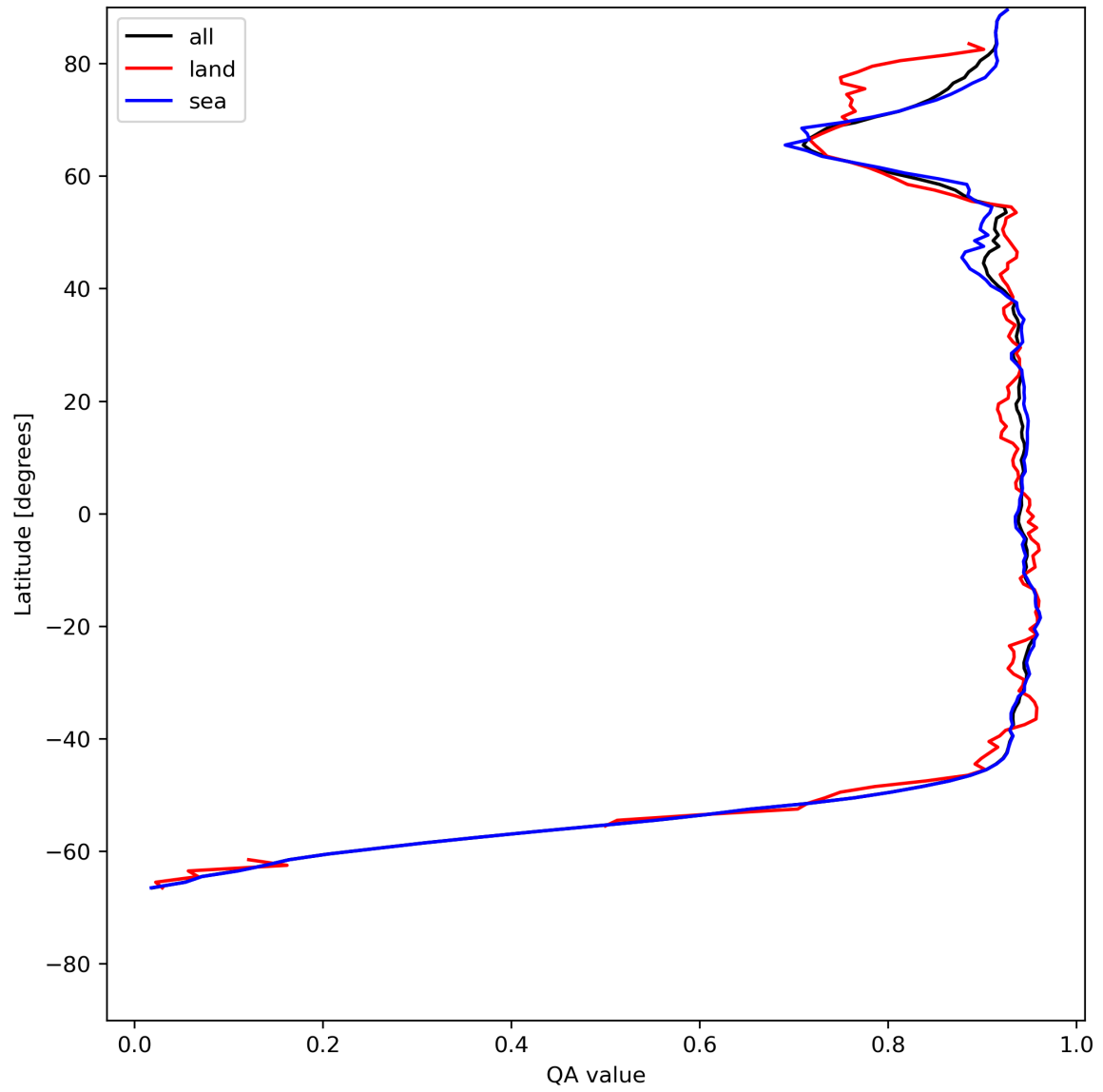
Figure 13: Zonal average of “QA value” for 2024-07-07 to 2024-07-09.
