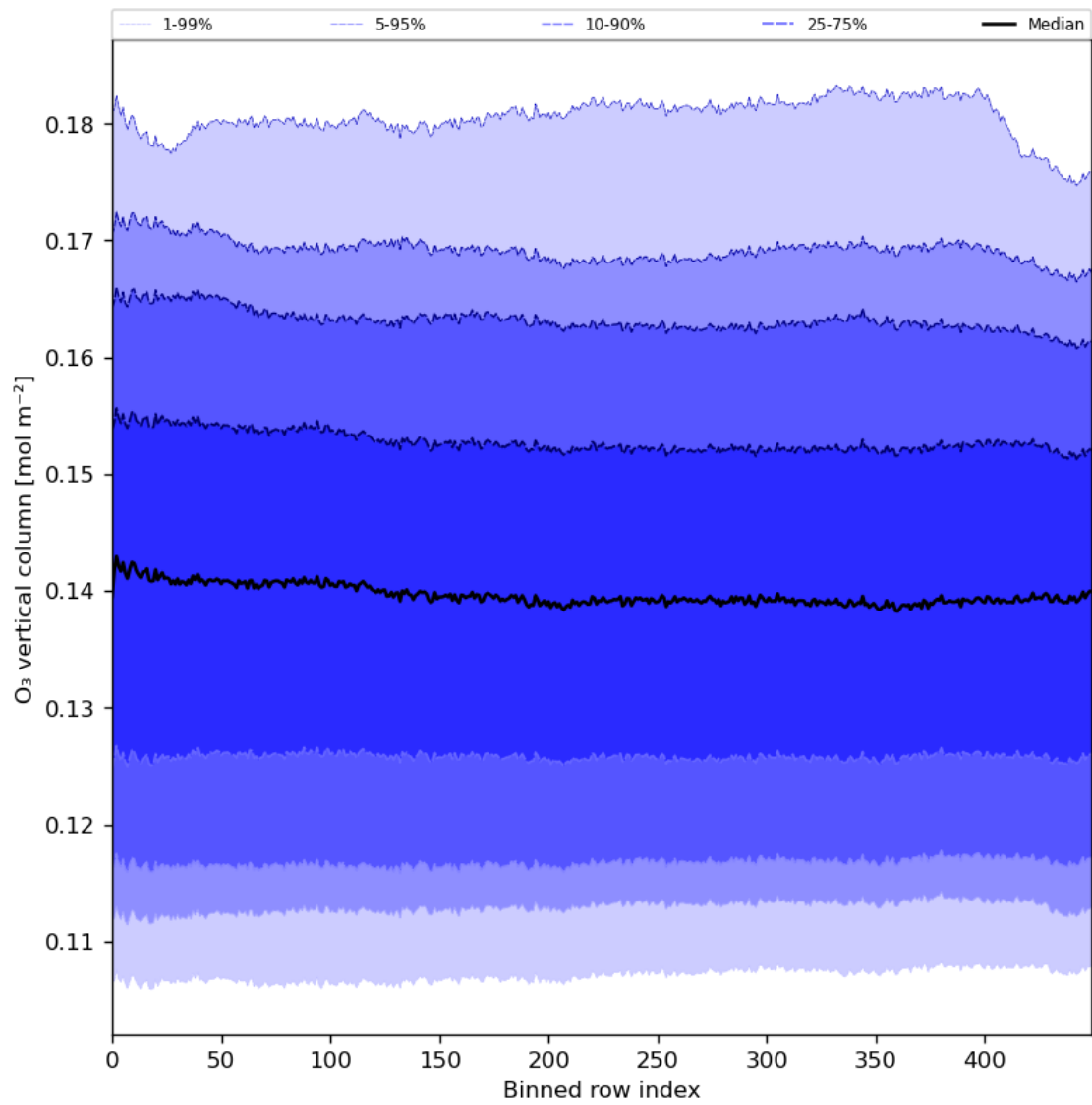
Figure 28: Along track statistics of “O 3 vertical column” for 2024-07-07 to 2024-07-09
