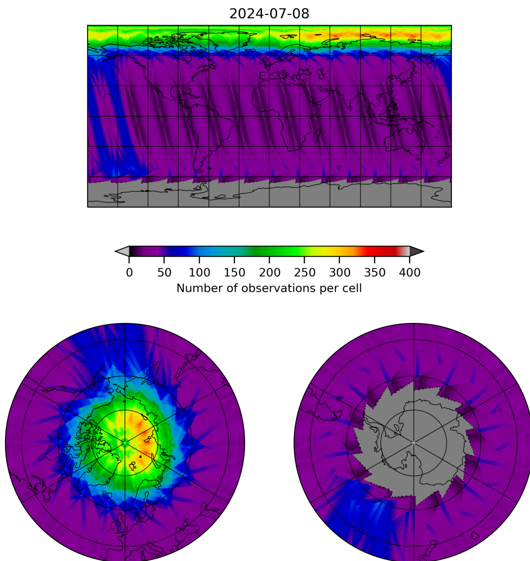
Figure 12: Map of the number of observations for 2024-07-07 to 2024-07-09
