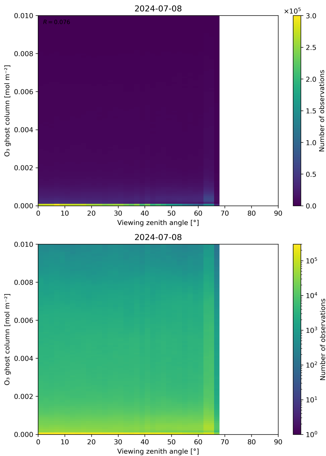
Figure 51: Scatter density plot of “Viewing zenith angle” against “O 3 ghost column” for 2024-07-07 to 2024-07-09.
