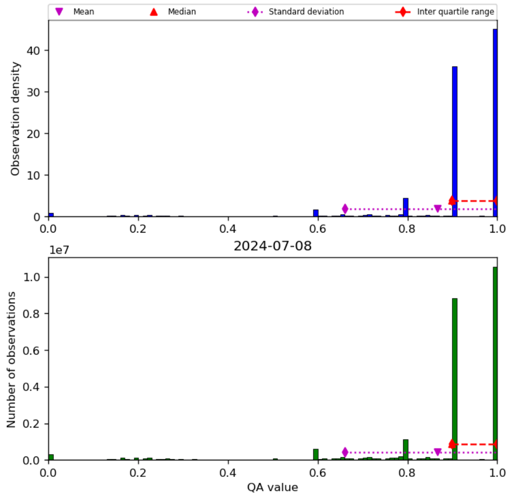
Figure 20: Histogram of “QA value” for 2024-07-07 to 2024-07-09
