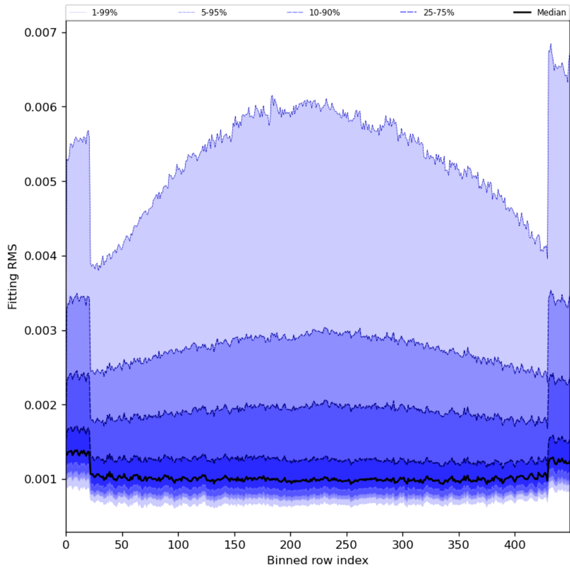
Figure 30: Along track statistics of “Fitting RMS” for 2024-07-07 to 2024-07-09
