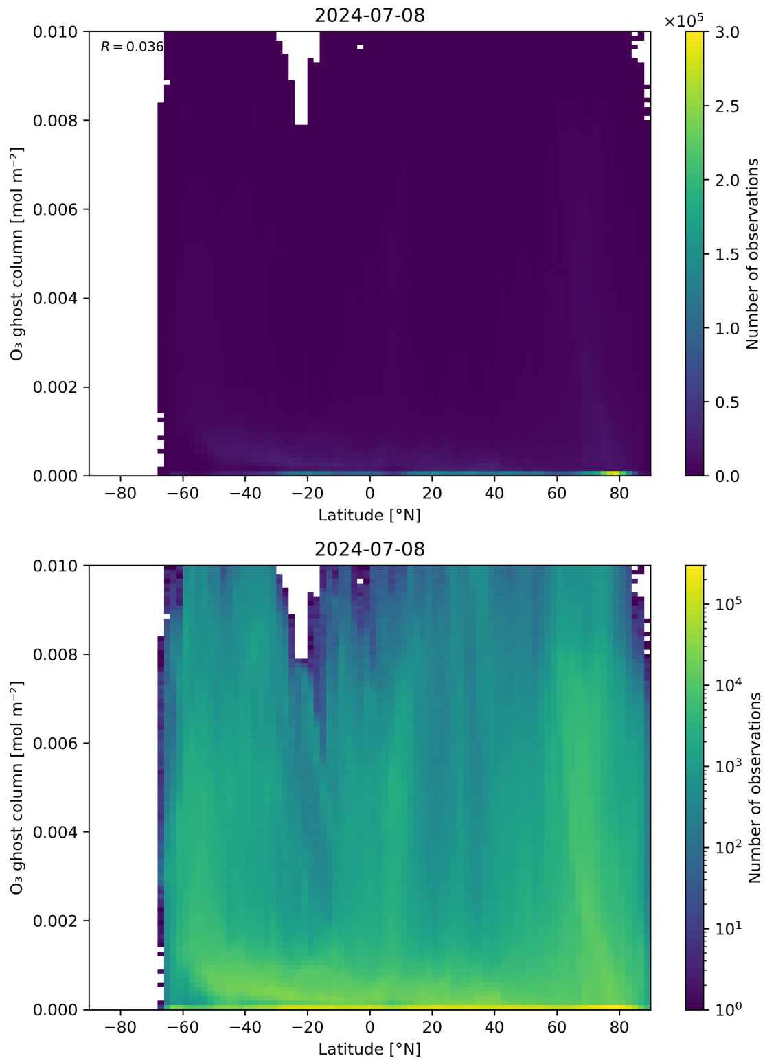
Figure 35: Scatter density plot of “Latitude” against “O 3 ghost column” for 2024-07-07 to 2024-07-09.
