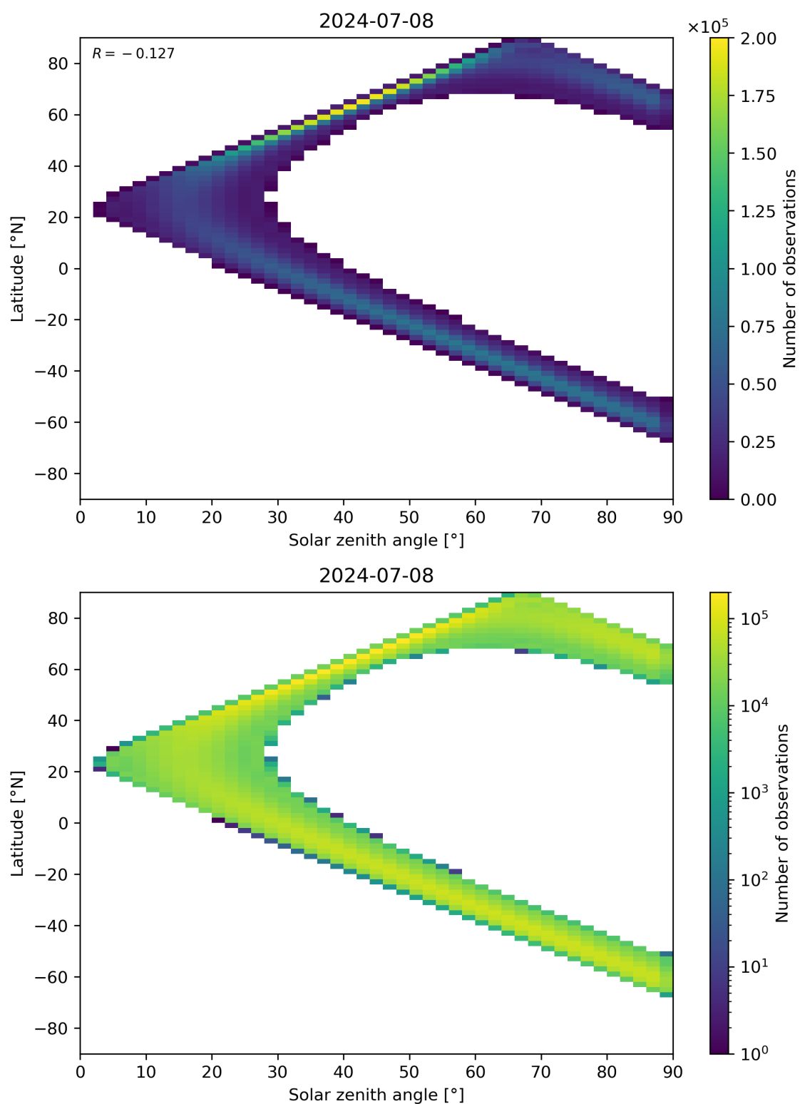
Figure 44: Scatter density plot of “Solar zenith angle” against “Latitude” for 2024-07-07 to 2024-07-09.
