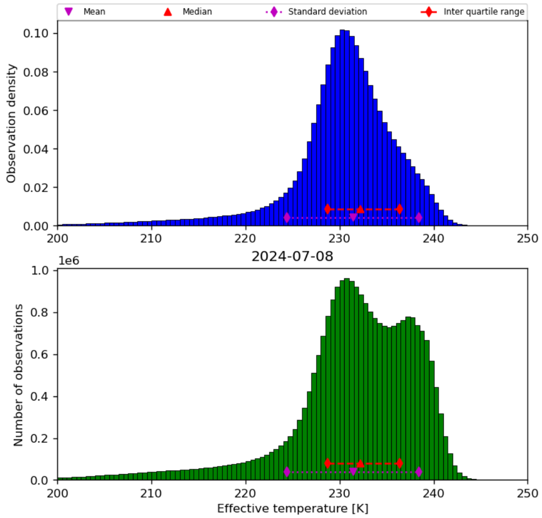
Figure 24: Histogram of “Effective temperature” for 2024-07-07 to 2024-07-09
