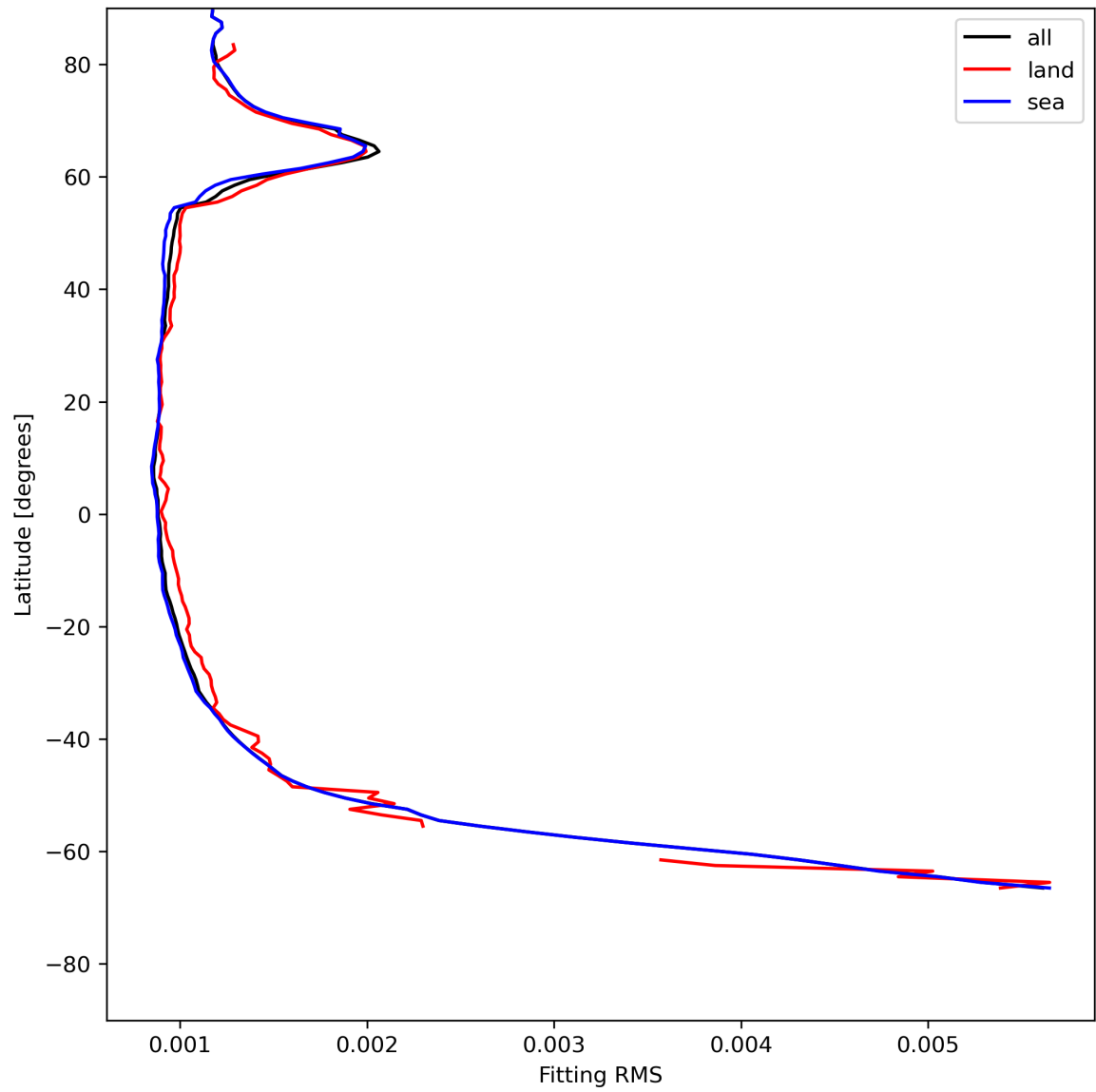
Figure 16: Zonal average of “Fitting RMS” for 2024-07-07 to 2024-07-09.
