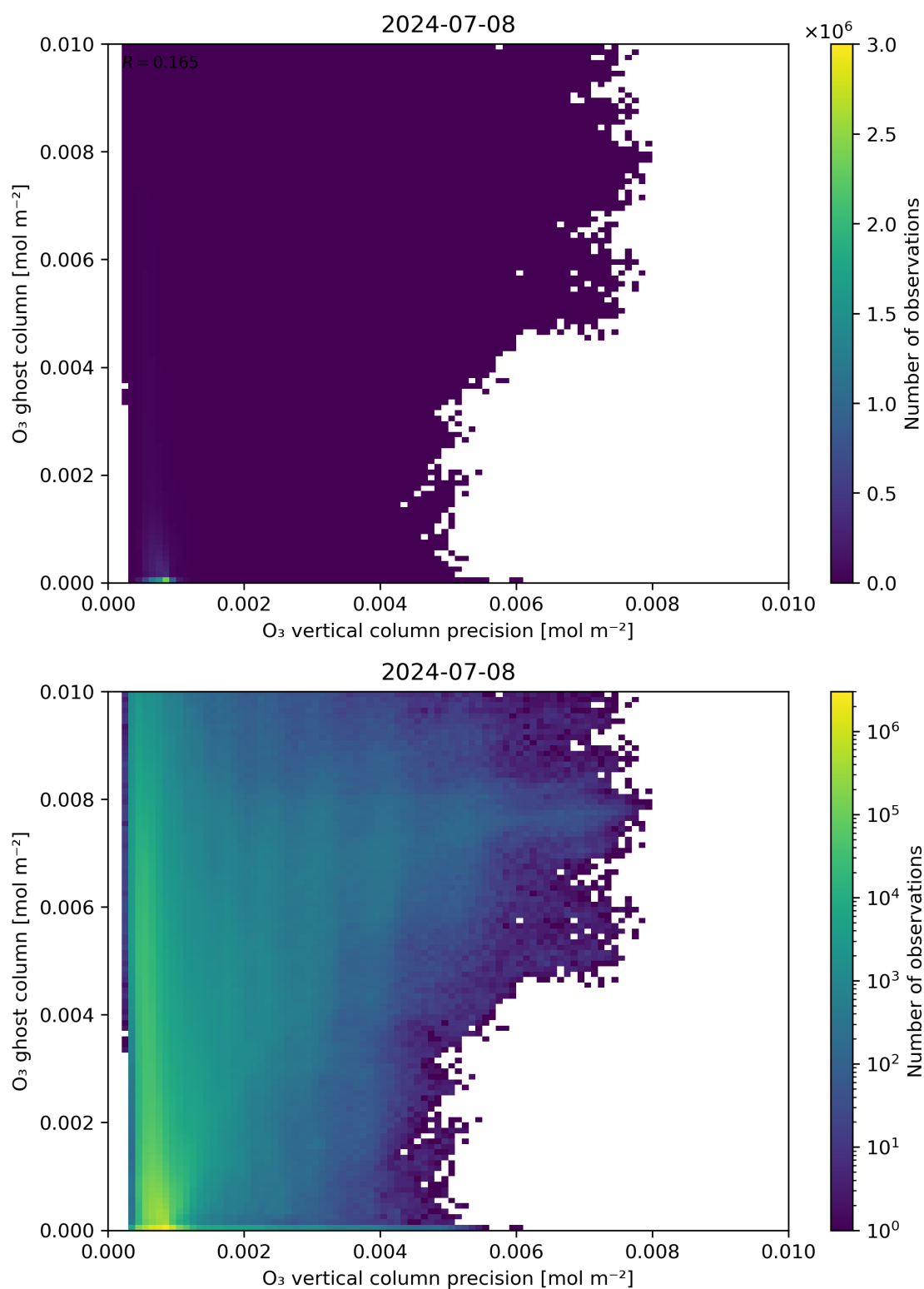
Figure 43: Scatter density plot of “ \text{O}_3 vertical column precision” against “ \text{O}_3 ghost column” for 2024-07-07 to 2024-07-09.
