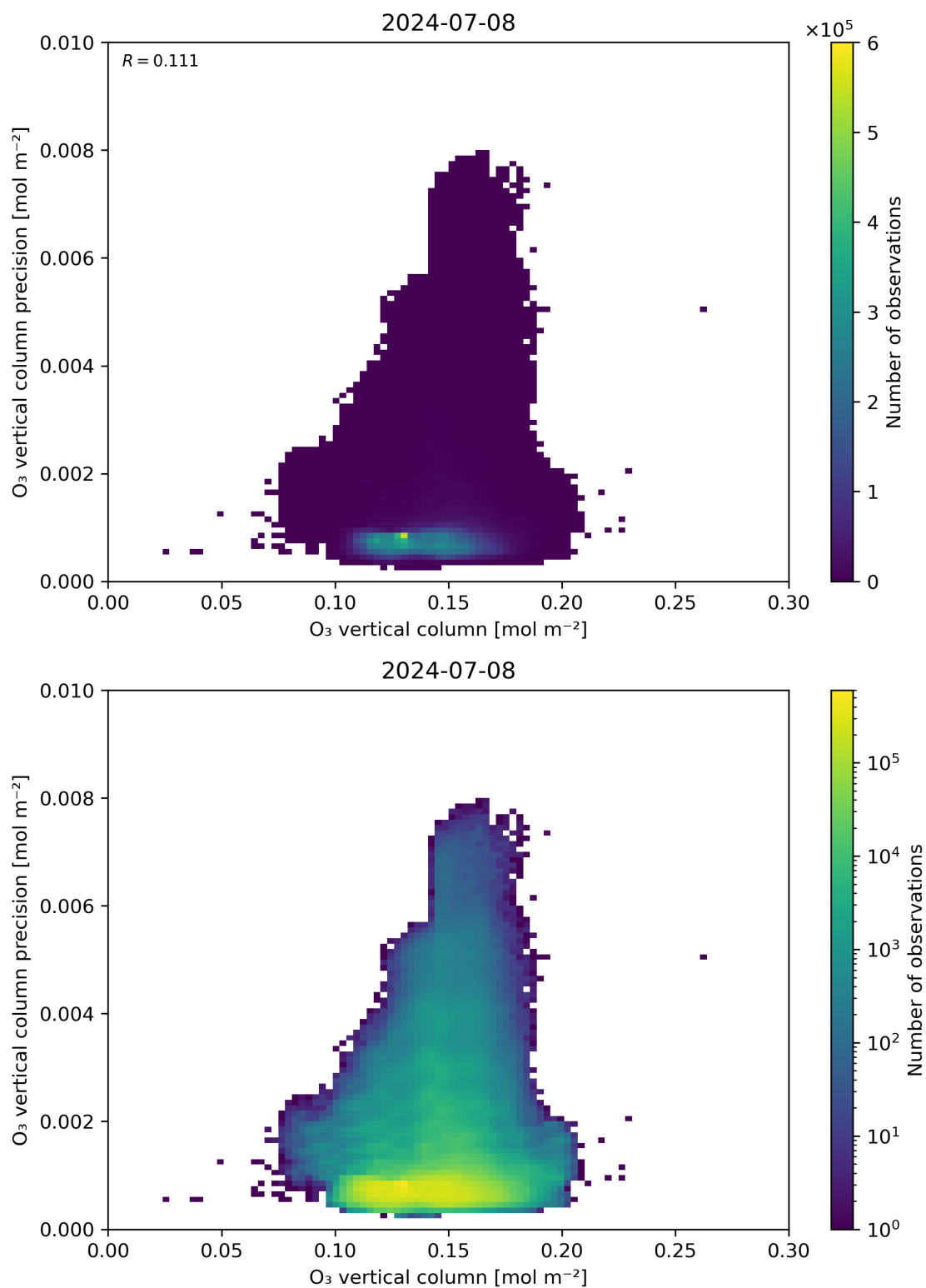
Figure 41: Scatter density plot of “O 3 vertical column” against “O 3 vertical column precision” for 2024-07-07 to 2024-07-09.
