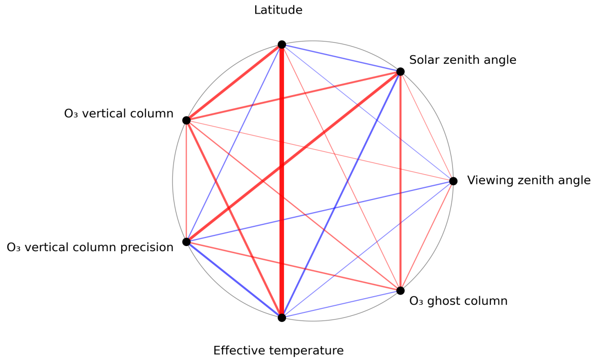
Figure 1: Map of correlation graph for 2024-07-07 to 2024-07-09.
