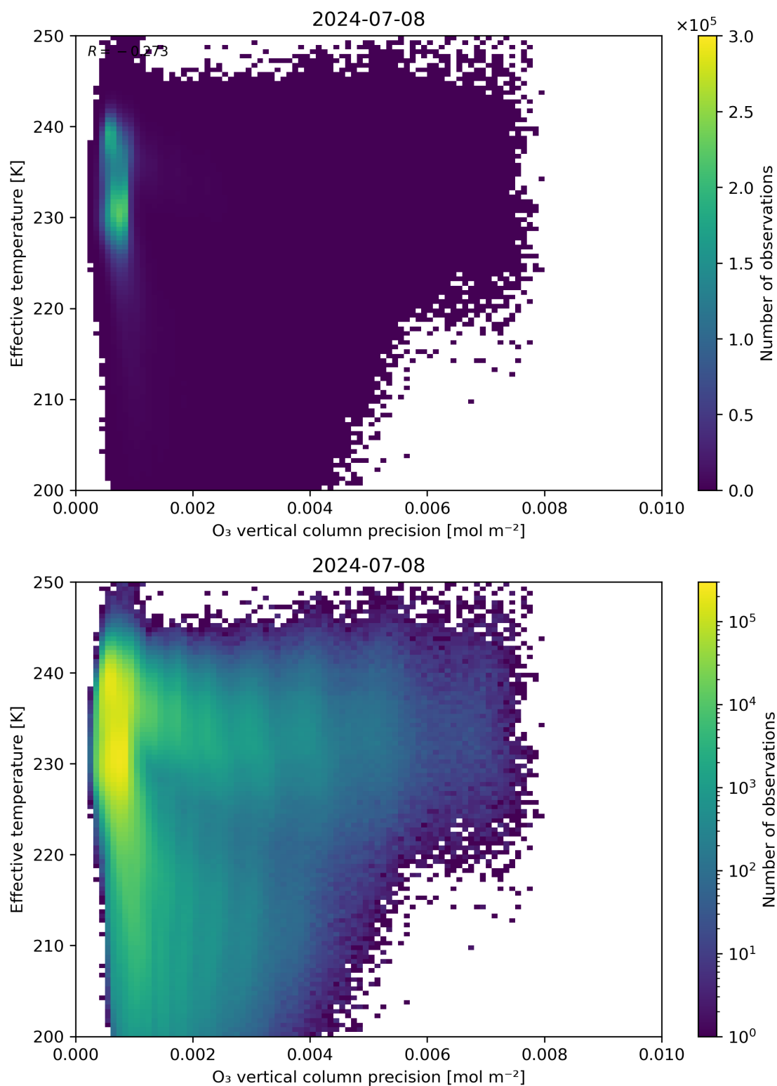
Figure 42: Scatter density plot of “O 3 vertical column precision” against “Effective temperature” for 2024-07-07 to 2024-07-09.
