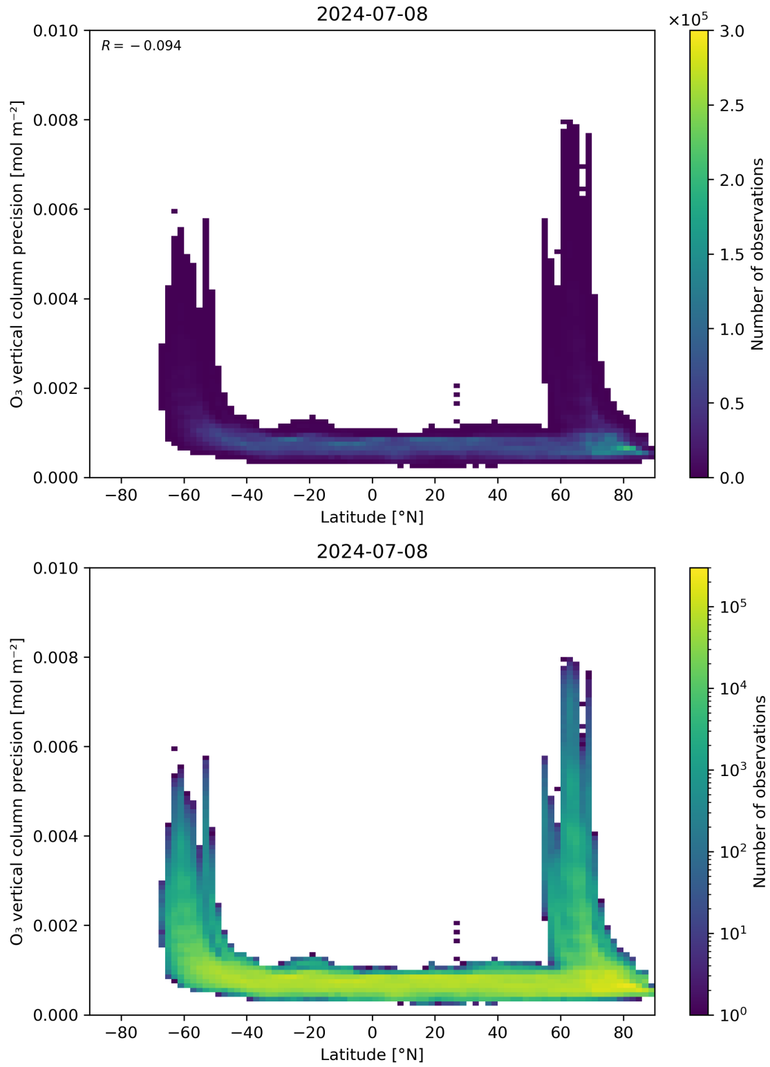
Figure 37: Scatter density plot of “Latitude” against “O 3 vertical column precision” for 2024-07-07 to 2024-07-09.
