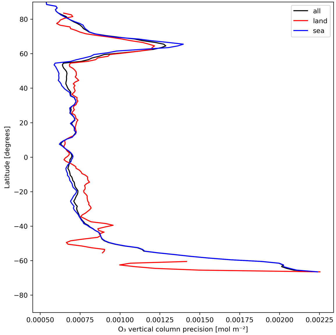
Figure 15: Zonal average of "O 3 vertical column precision" for 2024-07-08 to 2024-07-10.
