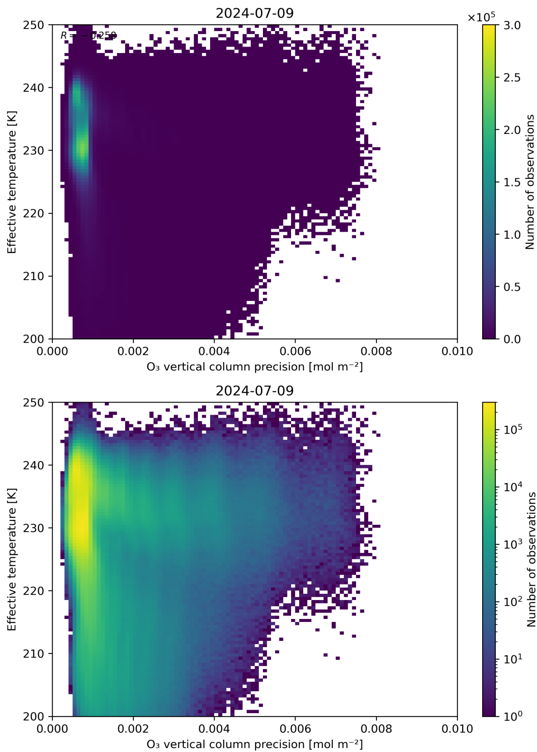
Figure 42: Scatter density plot of “O 3 vertical column precision” against “Effective temperature” for 2024-07-08 to 2024-07-10.
