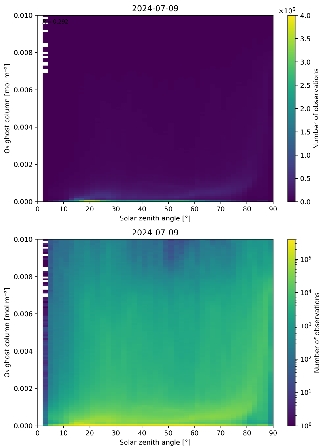
Figure 46: Scatter density plot of “Solar zenith angle” against “O 3 ghost column” for 2024-07-08 to 2024-07-10.
