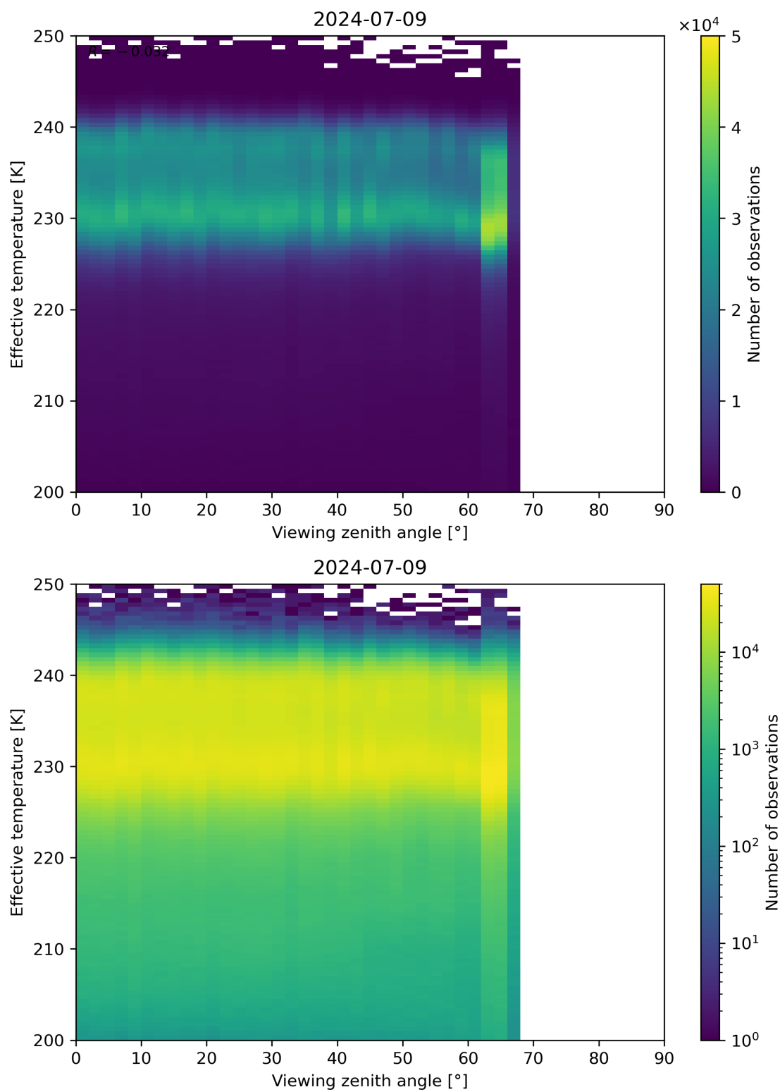
Figure 50: Scatter density plot of “Viewing zenith angle” against “Effective temperature” for 2024-07-08 to 2024-07-10.
