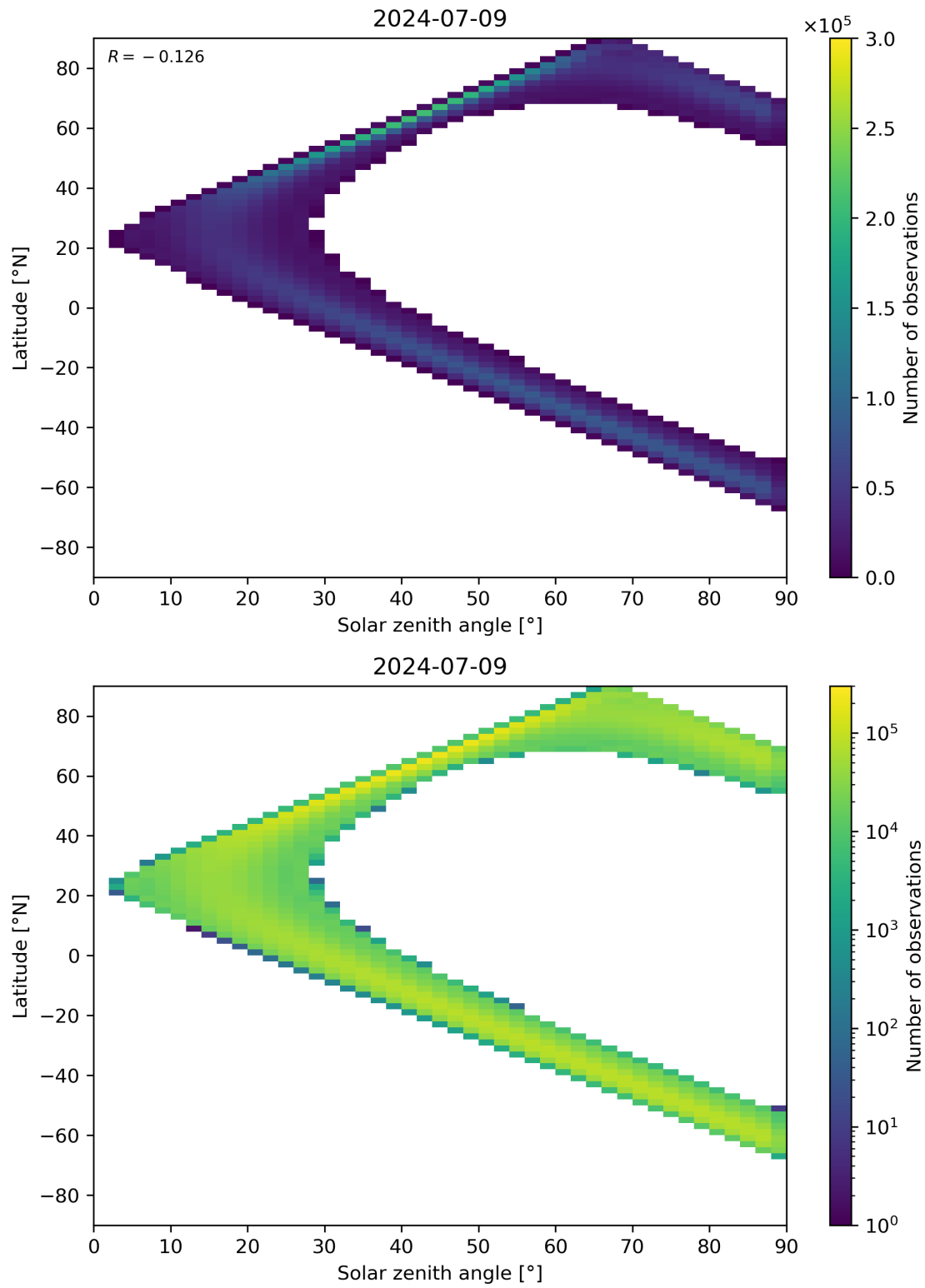
Figure 44: Scatter density plot of “Solar zenith angle” against “Latitude” for 2024-07-08 to 2024-07-10.
