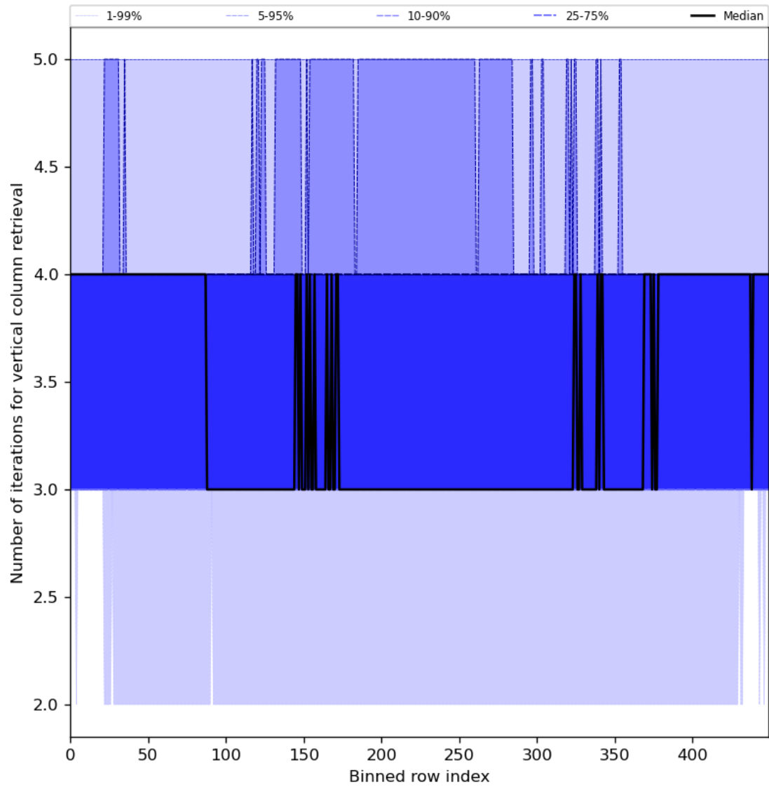
Figure 33: Along track statistics of “Number of iterations for vertical column retrieval” for 2024-07-08 to 2024-07-10
