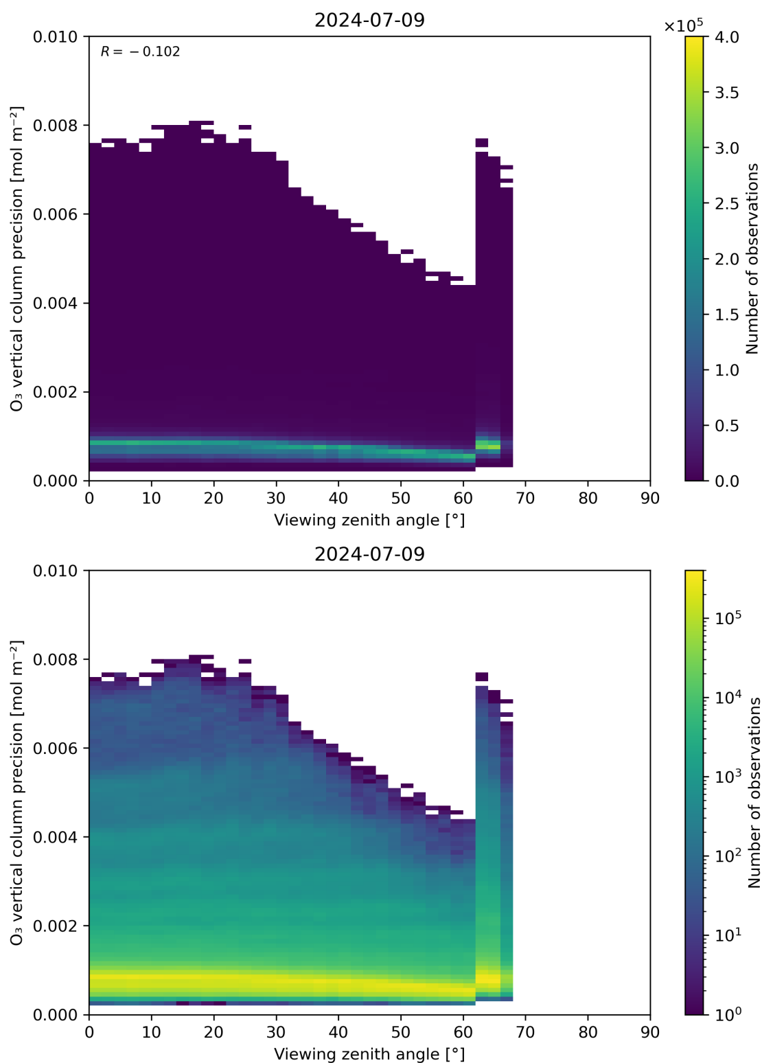
Figure 53: Scatter density plot of “Viewing zenith angle” against “O 3 vertical column precision” for 2024-07-08 to 2024-07-10.
