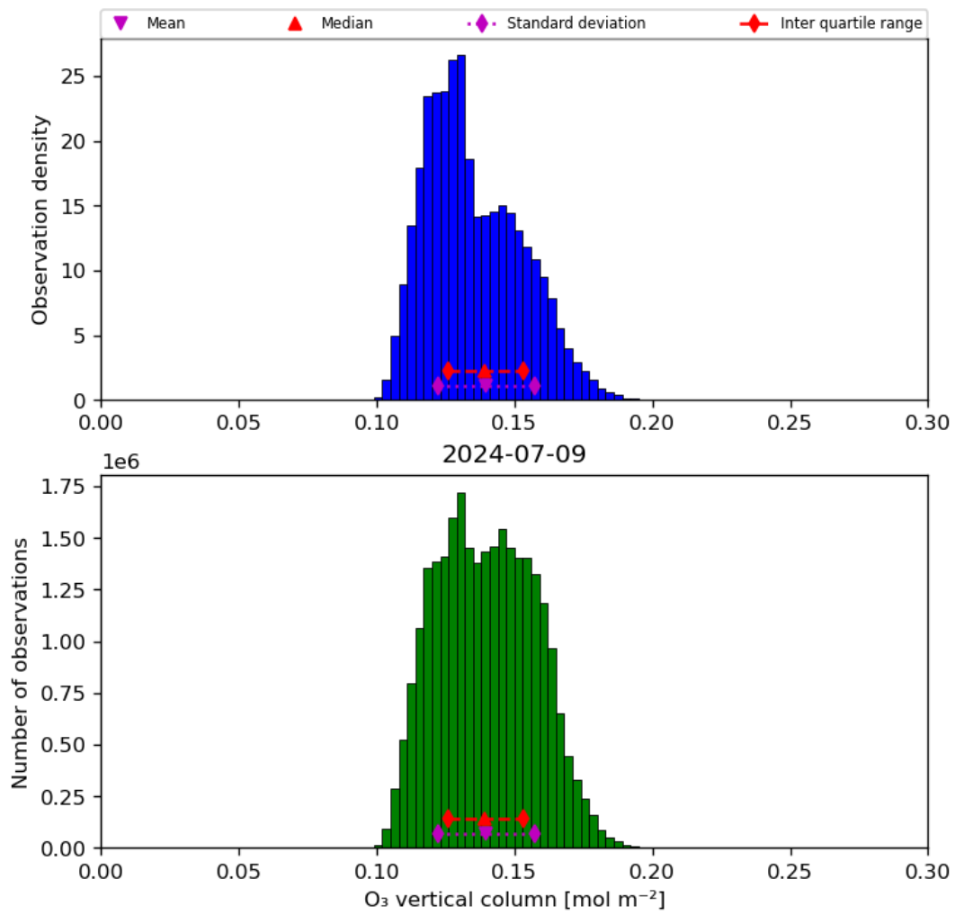
Figure 21: Histogram of “O 3 vertical column” for 2024-07-08 to 2024-07-10
