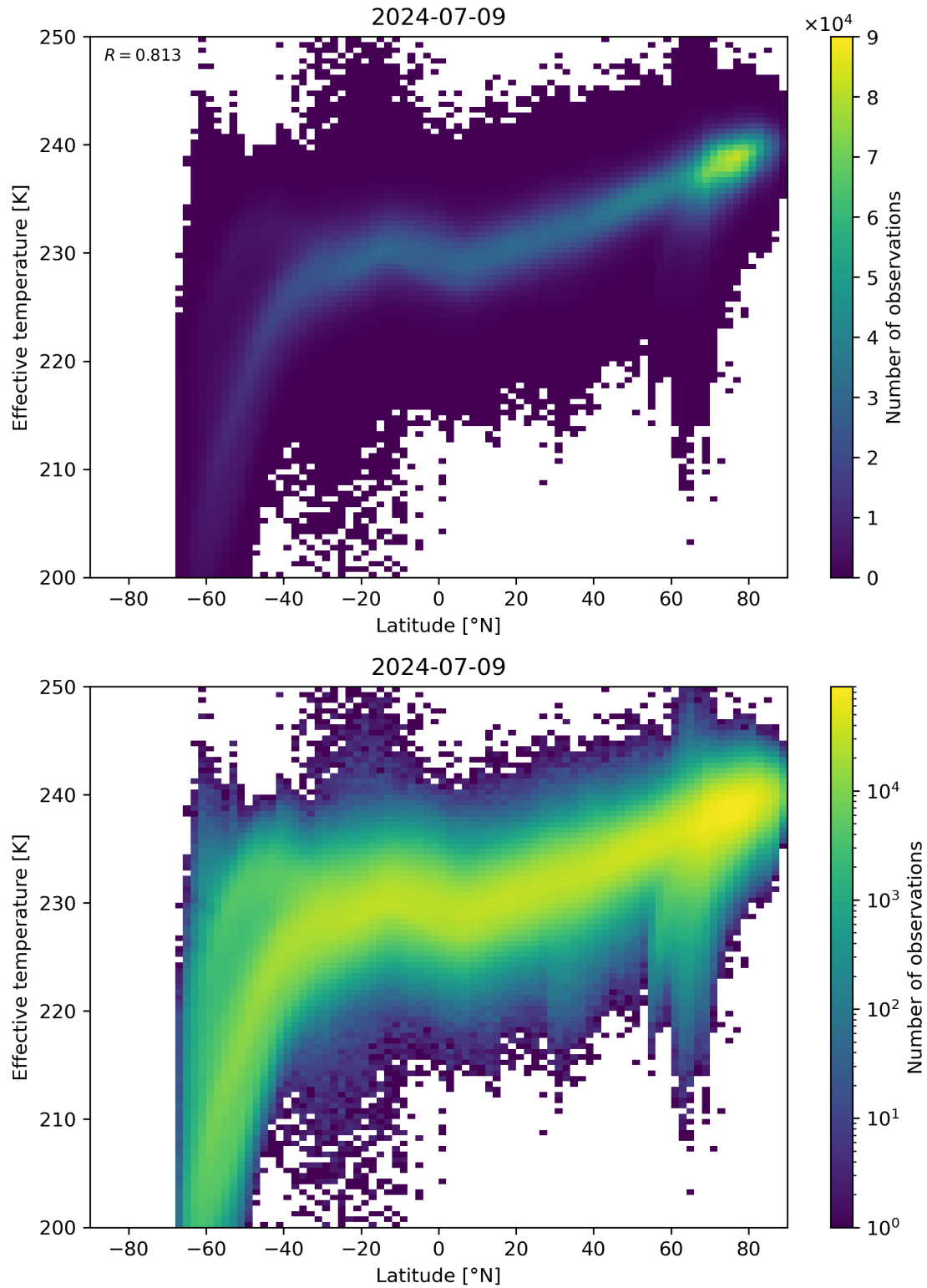
Figure 34: Scatter density plot of “Latitude” against “Effective temperature” for 2024-07-08 to 2024-07-10.
