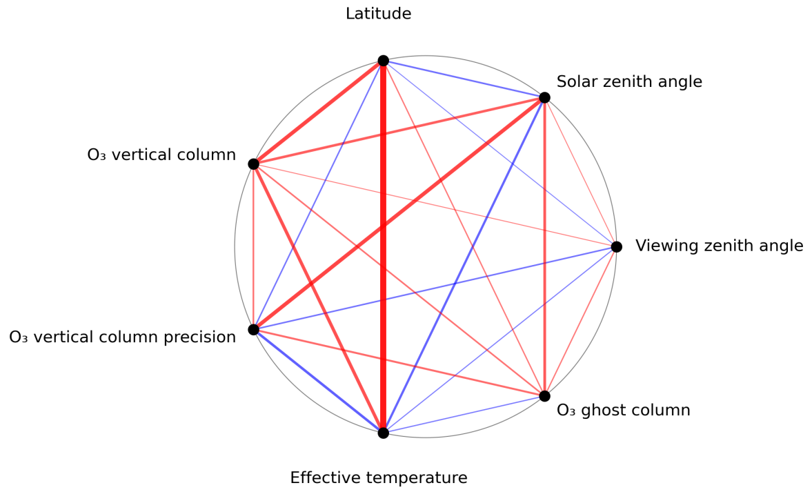
Figure 1: Map of correlation graph for 2024-07-08 to 2024-07-10.
