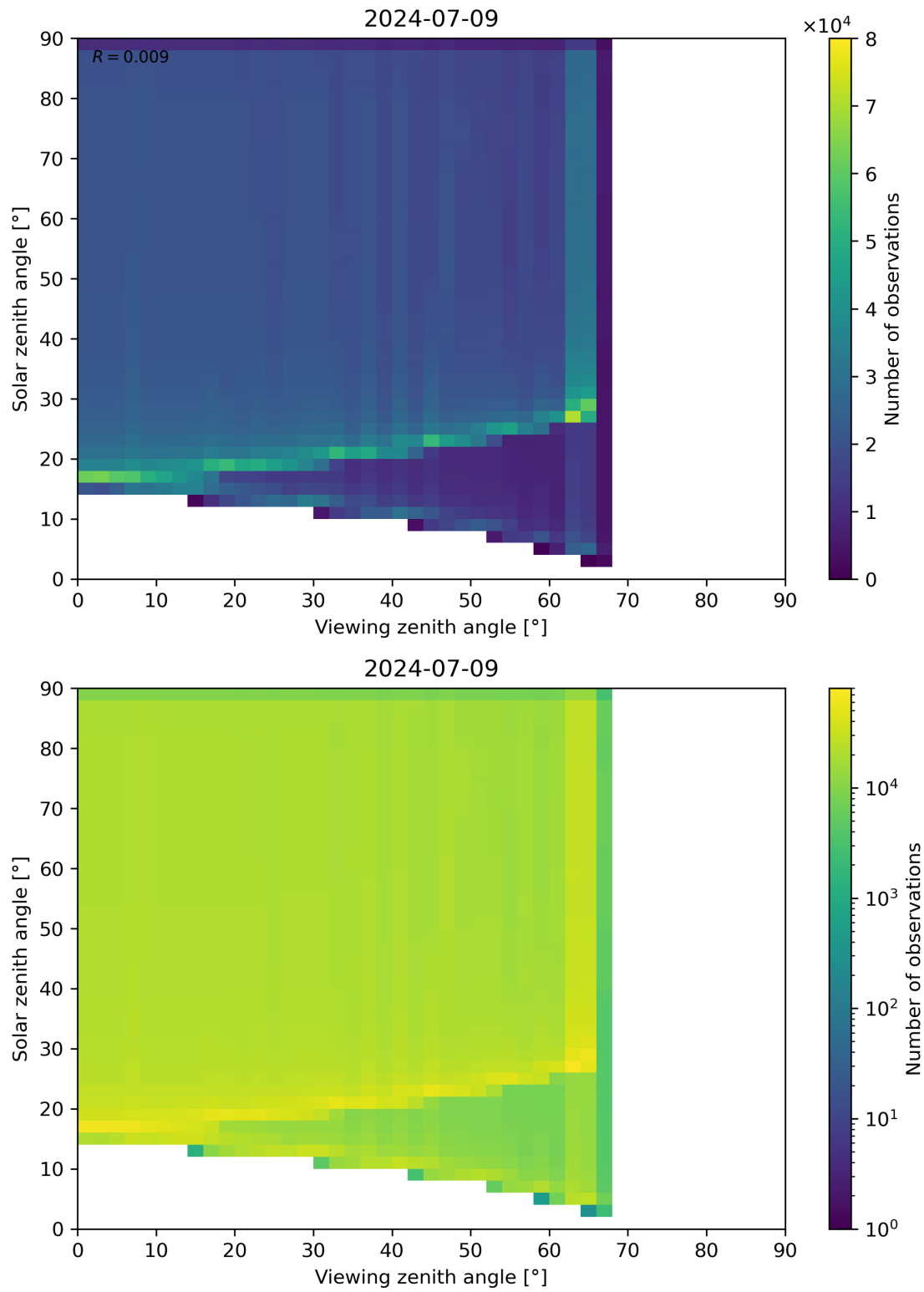
Figure 54: Scatter density plot of “Viewing zenith angle” against “Solar zenith angle” for 2024-07-08 to 2024-07-10.
