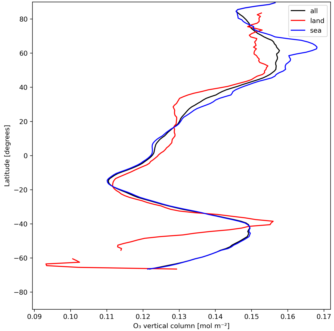
Figure 14: Zonal average of “O 3 vertical column” for 2024-07-08 to 2024-07-10.
