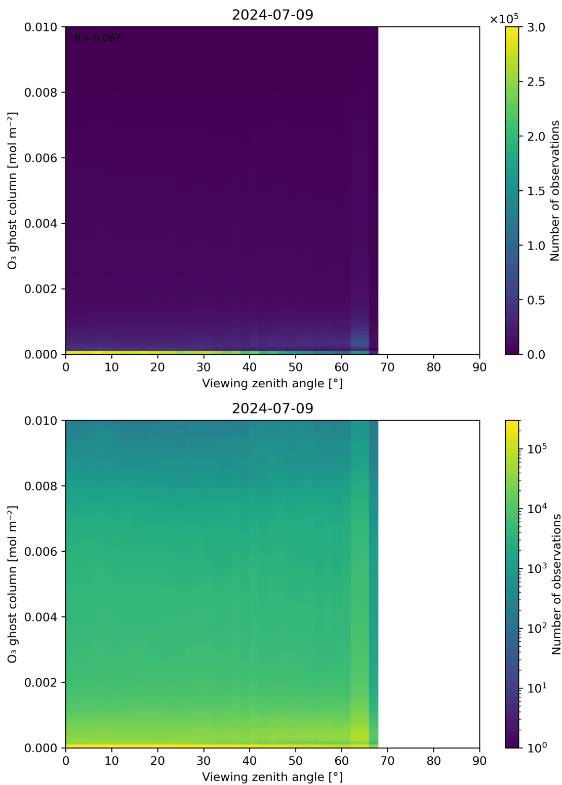
Figure 51: Scatter density plot of “Viewing zenith angle” against “O 3 ghost column” for 2024-07-08 to 2024-07-10.
