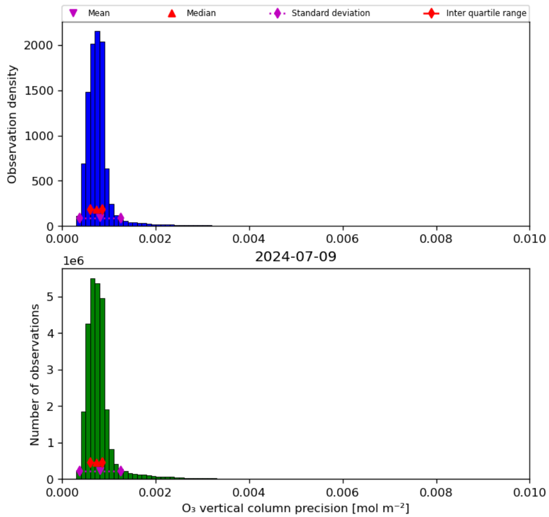
Figure 22: Histogram of “O 3 vertical column precision” for 2024-07-08 to 2024-07-10
