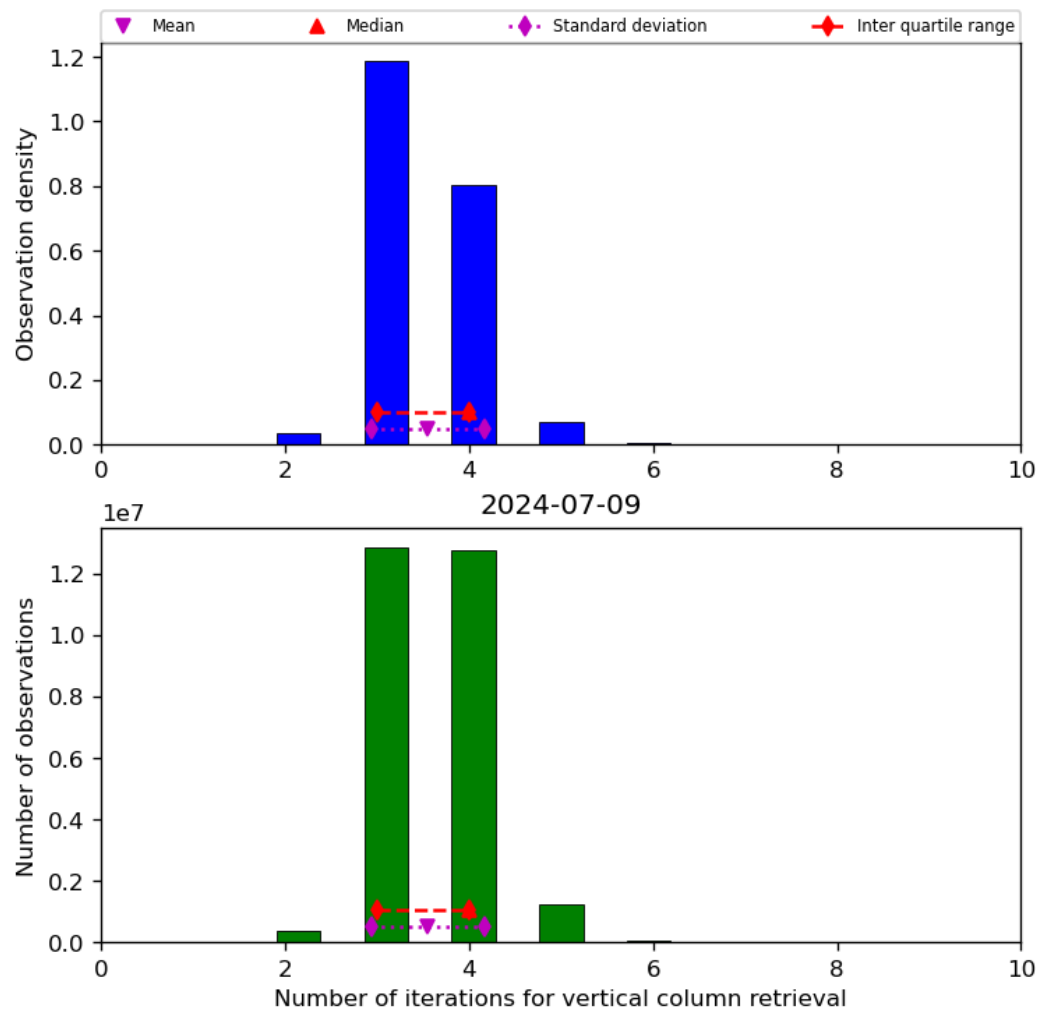
Figure 26: Histogram of “Number of iterations for vertical column retrieval” for 2024-07-08 to 2024-07-10
