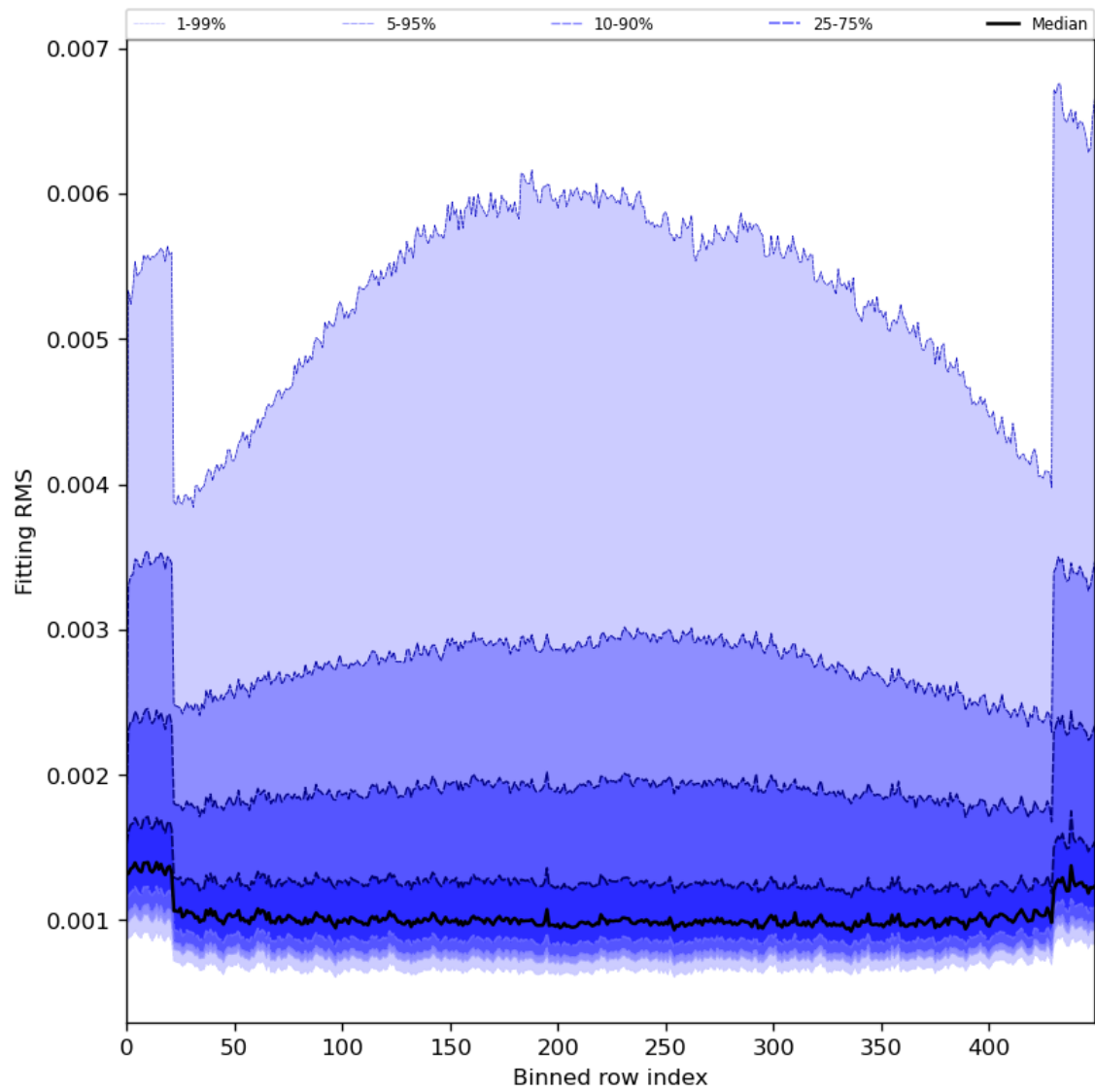
Figure 30: Along track statistics of “Fitting RMS” for 2024-07-08 to 2024-07-10
