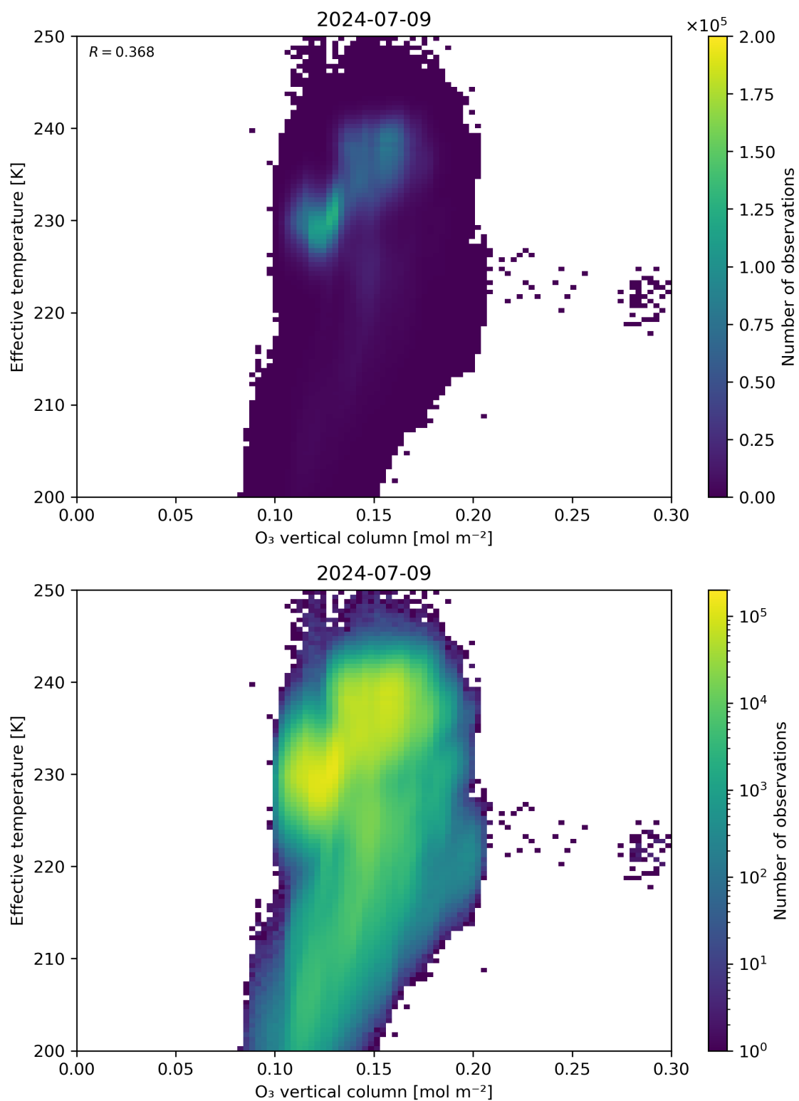
Figure 39: Scatter density plot of “O 3 vertical column” against “Effective temperature” for 2024-07-08 to 2024-07-10.
