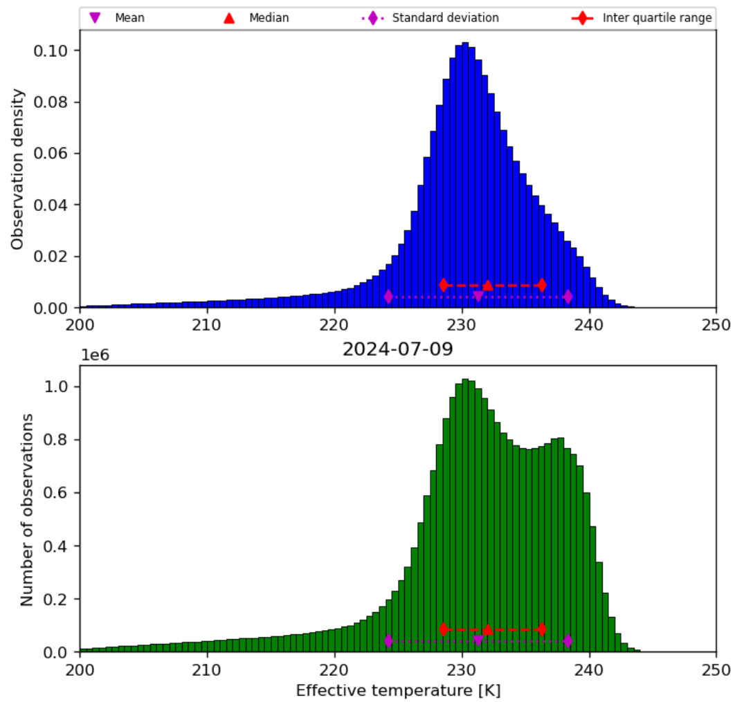
Figure 24: Histogram of “Effective temperature” for 2024-07-08 to 2024-07-10
