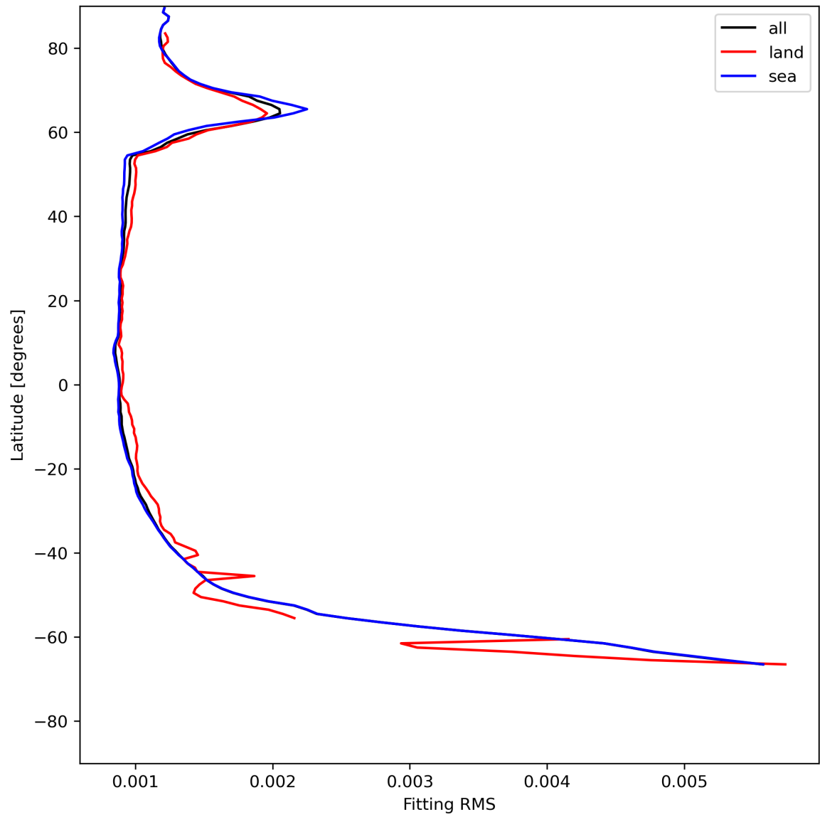
Figure 16: Zonal average of “Fitting RMS” for 2024-07-08 to 2024-07-10.
