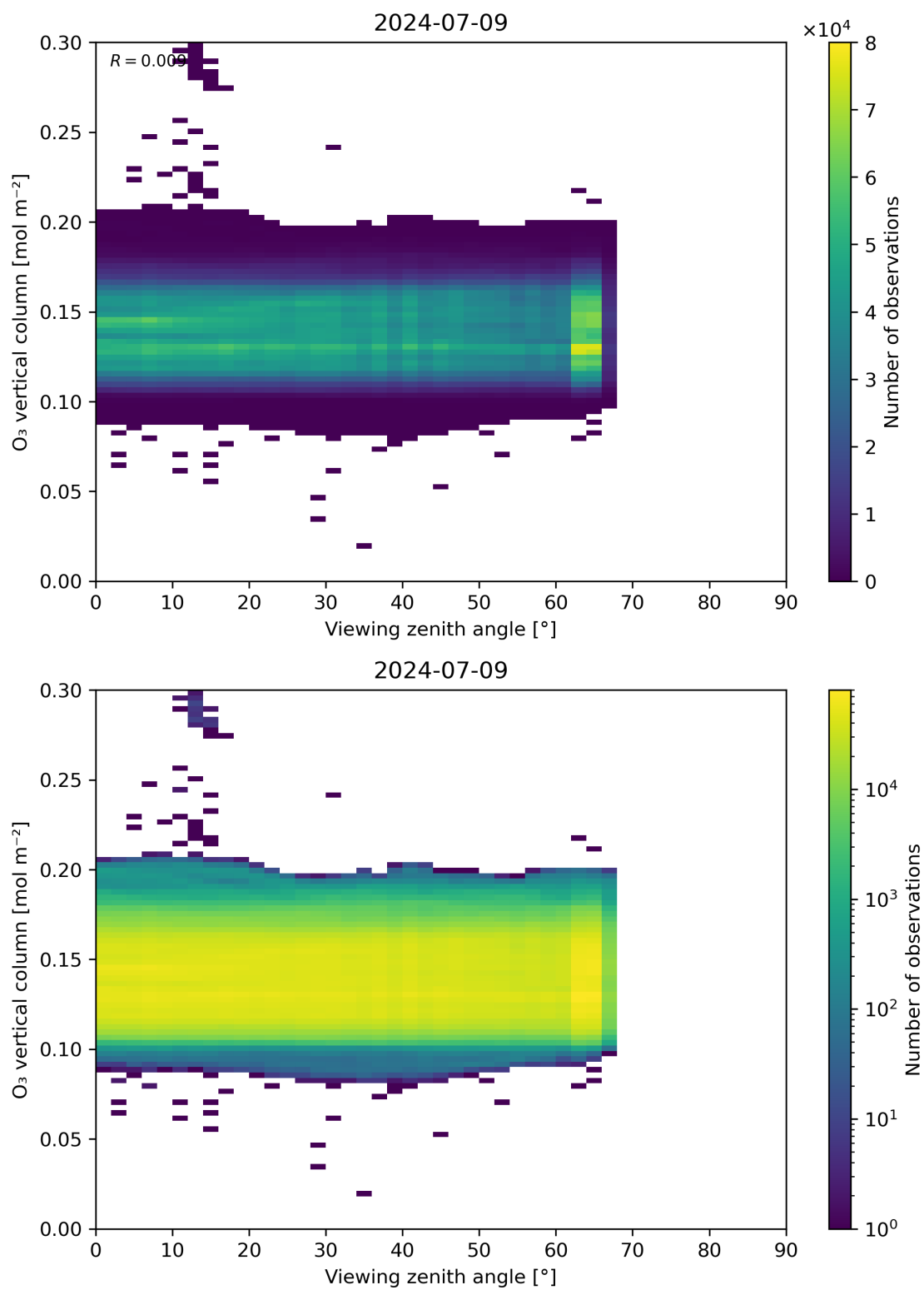
Figure 52: Scatter density plot of “Viewing zenith angle” against “O 3 vertical column” for 2024-07-08 to 2024-07-10.
