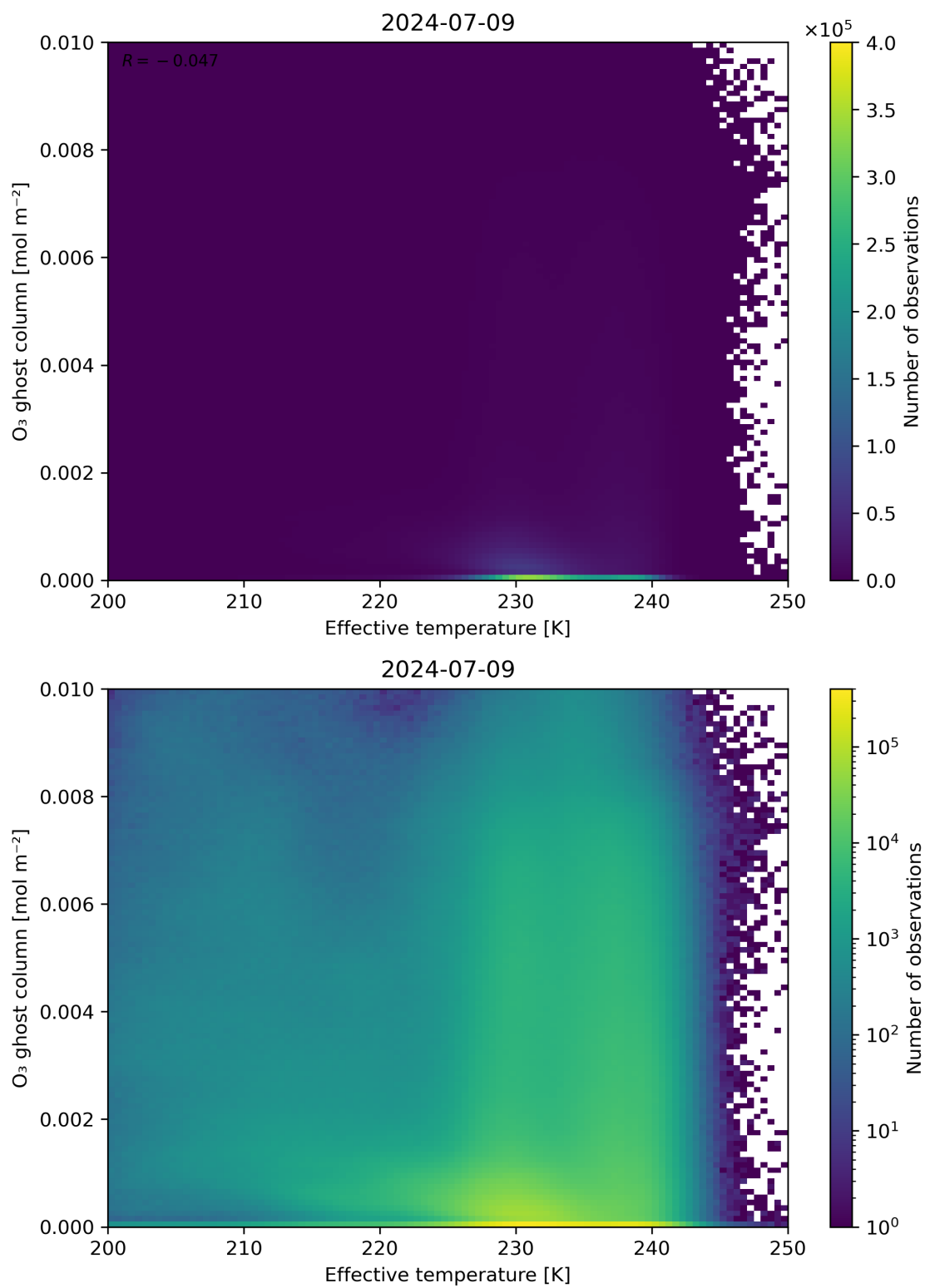
Figure 38: Scatter density plot of “Effective temperature” against “O 3 ghost column” for 2024-07-08 to 2024-07-10.
