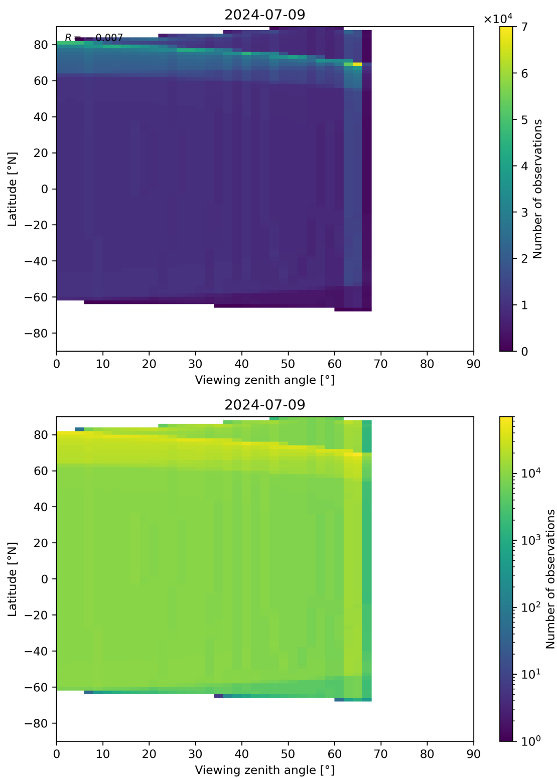
Figure 49: Scatter density plot of “Viewing zenith angle” against “Latitude” for 2024-07-08 to 2024-07-10.
