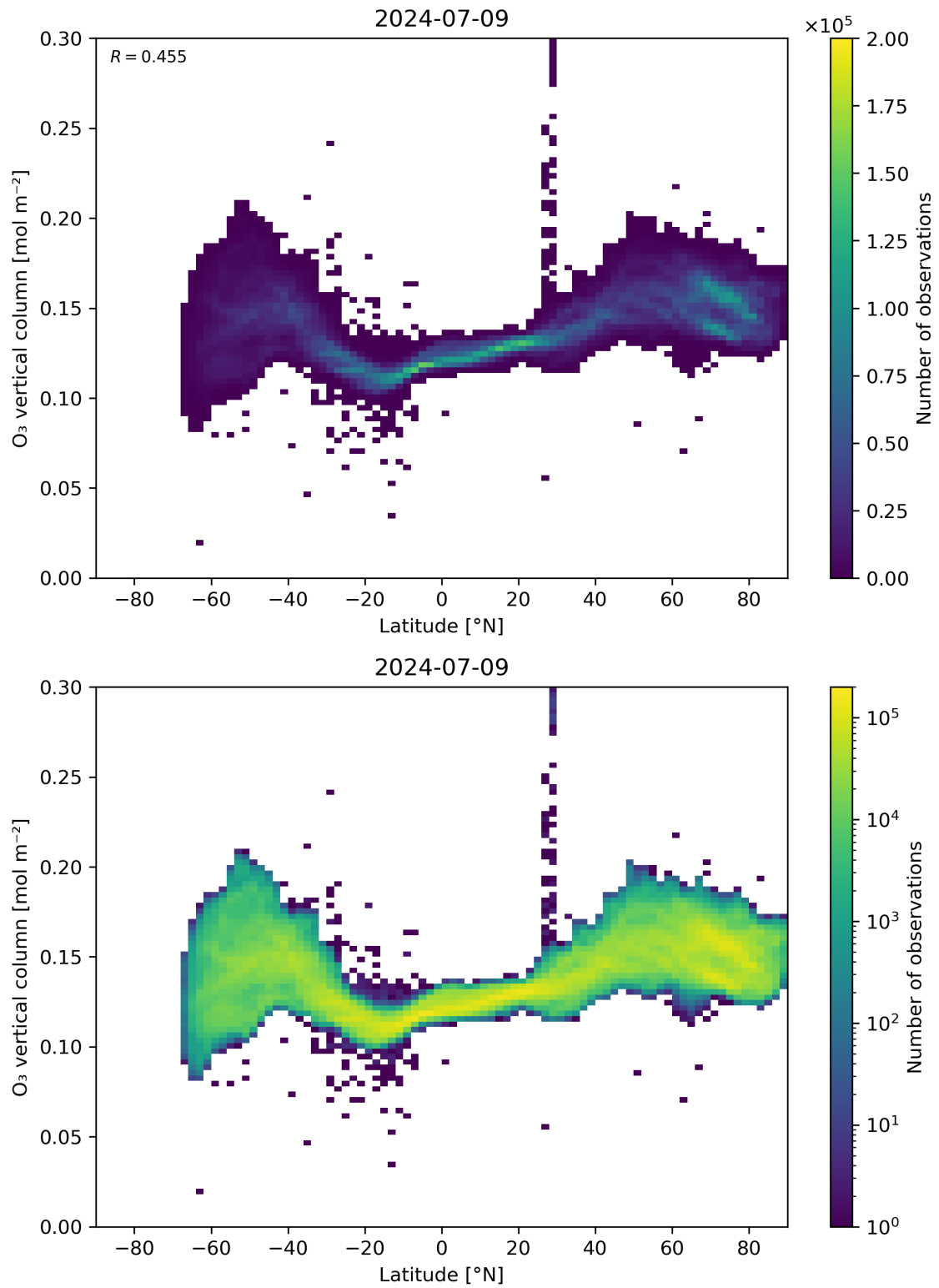
Figure 36: Scatter density plot of “Latitude” against “O 3 vertical column” for 2024-07-08 to 2024-07-10.
