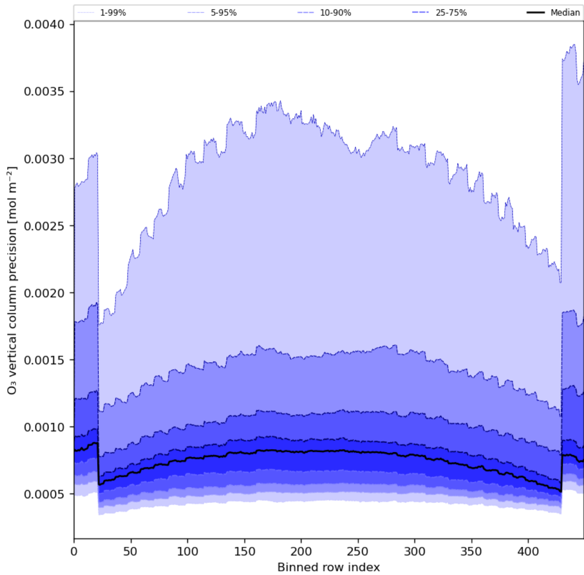
Figure 29: Along track statistics of “O 3 vertical column precision” for 2024-07-08 to 2024-07-10
