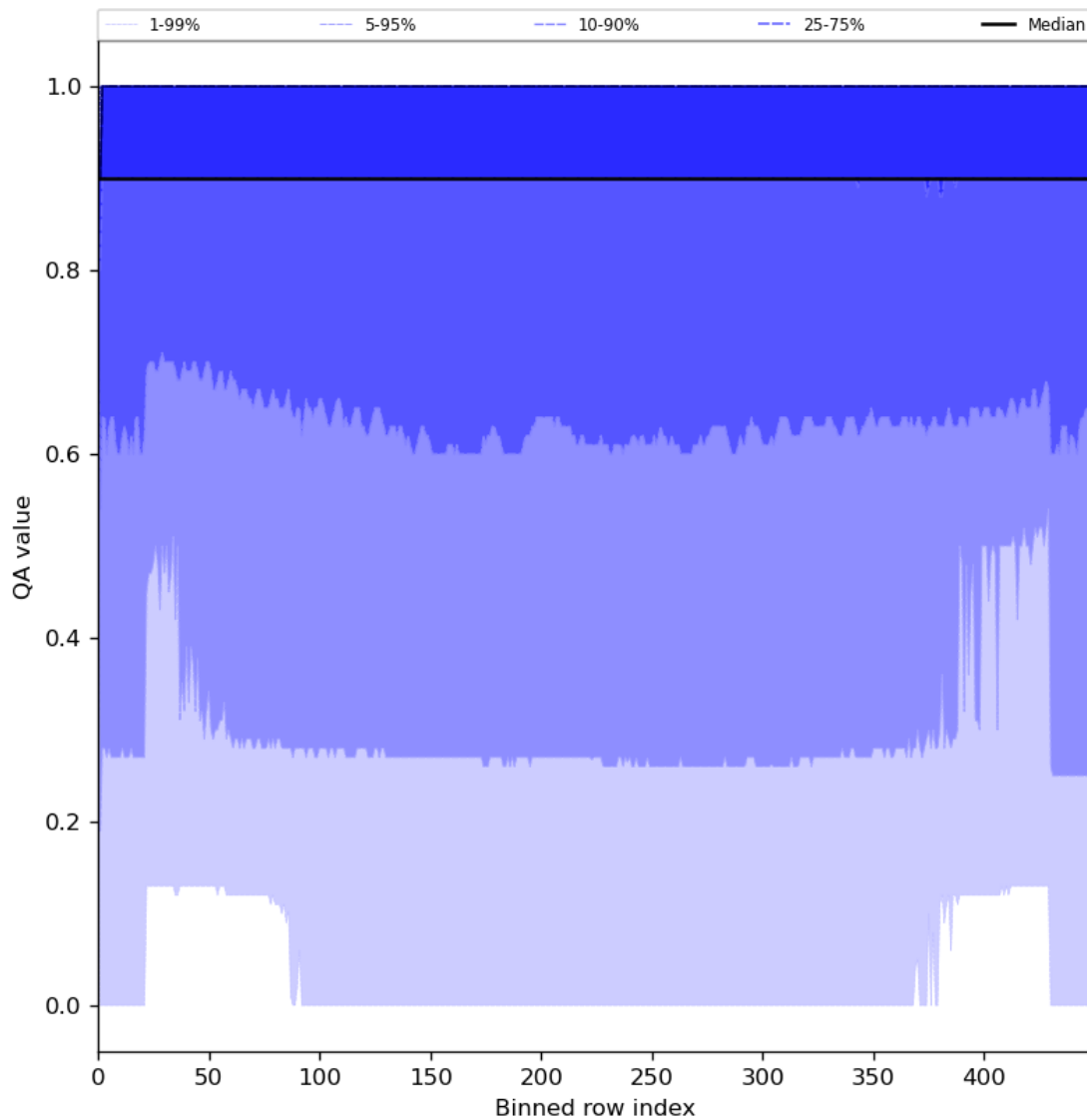
Figure 27: Along track statistics of “QA value” for 2024-07-08 to 2024-07-10
