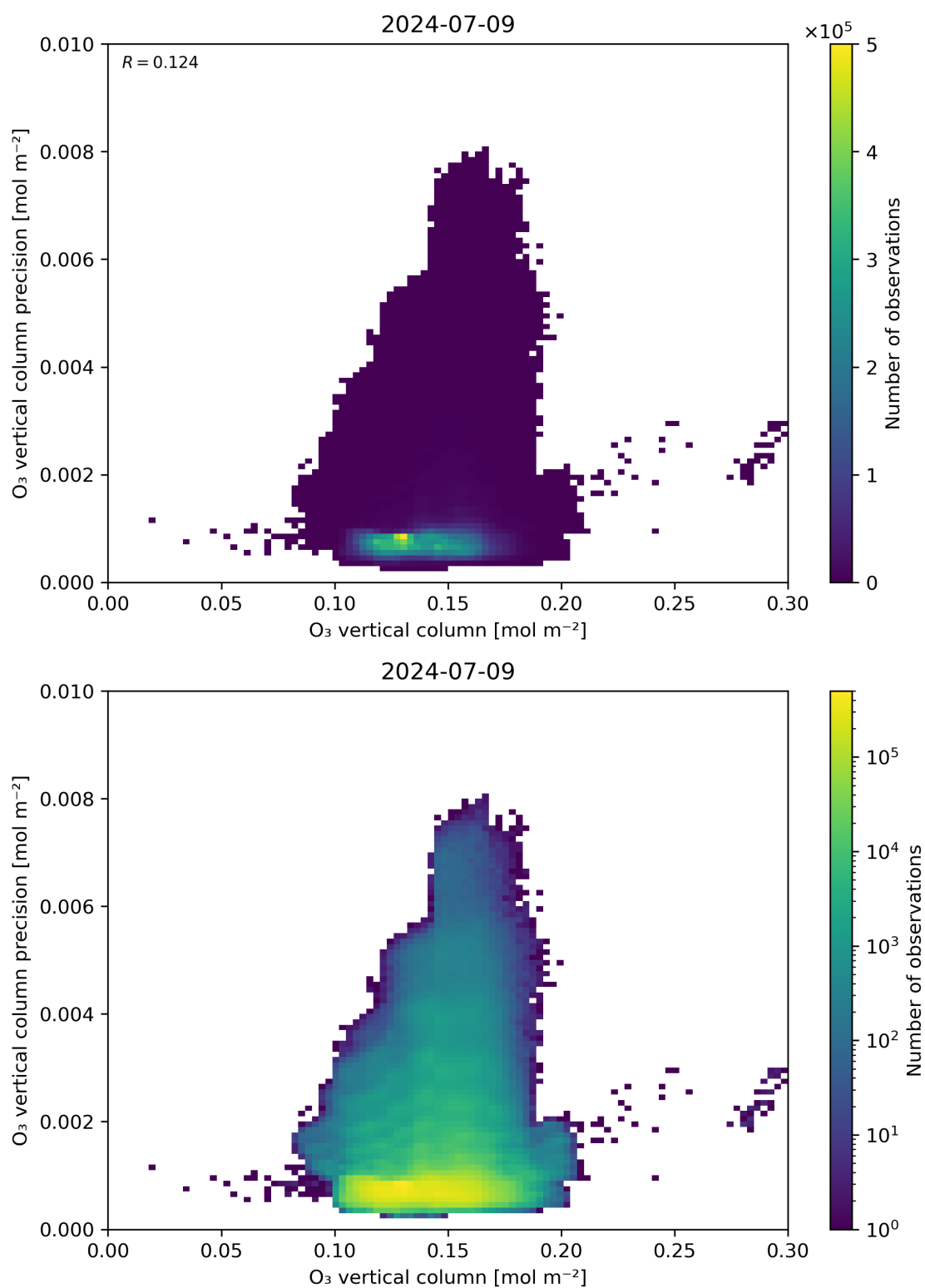
Figure 41: Scatter density plot of “O 3 vertical column” against “O 3 vertical column precision” for 2024-07-08 to 2024-07-10.
