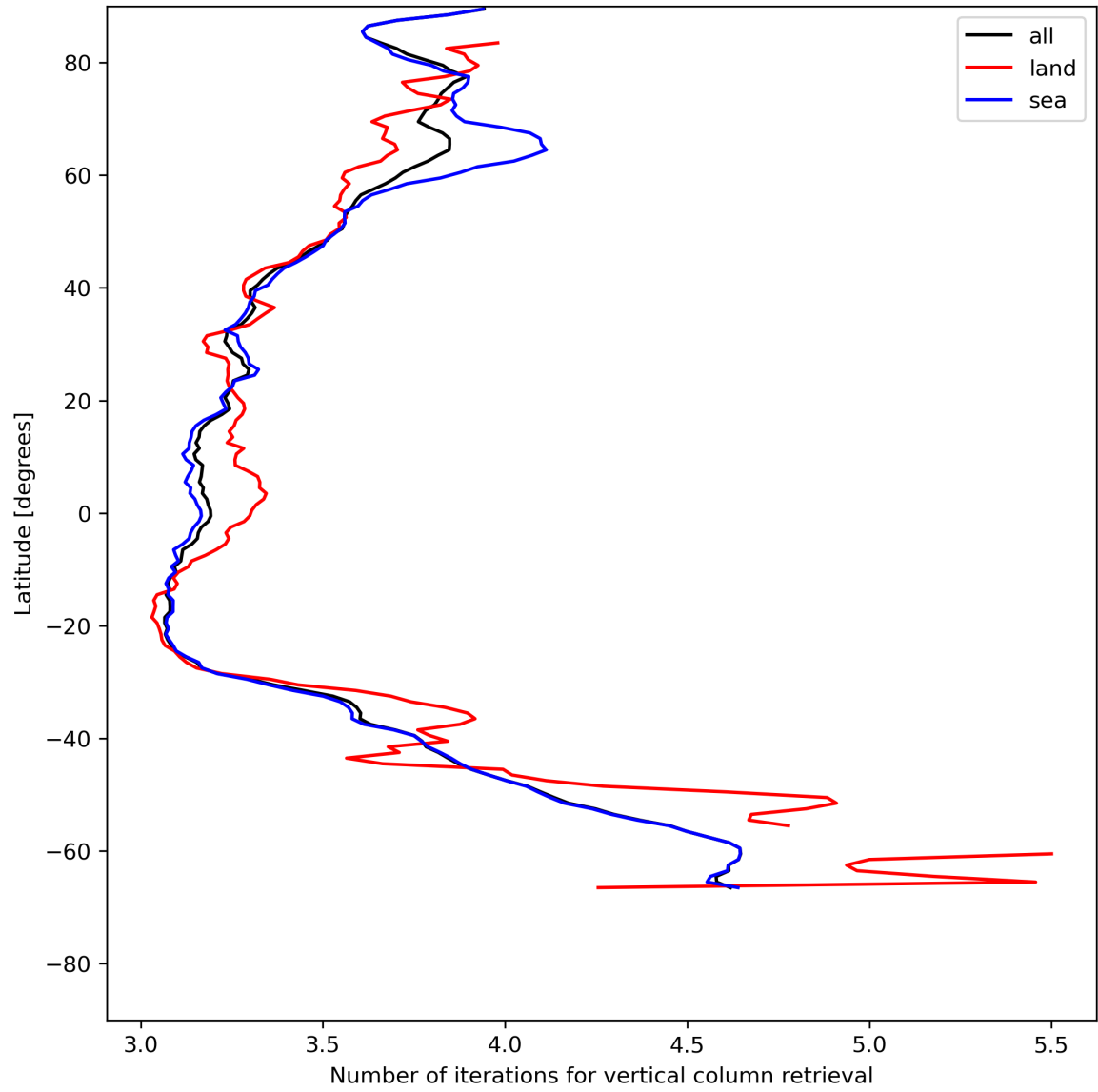
Figure 19: Zonal average of “Number of iterations for vertical column retrieval” for 2024-07-08 to 2024-07-10.
