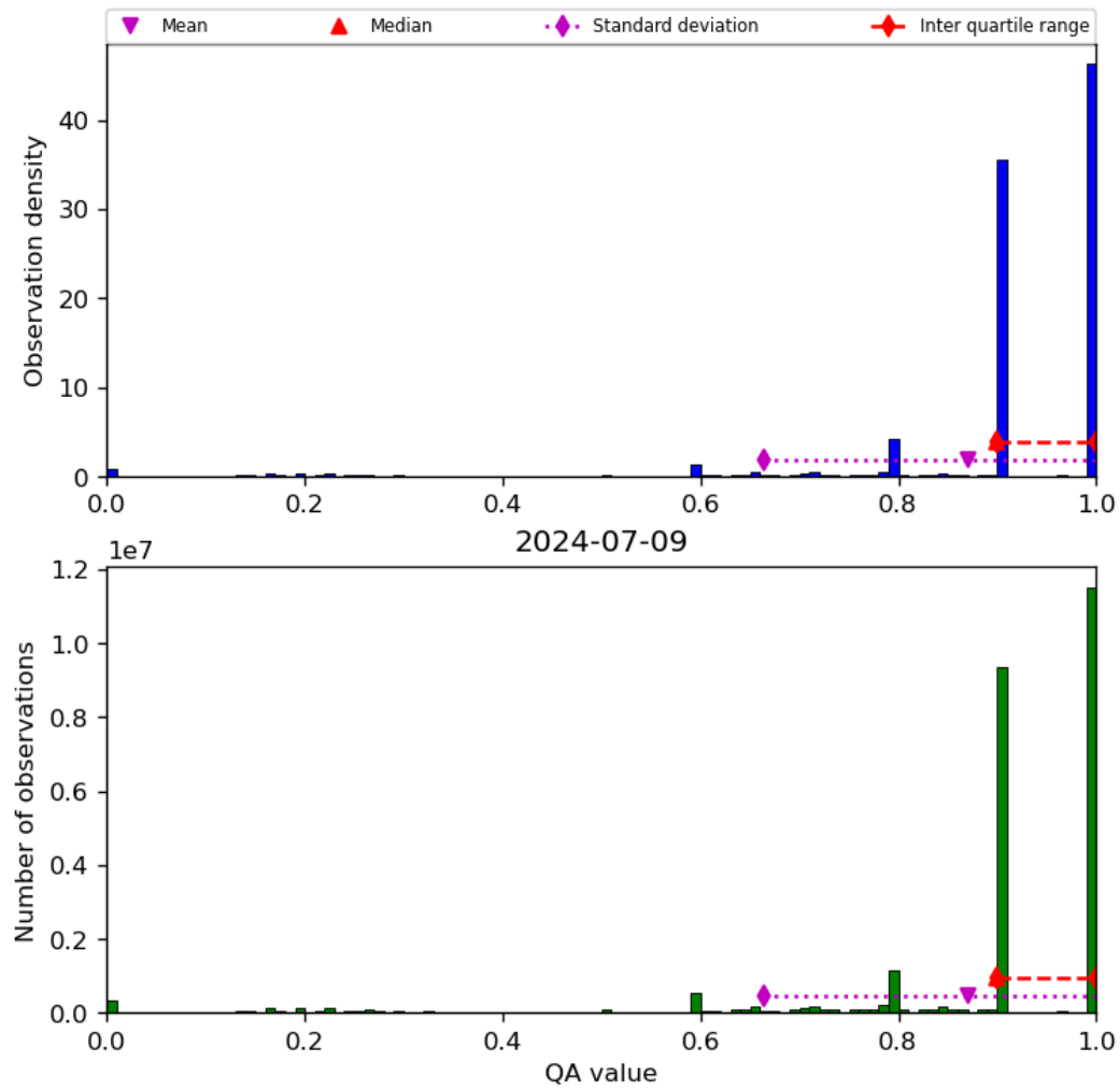
Figure 20: Histogram of “QA value” for 2024-07-08 to 2024-07-10
