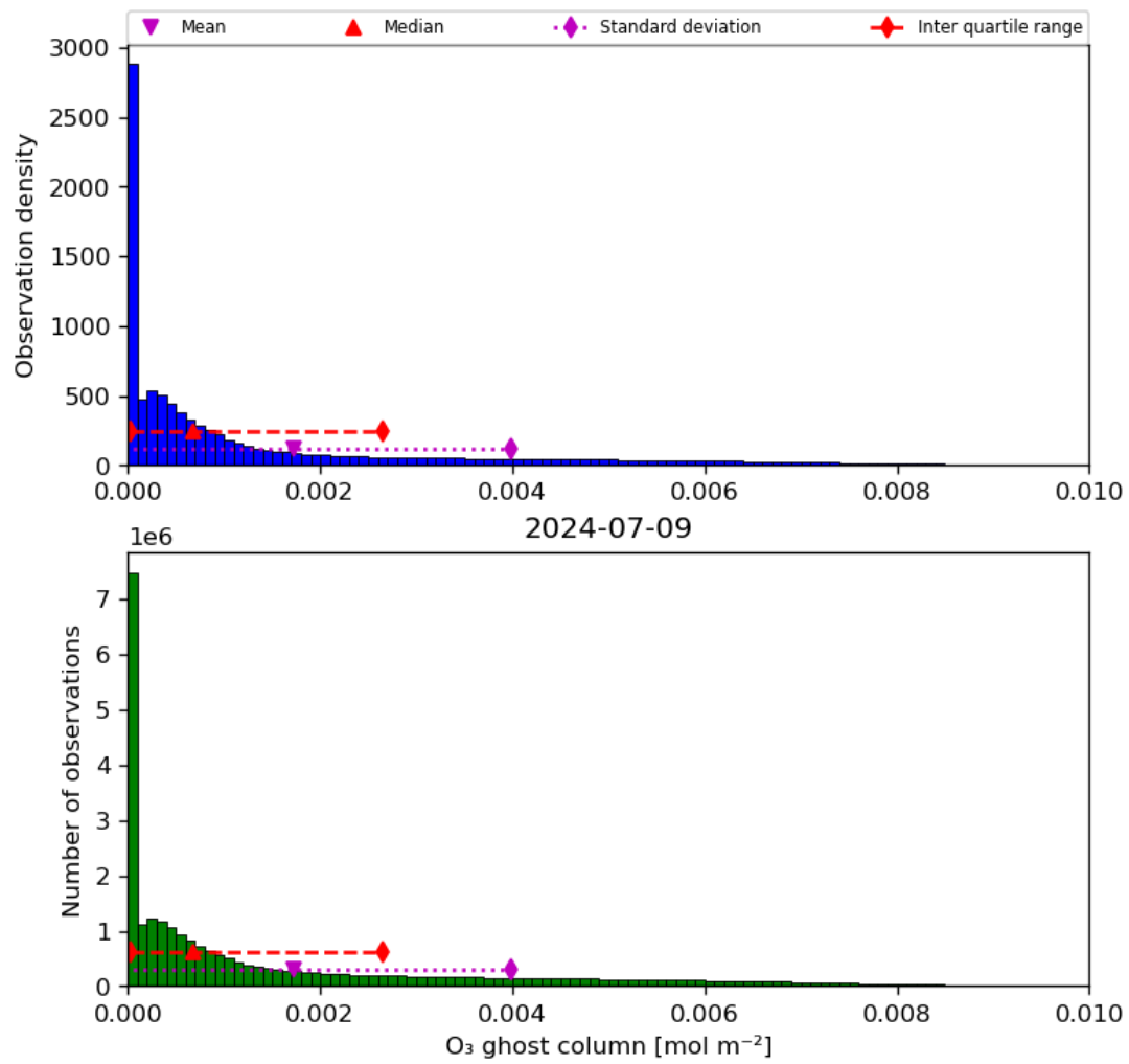
Figure 25: Histogram of "O 3 ghost column" for 2024-07-08 to 2024-07-10
