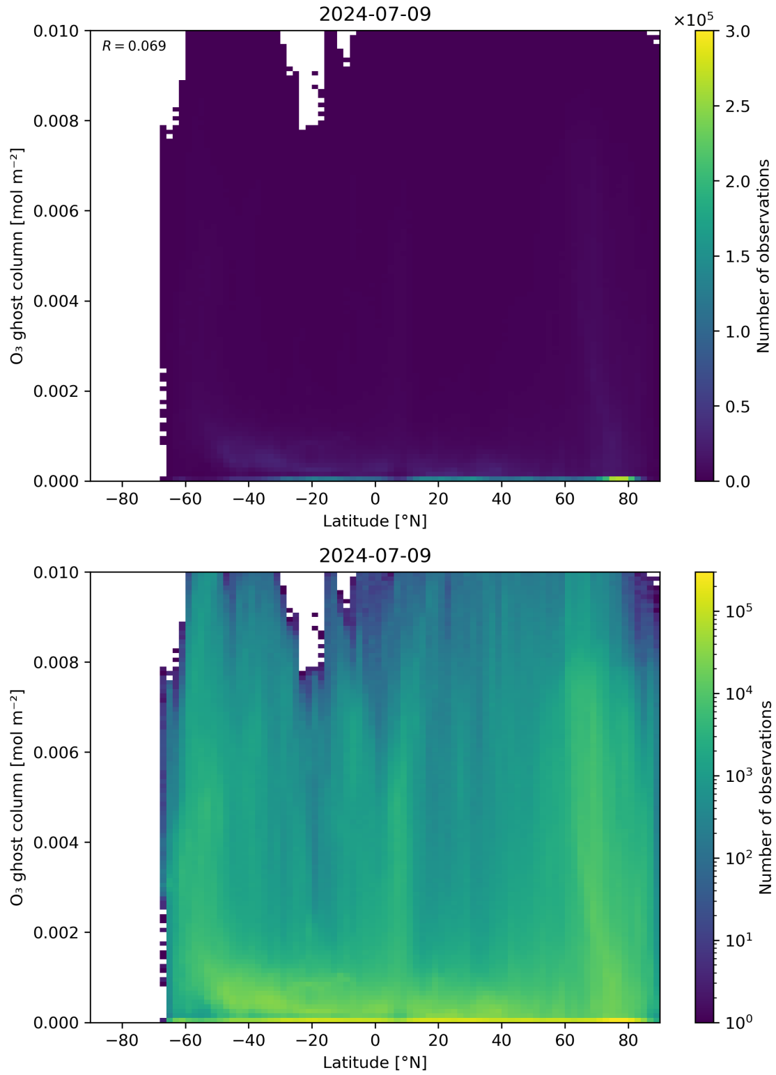
Figure 35: Scatter density plot of “Latitude” against “O 3 ghost column” for 2024-07-08 to 2024-07-10.
