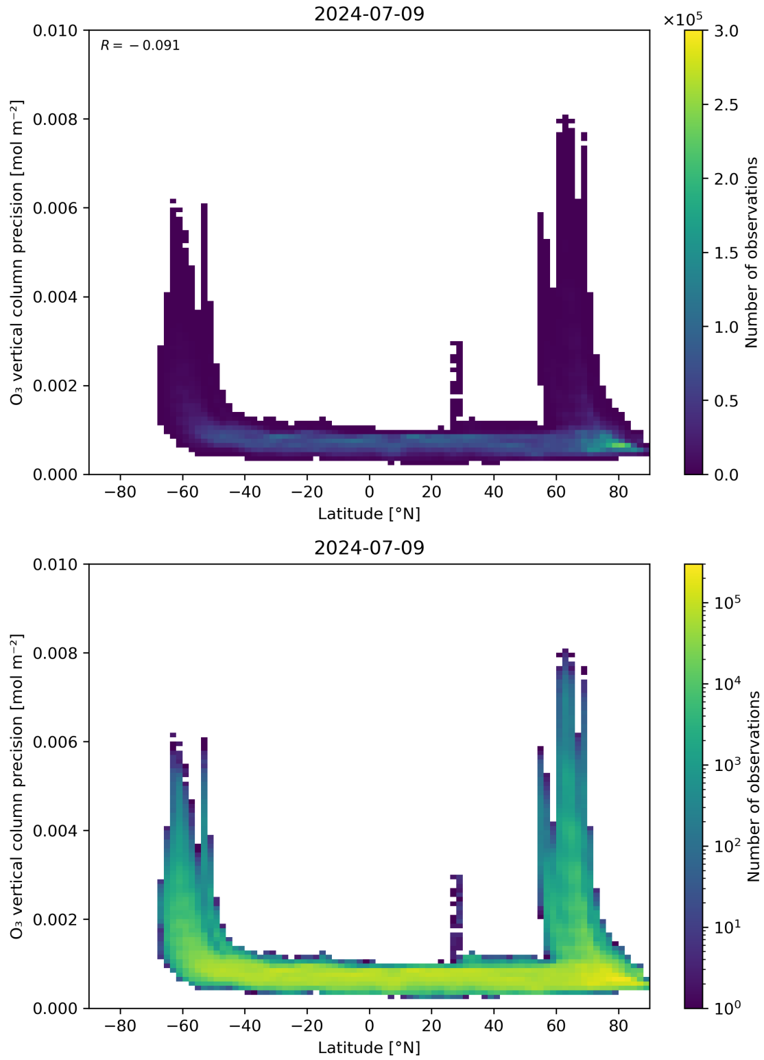
Figure 37: Scatter density plot of “Latitude” against “O 3 vertical column precision” for 2024-07-08 to 2024-07-10.
