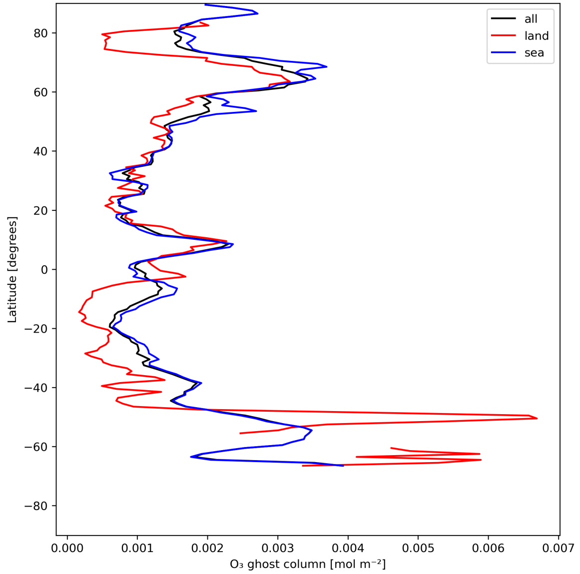
Figure 18: Zonal average of "O 3 ghost column" for 2024-07-08 to 2024-07-10.
