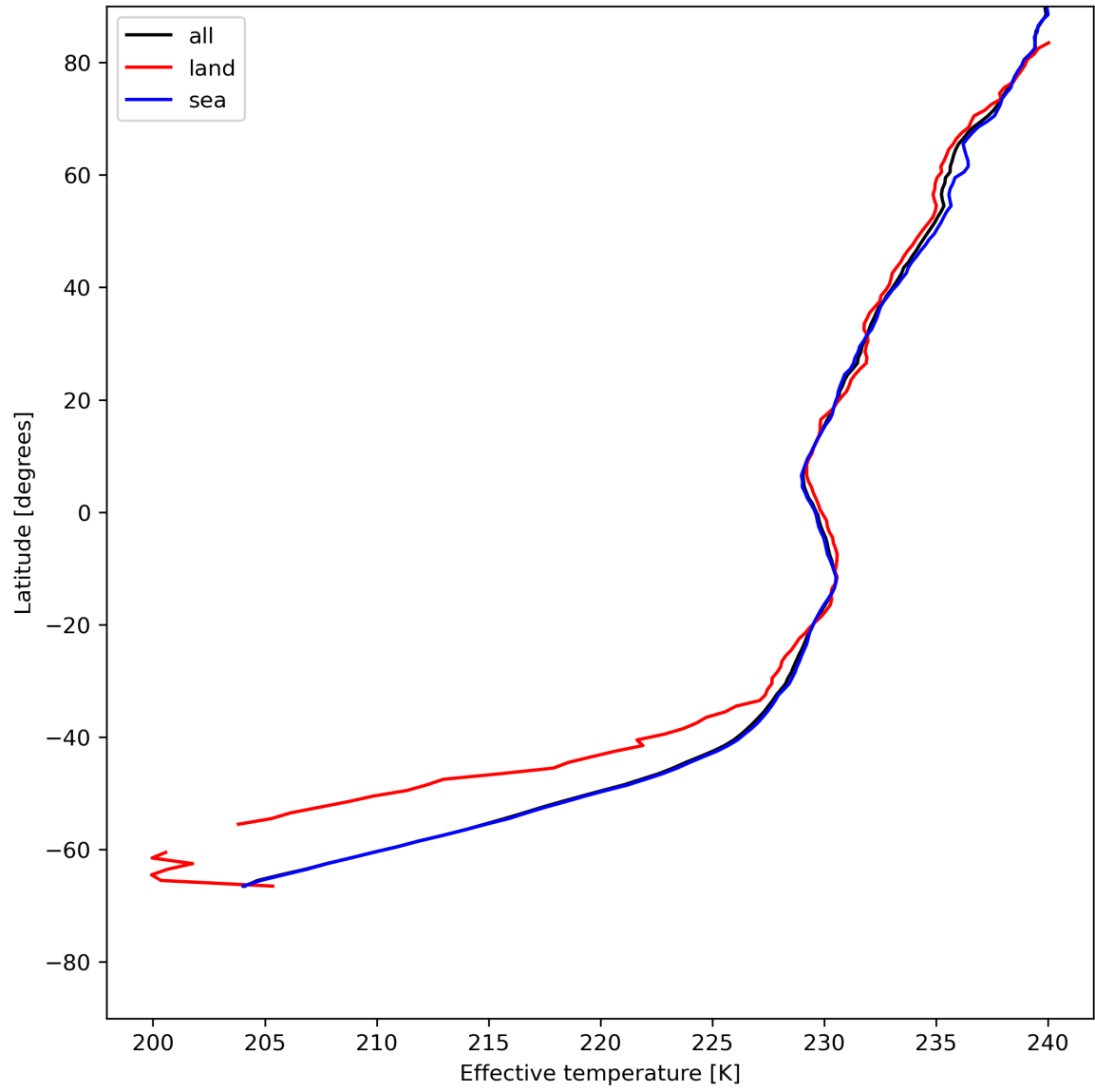
Figure 17: Zonal average of "Effective temperature" for 2024-07-08 to 2024-07-10.
