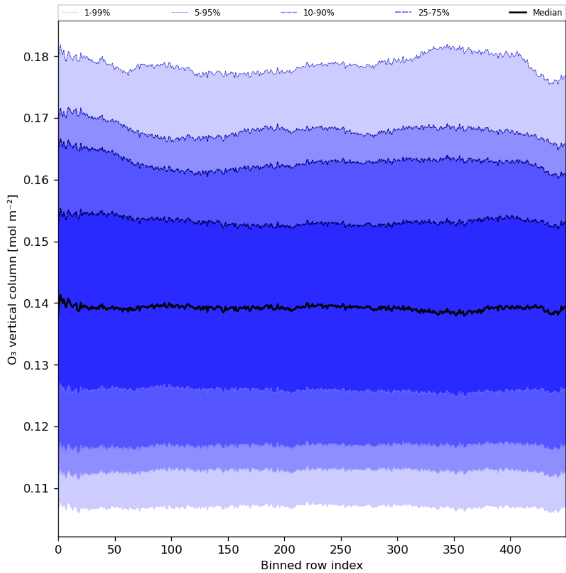
Figure 28: Along track statistics of “O 3 vertical column” for 2024-07-08 to 2024-07-10
