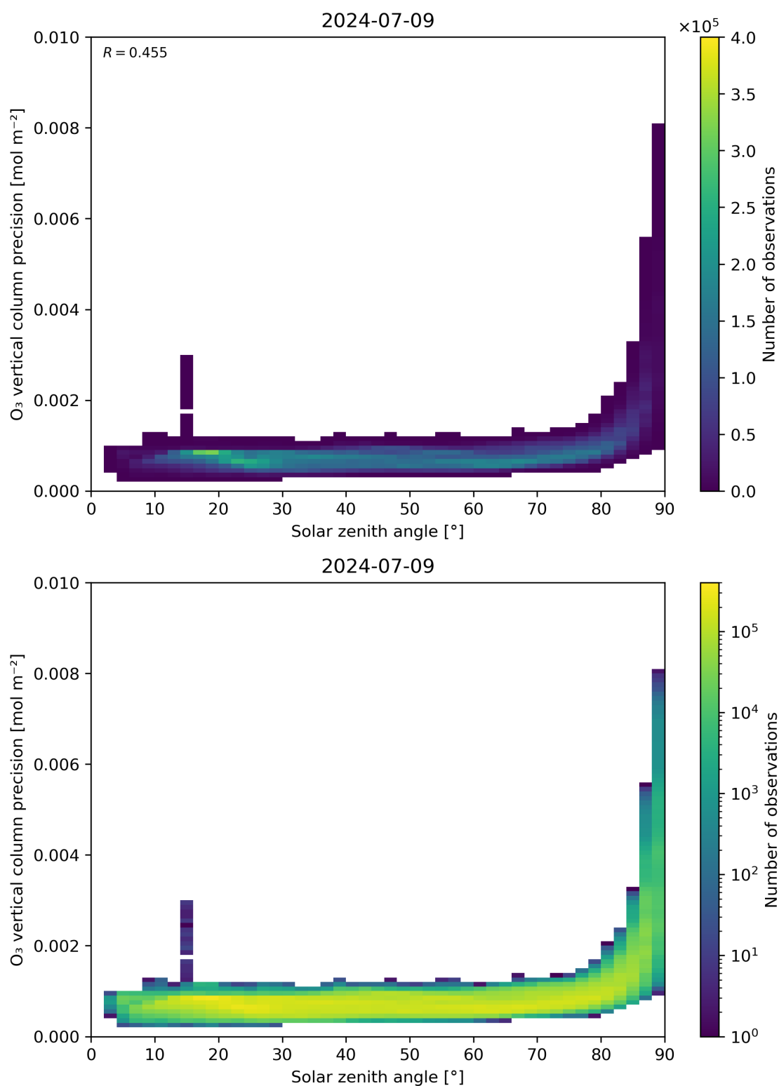
Figure 48: Scatter density plot of “Solar zenith angle” against “O 3 vertical column precision” for 2024-07-08 to 2024-07-10.
