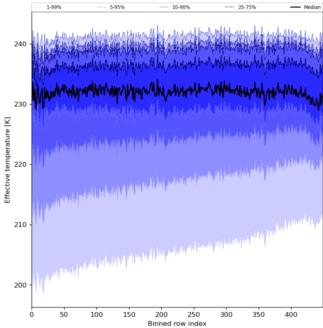
Figure 31: Along track statistics of “Effective temperature” for 2024-07-08 to 2024-07-10
