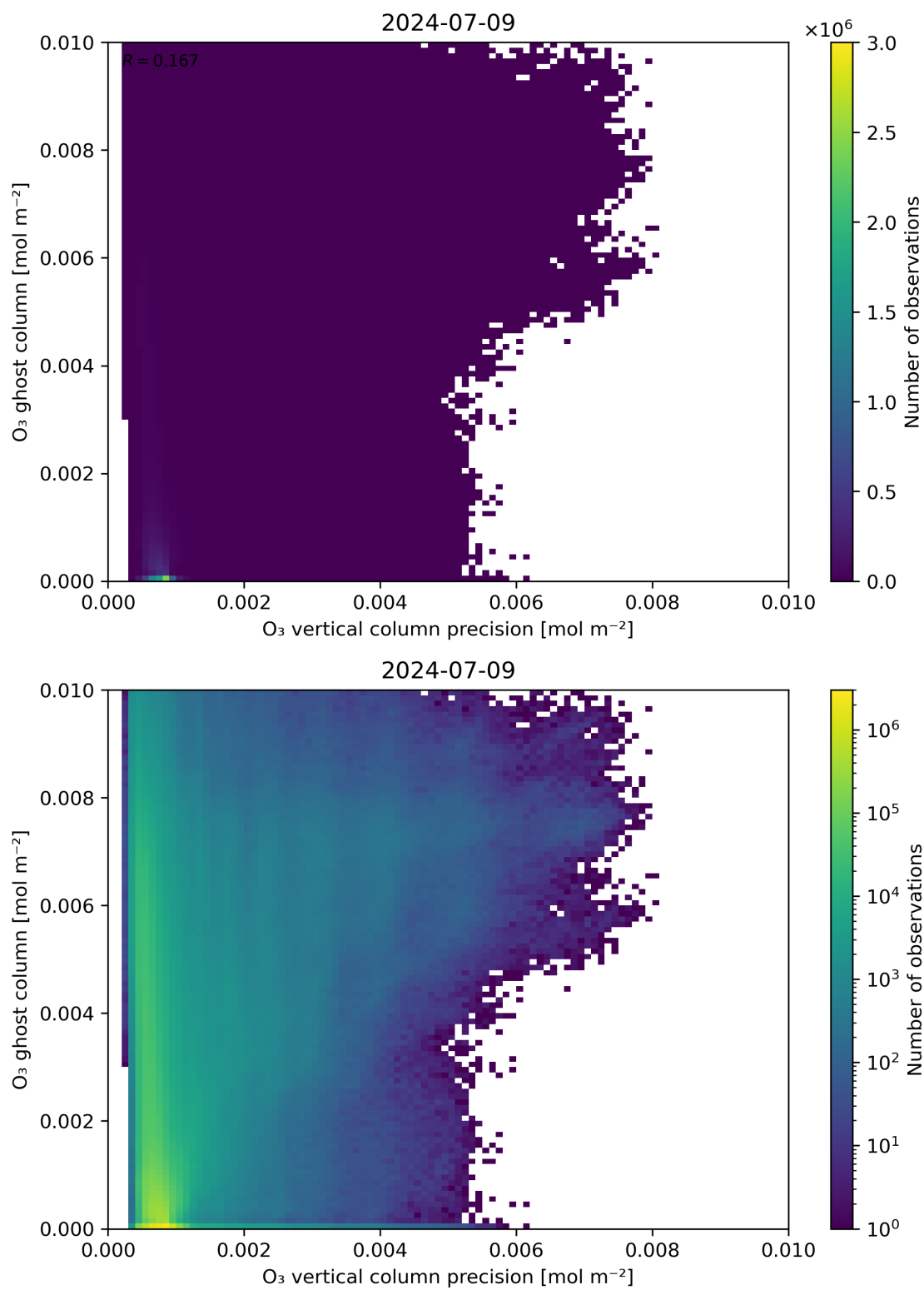
Figure 43: Scatter density plot of “ \text{O}_3 vertical column precision” against “ \text{O}_3 ghost column” for 2024-07-08 to 2024-07-10.
