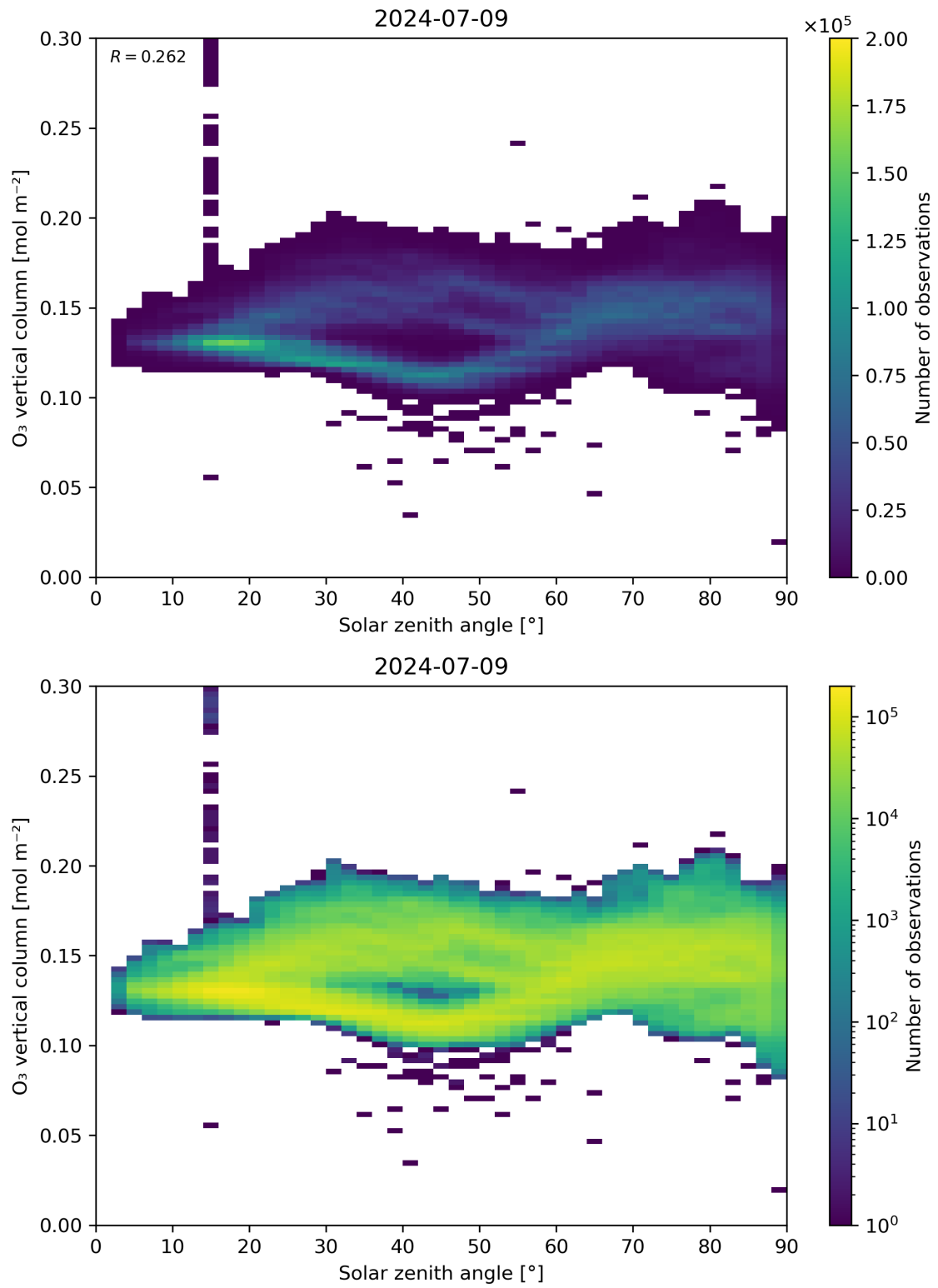
Figure 47: Scatter density plot of “Solar zenith angle” against “O 3 vertical column” for 2024-07-08 to 2024-07-10.
