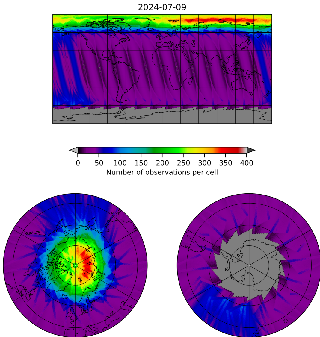
Figure 12: Map of the number of observations for 2024-07-08 to 2024-07-10
