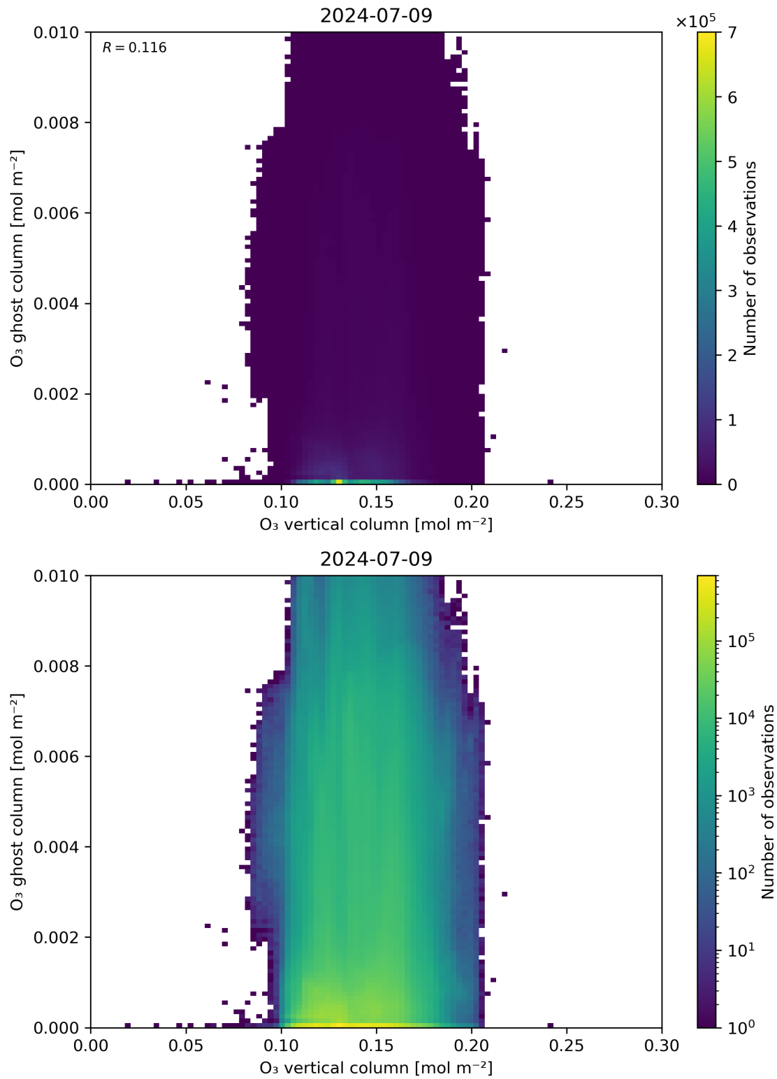
Figure 40: Scatter density plot of “O 3 vertical column” against “O 3 ghost column” for 2024-07-08 to 2024-07-10.
