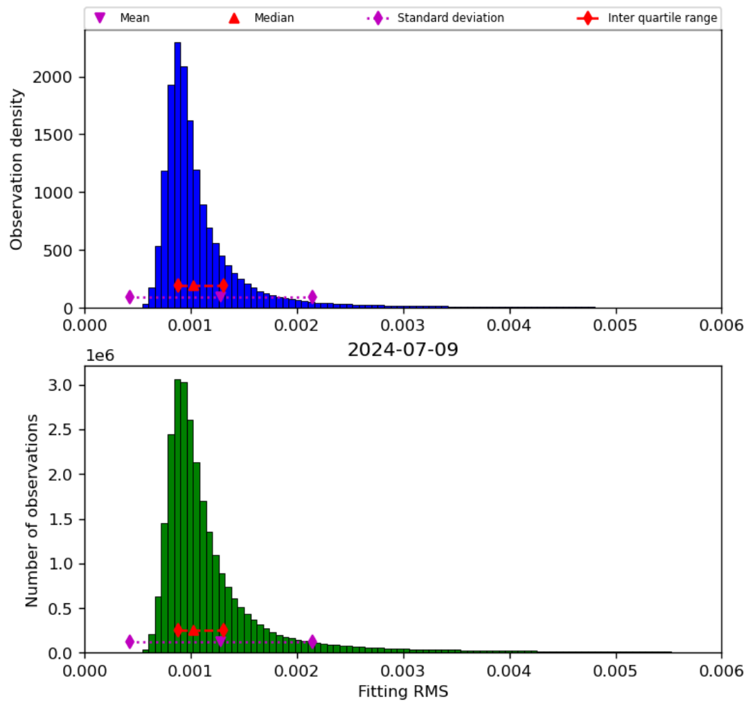
Figure 23: Histogram of “Fitting RMS” for 2024-07-08 to 2024-07-10
