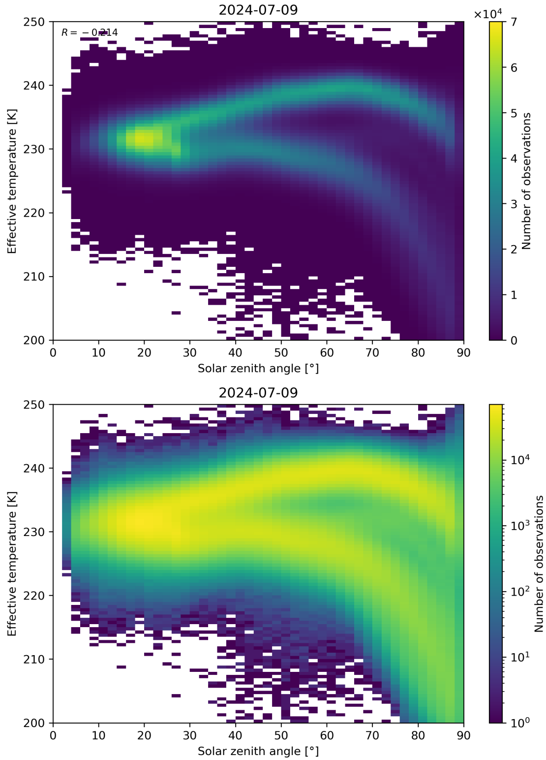
Figure 45: Scatter density plot of “Solar zenith angle” against “Effective temperature” for 2024-07-08 to 2024-07-10.
