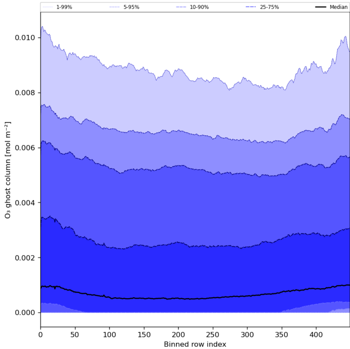
Figure 32: Along track statistics of “O 3 ghost column” for 2024-07-08 to 2024-07-10
