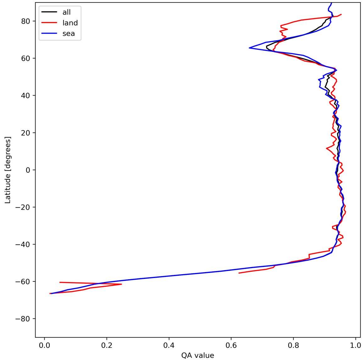
Figure 13: Zonal average of “QA value” for 2024-07-08 to 2024-07-10.
