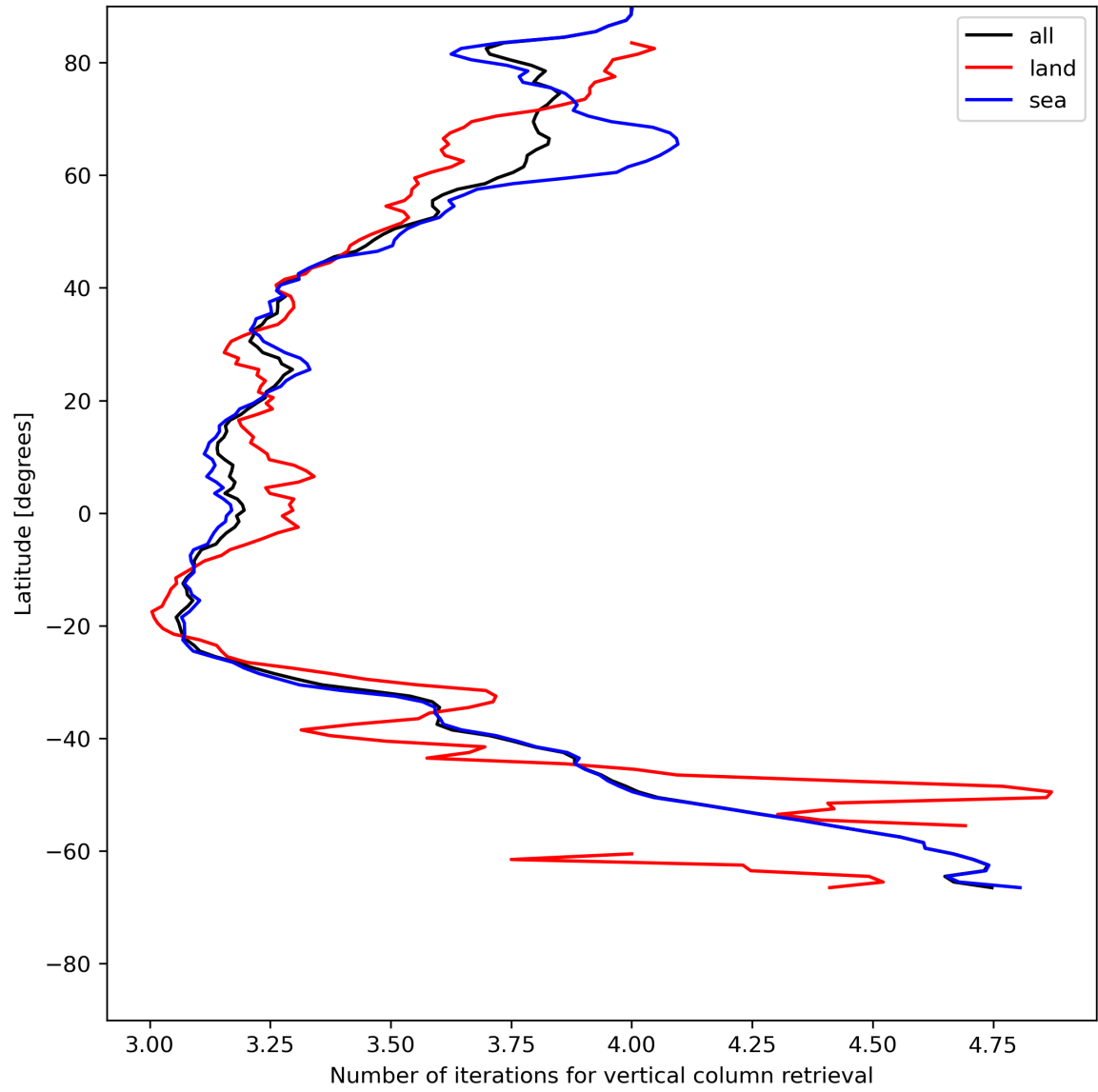
Figure 19: Zonal average of “Number of iterations for vertical column retrieval” for 2024-07-10 to 2024-07-11.
