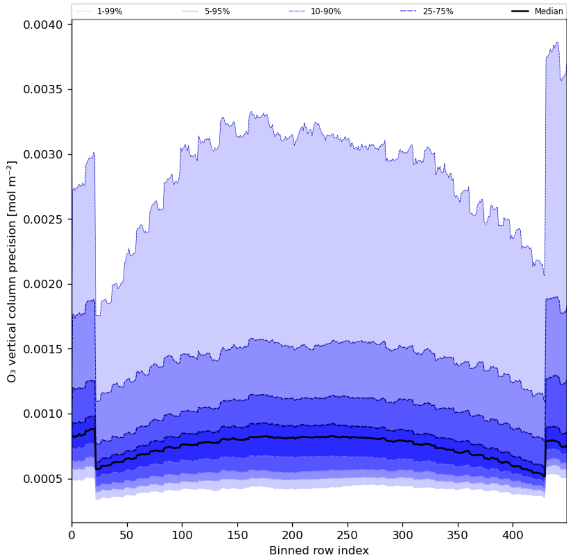
Figure 29: Along track statistics of “O 3 vertical column precision” for 2024-07-10 to 2024-07-11
