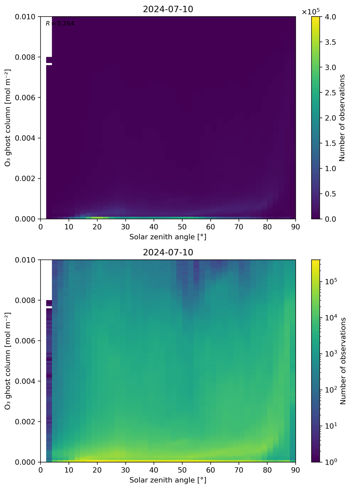
Figure 46: Scatter density plot of “Solar zenith angle” against “O 3 ghost column” for 2024-07-10 to 2024-07-11.
