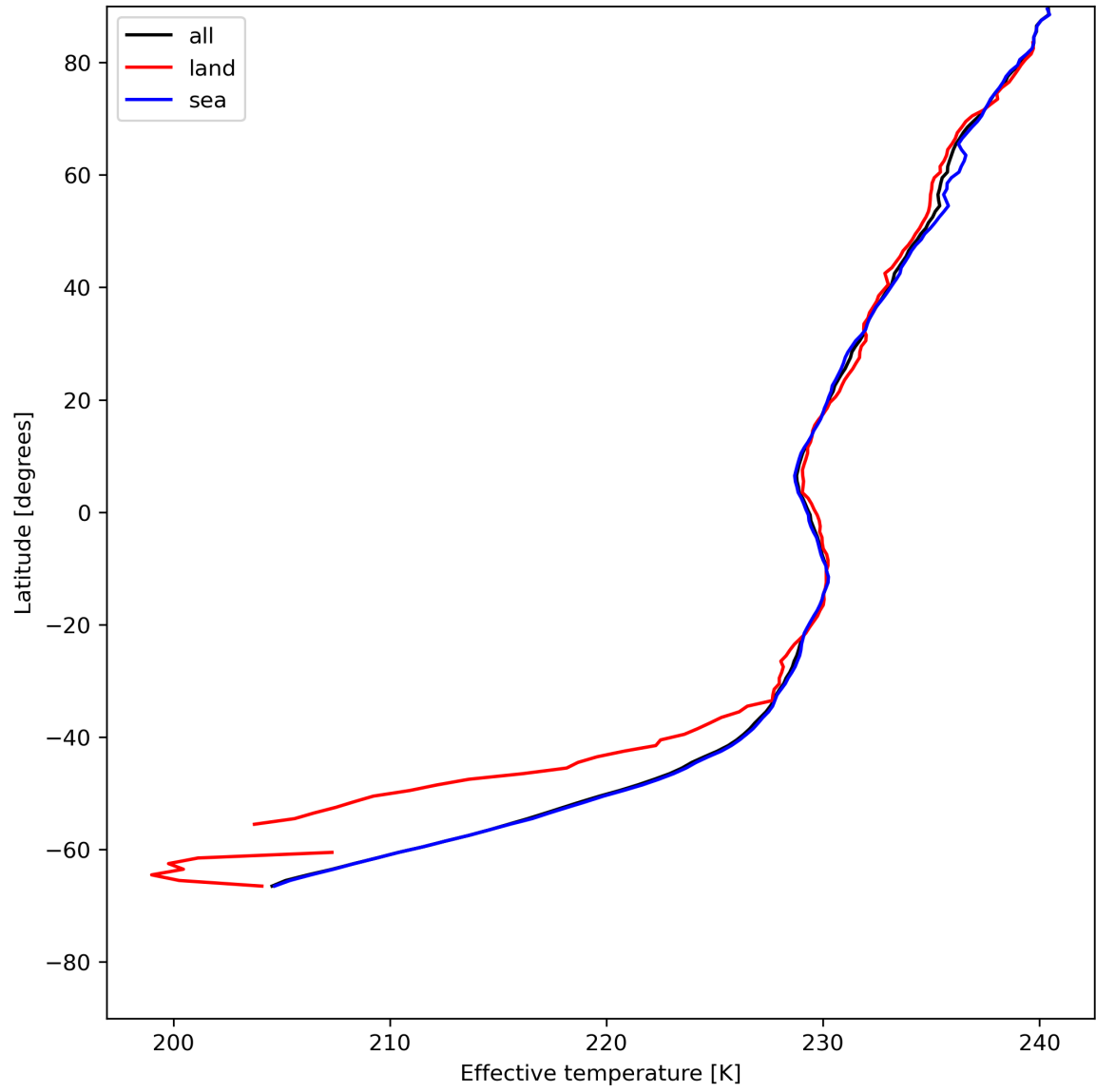
Figure 17: Zonal average of "Effective temperature" for 2024-07-10 to 2024-07-11.
