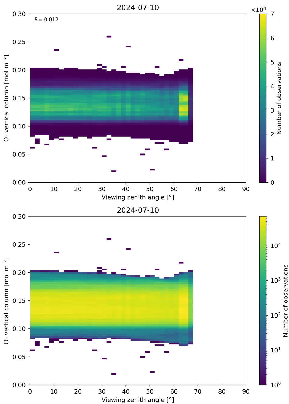
Figure 52: Scatter density plot of “Viewing zenith angle” against “O 3 vertical column” for 2024-07-10 to 2024-07-11.
