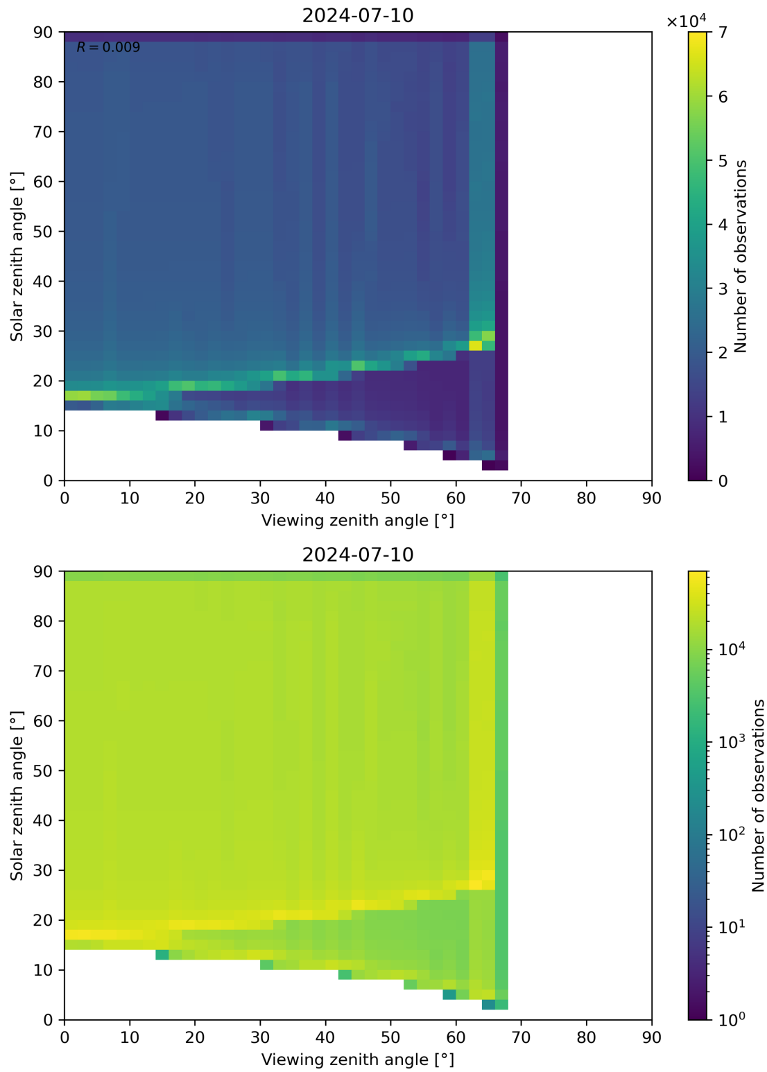
Figure 54: Scatter density plot of “Viewing zenith angle” against “Solar zenith angle” for 2024-07-10 to 2024-07-11.
