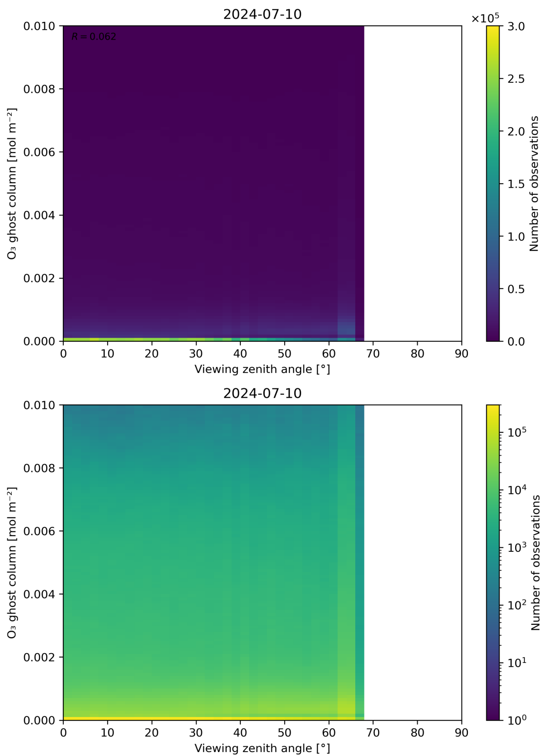
Figure 51: Scatter density plot of “Viewing zenith angle” against “O 3 ghost column” for 2024-07-10 to 2024-07-11.
