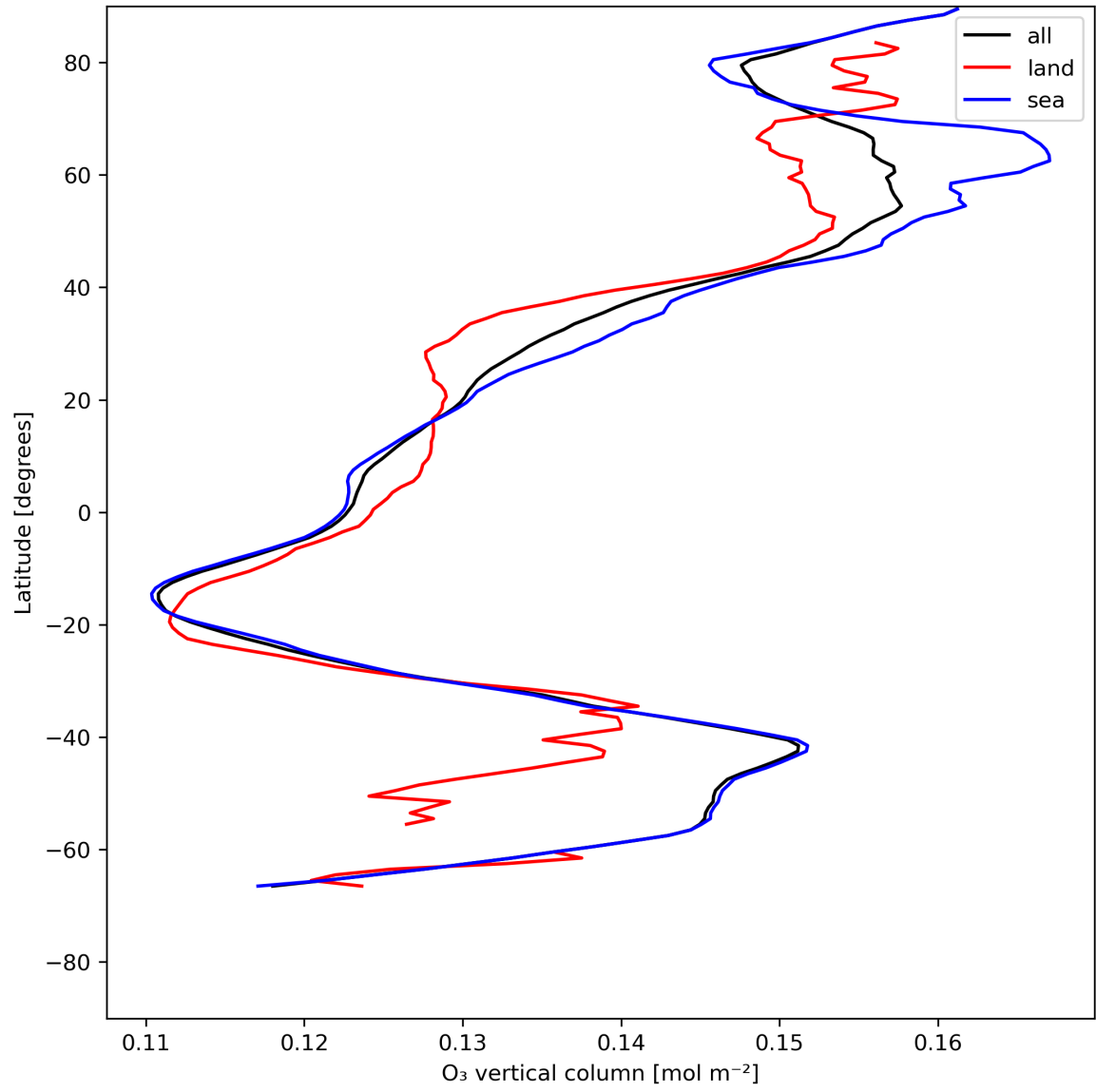
Figure 14: Zonal average of “O 3 vertical column” for 2024-07-10 to 2024-07-11.
