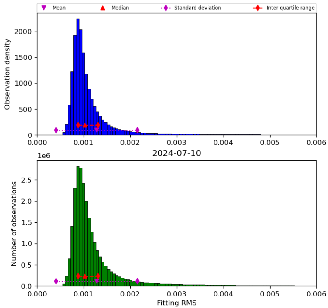
Figure 23: Histogram of “Fitting RMS” for 2024-07-10 to 2024-07-11
