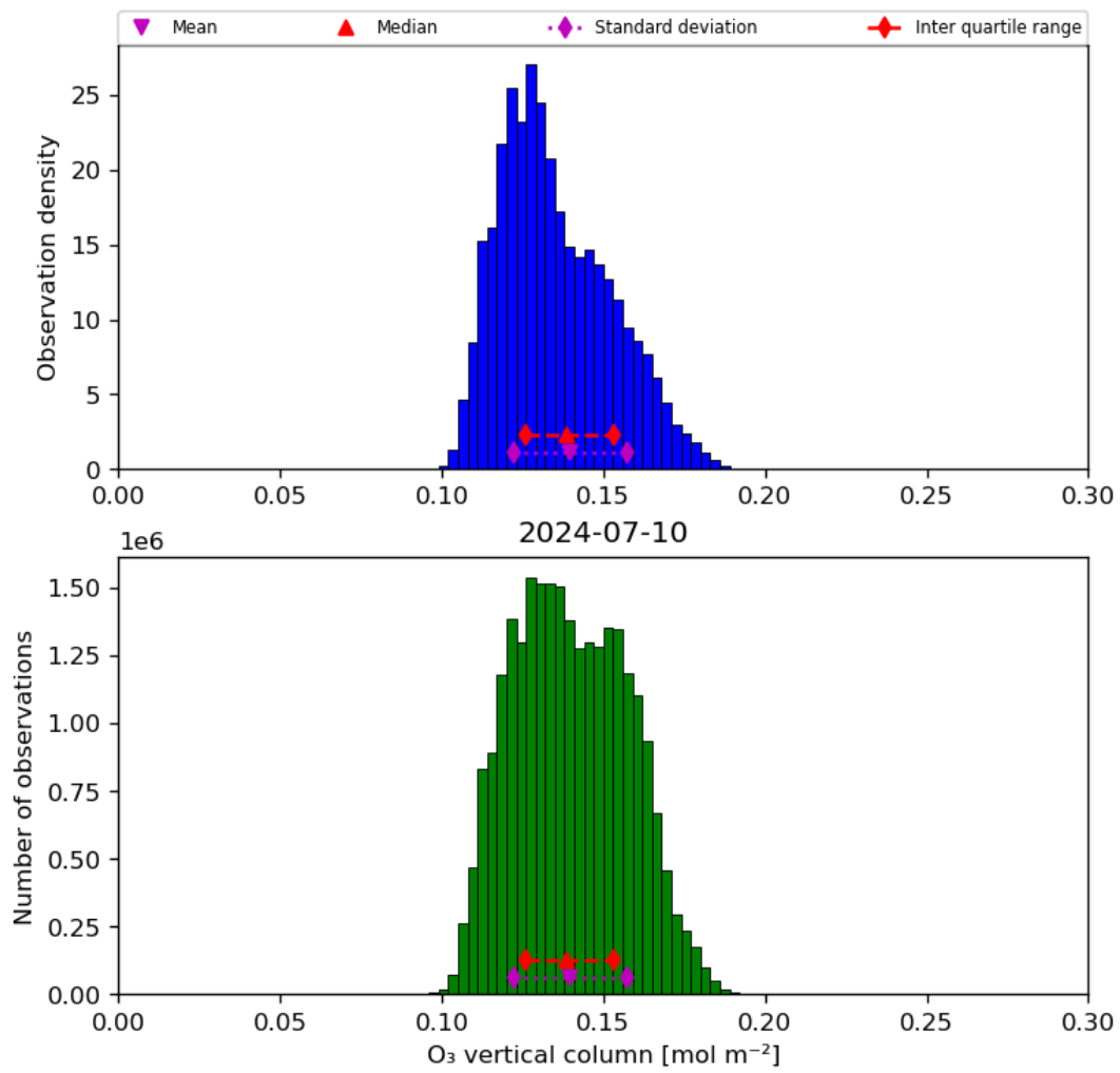
Figure 21: Histogram of “O 3 vertical column” for 2024-07-10 to 2024-07-11
