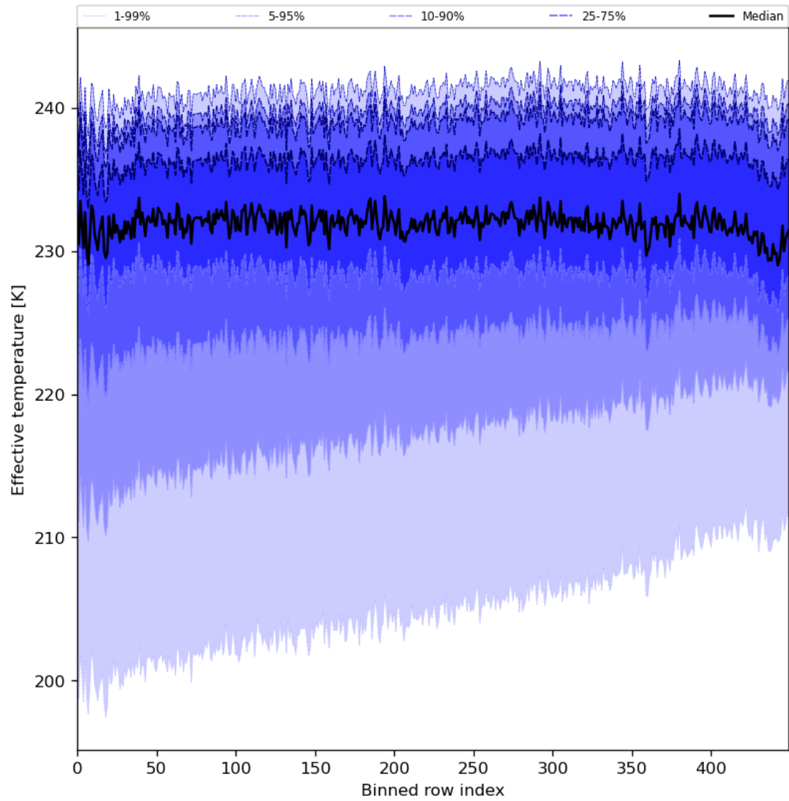
Figure 31: Along track statistics of “Effective temperature” for 2024-07-10 to 2024-07-11
