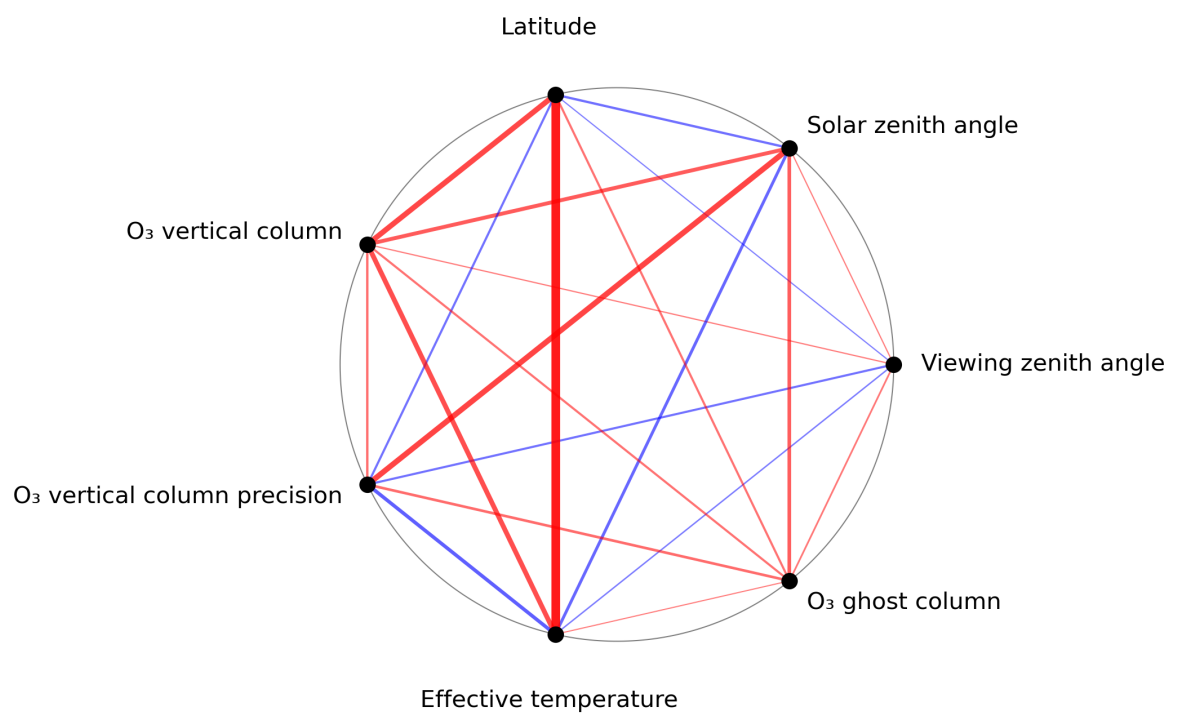
Figure 1: Map of correlation graph for 2024-07-10 to 2024-07-11.
