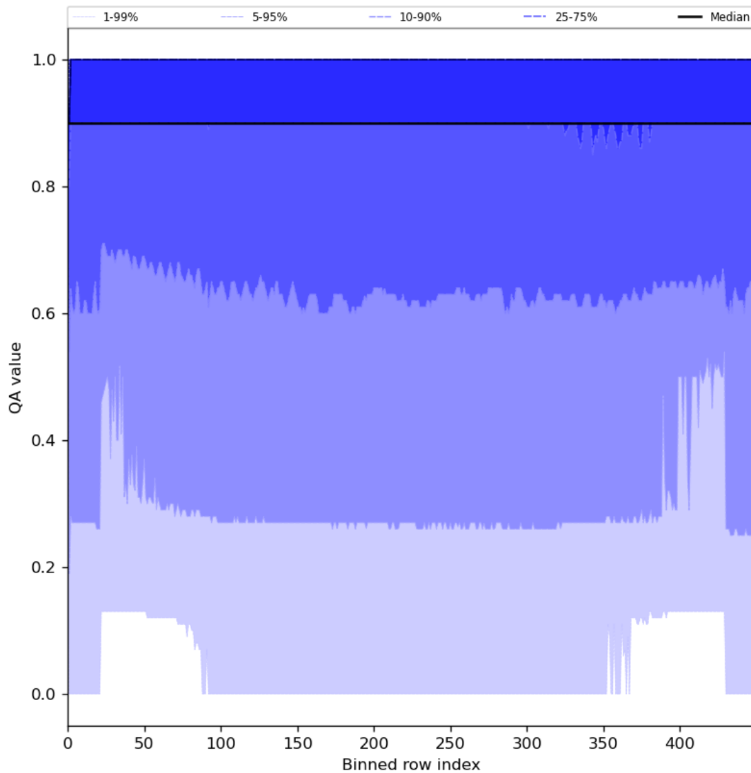
Figure 27: Along track statistics of “QA value” for 2024-07-10 to 2024-07-11
