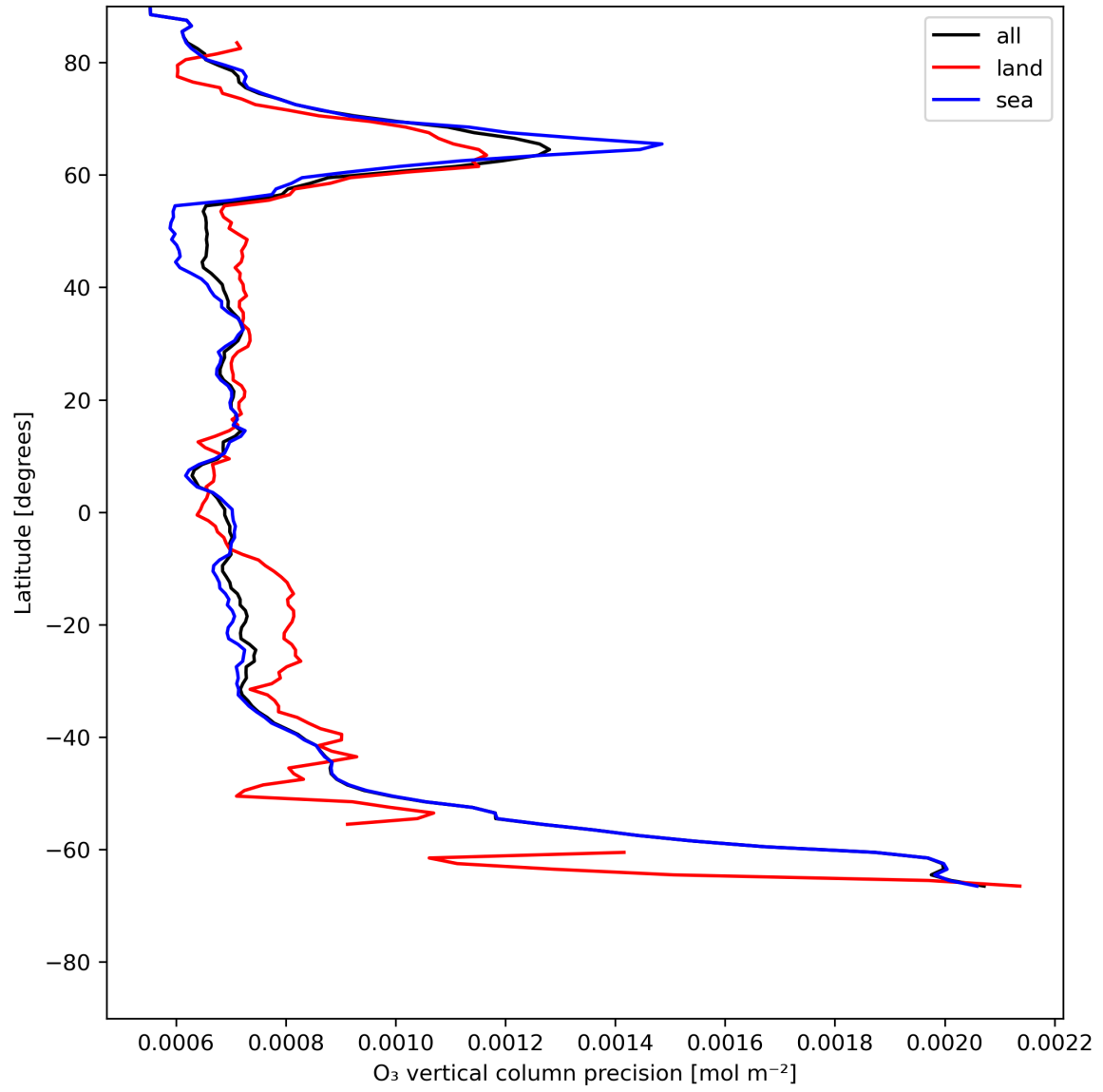
Figure 15: Zonal average of “O 3 vertical column precision” for 2024-07-10 to 2024-07-11.
