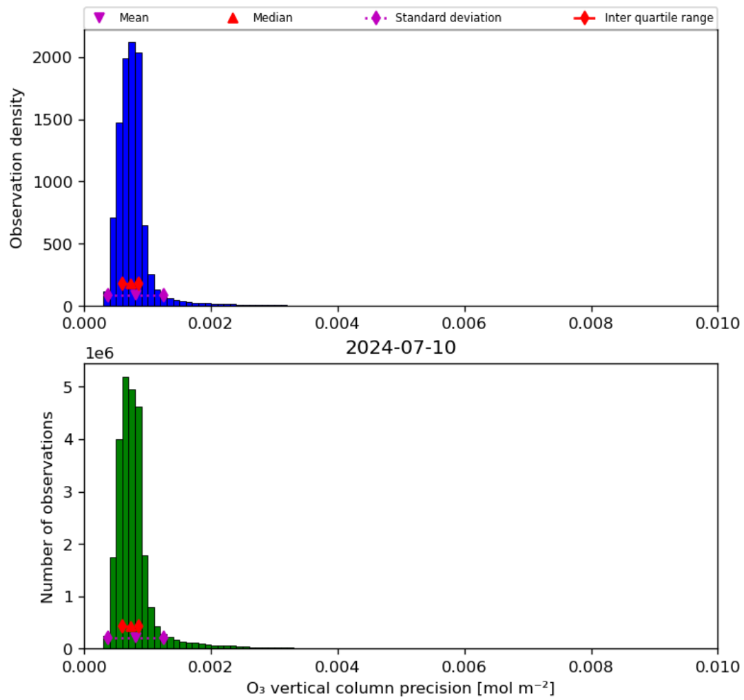
Figure 22: Histogram of “O 3 vertical column precision” for 2024-07-10 to 2024-07-11
