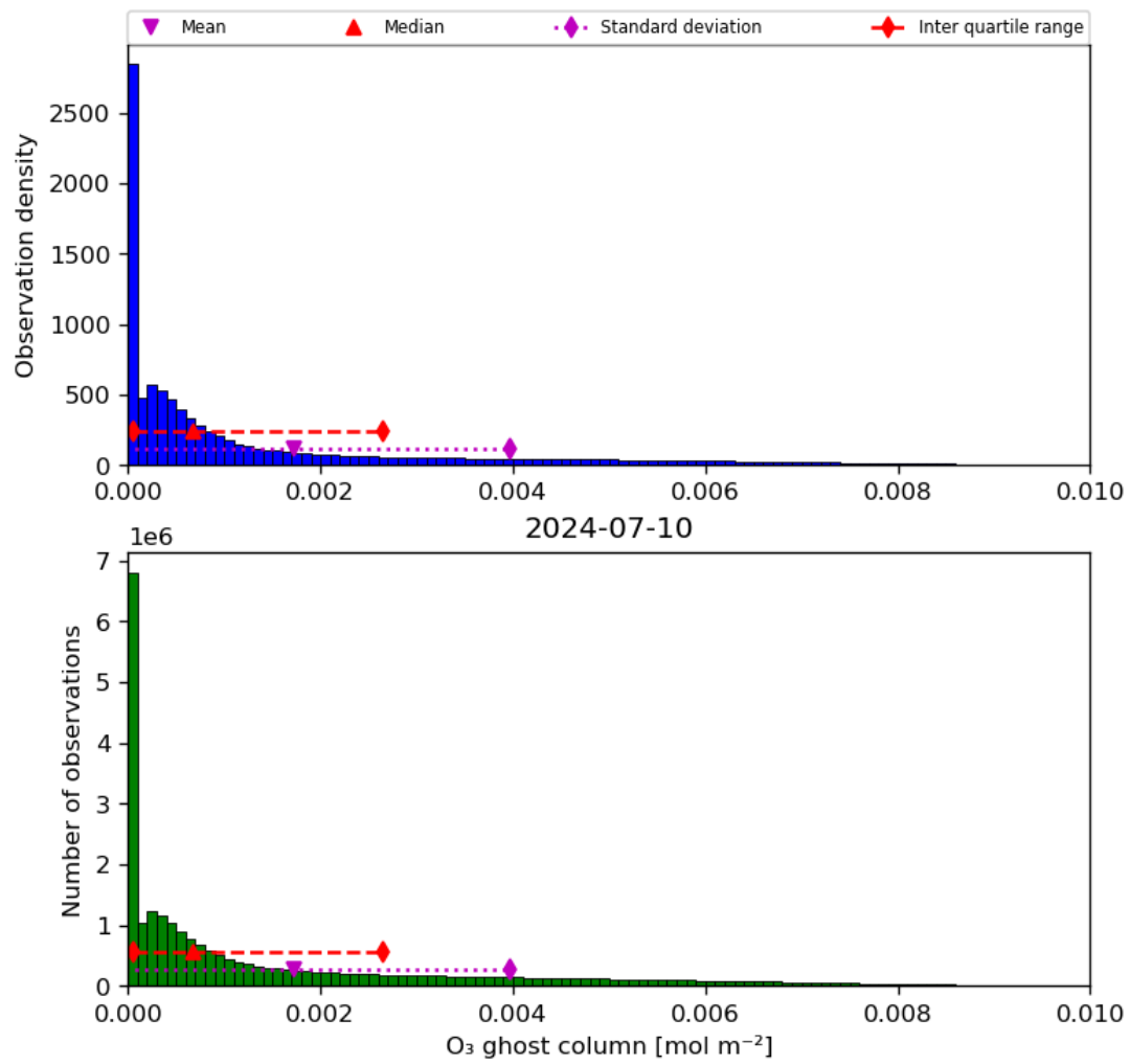
Figure 25: Histogram of “O 3 ghost column” for 2024-07-10 to 2024-07-11
