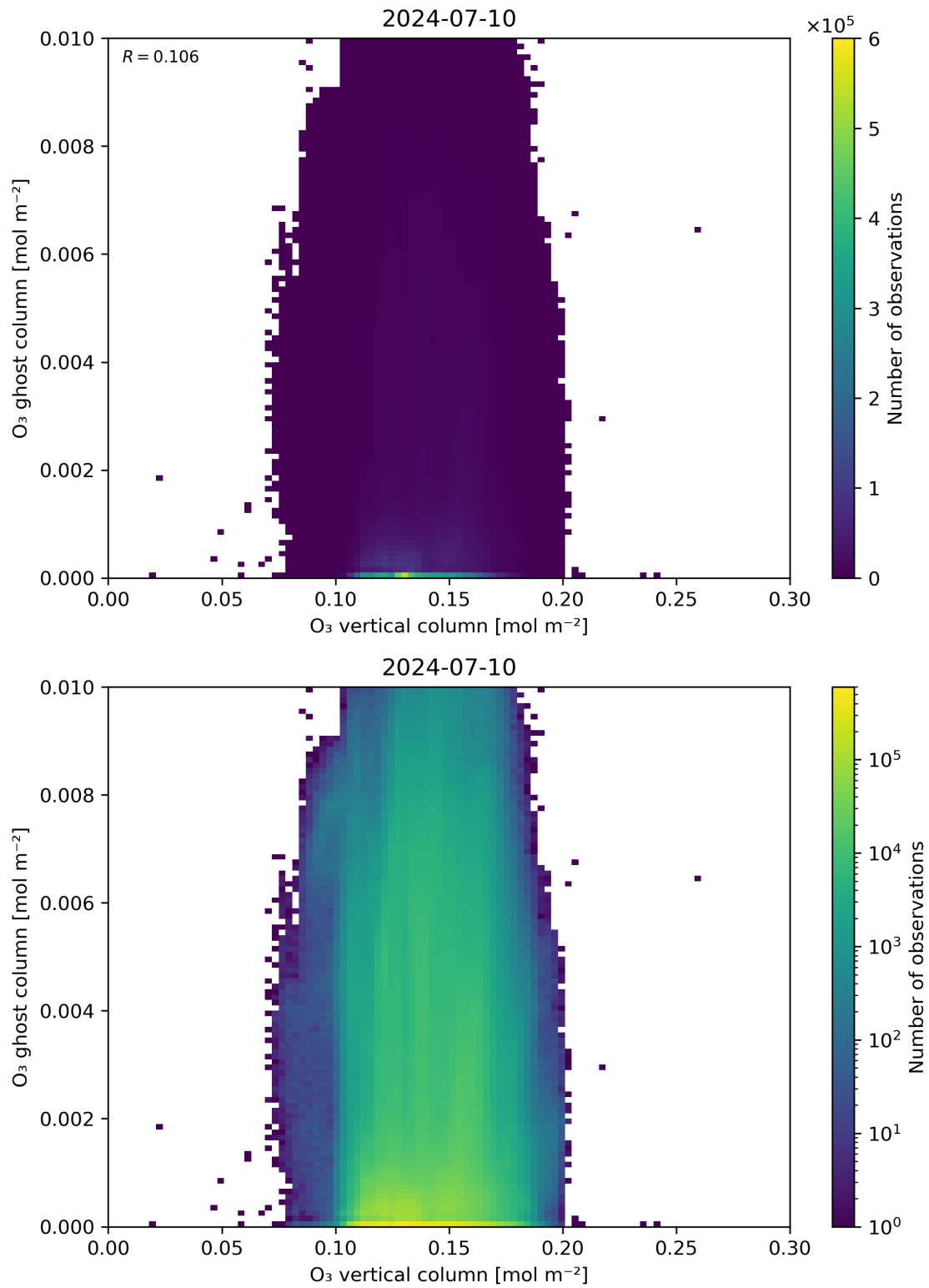
Figure 40: Scatter density plot of “O 3 vertical column” against “O 3 ghost column” for 2024-07-10 to 2024-07-11.
