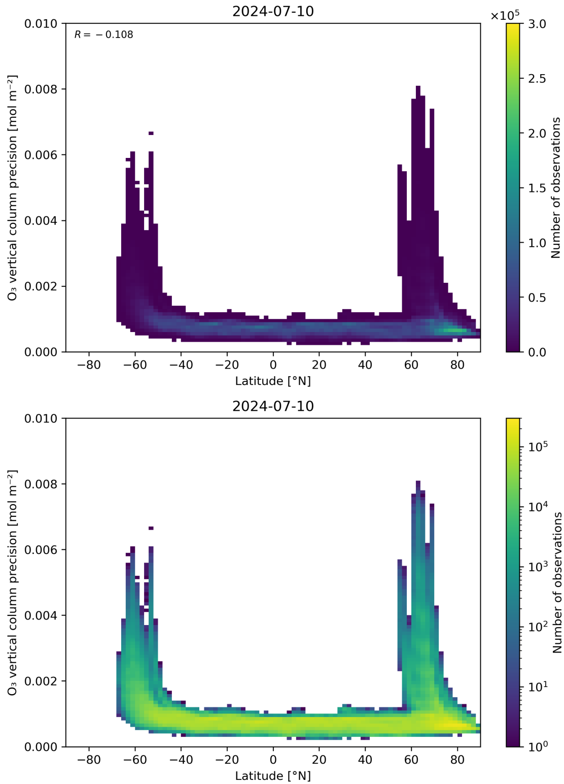
Figure 37: Scatter density plot of “Latitude” against “O 3 vertical column precision” for 2024-07-10 to 2024-07-11.
