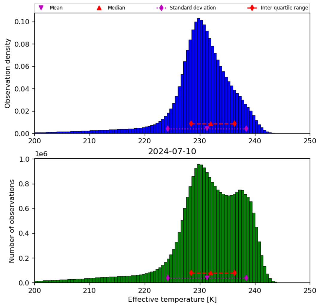
Figure 24: Histogram of “Effective temperature” for 2024-07-10 to 2024-07-11
