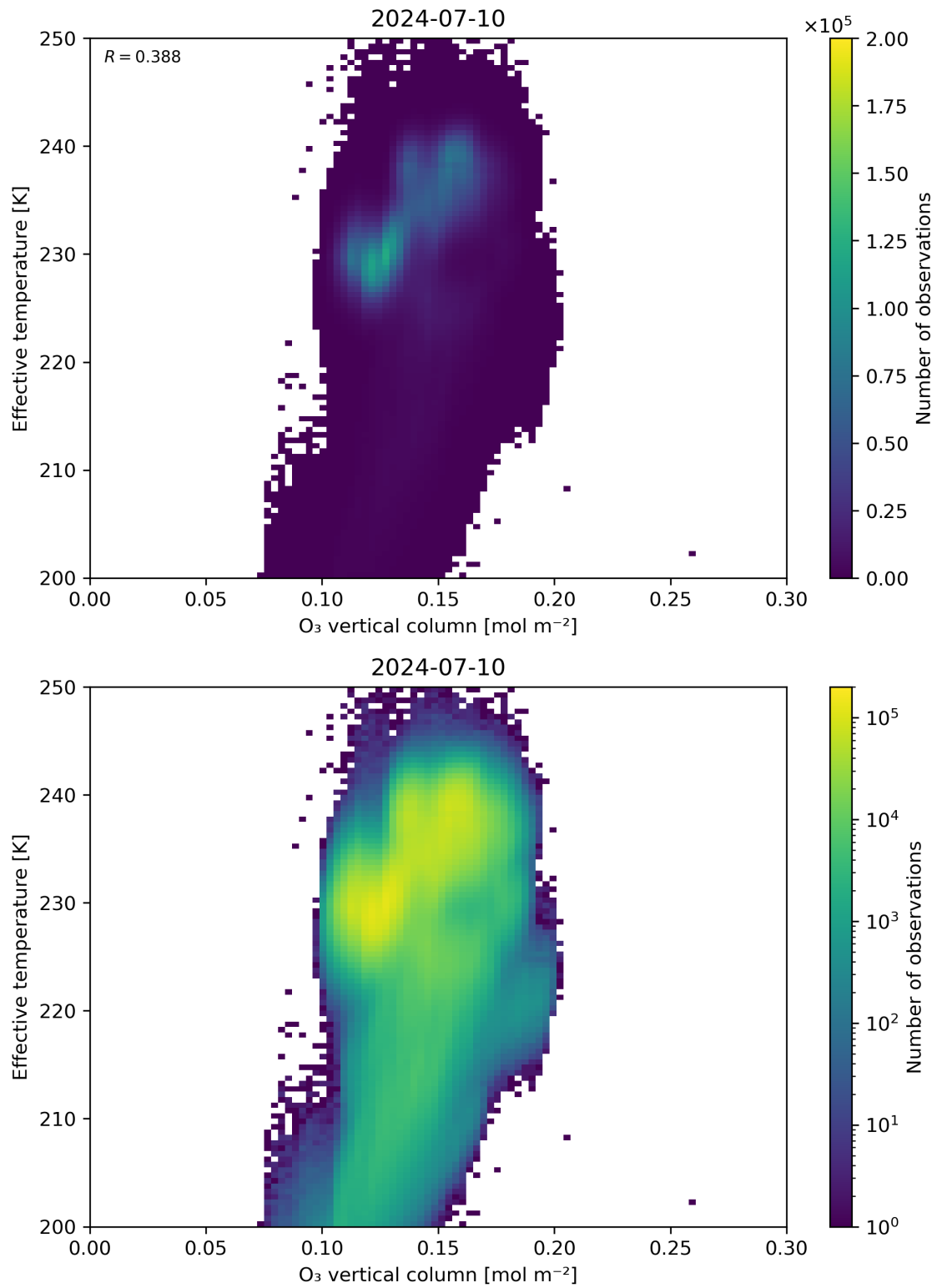
Figure 39: Scatter density plot of “O 3 vertical column” against “Effective temperature” for 2024-07-10 to 2024-07-11.
