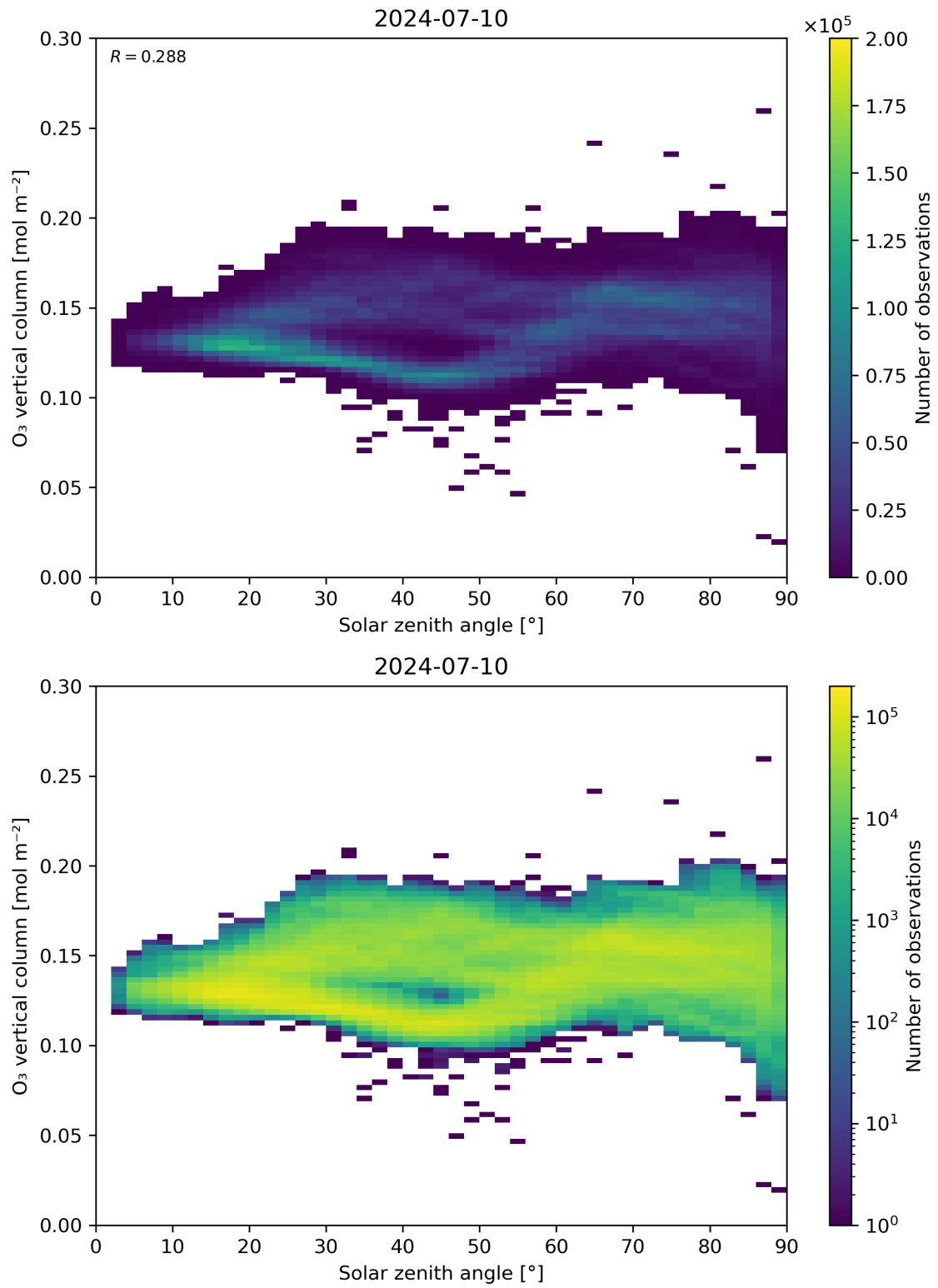
Figure 47: Scatter density plot of “Solar zenith angle” against “O 3 vertical column” for 2024-07-10 to 2024-07-11.
