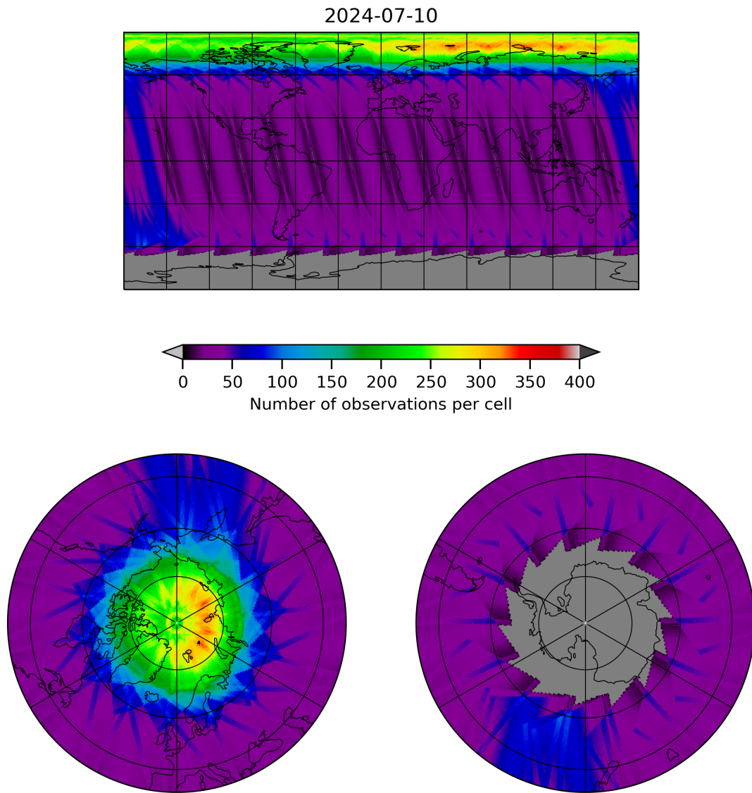
Figure 12: Map of the number of observations for 2024-07-10 to 2024-07-11
