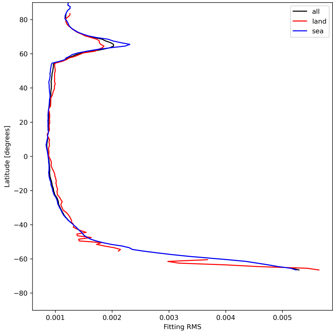
Figure 16: Zonal average of “Fitting RMS” for 2024-07-10 to 2024-07-11.
