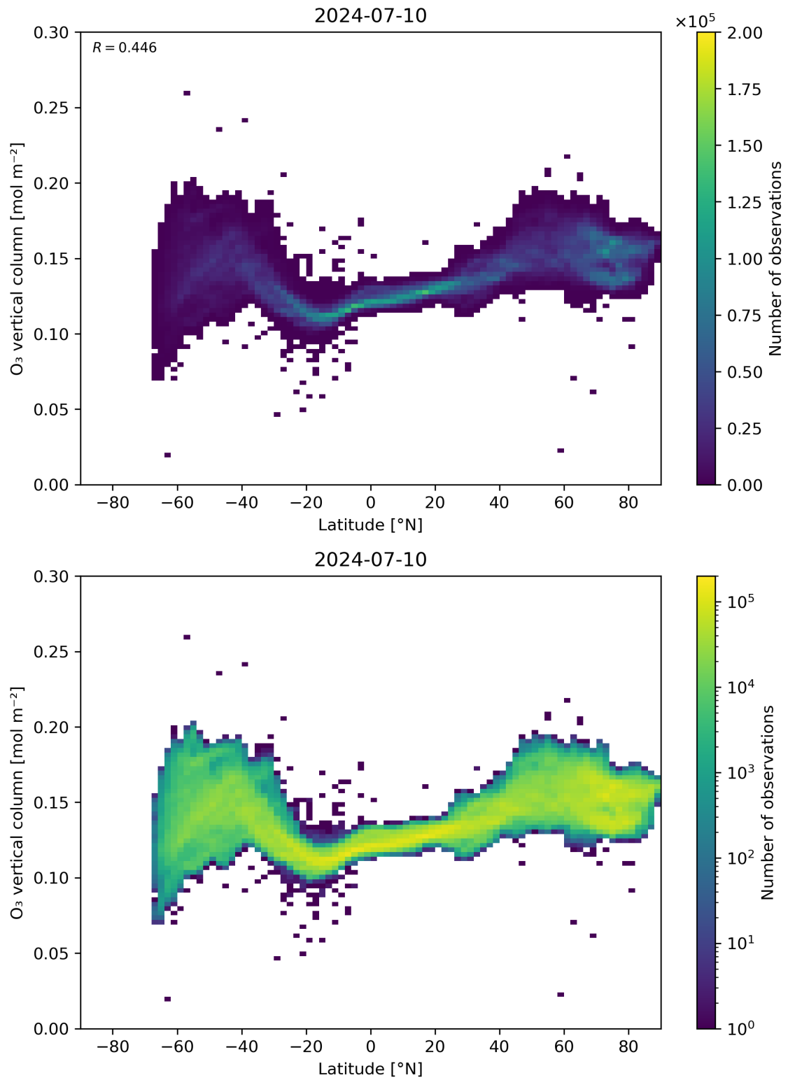
Figure 36: Scatter density plot of “Latitude” against “O 3 vertical column” for 2024-07-10 to 2024-07-11.
