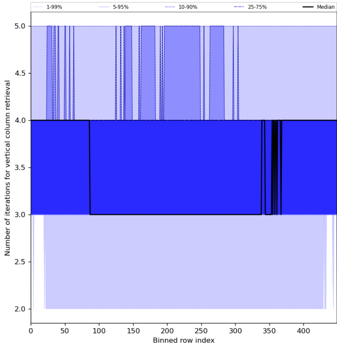
Figure 33: Along track statistics of “Number of iterations for vertical column retrieval” for 2024-07-10 to 2024-07-11
