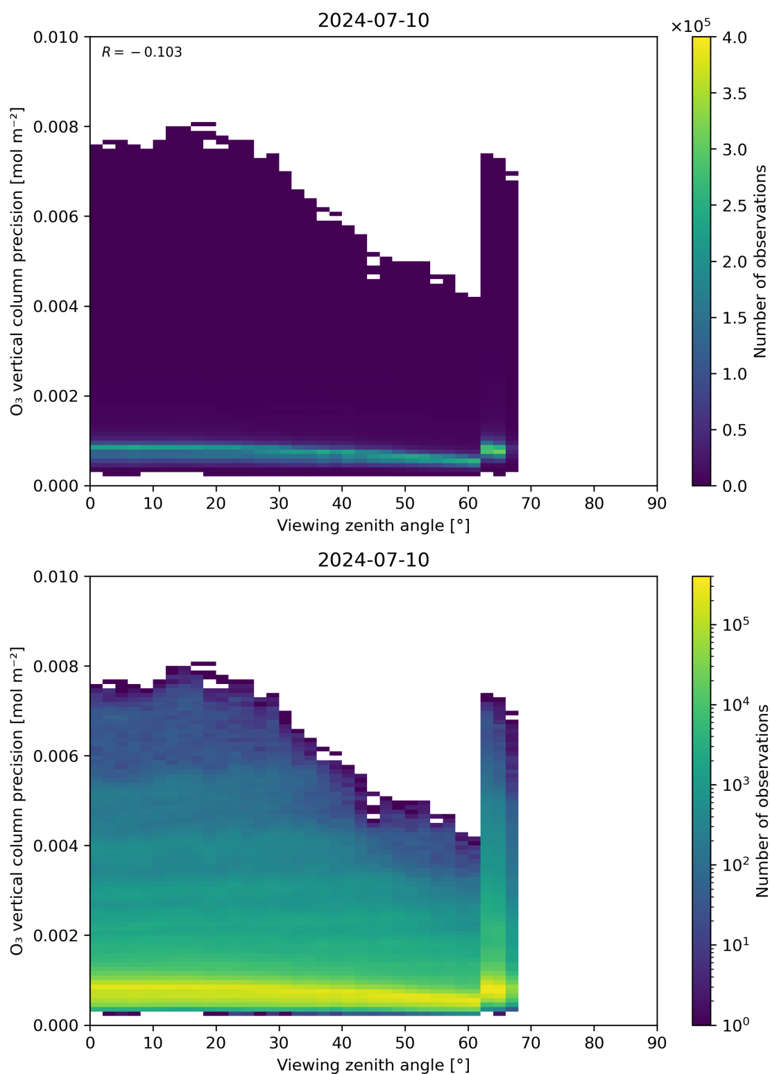
Figure 53: Scatter density plot of “Viewing zenith angle” against “O 3 vertical column precision” for 2024-07-10 to 2024-07-11.
