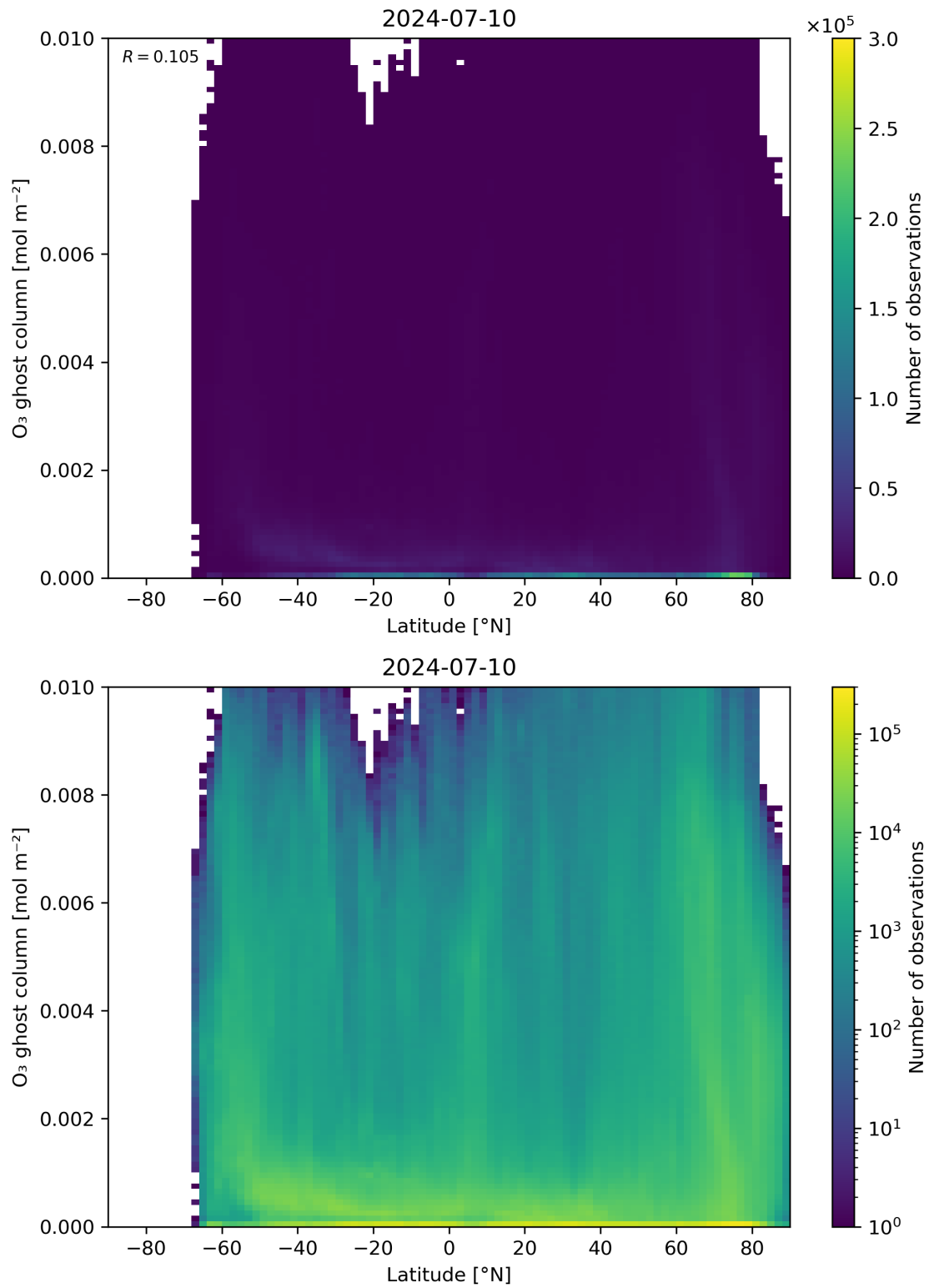
Figure 35: Scatter density plot of “Latitude” against “O 3 ghost column” for 2024-07-10 to 2024-07-11.
