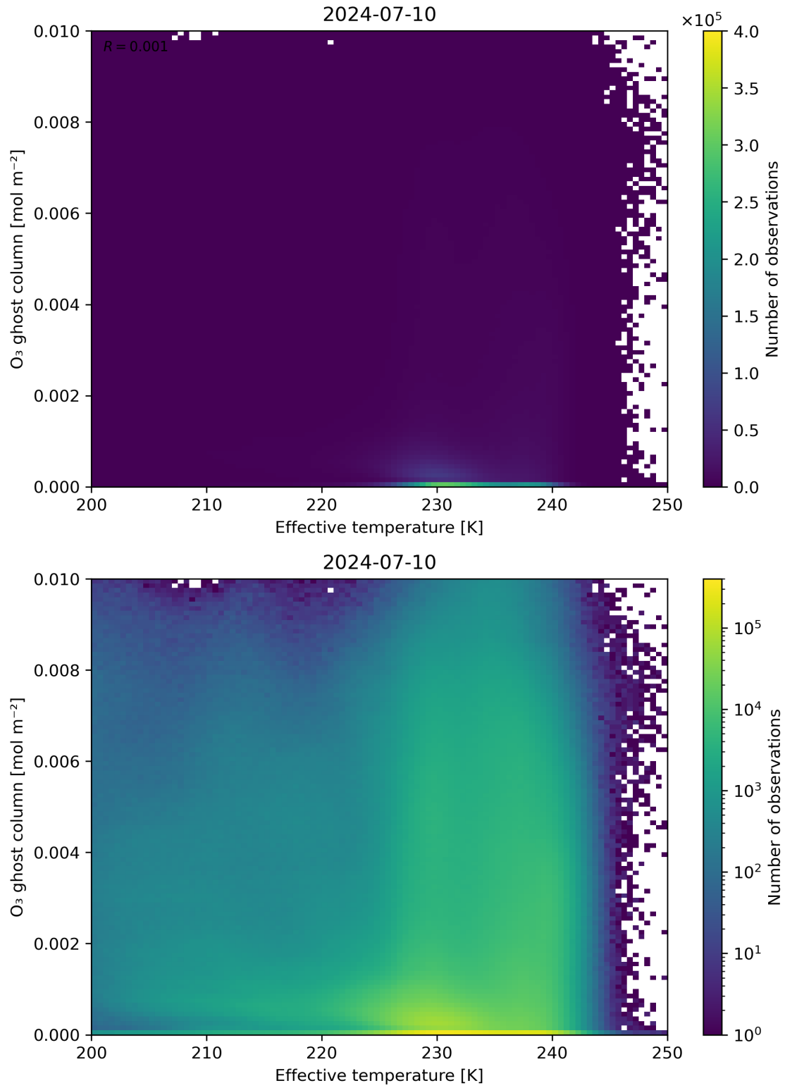
Figure 38: Scatter density plot of “Effective temperature” against “O 3 ghost column” for 2024-07-10 to 2024-07-11.
