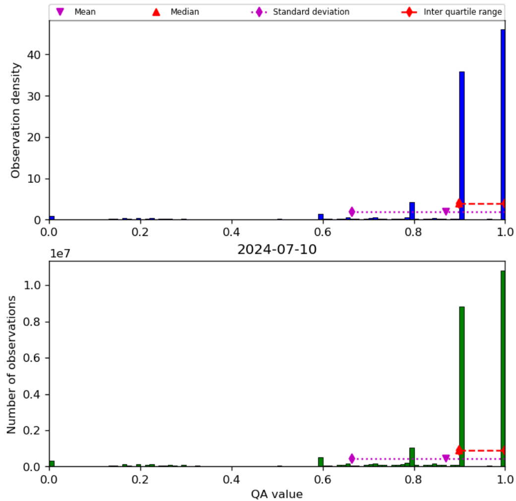
Figure 20: Histogram of “QA value” for 2024-07-10 to 2024-07-11
