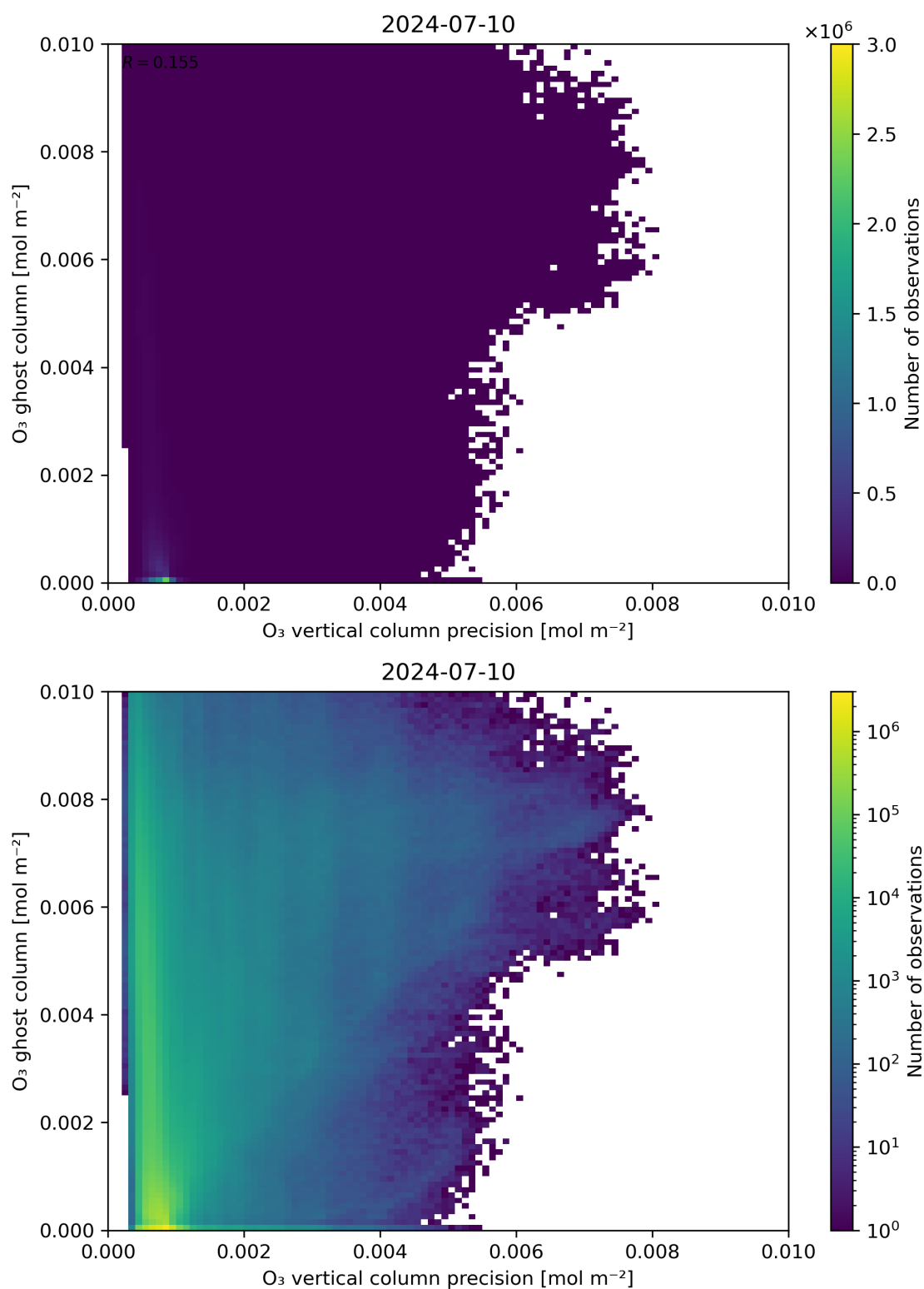
Figure 43: Scatter density plot of “ O_3 vertical column precision” against “ O_3 ghost column” for 2024-07-10 to 2024-07-11.
