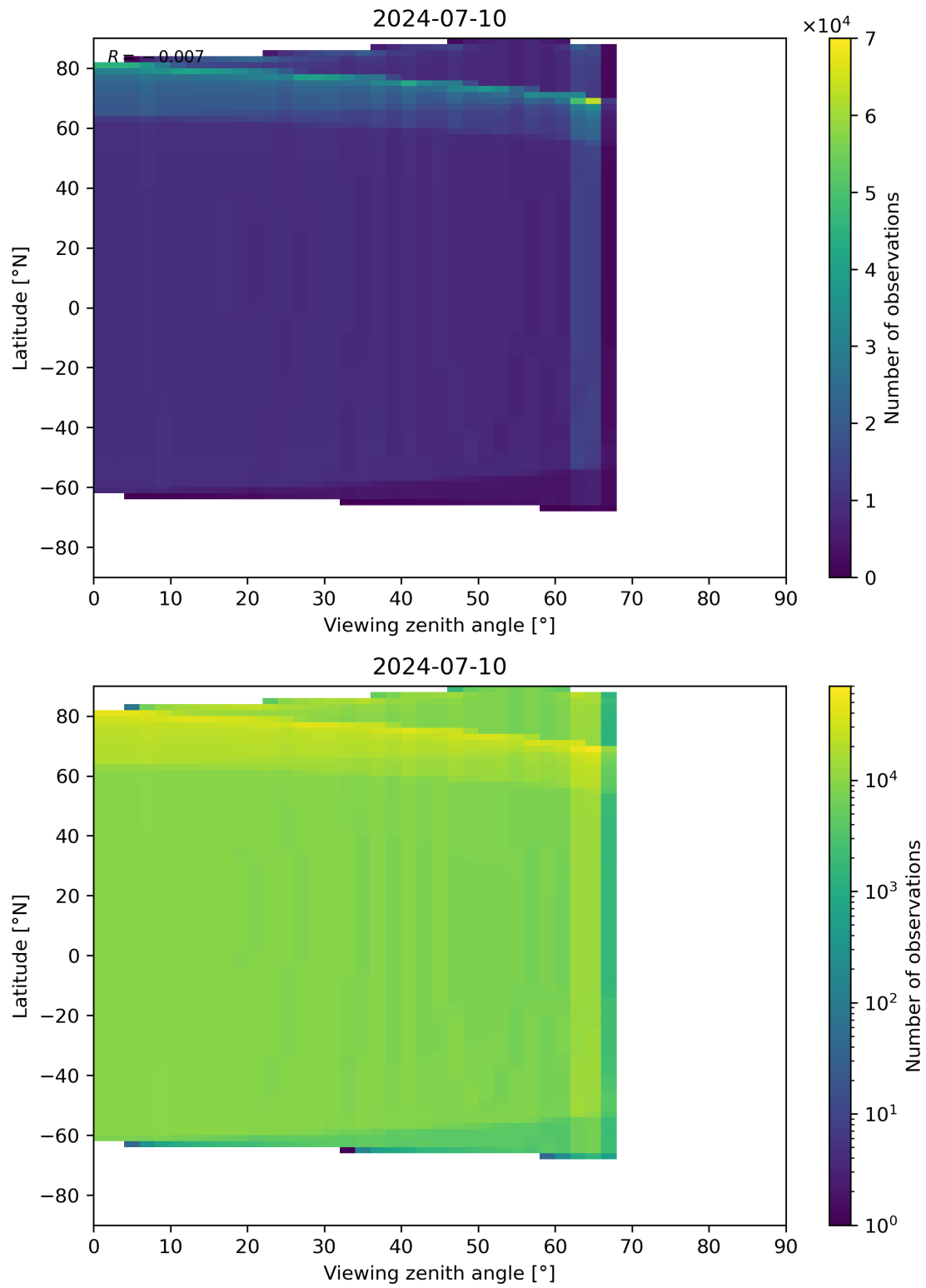
Figure 49: Scatter density plot of “Viewing zenith angle” against “Latitude” for 2024-07-10 to 2024-07-11.
