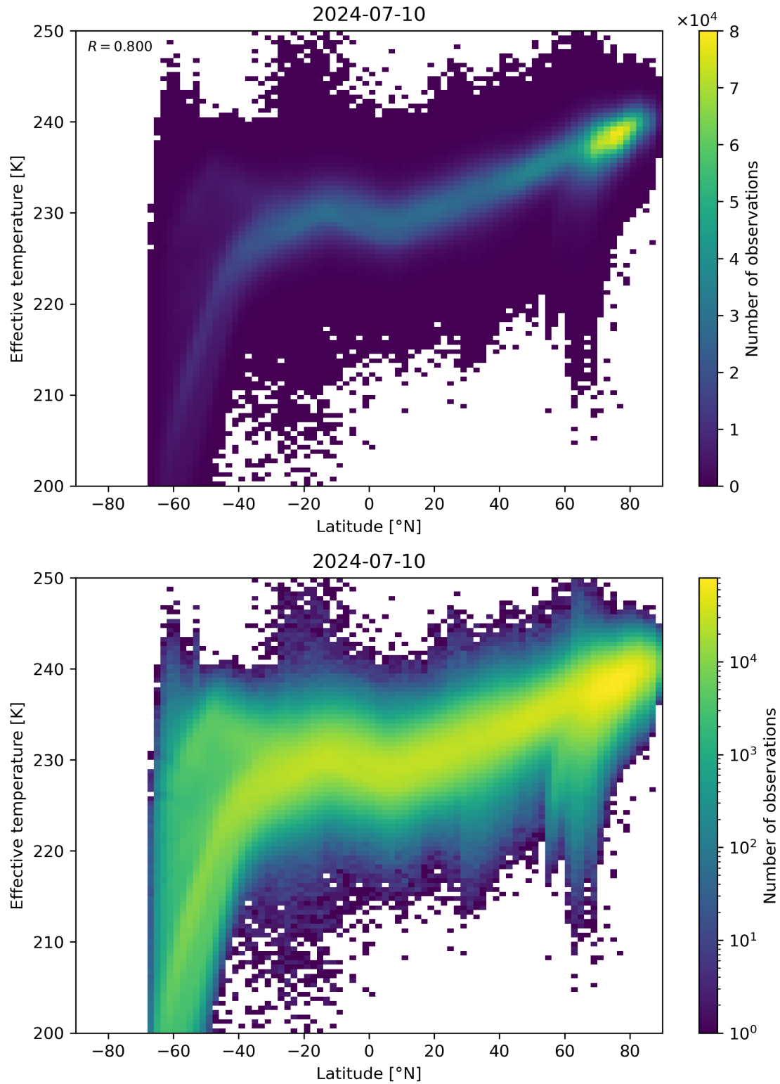
Figure 34: Scatter density plot of “Latitude” against “Effective temperature” for 2024-07-10 to 2024-07-11.
