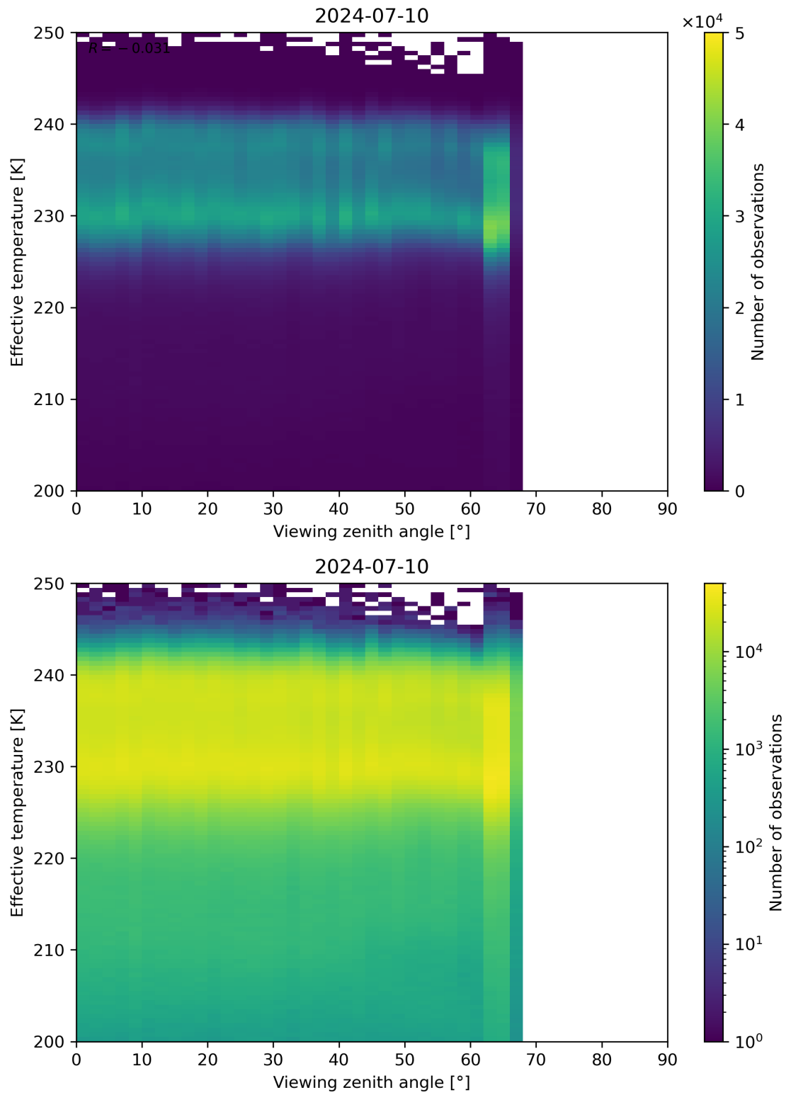
Figure 50: Scatter density plot of “Viewing zenith angle” against “Effective temperature” for 2024-07-10 to 2024-07-11.
