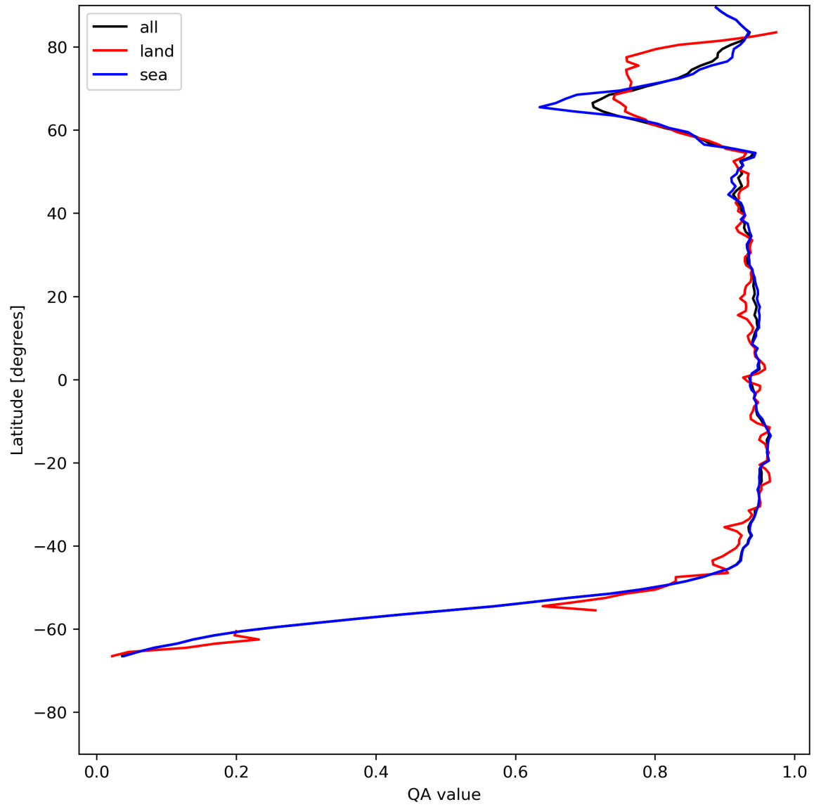
Figure 13: Zonal average of “QA value” for 2024-07-10 to 2024-07-11.
