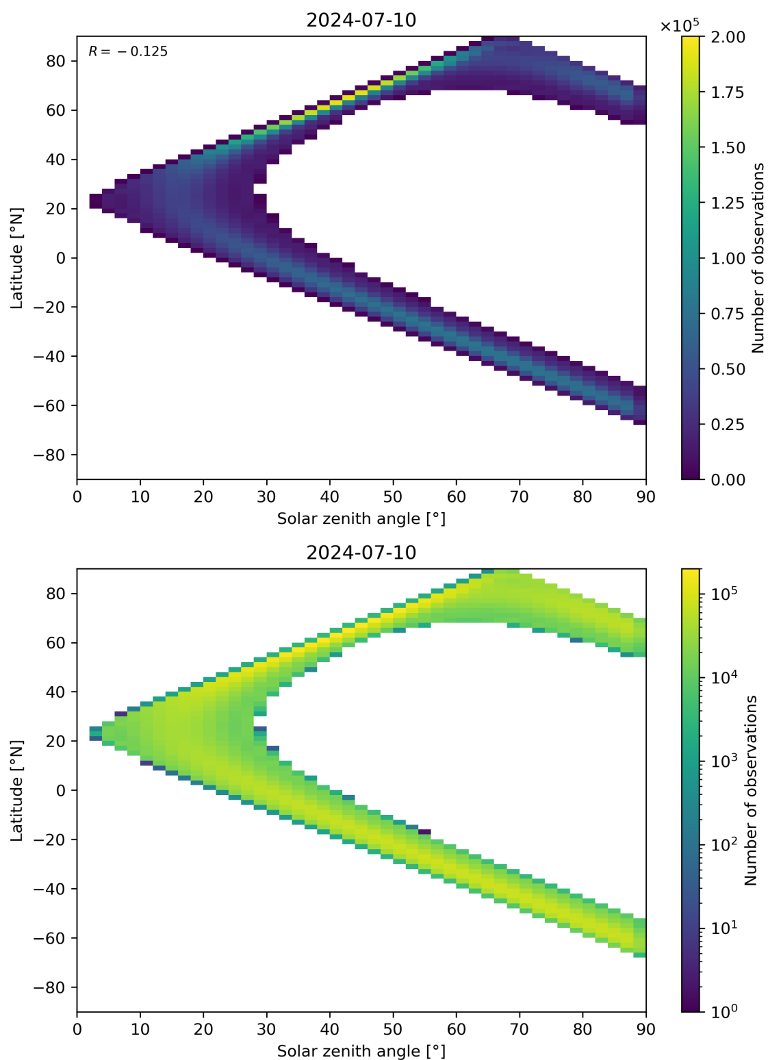
Figure 44: Scatter density plot of “Solar zenith angle” against “Latitude” for 2024-07-10 to 2024-07-11.
