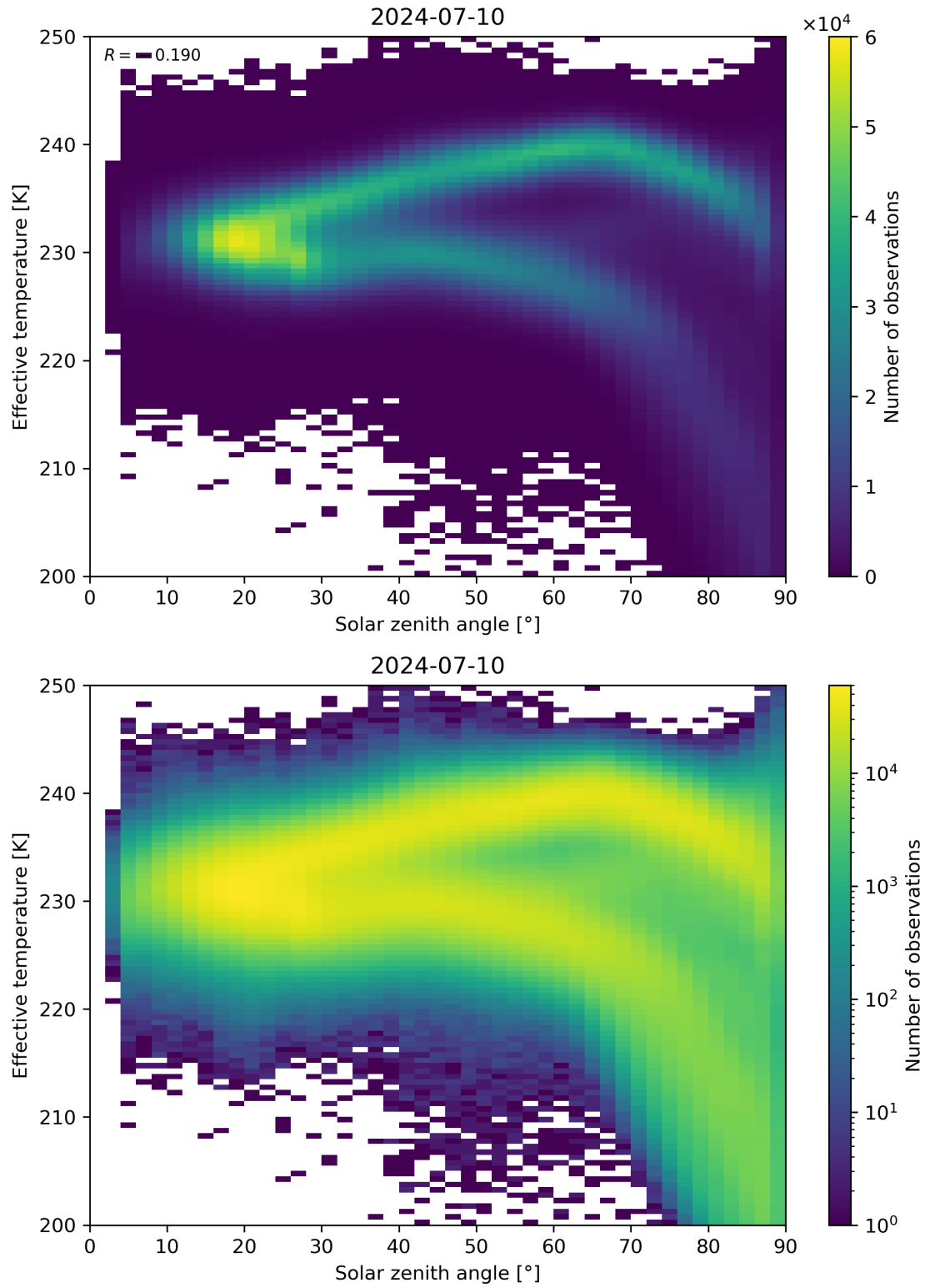
Figure 45: Scatter density plot of “Solar zenith angle” against “Effective temperature” for 2024-07-10 to 2024-07-11.
