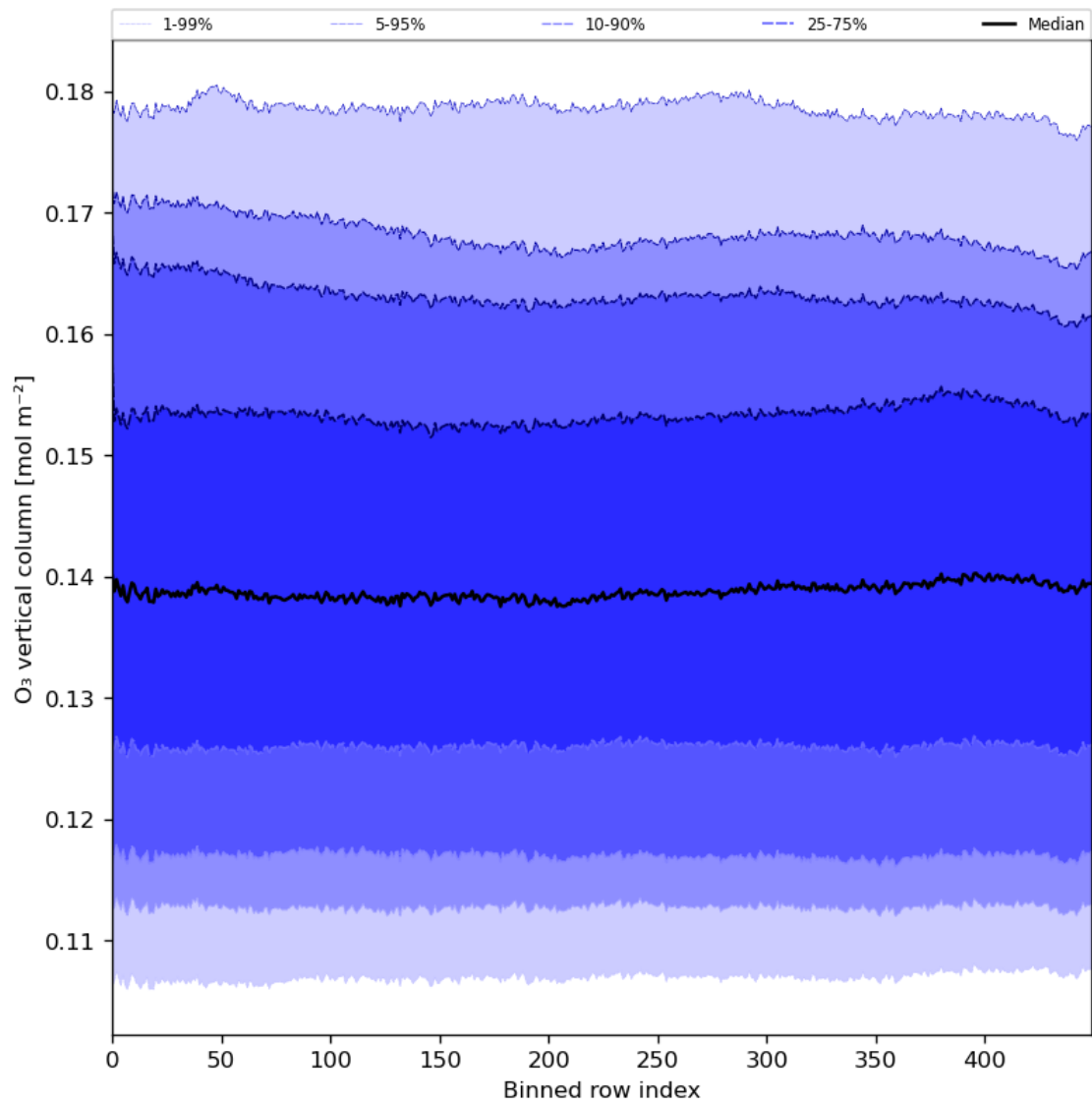
Figure 28: Along track statistics of “O 3 vertical column” for 2024-07-10 to 2024-07-11
