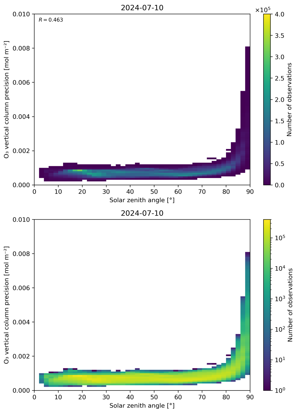
Figure 48: Scatter density plot of “Solar zenith angle” against “O 3 vertical column precision” for 2024-07-10 to 2024-07-11.
