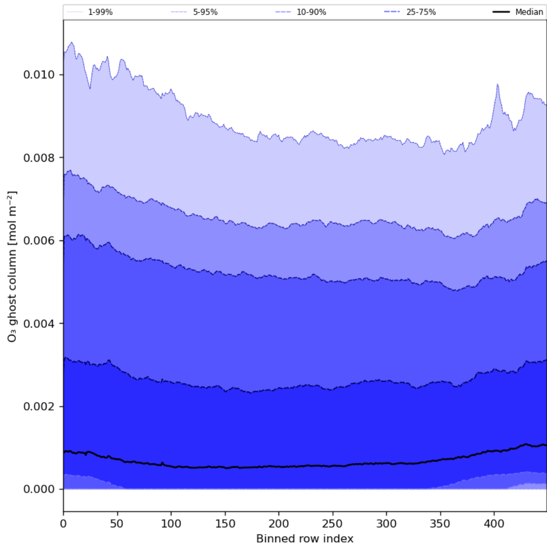
Figure 32: Along track statistics of “O 3 ghost column” for 2024-07-10 to 2024-07-11
