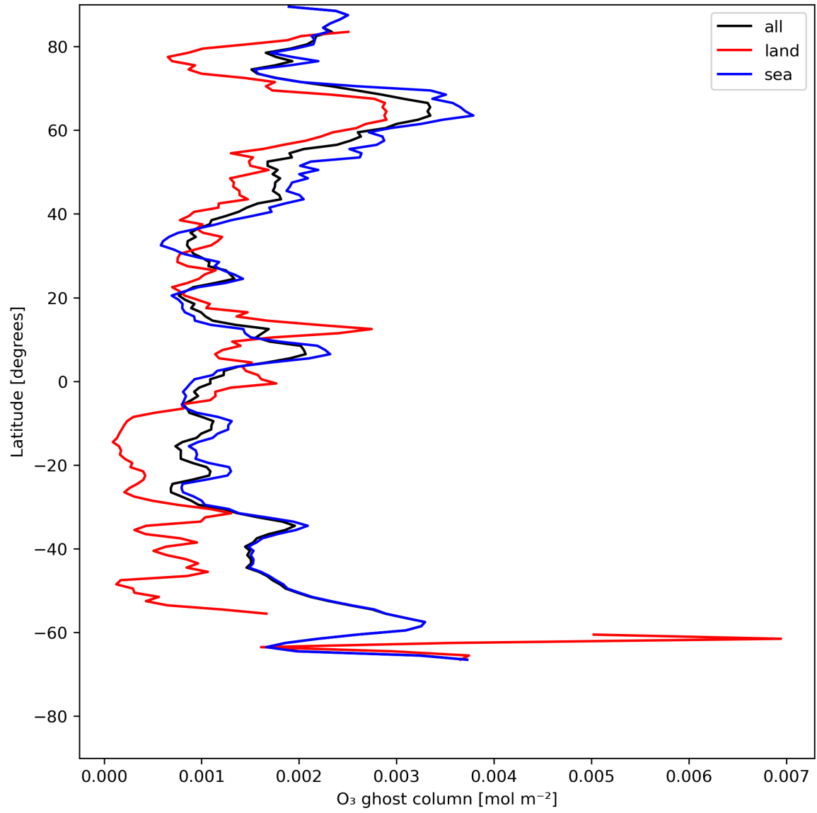
Figure 18: Zonal average of "O 3 ghost column" for 2024-07-10 to 2024-07-11.
