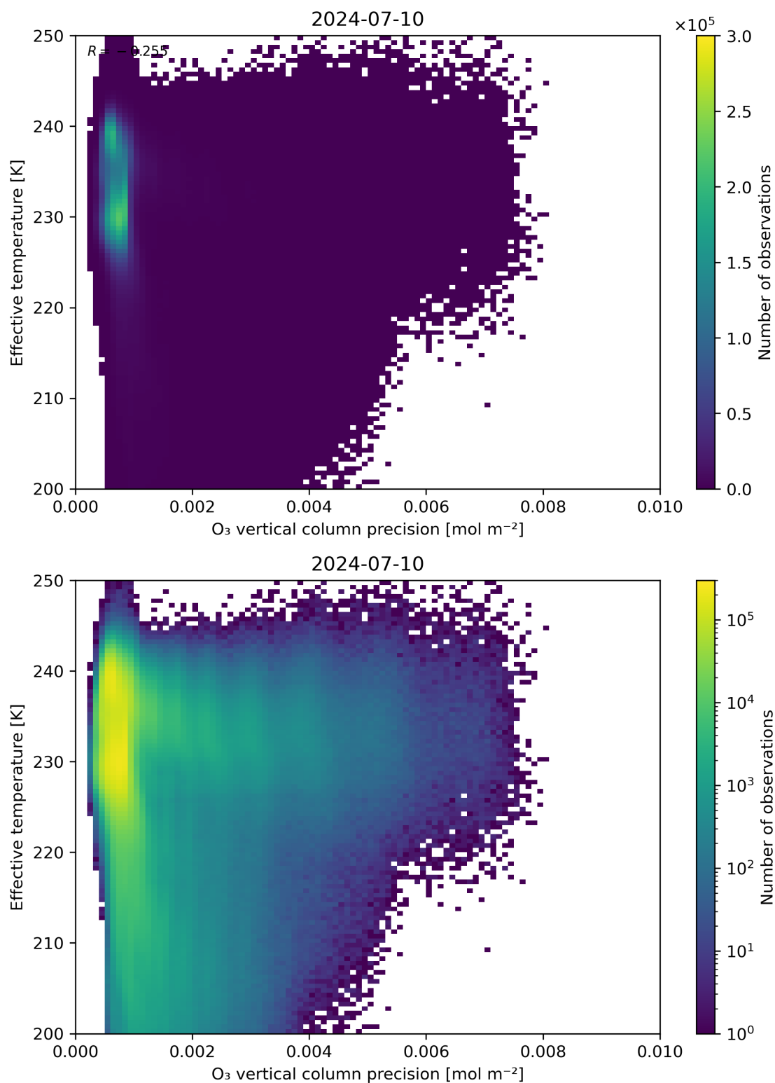
Figure 42: Scatter density plot of “O 3 vertical column precision” against “Effective temperature” for 2024-07-10 to 2024-07-11.
