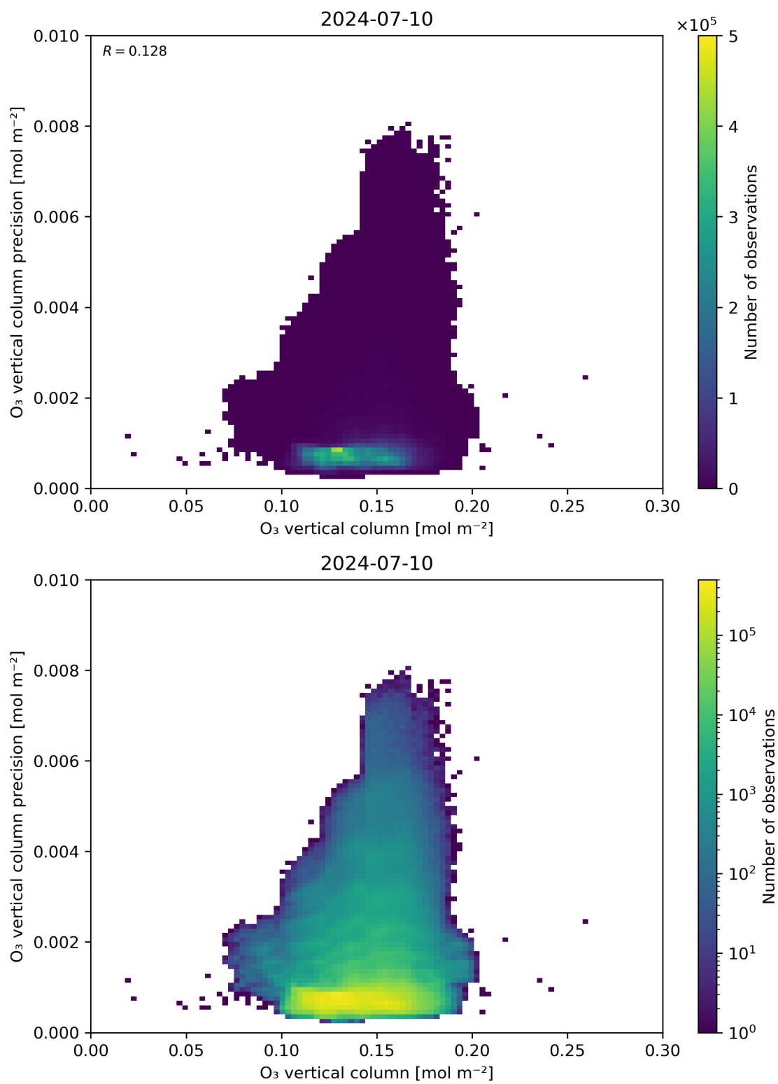
Figure 41: Scatter density plot of “O 3 vertical column” against “O 3 vertical column precision” for 2024-07-10 to 2024-07-11.
