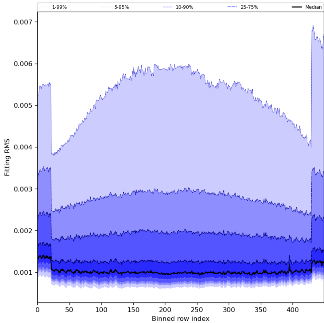
Figure 30: Along track statistics of “Fitting RMS” for 2024-07-10 to 2024-07-11
