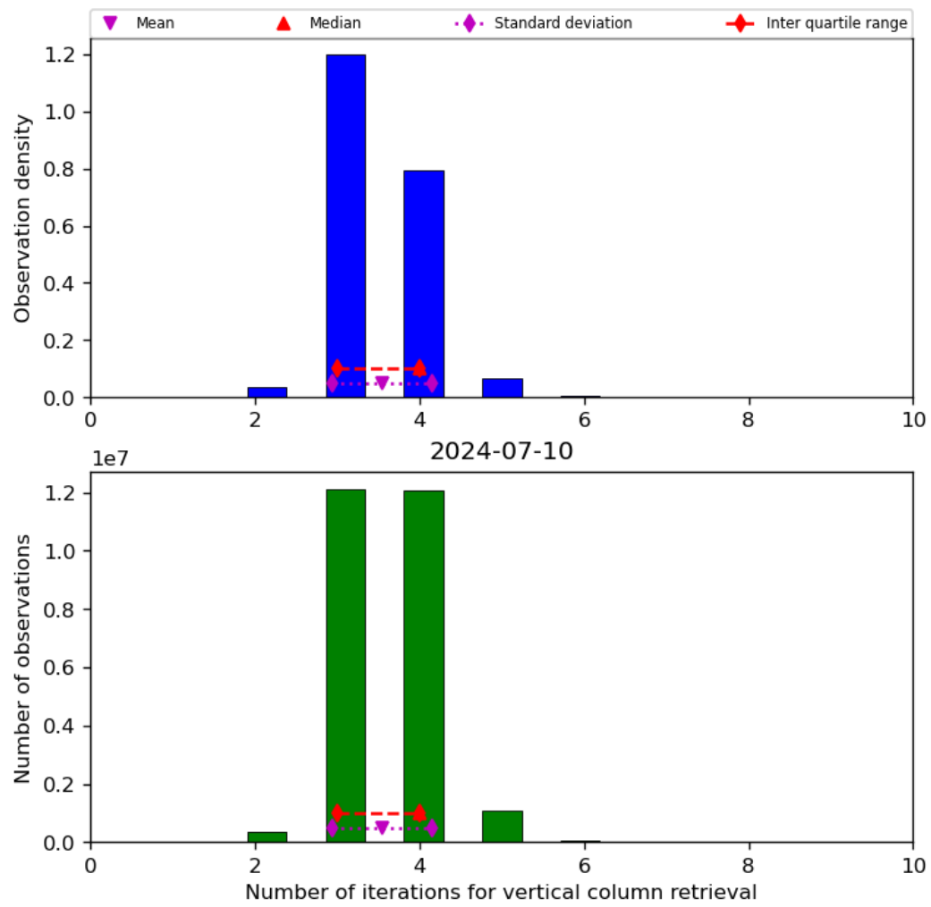
Figure 26: Histogram of “Number of iterations for vertical column retrieval” for 2024-07-10 to 2024-07-11
