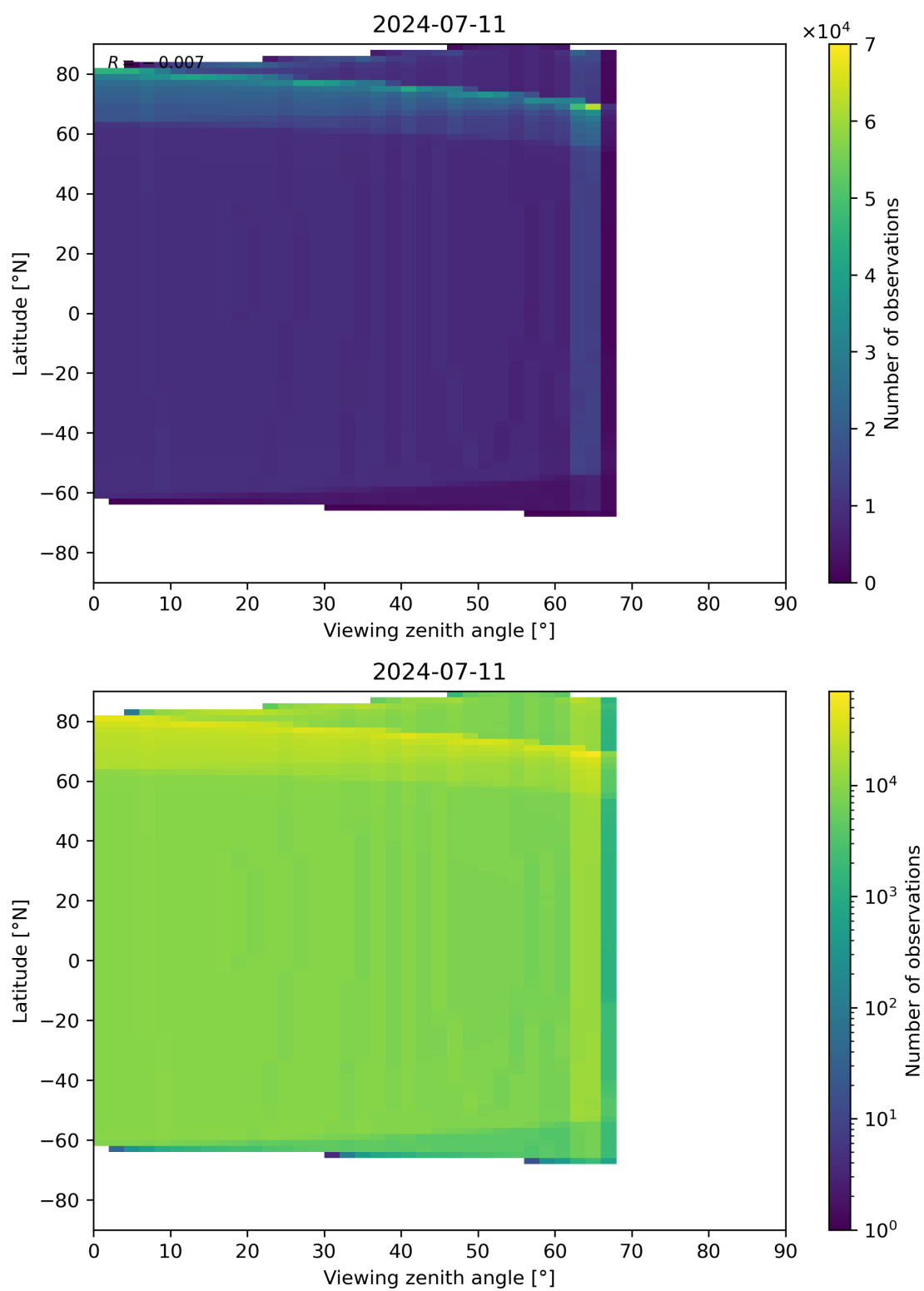
Figure 49: Scatter density plot of “Viewing zenith angle” against “Latitude” for 2024-07-10 to 2024-07-12.
