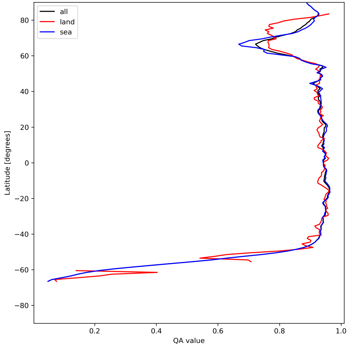
Figure 13: Zonal average of “QA value” for 2024-07-10 to 2024-07-12.
