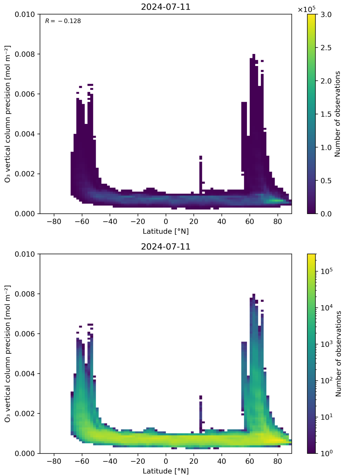
Figure 37: Scatter density plot of “Latitude” against “O 3 vertical column precision” for 2024-07-10 to 2024-07-12.
