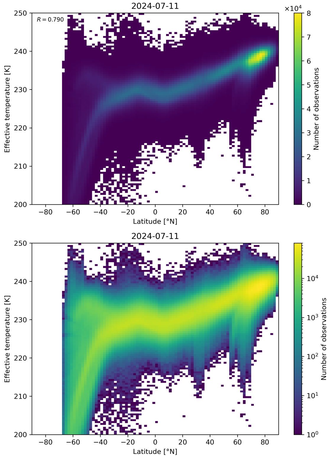
Figure 34: Scatter density plot of “Latitude” against “Effective temperature” for 2024-07-10 to 2024-07-12.
