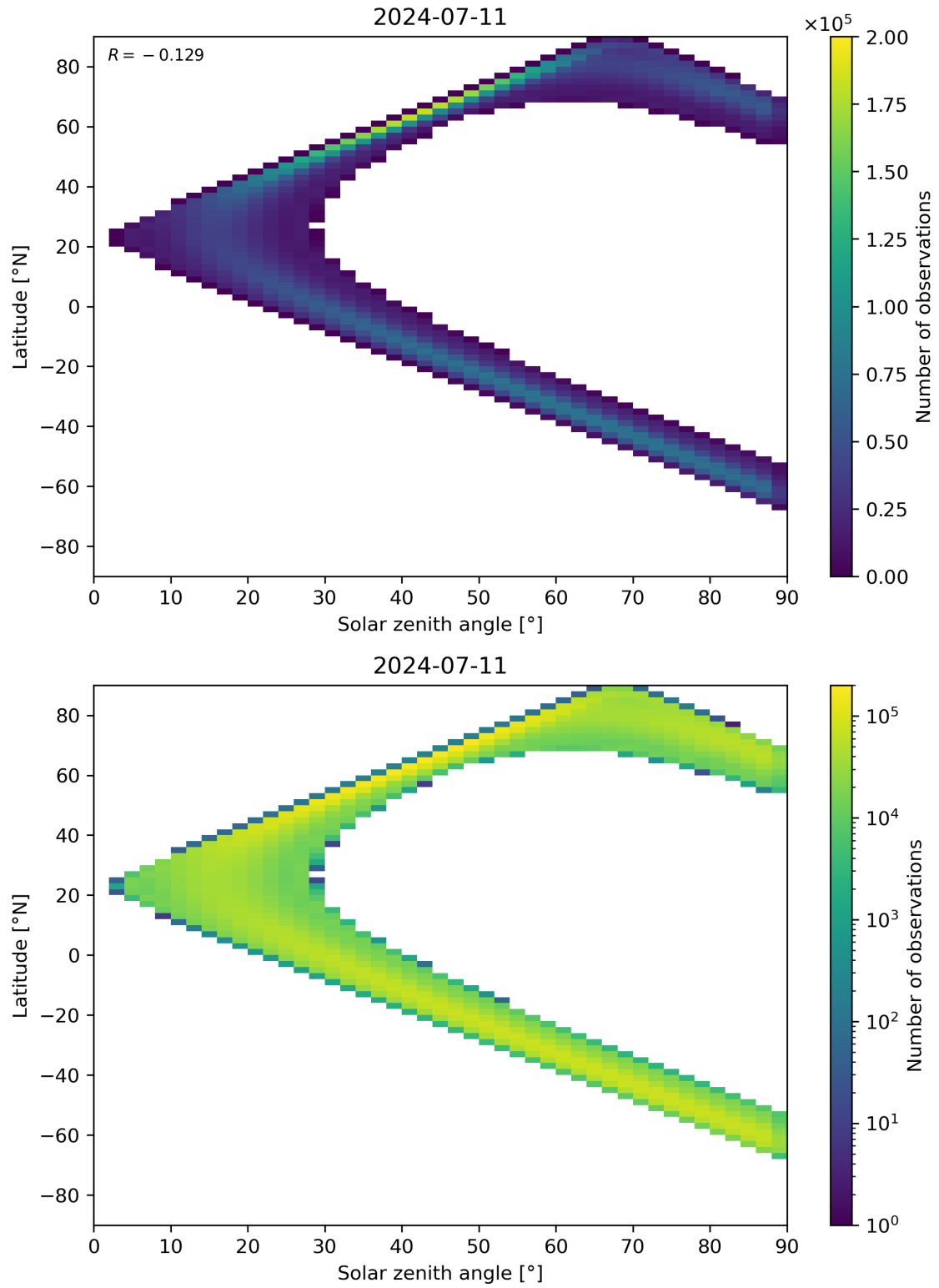
Figure 44: Scatter density plot of “Solar zenith angle” against “Latitude” for 2024-07-10 to 2024-07-12.
