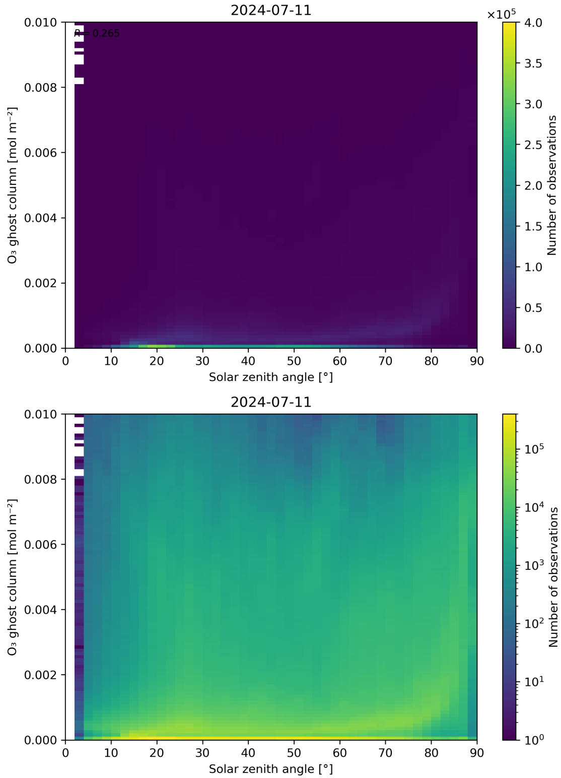
Figure 46: Scatter density plot of “Solar zenith angle” against “O 3 ghost column” for 2024-07-10 to 2024-07-12.
