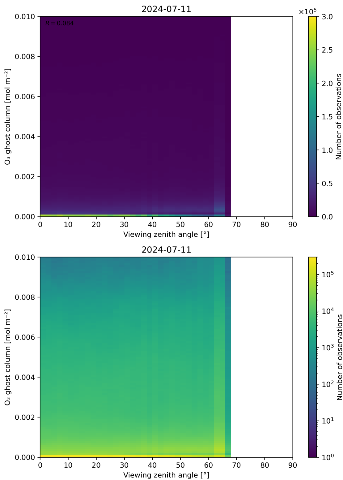
Figure 51: Scatter density plot of “Viewing zenith angle” against “O 3 ghost column” for 2024-07-10 to 2024-07-12.
