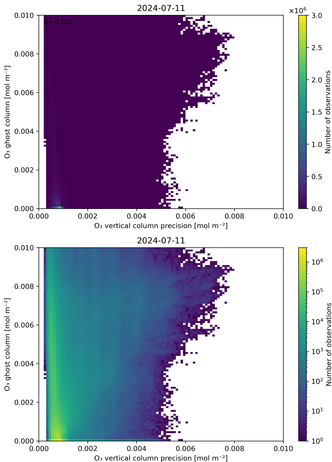
Figure 43: Scatter density plot of “ \text{O}_3 vertical column precision” against “ \text{O}_3 ghost column” for 2024-07-10 to 2024-07-12.
