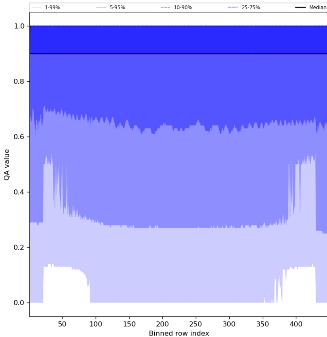
Figure 27: Along track statistics of “QA value” for 2024-07-10 to 2024-07-12
