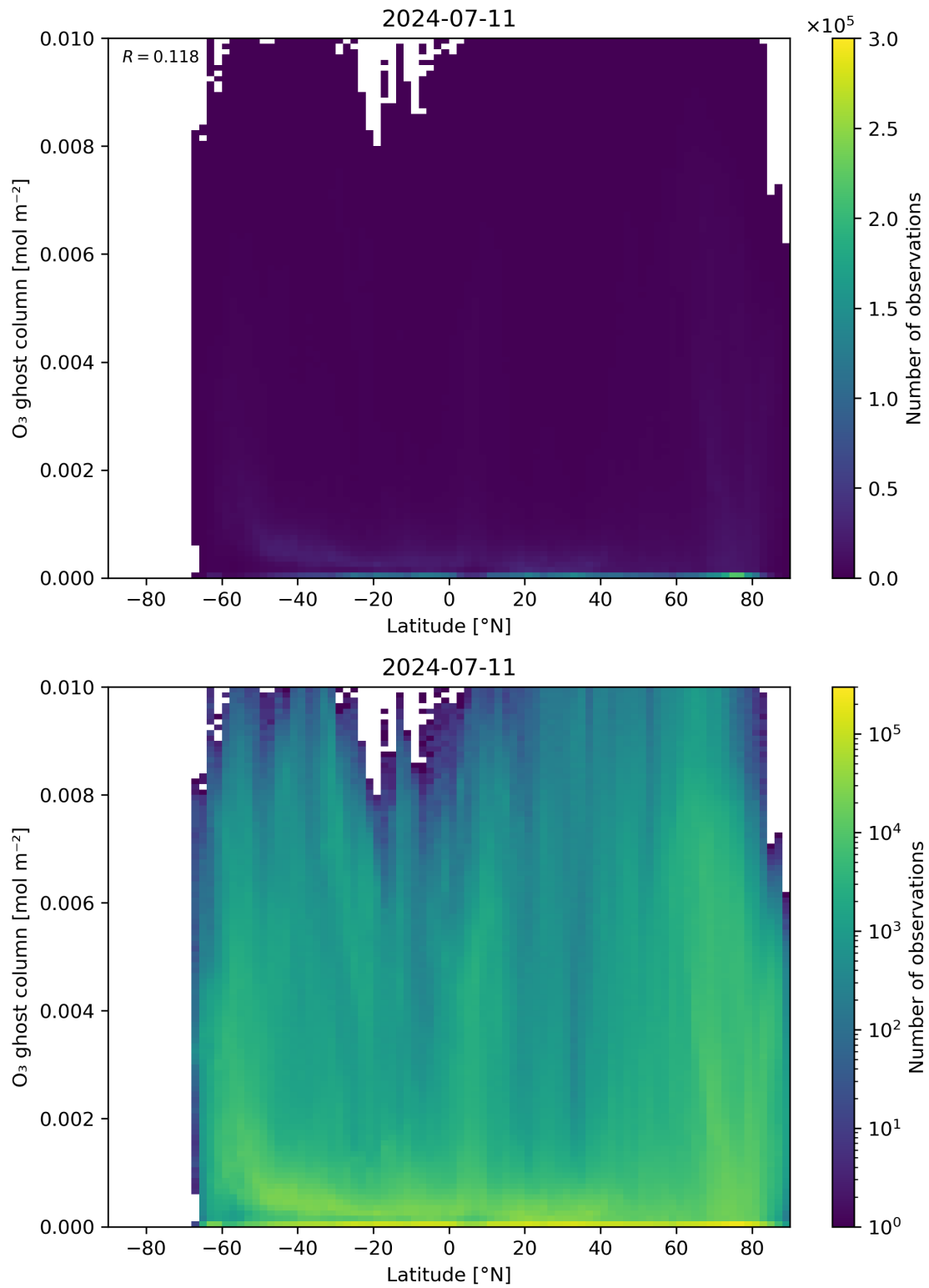
Figure 35: Scatter density plot of “Latitude” against “O 3 ghost column” for 2024-07-10 to 2024-07-12.
