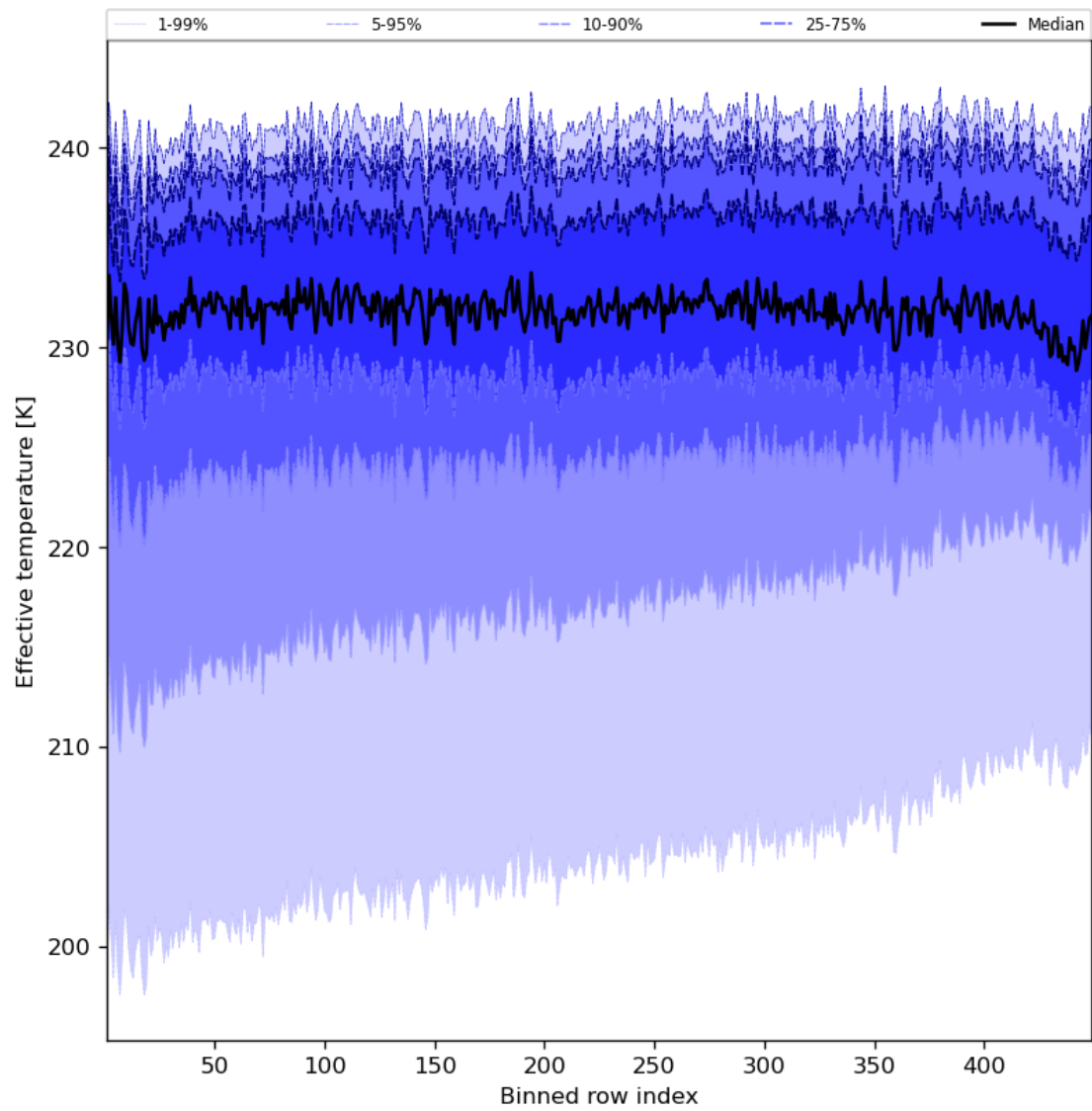
Figure 31: Along track statistics of “Effective temperature” for 2024-07-10 to 2024-07-12
