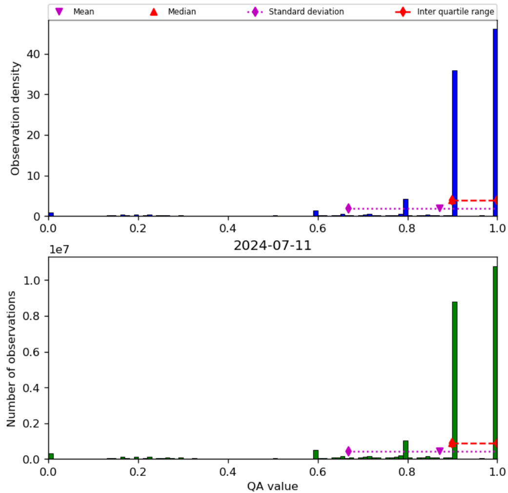
Figure 20: Histogram of “QA value” for 2024-07-10 to 2024-07-12
