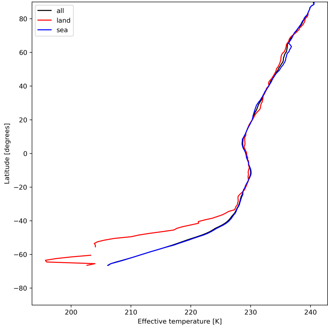
Figure 17: Zonal average of “Effective temperature” for 2024-07-10 to 2024-07-12.
