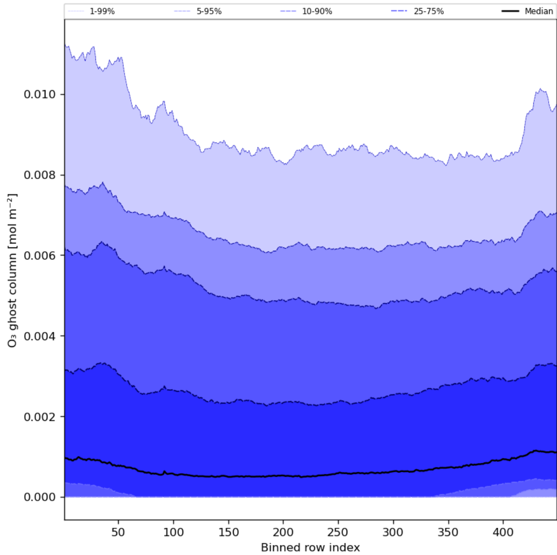
Figure 32: Along track statistics of “O 3 ghost column” for 2024-07-10 to 2024-07-12
