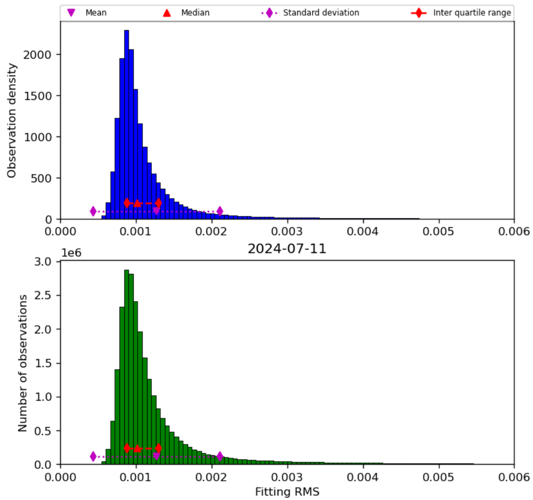
Figure 23: Histogram of “Fitting RMS” for 2024-07-10 to 2024-07-12
