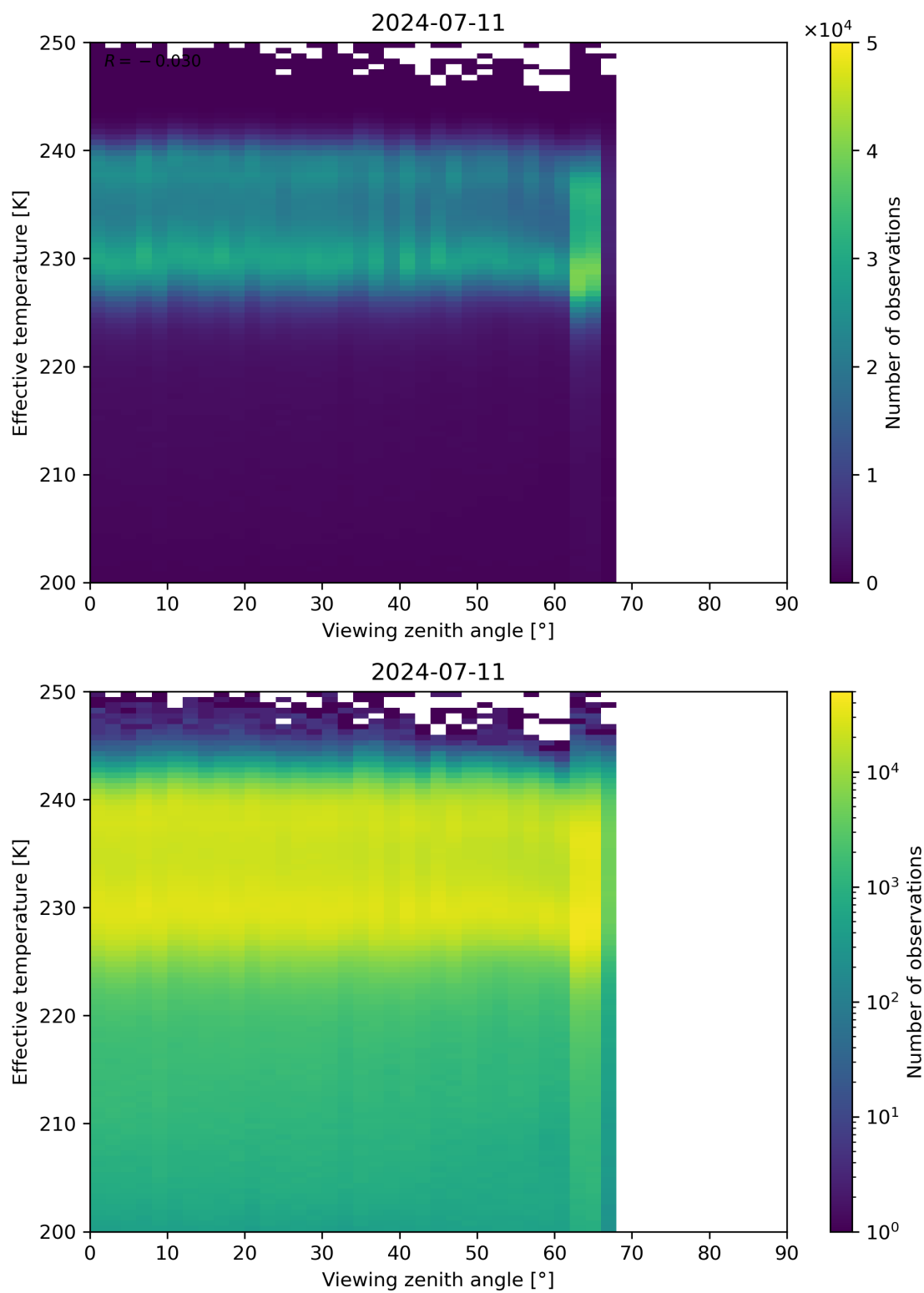
Figure 50: Scatter density plot of “Viewing zenith angle” against “Effective temperature” for 2024-07-10 to 2024-07-12.
