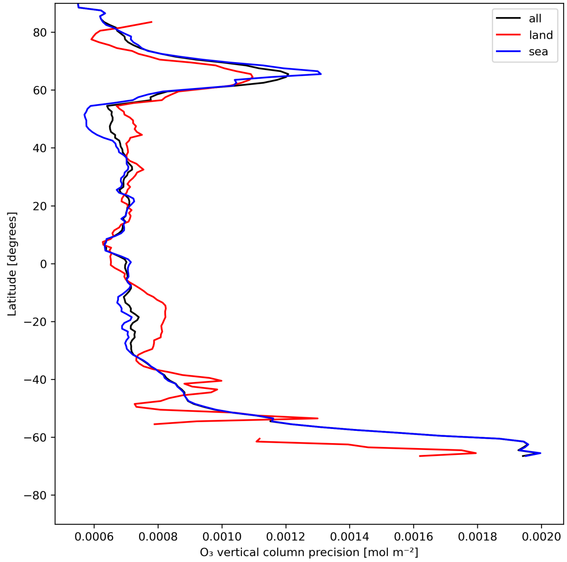
Figure 15: Zonal average of “O 3 vertical column precision” for 2024-07-10 to 2024-07-12.
