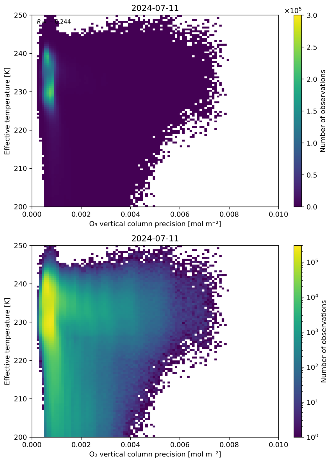
Figure 42: Scatter density plot of “O 3 vertical column precision” against “Effective temperature” for 2024-07-10 to 2024-07-12.
