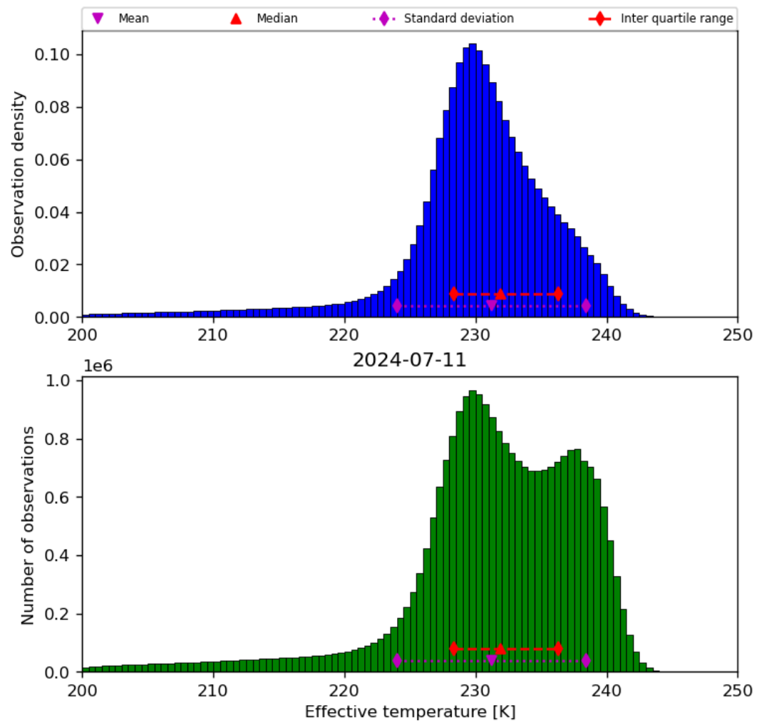
Figure 24: Histogram of “Effective temperature” for 2024-07-10 to 2024-07-12
