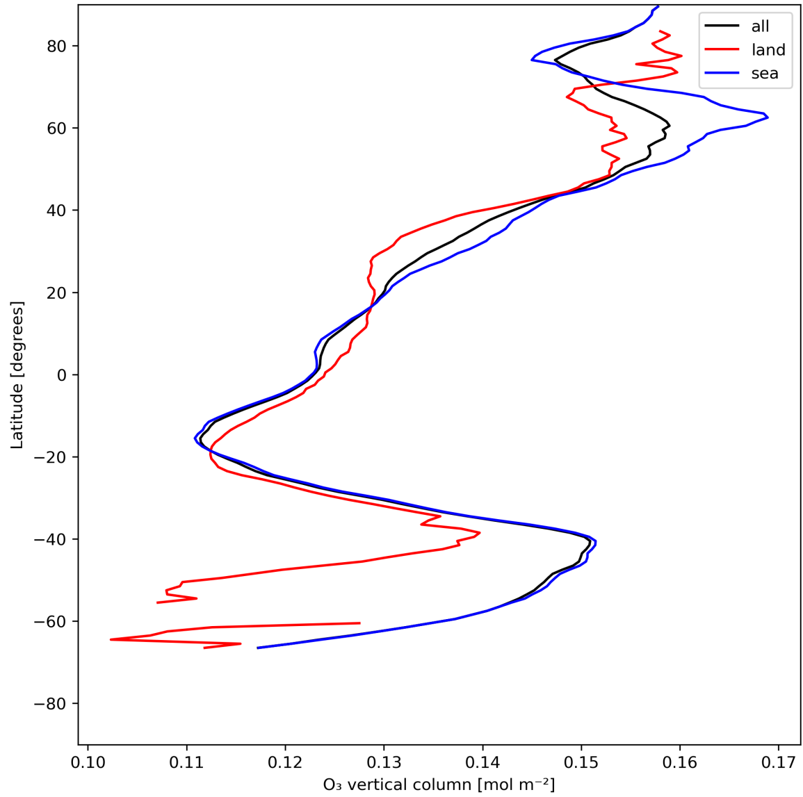
Figure 14: Zonal average of “O 3 vertical column” for 2024-07-10 to 2024-07-12.
