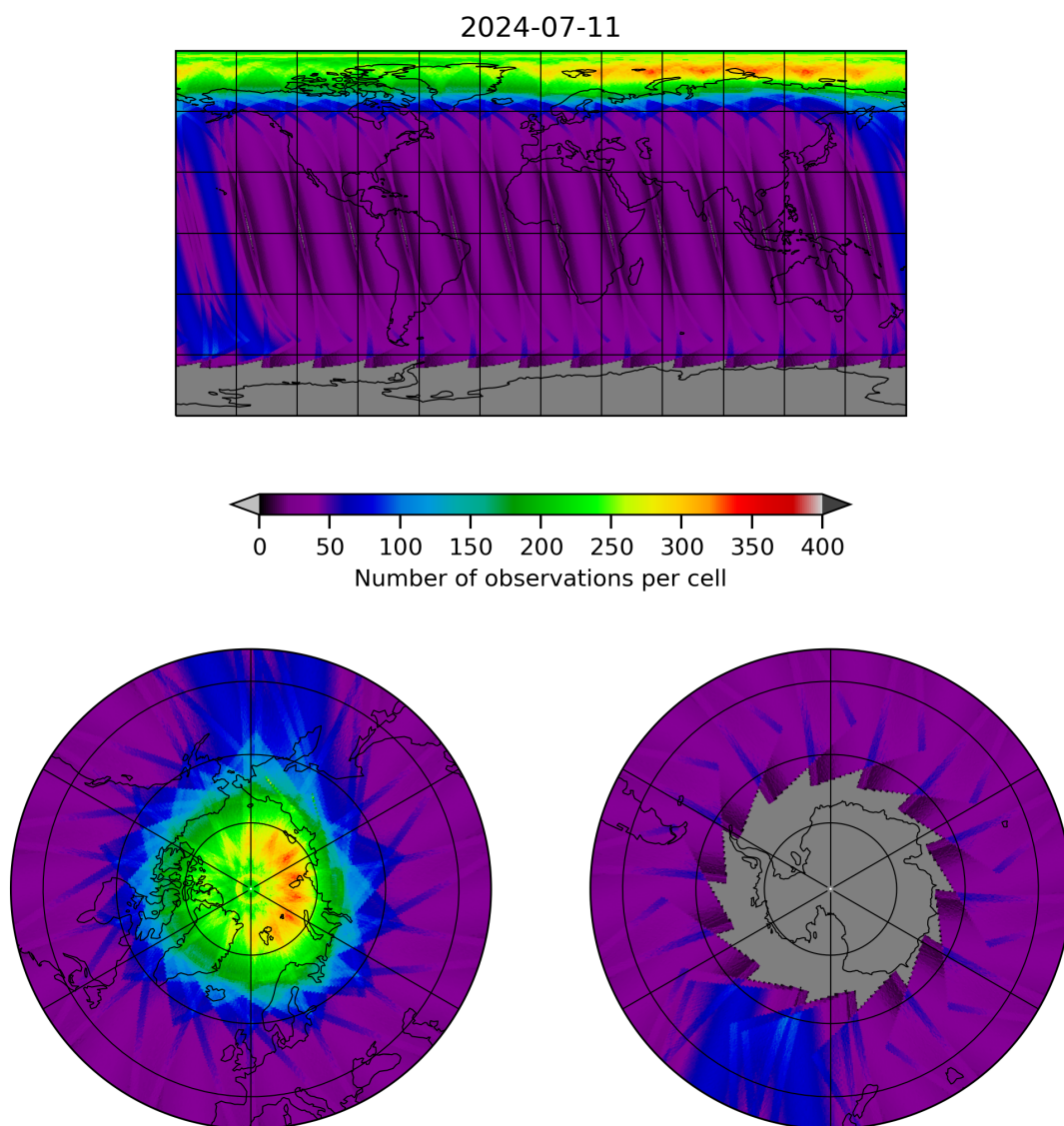
Figure 12: Map of the number of observations for 2024-07-10 to 2024-07-12
