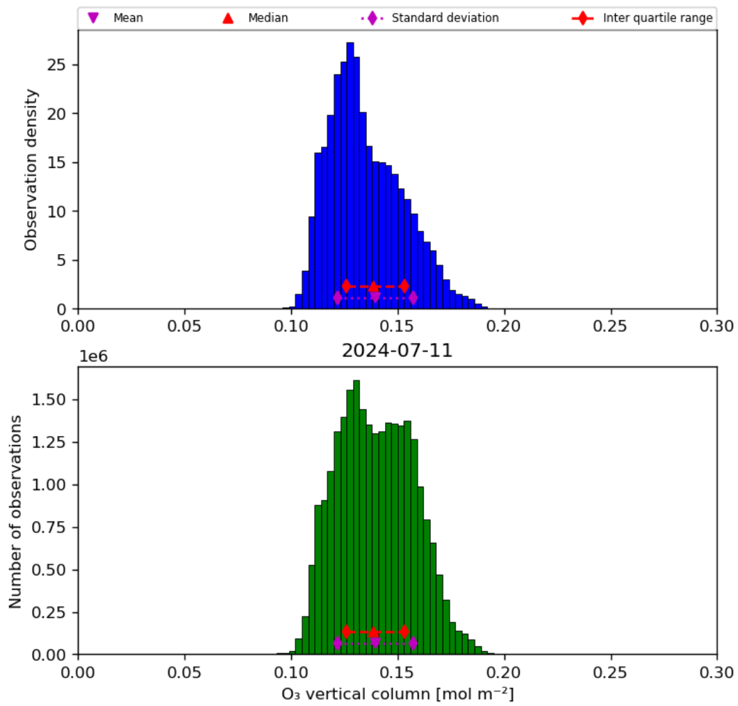
Figure 21: Histogram of “O 3 vertical column” for 2024-07-10 to 2024-07-12
