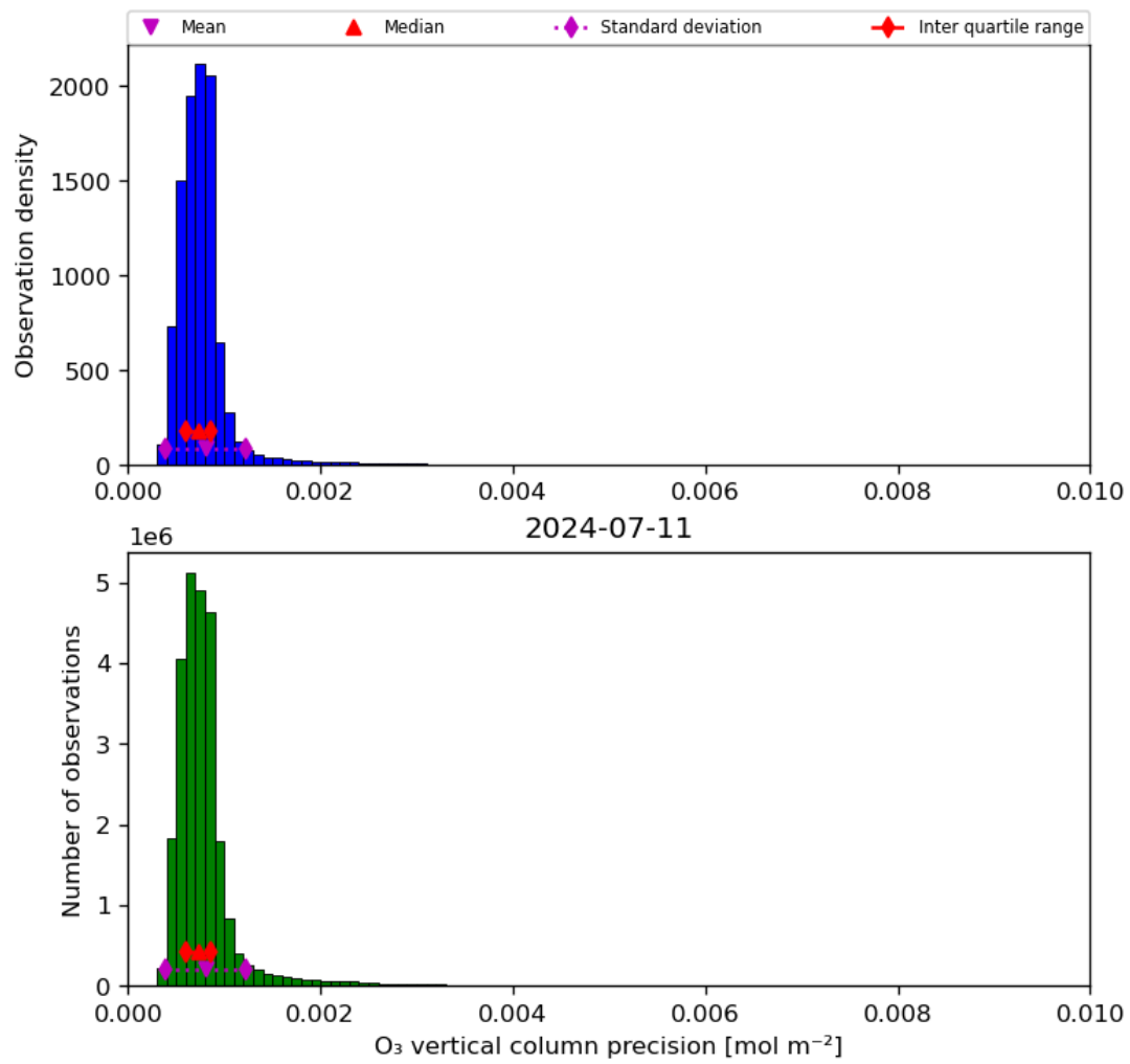
Figure 22: Histogram of “O 3 vertical column precision” for 2024-07-10 to 2024-07-12
