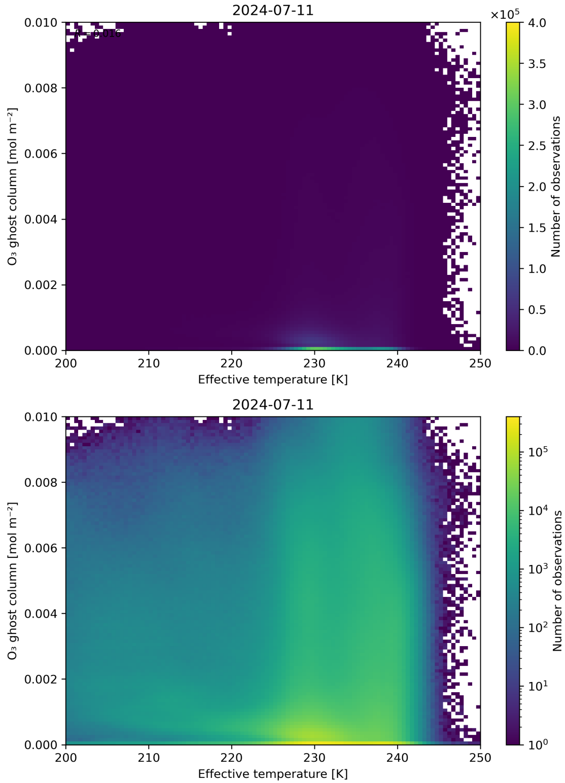
Figure 38: Scatter density plot of “Effective temperature” against “O 3 ghost column” for 2024-07-10 to 2024-07-12.
