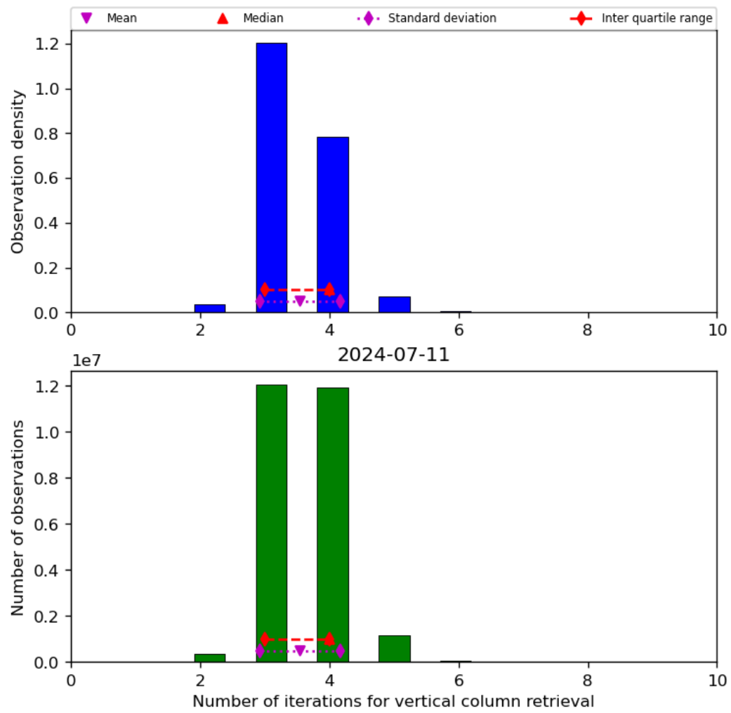
Figure 26: Histogram of “Number of iterations for vertical column retrieval” for 2024-07-10 to 2024-07-12
