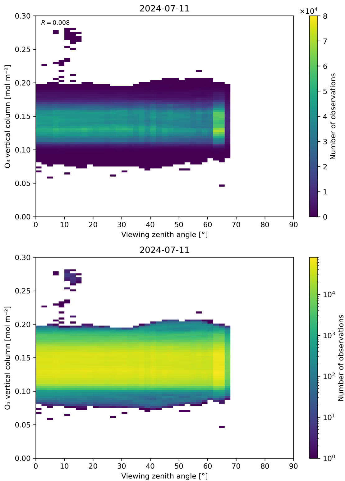
Figure 52: Scatter density plot of “Viewing zenith angle” against “O 3 vertical column” for 2024-07-10 to 2024-07-12.
