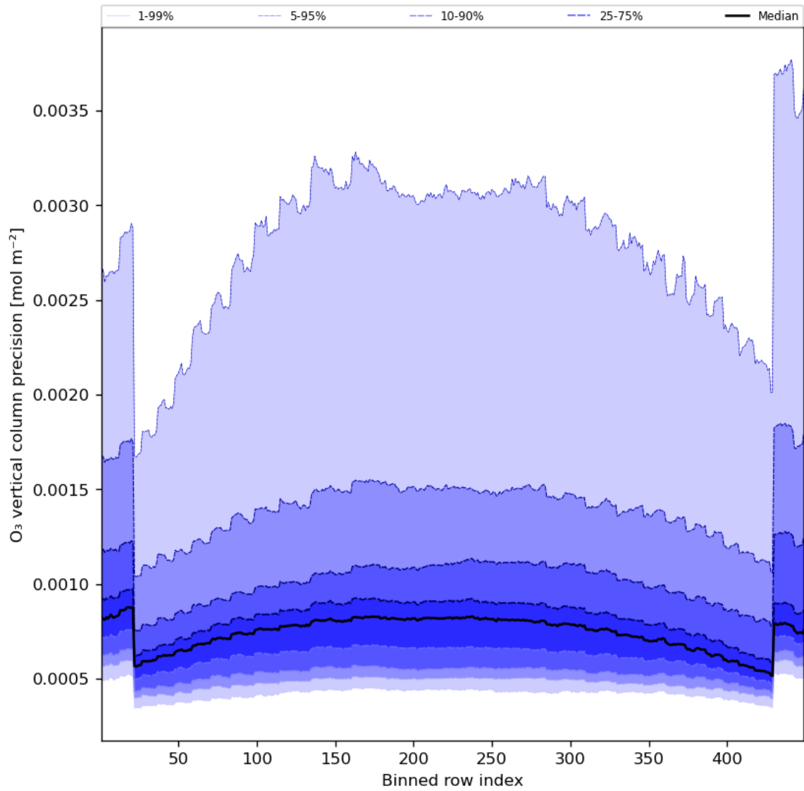
Figure 29: Along track statistics of “O 3 vertical column precision” for 2024-07-10 to 2024-07-12
