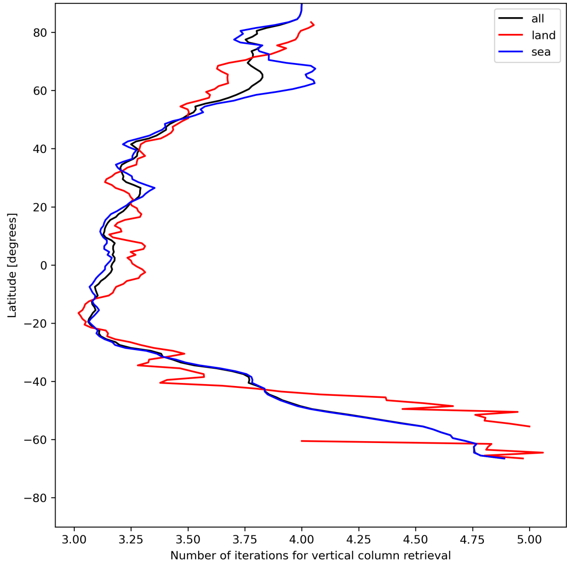
Figure 19: Zonal average of “Number of iterations for vertical column retrieval” for 2024-07-10 to 2024-07-12.
