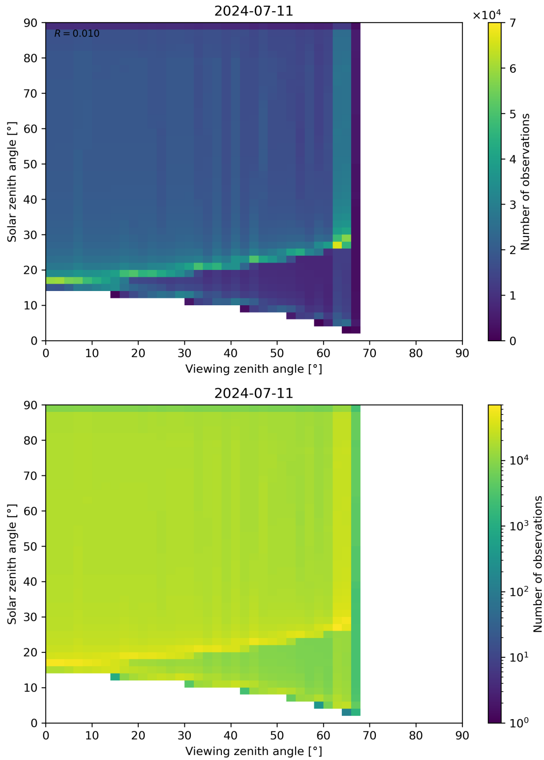
Figure 54: Scatter density plot of “Viewing zenith angle” against “Solar zenith angle” for 2024-07-10 to 2024-07-12.
