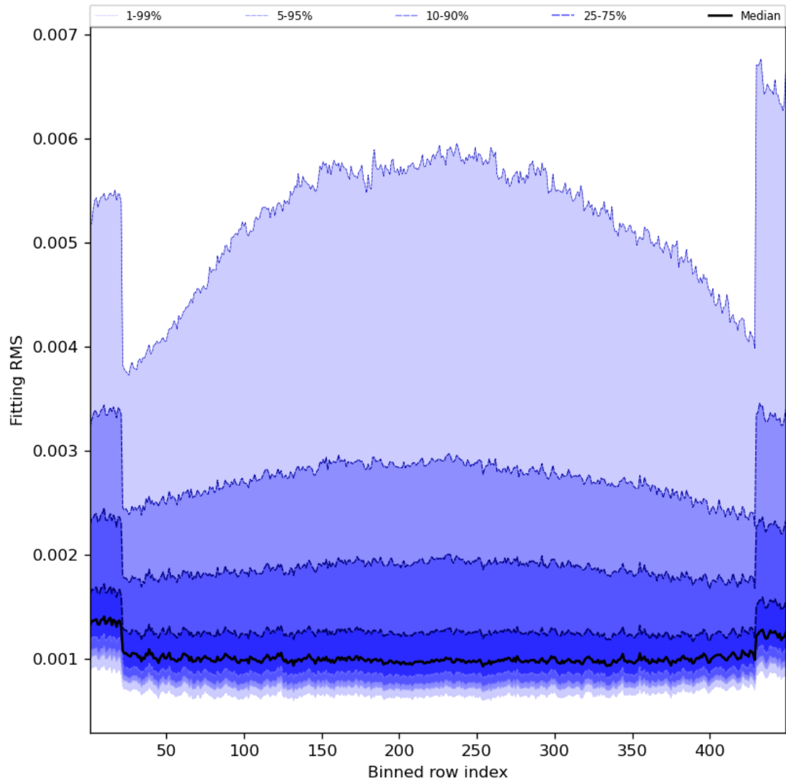
Figure 30: Along track statistics of “Fitting RMS” for 2024-07-10 to 2024-07-12
