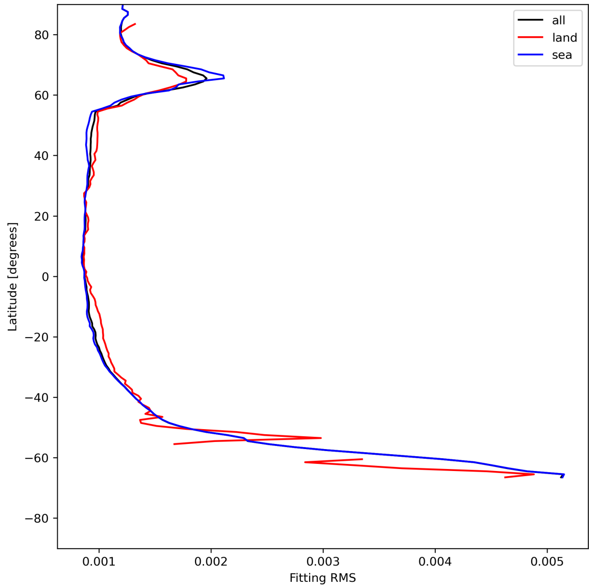
Figure 16: Zonal average of “Fitting RMS” for 2024-07-10 to 2024-07-12.
