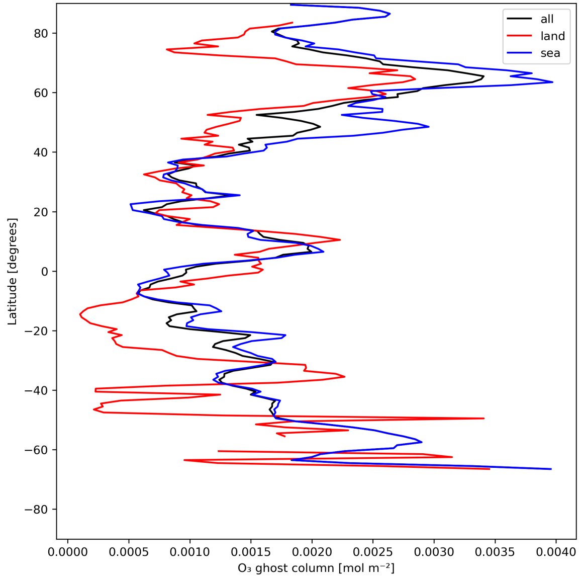
Figure 18: Zonal average of "O 3 ghost column" for 2024-07-10 to 2024-07-12.
