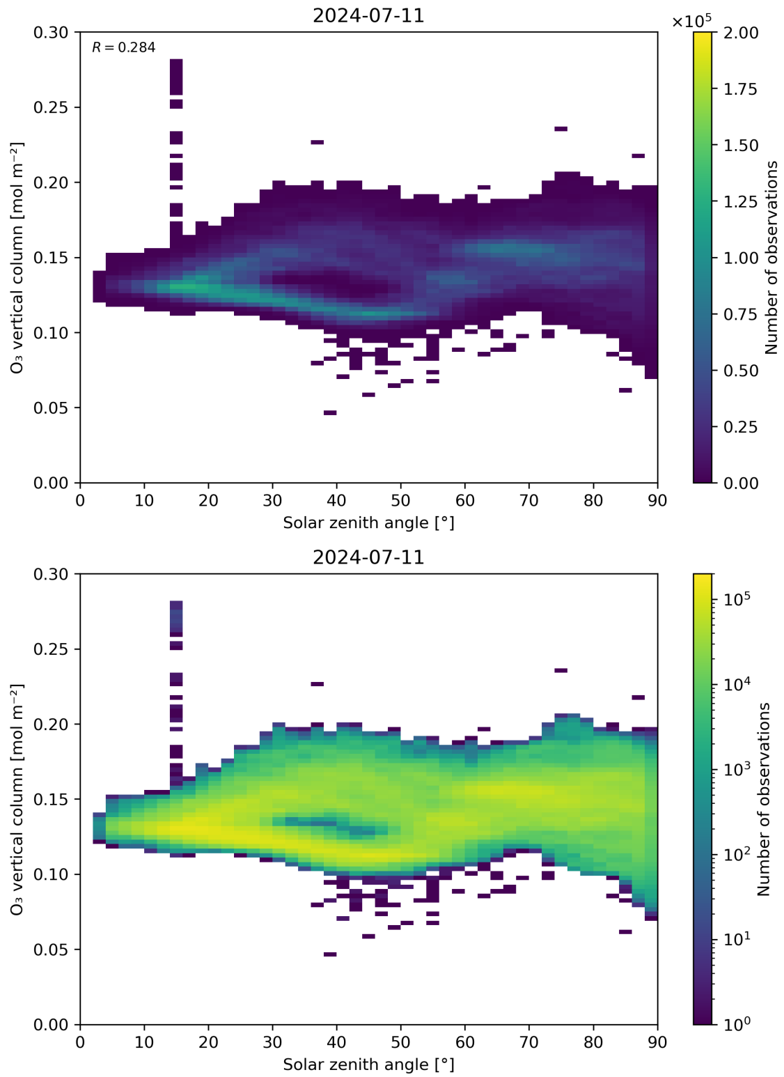
Figure 47: Scatter density plot of “Solar zenith angle” against “O 3 vertical column” for 2024-07-10 to 2024-07-12.
