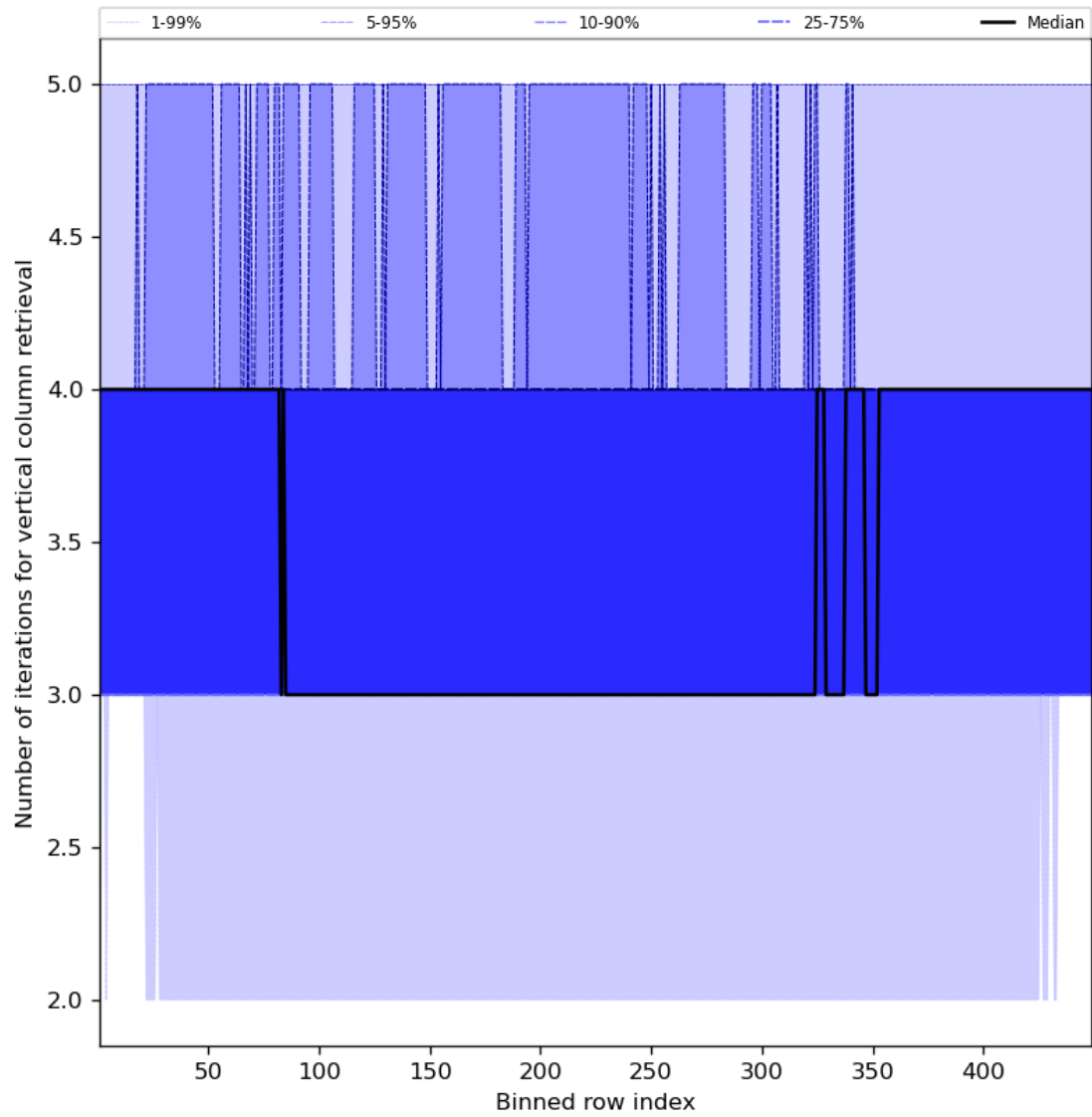
Figure 33: Along track statistics of “Number of iterations for vertical column retrieval” for 2024-07-10 to 2024-07-12
