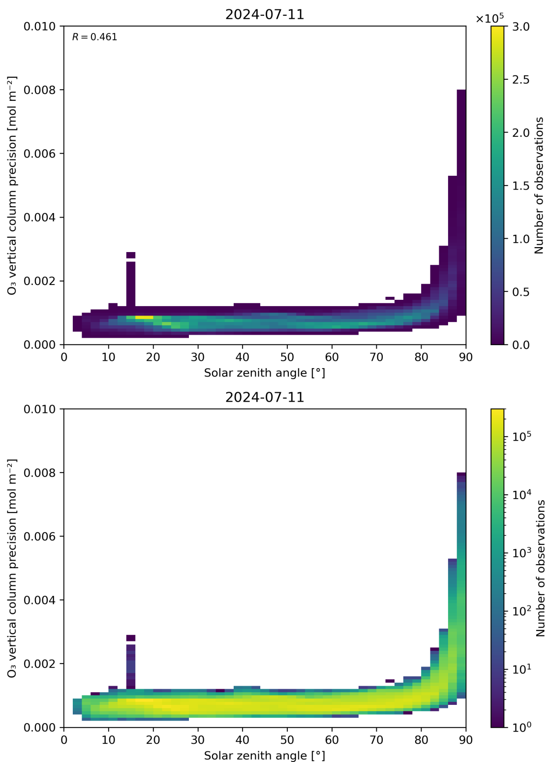
Figure 48: Scatter density plot of “Solar zenith angle” against “O 3 vertical column precision” for 2024-07-10 to 2024-07-12.
