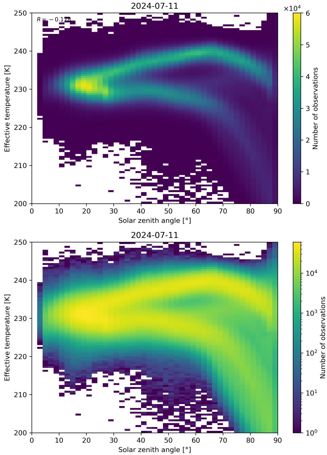
Figure 45: Scatter density plot of “Solar zenith angle” against “Effective temperature” for 2024-07-10 to 2024-07-12.
