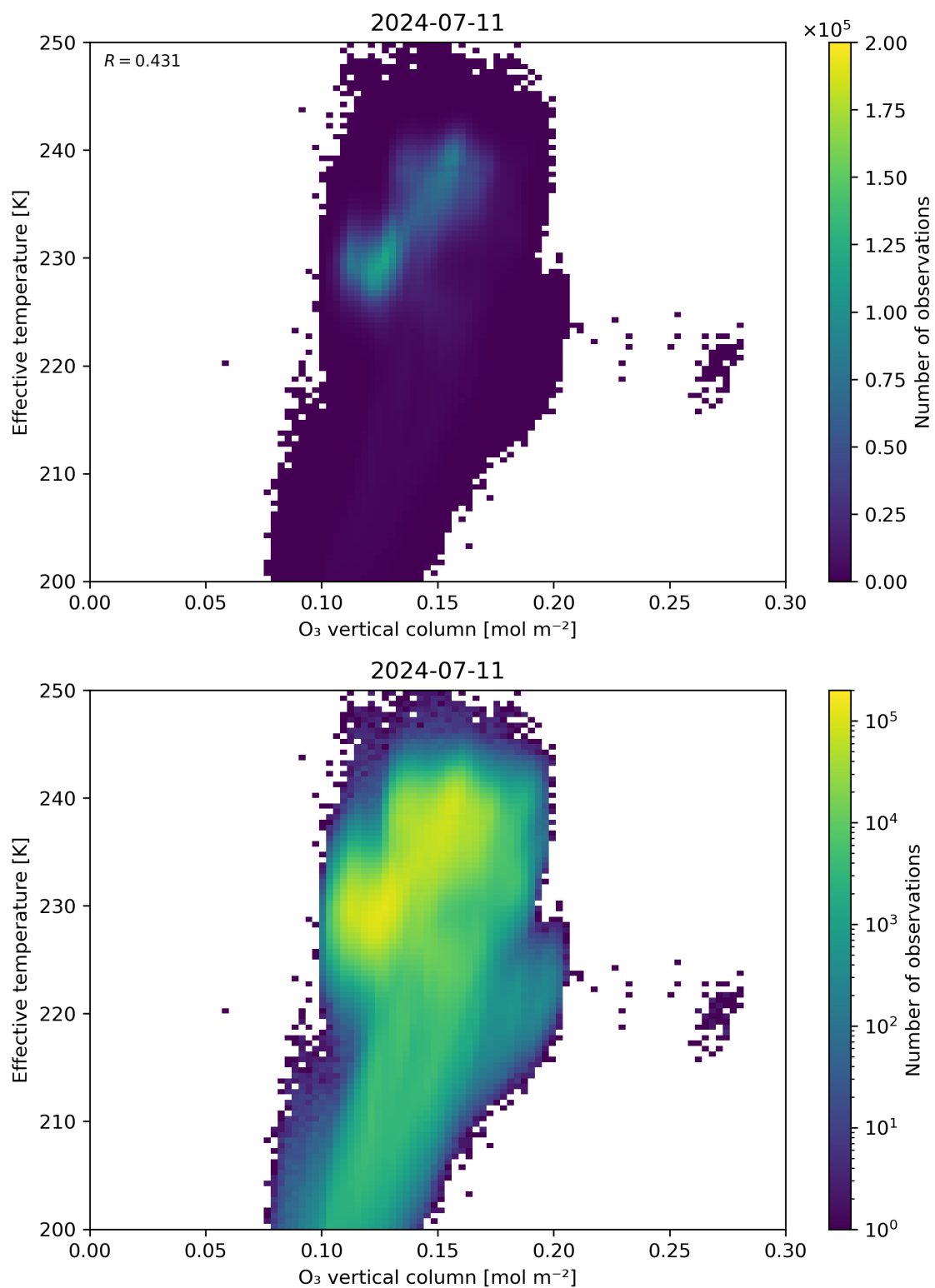
Figure 39: Scatter density plot of “O 3 vertical column” against “Effective temperature” for 2024-07-10 to 2024-07-12.
