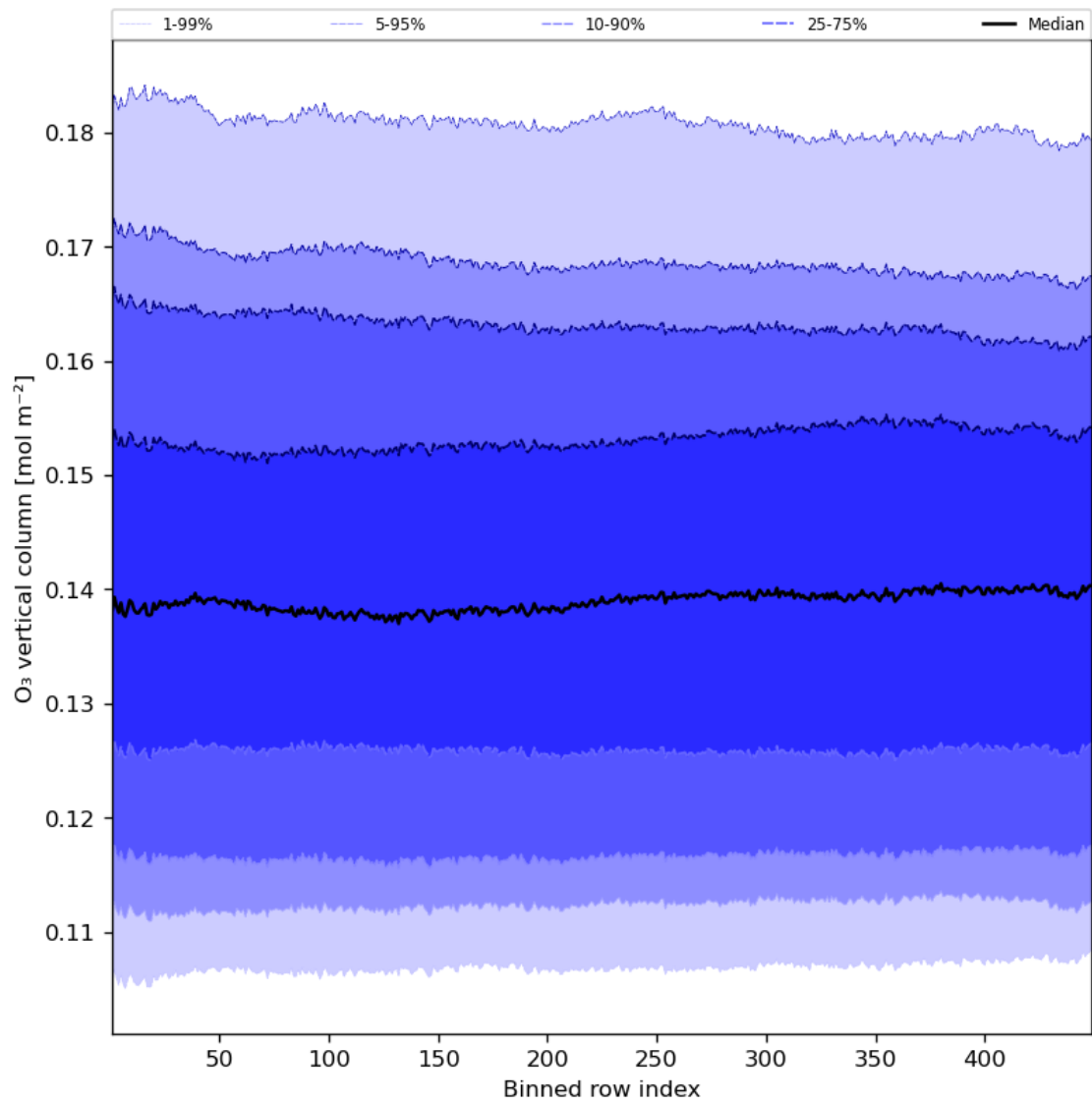
Figure 28: Along track statistics of “ \text{O}_3 vertical column” for 2024-07-10 to 2024-07-12
