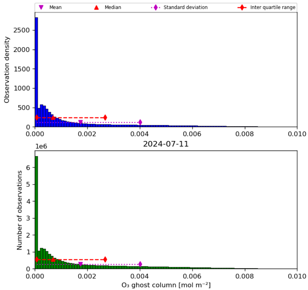
Figure 25: Histogram of “O 3 ghost column” for 2024-07-10 to 2024-07-12
