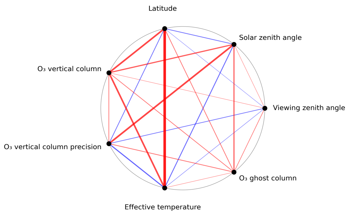
Figure 1: Map of correlation graph for 2024-07-10 to 2024-07-12.
