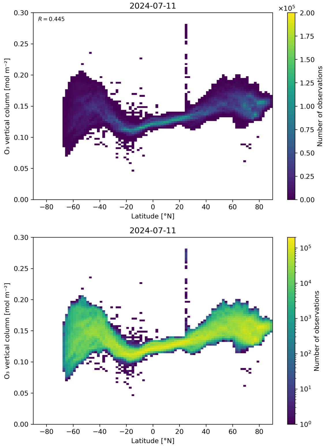
Figure 36: Scatter density plot of “Latitude” against “O 3 vertical column” for 2024-07-10 to 2024-07-12.
