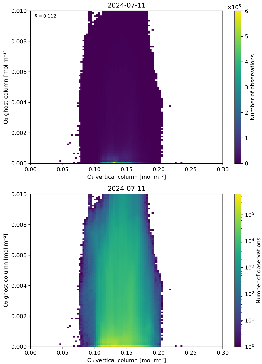
Figure 40: Scatter density plot of “O 3 vertical column” against “O 3 ghost column” for 2024-07-10 to 2024-07-12.
