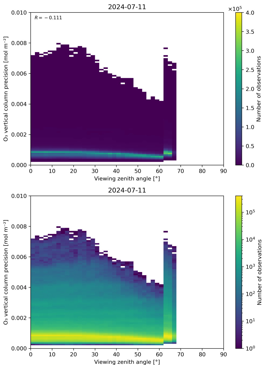
Figure 53: Scatter density plot of “Viewing zenith angle” against “O 3 vertical column precision” for 2024-07-10 to 2024-07-12.
