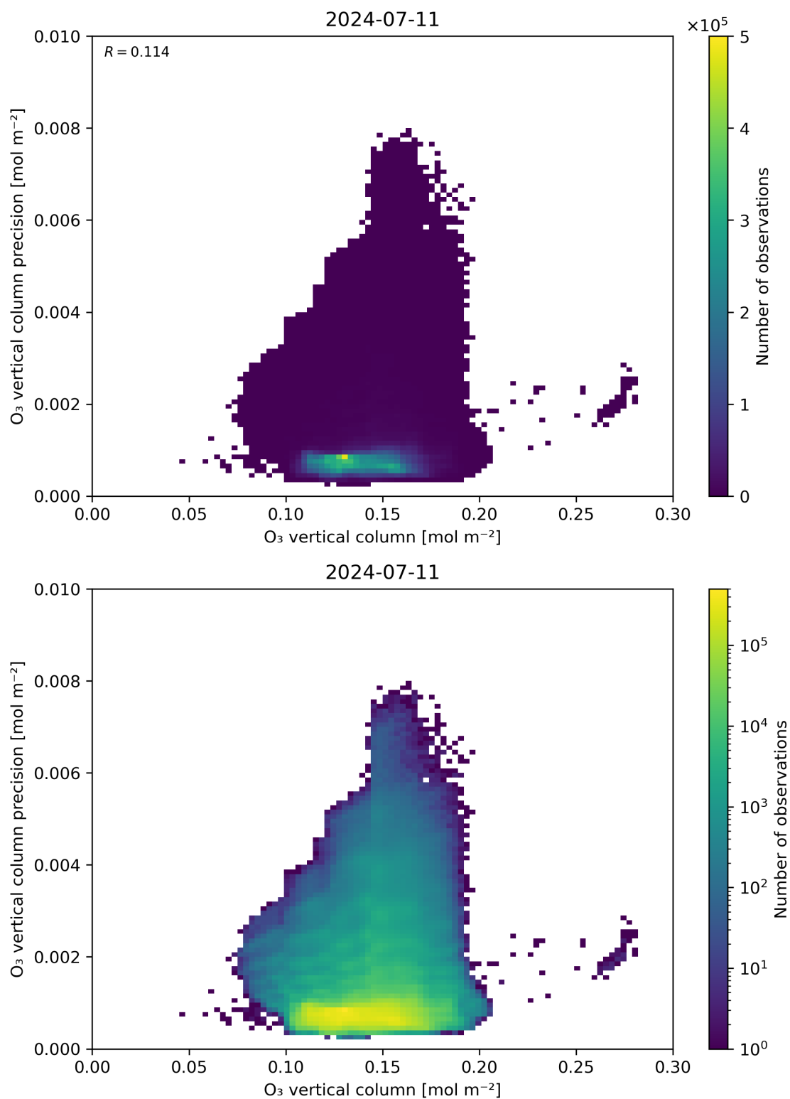
Figure 41: Scatter density plot of “O 3 vertical column” against “O 3 vertical column precision” for 2024-07-10 to 2024-07-12.
