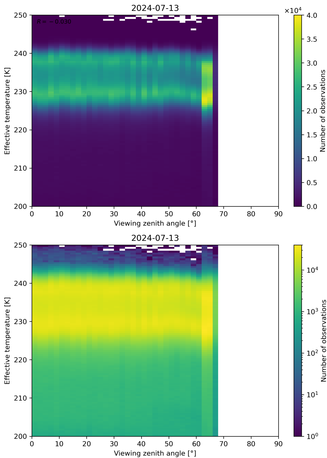
Figure 50: Scatter density plot of “Viewing zenith angle” against “Effective temperature” for 2024-07-12 to 2024-07-14.
