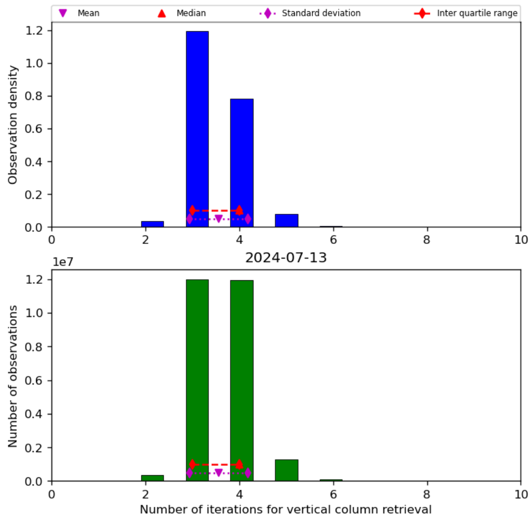
Figure 26: Histogram of “Number of iterations for vertical column retrieval” for 2024-07-12 to 2024-07-14
