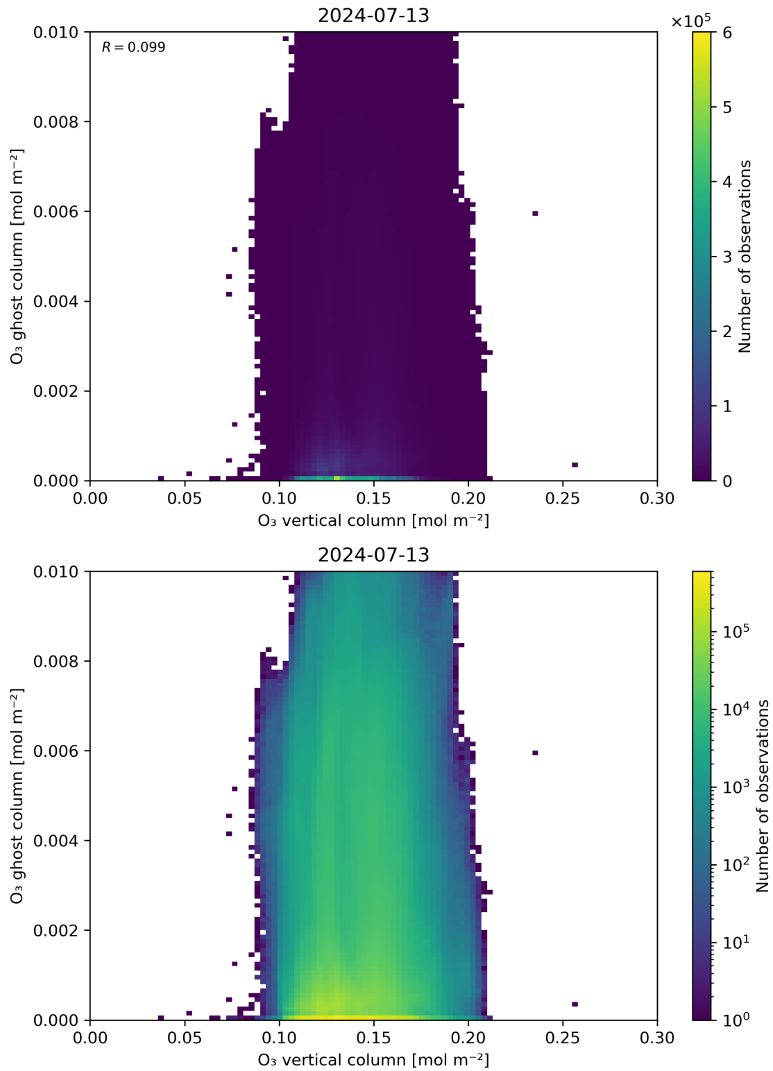
Figure 40: Scatter density plot of “O 3 vertical column” against “O 3 ghost column” for 2024-07-12 to 2024-07-14.
