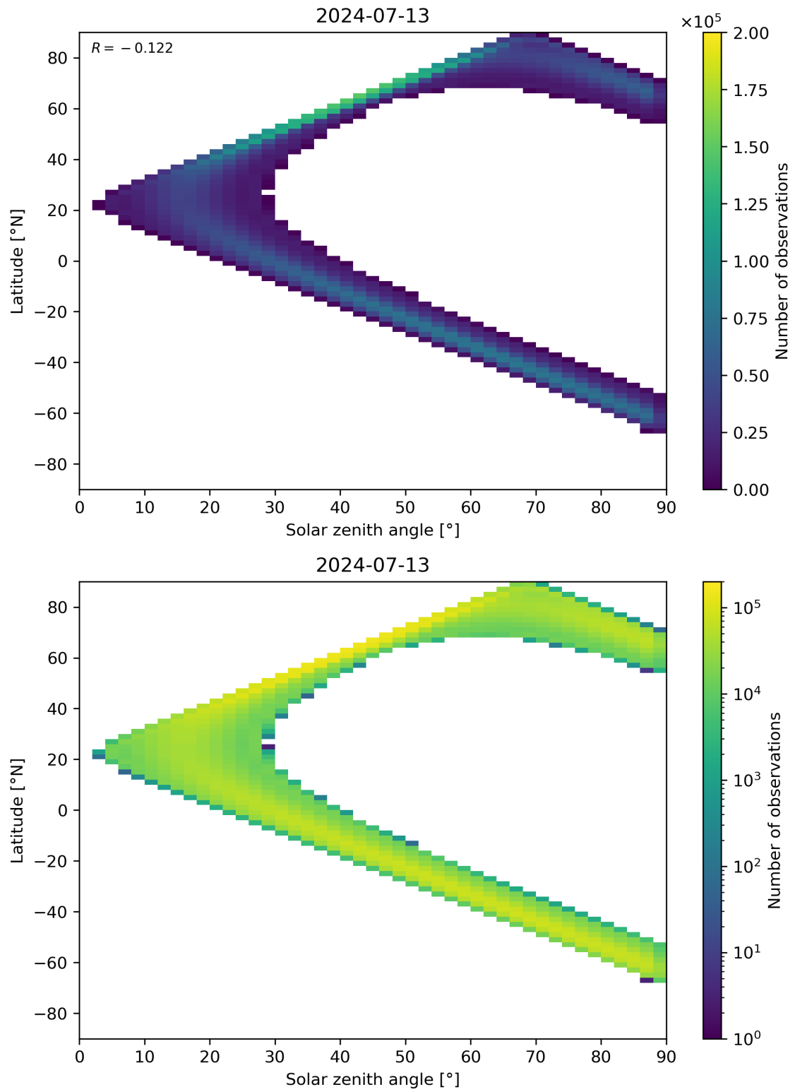
Figure 44: Scatter density plot of “Solar zenith angle” against “Latitude” for 2024-07-12 to 2024-07-14.
