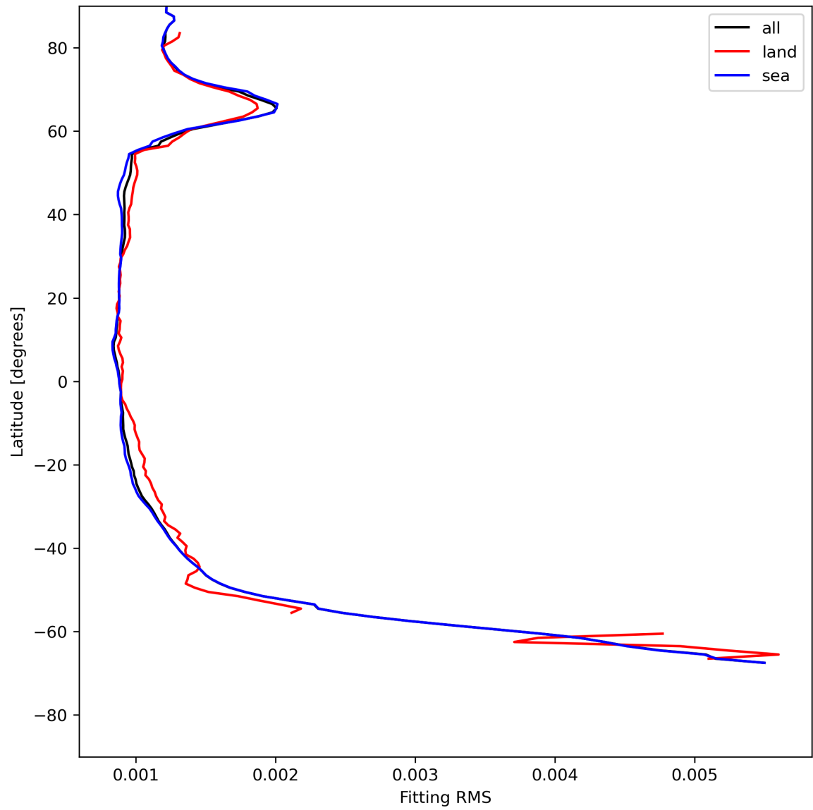
Figure 16: Zonal average of “Fitting RMS” for 2024-07-12 to 2024-07-14.
