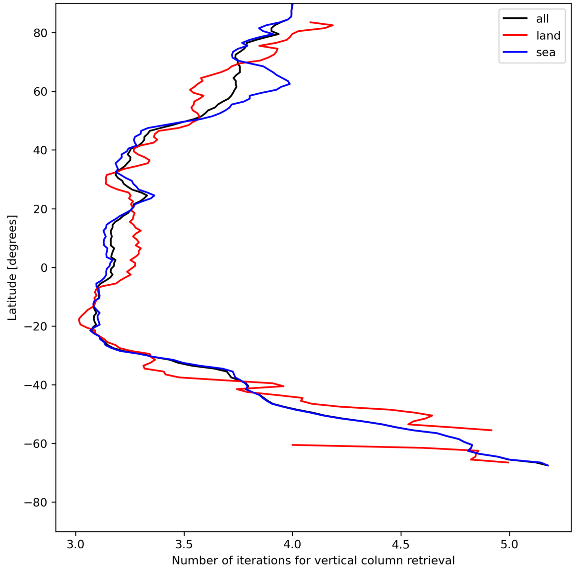
Figure 19: Zonal average of “Number of iterations for vertical column retrieval” for 2024-07-12 to 2024-07-14.
