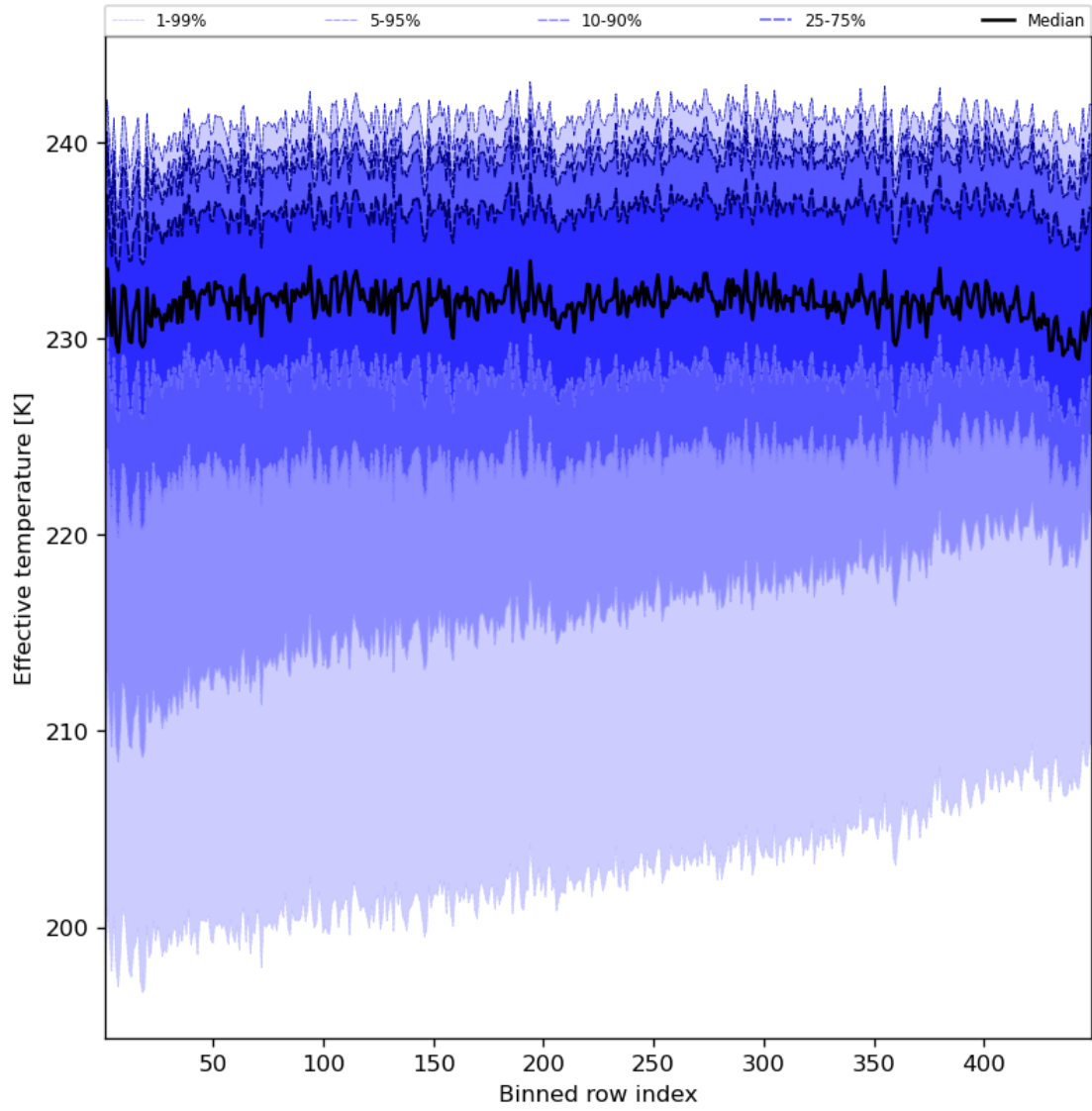
Figure 31: Along track statistics of “Effective temperature” for 2024-07-12 to 2024-07-14
