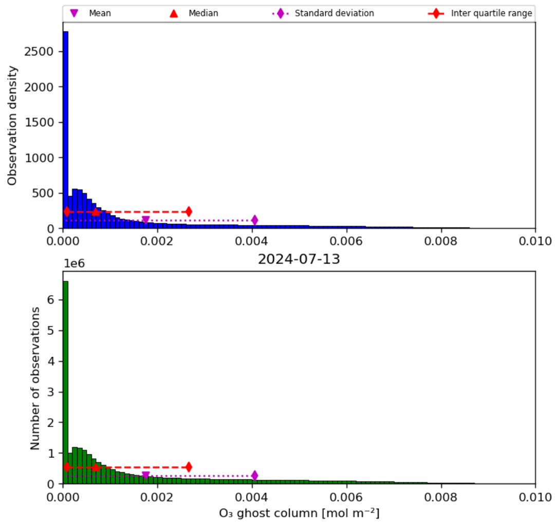
Figure 25: Histogram of “O 3 ghost column” for 2024-07-12 to 2024-07-14
