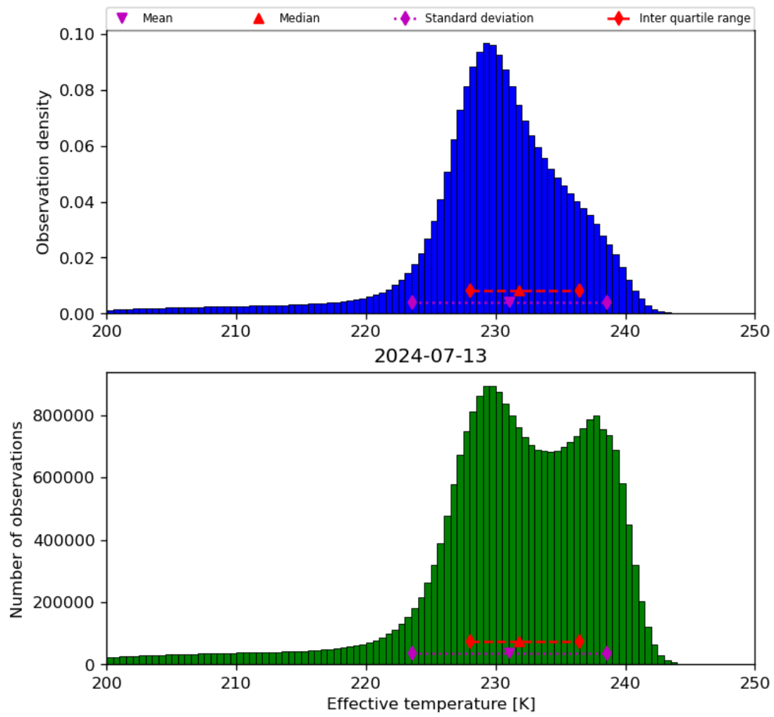
Figure 24: Histogram of “Effective temperature” for 2024-07-12 to 2024-07-14
