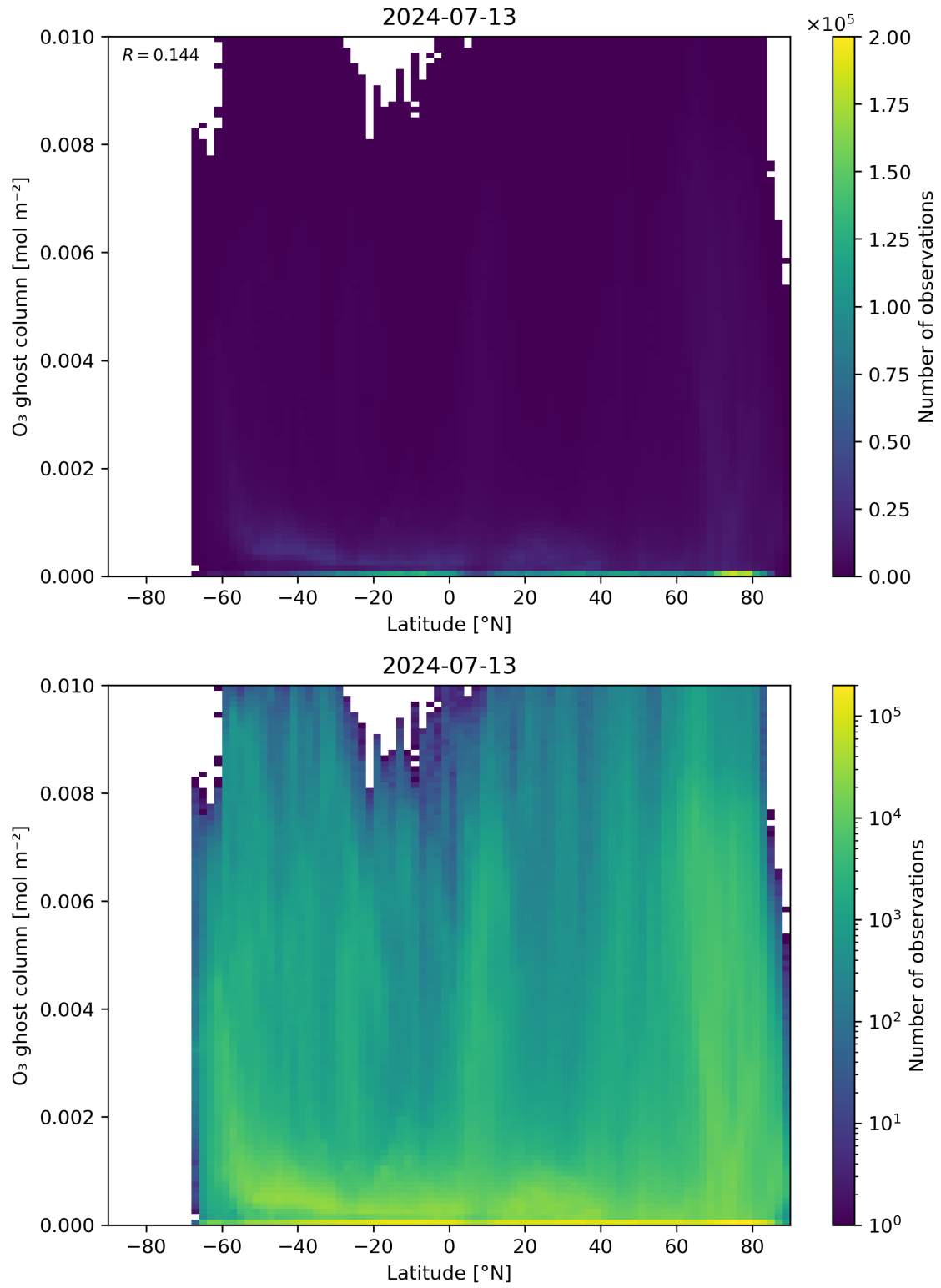
Figure 35: Scatter density plot of “Latitude” against “O 3 ghost column” for 2024-07-12 to 2024-07-14.
