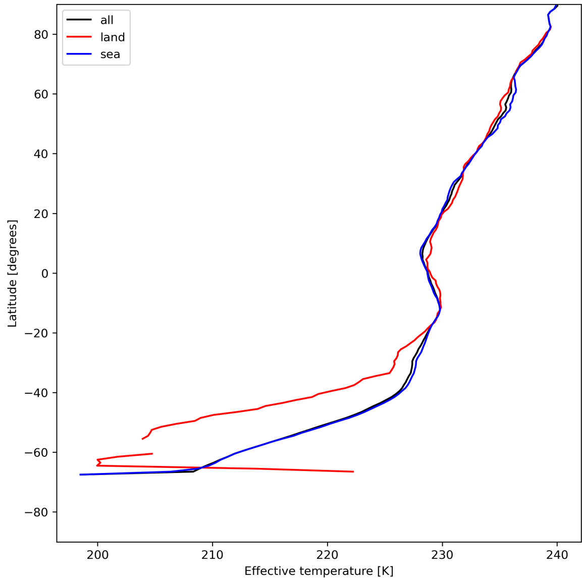
Figure 17: Zonal average of “Effective temperature” for 2024-07-12 to 2024-07-14.
