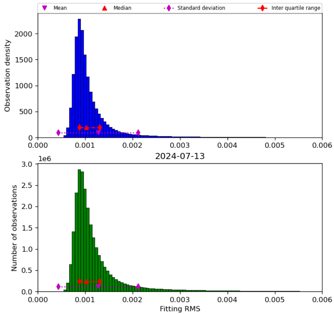
Figure 23: Histogram of “Fitting RMS” for 2024-07-12 to 2024-07-14
