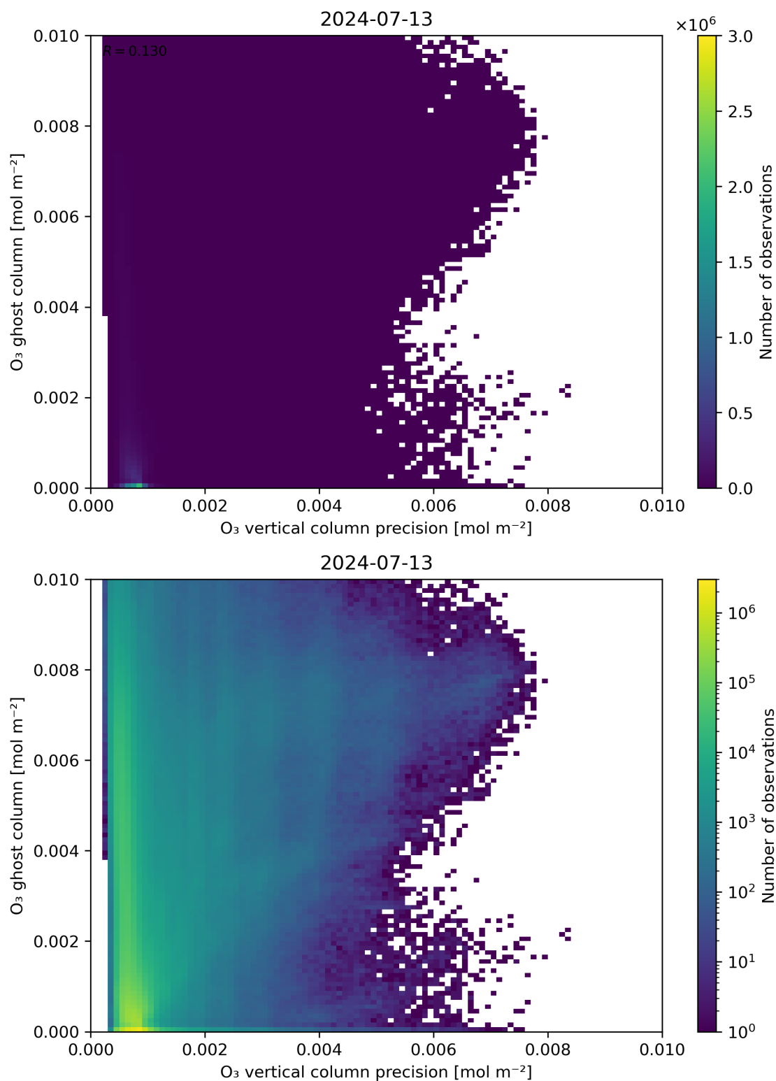
Figure 43: Scatter density plot of “ \text{O}_3 vertical column precision” against “ \text{O}_3 ghost column” for 2024-07-12 to 2024-07-14.
