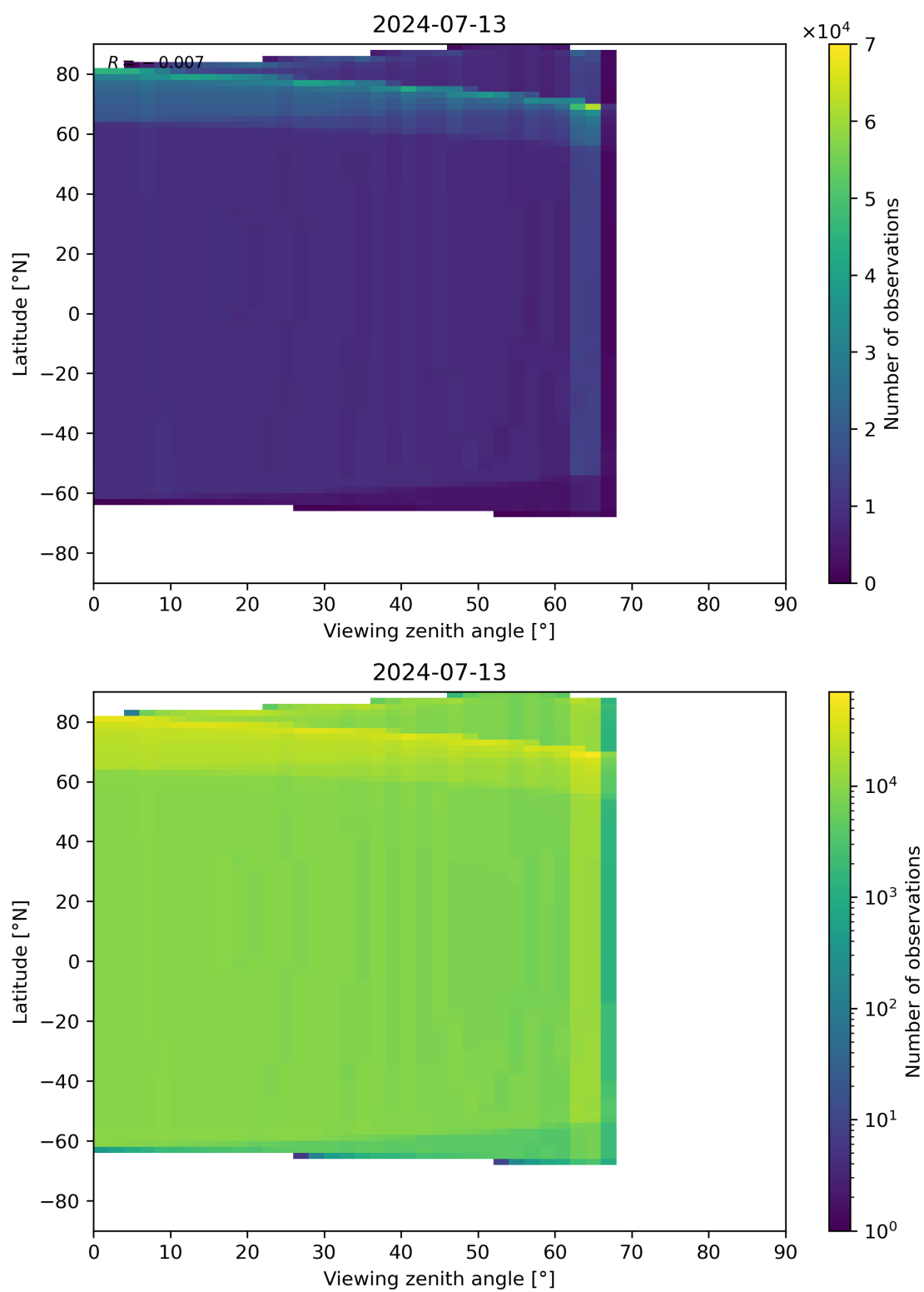
Figure 49: Scatter density plot of “Viewing zenith angle” against “Latitude” for 2024-07-12 to 2024-07-14.
