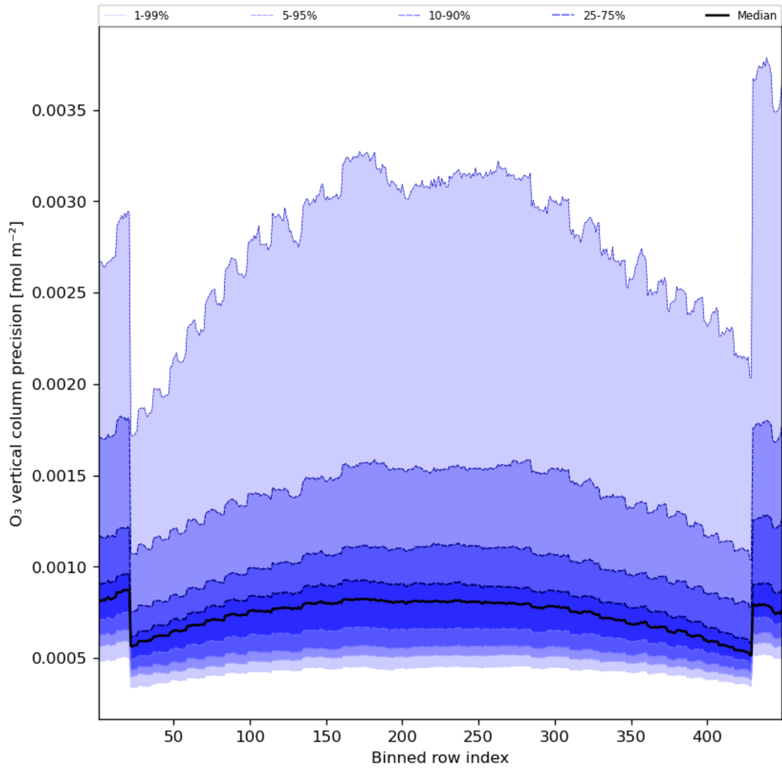
Figure 29: Along track statistics of “O 3 vertical column precision” for 2024-07-12 to 2024-07-14
