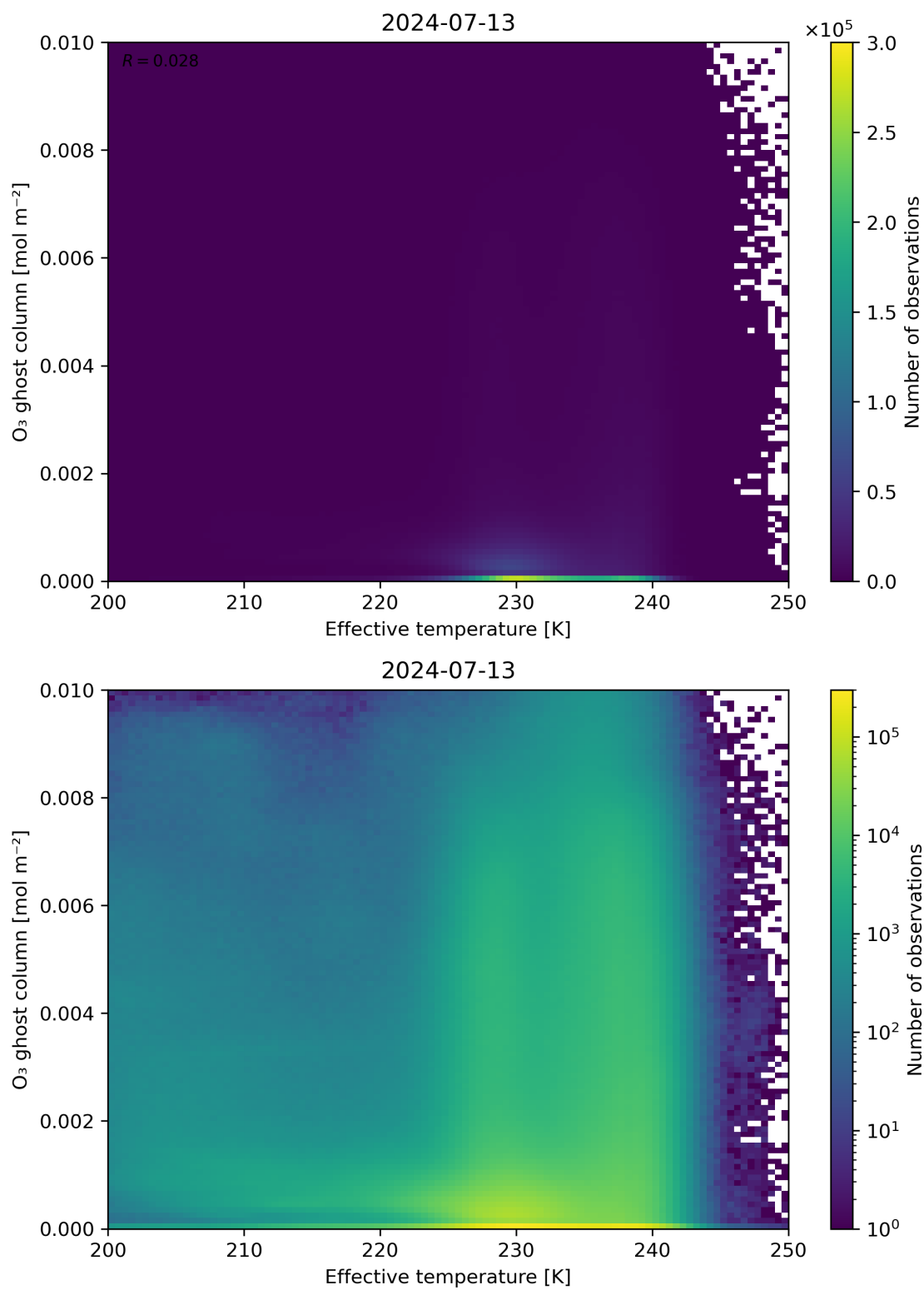
Figure 38: Scatter density plot of “Effective temperature” against “O 3 ghost column” for 2024-07-12 to 2024-07-14.
