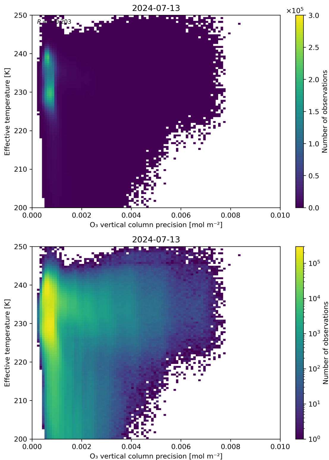
Figure 42: Scatter density plot of “O 3 vertical column precision” against “Effective temperature” for 2024-07-12 to 2024-07-14.
