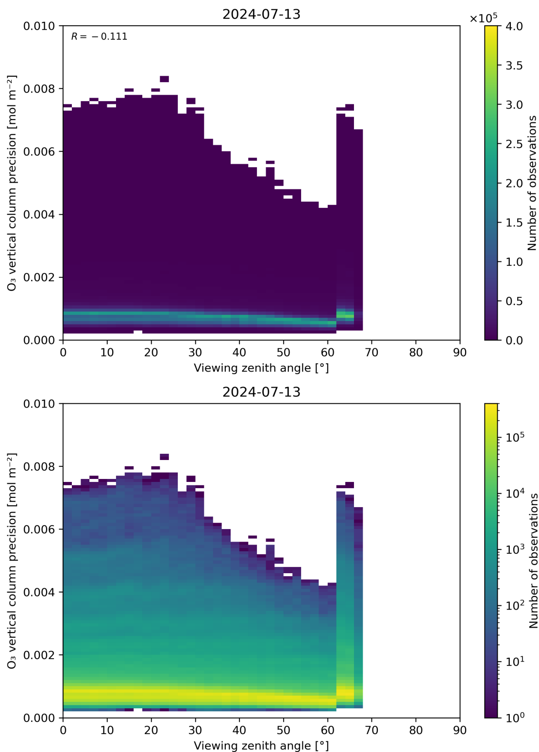
Figure 53: Scatter density plot of “Viewing zenith angle” against “O 3 vertical column precision” for 2024-07-12 to 2024-07-14.
