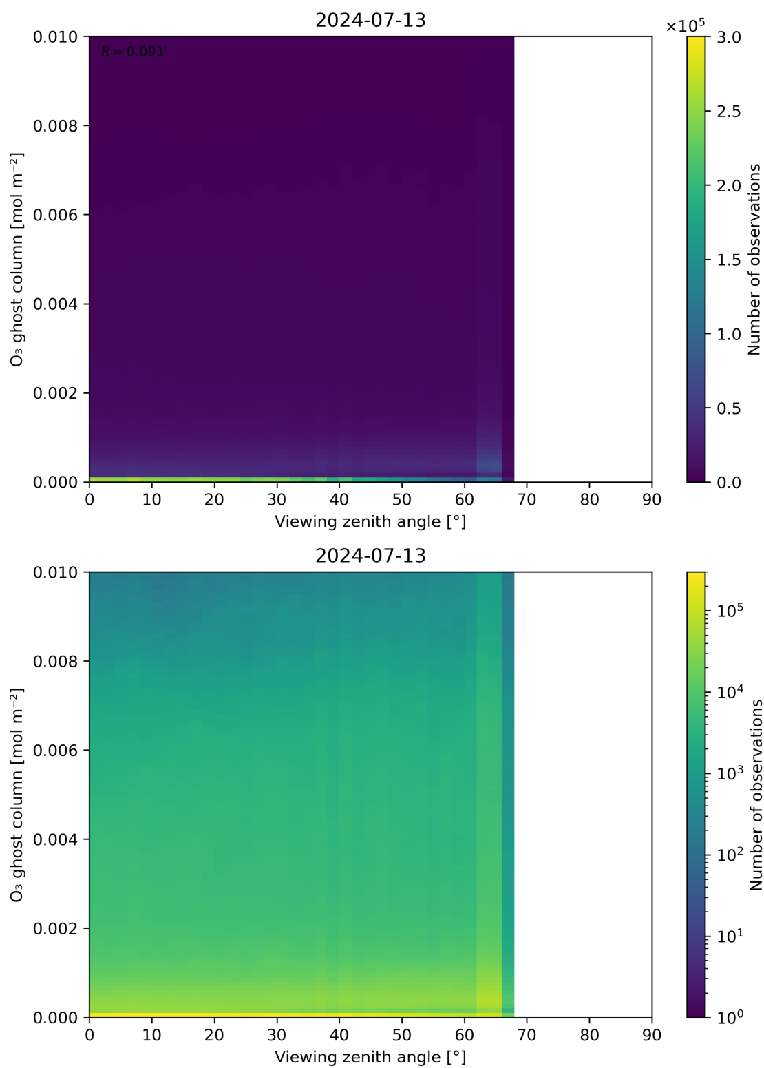
Figure 51: Scatter density plot of “Viewing zenith angle” against “O 3 ghost column” for 2024-07-12 to 2024-07-14.
