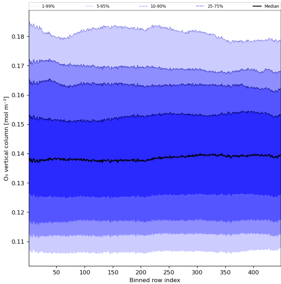
Figure 28: Along track statistics of “O 3 vertical column” for 2024-07-12 to 2024-07-14
