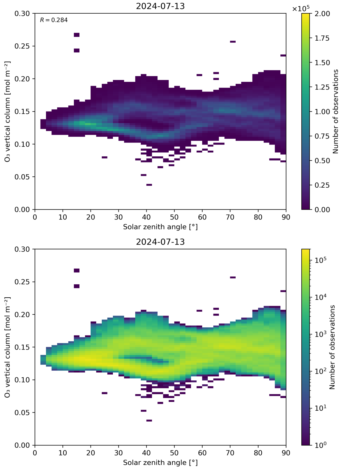
Figure 47: Scatter density plot of “Solar zenith angle” against “O 3 vertical column” for 2024-07-12 to 2024-07-14.
