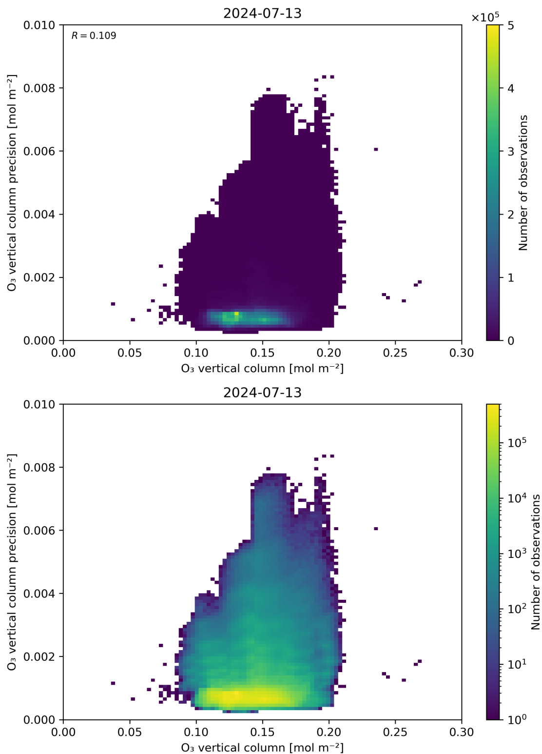
Figure 41: Scatter density plot of “O 3 vertical column” against “O 3 vertical column precision” for 2024-07-12 to 2024-07-14.
