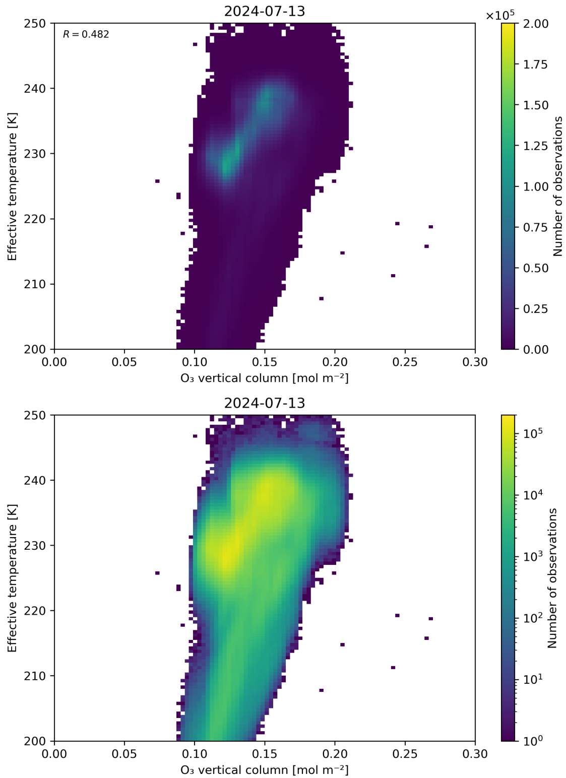
Figure 39: Scatter density plot of “O 3 vertical column” against “Effective temperature” for 2024-07-12 to 2024-07-14.
