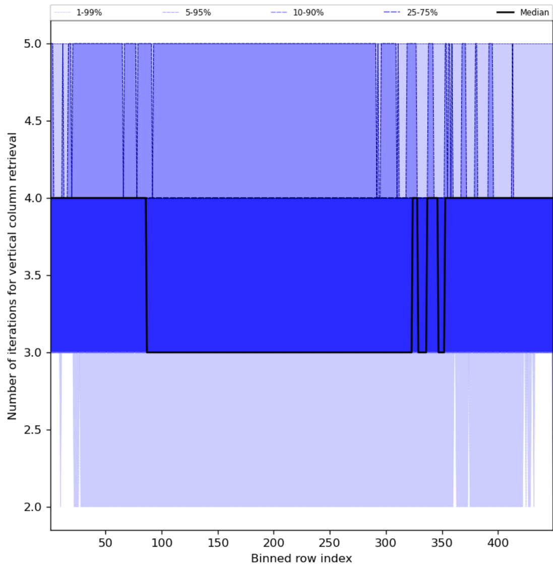
Figure 33: Along track statistics of “Number of iterations for vertical column retrieval” for 2024-07-12 to 2024-07-14
