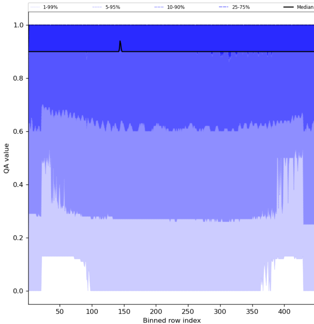
Figure 27: Along track statistics of “QA value” for 2024-07-12 to 2024-07-14
