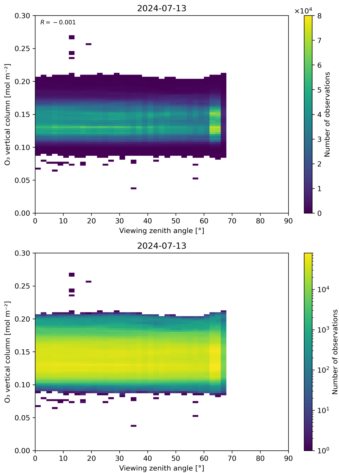
Figure 52: Scatter density plot of “Viewing zenith angle” against “O 3 vertical column” for 2024-07-12 to 2024-07-14.
