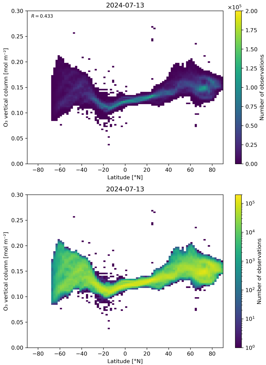
Figure 36: Scatter density plot of “Latitude” against “O 3 vertical column” for 2024-07-12 to 2024-07-14.
