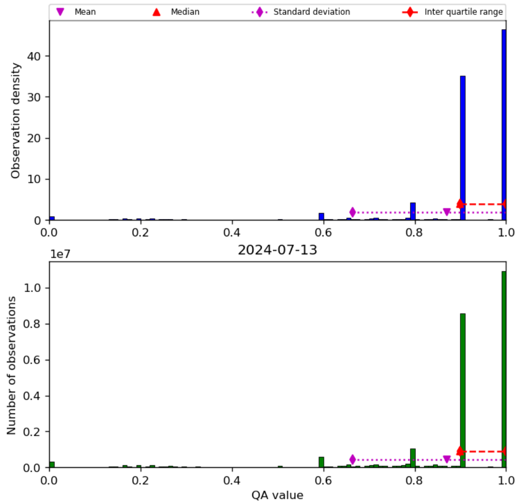
Figure 20: Histogram of “QA value” for 2024-07-12 to 2024-07-14
