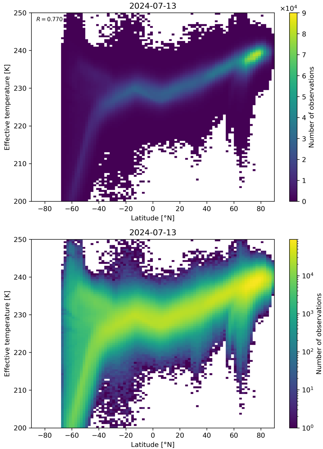
Figure 34: Scatter density plot of “Latitude” against “Effective temperature” for 2024-07-12 to 2024-07-14.
