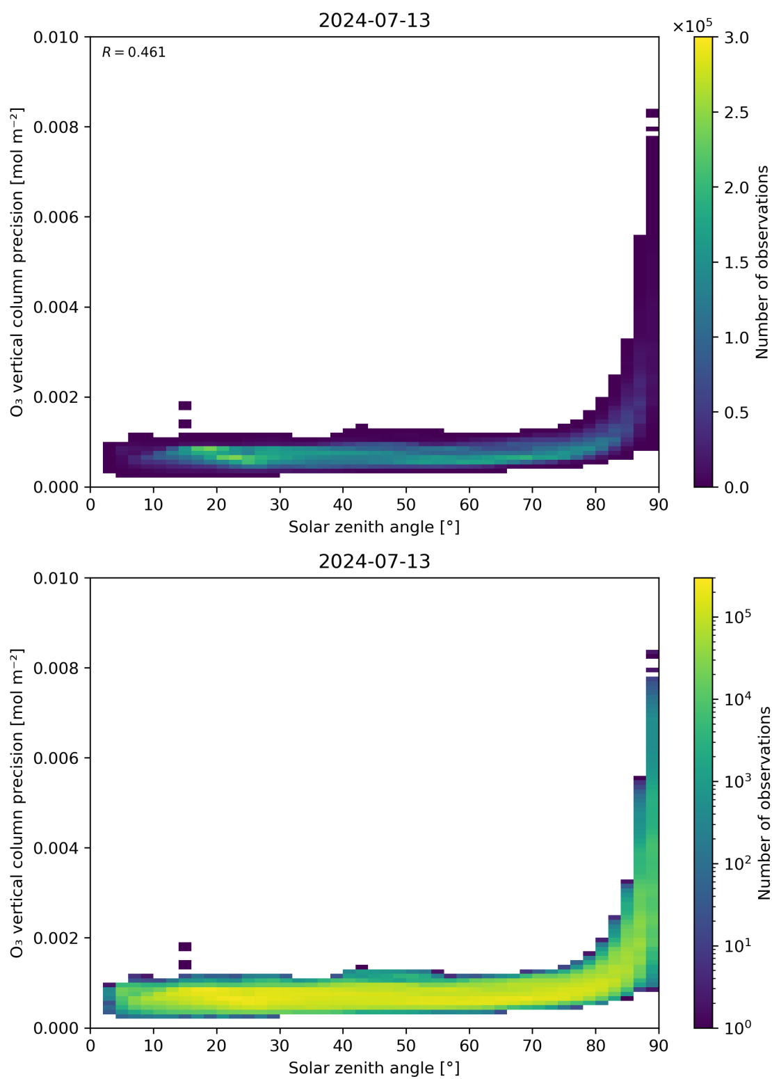
Figure 48: Scatter density plot of “Solar zenith angle” against “O 3 vertical column precision” for 2024-07-12 to 2024-07-14.
