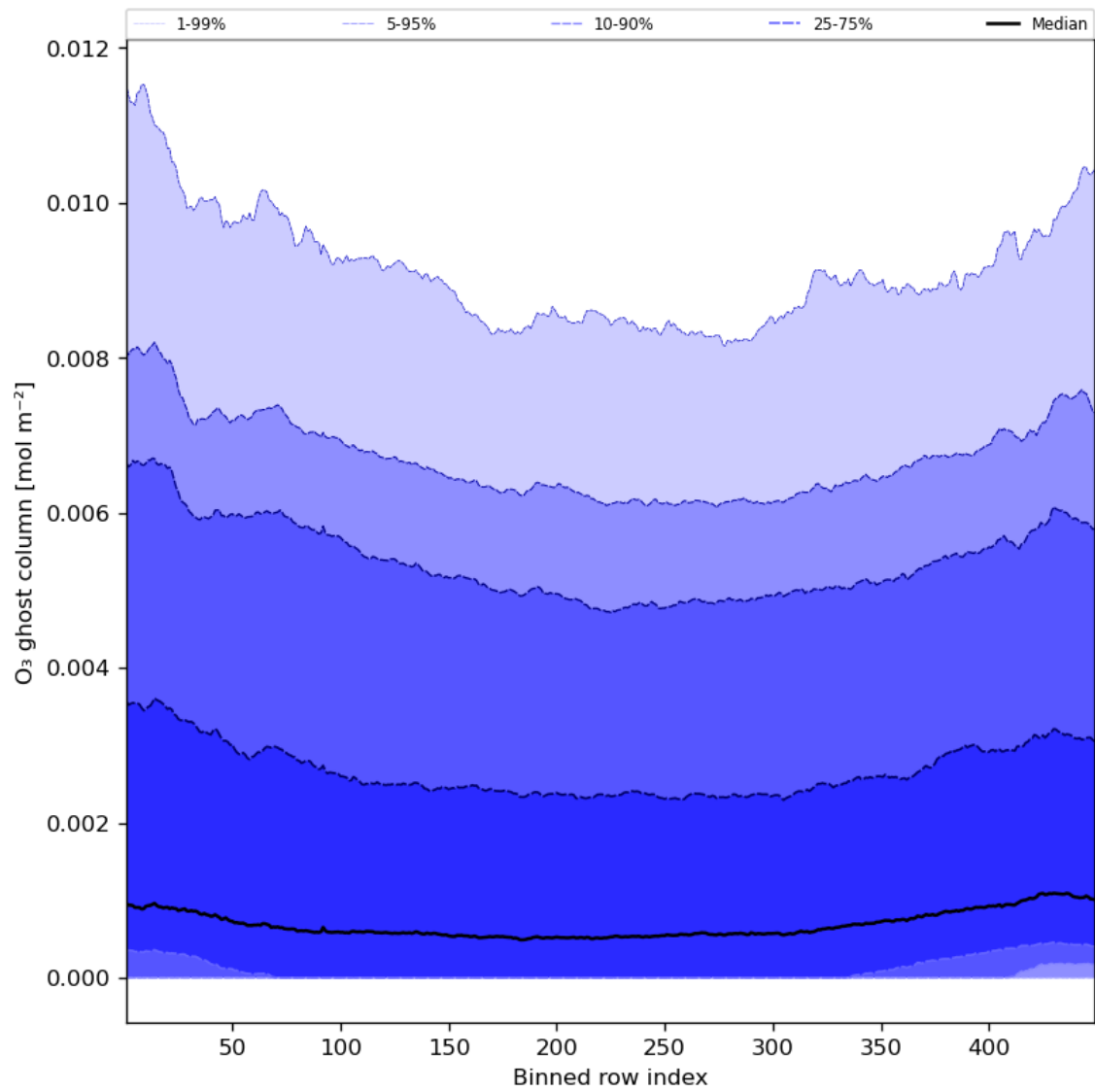
Figure 32: Along track statistics of “O 3 ghost column” for 2024-07-12 to 2024-07-14
