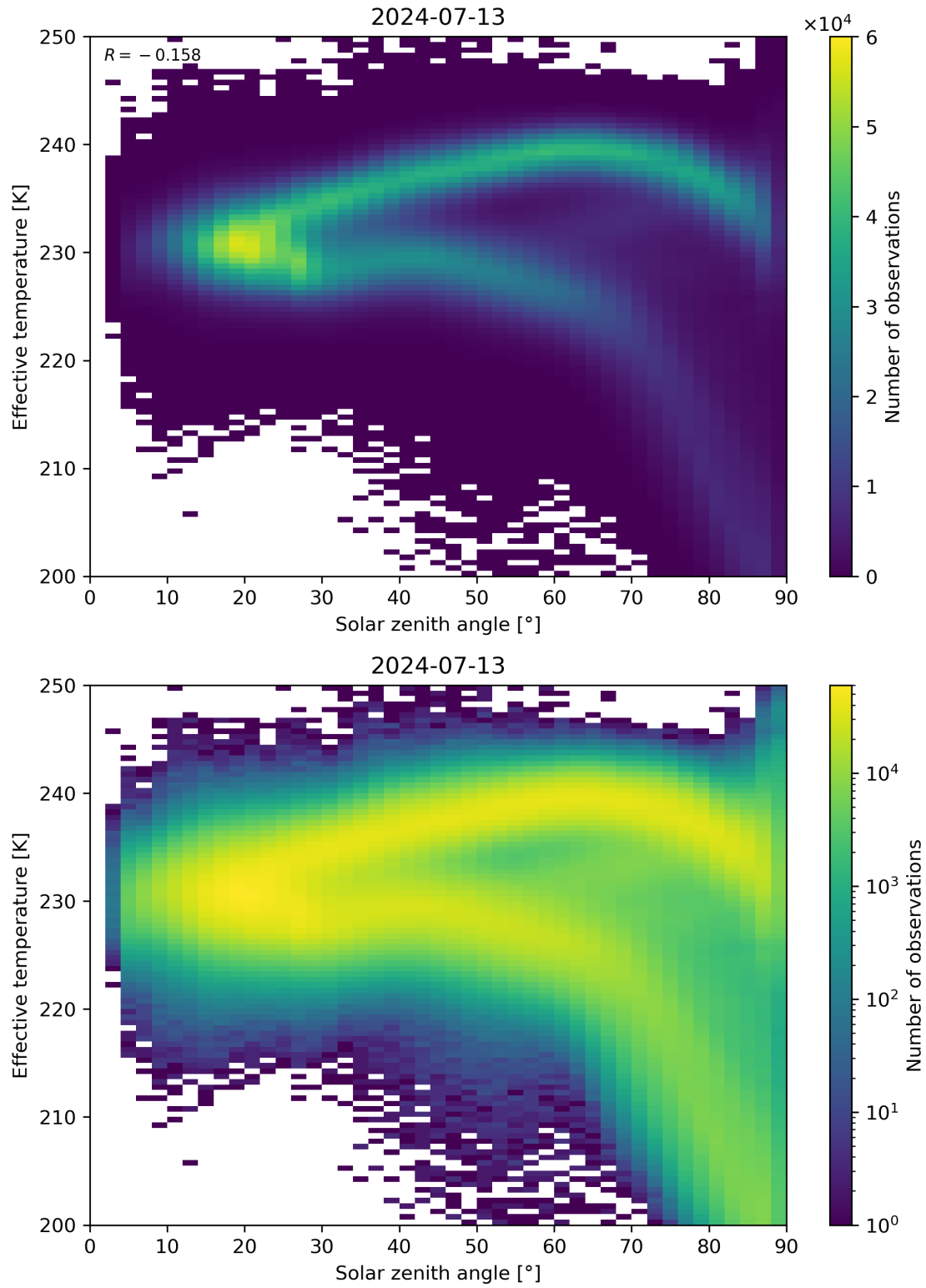
Figure 45: Scatter density plot of “Solar zenith angle” against “Effective temperature” for 2024-07-12 to 2024-07-14.
