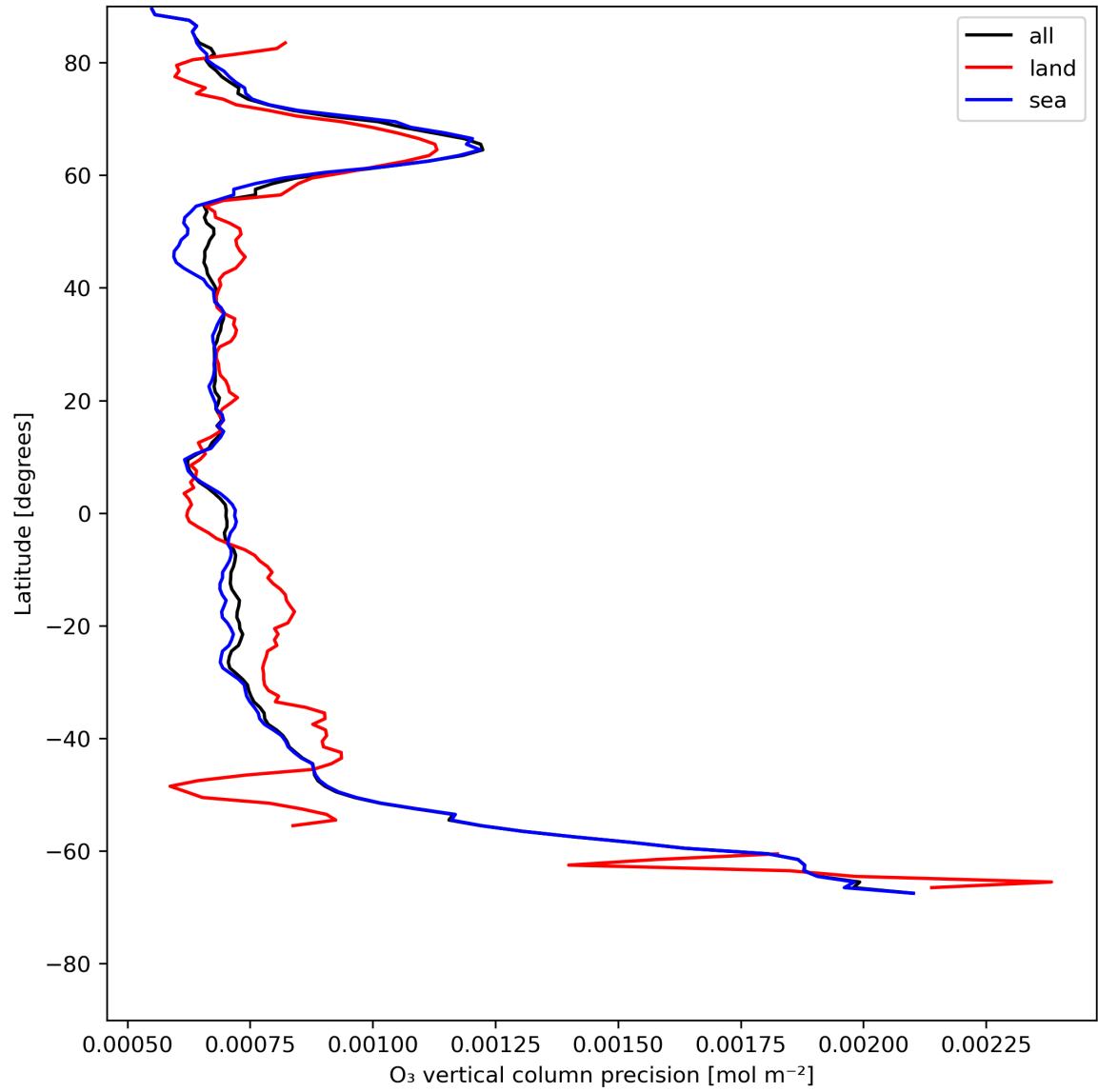
Figure 15: Zonal average of “O 3 vertical column precision” for 2024-07-12 to 2024-07-14.
