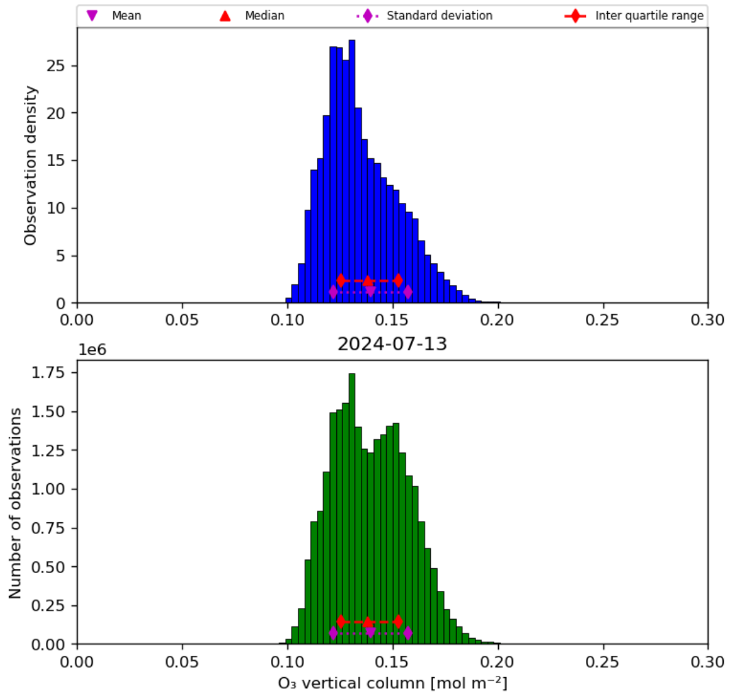
Figure 21: Histogram of “O 3 vertical column” for 2024-07-12 to 2024-07-14
