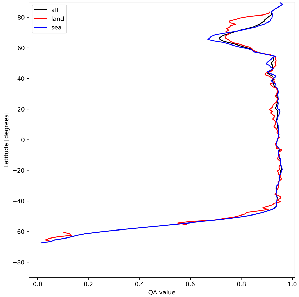
Figure 13: Zonal average of “QA value” for 2024-07-12 to 2024-07-14.
