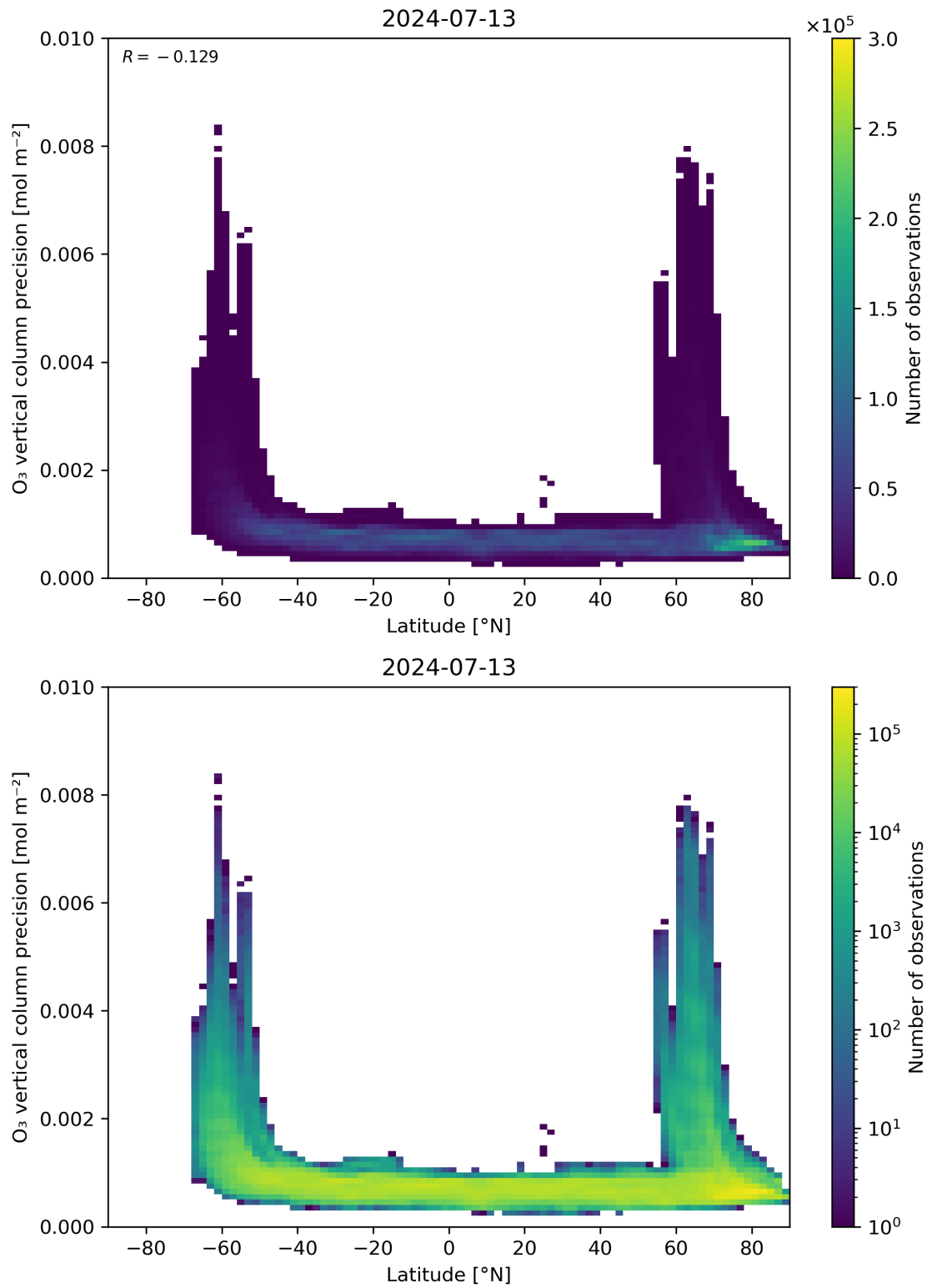
Figure 37: Scatter density plot of “Latitude” against “O 3 vertical column precision” for 2024-07-12 to 2024-07-14.
