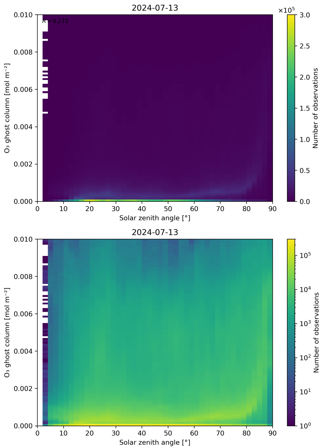
Figure 46: Scatter density plot of “Solar zenith angle” against “O 3 ghost column” for 2024-07-12 to 2024-07-14.
