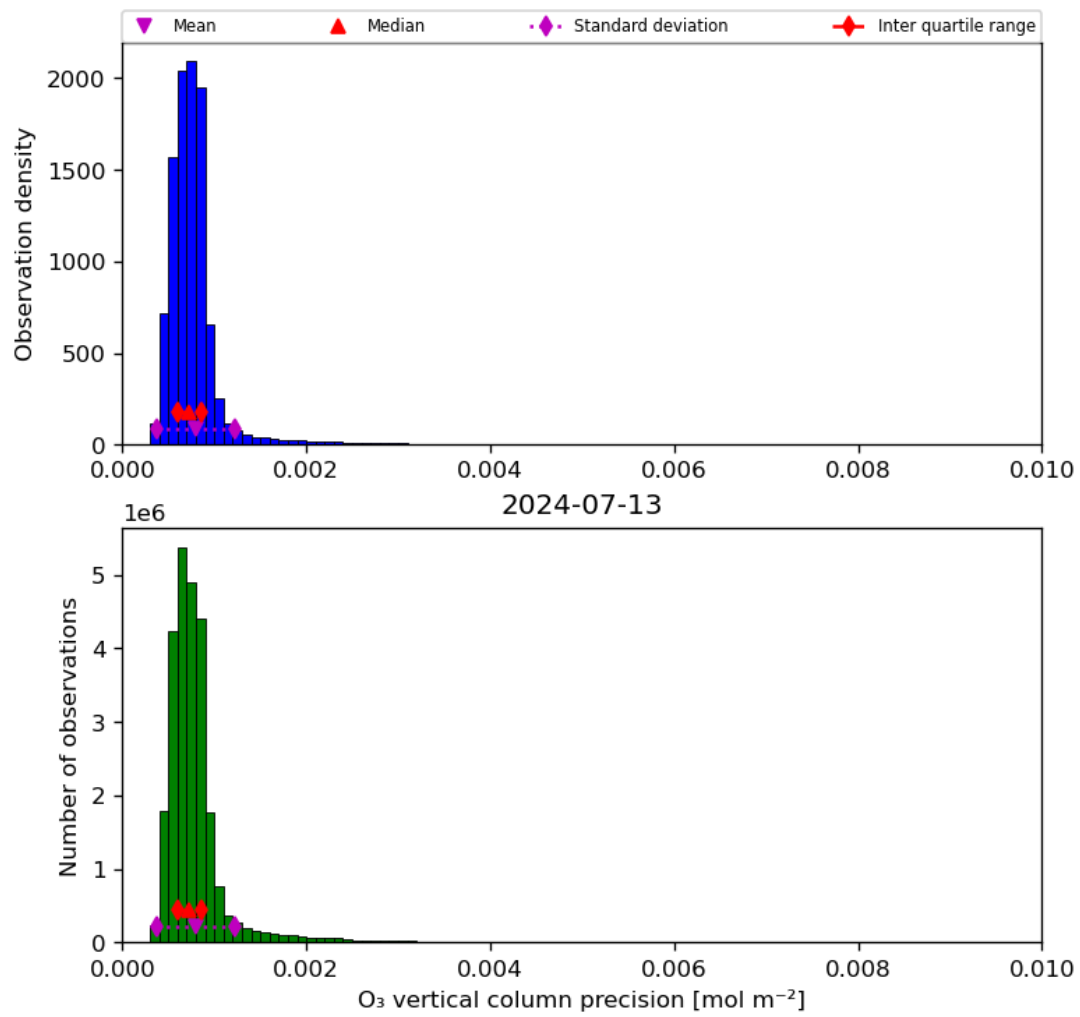
Figure 22: Histogram of “O 3 vertical column precision” for 2024-07-12 to 2024-07-14
