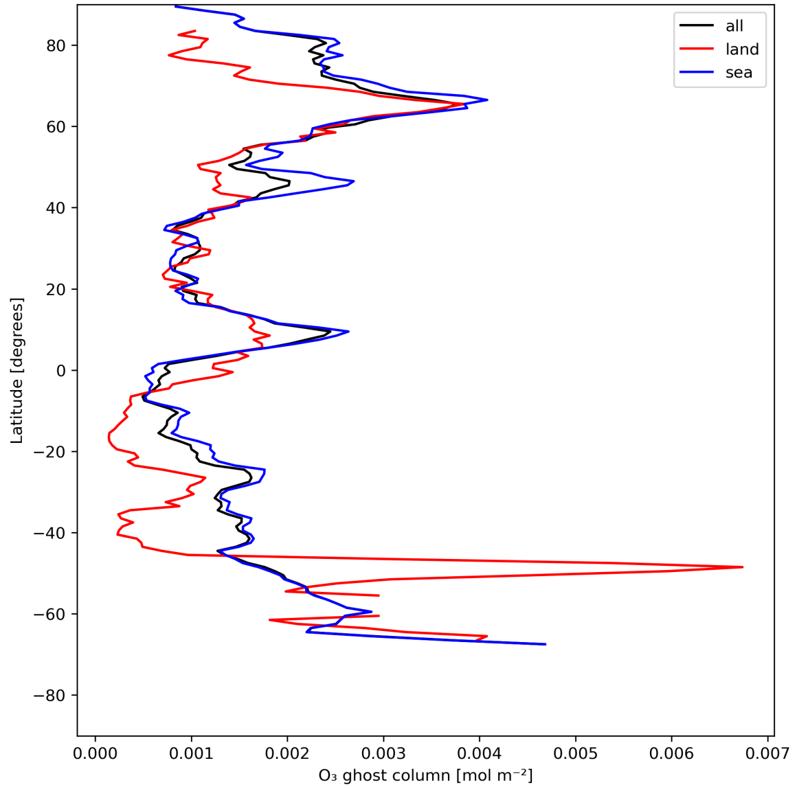
Figure 18: Zonal average of "O 3 ghost column" for 2024-07-12 to 2024-07-14.
