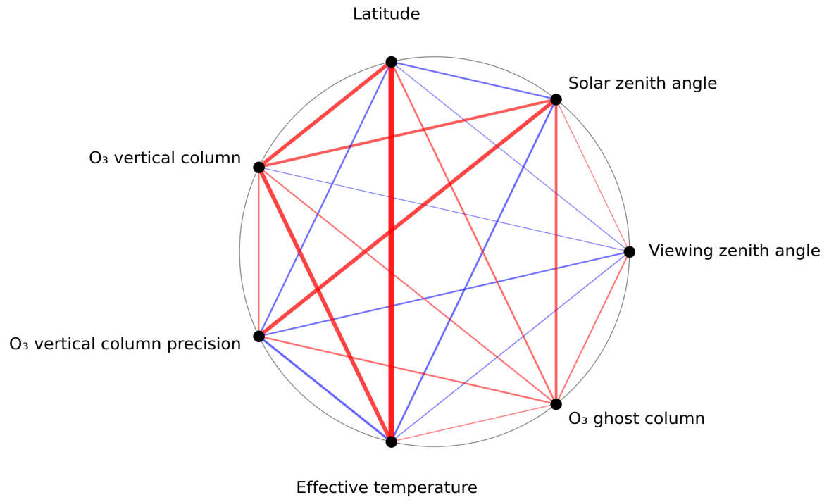
Figure 1: Map of correlation graph for 2024-07-12 to 2024-07-14.
