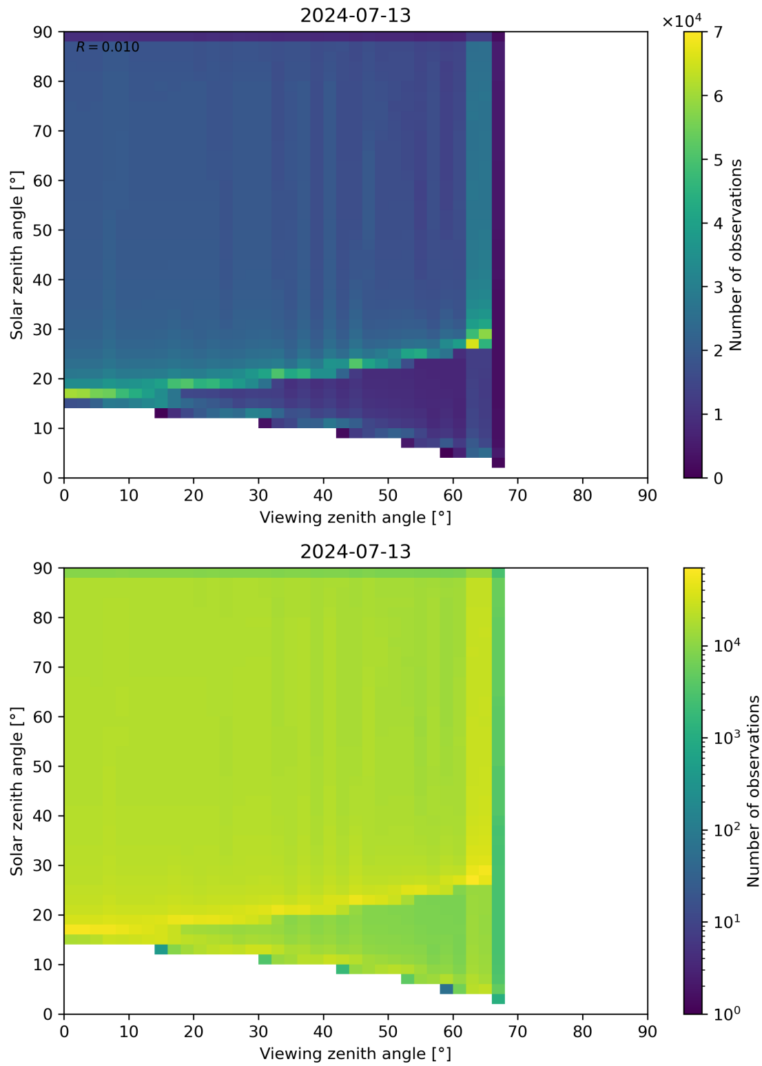
Figure 54: Scatter density plot of “Viewing zenith angle” against “Solar zenith angle” for 2024-07-12 to 2024-07-14.
