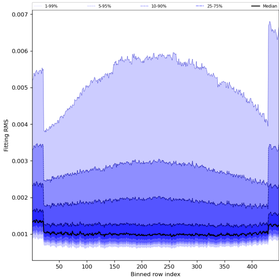
Figure 30: Along track statistics of “Fitting RMS” for 2024-07-12 to 2024-07-14
