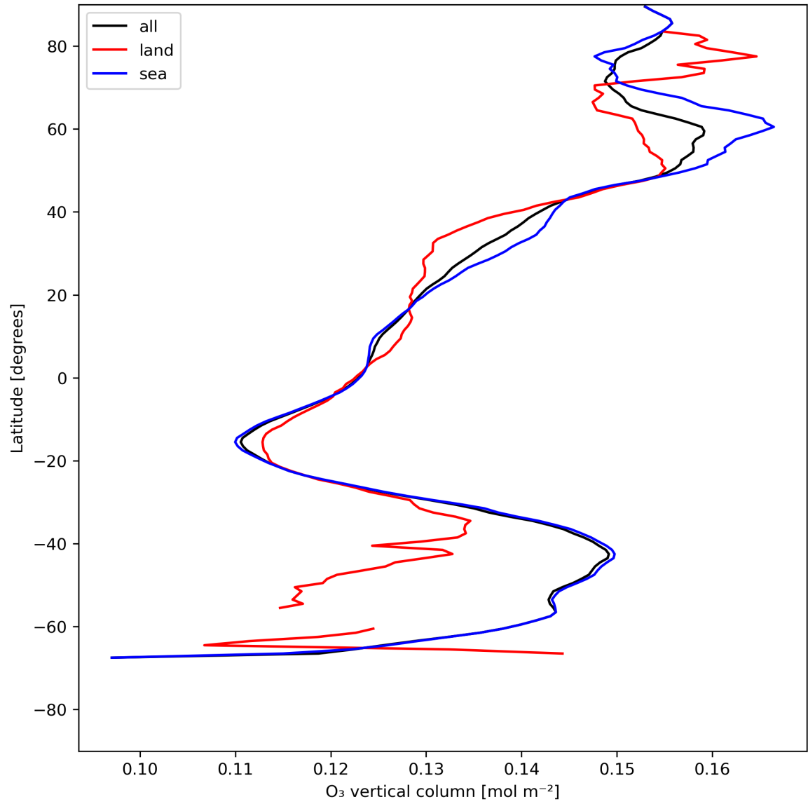
Figure 14: Zonal average of “O 3 vertical column” for 2024-07-12 to 2024-07-14.
