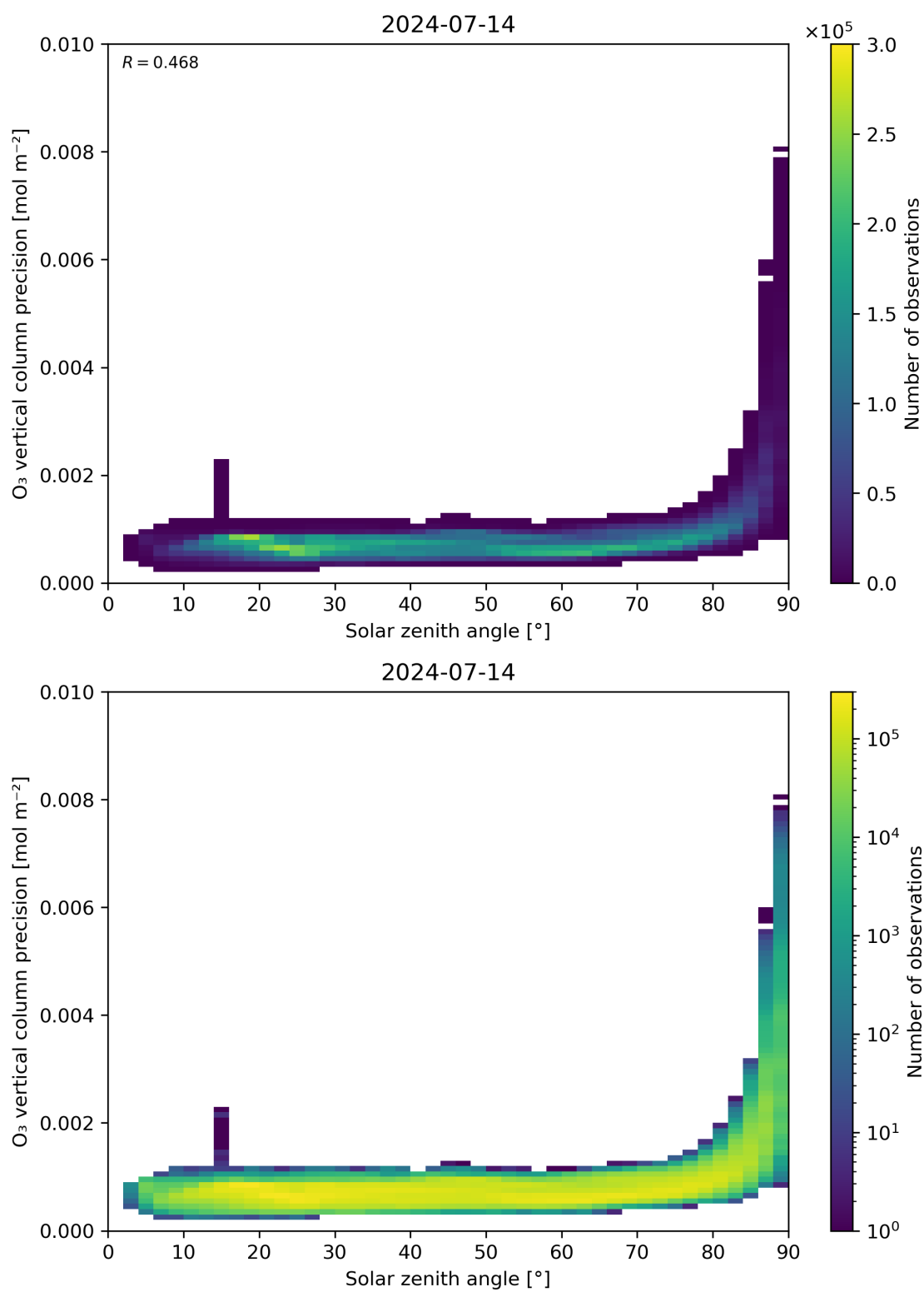
Figure 48: Scatter density plot of “Solar zenith angle” against “O 3 vertical column precision” for 2024-07-13 to 2024-07-15.
