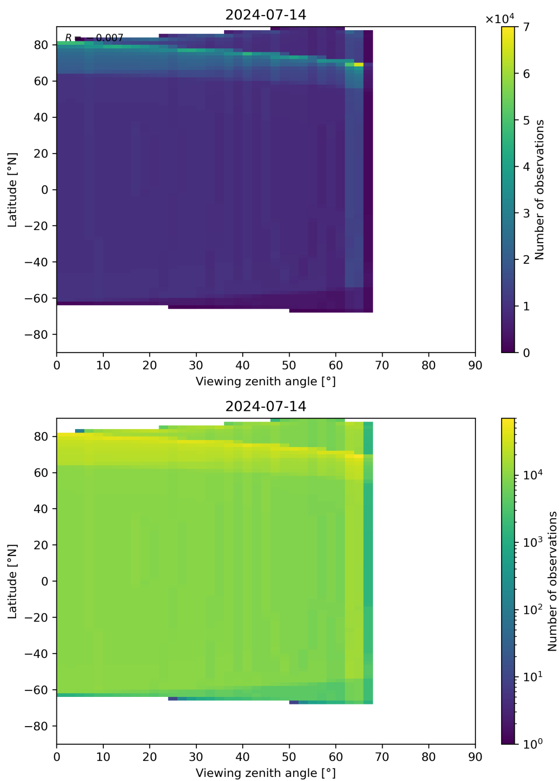
Figure 49: Scatter density plot of “Viewing zenith angle” against “Latitude” for 2024-07-13 to 2024-07-15.
