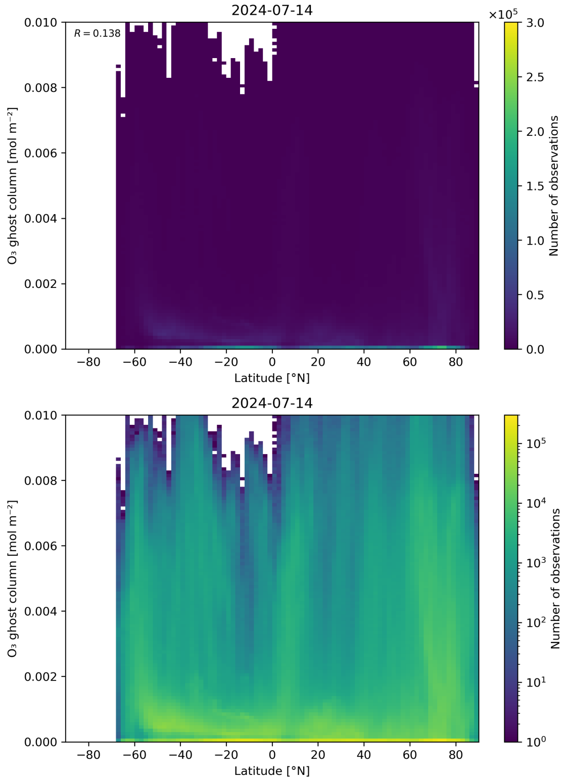
Figure 35: Scatter density plot of “Latitude” against “O 3 ghost column” for 2024-07-13 to 2024-07-15.
