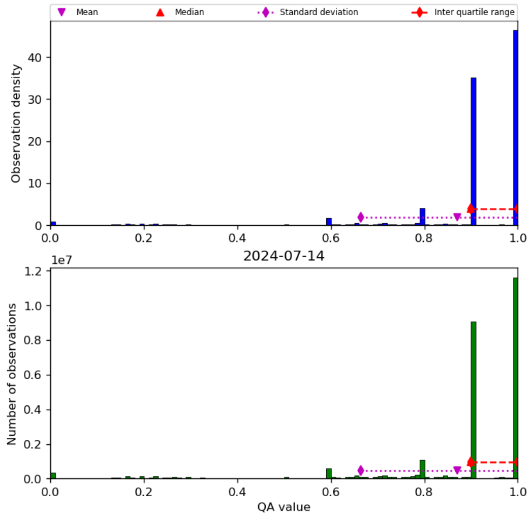
Figure 20: Histogram of “QA value” for 2024-07-13 to 2024-07-15
