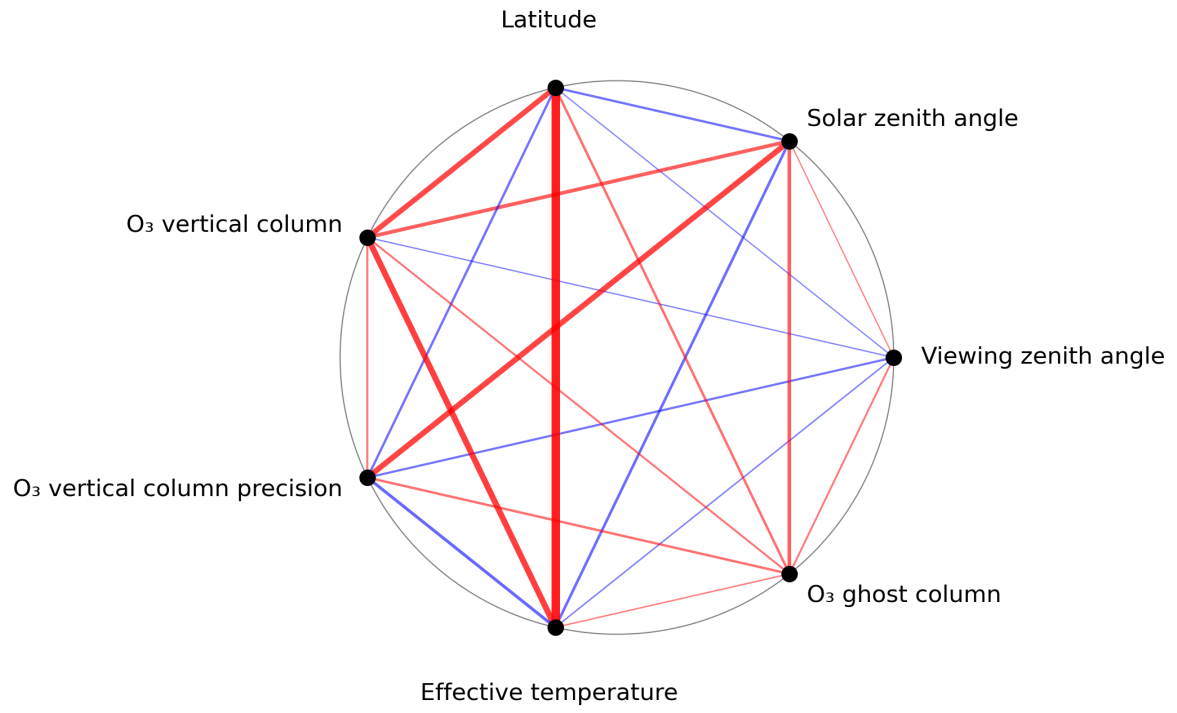
Figure 1: Map of correlation graph for 2024-07-13 to 2024-07-15.
