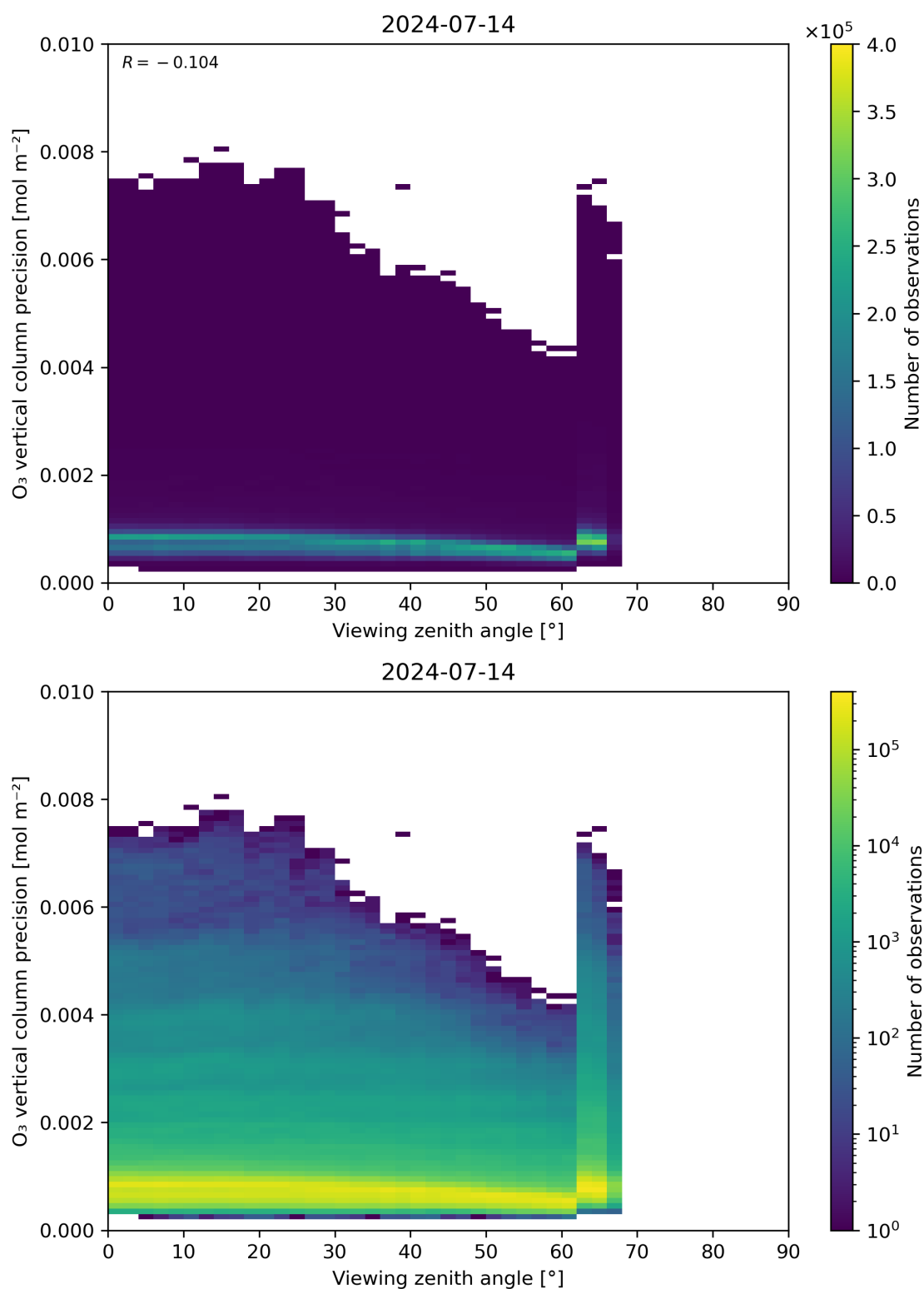
Figure 53: Scatter density plot of “Viewing zenith angle” against “O 3 vertical column precision” for 2024-07-13 to 2024-07-15.
