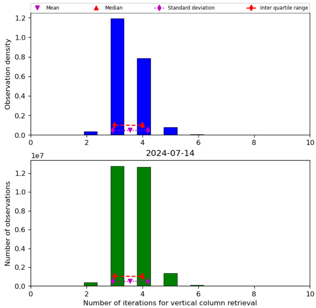
Figure 26: Histogram of “Number of iterations for vertical column retrieval” for 2024-07-13 to 2024-07-15
