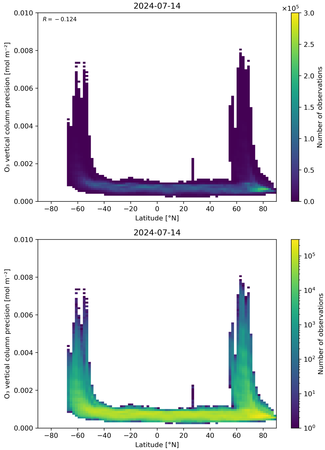
Figure 37: Scatter density plot of “Latitude” against “O 3 vertical column precision” for 2024-07-13 to 2024-07-15.
