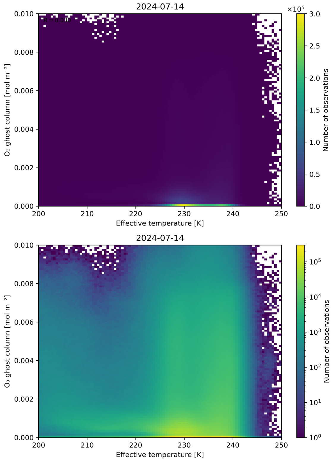
Figure 38: Scatter density plot of “Effective temperature” against “O 3 ghost column” for 2024-07-13 to 2024-07-15.
