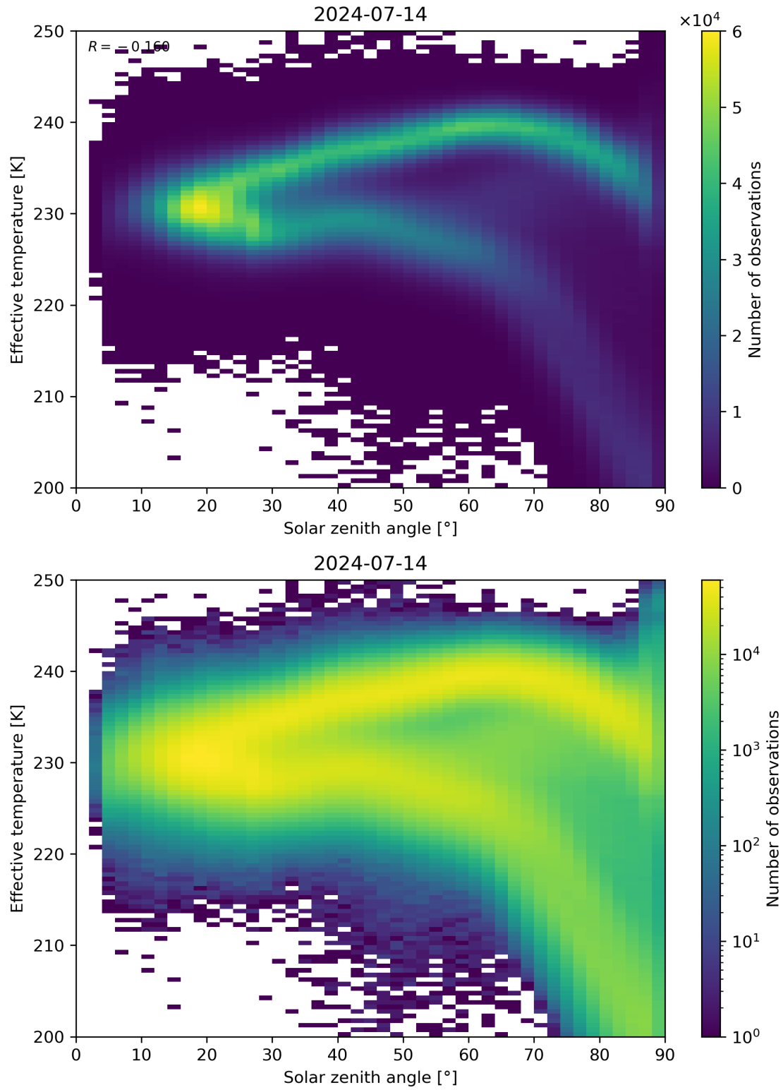
Figure 45: Scatter density plot of “Solar zenith angle” against “Effective temperature” for 2024-07-13 to 2024-07-15.
