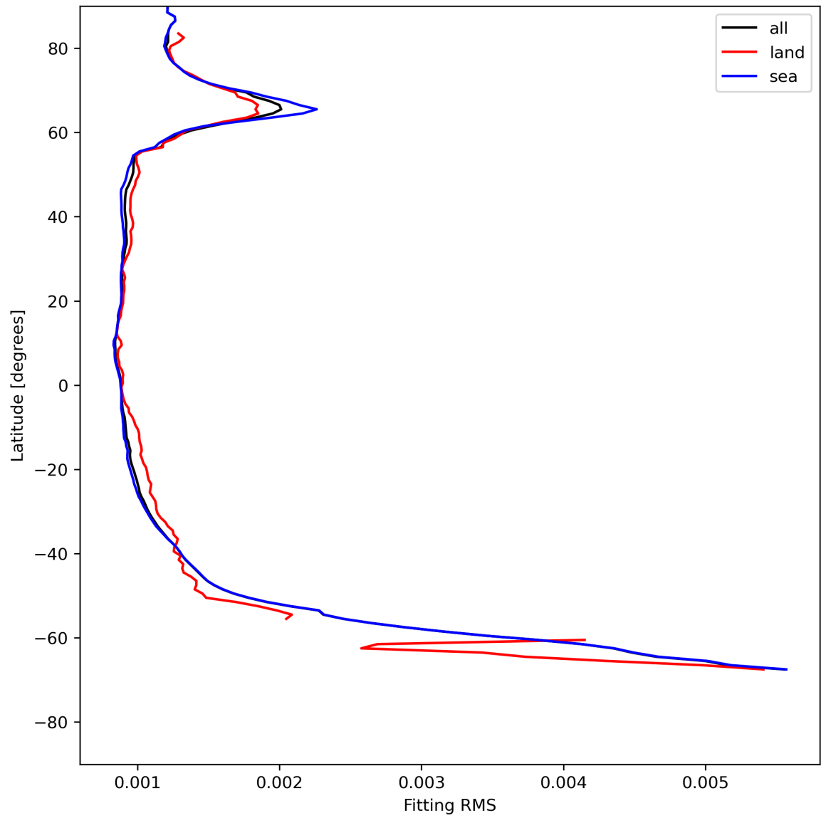
Figure 16: Zonal average of “Fitting RMS” for 2024-07-13 to 2024-07-15.
