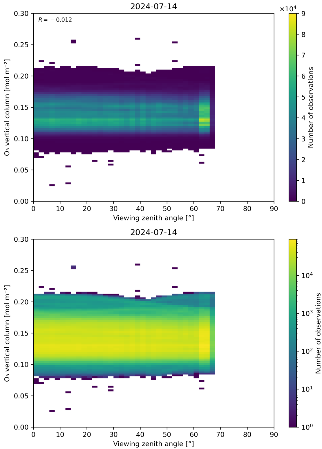
Figure 52: Scatter density plot of “Viewing zenith angle” against “O 3 vertical column” for 2024-07-13 to 2024-07-15.
