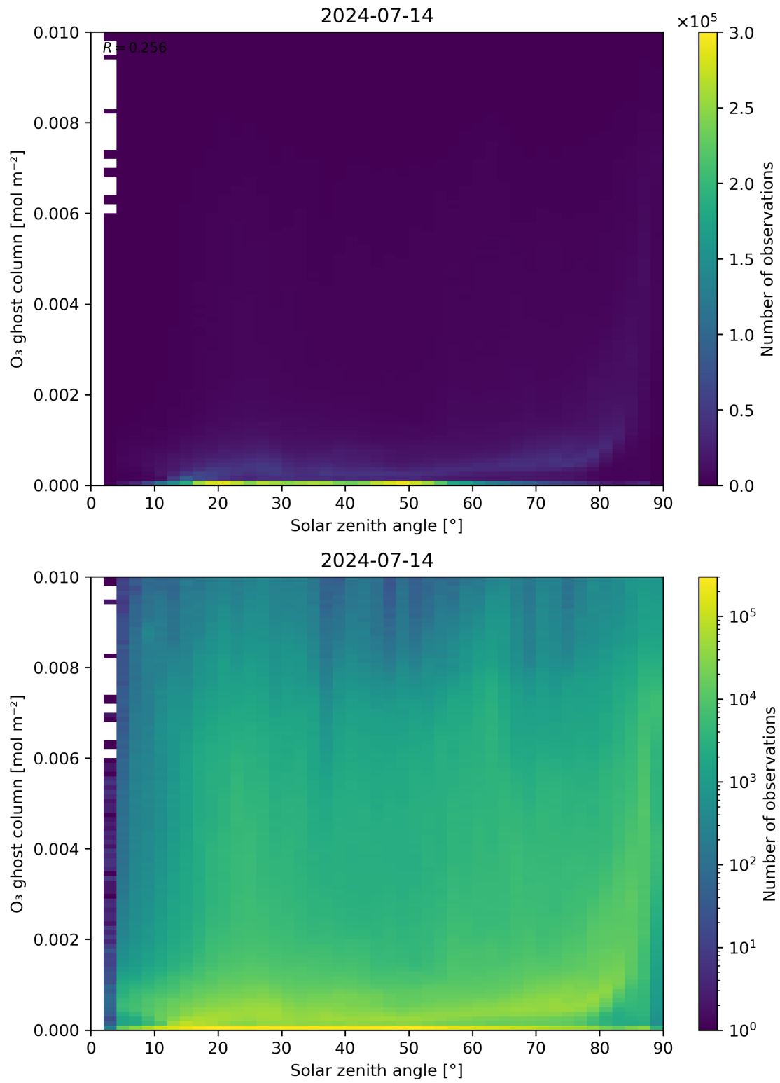
Figure 46: Scatter density plot of “Solar zenith angle” against “O 3 ghost column” for 2024-07-13 to 2024-07-15.
