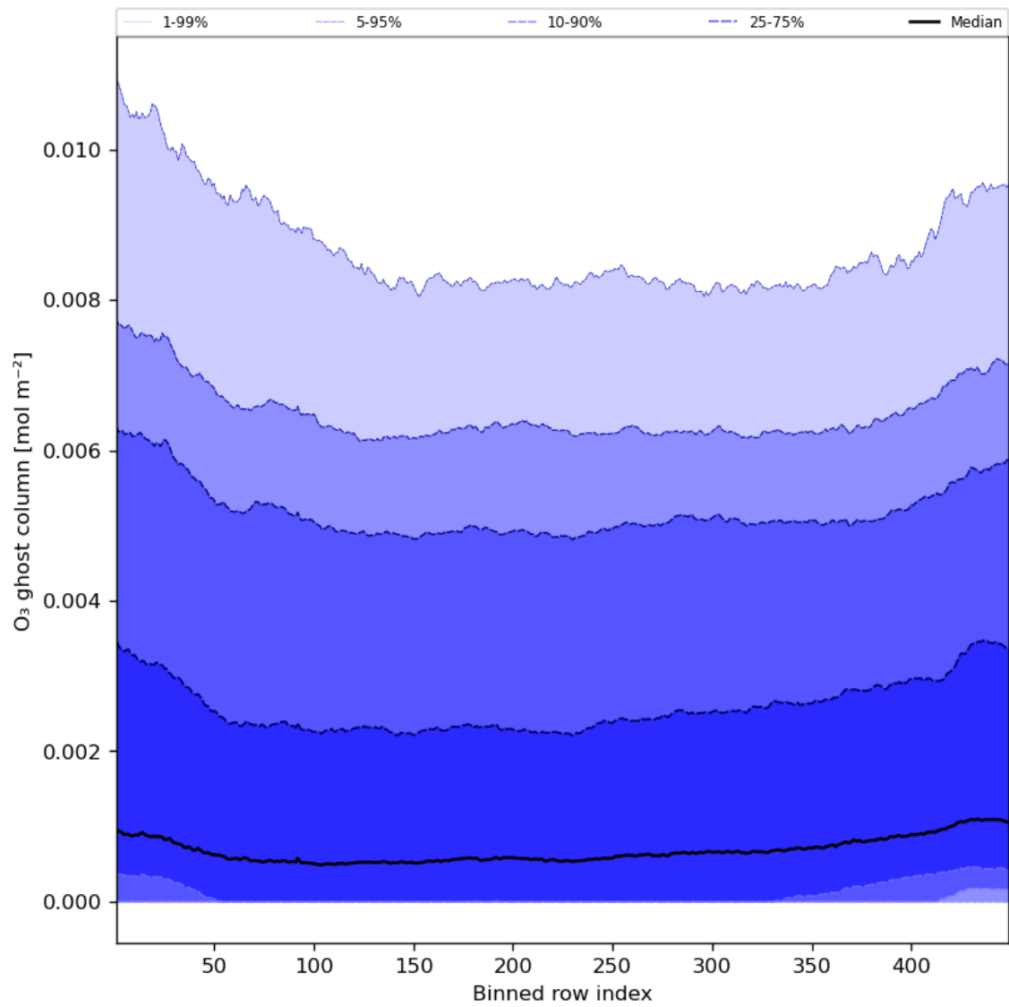
Figure 32: Along track statistics of “O 3 ghost column” for 2024-07-13 to 2024-07-15
