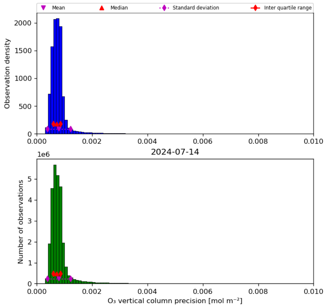
Figure 22: Histogram of “O 3 vertical column precision” for 2024-07-13 to 2024-07-15
