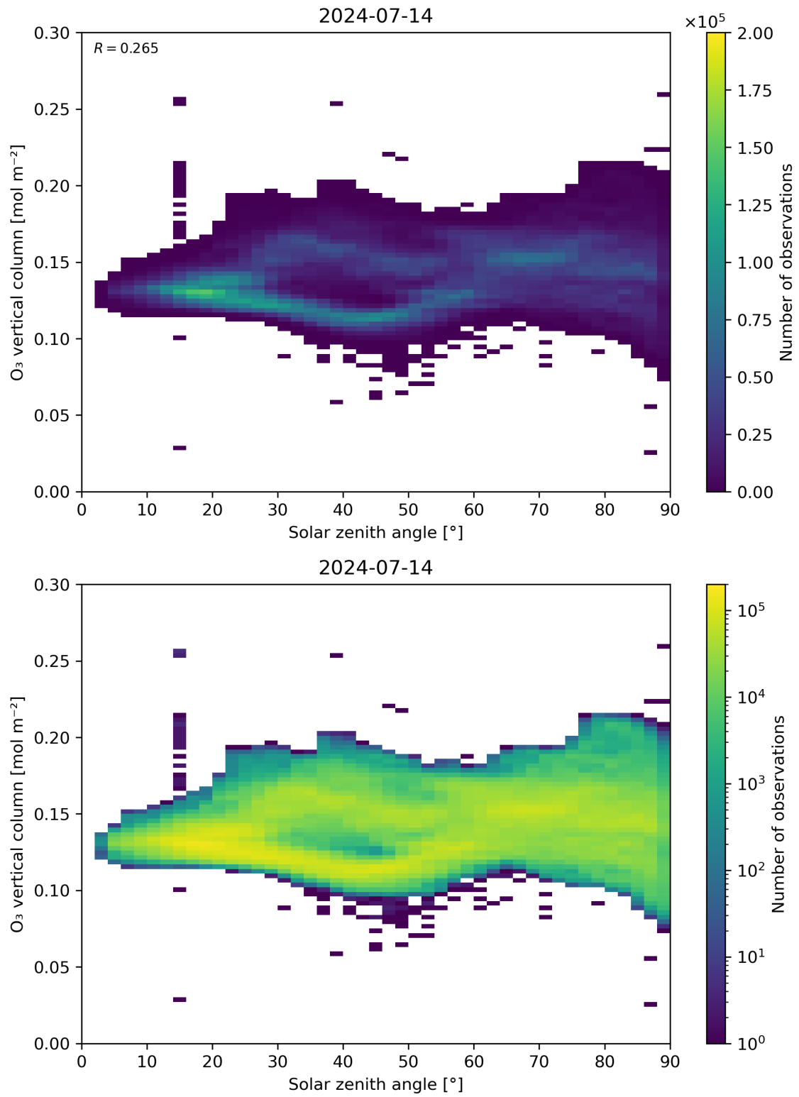
Figure 47: Scatter density plot of “Solar zenith angle” against “O 3 vertical column” for 2024-07-13 to 2024-07-15.
