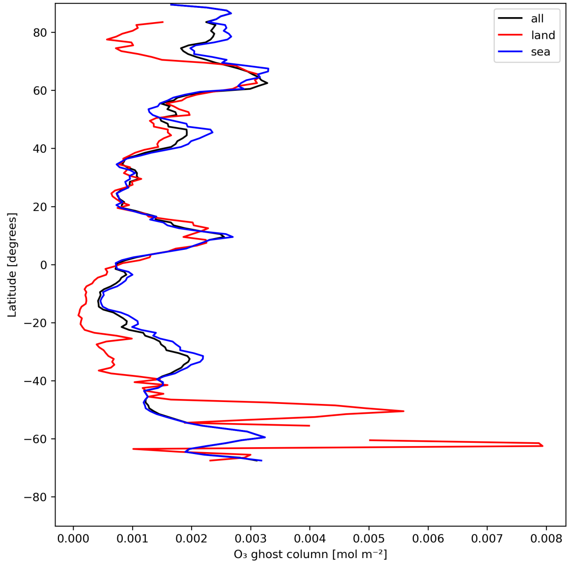
Figure 18: Zonal average of “O 3 ghost column” for 2024-07-13 to 2024-07-15.
