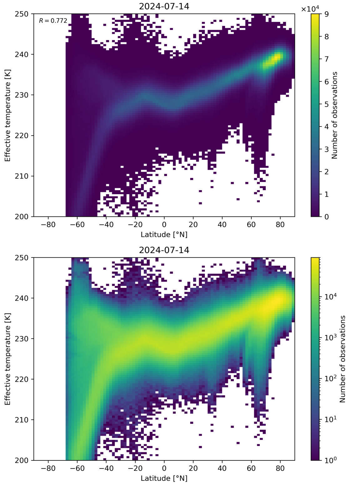
Figure 34: Scatter density plot of “Latitude” against “Effective temperature” for 2024-07-13 to 2024-07-15.
