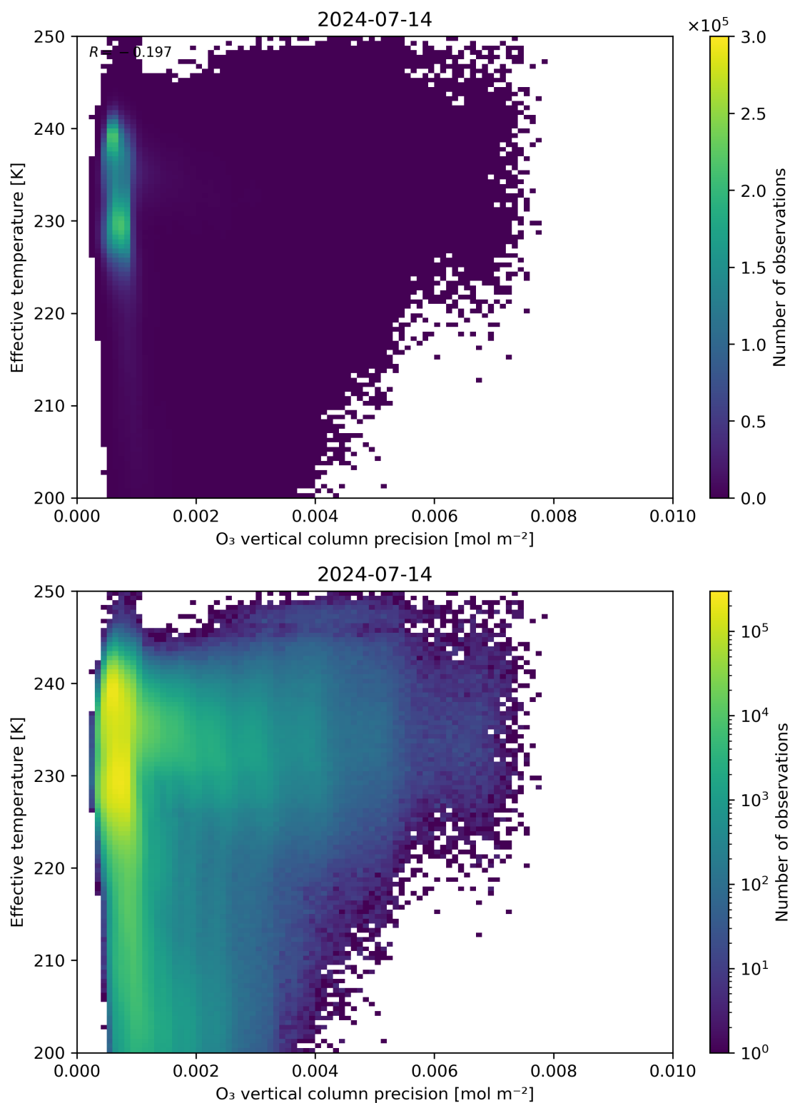
Figure 42: Scatter density plot of “O 3 vertical column precision” against “Effective temperature” for 2024-07-13 to 2024-07-15.
