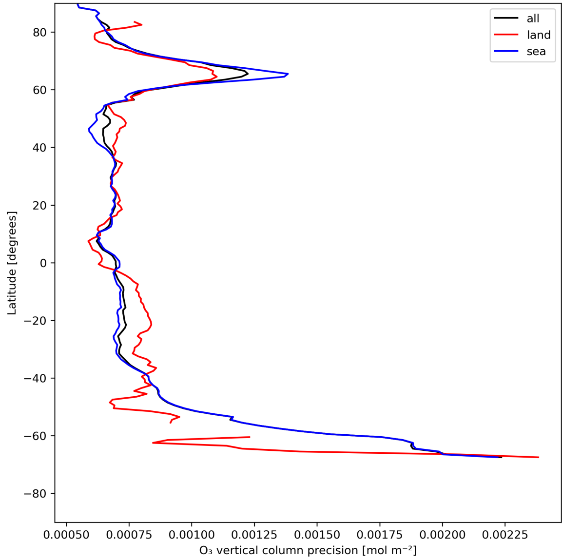
Figure 15: Zonal average of "O 3 vertical column precision" for 2024-07-13 to 2024-07-15.
