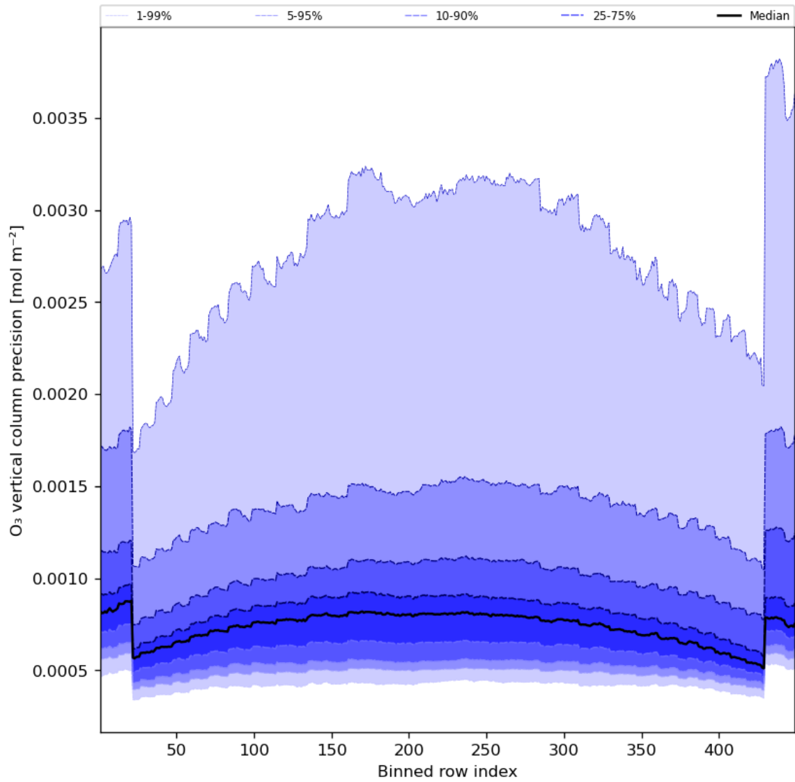
Figure 29: Along track statistics of “O 3 vertical column precision” for 2024-07-13 to 2024-07-15
