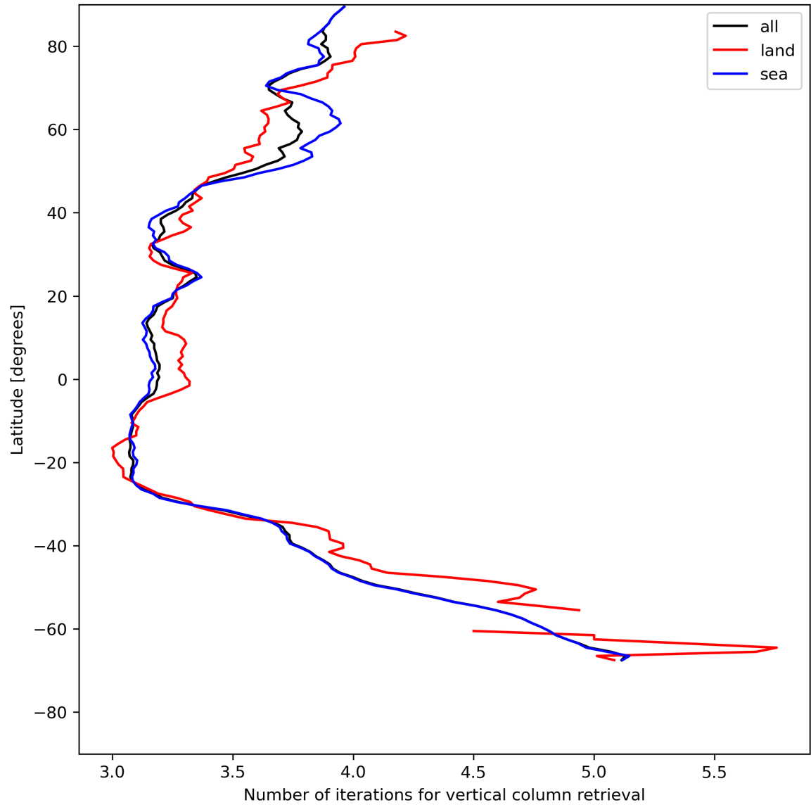
Figure 19: Zonal average of “Number of iterations for vertical column retrieval” for 2024-07-13 to 2024-07-15.
