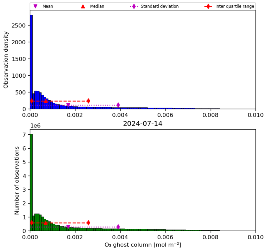
Figure 25: Histogram of “O 3 ghost column” for 2024-07-13 to 2024-07-15
