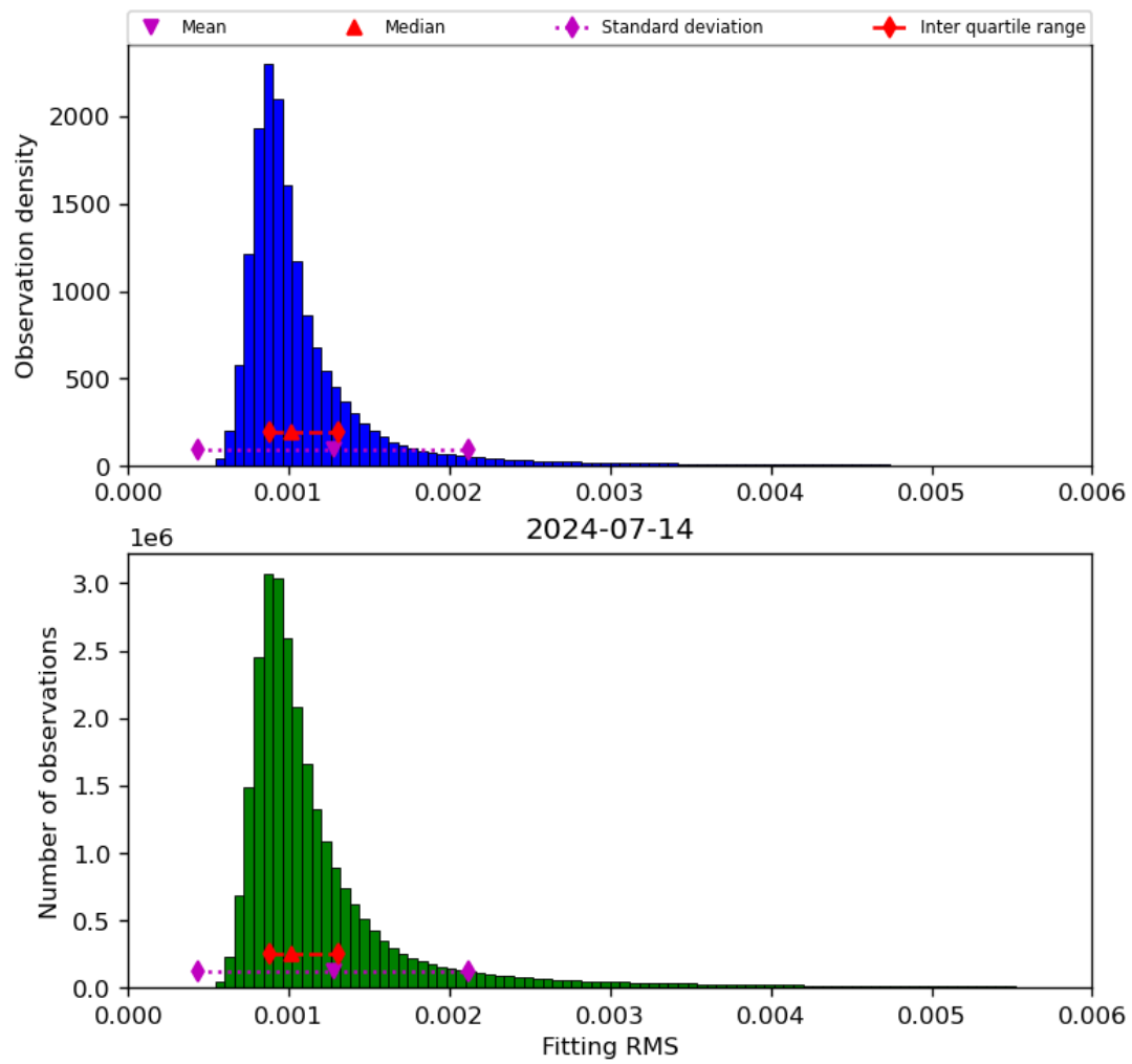
Figure 23: Histogram of “Fitting RMS” for 2024-07-13 to 2024-07-15
