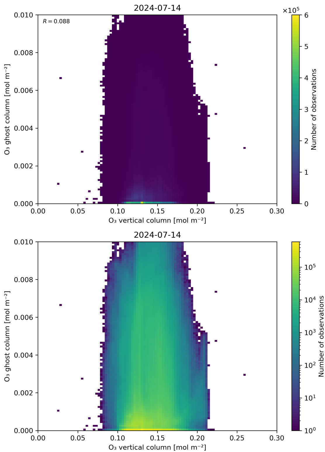
Figure 40: Scatter density plot of “O 3 vertical column” against “O 3 ghost column” for 2024-07-13 to 2024-07-15.
