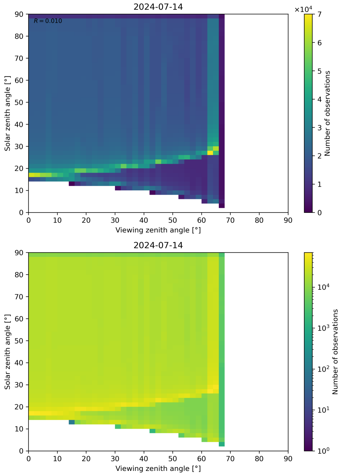
Figure 54: Scatter density plot of “Viewing zenith angle” against “Solar zenith angle” for 2024-07-13 to 2024-07-15.
