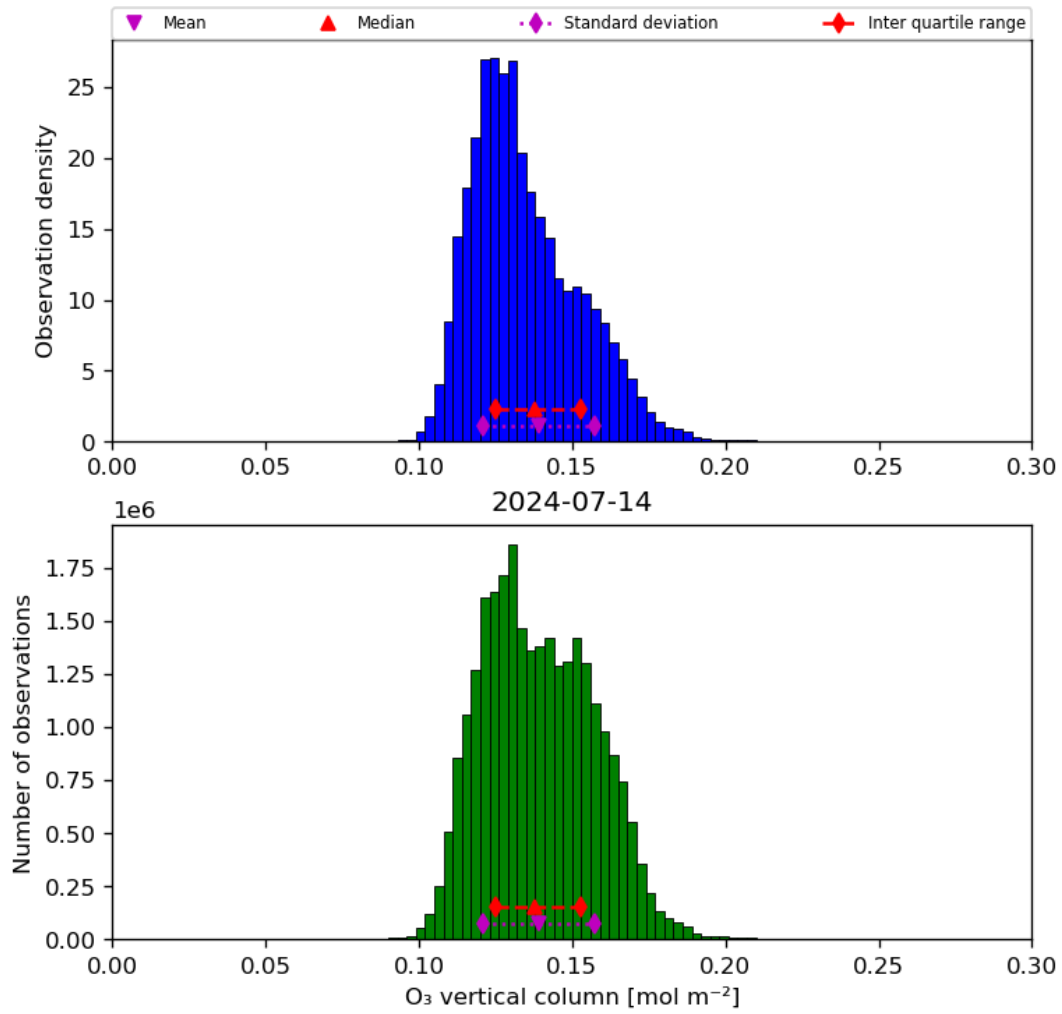
Figure 21: Histogram of “O 3 vertical column” for 2024-07-13 to 2024-07-15
