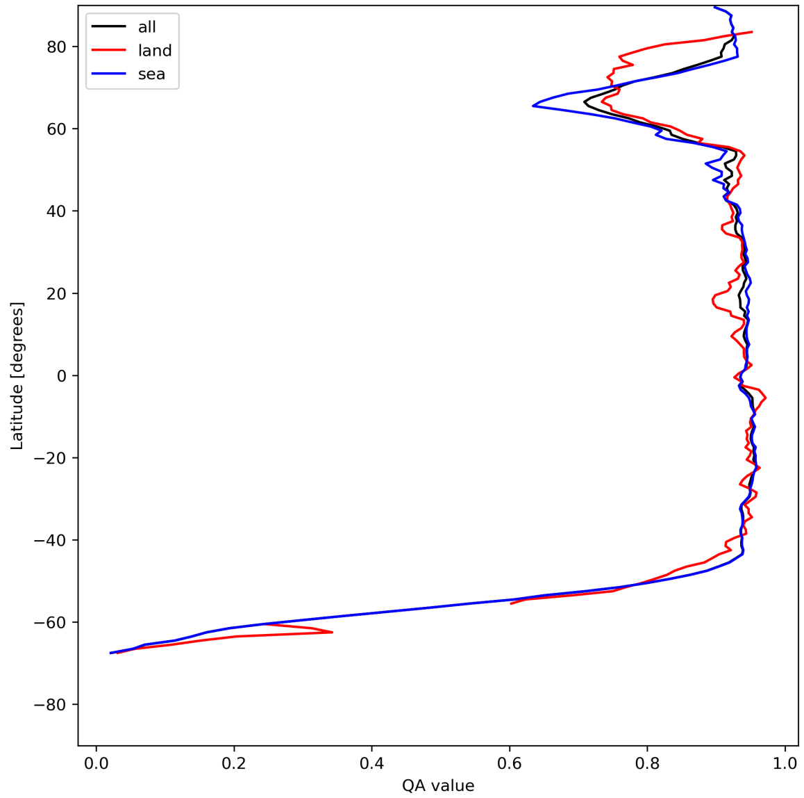
Figure 13: Zonal average of “QA value” for 2024-07-13 to 2024-07-15.
