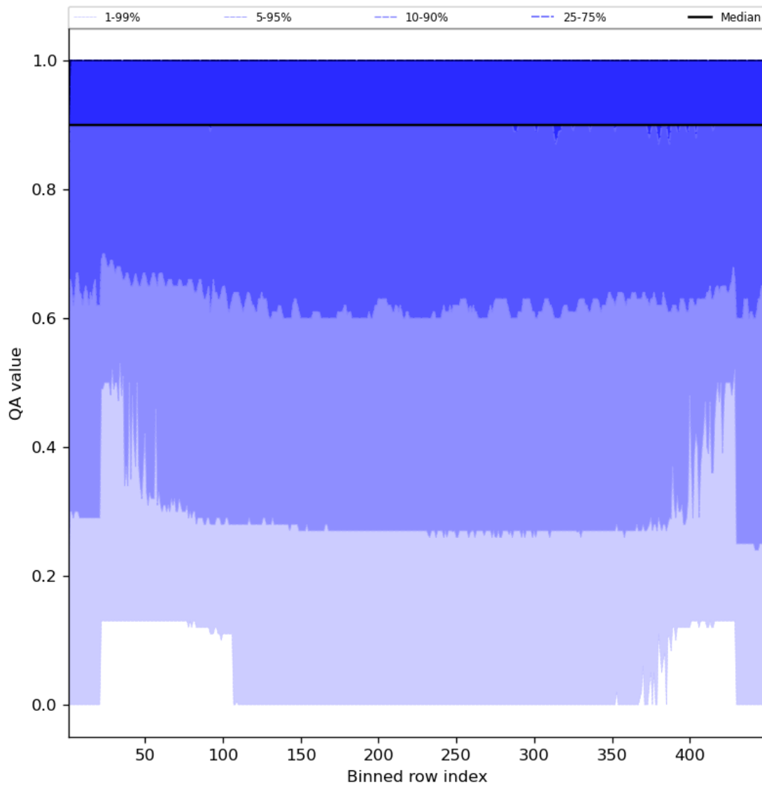
Figure 27: Along track statistics of “QA value” for 2024-07-13 to 2024-07-15
