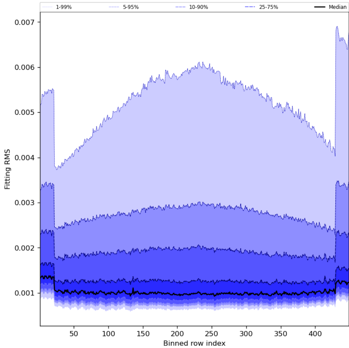
Figure 30: Along track statistics of “Fitting RMS” for 2024-07-13 to 2024-07-15
