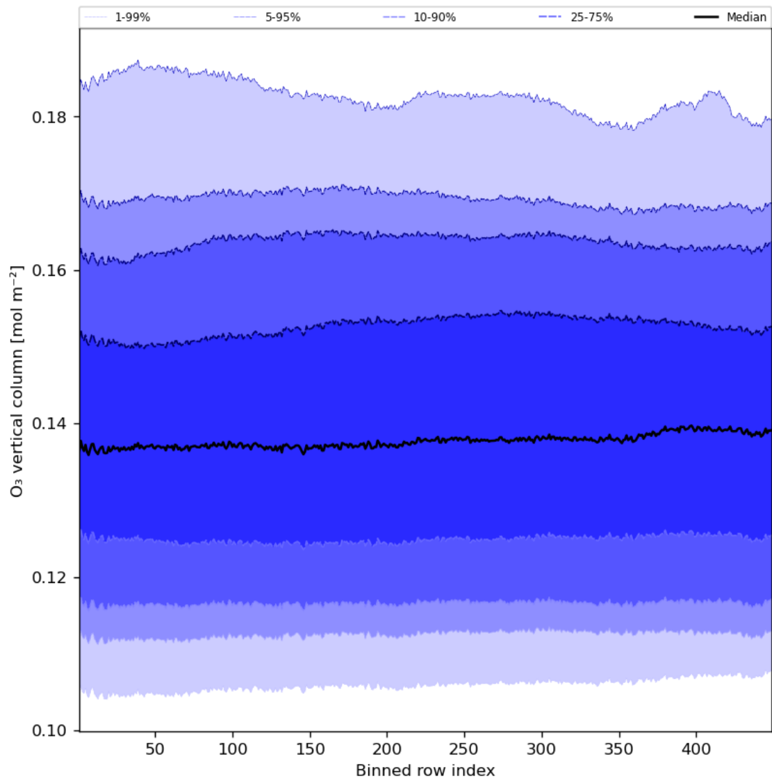
Figure 28: Along track statistics of “ O_3 vertical column” for 2024-07-13 to 2024-07-15
