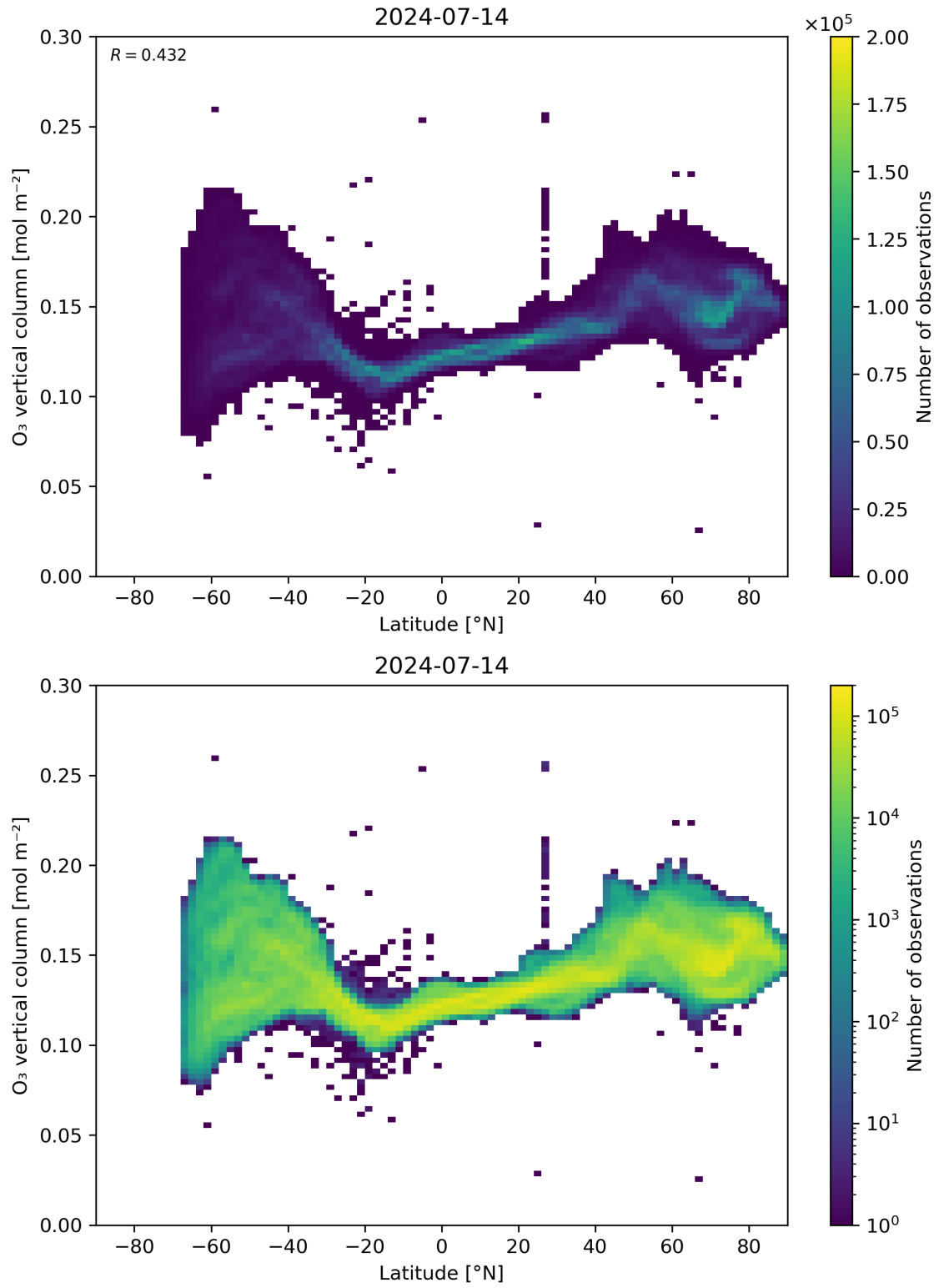
Figure 36: Scatter density plot of “Latitude” against “O 3 vertical column” for 2024-07-13 to 2024-07-15.
