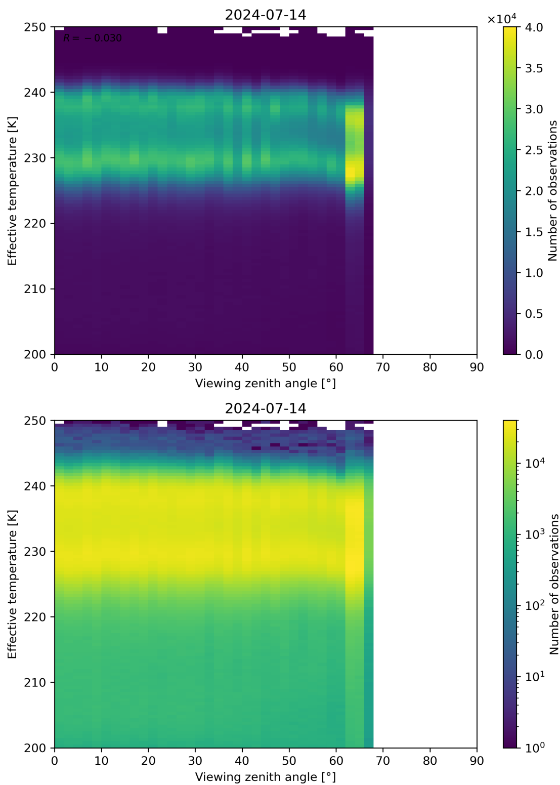
Figure 50: Scatter density plot of “Viewing zenith angle” against “Effective temperature” for 2024-07-13 to 2024-07-15.
