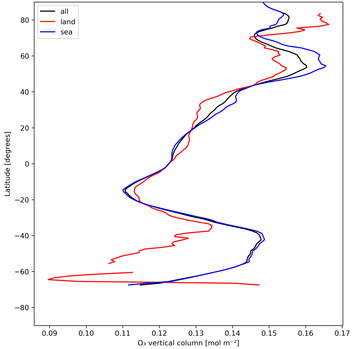
Figure 14: Zonal average of “O 3 vertical column” for 2024-07-13 to 2024-07-15.
