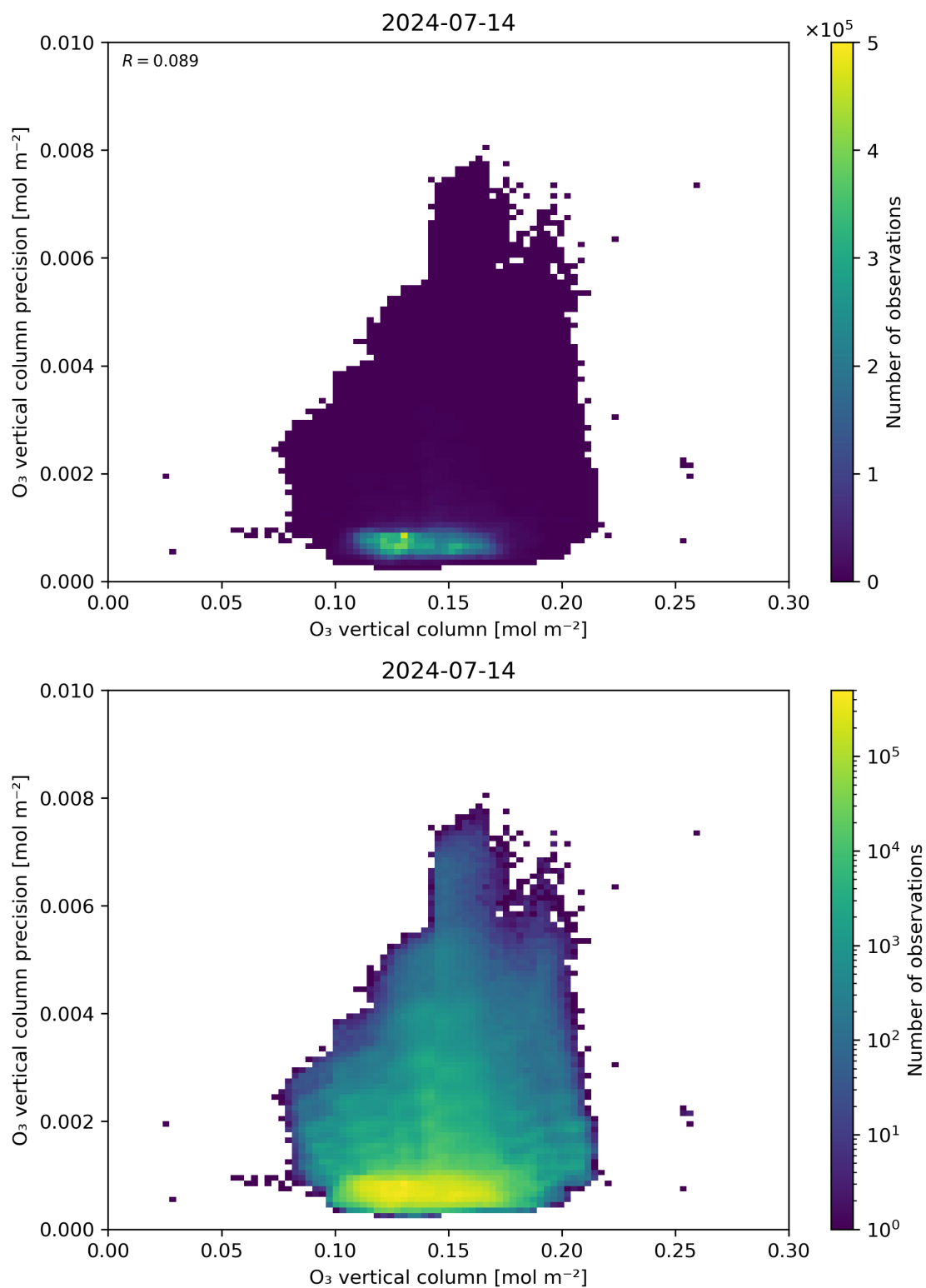
Figure 41: Scatter density plot of “O 3 vertical column” against “O 3 vertical column precision” for 2024-07-13 to 2024-07-15.
