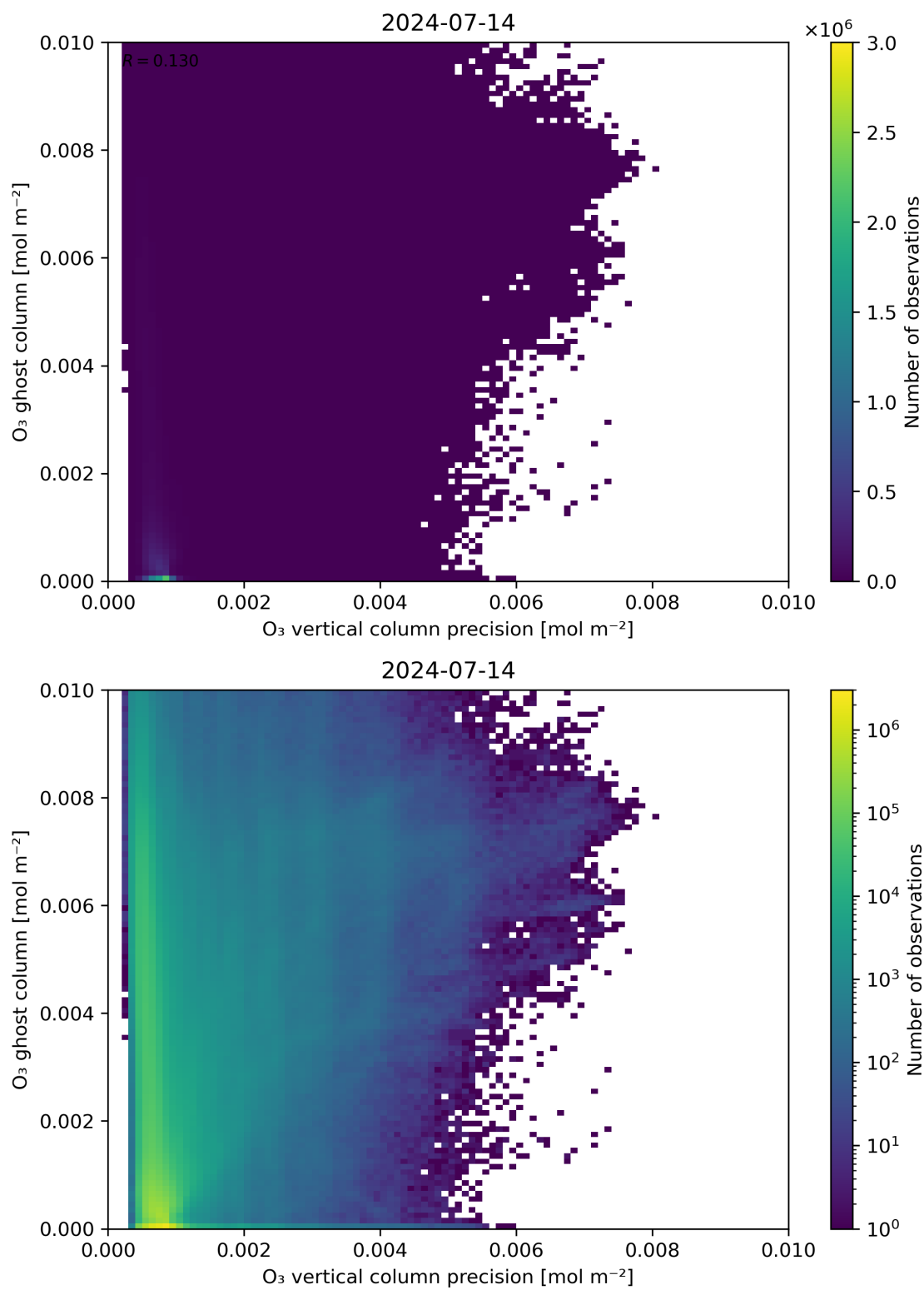
Figure 43: Scatter density plot of “ \text{O}_3 vertical column precision” against “ \text{O}_3 ghost column” for 2024-07-13 to 2024-07-15.
