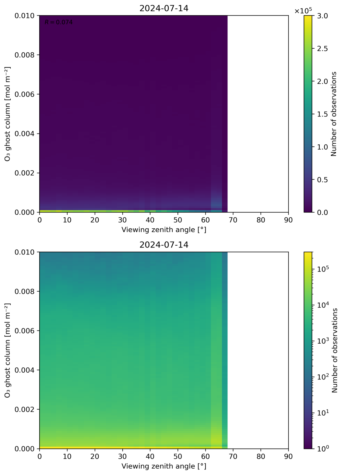
Figure 51: Scatter density plot of “Viewing zenith angle” against “O 3 ghost column” for 2024-07-13 to 2024-07-15.
