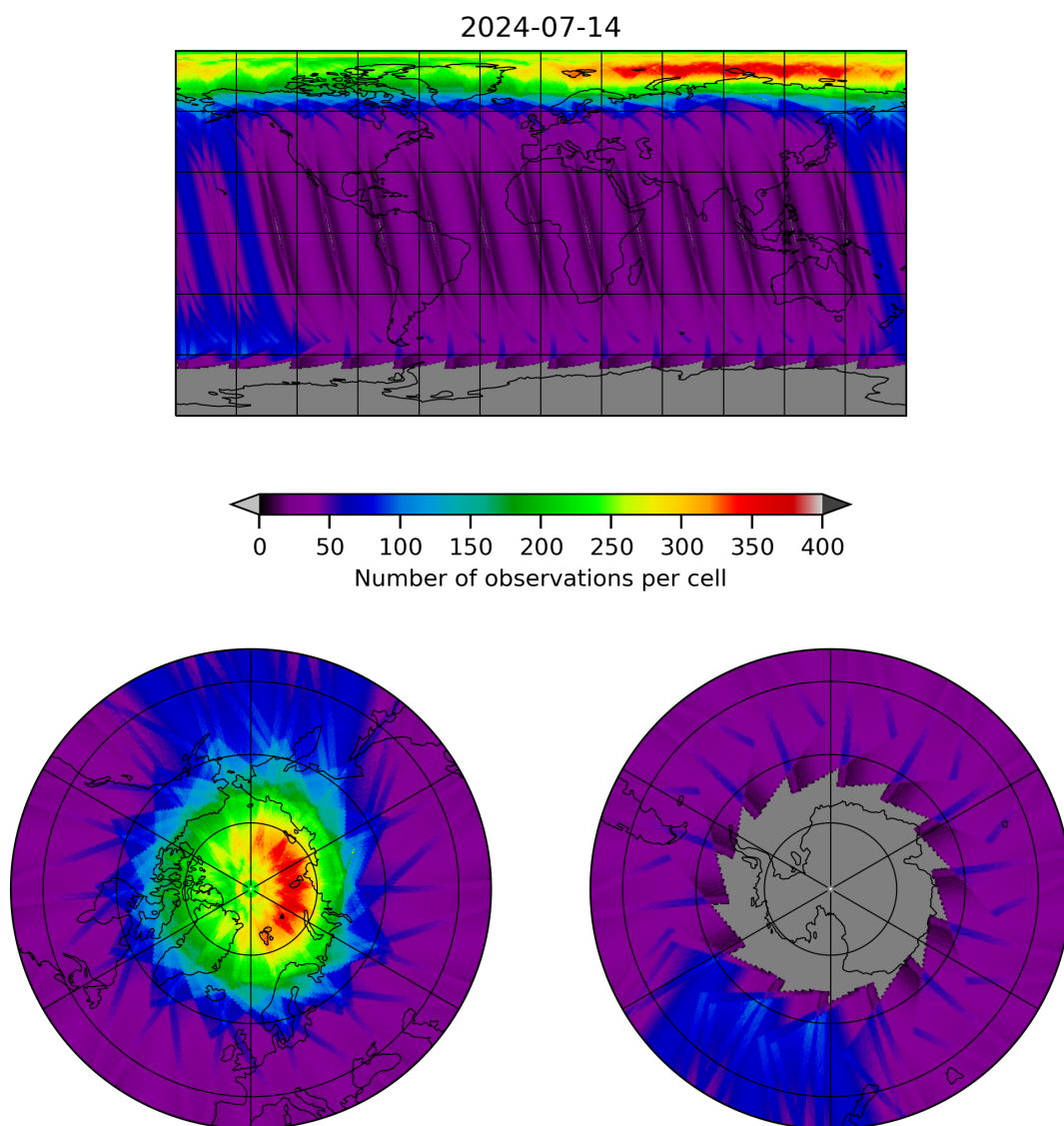
Figure 12: Map of the number of observations for 2024-07-13 to 2024-07-15
