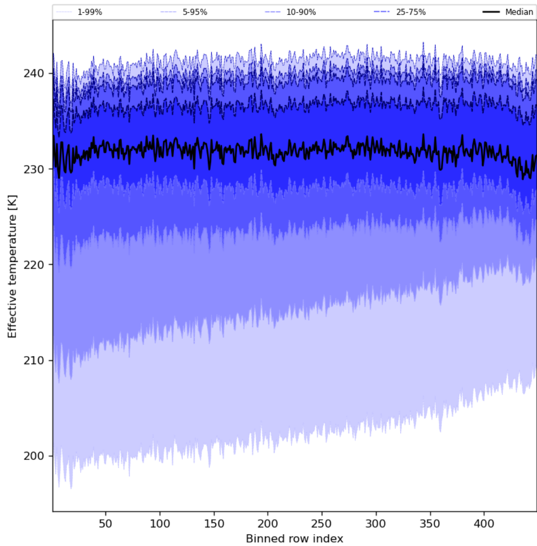
Figure 31: Along track statistics of “Effective temperature” for 2024-07-13 to 2024-07-15
