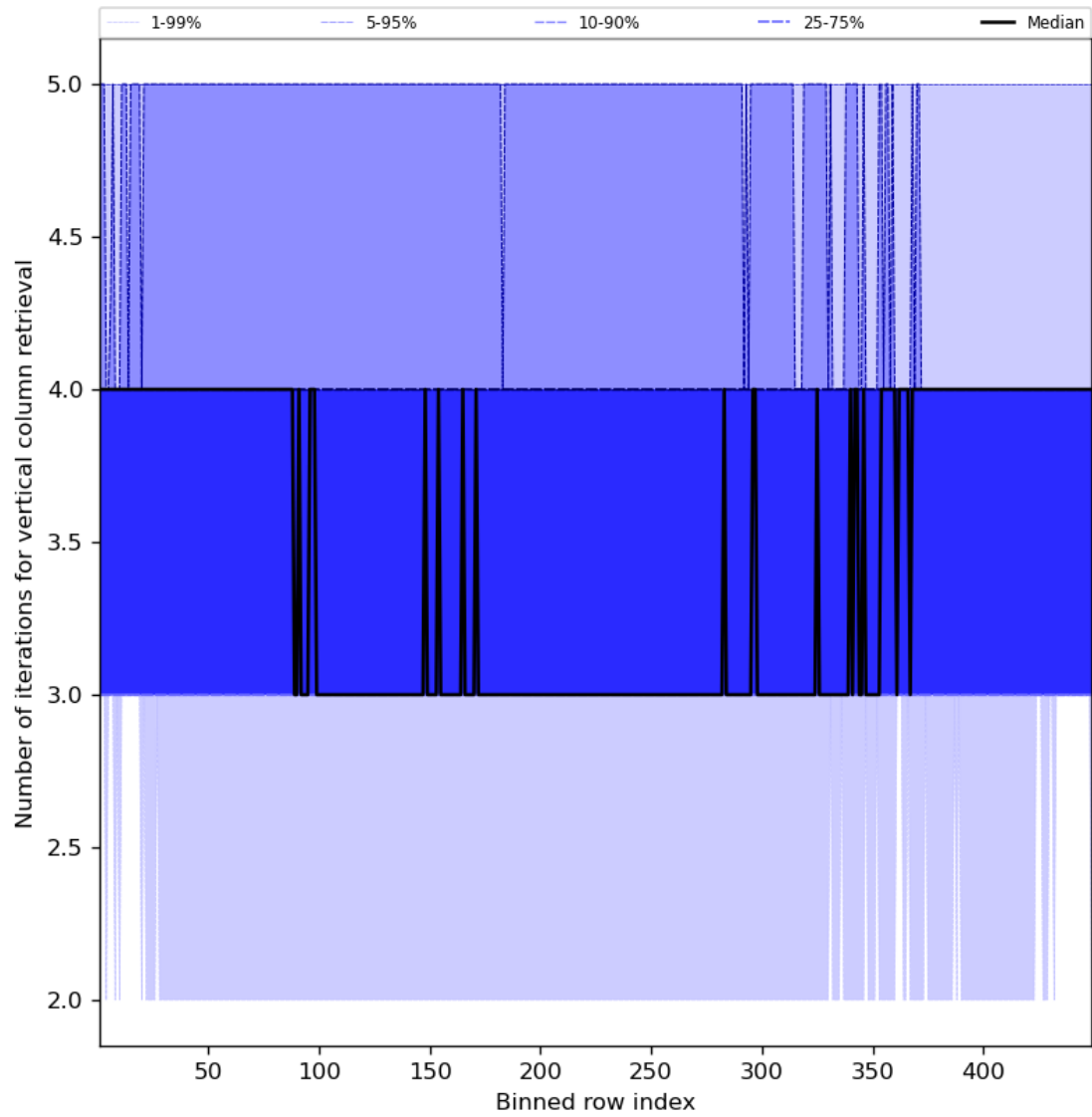
Figure 33: Along track statistics of “Number of iterations for vertical column retrieval” for 2024-07-13 to 2024-07-15
