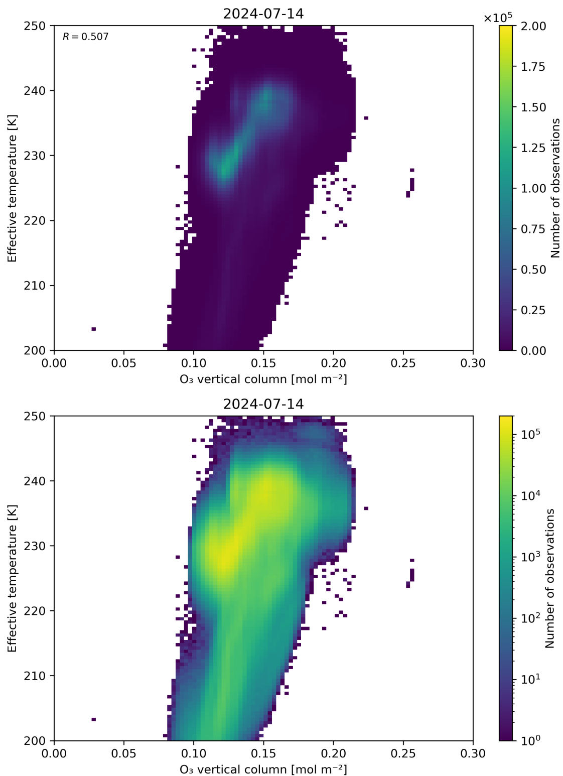
Figure 39: Scatter density plot of “O 3 vertical column” against “Effective temperature” for 2024-07-13 to 2024-07-15.
