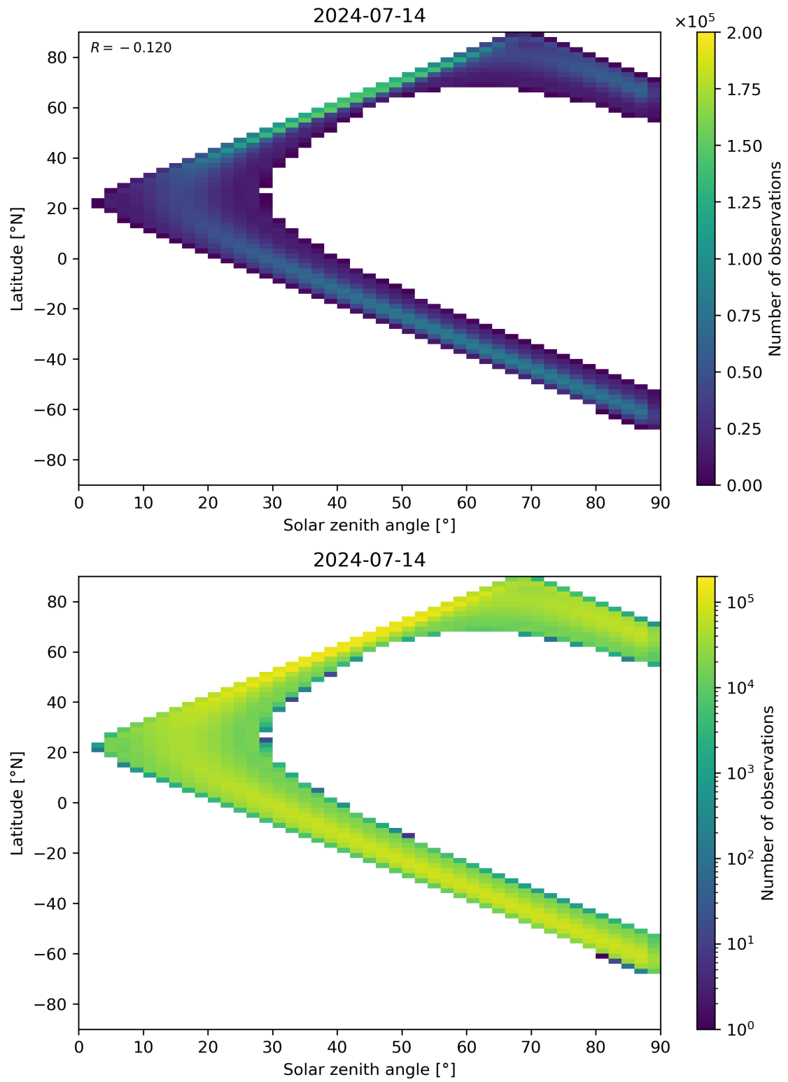
Figure 44: Scatter density plot of “Solar zenith angle” against “Latitude” for 2024-07-13 to 2024-07-15.
