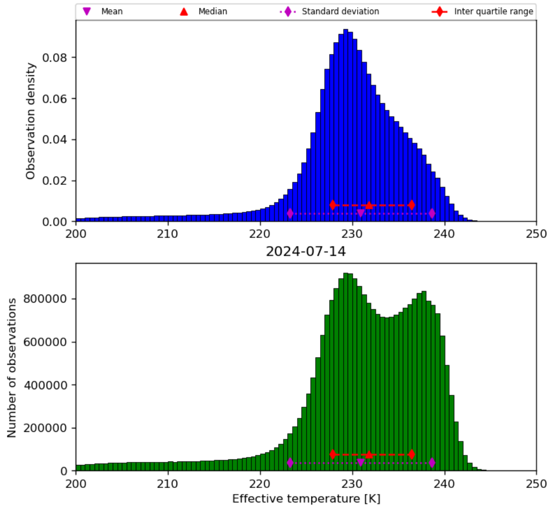
Figure 24: Histogram of “Effective temperature” for 2024-07-13 to 2024-07-15
