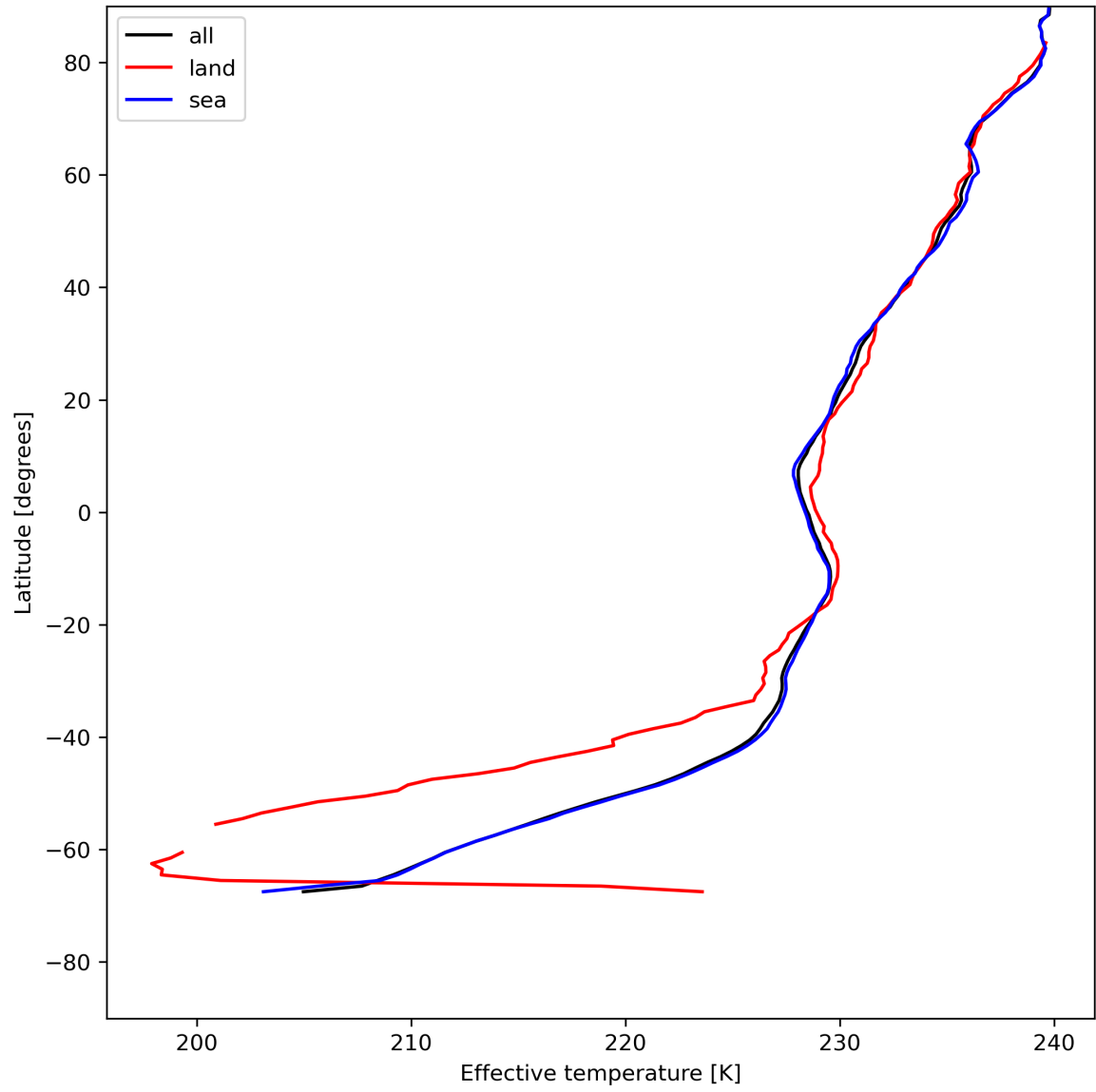
Figure 17: Zonal average of “Effective temperature” for 2024-07-13 to 2024-07-15.
