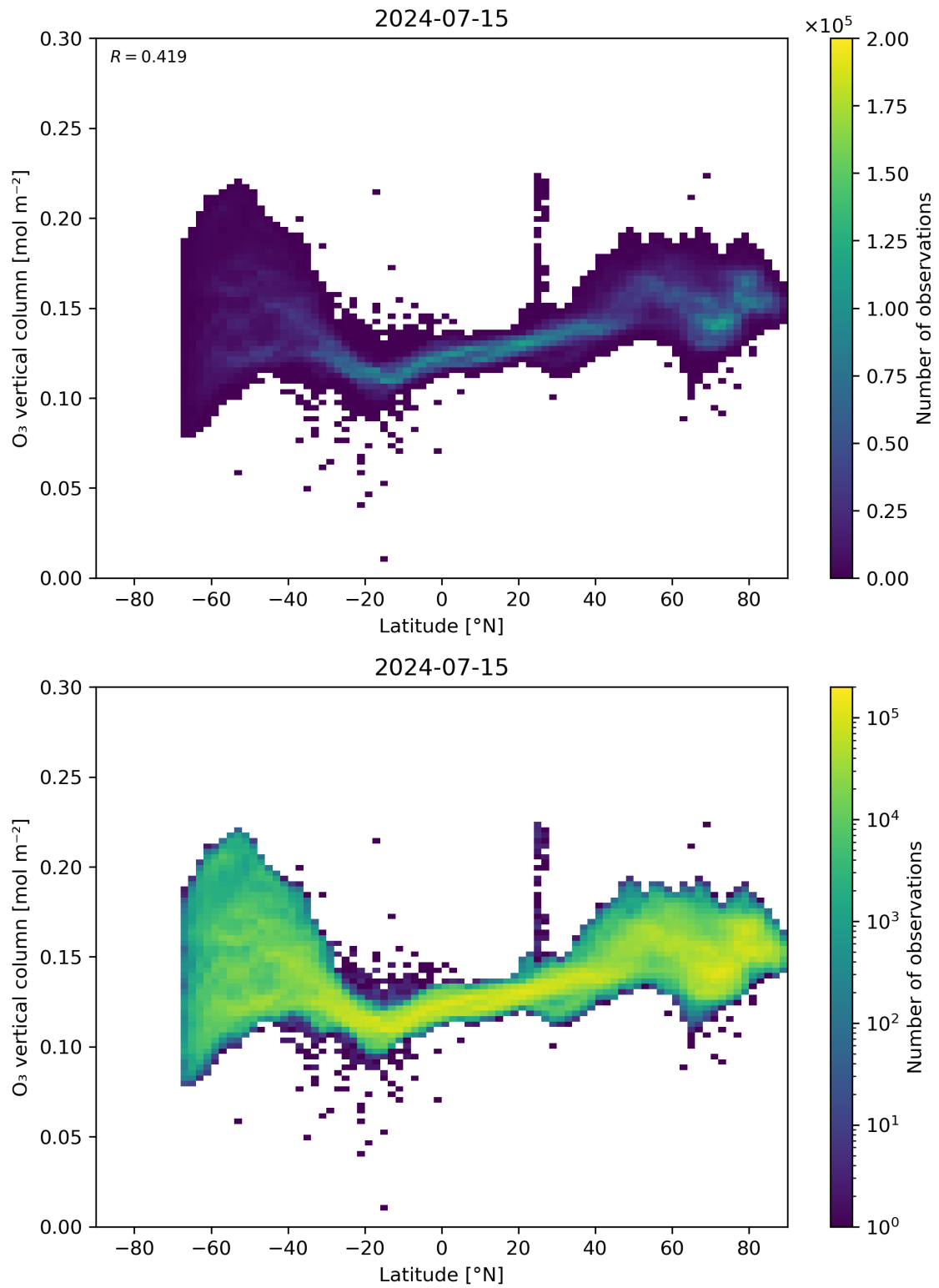
Figure 36: Scatter density plot of “Latitude” against “O 3 vertical column” for 2024-07-15 to 2024-07-16.
