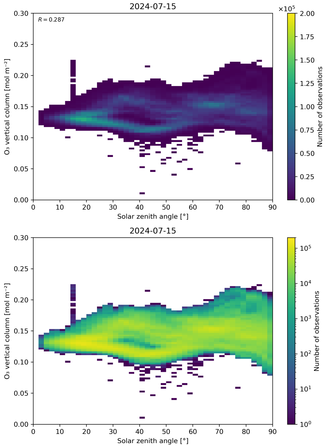
Figure 47: Scatter density plot of “Solar zenith angle” against “O 3 vertical column” for 2024-07-15 to 2024-07-16.
