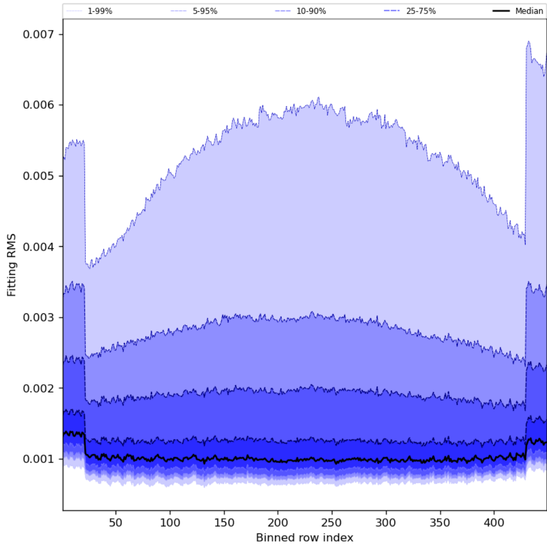
Figure 30: Along track statistics of “Fitting RMS” for 2024-07-15 to 2024-07-16
