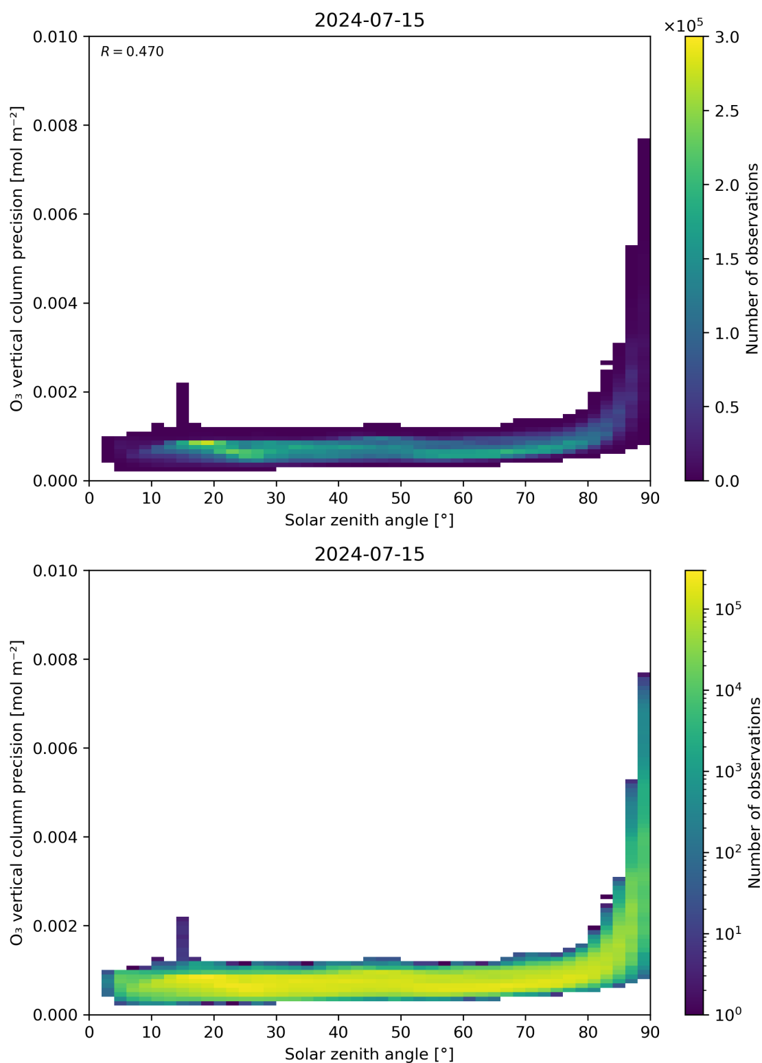
Figure 48: Scatter density plot of “Solar zenith angle” against “O 3 vertical column precision” for 2024-07-15 to 2024-07-16.
