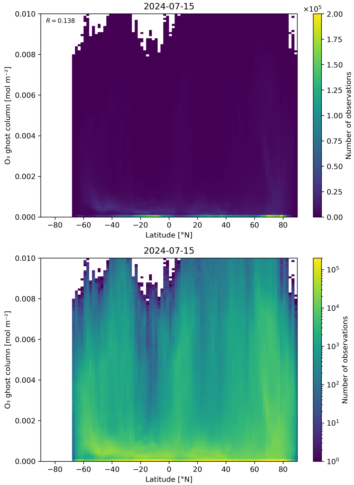
Figure 35: Scatter density plot of “Latitude” against “O 3 ghost column” for 2024-07-15 to 2024-07-16.
