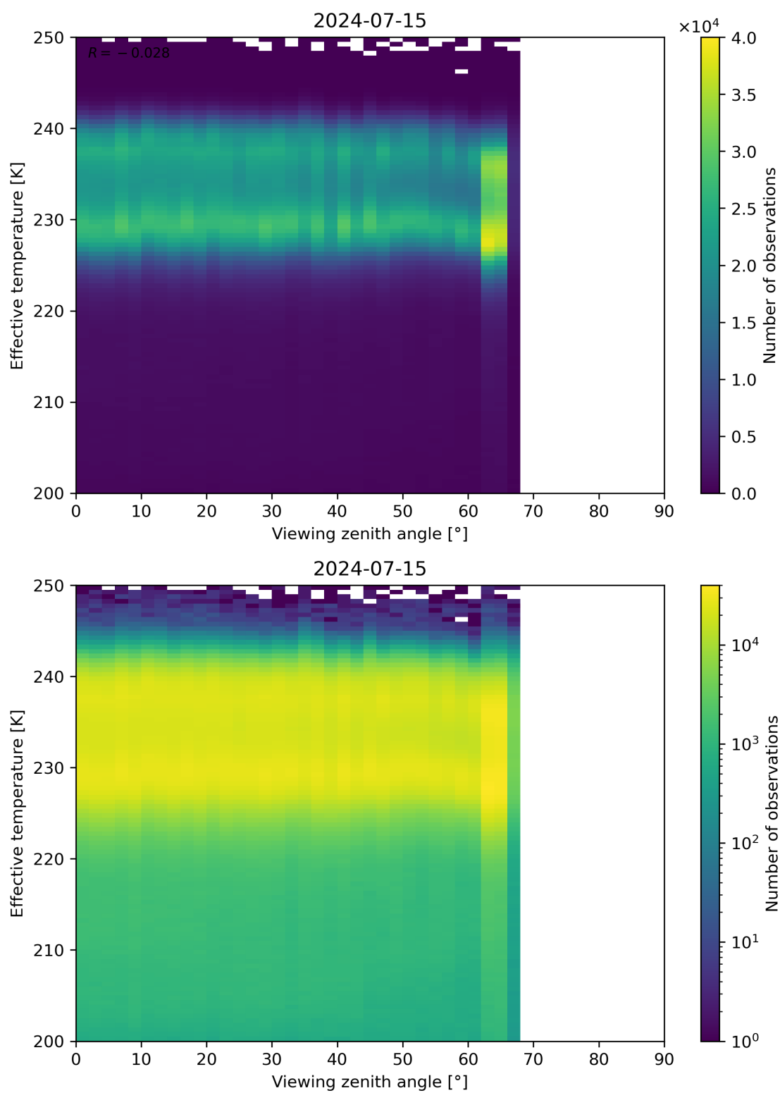
Figure 50: Scatter density plot of “Viewing zenith angle” against “Effective temperature” for 2024-07-15 to 2024-07-16.
