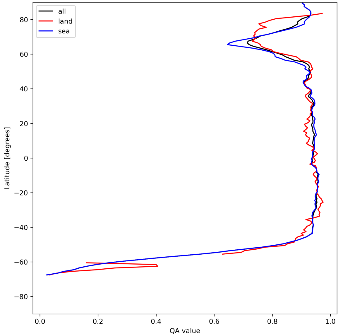
Figure 13: Zonal average of “QA value” for 2024-07-15 to 2024-07-16.
