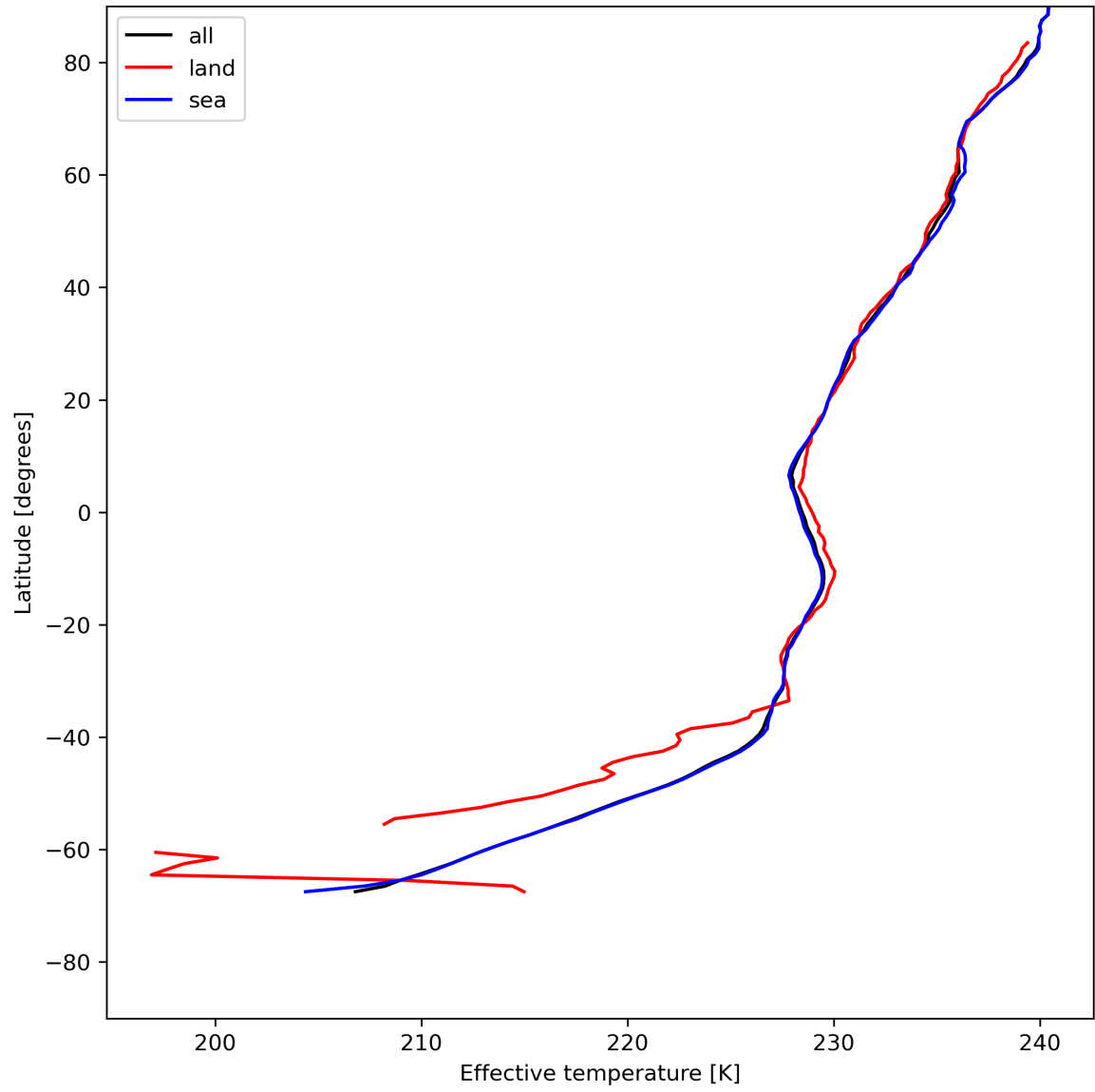
Figure 17: Zonal average of "Effective temperature" for 2024-07-15 to 2024-07-16.
