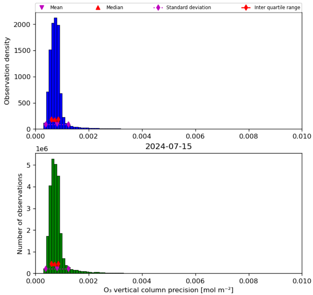
Figure 22: Histogram of “O 3 vertical column precision” for 2024-07-15 to 2024-07-16
