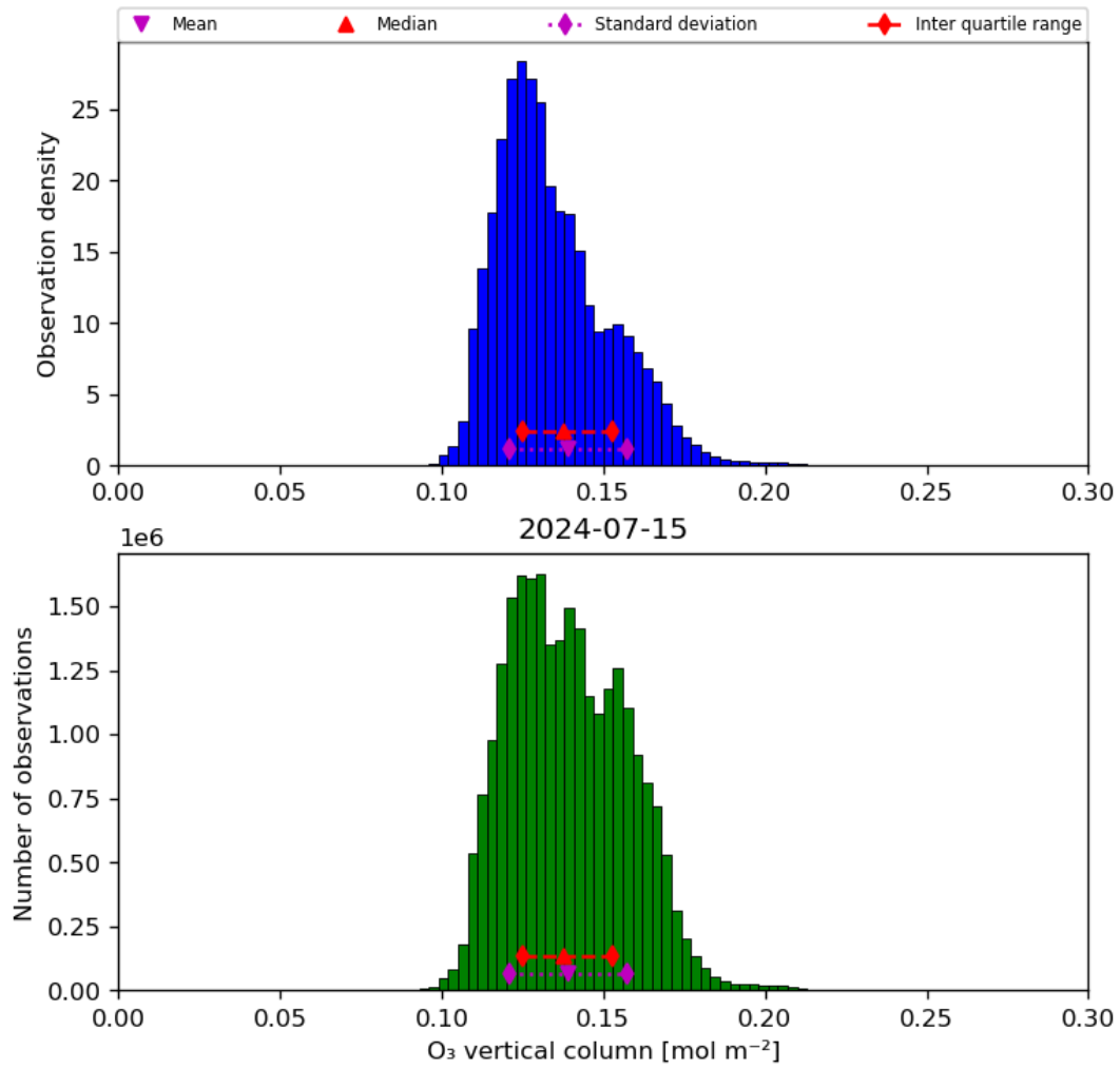
Figure 21: Histogram of “O 3 vertical column” for 2024-07-15 to 2024-07-16
