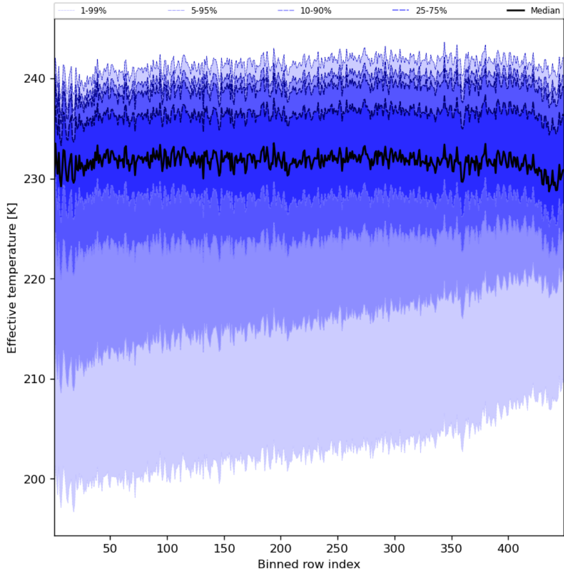
Figure 31: Along track statistics of “Effective temperature” for 2024-07-15 to 2024-07-16
