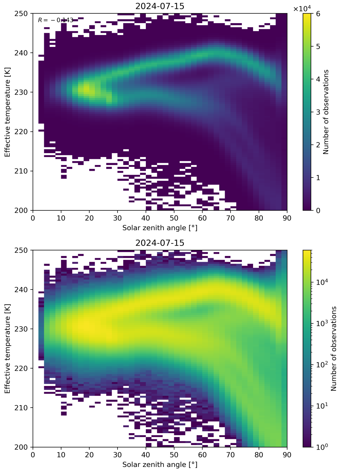
Figure 45: Scatter density plot of “Solar zenith angle” against “Effective temperature” for 2024-07-15 to 2024-07-16.
