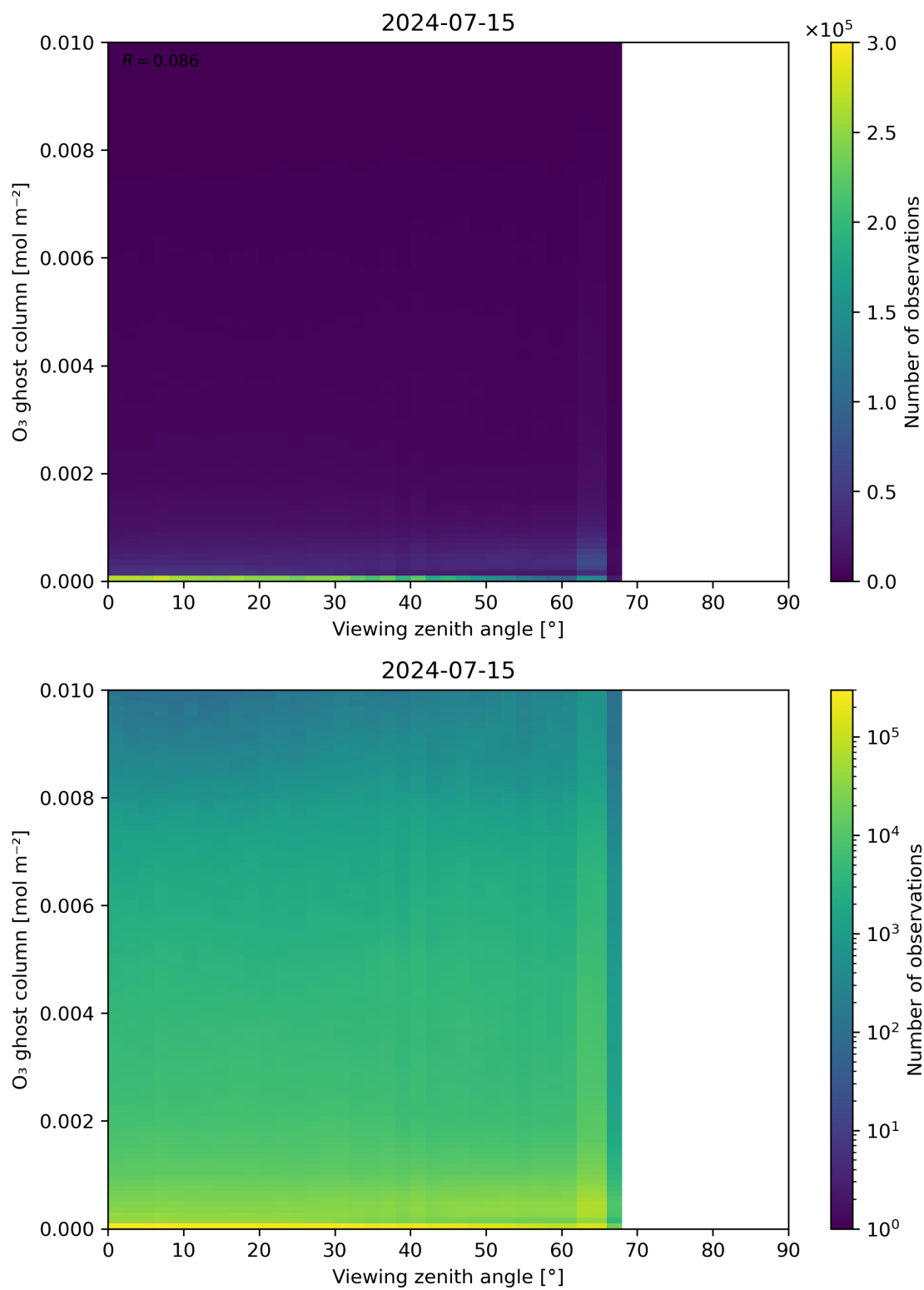
Figure 51: Scatter density plot of “Viewing zenith angle” against “O 3 ghost column” for 2024-07-15 to 2024-07-16.
