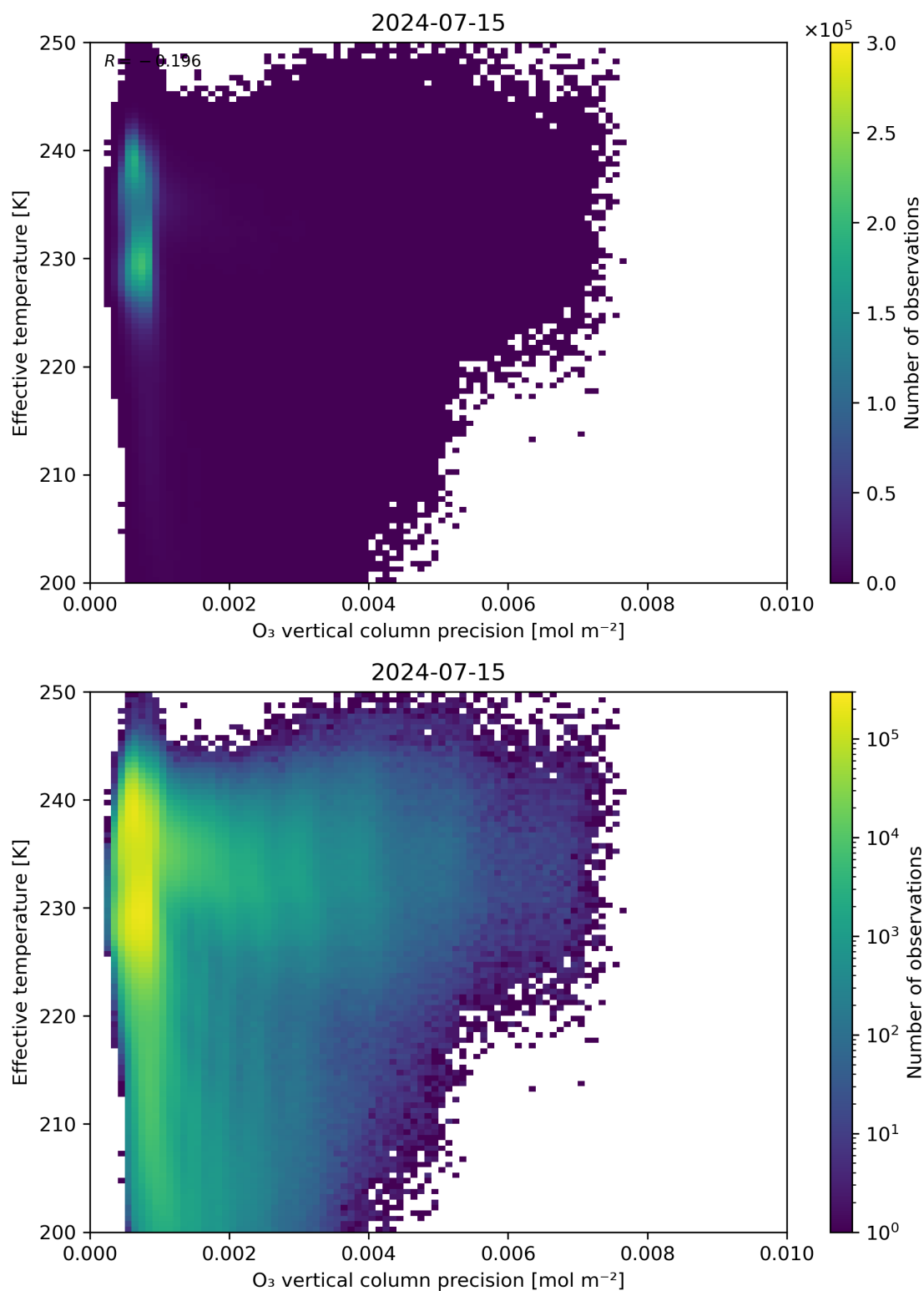
Figure 42: Scatter density plot of “O 3 vertical column precision” against “Effective temperature” for 2024-07-15 to 2024-07-16.
