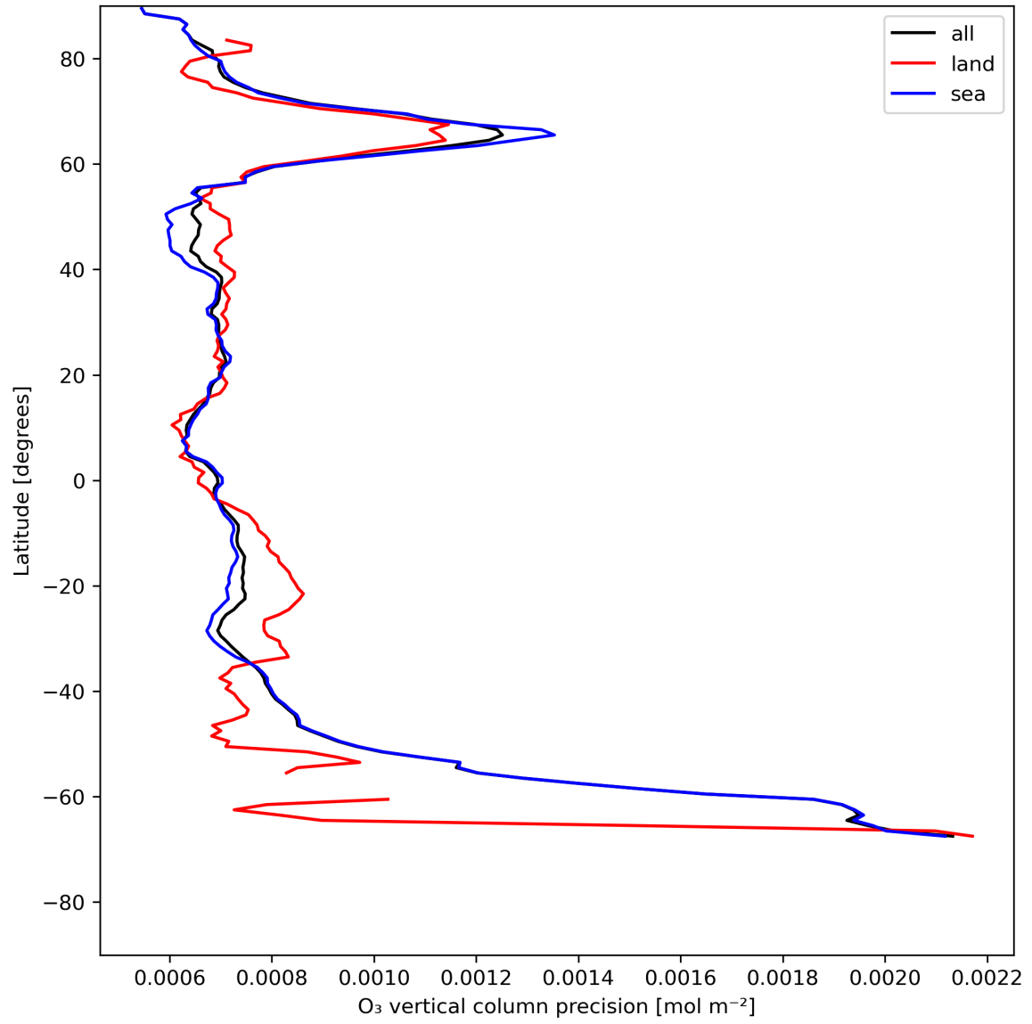
Figure 15: Zonal average of “O 3 vertical column precision” for 2024-07-15 to 2024-07-16.
