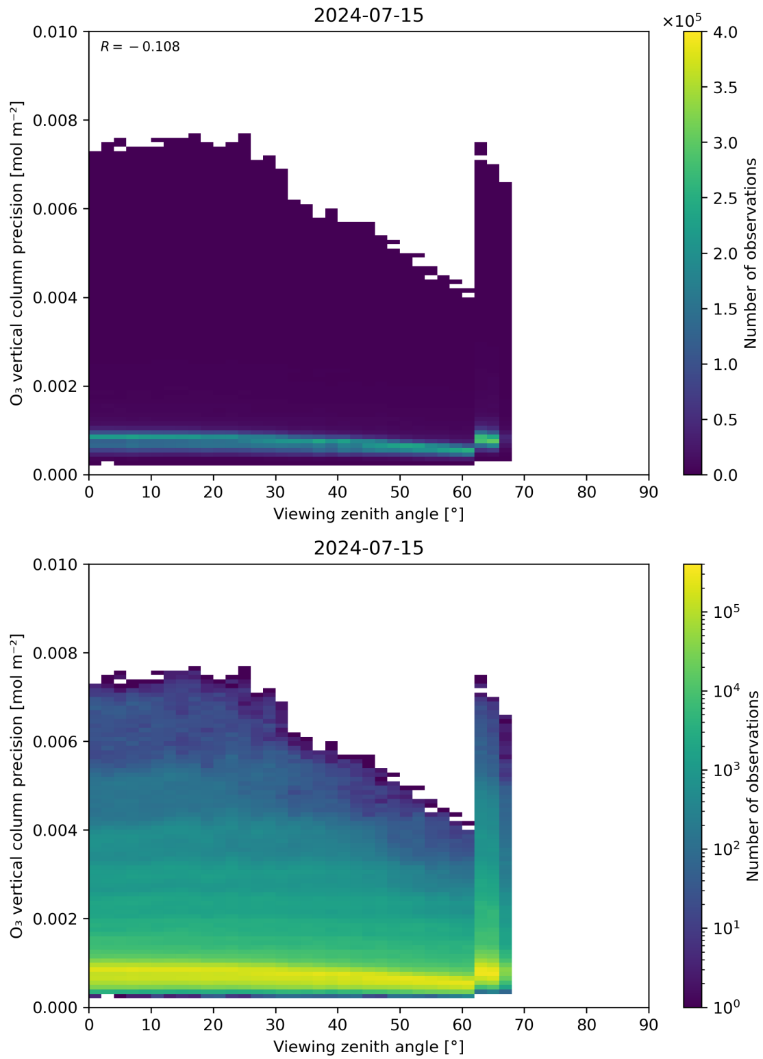
Figure 53: Scatter density plot of “Viewing zenith angle” against “O 3 vertical column precision” for 2024-07-15 to 2024-07-16.
