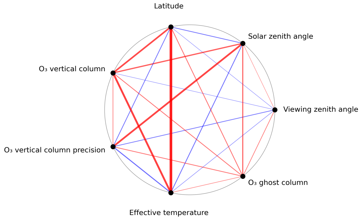
Figure 1: Map of correlation graph for 2024-07-15 to 2024-07-16.
