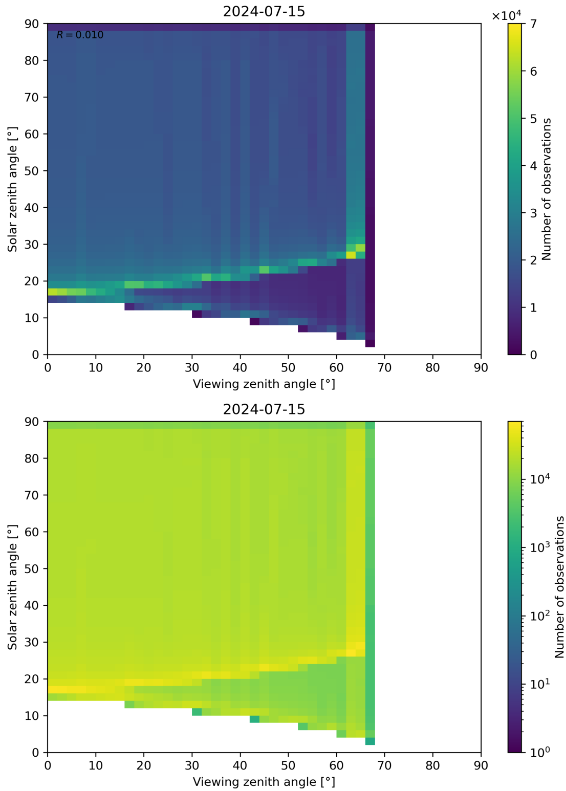
Figure 54: Scatter density plot of “Viewing zenith angle” against “Solar zenith angle” for 2024-07-15 to 2024-07-16.
