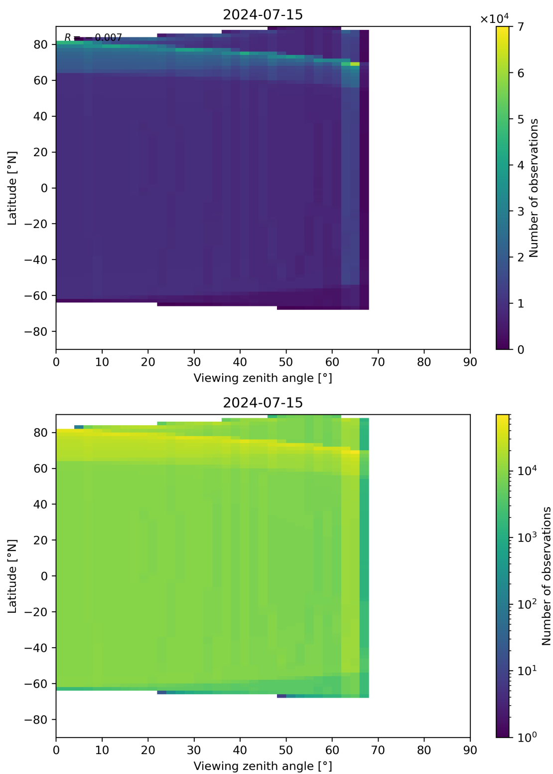
Figure 49: Scatter density plot of “Viewing zenith angle” against “Latitude” for 2024-07-15 to 2024-07-16.
