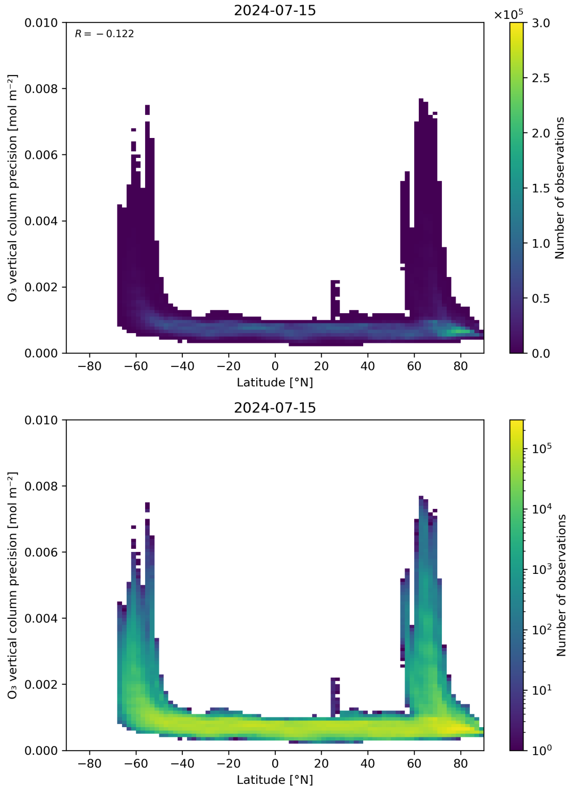
Figure 37: Scatter density plot of “Latitude” against “O 3 vertical column precision” for 2024-07-15 to 2024-07-16.
