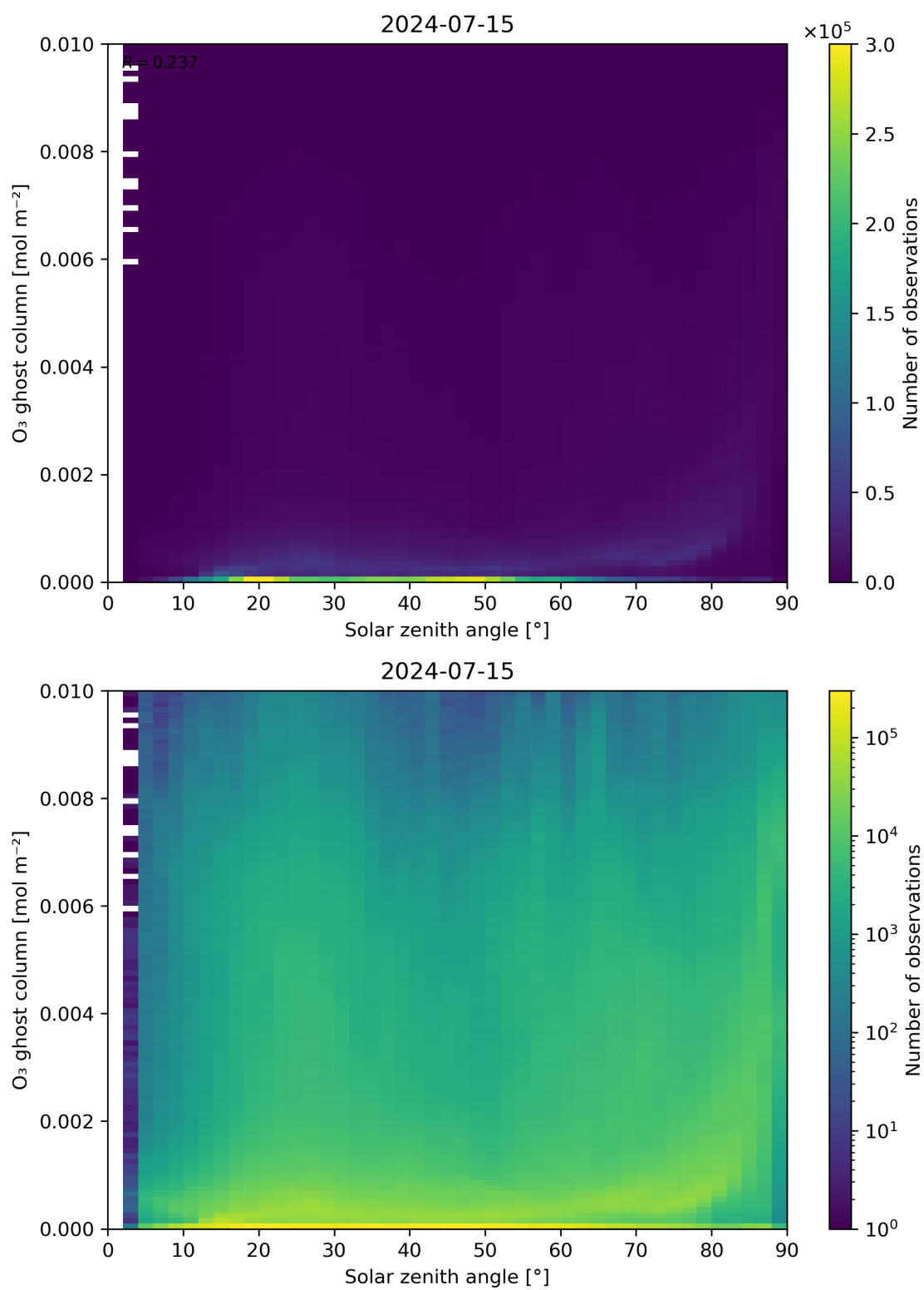
Figure 46: Scatter density plot of “Solar zenith angle” against “O 3 ghost column” for 2024-07-15 to 2024-07-16.
