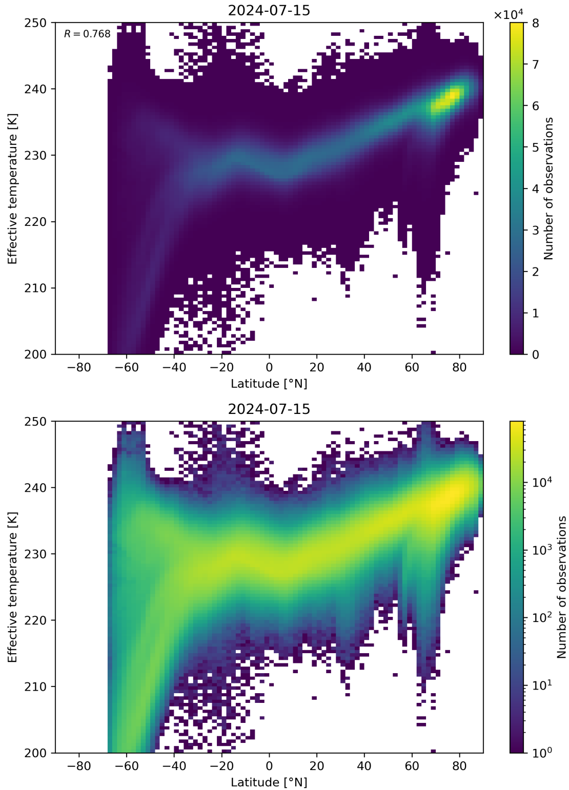
Figure 34: Scatter density plot of “Latitude” against “Effective temperature” for 2024-07-15 to 2024-07-16.
