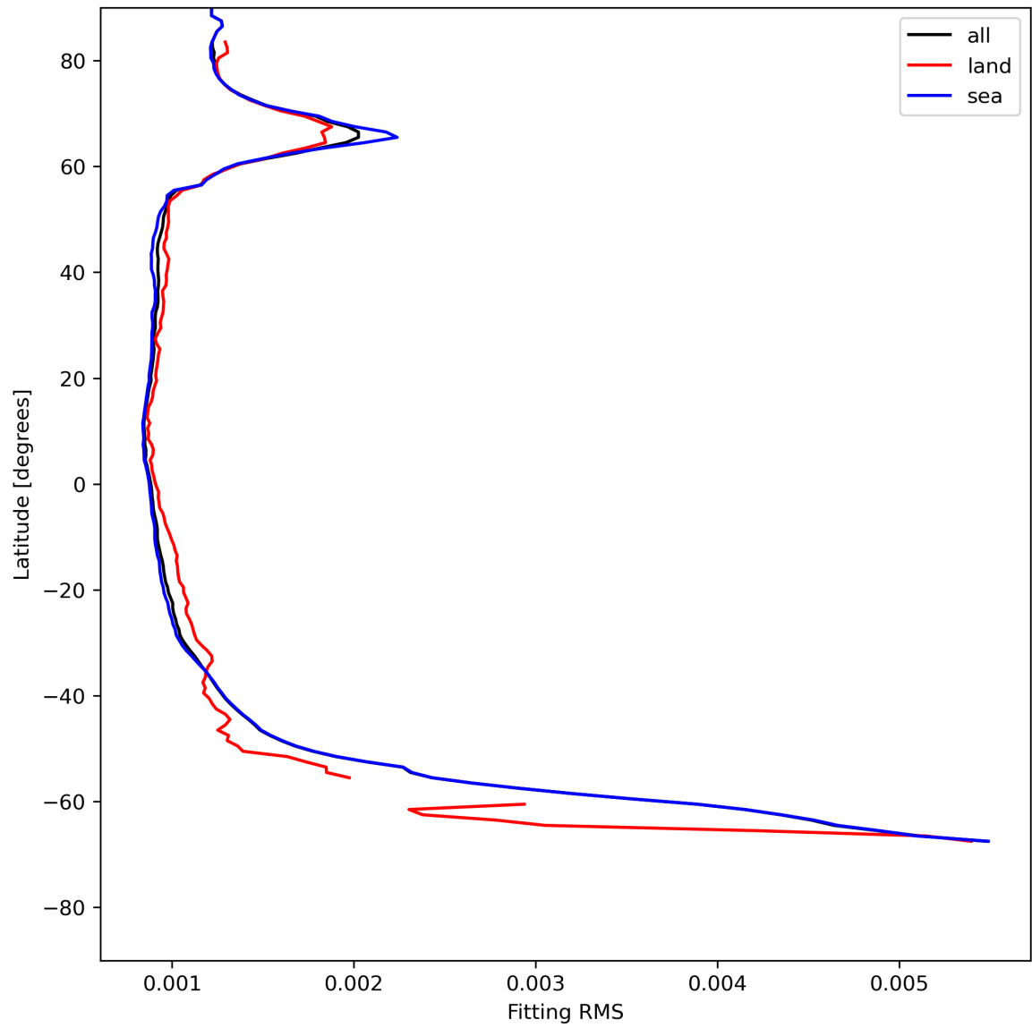
Figure 16: Zonal average of “Fitting RMS” for 2024-07-15 to 2024-07-16.
