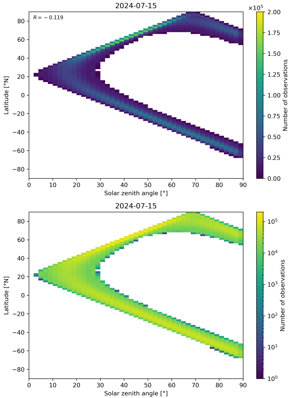
Figure 44: Scatter density plot of “Solar zenith angle” against “Latitude” for 2024-07-15 to 2024-07-16.
