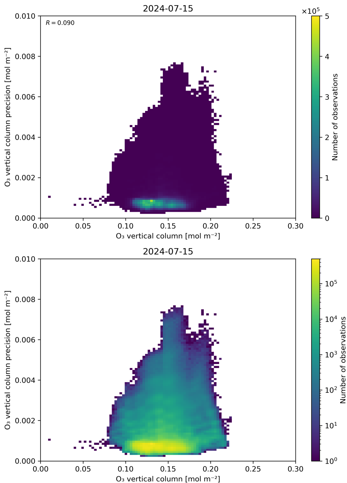
Figure 41: Scatter density plot of “O 3 vertical column” against “O 3 vertical column precision” for 2024-07-15 to 2024-07-16.
