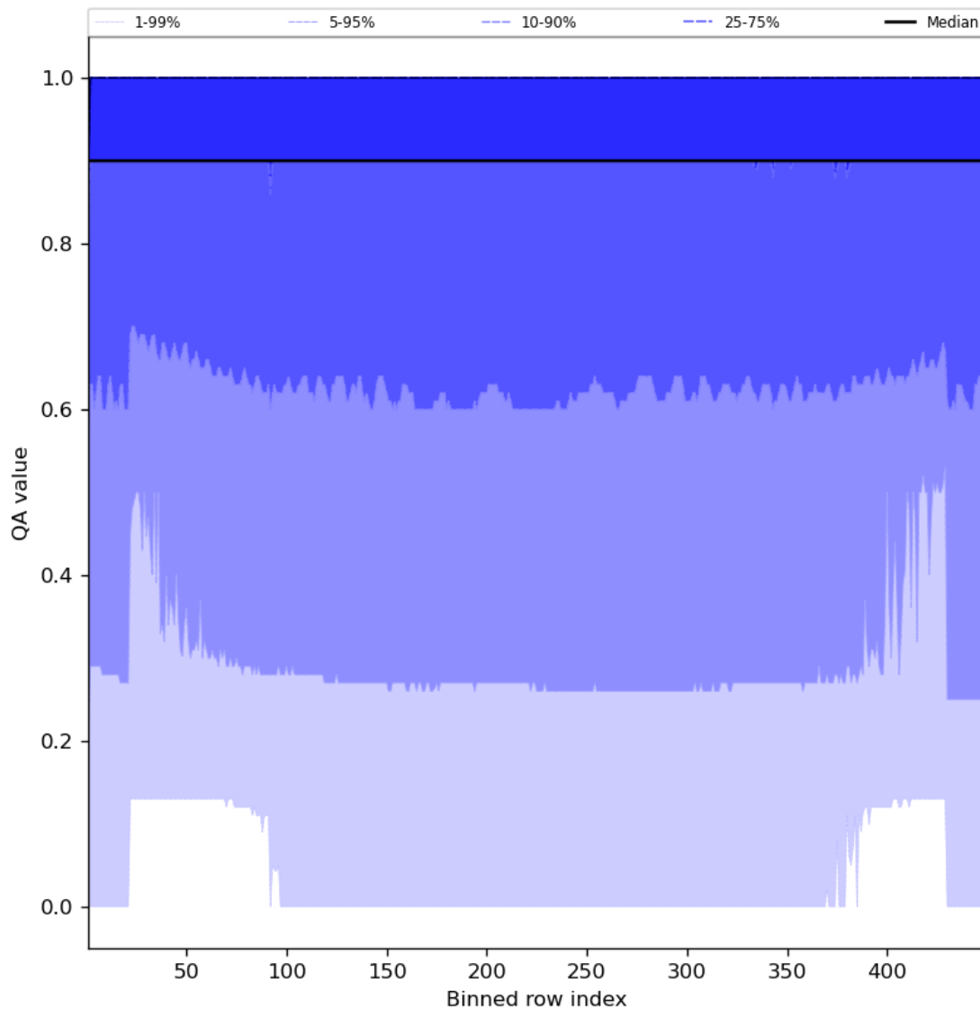
Figure 27: Along track statistics of “QA value” for 2024-07-15 to 2024-07-16
