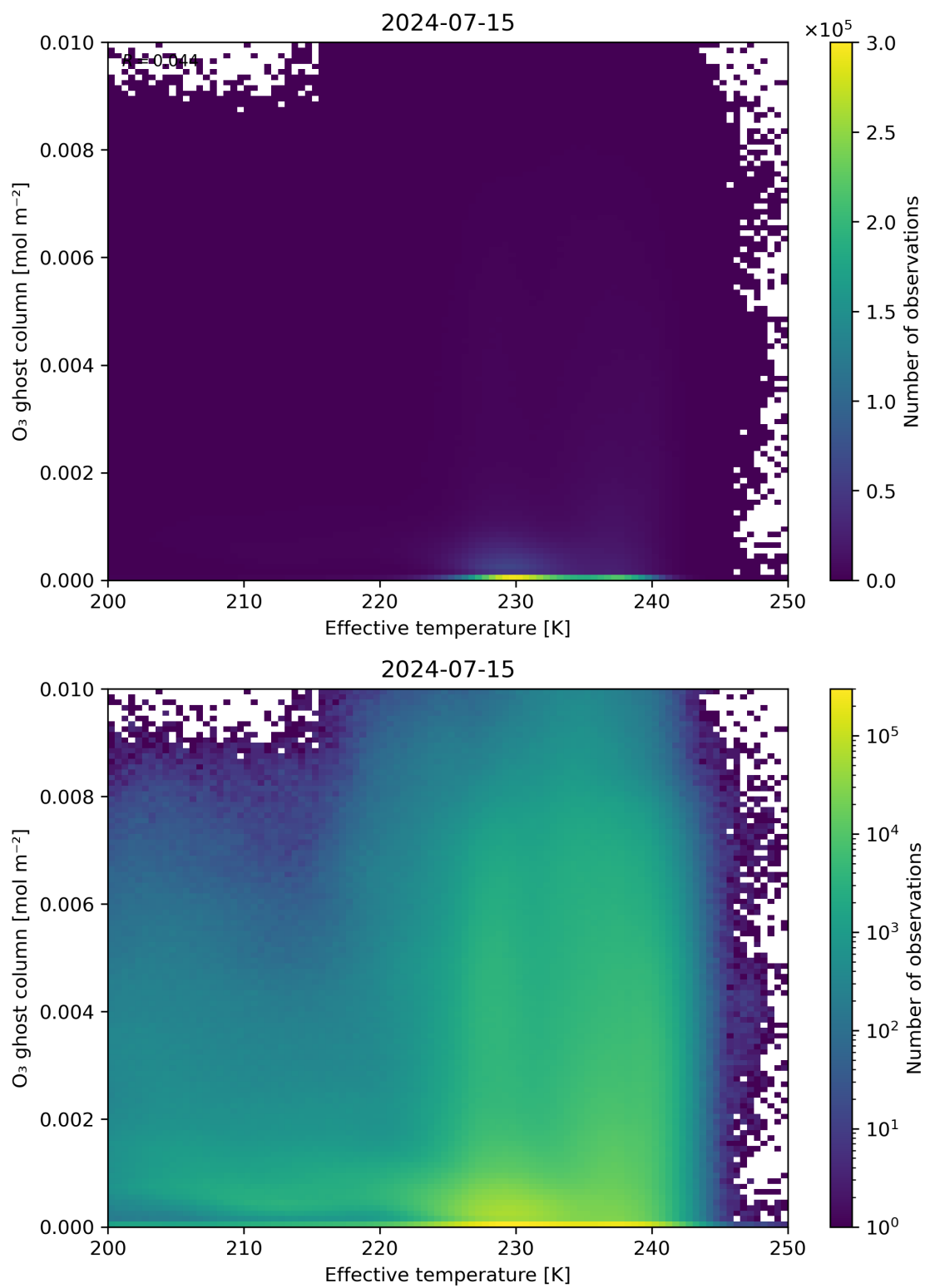
Figure 38: Scatter density plot of “Effective temperature” against “O 3 ghost column” for 2024-07-15 to 2024-07-16.
