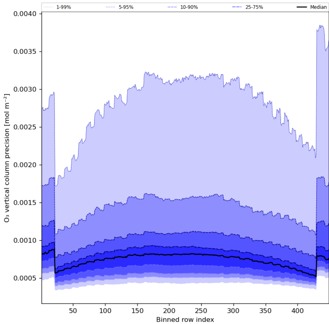
Figure 29: Along track statistics of “O 3 vertical column precision” for 2024-07-15 to 2024-07-16
