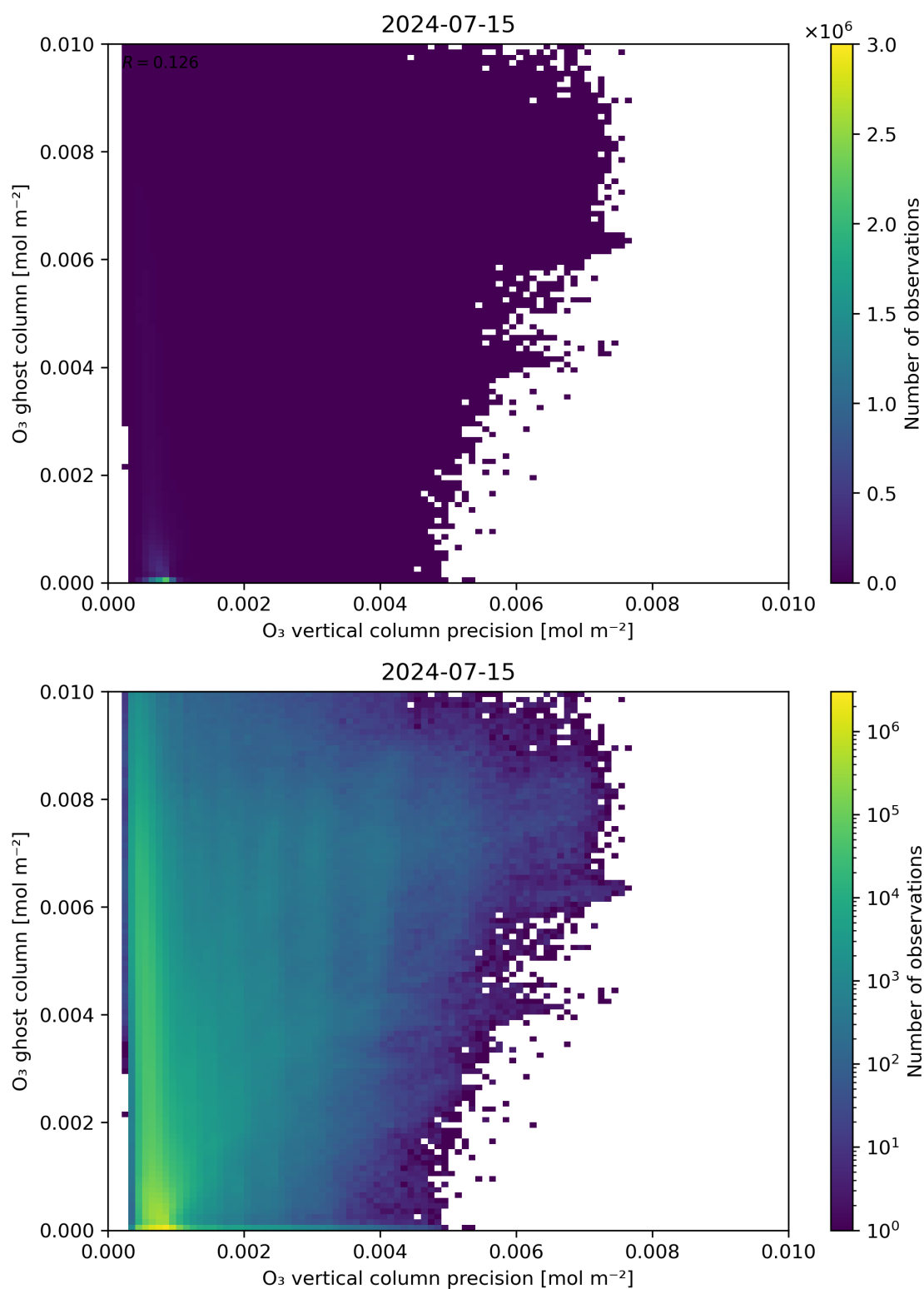
Figure 43: Scatter density plot of “ O_3 vertical column precision” against “ O_3 ghost column” for 2024-07-15 to 2024-07-16.
