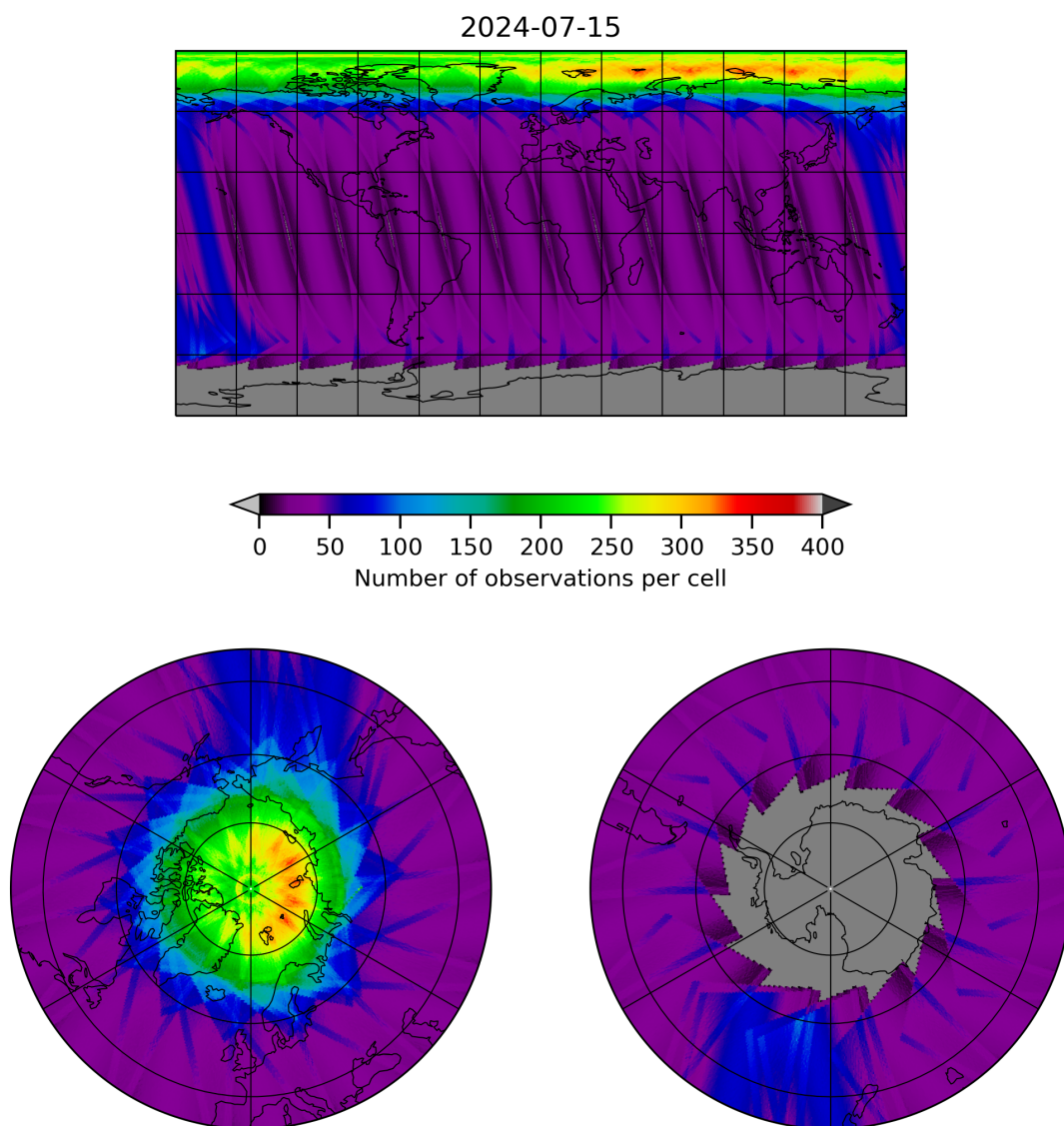
Figure 12: Map of the number of observations for 2024-07-15 to 2024-07-16
