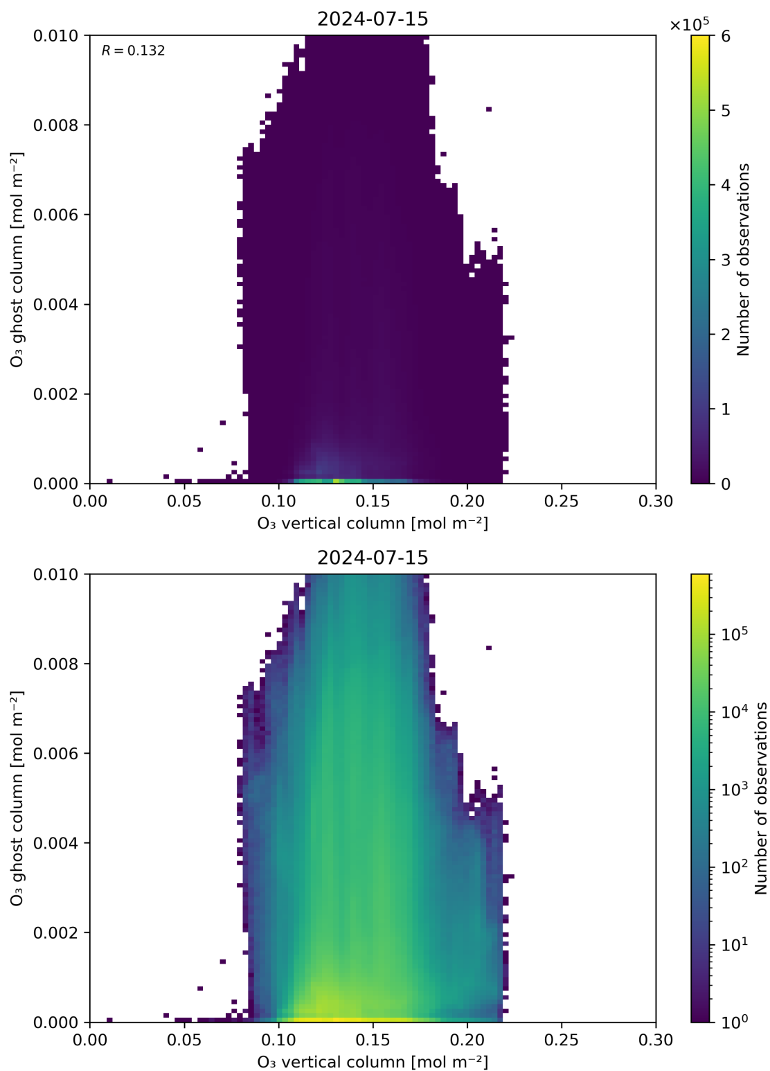
Figure 40: Scatter density plot of “O 3 vertical column” against “O 3 ghost column” for 2024-07-15 to 2024-07-16.
