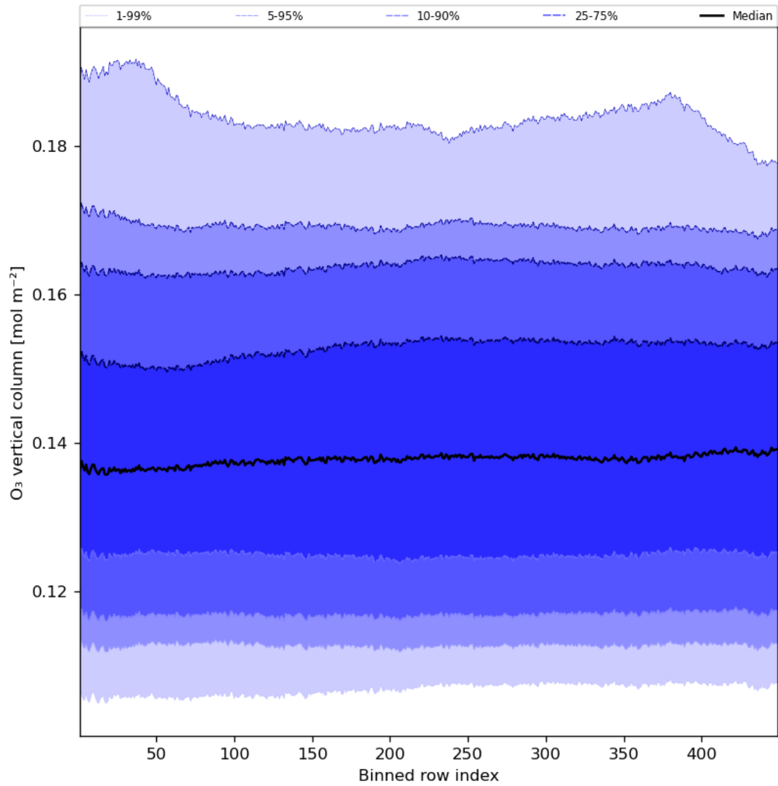
Figure 28: Along track statistics of “O 3 vertical column” for 2024-07-15 to 2024-07-16
