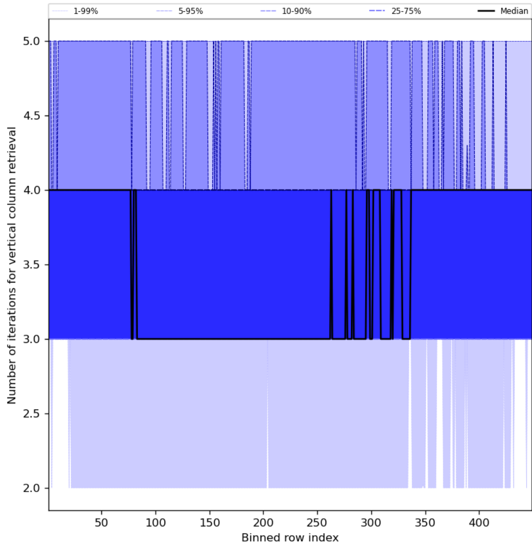
Figure 33: Along track statistics of “Number of iterations for vertical column retrieval” for 2024-07-15 to 2024-07-16
