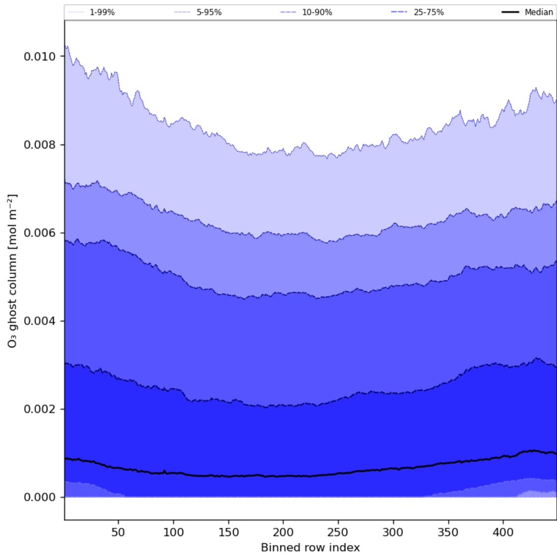
Figure 32: Along track statistics of “O 3 ghost column” for 2024-07-15 to 2024-07-16
