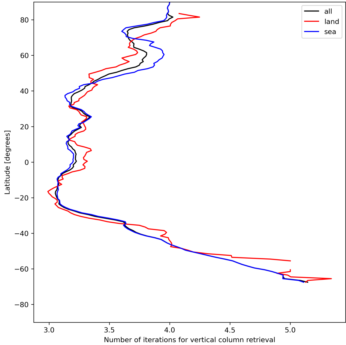
Figure 19: Zonal average of “Number of iterations for vertical column retrieval” for 2024-07-15 to 2024-07-16.
