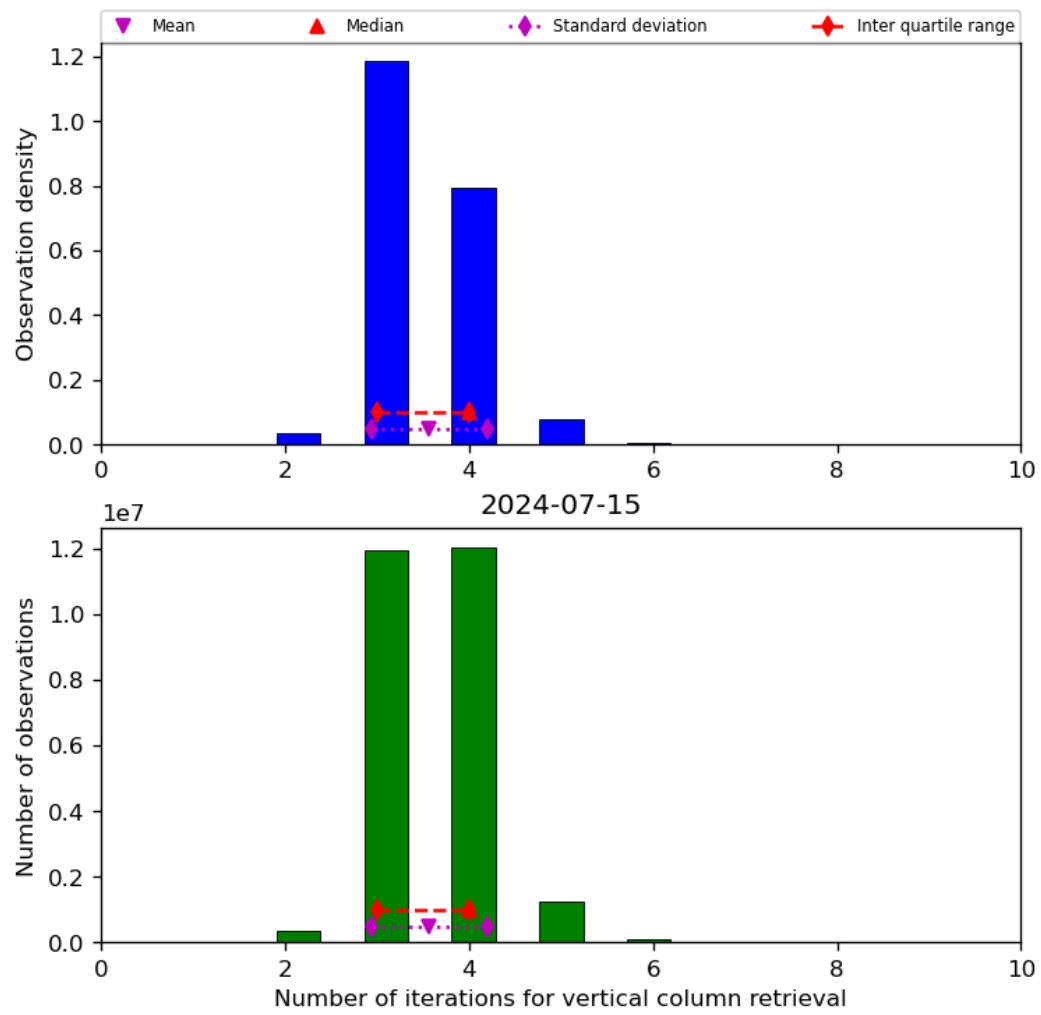
Figure 26: Histogram of “Number of iterations for vertical column retrieval” for 2024-07-15 to 2024-07-16
