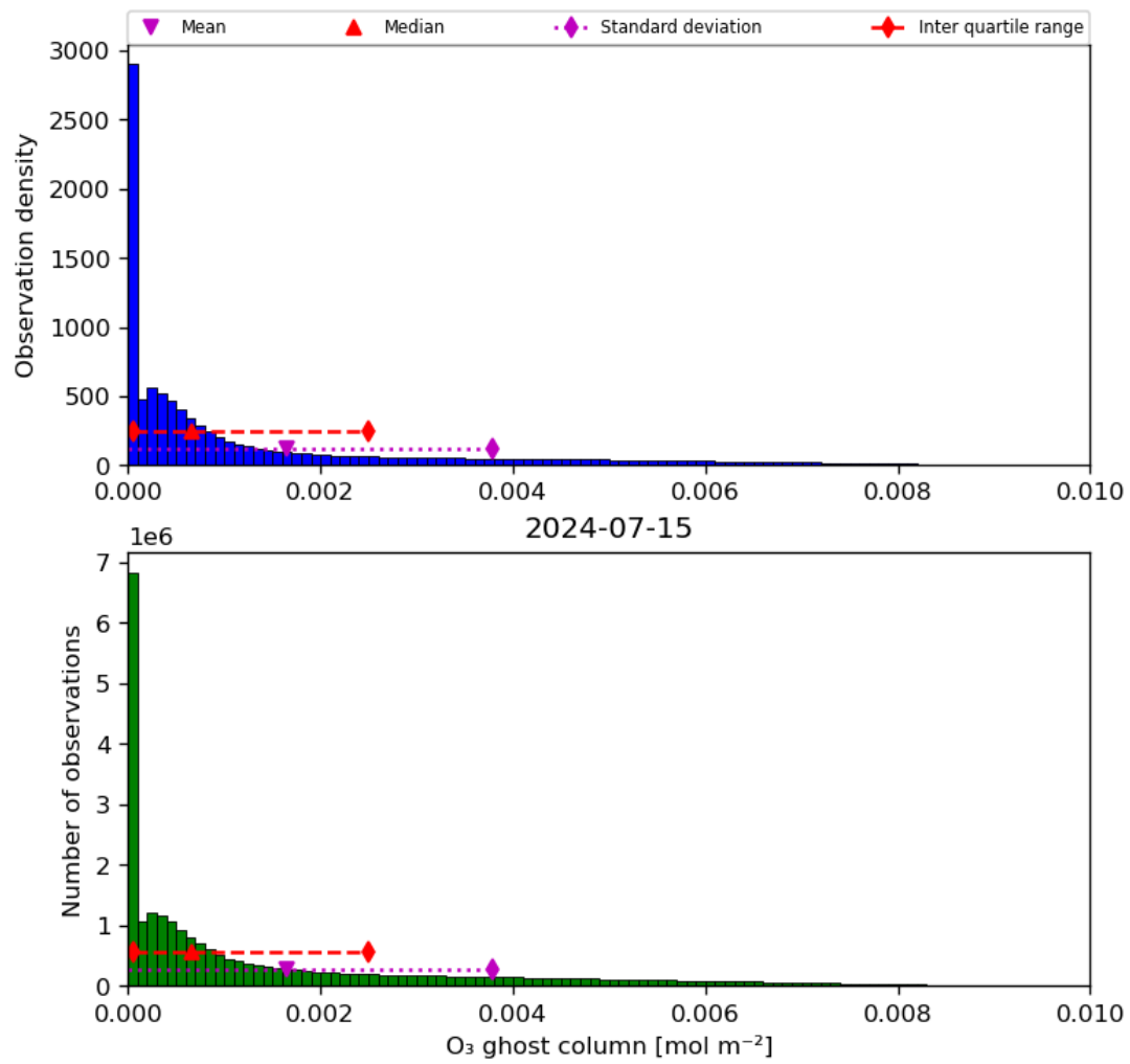
Figure 25: Histogram of “O 3 ghost column” for 2024-07-15 to 2024-07-16
