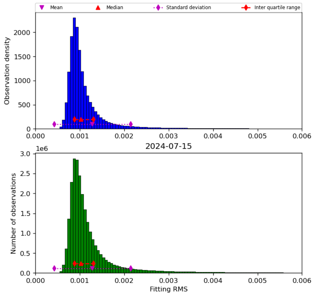
Figure 23: Histogram of “Fitting RMS” for 2024-07-15 to 2024-07-16
