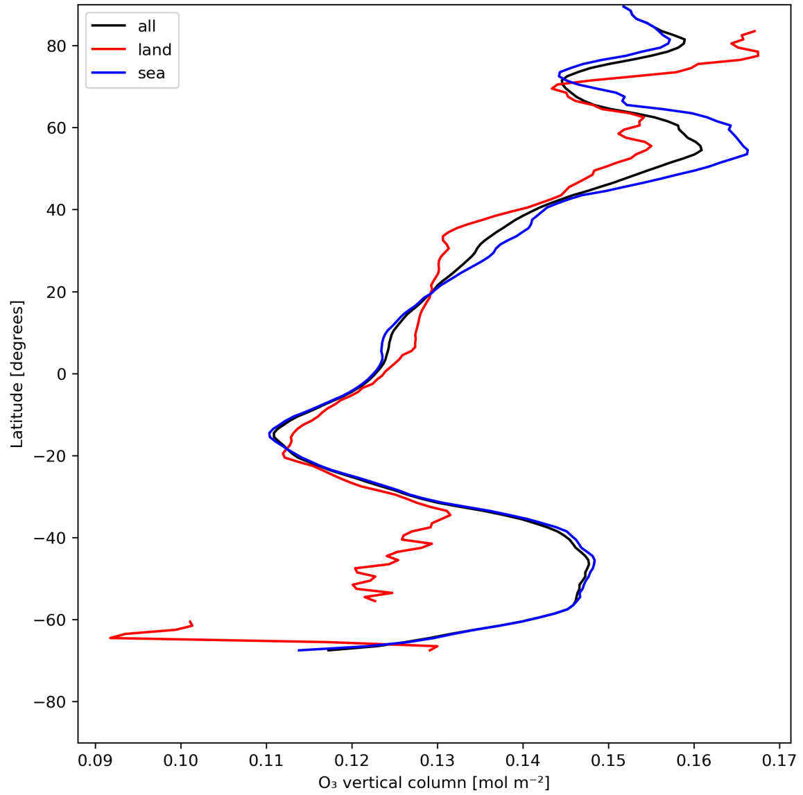
Figure 14: Zonal average of “O 3 vertical column” for 2024-07-15 to 2024-07-16.
