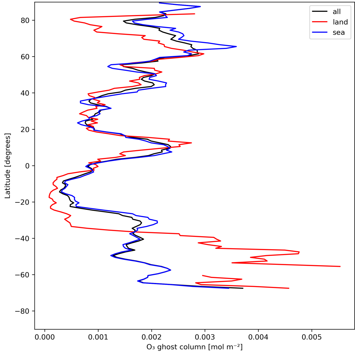
Figure 18: Zonal average of “O 3 ghost column” for 2024-07-15 to 2024-07-16.
