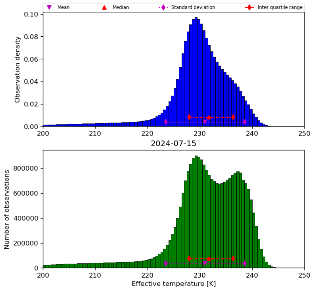
Figure 24: Histogram of “Effective temperature” for 2024-07-15 to 2024-07-16
