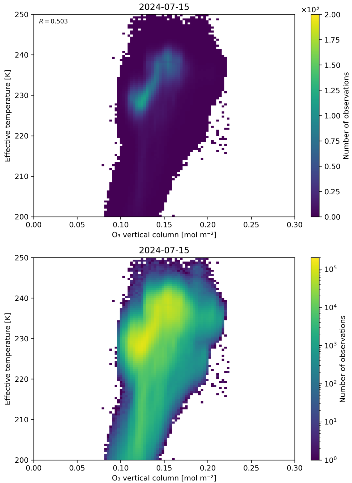
Figure 39: Scatter density plot of “O 3 vertical column” against “Effective temperature” for 2024-07-15 to 2024-07-16.
