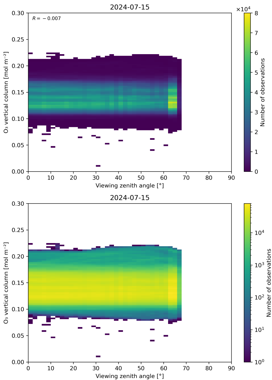
Figure 52: Scatter density plot of “Viewing zenith angle” against “O 3 vertical column” for 2024-07-15 to 2024-07-16.
