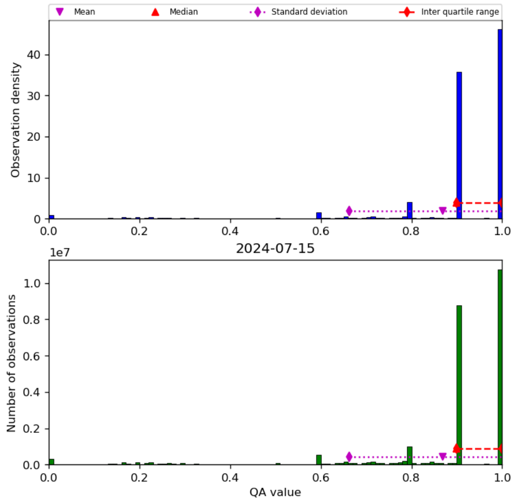
Figure 20: Histogram of “QA value” for 2024-07-15 to 2024-07-16
