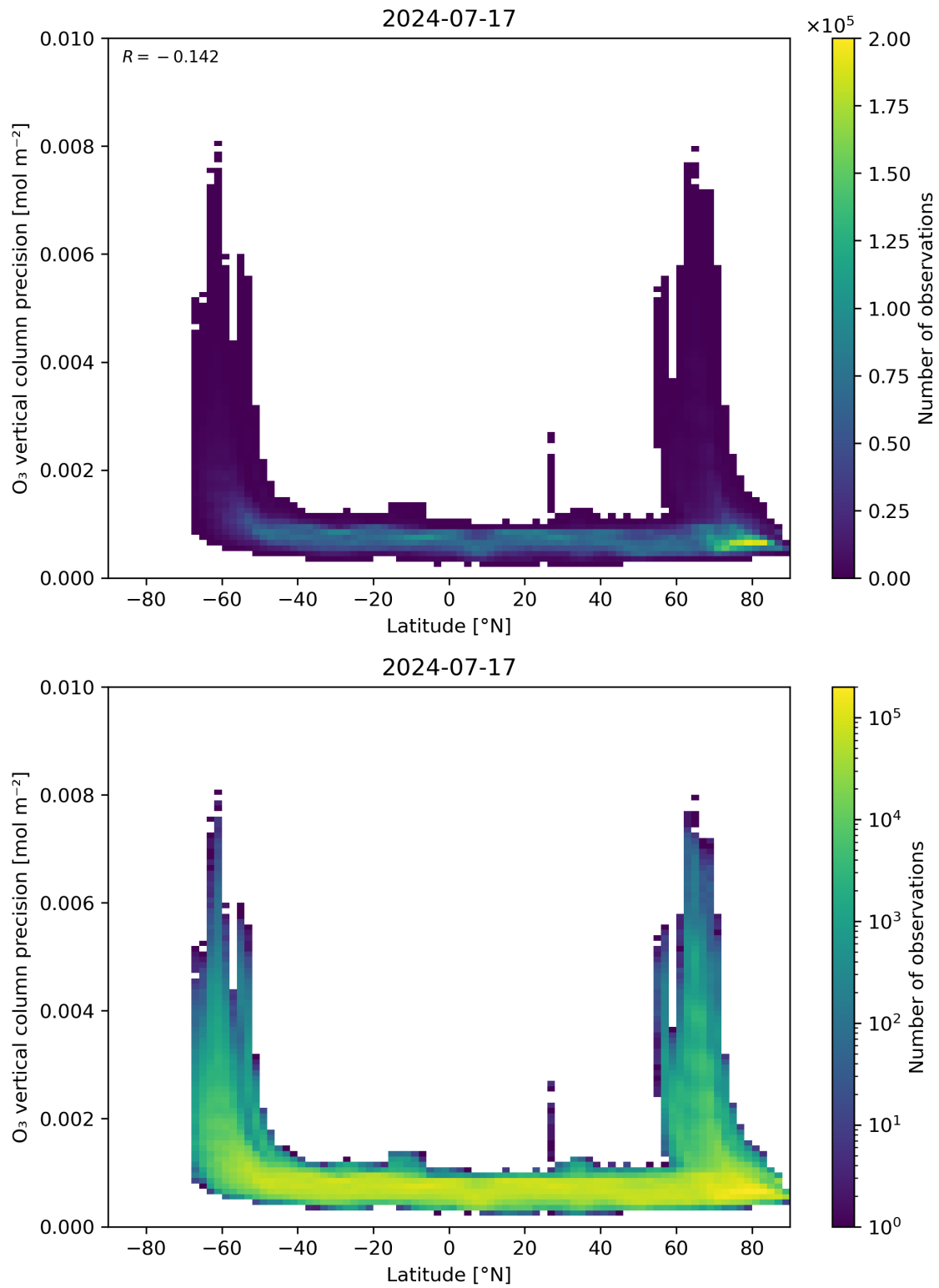
Figure 37: Scatter density plot of “Latitude” against “O 3 vertical column precision” for 2024-07-16 to 2024-07-18.
