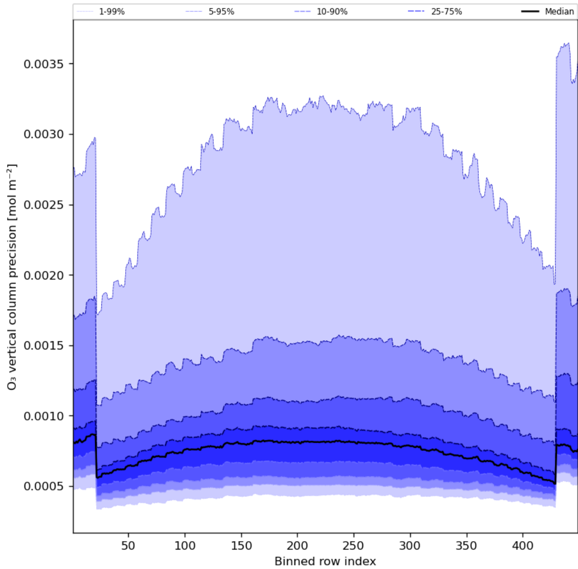
Figure 29: Along track statistics of “O 3 vertical column precision” for 2024-07-16 to 2024-07-18
