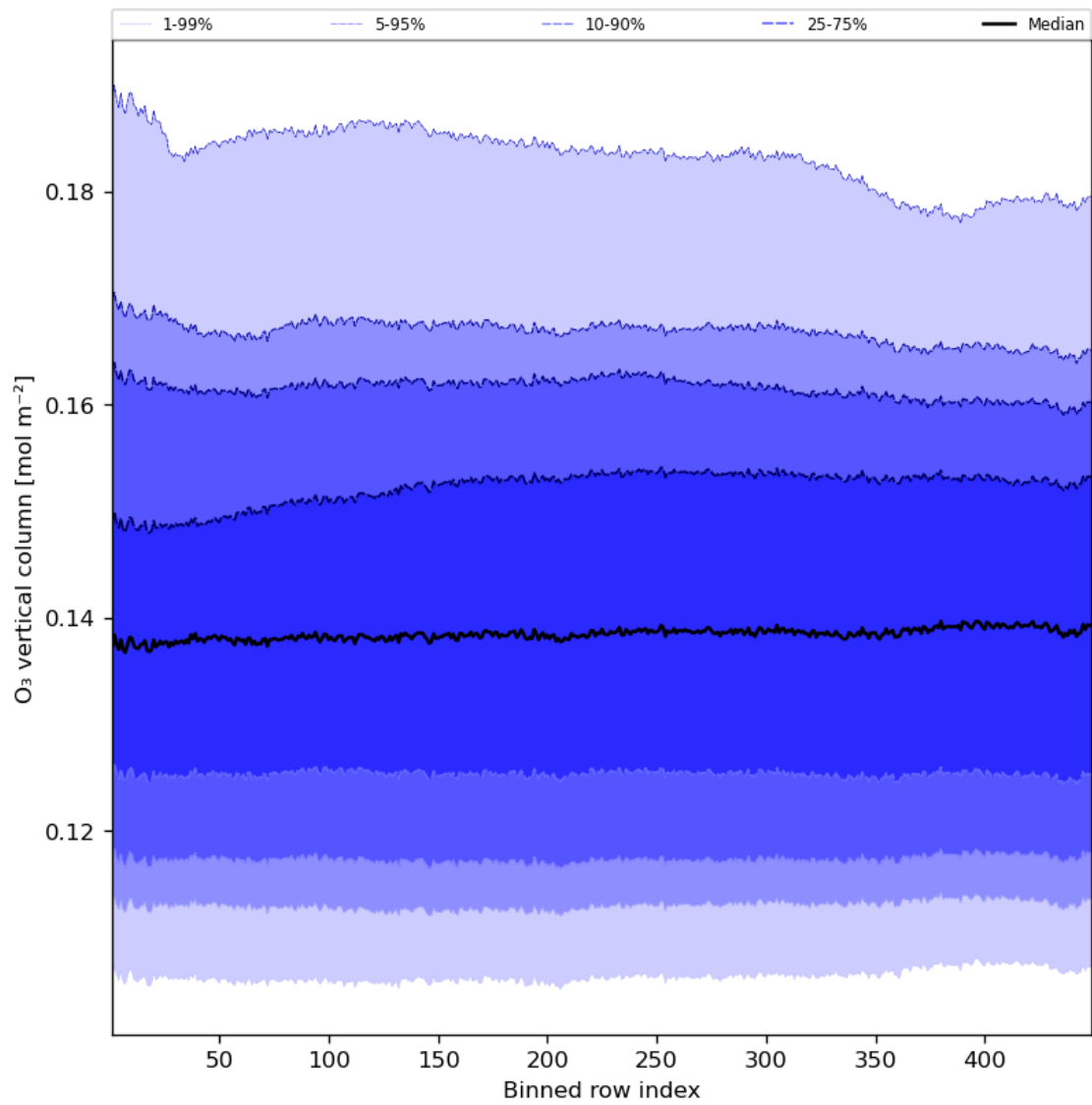
Figure 28: Along track statistics of “O 3 vertical column” for 2024-07-16 to 2024-07-18
