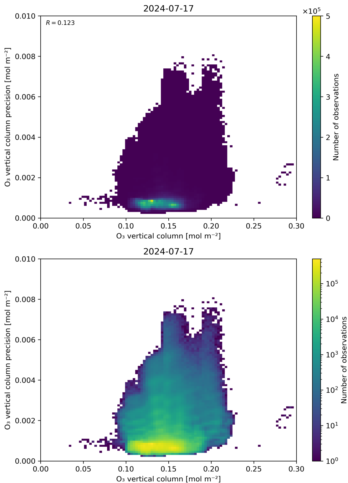
Figure 41: Scatter density plot of “O 3 vertical column” against “O 3 vertical column precision” for 2024-07-16 to 2024-07-18.
