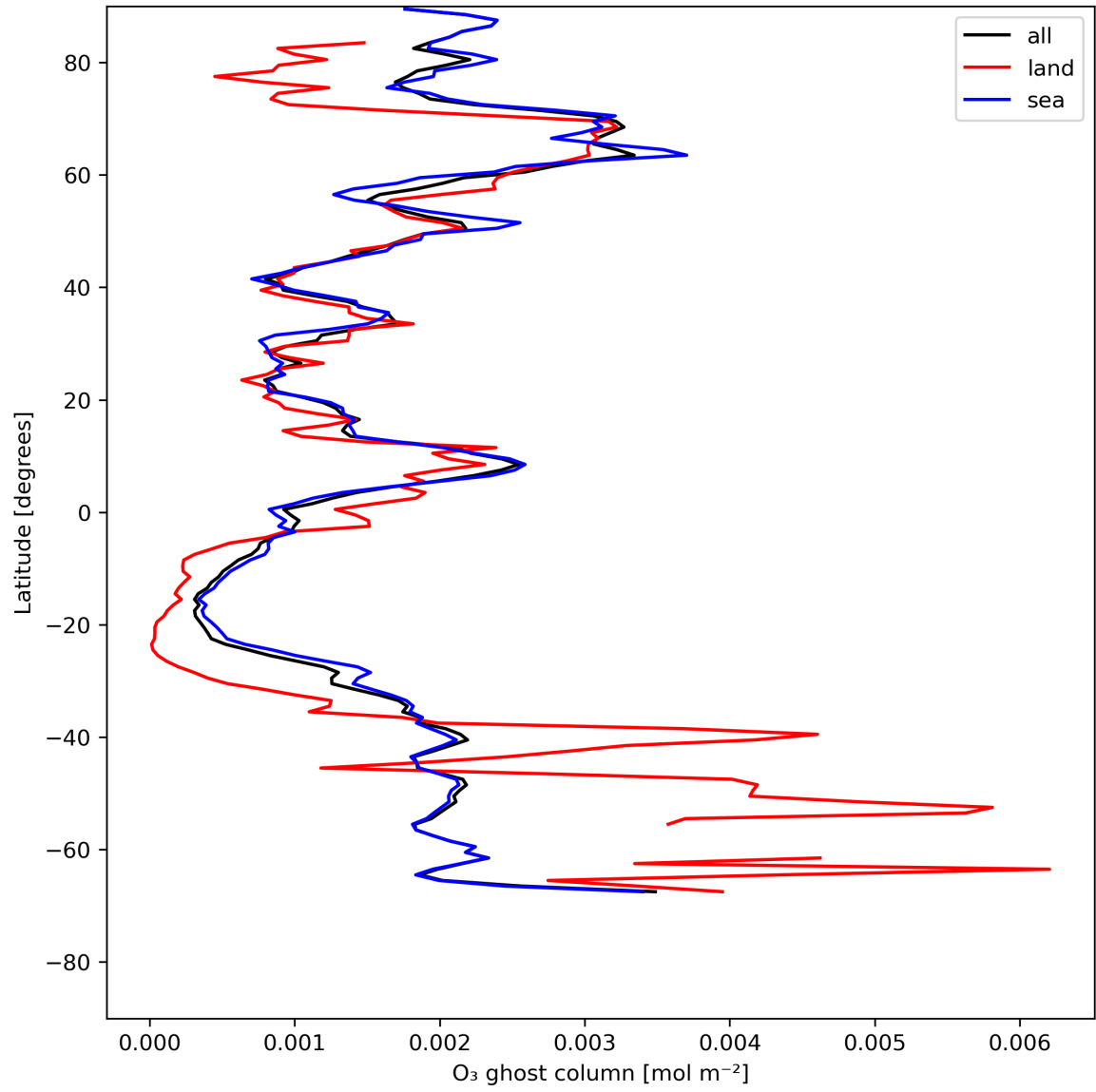
Figure 18: Zonal average of “O 3 ghost column” for 2024-07-16 to 2024-07-18.
