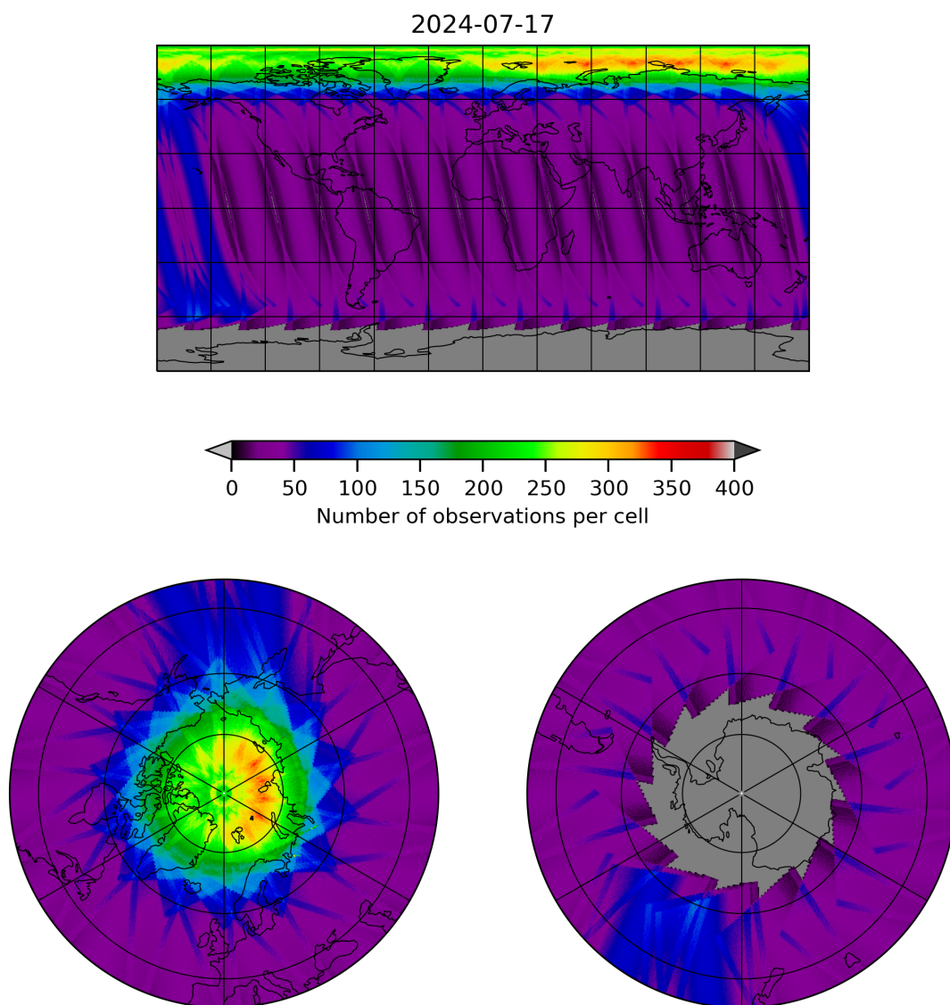
Figure 12: Map of the number of observations for 2024-07-16 to 2024-07-18
