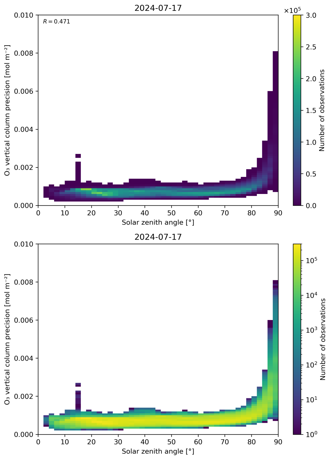
Figure 48: Scatter density plot of “Solar zenith angle” against “O 3 vertical column precision” for 2024-07-16 to 2024-07-18.
