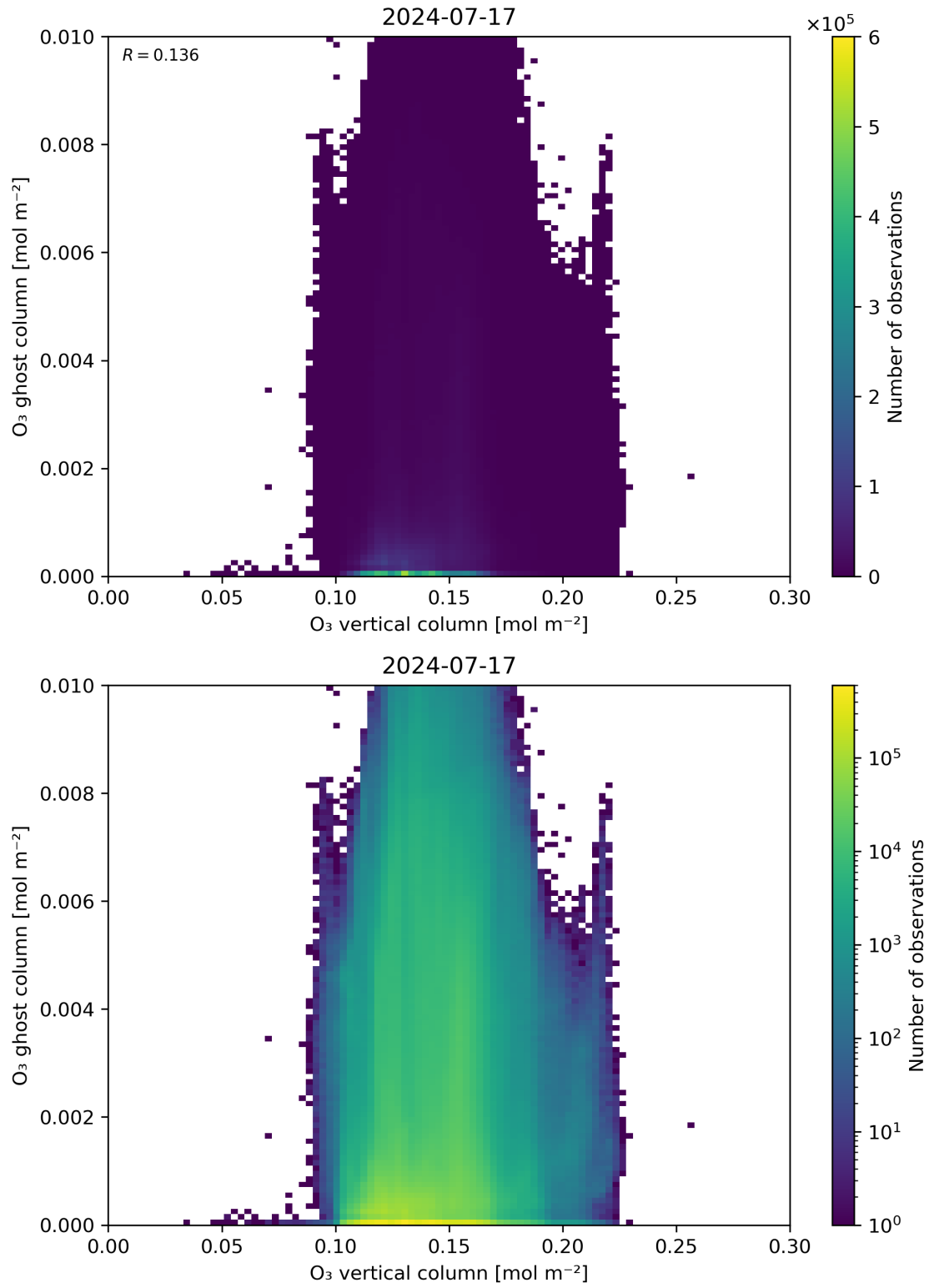
Figure 40: Scatter density plot of “O 3 vertical column” against “O 3 ghost column” for 2024-07-16 to 2024-07-18.
