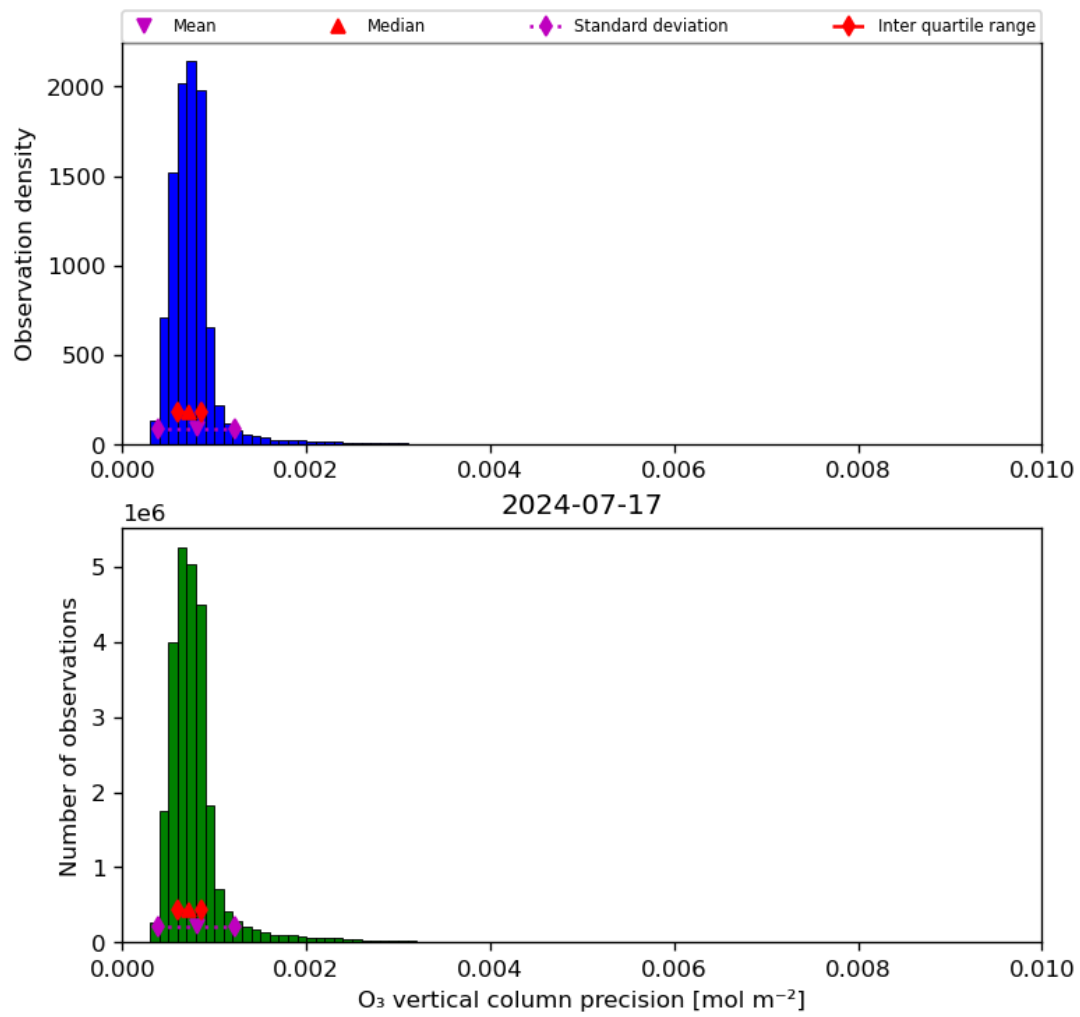
Figure 22: Histogram of “O 3 vertical column precision” for 2024-07-16 to 2024-07-18
