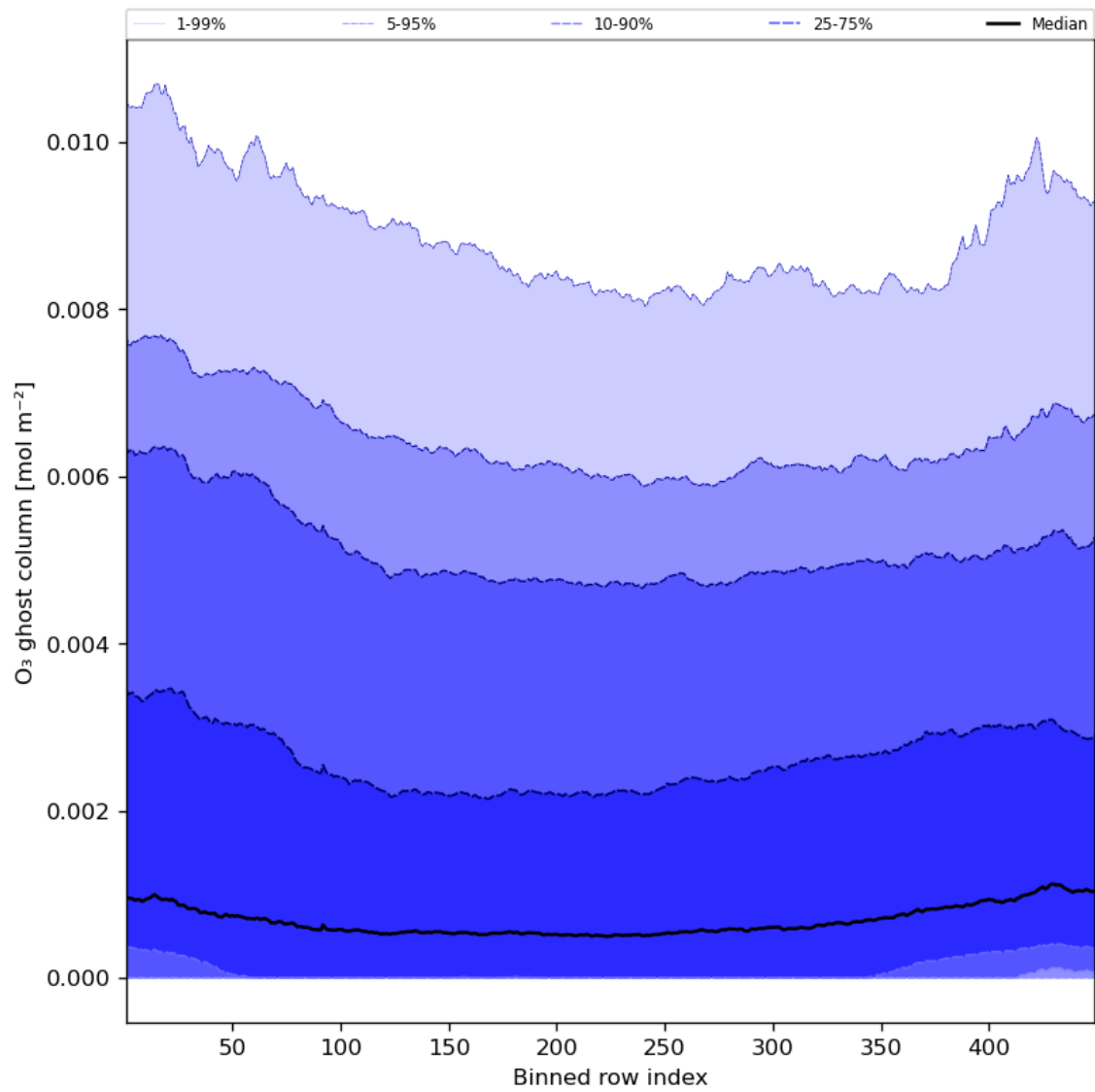
Figure 32: Along track statistics of “O 3 ghost column” for 2024-07-16 to 2024-07-18
