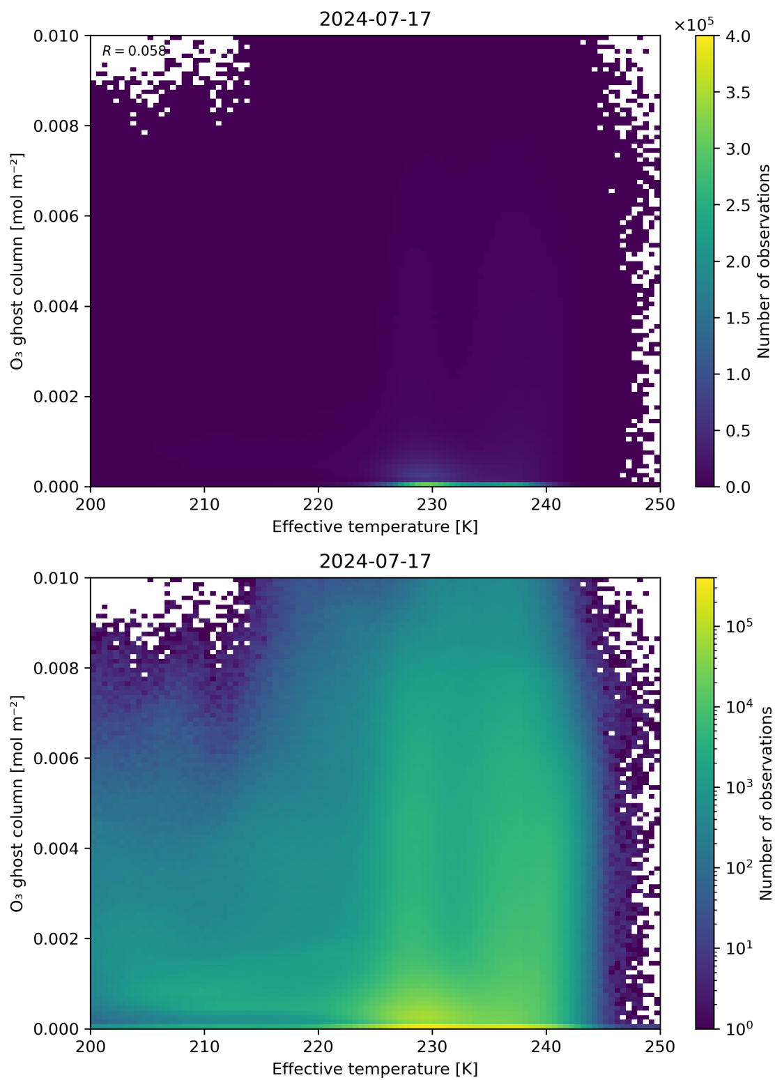
Figure 38: Scatter density plot of “Effective temperature” against “O 3 ghost column” for 2024-07-16 to 2024-07-18.
