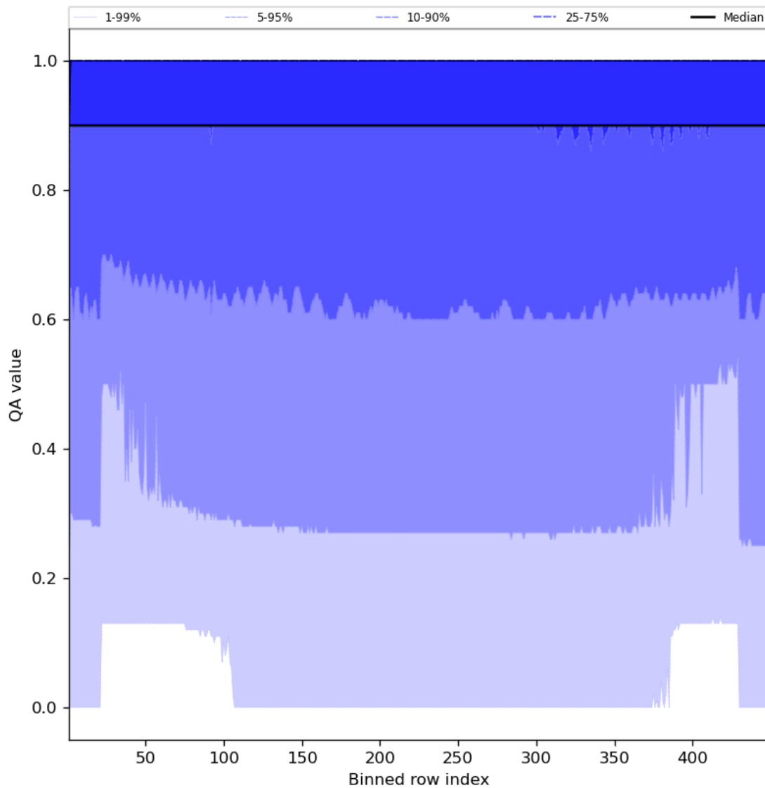
Figure 27: Along track statistics of “QA value” for 2024-07-16 to 2024-07-18
