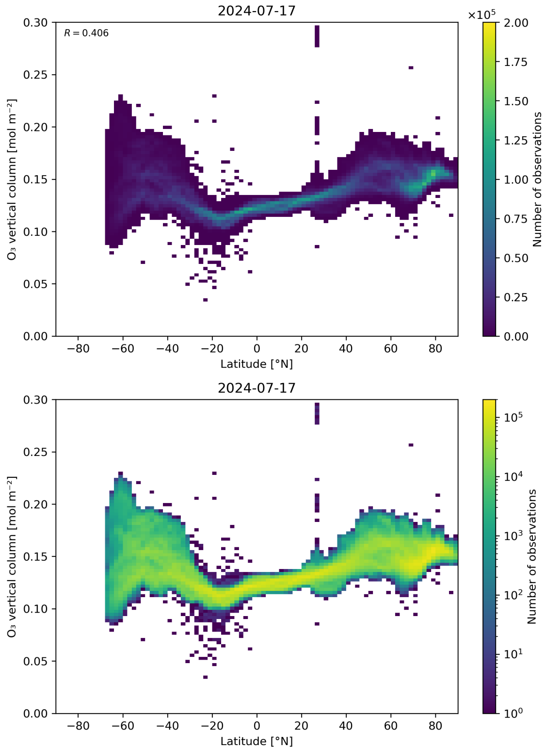
Figure 36: Scatter density plot of “Latitude” against “O 3 vertical column” for 2024-07-16 to 2024-07-18.
