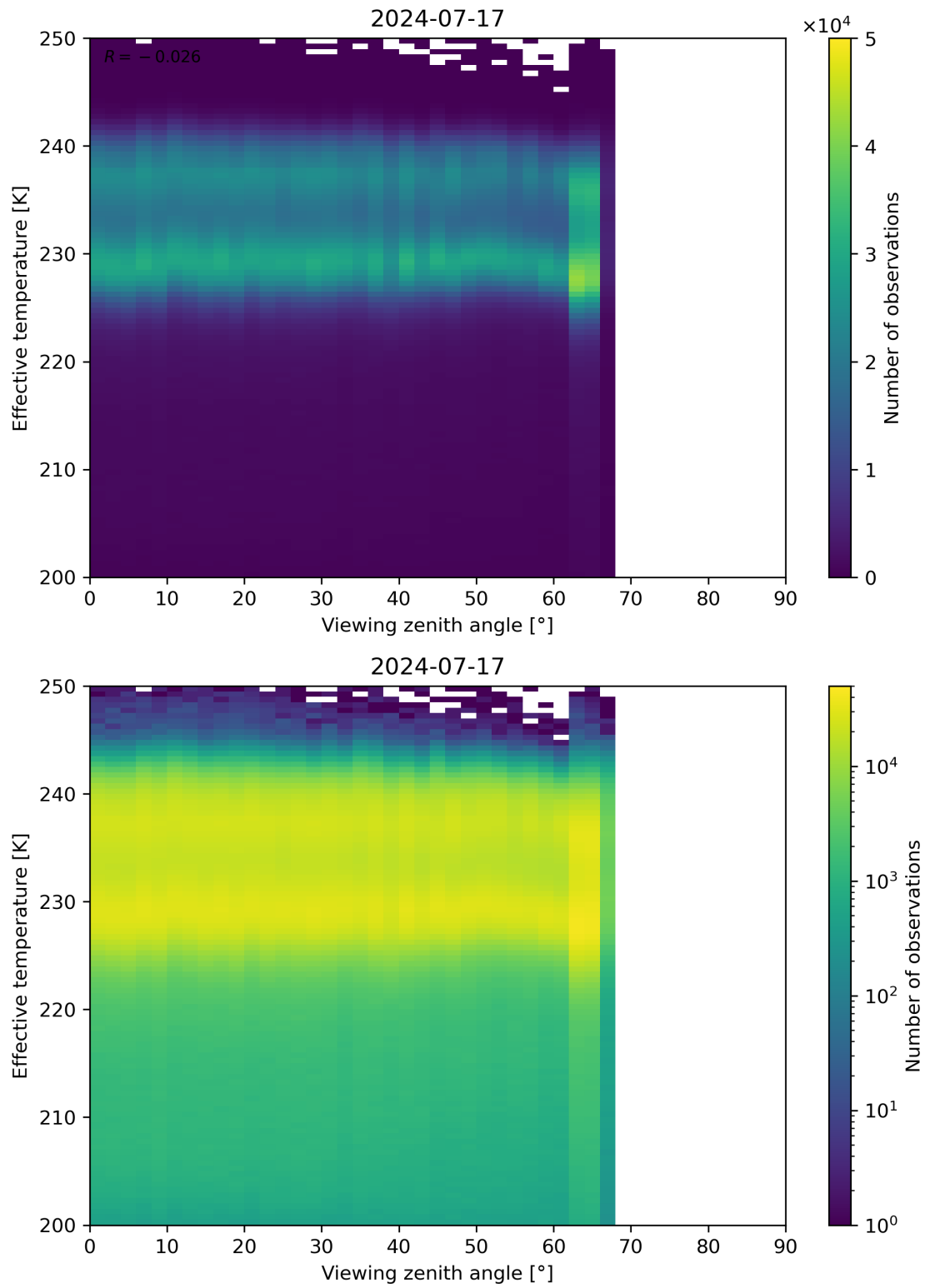
Figure 50: Scatter density plot of “Viewing zenith angle” against “Effective temperature” for 2024-07-16 to 2024-07-18.
