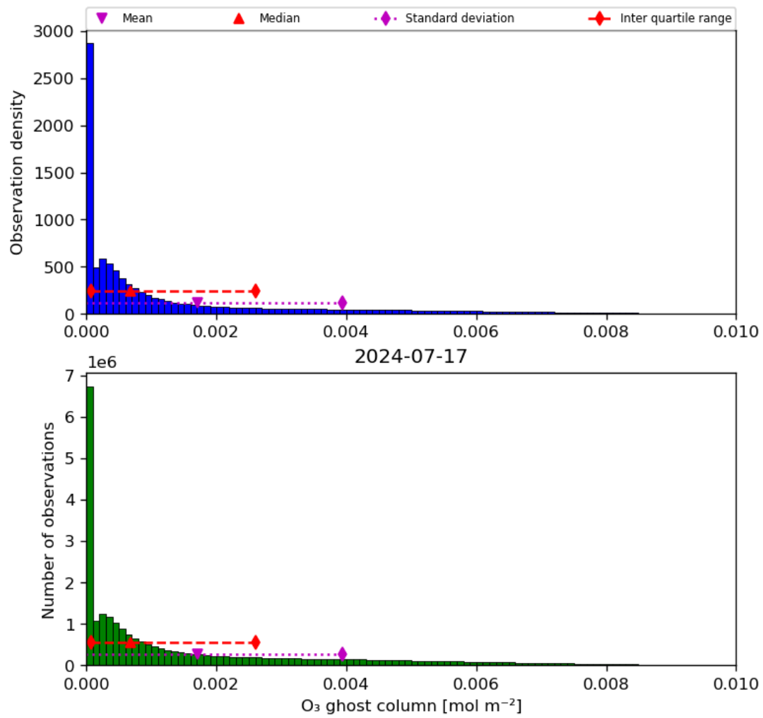
Figure 25: Histogram of “O 3 ghost column” for 2024-07-16 to 2024-07-18
