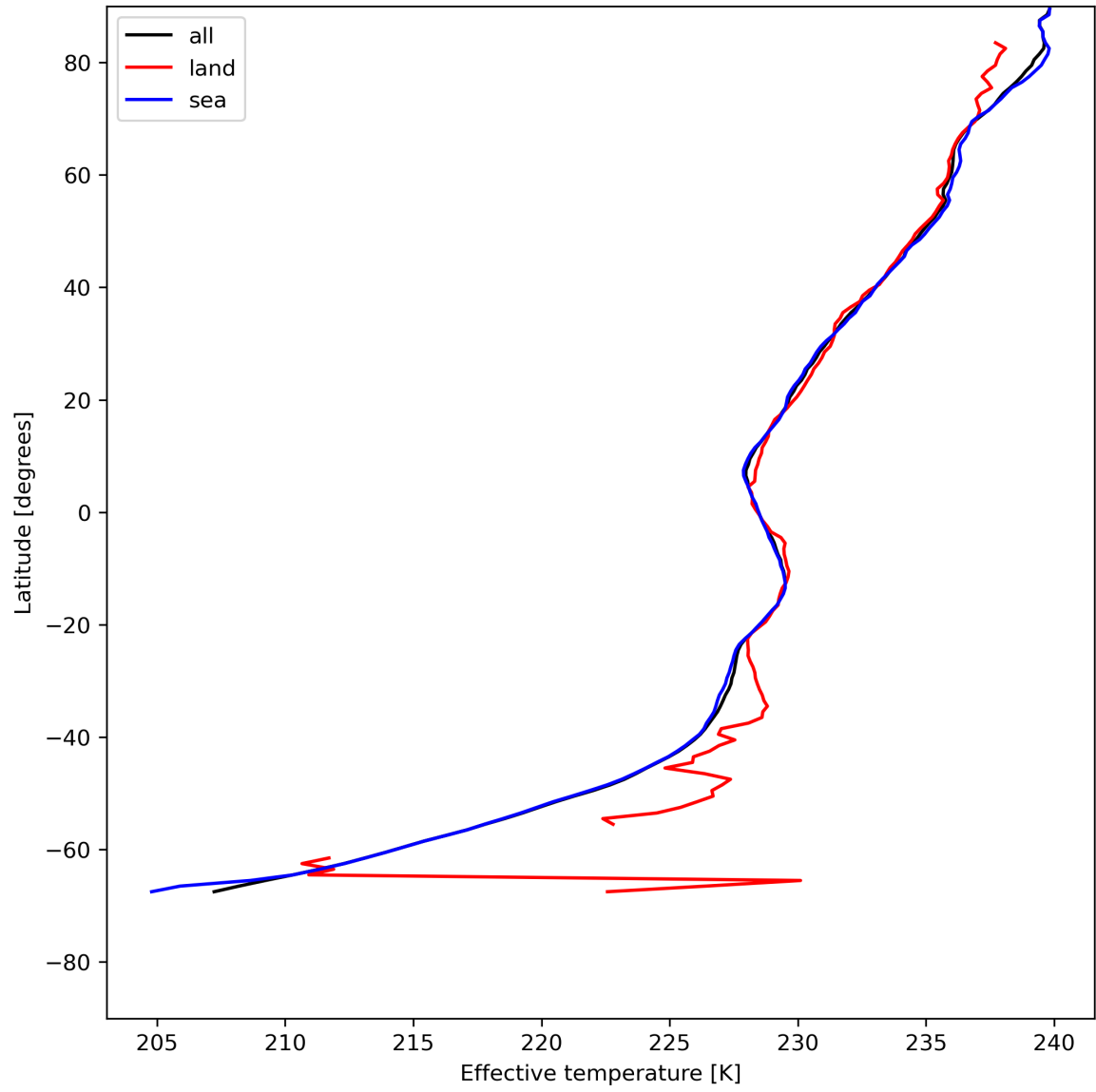
Figure 17: Zonal average of "Effective temperature" for 2024-07-16 to 2024-07-18.
