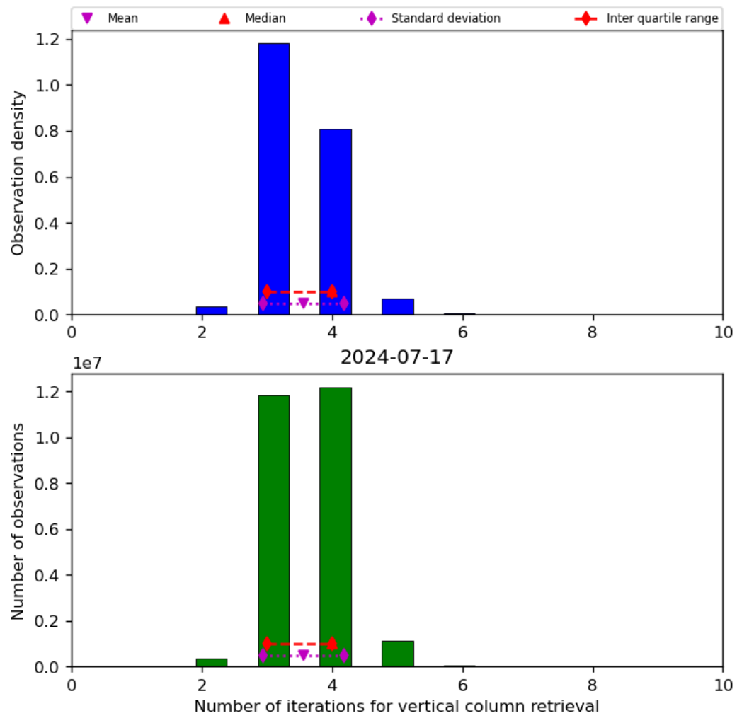
Figure 26: Histogram of “Number of iterations for vertical column retrieval” for 2024-07-16 to 2024-07-18
