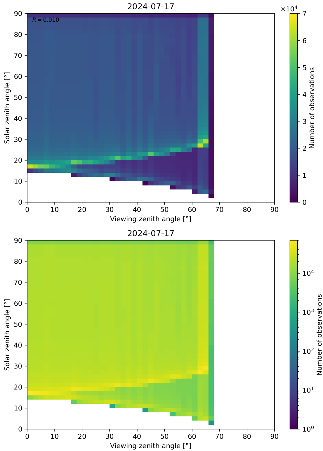
Figure 54: Scatter density plot of “Viewing zenith angle” against “Solar zenith angle” for 2024-07-16 to 2024-07-18.
