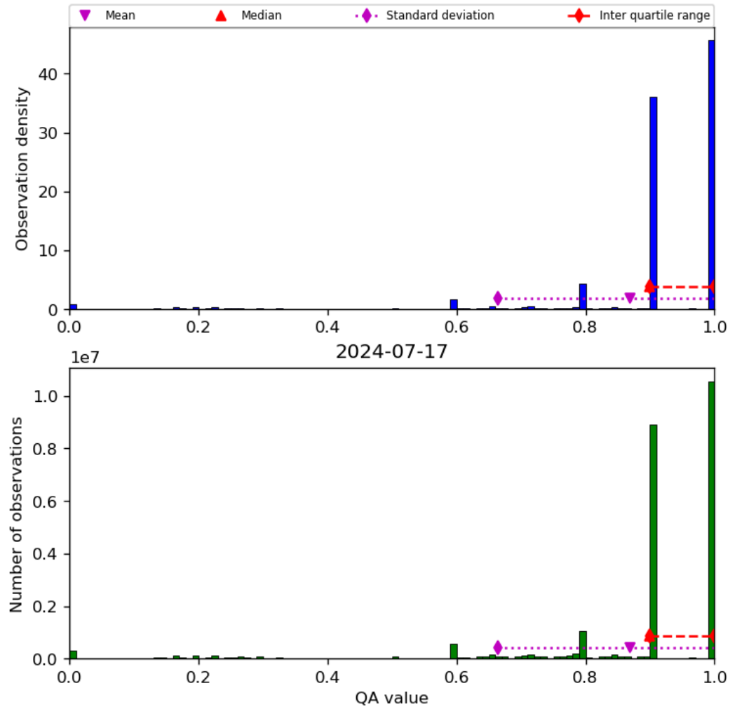
Figure 20: Histogram of “QA value” for 2024-07-16 to 2024-07-18
