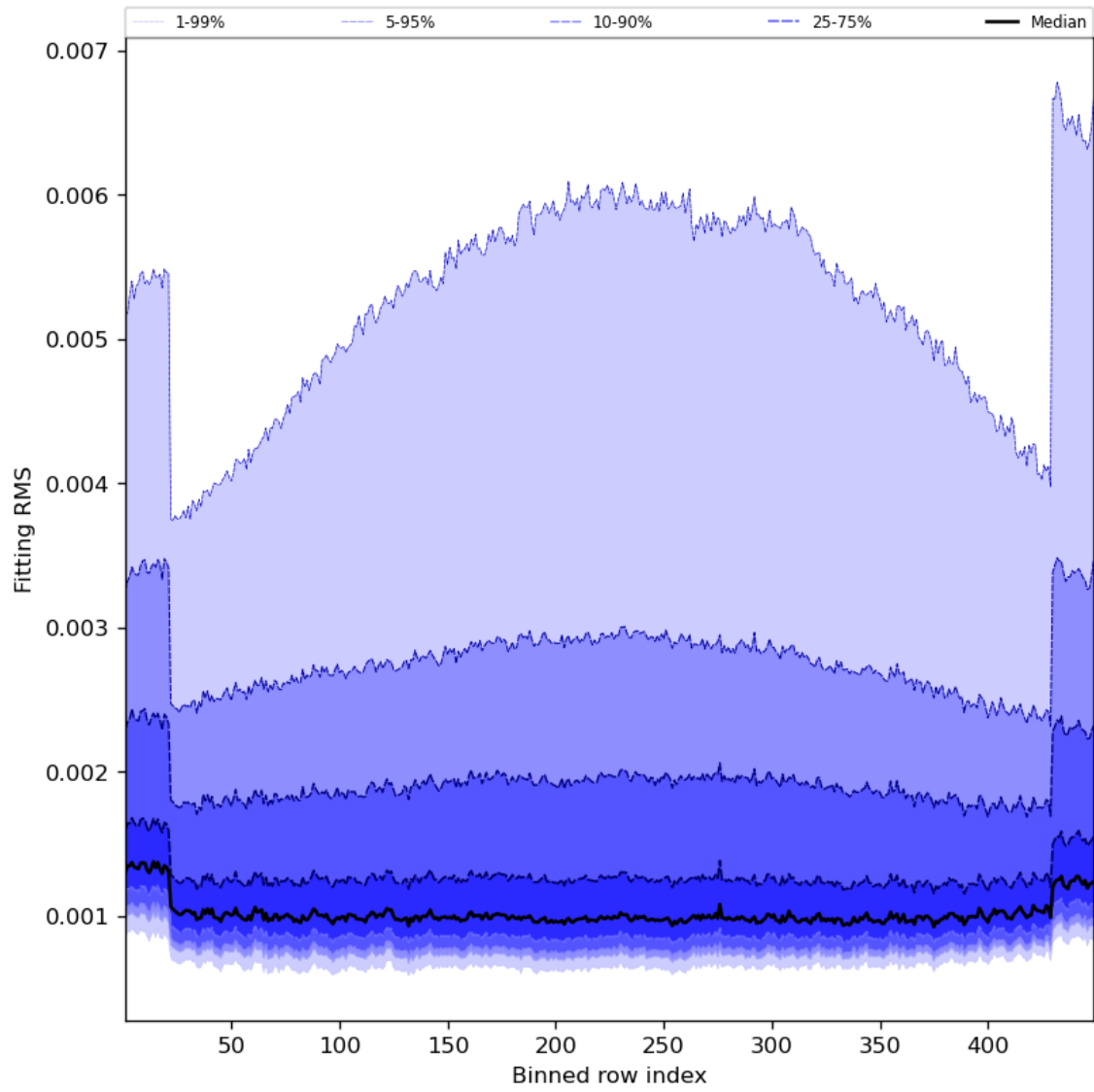
Figure 30: Along track statistics of “Fitting RMS” for 2024-07-16 to 2024-07-18
