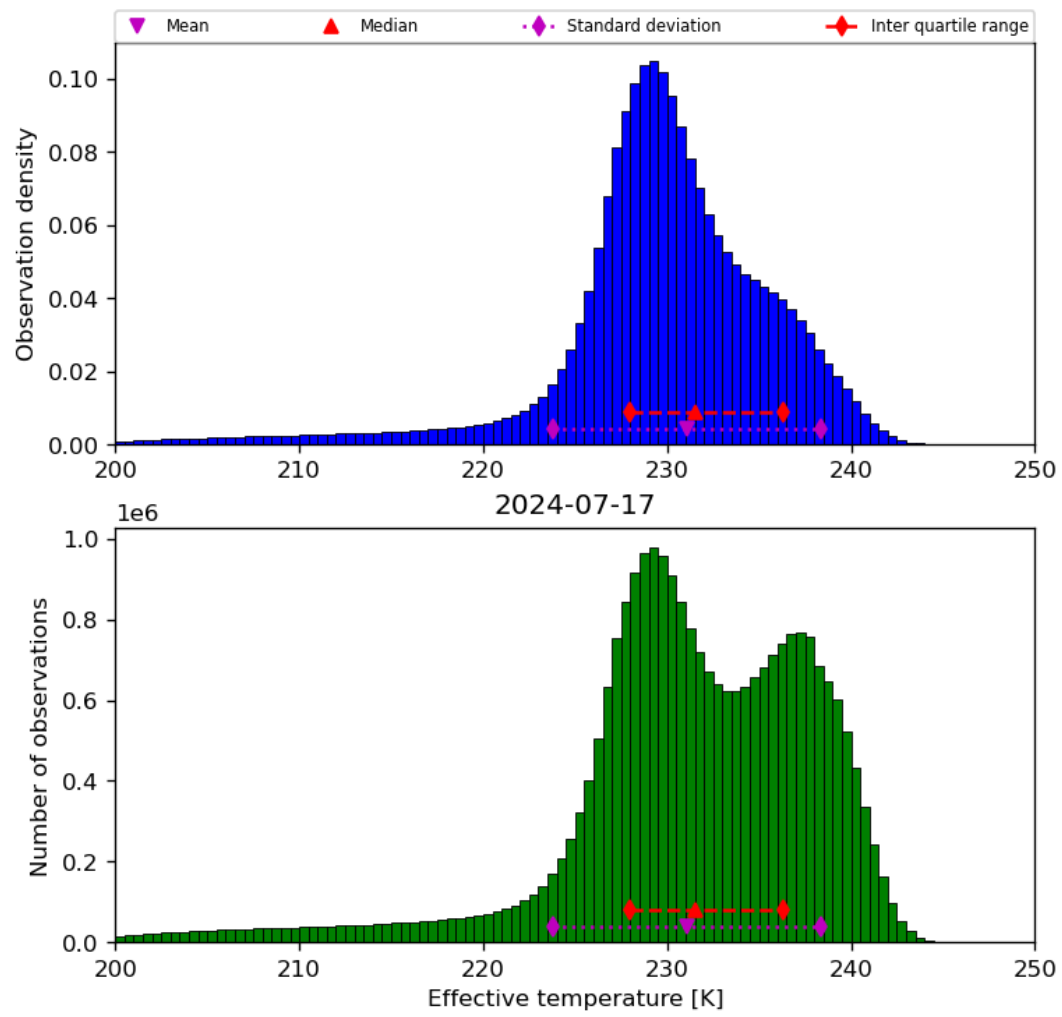
Figure 24: Histogram of “Effective temperature” for 2024-07-16 to 2024-07-18
