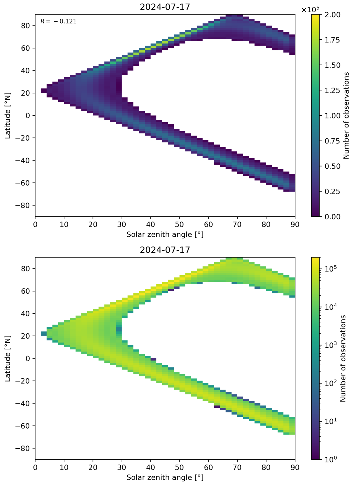
Figure 44: Scatter density plot of “Solar zenith angle” against “Latitude” for 2024-07-16 to 2024-07-18.
