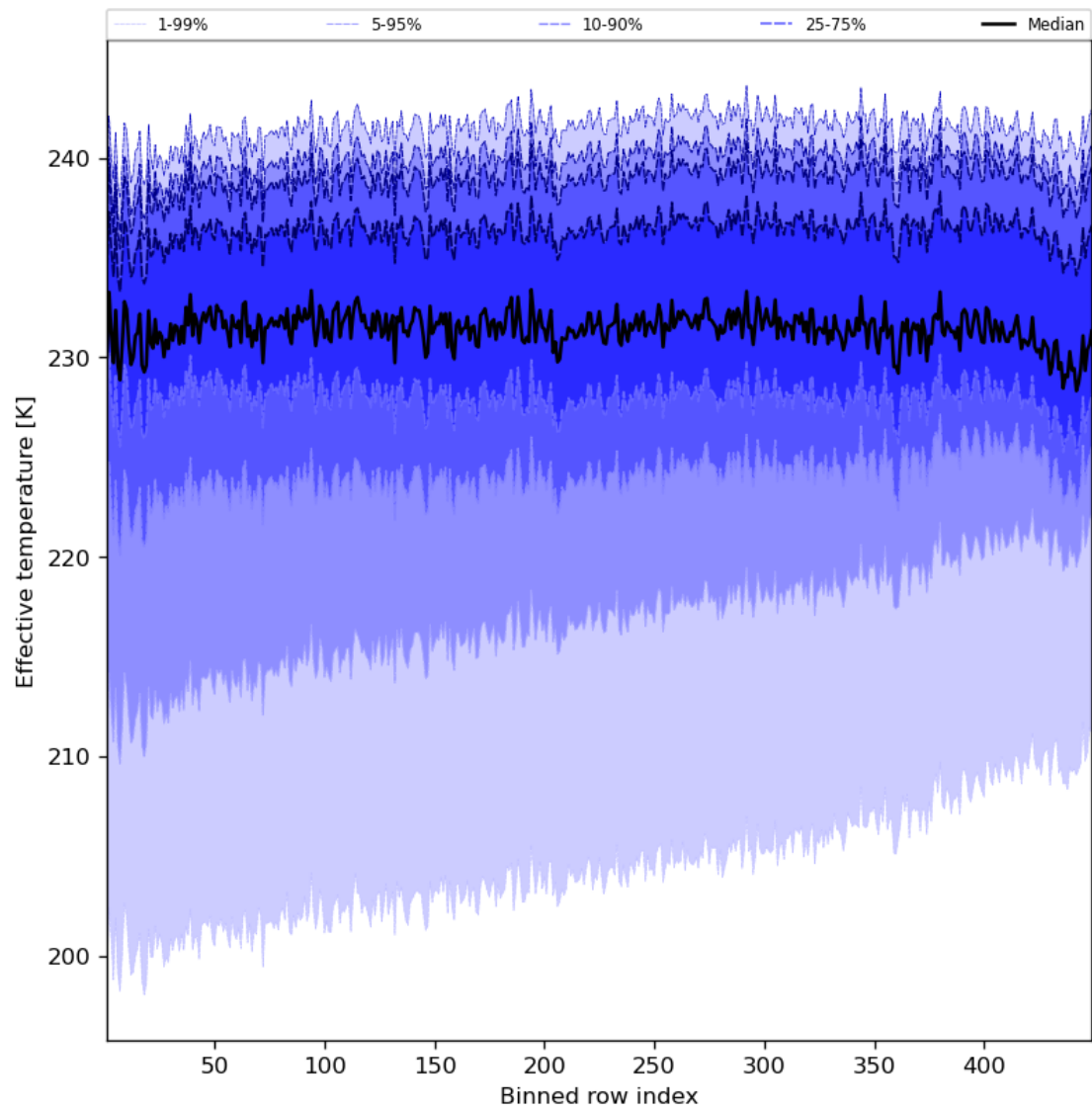
Figure 31: Along track statistics of “Effective temperature” for 2024-07-16 to 2024-07-18
