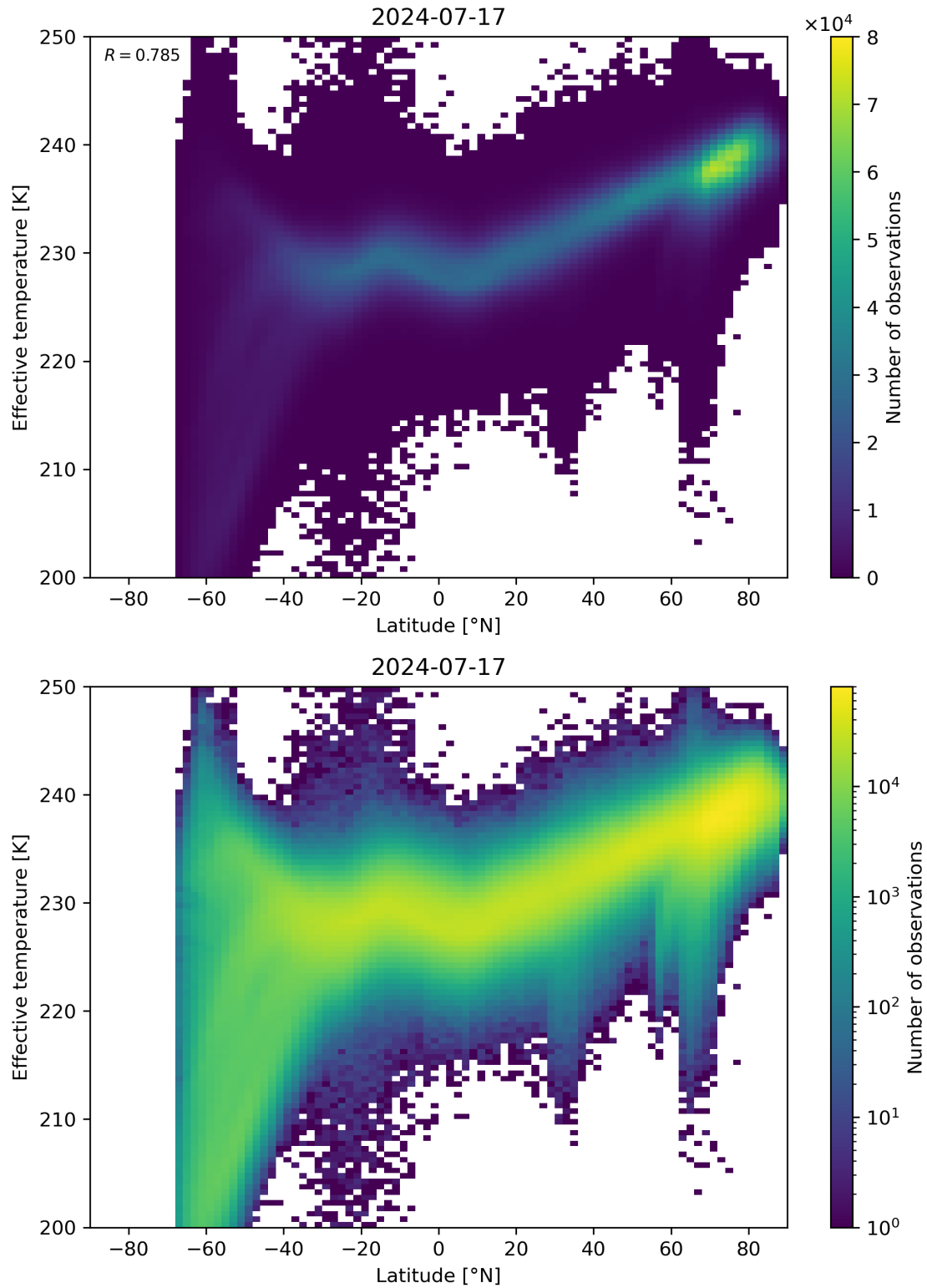
Figure 34: Scatter density plot of “Latitude” against “Effective temperature” for 2024-07-16 to 2024-07-18.
