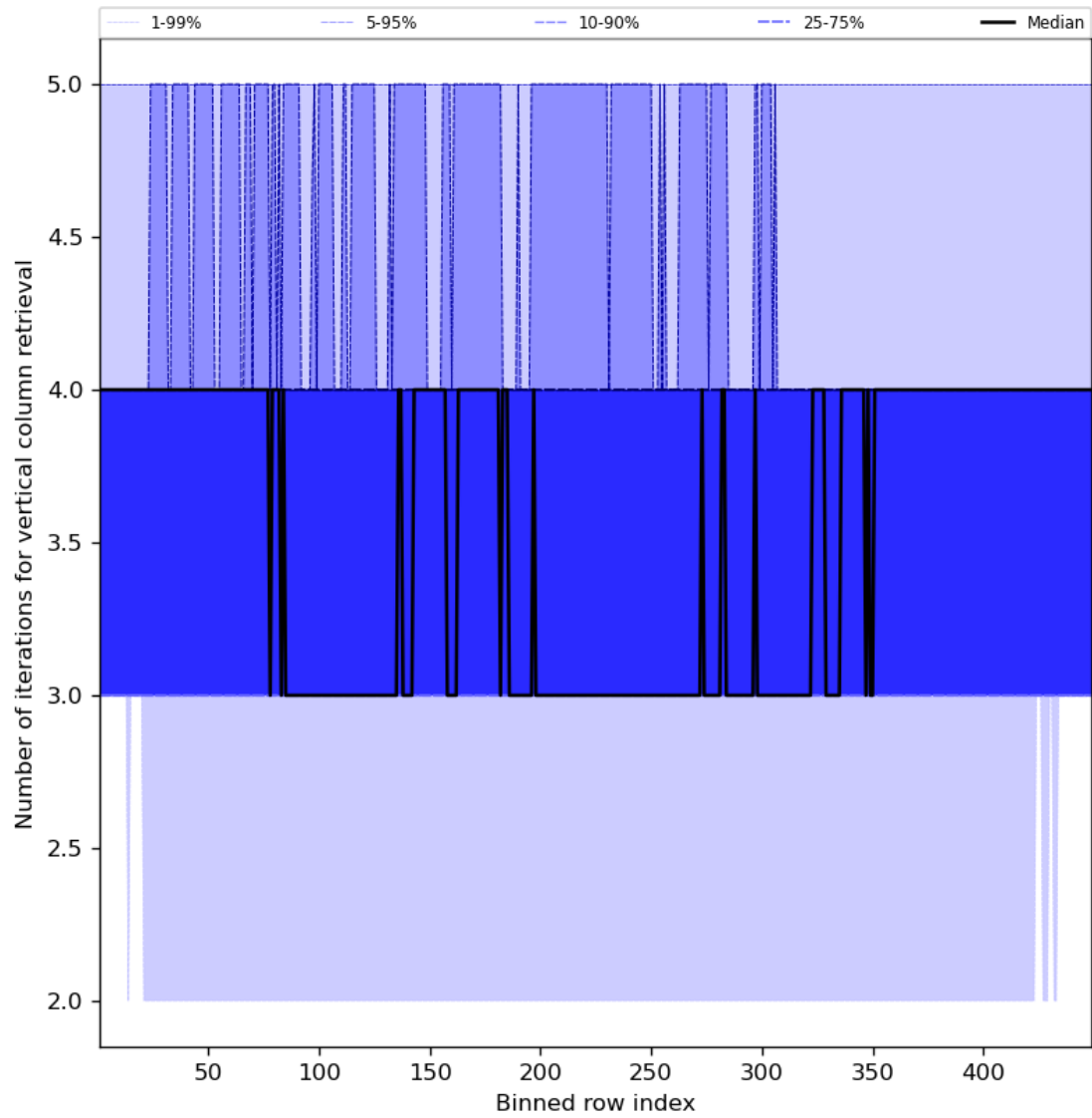
Figure 33: Along track statistics of “Number of iterations for vertical column retrieval” for 2024-07-16 to 2024-07-18
