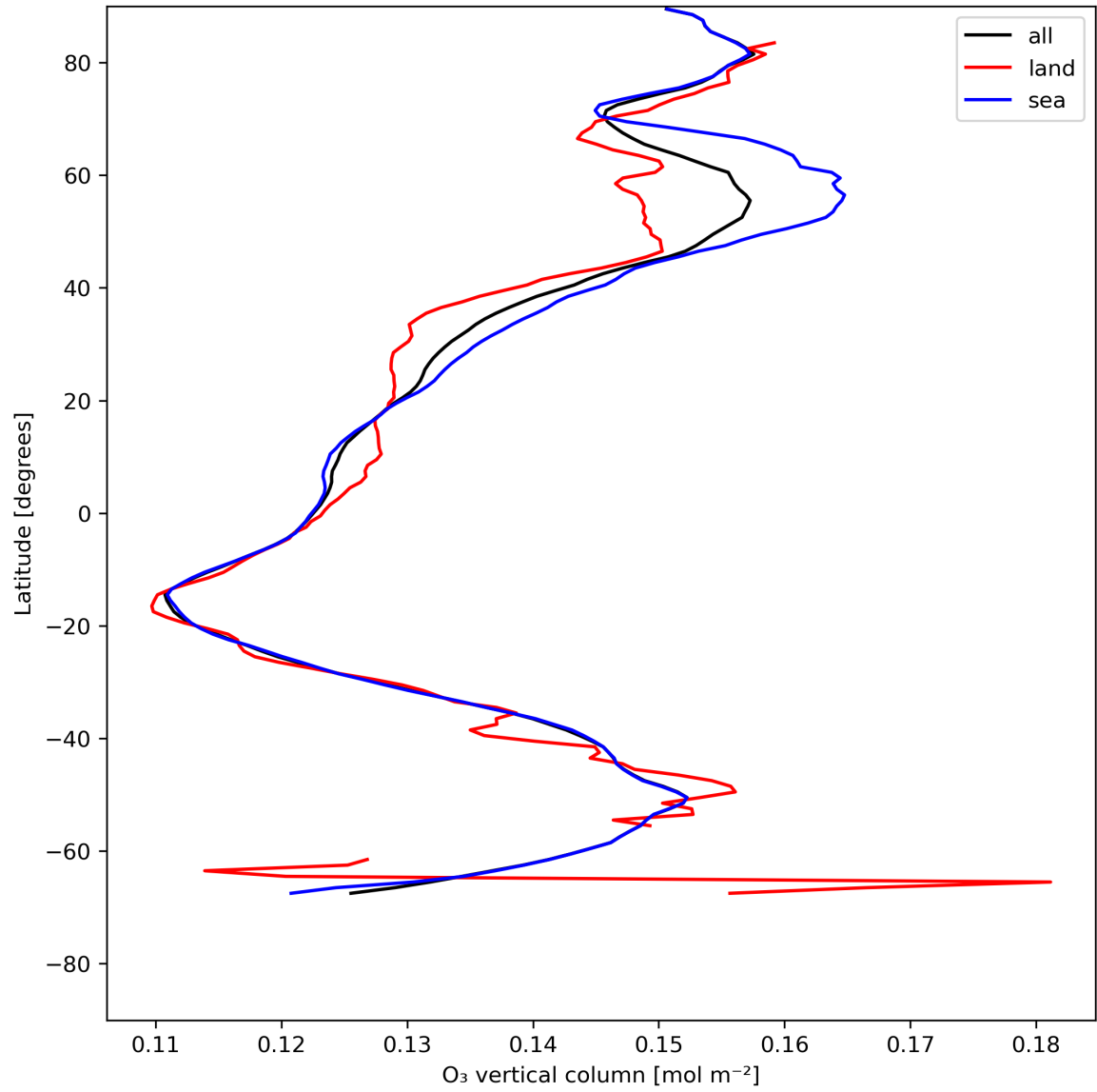
Figure 14: Zonal average of “O 3 vertical column” for 2024-07-16 to 2024-07-18.
