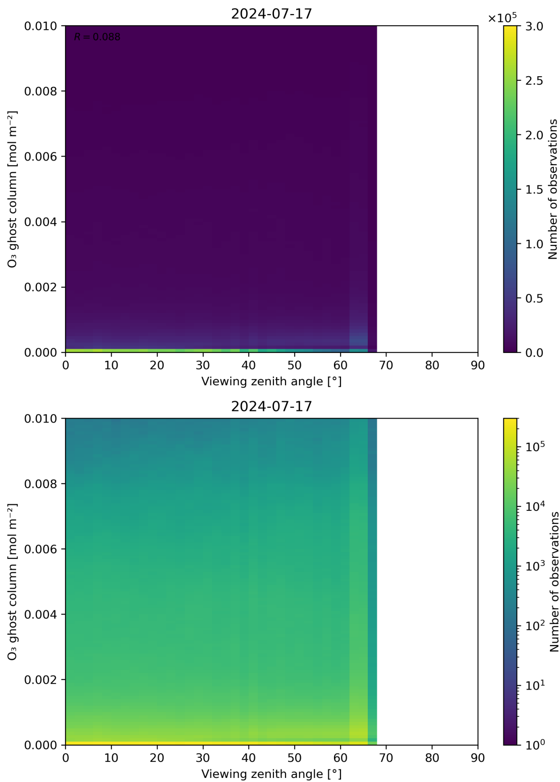
Figure 51: Scatter density plot of “Viewing zenith angle” against “O 3 ghost column” for 2024-07-16 to 2024-07-18.
