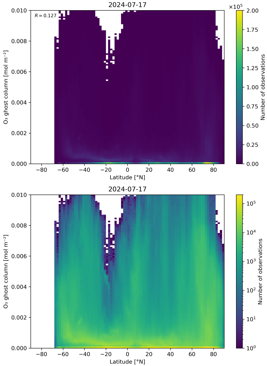
Figure 35: Scatter density plot of “Latitude” against “O 3 ghost column” for 2024-07-16 to 2024-07-18.
