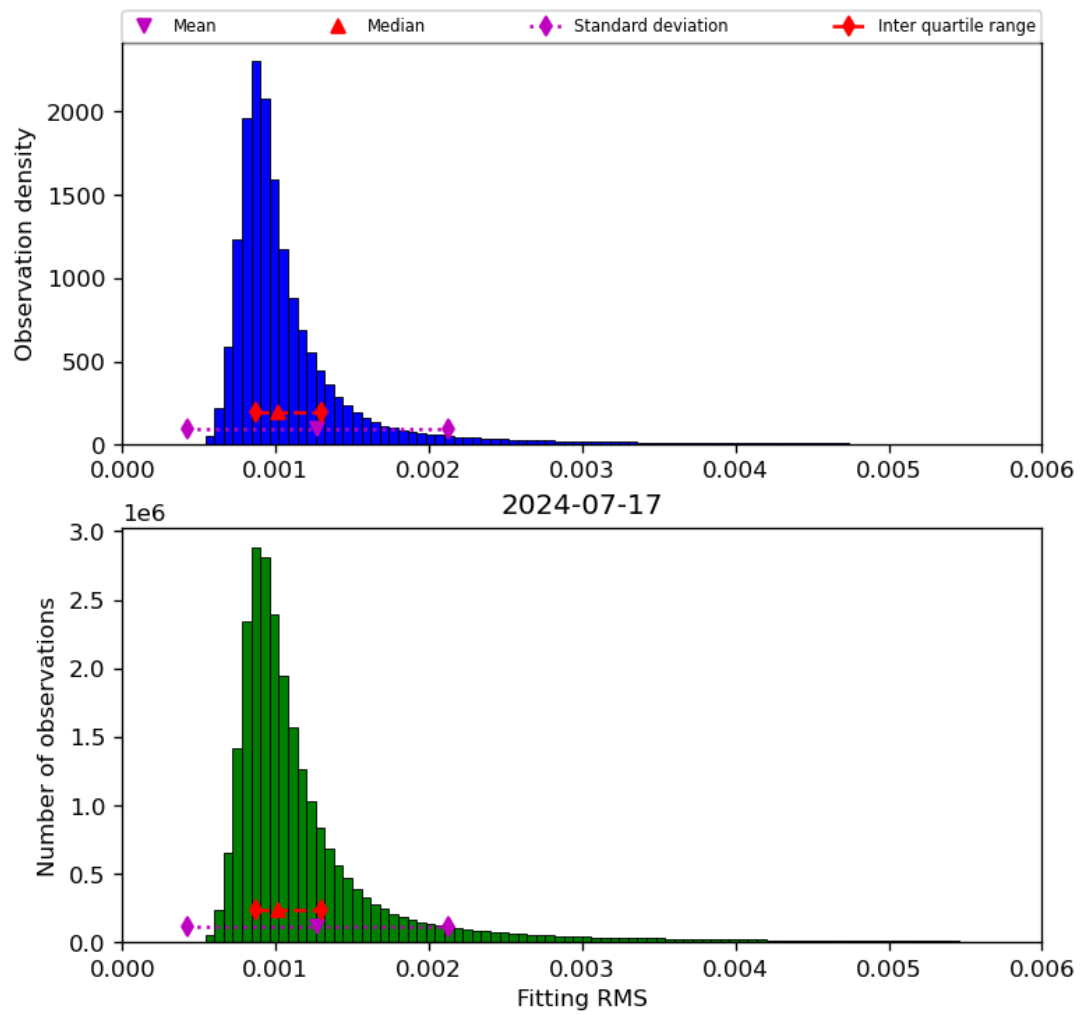
Figure 23: Histogram of “Fitting RMS” for 2024-07-16 to 2024-07-18
