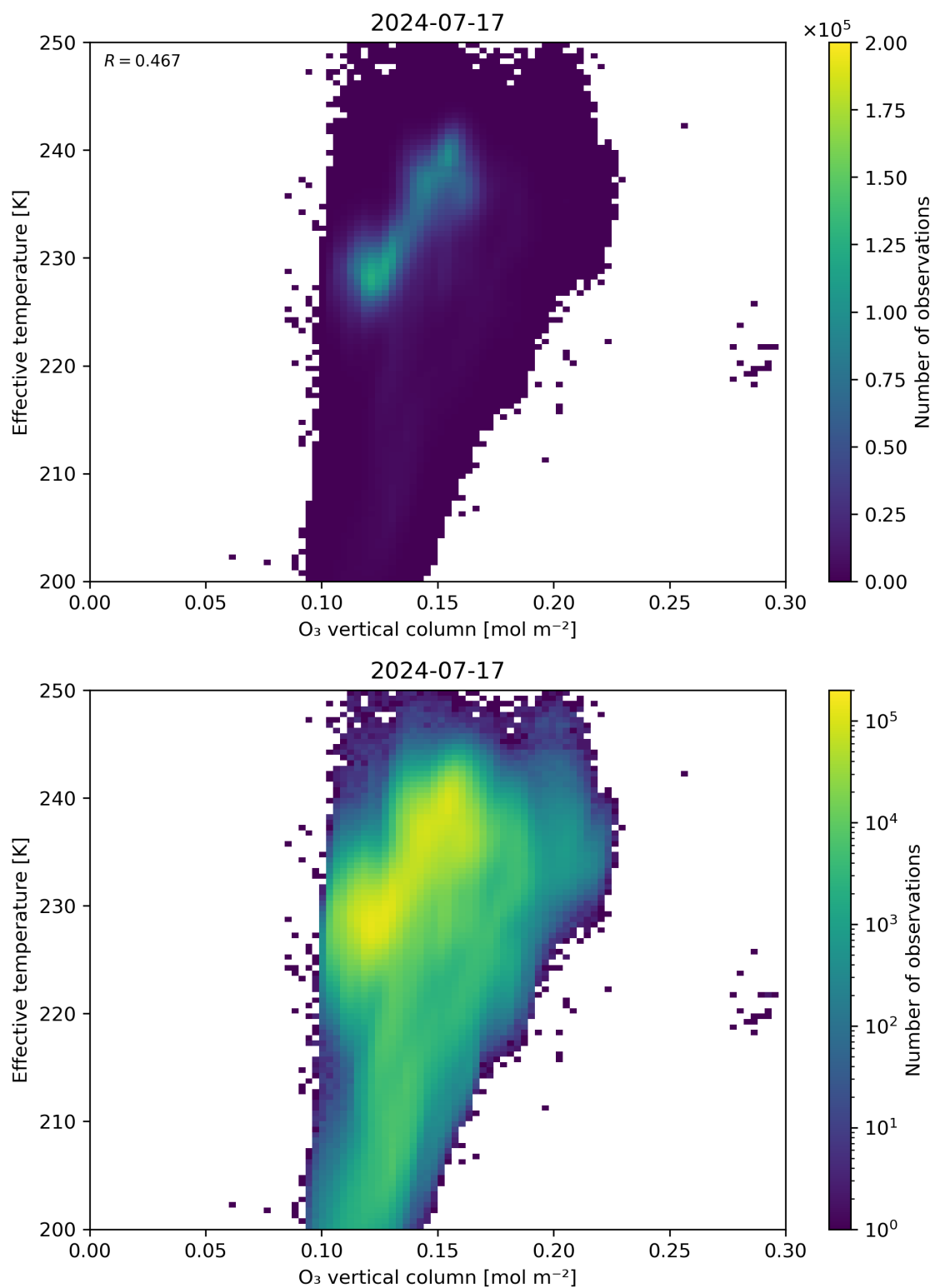
Figure 39: Scatter density plot of “O 3 vertical column” against “Effective temperature” for 2024-07-16 to 2024-07-18.
