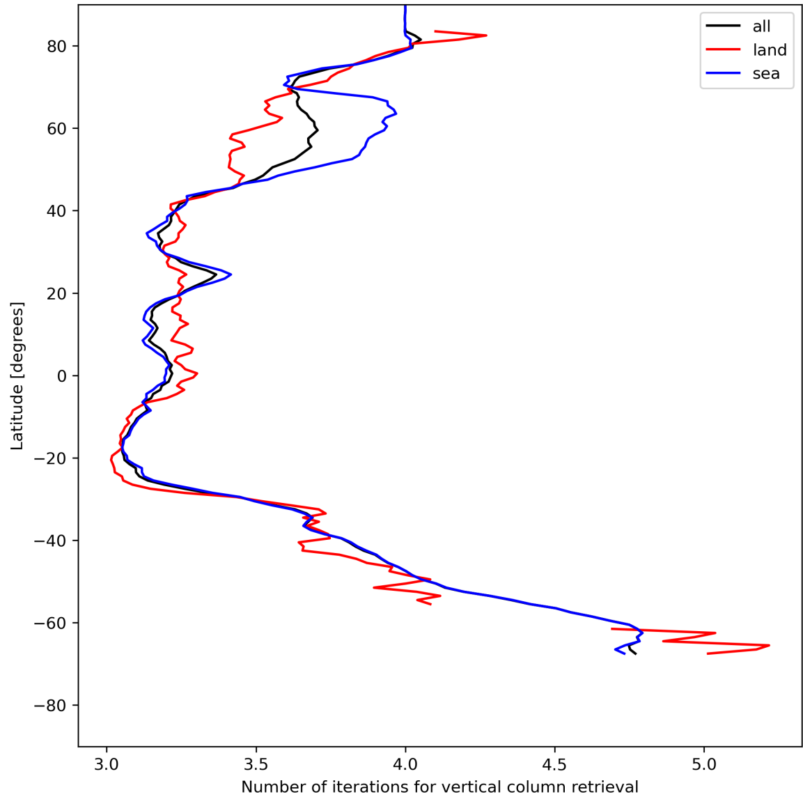
Figure 19: Zonal average of “Number of iterations for vertical column retrieval” for 2024-07-16 to 2024-07-18.
