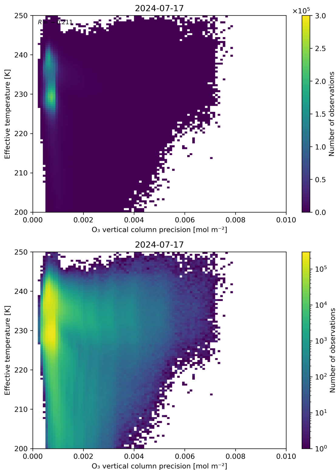
Figure 42: Scatter density plot of “O 3 vertical column precision” against “Effective temperature” for 2024-07-16 to 2024-07-18.
