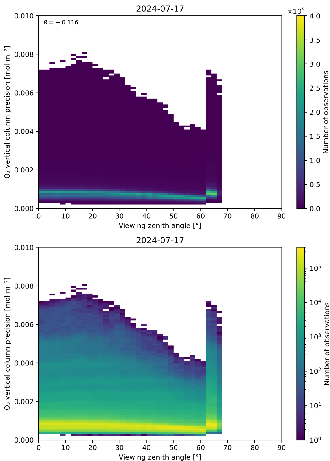
Figure 53: Scatter density plot of “Viewing zenith angle” against “O 3 vertical column precision” for 2024-07-16 to 2024-07-18.
