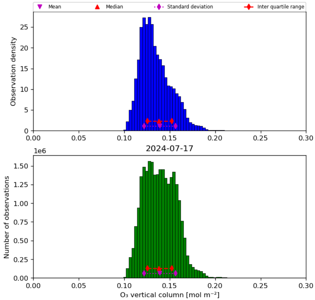
Figure 21: Histogram of “O 3 vertical column” for 2024-07-16 to 2024-07-18
