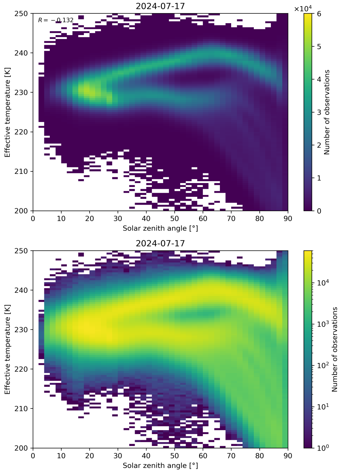
Figure 45: Scatter density plot of “Solar zenith angle” against “Effective temperature” for 2024-07-16 to 2024-07-18.
