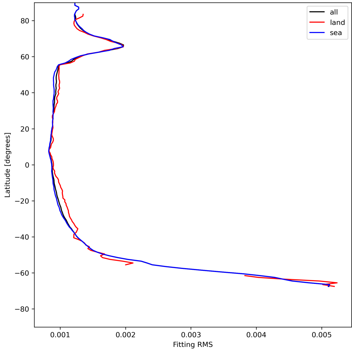
Figure 16: Zonal average of “Fitting RMS” for 2024-07-16 to 2024-07-18.
