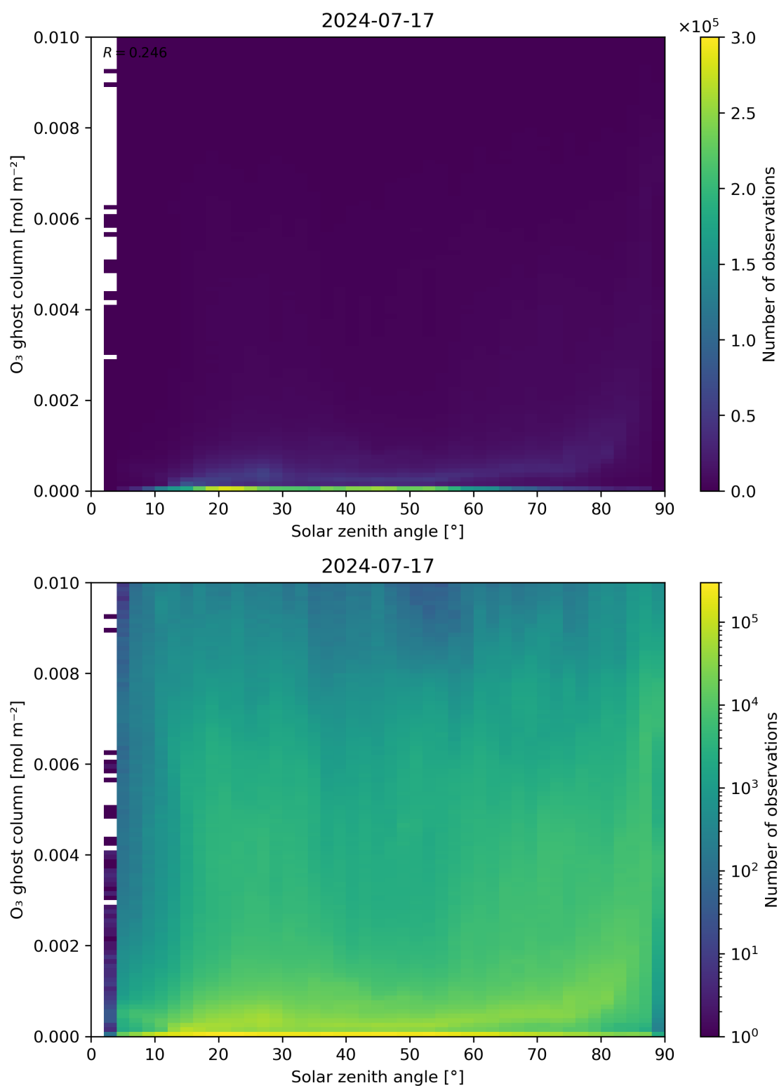
Figure 46: Scatter density plot of “Solar zenith angle” against “O 3 ghost column” for 2024-07-16 to 2024-07-18.
