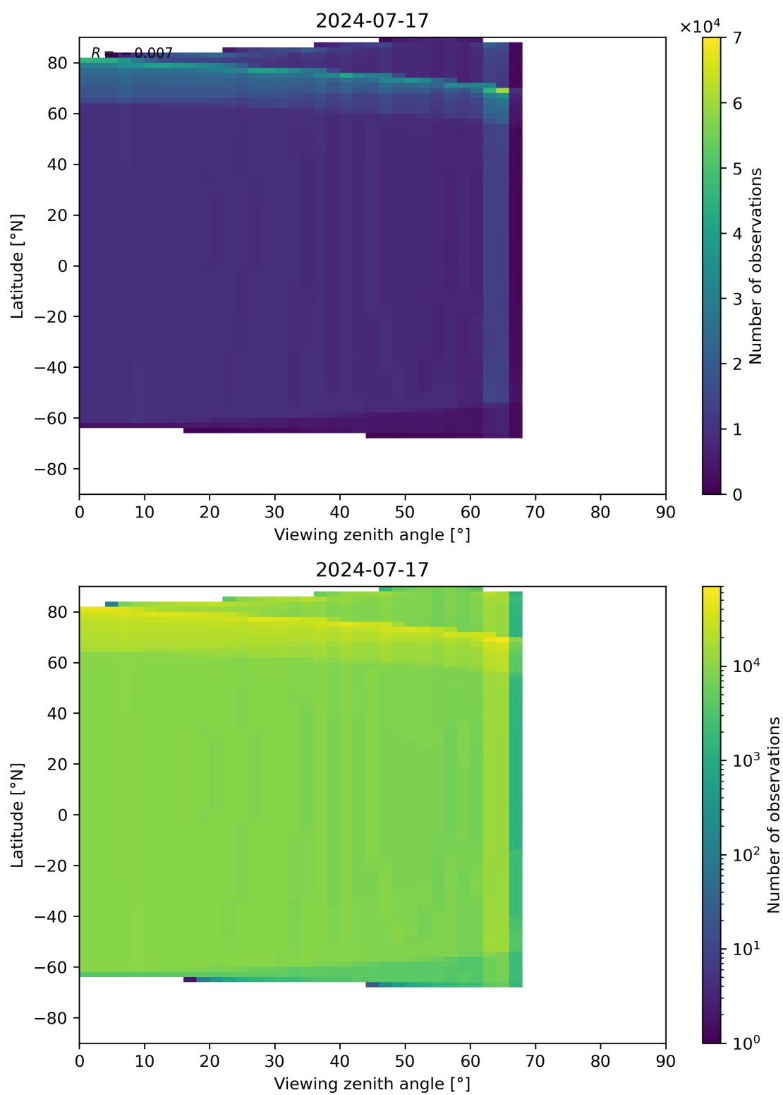
Figure 49: Scatter density plot of “Viewing zenith angle” against “Latitude” for 2024-07-16 to 2024-07-18.
