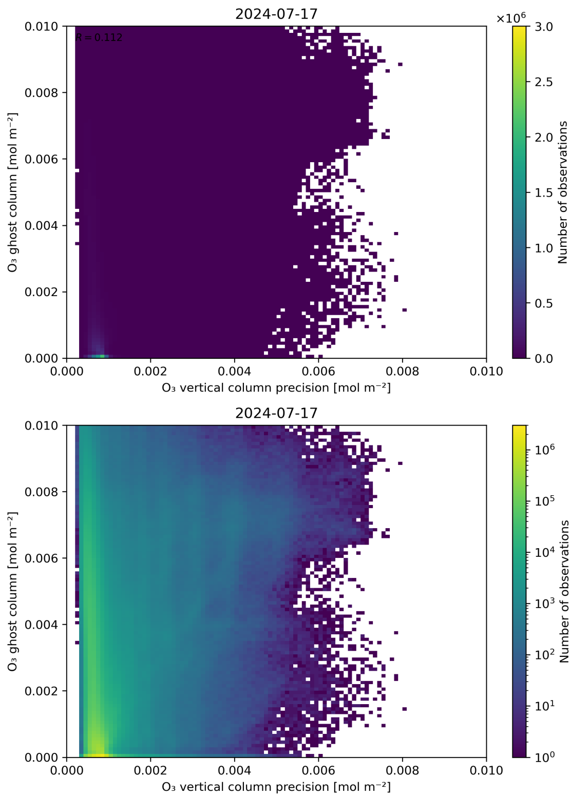
Figure 43: Scatter density plot of “ \text{O}_3 vertical column precision” against “ \text{O}_3 ghost column” for 2024-07-16 to 2024-07-18.
