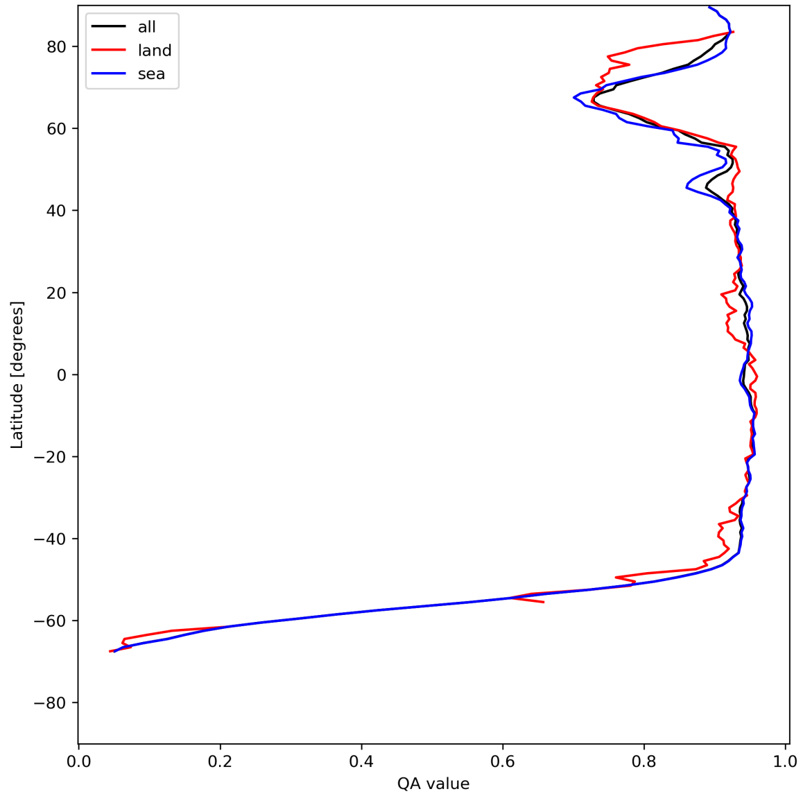
Figure 13: Zonal average of “QA value” for 2024-07-16 to 2024-07-18.
