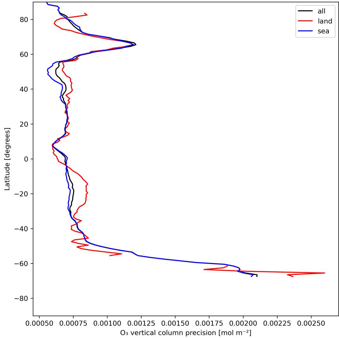
Figure 15: Zonal average of “O 3 vertical column precision” for 2024-07-16 to 2024-07-18.
