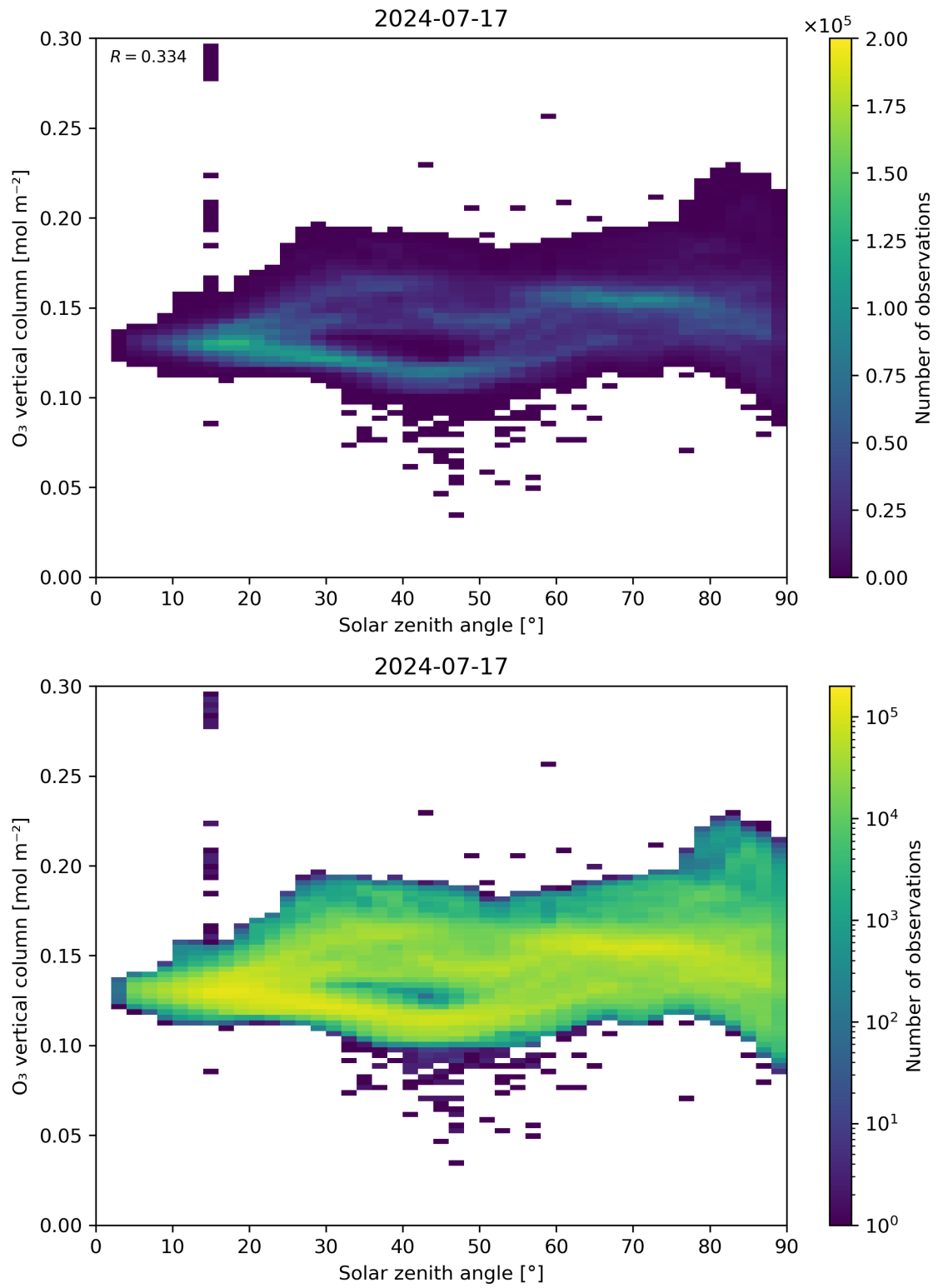
Figure 47: Scatter density plot of “Solar zenith angle” against “O 3 vertical column” for 2024-07-16 to 2024-07-18.
