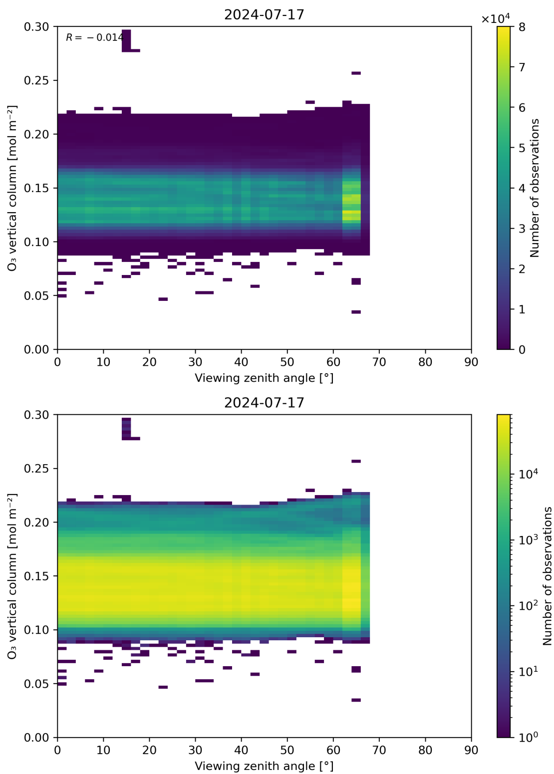
Figure 52: Scatter density plot of “Viewing zenith angle” against “O 3 vertical column” for 2024-07-16 to 2024-07-18.
