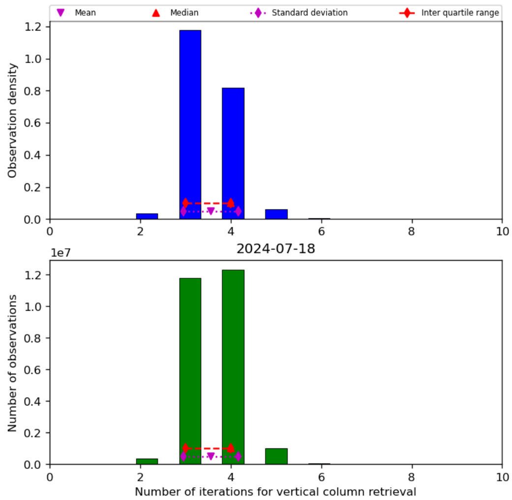
Figure 26: Histogram of “Number of iterations for vertical column retrieval” for 2024-07-17 to 2024-07-19
