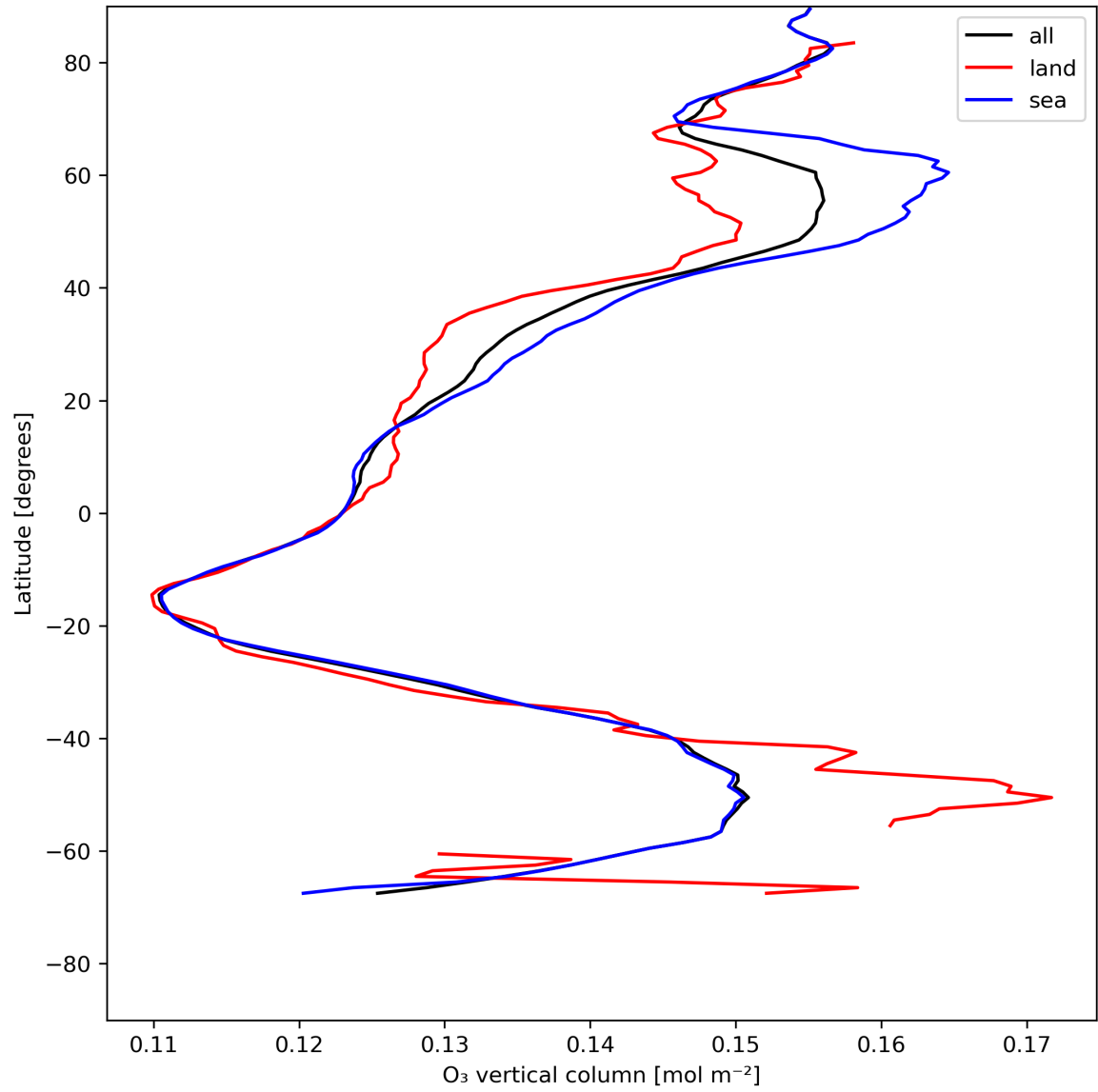
Figure 14: Zonal average of “O 3 vertical column” for 2024-07-17 to 2024-07-19.
