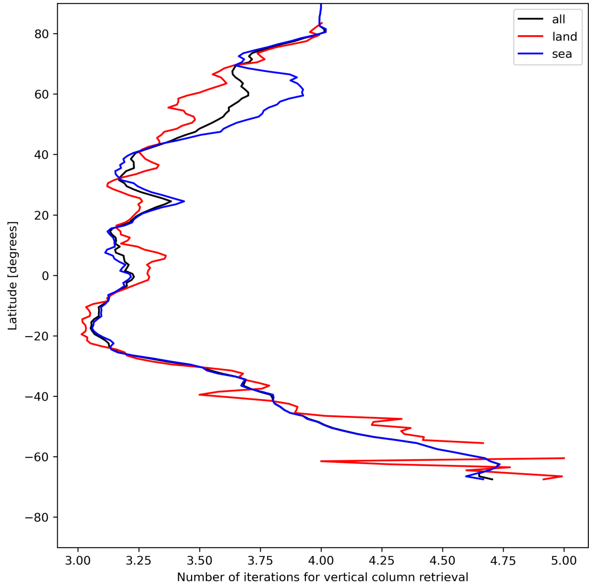
Figure 19: Zonal average of “Number of iterations for vertical column retrieval” for 2024-07-17 to 2024-07-19.
