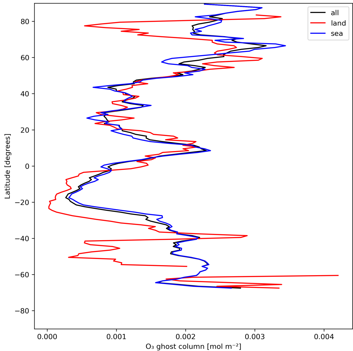
Figure 18: Zonal average of “O 3 ghost column” for 2024-07-17 to 2024-07-19.
