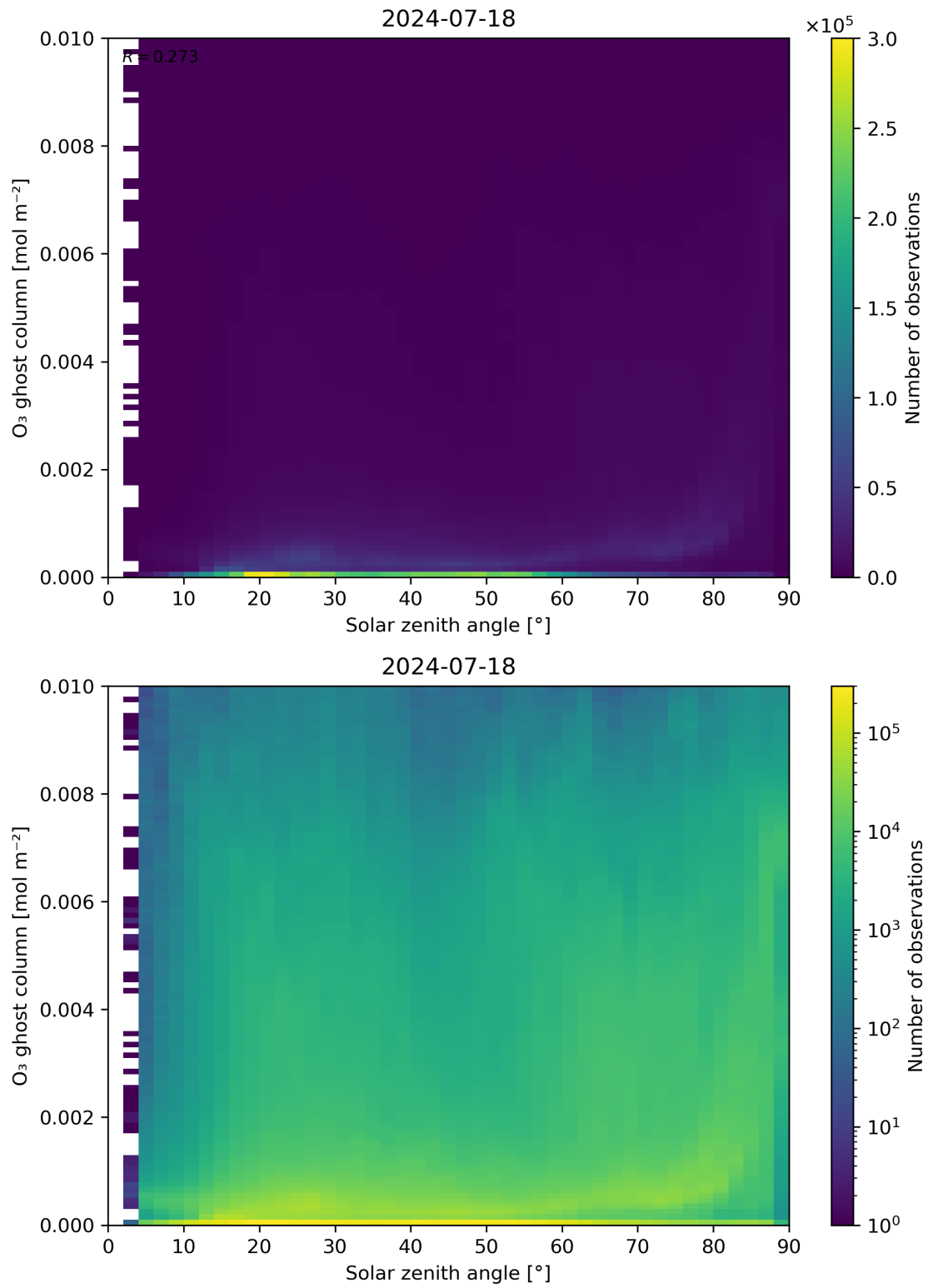
Figure 46: Scatter density plot of “Solar zenith angle” against “O 3 ghost column” for 2024-07-17 to 2024-07-19.
