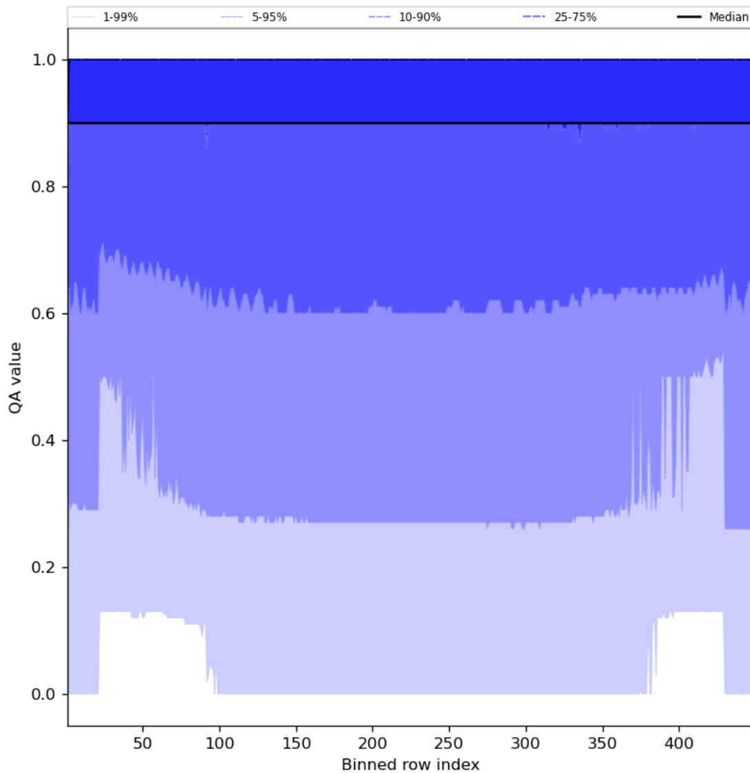
Figure 27: Along track statistics of “QA value” for 2024-07-17 to 2024-07-19
