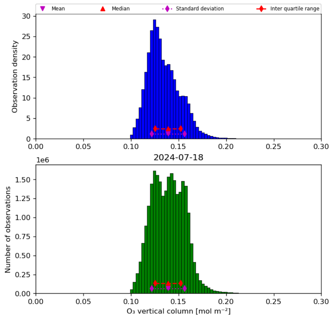
Figure 21: Histogram of “O 3 vertical column” for 2024-07-17 to 2024-07-19
