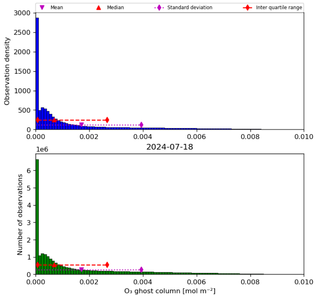
Figure 25: Histogram of “O 3 ghost column” for 2024-07-17 to 2024-07-19
