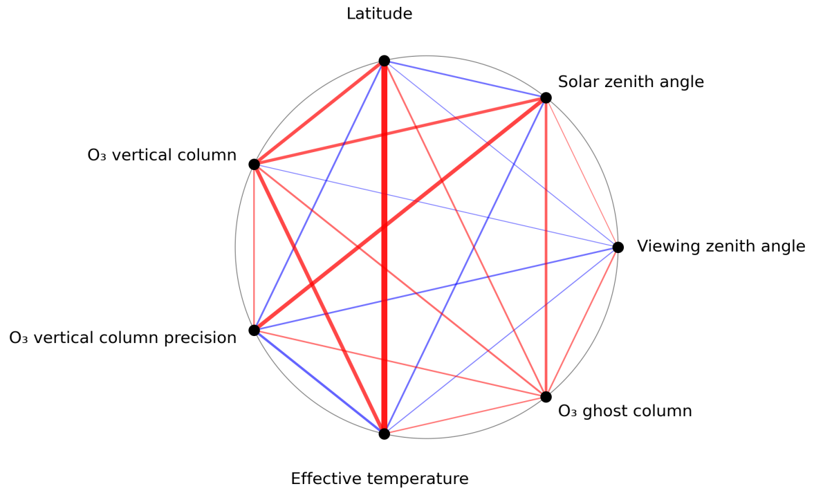
Figure 1: Map of correlation graph for 2024-07-17 to 2024-07-19.
