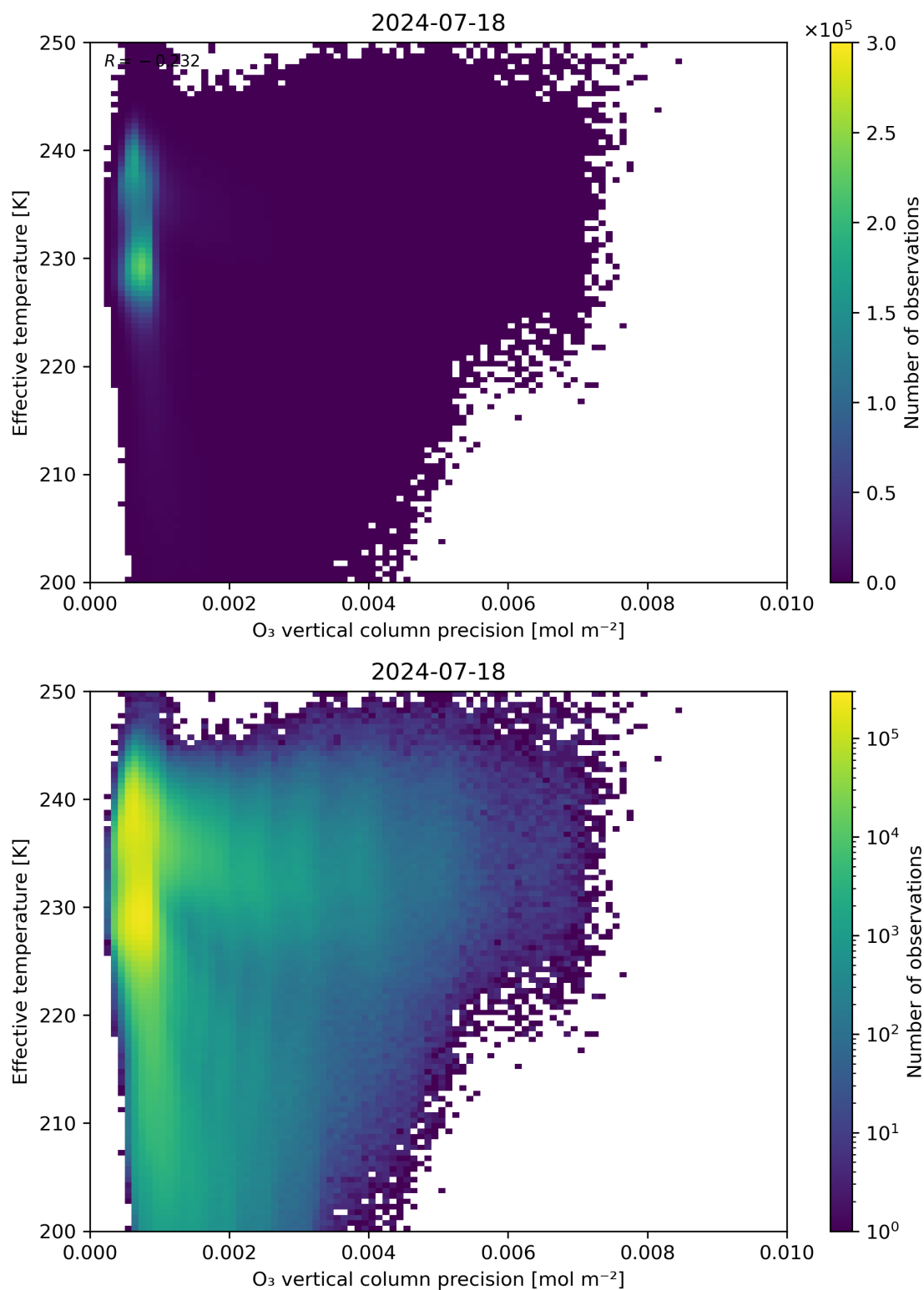
Figure 42: Scatter density plot of “O 3 vertical column precision” against “Effective temperature” for 2024-07-17 to 2024-07-19.
