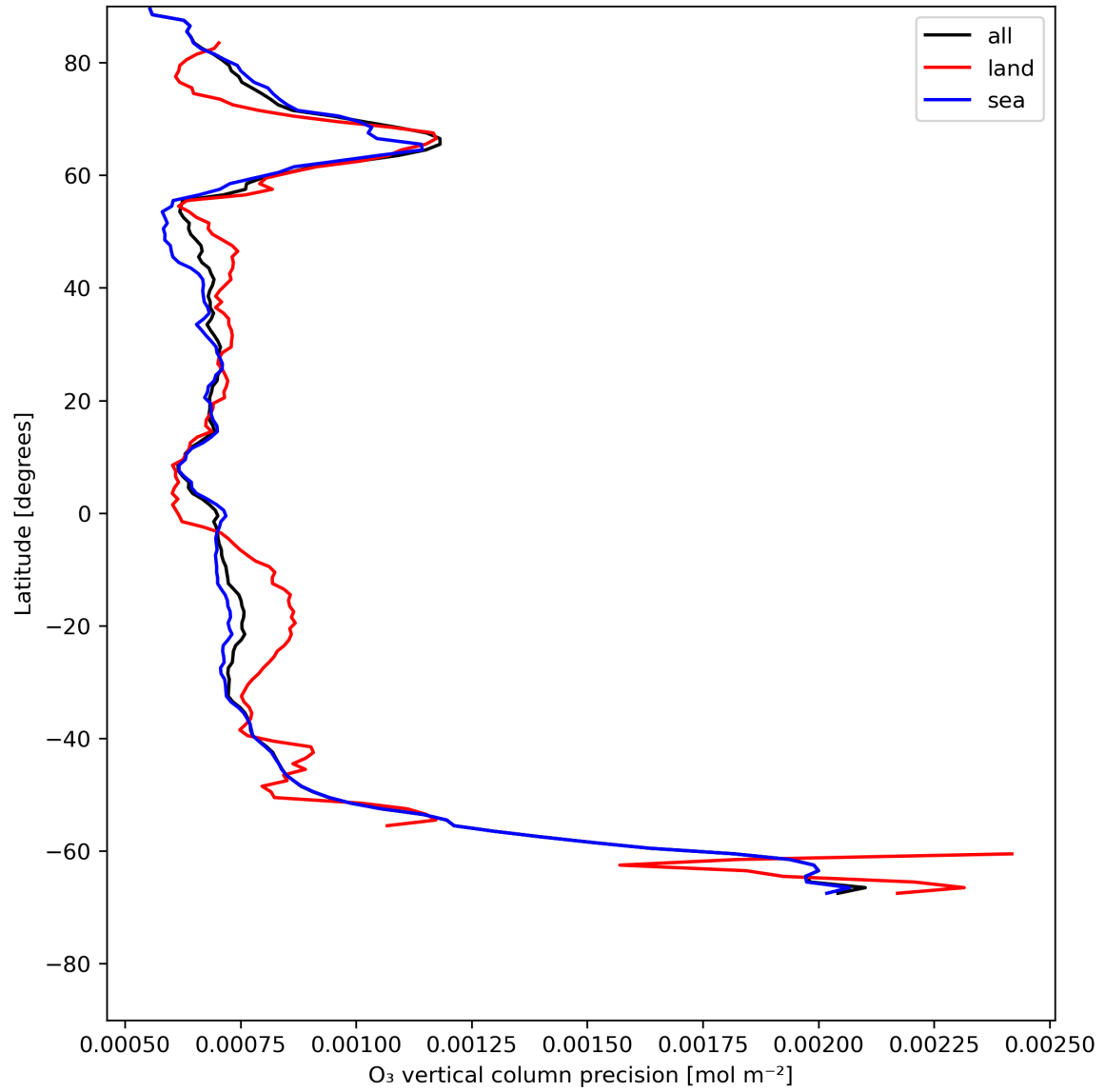
Figure 15: Zonal average of “O 3 vertical column precision” for 2024-07-17 to 2024-07-19.
