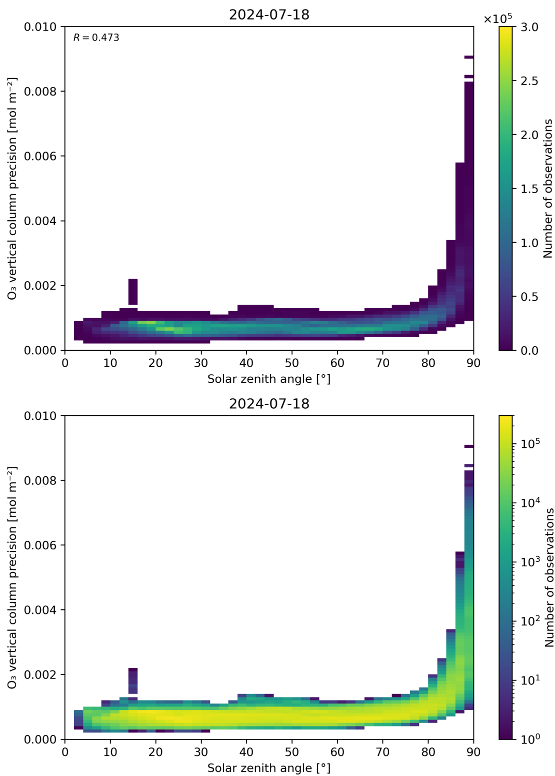
Figure 48: Scatter density plot of “Solar zenith angle” against “O 3 vertical column precision” for 2024-07-17 to 2024-07-19.
