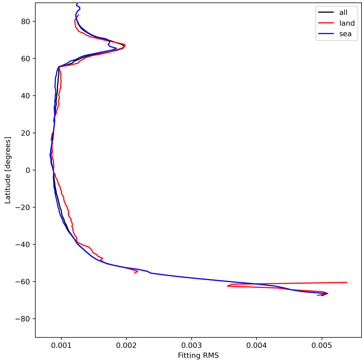
Figure 16: Zonal average of “Fitting RMS” for 2024-07-17 to 2024-07-19.
