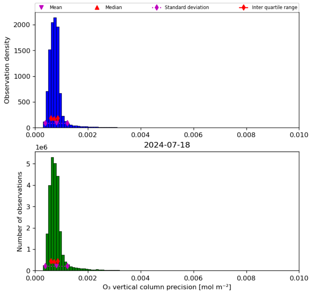
Figure 22: Histogram of “O 3 vertical column precision” for 2024-07-17 to 2024-07-19
