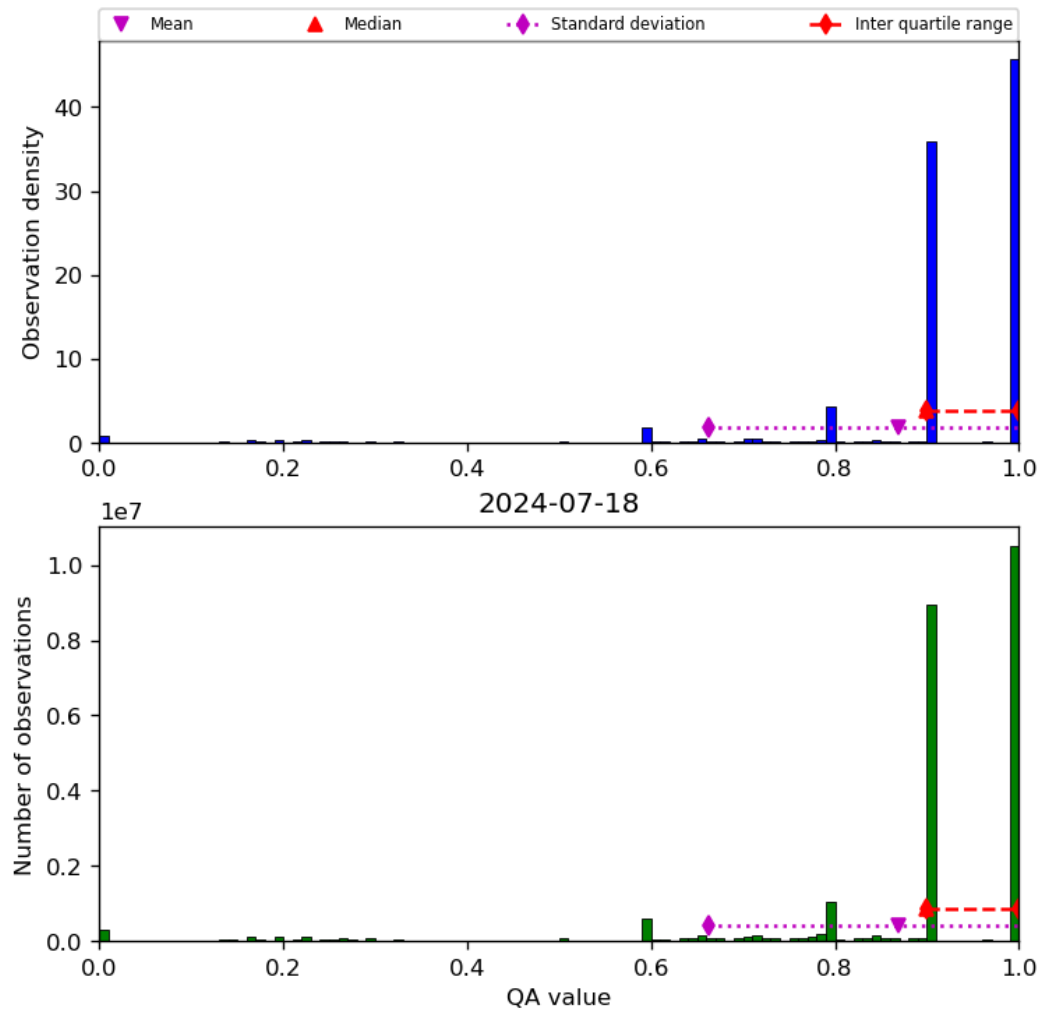
Figure 20: Histogram of “QA value” for 2024-07-17 to 2024-07-19
