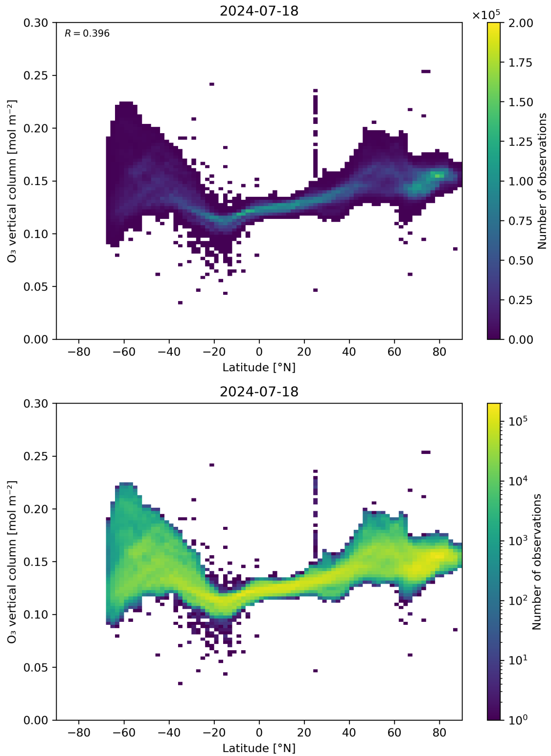
Figure 36: Scatter density plot of “Latitude” against “O 3 vertical column” for 2024-07-17 to 2024-07-19.
