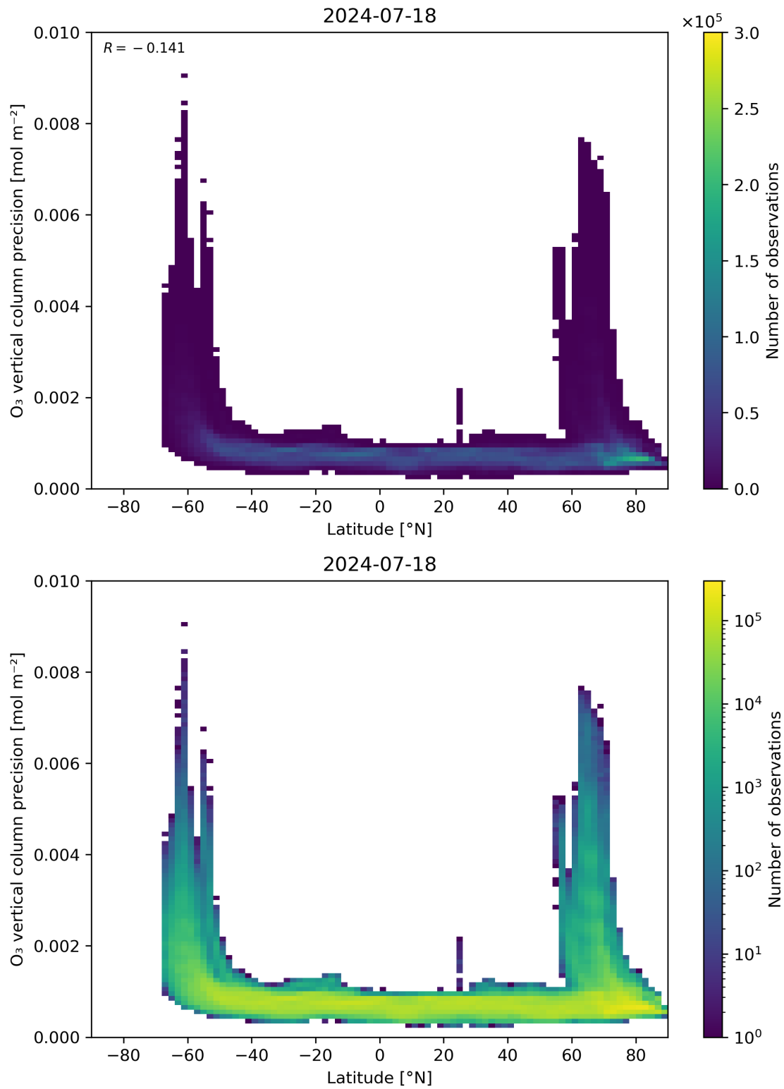
Figure 37: Scatter density plot of “Latitude” against “O 3 vertical column precision” for 2024-07-17 to 2024-07-19.
