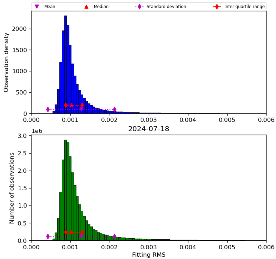
Figure 23: Histogram of “Fitting RMS” for 2024-07-17 to 2024-07-19
