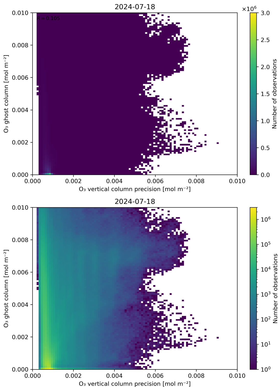
Figure 43: Scatter density plot of “ \text{O}_3 vertical column precision” against “ \text{O}_3 ghost column” for 2024-07-17 to 2024-07-19.
