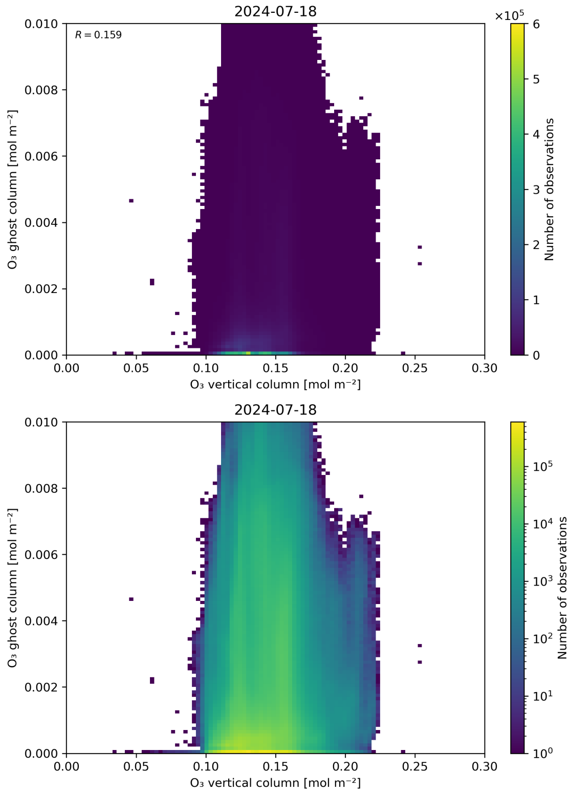
Figure 40: Scatter density plot of “O 3 vertical column” against “O 3 ghost column” for 2024-07-17 to 2024-07-19.
