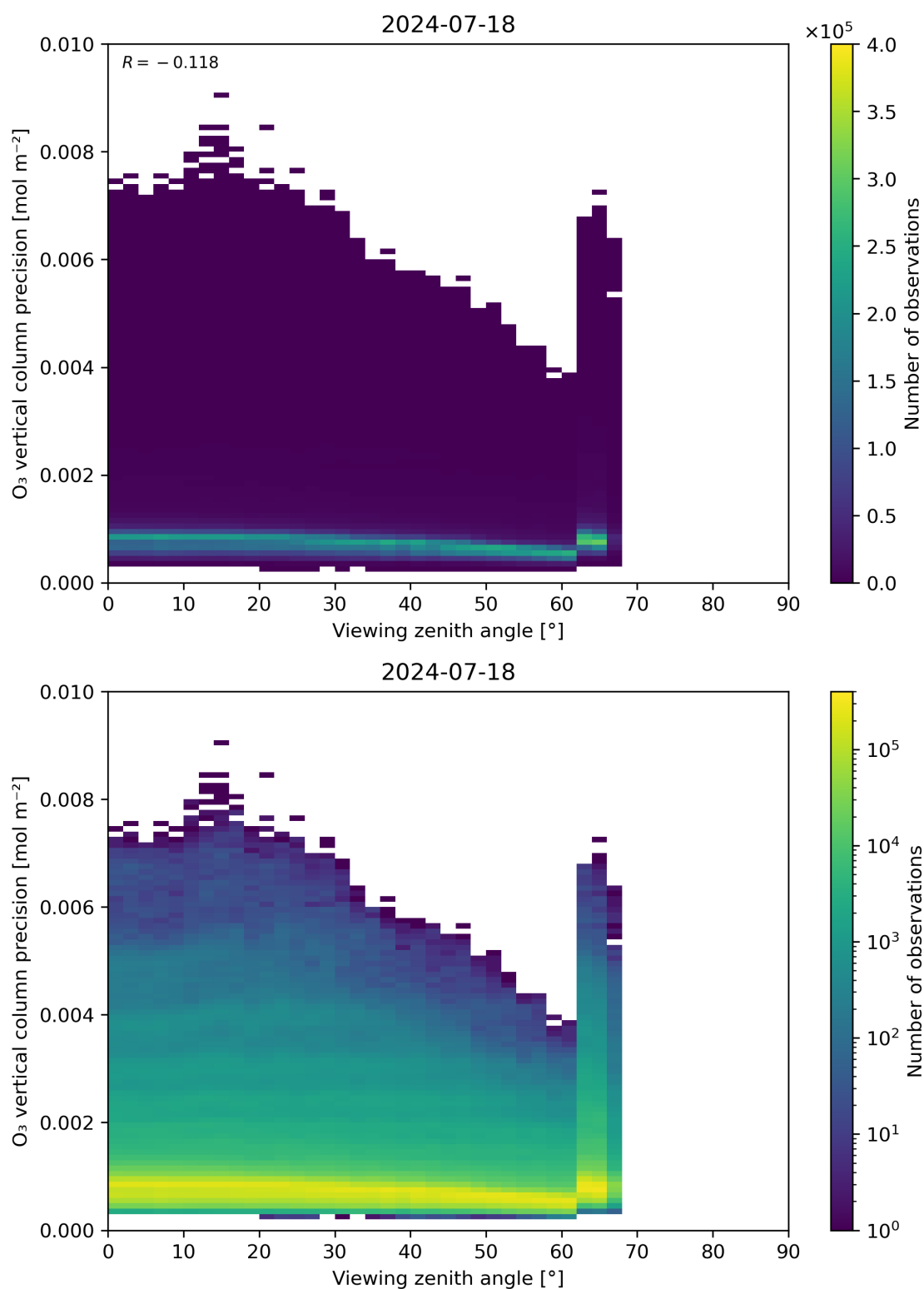
Figure 53: Scatter density plot of “Viewing zenith angle” against “O 3 vertical column precision” for 2024-07-17 to 2024-07-19.
