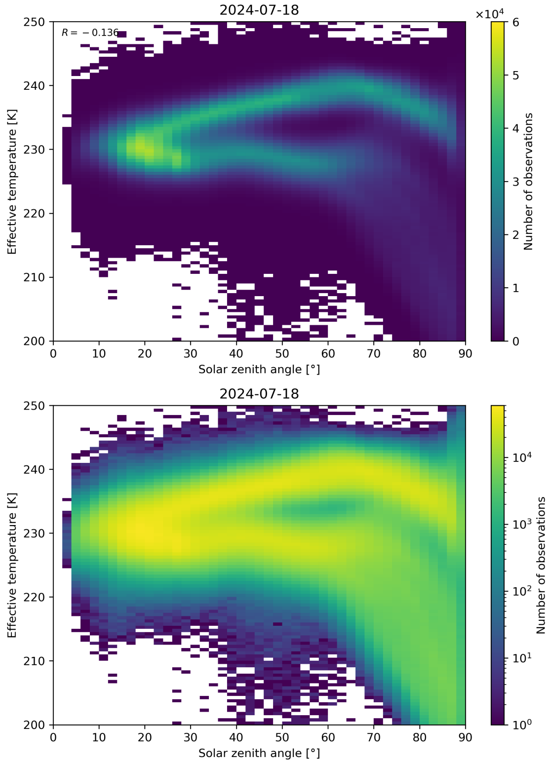
Figure 45: Scatter density plot of “Solar zenith angle” against “Effective temperature” for 2024-07-17 to 2024-07-19.
