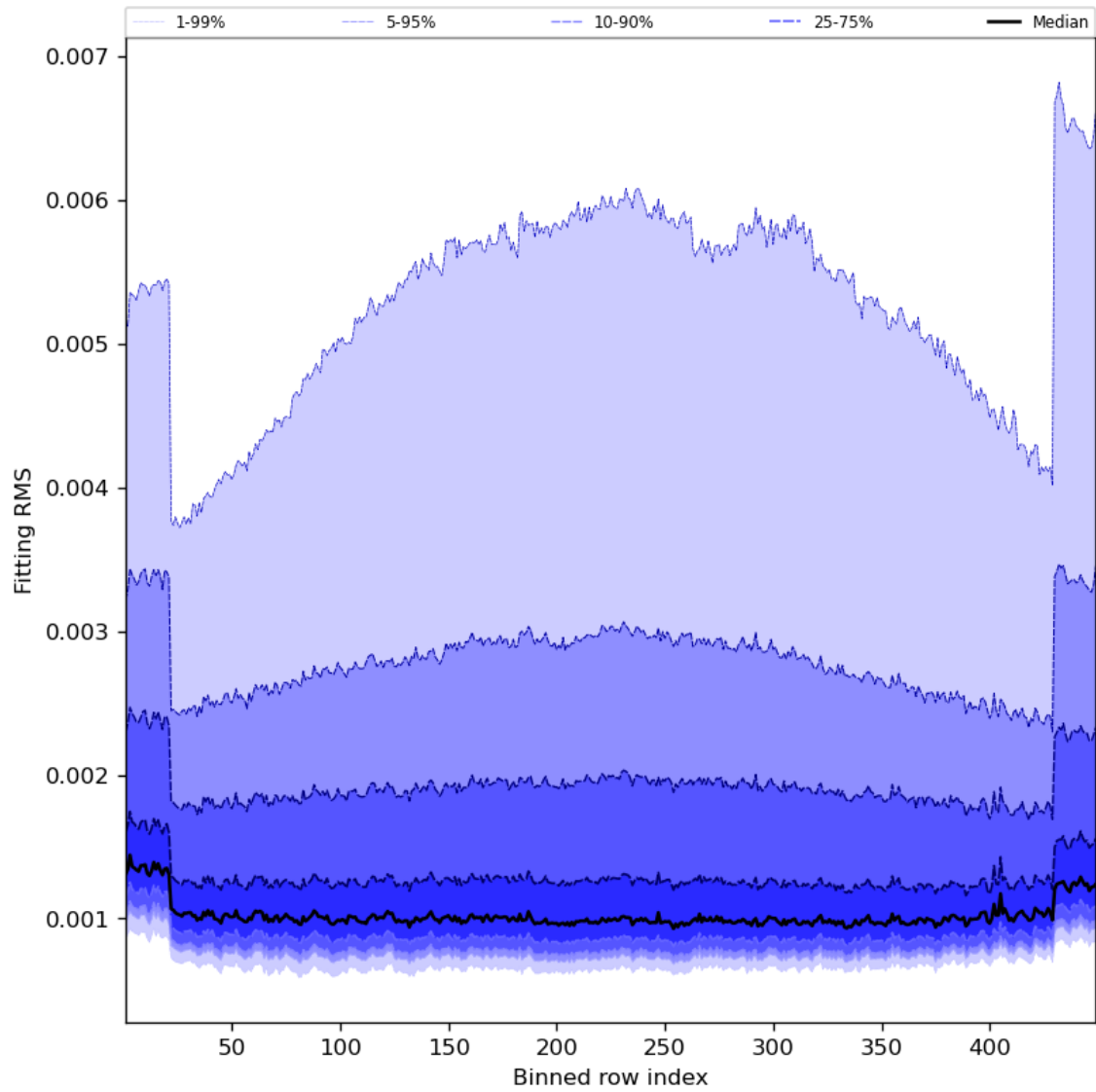
Figure 30: Along track statistics of “Fitting RMS” for 2024-07-17 to 2024-07-19
