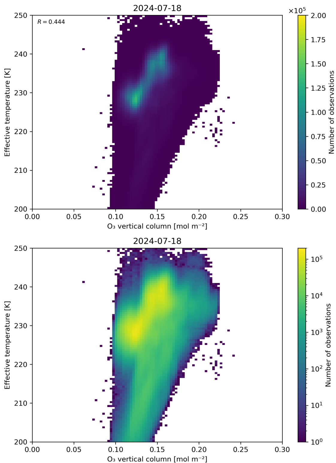
Figure 39: Scatter density plot of “O 3 vertical column” against “Effective temperature” for 2024-07-17 to 2024-07-19.
