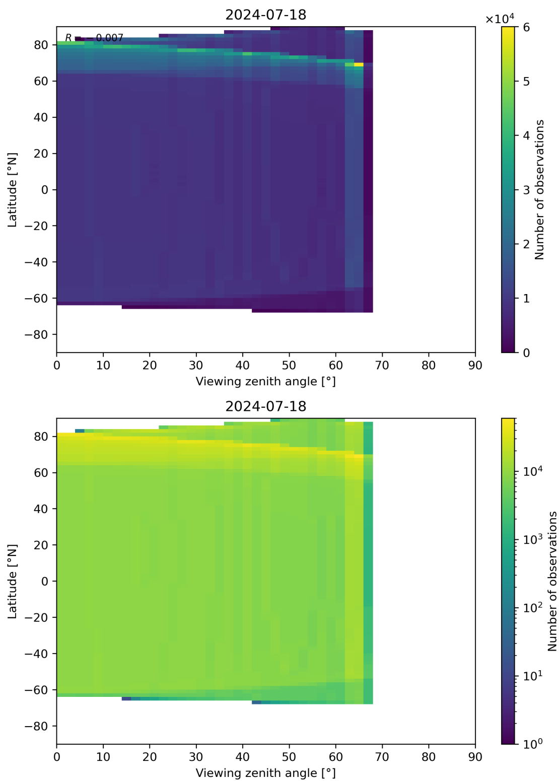
Figure 49: Scatter density plot of “Viewing zenith angle” against “Latitude” for 2024-07-17 to 2024-07-19.
