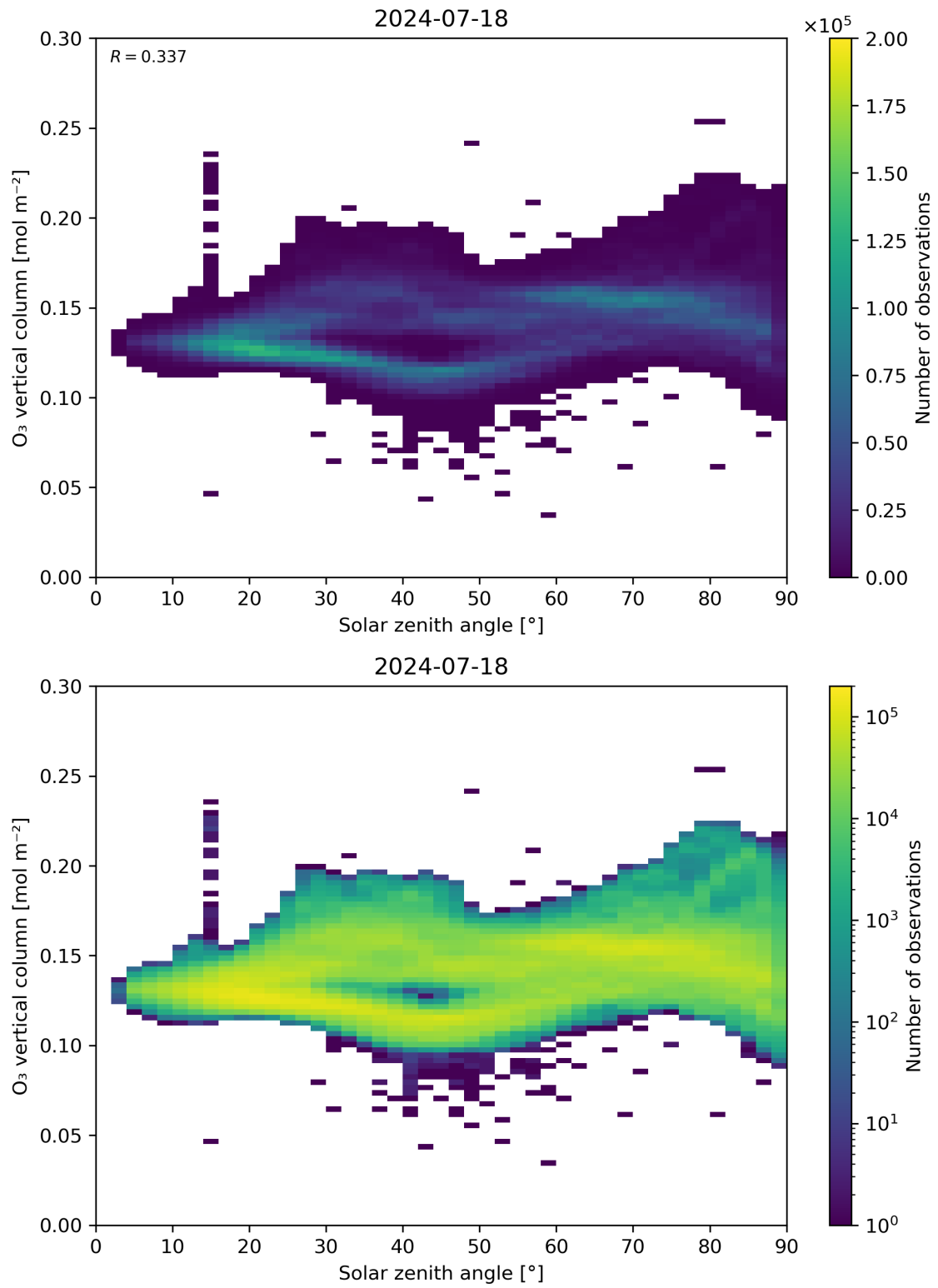
Figure 47: Scatter density plot of “Solar zenith angle” against “O 3 vertical column” for 2024-07-17 to 2024-07-19.
