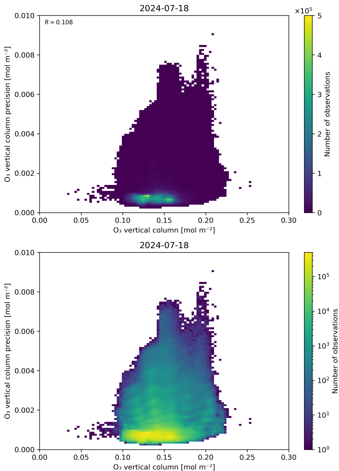
Figure 41: Scatter density plot of “O 3 vertical column” against “O 3 vertical column precision” for 2024-07-17 to 2024-07-19.
