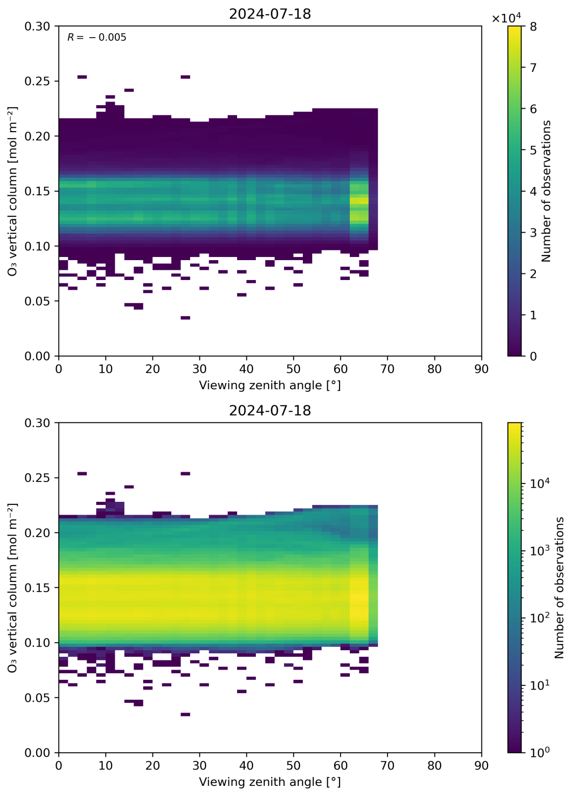
Figure 52: Scatter density plot of “Viewing zenith angle” against “O 3 vertical column” for 2024-07-17 to 2024-07-19.
