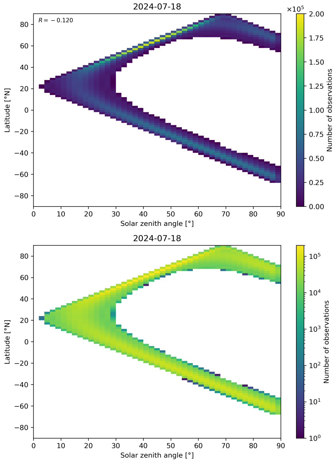
Figure 44: Scatter density plot of “Solar zenith angle” against “Latitude” for 2024-07-17 to 2024-07-19.
