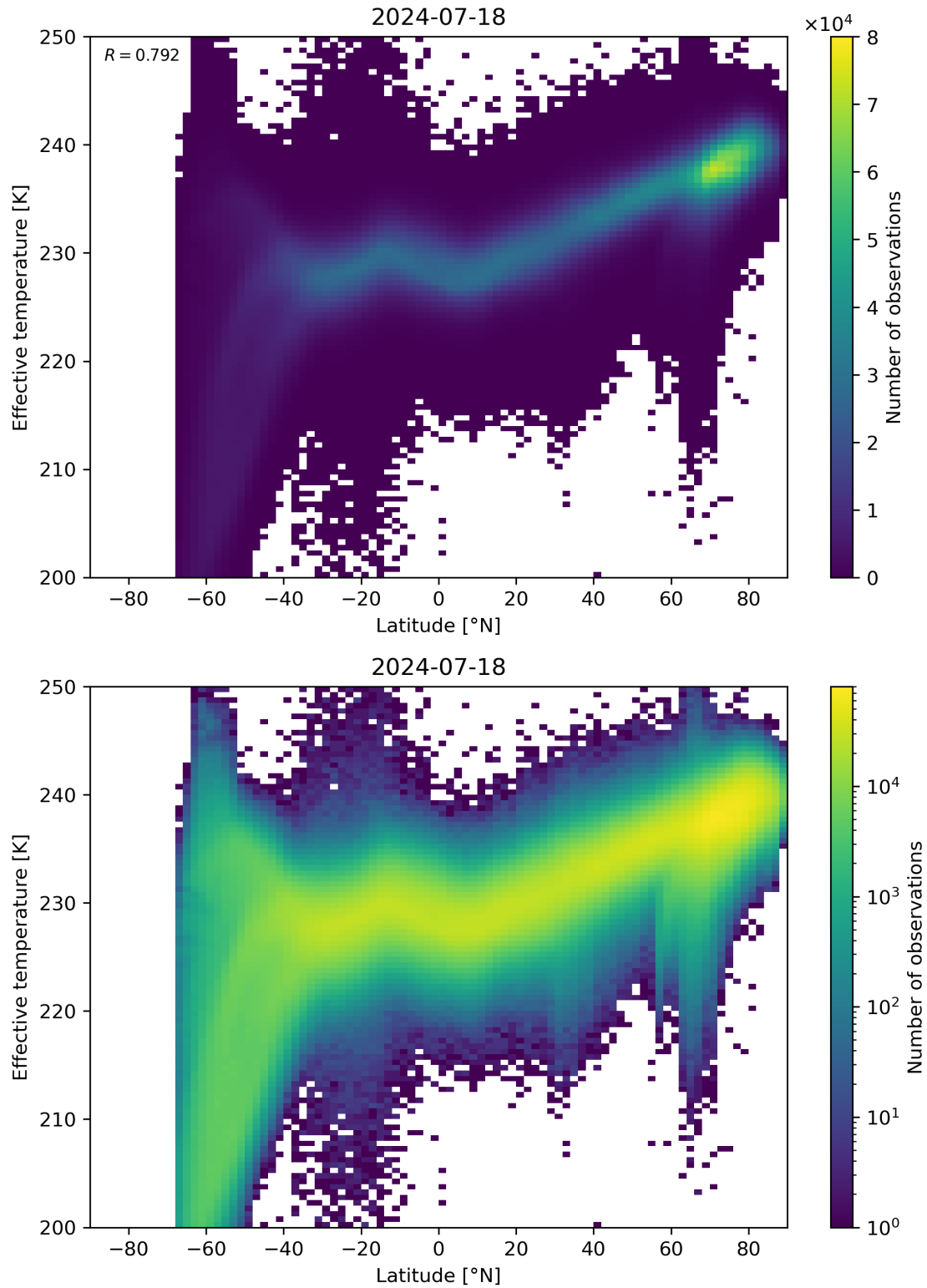
Figure 34: Scatter density plot of “Latitude” against “Effective temperature” for 2024-07-17 to 2024-07-19.
