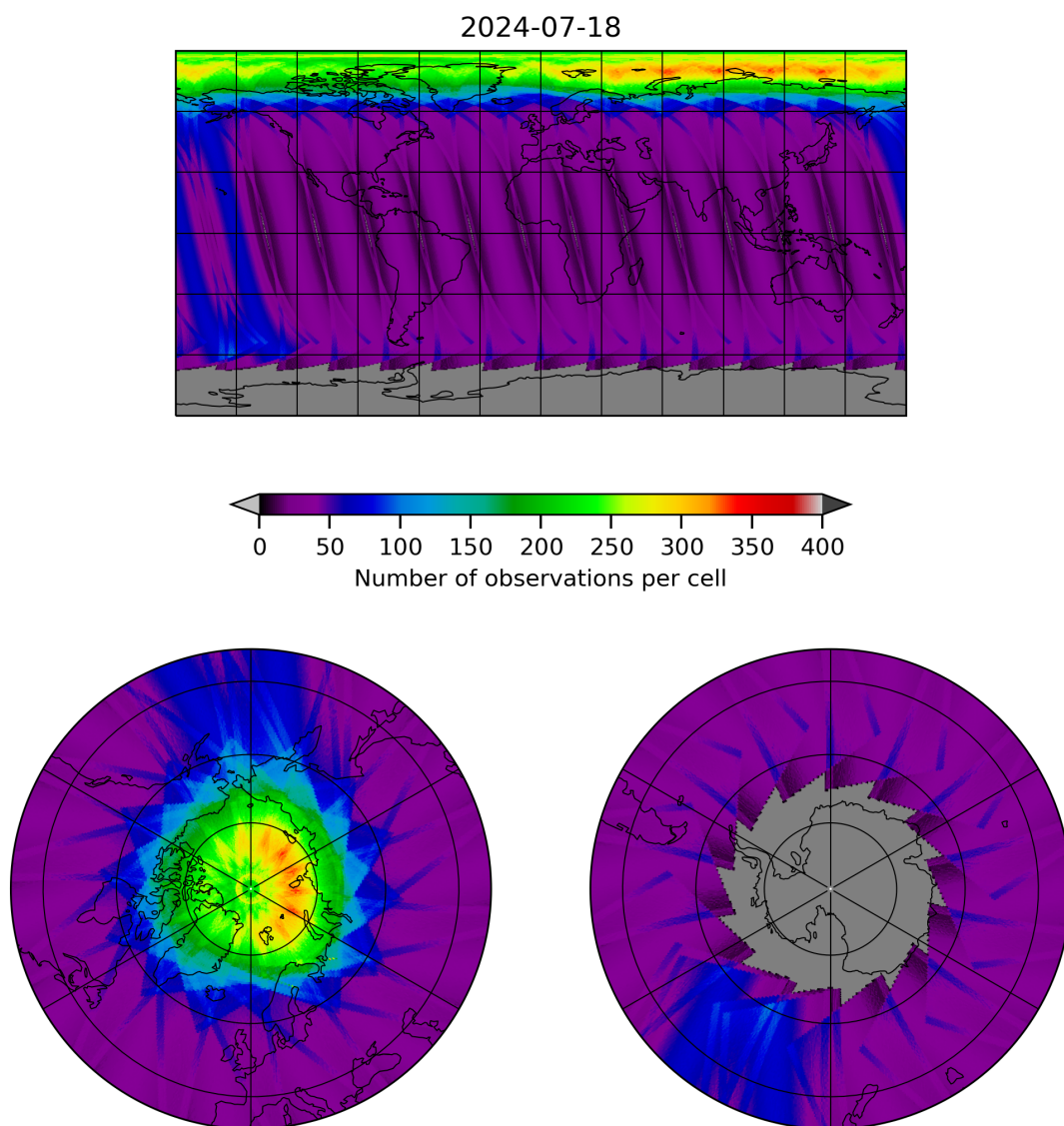
Figure 12: Map of the number of observations for 2024-07-17 to 2024-07-19
