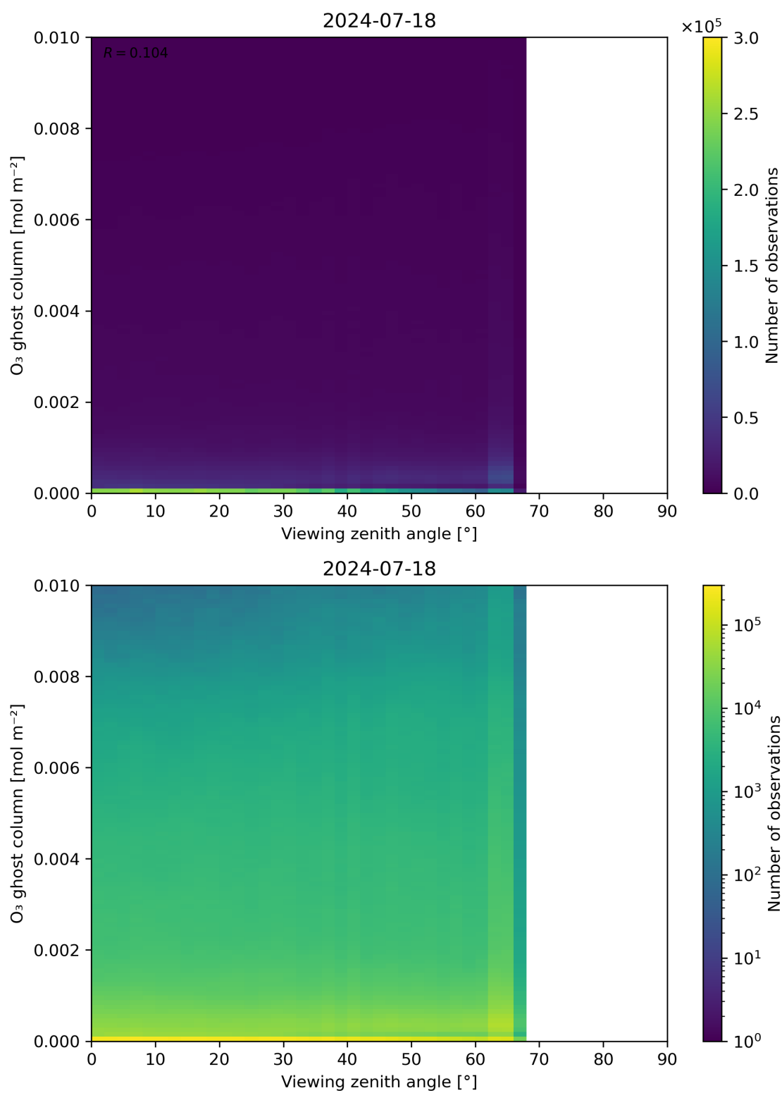
Figure 51: Scatter density plot of “Viewing zenith angle” against “O 3 ghost column” for 2024-07-17 to 2024-07-19.
