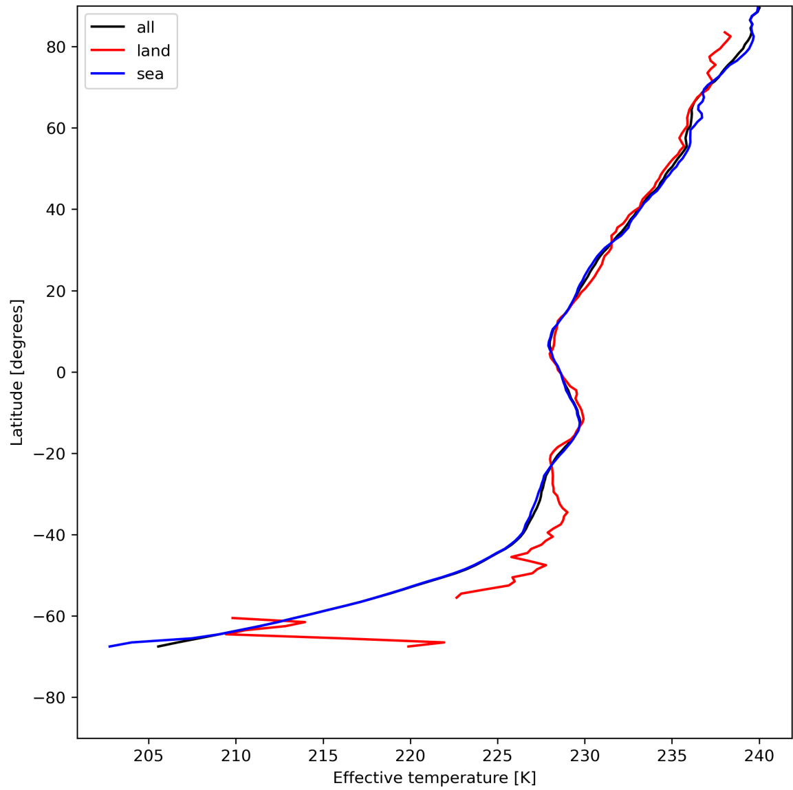
Figure 17: Zonal average of "Effective temperature" for 2024-07-17 to 2024-07-19.
