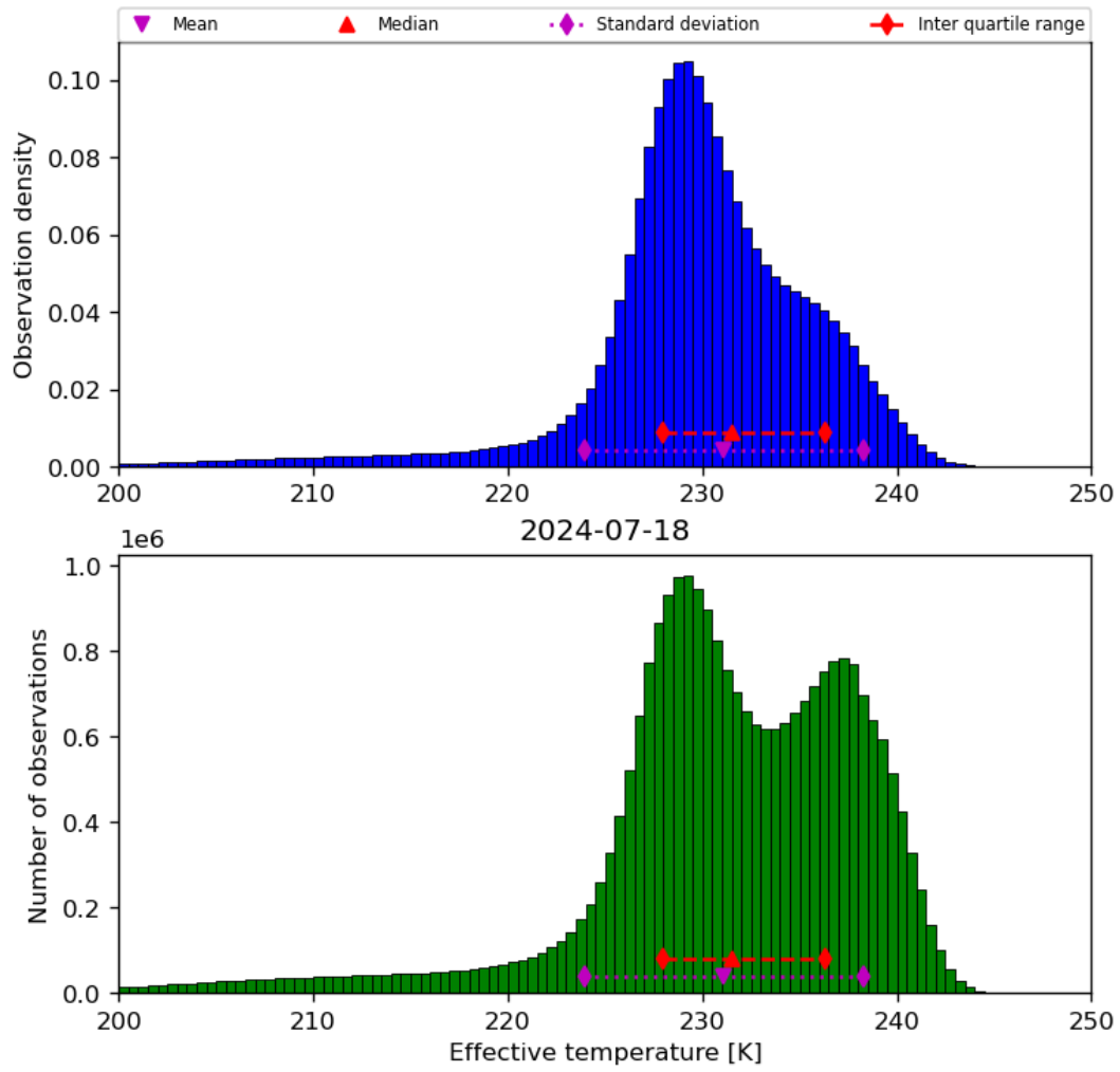
Figure 24: Histogram of “Effective temperature” for 2024-07-17 to 2024-07-19
