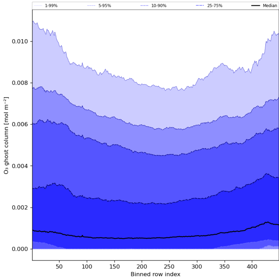
Figure 32: Along track statistics of “O 3 ghost column” for 2024-07-17 to 2024-07-19
