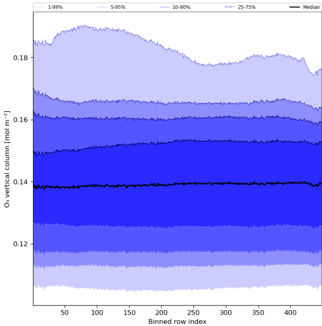
Figure 28: Along track statistics of “O 3 vertical column” for 2024-07-17 to 2024-07-19
