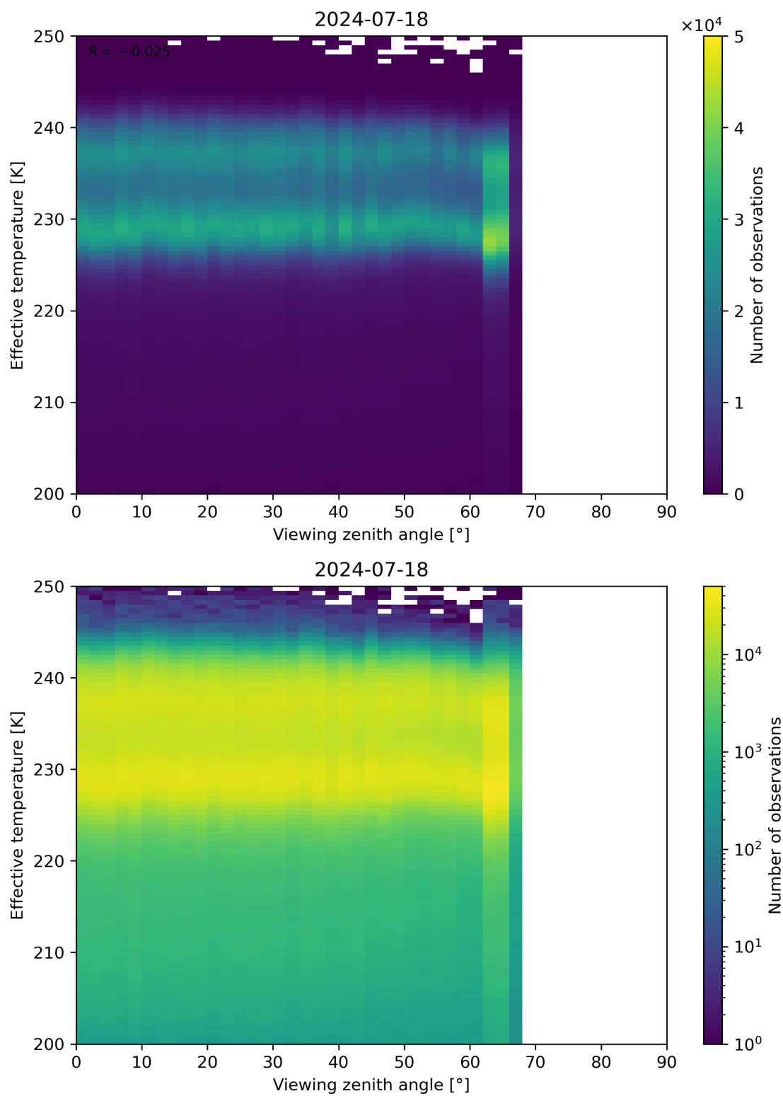
Figure 50: Scatter density plot of “Viewing zenith angle” against “Effective temperature” for 2024-07-17 to 2024-07-19.
