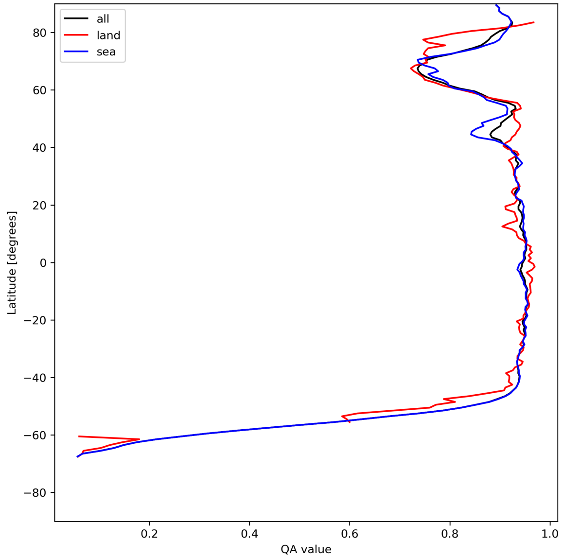
Figure 13: Zonal average of “QA value” for 2024-07-17 to 2024-07-19.
