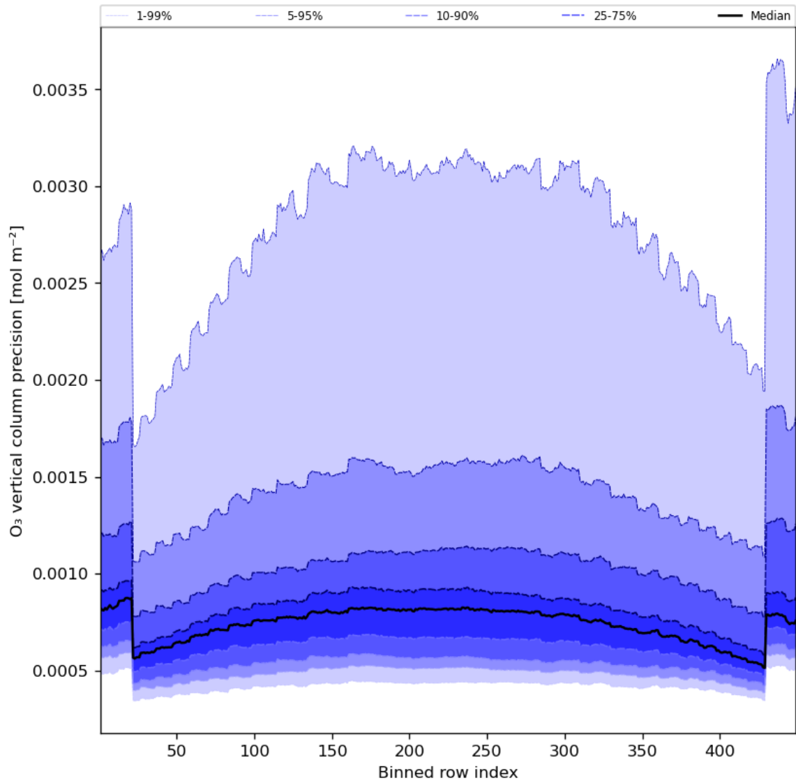
Figure 29: Along track statistics of “O 3 vertical column precision” for 2024-07-17 to 2024-07-19
