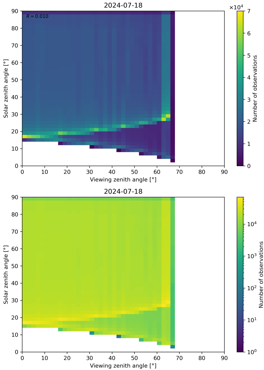
Figure 54: Scatter density plot of “Viewing zenith angle” against “Solar zenith angle” for 2024-07-17 to 2024-07-19.
