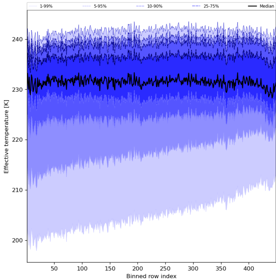
Figure 31: Along track statistics of “Effective temperature” for 2024-07-17 to 2024-07-19
