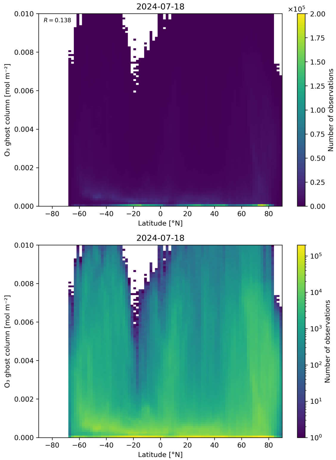
Figure 35: Scatter density plot of “Latitude” against “O 3 ghost column” for 2024-07-17 to 2024-07-19.
