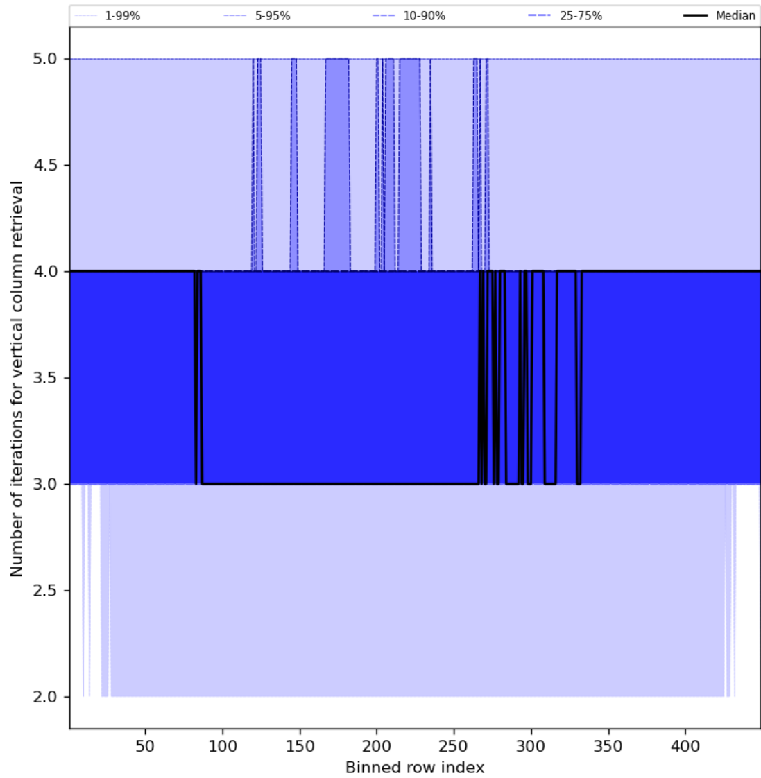
Figure 33: Along track statistics of “Number of iterations for vertical column retrieval” for 2024-07-17 to 2024-07-19
