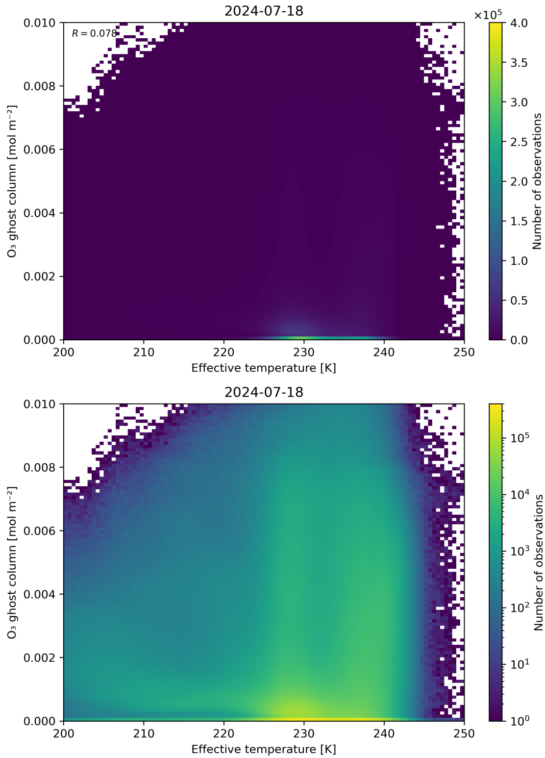
Figure 38: Scatter density plot of “Effective temperature” against “O 3 ghost column” for 2024-07-17 to 2024-07-19.
