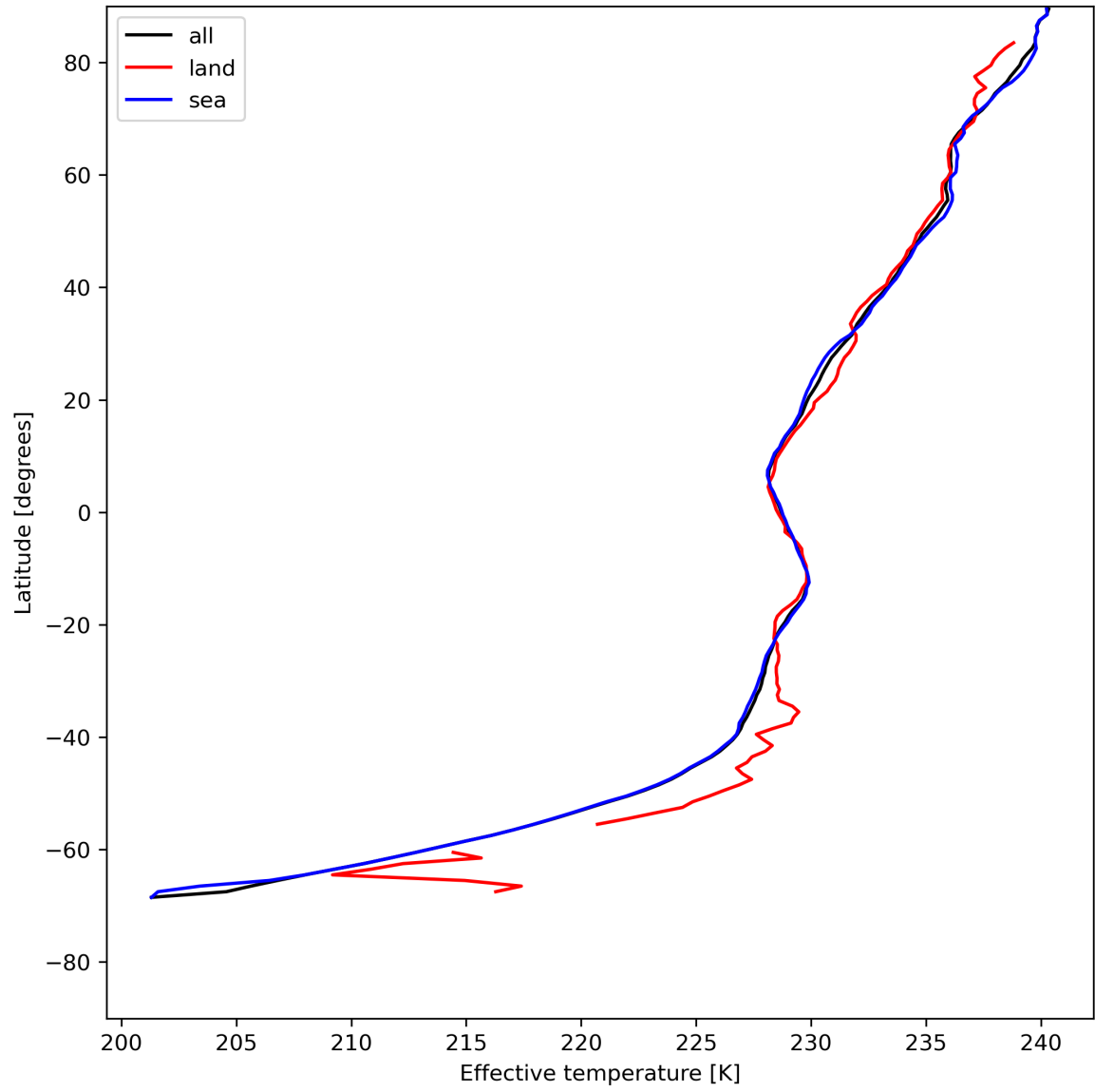
Figure 17: Zonal average of "Effective temperature" for 2024-07-18 to 2024-07-20.
