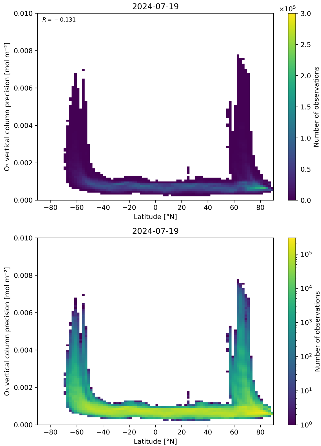
Figure 37: Scatter density plot of “Latitude” against “O 3 vertical column precision” for 2024-07-18 to 2024-07-20.
