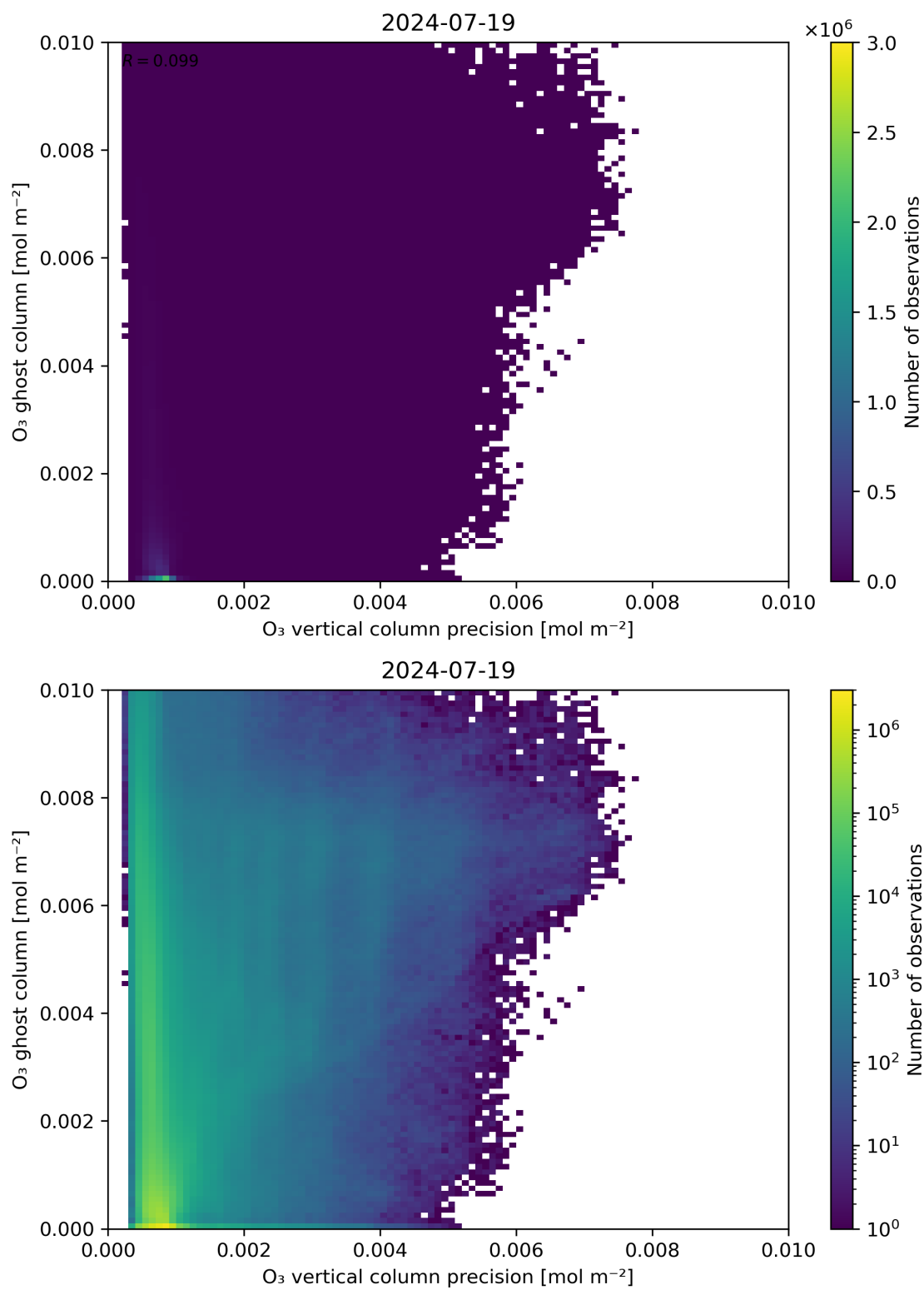
Figure 43: Scatter density plot of “ \text{O}_3 vertical column precision” against “ \text{O}_3 ghost column” for 2024-07-18 to 2024-07-20.
