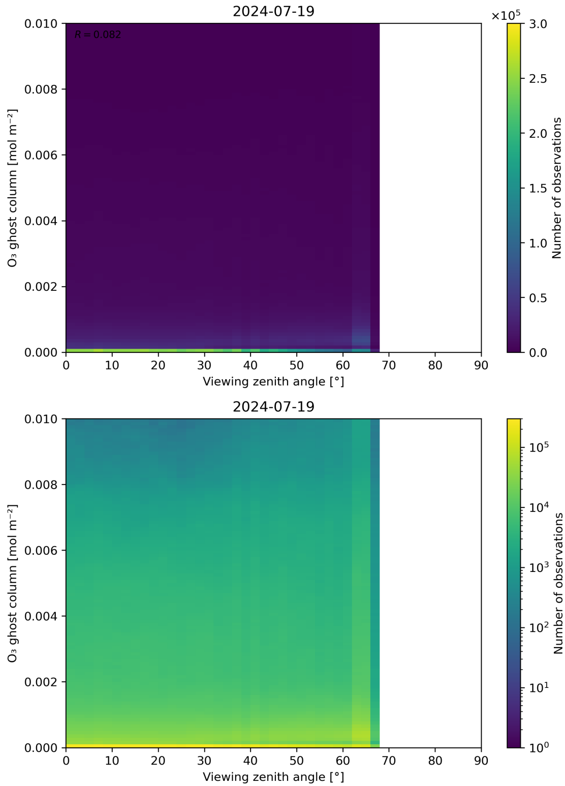
Figure 51: Scatter density plot of “Viewing zenith angle” against “O 3 ghost column” for 2024-07-18 to 2024-07-20.
