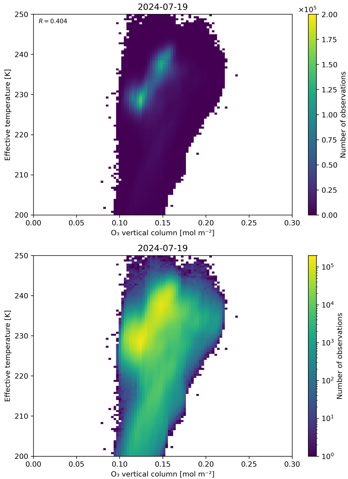
Figure 39: Scatter density plot of “O 3 vertical column” against “Effective temperature” for 2024-07-18 to 2024-07-20.
