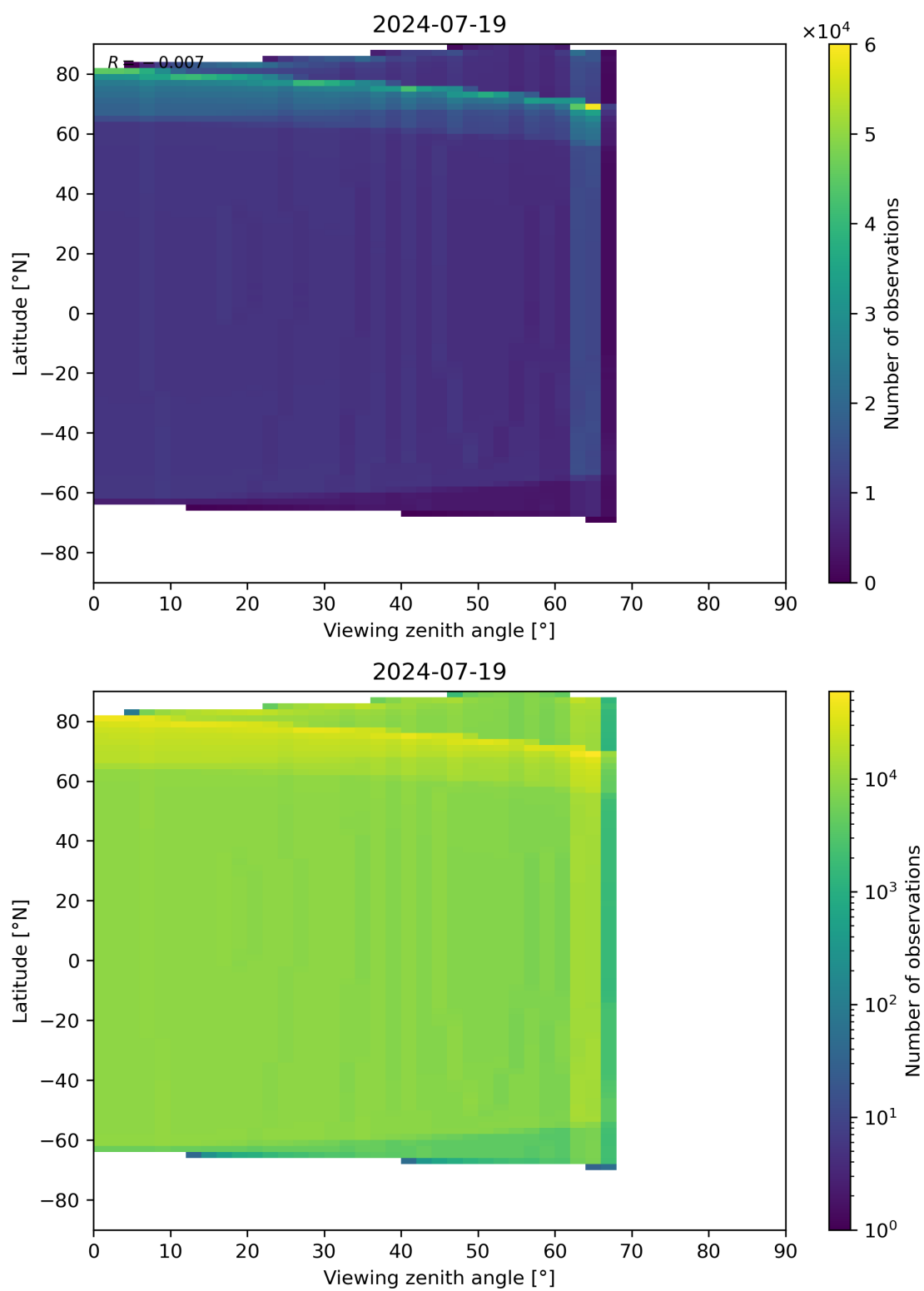
Figure 49: Scatter density plot of “Viewing zenith angle” against “Latitude” for 2024-07-18 to 2024-07-20.
