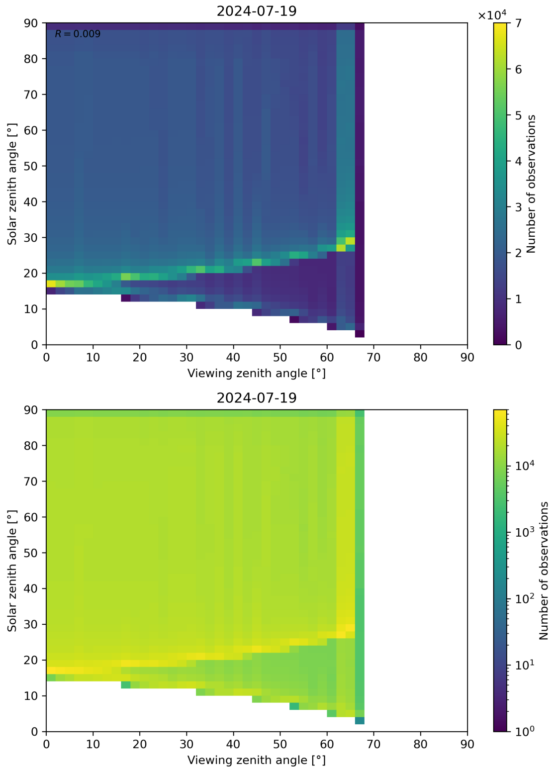
Figure 54: Scatter density plot of “Viewing zenith angle” against “Solar zenith angle” for 2024-07-18 to 2024-07-20.
