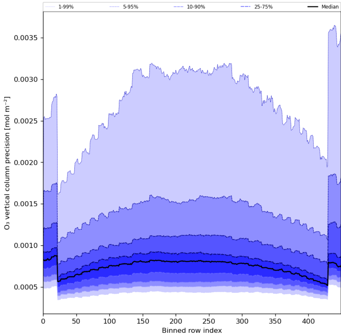
Figure 29: Along track statistics of “O 3 vertical column precision” for 2024-07-18 to 2024-07-20
