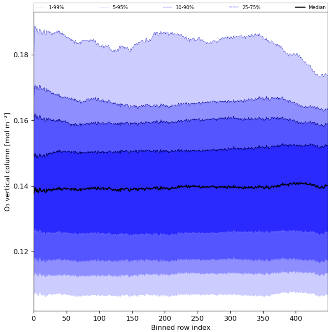
Figure 28: Along track statistics of “O 3 vertical column” for 2024-07-18 to 2024-07-20
