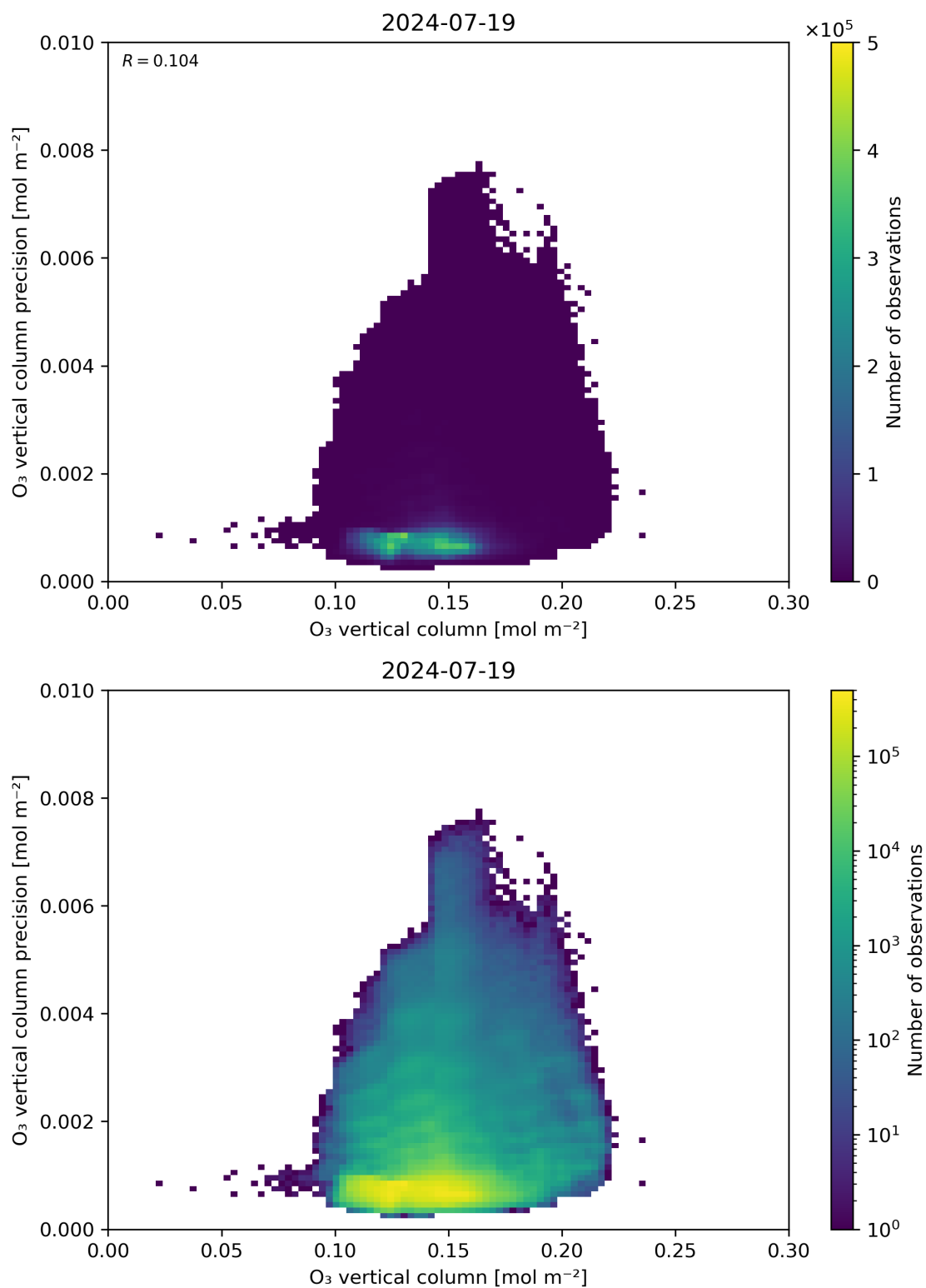
Figure 41: Scatter density plot of “O 3 vertical column” against “O 3 vertical column precision” for 2024-07-18 to 2024-07-20.
