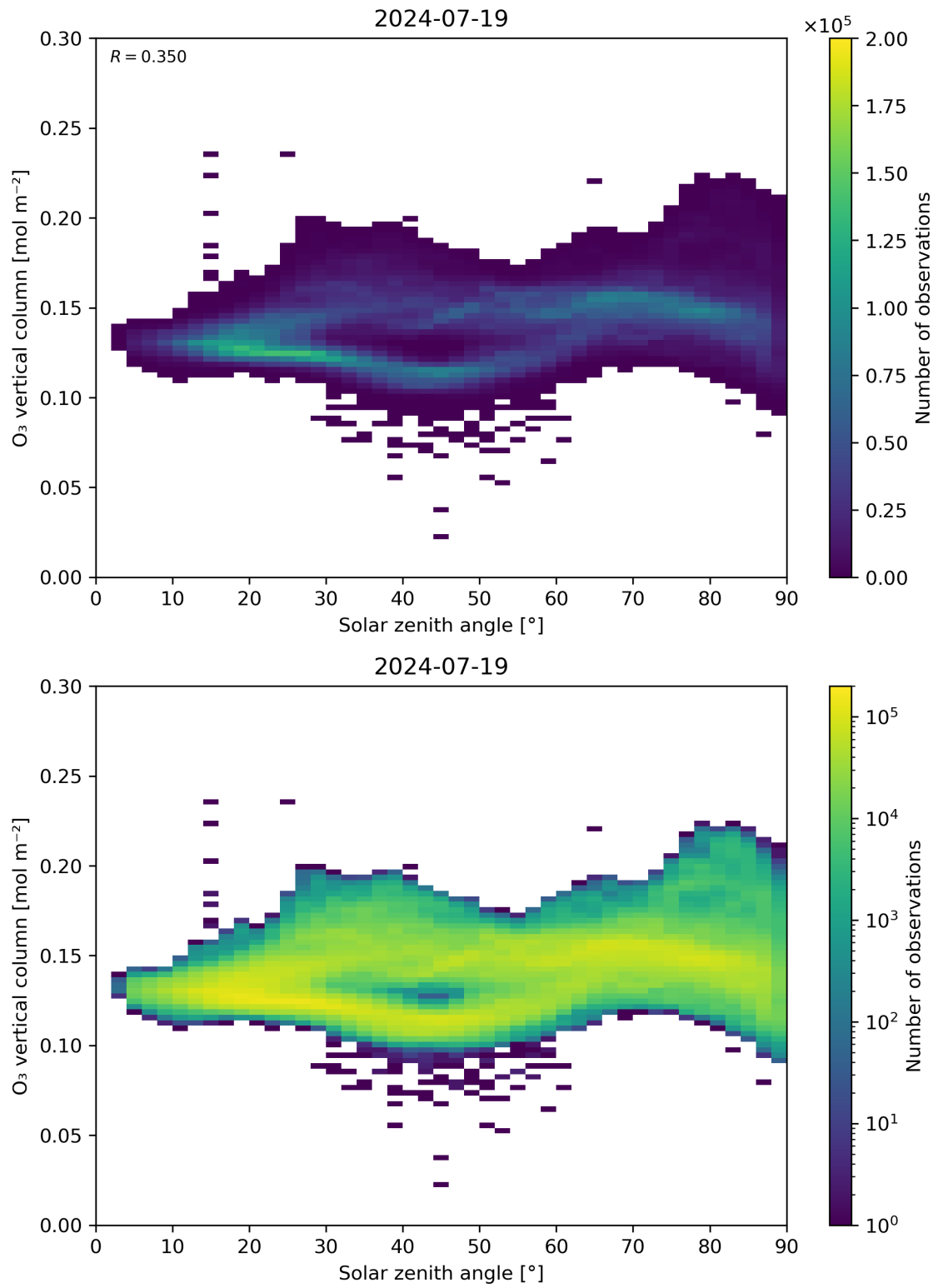
Figure 47: Scatter density plot of “Solar zenith angle” against “O 3 vertical column” for 2024-07-18 to 2024-07-20.
