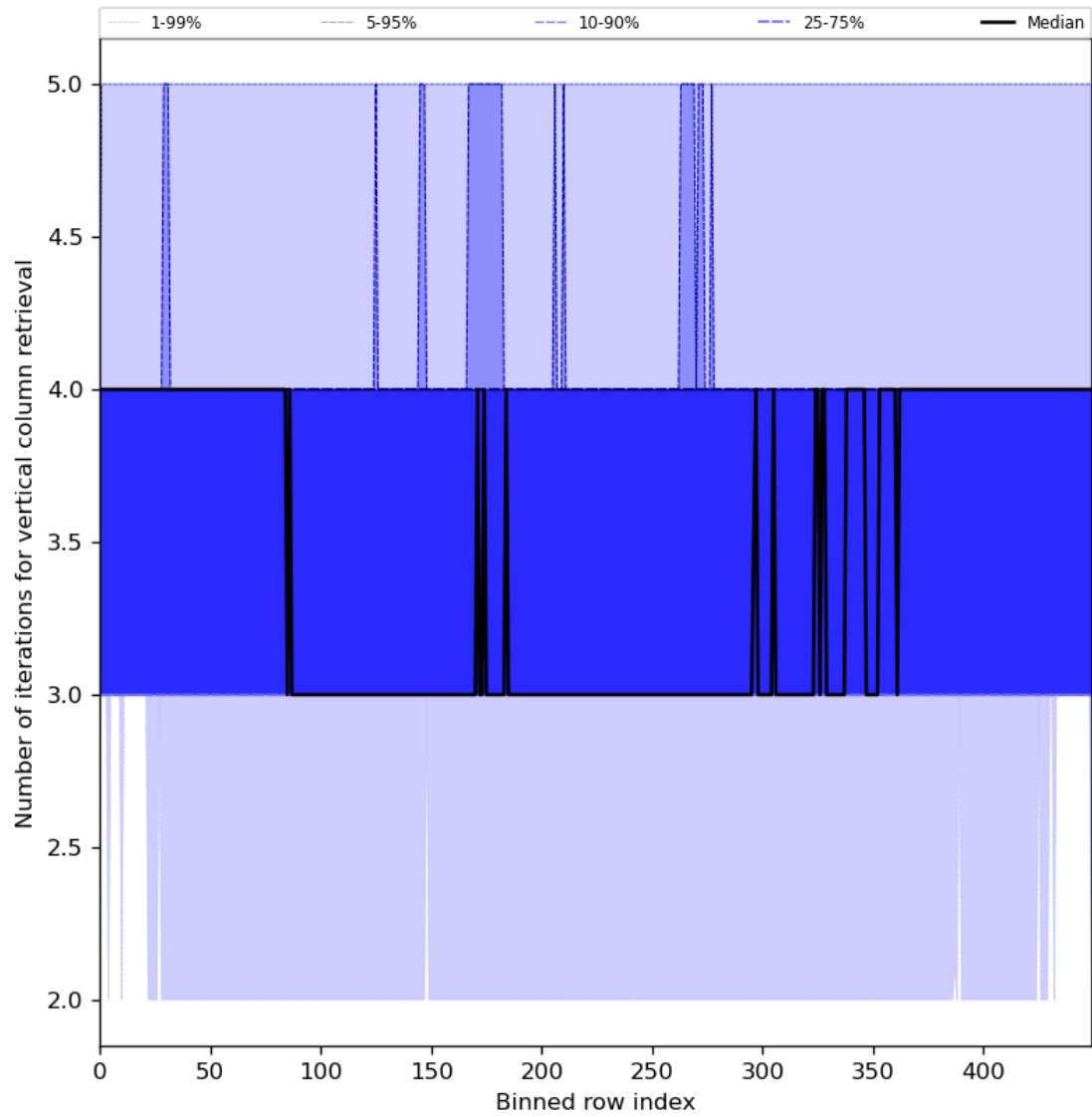
Figure 33: Along track statistics of “Number of iterations for vertical column retrieval” for 2024-07-18 to 2024-07-20
