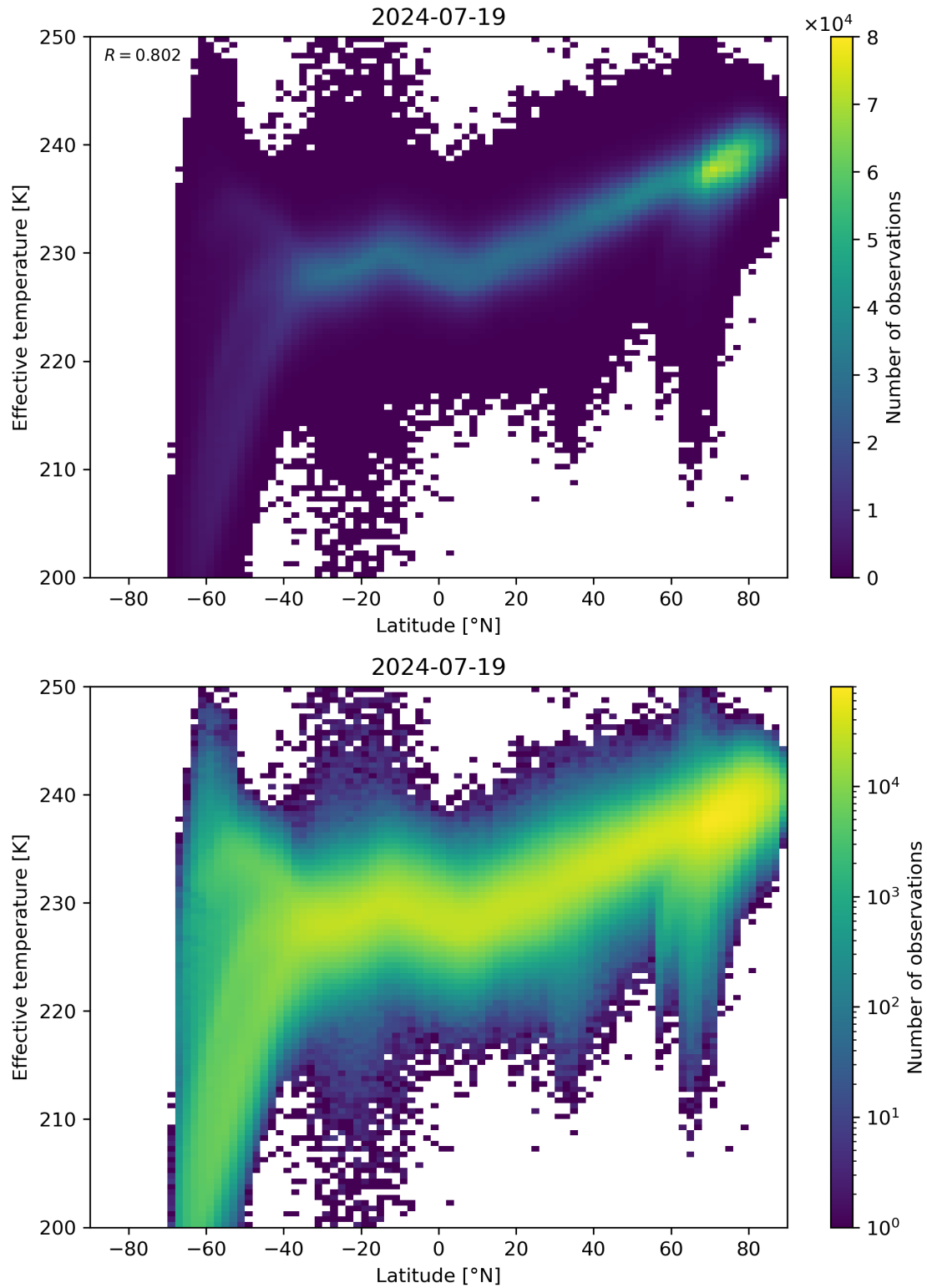
Figure 34: Scatter density plot of “Latitude” against “Effective temperature” for 2024-07-18 to 2024-07-20.
