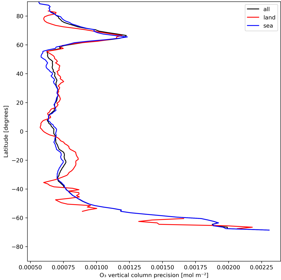
Figure 15: Zonal average of "O 3 vertical column precision" for 2024-07-18 to 2024-07-20.
