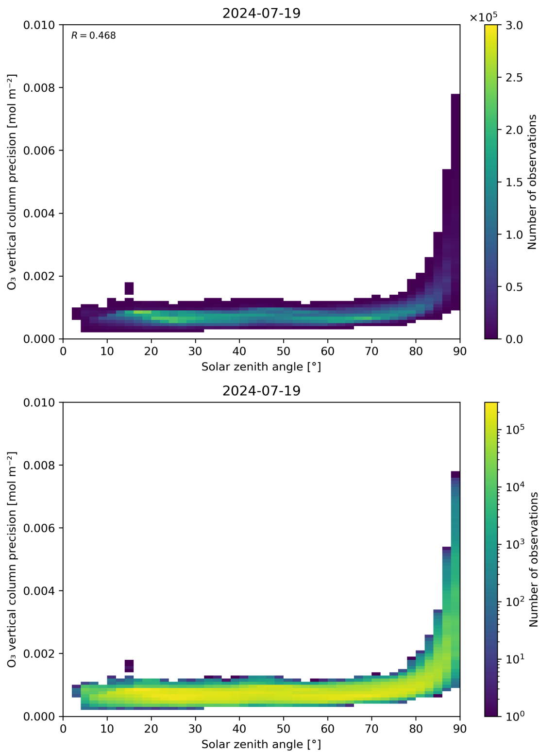
Figure 48: Scatter density plot of “Solar zenith angle” against “O 3 vertical column precision” for 2024-07-18 to 2024-07-20.
