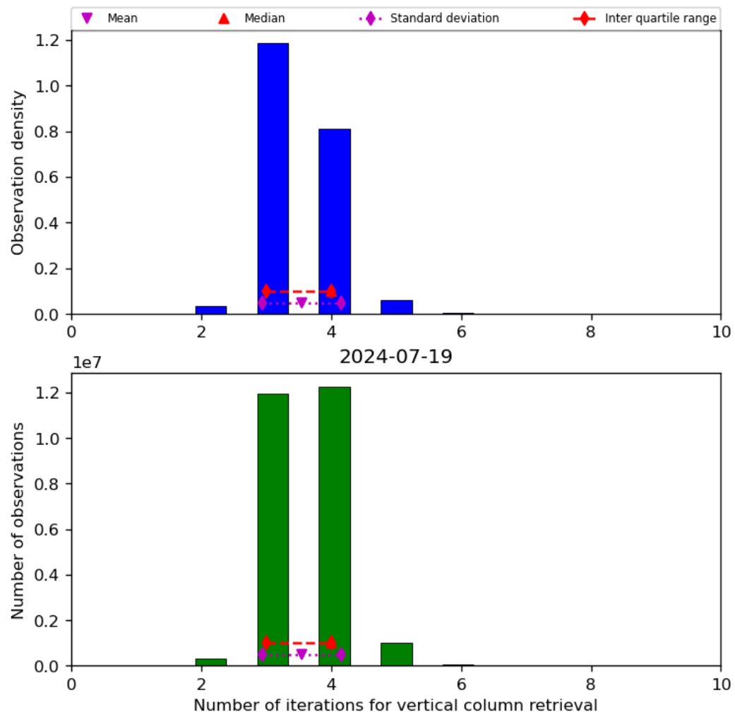
Figure 26: Histogram of “Number of iterations for vertical column retrieval” for 2024-07-18 to 2024-07-20
