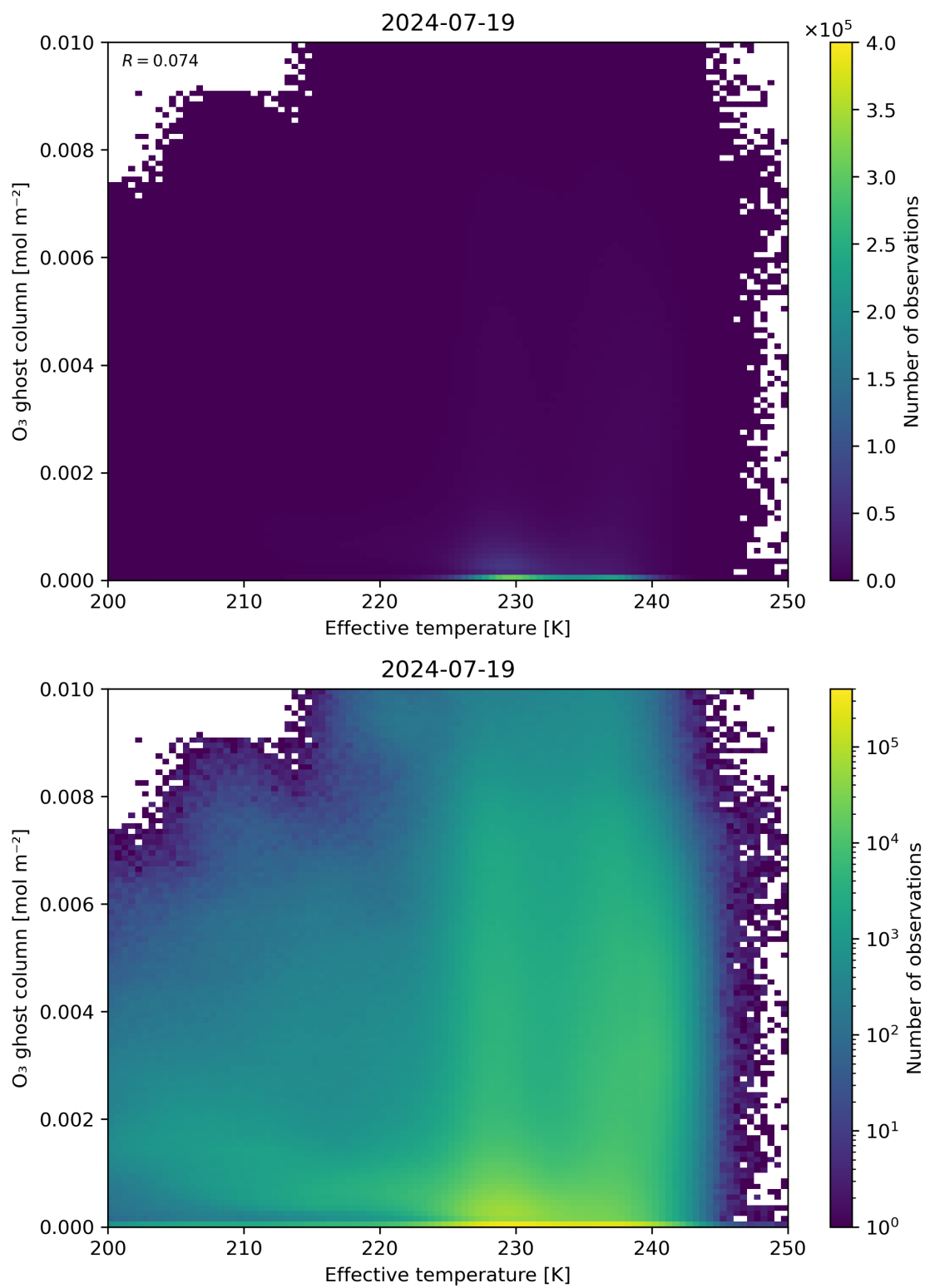
Figure 38: Scatter density plot of “Effective temperature” against “O 3 ghost column” for 2024-07-18 to 2024-07-20.
