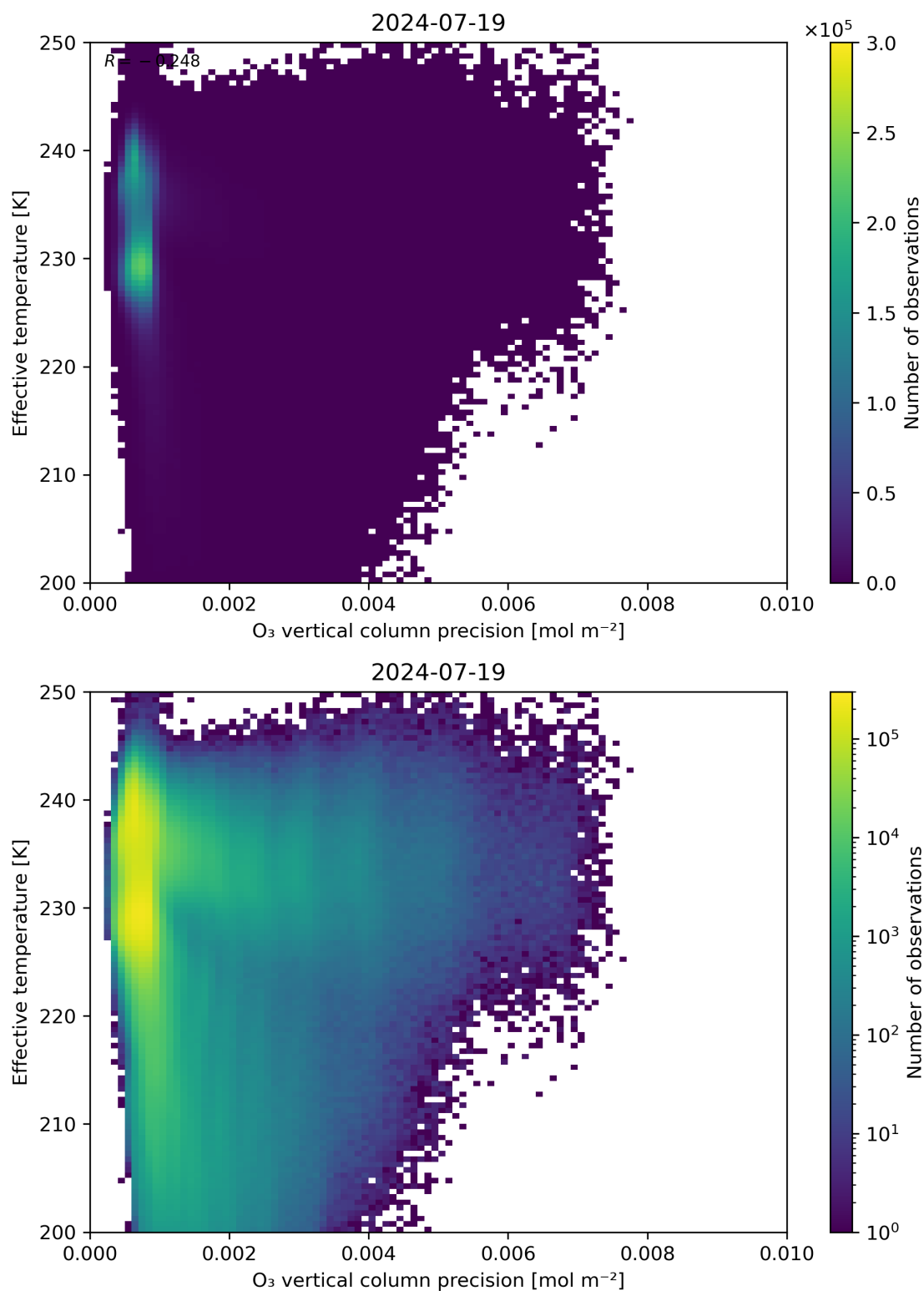
Figure 42: Scatter density plot of “O 3 vertical column precision” against “Effective temperature” for 2024-07-18 to 2024-07-20.
