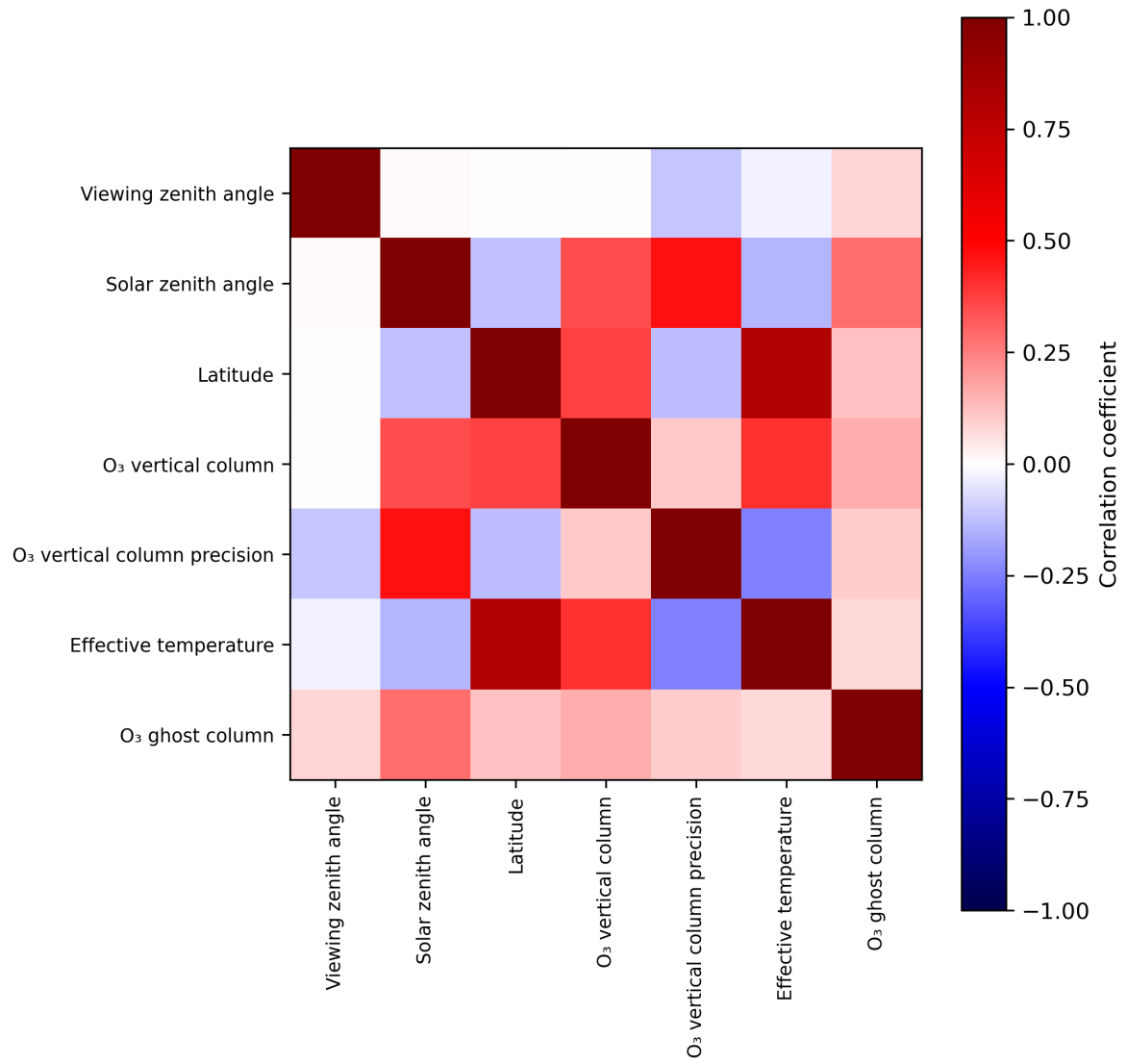
Figure 2: Map of correlation matrix for 2024-07-18 to 2024-07-20.
