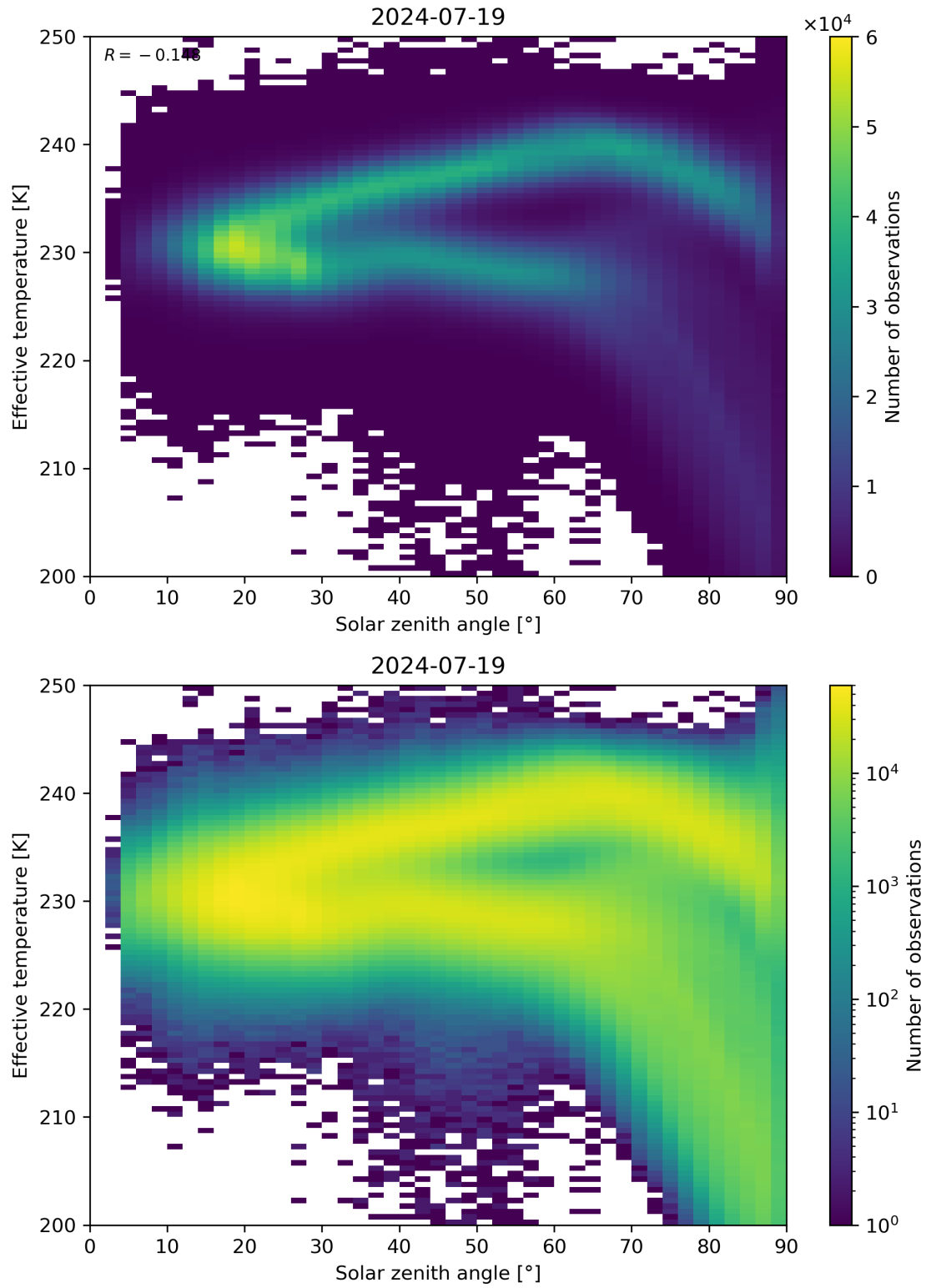
Figure 45: Scatter density plot of “Solar zenith angle” against “Effective temperature” for 2024-07-18 to 2024-07-20.
