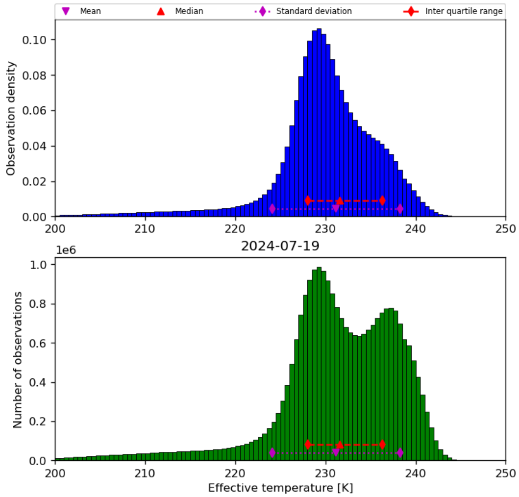
Figure 24: Histogram of “Effective temperature” for 2024-07-18 to 2024-07-20
