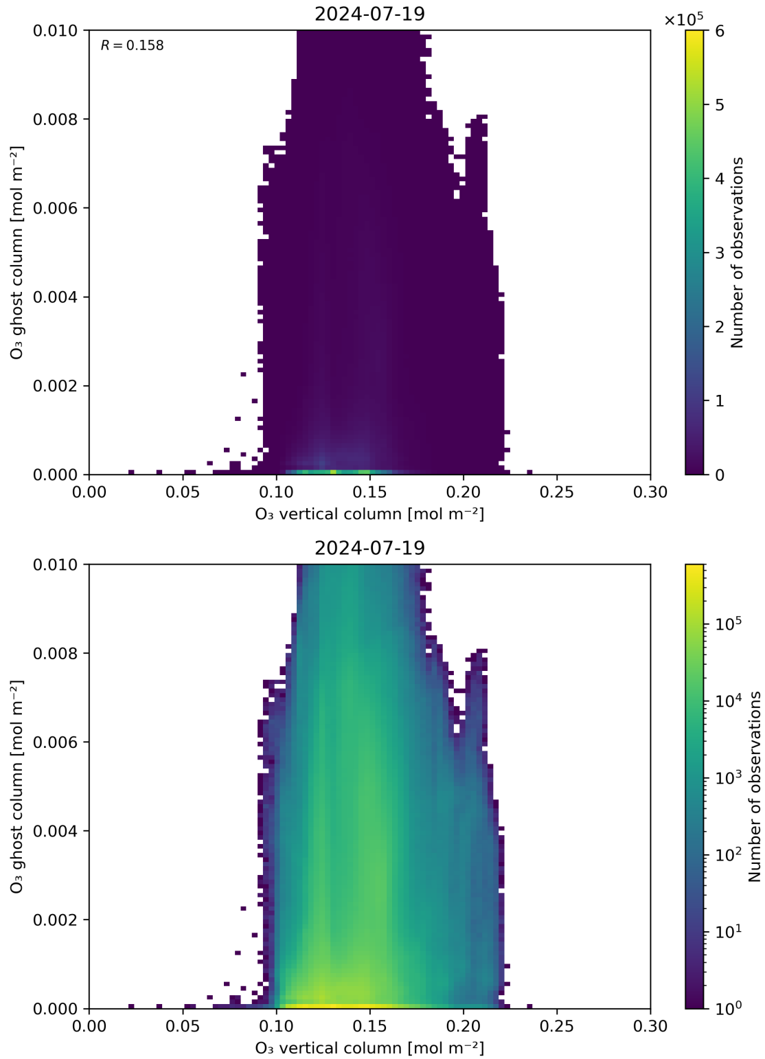
Figure 40: Scatter density plot of “O 3 vertical column” against “O 3 ghost column” for 2024-07-18 to 2024-07-20.
