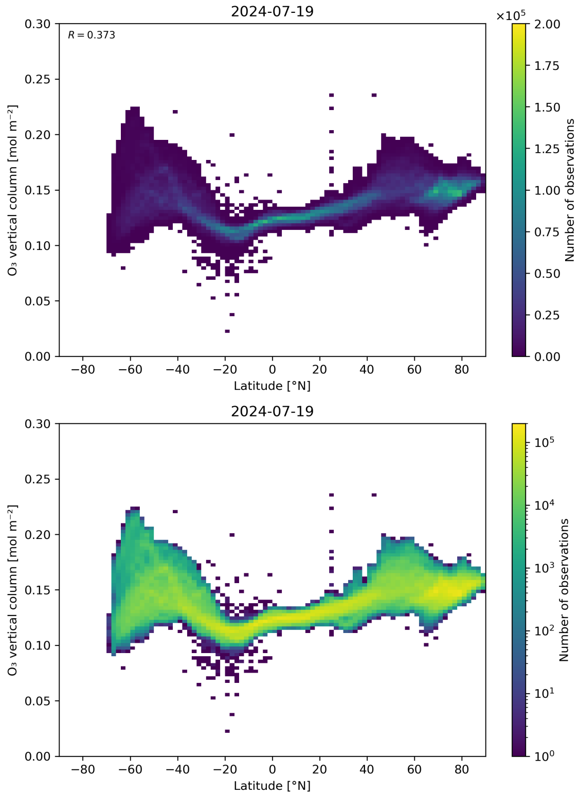
Figure 36: Scatter density plot of “Latitude” against “O 3 vertical column” for 2024-07-18 to 2024-07-20.
