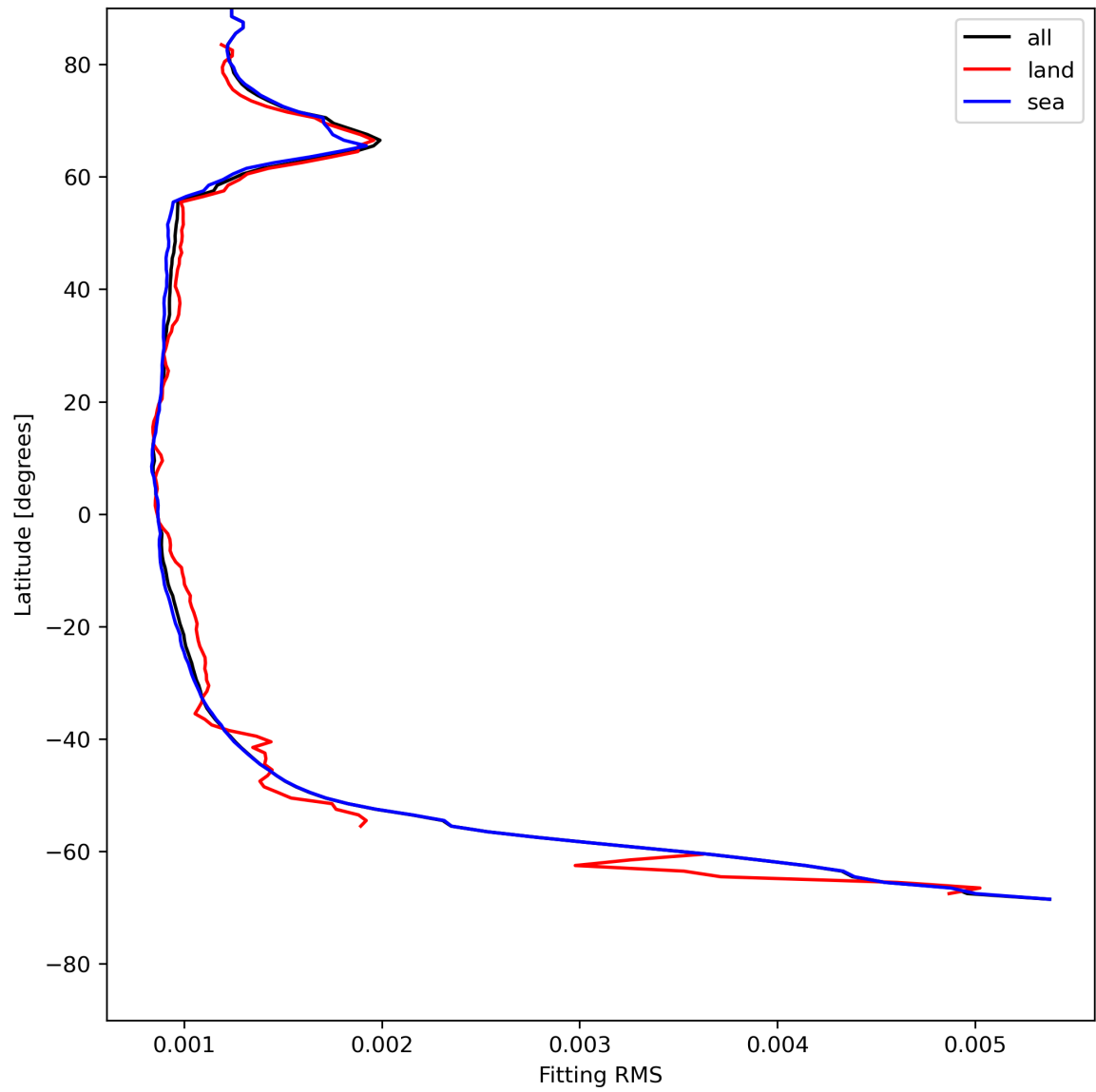
Figure 16: Zonal average of “Fitting RMS” for 2024-07-18 to 2024-07-20.
