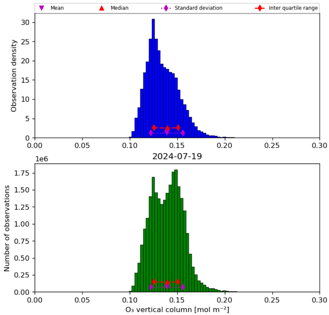
Figure 21: Histogram of “O 3 vertical column” for 2024-07-18 to 2024-07-20
