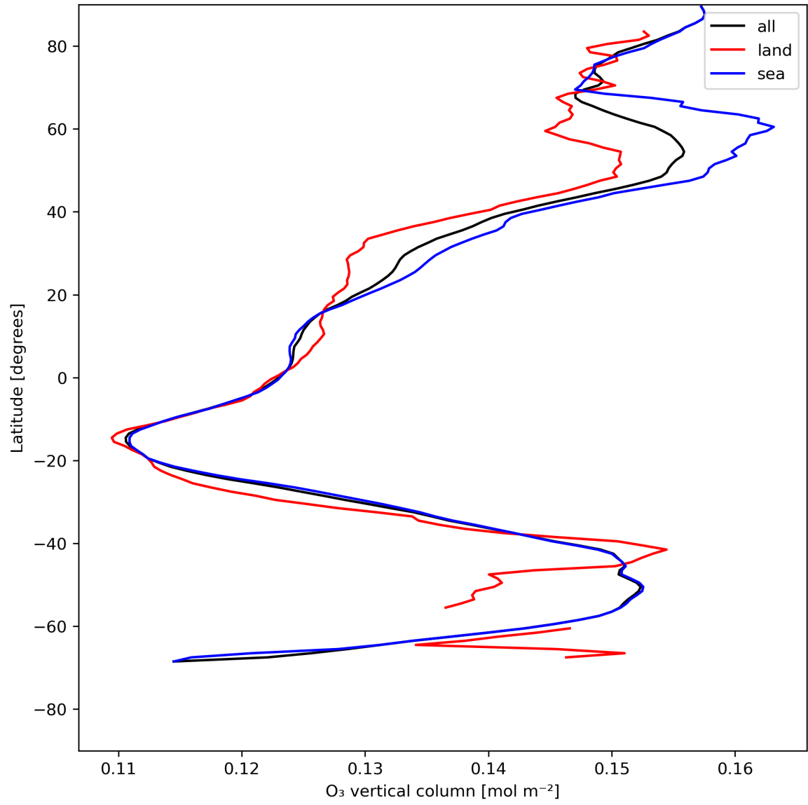
Figure 14: Zonal average of “O 3 vertical column” for 2024-07-18 to 2024-07-20.
