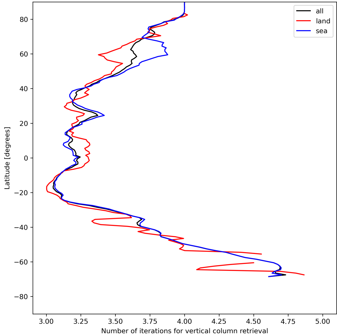
Figure 19: Zonal average of “Number of iterations for vertical column retrieval” for 2024-07-18 to 2024-07-20.
