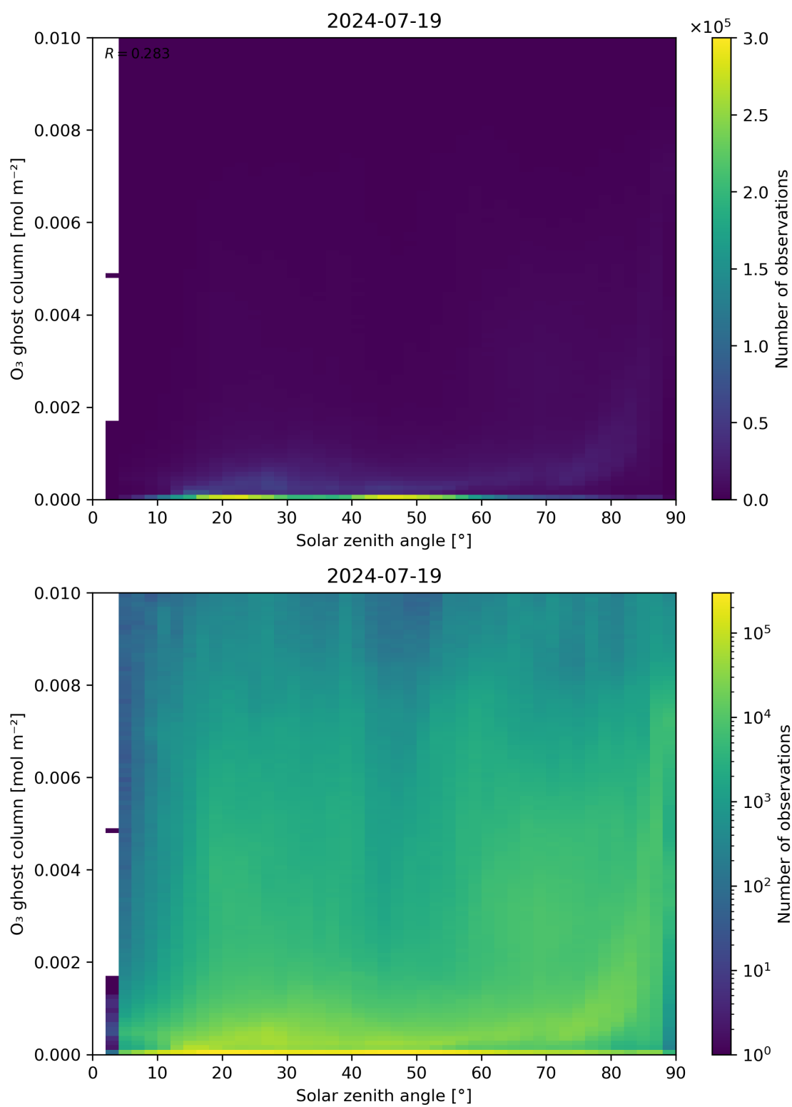
Figure 46: Scatter density plot of “Solar zenith angle” against “O 3 ghost column” for 2024-07-18 to 2024-07-20.
