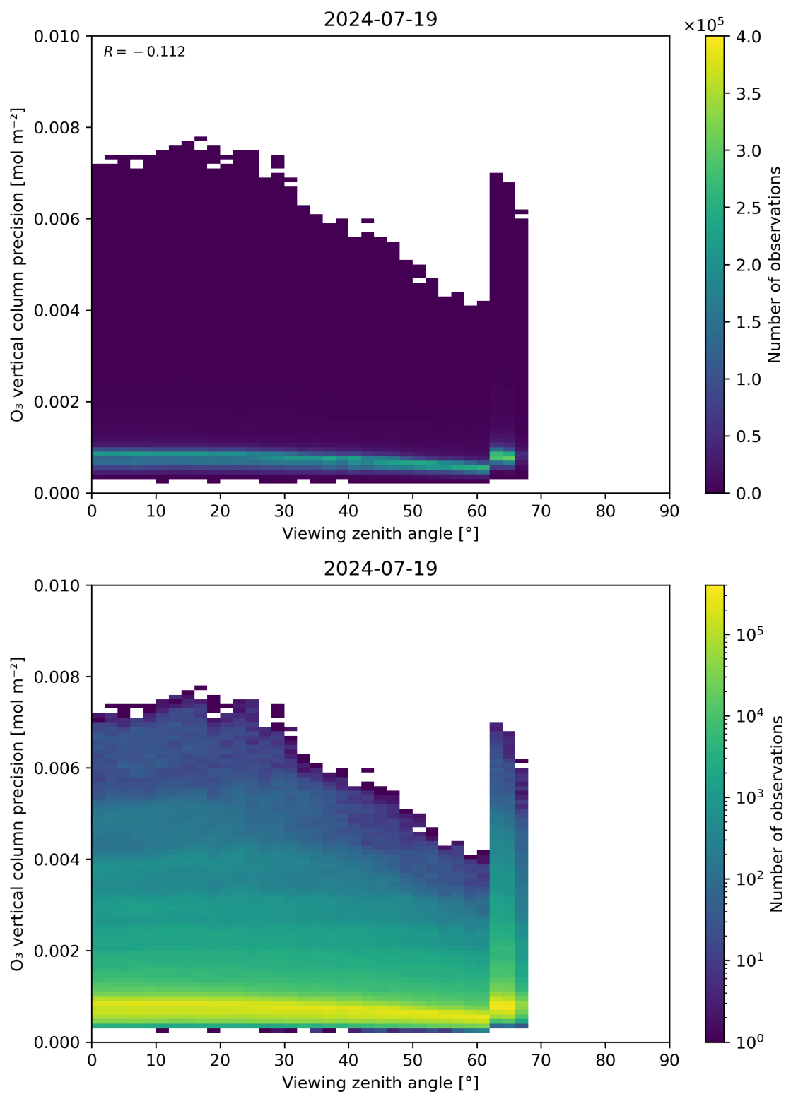
Figure 53: Scatter density plot of “Viewing zenith angle” against “O 3 vertical column precision” for 2024-07-18 to 2024-07-20.
