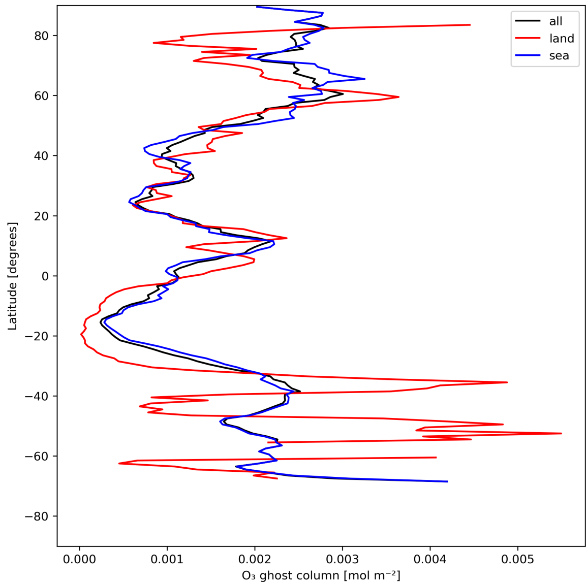
Figure 18: Zonal average of “O 3 ghost column” for 2024-07-18 to 2024-07-20.
