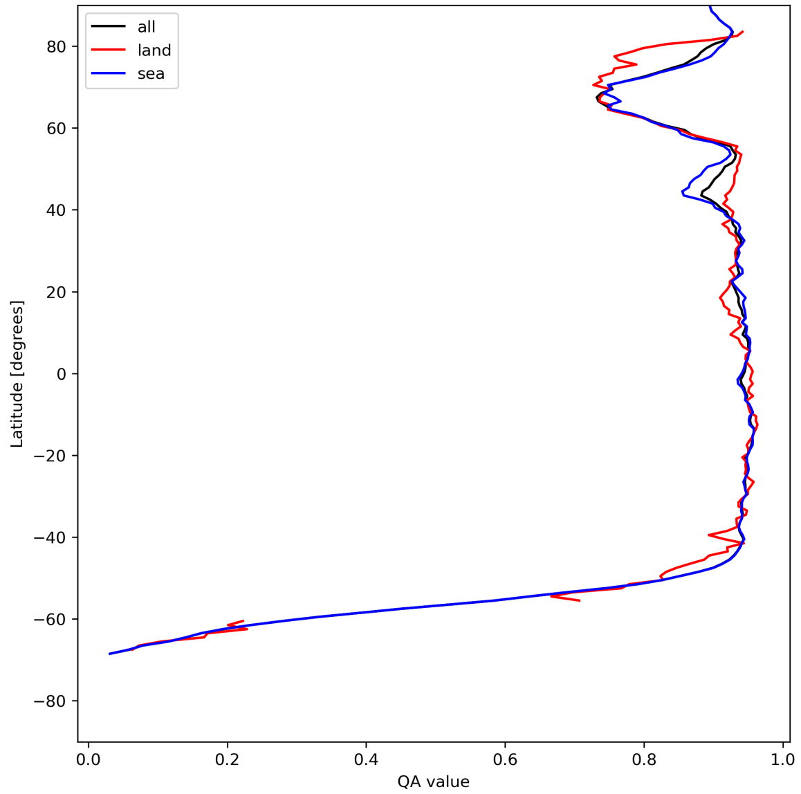
Figure 13: Zonal average of “QA value” for 2024-07-18 to 2024-07-20.
