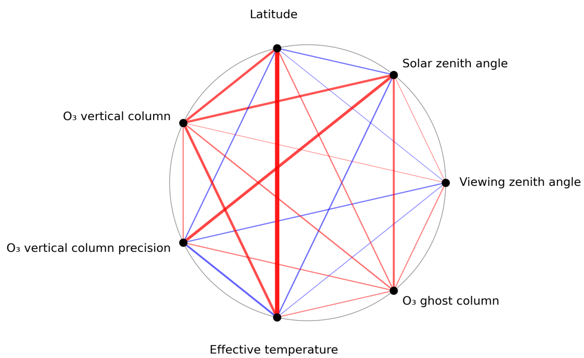
Figure 1: Map of correlation graph for 2024-07-18 to 2024-07-20.
