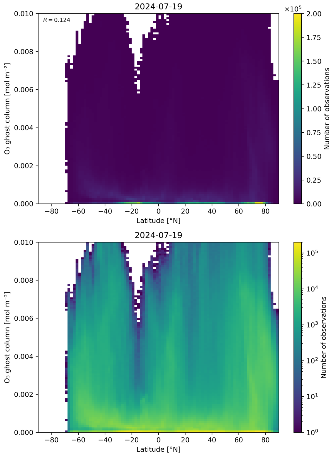
Figure 35: Scatter density plot of “Latitude” against “O 3 ghost column” for 2024-07-18 to 2024-07-20.
