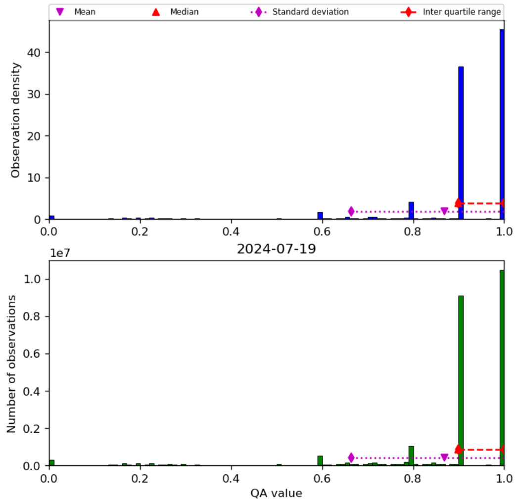
Figure 20: Histogram of “QA value” for 2024-07-18 to 2024-07-20
