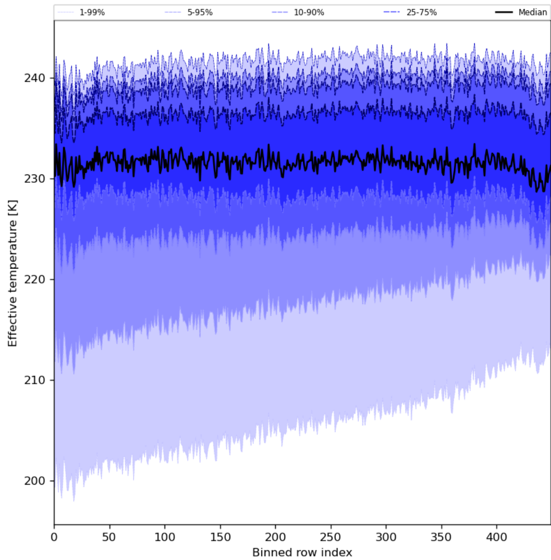
Figure 31: Along track statistics of “Effective temperature” for 2024-07-18 to 2024-07-20
