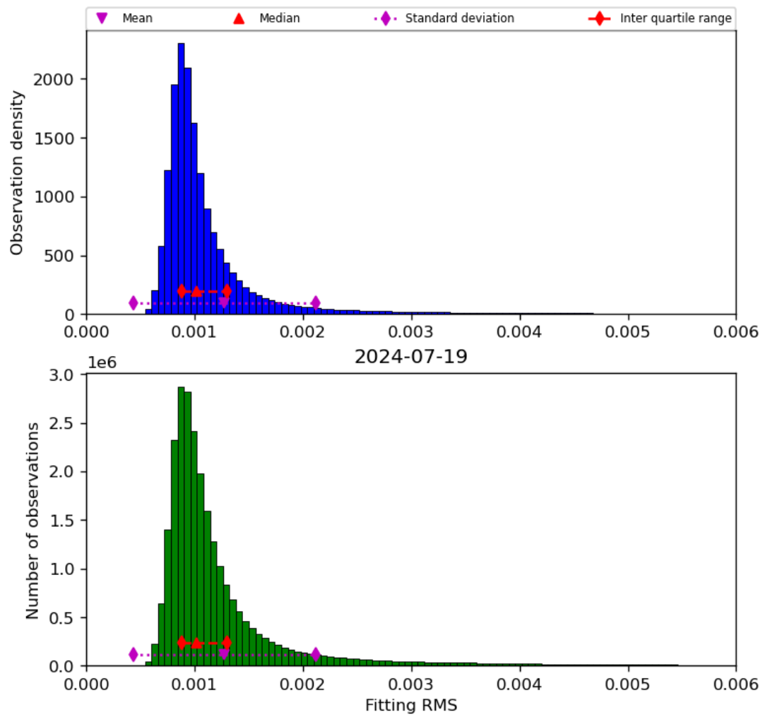
Figure 23: Histogram of “Fitting RMS” for 2024-07-18 to 2024-07-20
