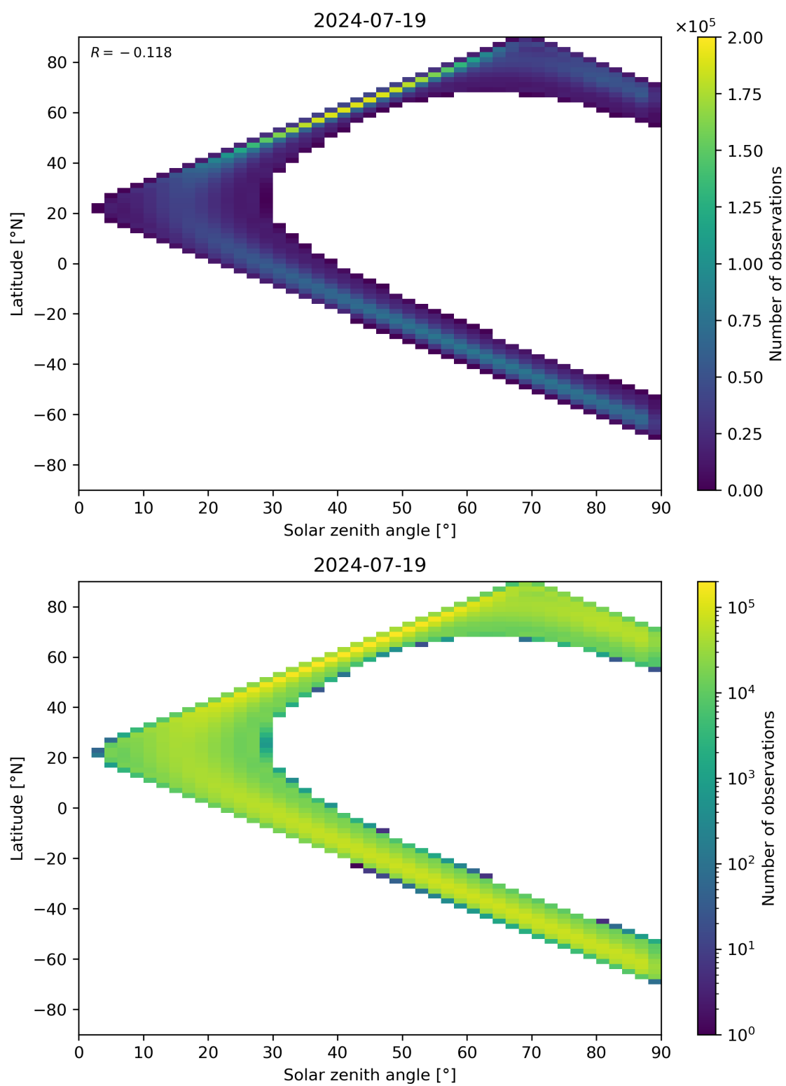
Figure 44: Scatter density plot of “Solar zenith angle” against “Latitude” for 2024-07-18 to 2024-07-20.
