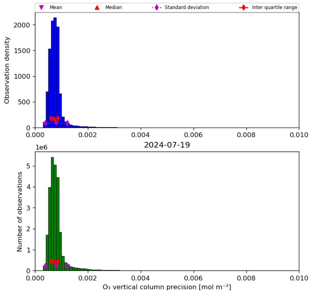
Figure 22: Histogram of “O 3 vertical column precision” for 2024-07-18 to 2024-07-20
