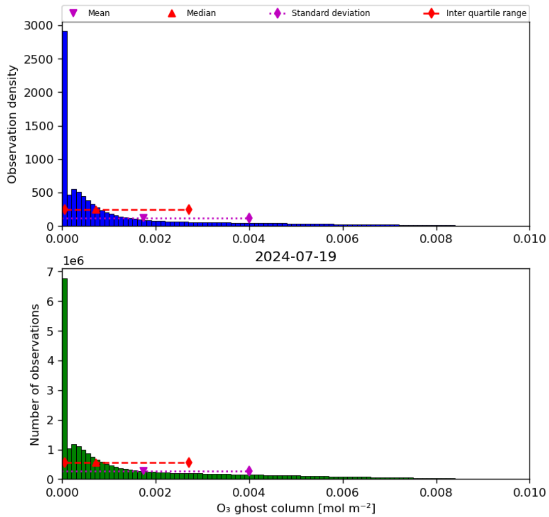
Figure 25: Histogram of “O 3 ghost column” for 2024-07-18 to 2024-07-20
