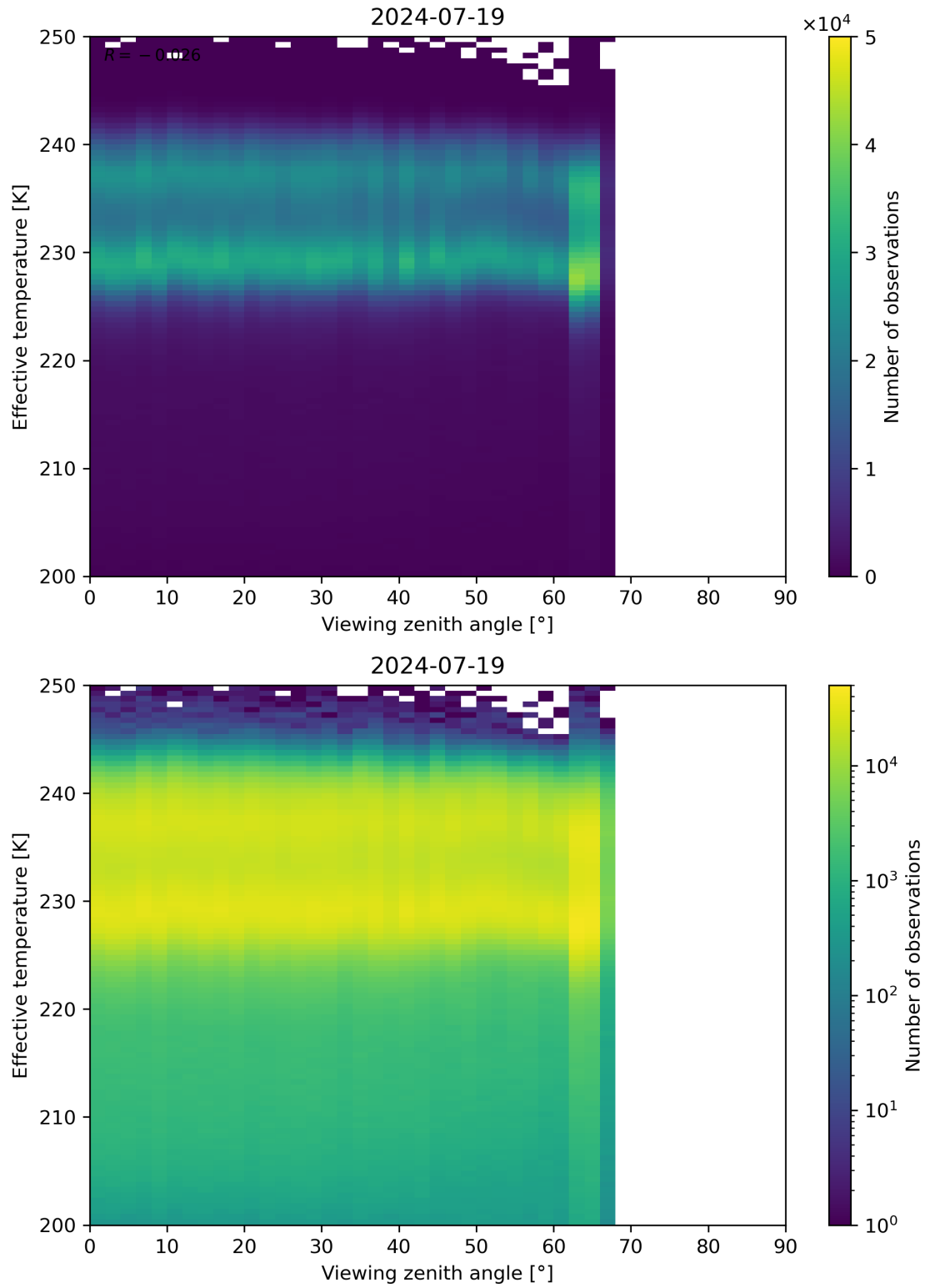
Figure 50: Scatter density plot of “Viewing zenith angle” against “Effective temperature” for 2024-07-18 to 2024-07-20.
