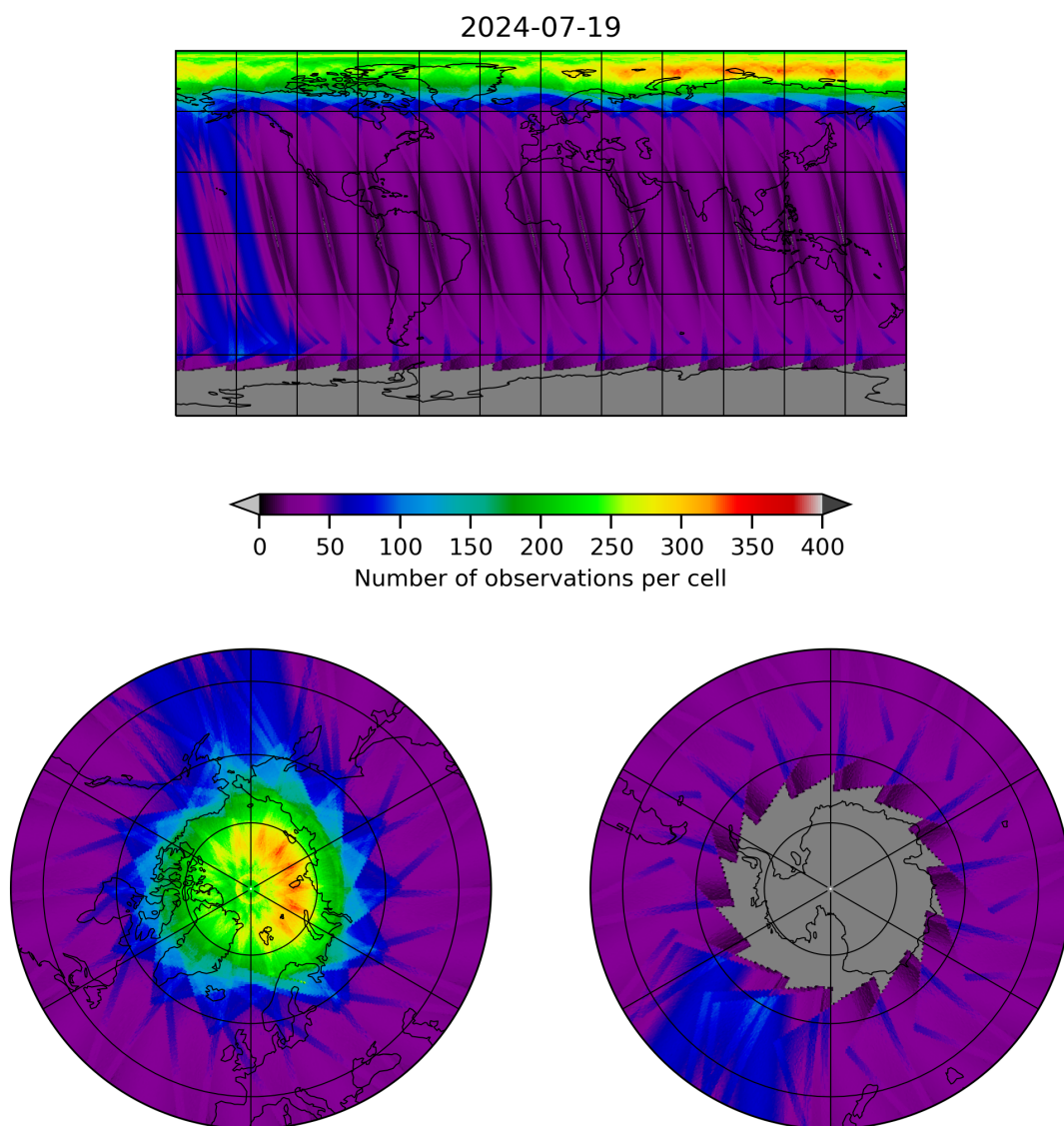
Figure 12: Map of the number of observations for 2024-07-18 to 2024-07-20
