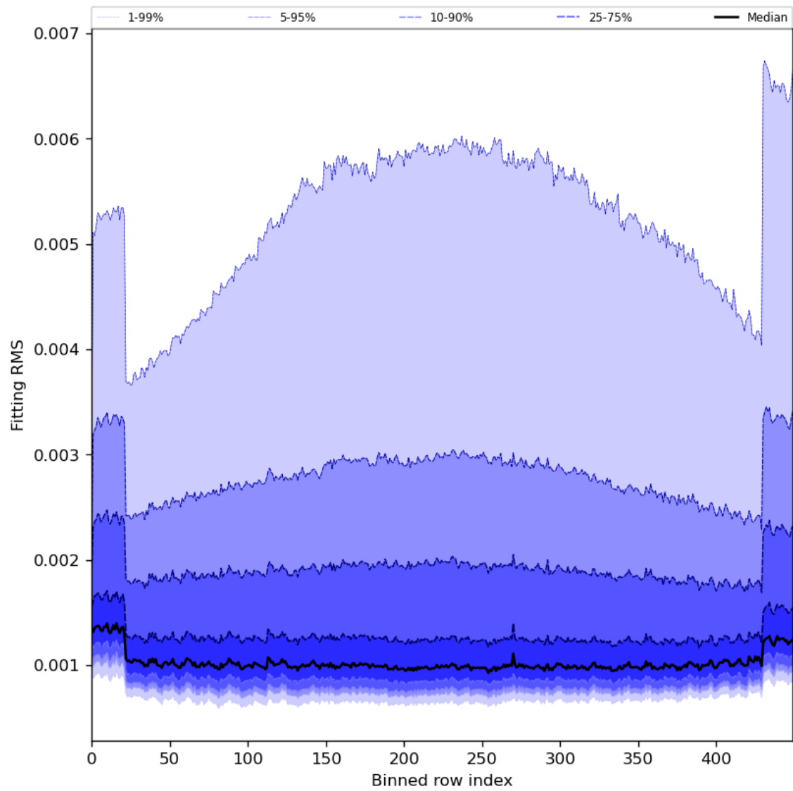
Figure 30: Along track statistics of “Fitting RMS” for 2024-07-18 to 2024-07-20
