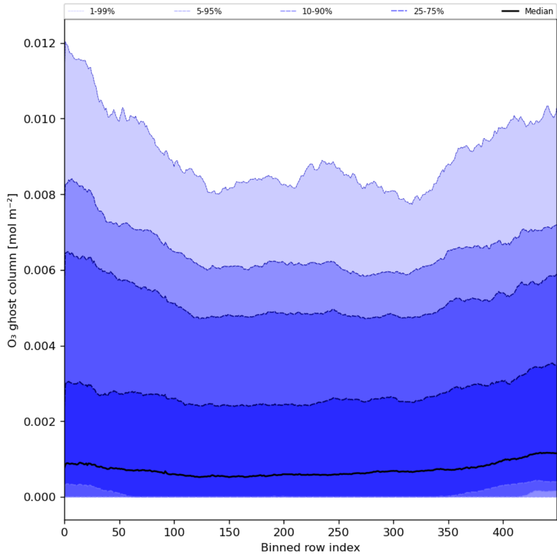
Figure 32: Along track statistics of "O 3 ghost column" for 2024-07-18 to 2024-07-20
