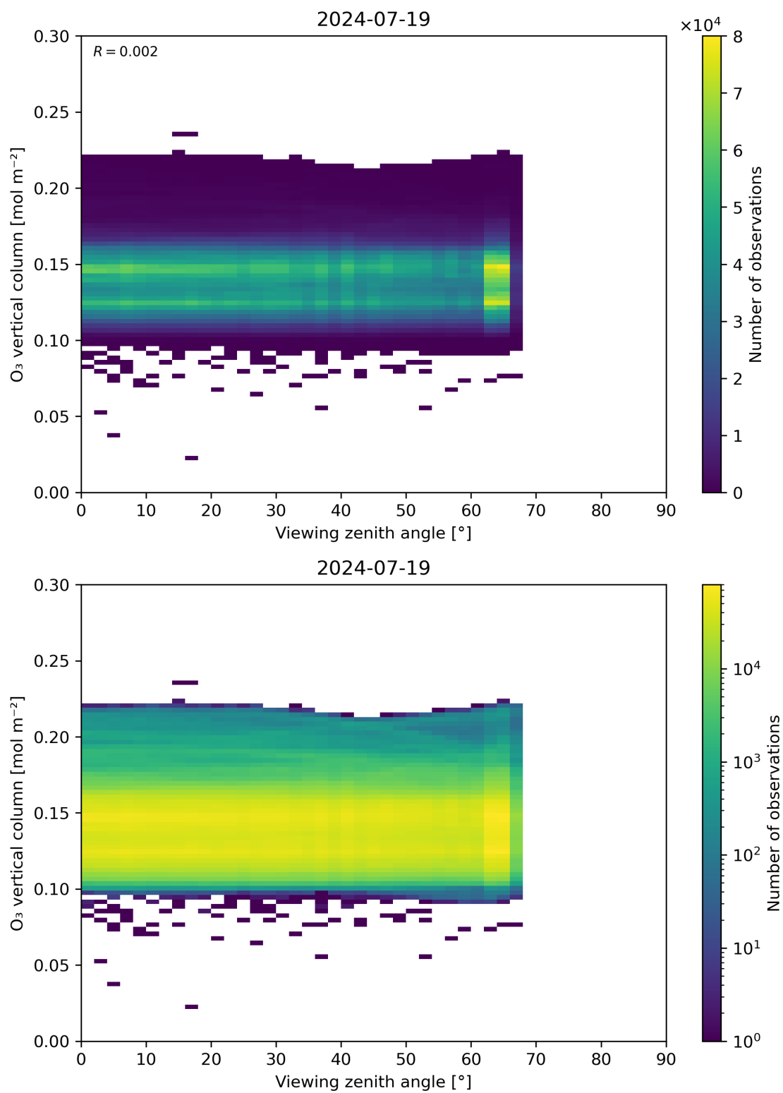
Figure 52: Scatter density plot of “Viewing zenith angle” against “O 3 vertical column” for 2024-07-18 to 2024-07-20.
