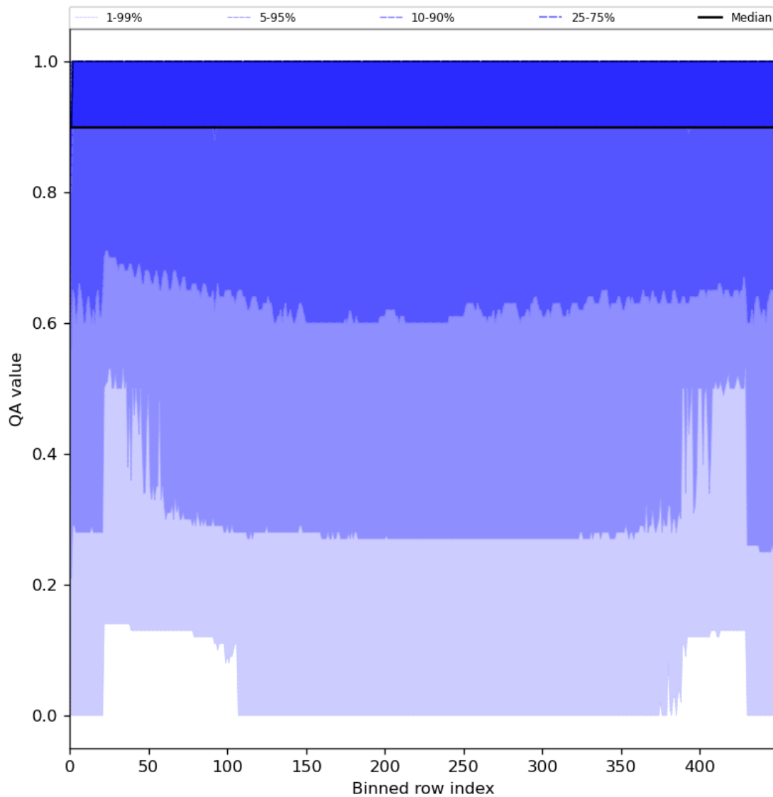
Figure 27: Along track statistics of “QA value” for 2024-07-18 to 2024-07-20
