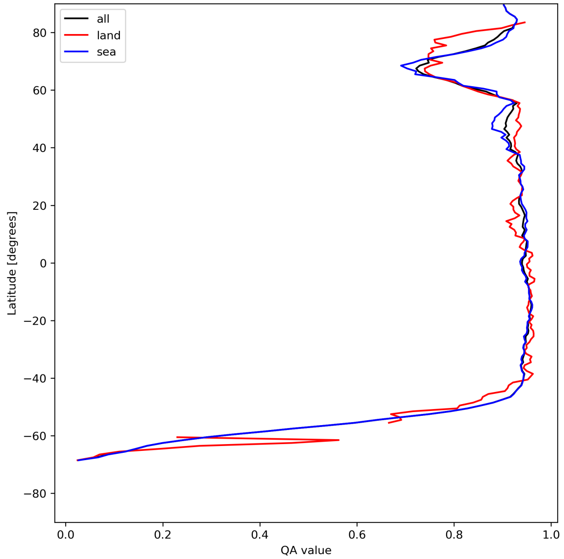
Figure 13: Zonal average of “QA value” for 2024-07-19 to 2024-07-21.
