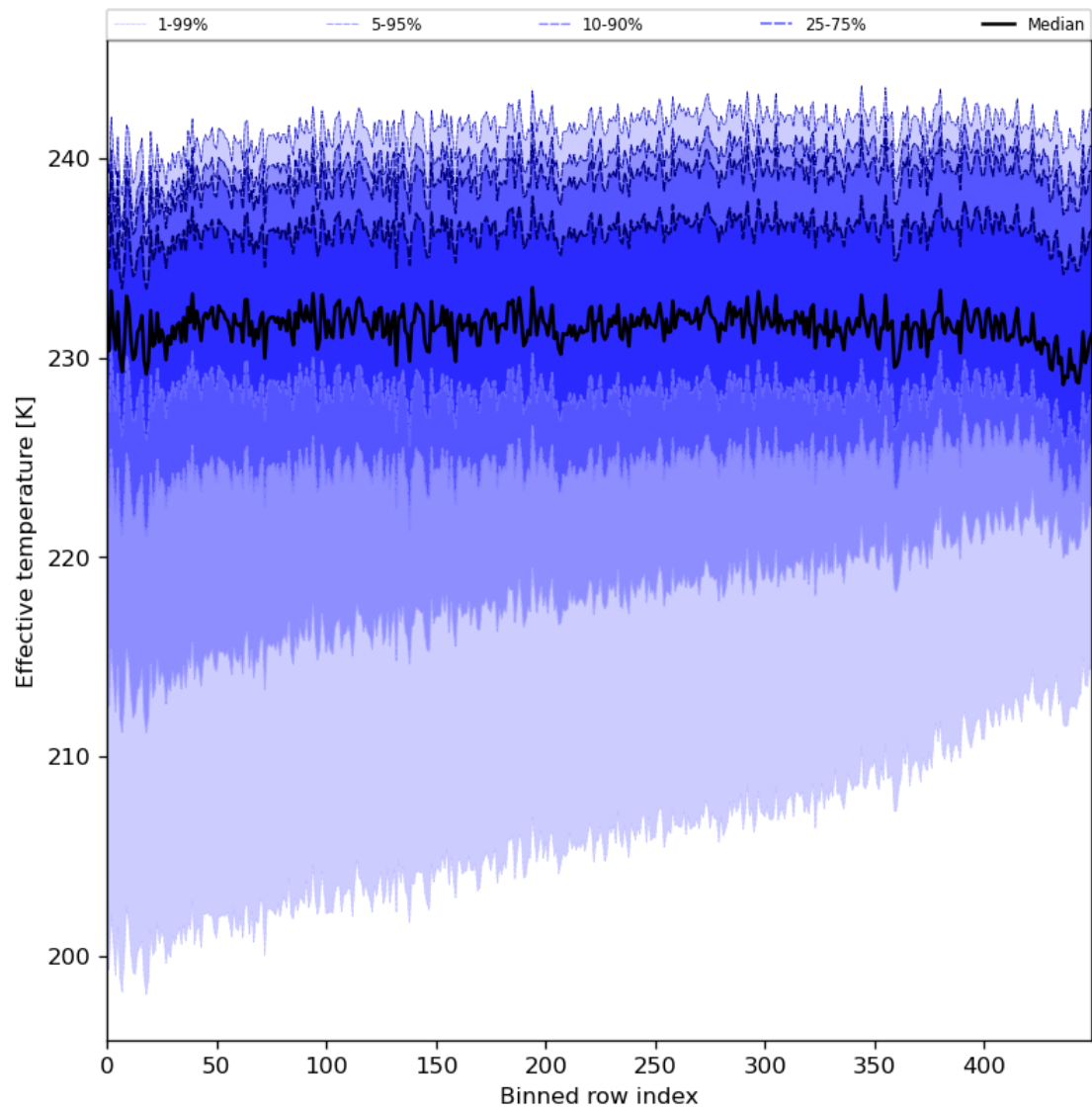
Figure 31: Along track statistics of “Effective temperature” for 2024-07-19 to 2024-07-21
