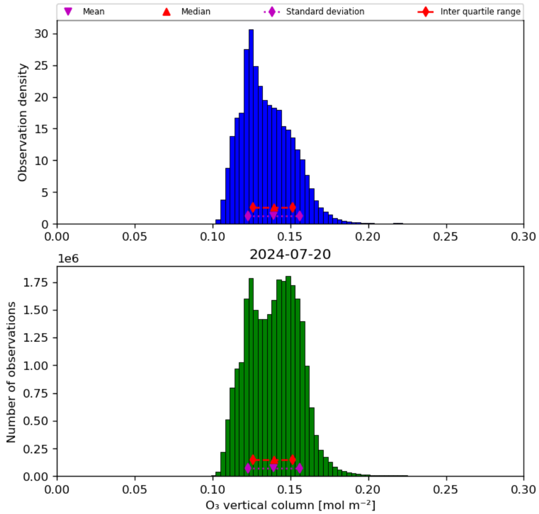
Figure 21: Histogram of “O 3 vertical column” for 2024-07-19 to 2024-07-21
