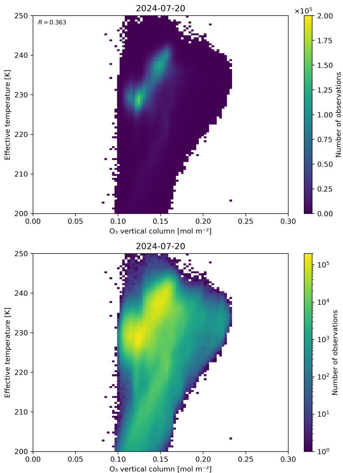
Figure 39: Scatter density plot of “O 3 vertical column” against “Effective temperature” for 2024-07-19 to 2024-07-21.
