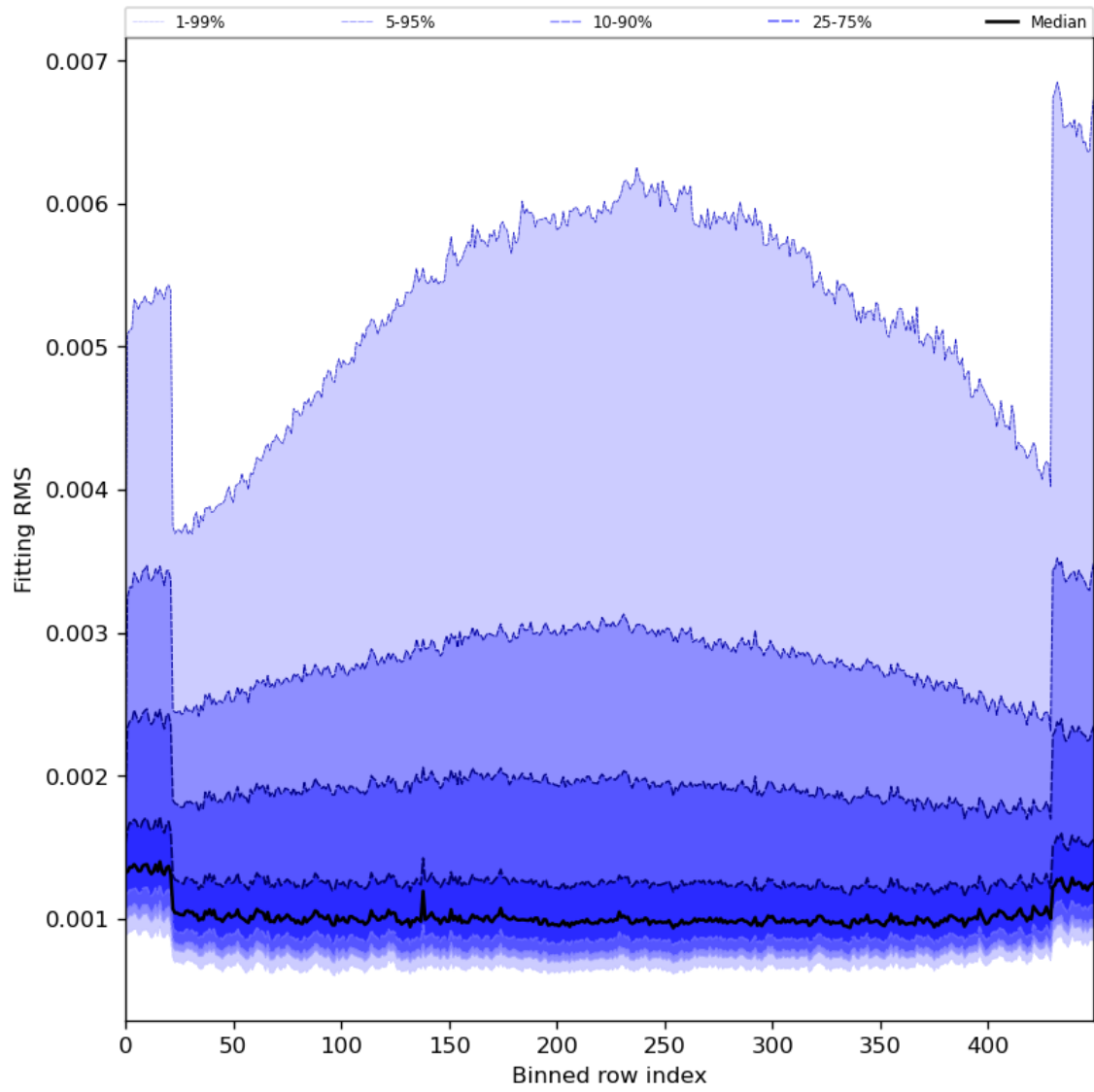
Figure 30: Along track statistics of “Fitting RMS” for 2024-07-19 to 2024-07-21
