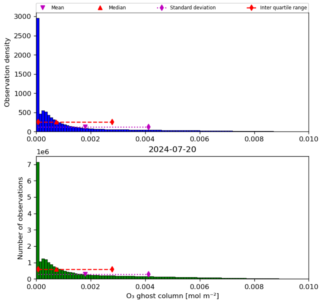
Figure 25: Histogram of “O 3 ghost column” for 2024-07-19 to 2024-07-21
