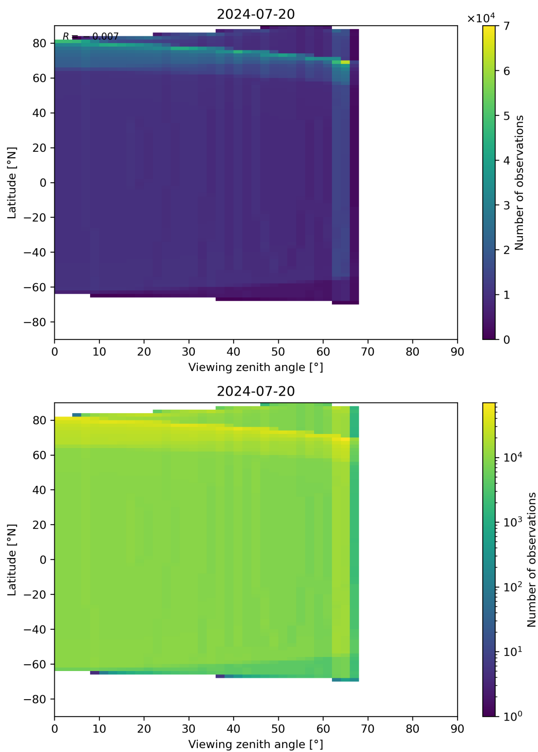
Figure 49: Scatter density plot of “Viewing zenith angle” against “Latitude” for 2024-07-19 to 2024-07-21.
