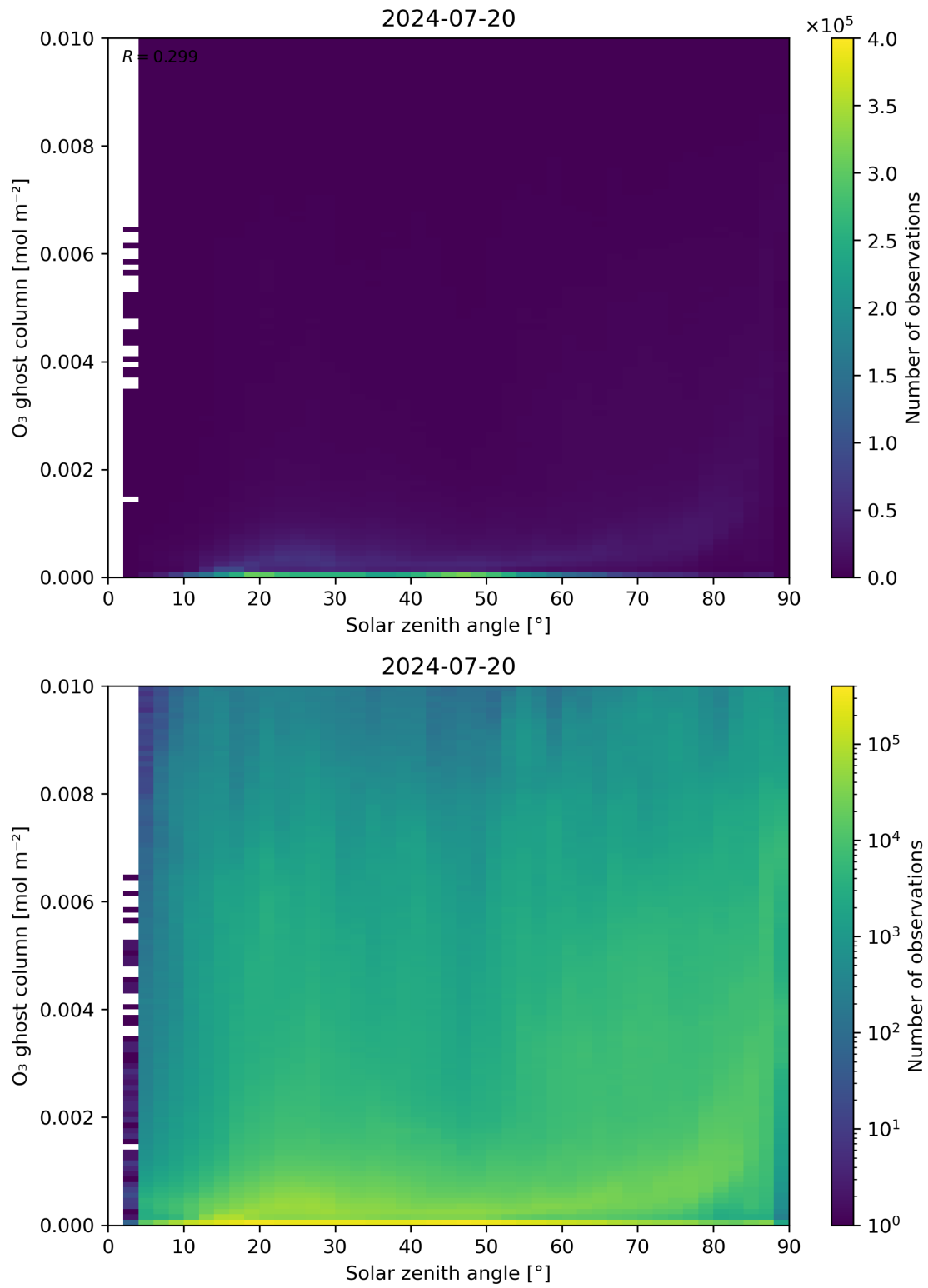
Figure 46: Scatter density plot of “Solar zenith angle” against “O 3 ghost column” for 2024-07-19 to 2024-07-21.
