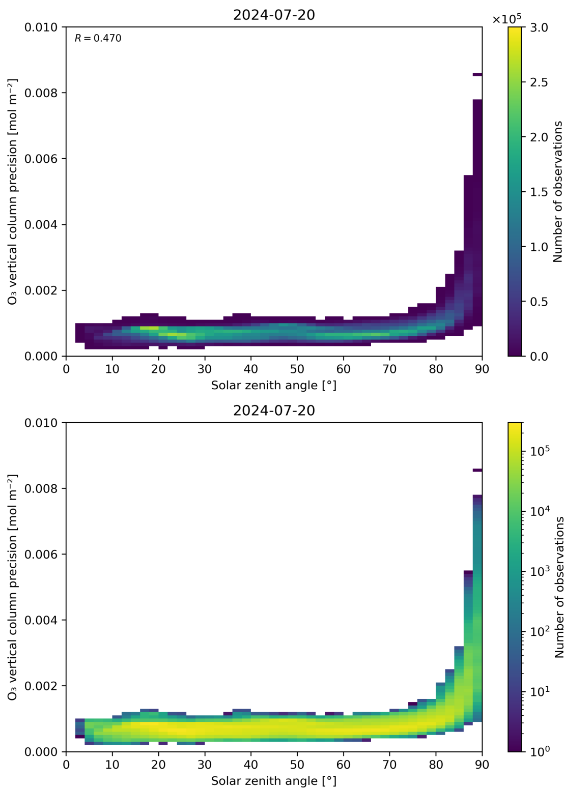
Figure 48: Scatter density plot of “Solar zenith angle” against “O 3 vertical column precision” for 2024-07-19 to 2024-07-21.
