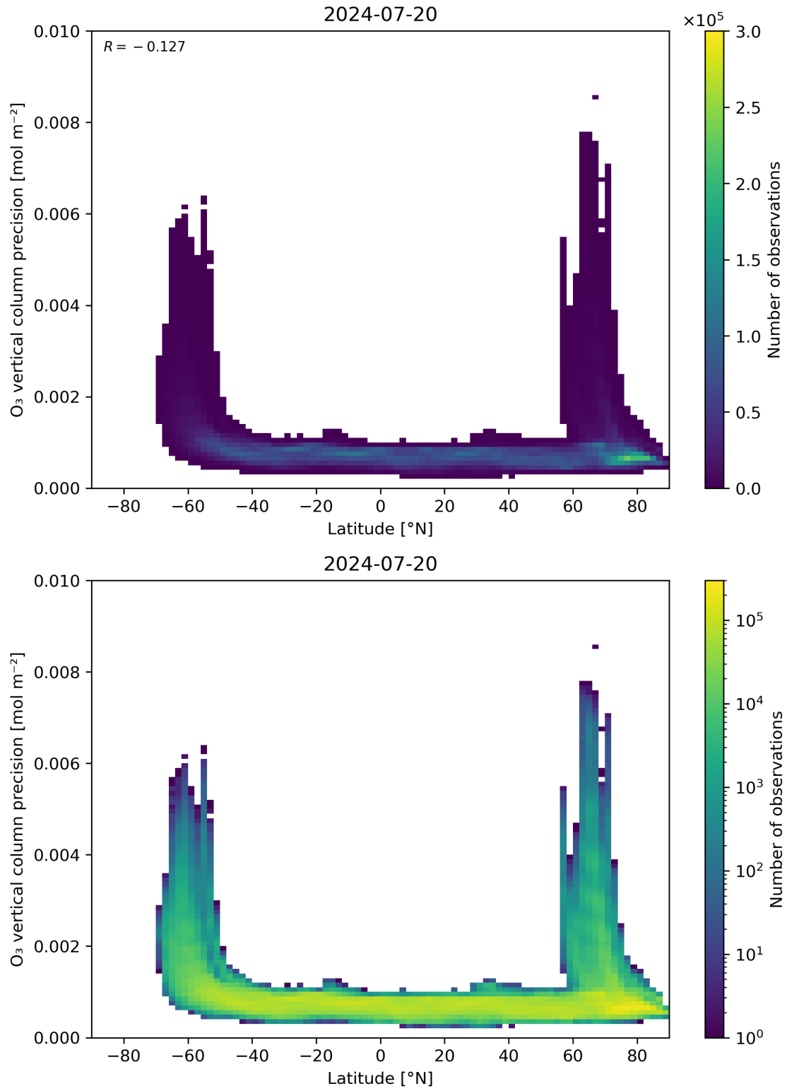
Figure 37: Scatter density plot of “Latitude” against “O 3 vertical column precision” for 2024-07-19 to 2024-07-21.
