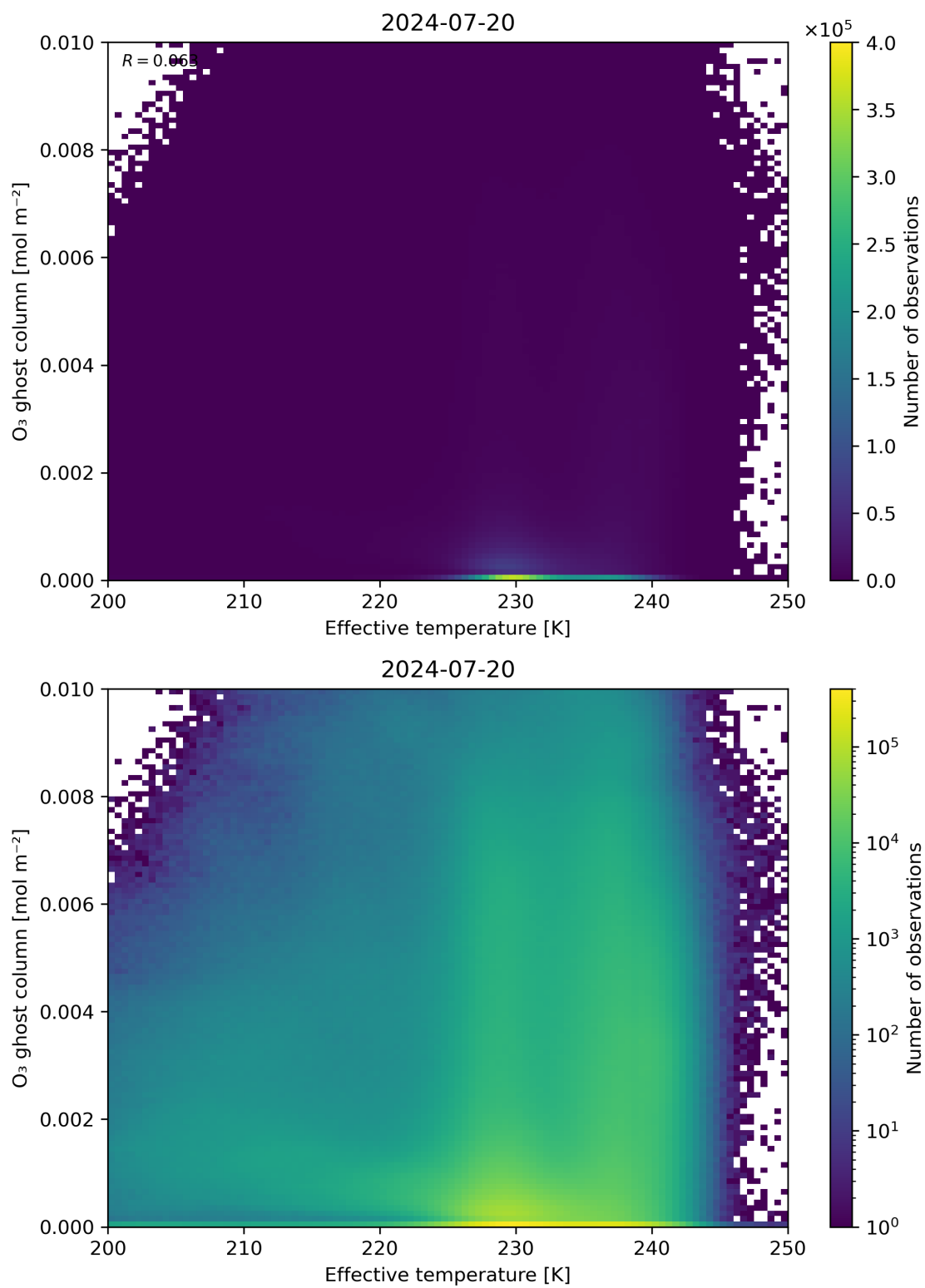
Figure 38: Scatter density plot of “Effective temperature” against “O 3 ghost column” for 2024-07-19 to 2024-07-21.
