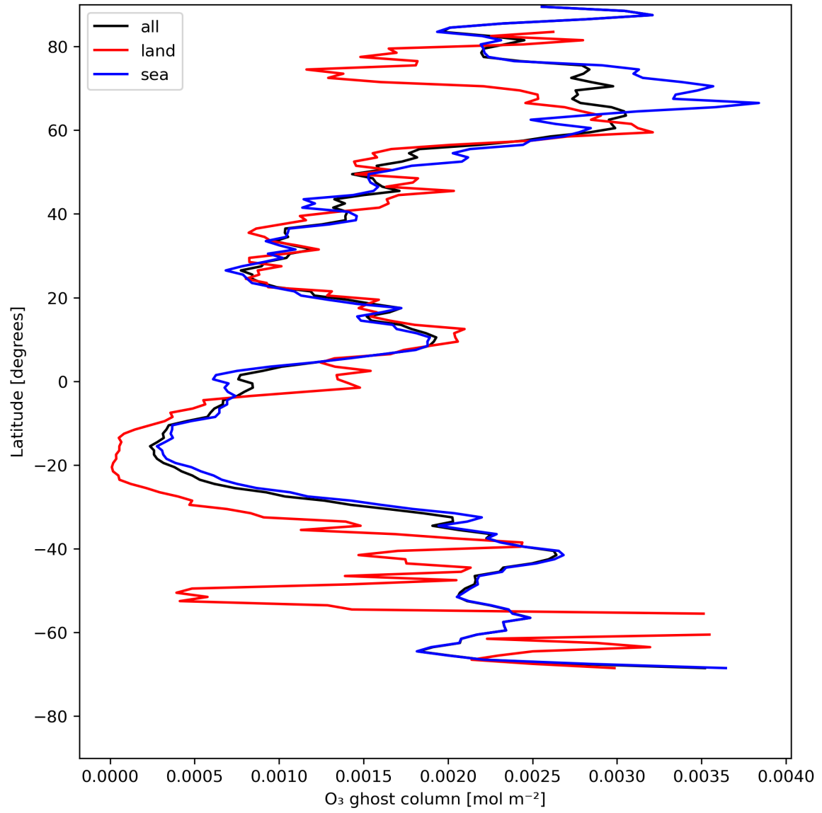
Figure 18: Zonal average of “O 3 ghost column” for 2024-07-19 to 2024-07-21.
