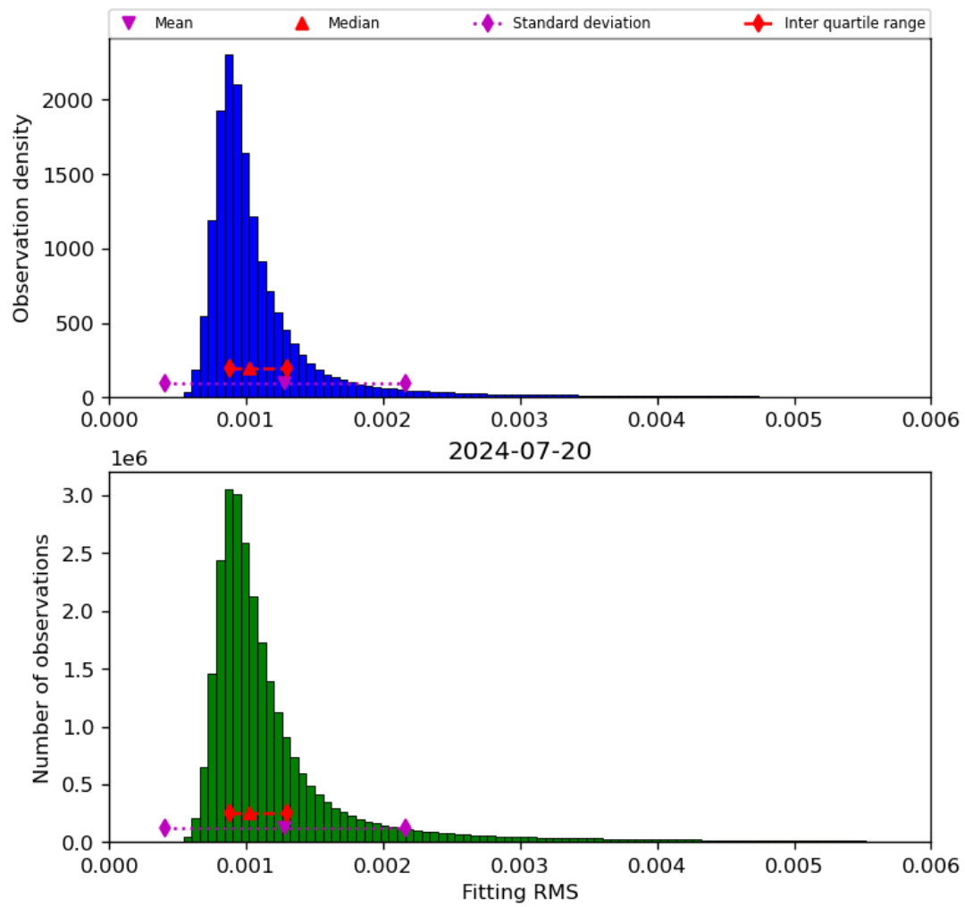
Figure 23: Histogram of “Fitting RMS” for 2024-07-19 to 2024-07-21
