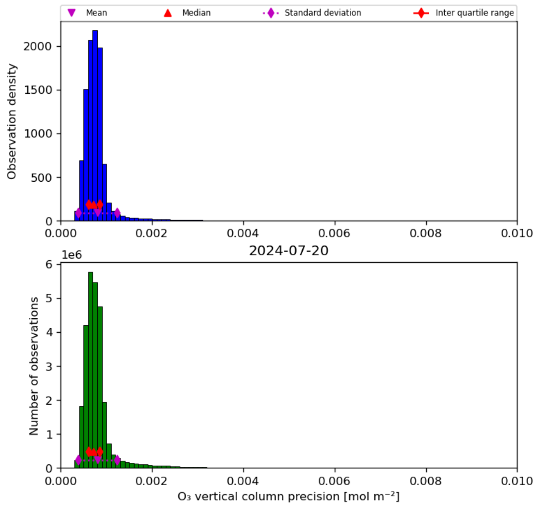
Figure 22: Histogram of “O 3 vertical column precision” for 2024-07-19 to 2024-07-21
