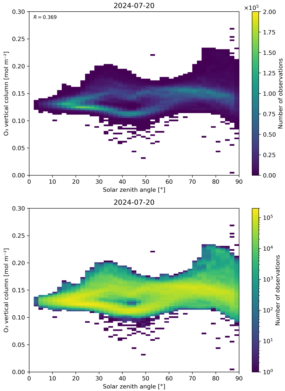
Figure 47: Scatter density plot of “Solar zenith angle” against “O 3 vertical column” for 2024-07-19 to 2024-07-21.
