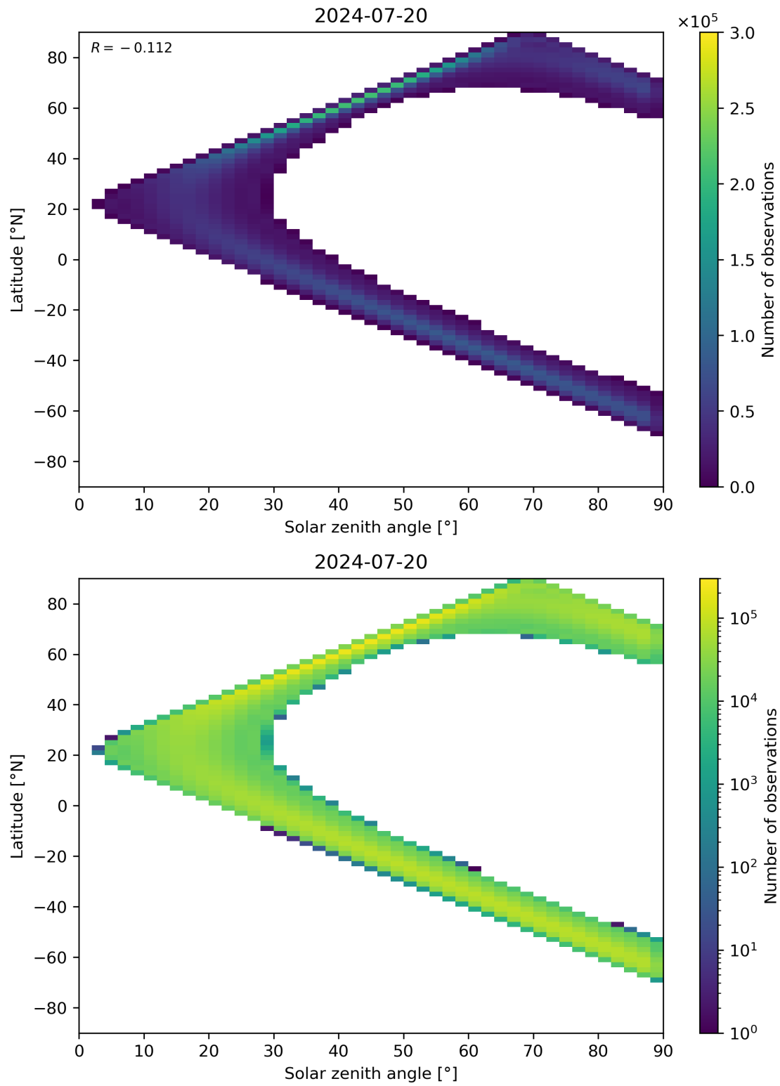
Figure 44: Scatter density plot of “Solar zenith angle” against “Latitude” for 2024-07-19 to 2024-07-21.
