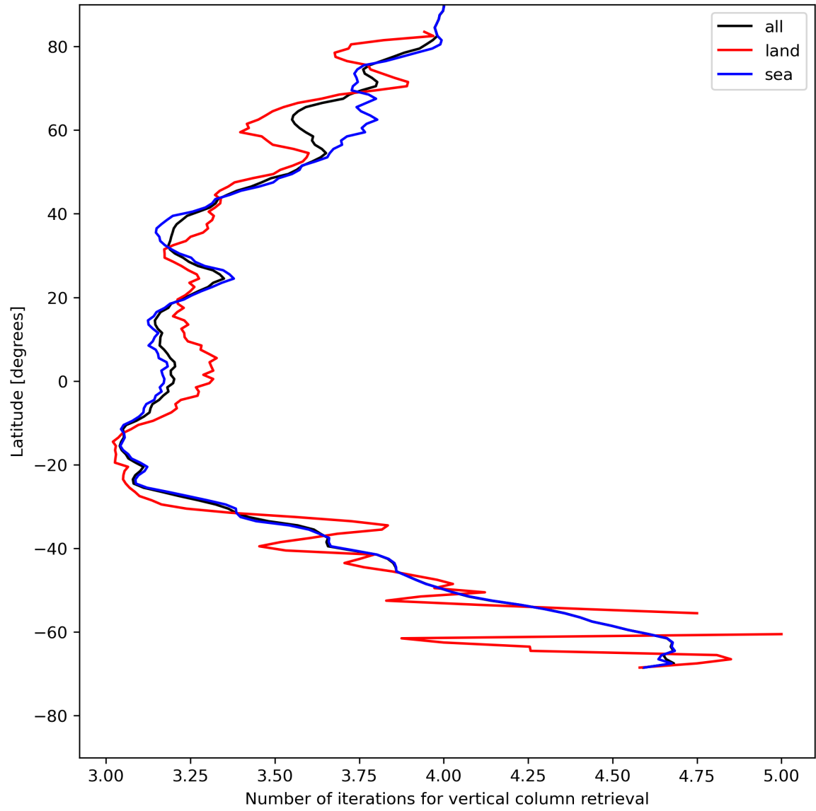
Figure 19: Zonal average of “Number of iterations for vertical column retrieval” for 2024-07-19 to 2024-07-21.
