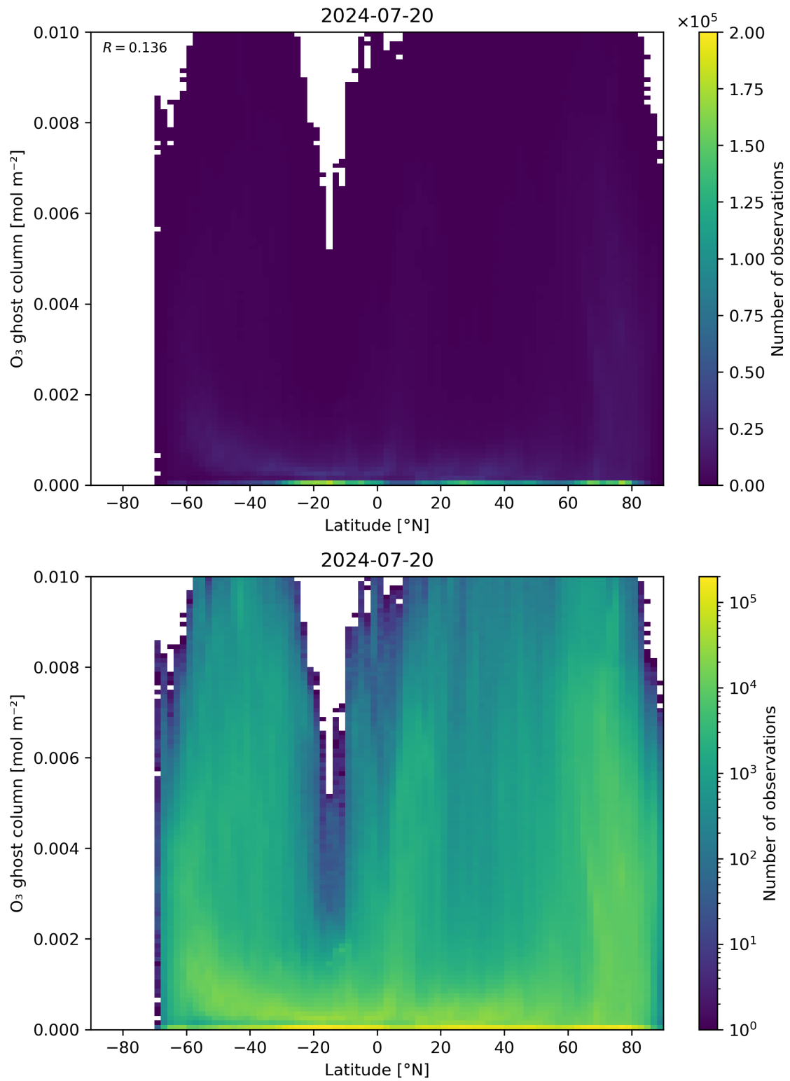
Figure 35: Scatter density plot of “Latitude” against “O 3 ghost column” for 2024-07-19 to 2024-07-21.
