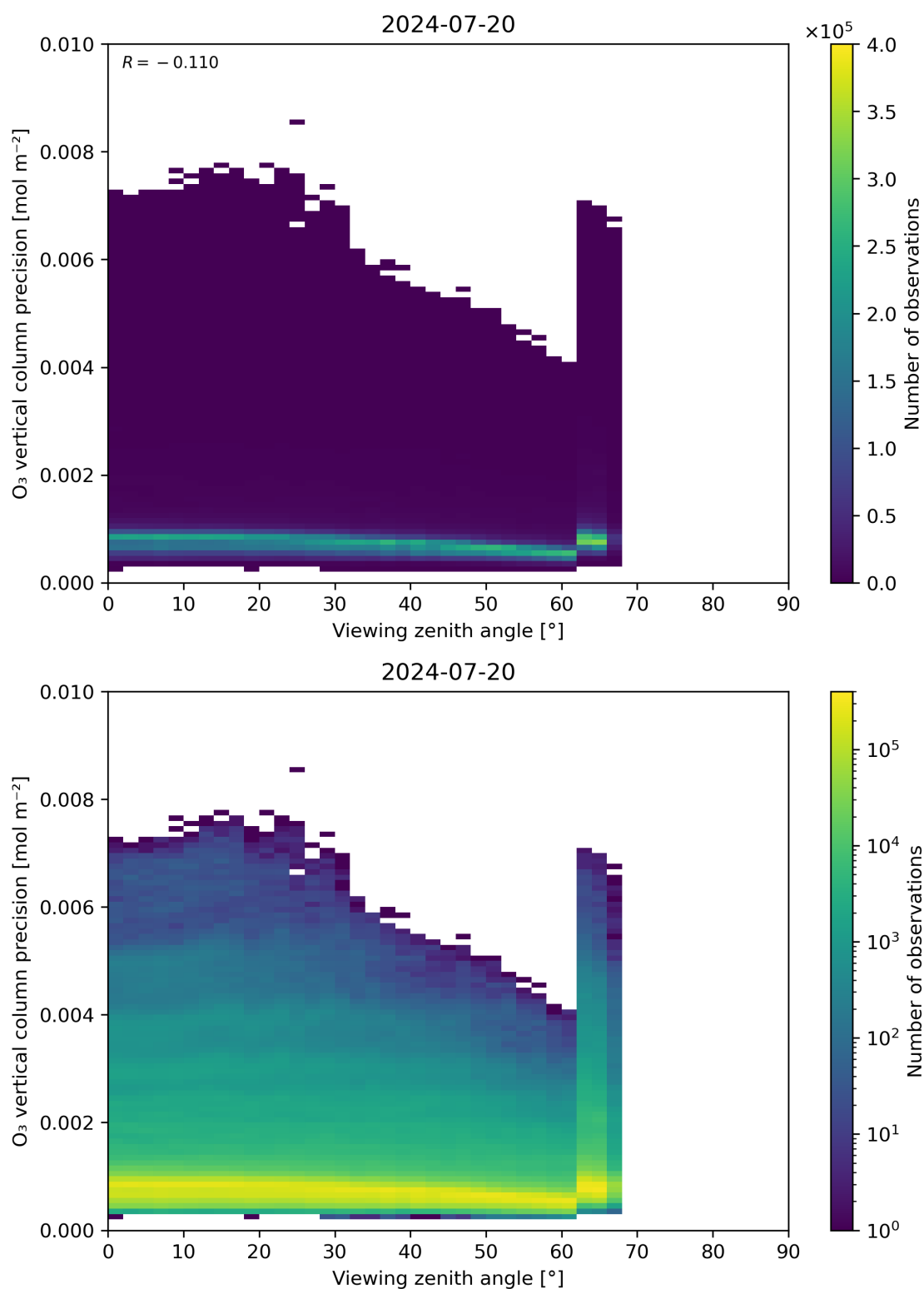
Figure 53: Scatter density plot of “Viewing zenith angle” against “O 3 vertical column precision” for 2024-07-19 to 2024-07-21.
