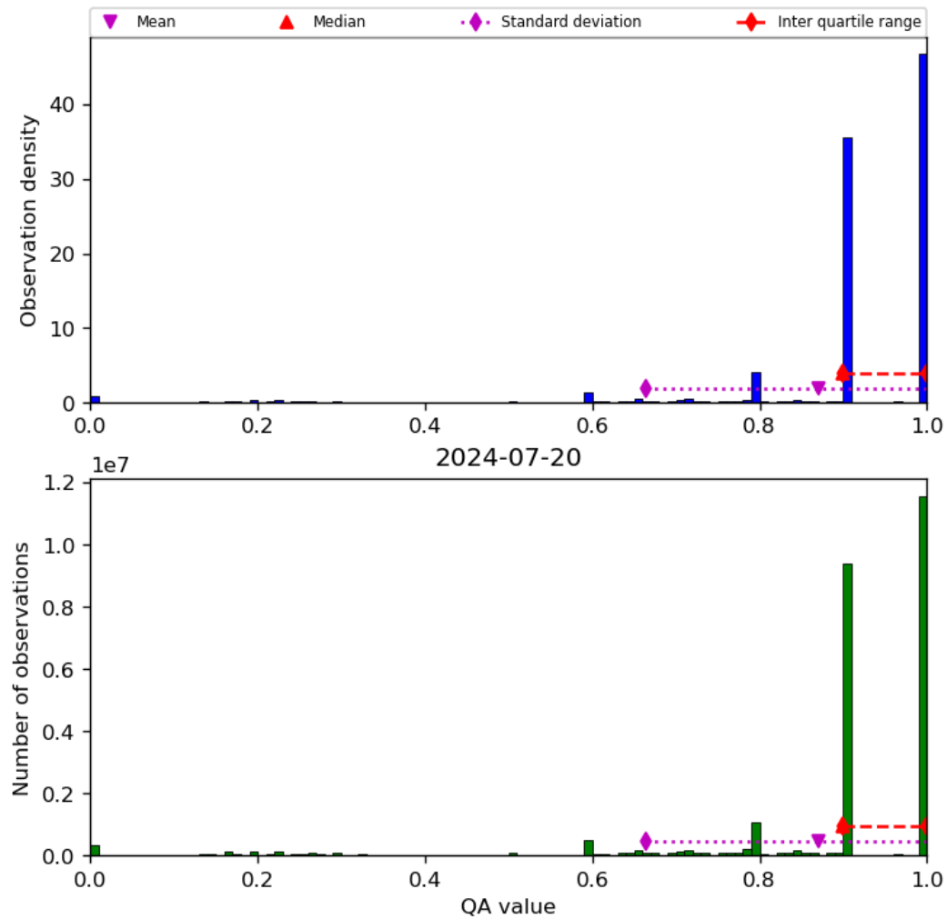
Figure 20: Histogram of “QA value” for 2024-07-19 to 2024-07-21
