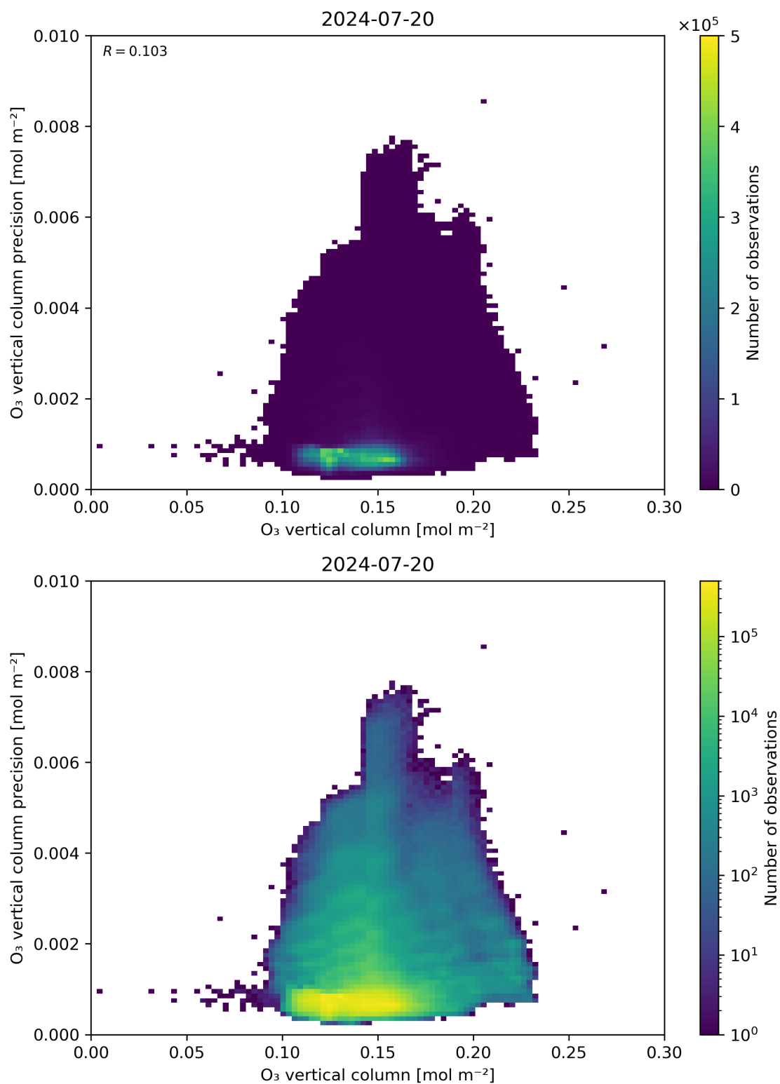
Figure 41: Scatter density plot of “O 3 vertical column” against “O 3 vertical column precision” for 2024-07-19 to 2024-07-21.
