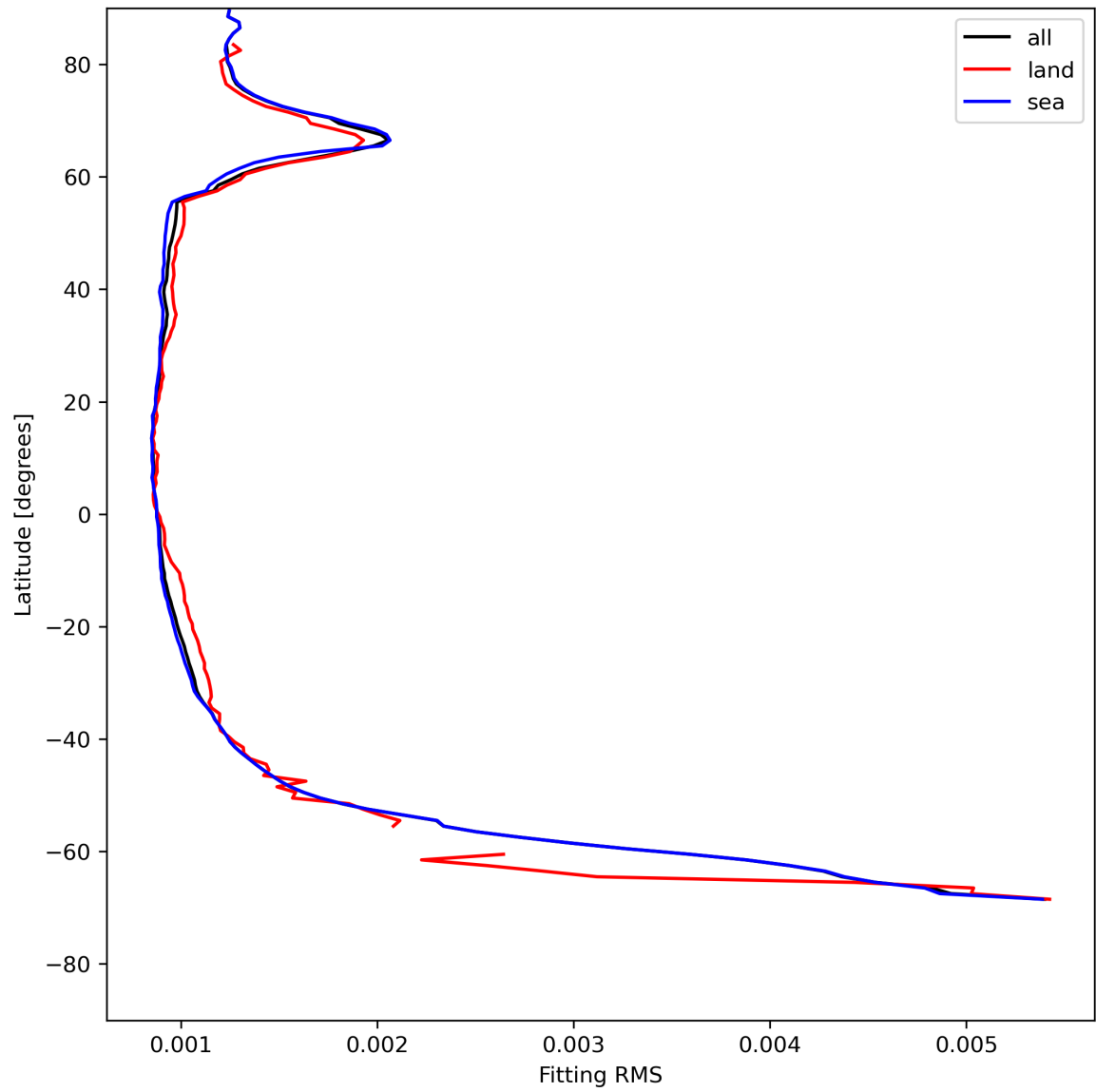
Figure 16: Zonal average of “Fitting RMS” for 2024-07-19 to 2024-07-21.
