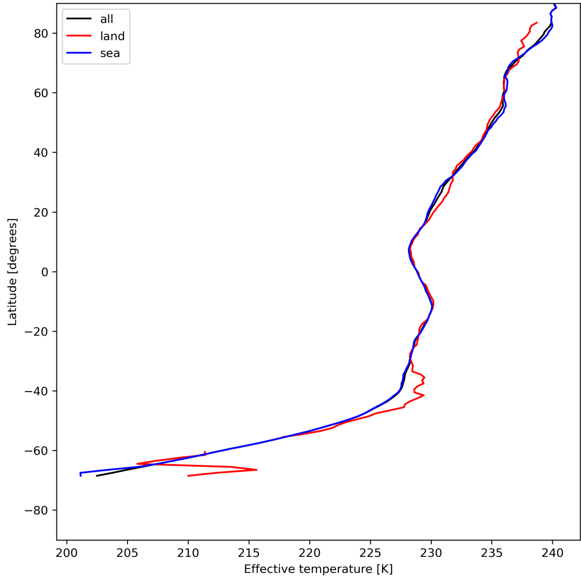
Figure 17: Zonal average of "Effective temperature" for 2024-07-19 to 2024-07-21.
