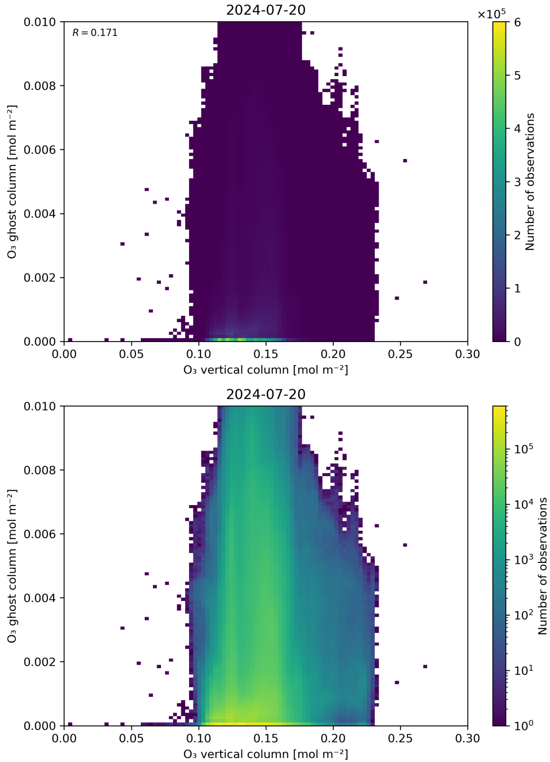
Figure 40: Scatter density plot of “O 3 vertical column” against “O 3 ghost column” for 2024-07-19 to 2024-07-21.
