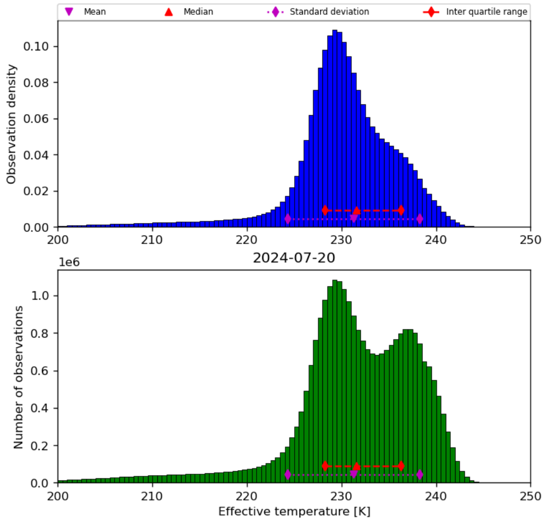
Figure 24: Histogram of “Effective temperature” for 2024-07-19 to 2024-07-21
