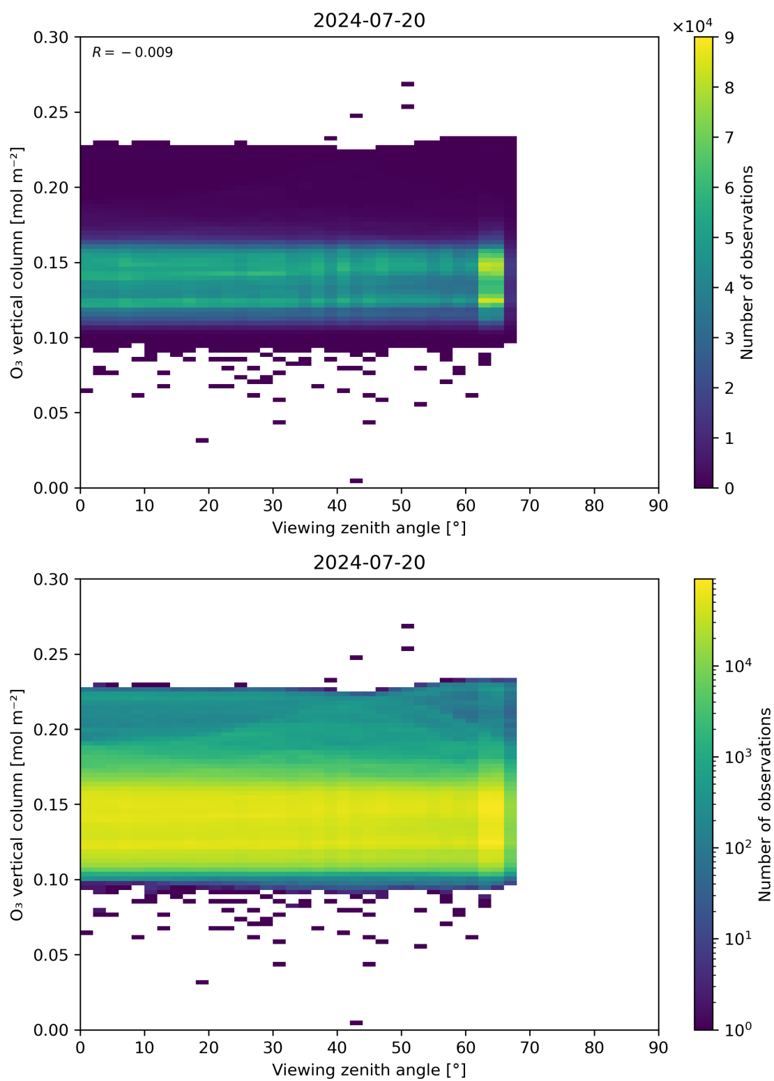
Figure 52: Scatter density plot of “Viewing zenith angle” against “O 3 vertical column” for 2024-07-19 to 2024-07-21.
