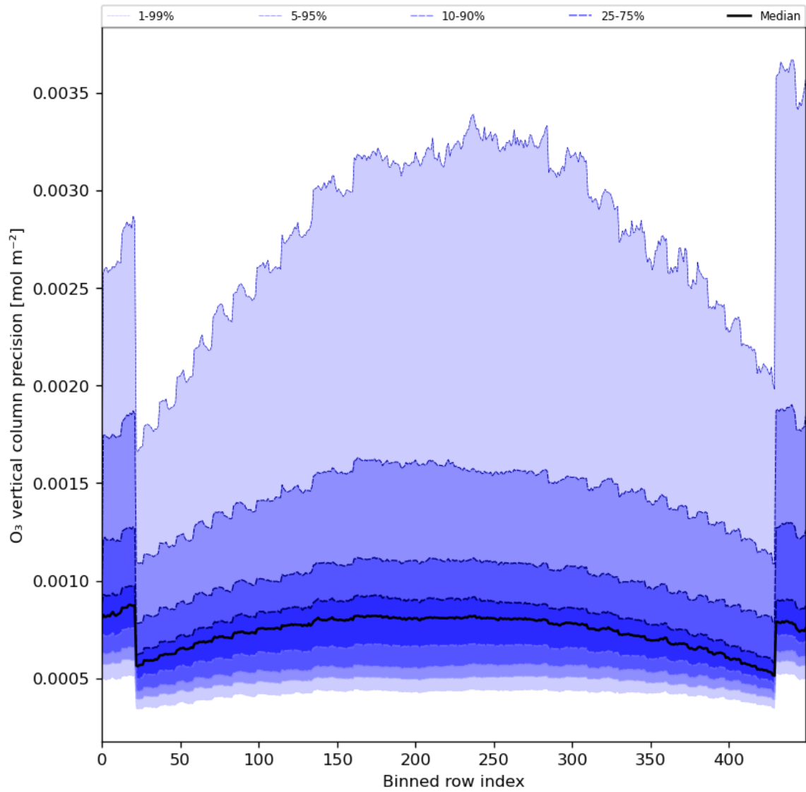
Figure 29: Along track statistics of “O 3 vertical column precision” for 2024-07-19 to 2024-07-21
