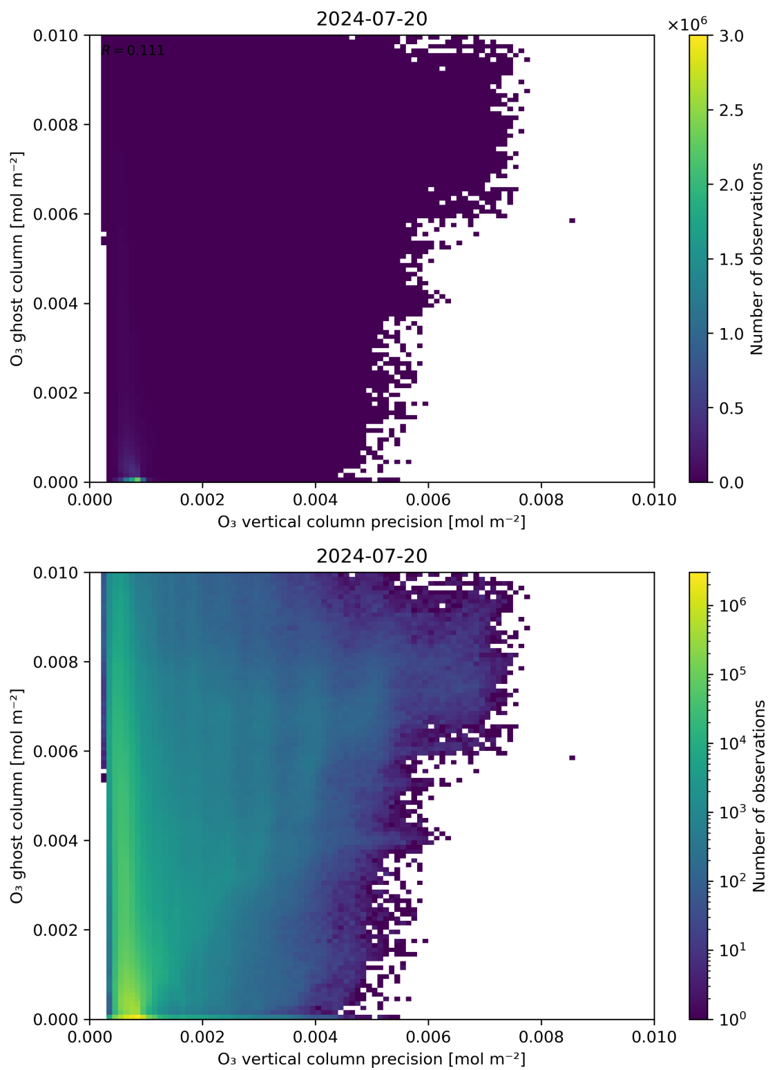
Figure 43: Scatter density plot of “ \text{O}_3 vertical column precision” against “ \text{O}_3 ghost column” for 2024-07-19 to 2024-07-21.
