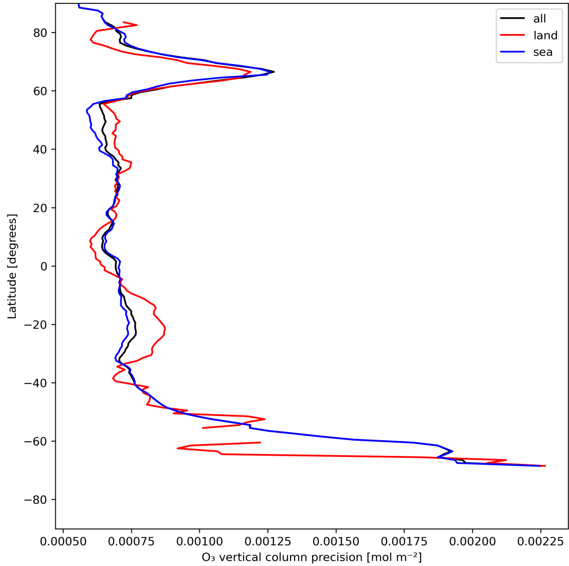
Figure 15: Zonal average of “O 3 vertical column precision” for 2024-07-19 to 2024-07-21.
