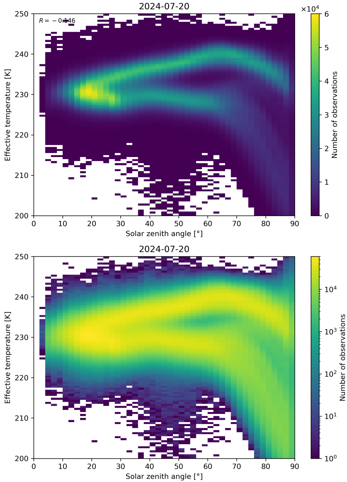
Figure 45: Scatter density plot of “Solar zenith angle” against “Effective temperature” for 2024-07-19 to 2024-07-21.
