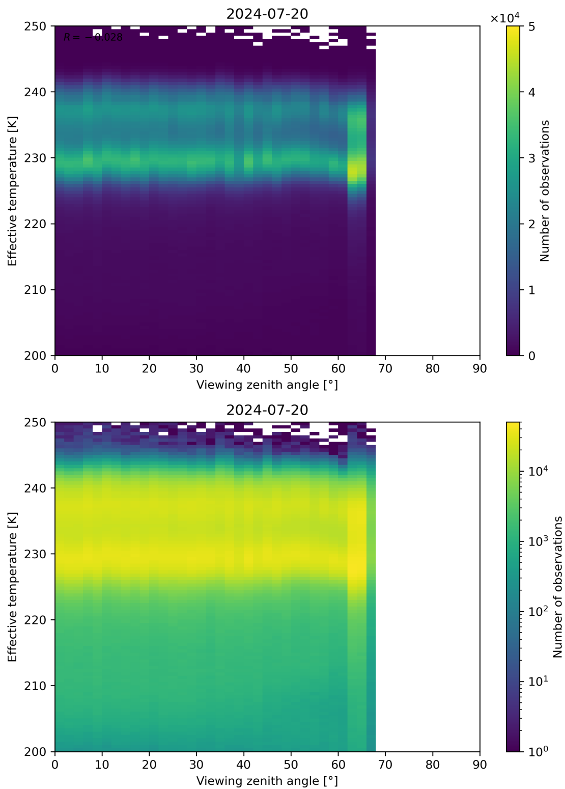
Figure 50: Scatter density plot of “Viewing zenith angle” against “Effective temperature” for 2024-07-19 to 2024-07-21.
