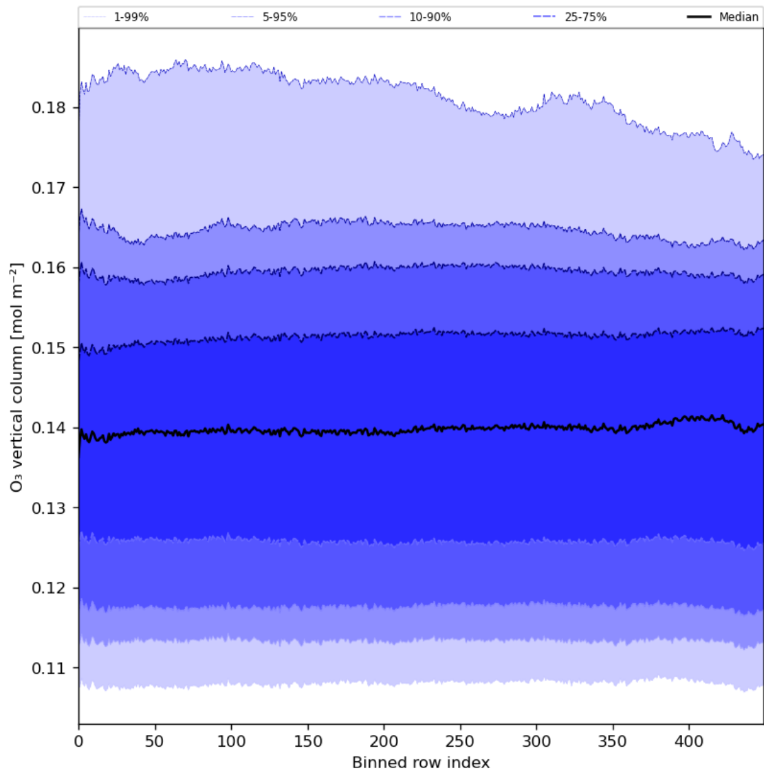
Figure 28: Along track statistics of “O 3 vertical column” for 2024-07-19 to 2024-07-21
