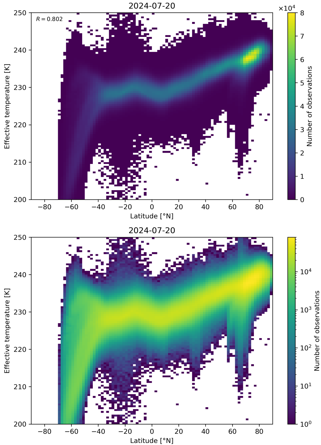
Figure 34: Scatter density plot of “Latitude” against “Effective temperature” for 2024-07-19 to 2024-07-21.
