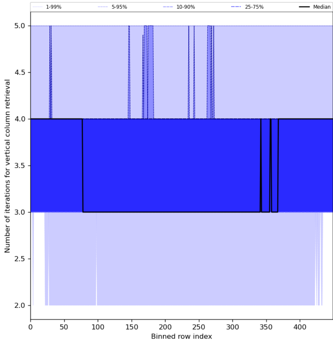
Figure 33: Along track statistics of “Number of iterations for vertical column retrieval” for 2024-07-19 to 2024-07-21
