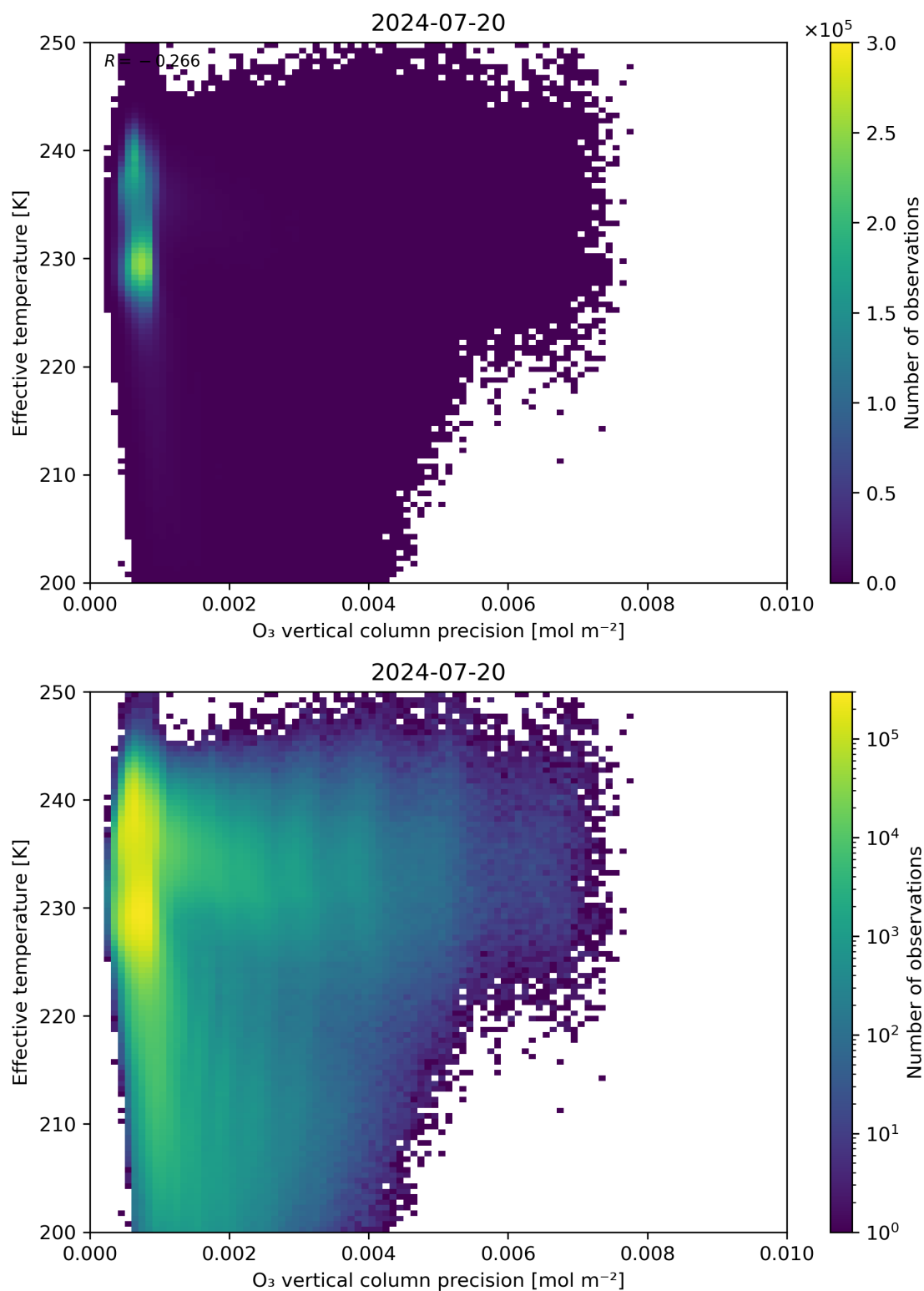
Figure 42: Scatter density plot of “O 3 vertical column precision” against “Effective temperature” for 2024-07-19 to 2024-07-21.
