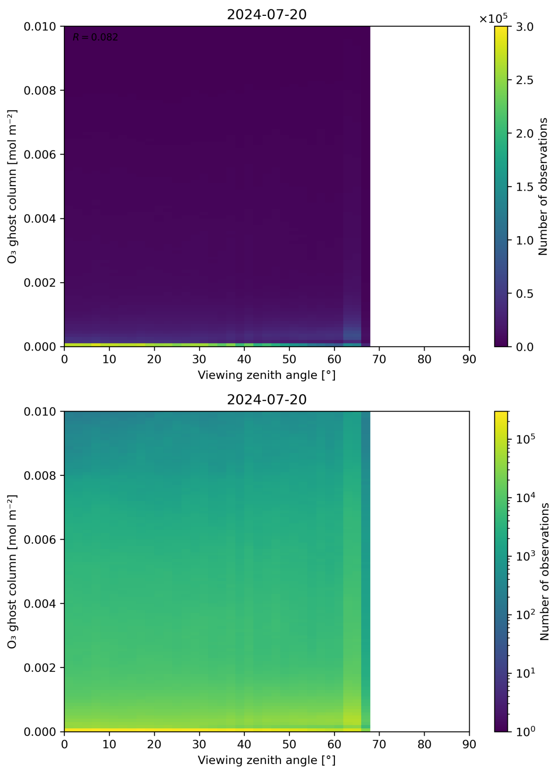
Figure 51: Scatter density plot of “Viewing zenith angle” against “O 3 ghost column” for 2024-07-19 to 2024-07-21.
