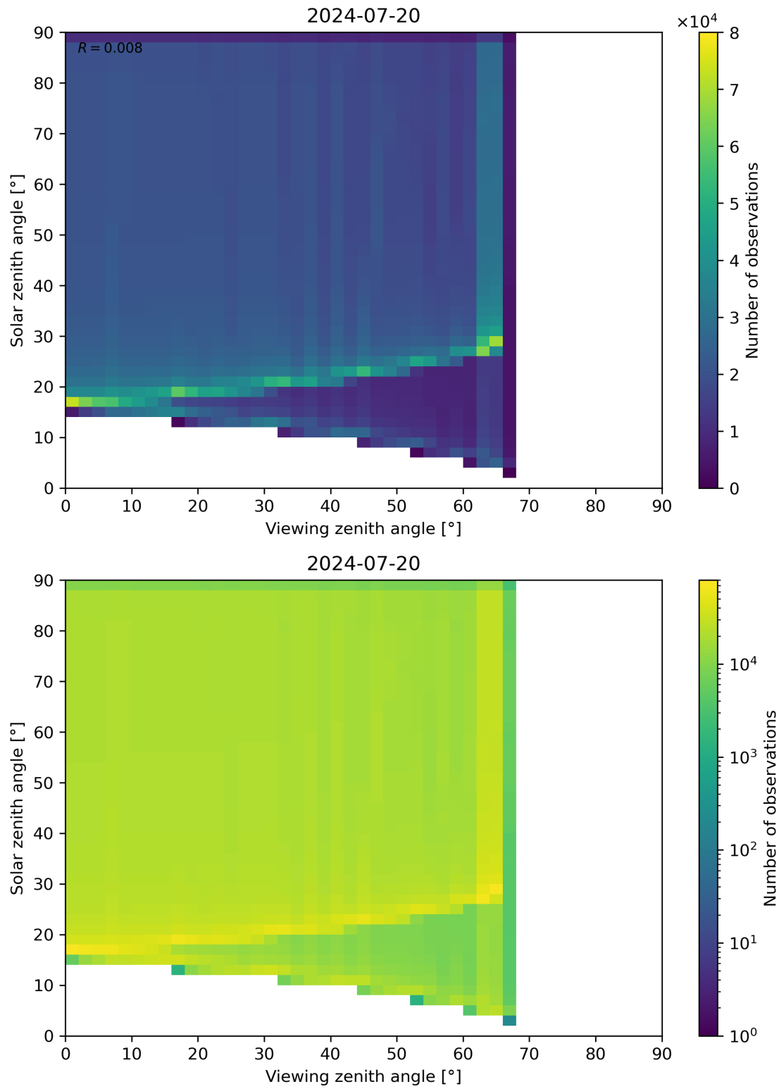
Figure 54: Scatter density plot of “Viewing zenith angle” against “Solar zenith angle” for 2024-07-19 to 2024-07-21.
