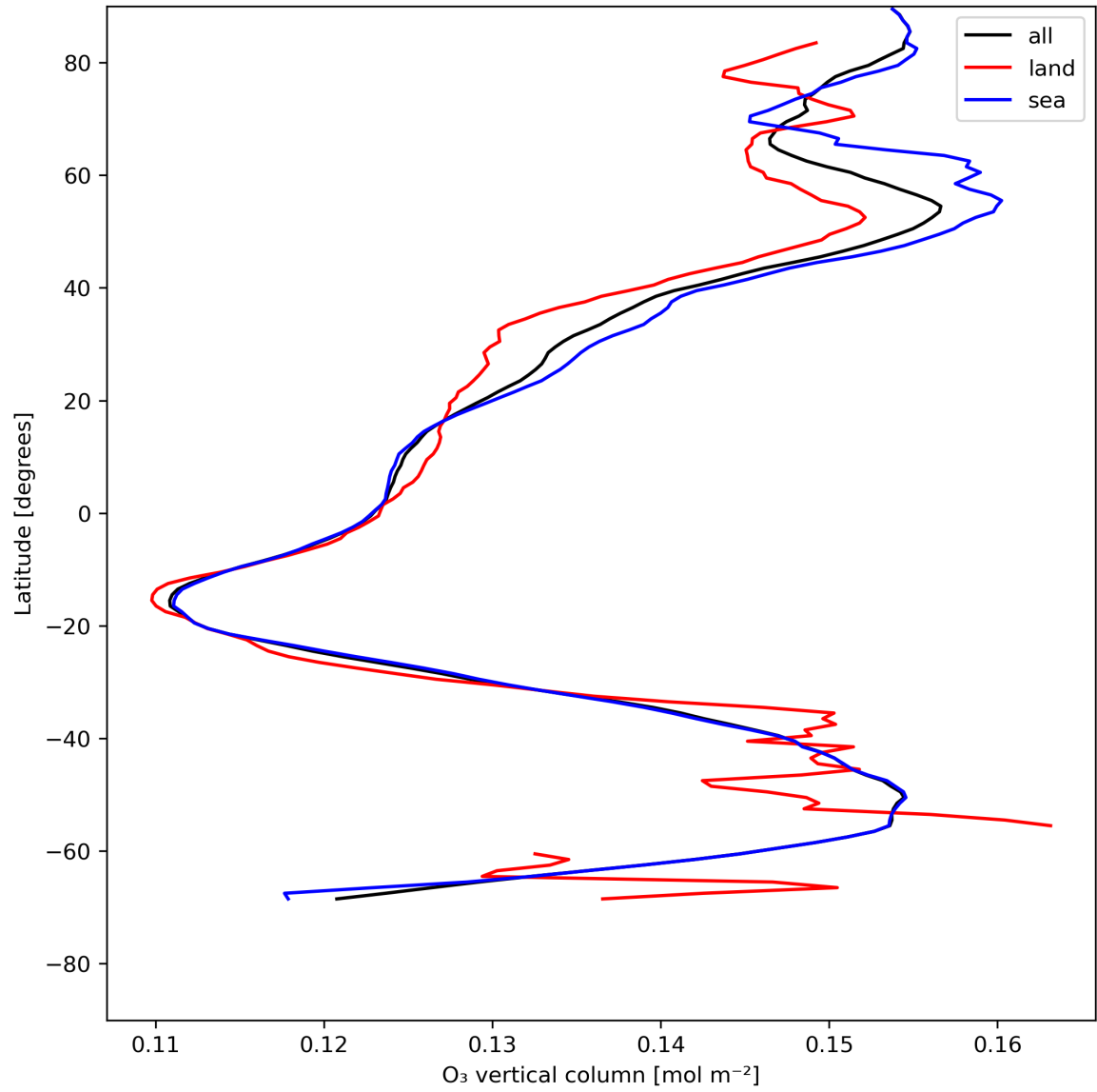
Figure 14: Zonal average of “O 3 vertical column” for 2024-07-19 to 2024-07-21.
