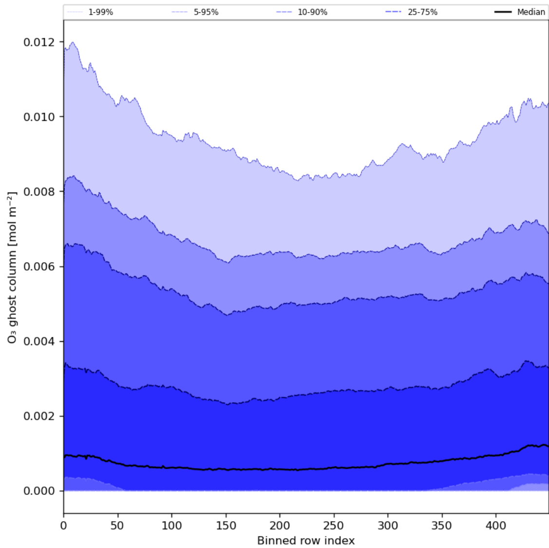
Figure 32: Along track statistics of “O 3 ghost column” for 2024-07-19 to 2024-07-21
