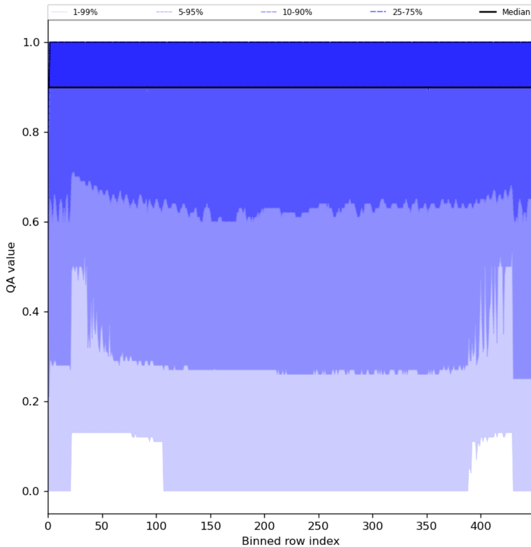
Figure 27: Along track statistics of “QA value” for 2024-07-19 to 2024-07-21
