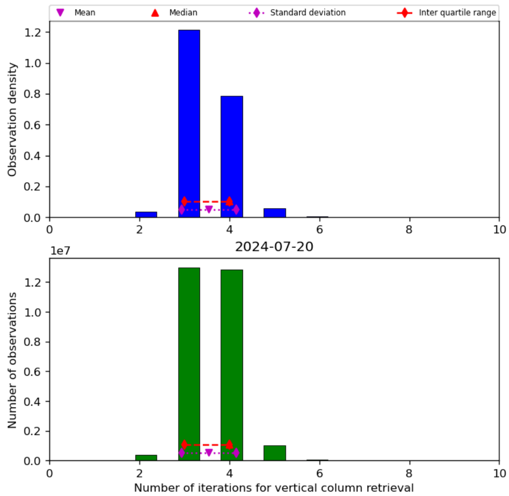
Figure 26: Histogram of “Number of iterations for vertical column retrieval” for 2024-07-19 to 2024-07-21
