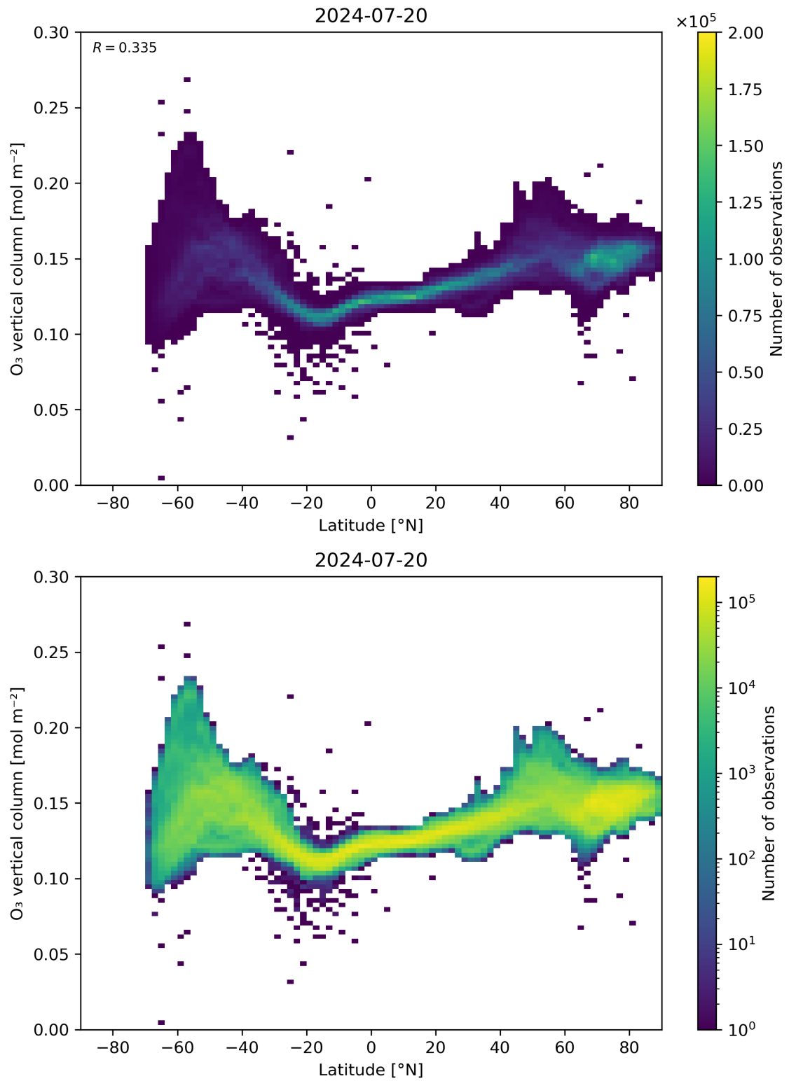
Figure 36: Scatter density plot of “Latitude” against “O 3 vertical column” for 2024-07-19 to 2024-07-21.
