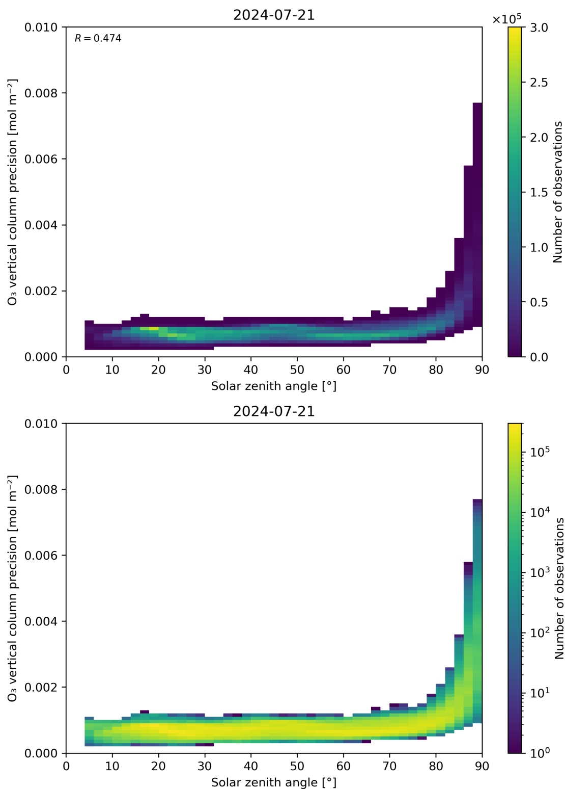
Figure 48: Scatter density plot of “Solar zenith angle” against “O 3 vertical column precision” for 2024-07-21 to 2024-07-22.
