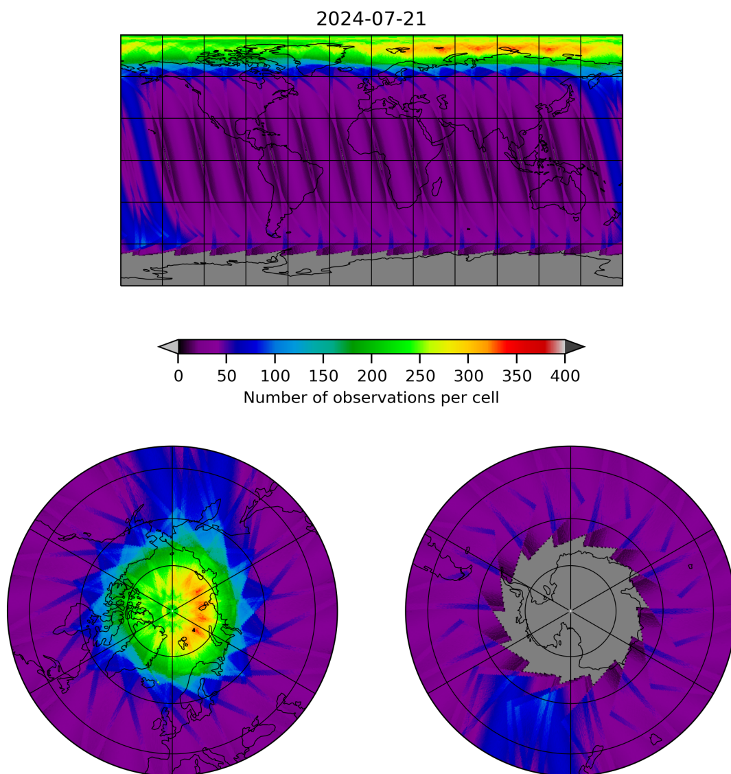
Figure 12: Map of the number of observations for 2024-07-21 to 2024-07-22
