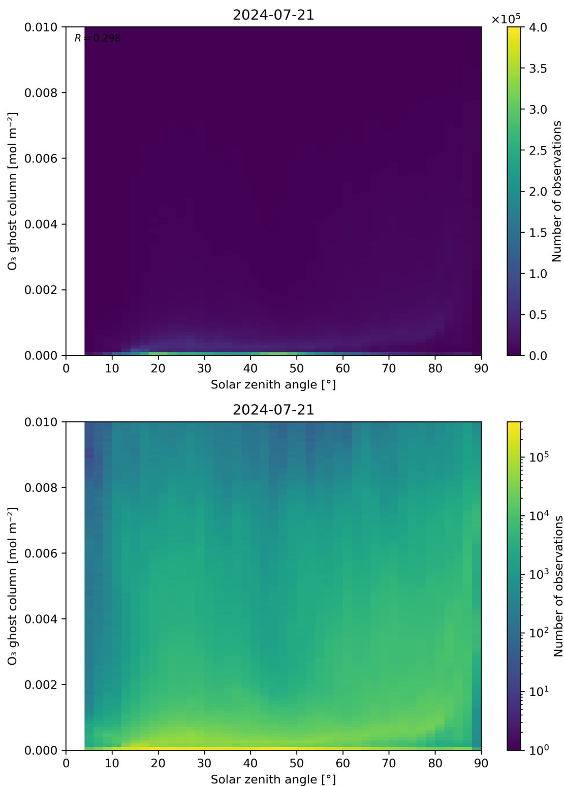
Figure 46: Scatter density plot of “Solar zenith angle” against “O 3 ghost column” for 2024-07-21 to 2024-07-22.
