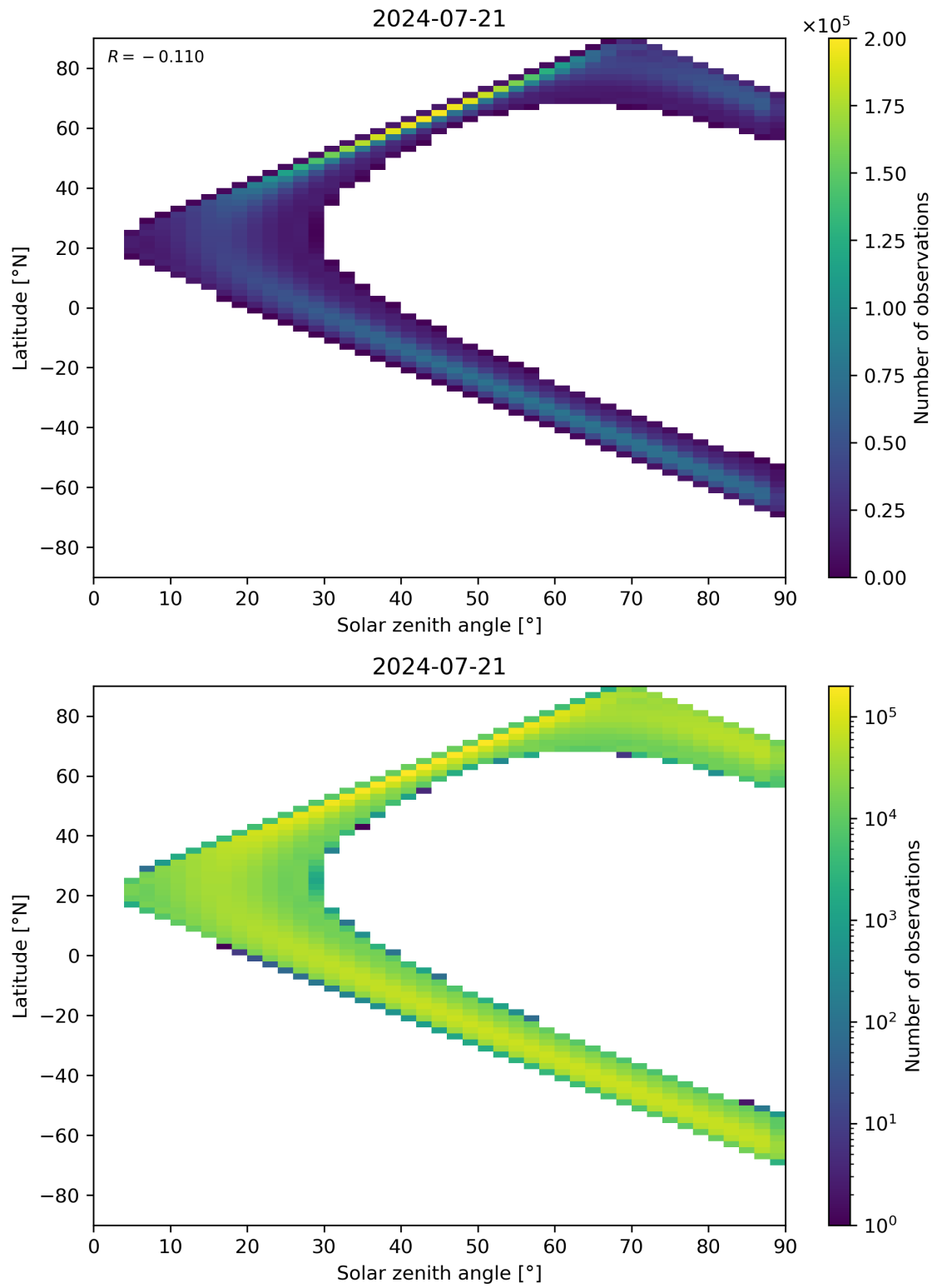
Figure 44: Scatter density plot of “Solar zenith angle” against “Latitude” for 2024-07-21 to 2024-07-22.
