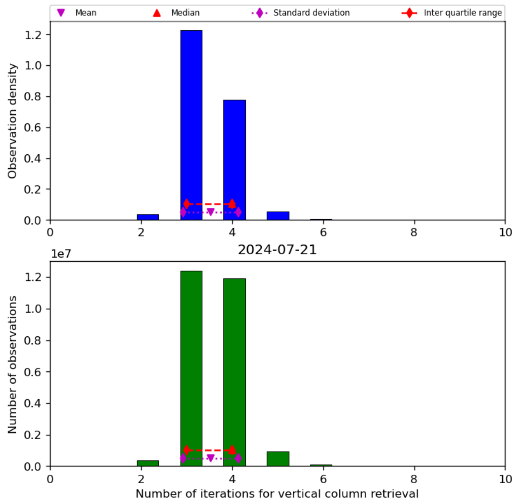
Figure 26: Histogram of “Number of iterations for vertical column retrieval” for 2024-07-21 to 2024-07-22
