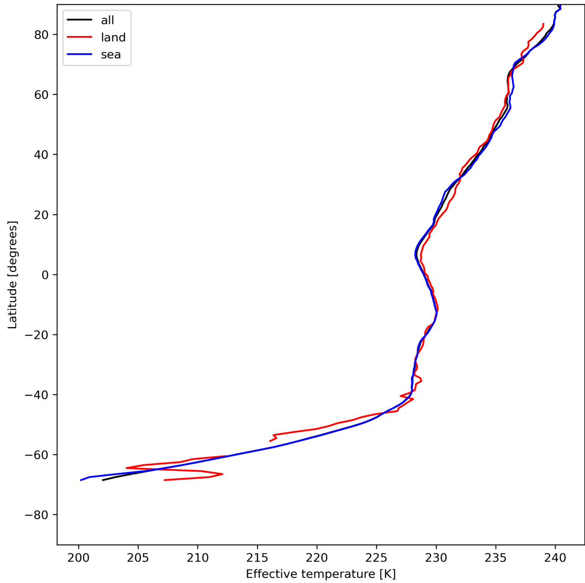
Figure 17: Zonal average of “Effective temperature” for 2024-07-21 to 2024-07-22.
