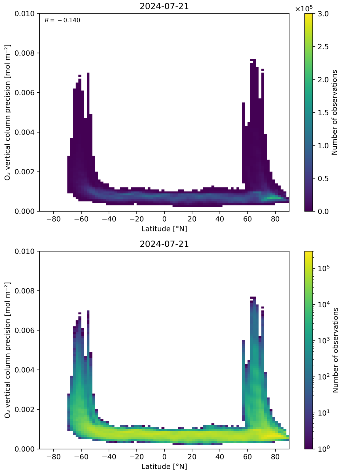
Figure 37: Scatter density plot of “Latitude” against “O 3 vertical column precision” for 2024-07-21 to 2024-07-22.
