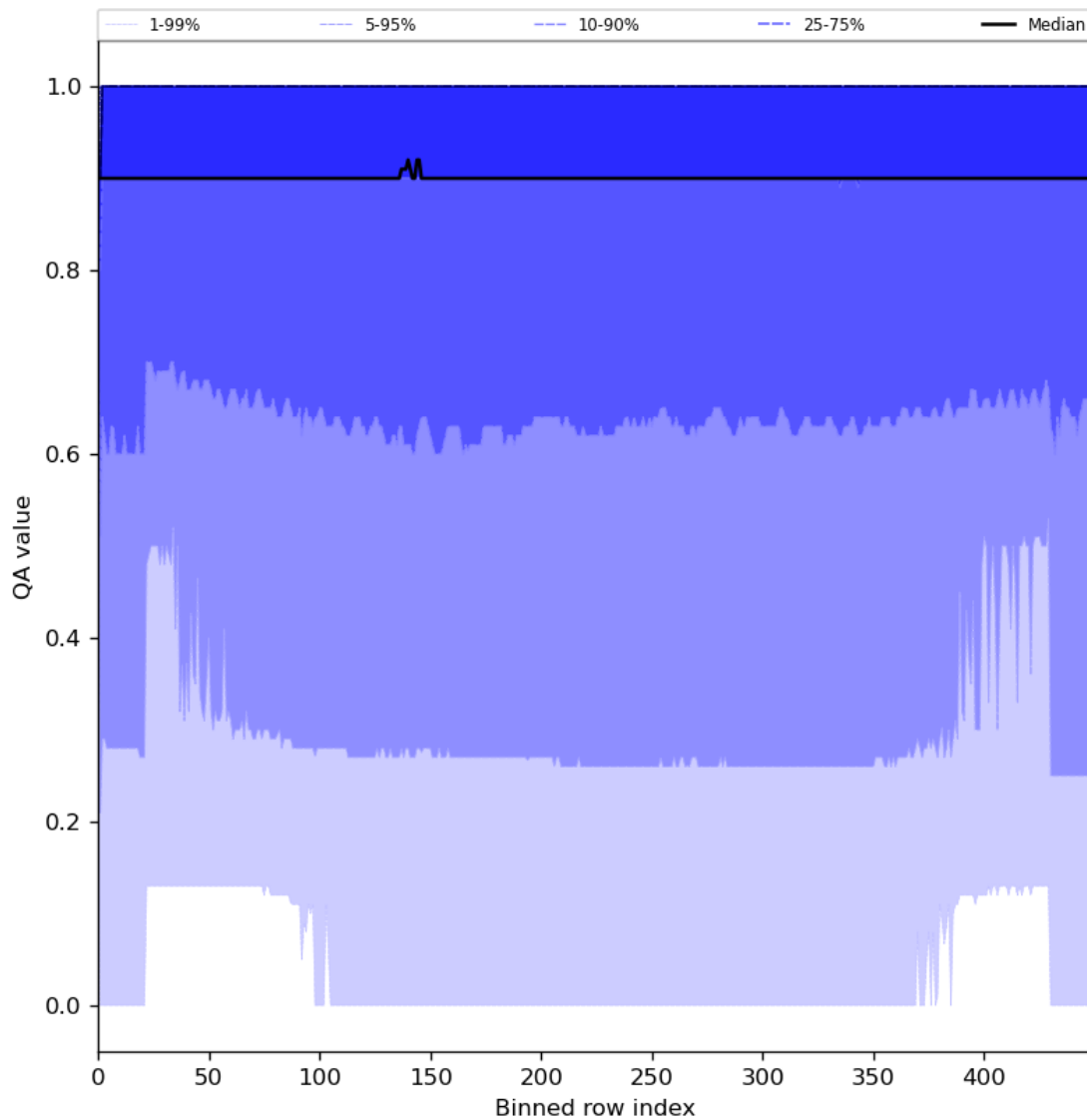
Figure 27: Along track statistics of “QA value” for 2024-07-21 to 2024-07-22
