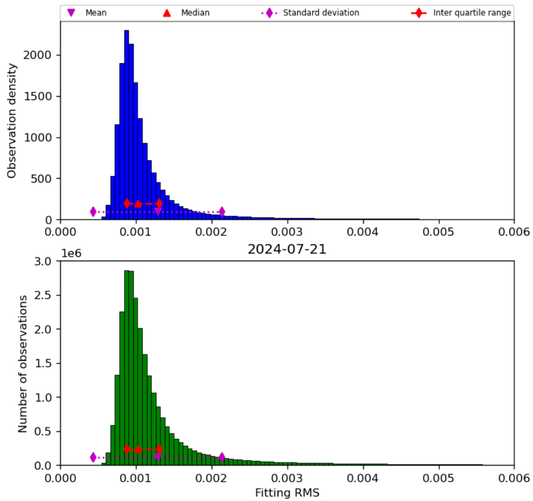
Figure 23: Histogram of “Fitting RMS” for 2024-07-21 to 2024-07-22
