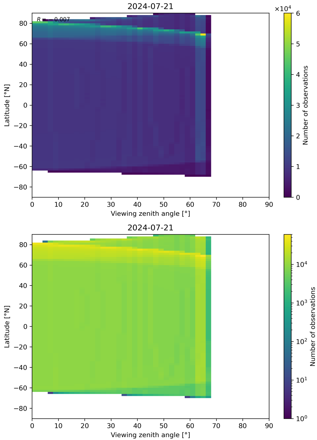
Figure 49: Scatter density plot of “Viewing zenith angle” against “Latitude” for 2024-07-21 to 2024-07-22.
