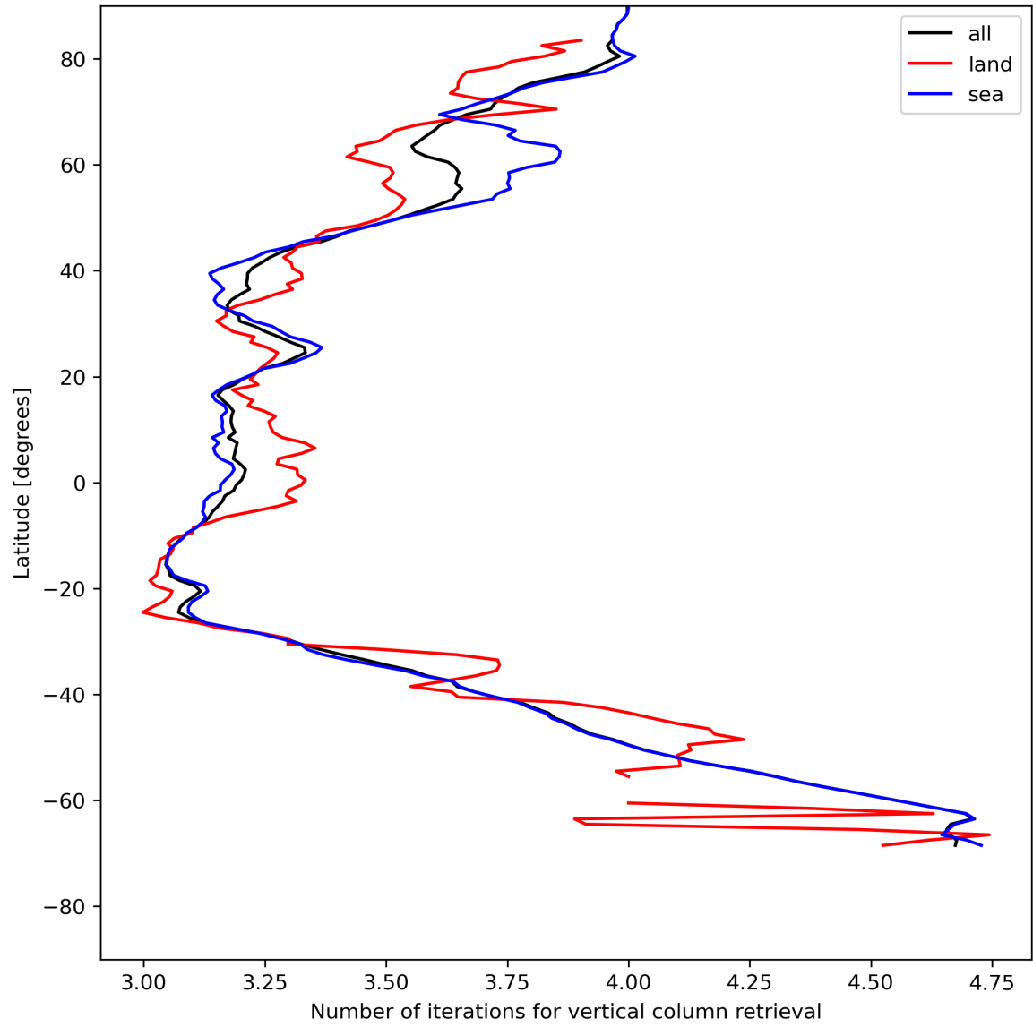
Figure 19: Zonal average of “Number of iterations for vertical column retrieval” for 2024-07-21 to 2024-07-22.
