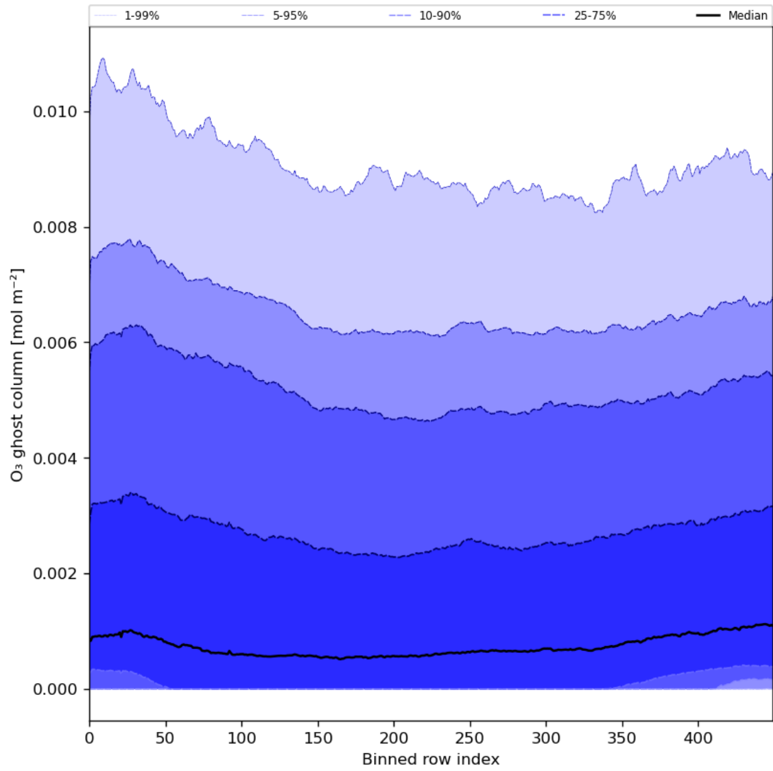
Figure 32: Along track statistics of “O 3 ghost column” for 2024-07-21 to 2024-07-22
