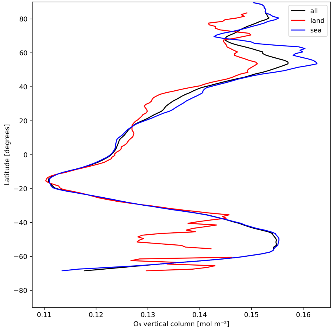
Figure 14: Zonal average of “O 3 vertical column” for 2024-07-21 to 2024-07-22.
