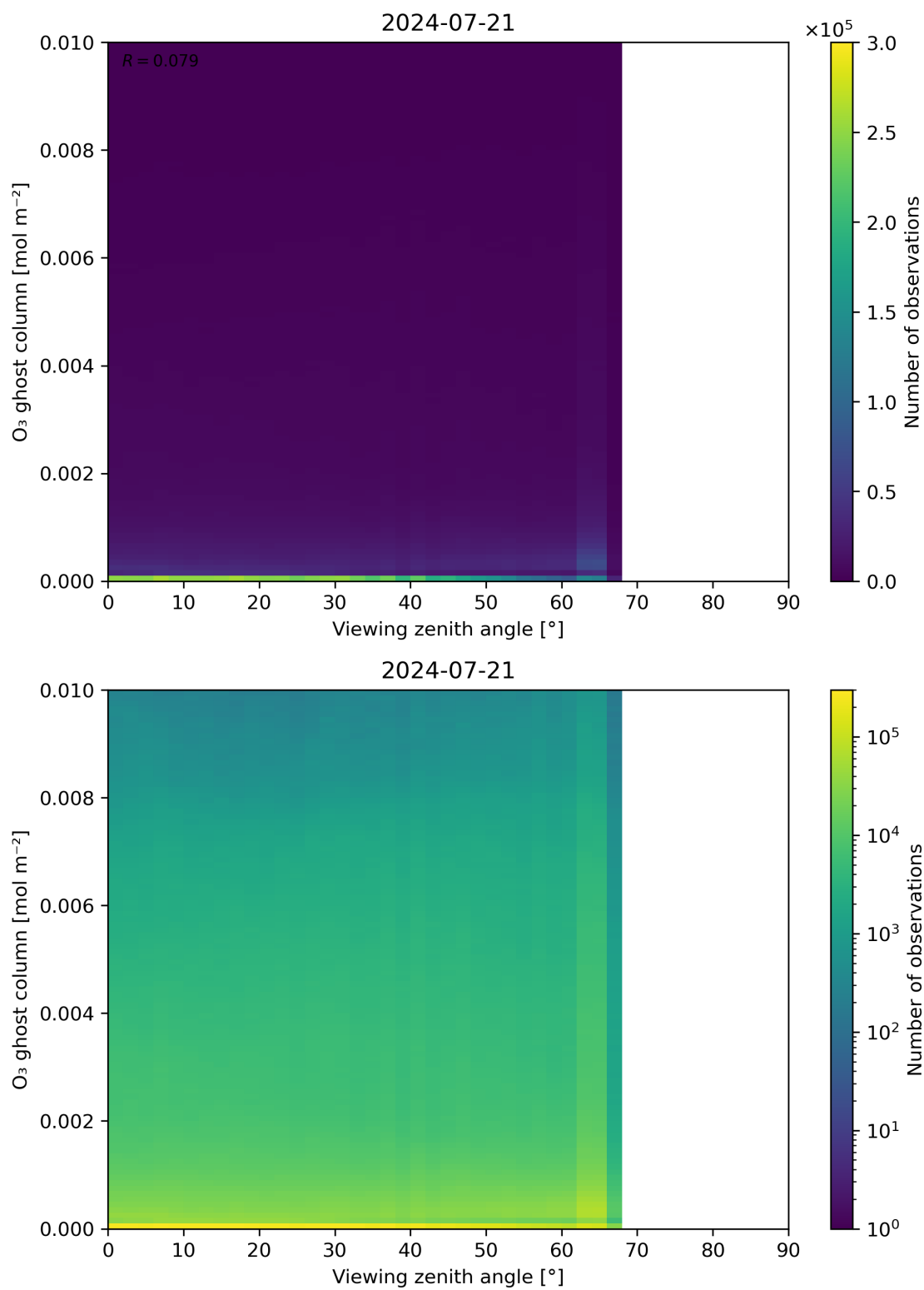
Figure 51: Scatter density plot of “Viewing zenith angle” against “O 3 ghost column” for 2024-07-21 to 2024-07-22.
