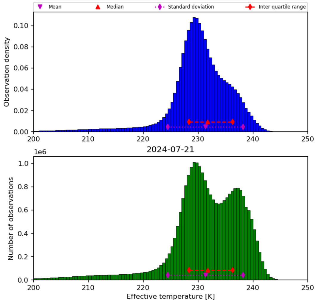
Figure 24: Histogram of “Effective temperature” for 2024-07-21 to 2024-07-22
