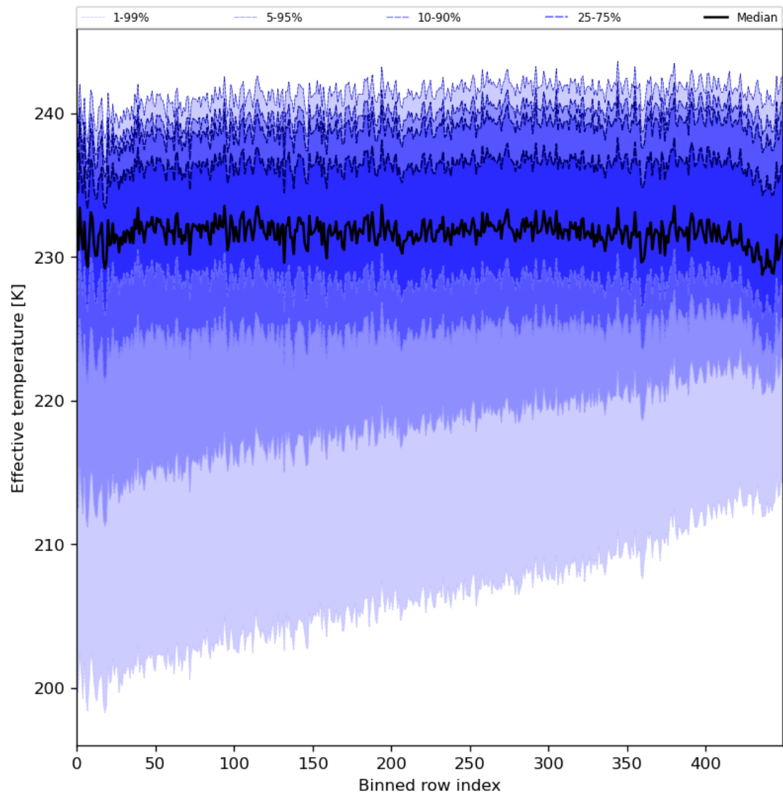
Figure 31: Along track statistics of “Effective temperature” for 2024-07-21 to 2024-07-22
