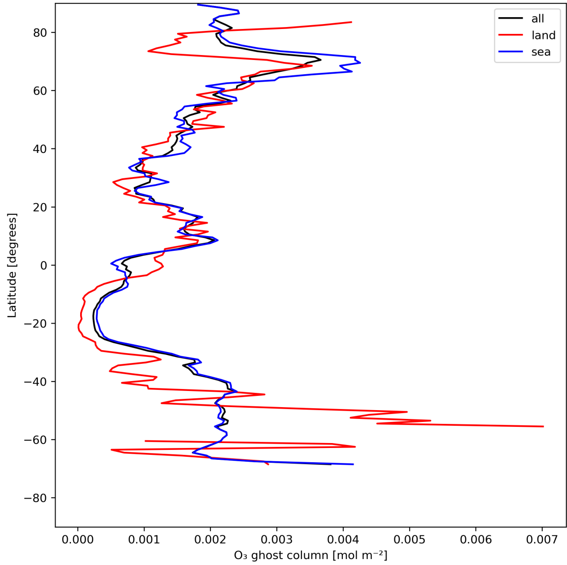
Figure 18: Zonal average of “O 3 ghost column” for 2024-07-21 to 2024-07-22.
