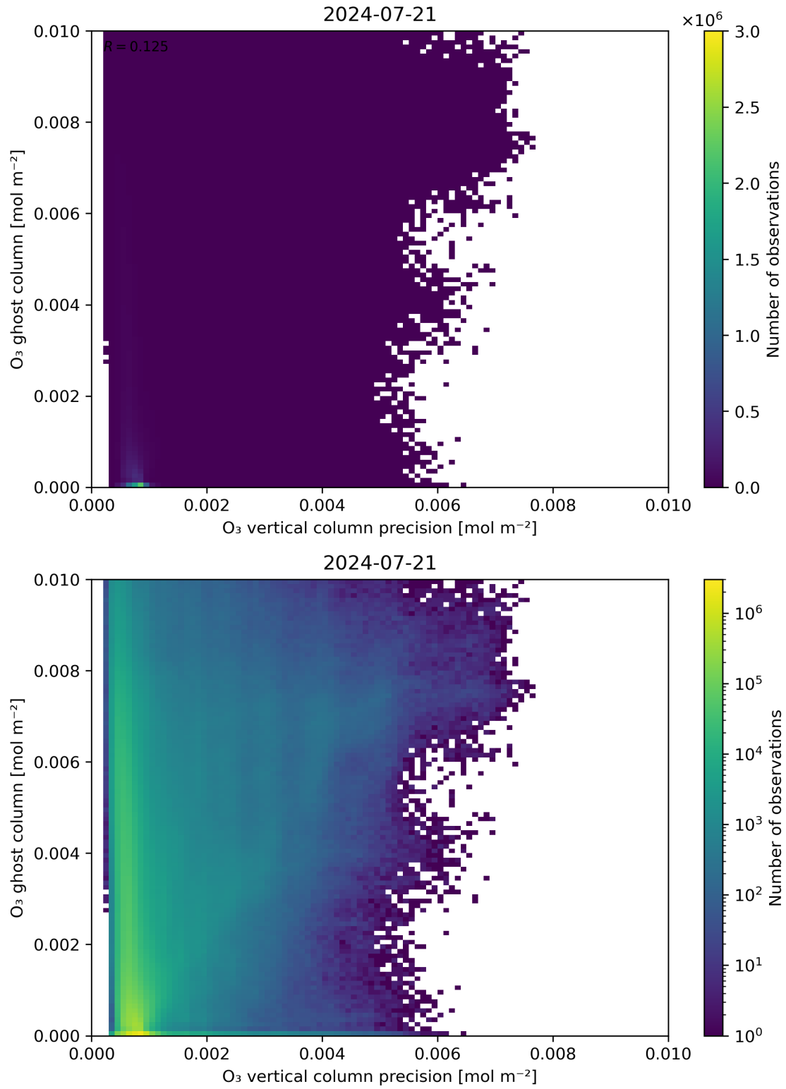
Figure 43: Scatter density plot of “ \text{O}_3 vertical column precision” against “ \text{O}_3 ghost column” for 2024-07-21 to 2024-07-22.
