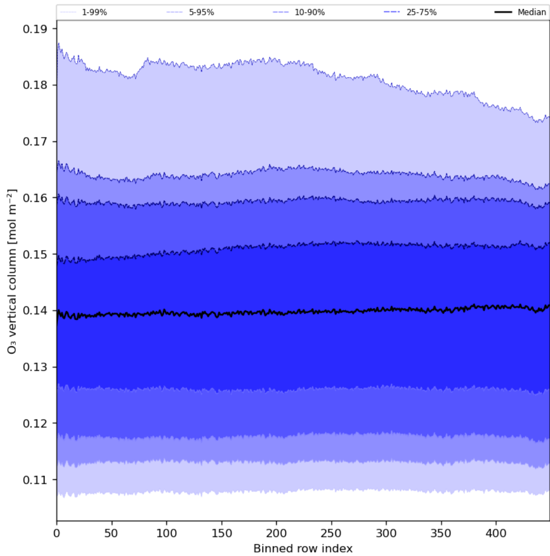
Figure 28: Along track statistics of “O 3 vertical column” for 2024-07-21 to 2024-07-22
