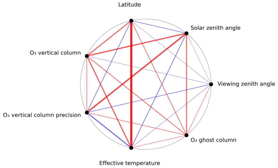
Figure 1: Map of correlation graph for 2024-07-21 to 2024-07-22.
