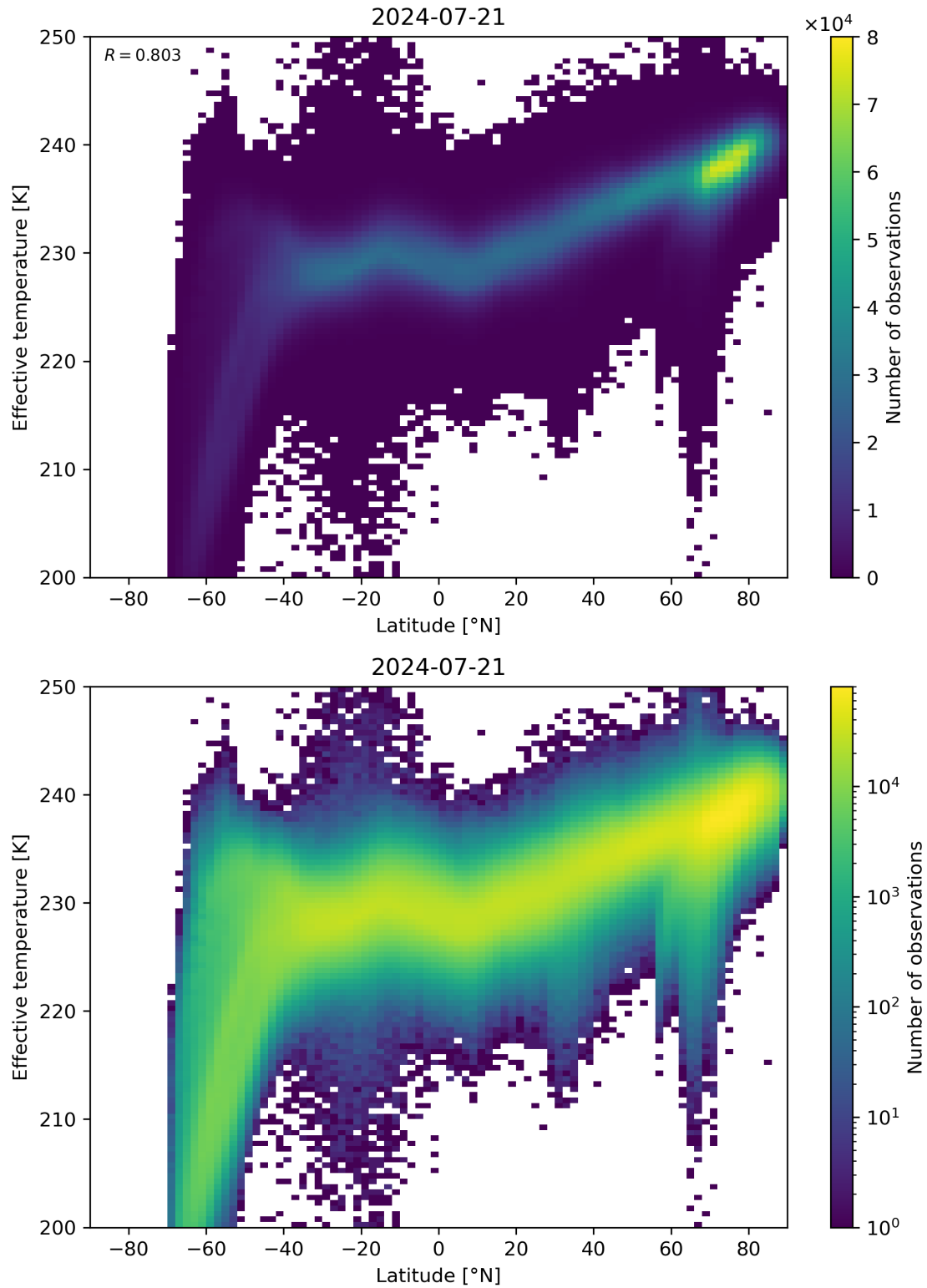
Figure 34: Scatter density plot of “Latitude” against “Effective temperature” for 2024-07-21 to 2024-07-22.
