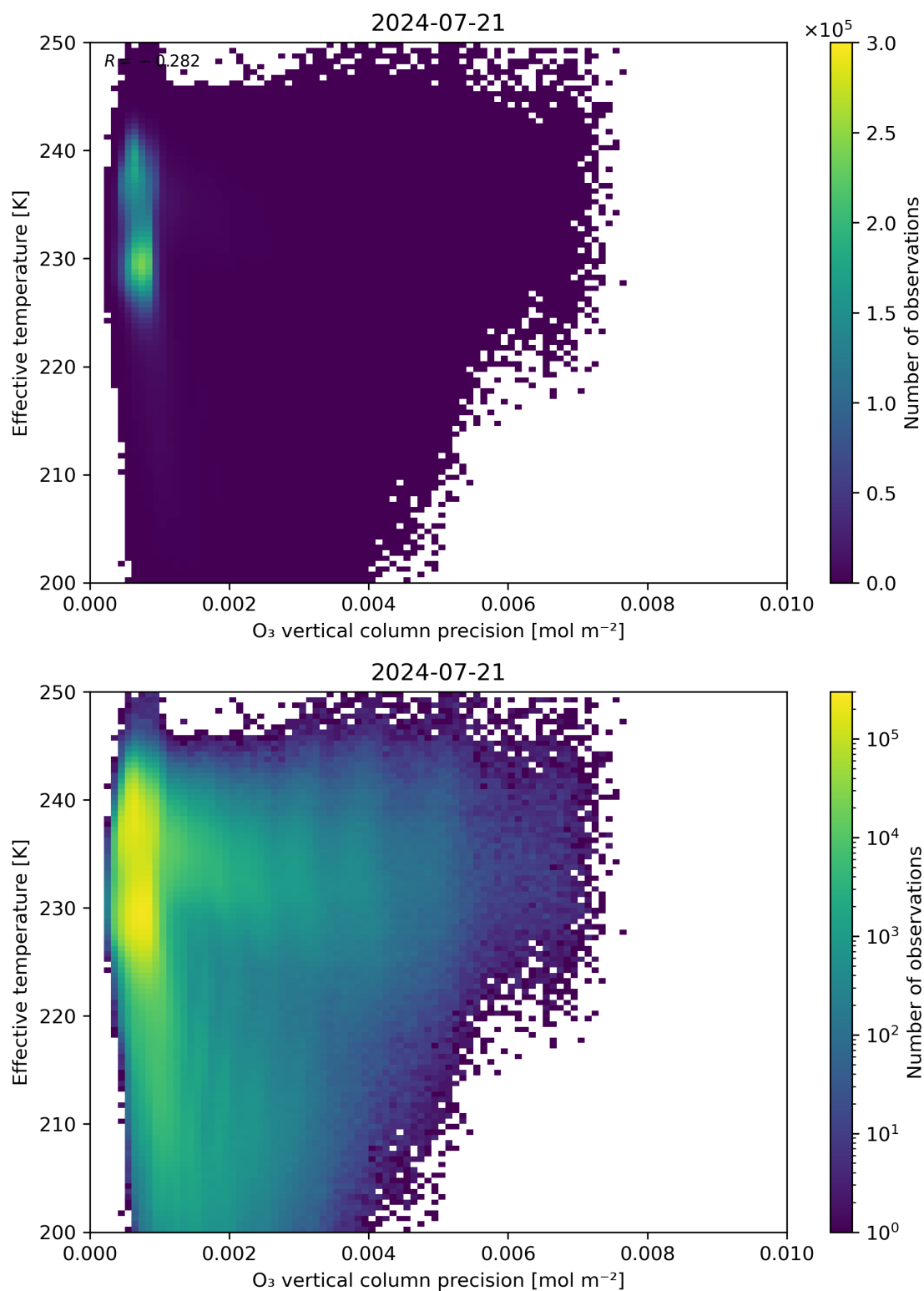
Figure 42: Scatter density plot of “O 3 vertical column precision” against “Effective temperature” for 2024-07-21 to 2024-07-22.
