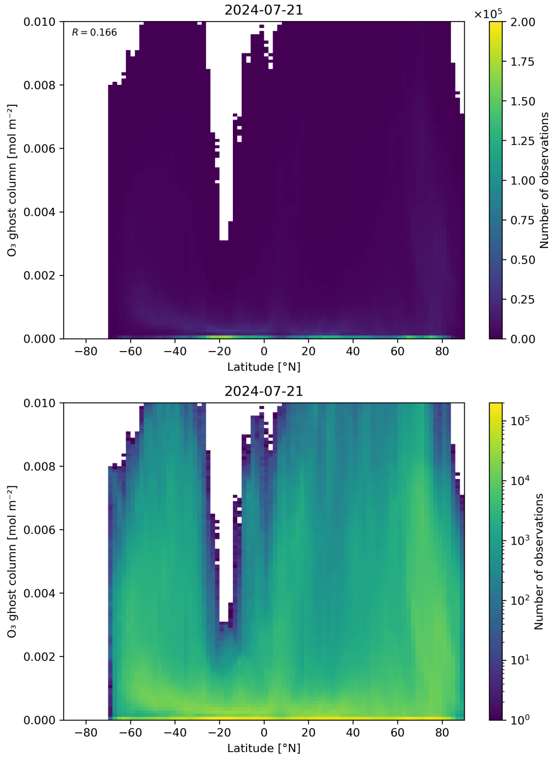
Figure 35: Scatter density plot of “Latitude” against “O 3 ghost column” for 2024-07-21 to 2024-07-22.
