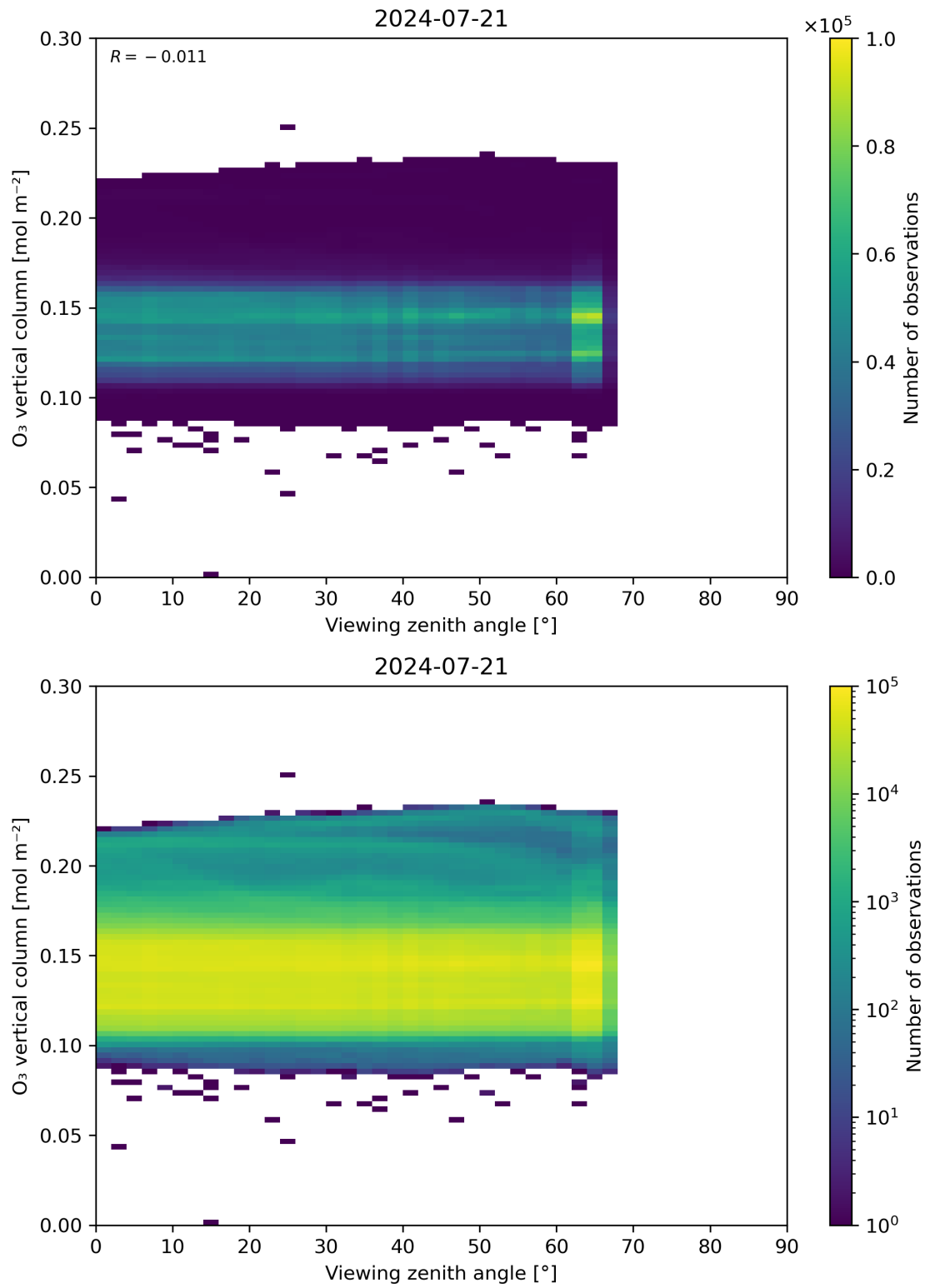
Figure 52: Scatter density plot of “Viewing zenith angle” against “O 3 vertical column” for 2024-07-21 to 2024-07-22.
