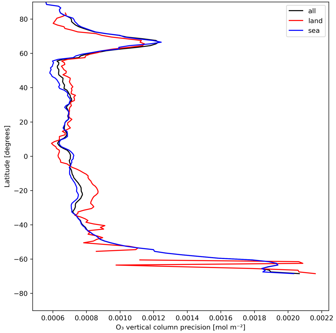
Figure 15: Zonal average of “O 3 vertical column precision” for 2024-07-21 to 2024-07-22.
