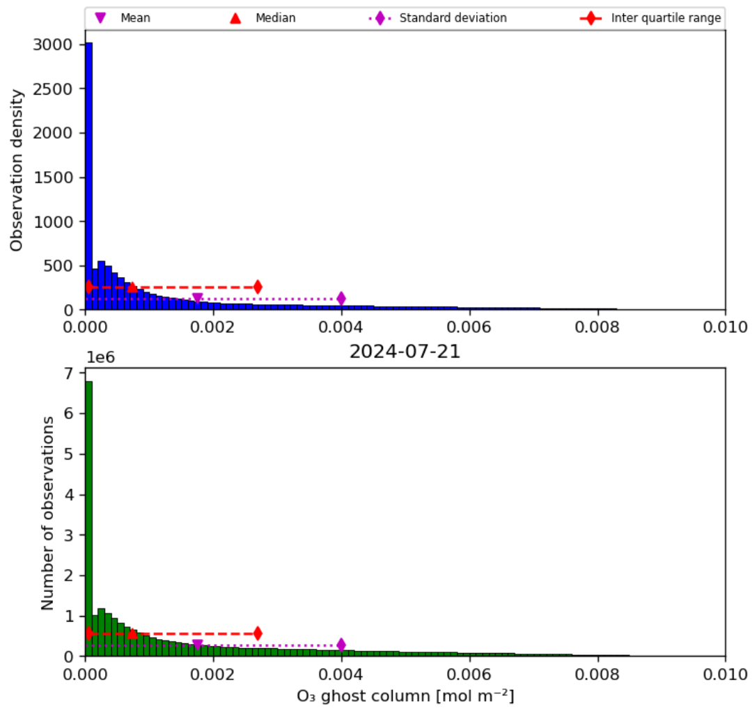
Figure 25: Histogram of “O 3 ghost column” for 2024-07-21 to 2024-07-22
