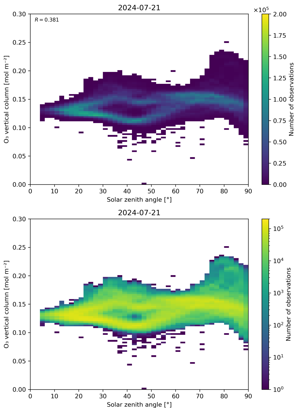
Figure 47: Scatter density plot of “Solar zenith angle” against “O 3 vertical column” for 2024-07-21 to 2024-07-22.
