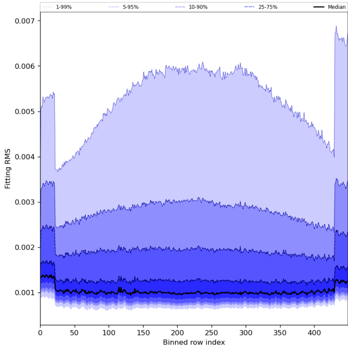
Figure 30: Along track statistics of “Fitting RMS” for 2024-07-21 to 2024-07-22
