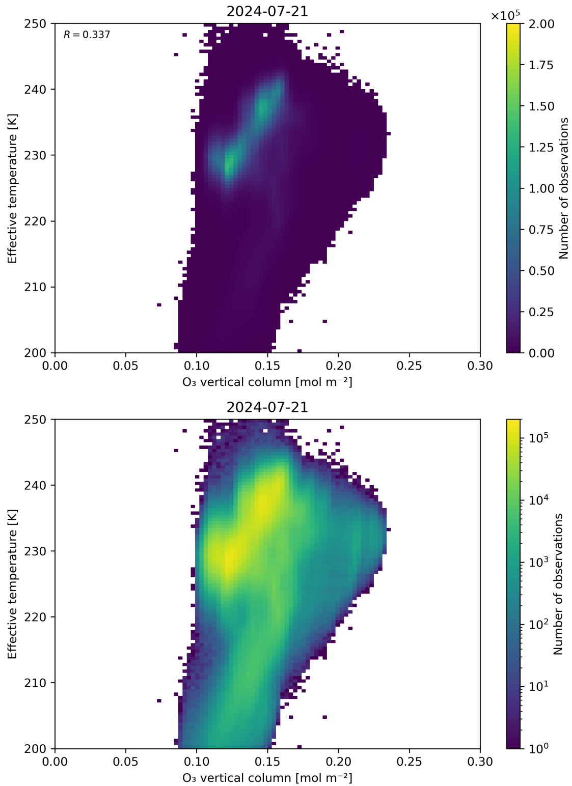
Figure 39: Scatter density plot of “O 3 vertical column” against “Effective temperature” for 2024-07-21 to 2024-07-22.
