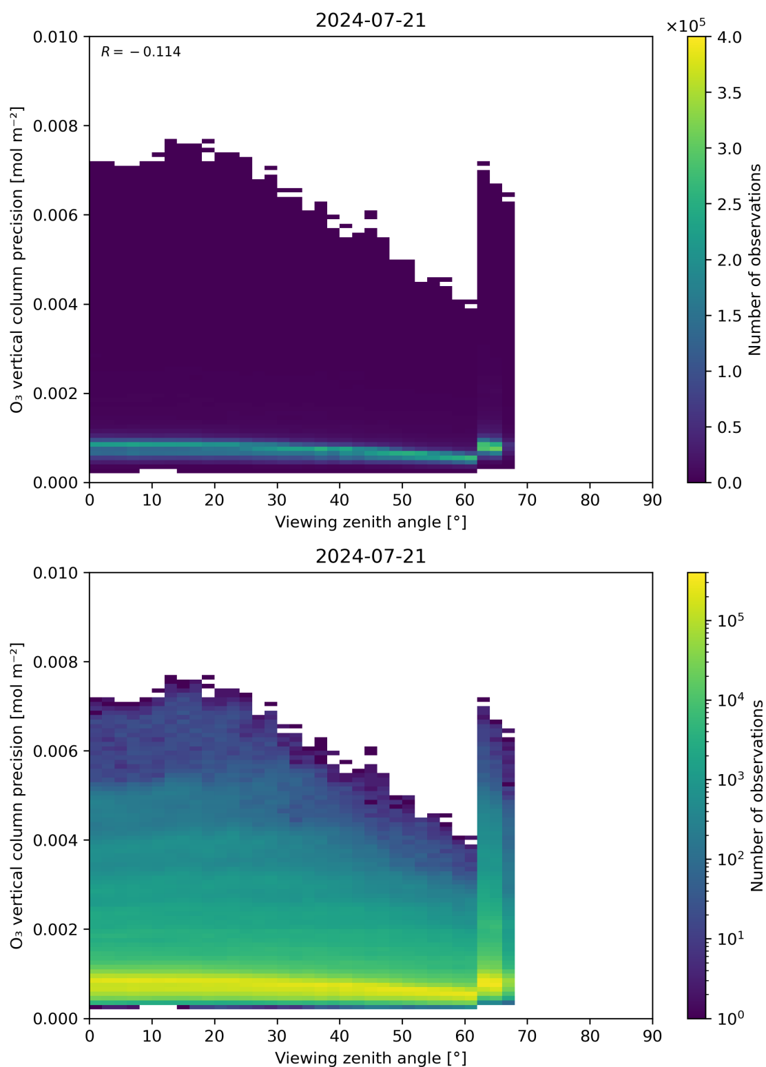
Figure 53: Scatter density plot of “Viewing zenith angle” against “O 3 vertical column precision” for 2024-07-21 to 2024-07-22.
