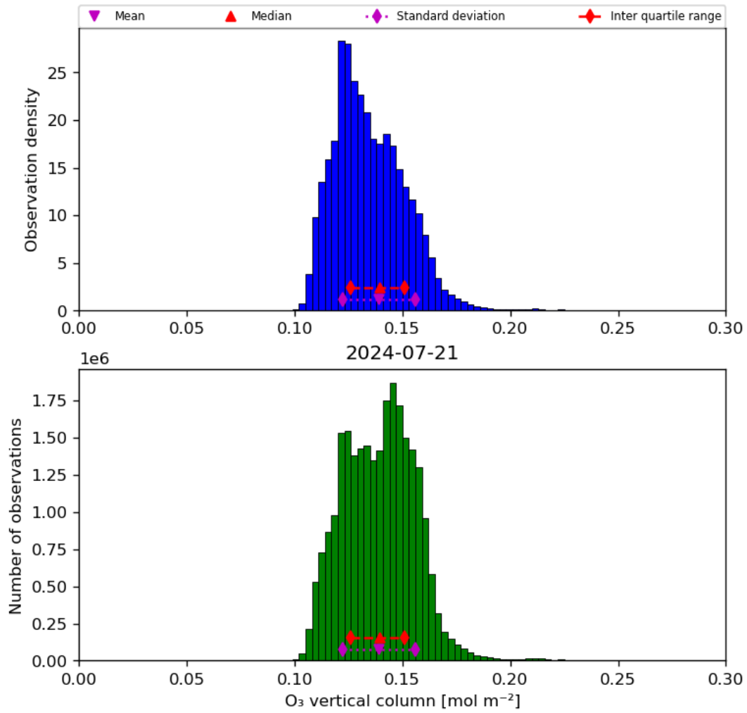
Figure 21: Histogram of “O 3 vertical column” for 2024-07-21 to 2024-07-22
