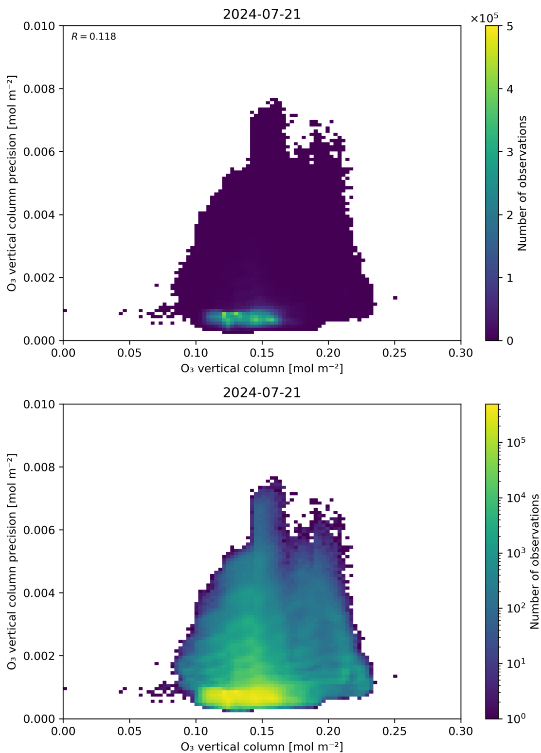
Figure 41: Scatter density plot of “O 3 vertical column” against “O 3 vertical column precision” for 2024-07-21 to 2024-07-22.
