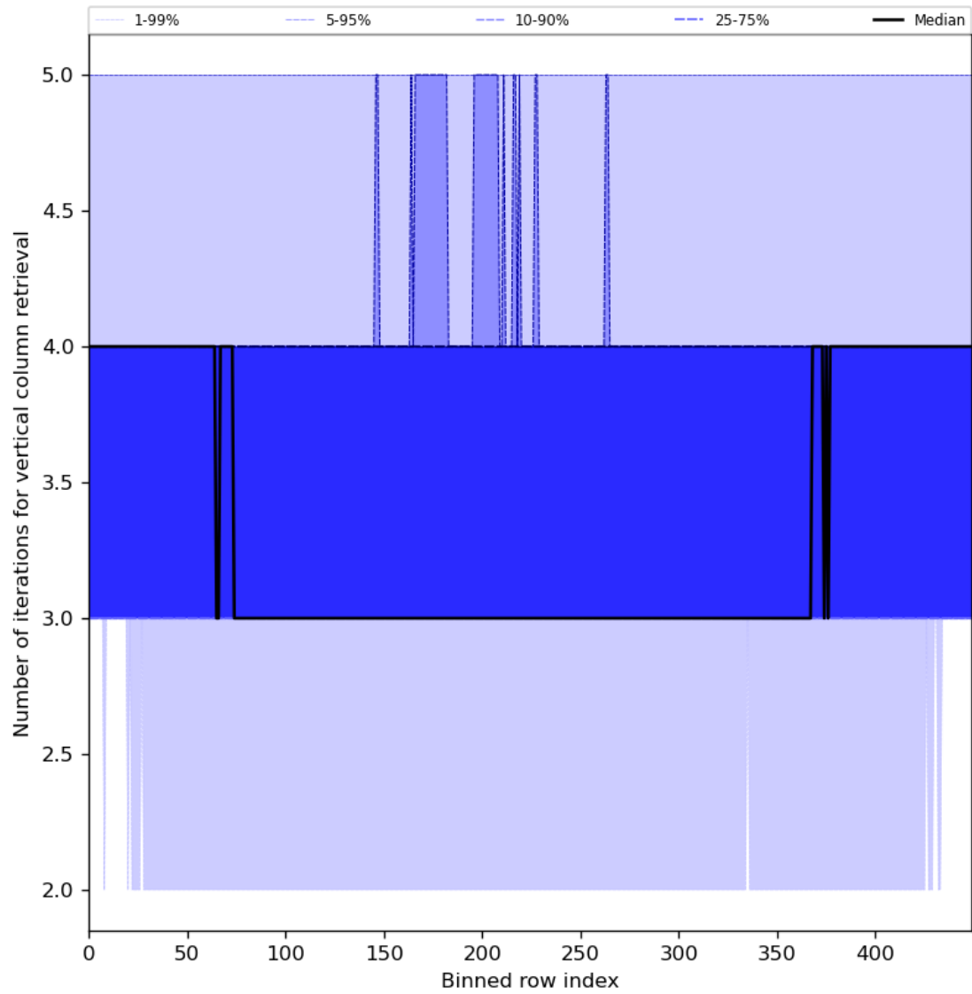
Figure 33: Along track statistics of “Number of iterations for vertical column retrieval” for 2024-07-21 to 2024-07-22
