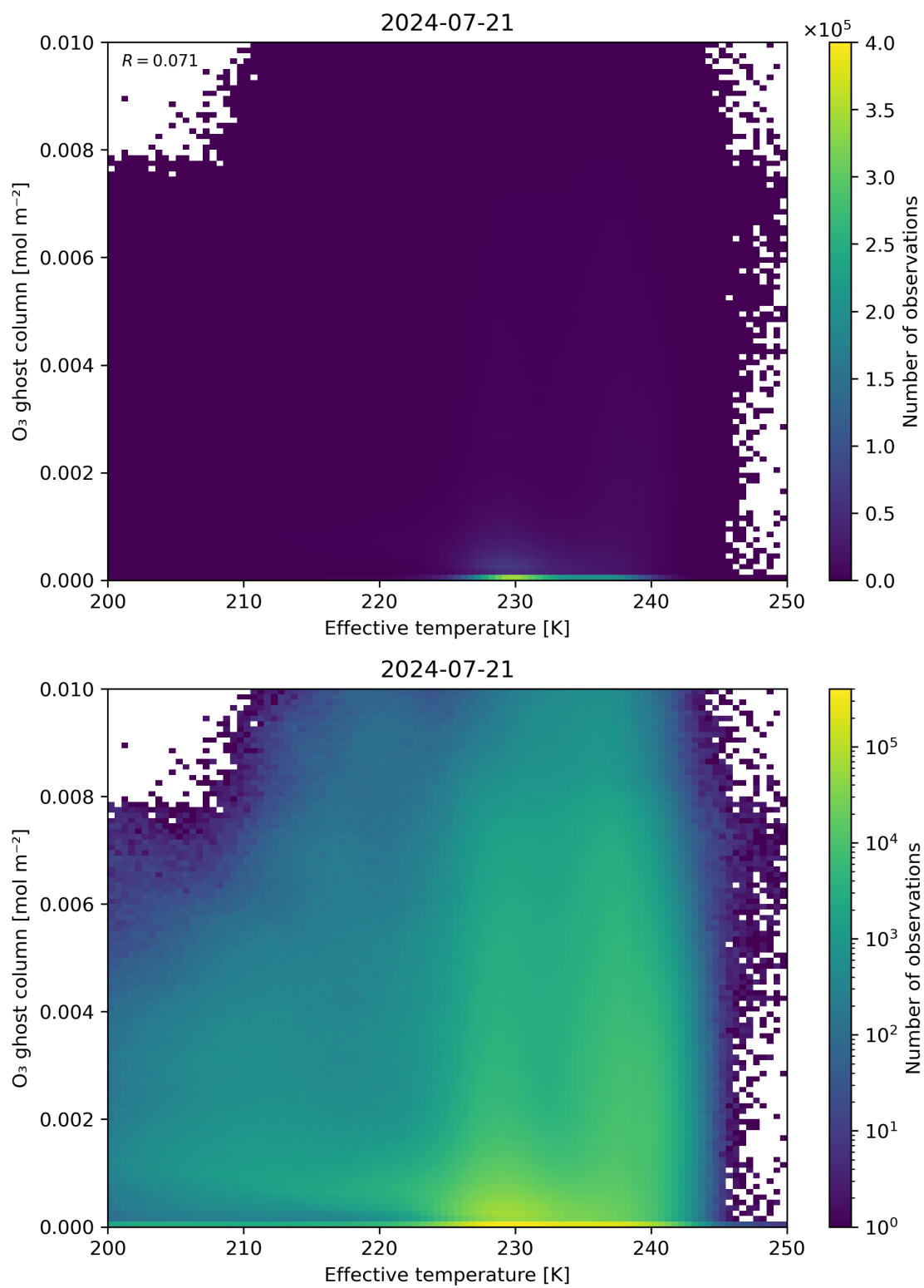
Figure 38: Scatter density plot of “Effective temperature” against “O 3 ghost column” for 2024-07-21 to 2024-07-22.
