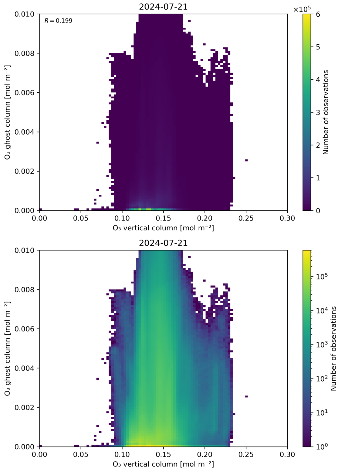
Figure 40: Scatter density plot of “O 3 vertical column” against “O 3 ghost column” for 2024-07-21 to 2024-07-22.
