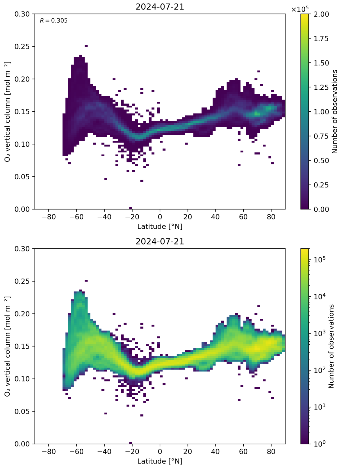
Figure 36: Scatter density plot of “Latitude” against “O 3 vertical column” for 2024-07-21 to 2024-07-22.
