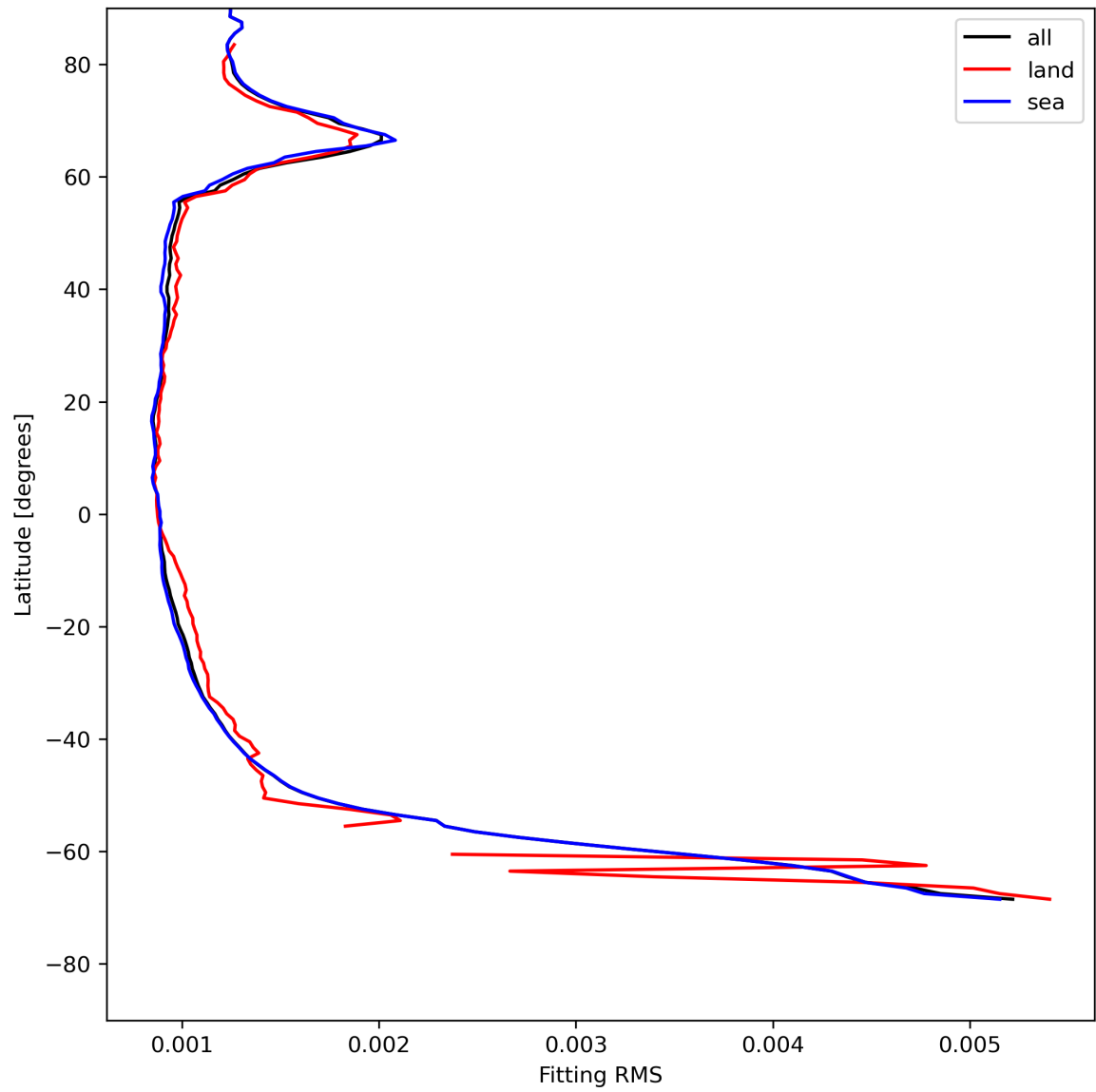
Figure 16: Zonal average of “Fitting RMS” for 2024-07-21 to 2024-07-22.
