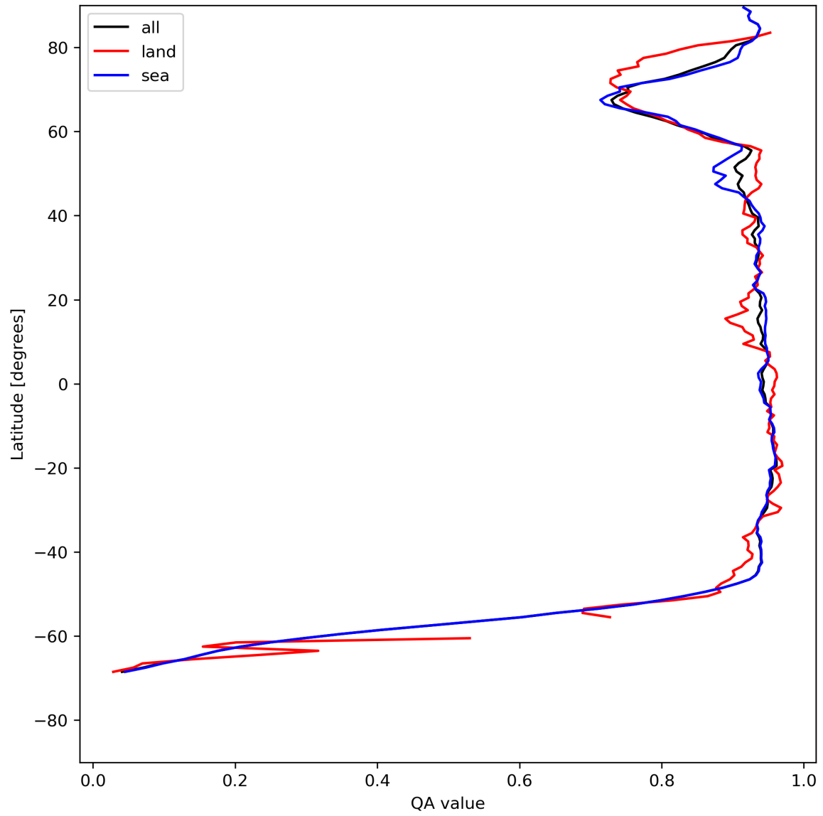
Figure 13: Zonal average of “QA value” for 2024-07-21 to 2024-07-22.
