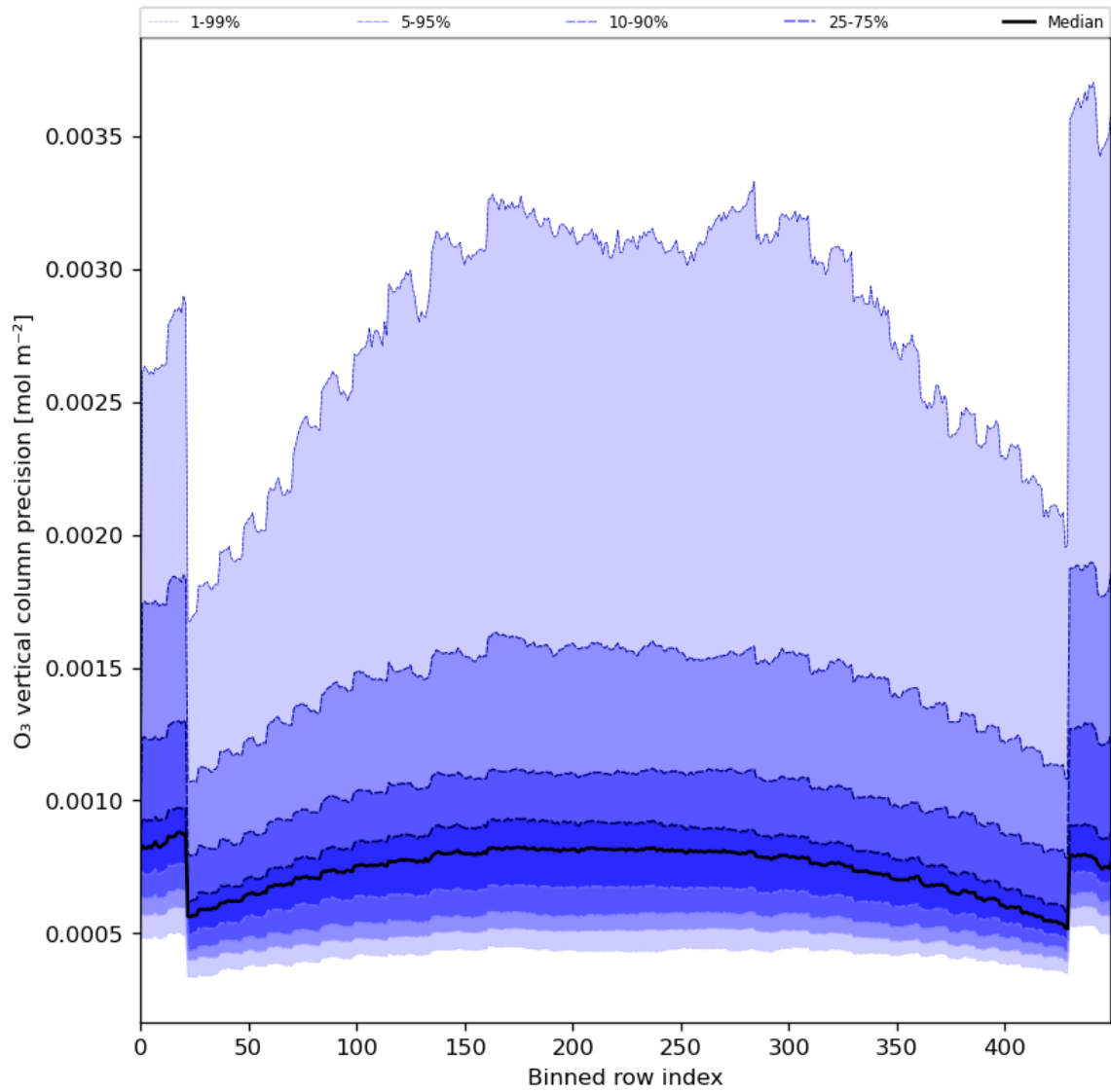
Figure 29: Along track statistics of “O 3 vertical column precision” for 2024-07-21 to 2024-07-22
