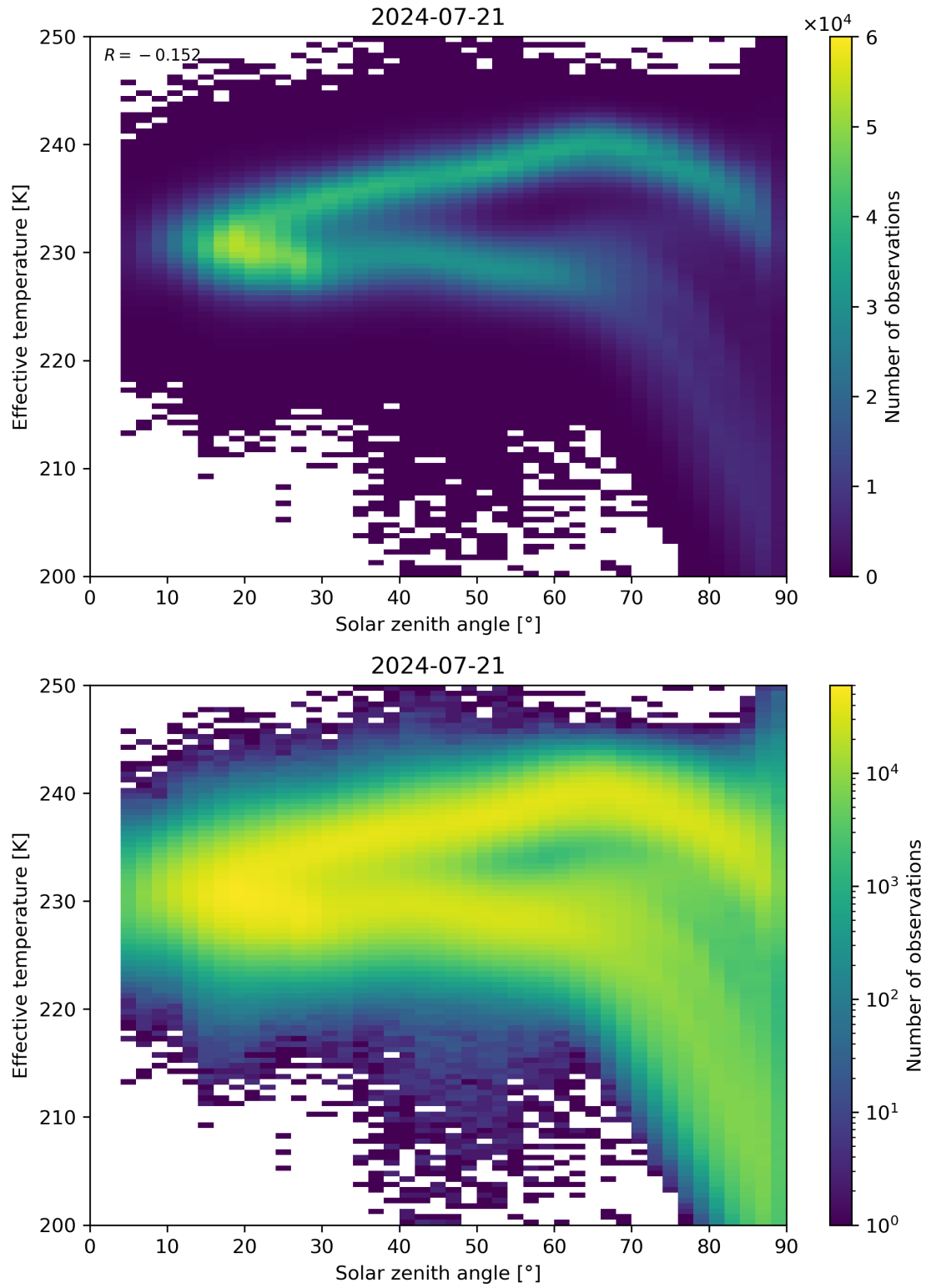
Figure 45: Scatter density plot of “Solar zenith angle” against “Effective temperature” for 2024-07-21 to 2024-07-22.
