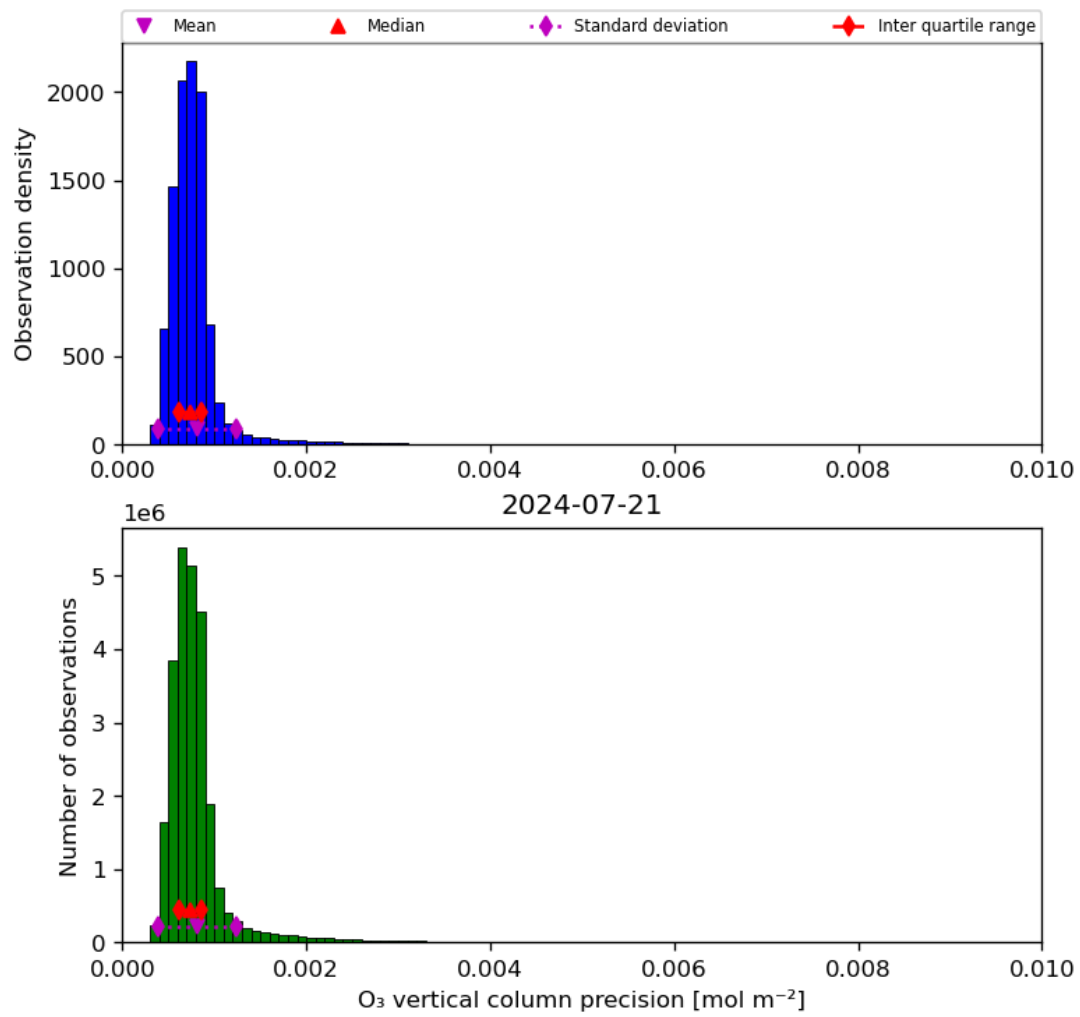
Figure 22: Histogram of “O 3 vertical column precision” for 2024-07-21 to 2024-07-22
