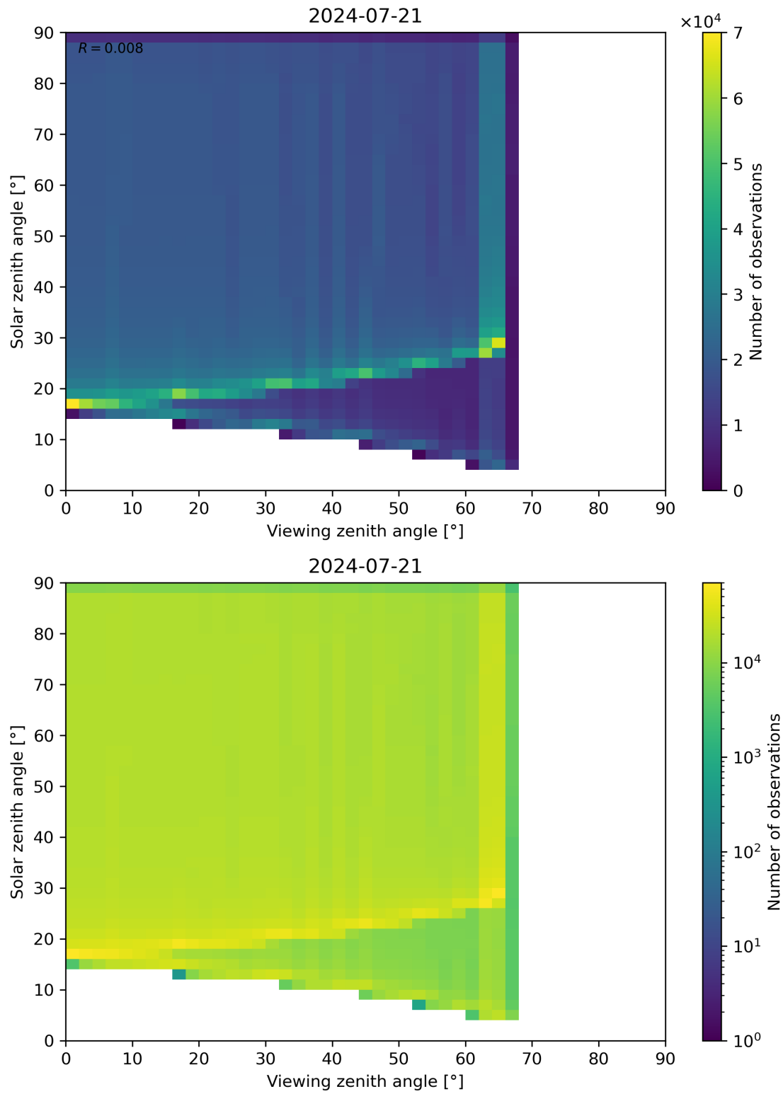
Figure 54: Scatter density plot of “Viewing zenith angle” against “Solar zenith angle” for 2024-07-21 to 2024-07-22.
