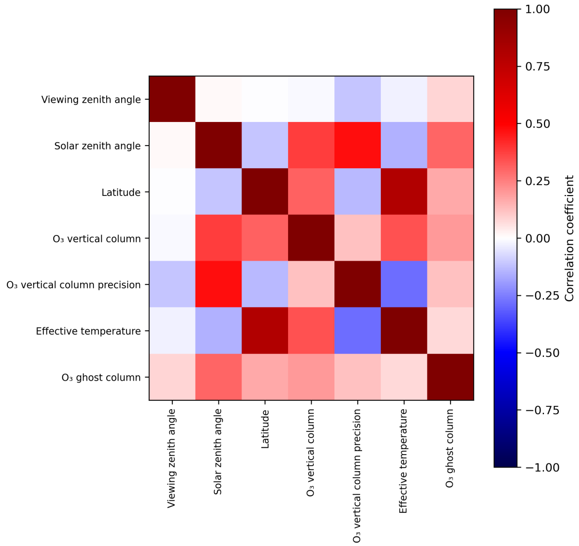
Figure 2: Map of correlation matrix for 2024-07-21 to 2024-07-22.
