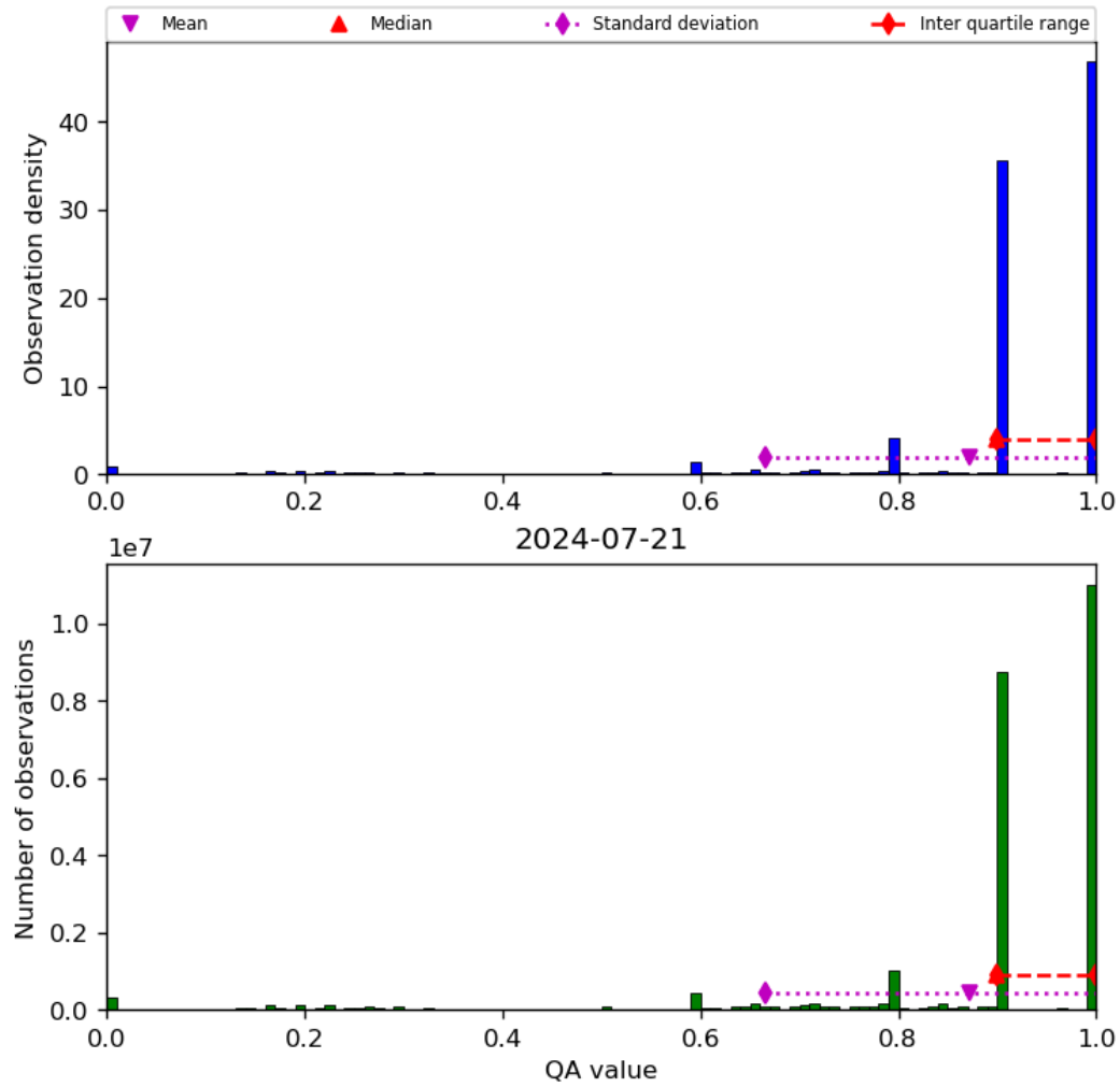
Figure 20: Histogram of “QA value” for 2024-07-21 to 2024-07-22
