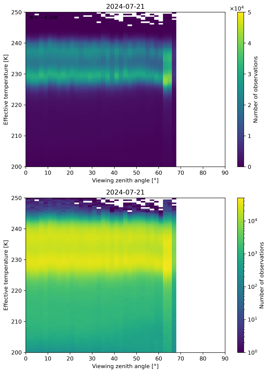
Figure 50: Scatter density plot of “Viewing zenith angle” against “Effective temperature” for 2024-07-21 to 2024-07-22.
