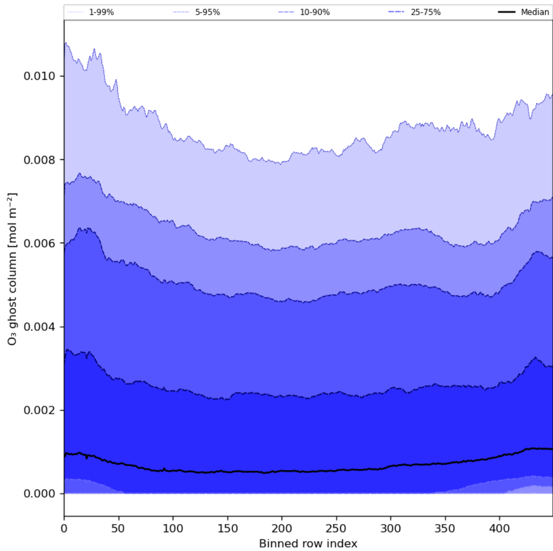
Figure 32: Along track statistics of “O 3 ghost column” for 2024-07-21 to 2024-07-23
