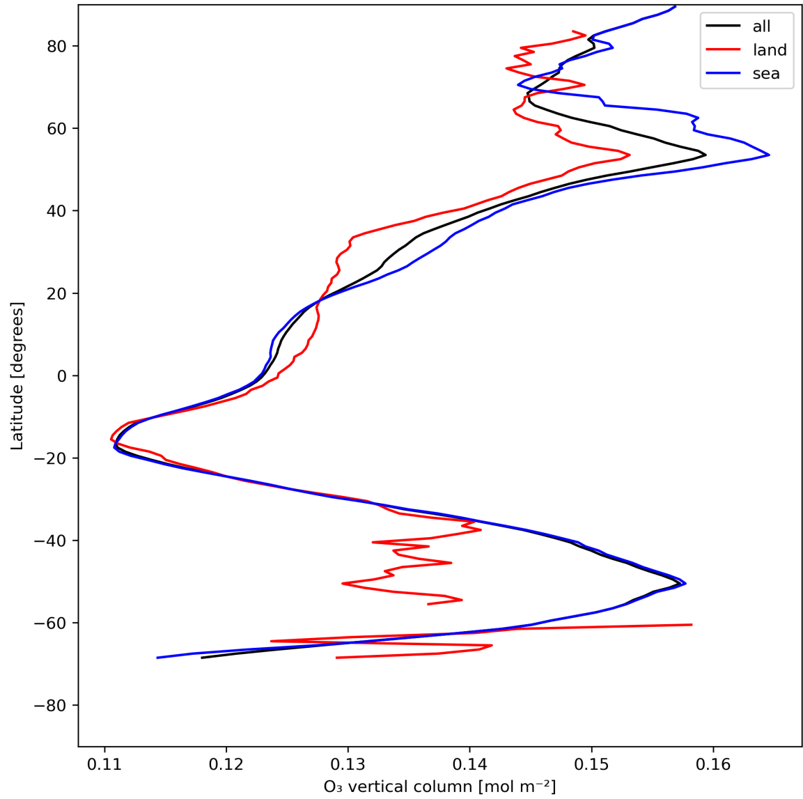
Figure 14: Zonal average of “O 3 vertical column” for 2024-07-21 to 2024-07-23.
