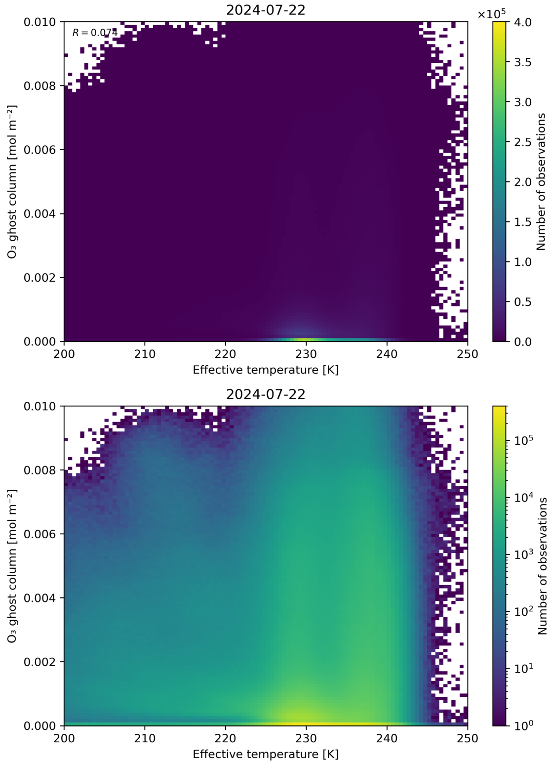
Figure 38: Scatter density plot of “Effective temperature” against “O 3 ghost column” for 2024-07-21 to 2024-07-23.
