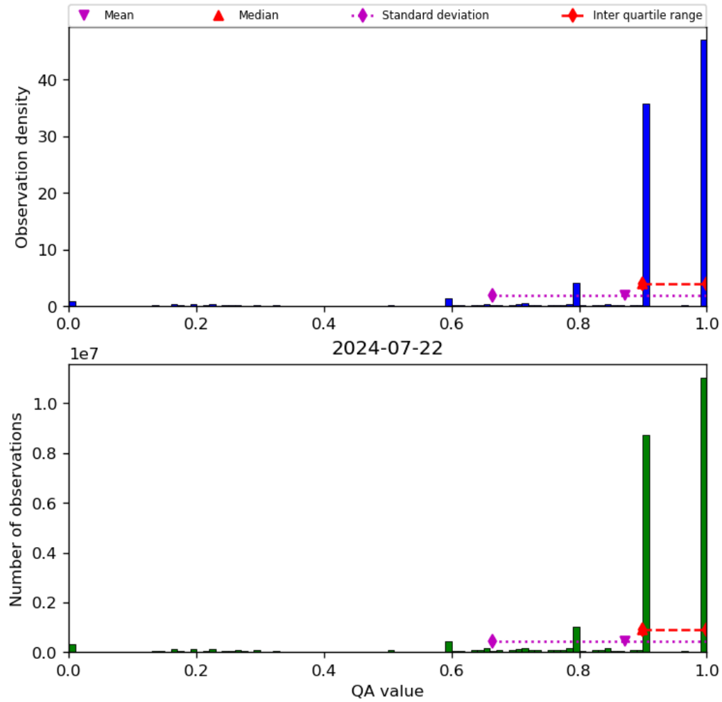
Figure 20: Histogram of “QA value” for 2024-07-21 to 2024-07-23
