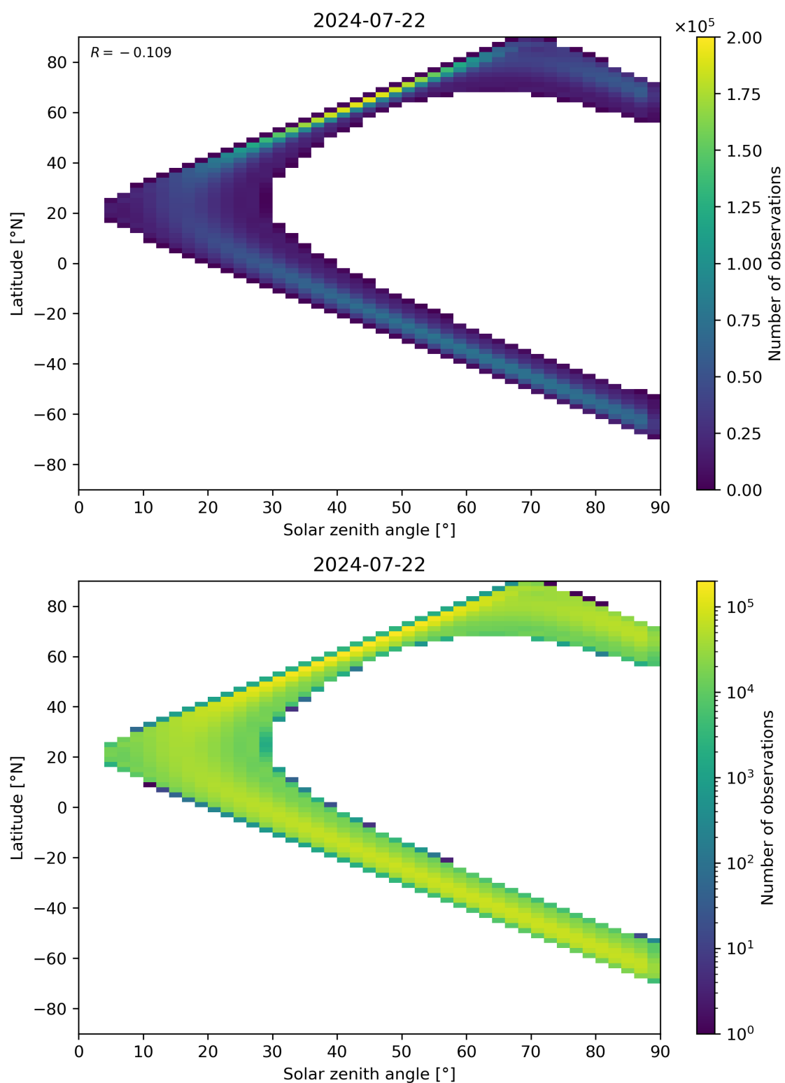
Figure 44: Scatter density plot of “Solar zenith angle” against “Latitude” for 2024-07-21 to 2024-07-23.
