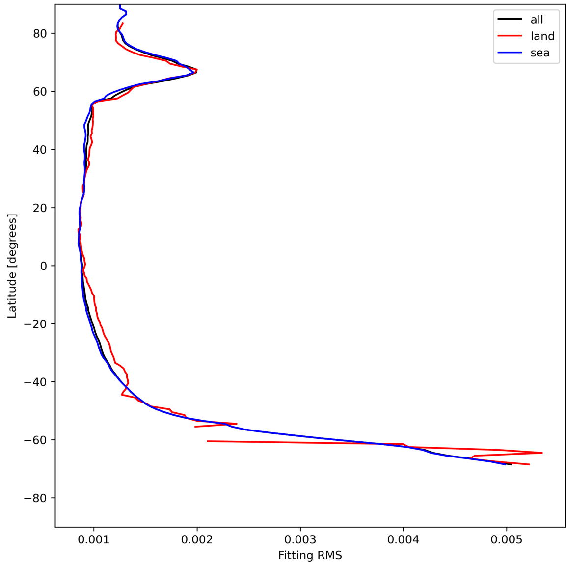
Figure 16: Zonal average of “Fitting RMS” for 2024-07-21 to 2024-07-23.
