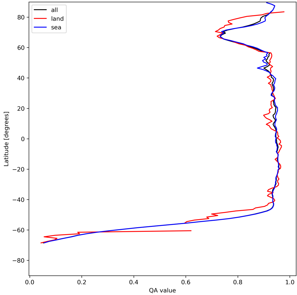
Figure 13: Zonal average of “QA value” for 2024-07-21 to 2024-07-23.
