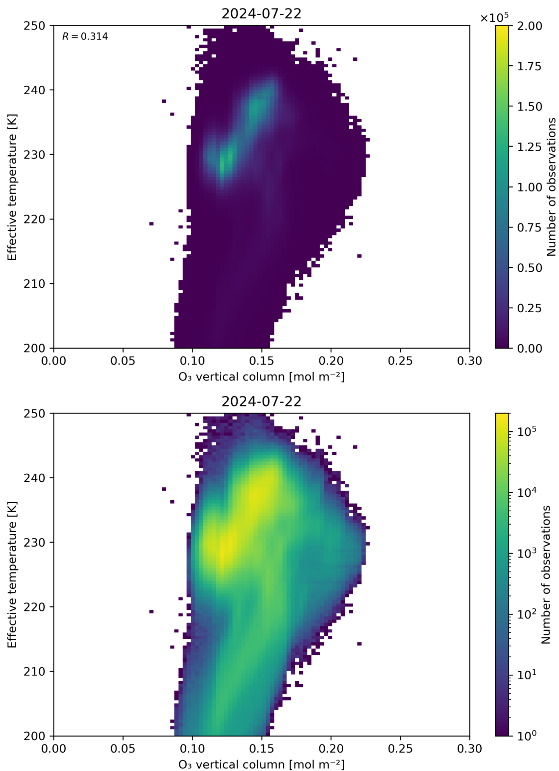
Figure 39: Scatter density plot of “O 3 vertical column” against “Effective temperature” for 2024-07-21 to 2024-07-23.
