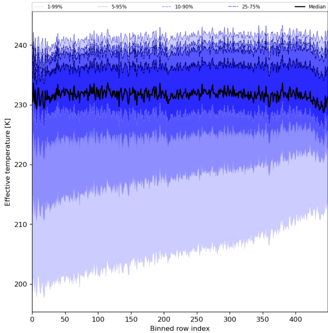
Figure 31: Along track statistics of “Effective temperature” for 2024-07-21 to 2024-07-23
