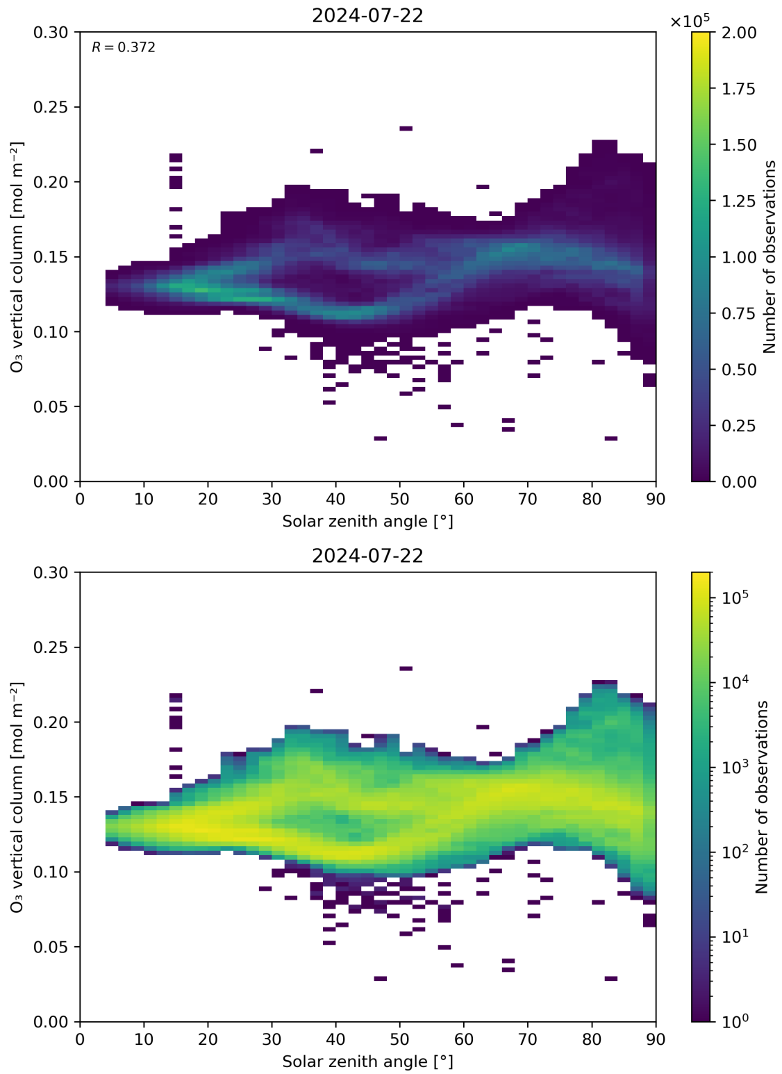
Figure 47: Scatter density plot of “Solar zenith angle” against “O 3 vertical column” for 2024-07-21 to 2024-07-23.
