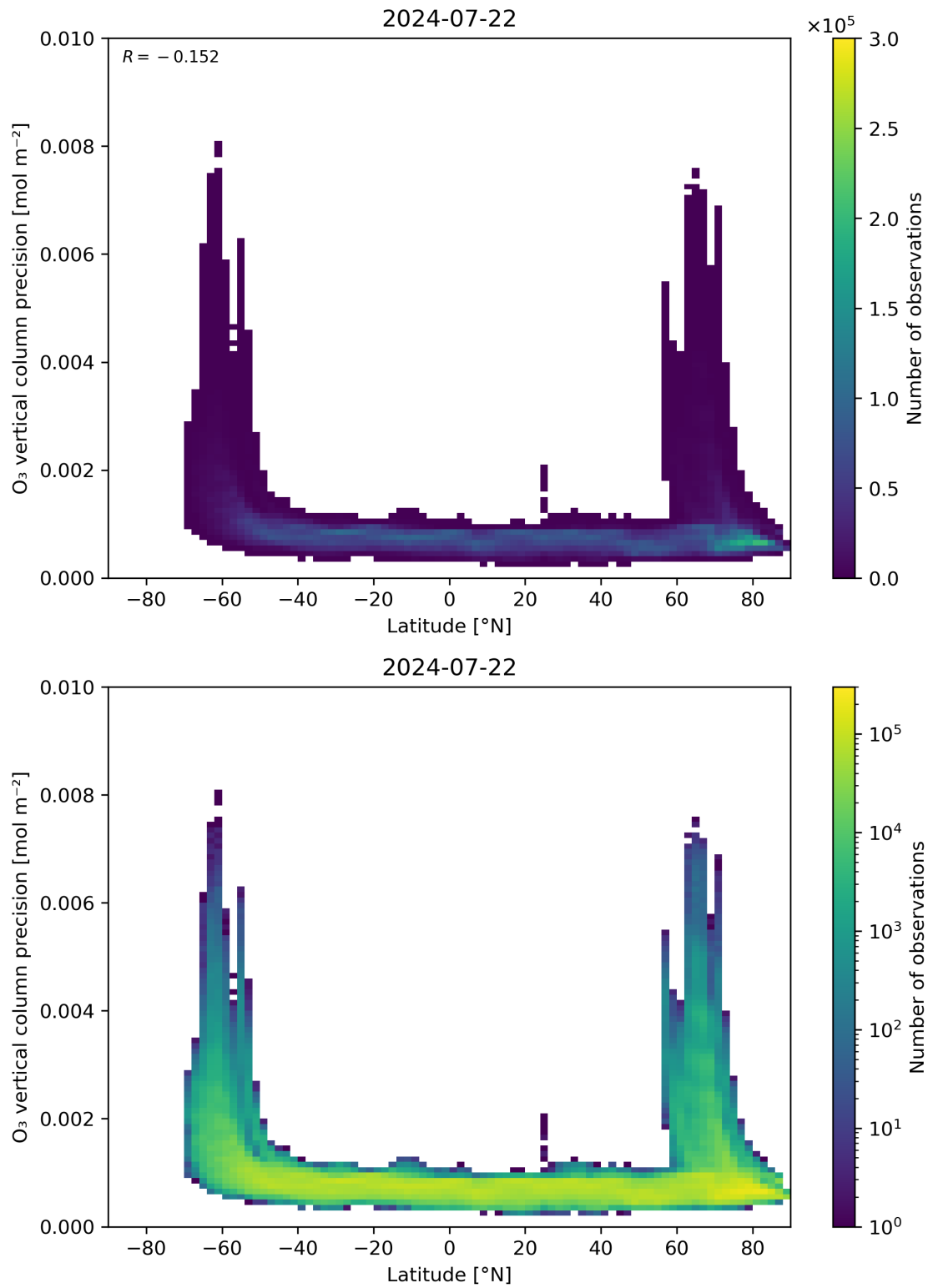
Figure 37: Scatter density plot of “Latitude” against “O 3 vertical column precision” for 2024-07-21 to 2024-07-23.
