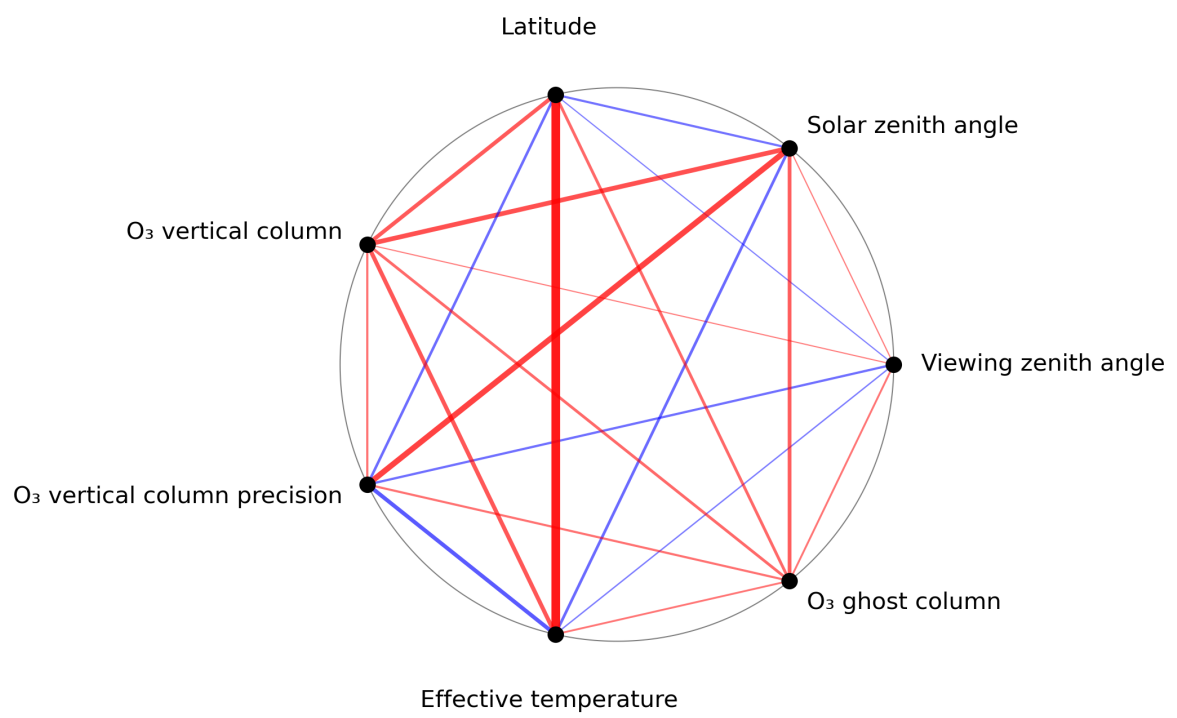
Figure 1: Map of correlation graph for 2024-07-21 to 2024-07-23.
