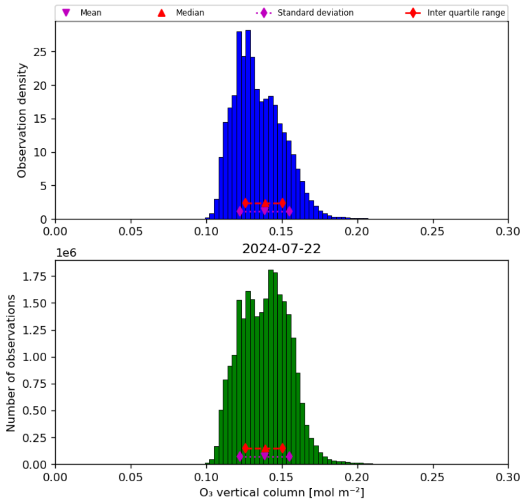
Figure 21: Histogram of “O 3 vertical column” for 2024-07-21 to 2024-07-23
