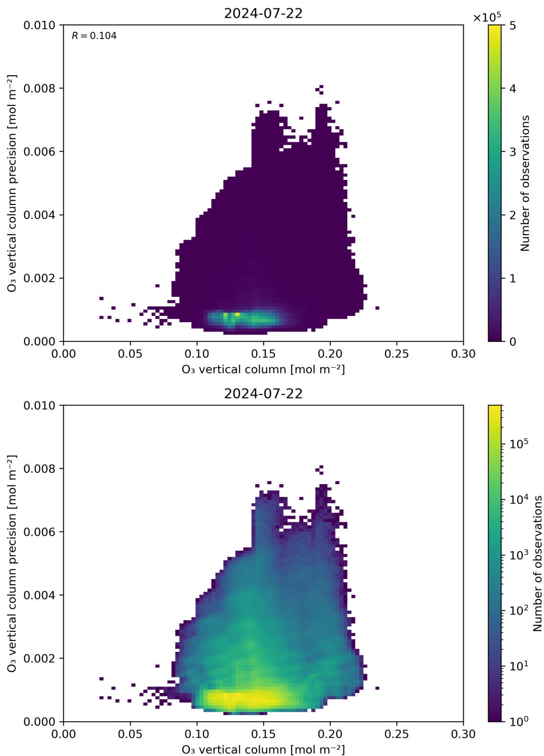
Figure 41: Scatter density plot of “O 3 vertical column” against “O 3 vertical column precision” for 2024-07-21 to 2024-07-23.
