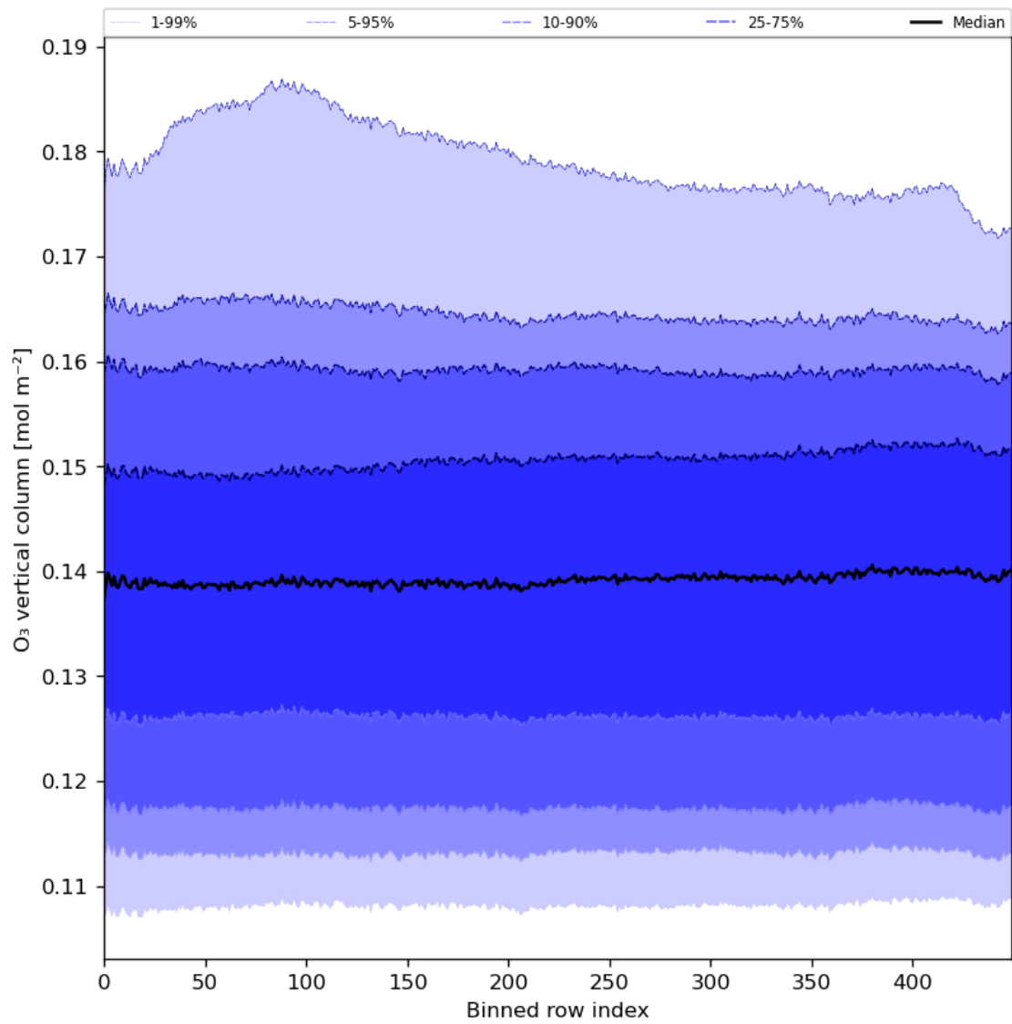
Figure 28: Along track statistics of “O 3 vertical column” for 2024-07-21 to 2024-07-23
