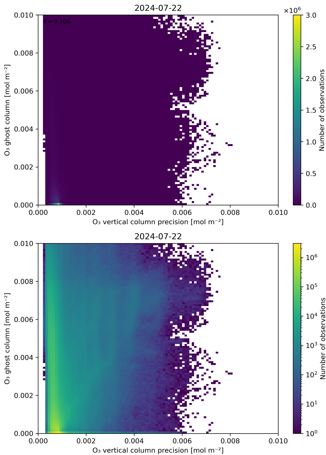
Figure 43: Scatter density plot of “O 3 vertical column precision” against “O 3 ghost column” for 2024-07-21 to 2024-07-23.
