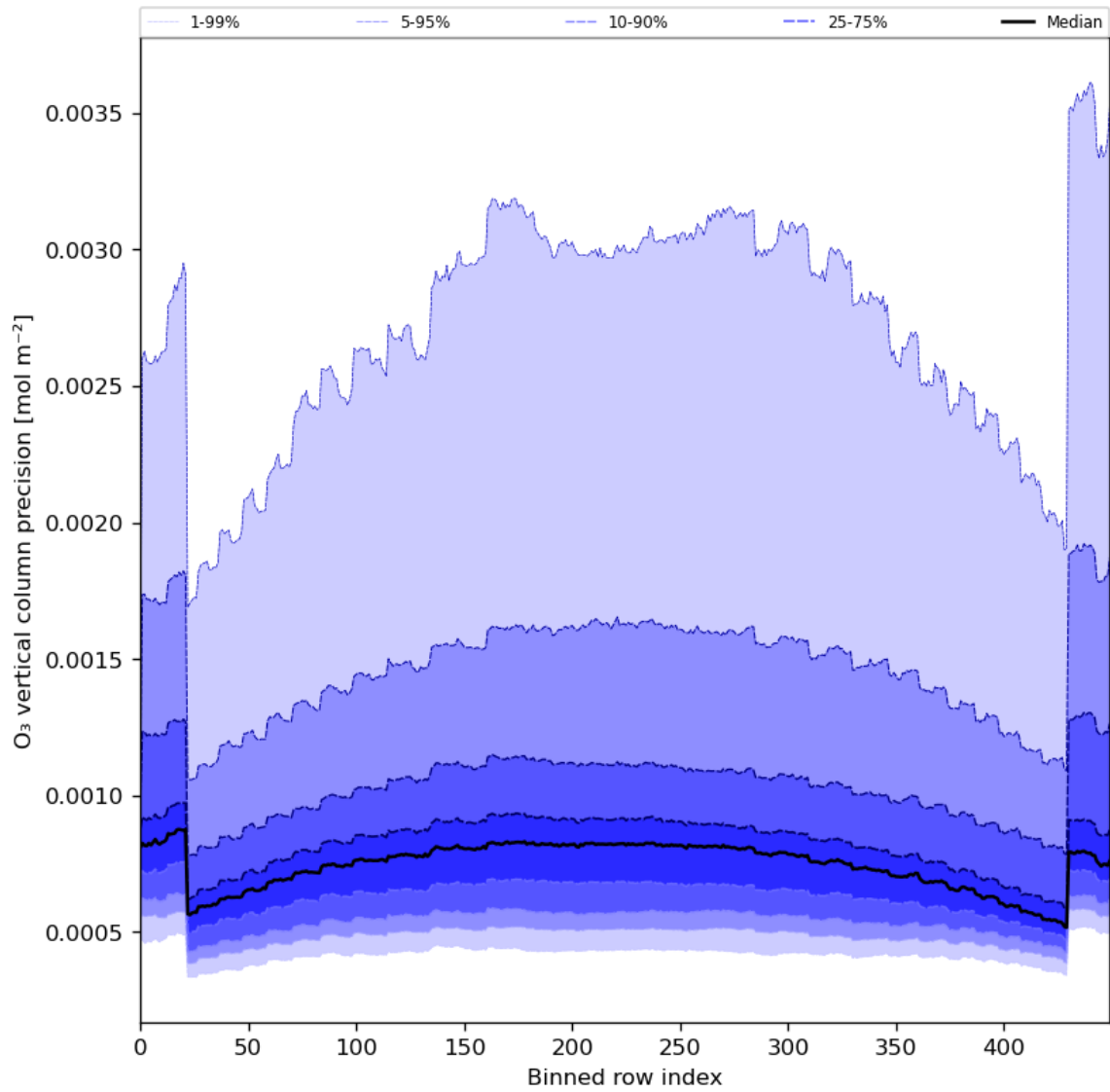
Figure 29: Along track statistics of “O 3 vertical column precision” for 2024-07-21 to 2024-07-23
