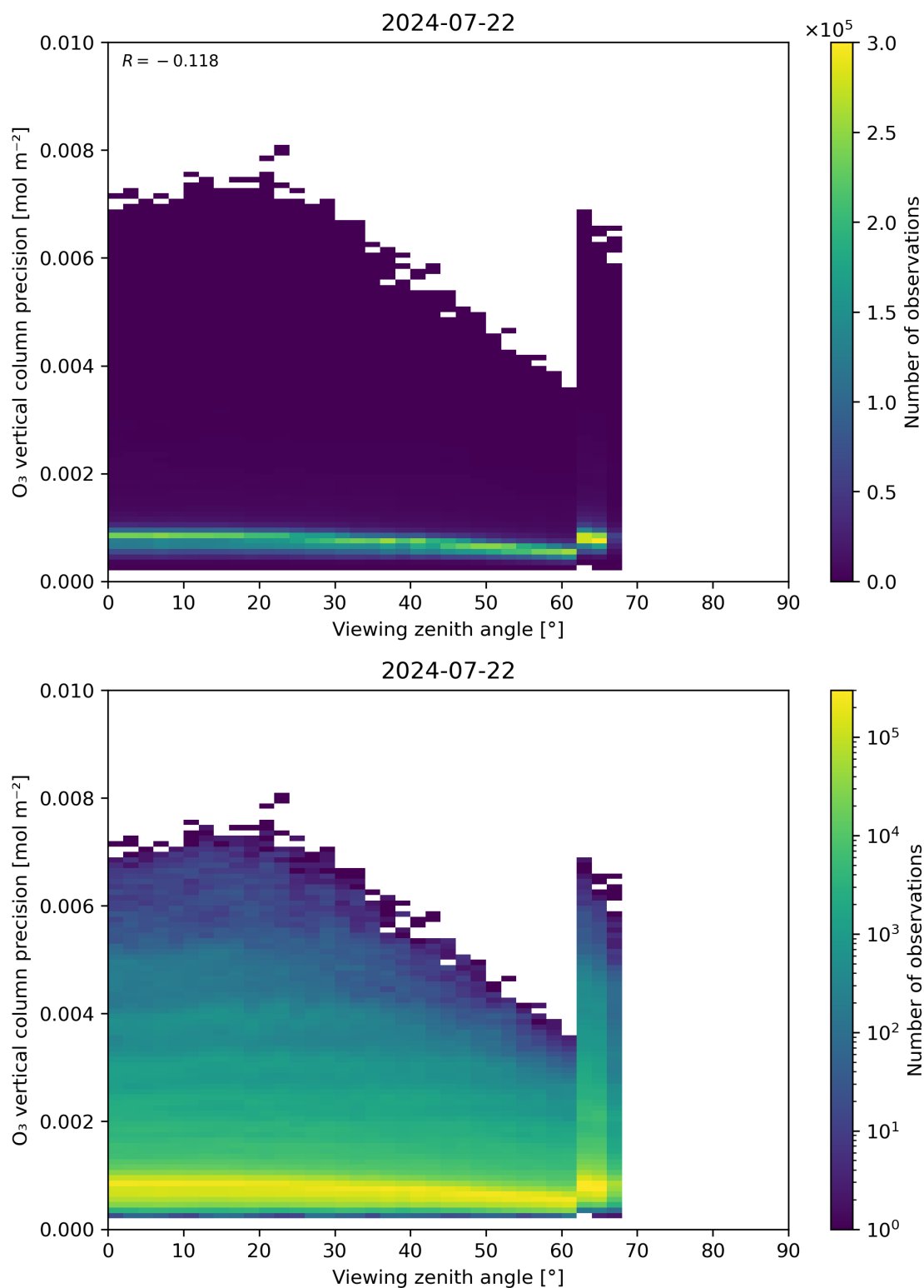
Figure 53: Scatter density plot of “Viewing zenith angle” against “O 3 vertical column precision” for 2024-07-21 to 2024-07-23.
