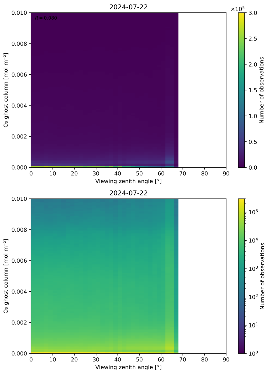
Figure 51: Scatter density plot of “Viewing zenith angle” against “O 3 ghost column” for 2024-07-21 to 2024-07-23.
