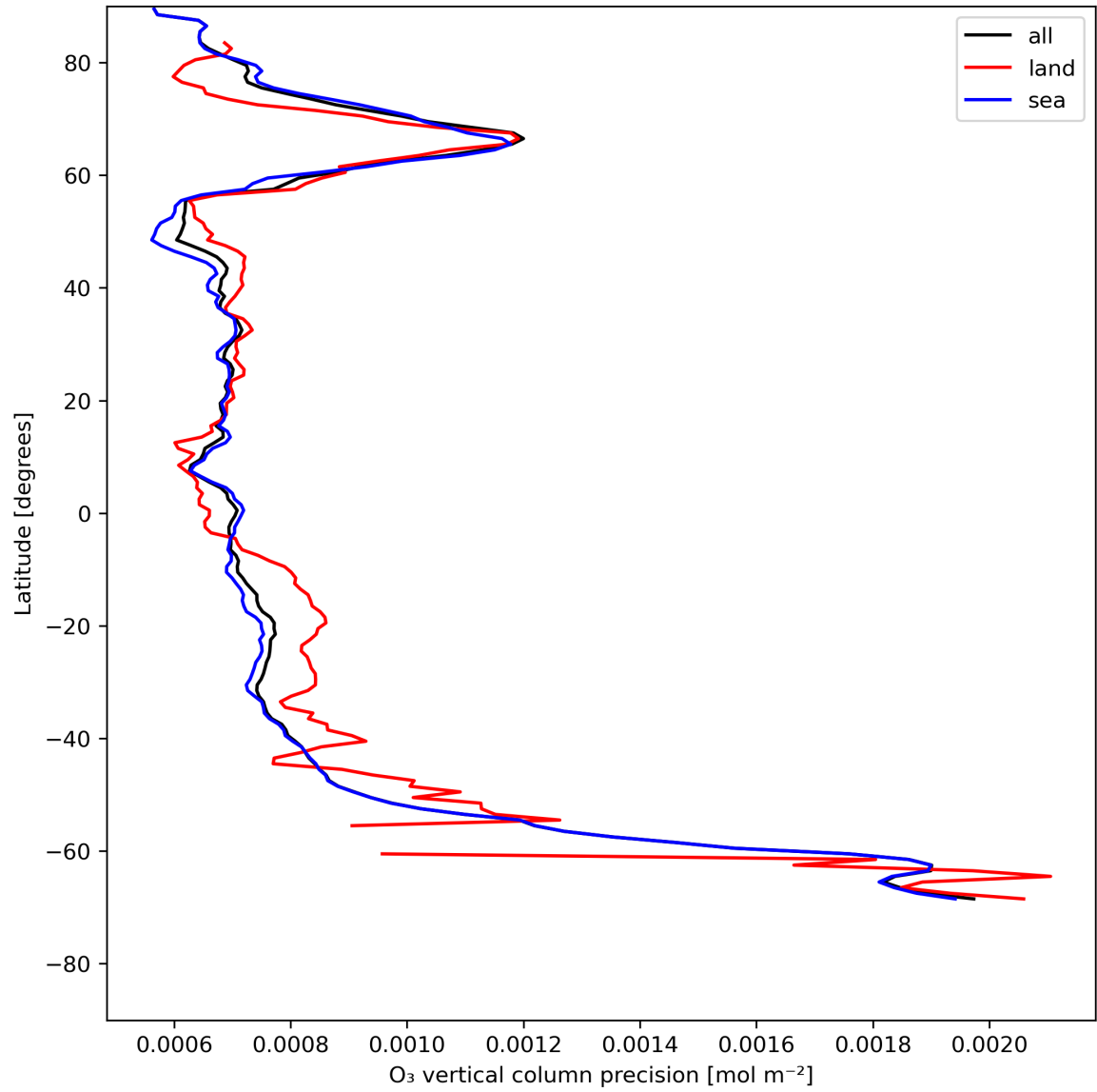
Figure 15: Zonal average of “O 3 vertical column precision” for 2024-07-21 to 2024-07-23.
