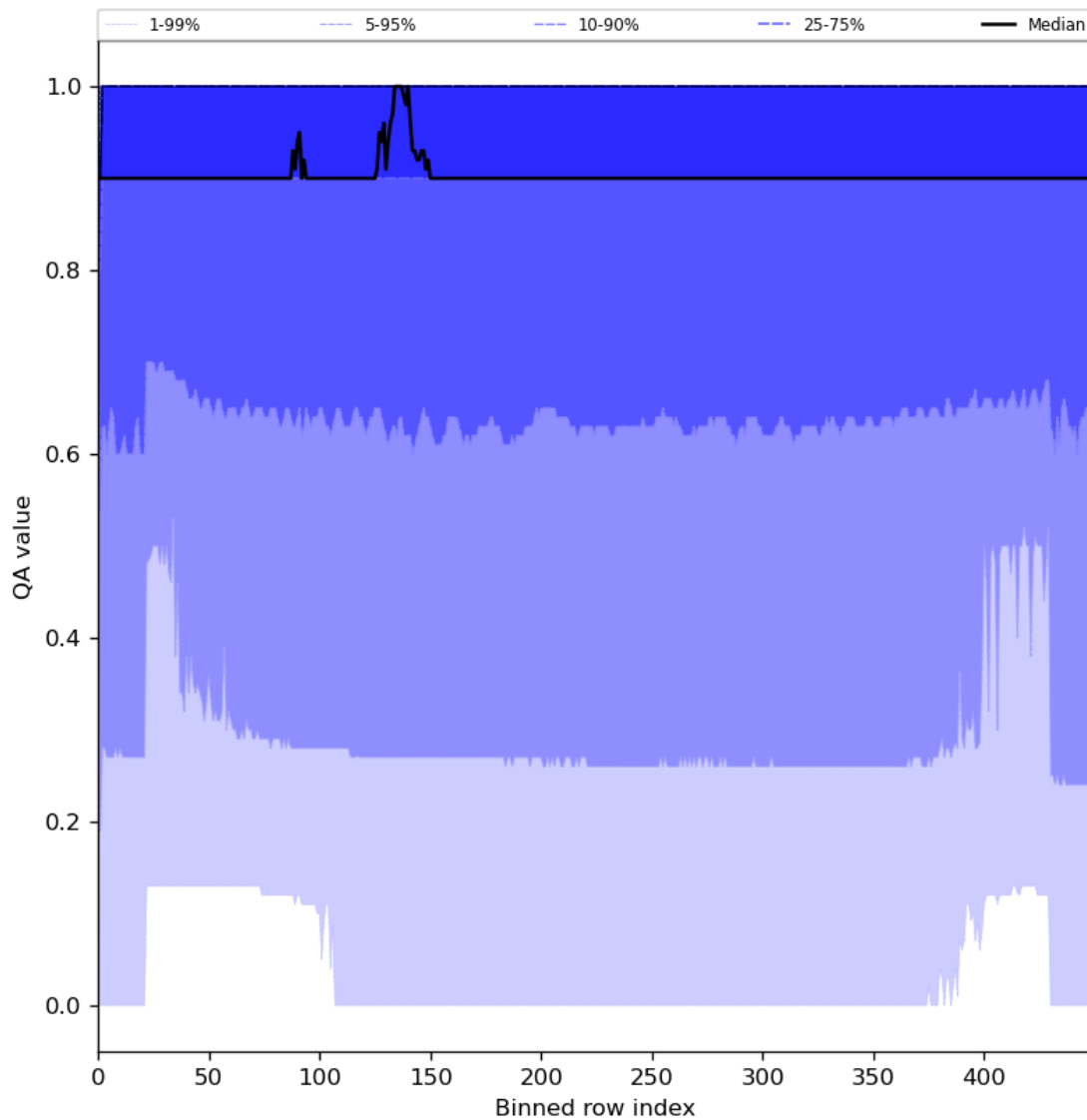
Figure 27: Along track statistics of “QA value” for 2024-07-21 to 2024-07-23
