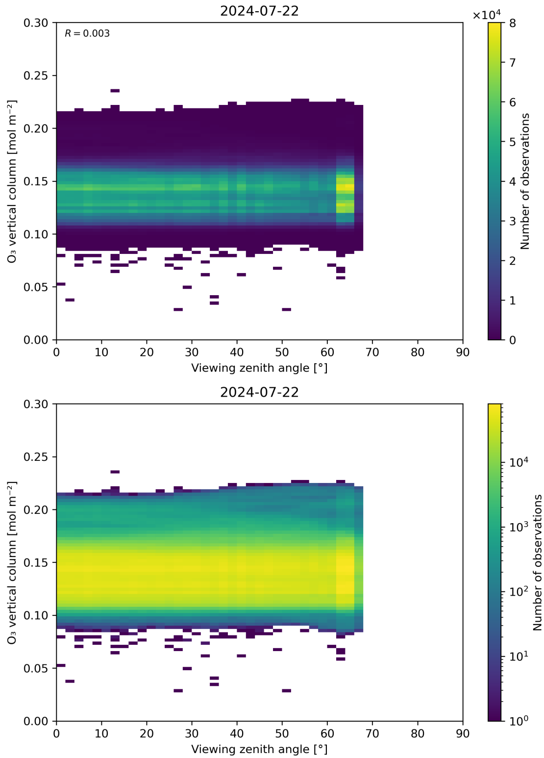
Figure 52: Scatter density plot of “Viewing zenith angle” against “O 3 vertical column” for 2024-07-21 to 2024-07-23.
