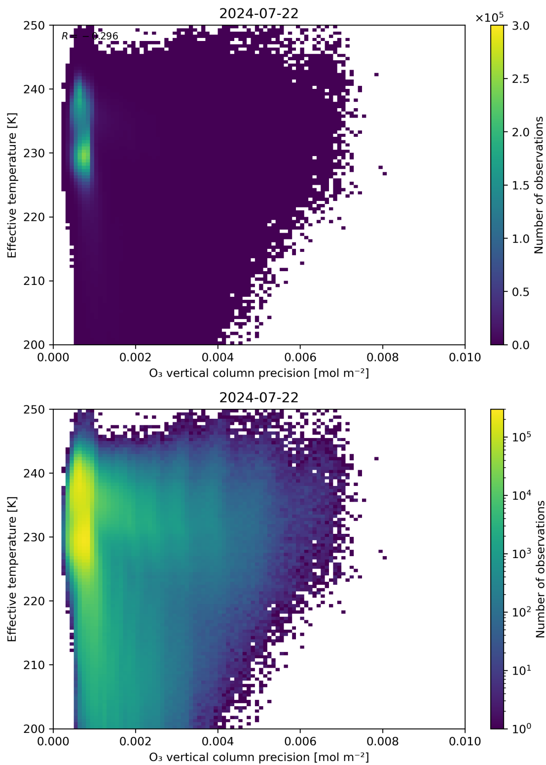
Figure 42: Scatter density plot of “O 3 vertical column precision” against “Effective temperature” for 2024-07-21 to 2024-07-23.
