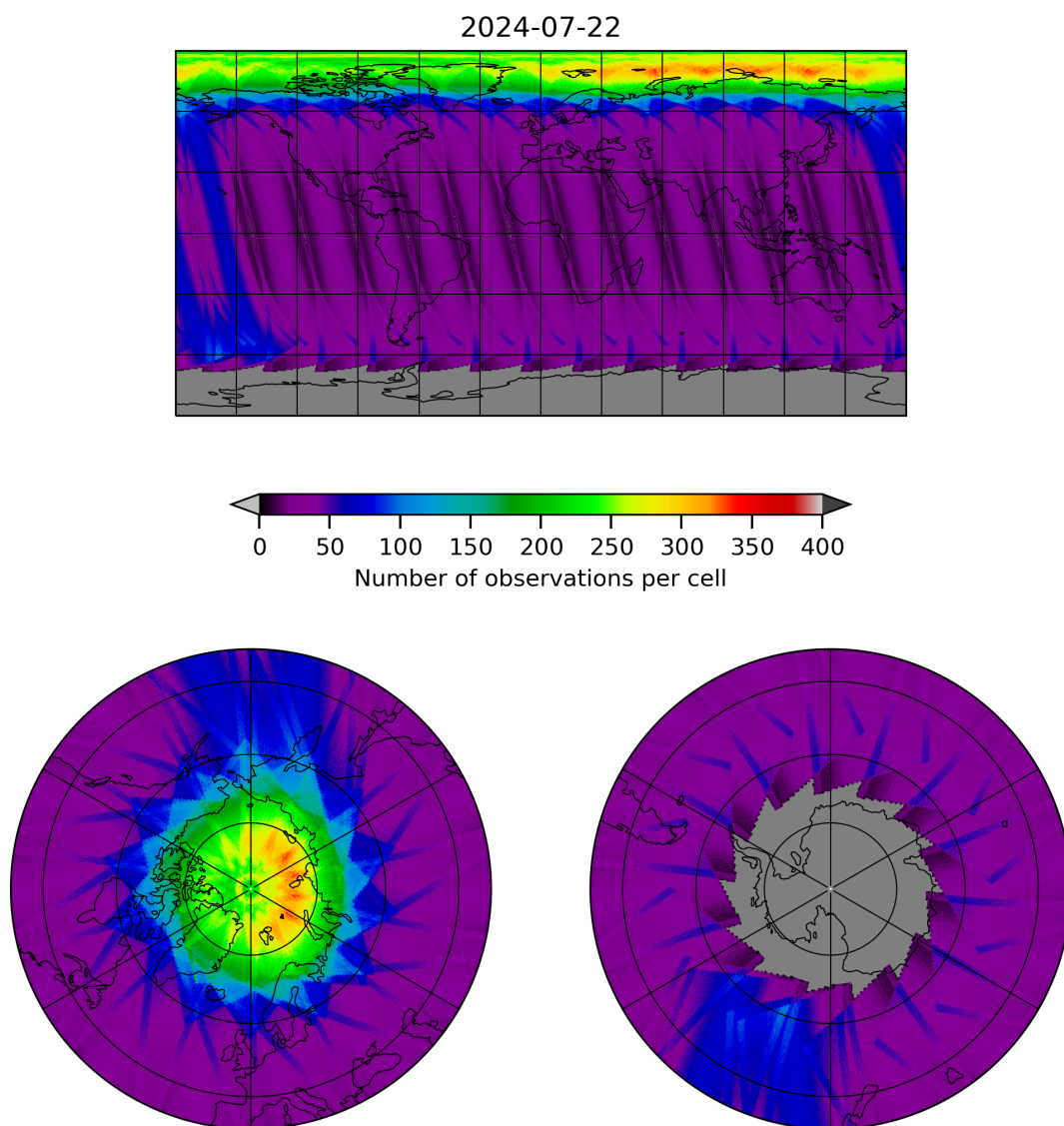
Figure 12: Map of the number of observations for 2024-07-21 to 2024-07-23
