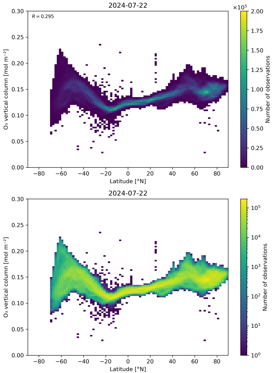
Figure 36: Scatter density plot of “Latitude” against “O 3 vertical column” for 2024-07-21 to 2024-07-23.
