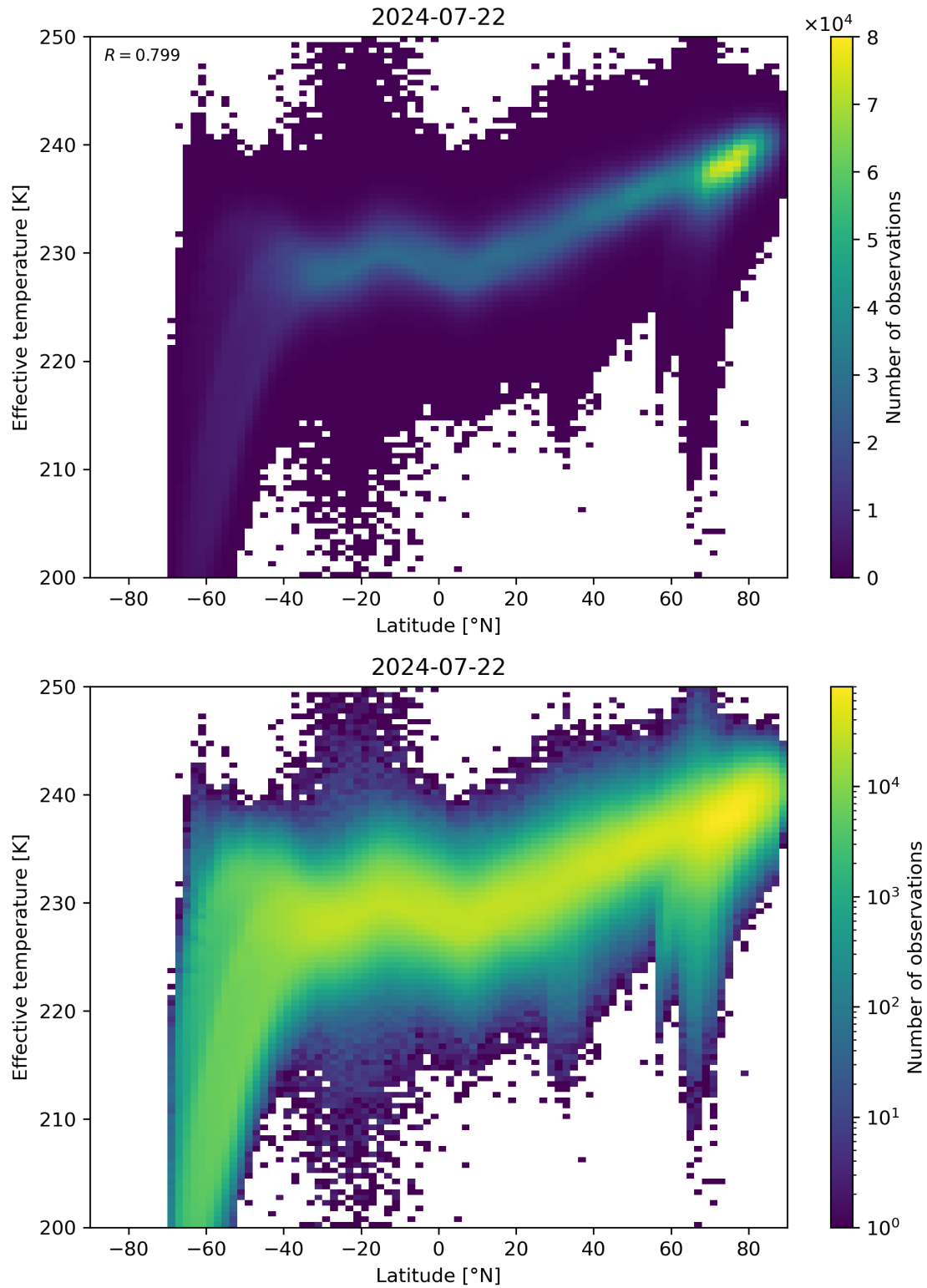
Figure 34: Scatter density plot of “Latitude” against “Effective temperature” for 2024-07-21 to 2024-07-23.
