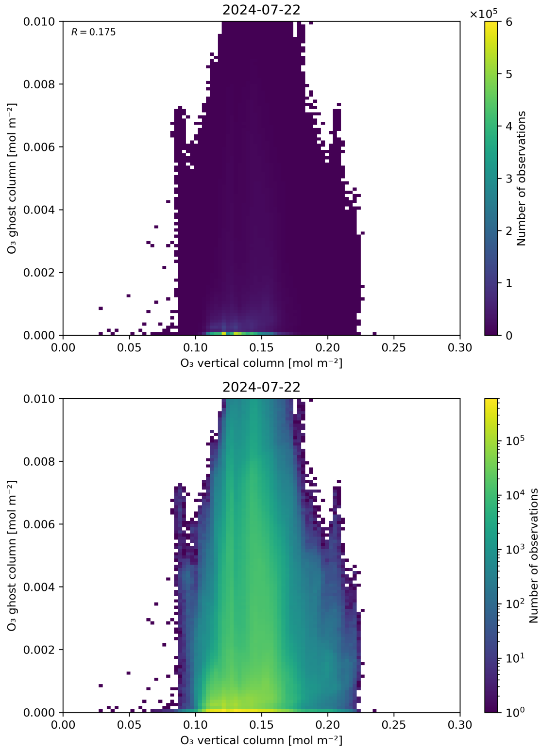
Figure 40: Scatter density plot of “O 3 vertical column” against “O 3 ghost column” for 2024-07-21 to 2024-07-23.
