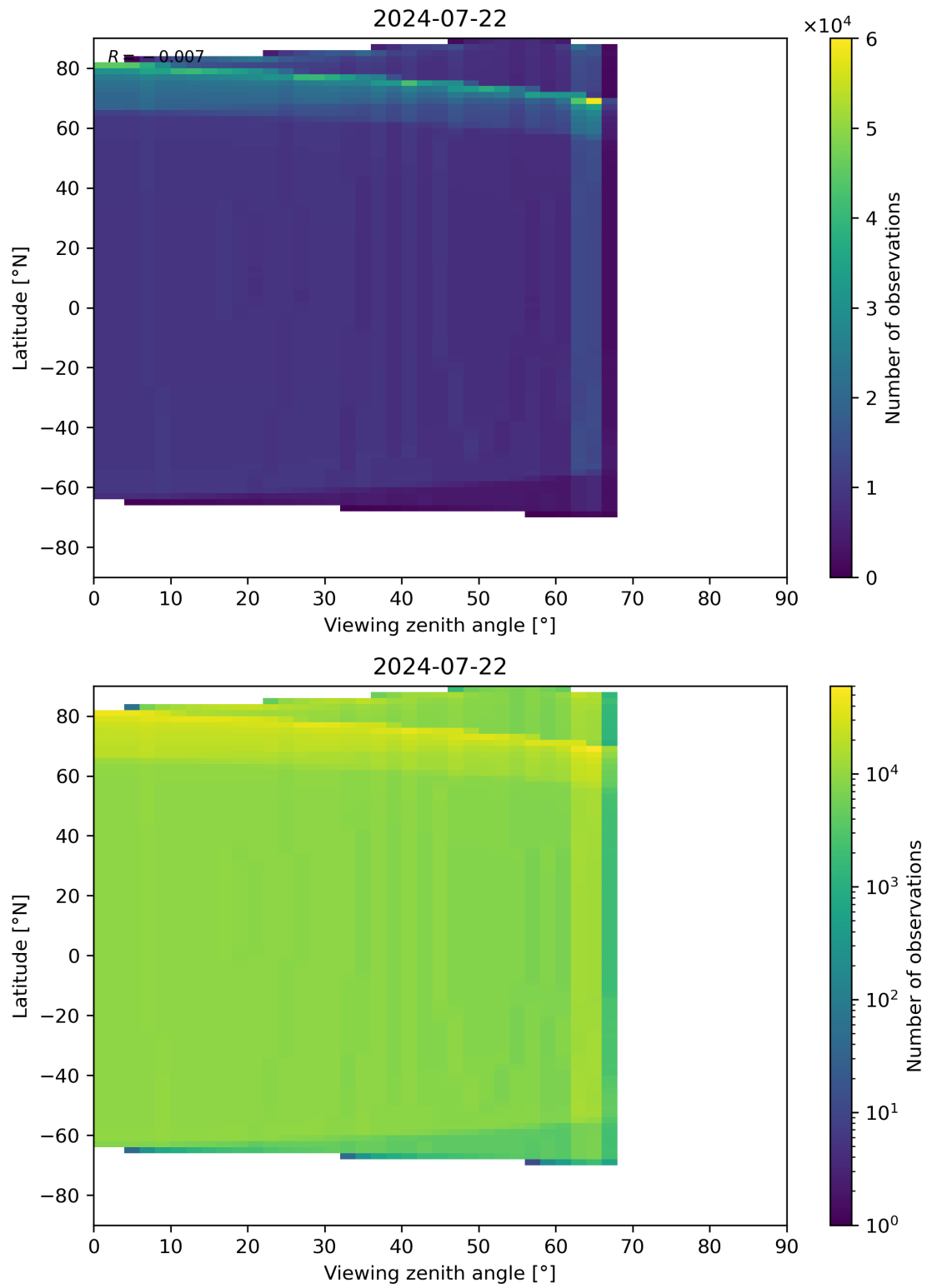
Figure 49: Scatter density plot of “Viewing zenith angle” against “Latitude” for 2024-07-21 to 2024-07-23.
