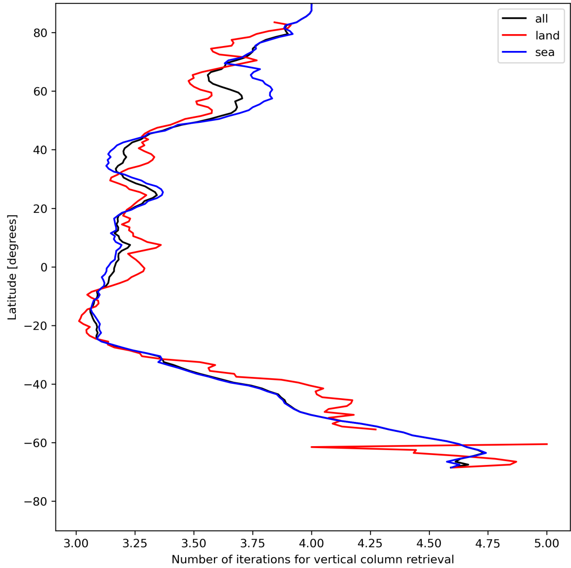
Figure 19: Zonal average of “Number of iterations for vertical column retrieval” for 2024-07-21 to 2024-07-23.
