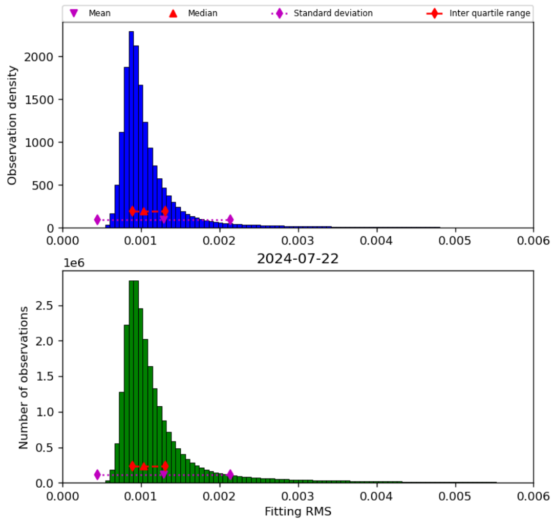
Figure 23: Histogram of “Fitting RMS” for 2024-07-21 to 2024-07-23
