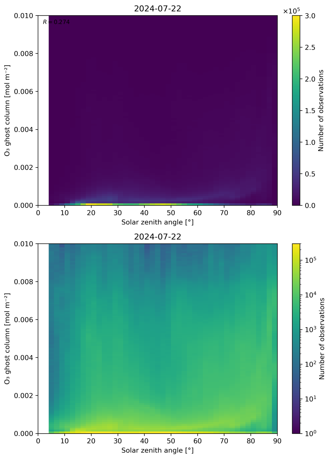
Figure 46: Scatter density plot of “Solar zenith angle” against “O 3 ghost column” for 2024-07-21 to 2024-07-23.
