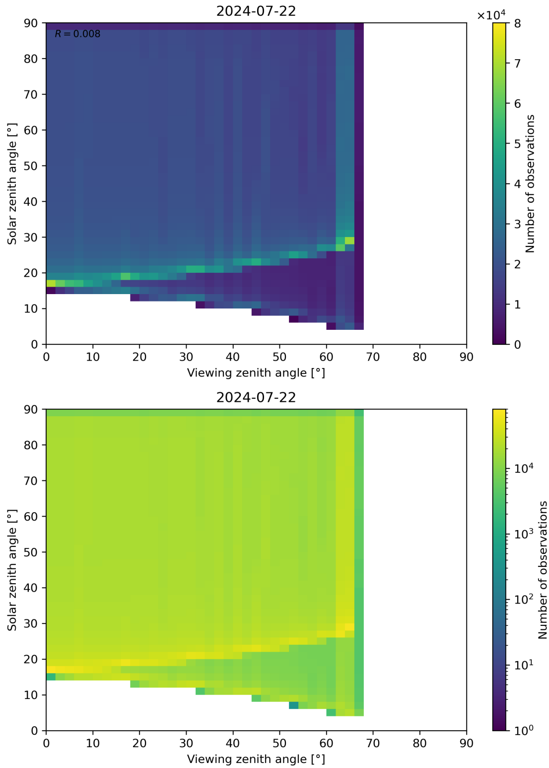
Figure 54: Scatter density plot of “Viewing zenith angle” against “Solar zenith angle” for 2024-07-21 to 2024-07-23.
