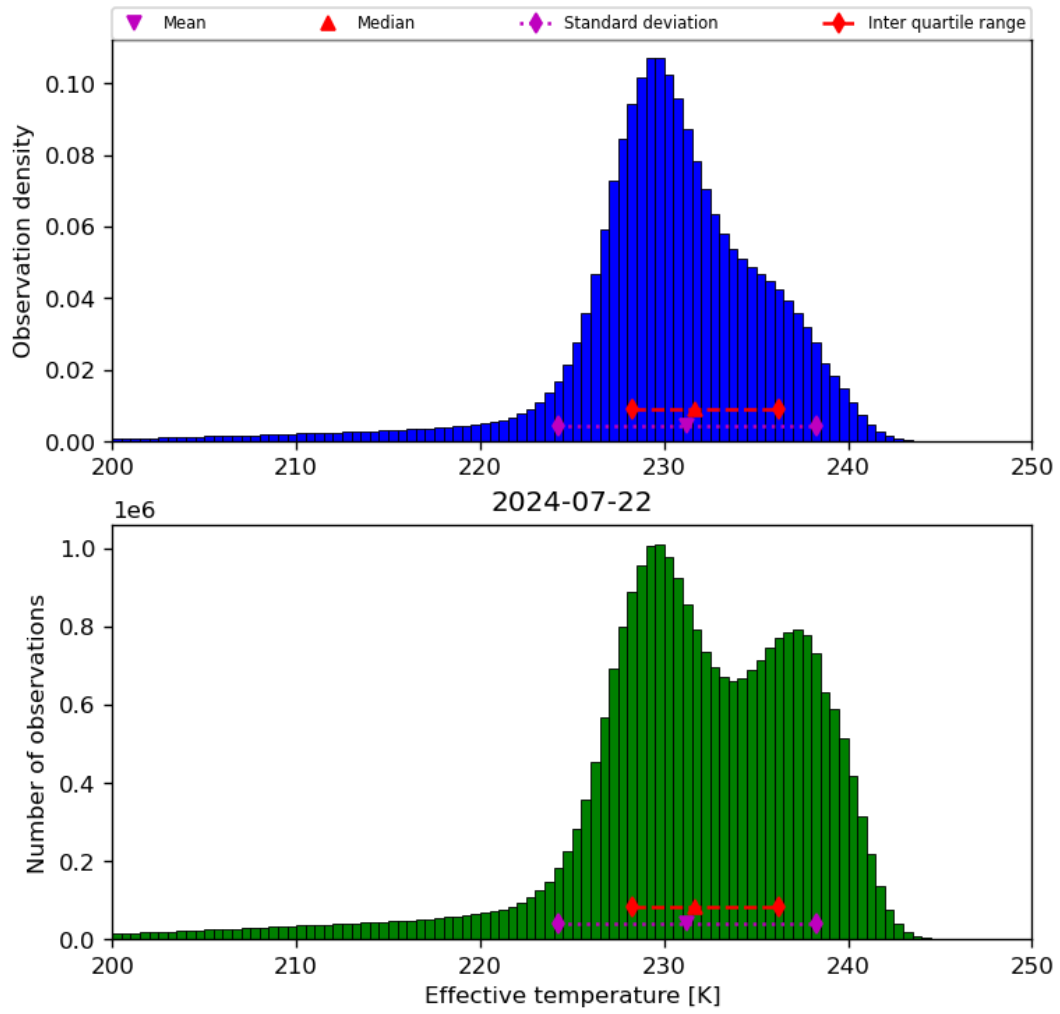
Figure 24: Histogram of “Effective temperature” for 2024-07-21 to 2024-07-23
