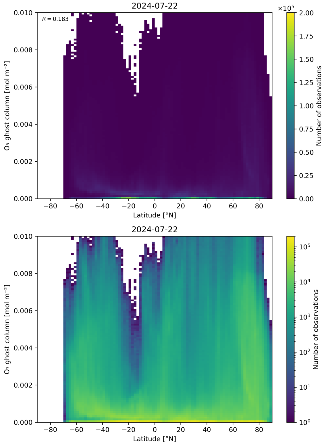
Figure 35: Scatter density plot of “Latitude” against “O 3 ghost column” for 2024-07-21 to 2024-07-23.
