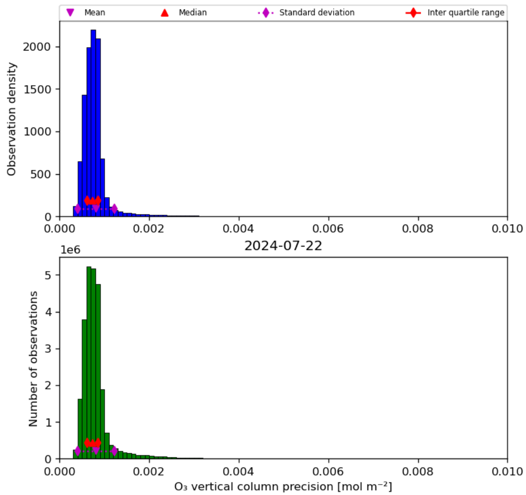
Figure 22: Histogram of “O 3 vertical column precision” for 2024-07-21 to 2024-07-23
