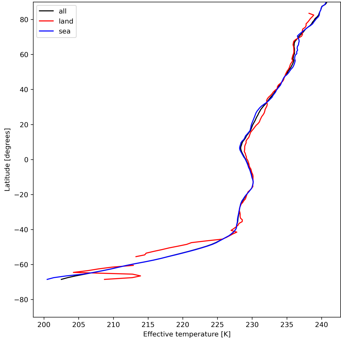
Figure 17: Zonal average of "Effective temperature" for 2024-07-21 to 2024-07-23.
