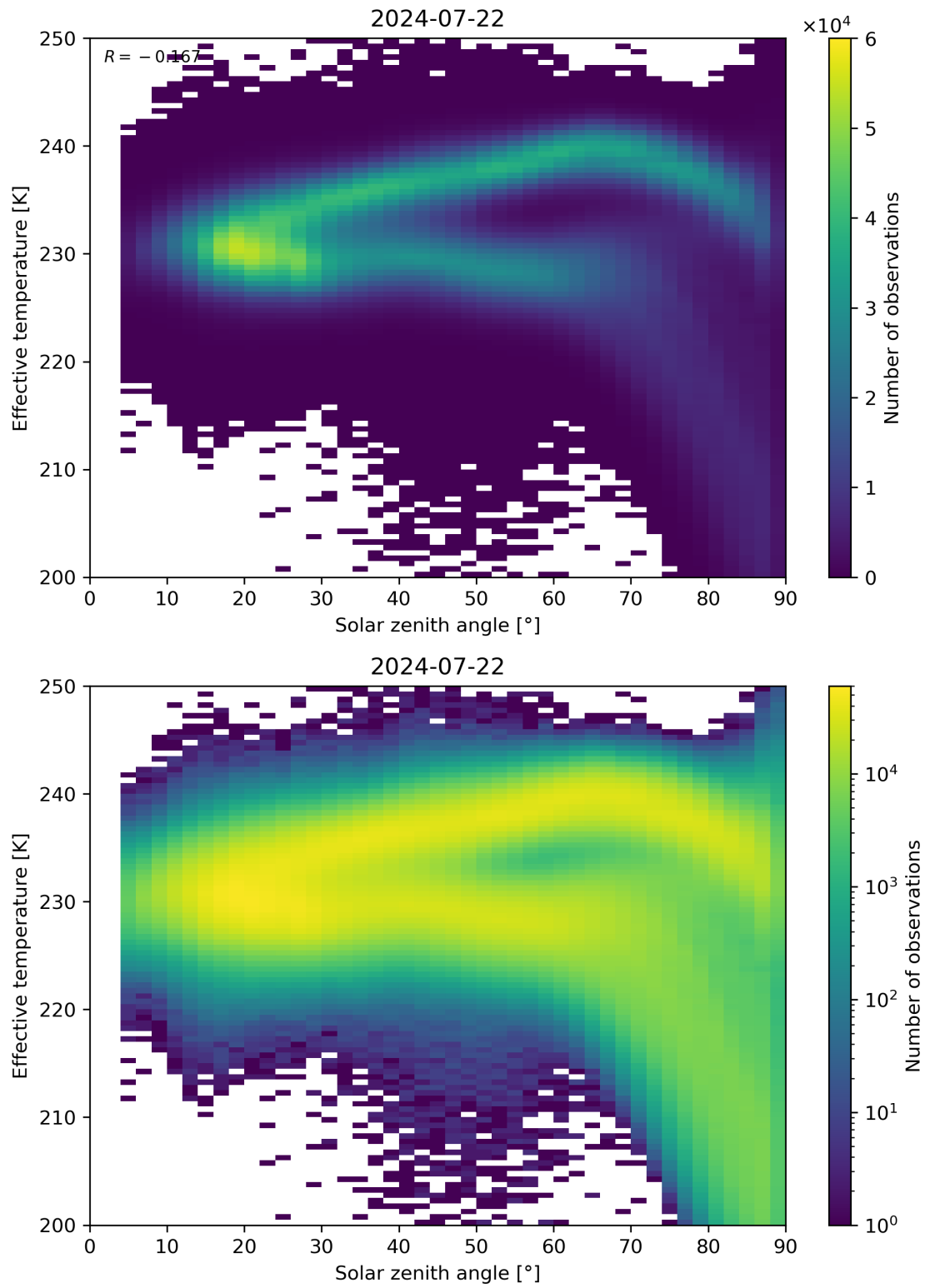
Figure 45: Scatter density plot of “Solar zenith angle” against “Effective temperature” for 2024-07-21 to 2024-07-23.
