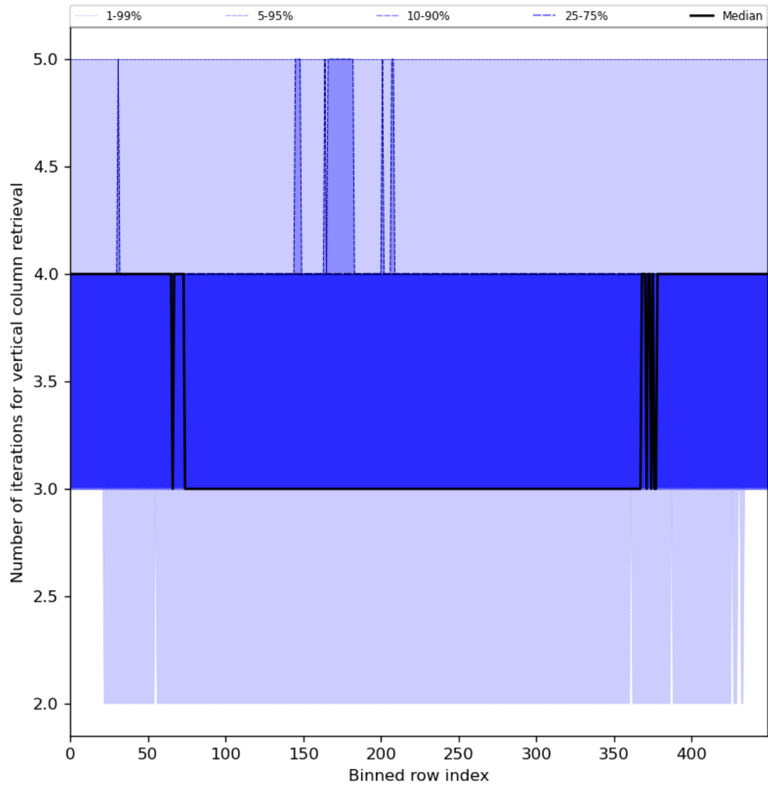
Figure 33: Along track statistics of “Number of iterations for vertical column retrieval” for 2024-07-21 to 2024-07-23
