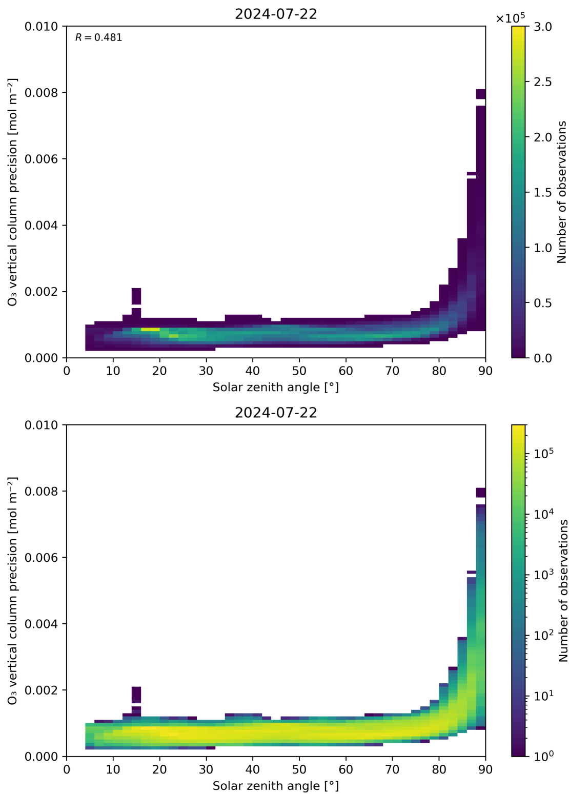
Figure 48: Scatter density plot of “Solar zenith angle” against “O 3 vertical column precision” for 2024-07-21 to 2024-07-23.
