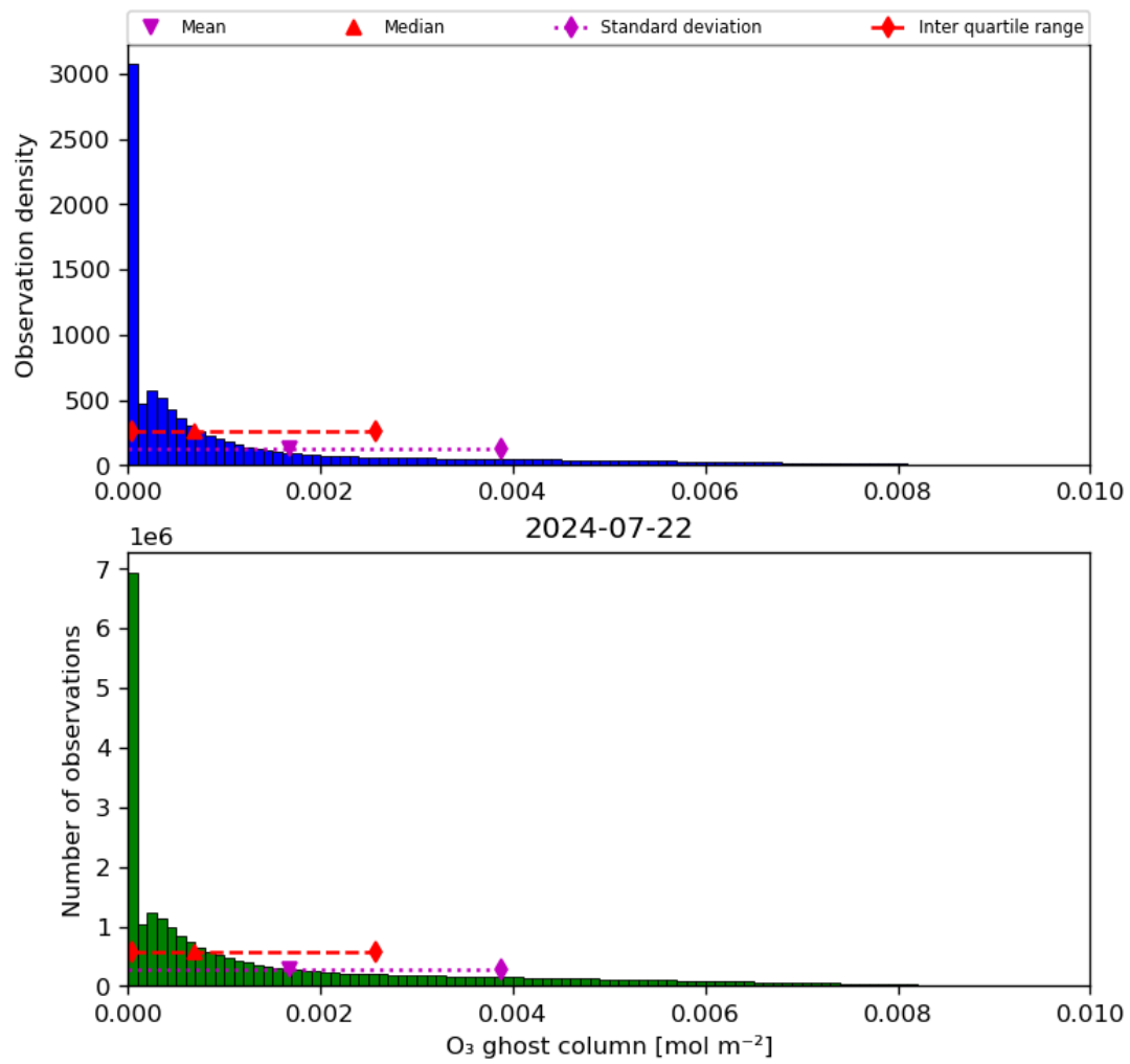
Figure 25: Histogram of “O 3 ghost column” for 2024-07-21 to 2024-07-23
