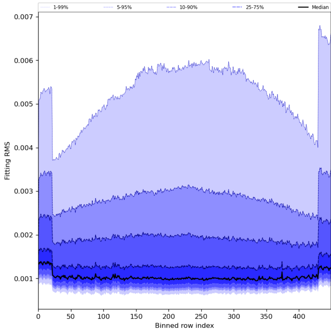
Figure 30: Along track statistics of “Fitting RMS” for 2024-07-21 to 2024-07-23
