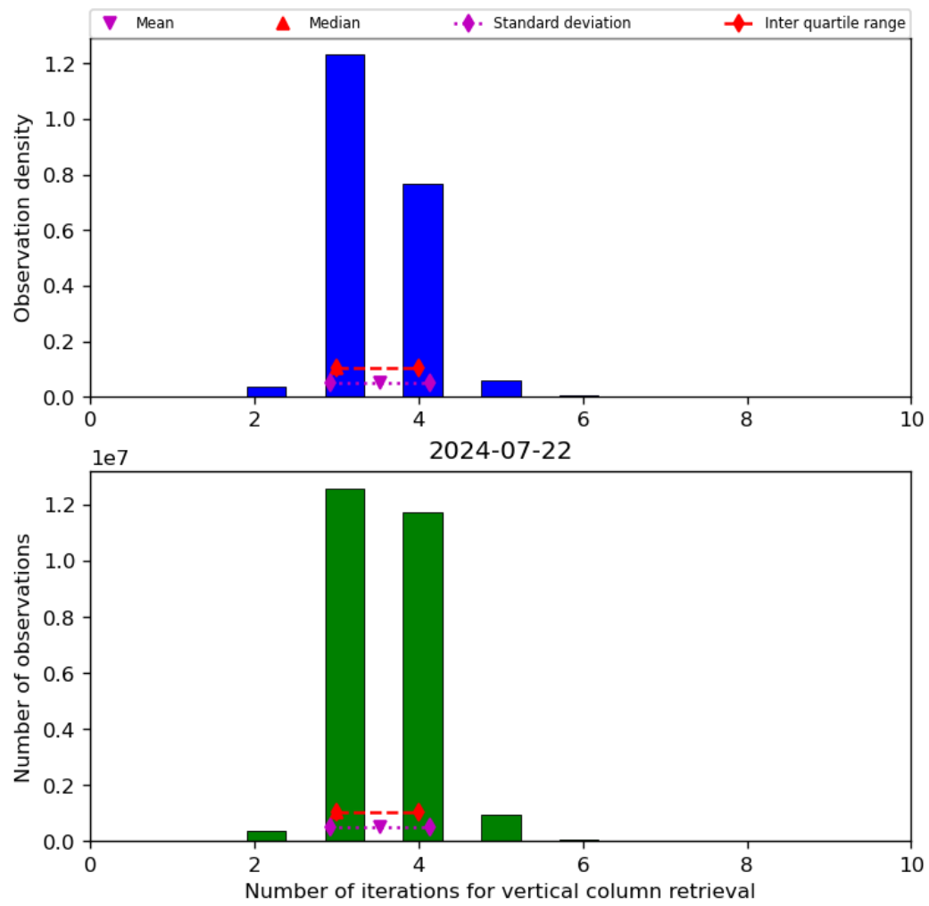
Figure 26: Histogram of “Number of iterations for vertical column retrieval” for 2024-07-21 to 2024-07-23
