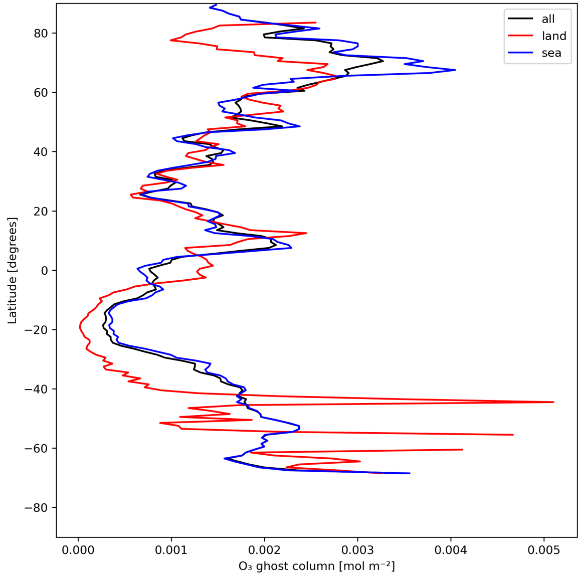
Figure 18: Zonal average of "O 3 ghost column" for 2024-07-21 to 2024-07-23.
