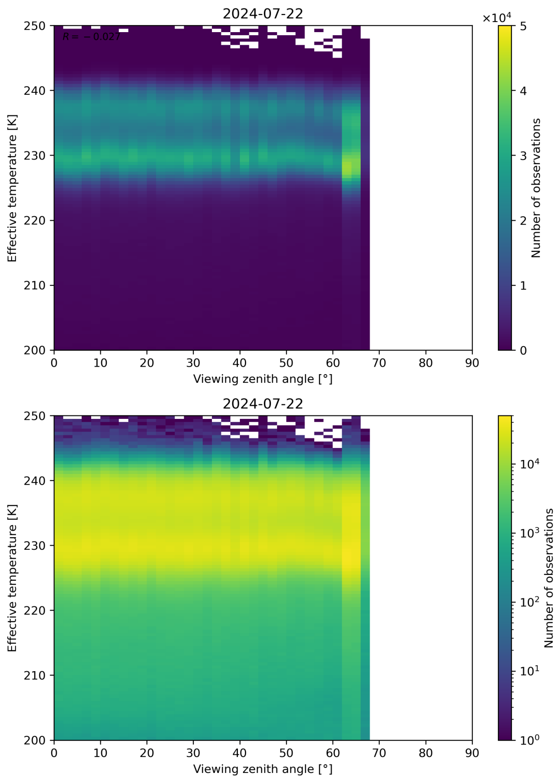
Figure 50: Scatter density plot of “Viewing zenith angle” against “Effective temperature” for 2024-07-21 to 2024-07-23.
