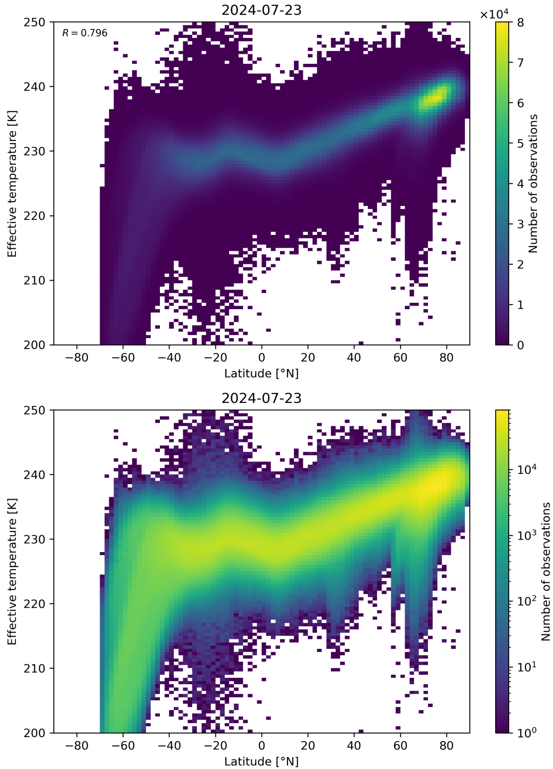
Figure 34: Scatter density plot of “Latitude” against “Effective temperature” for 2024-07-22 to 2024-07-24.
