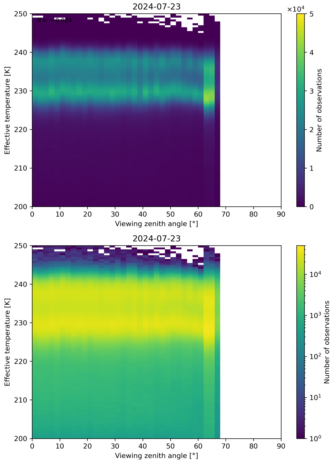
Figure 50: Scatter density plot of “Viewing zenith angle” against “Effective temperature” for 2024-07-22 to 2024-07-24.
