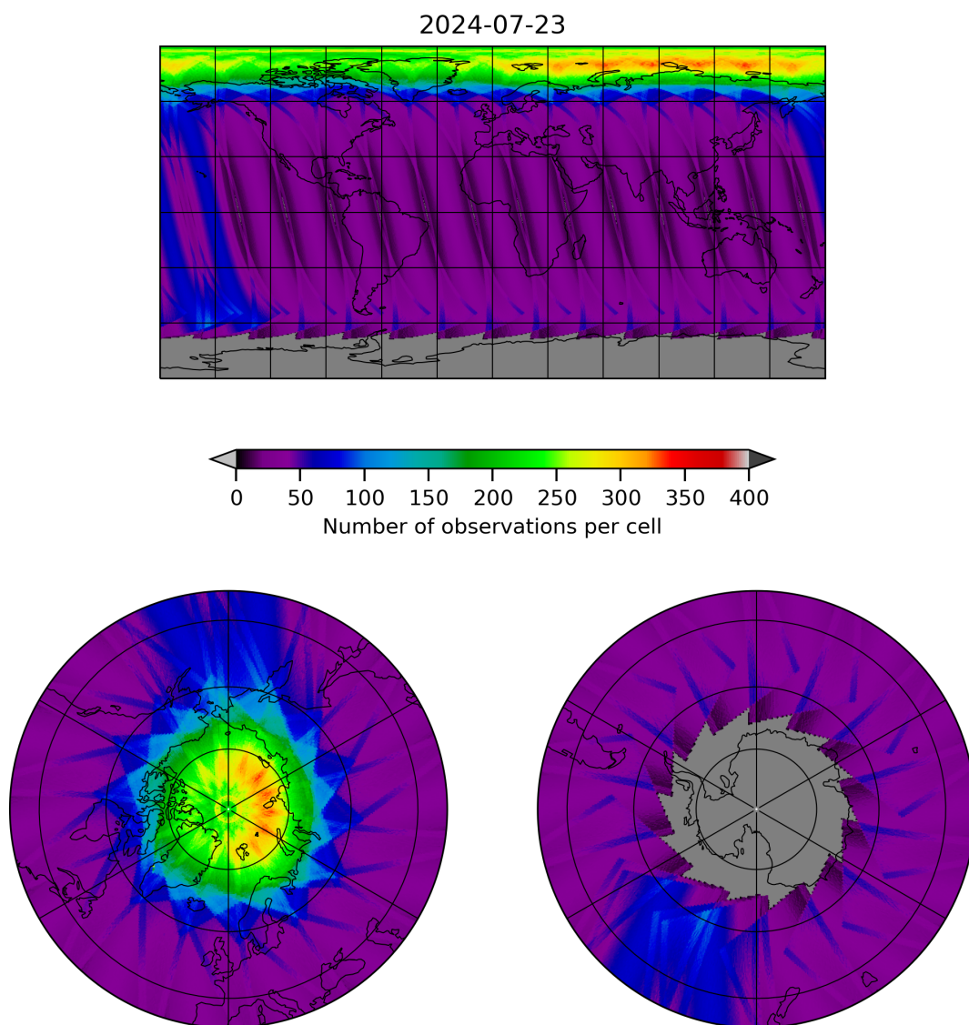
Figure 12: Map of the number of observations for 2024-07-22 to 2024-07-24
