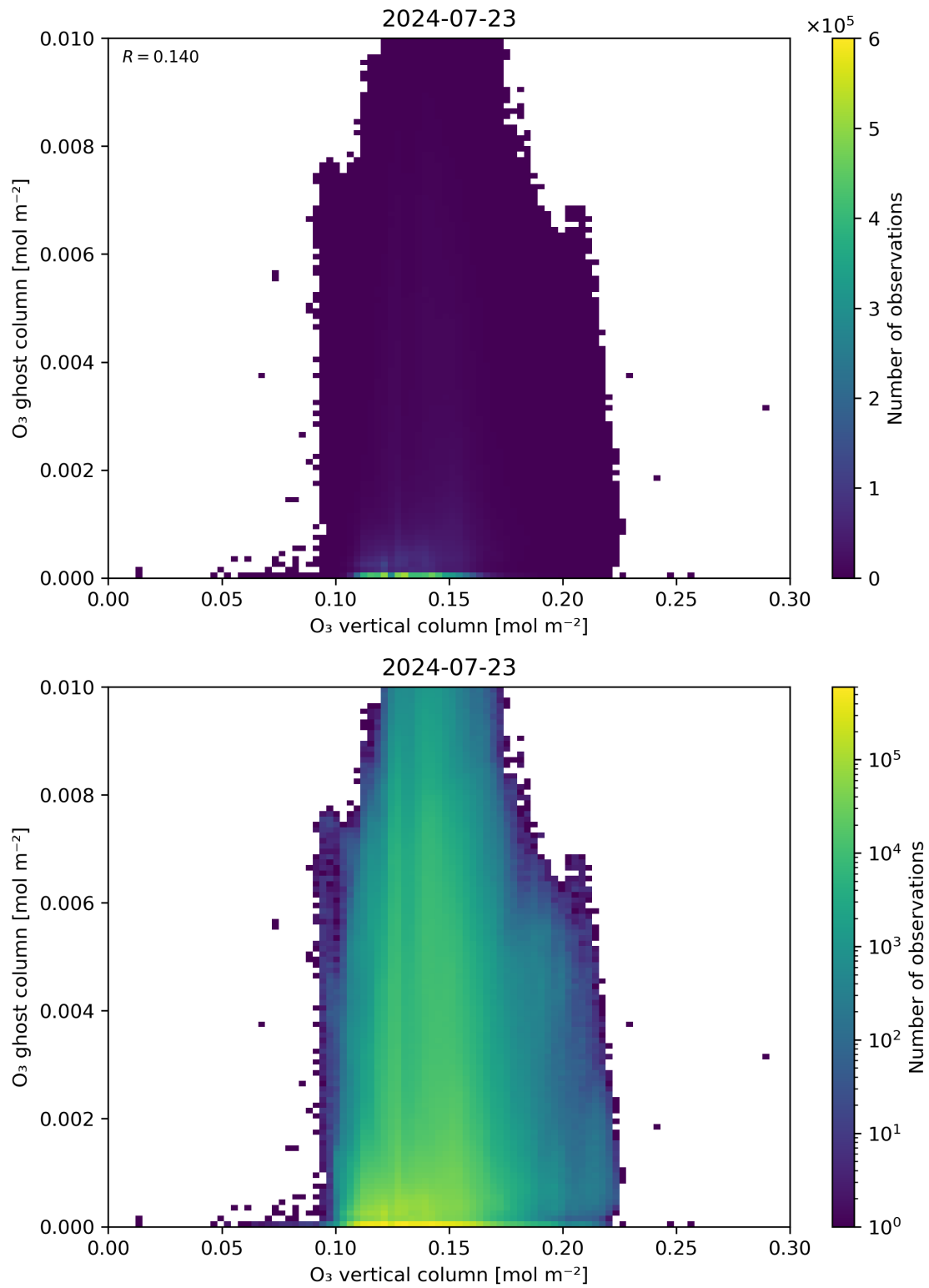
Figure 40: Scatter density plot of “O 3 vertical column” against “O 3 ghost column” for 2024-07-22 to 2024-07-24.
