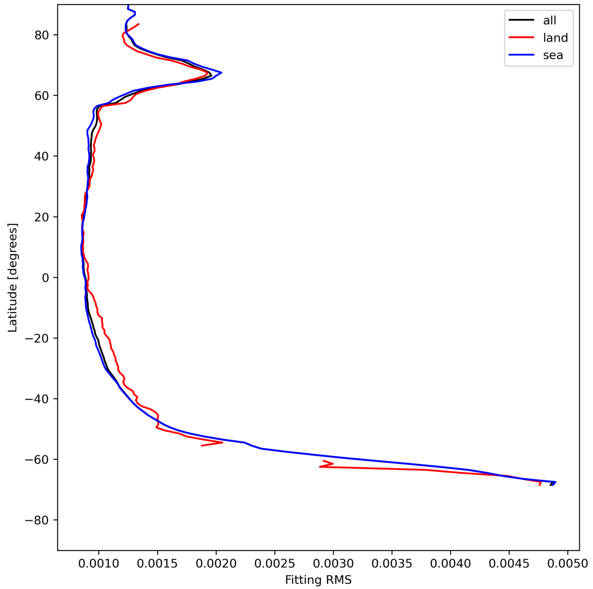
Figure 16: Zonal average of “Fitting RMS” for 2024-07-22 to 2024-07-24.
