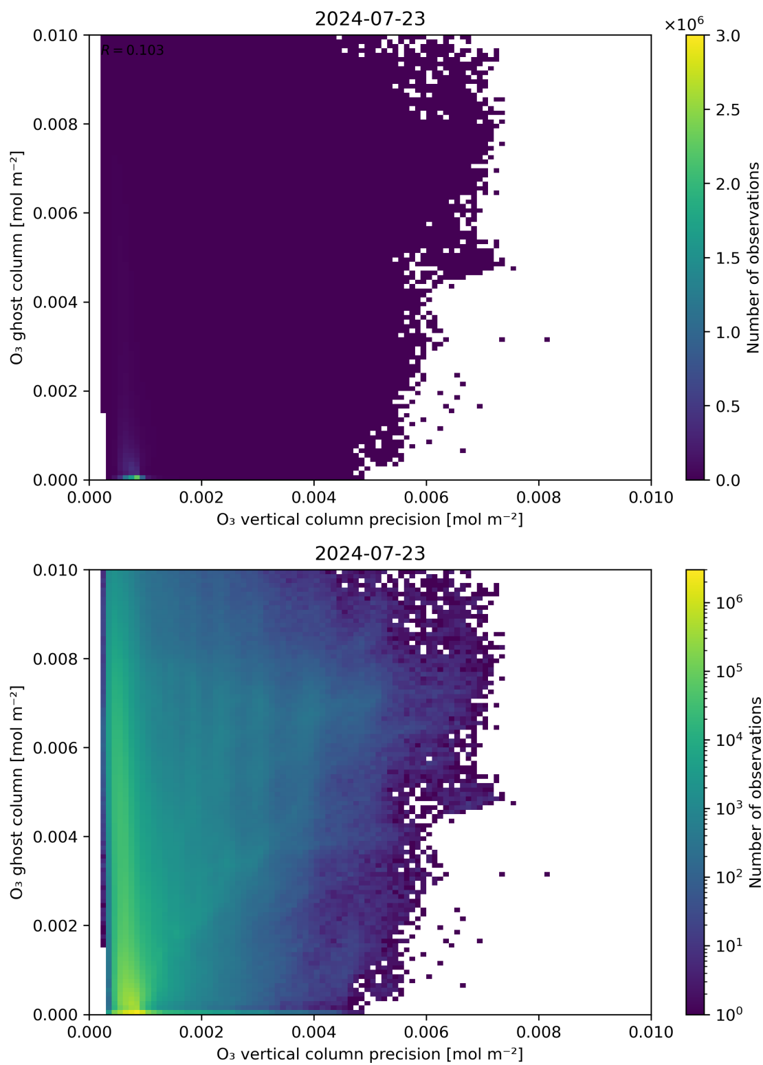
Figure 43: Scatter density plot of “ \text{O}_3 vertical column precision” against “ \text{O}_3 ghost column” for 2024-07-22 to 2024-07-24.
