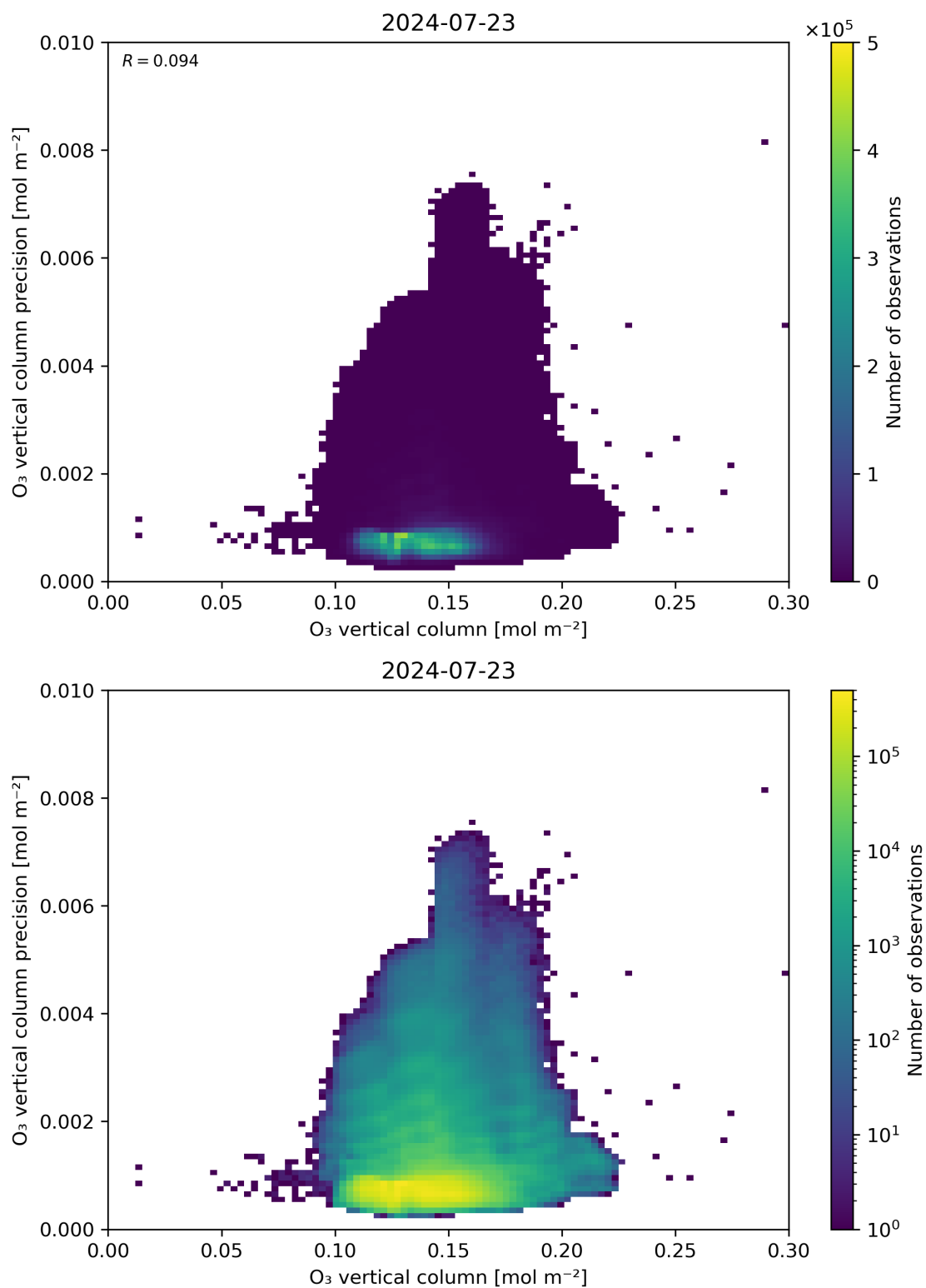
Figure 41: Scatter density plot of “O 3 vertical column” against “O 3 vertical column precision” for 2024-07-22 to 2024-07-24.
