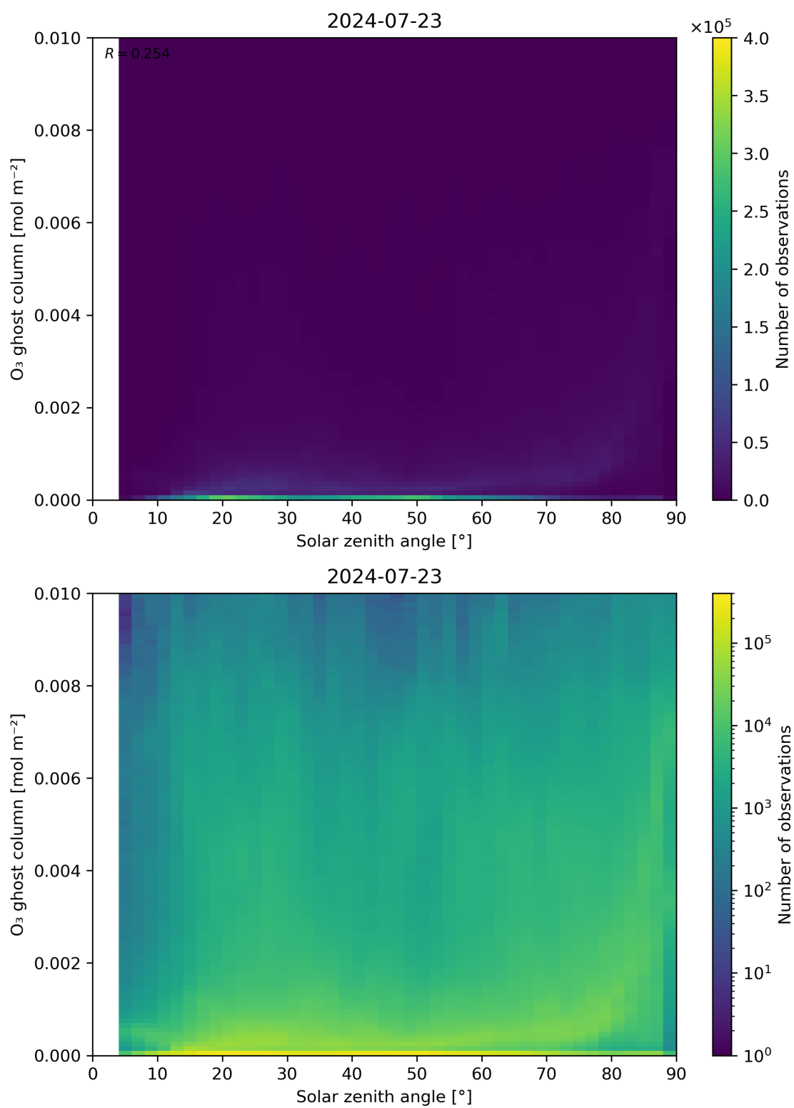
Figure 46: Scatter density plot of “Solar zenith angle” against “O 3 ghost column” for 2024-07-22 to 2024-07-24.
