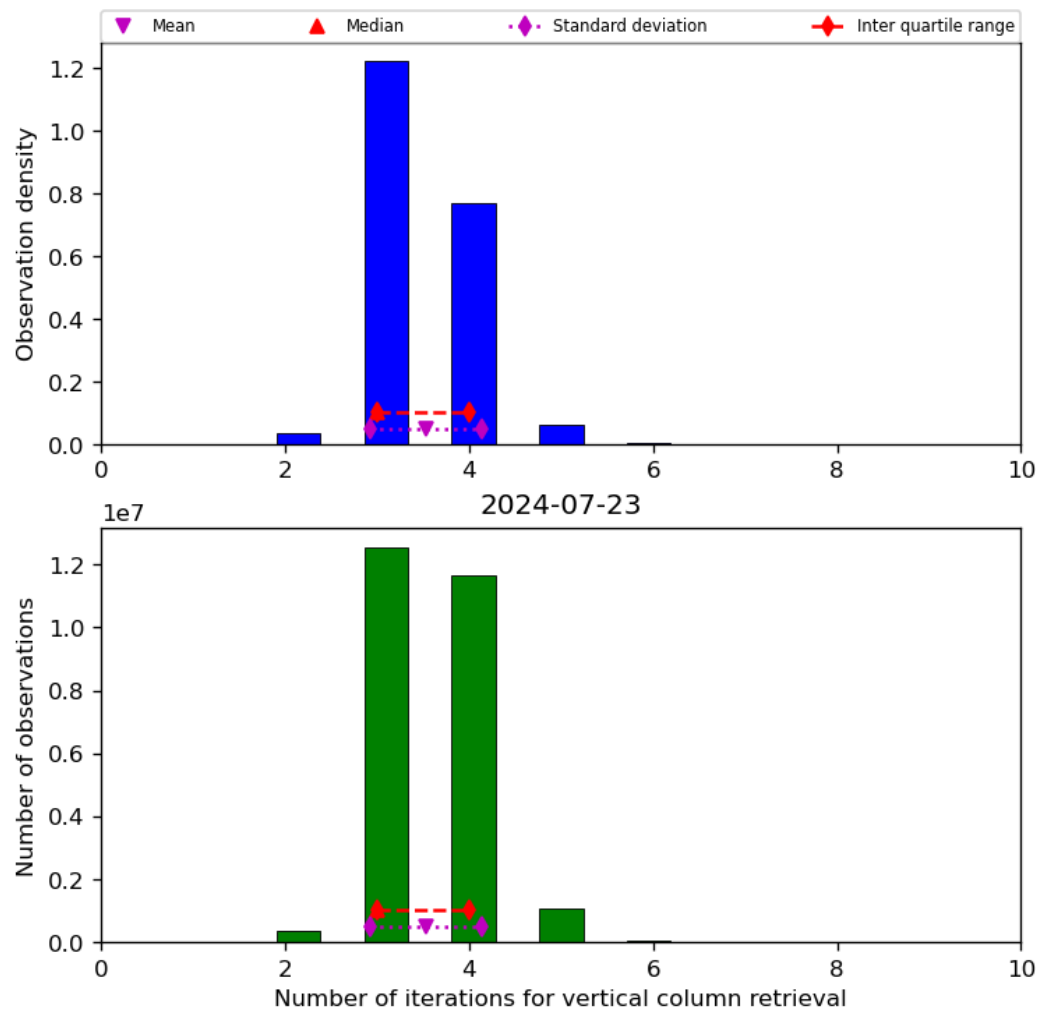
Figure 26: Histogram of “Number of iterations for vertical column retrieval” for 2024-07-22 to 2024-07-24
