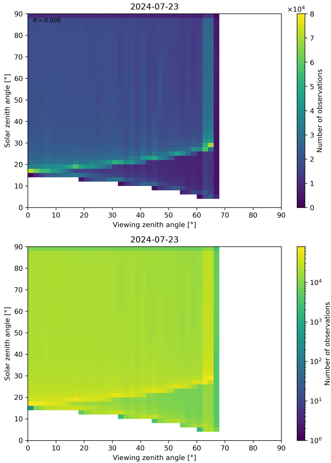
Figure 54: Scatter density plot of “Viewing zenith angle” against “Solar zenith angle” for 2024-07-22 to 2024-07-24.
