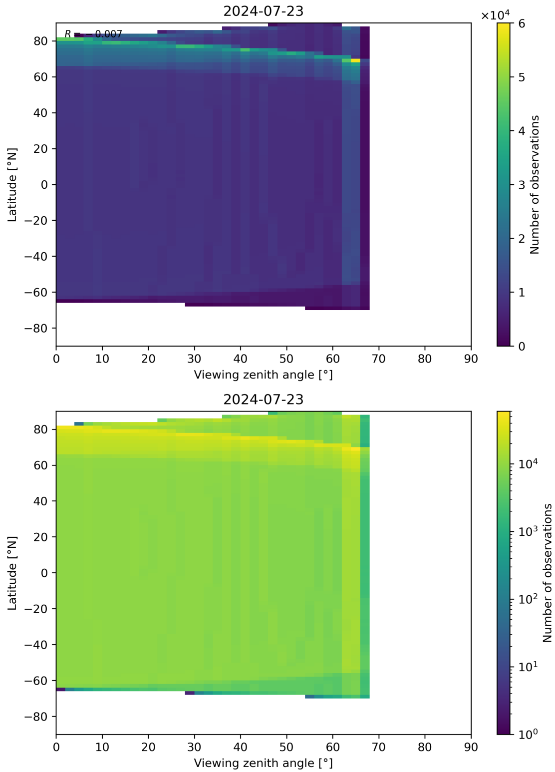
Figure 49: Scatter density plot of “Viewing zenith angle” against “Latitude” for 2024-07-22 to 2024-07-24.
