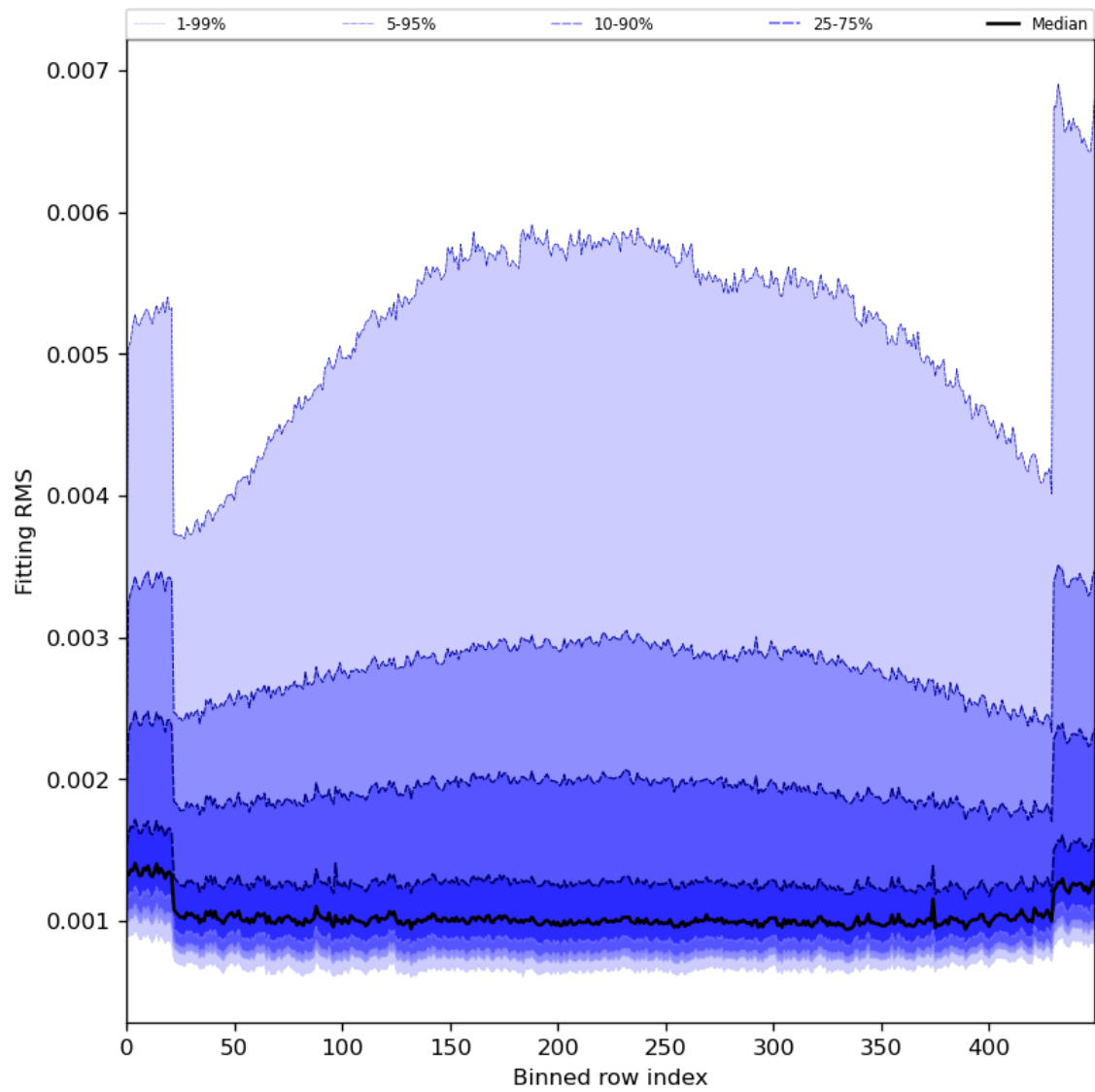
Figure 30: Along track statistics of “Fitting RMS” for 2024-07-22 to 2024-07-24
