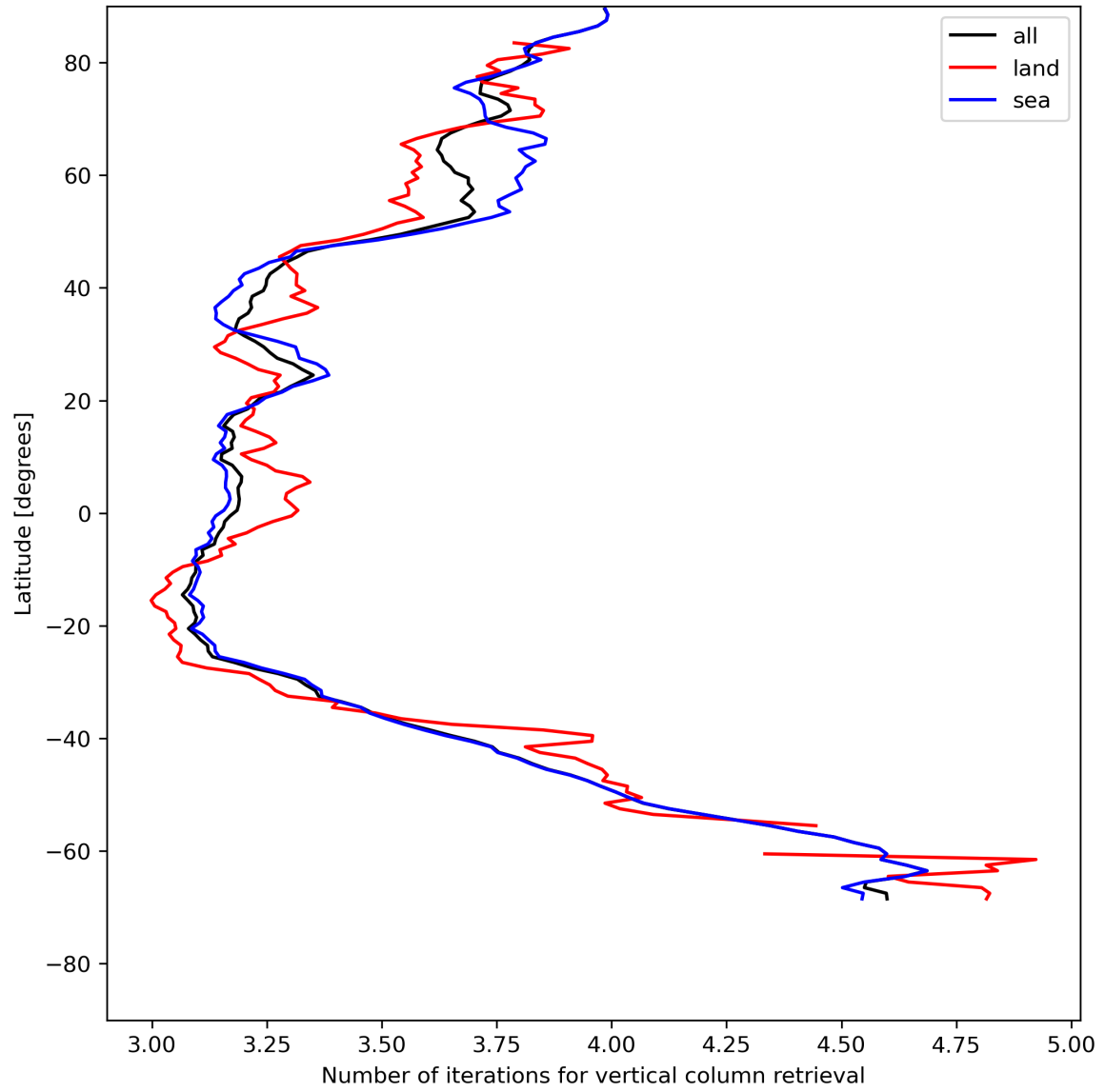
Figure 19: Zonal average of “Number of iterations for vertical column retrieval” for 2024-07-22 to 2024-07-24.
