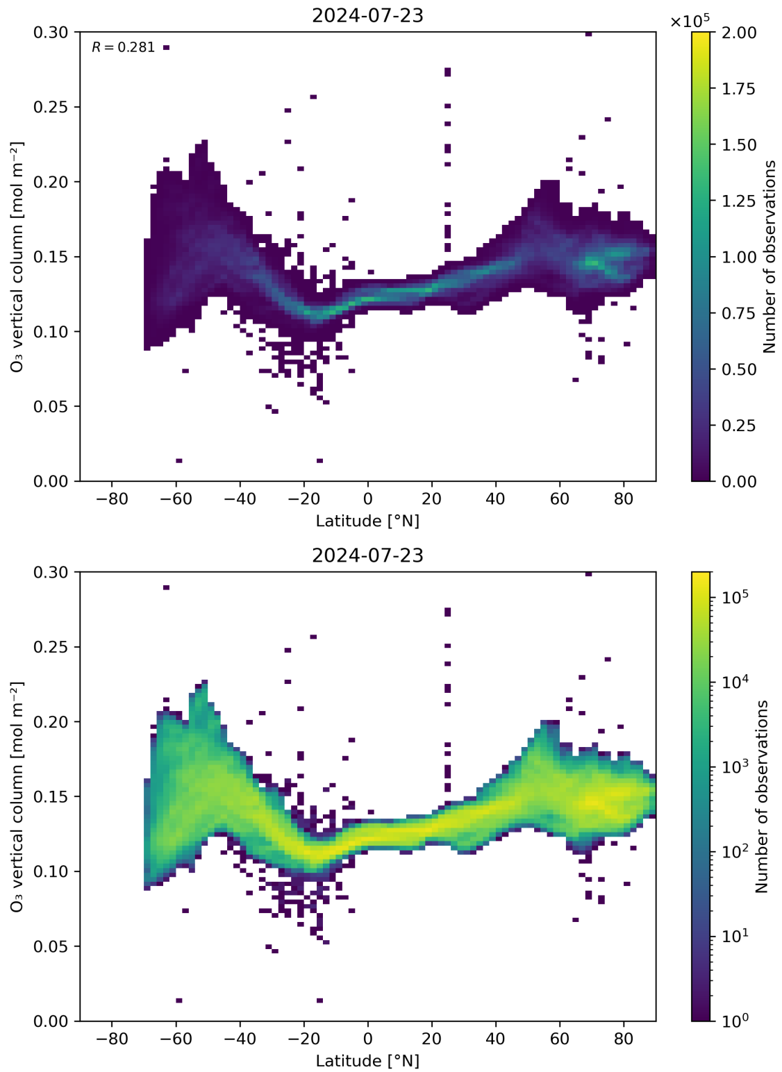
Figure 36: Scatter density plot of “Latitude” against “O 3 vertical column” for 2024-07-22 to 2024-07-24.
