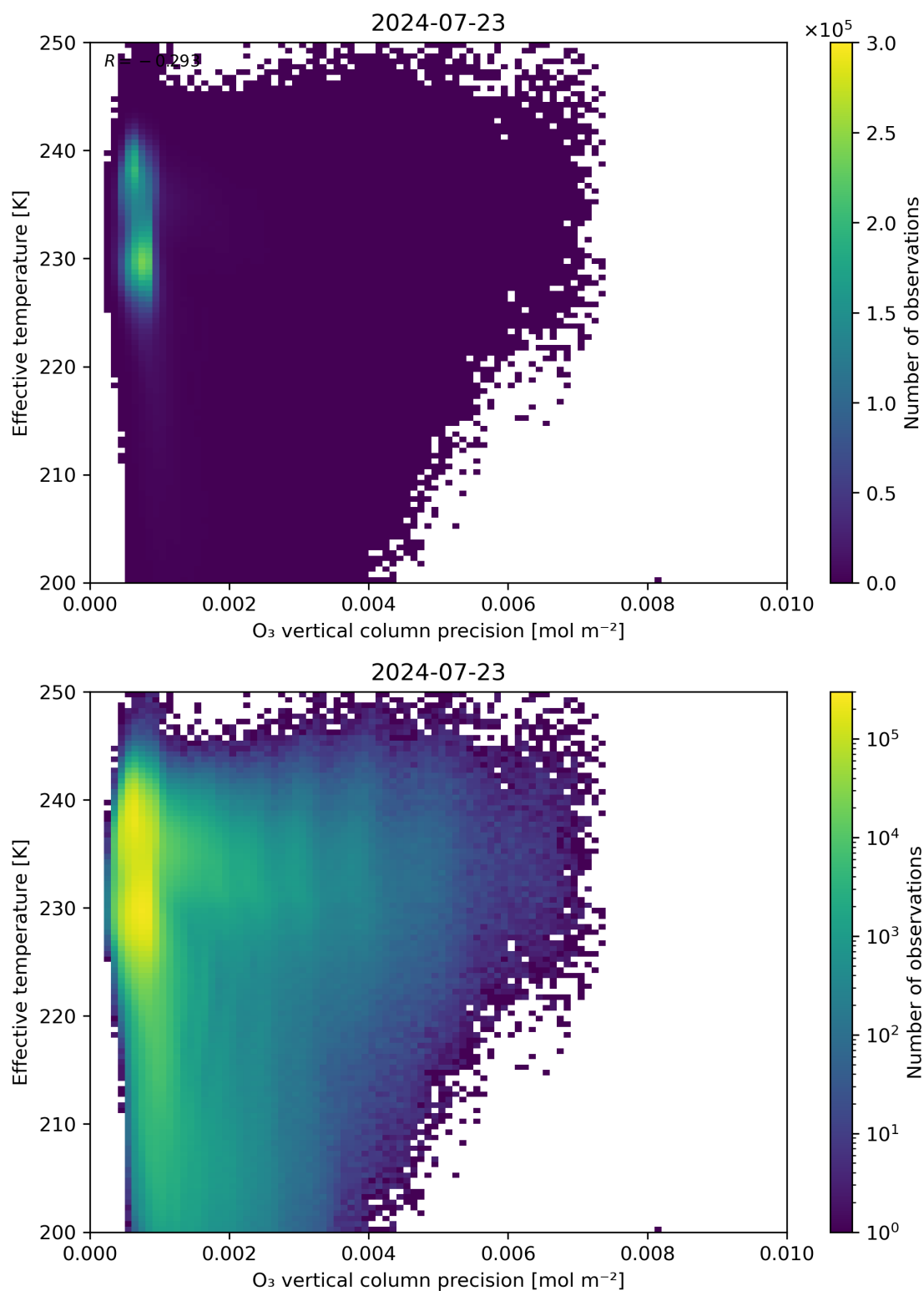
Figure 42: Scatter density plot of “O 3 vertical column precision” against “Effective temperature” for 2024-07-22 to 2024-07-24.
