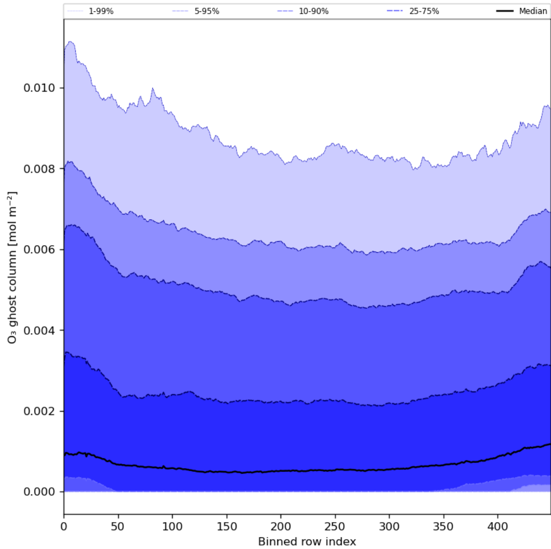
Figure 32: Along track statistics of “O 3 ghost column” for 2024-07-22 to 2024-07-24
