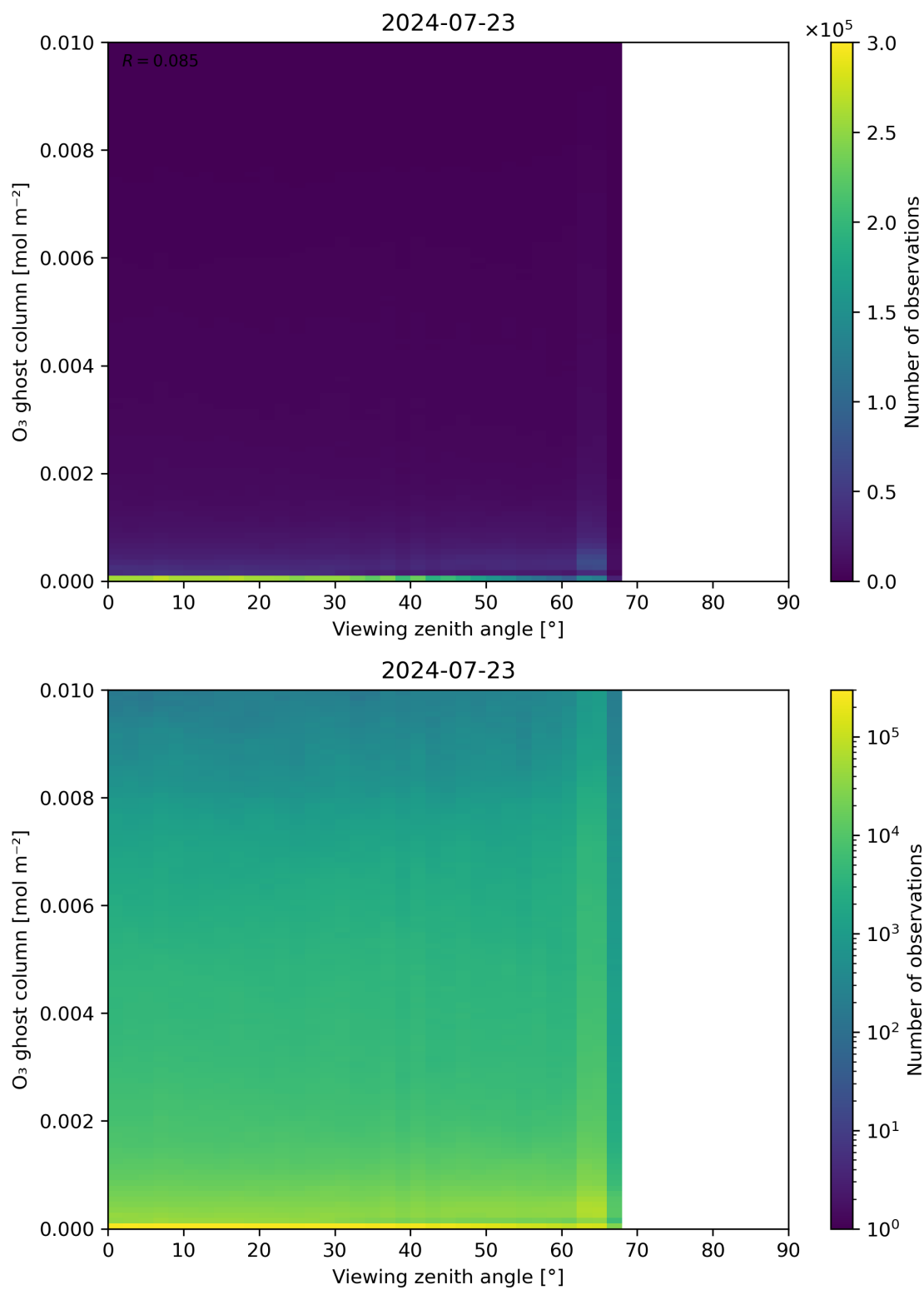
Figure 51: Scatter density plot of “Viewing zenith angle” against “O 3 ghost column” for 2024-07-22 to 2024-07-24.
