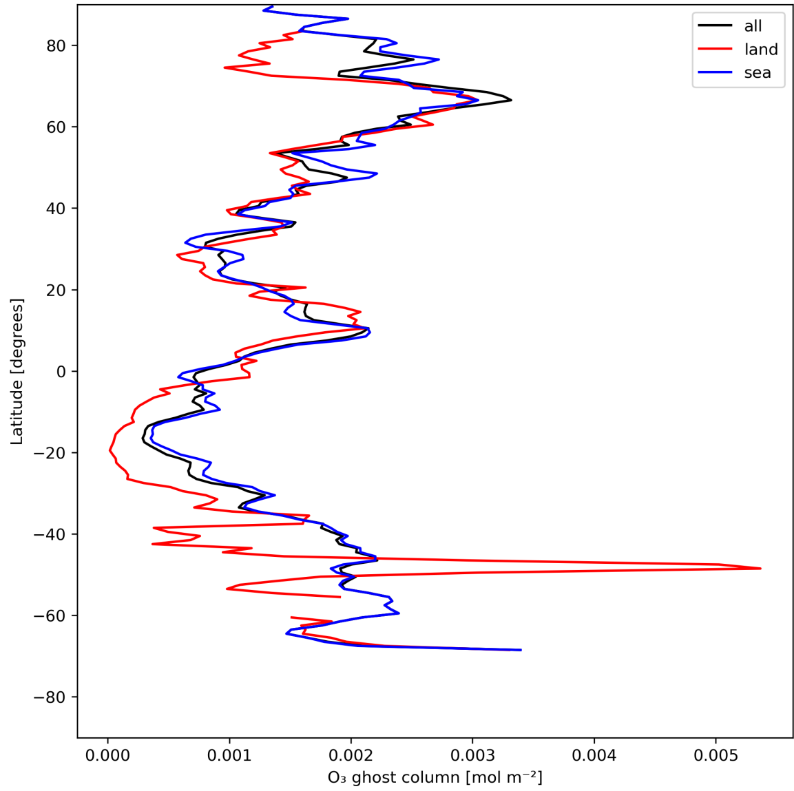
Figure 18: Zonal average of "O 3 ghost column" for 2024-07-22 to 2024-07-24.
