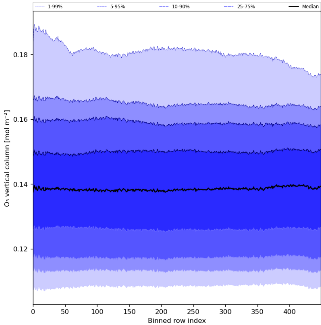
Figure 28: Along track statistics of “O 3 vertical column” for 2024-07-22 to 2024-07-24
