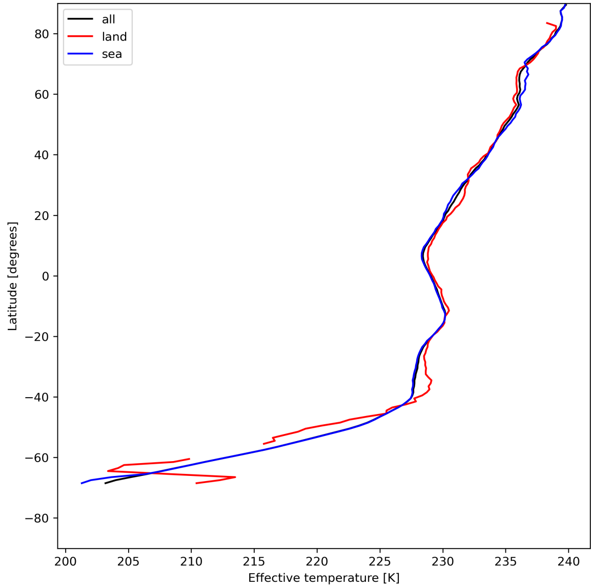
Figure 17: Zonal average of "Effective temperature" for 2024-07-22 to 2024-07-24.
