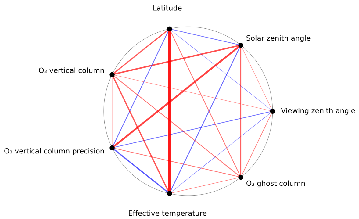
Figure 1: Map of correlation graph for 2024-07-22 to 2024-07-24.
