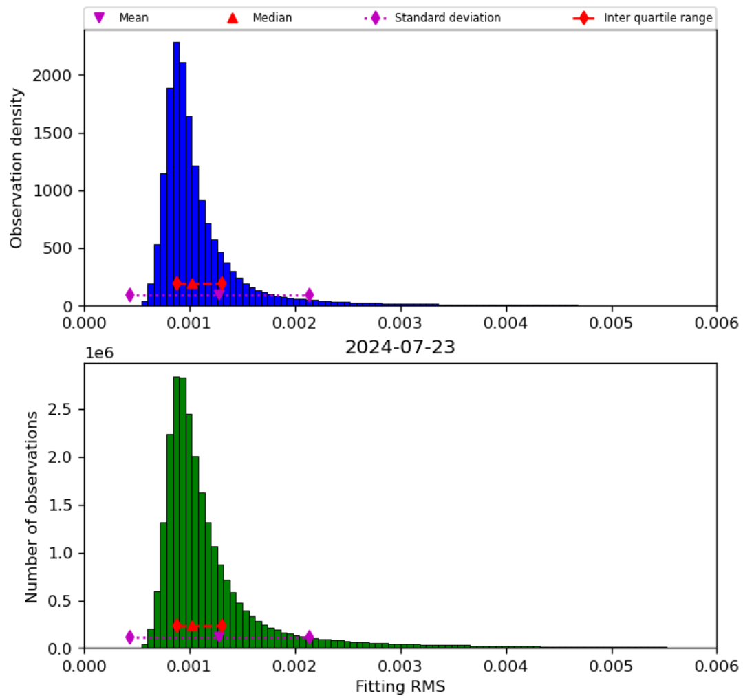
Figure 23: Histogram of “Fitting RMS” for 2024-07-22 to 2024-07-24
