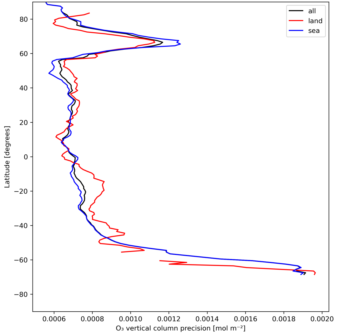
Figure 15: Zonal average of “O 3 vertical column precision” for 2024-07-22 to 2024-07-24.
