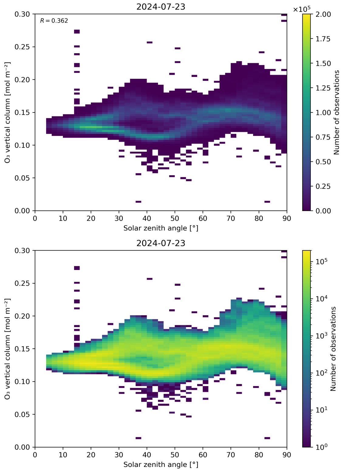
Figure 47: Scatter density plot of “Solar zenith angle” against “O 3 vertical column” for 2024-07-22 to 2024-07-24.
