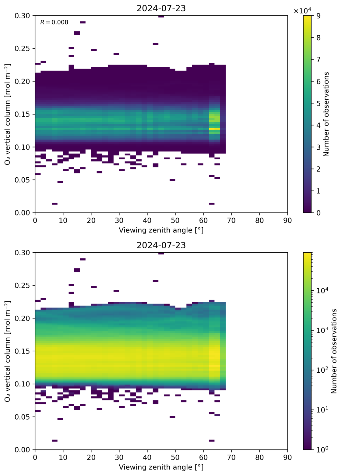
Figure 52: Scatter density plot of “Viewing zenith angle” against “O 3 vertical column” for 2024-07-22 to 2024-07-24.
