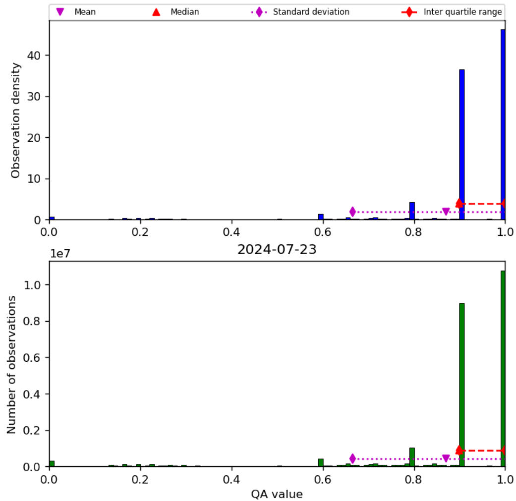
Figure 20: Histogram of “QA value” for 2024-07-22 to 2024-07-24
