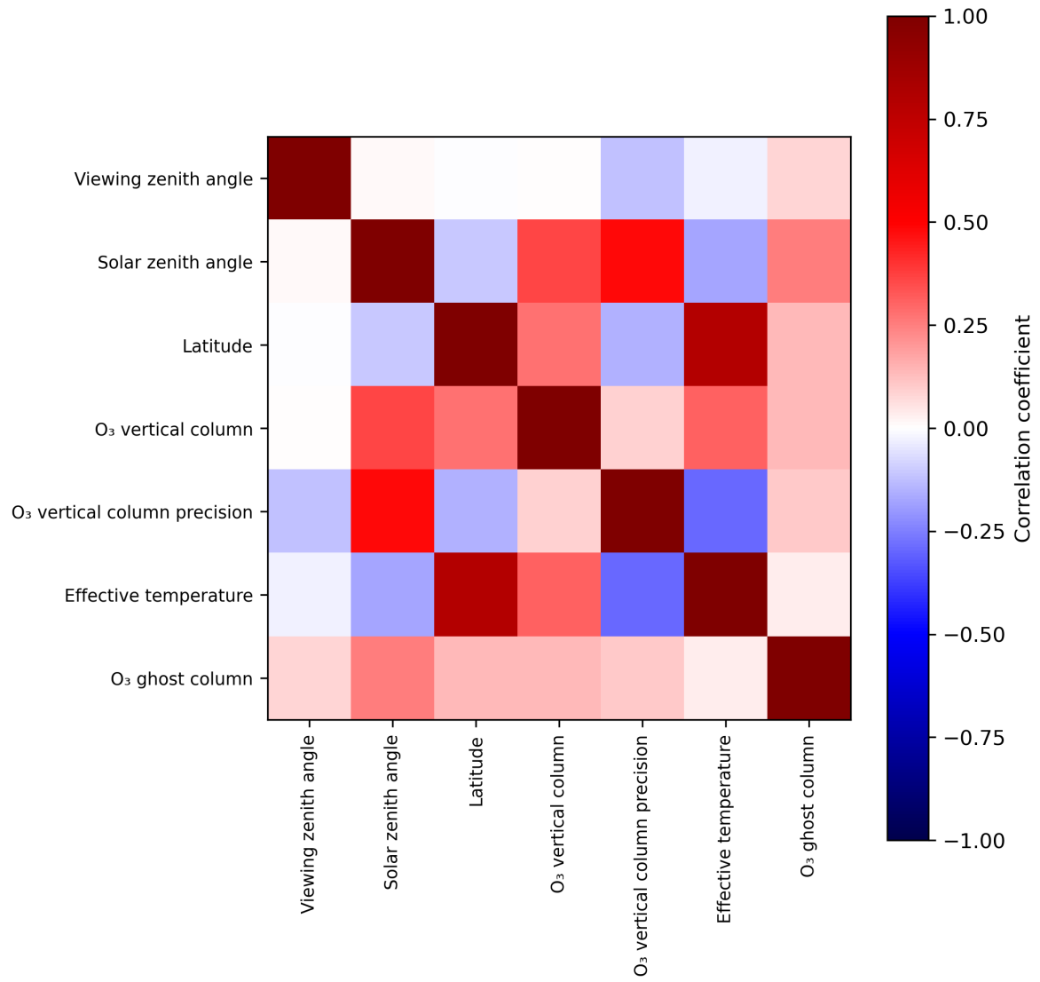
Figure 2: Map of correlation matrix for 2024-07-22 to 2024-07-24.
