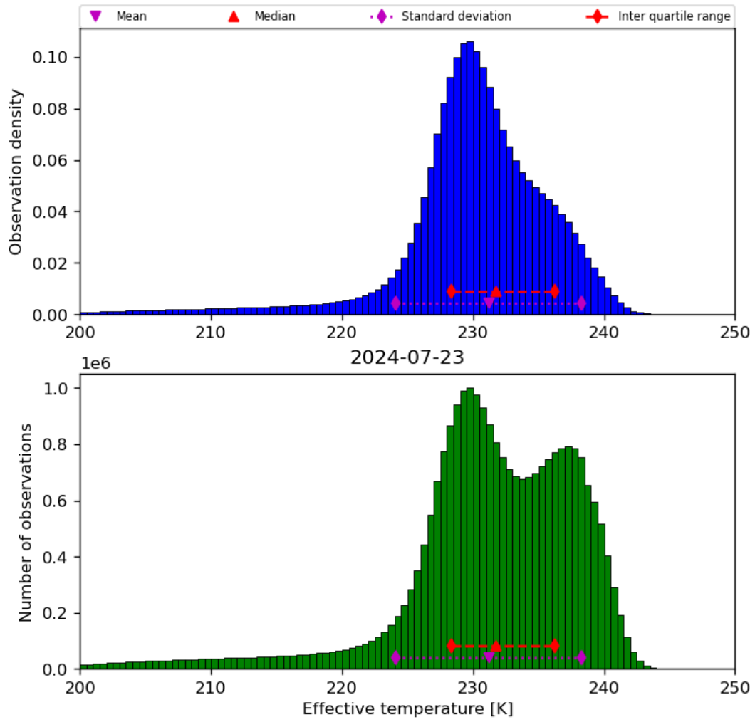
Figure 24: Histogram of “Effective temperature” for 2024-07-22 to 2024-07-24
