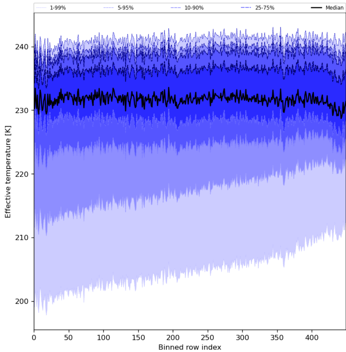
Figure 31: Along track statistics of “Effective temperature” for 2024-07-22 to 2024-07-24
