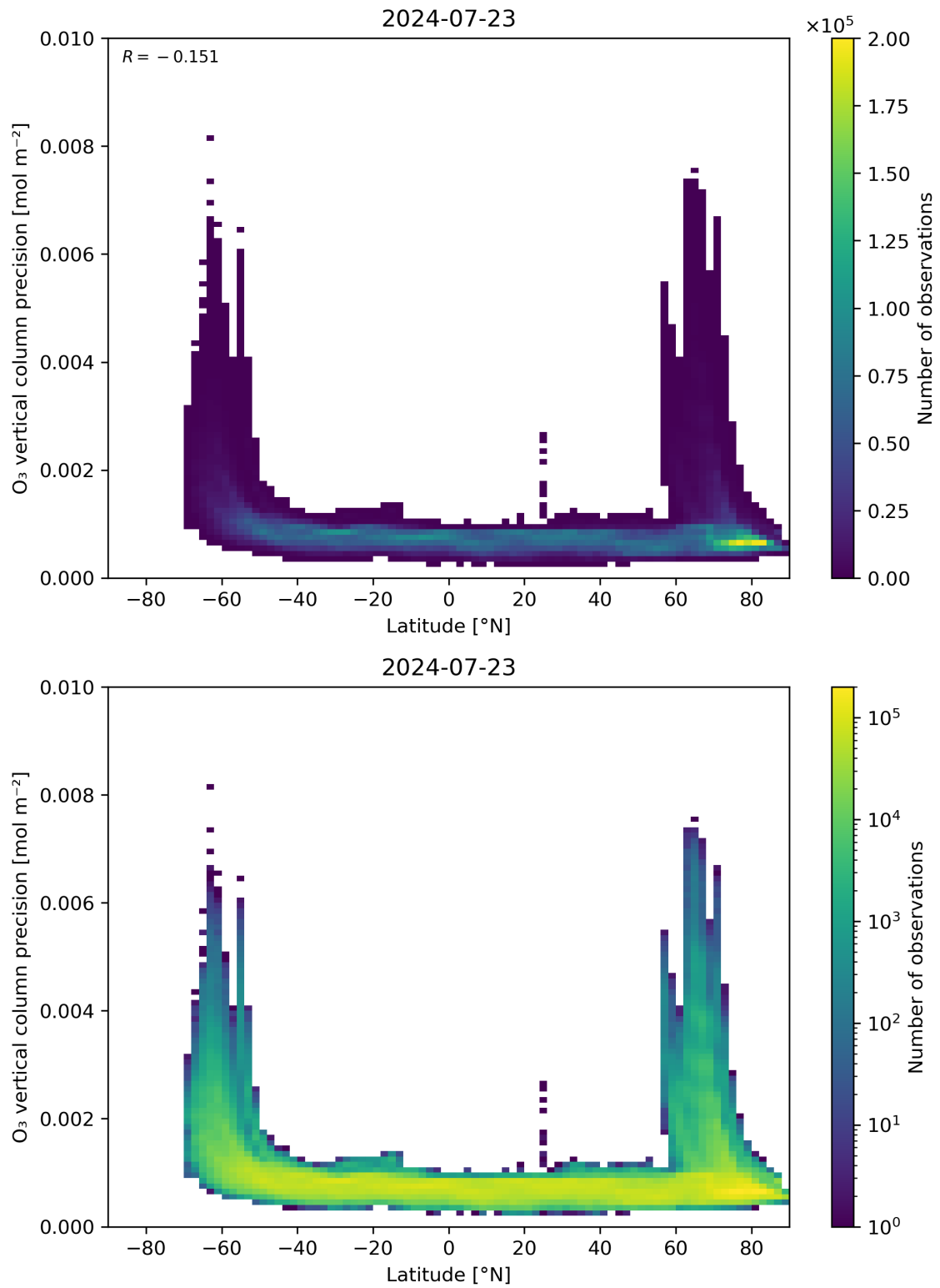
Figure 37: Scatter density plot of “Latitude” against “O 3 vertical column precision” for 2024-07-22 to 2024-07-24.
