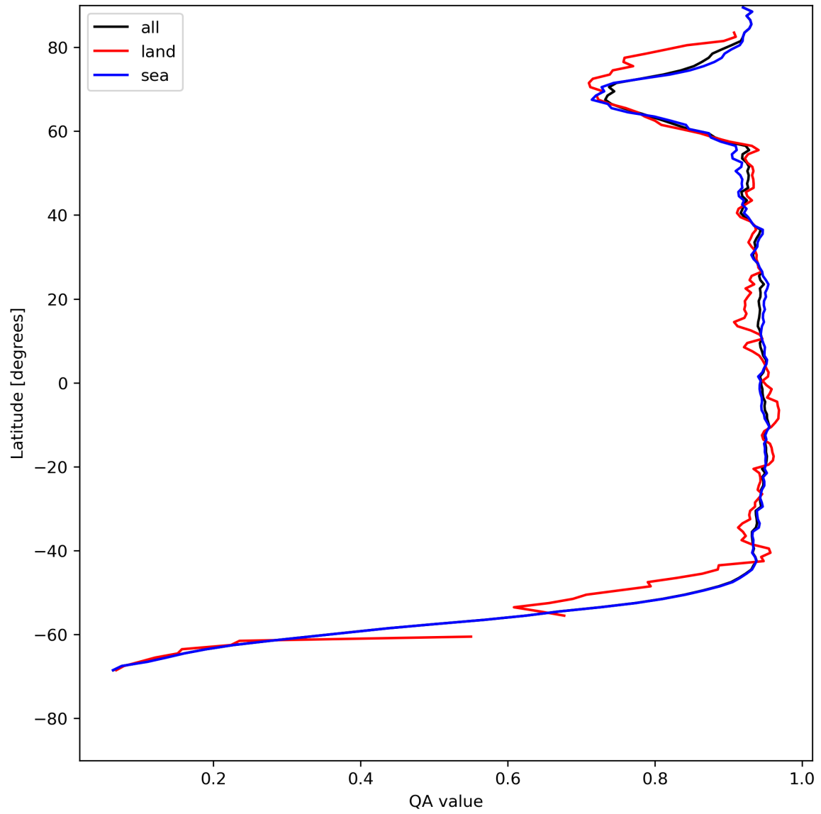
Figure 13: Zonal average of “QA value” for 2024-07-22 to 2024-07-24.
