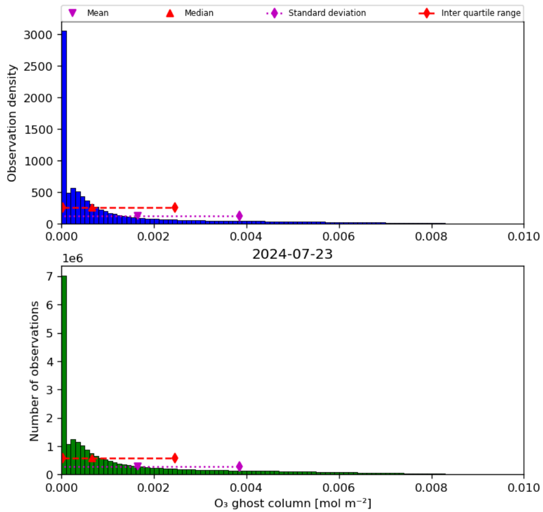
Figure 25: Histogram of “O 3 ghost column” for 2024-07-22 to 2024-07-24
