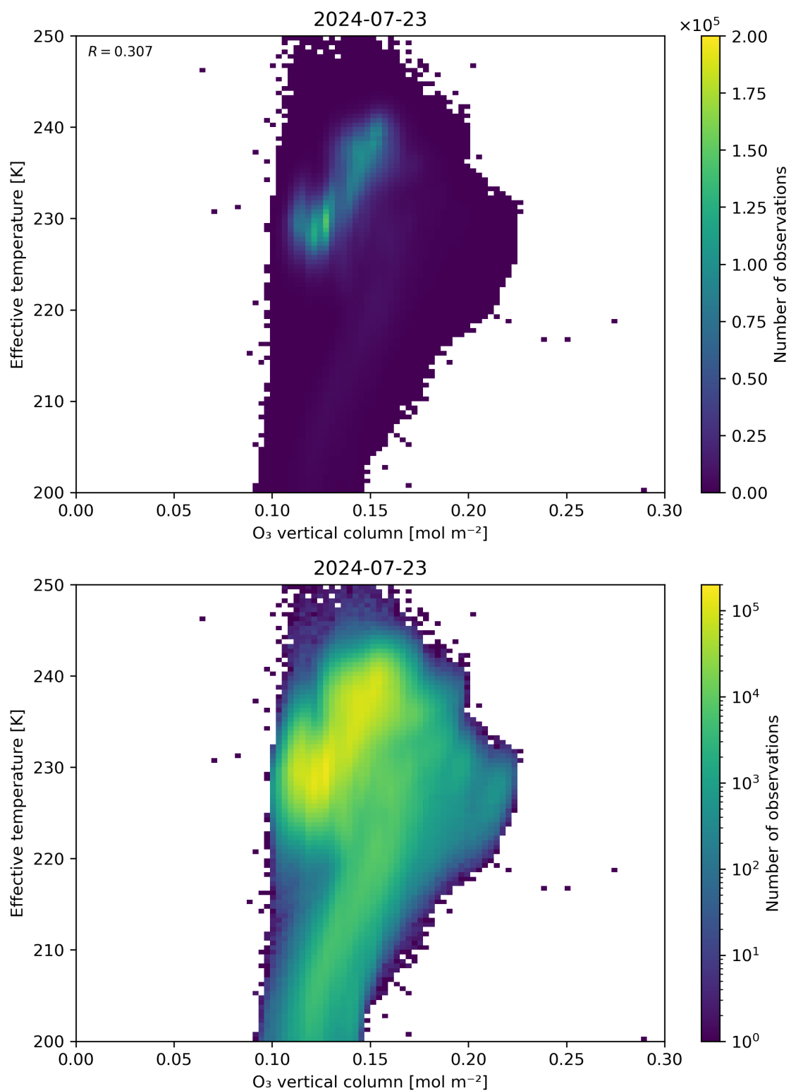
Figure 39: Scatter density plot of “O 3 vertical column” against “Effective temperature” for 2024-07-22 to 2024-07-24.
