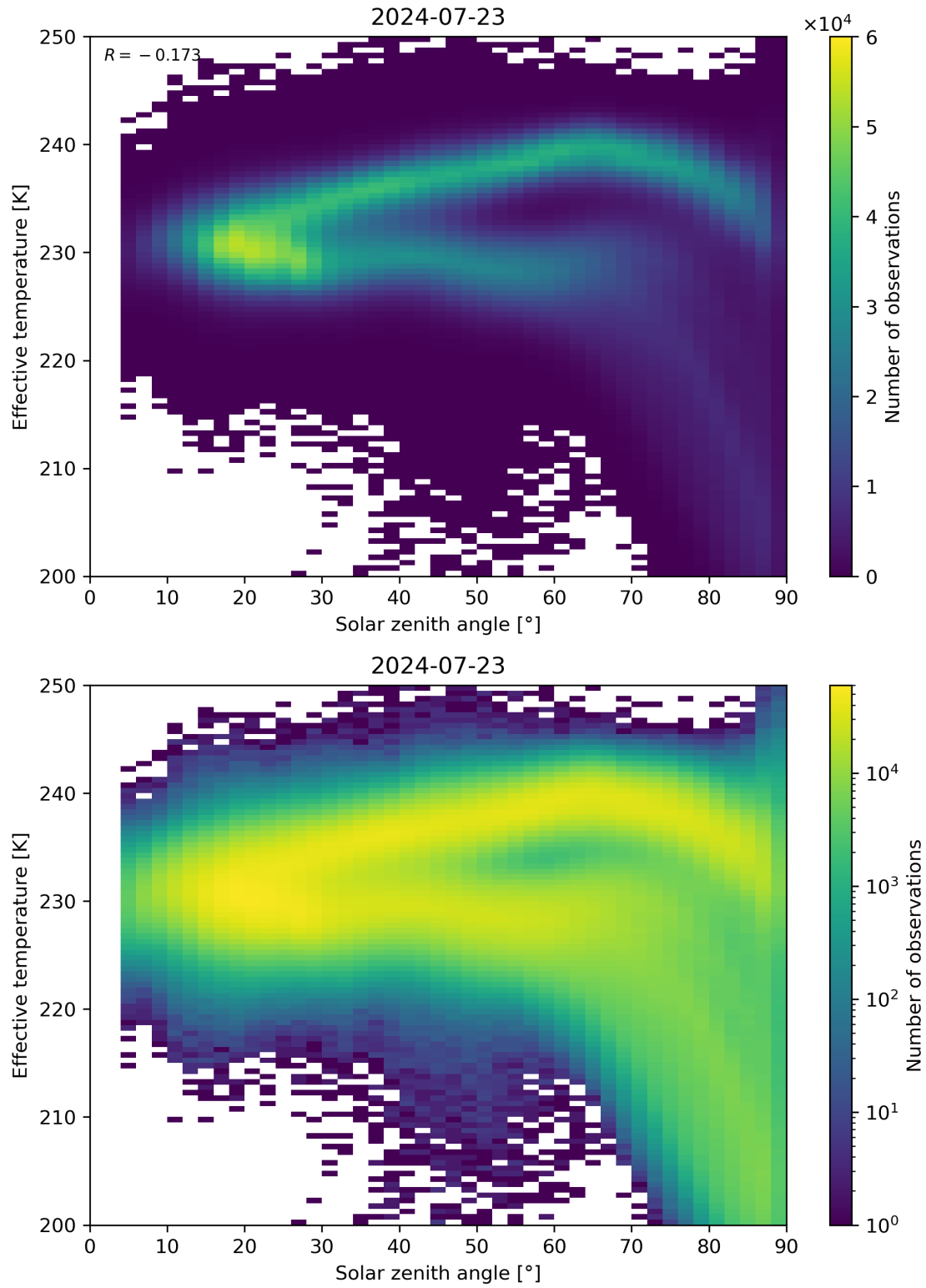
Figure 45: Scatter density plot of “Solar zenith angle” against “Effective temperature” for 2024-07-22 to 2024-07-24.
