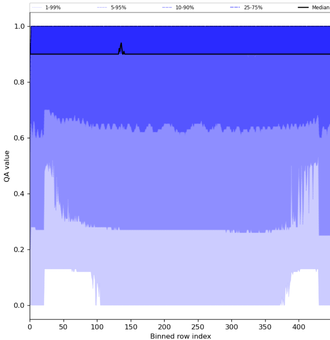
Figure 27: Along track statistics of “QA value” for 2024-07-22 to 2024-07-24
