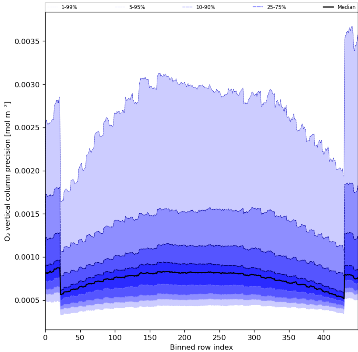
Figure 29: Along track statistics of “O 3 vertical column precision” for 2024-07-22 to 2024-07-24
