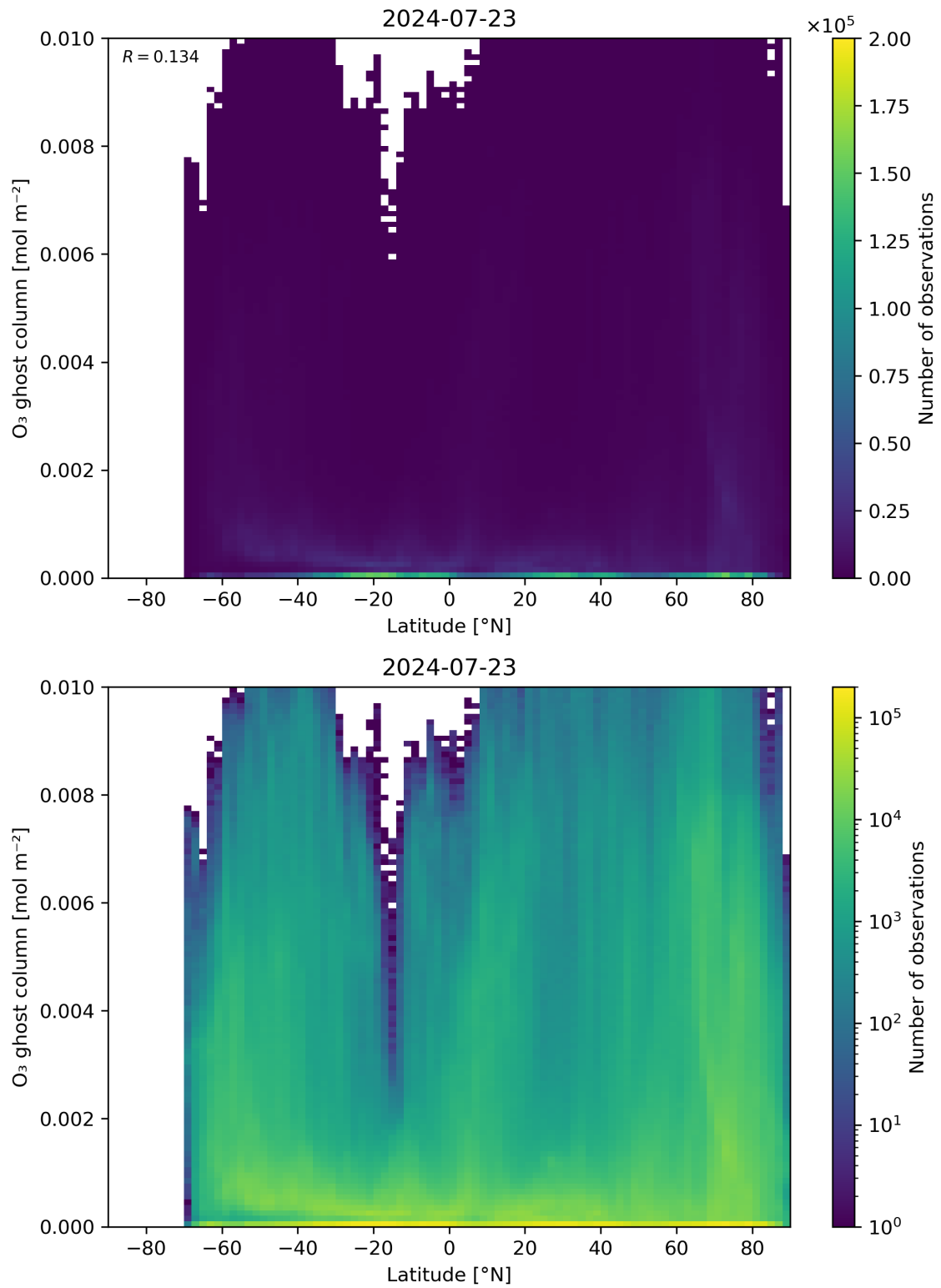
Figure 35: Scatter density plot of “Latitude” against “O 3 ghost column” for 2024-07-22 to 2024-07-24.
