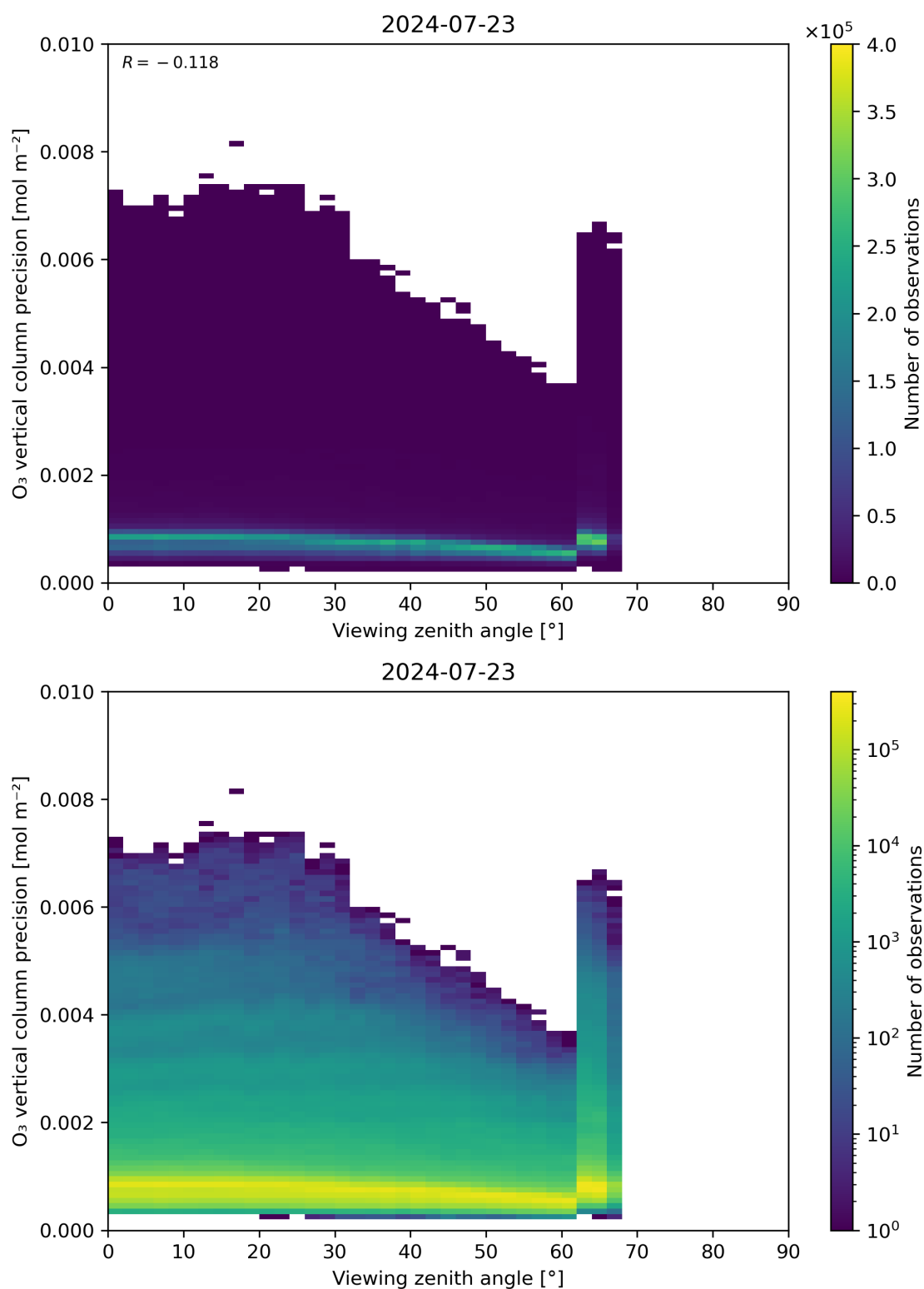
Figure 53: Scatter density plot of “Viewing zenith angle” against “O 3 vertical column precision” for 2024-07-22 to 2024-07-24.
