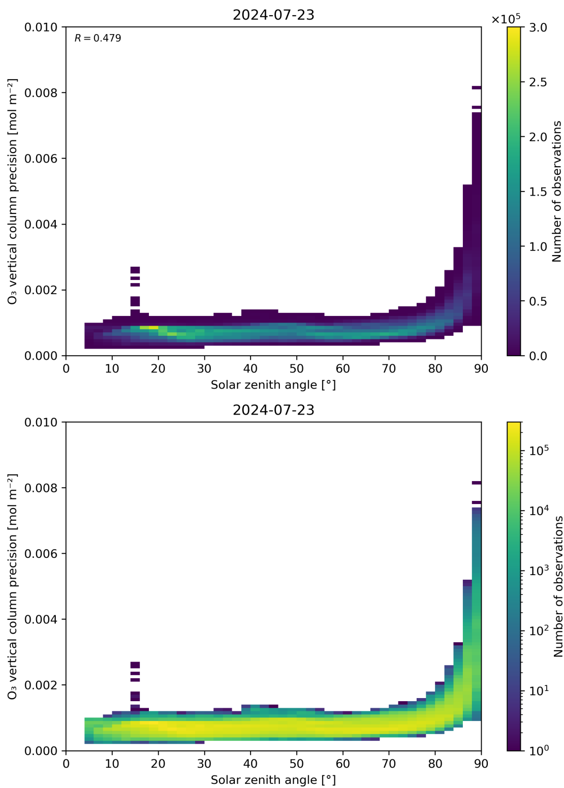
Figure 48: Scatter density plot of “Solar zenith angle” against “O 3 vertical column precision” for 2024-07-22 to 2024-07-24.
