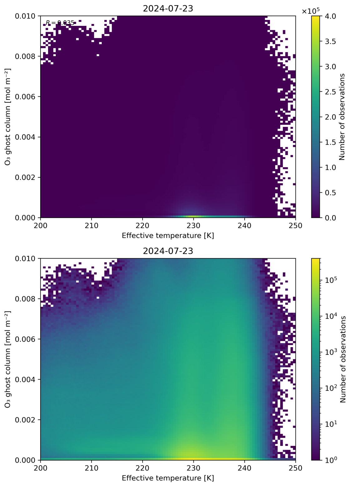
Figure 38: Scatter density plot of “Effective temperature” against “O 3 ghost column” for 2024-07-22 to 2024-07-24.
