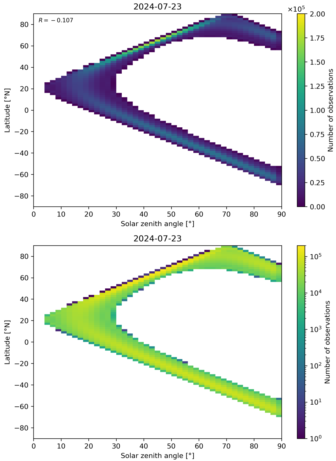
Figure 44: Scatter density plot of “Solar zenith angle” against “Latitude” for 2024-07-22 to 2024-07-24.
