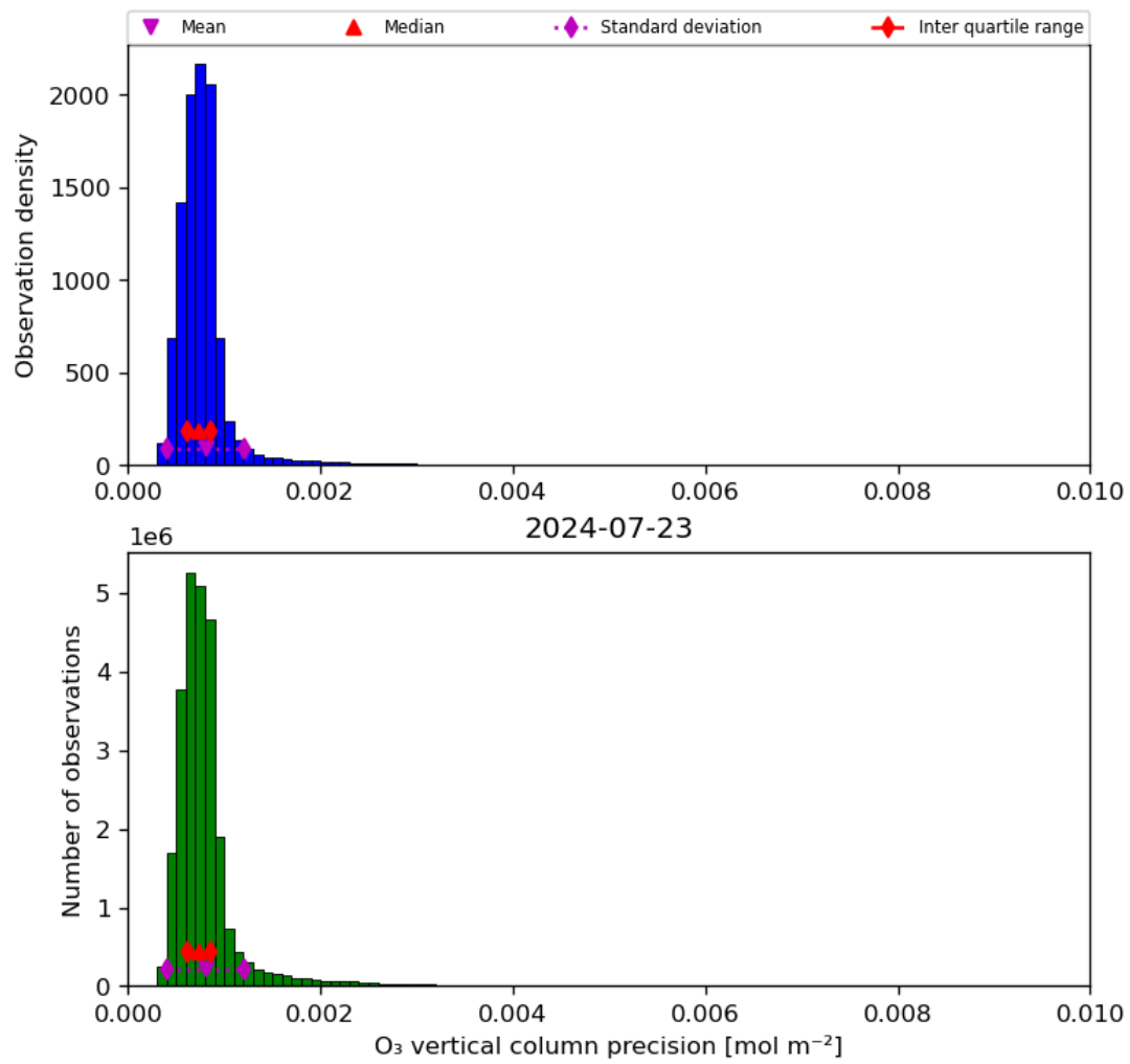
Figure 22: Histogram of “O 3 vertical column precision” for 2024-07-22 to 2024-07-24
