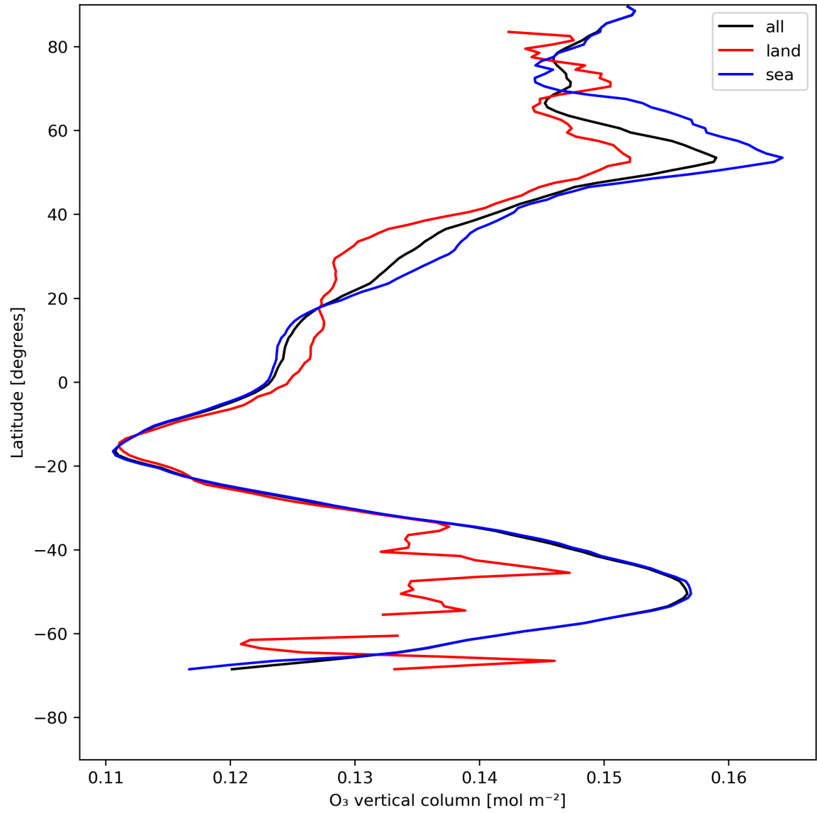
Figure 14: Zonal average of “O 3 vertical column” for 2024-07-22 to 2024-07-24.
