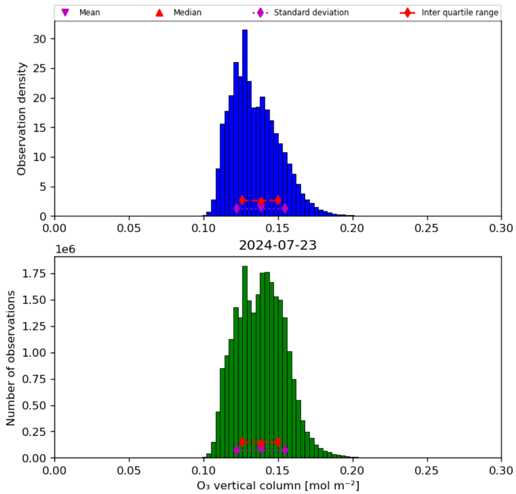
Figure 21: Histogram of “O 3 vertical column” for 2024-07-22 to 2024-07-24
