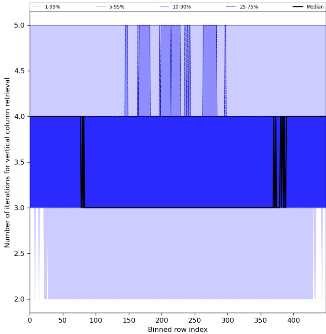
Figure 33: Along track statistics of “Number of iterations for vertical column retrieval” for 2024-07-22 to 2024-07-24
