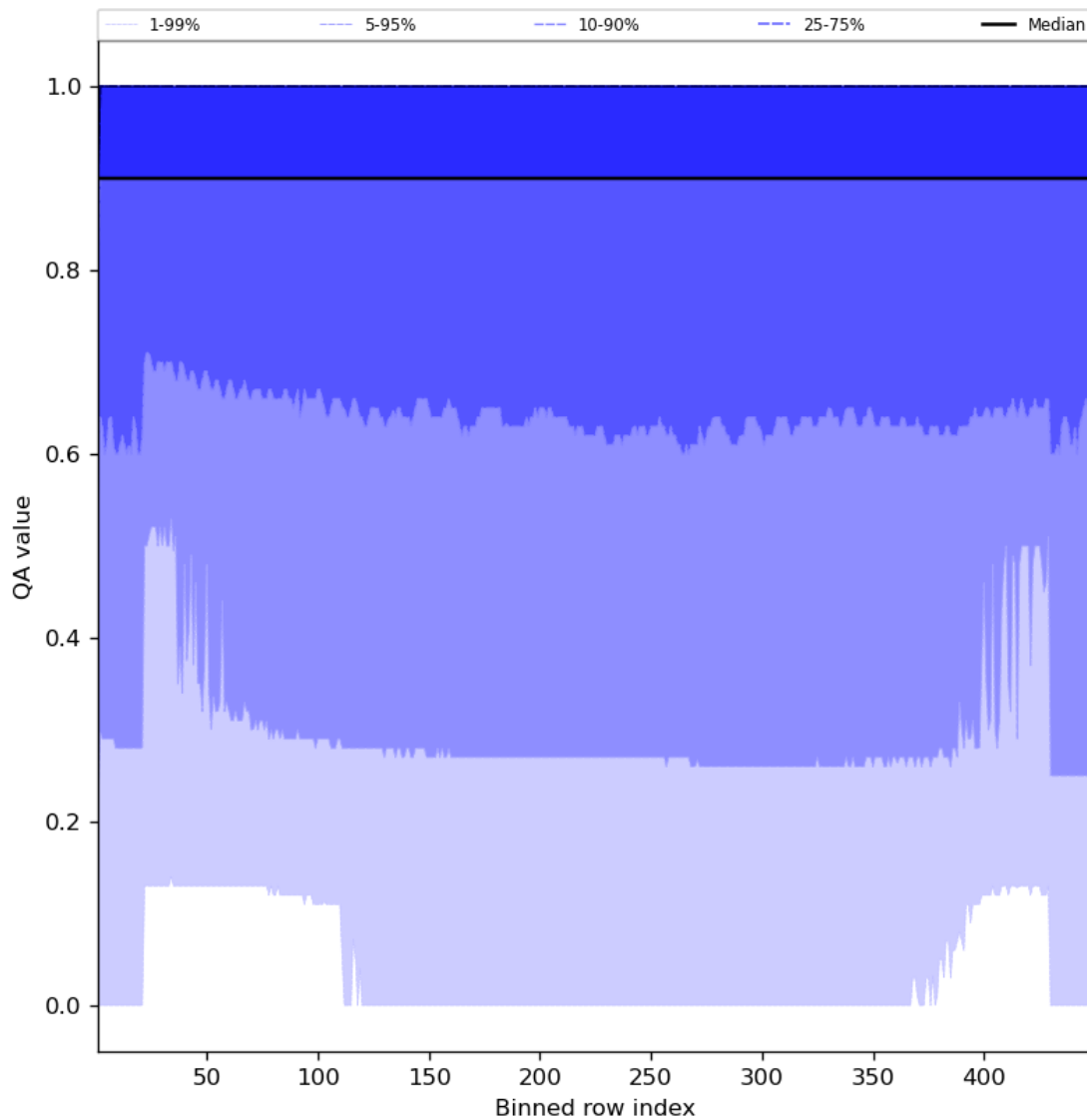
Figure 27: Along track statistics of “QA value” for 2024-07-24 to 2024-07-26
