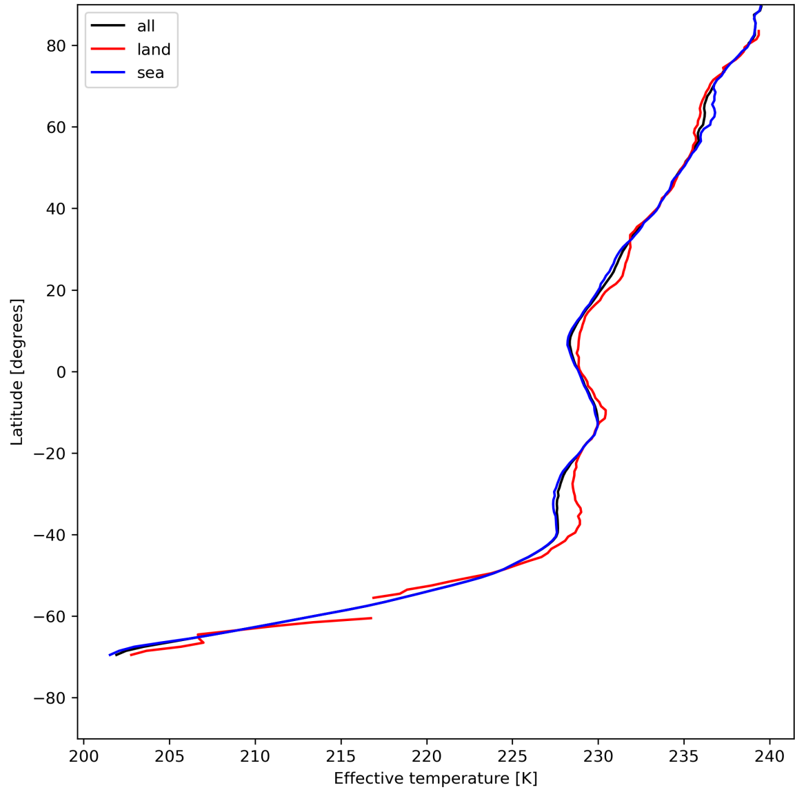
Figure 17: Zonal average of “Effective temperature” for 2024-07-24 to 2024-07-26.
