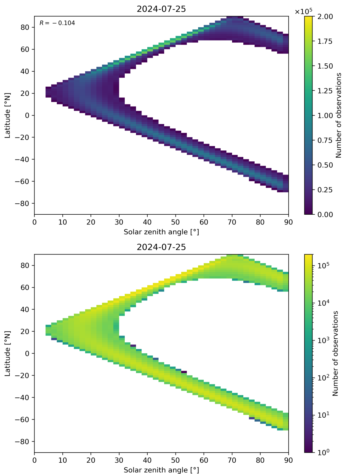
Figure 44: Scatter density plot of “Solar zenith angle” against “Latitude” for 2024-07-24 to 2024-07-26.
