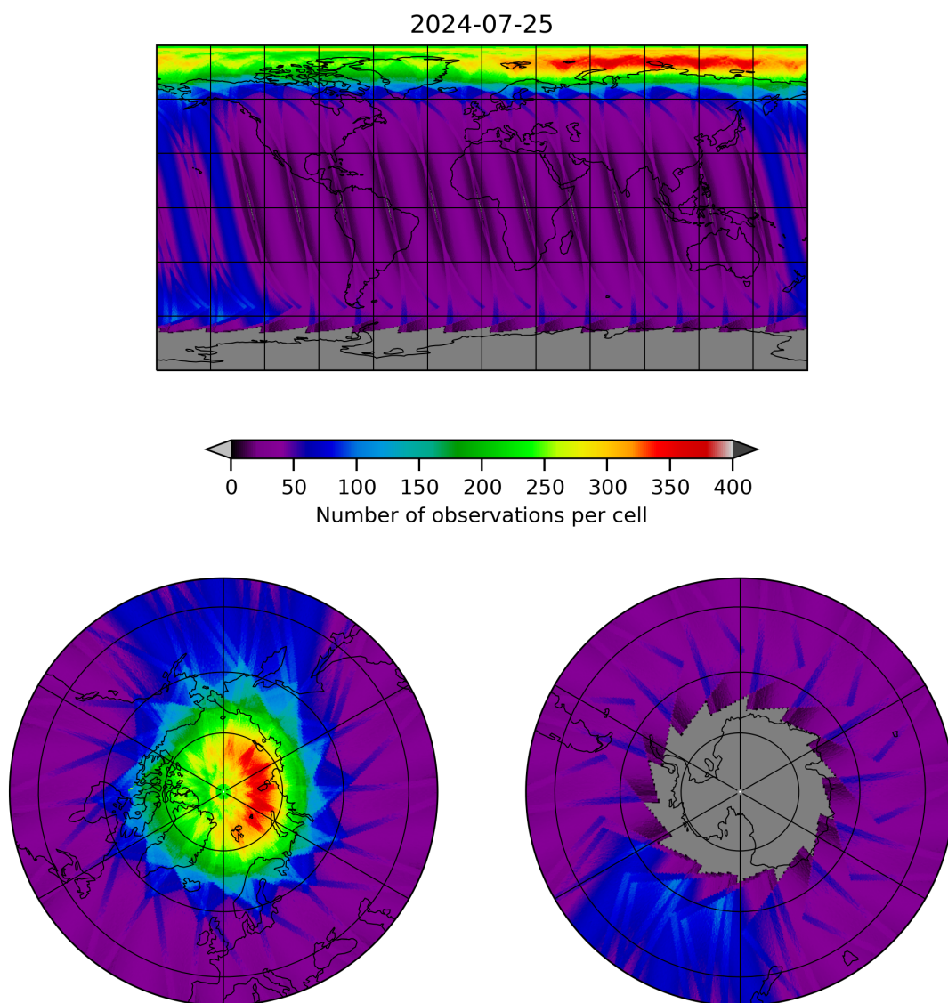
Figure 12: Map of the number of observations for 2024-07-24 to 2024-07-26
