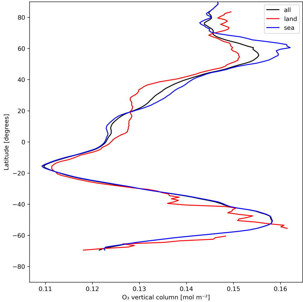
Figure 14: Zonal average of “O 3 vertical column” for 2024-07-24 to 2024-07-26.
