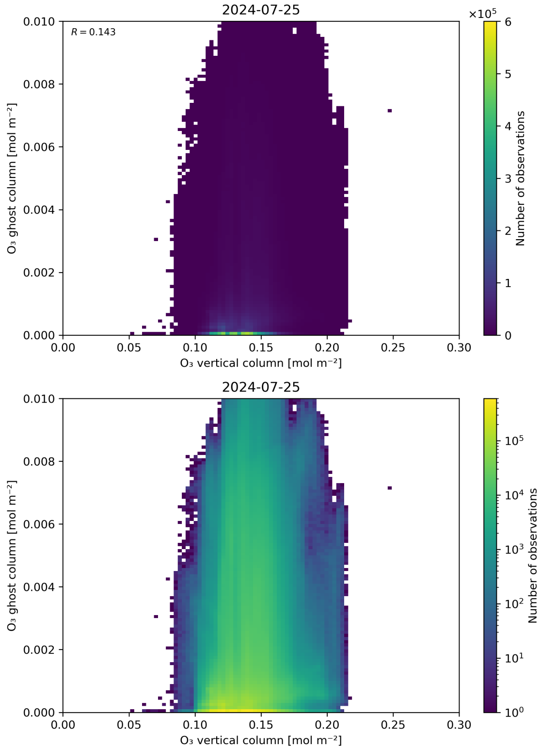
Figure 40: Scatter density plot of “O 3 vertical column” against “O 3 ghost column” for 2024-07-24 to 2024-07-26.
