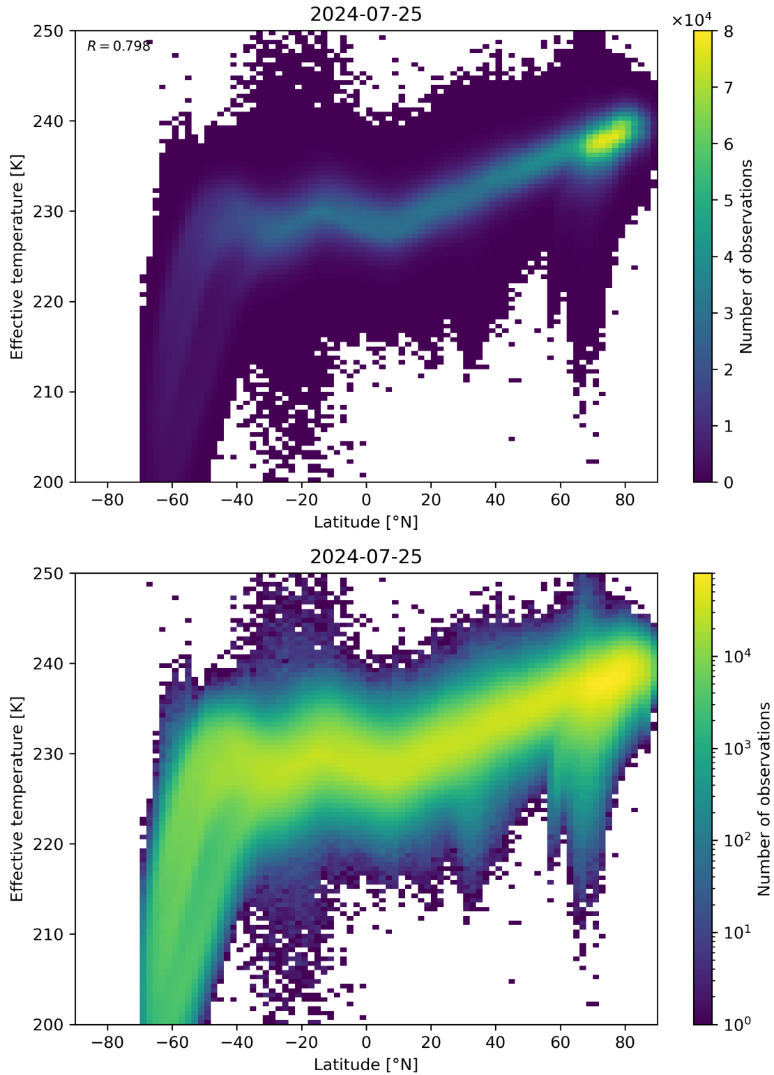
Figure 34: Scatter density plot of “Latitude” against “Effective temperature” for 2024-07-24 to 2024-07-26.
