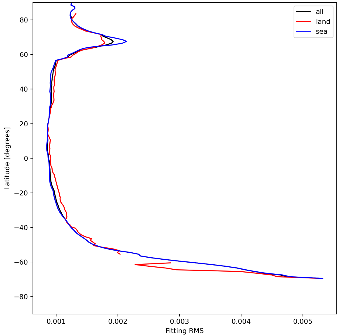
Figure 16: Zonal average of “Fitting RMS” for 2024-07-24 to 2024-07-26.
