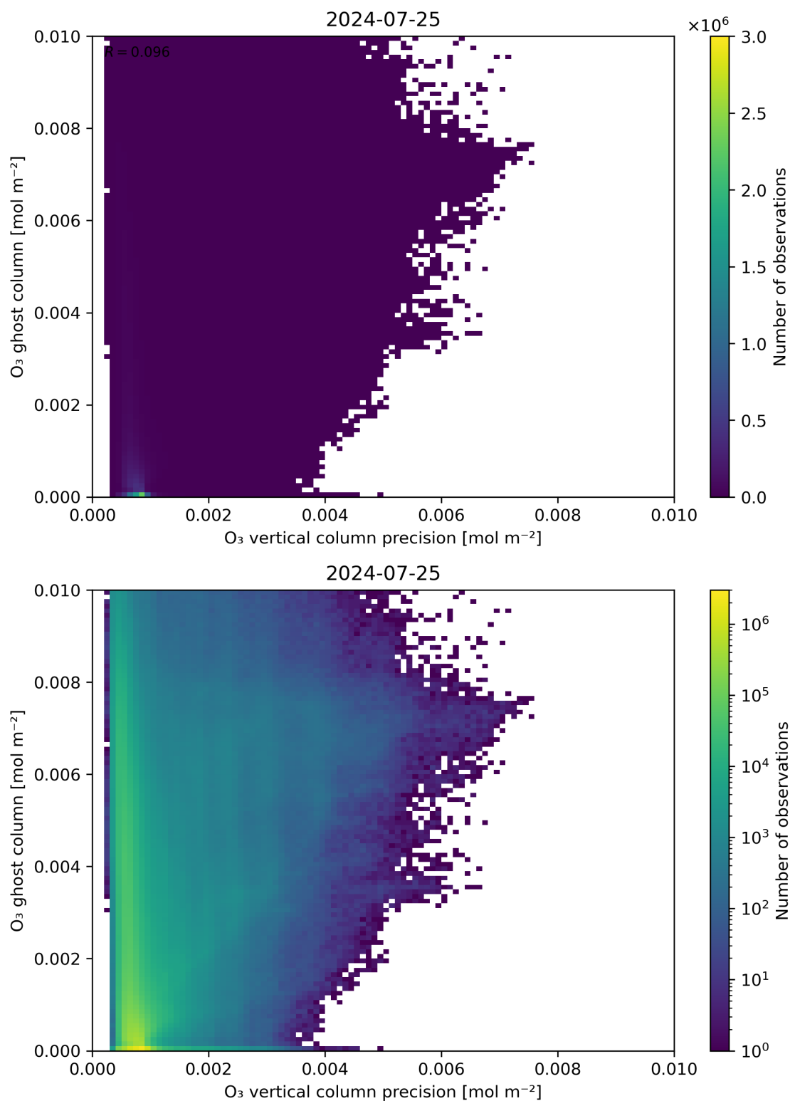
Figure 43: Scatter density plot of “ \text{O}_3 vertical column precision” against “ \text{O}_3 ghost column” for 2024-07-24 to 2024-07-26.
