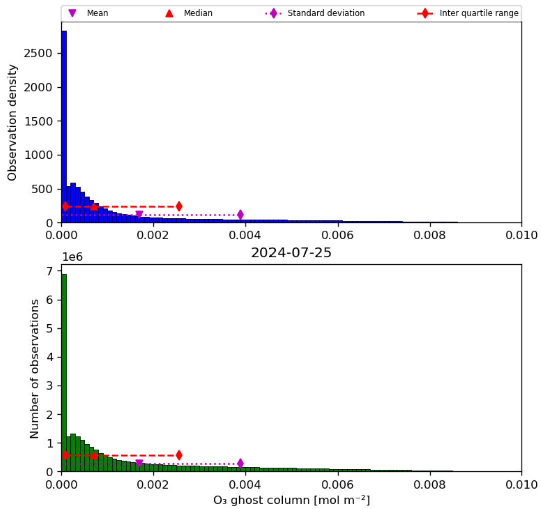
Figure 25: Histogram of “O 3 ghost column” for 2024-07-24 to 2024-07-26
