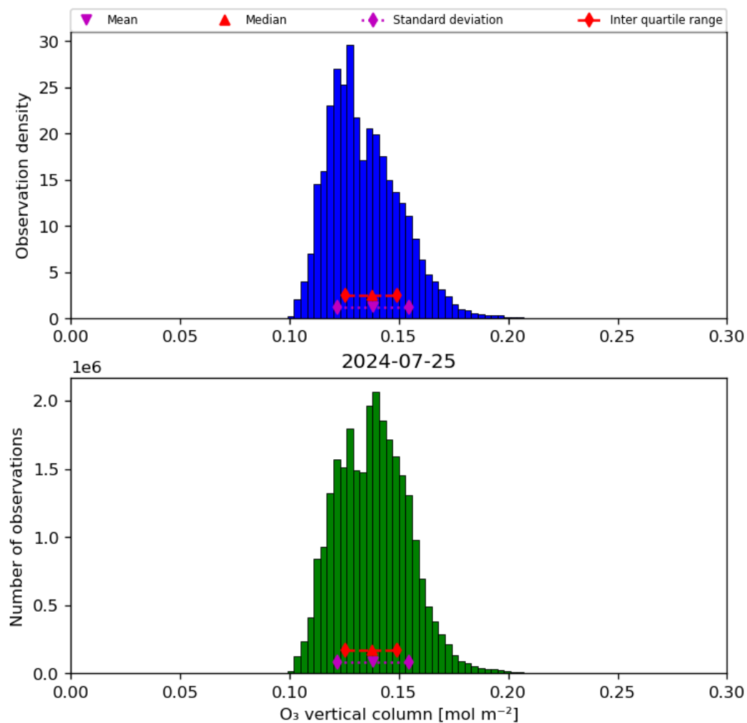
Figure 21: Histogram of “O 3 vertical column” for 2024-07-24 to 2024-07-26
