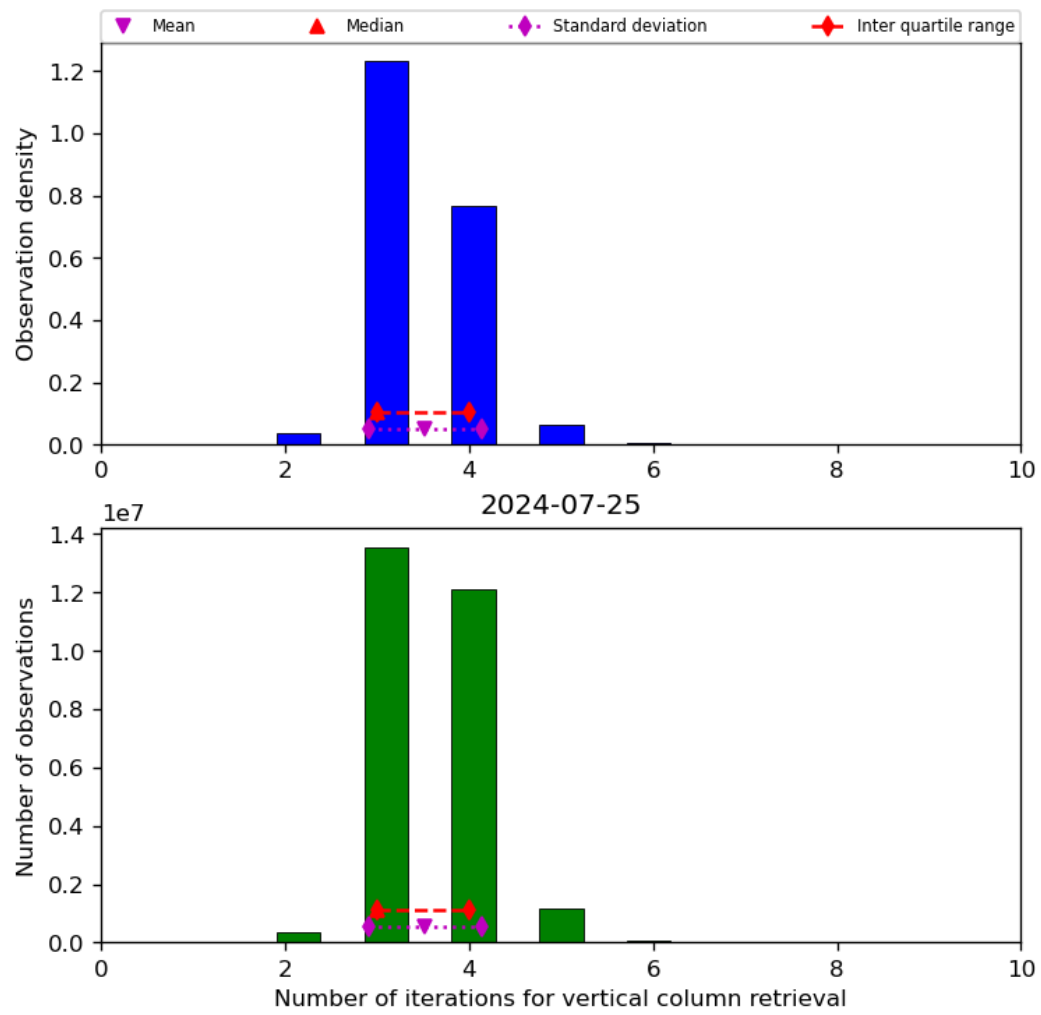
Figure 26: Histogram of “Number of iterations for vertical column retrieval” for 2024-07-24 to 2024-07-26
