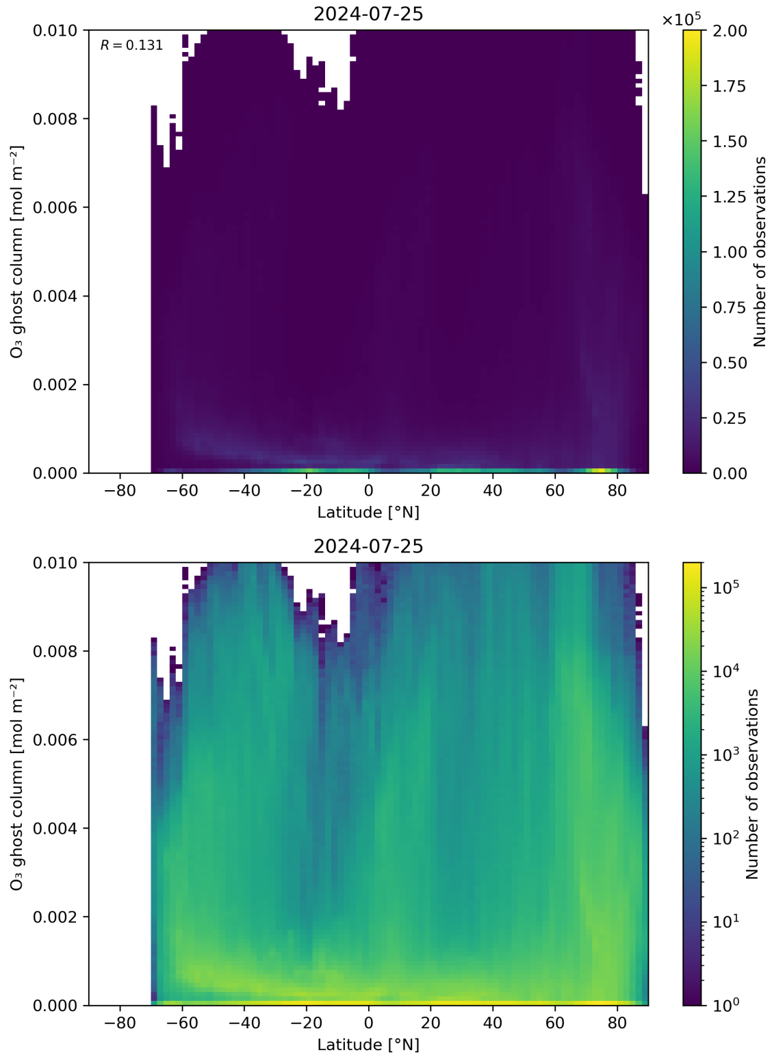
Figure 35: Scatter density plot of “Latitude” against “O 3 ghost column” for 2024-07-24 to 2024-07-26.
