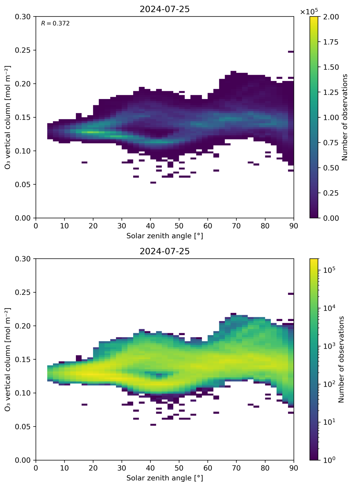
Figure 47: Scatter density plot of “Solar zenith angle” against “O 3 vertical column” for 2024-07-24 to 2024-07-26.
