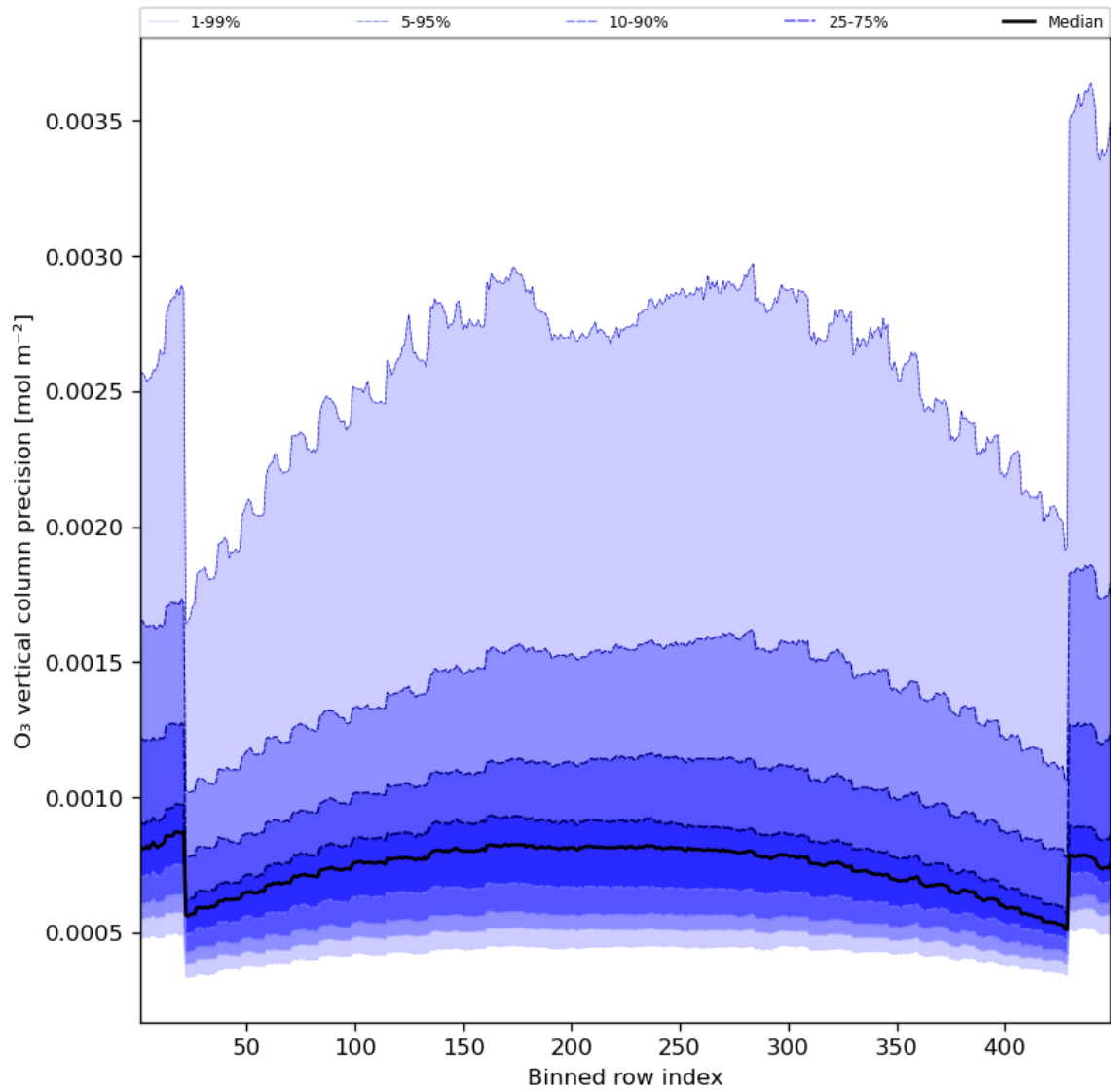
Figure 29: Along track statistics of “O 3 vertical column precision” for 2024-07-24 to 2024-07-26
