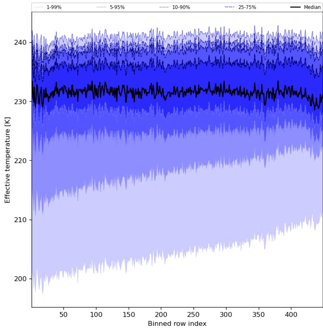
Figure 31: Along track statistics of “Effective temperature” for 2024-07-24 to 2024-07-26
