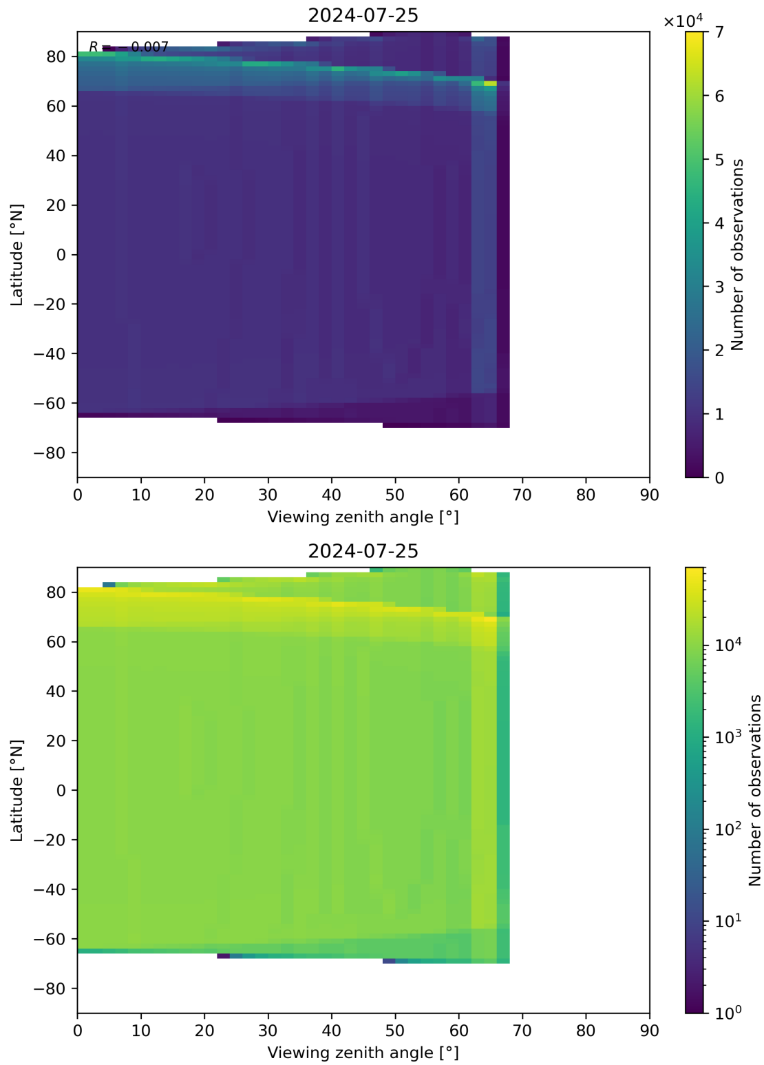
Figure 49: Scatter density plot of “Viewing zenith angle” against “Latitude” for 2024-07-24 to 2024-07-26.
