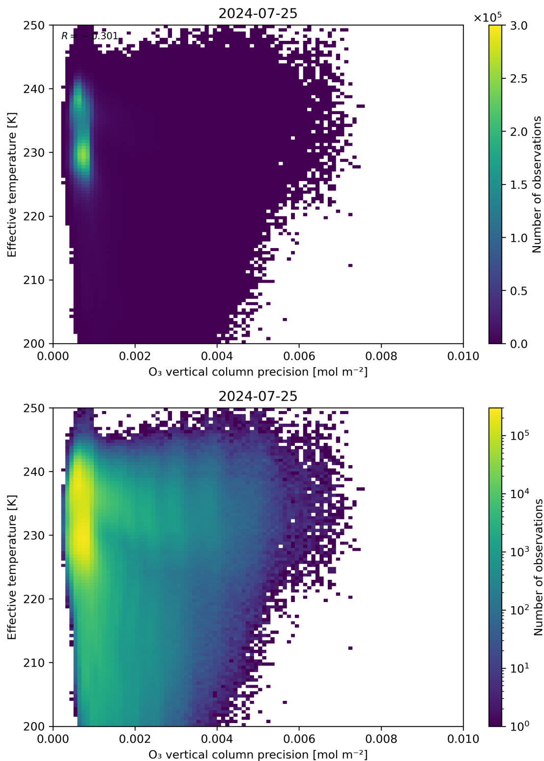
Figure 42: Scatter density plot of “O 3 vertical column precision” against “Effective temperature” for 2024-07-24 to 2024-07-26.
