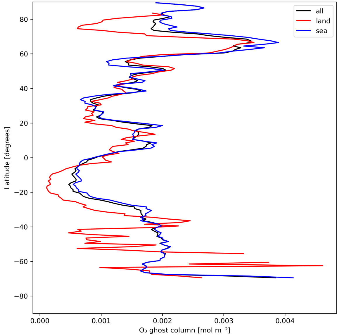
Figure 18: Zonal average of "O 3 ghost column" for 2024-07-24 to 2024-07-26.
