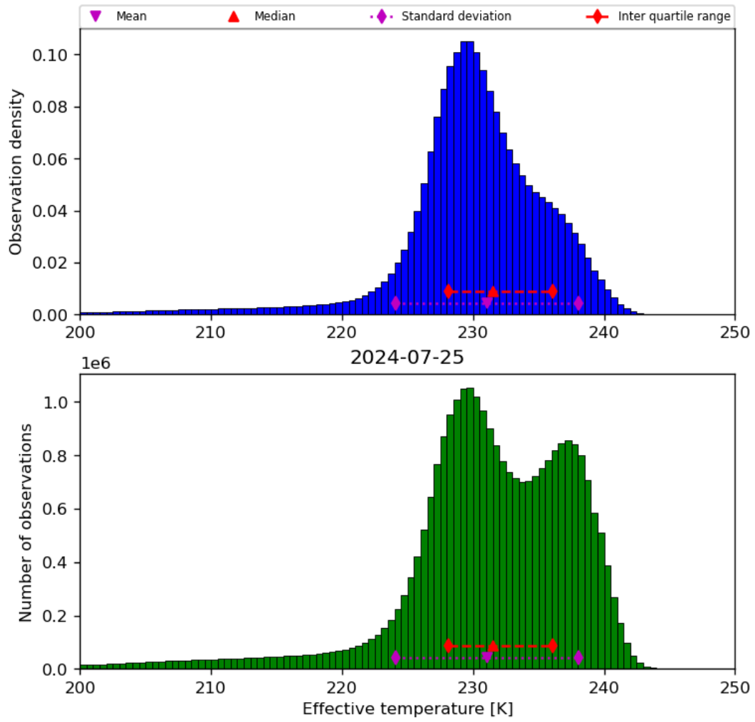
Figure 24: Histogram of “Effective temperature” for 2024-07-24 to 2024-07-26
