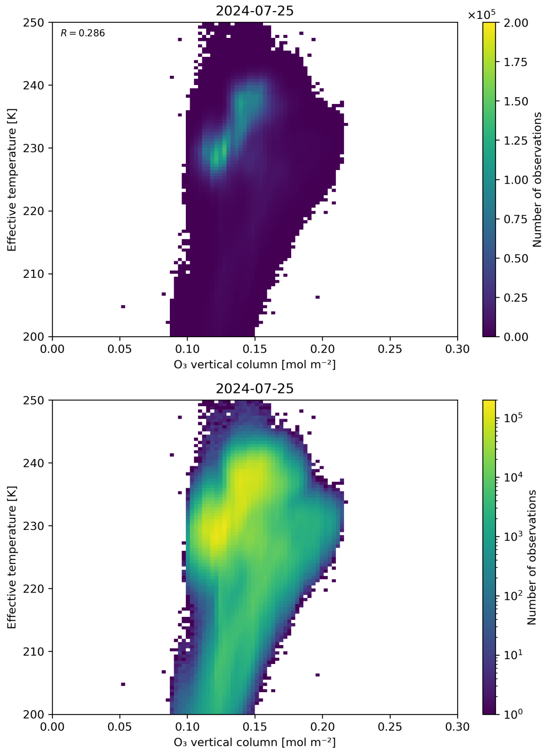
Figure 39: Scatter density plot of “O 3 vertical column” against “Effective temperature” for 2024-07-24 to 2024-07-26.
