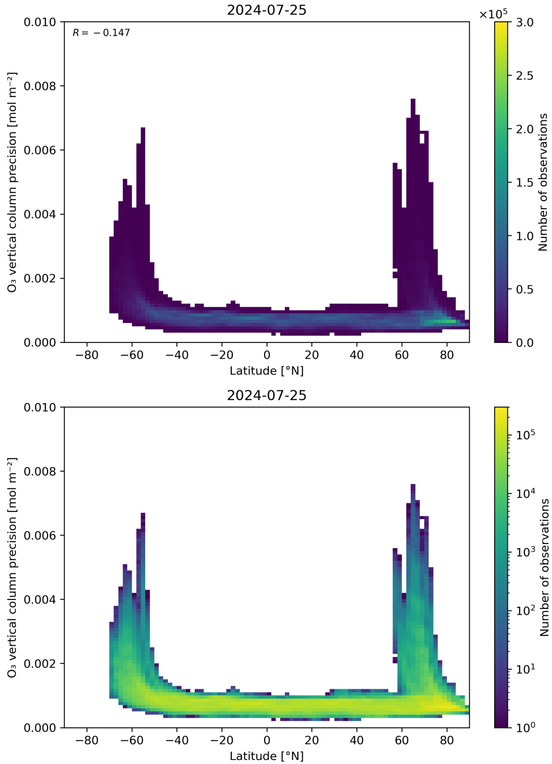
Figure 37: Scatter density plot of “Latitude” against “O 3 vertical column precision” for 2024-07-24 to 2024-07-26.
