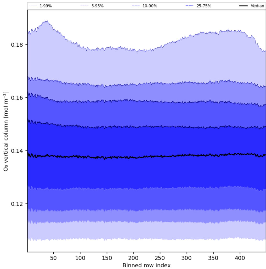
Figure 28: Along track statistics of “O 3 vertical column” for 2024-07-24 to 2024-07-26
