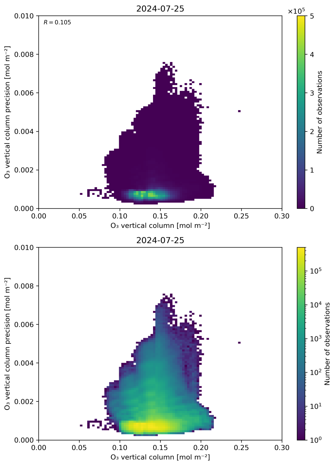
Figure 41: Scatter density plot of “O 3 vertical column” against “O 3 vertical column precision” for 2024-07-24 to 2024-07-26.
