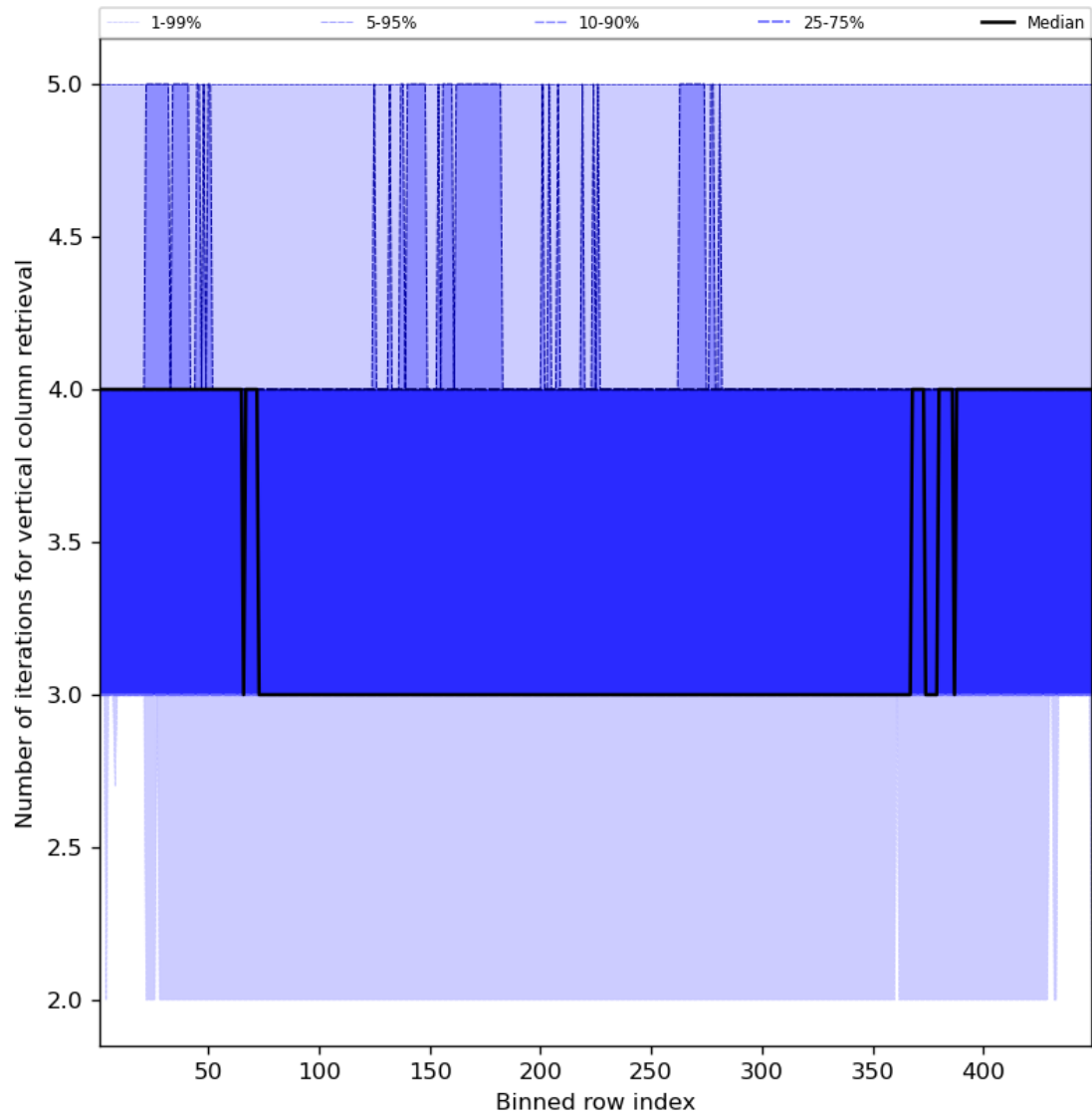
Figure 33: Along track statistics of “Number of iterations for vertical column retrieval” for 2024-07-24 to 2024-07-26
