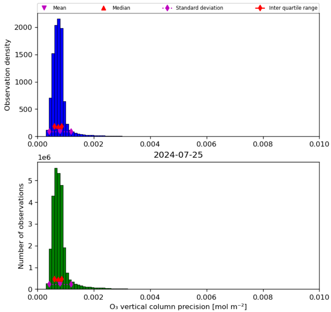
Figure 22: Histogram of “O 3 vertical column precision” for 2024-07-24 to 2024-07-26
