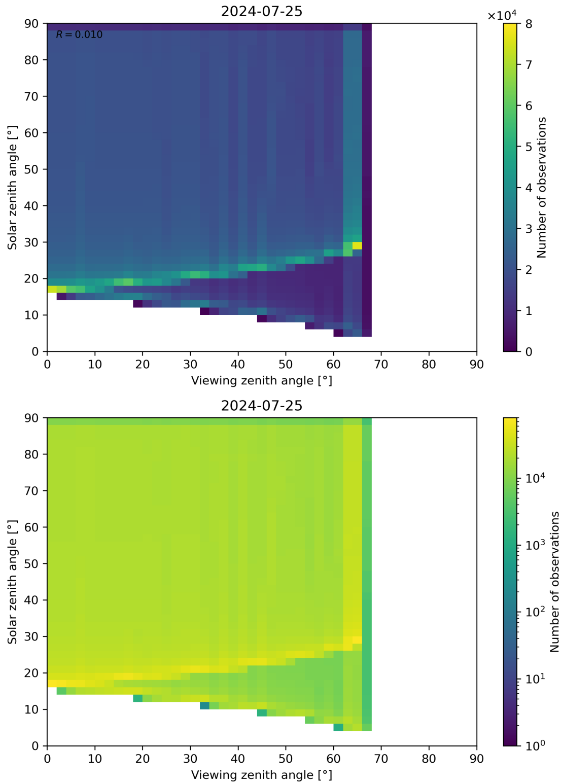
Figure 54: Scatter density plot of “Viewing zenith angle” against “Solar zenith angle” for 2024-07-24 to 2024-07-26.
