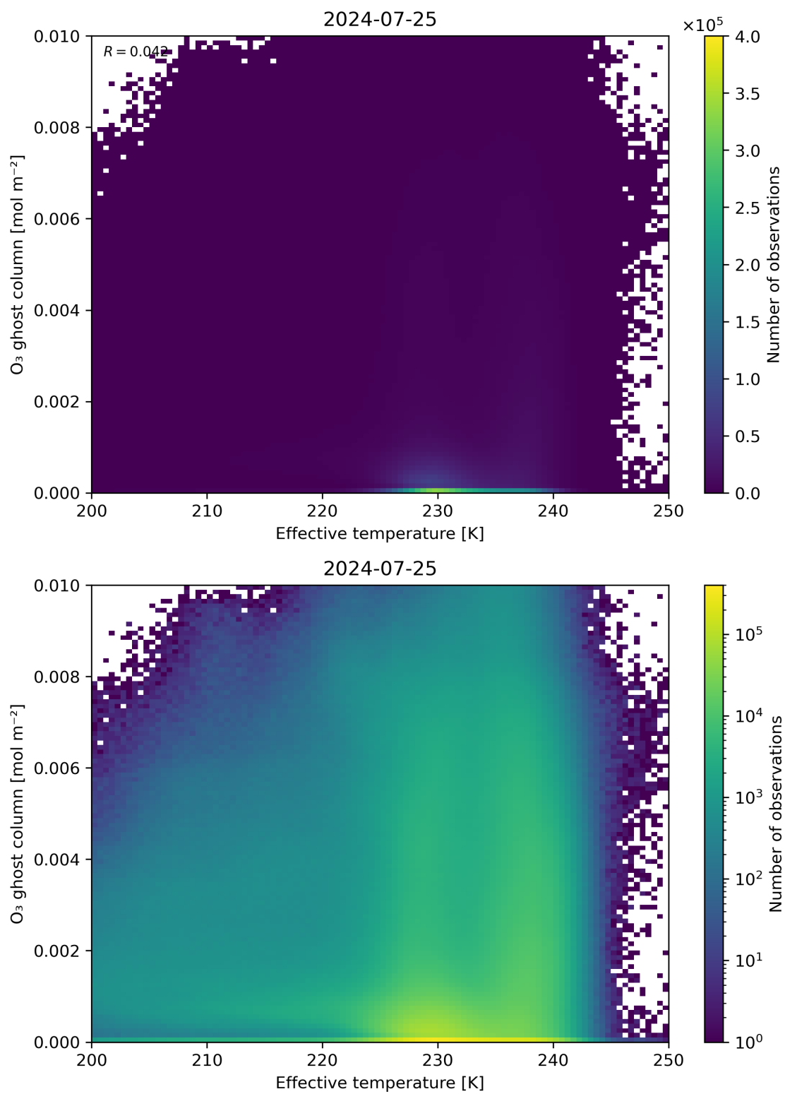
Figure 38: Scatter density plot of “Effective temperature” against “O 3 ghost column” for 2024-07-24 to 2024-07-26.
