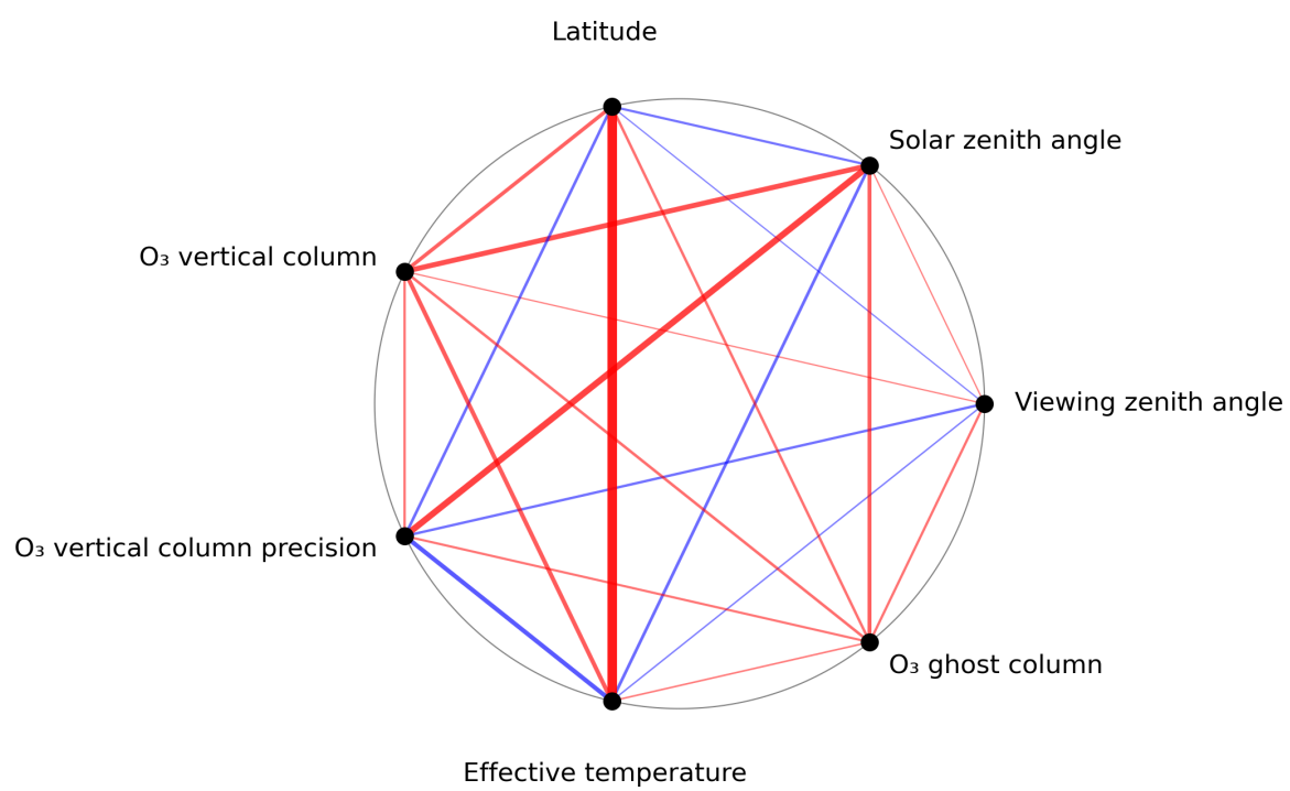
Figure 1: Map of correlation graph for 2024-07-24 to 2024-07-26.
