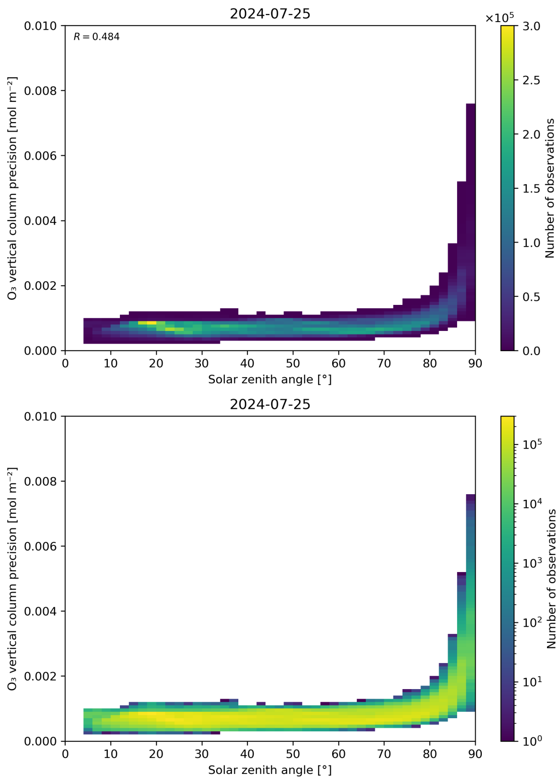
Figure 48: Scatter density plot of “Solar zenith angle” against “O 3 vertical column precision” for 2024-07-24 to 2024-07-26.
