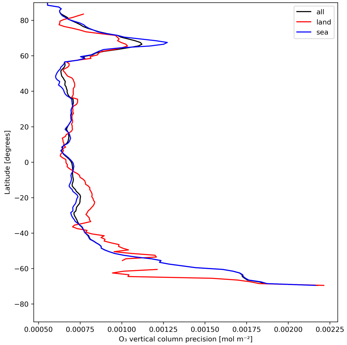
Figure 15: Zonal average of "O 3 vertical column precision" for 2024-07-24 to 2024-07-26.
