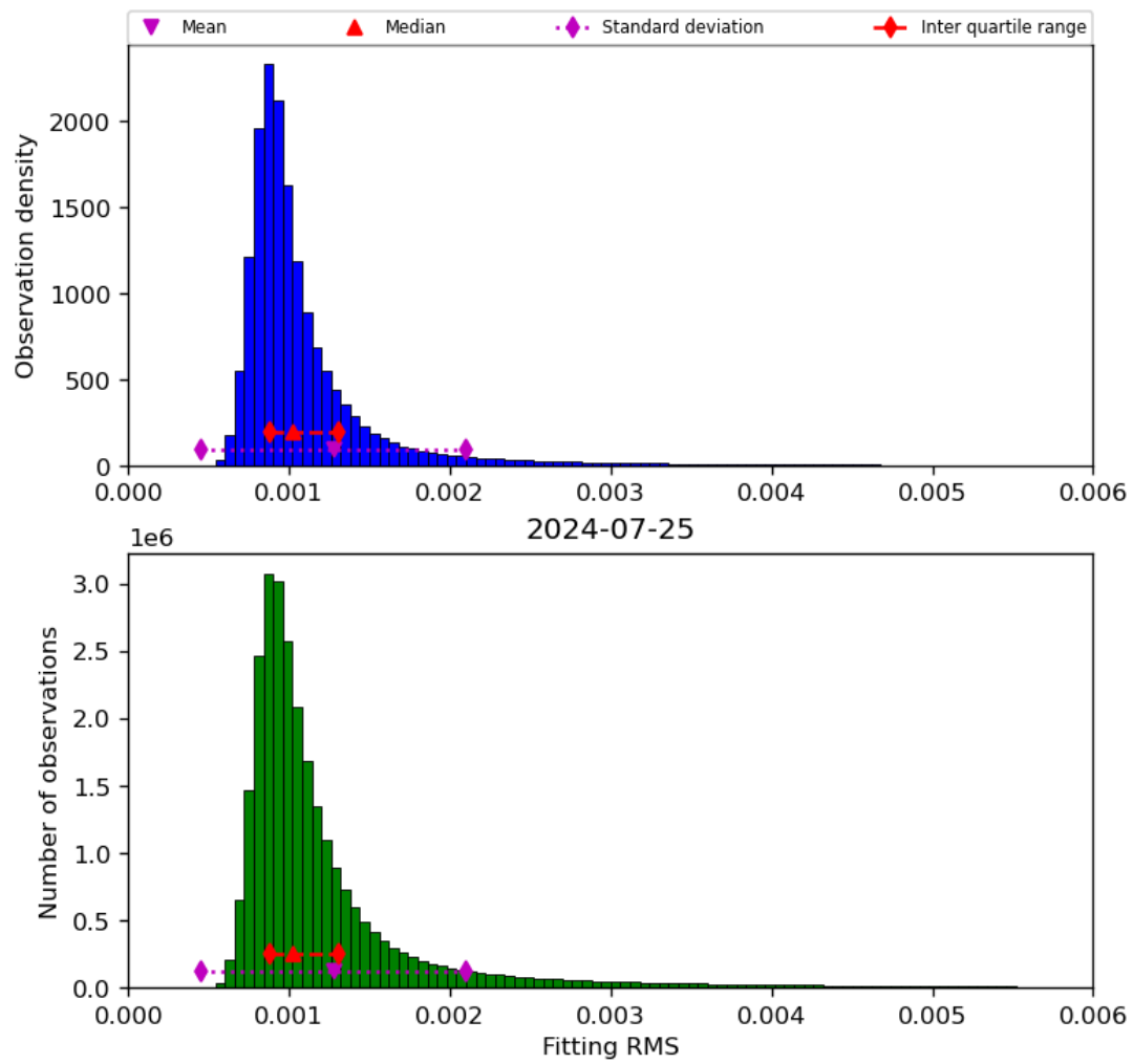
Figure 23: Histogram of “Fitting RMS” for 2024-07-24 to 2024-07-26
