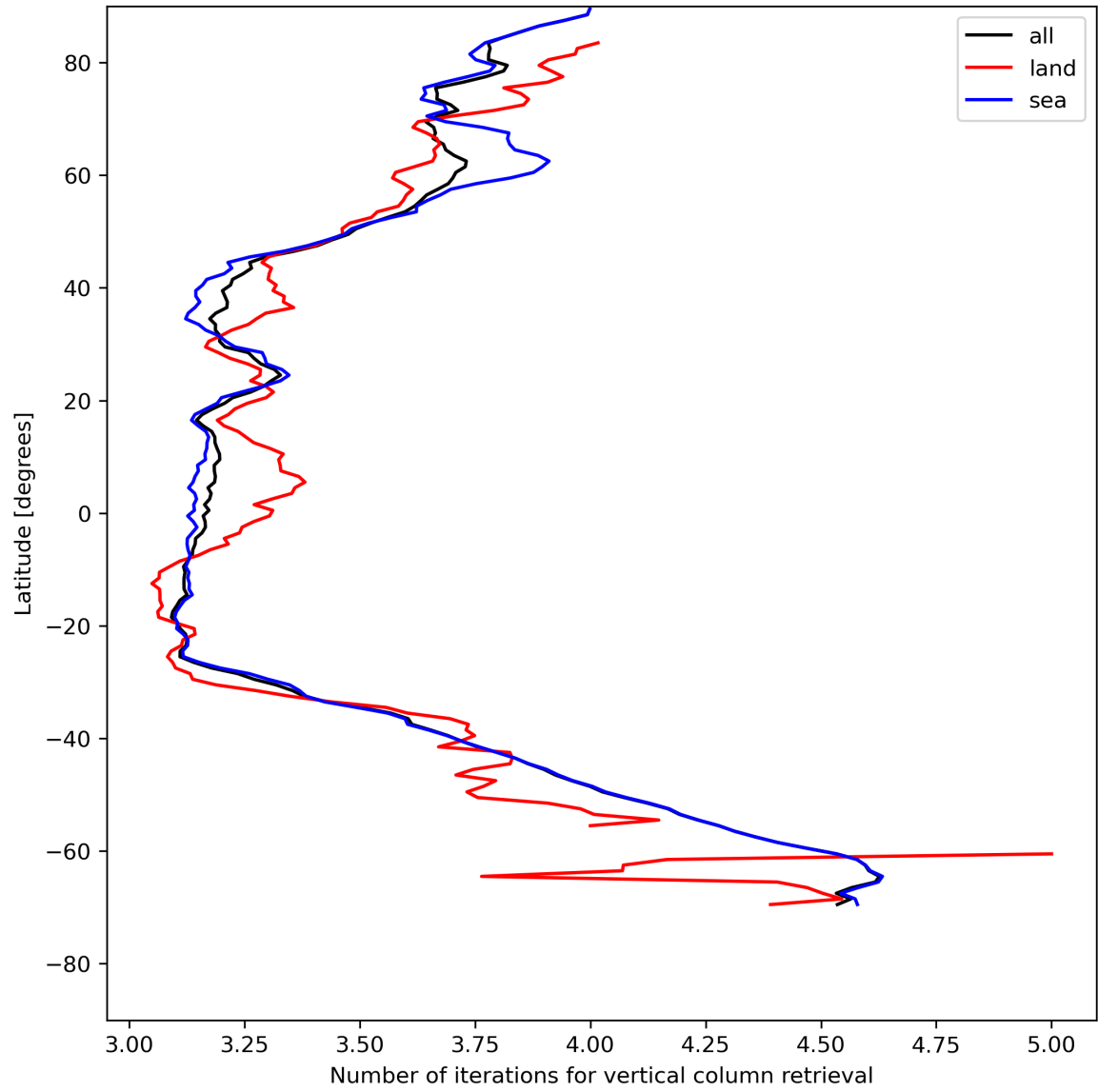
Figure 19: Zonal average of “Number of iterations for vertical column retrieval” for 2024-07-24 to 2024-07-26.
