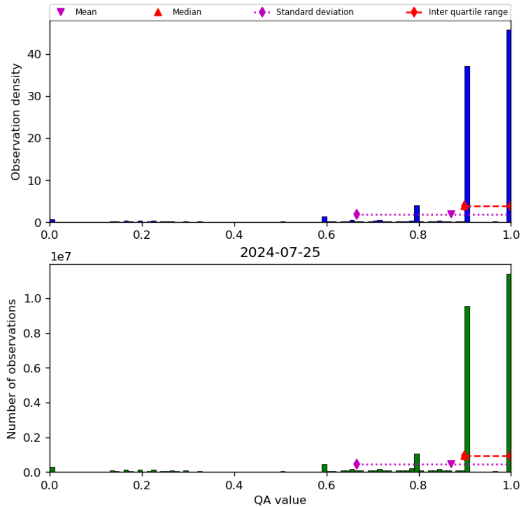
Figure 20: Histogram of “QA value” for 2024-07-24 to 2024-07-26
