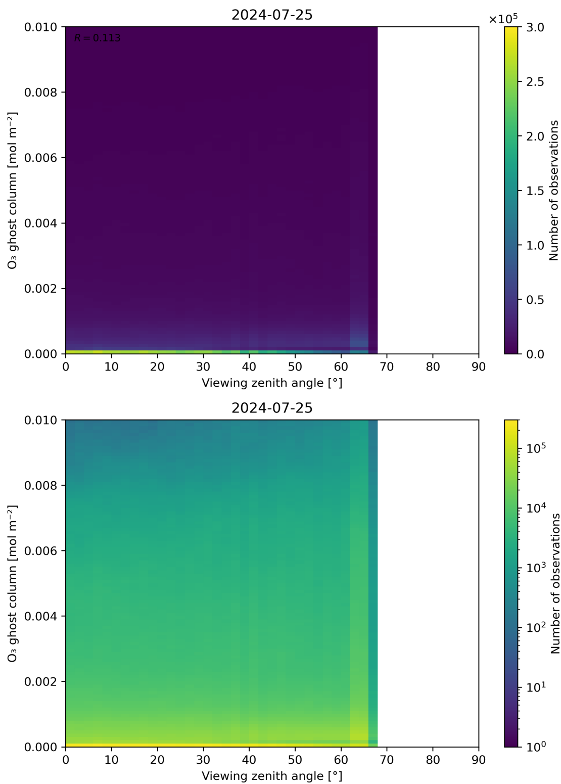
Figure 51: Scatter density plot of “Viewing zenith angle” against “O 3 ghost column” for 2024-07-24 to 2024-07-26.
