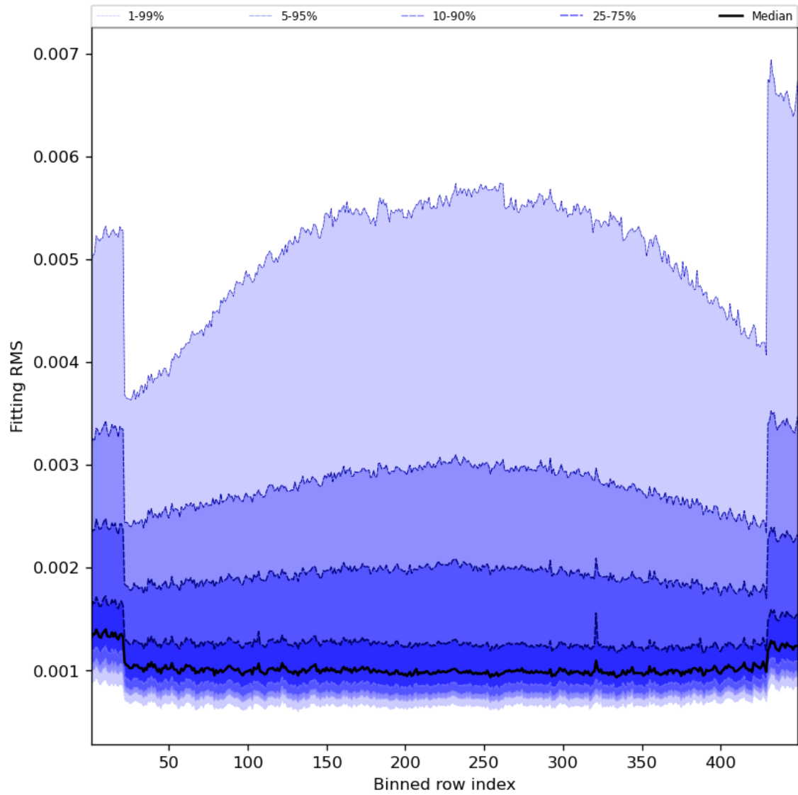
Figure 30: Along track statistics of “Fitting RMS” for 2024-07-24 to 2024-07-26
