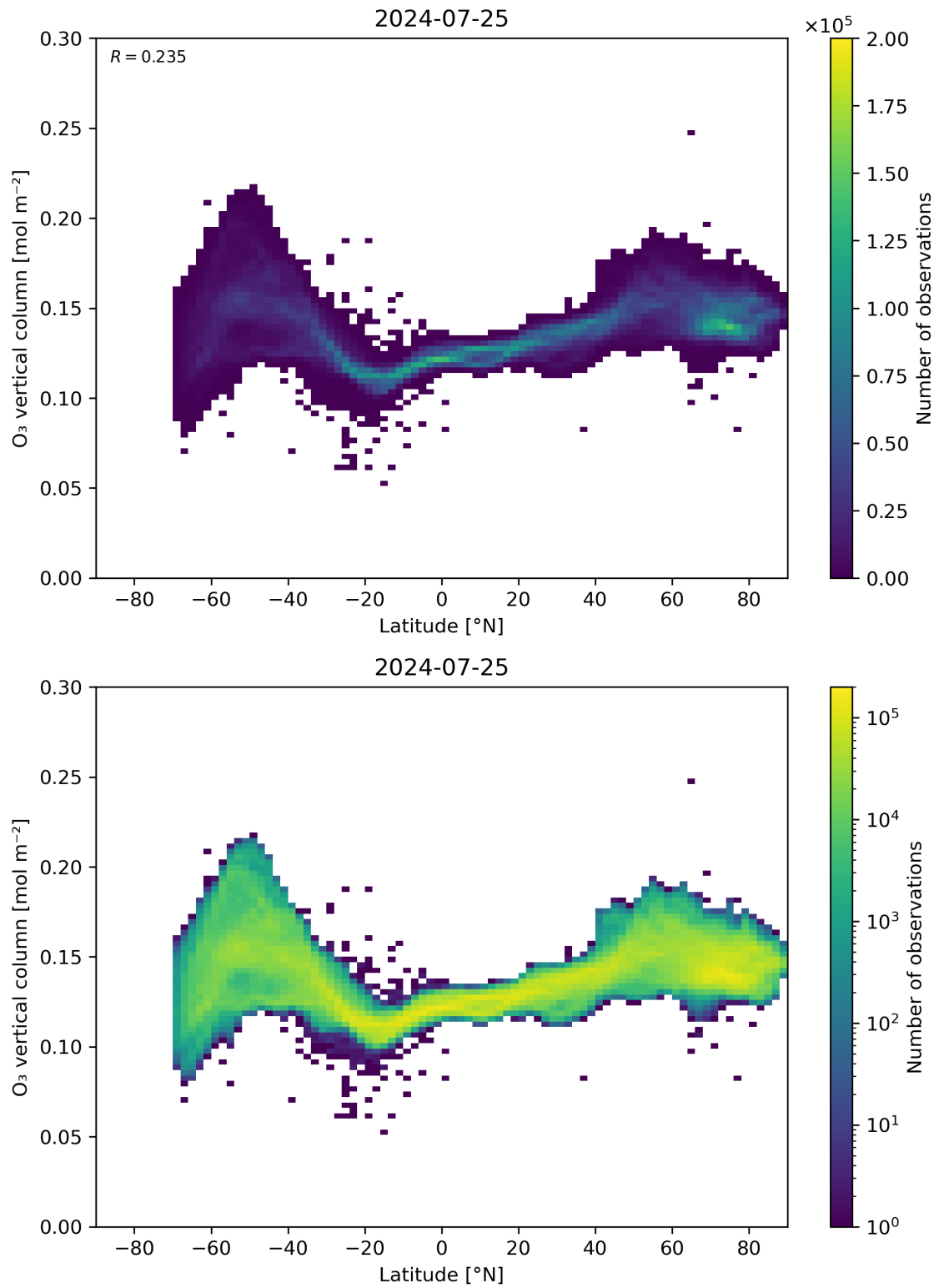
Figure 36: Scatter density plot of “Latitude” against “O 3 vertical column” for 2024-07-24 to 2024-07-26.
