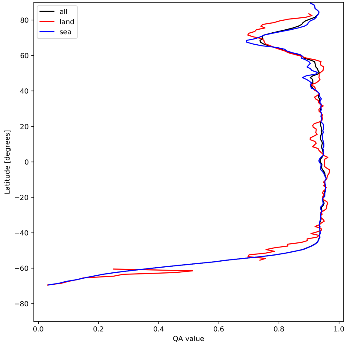
Figure 13: Zonal average of “QA value” for 2024-07-24 to 2024-07-26.
