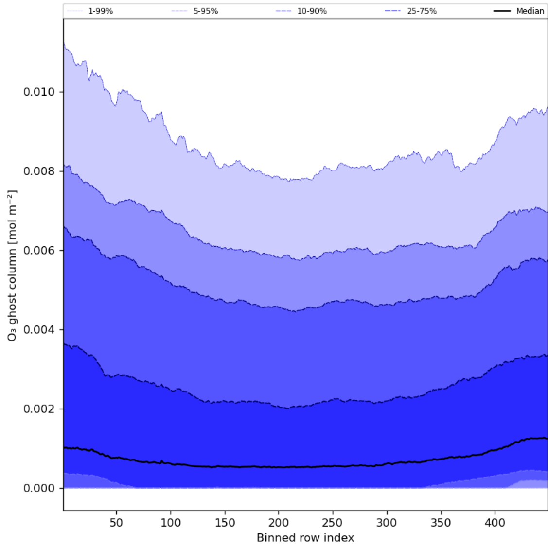
Figure 32: Along track statistics of “O 3 ghost column” for 2024-07-24 to 2024-07-26
