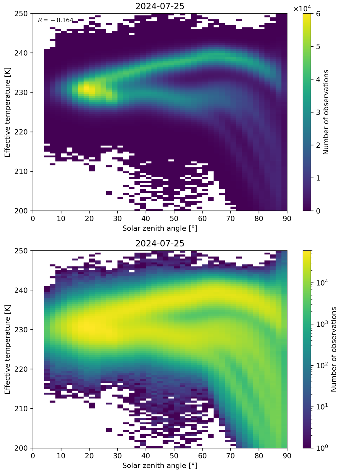
Figure 45: Scatter density plot of “Solar zenith angle” against “Effective temperature” for 2024-07-24 to 2024-07-26.
