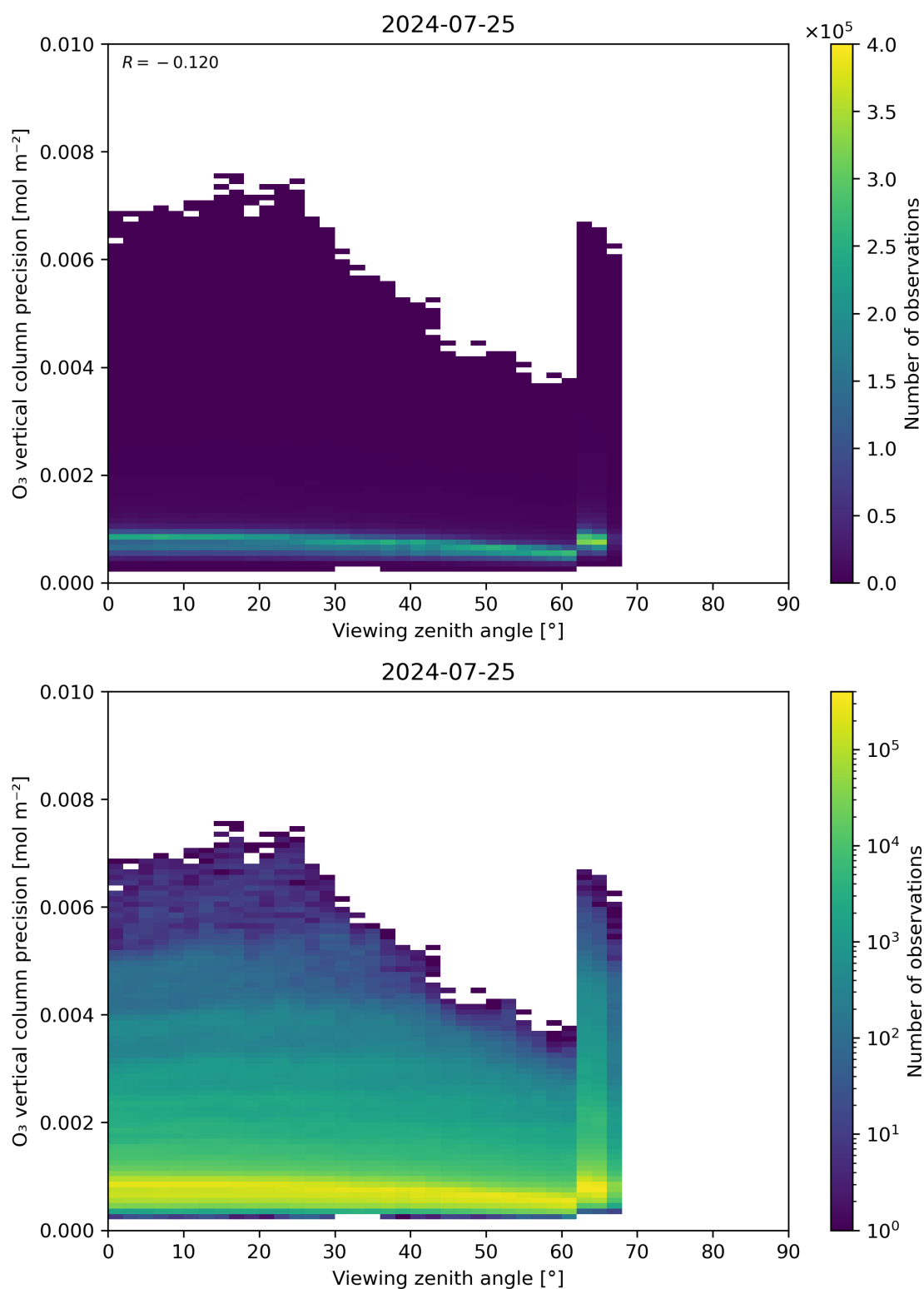
Figure 53: Scatter density plot of “Viewing zenith angle” against “O 3 vertical column precision” for 2024-07-24 to 2024-07-26.
