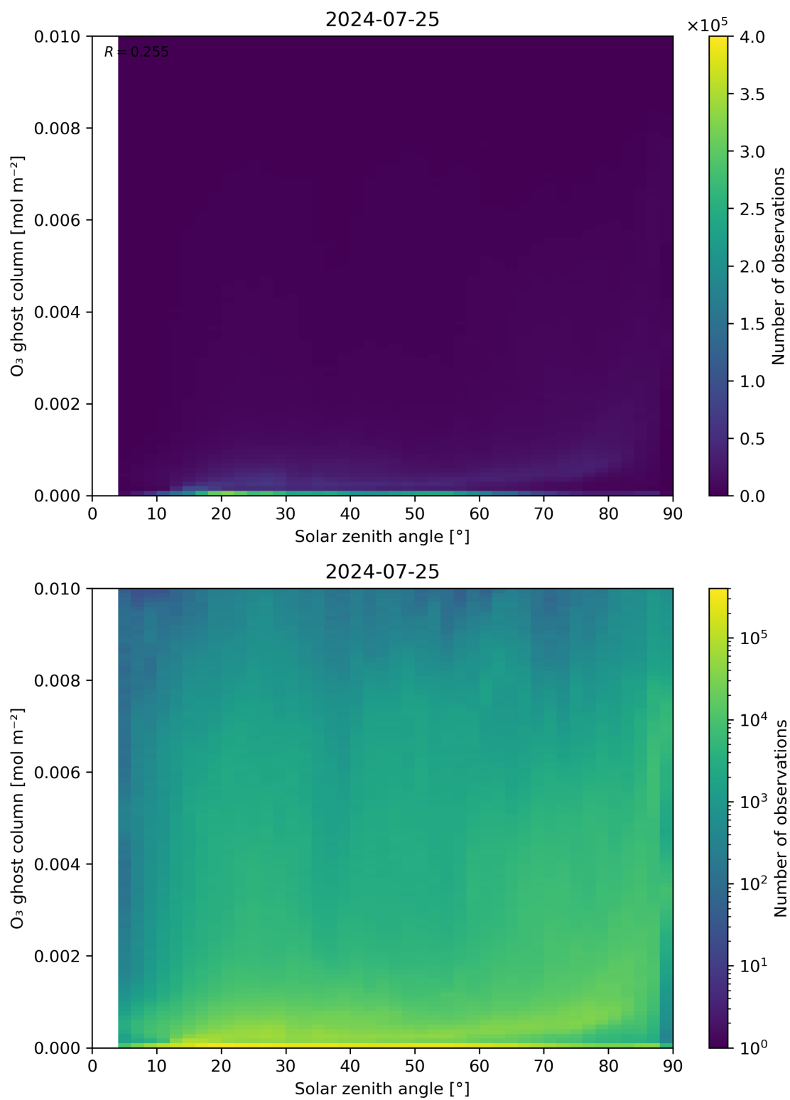
Figure 46: Scatter density plot of “Solar zenith angle” against “O 3 ghost column” for 2024-07-24 to 2024-07-26.
