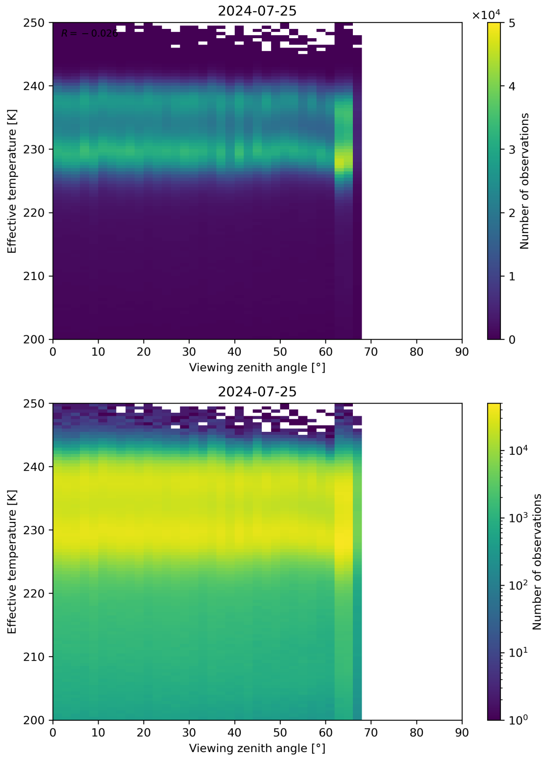
Figure 50: Scatter density plot of “Viewing zenith angle” against “Effective temperature” for 2024-07-24 to 2024-07-26.
