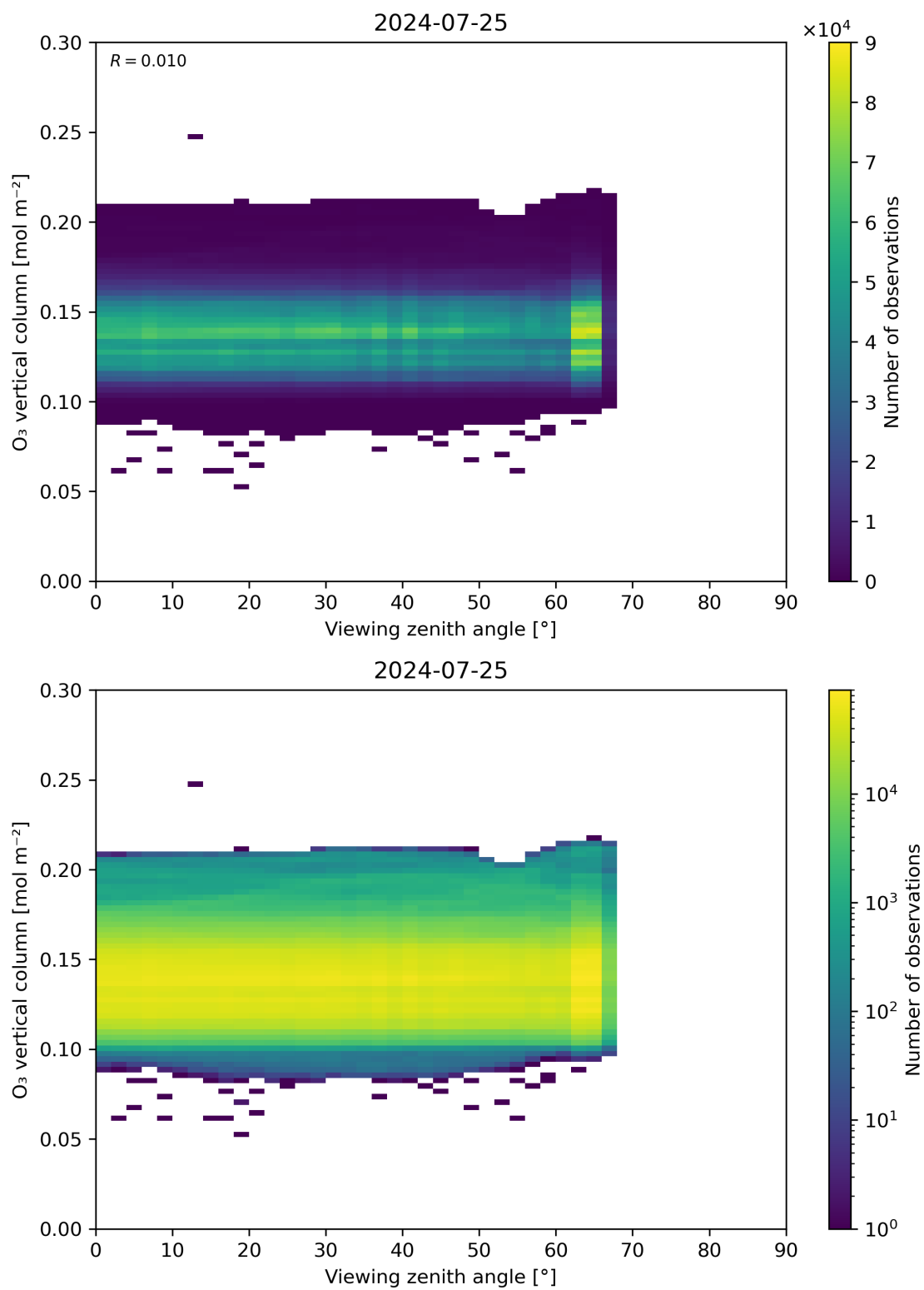
Figure 52: Scatter density plot of “Viewing zenith angle” against “O 3 vertical column” for 2024-07-24 to 2024-07-26.
