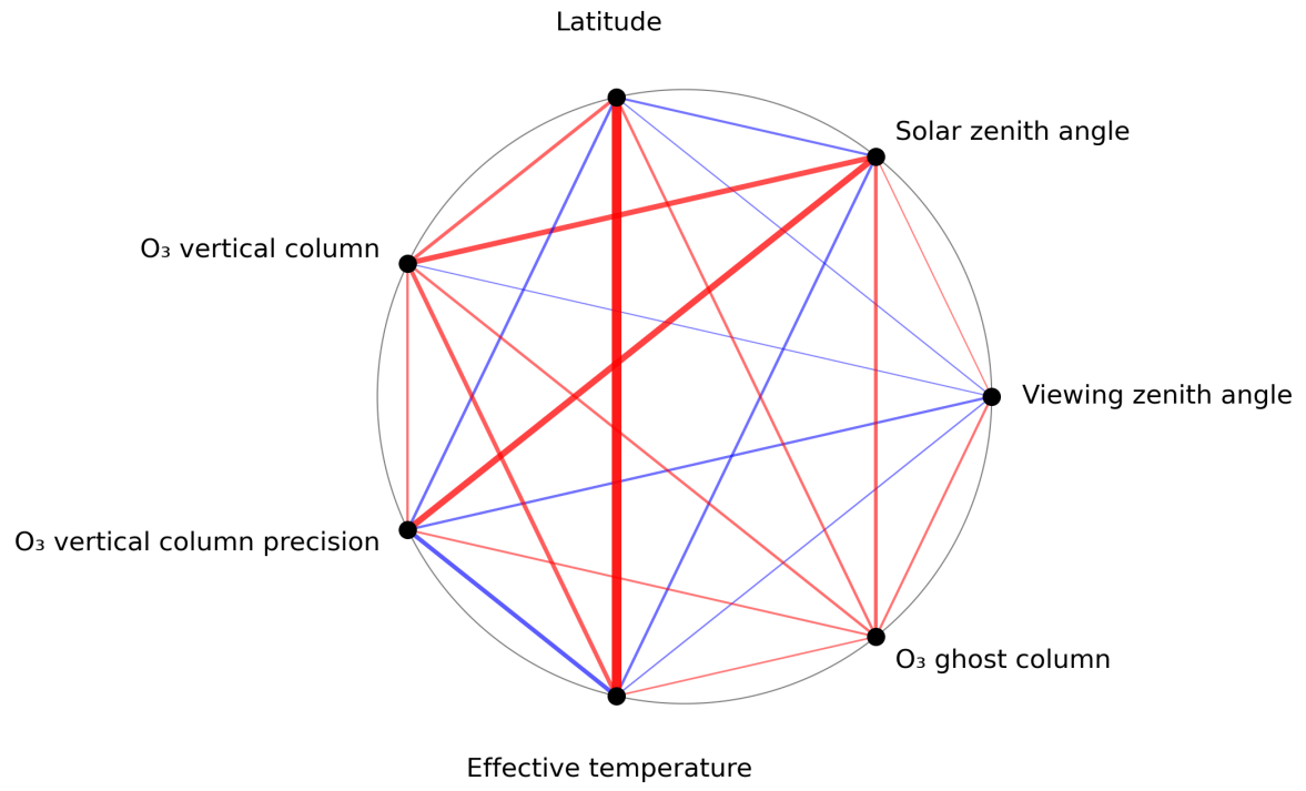
Figure 1: Map of correlation graph for 2024-07-26 to 2024-07-27.
