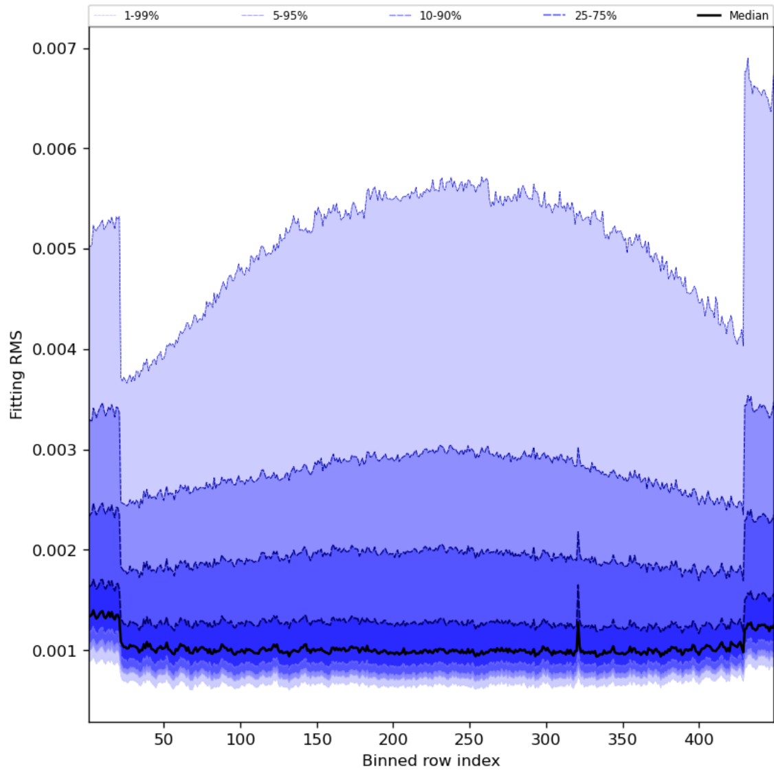
Figure 30: Along track statistics of “Fitting RMS” for 2024-07-26 to 2024-07-27
