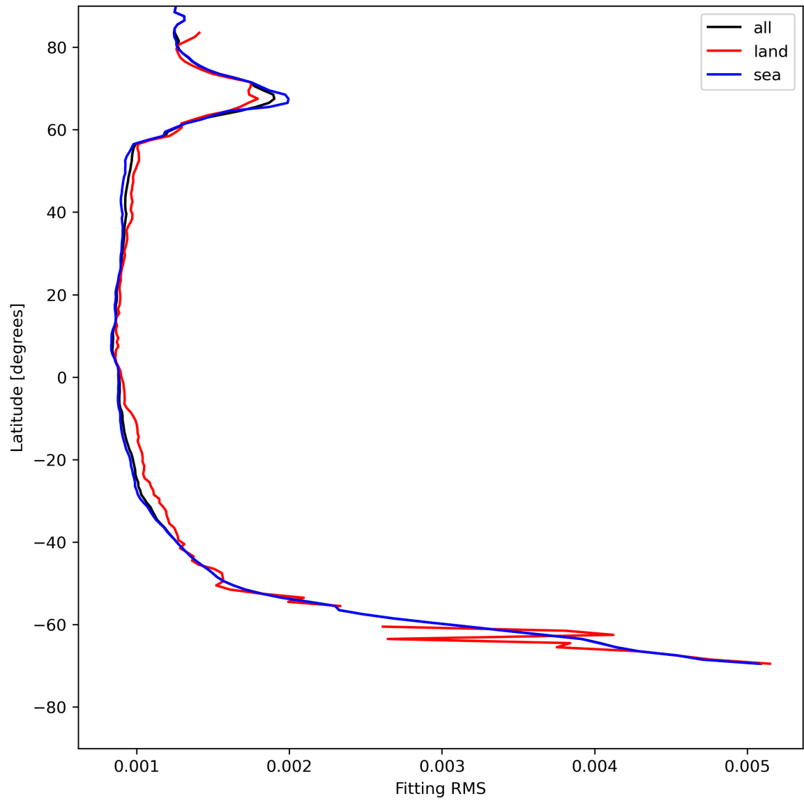
Figure 16: Zonal average of “Fitting RMS” for 2024-07-26 to 2024-07-27.
