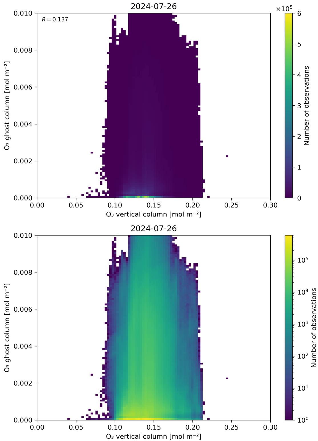
Figure 40: Scatter density plot of “O 3 vertical column” against “O 3 ghost column” for 2024-07-26 to 2024-07-27.
