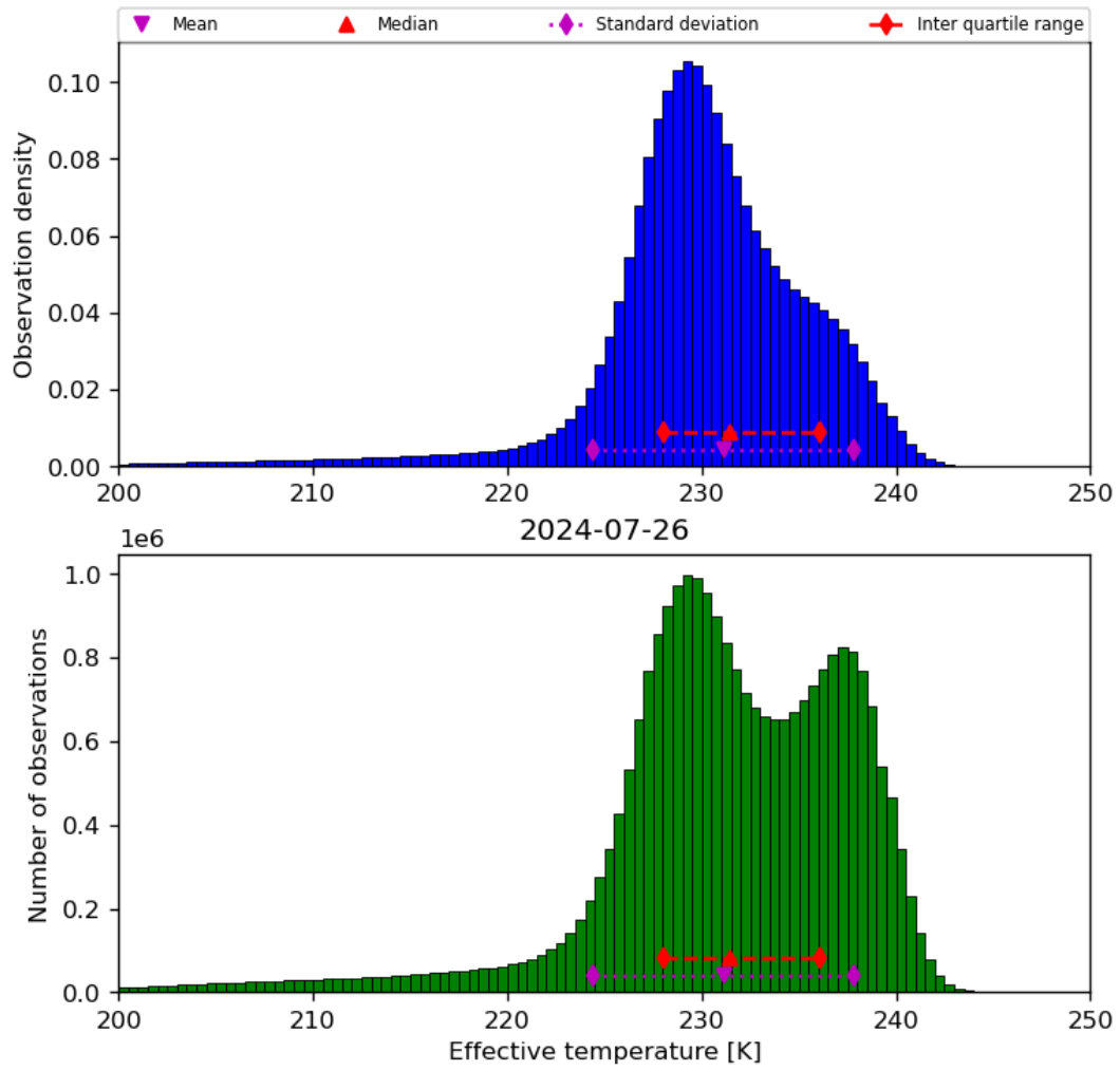
Figure 24: Histogram of “Effective temperature” for 2024-07-26 to 2024-07-27
