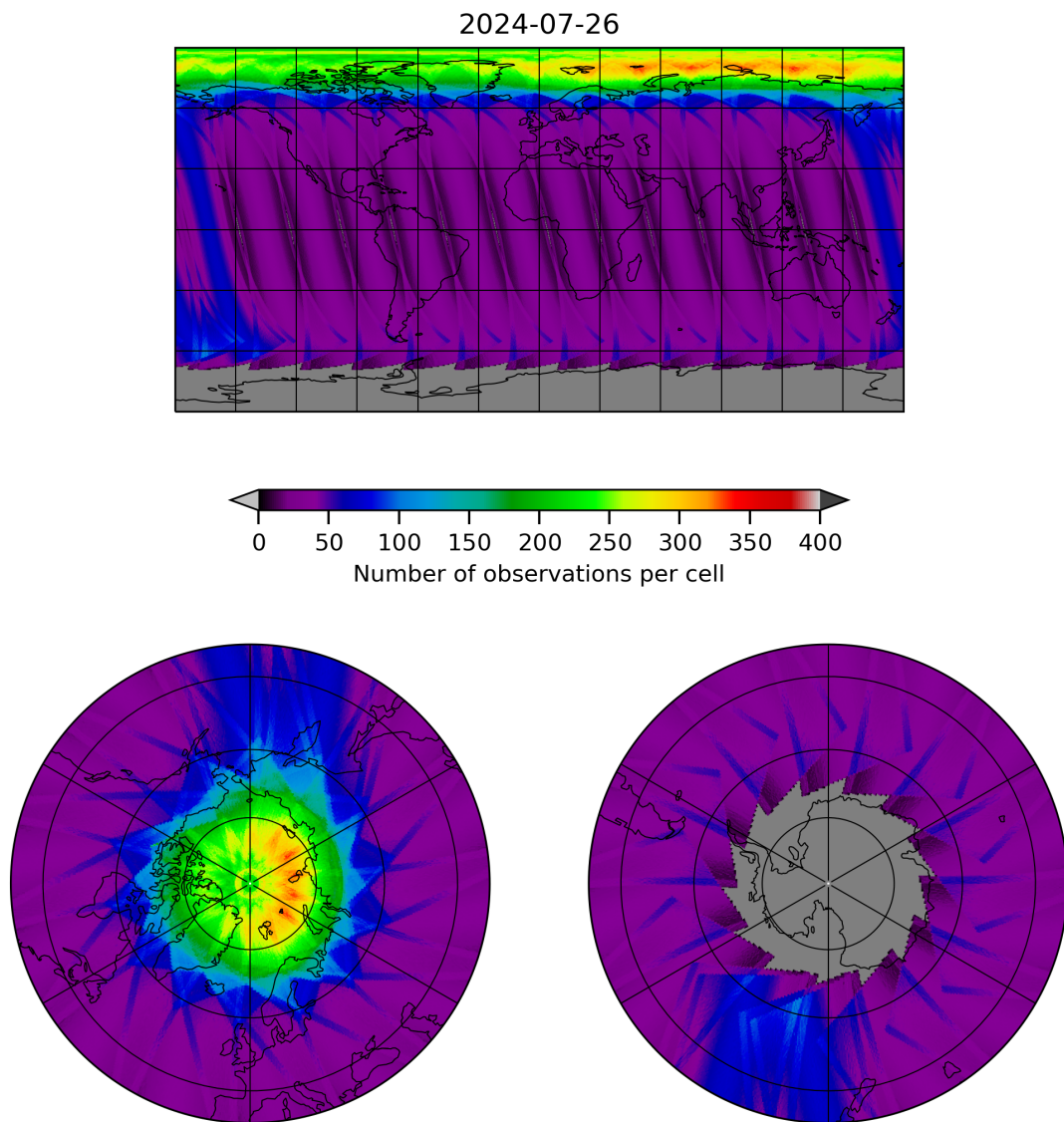
Figure 12: Map of the number of observations for 2024-07-26 to 2024-07-27
