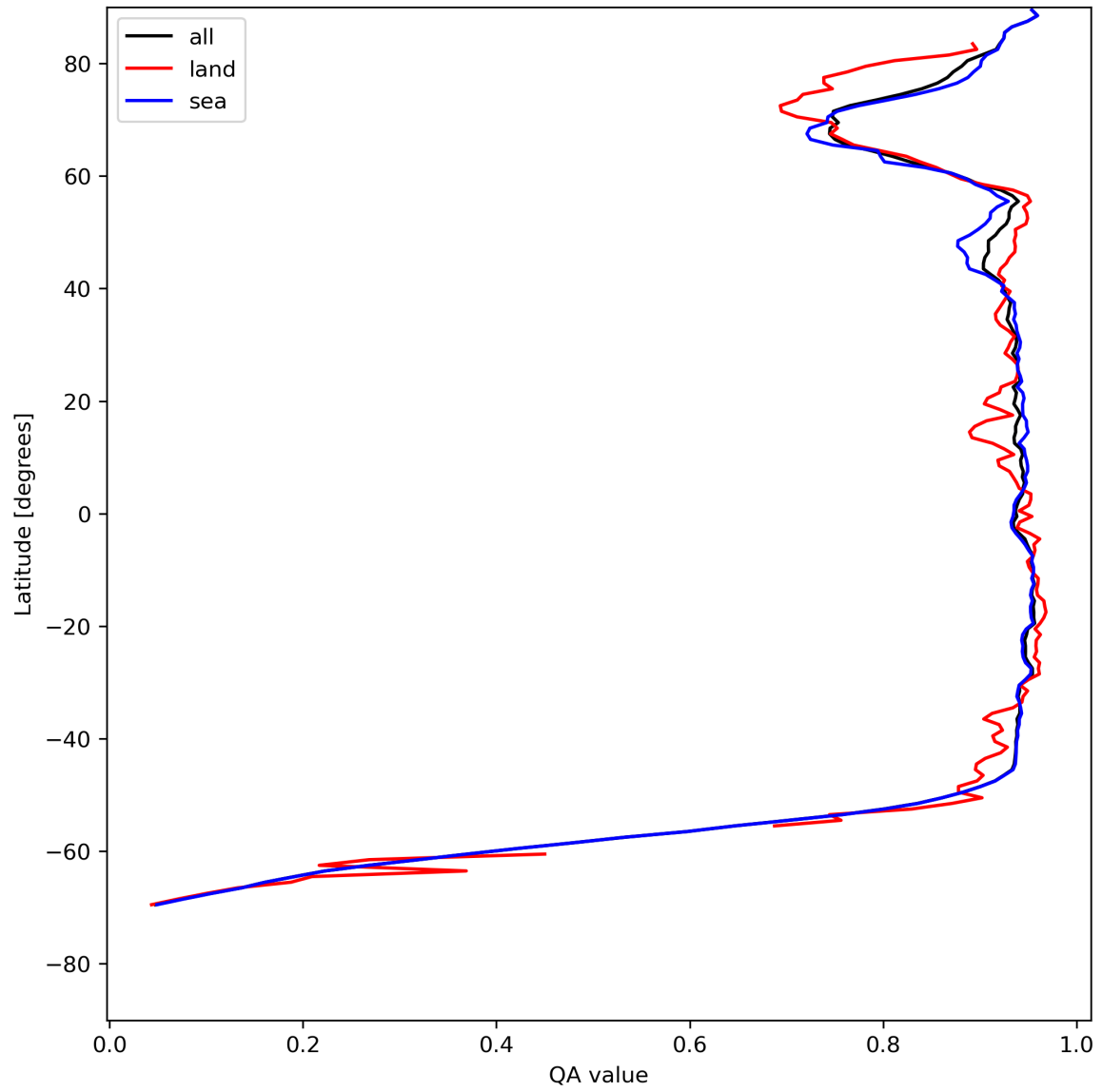
Figure 13: Zonal average of “QA value” for 2024-07-26 to 2024-07-27.
