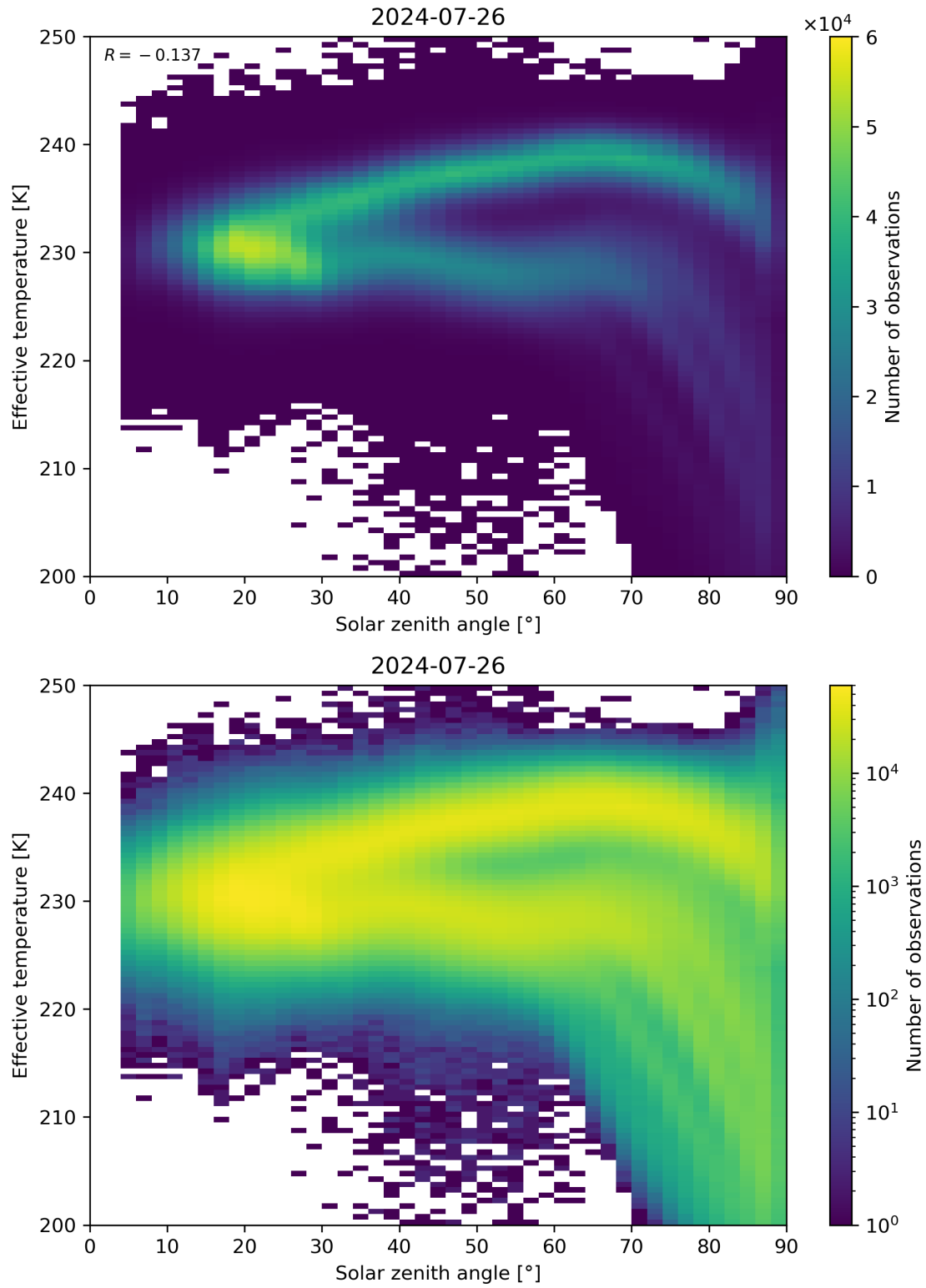
Figure 45: Scatter density plot of “Solar zenith angle” against “Effective temperature” for 2024-07-26 to 2024-07-27.
