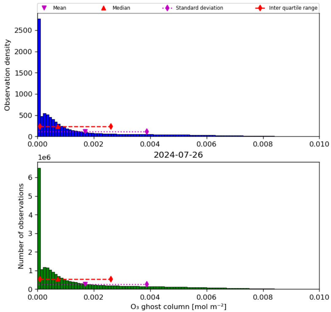
Figure 25: Histogram of “O 3 ghost column” for 2024-07-26 to 2024-07-27
