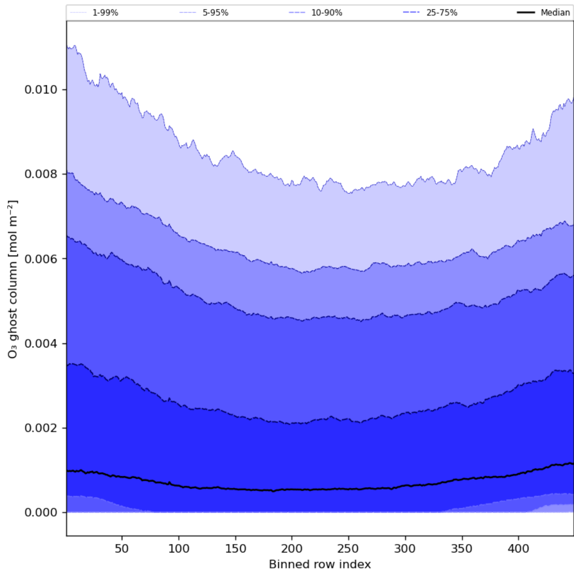
Figure 32: Along track statistics of “O 3 ghost column” for 2024-07-26 to 2024-07-27
