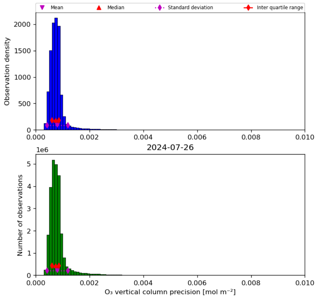
Figure 22: Histogram of “O 3 vertical column precision” for 2024-07-26 to 2024-07-27
