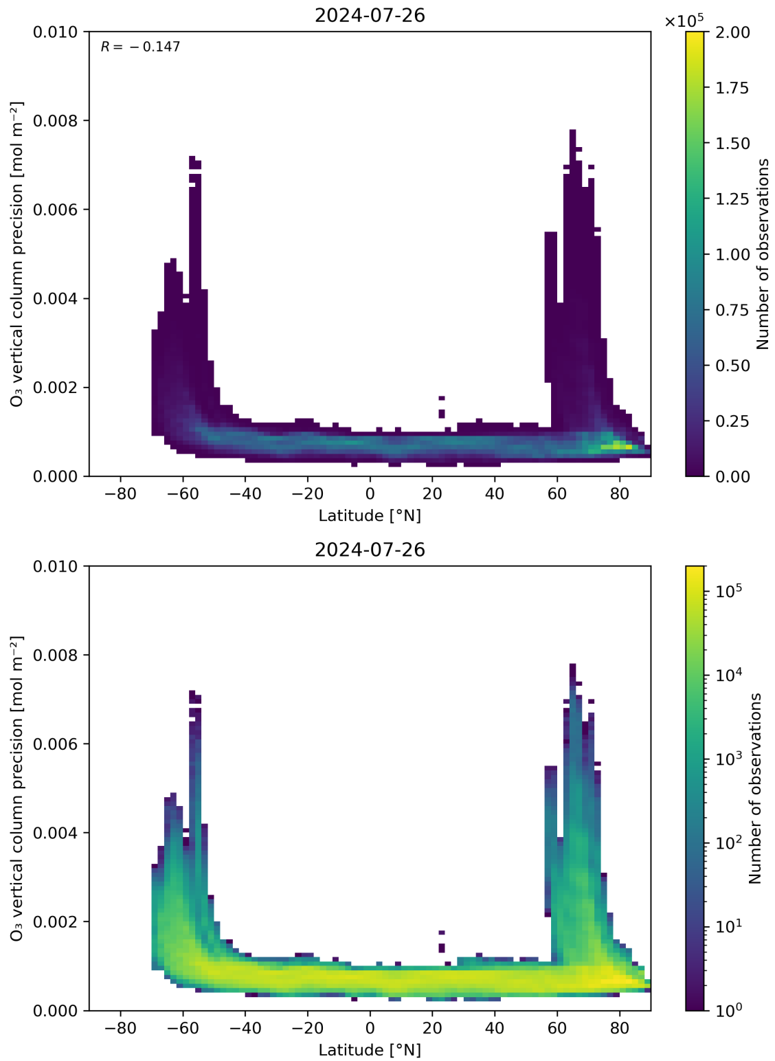
Figure 37: Scatter density plot of “Latitude” against “O 3 vertical column precision” for 2024-07-26 to 2024-07-27.
