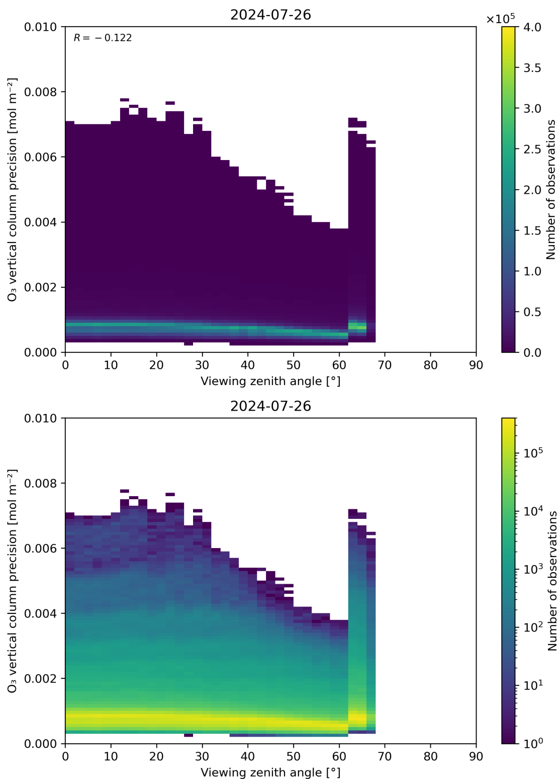
Figure 53: Scatter density plot of “Viewing zenith angle” against “O 3 vertical column precision” for 2024-07-26 to 2024-07-27.
