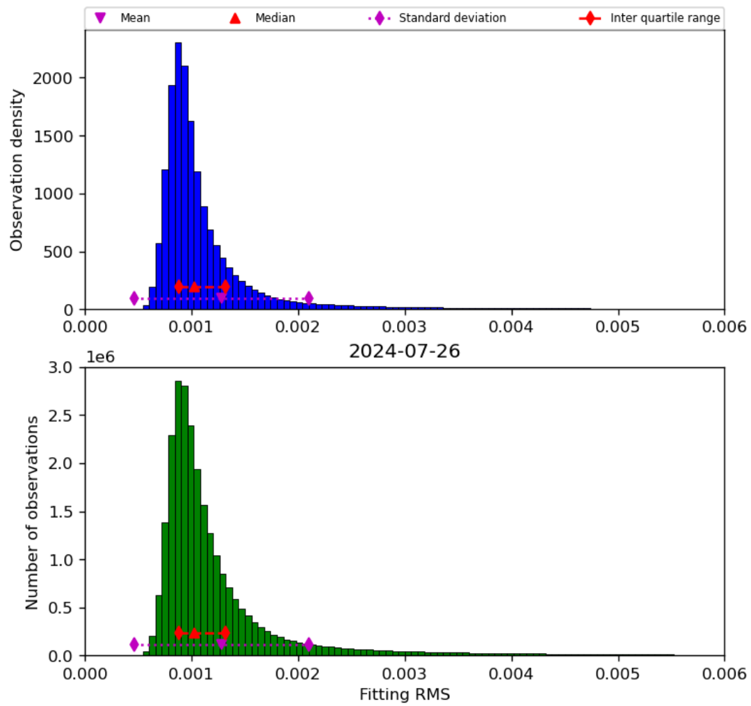
Figure 23: Histogram of “Fitting RMS” for 2024-07-26 to 2024-07-27
