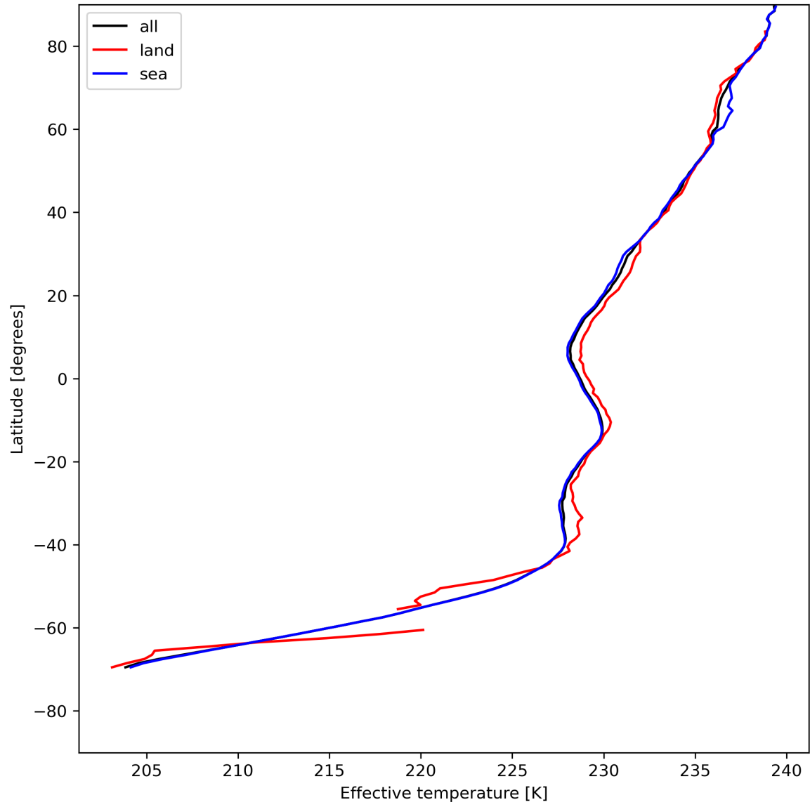
Figure 17: Zonal average of “Effective temperature” for 2024-07-26 to 2024-07-27.
