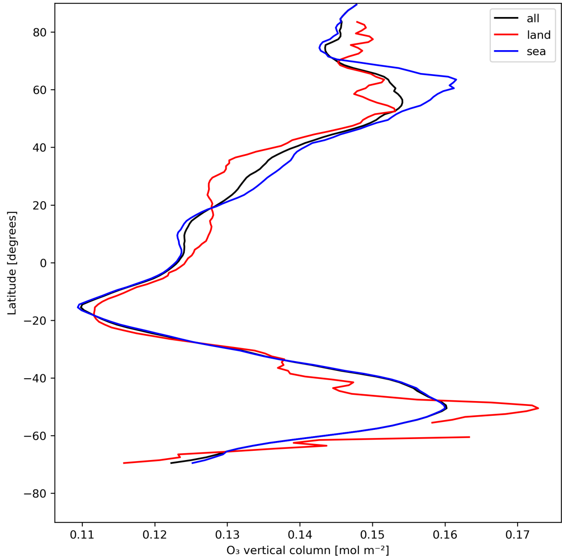
Figure 14: Zonal average of “O 3 vertical column” for 2024-07-26 to 2024-07-27.
