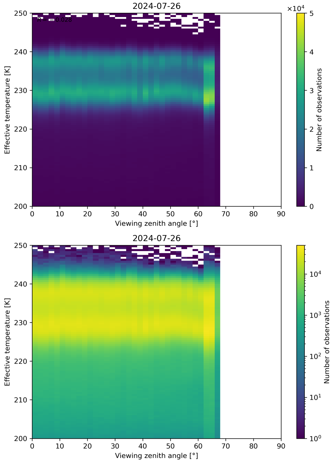
Figure 50: Scatter density plot of “Viewing zenith angle” against “Effective temperature” for 2024-07-26 to 2024-07-27.
