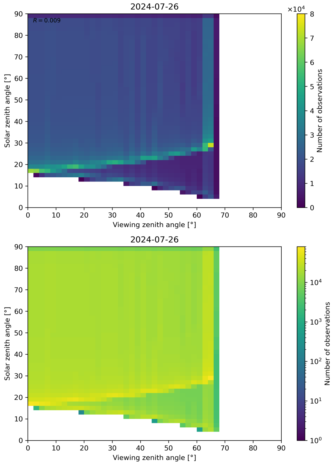
Figure 54: Scatter density plot of “Viewing zenith angle” against “Solar zenith angle” for 2024-07-26 to 2024-07-27.
