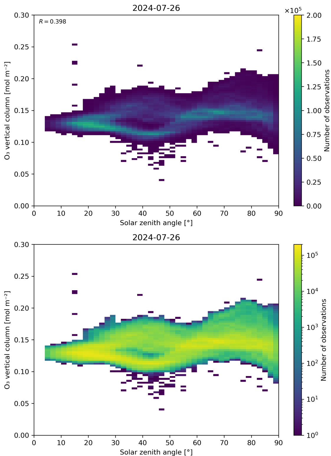
Figure 47: Scatter density plot of “Solar zenith angle” against “O 3 vertical column” for 2024-07-26 to 2024-07-27.
