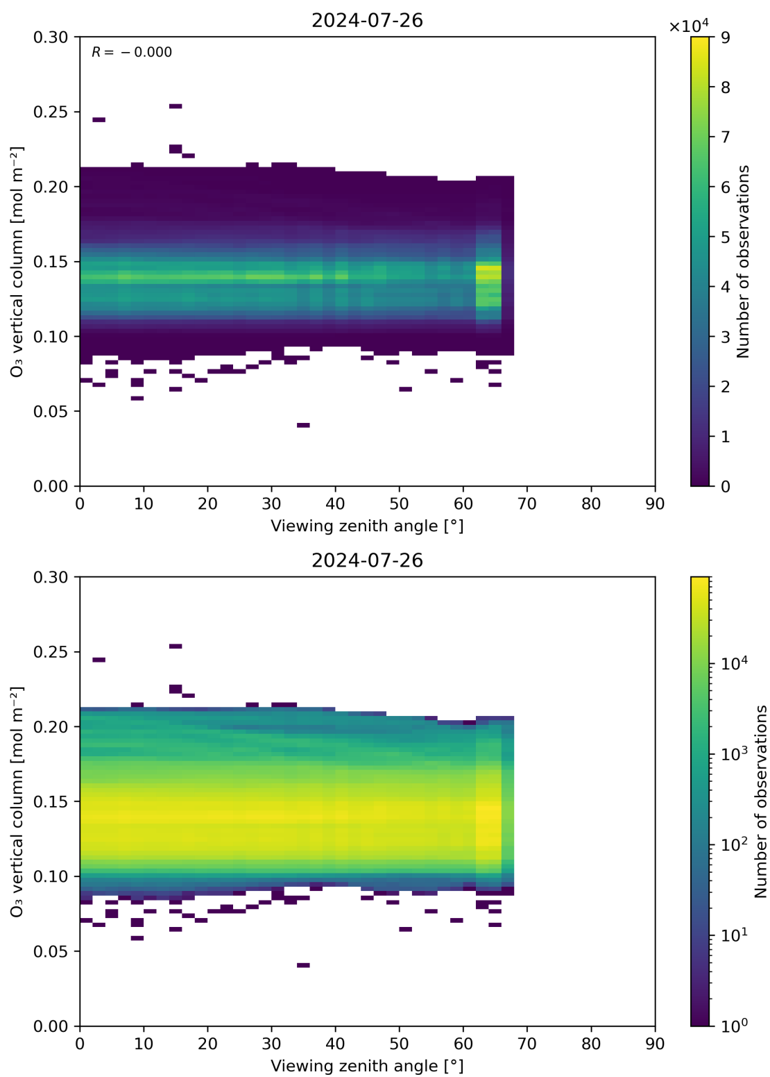
Figure 52: Scatter density plot of “Viewing zenith angle” against “O 3 vertical column” for 2024-07-26 to 2024-07-27.
