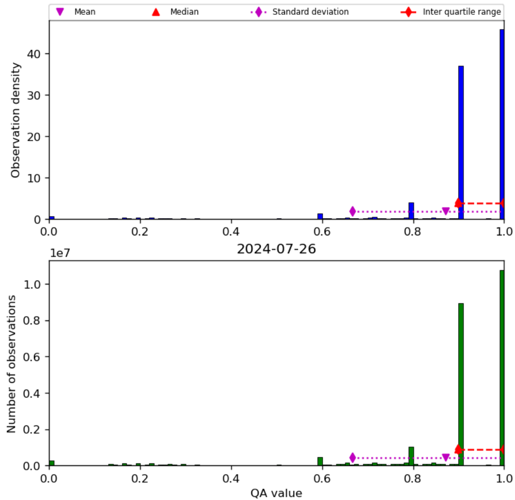
Figure 20: Histogram of “QA value” for 2024-07-26 to 2024-07-27
