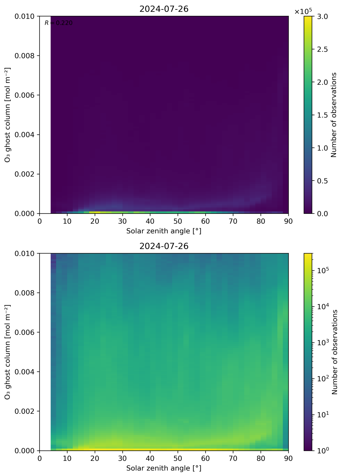
Figure 46: Scatter density plot of “Solar zenith angle” against “O 3 ghost column” for 2024-07-26 to 2024-07-27.
