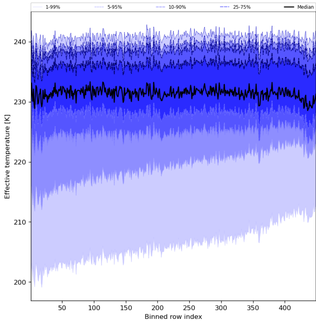
Figure 31: Along track statistics of “Effective temperature” for 2024-07-26 to 2024-07-27
