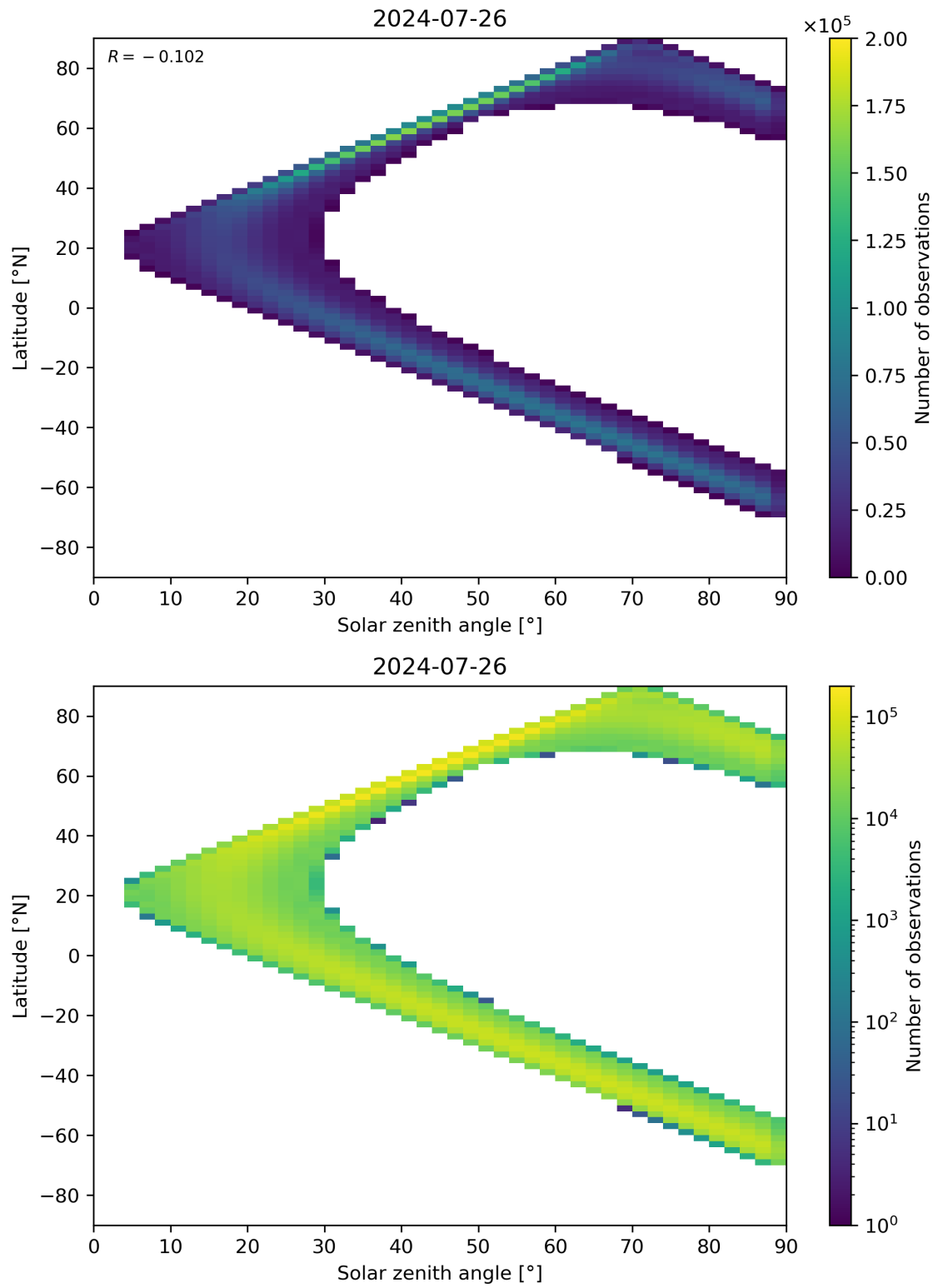
Figure 44: Scatter density plot of “Solar zenith angle” against “Latitude” for 2024-07-26 to 2024-07-27.
