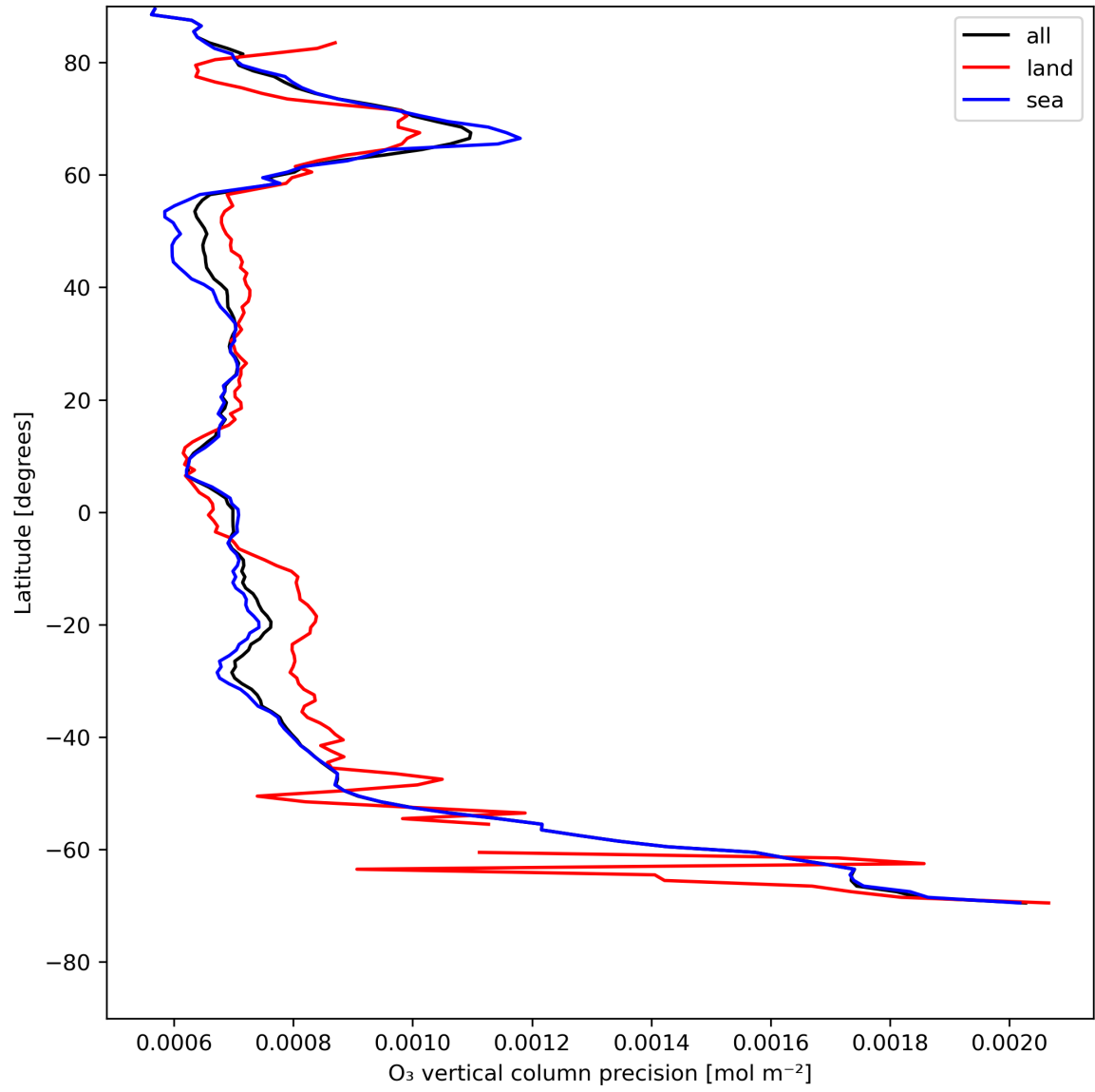
Figure 15: Zonal average of “O 3 vertical column precision” for 2024-07-26 to 2024-07-27.
