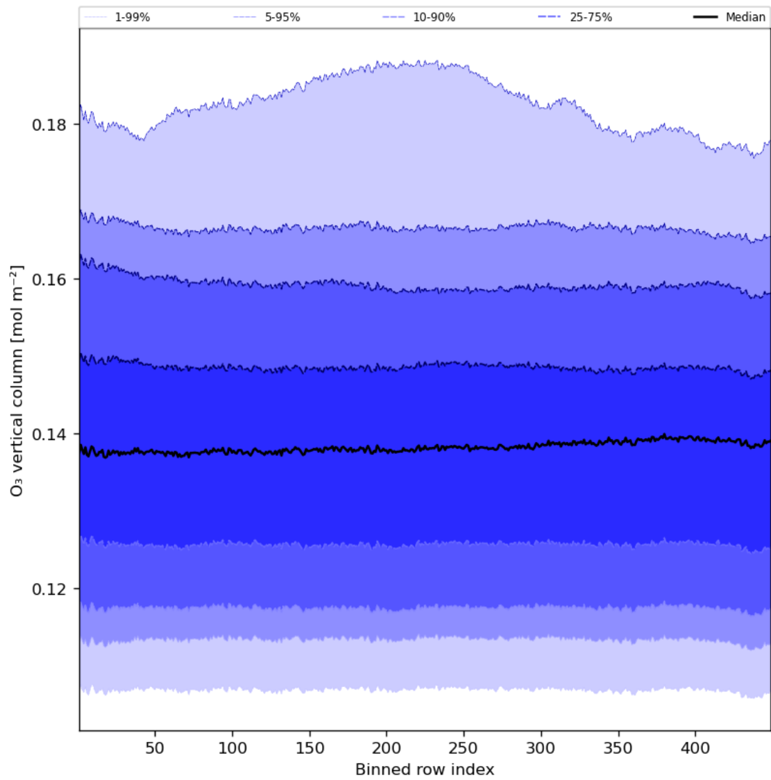
Figure 28: Along track statistics of “O 3 vertical column” for 2024-07-26 to 2024-07-27
