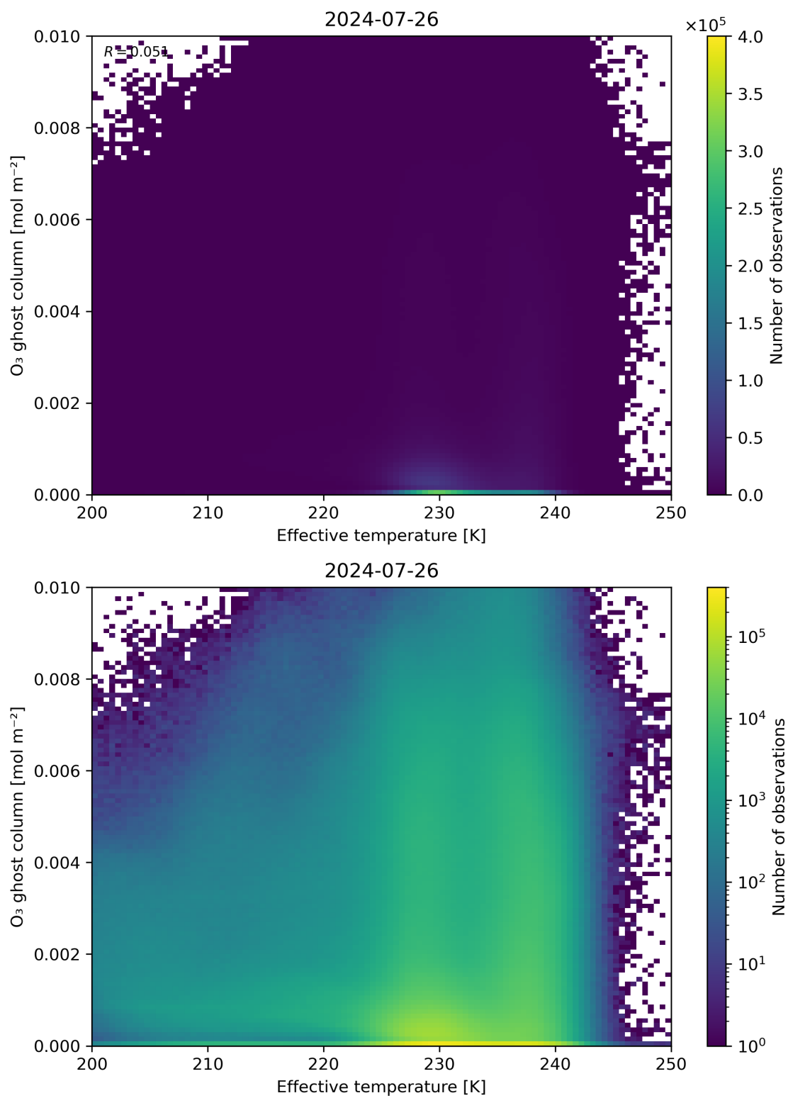
Figure 38: Scatter density plot of “Effective temperature” against “O 3 ghost column” for 2024-07-26 to 2024-07-27.
