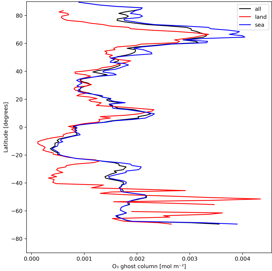
Figure 18: Zonal average of "O 3 ghost column" for 2024-07-26 to 2024-07-27.
