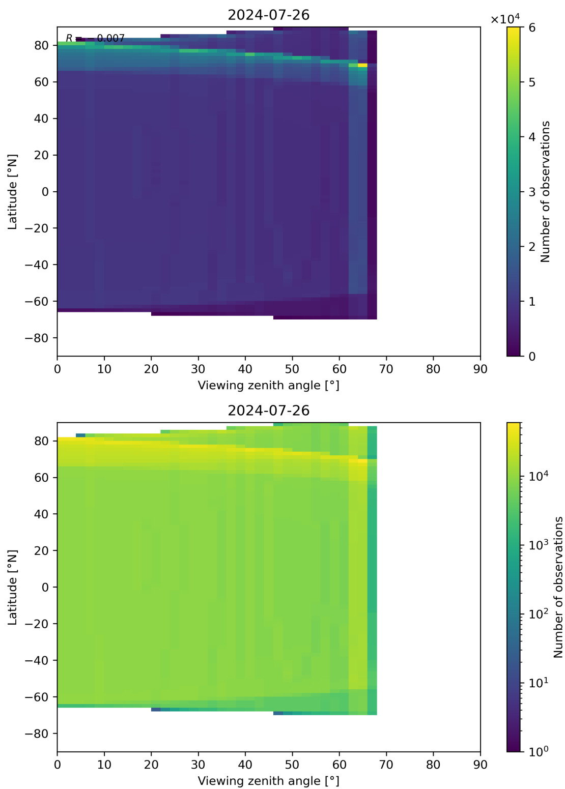
Figure 49: Scatter density plot of “Viewing zenith angle” against “Latitude” for 2024-07-26 to 2024-07-27.
