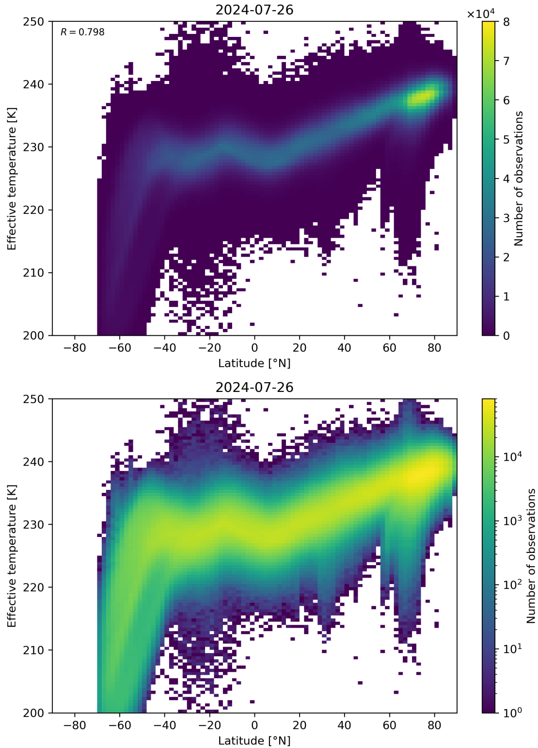
Figure 34: Scatter density plot of “Latitude” against “Effective temperature” for 2024-07-26 to 2024-07-27.
