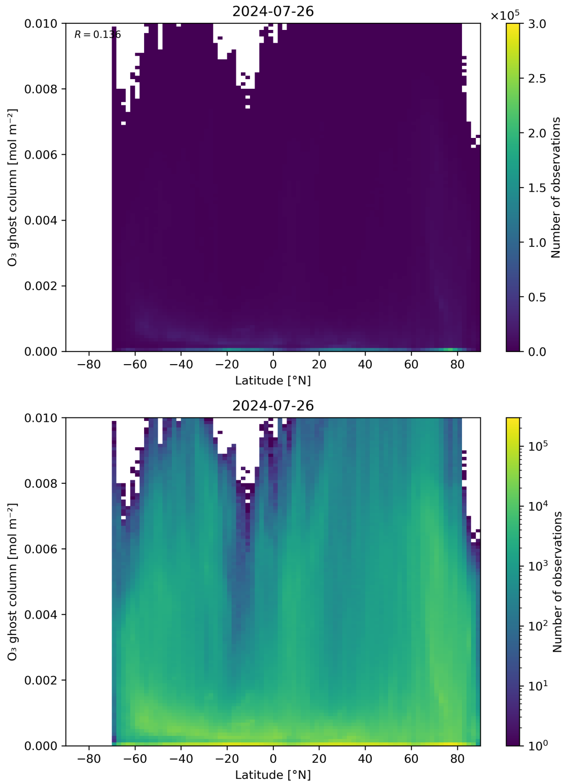
Figure 35: Scatter density plot of “Latitude” against “O 3 ghost column” for 2024-07-26 to 2024-07-27.
