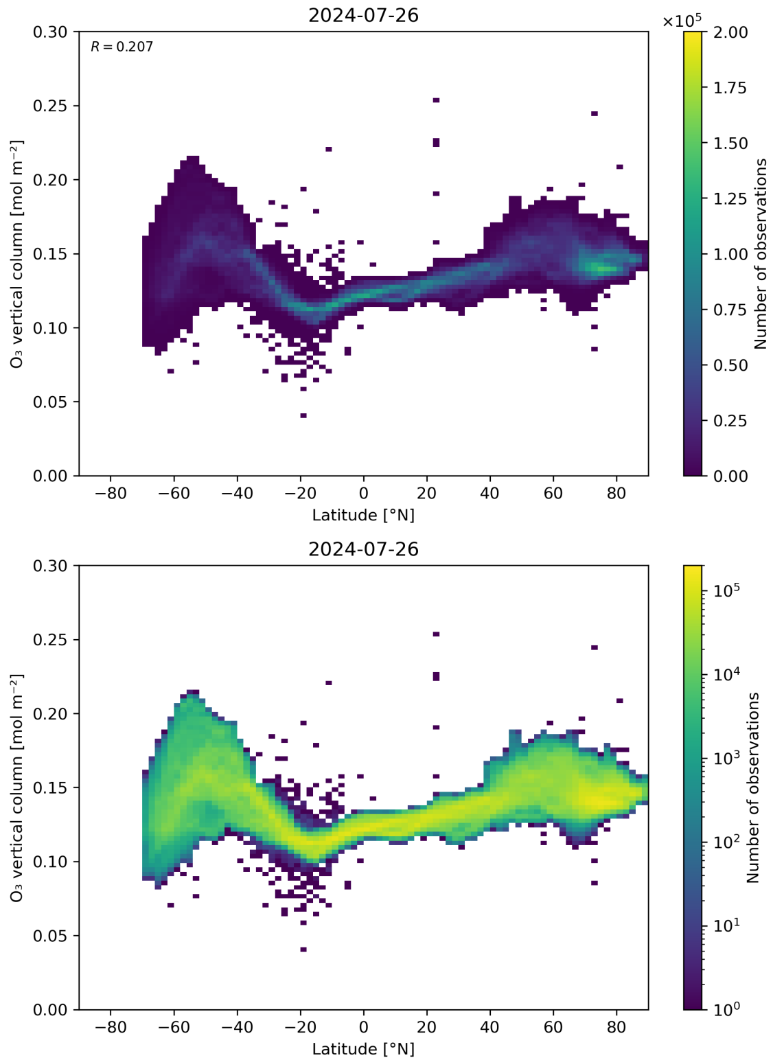
Figure 36: Scatter density plot of “Latitude” against “O 3 vertical column” for 2024-07-26 to 2024-07-27.
