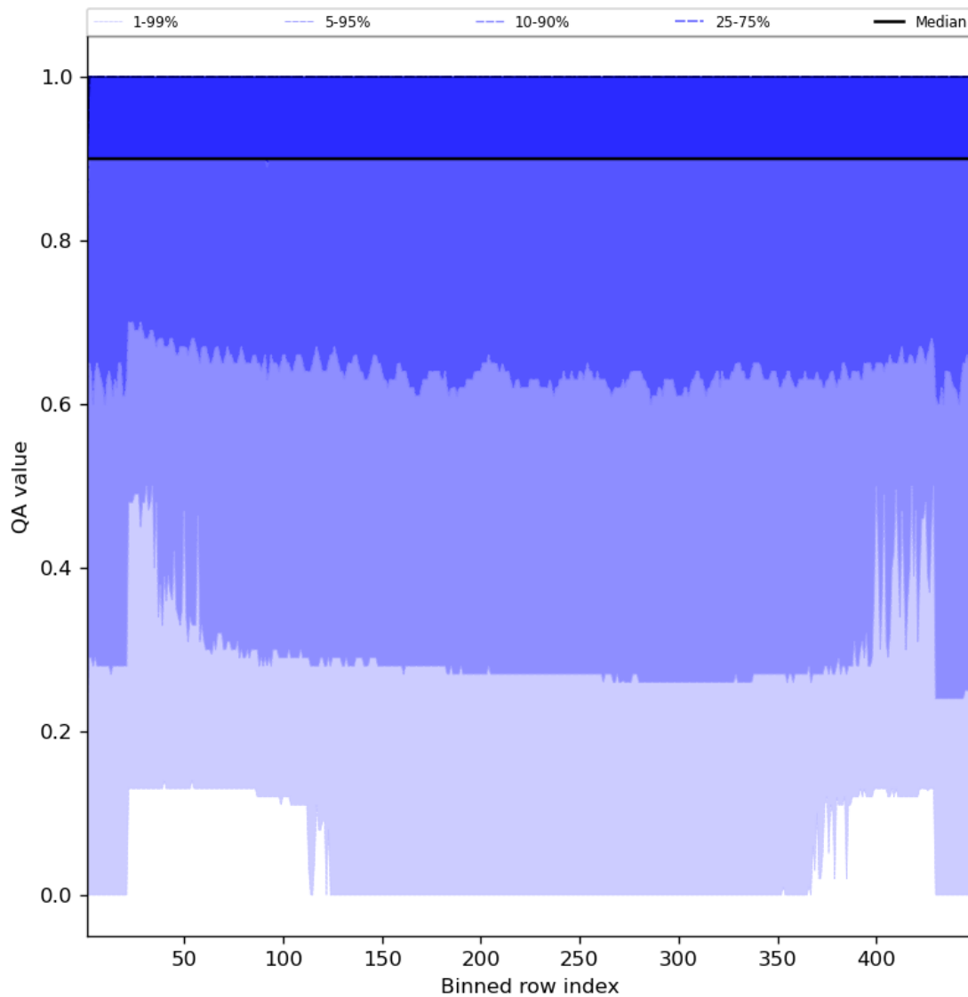
Figure 27: Along track statistics of “QA value” for 2024-07-26 to 2024-07-27
