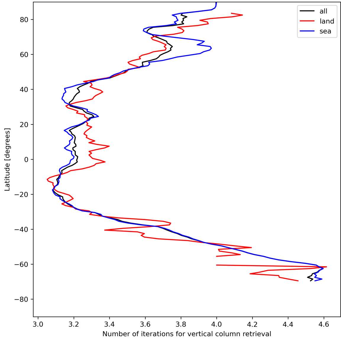
Figure 19: Zonal average of “Number of iterations for vertical column retrieval” for 2024-07-26 to 2024-07-27.
