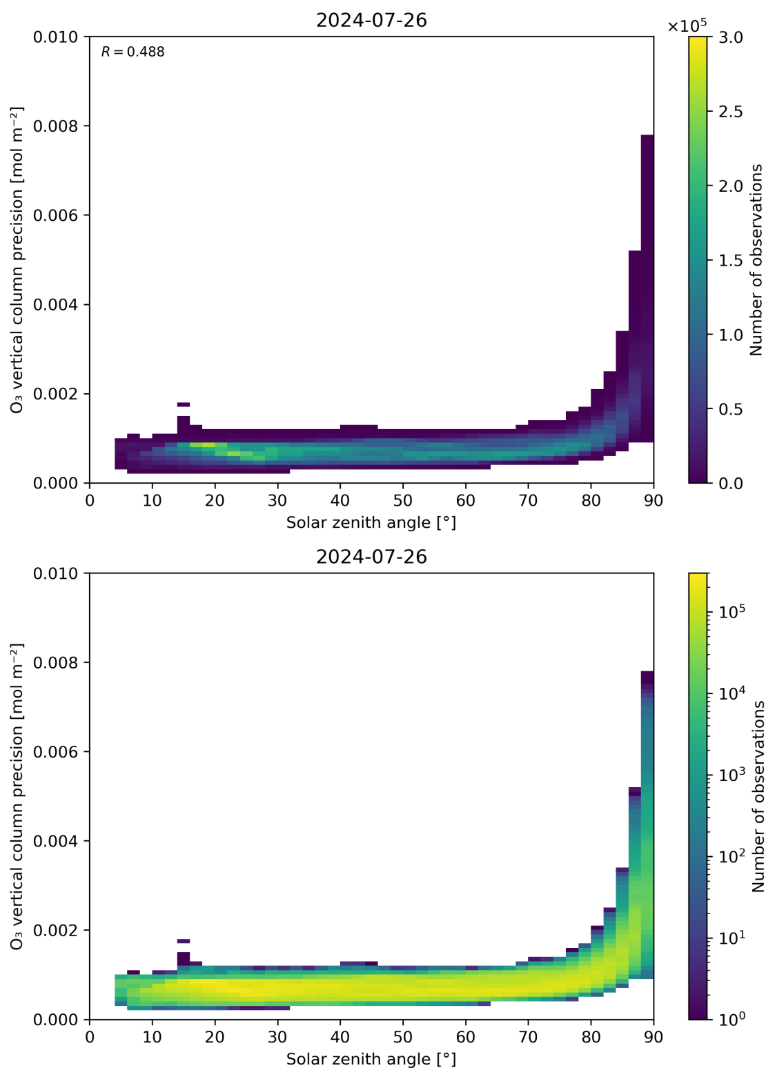
Figure 48: Scatter density plot of “Solar zenith angle” against “O 3 vertical column precision” for 2024-07-26 to 2024-07-27.
