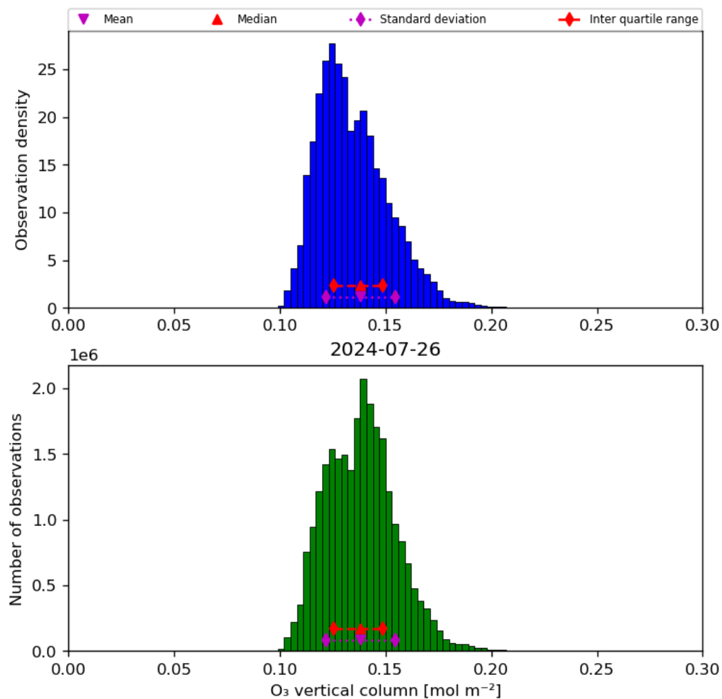
Figure 21: Histogram of “O 3 vertical column” for 2024-07-26 to 2024-07-27
