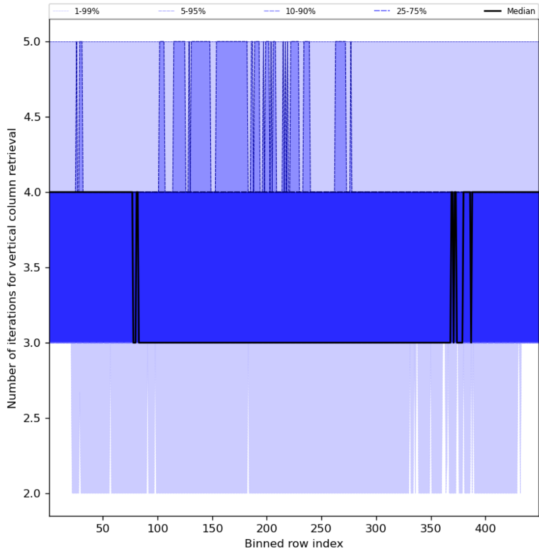
Figure 33: Along track statistics of “Number of iterations for vertical column retrieval” for 2024-07-26 to 2024-07-27
