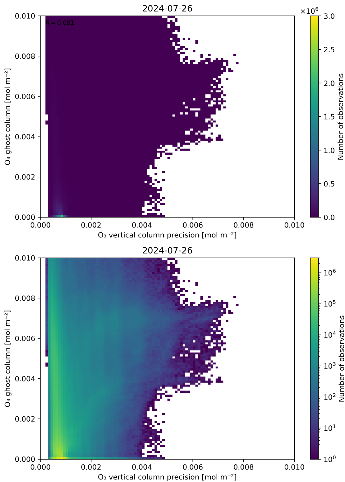
Figure 43: Scatter density plot of “ \text{O}_3 vertical column precision” against “ \text{O}_3 ghost column” for 2024-07-26 to 2024-07-27.
