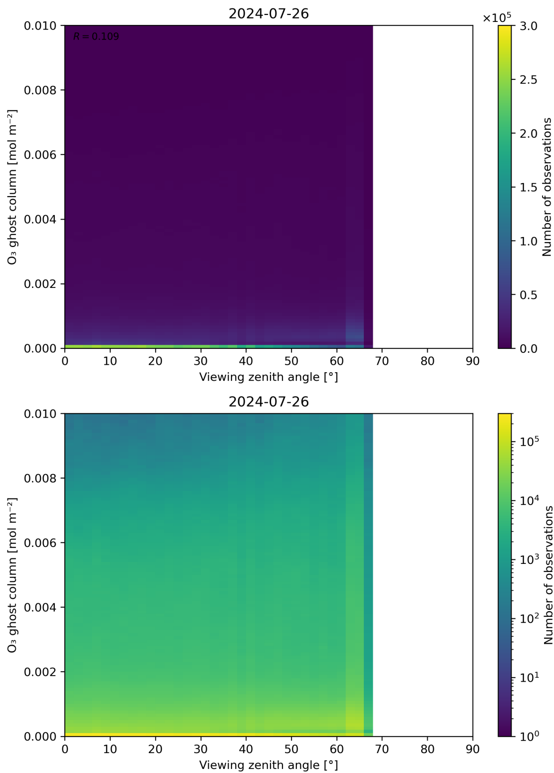
Figure 51: Scatter density plot of “Viewing zenith angle” against “O 3 ghost column” for 2024-07-26 to 2024-07-27.
