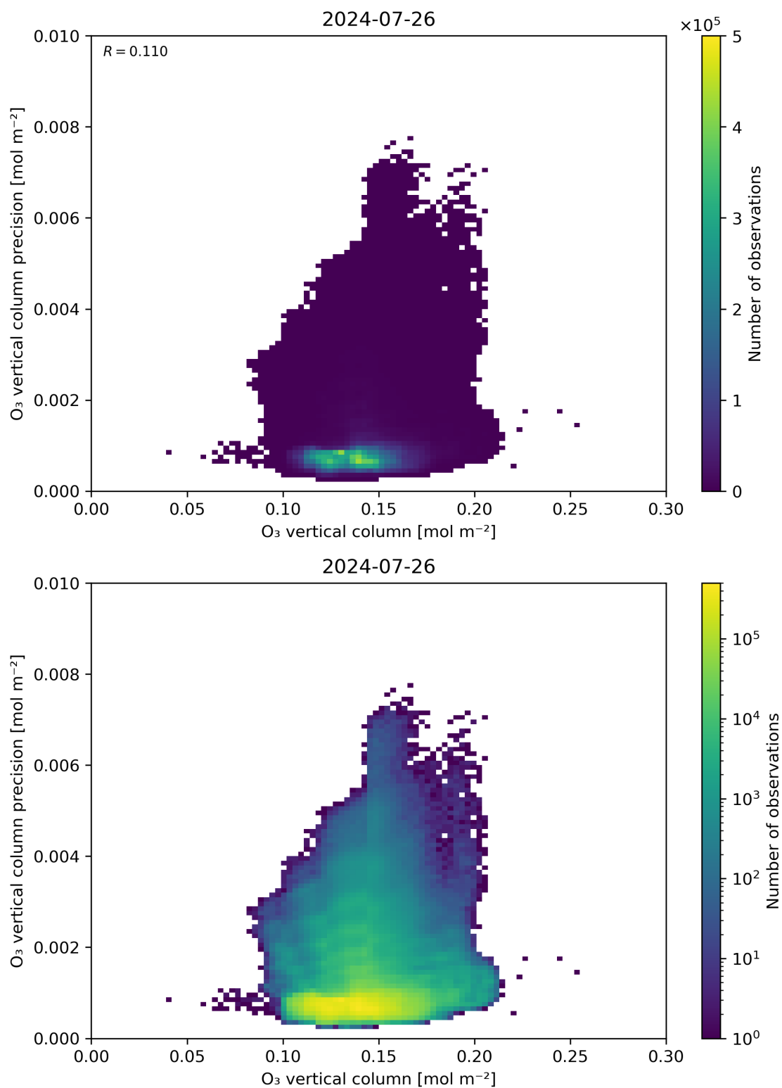
Figure 41: Scatter density plot of “O 3 vertical column” against “O 3 vertical column precision” for 2024-07-26 to 2024-07-27.
