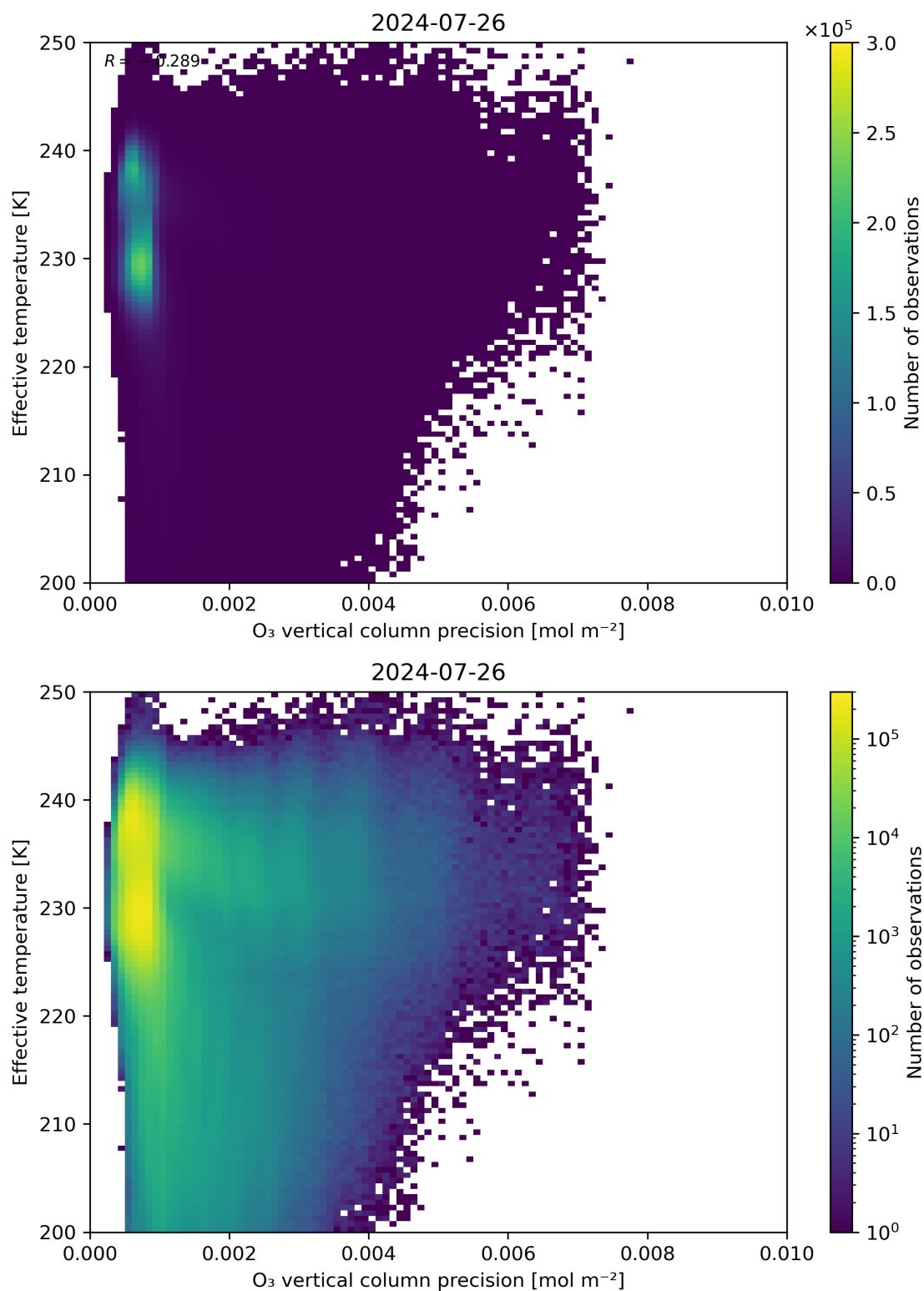
Figure 42: Scatter density plot of “O 3 vertical column precision” against “Effective temperature” for 2024-07-26 to 2024-07-27.
