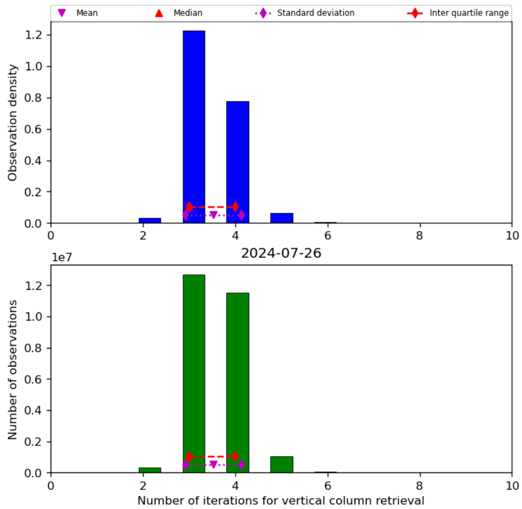
Figure 26: Histogram of “Number of iterations for vertical column retrieval” for 2024-07-26 to 2024-07-27
