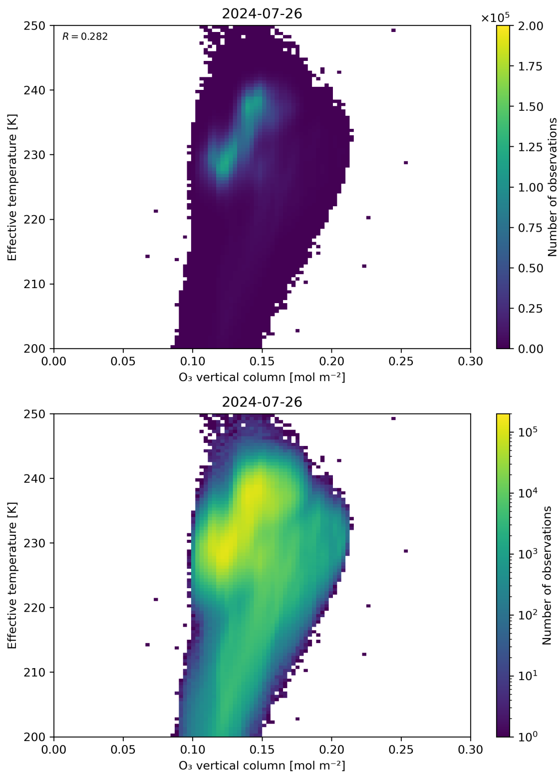
Figure 39: Scatter density plot of “O 3 vertical column” against “Effective temperature” for 2024-07-26 to 2024-07-27.
