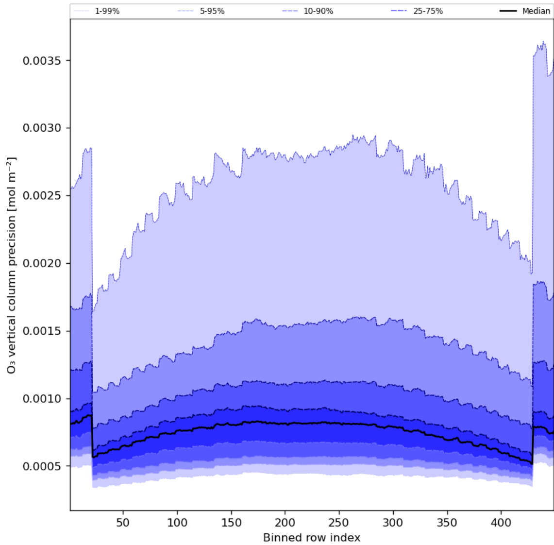
Figure 29: Along track statistics of “O 3 vertical column precision” for 2024-07-26 to 2024-07-27
