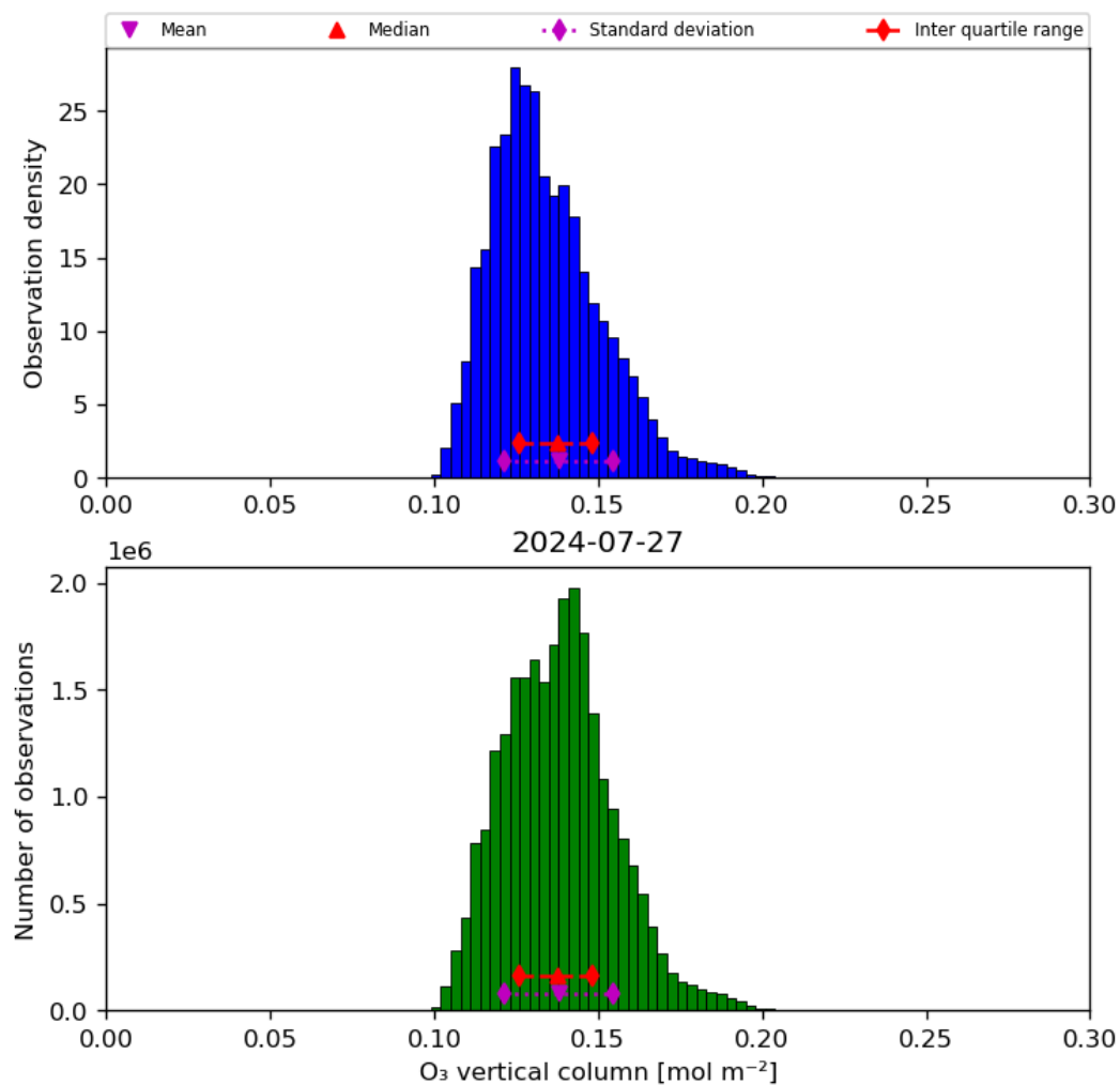
Figure 21: Histogram of “O 3 vertical column” for 2024-07-26 to 2024-07-28
