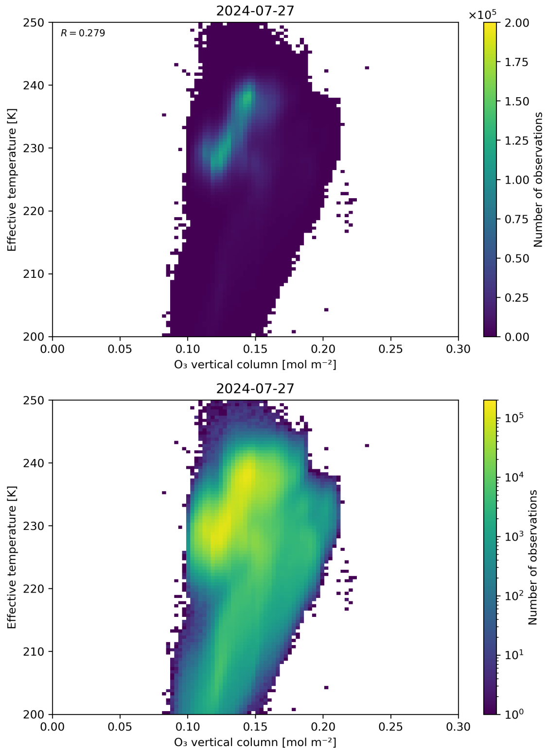
Figure 39: Scatter density plot of “O 3 vertical column” against “Effective temperature” for 2024-07-26 to 2024-07-28.
