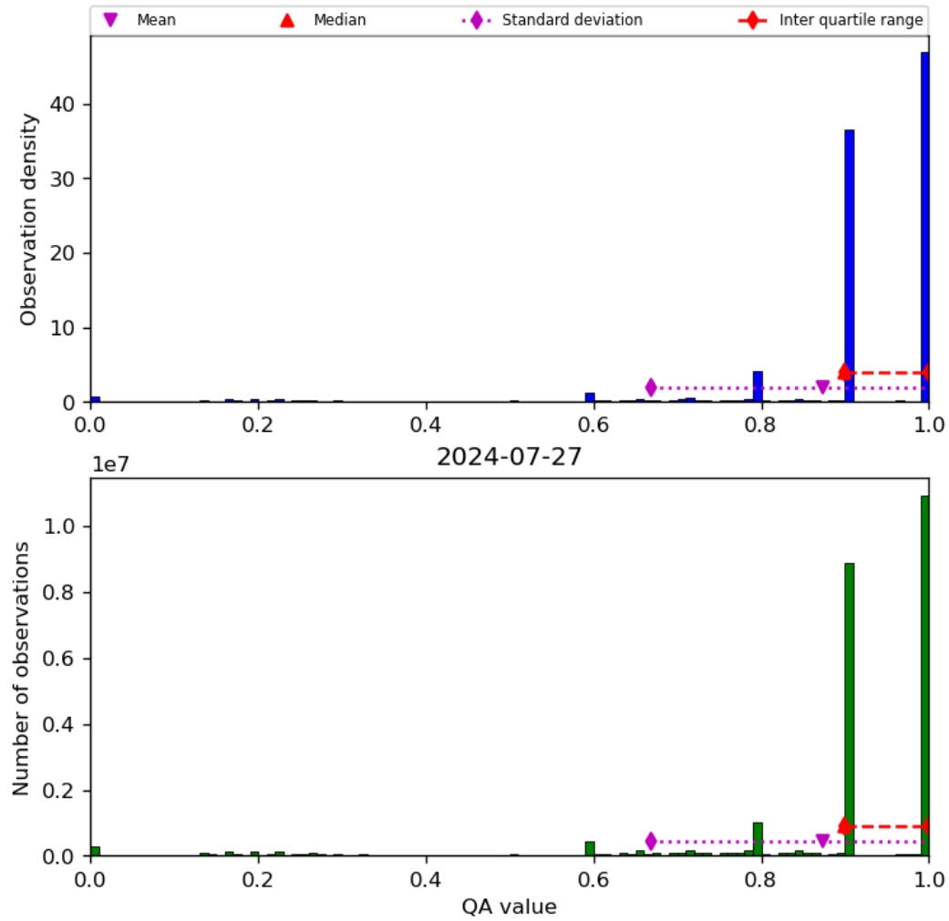
Figure 20: Histogram of “QA value” for 2024-07-26 to 2024-07-28
