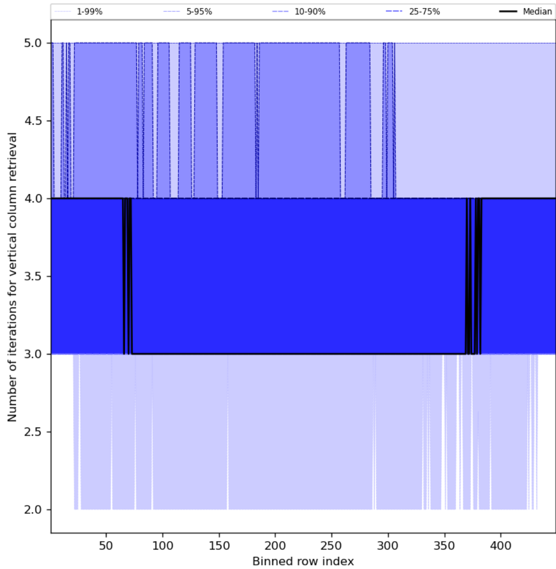
Figure 33: Along track statistics of “Number of iterations for vertical column retrieval” for 2024-07-26 to 2024-07-28
