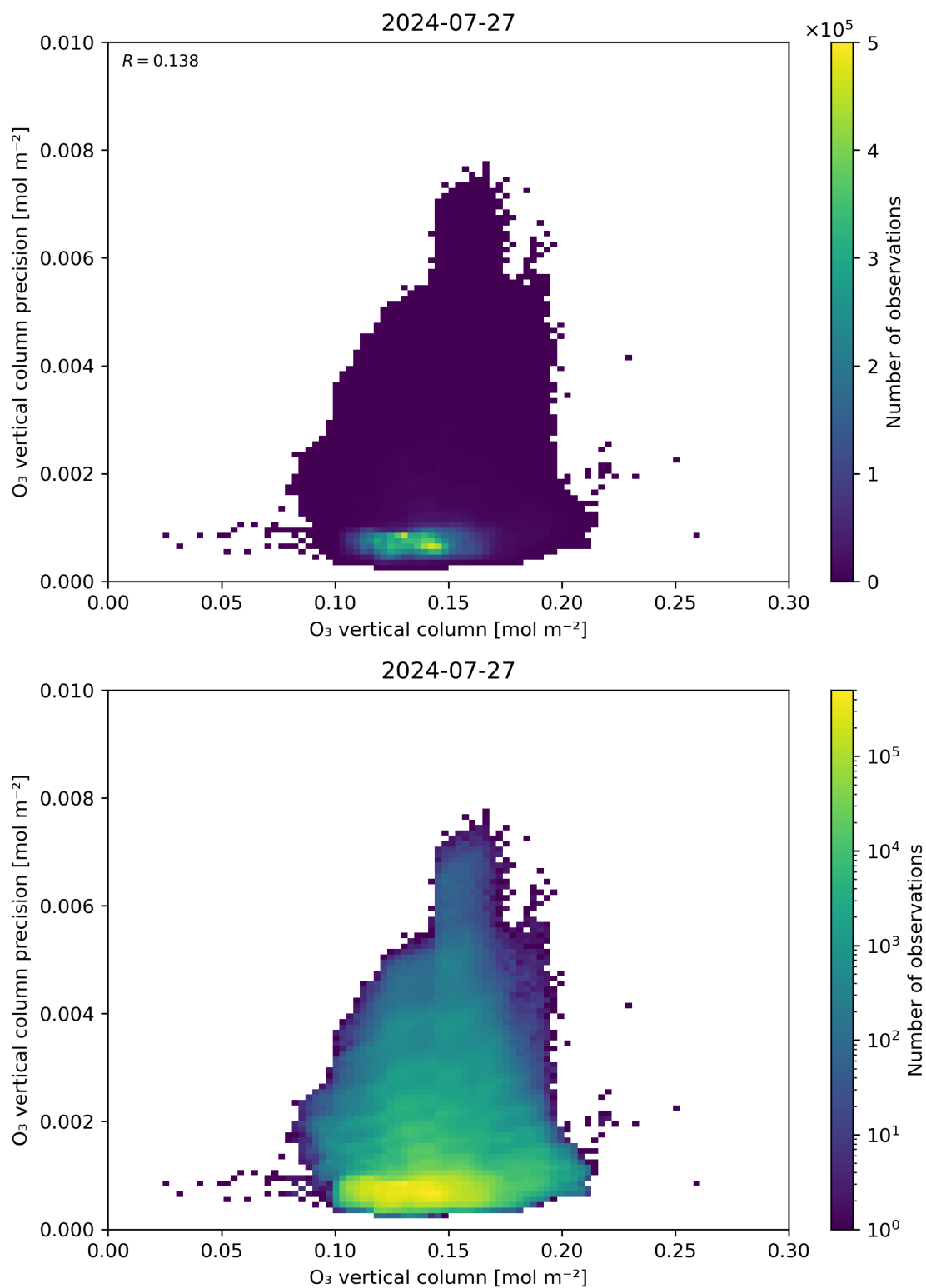
Figure 41: Scatter density plot of “O 3 vertical column” against “O 3 vertical column precision” for 2024-07-26 to 2024-07-28.
