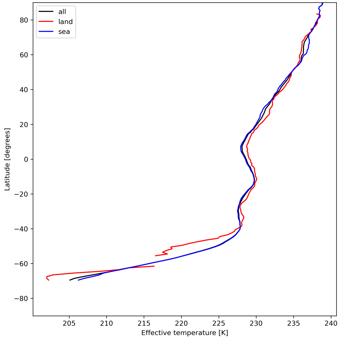
Figure 17: Zonal average of "Effective temperature" for 2024-07-26 to 2024-07-28.
