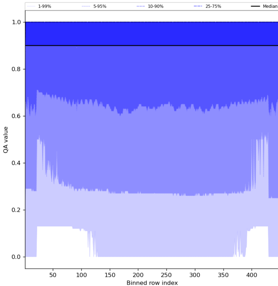
Figure 27: Along track statistics of “QA value” for 2024-07-26 to 2024-07-28
