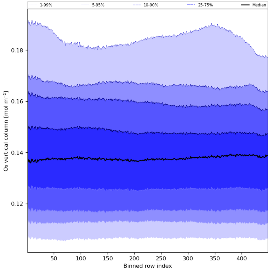
Figure 28: Along track statistics of “O 3 vertical column” for 2024-07-26 to 2024-07-28
