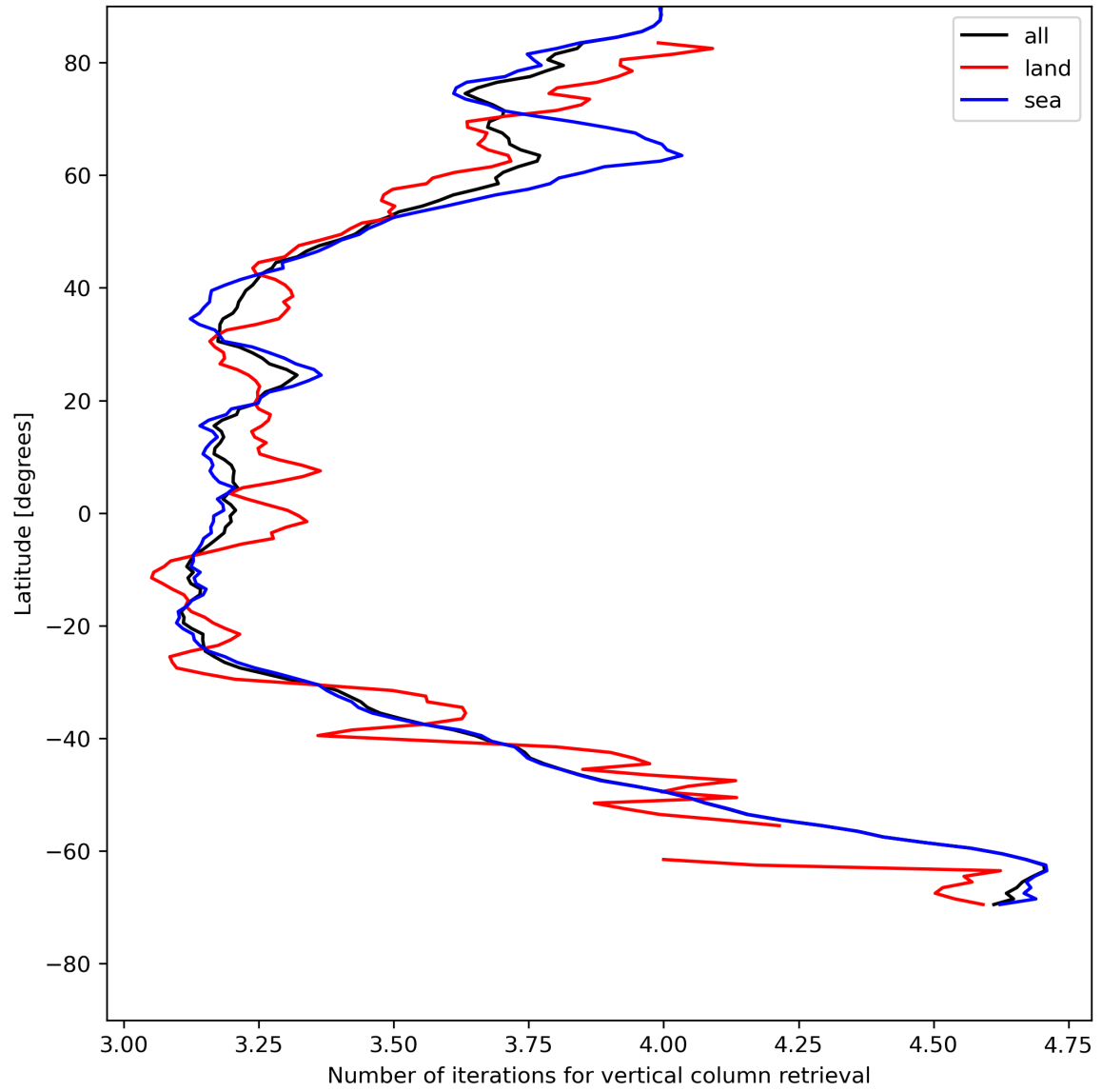
Figure 19: Zonal average of “Number of iterations for vertical column retrieval” for 2024-07-26 to 2024-07-28.
