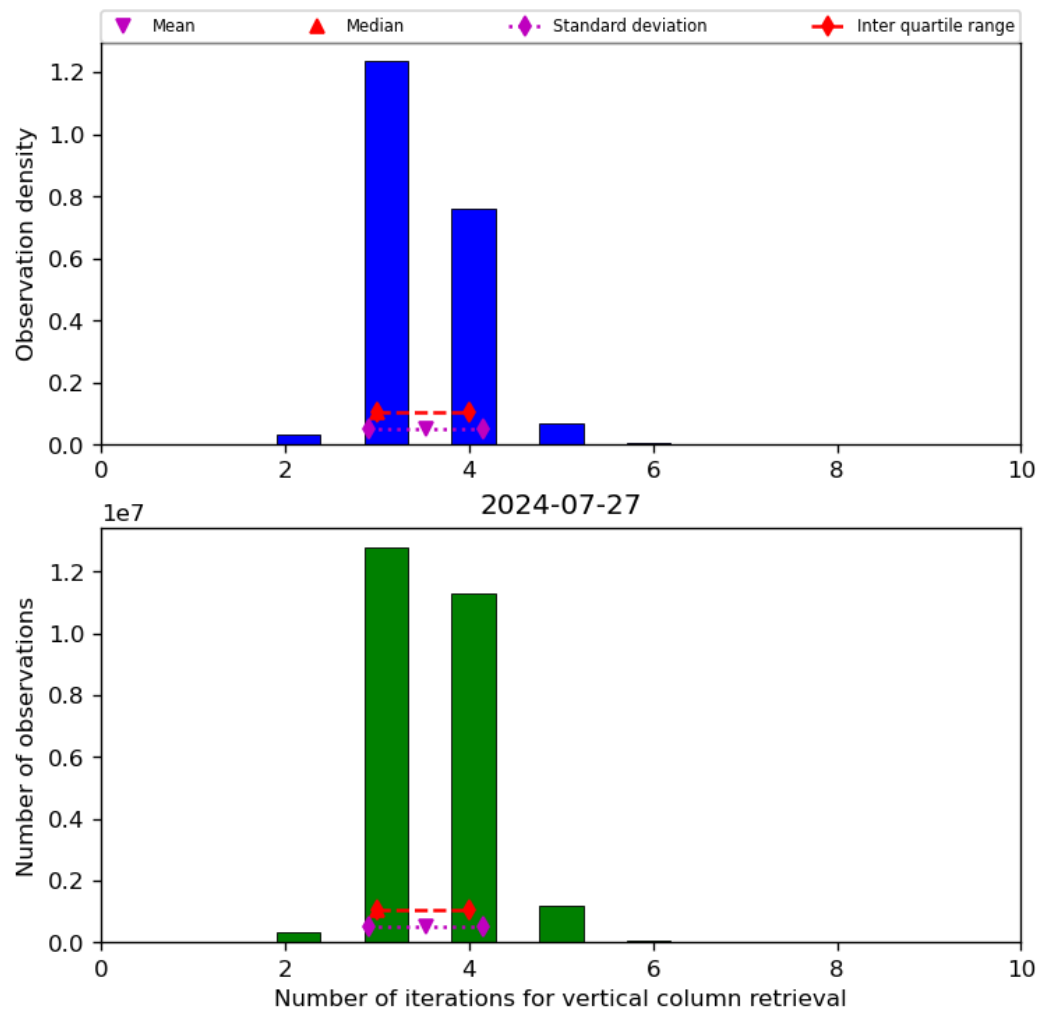
Figure 26: Histogram of “Number of iterations for vertical column retrieval” for 2024-07-26 to 2024-07-28
