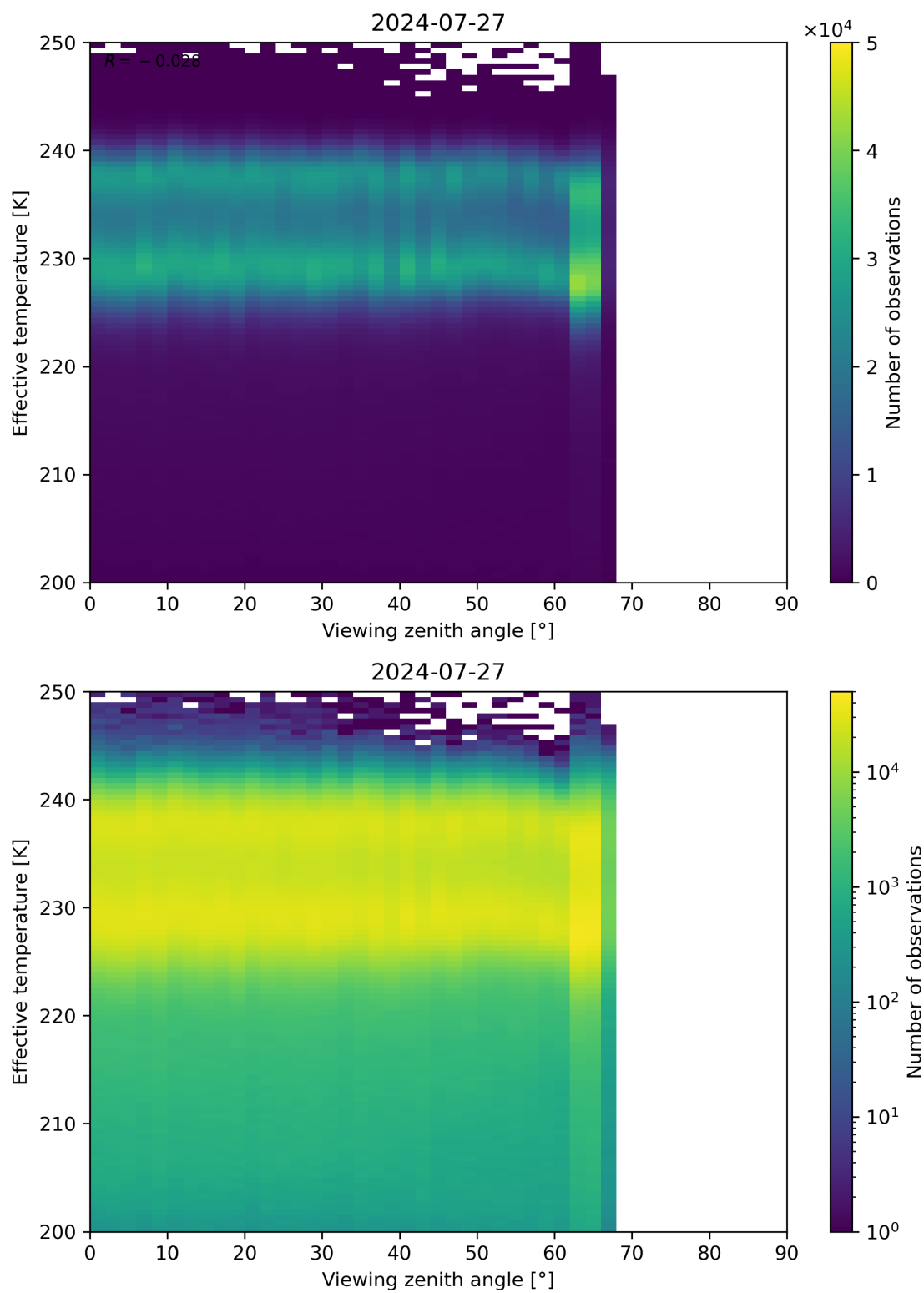
Figure 50: Scatter density plot of “Viewing zenith angle” against “Effective temperature” for 2024-07-26 to 2024-07-28.
