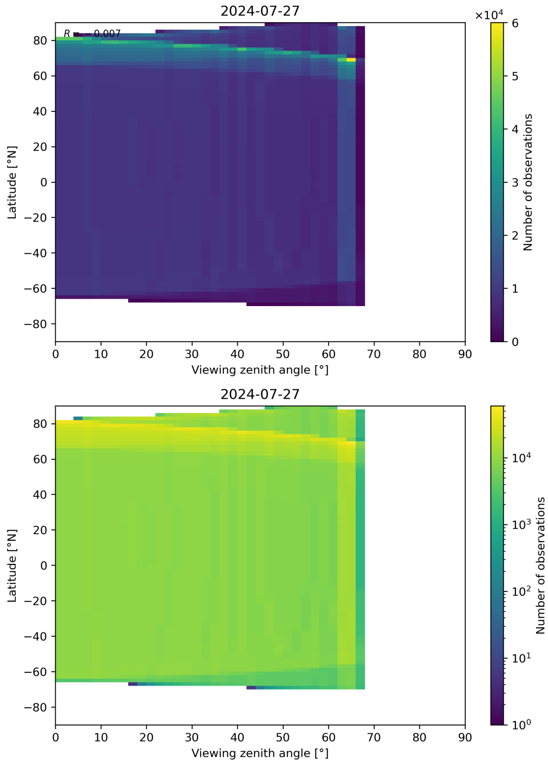
Figure 49: Scatter density plot of “Viewing zenith angle” against “Latitude” for 2024-07-26 to 2024-07-28.
