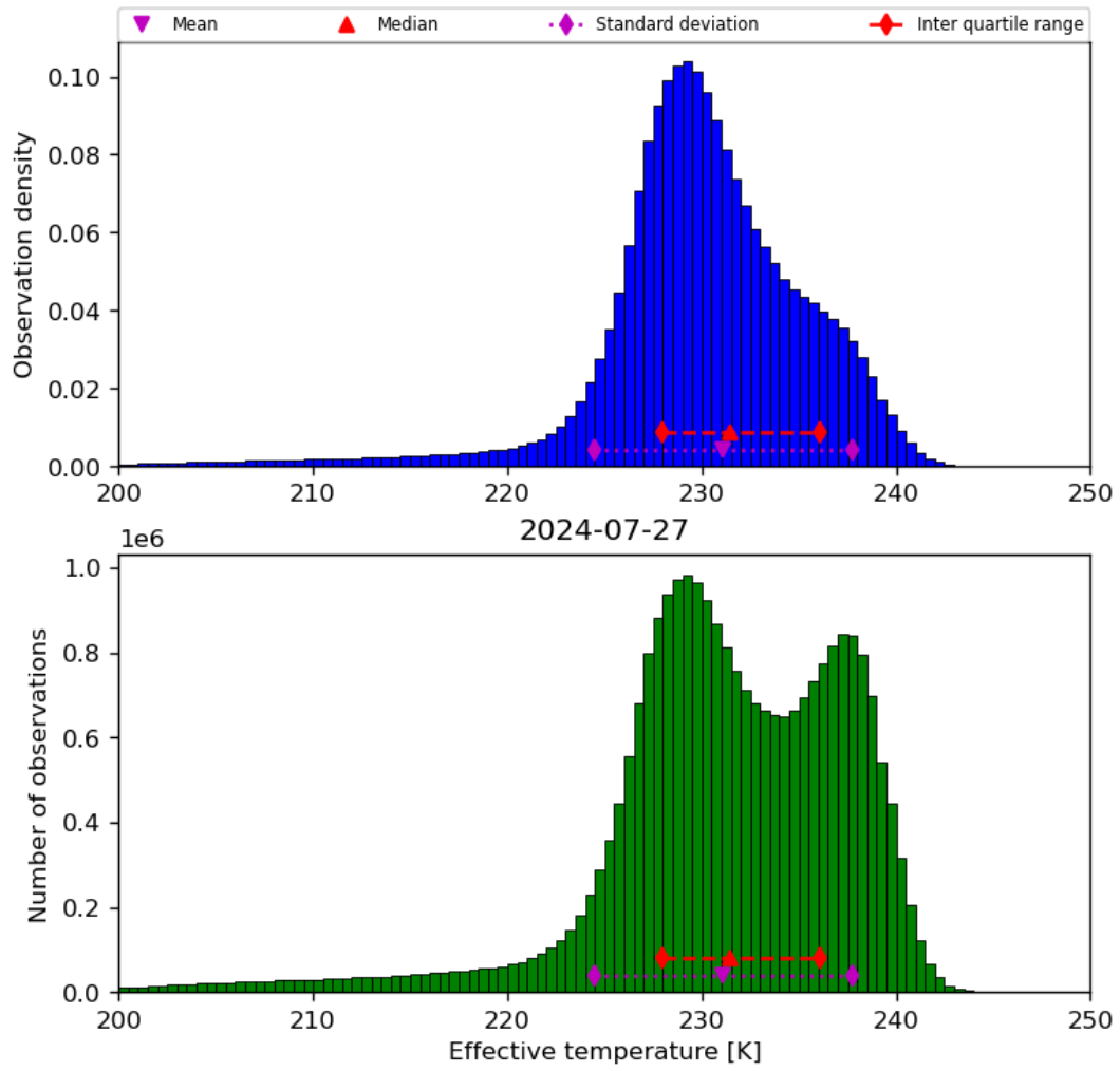
Figure 24: Histogram of “Effective temperature” for 2024-07-26 to 2024-07-28
