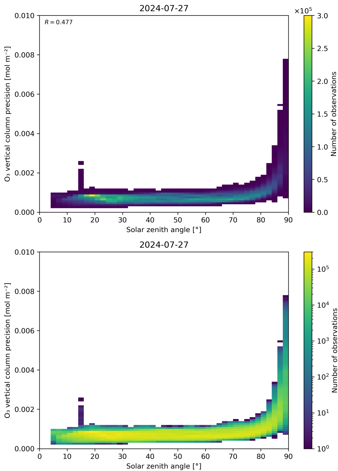
Figure 48: Scatter density plot of “Solar zenith angle” against “O 3 vertical column precision” for 2024-07-26 to 2024-07-28.
