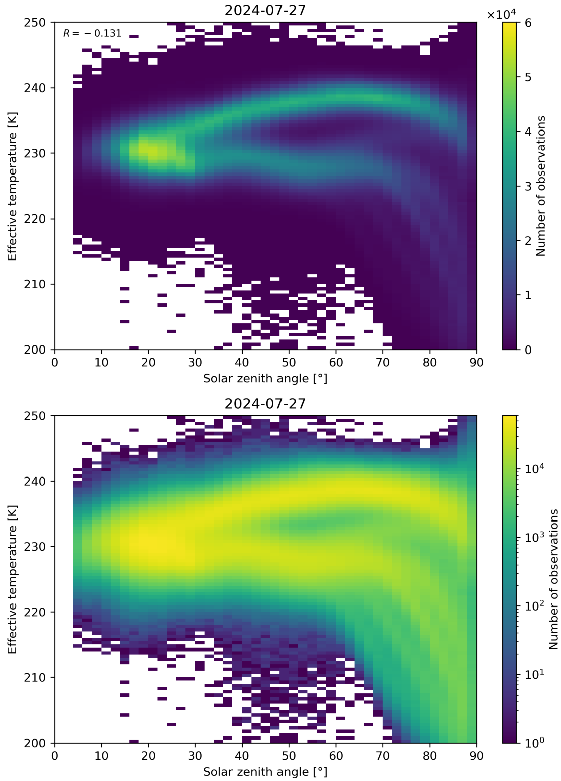
Figure 45: Scatter density plot of “Solar zenith angle” against “Effective temperature” for 2024-07-26 to 2024-07-28.
