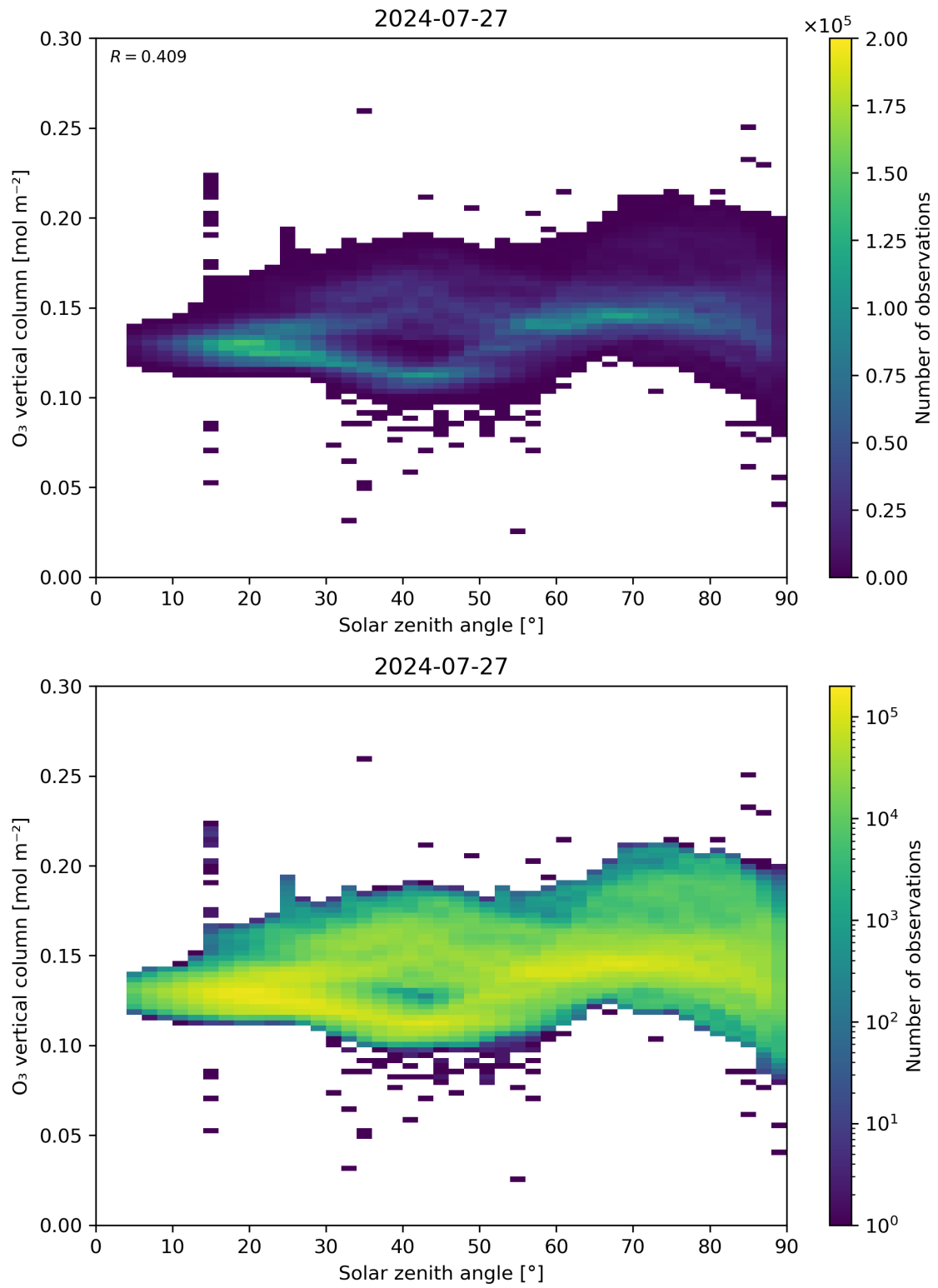
Figure 47: Scatter density plot of “Solar zenith angle” against “O 3 vertical column” for 2024-07-26 to 2024-07-28.
