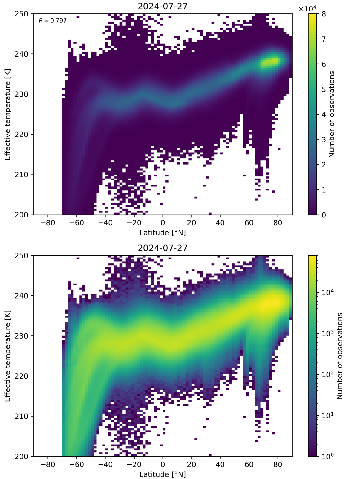
Figure 34: Scatter density plot of “Latitude” against “Effective temperature” for 2024-07-26 to 2024-07-28.
