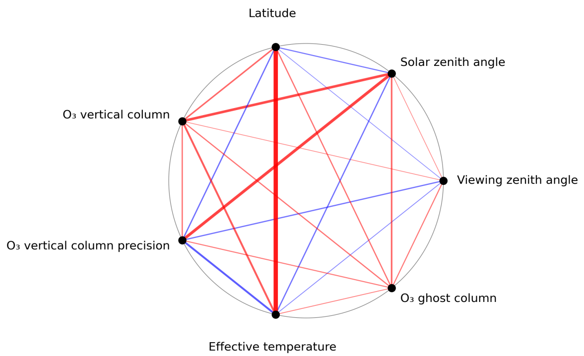
Figure 1: Map of correlation graph for 2024-07-26 to 2024-07-28.
