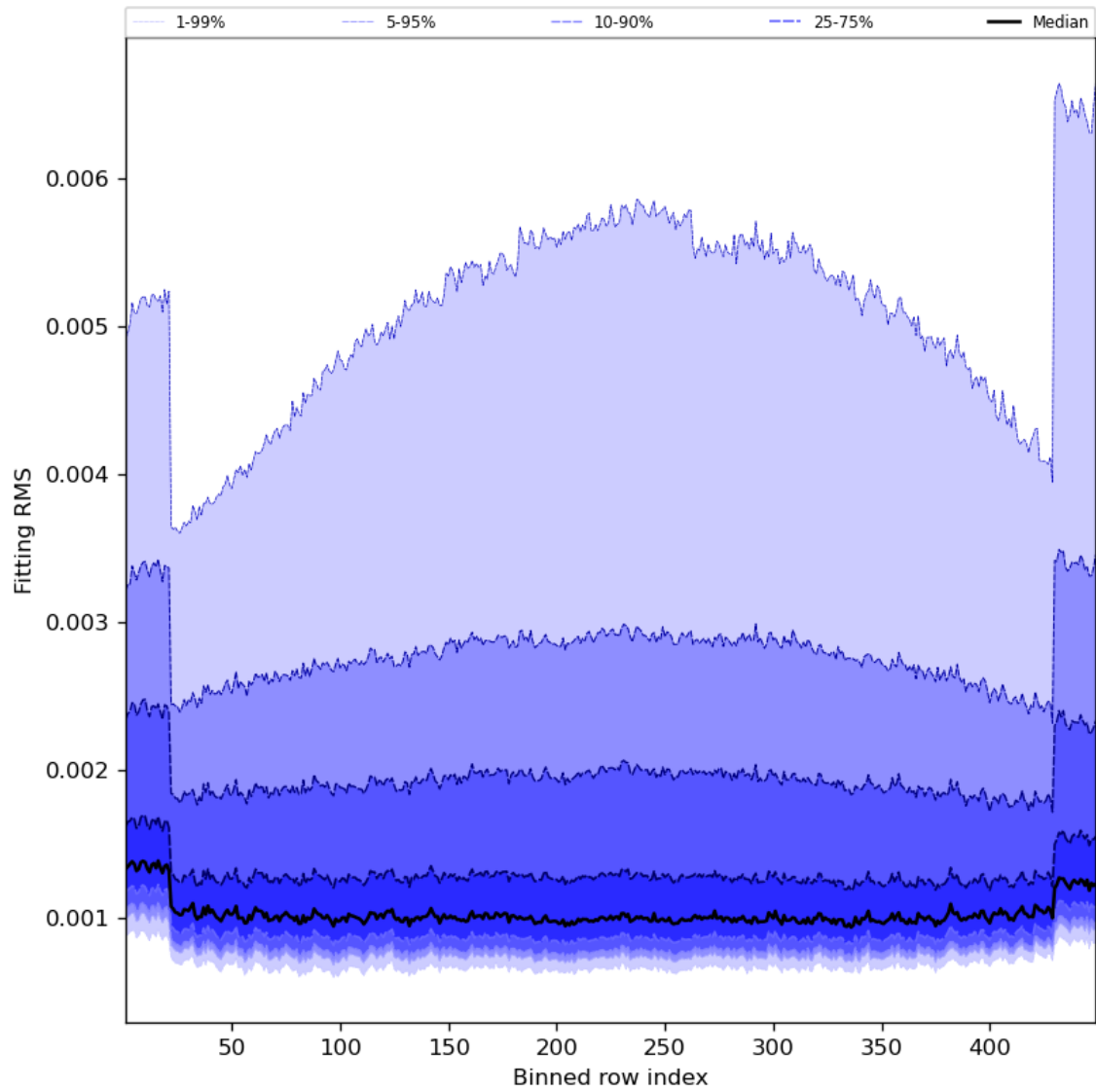
Figure 30: Along track statistics of “Fitting RMS” for 2024-07-26 to 2024-07-28
