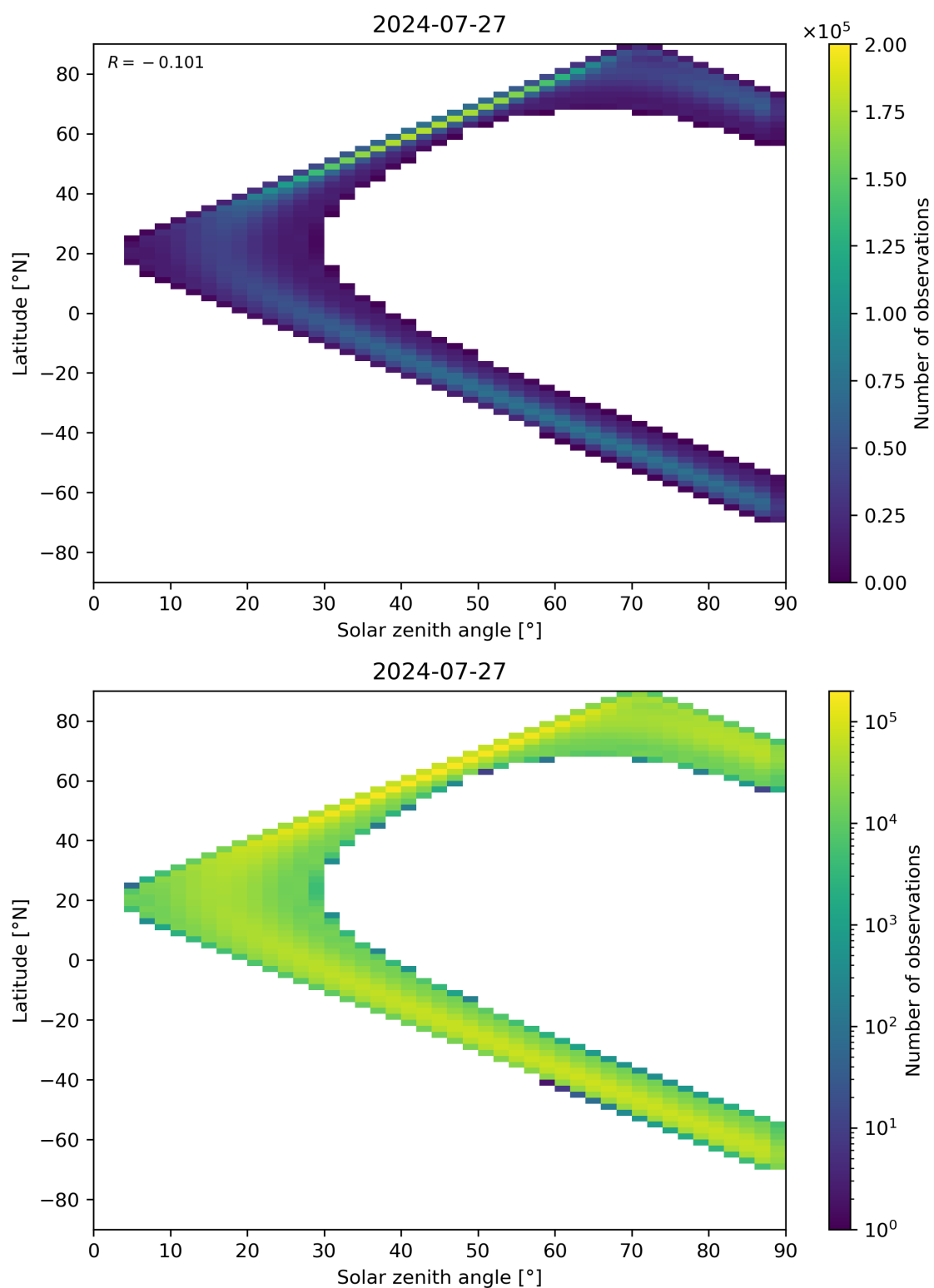
Figure 44: Scatter density plot of “Solar zenith angle” against “Latitude” for 2024-07-26 to 2024-07-28.
