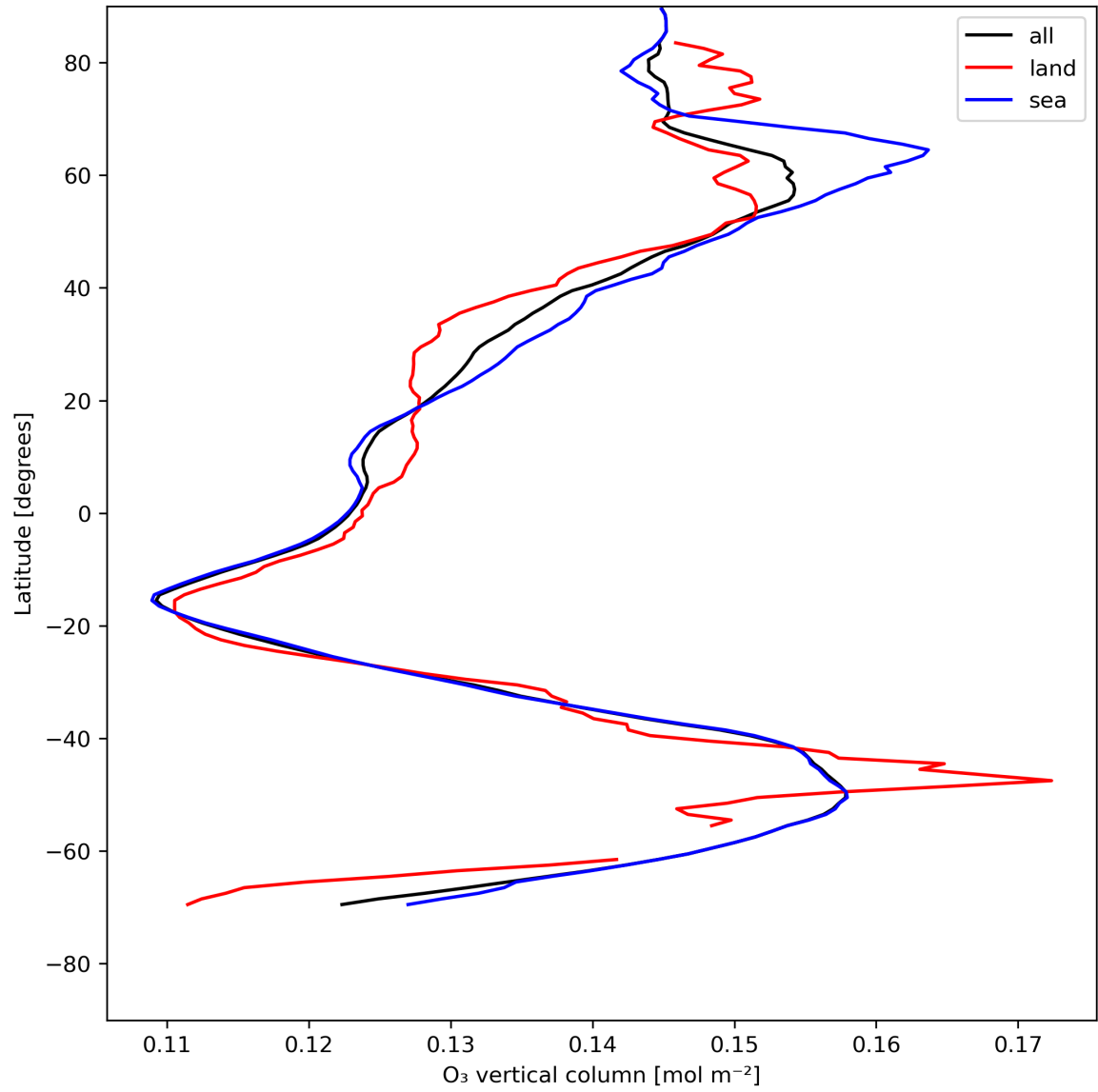
Figure 14: Zonal average of “O 3 vertical column” for 2024-07-26 to 2024-07-28.
