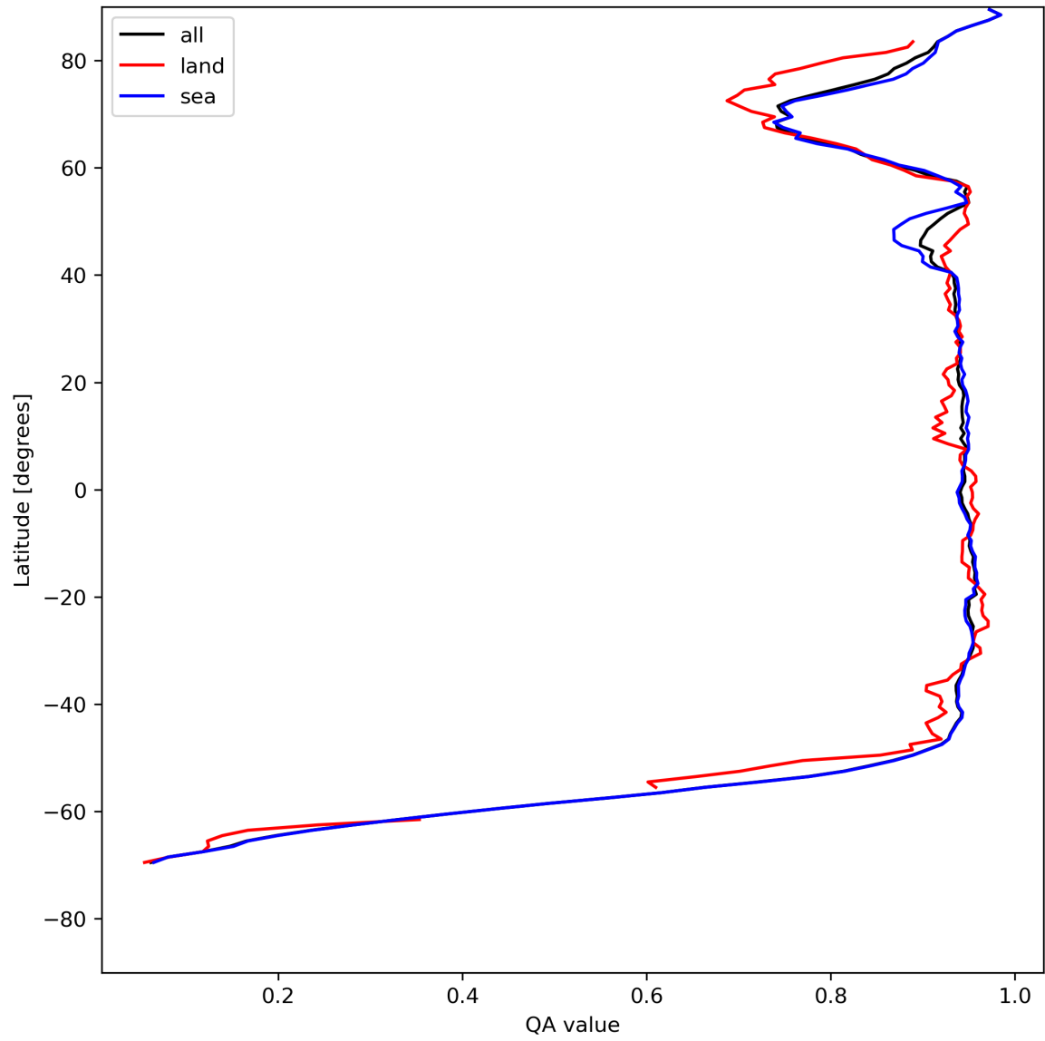
Figure 13: Zonal average of “QA value” for 2024-07-26 to 2024-07-28.
