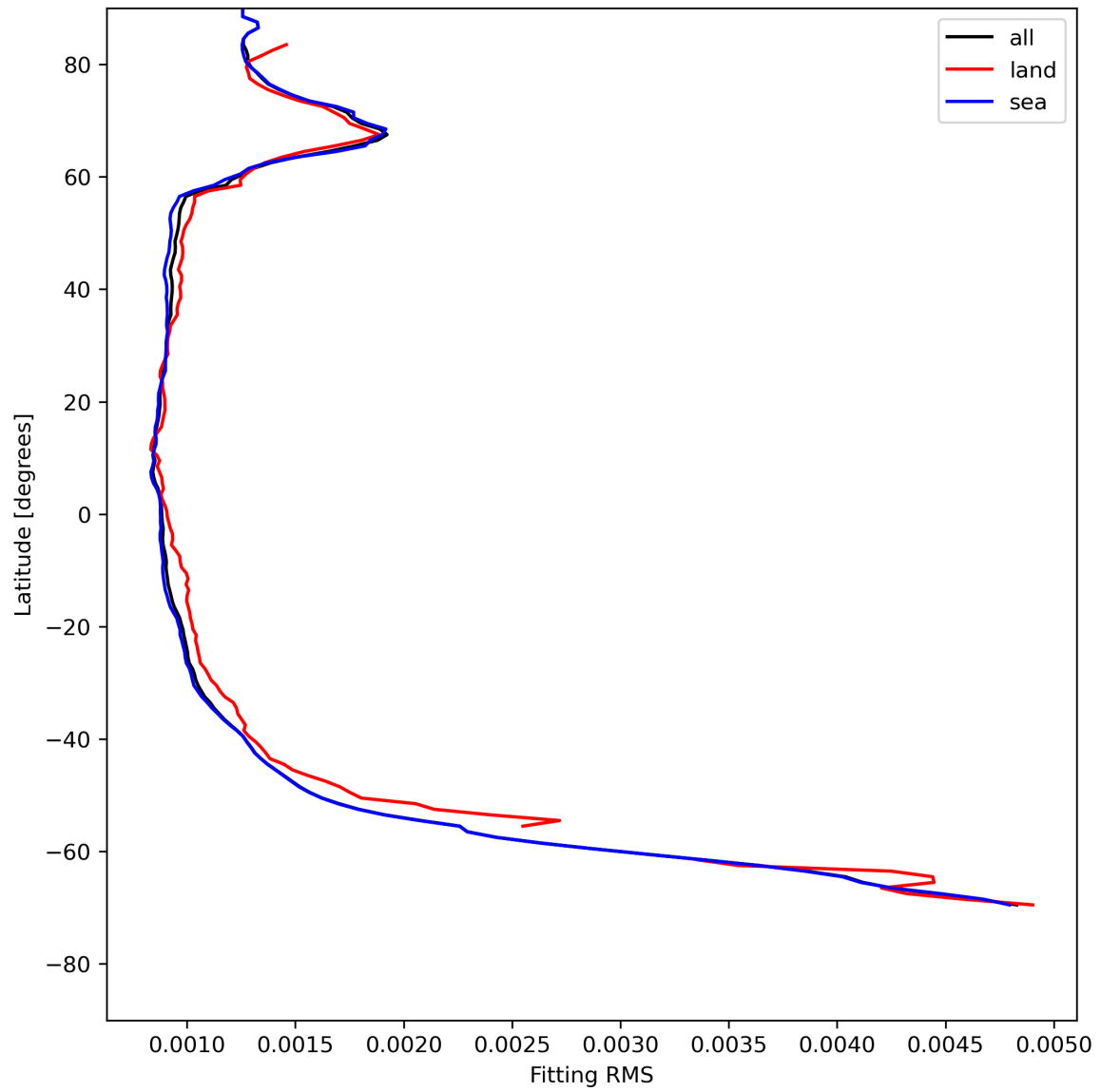
Figure 16: Zonal average of “Fitting RMS” for 2024-07-26 to 2024-07-28.
