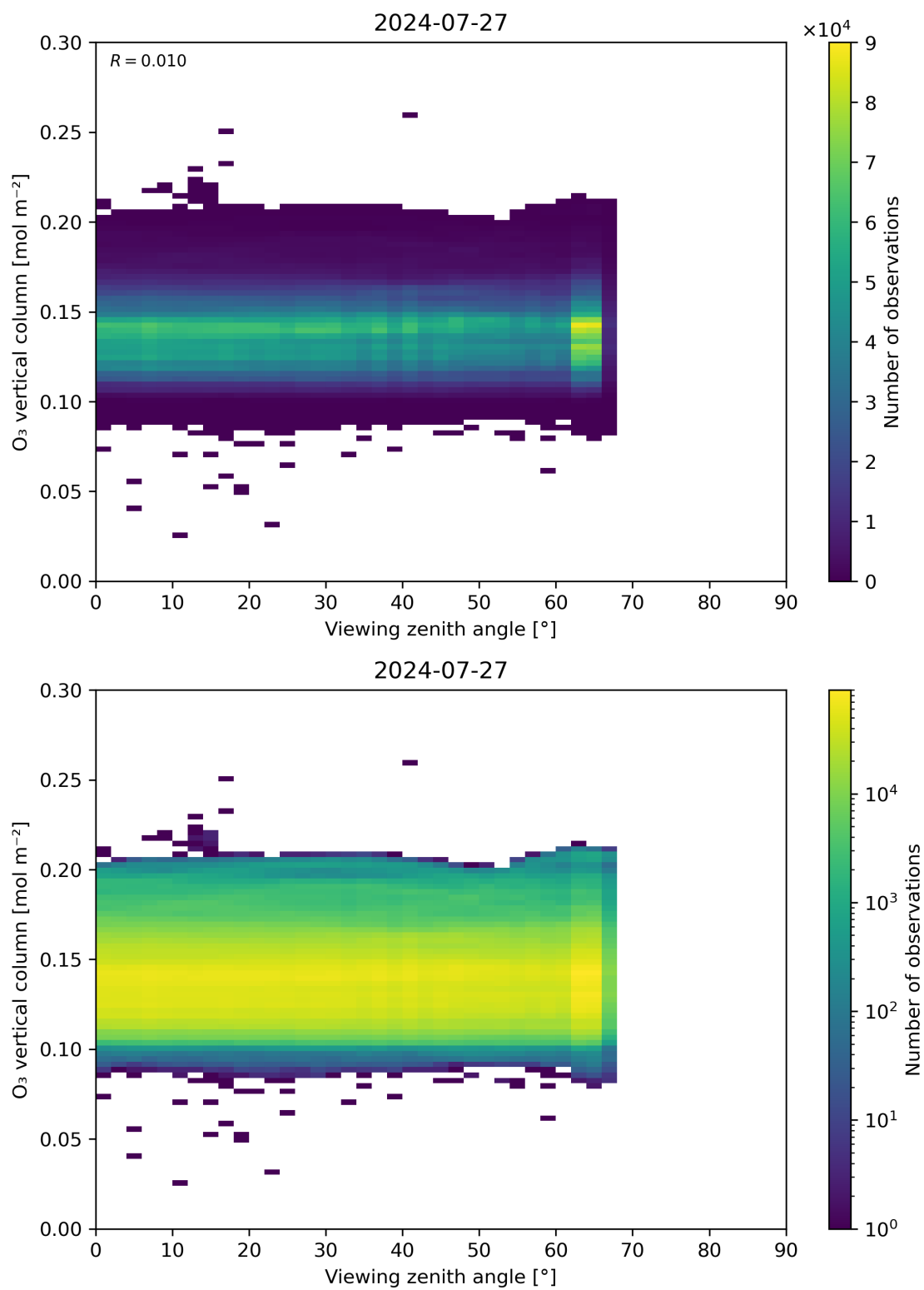
Figure 52: Scatter density plot of “Viewing zenith angle” against “O 3 vertical column” for 2024-07-26 to 2024-07-28.
