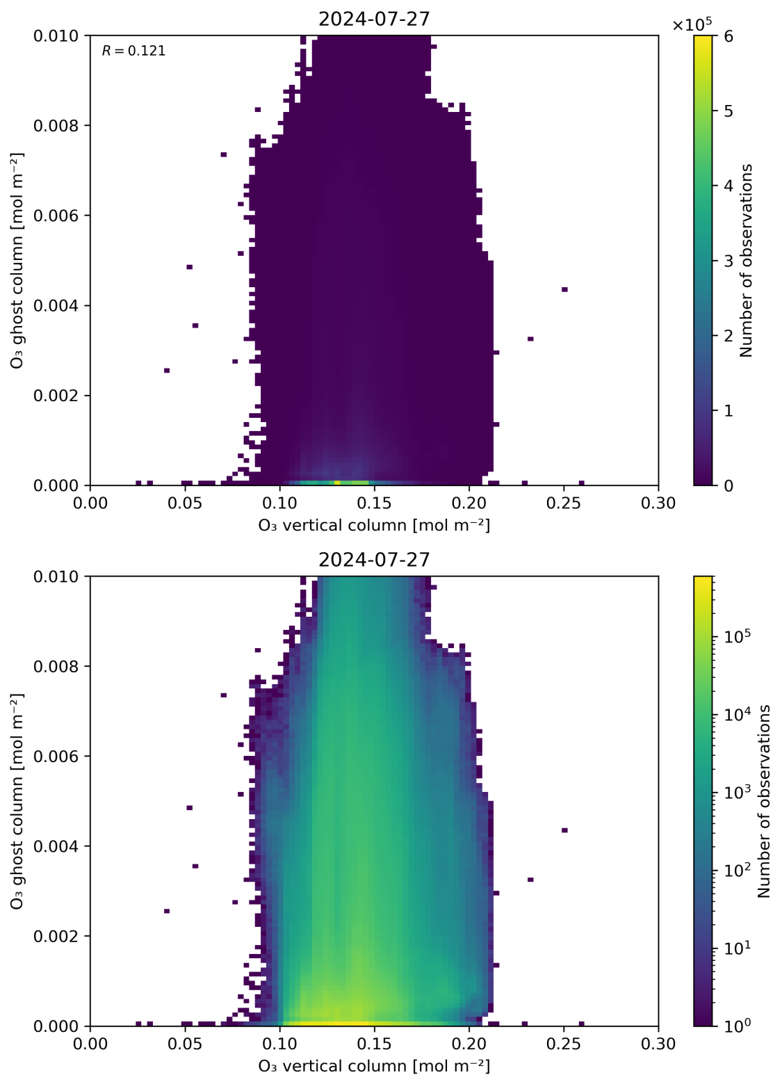
Figure 40: Scatter density plot of “O 3 vertical column” against “O 3 ghost column” for 2024-07-26 to 2024-07-28.
