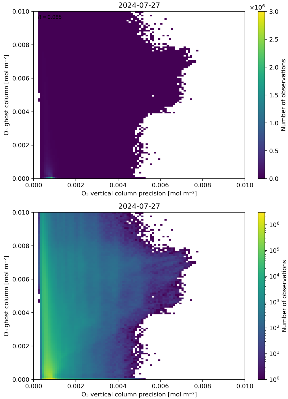
Figure 43: Scatter density plot of “ \text{O}_3 vertical column precision” against “ \text{O}_3 ghost column” for 2024-07-26 to 2024-07-28.
