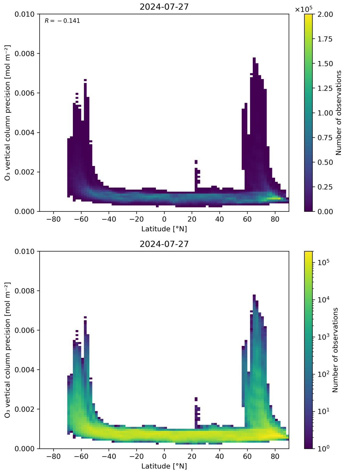
Figure 37: Scatter density plot of “Latitude” against “O 3 vertical column precision” for 2024-07-26 to 2024-07-28.
