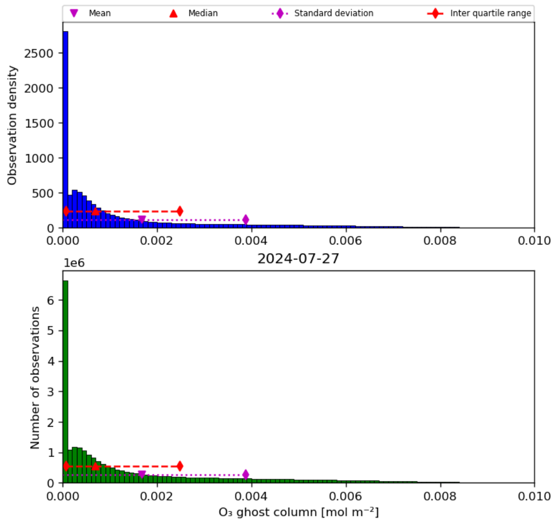
Figure 25: Histogram of “O 3 ghost column” for 2024-07-26 to 2024-07-28
