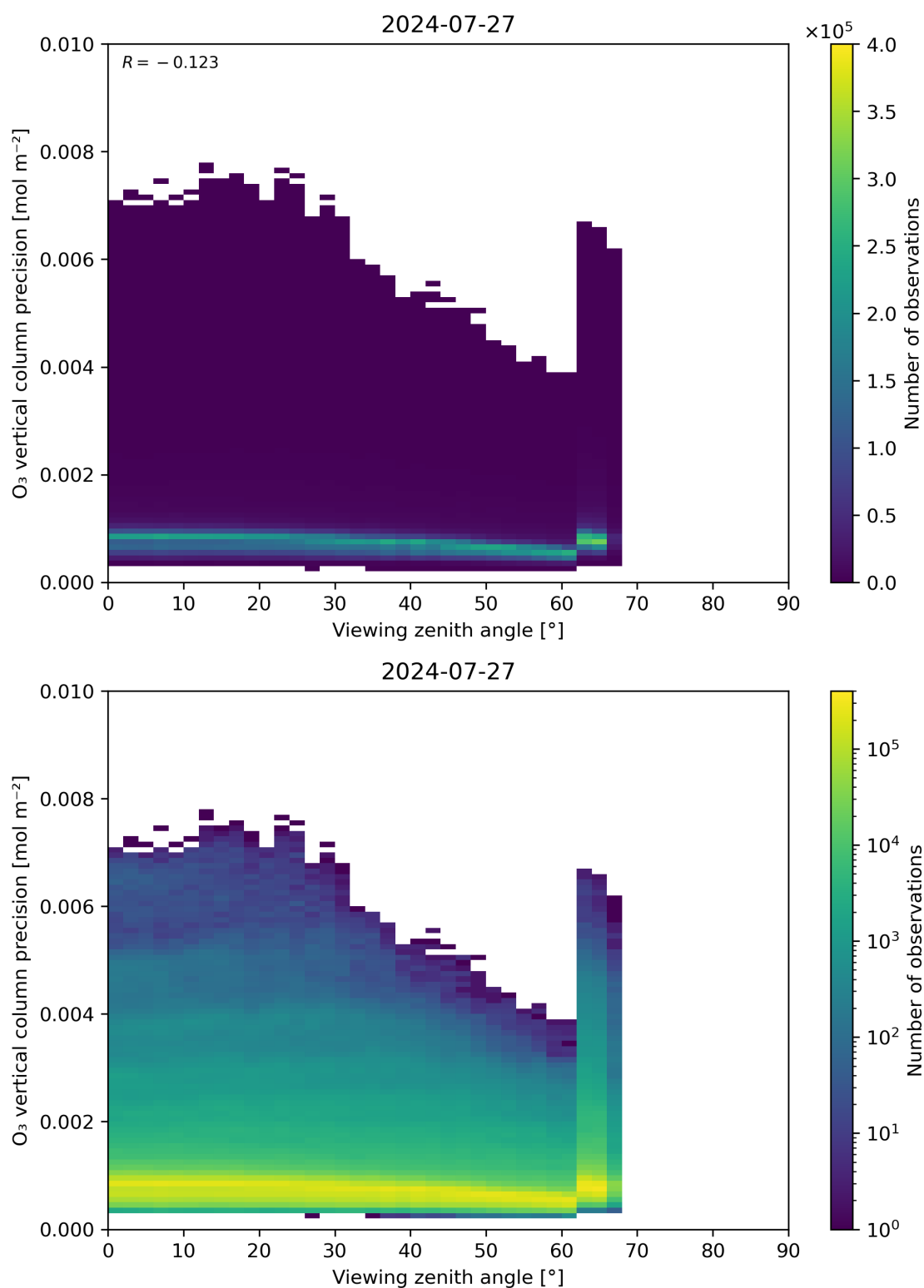
Figure 53: Scatter density plot of “Viewing zenith angle” against “O 3 vertical column precision” for 2024-07-26 to 2024-07-28.
