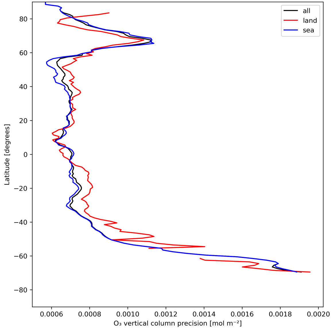
Figure 15: Zonal average of “O 3 vertical column precision” for 2024-07-26 to 2024-07-28.
