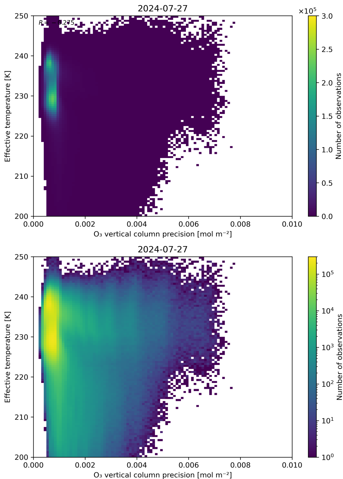
Figure 42: Scatter density plot of “O 3 vertical column precision” against “Effective temperature” for 2024-07-26 to 2024-07-28.
