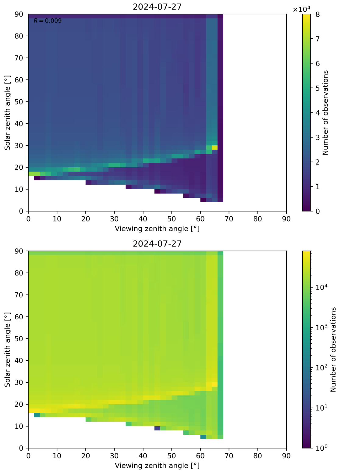
Figure 54: Scatter density plot of “Viewing zenith angle” against “Solar zenith angle” for 2024-07-26 to 2024-07-28.
