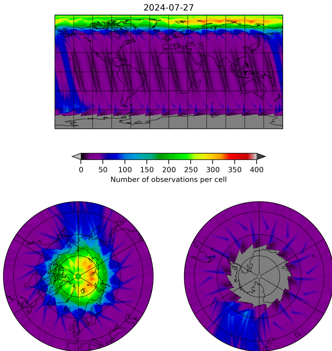
Figure 12: Map of the number of observations for 2024-07-26 to 2024-07-28
