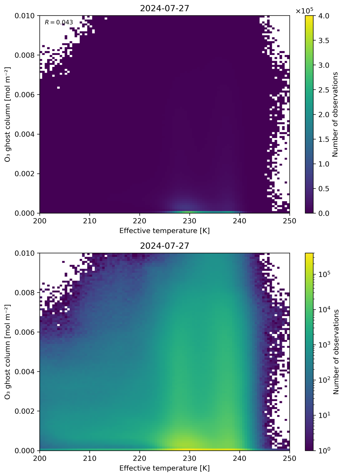
Figure 38: Scatter density plot of “Effective temperature” against “O 3 ghost column” for 2024-07-26 to 2024-07-28.
