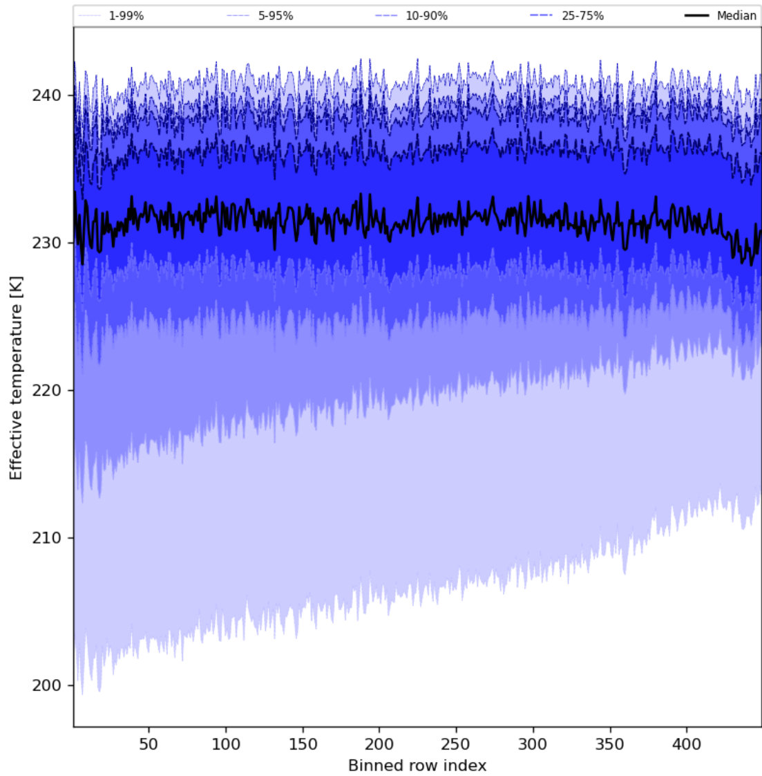
Figure 31: Along track statistics of “Effective temperature” for 2024-07-26 to 2024-07-28
