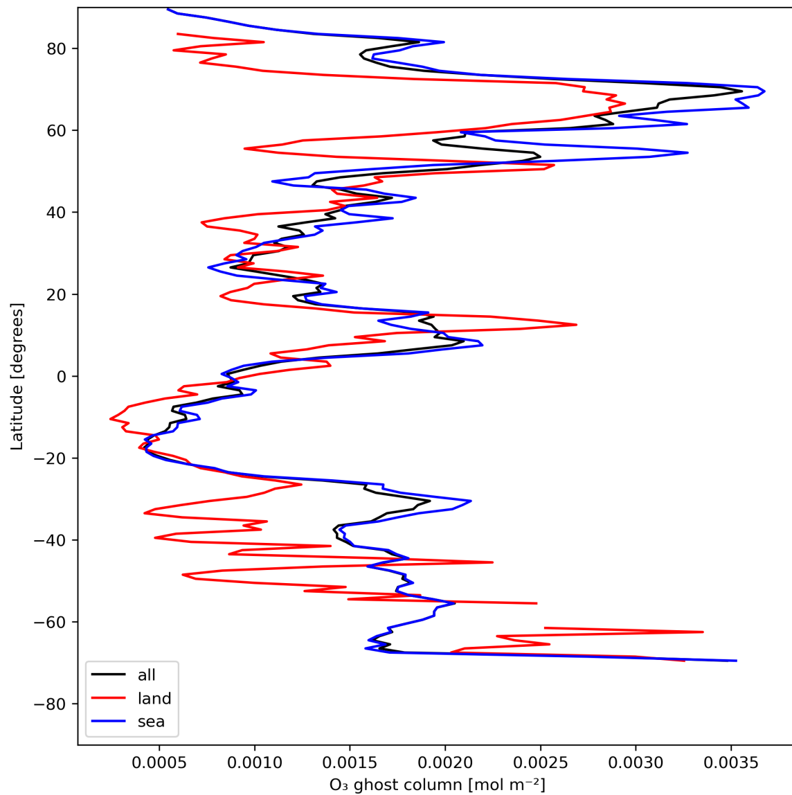
Figure 18: Zonal average of “O 3 ghost column” for 2024-07-26 to 2024-07-28.
