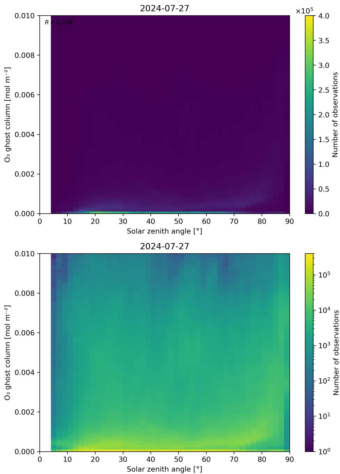
Figure 46: Scatter density plot of “Solar zenith angle” against “O 3 ghost column” for 2024-07-26 to 2024-07-28.
