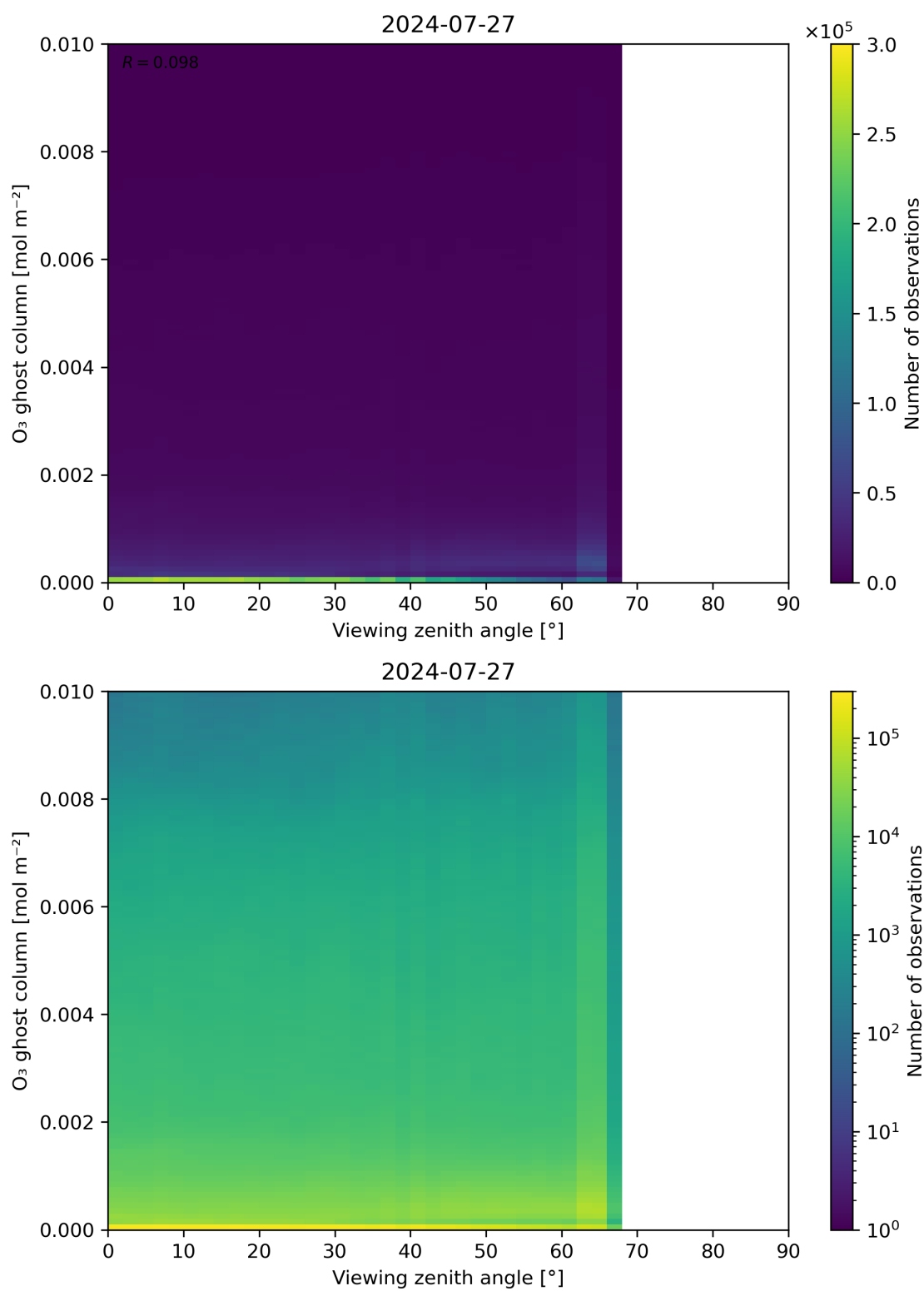
Figure 51: Scatter density plot of “Viewing zenith angle” against “O 3 ghost column” for 2024-07-26 to 2024-07-28.
