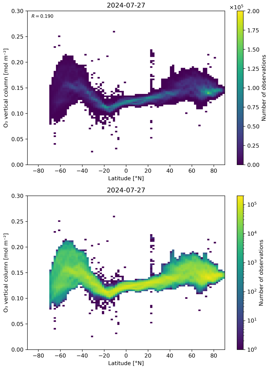
Figure 36: Scatter density plot of “Latitude” against “O 3 vertical column” for 2024-07-26 to 2024-07-28.
