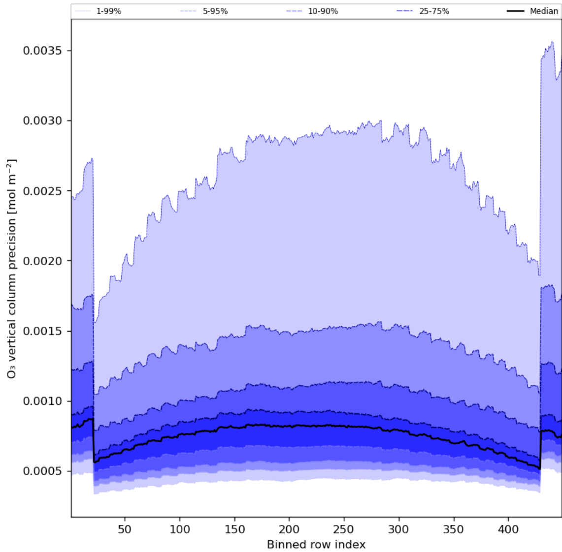
Figure 29: Along track statistics of “O 3 vertical column precision” for 2024-07-26 to 2024-07-28
