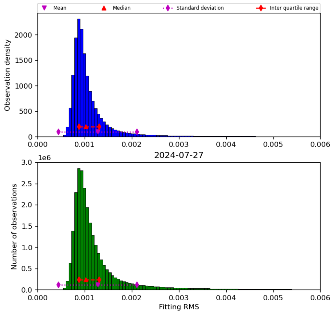
Figure 23: Histogram of “Fitting RMS” for 2024-07-26 to 2024-07-28
