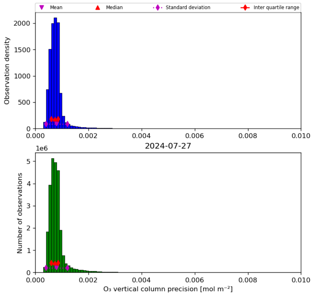
Figure 22: Histogram of “O 3 vertical column precision” for 2024-07-26 to 2024-07-28
