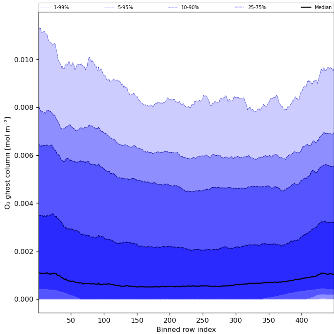
Figure 32: Along track statistics of “O 3 ghost column” for 2024-07-26 to 2024-07-28
