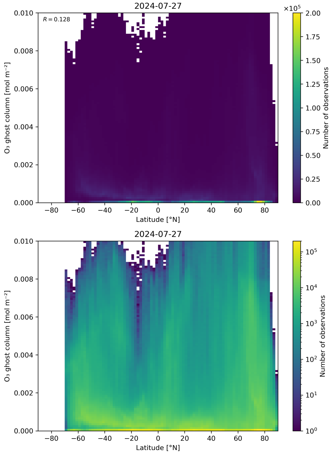
Figure 35: Scatter density plot of “Latitude” against “O 3 ghost column” for 2024-07-26 to 2024-07-28.
