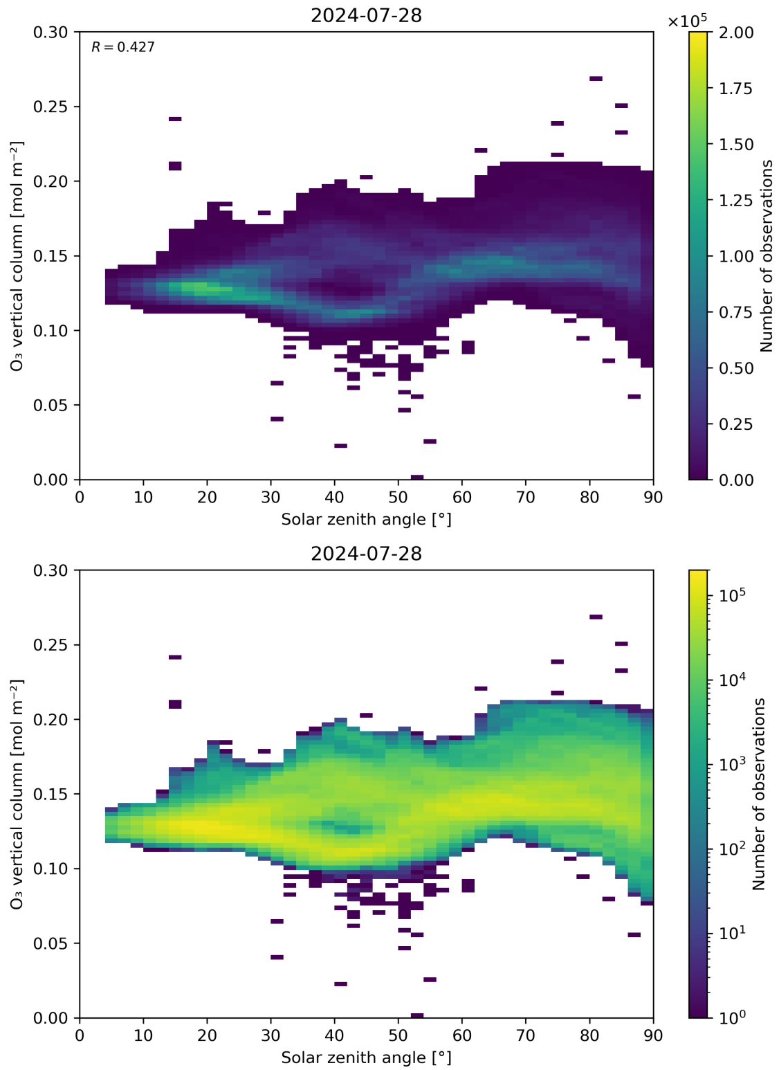
Figure 47: Scatter density plot of “Solar zenith angle” against “O 3 vertical column” for 2024-07-27 to 2024-07-29.
