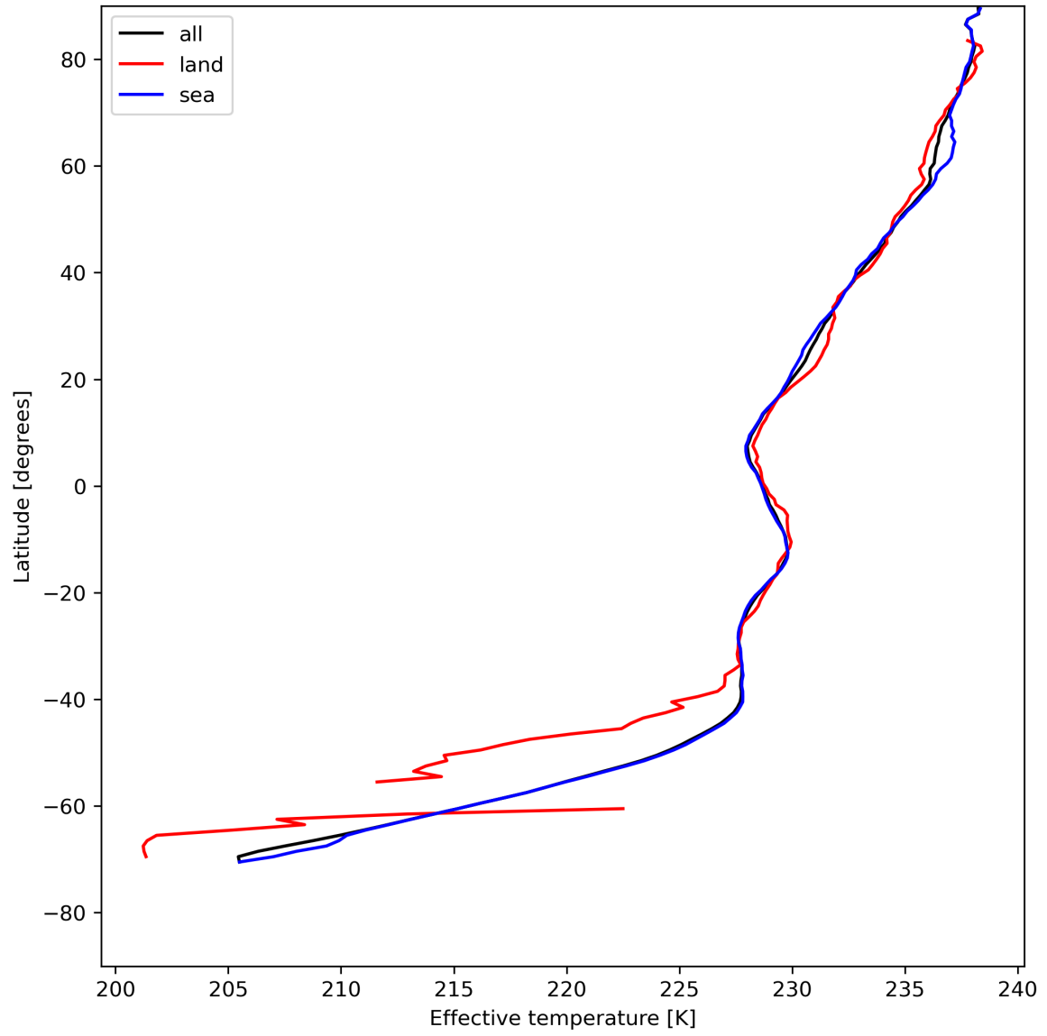
Figure 17: Zonal average of "Effective temperature" for 2024-07-27 to 2024-07-29.
