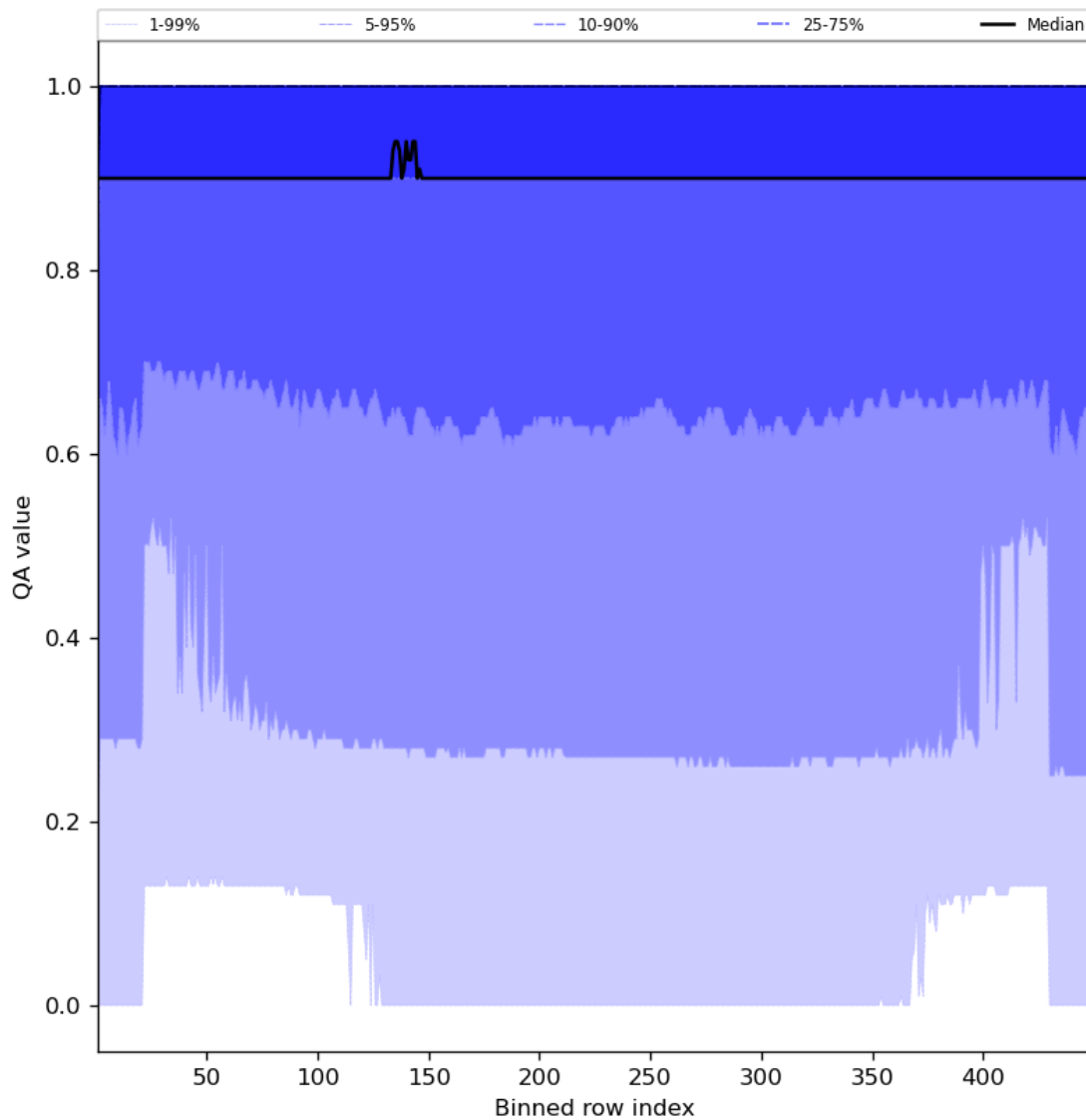
Figure 27: Along track statistics of “QA value” for 2024-07-27 to 2024-07-29
