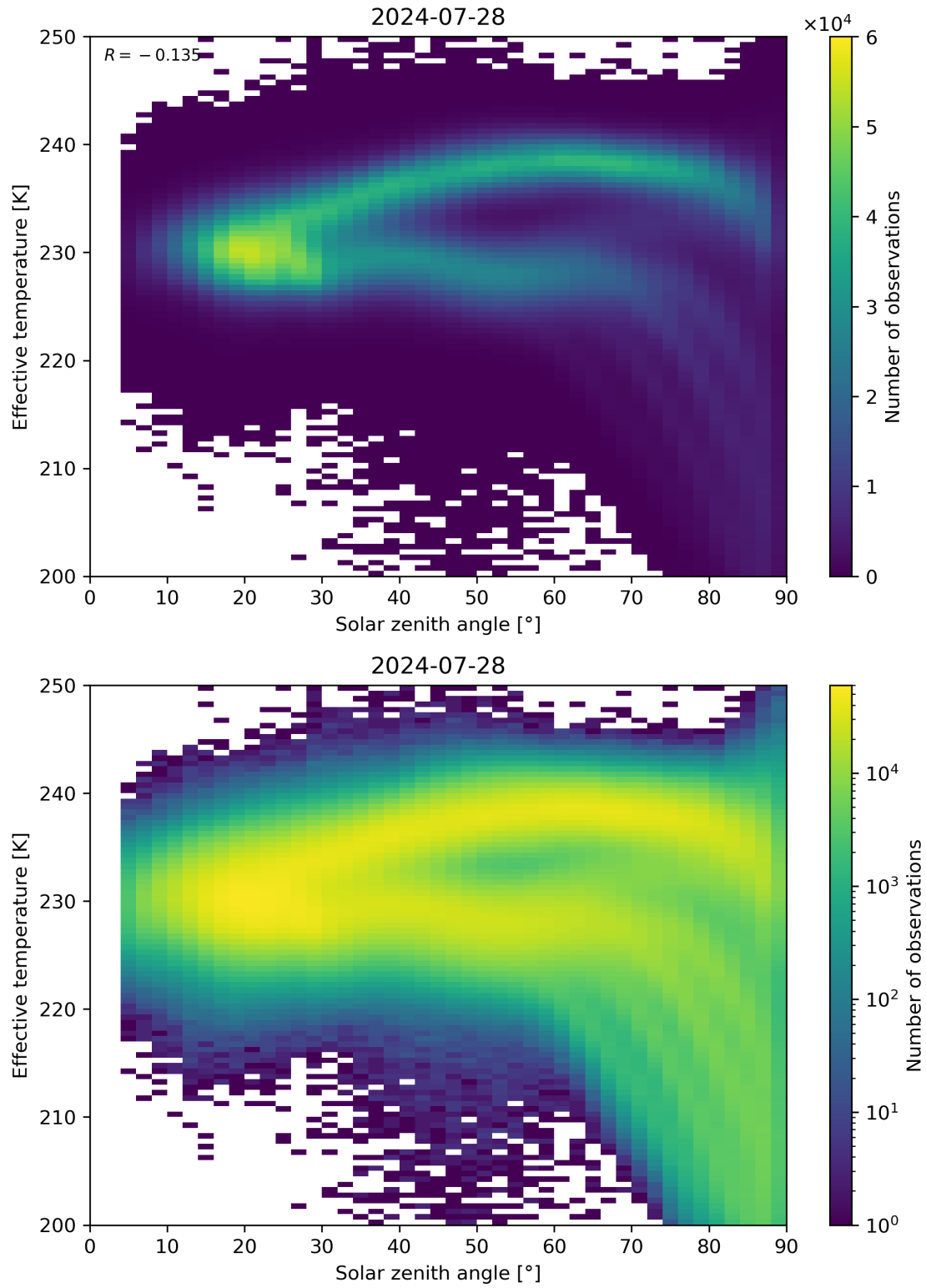
Figure 45: Scatter density plot of “Solar zenith angle” against “Effective temperature” for 2024-07-27 to 2024-07-29.
