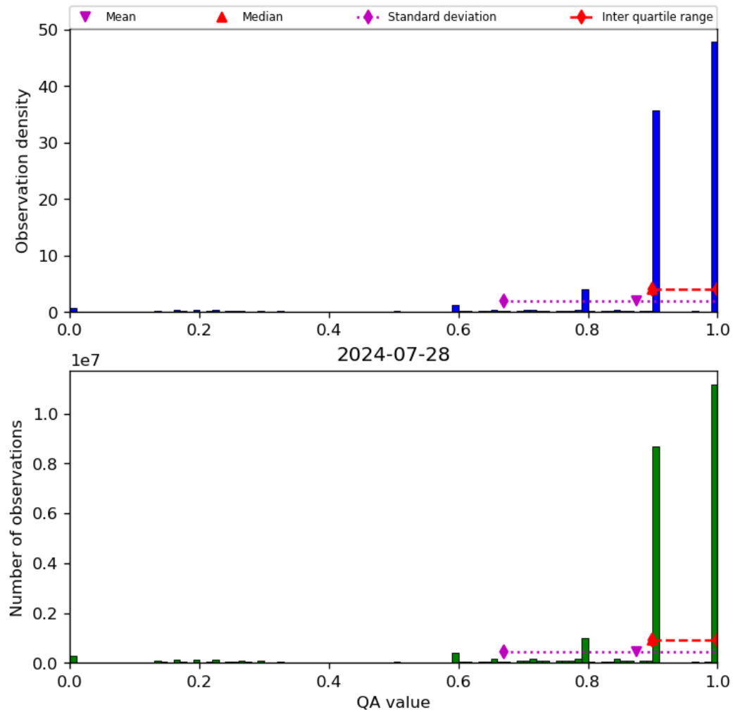
Figure 20: Histogram of “QA value” for 2024-07-27 to 2024-07-29
