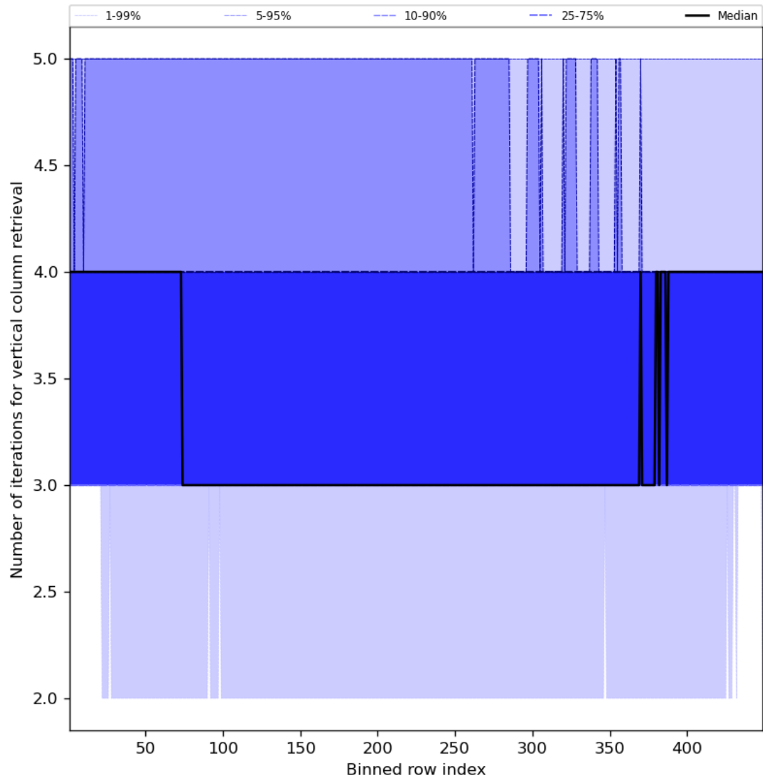
Figure 33: Along track statistics of “Number of iterations for vertical column retrieval” for 2024-07-27 to 2024-07-29
