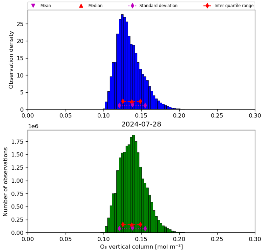
Figure 21: Histogram of “O 3 vertical column” for 2024-07-27 to 2024-07-29
