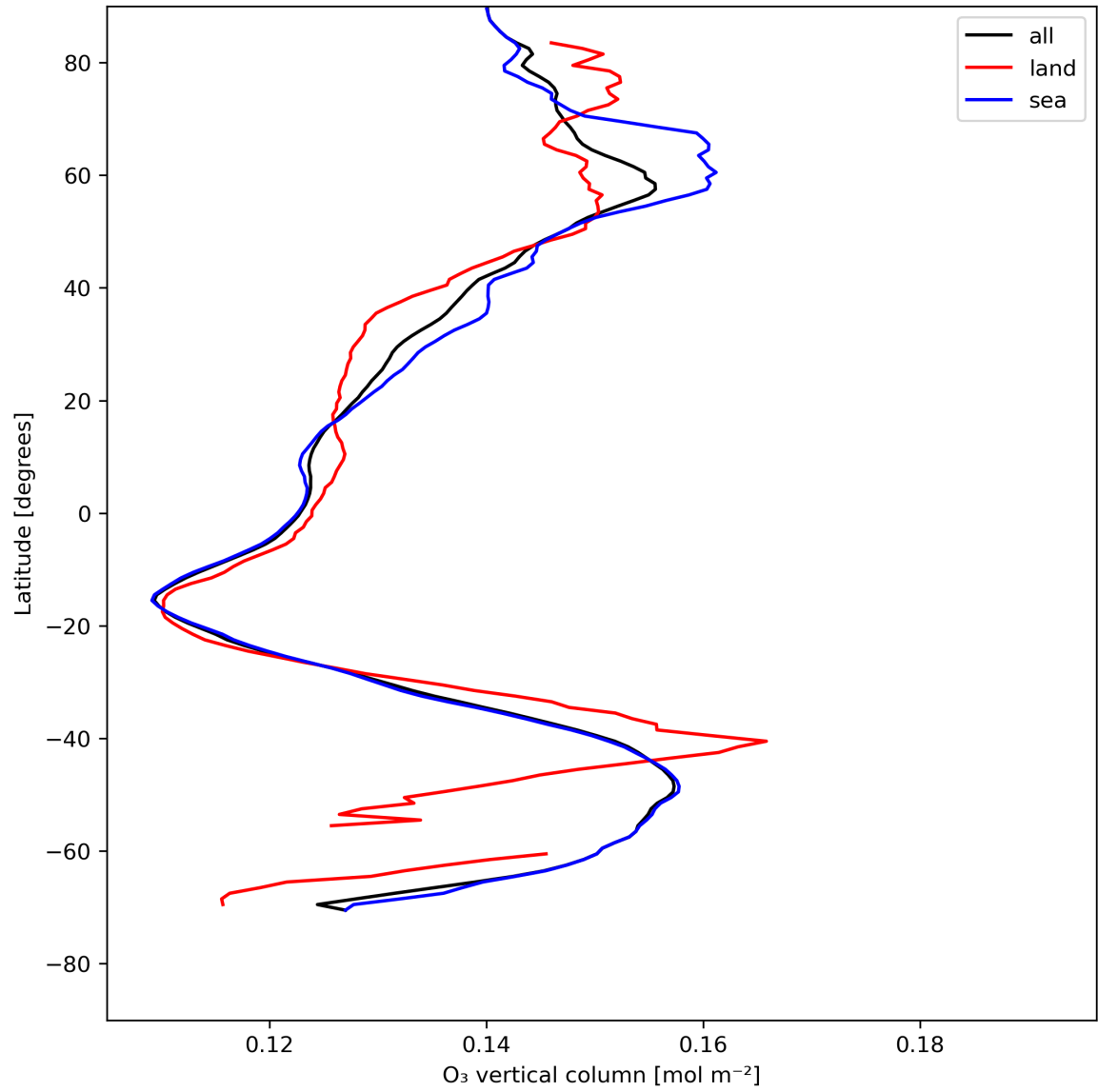
Figure 14: Zonal average of “O 3 vertical column” for 2024-07-27 to 2024-07-29.
