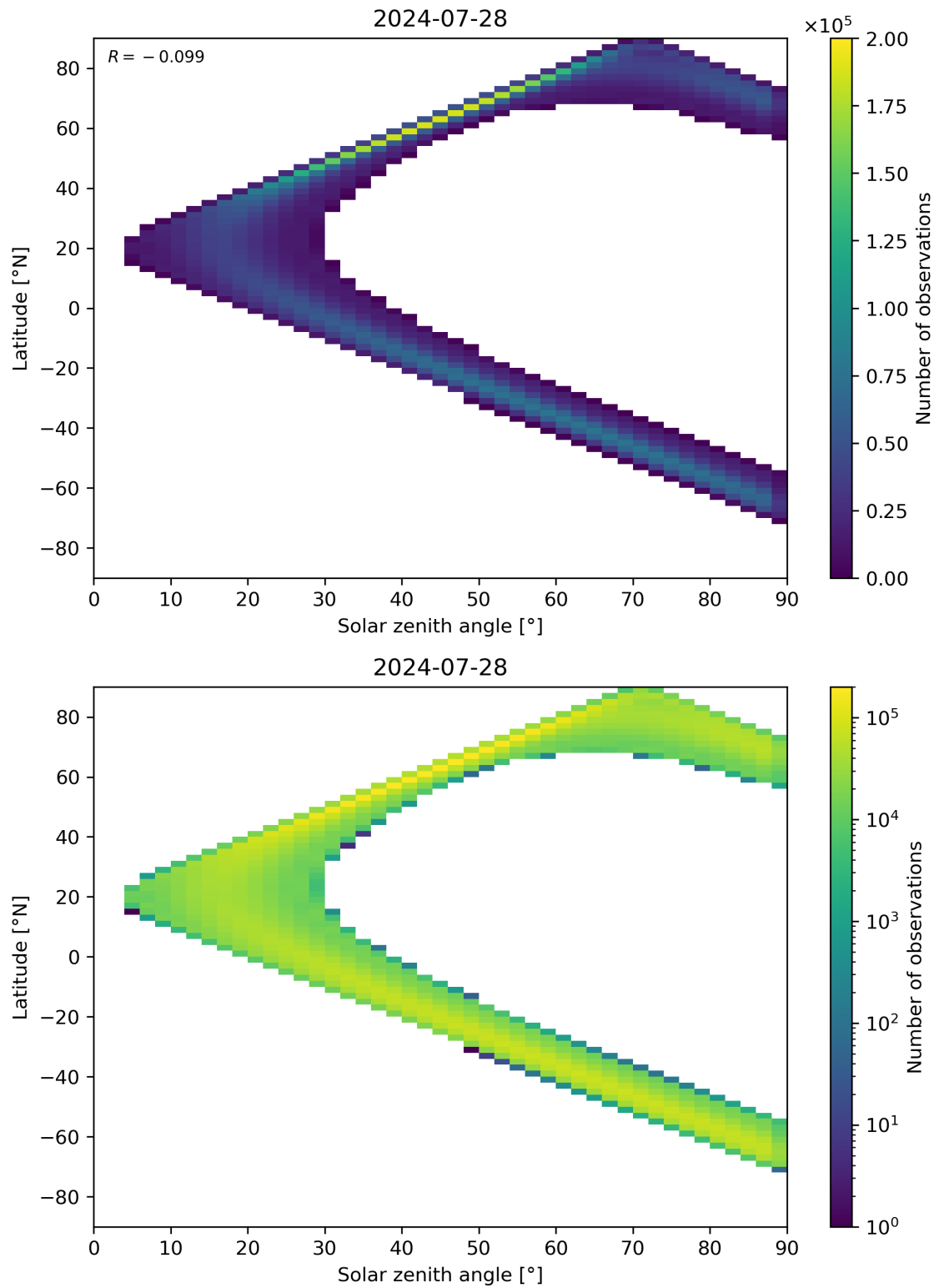
Figure 44: Scatter density plot of “Solar zenith angle” against “Latitude” for 2024-07-27 to 2024-07-29.
