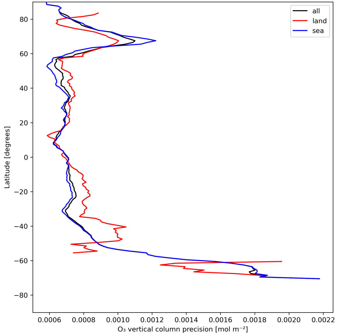
Figure 15: Zonal average of "O 3 vertical column precision" for 2024-07-27 to 2024-07-29.
