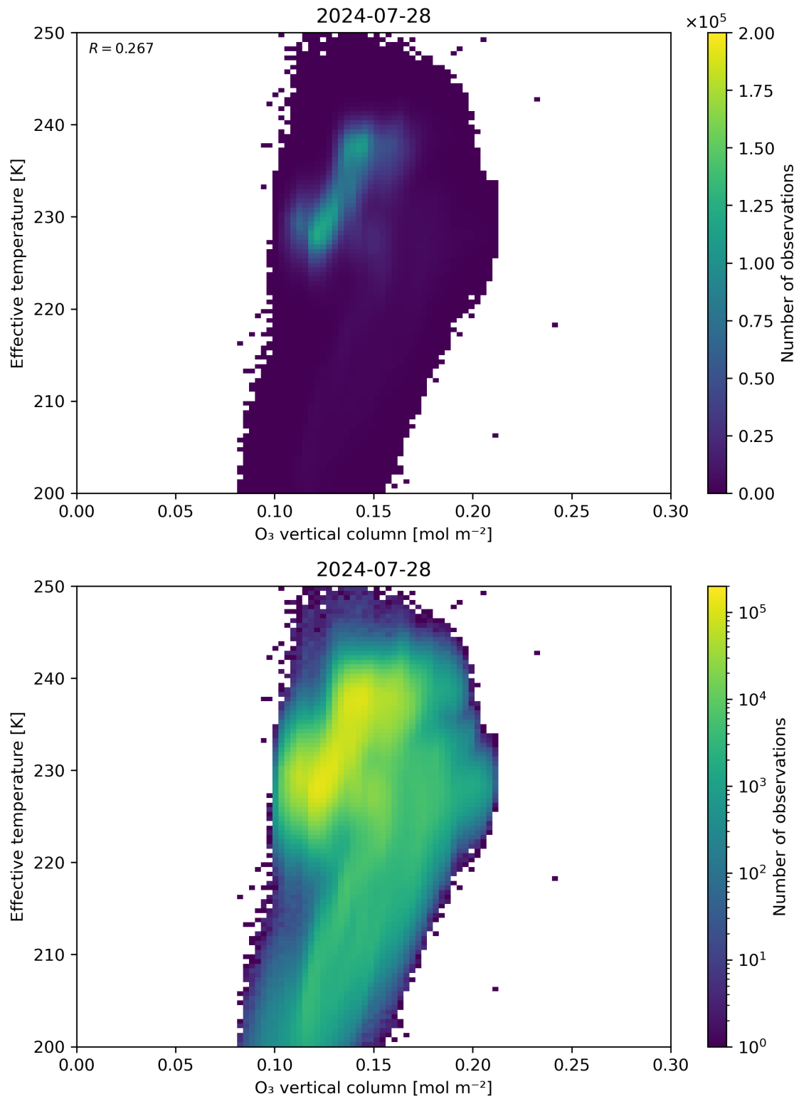
Figure 39: Scatter density plot of “O 3 vertical column” against “Effective temperature” for 2024-07-27 to 2024-07-29.
