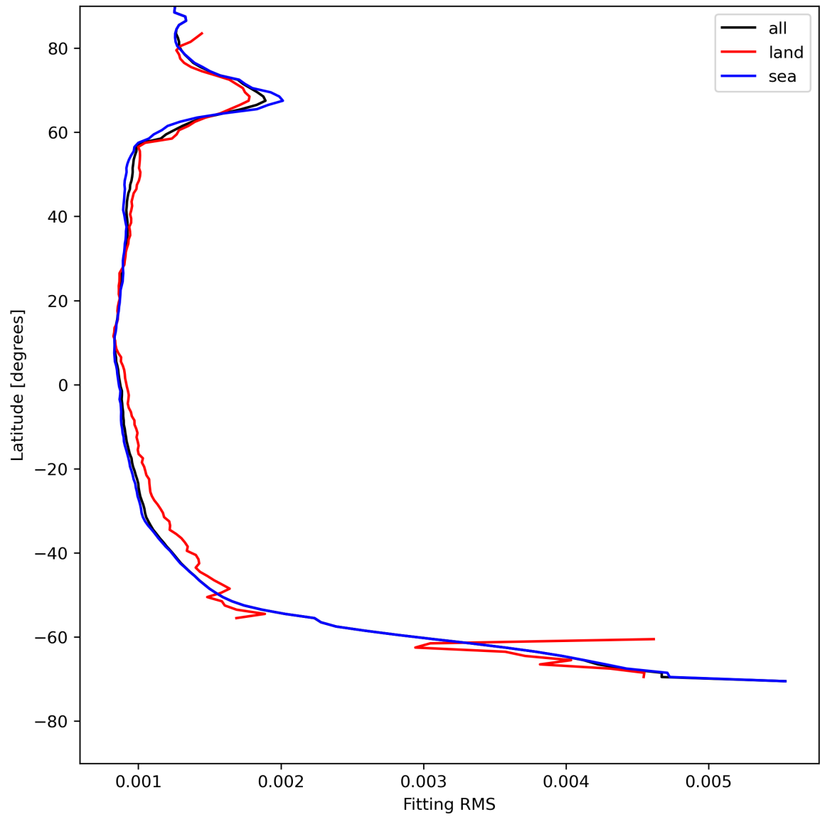
Figure 16: Zonal average of “Fitting RMS” for 2024-07-27 to 2024-07-29.
