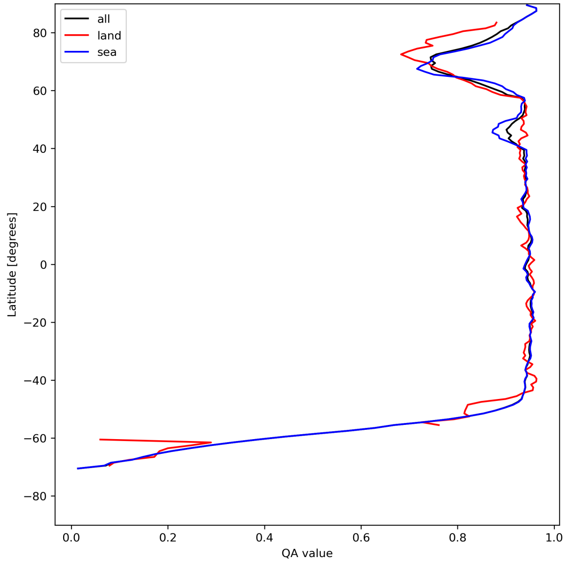
Figure 13: Zonal average of “QA value” for 2024-07-27 to 2024-07-29.
