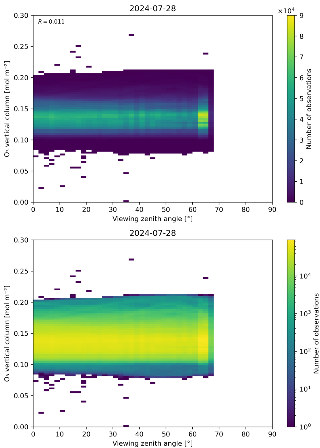
Figure 52: Scatter density plot of “Viewing zenith angle” against “O 3 vertical column” for 2024-07-27 to 2024-07-29.
