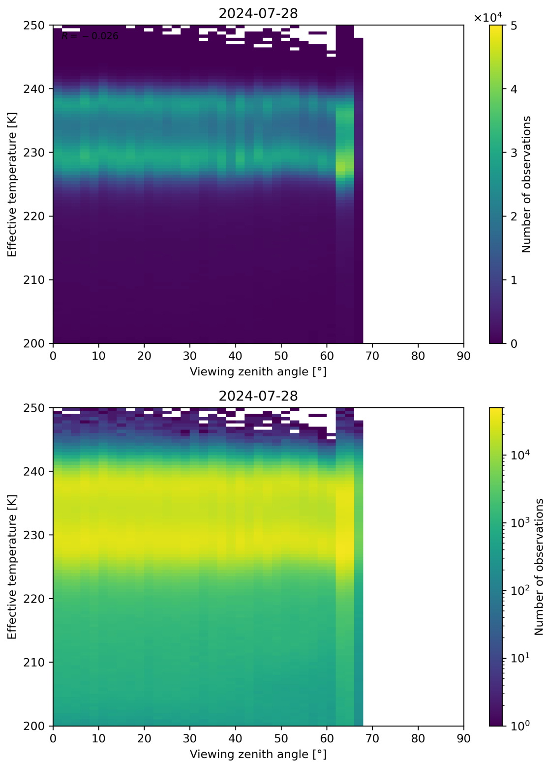
Figure 50: Scatter density plot of “Viewing zenith angle” against “Effective temperature” for 2024-07-27 to 2024-07-29.
