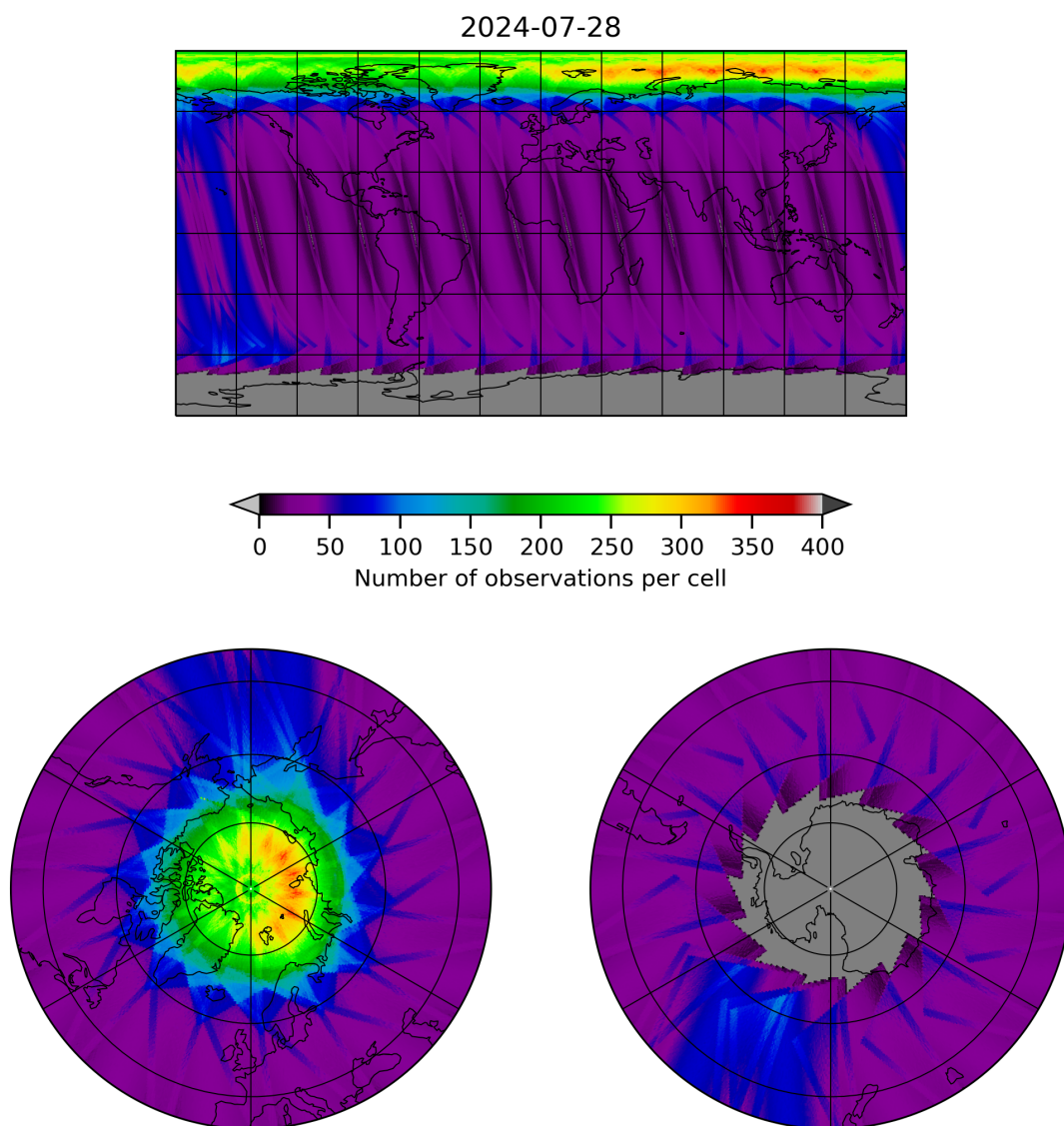
Figure 12: Map of the number of observations for 2024-07-27 to 2024-07-29
