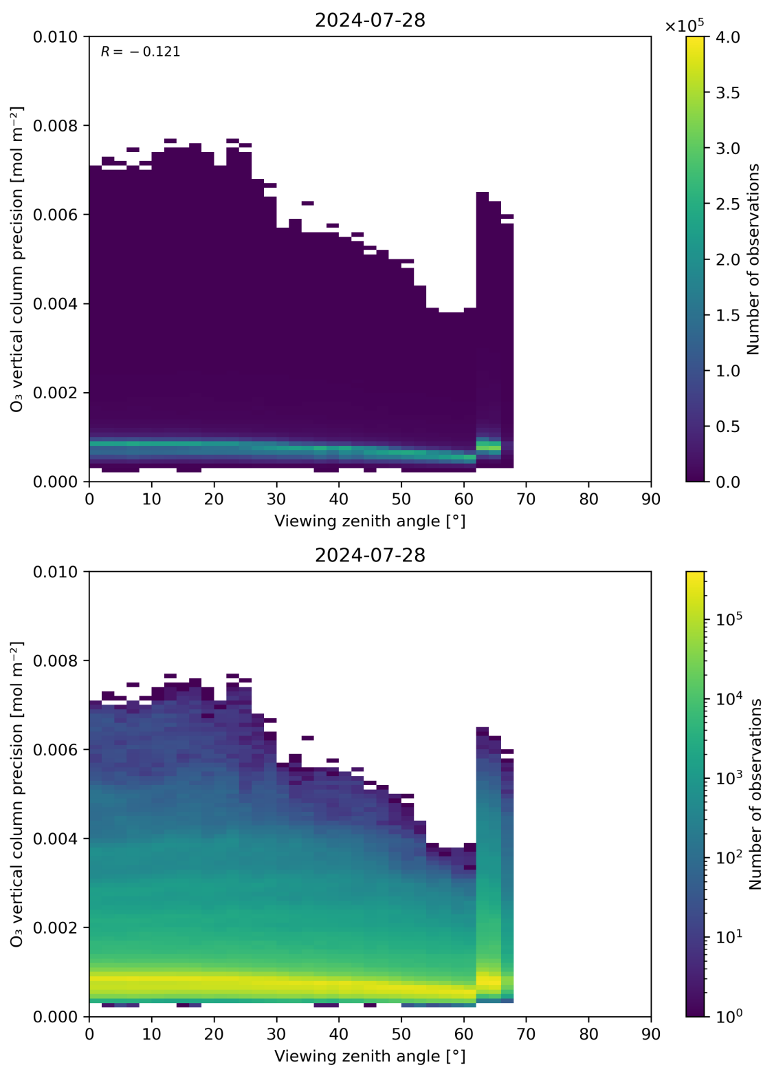
Figure 53: Scatter density plot of “Viewing zenith angle” against “O 3 vertical column precision” for 2024-07-27 to 2024-07-29.
