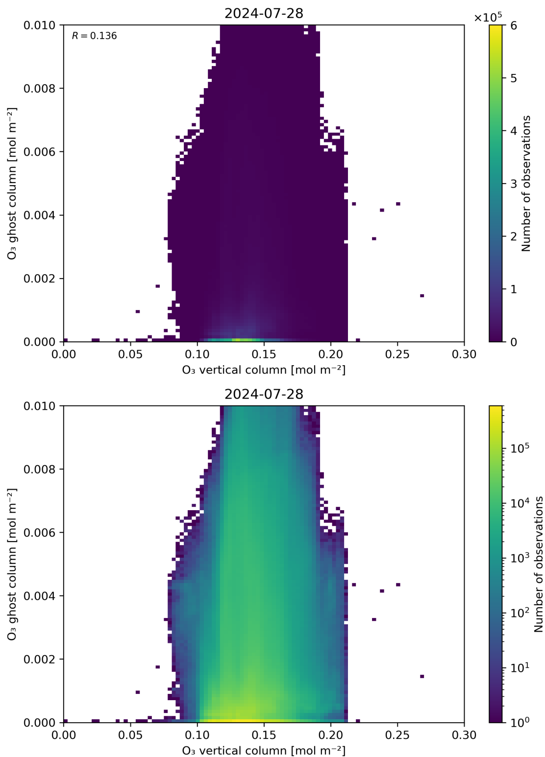
Figure 40: Scatter density plot of “O 3 vertical column” against “O 3 ghost column” for 2024-07-27 to 2024-07-29.
