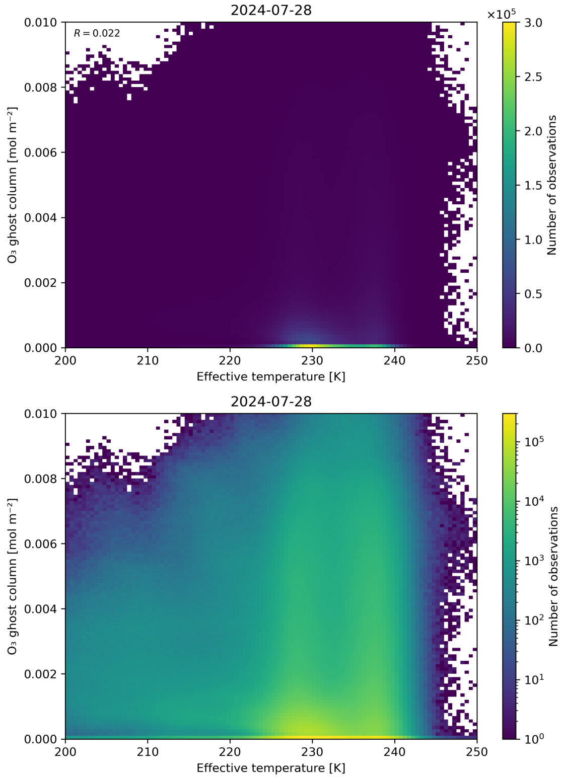
Figure 38: Scatter density plot of “Effective temperature” against “O 3 ghost column” for 2024-07-27 to 2024-07-29.
