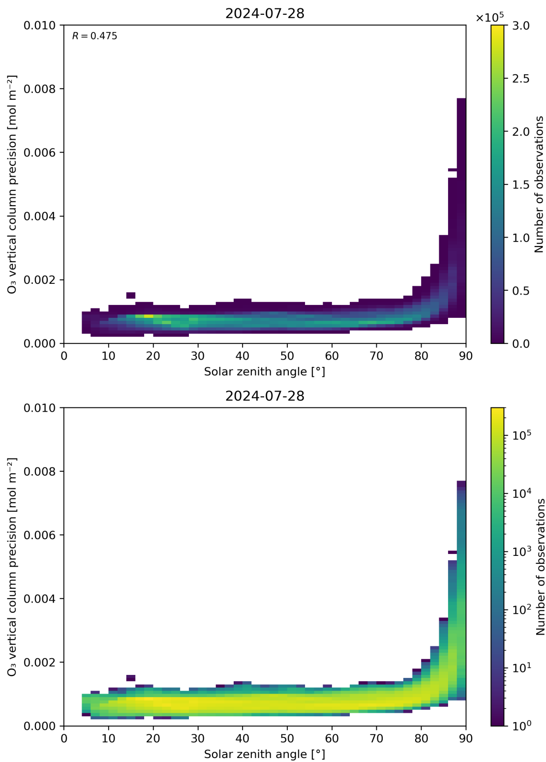
Figure 48: Scatter density plot of “Solar zenith angle” against “O 3 vertical column precision” for 2024-07-27 to 2024-07-29.
