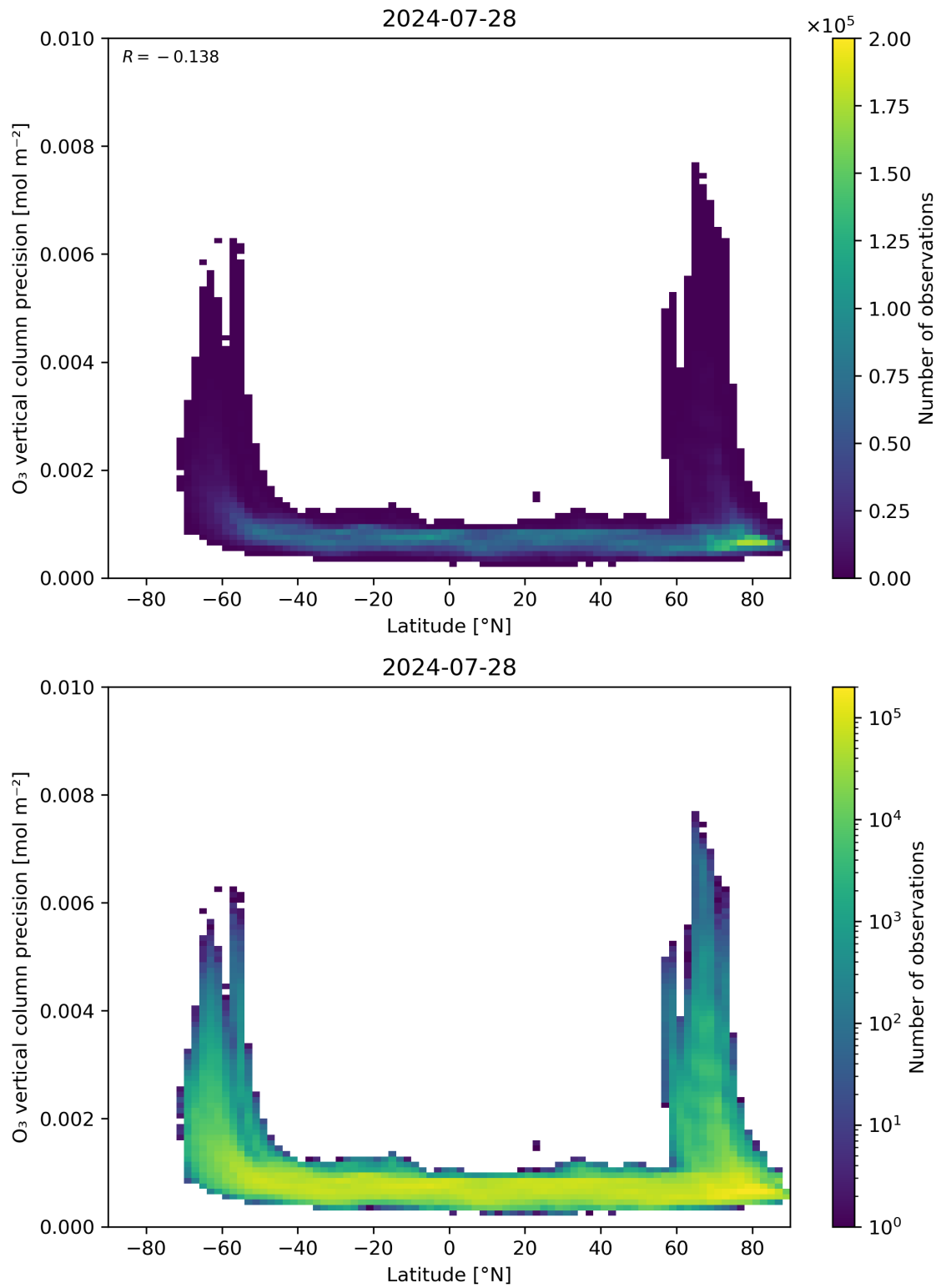
Figure 37: Scatter density plot of “Latitude” against “O 3 vertical column precision” for 2024-07-27 to 2024-07-29.
