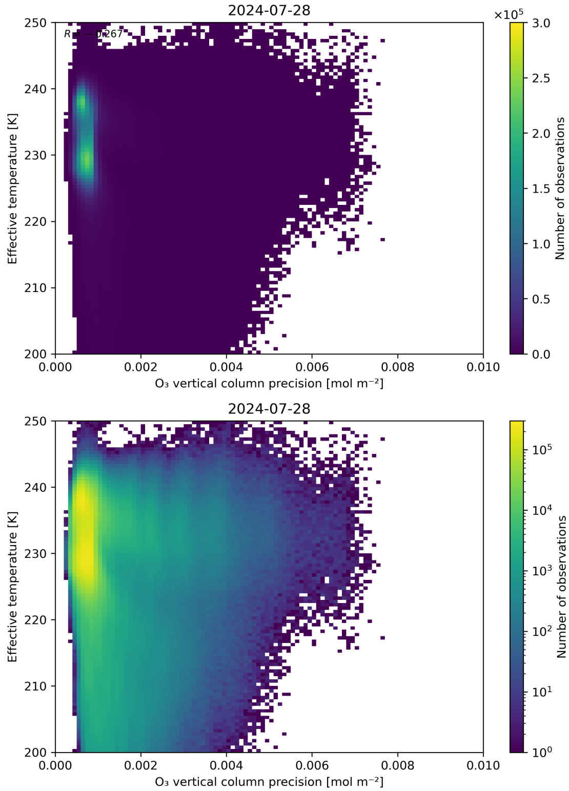
Figure 42: Scatter density plot of “O 3 vertical column precision” against “Effective temperature” for 2024-07-27 to 2024-07-29.
