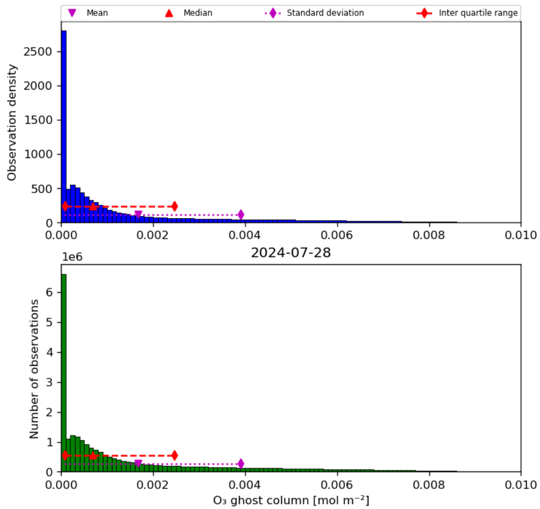
Figure 25: Histogram of “O 3 ghost column” for 2024-07-27 to 2024-07-29
