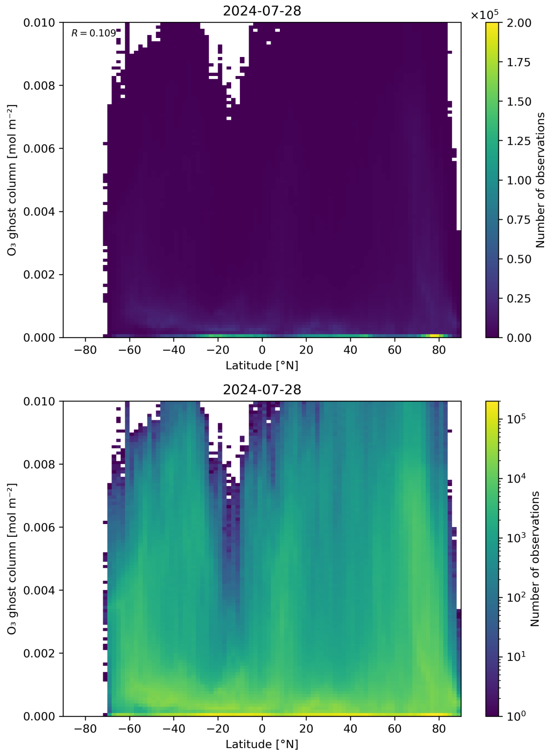
Figure 35: Scatter density plot of “Latitude” against “O 3 ghost column” for 2024-07-27 to 2024-07-29.
