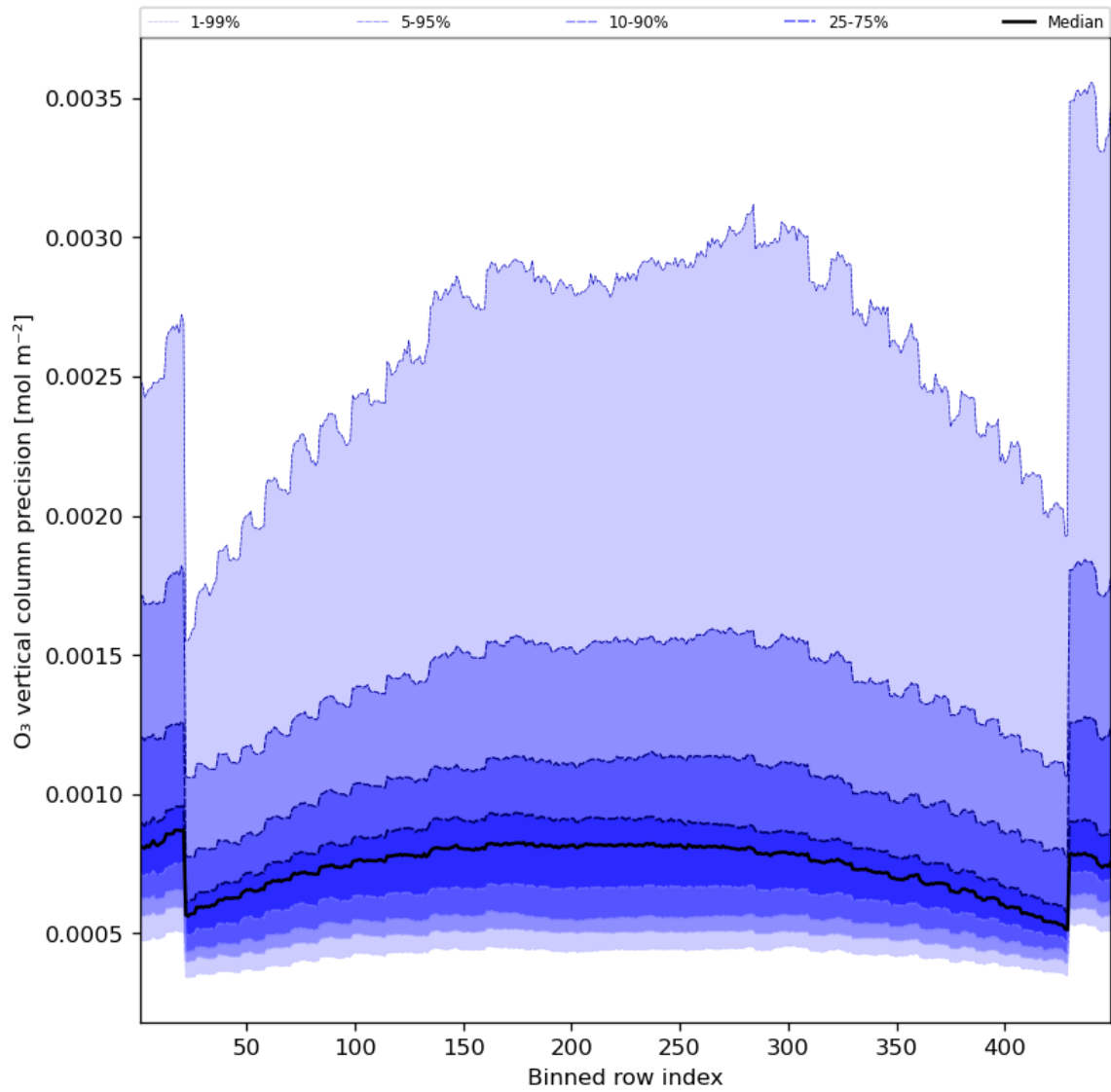
Figure 29: Along track statistics of “O 3 vertical column precision” for 2024-07-27 to 2024-07-29
