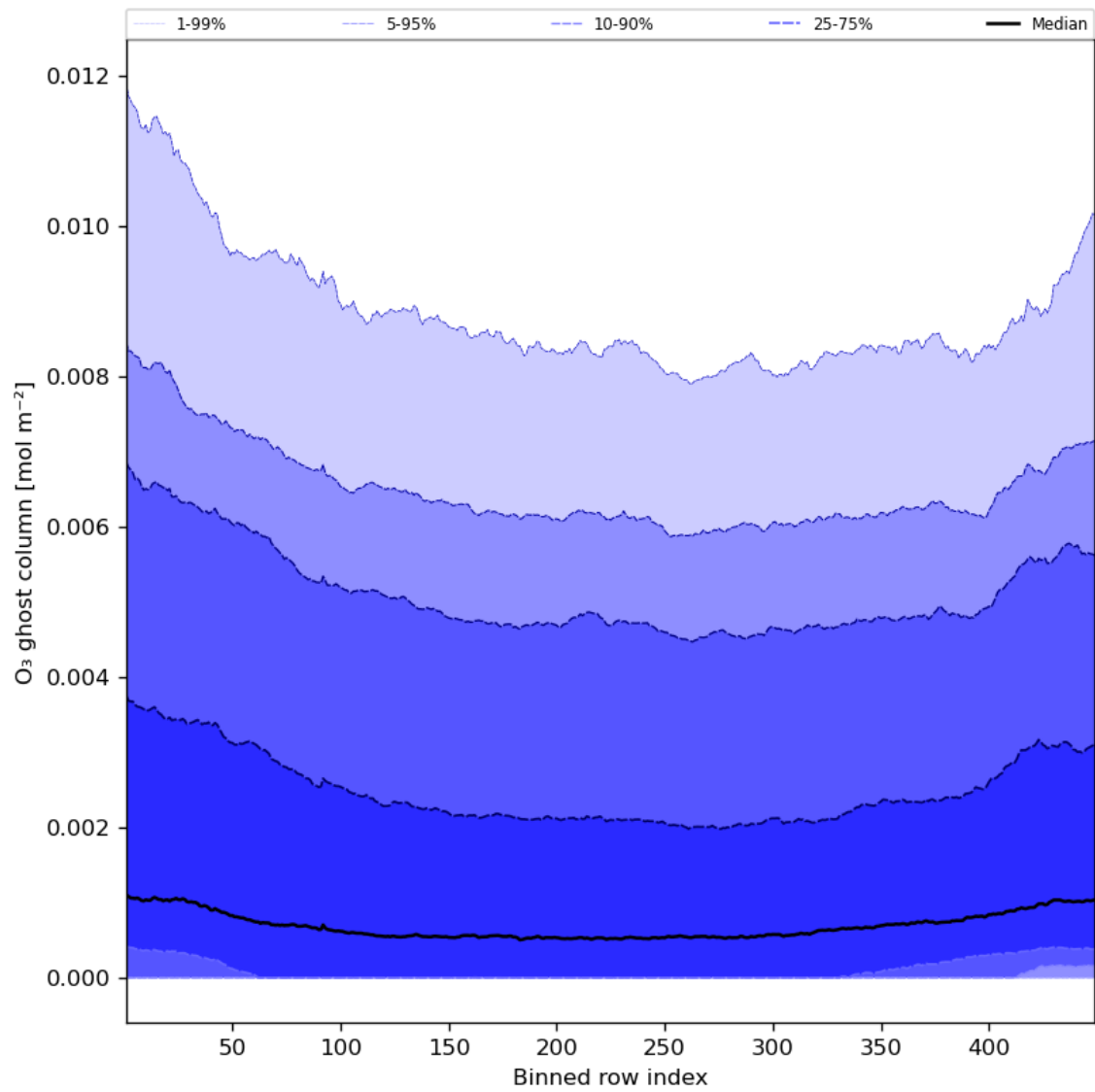
Figure 32: Along track statistics of “O 3 ghost column” for 2024-07-27 to 2024-07-29
