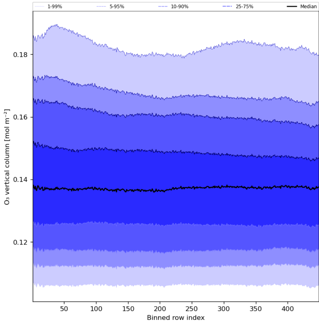
Figure 28: Along track statistics of “O 3 vertical column” for 2024-07-27 to 2024-07-29
