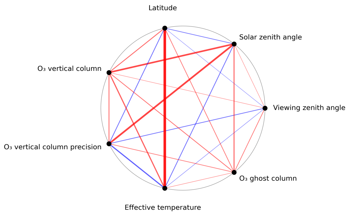
Figure 1: Map of correlation graph for 2024-07-27 to 2024-07-29.
