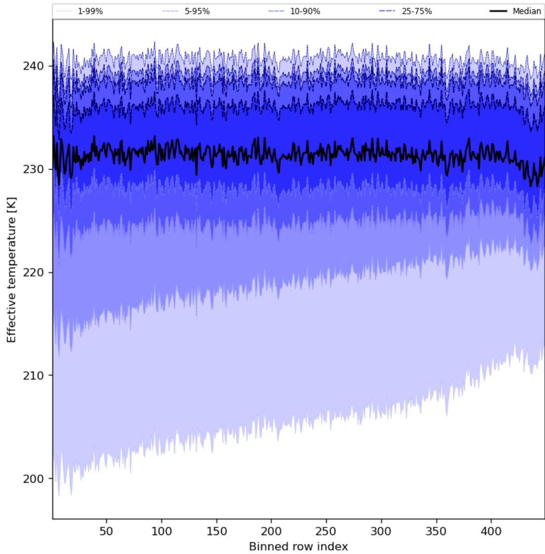
Figure 31: Along track statistics of “Effective temperature” for 2024-07-27 to 2024-07-29
