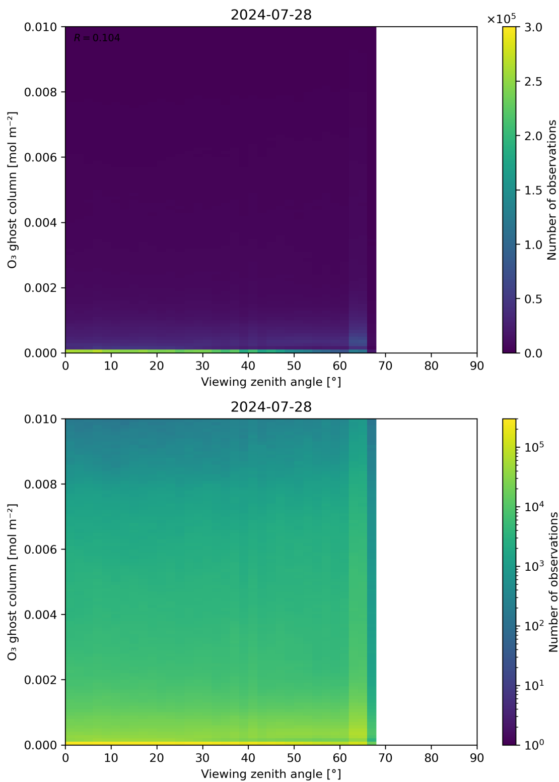
Figure 51: Scatter density plot of “Viewing zenith angle” against “O 3 ghost column” for 2024-07-27 to 2024-07-29.
