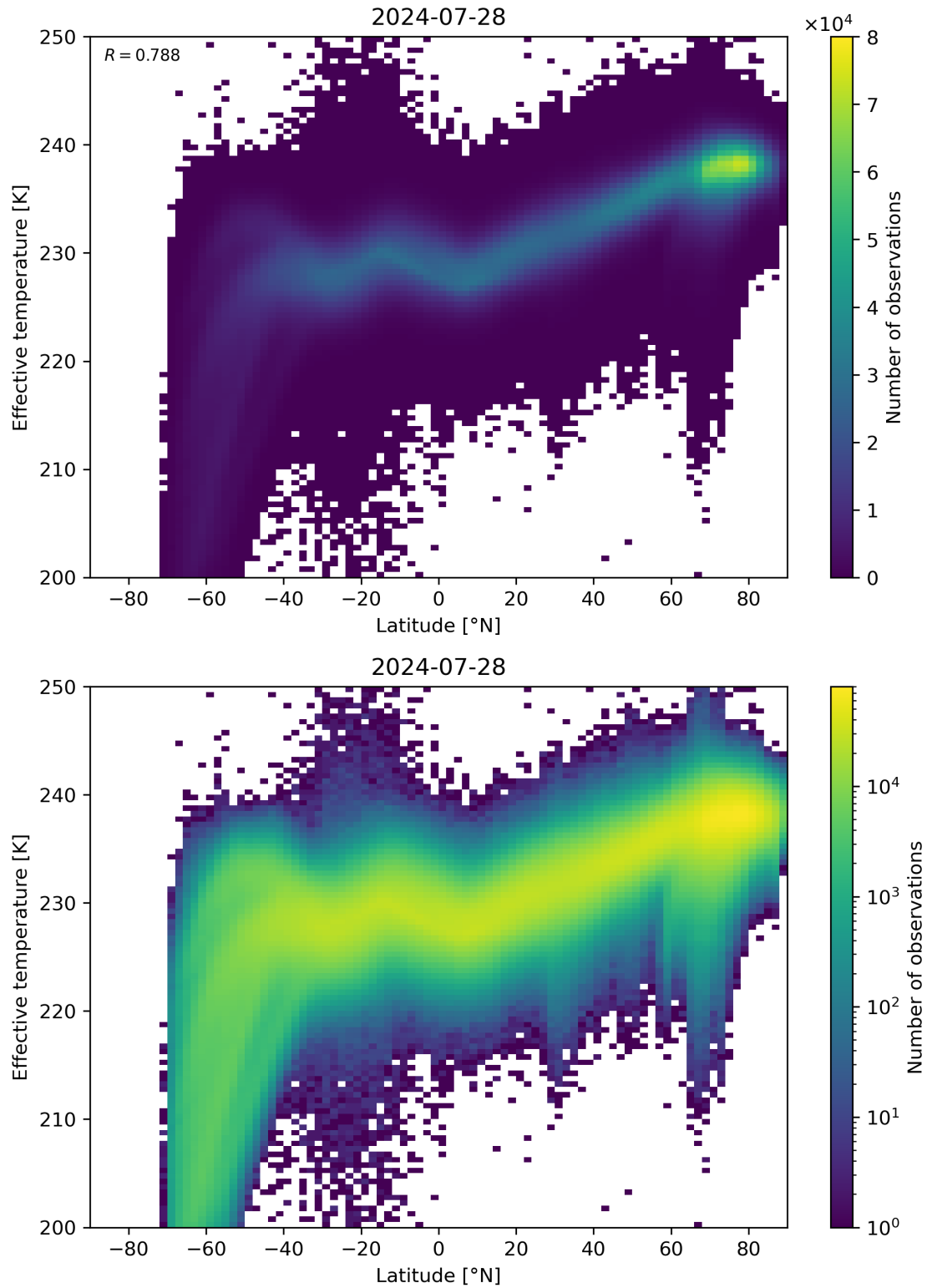
Figure 34: Scatter density plot of “Latitude” against “Effective temperature” for 2024-07-27 to 2024-07-29.
