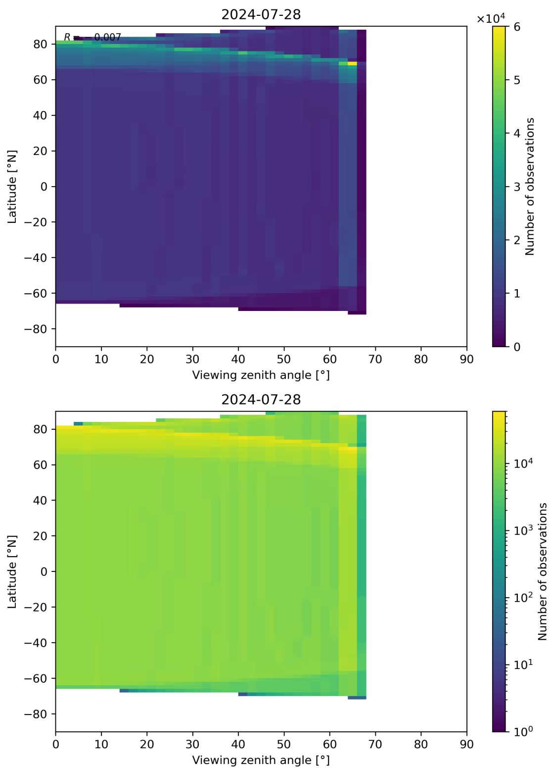
Figure 49: Scatter density plot of “Viewing zenith angle” against “Latitude” for 2024-07-27 to 2024-07-29.
