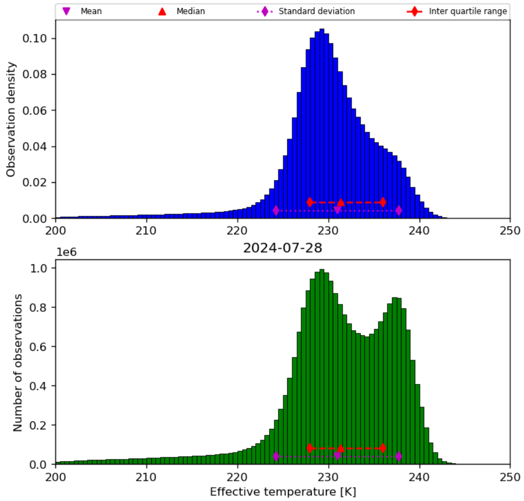
Figure 24: Histogram of “Effective temperature” for 2024-07-27 to 2024-07-29
