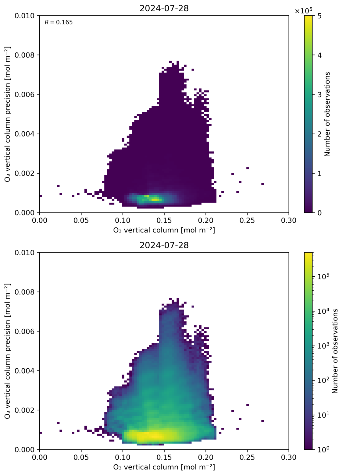
Figure 41: Scatter density plot of “O 3 vertical column” against “O 3 vertical column precision” for 2024-07-27 to 2024-07-29.
