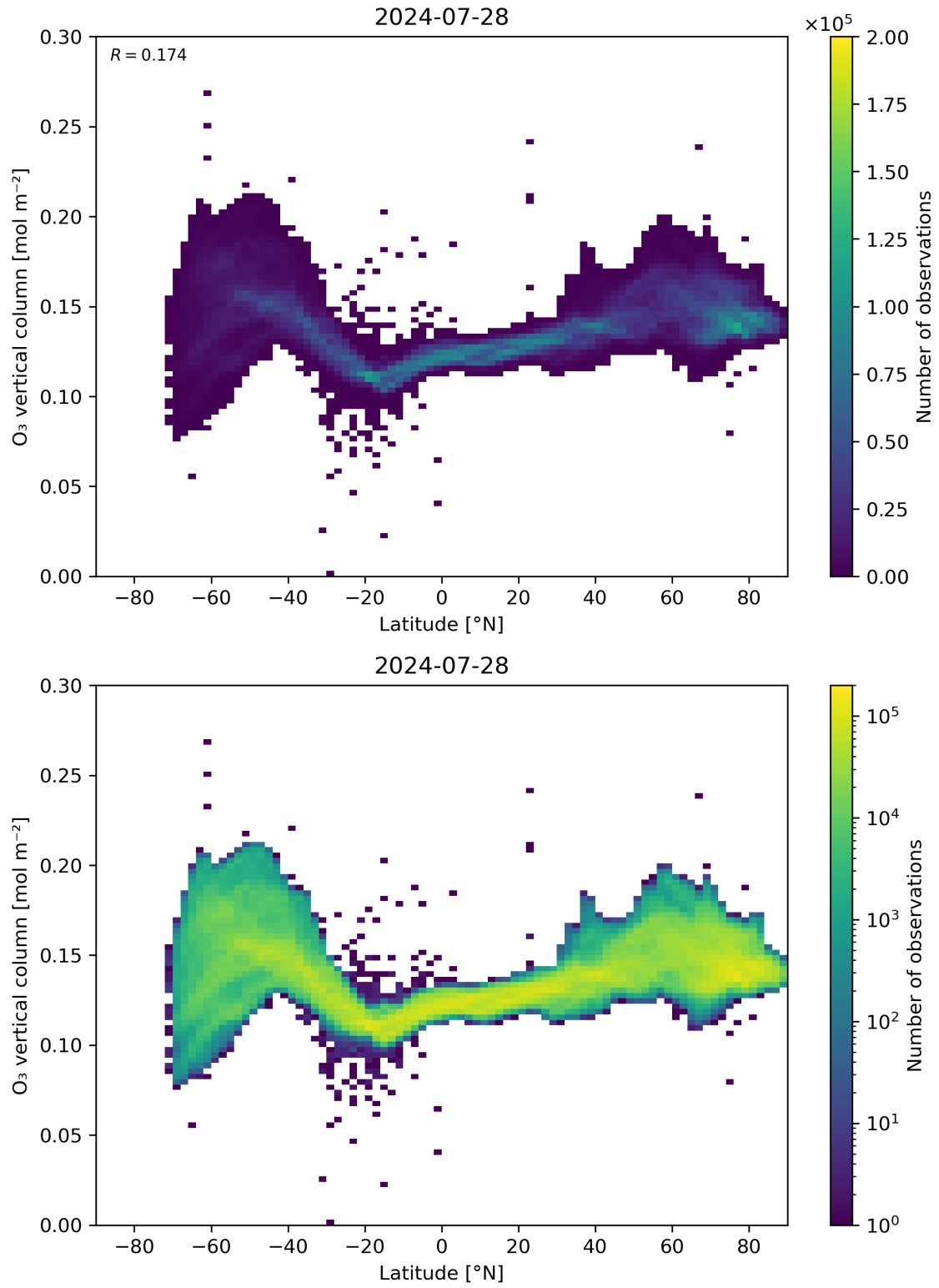
Figure 36: Scatter density plot of “Latitude” against “O 3 vertical column” for 2024-07-27 to 2024-07-29.
