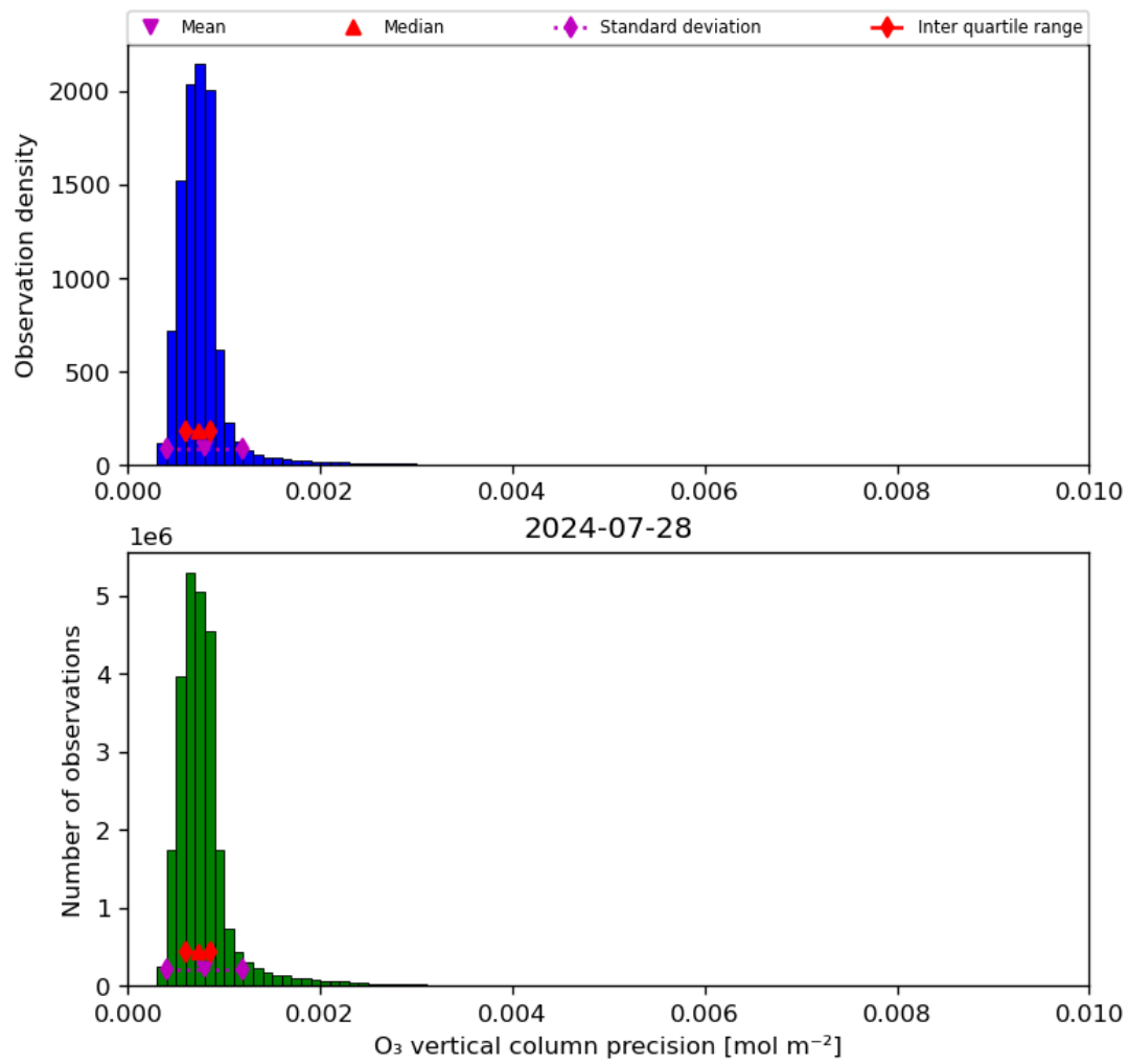
Figure 22: Histogram of “O 3 vertical column precision” for 2024-07-27 to 2024-07-29
