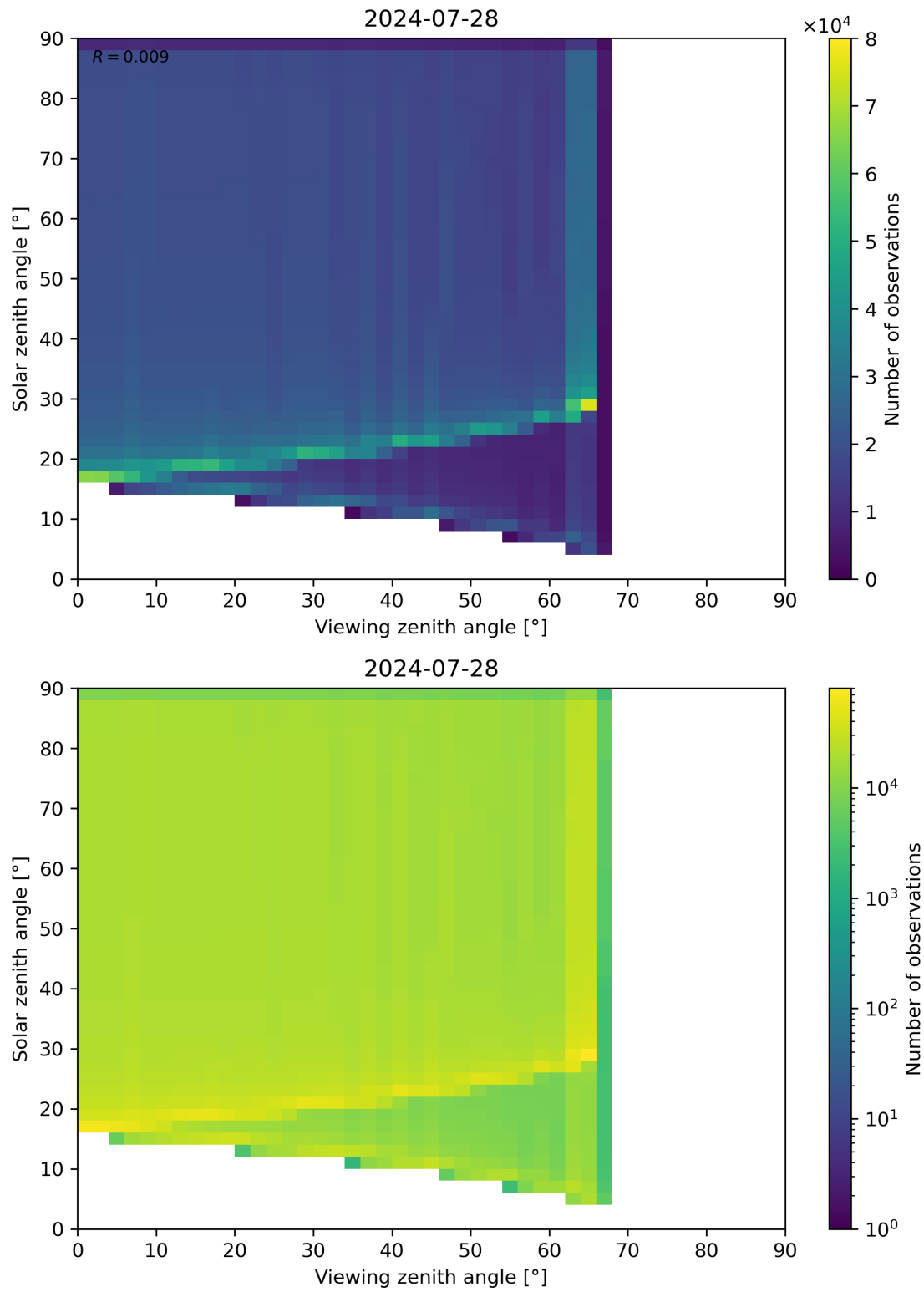
Figure 54: Scatter density plot of “Viewing zenith angle” against “Solar zenith angle” for 2024-07-27 to 2024-07-29.
