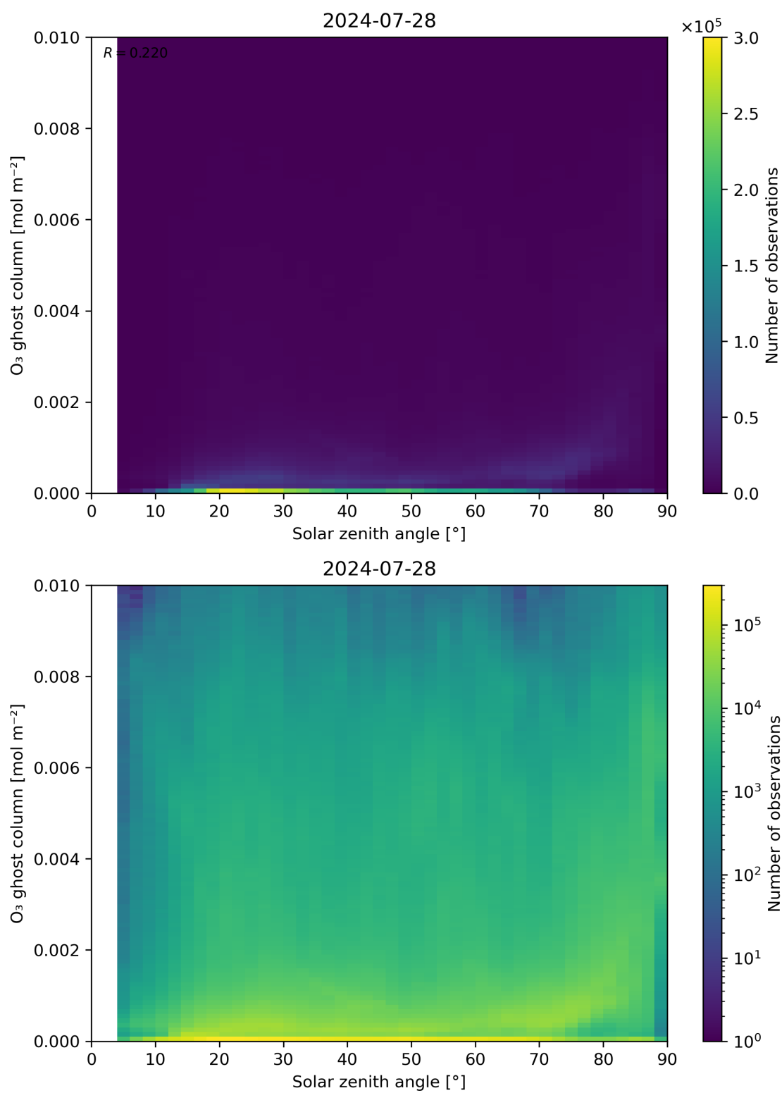
Figure 46: Scatter density plot of “Solar zenith angle” against “O 3 ghost column” for 2024-07-27 to 2024-07-29.
