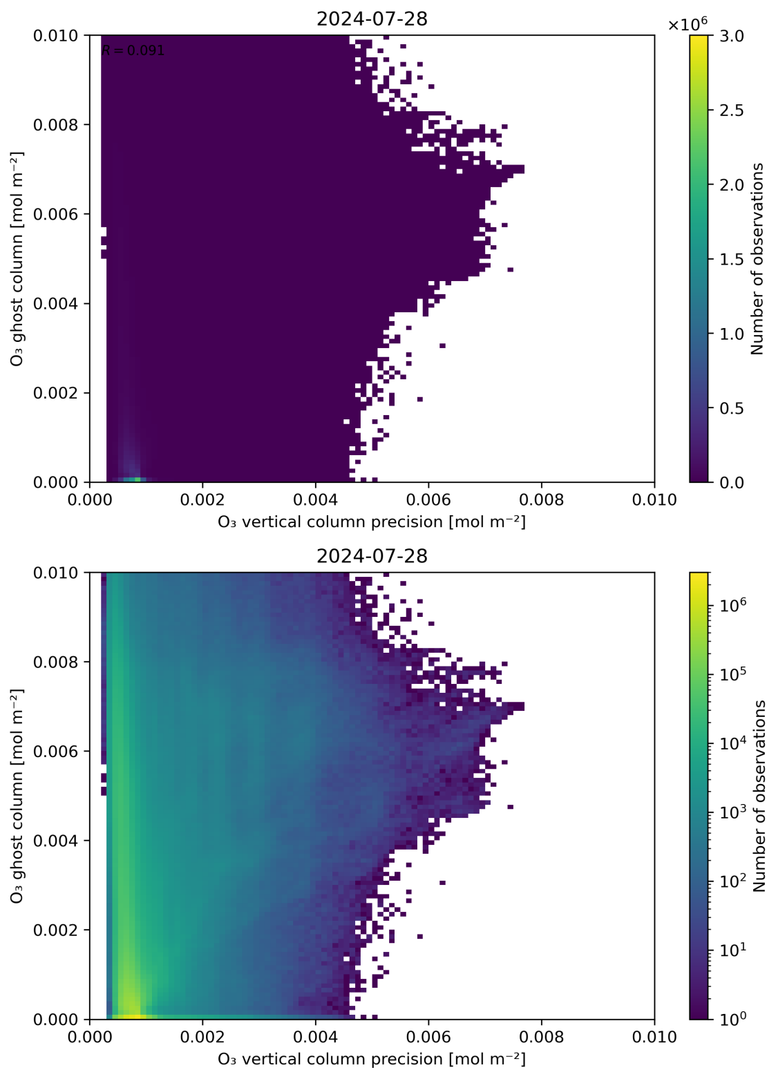
Figure 43: Scatter density plot of “ \text{O}_3 vertical column precision” against “ \text{O}_3 ghost column” for 2024-07-27 to 2024-07-29.
