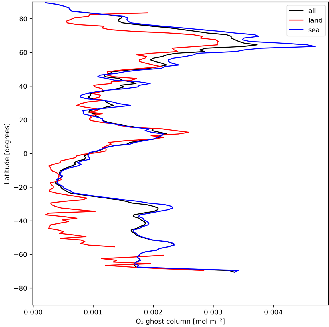
Figure 18: Zonal average of "O 3 ghost column" for 2024-07-27 to 2024-07-29.
