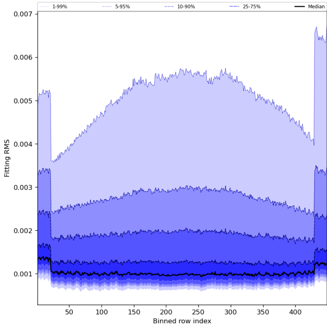
Figure 30: Along track statistics of “Fitting RMS” for 2024-07-27 to 2024-07-29
