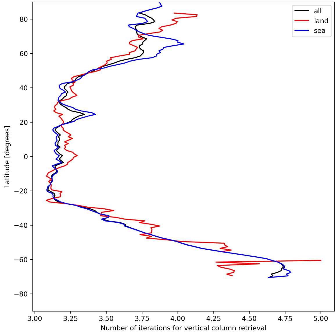
Figure 19: Zonal average of “Number of iterations for vertical column retrieval” for 2024-07-27 to 2024-07-29.
