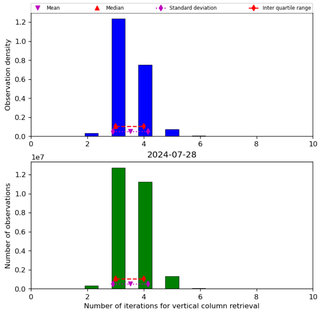
Figure 26: Histogram of “Number of iterations for vertical column retrieval” for 2024-07-27 to 2024-07-29
