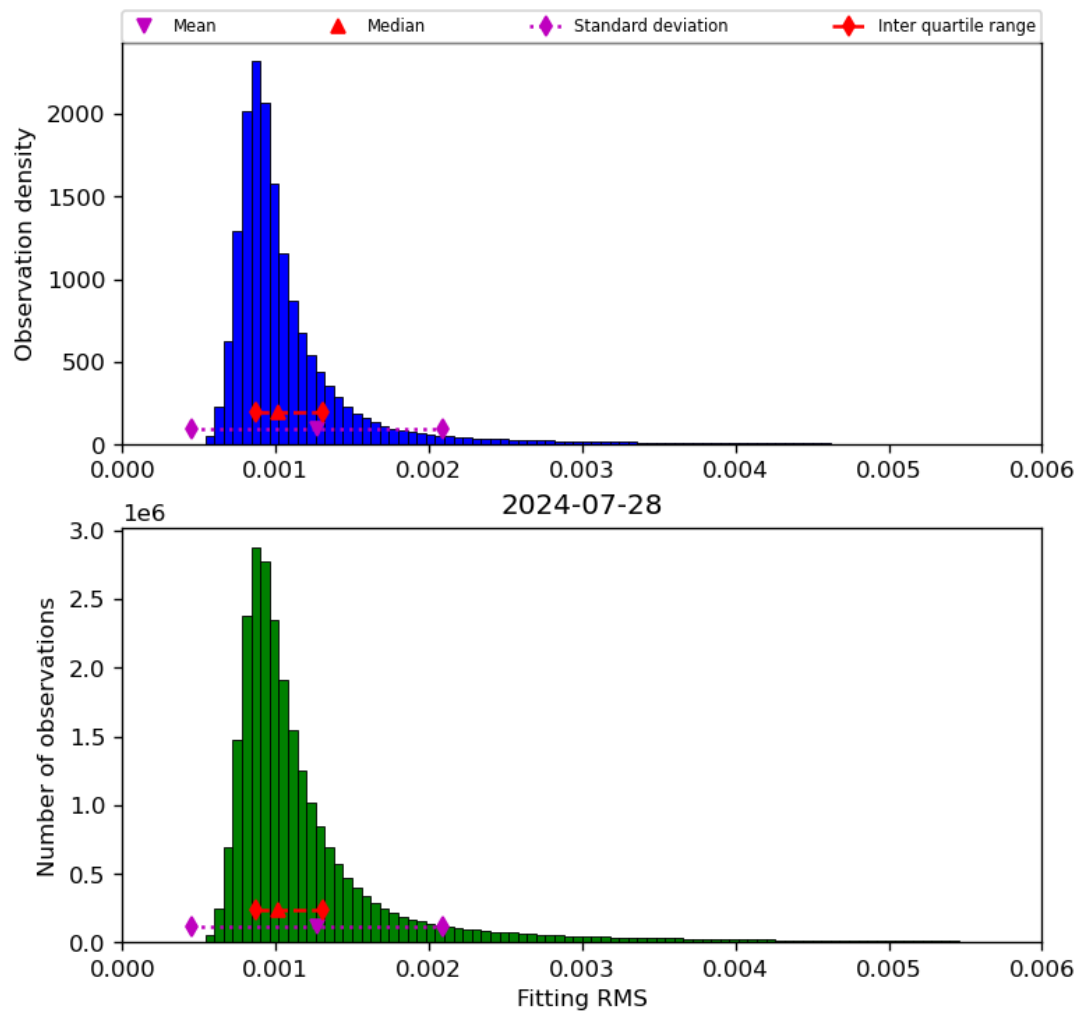
Figure 23: Histogram of “Fitting RMS” for 2024-07-27 to 2024-07-29
