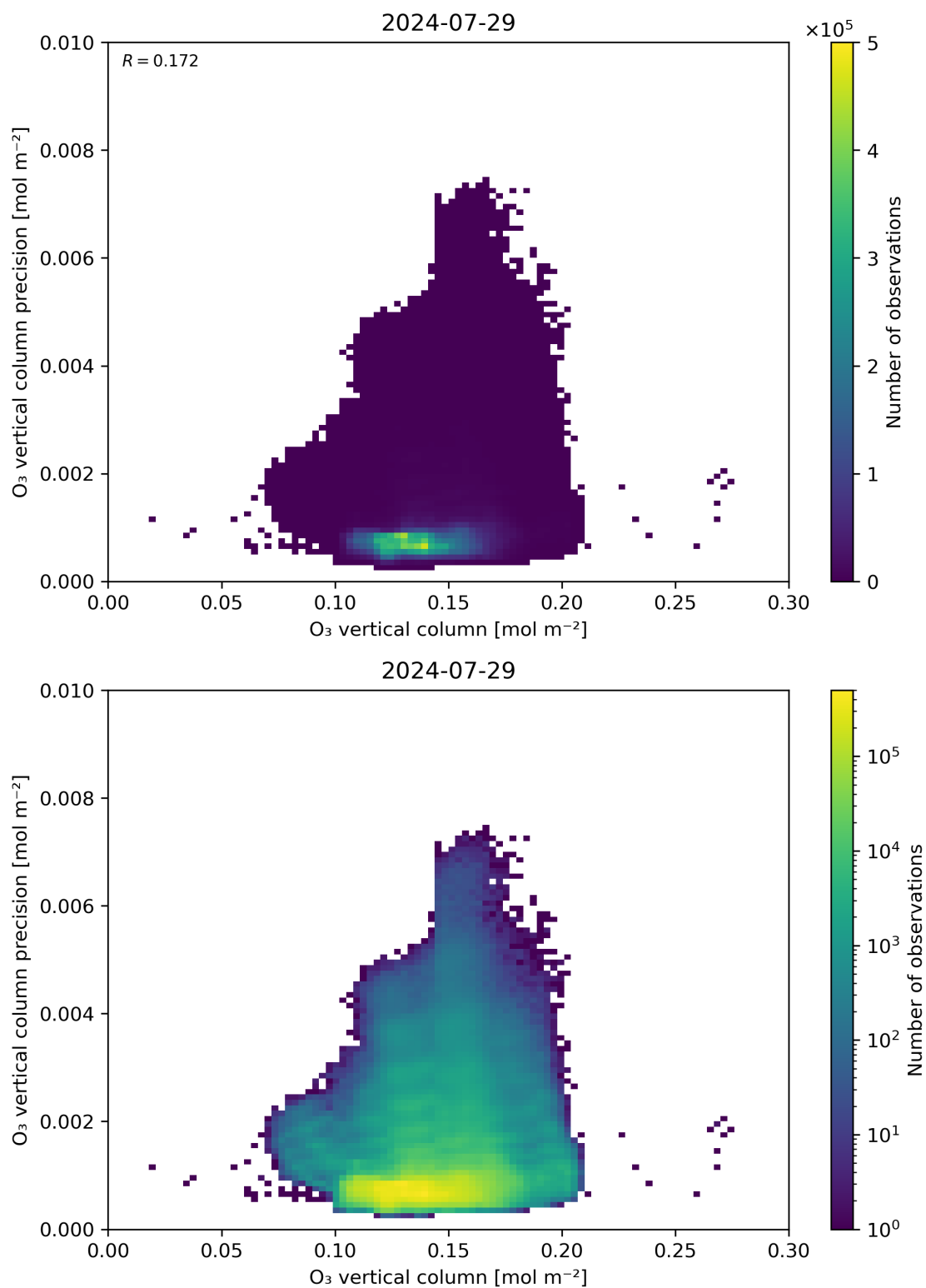
Figure 41: Scatter density plot of “O 3 vertical column” against “O 3 vertical column precision” for 2024-07-28 to 2024-07-30.
