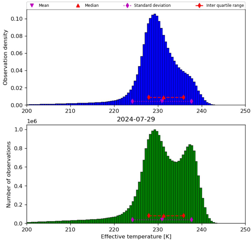
Figure 24: Histogram of “Effective temperature” for 2024-07-28 to 2024-07-30
