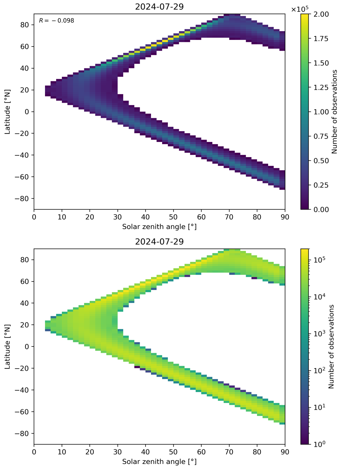
Figure 44: Scatter density plot of “Solar zenith angle” against “Latitude” for 2024-07-28 to 2024-07-30.
