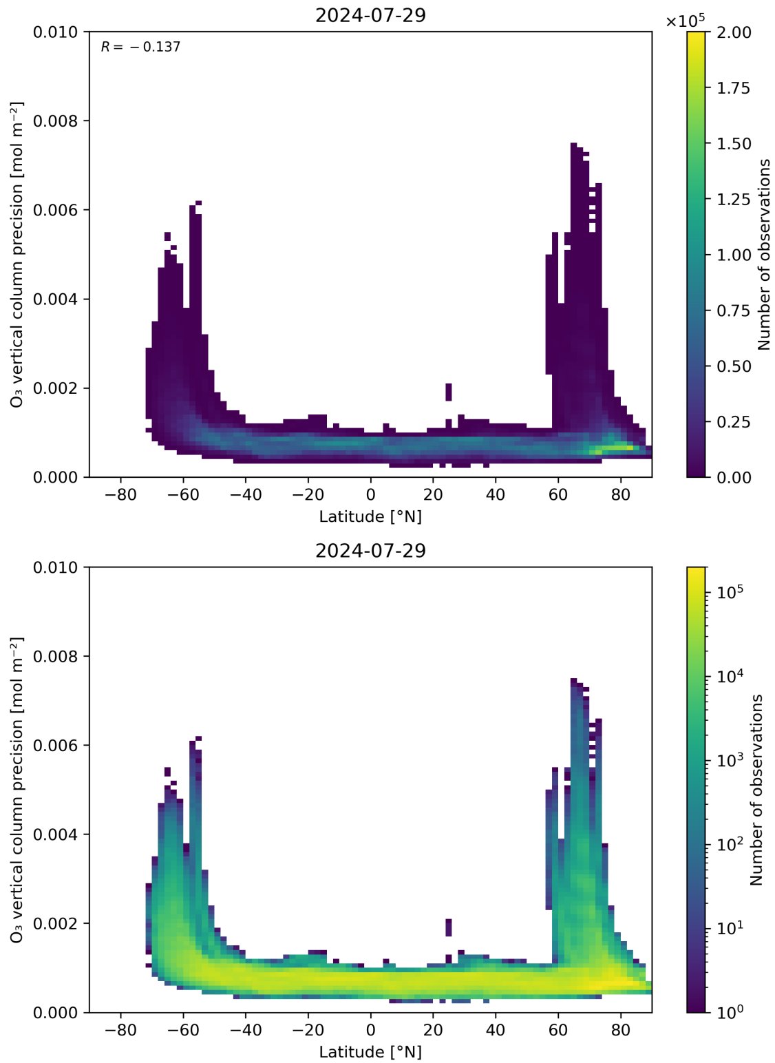
Figure 37: Scatter density plot of “Latitude” against “O 3 vertical column precision” for 2024-07-28 to 2024-07-30.
