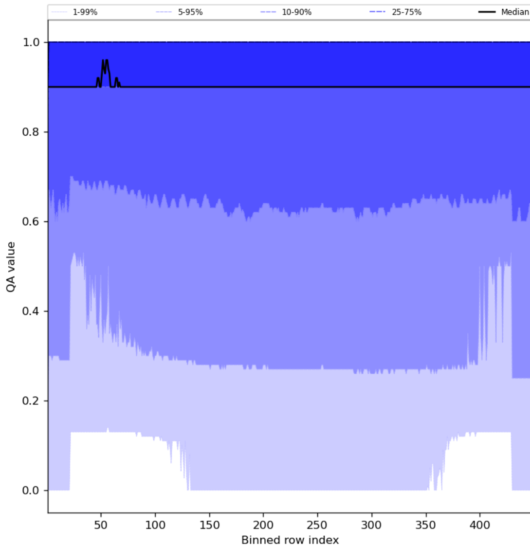
Figure 27: Along track statistics of “QA value” for 2024-07-28 to 2024-07-30
