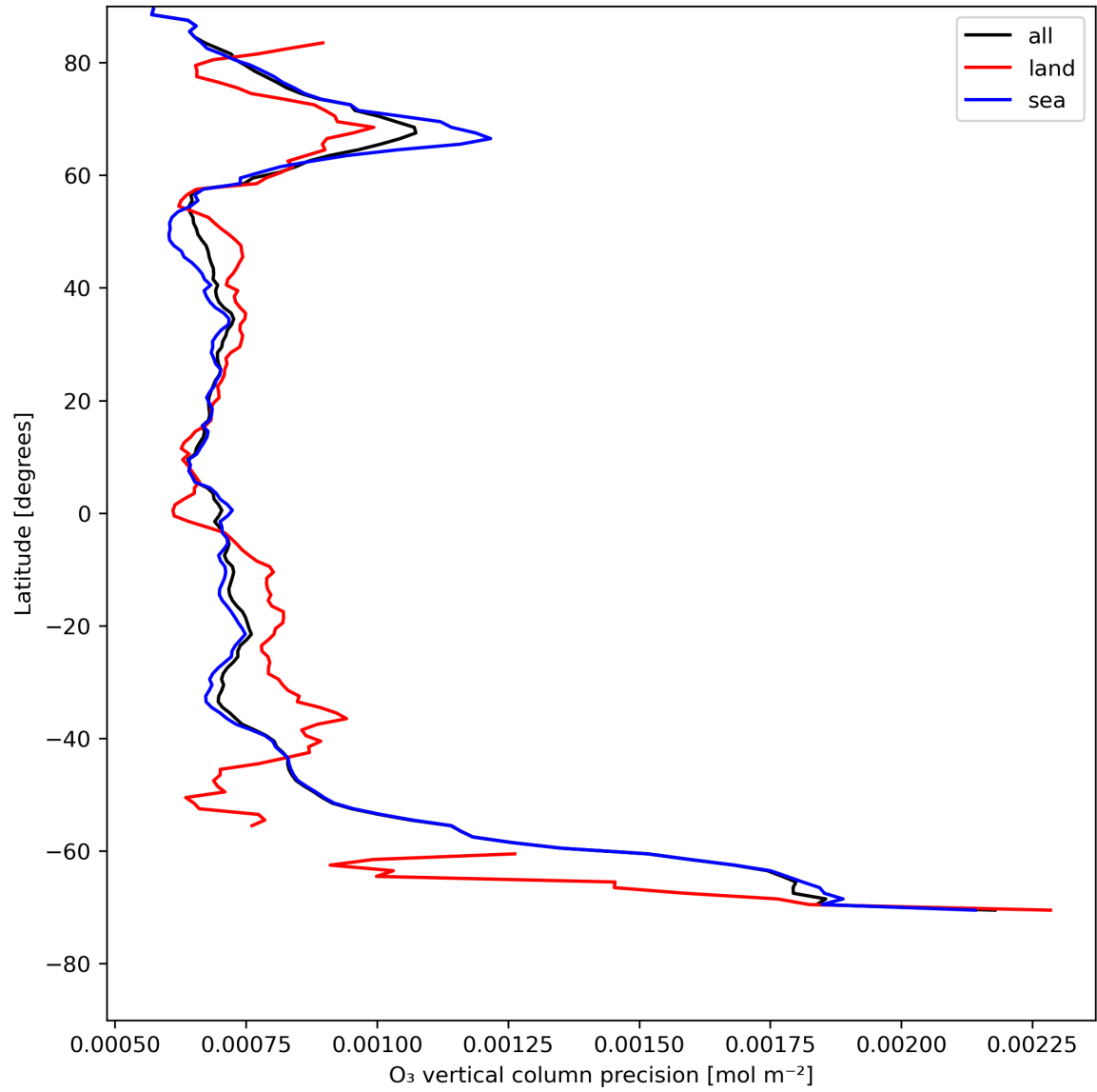
Figure 15: Zonal average of “O 3 vertical column precision” for 2024-07-28 to 2024-07-30.
