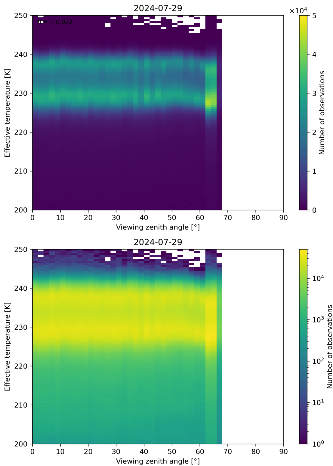
Figure 50: Scatter density plot of “Viewing zenith angle” against “Effective temperature” for 2024-07-28 to 2024-07-30.
