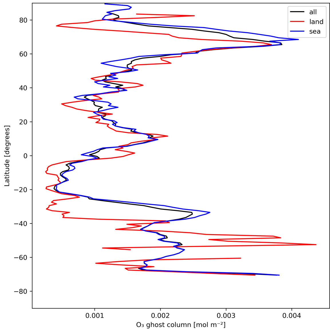
Figure 18: Zonal average of "O 3 ghost column" for 2024-07-28 to 2024-07-30.
