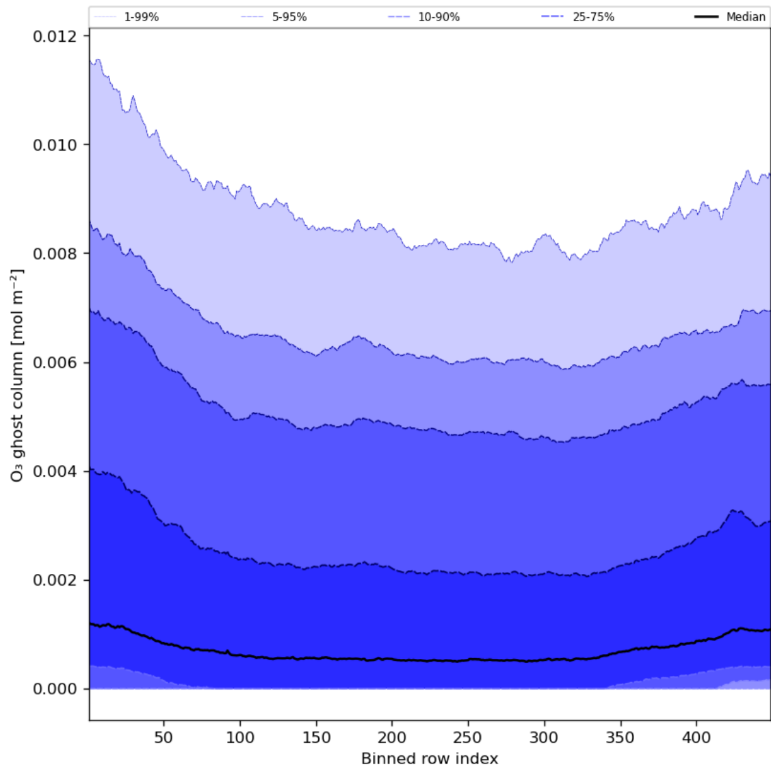
Figure 32: Along track statistics of “O 3 ghost column” for 2024-07-28 to 2024-07-30
