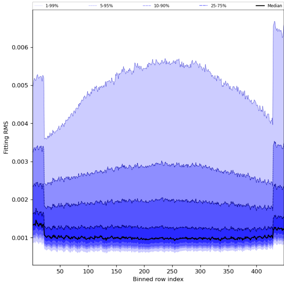
Figure 30: Along track statistics of “Fitting RMS” for 2024-07-28 to 2024-07-30
