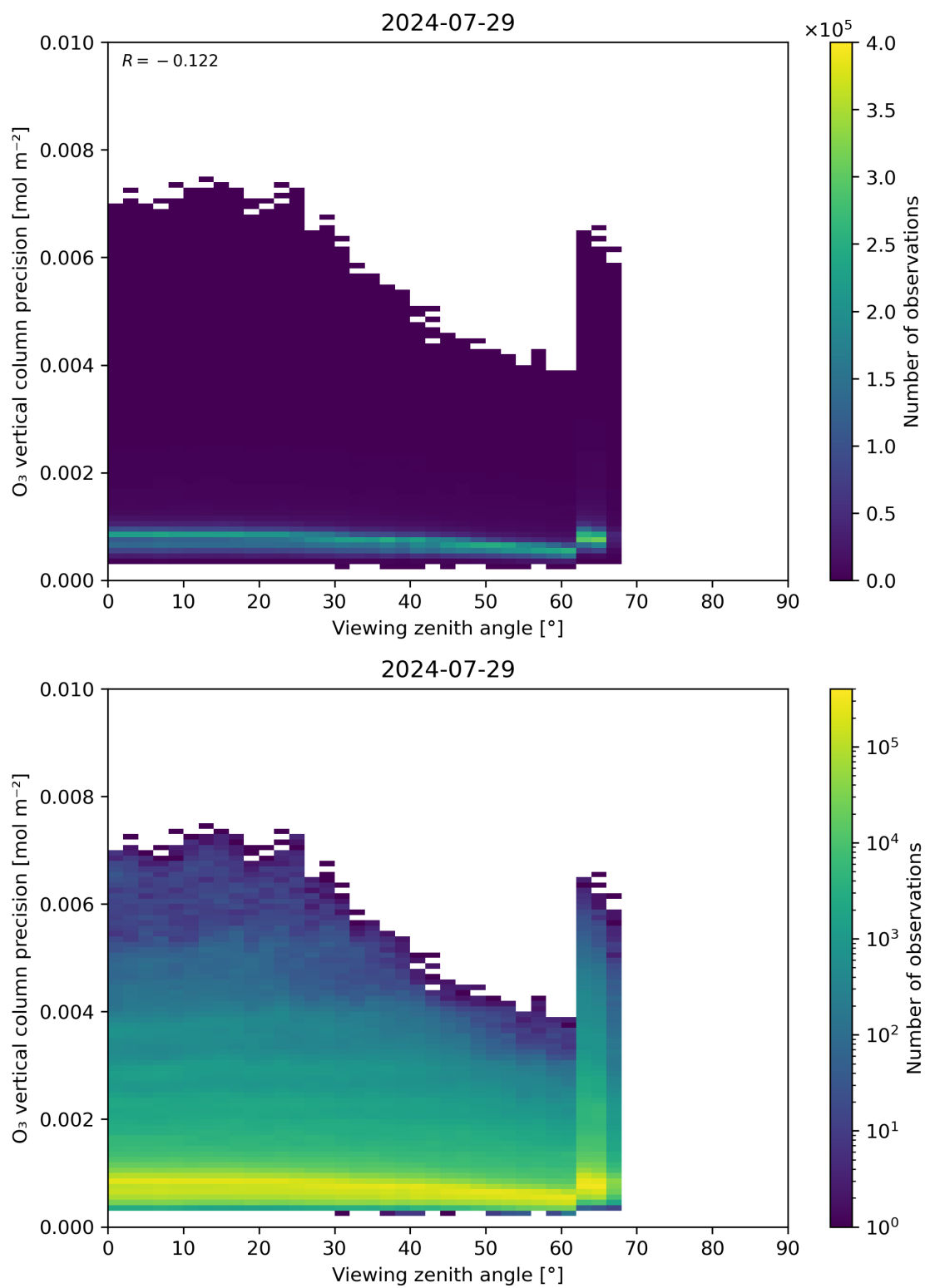
Figure 53: Scatter density plot of “Viewing zenith angle” against “O 3 vertical column precision” for 2024-07-28 to 2024-07-30.
