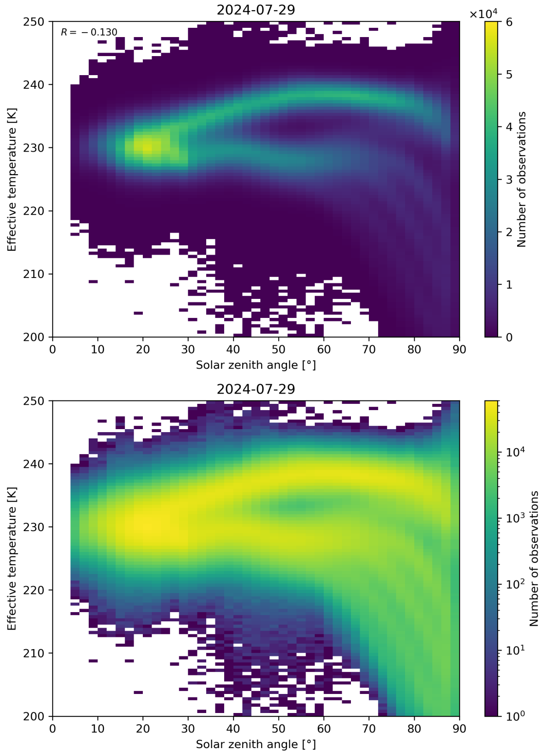
Figure 45: Scatter density plot of “Solar zenith angle” against “Effective temperature” for 2024-07-28 to 2024-07-30.
