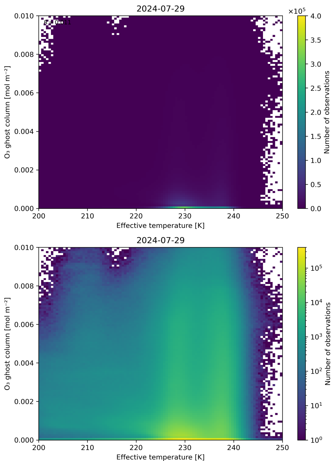
Figure 38: Scatter density plot of “Effective temperature” against “O 3 ghost column” for 2024-07-28 to 2024-07-30.
