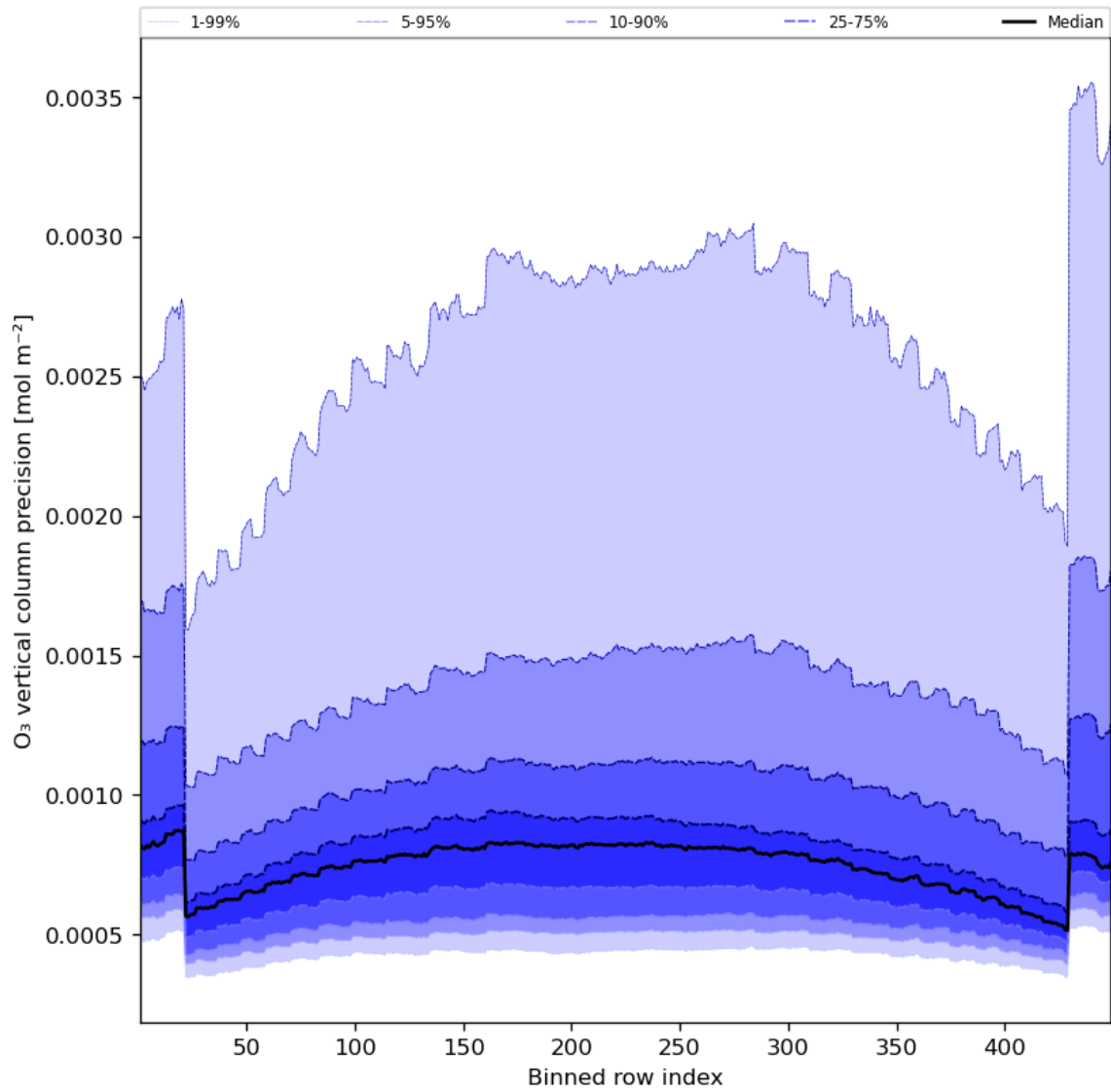
Figure 29: Along track statistics of “O 3 vertical column precision” for 2024-07-28 to 2024-07-30
