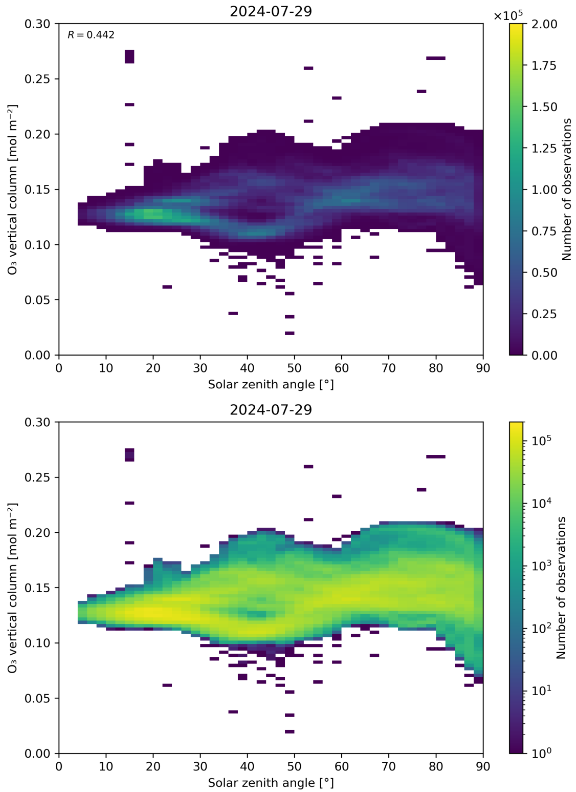
Figure 47: Scatter density plot of “Solar zenith angle” against “O 3 vertical column” for 2024-07-28 to 2024-07-30.
