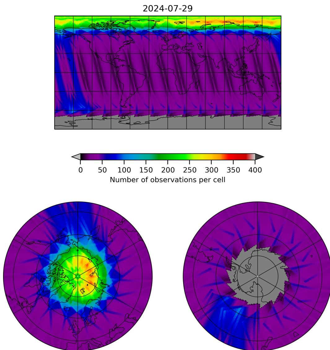
Figure 12: Map of the number of observations for 2024-07-28 to 2024-07-30
