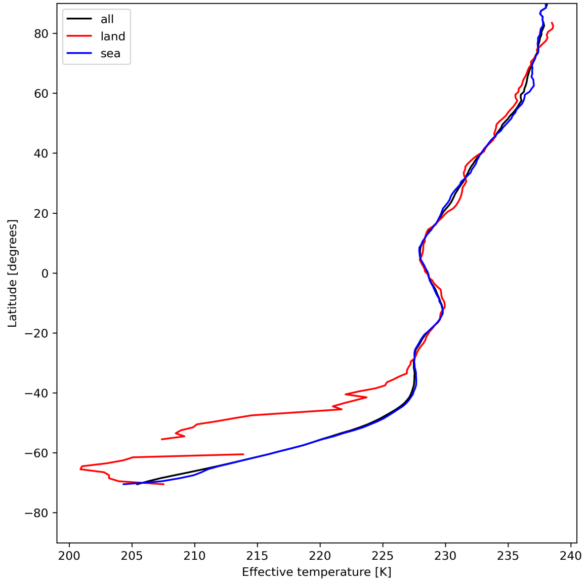
Figure 17: Zonal average of "Effective temperature" for 2024-07-28 to 2024-07-30.
