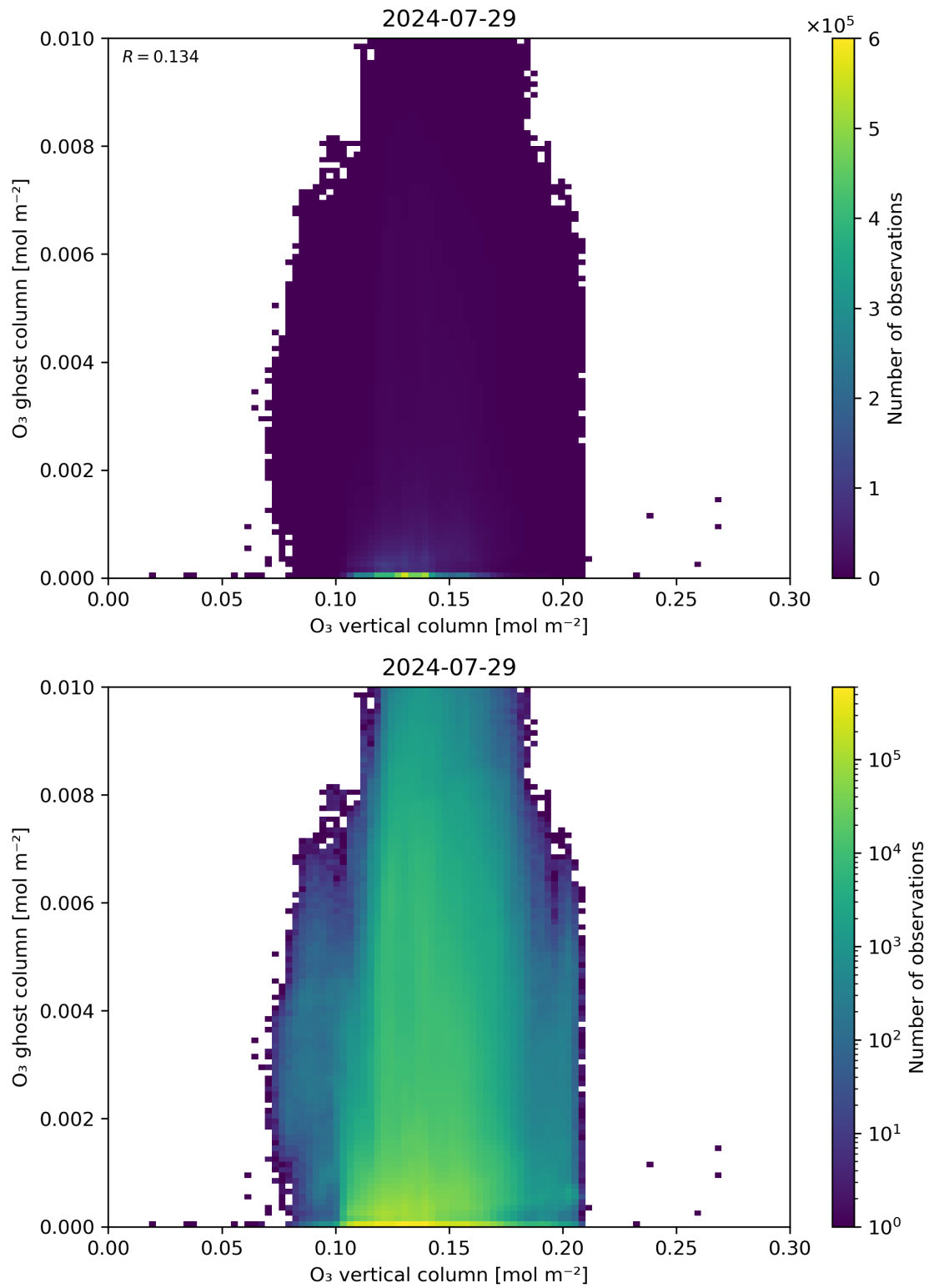
Figure 40: Scatter density plot of “O 3 vertical column” against “O 3 ghost column” for 2024-07-28 to 2024-07-30.
