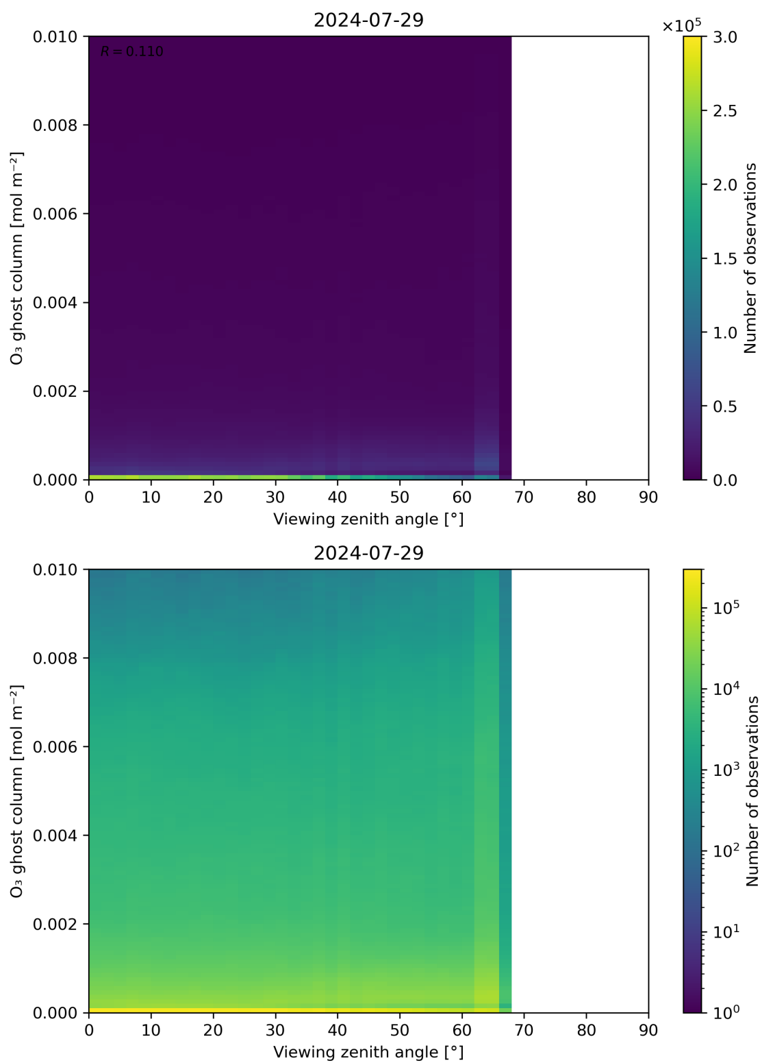
Figure 51: Scatter density plot of “Viewing zenith angle” against “O 3 ghost column” for 2024-07-28 to 2024-07-30.
