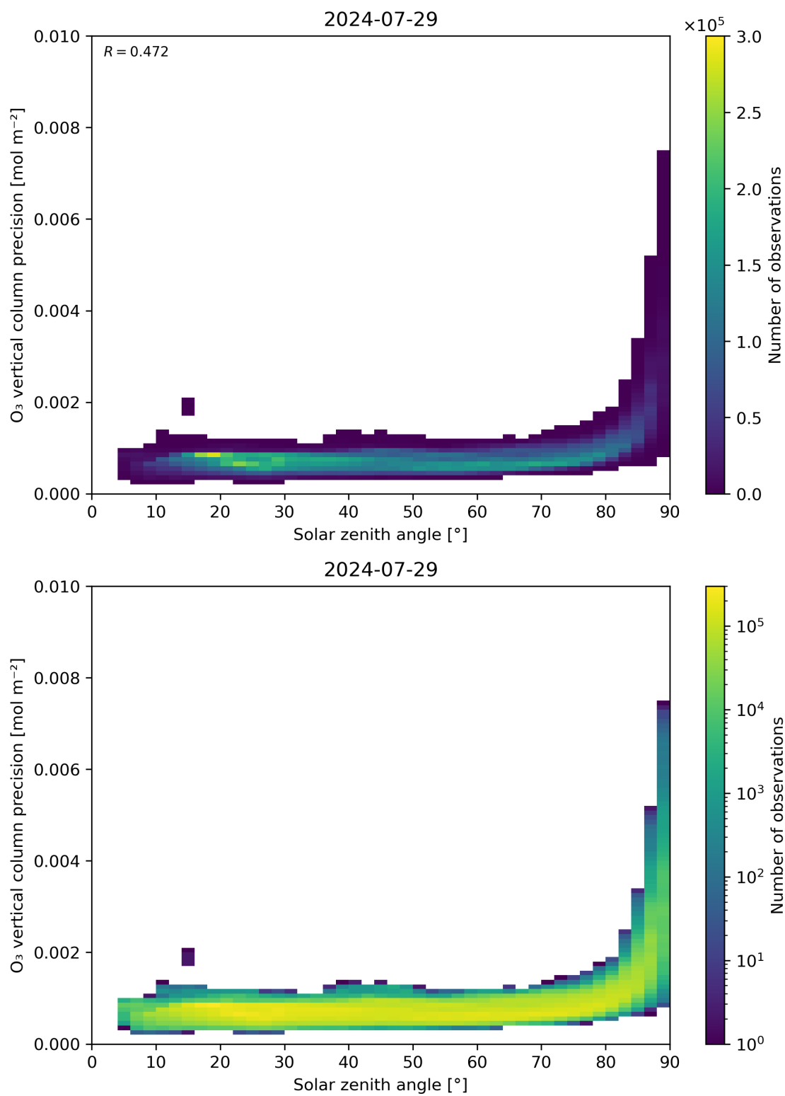
Figure 48: Scatter density plot of “Solar zenith angle” against “O 3 vertical column precision” for 2024-07-28 to 2024-07-30.
