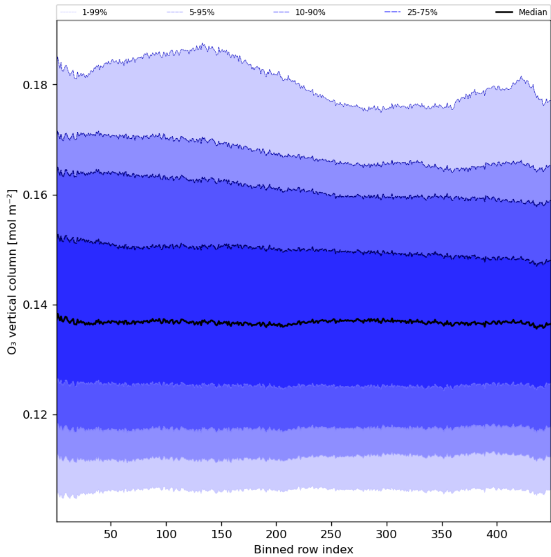
Figure 28: Along track statistics of “O 3 vertical column” for 2024-07-28 to 2024-07-30
