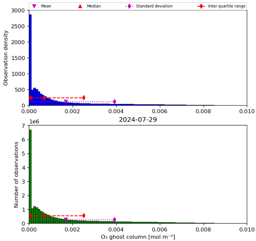
Figure 25: Histogram of “O 3 ghost column” for 2024-07-28 to 2024-07-30
