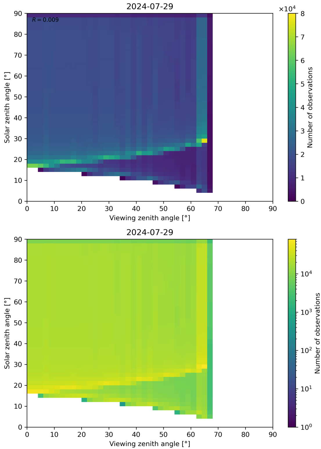
Figure 54: Scatter density plot of “Viewing zenith angle” against “Solar zenith angle” for 2024-07-28 to 2024-07-30.
