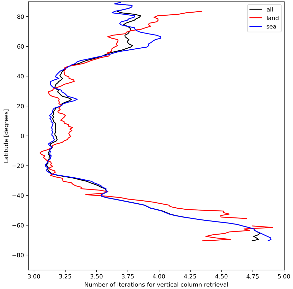
Figure 19: Zonal average of “Number of iterations for vertical column retrieval” for 2024-07-28 to 2024-07-30.
