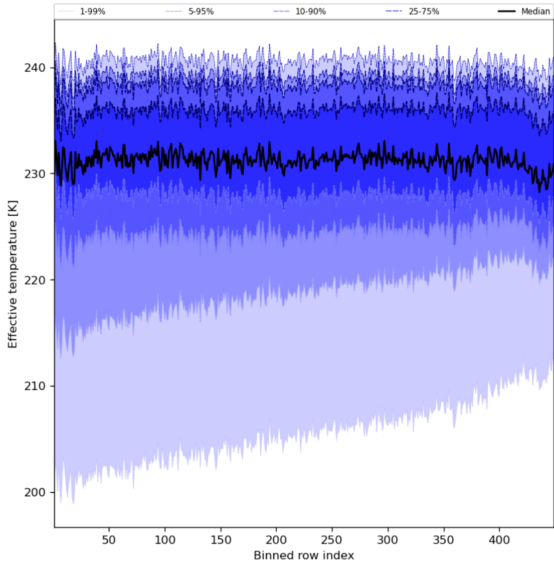
Figure 31: Along track statistics of “Effective temperature” for 2024-07-28 to 2024-07-30
