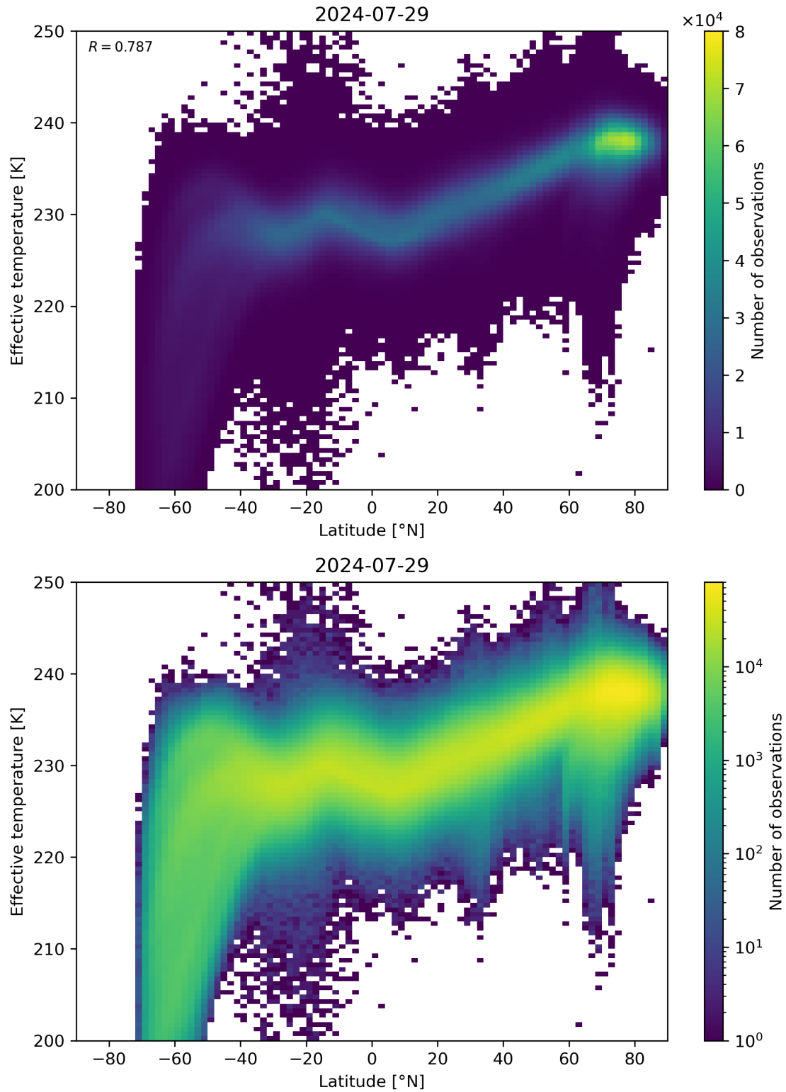
Figure 34: Scatter density plot of “Latitude” against “Effective temperature” for 2024-07-28 to 2024-07-30.
