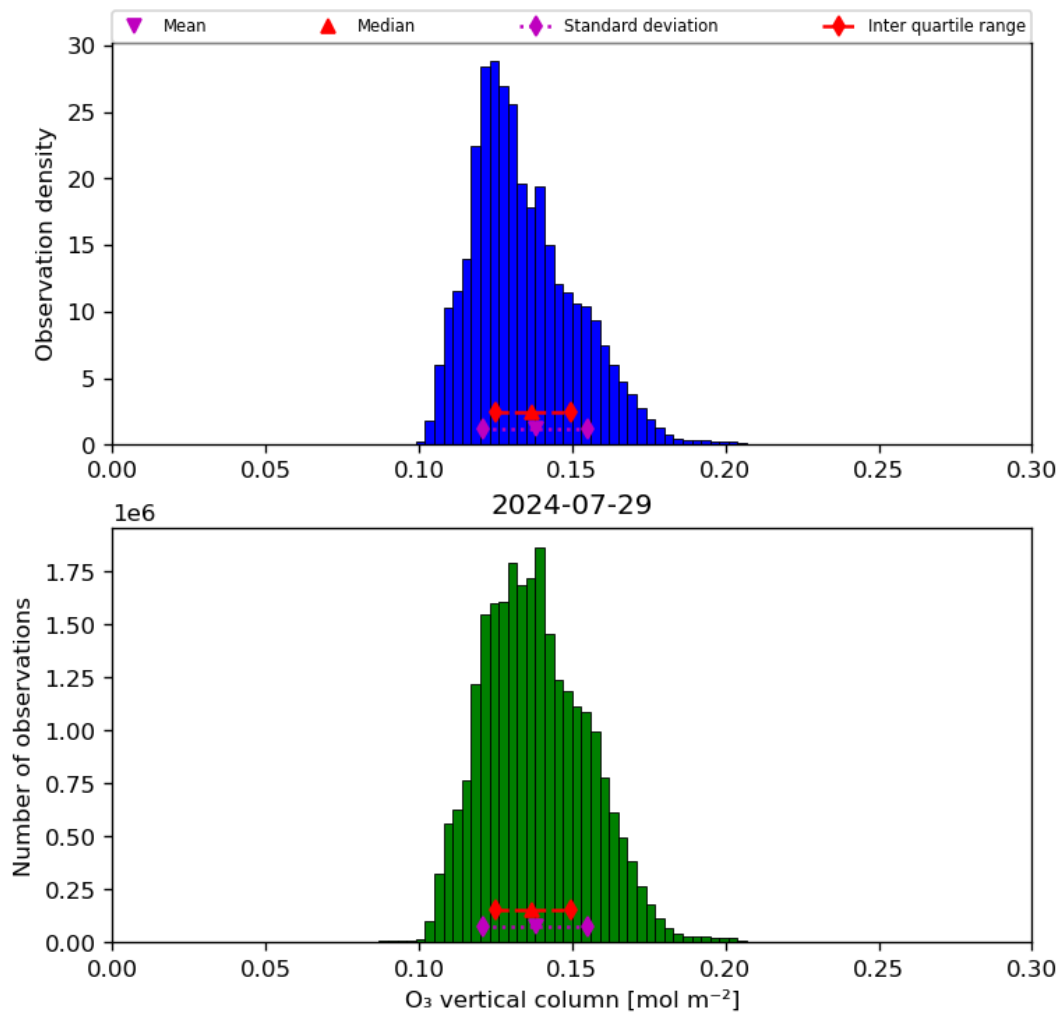
Figure 21: Histogram of “O 3 vertical column” for 2024-07-28 to 2024-07-30
