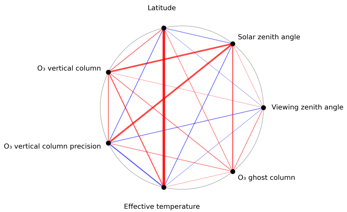
Figure 1: Map of correlation graph for 2024-07-28 to 2024-07-30.
