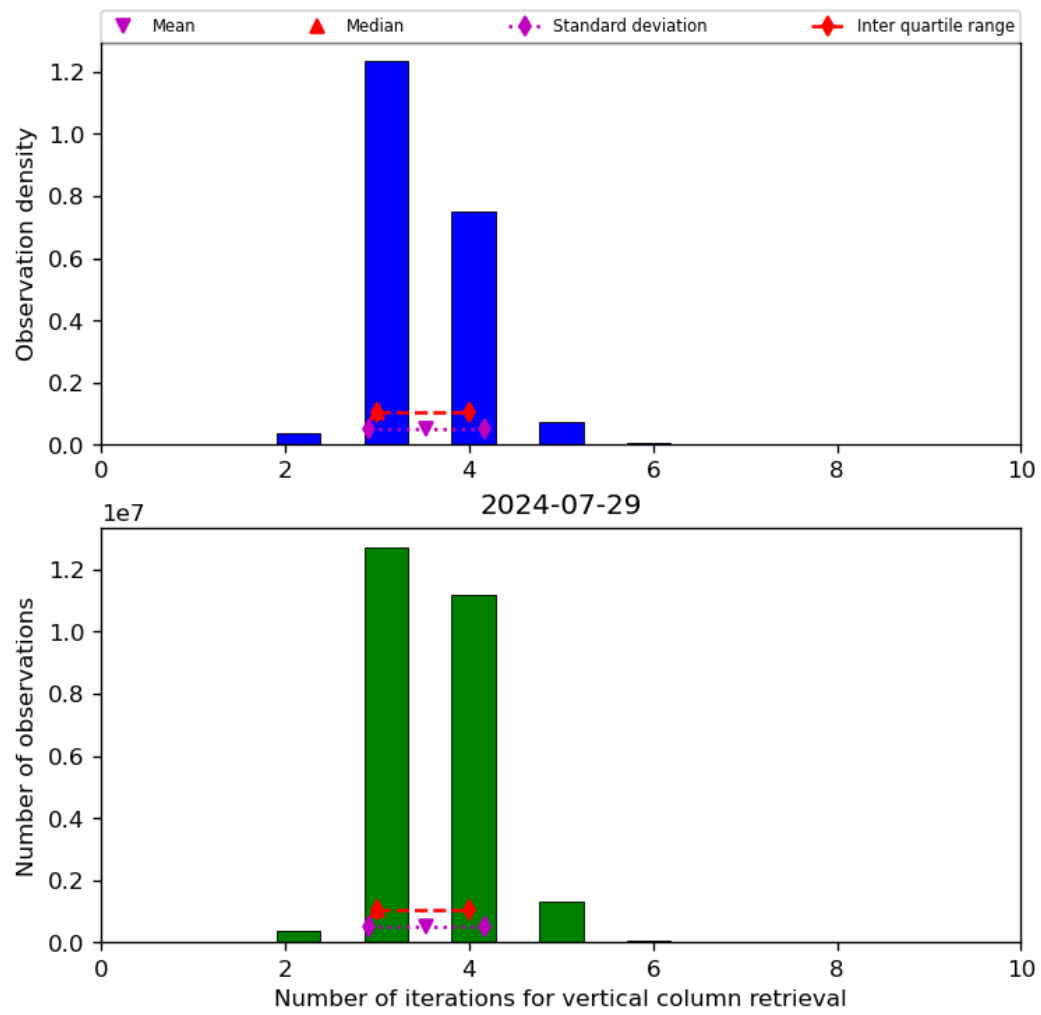
Figure 26: Histogram of “Number of iterations for vertical column retrieval” for 2024-07-28 to 2024-07-30
