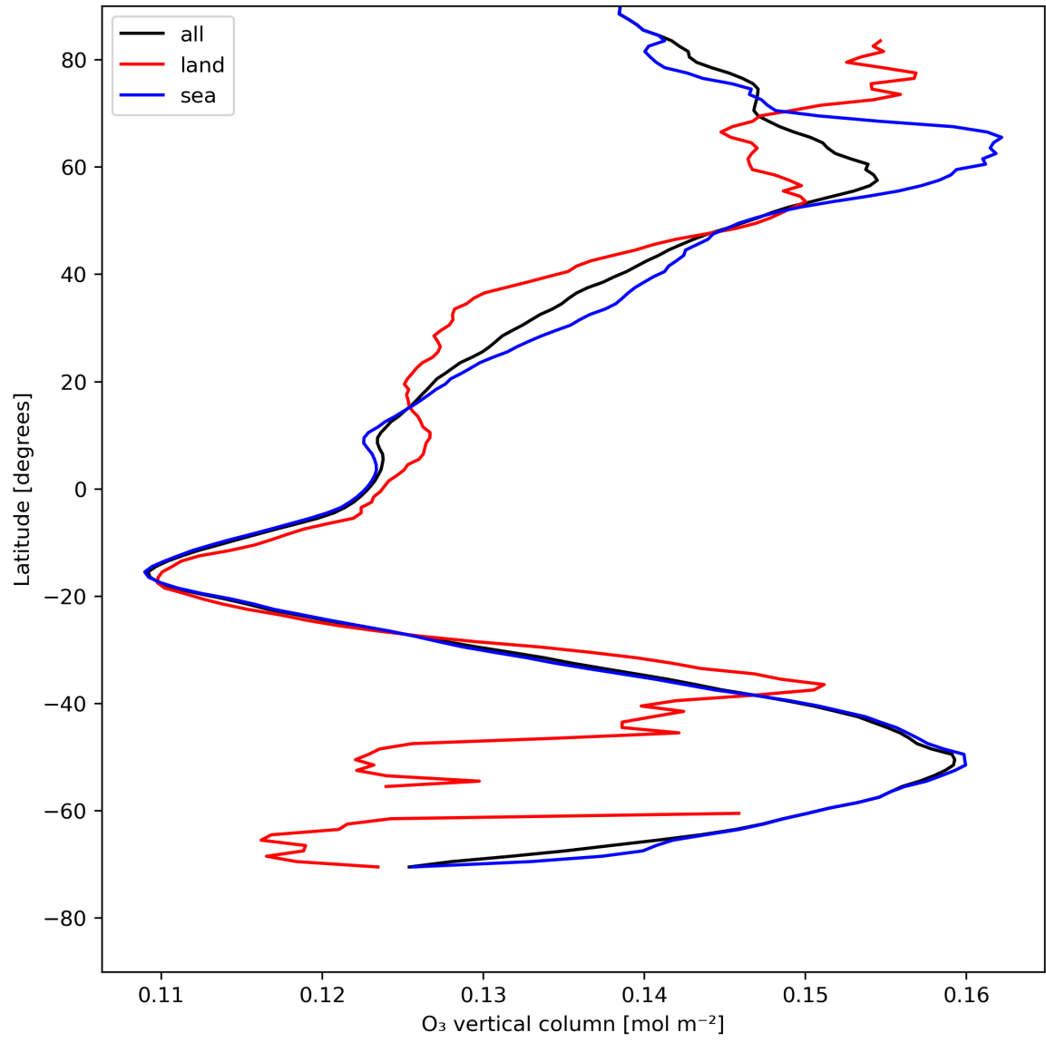
Figure 14: Zonal average of “O 3 vertical column” for 2024-07-28 to 2024-07-30.
