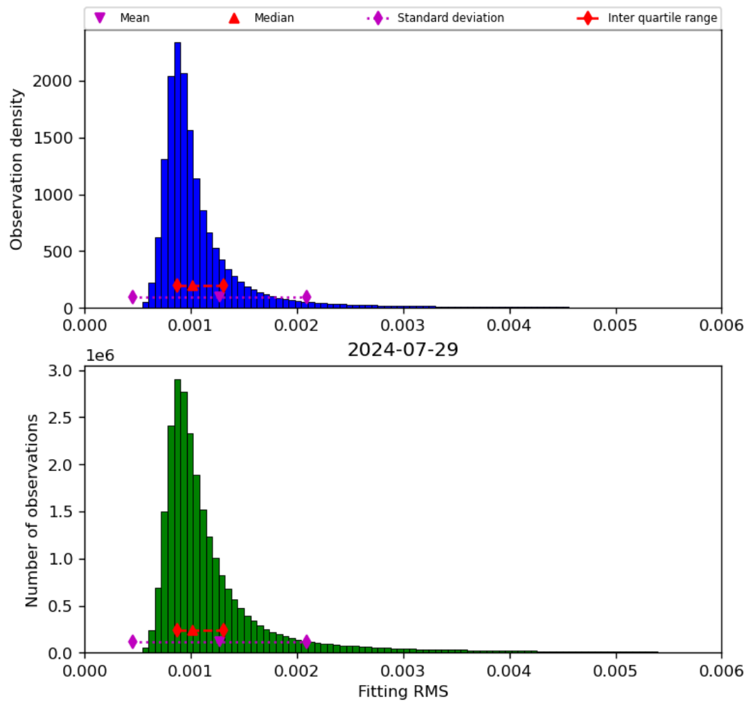
Figure 23: Histogram of “Fitting RMS” for 2024-07-28 to 2024-07-30
