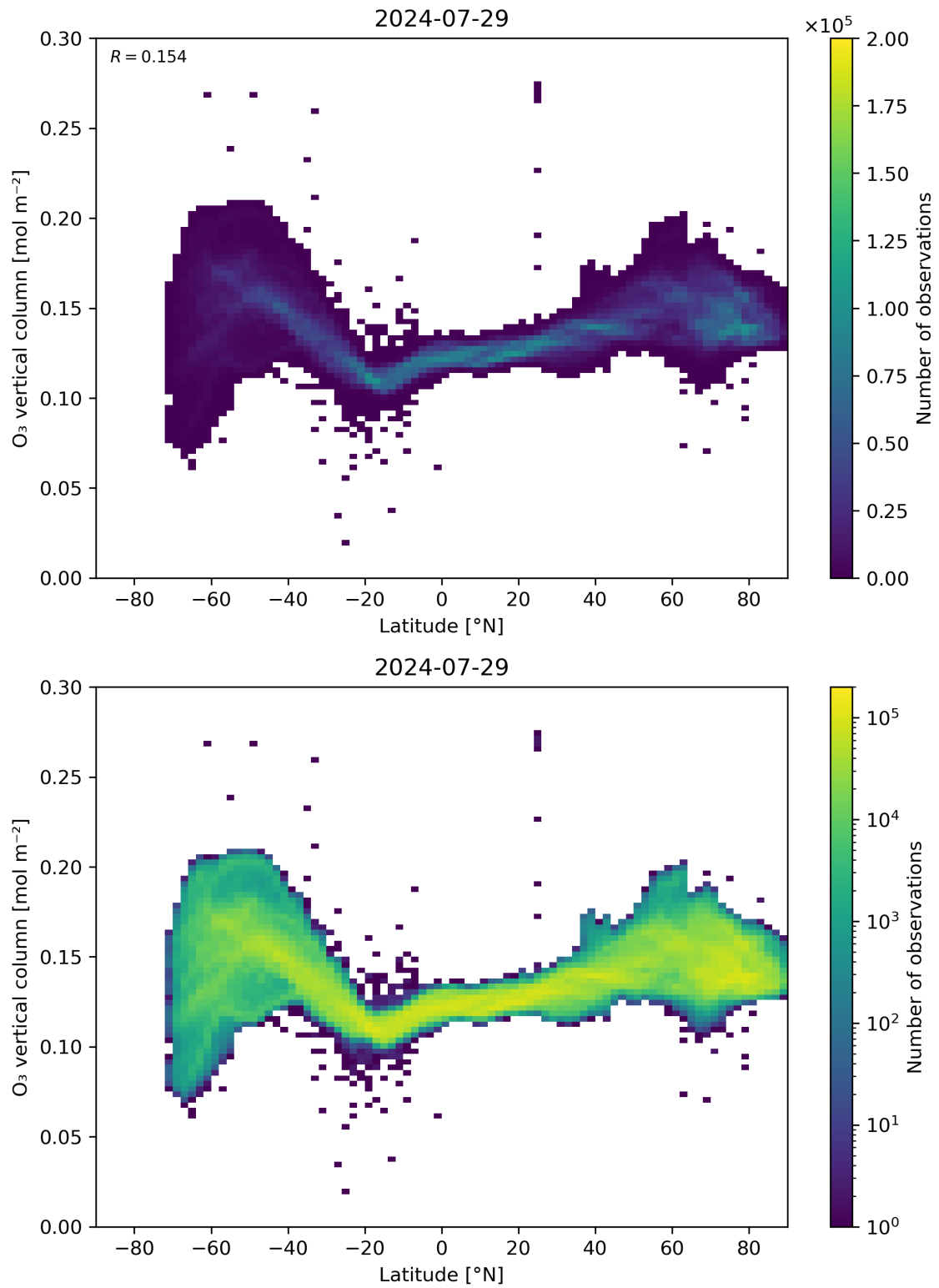
Figure 36: Scatter density plot of “Latitude” against “O 3 vertical column” for 2024-07-28 to 2024-07-30.
