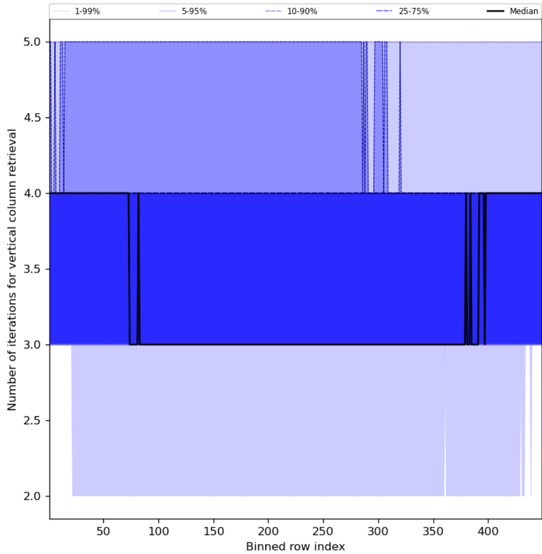
Figure 33: Along track statistics of “Number of iterations for vertical column retrieval” for 2024-07-28 to 2024-07-30
