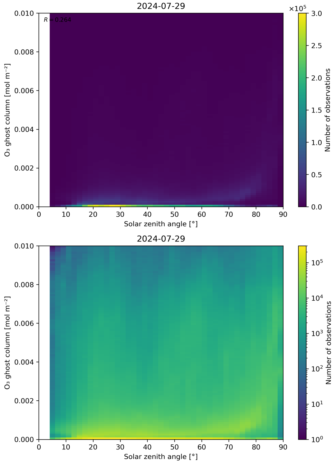
Figure 46: Scatter density plot of “Solar zenith angle” against “O 3 ghost column” for 2024-07-28 to 2024-07-30.
