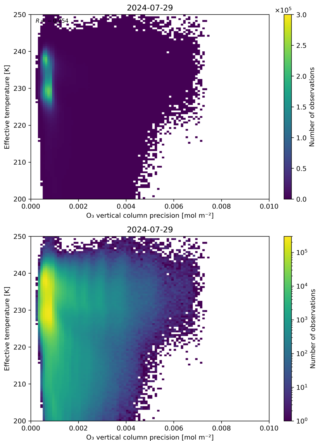
Figure 42: Scatter density plot of “O 3 vertical column precision” against “Effective temperature” for 2024-07-28 to 2024-07-30.
