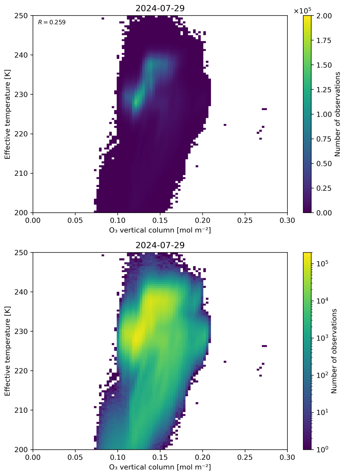
Figure 39: Scatter density plot of “O 3 vertical column” against “Effective temperature” for 2024-07-28 to 2024-07-30.
