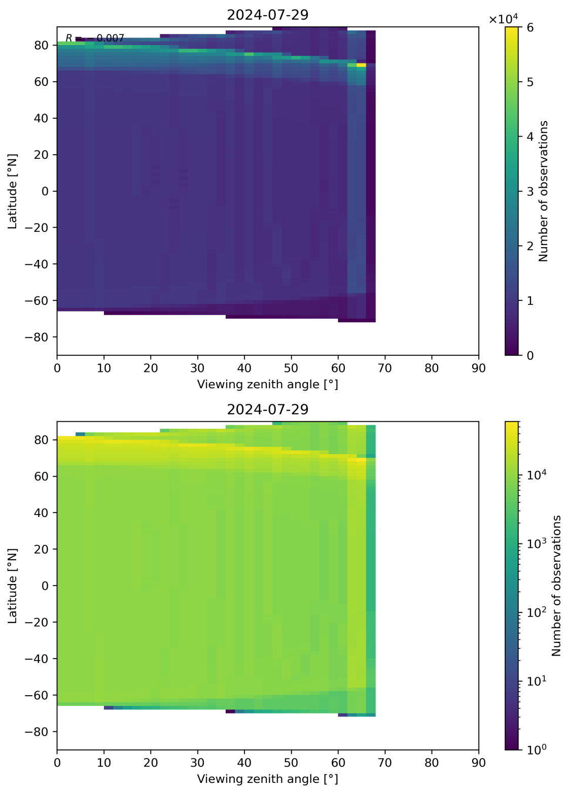
Figure 49: Scatter density plot of “Viewing zenith angle” against “Latitude” for 2024-07-28 to 2024-07-30.
