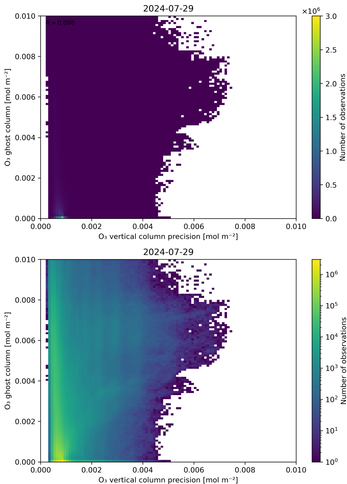
Figure 43: Scatter density plot of “ \text{O}_3 vertical column precision” against “ \text{O}_3 ghost column” for 2024-07-28 to 2024-07-30.
