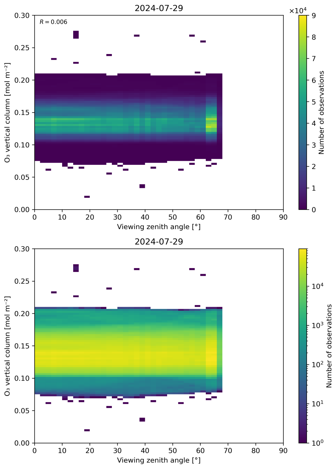
Figure 52: Scatter density plot of “Viewing zenith angle” against “O 3 vertical column” for 2024-07-28 to 2024-07-30.
