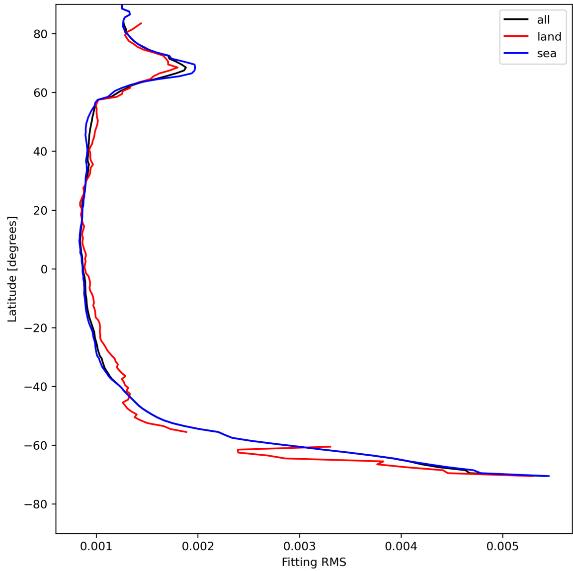
Figure 16: Zonal average of “Fitting RMS” for 2024-07-28 to 2024-07-30.
