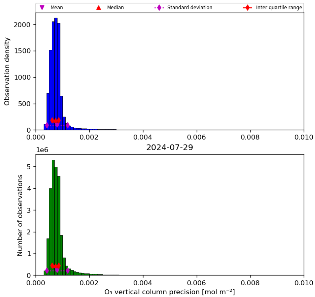
Figure 22: Histogram of “O 3 vertical column precision” for 2024-07-28 to 2024-07-30
