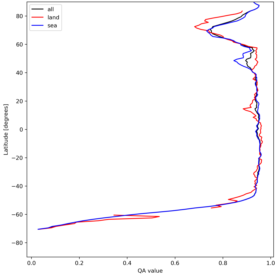
Figure 13: Zonal average of “QA value” for 2024-07-28 to 2024-07-30.
