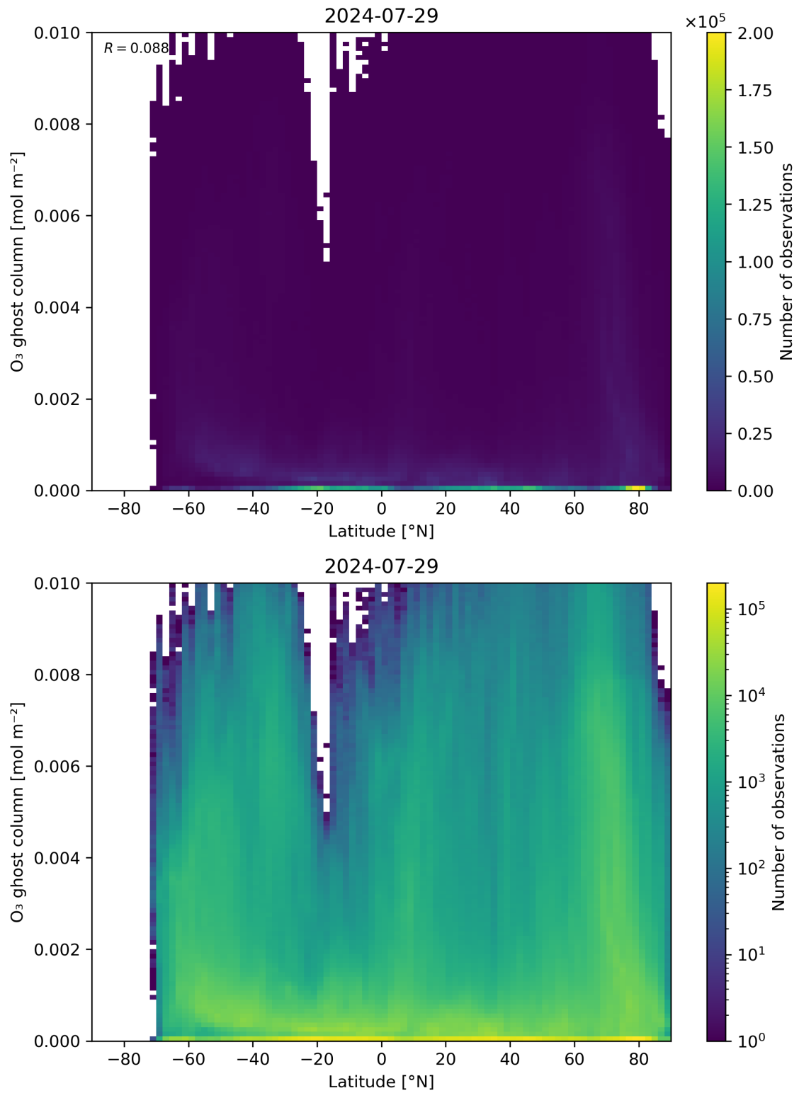
Figure 35: Scatter density plot of “Latitude” against “O 3 ghost column” for 2024-07-28 to 2024-07-30.
