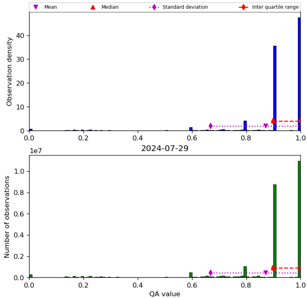
Figure 20: Histogram of “QA value” for 2024-07-28 to 2024-07-30
