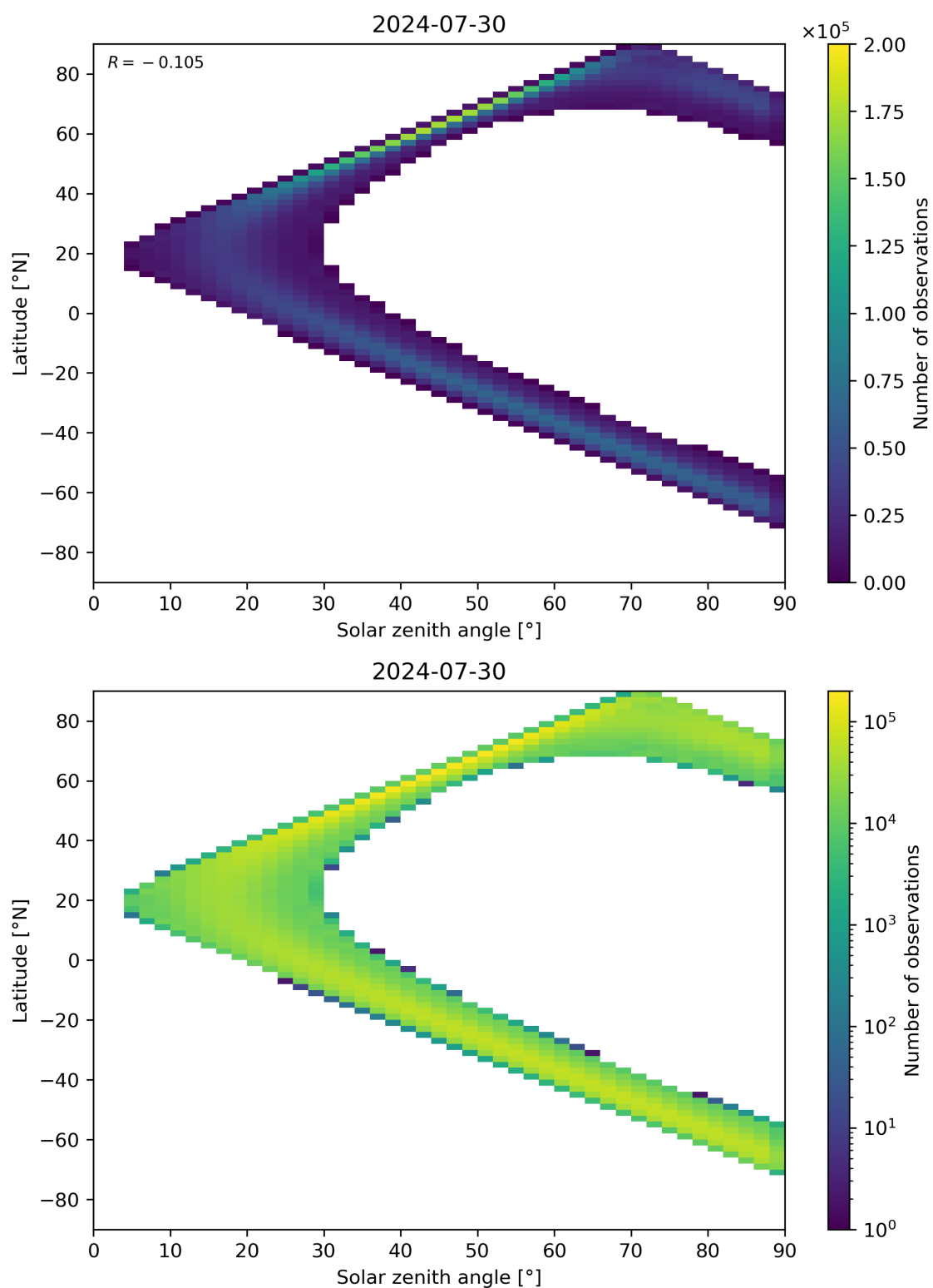
Figure 44: Scatter density plot of “Solar zenith angle” against “Latitude” for 2024-07-29 to 2024-07-31.
