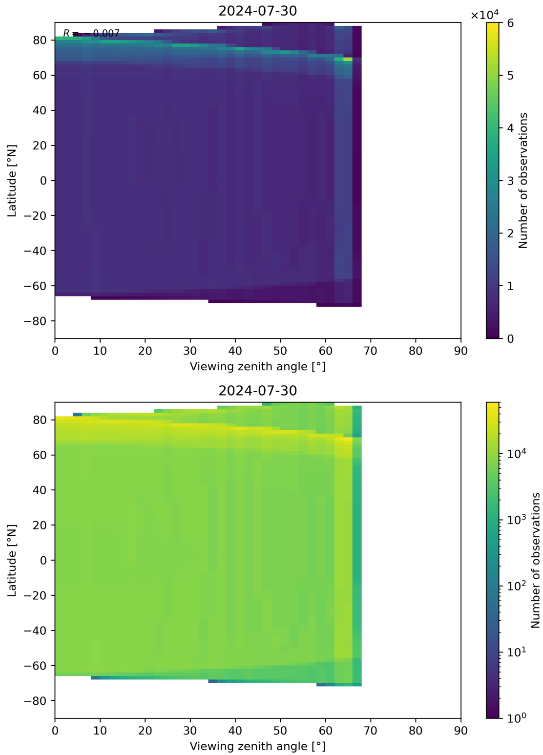
Figure 49: Scatter density plot of “Viewing zenith angle” against “Latitude” for 2024-07-29 to 2024-07-31.
