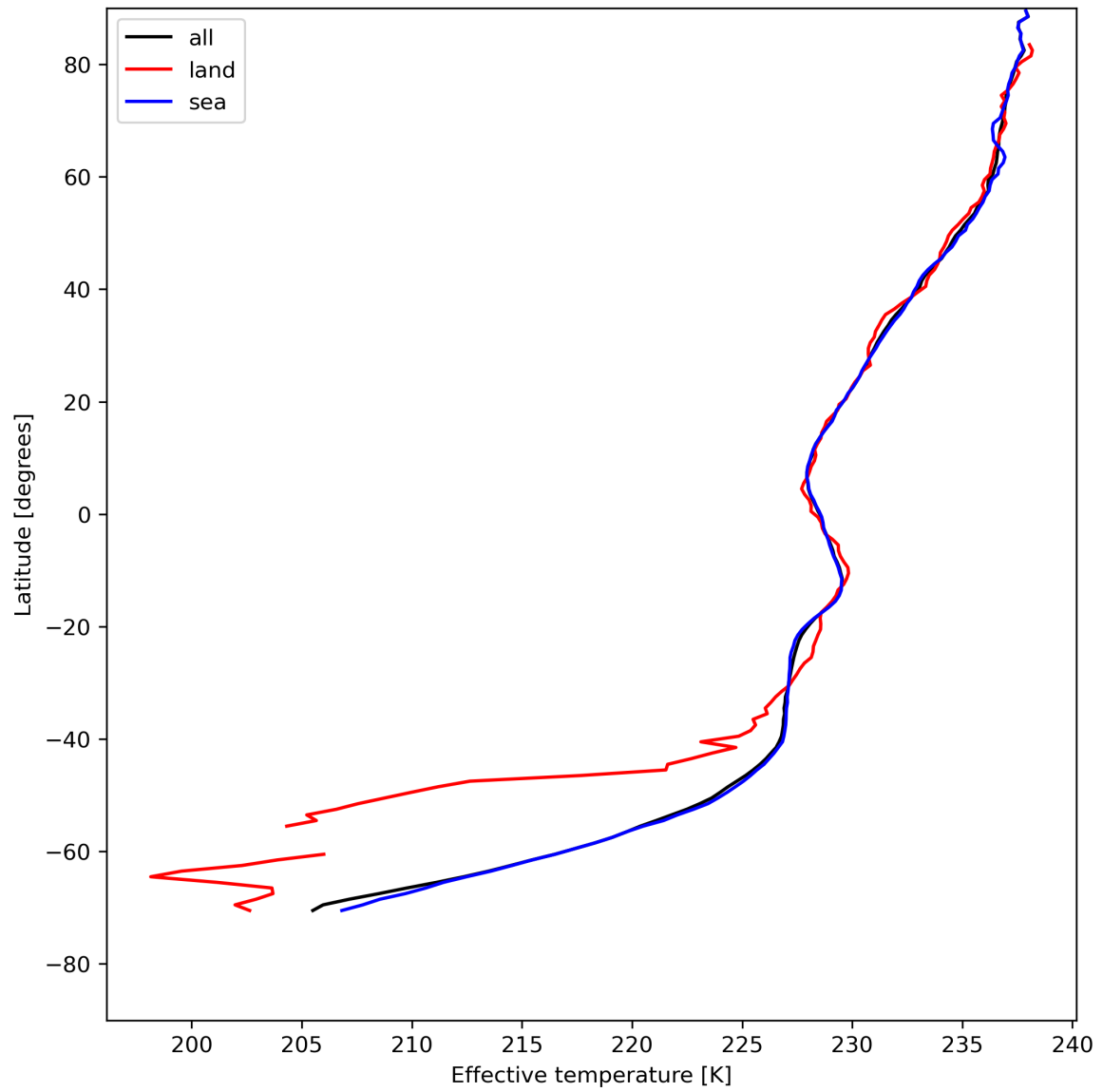
Figure 17: Zonal average of "Effective temperature" for 2024-07-29 to 2024-07-31.
