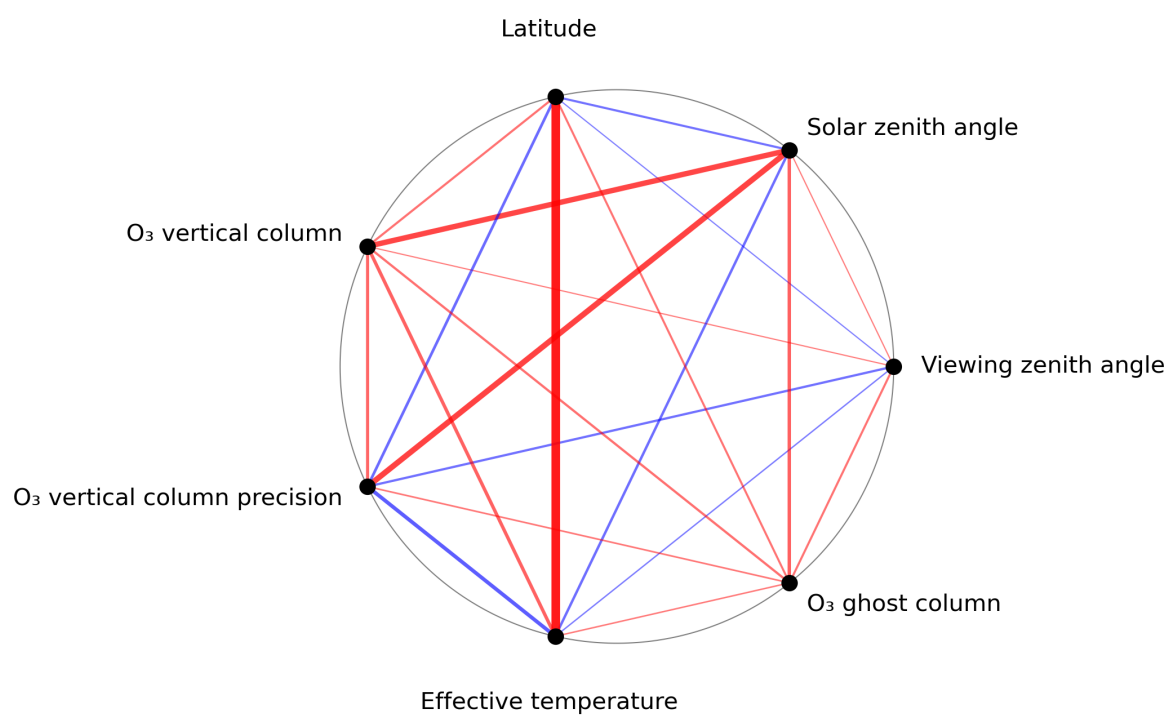
Figure 1: Map of correlation graph for 2024-07-29 to 2024-07-31.
