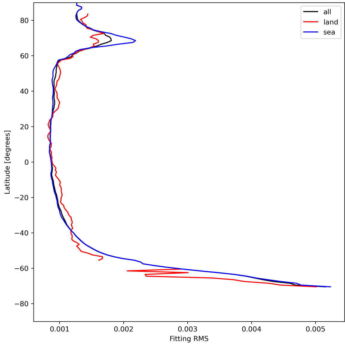
Figure 16: Zonal average of “Fitting RMS” for 2024-07-29 to 2024-07-31.
