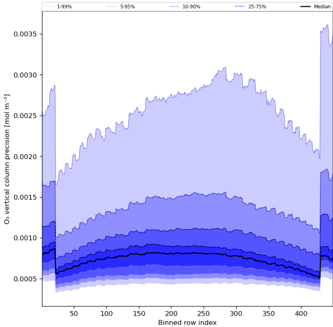
Figure 29: Along track statistics of “O 3 vertical column precision” for 2024-07-29 to 2024-07-31
