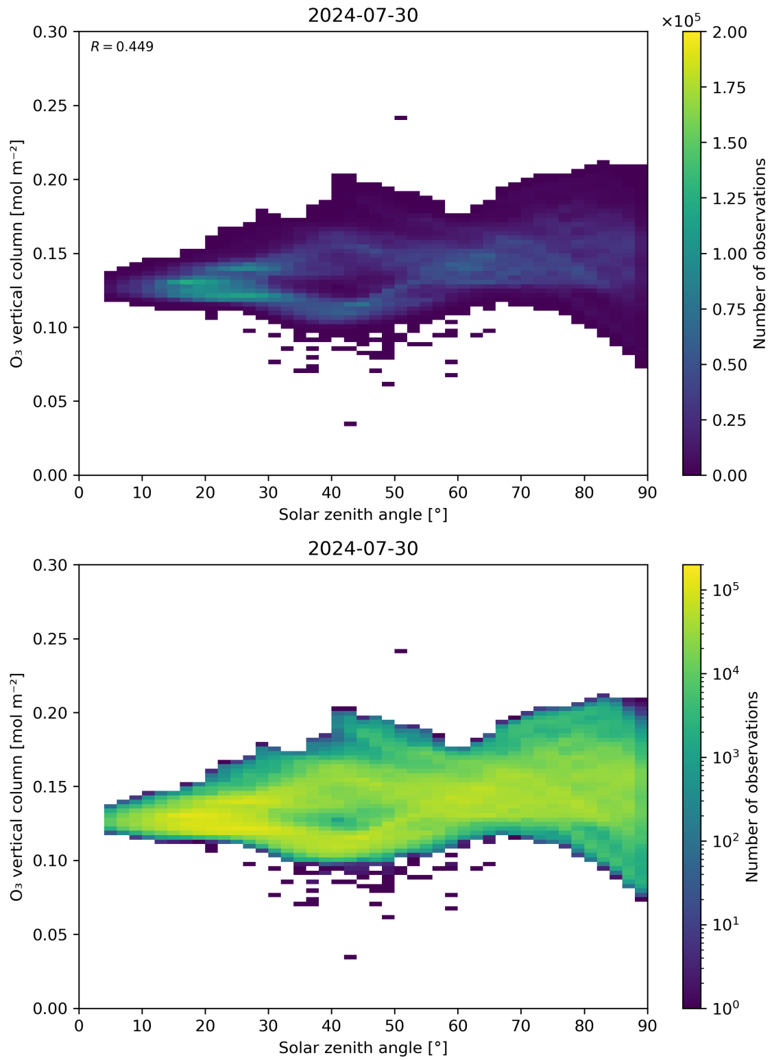
Figure 47: Scatter density plot of “Solar zenith angle” against “O 3 vertical column” for 2024-07-29 to 2024-07-31.
