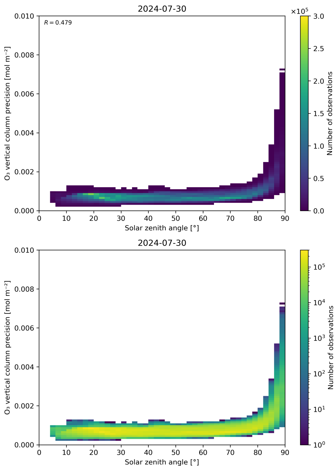
Figure 48: Scatter density plot of “Solar zenith angle” against “O 3 vertical column precision” for 2024-07-29 to 2024-07-31.
