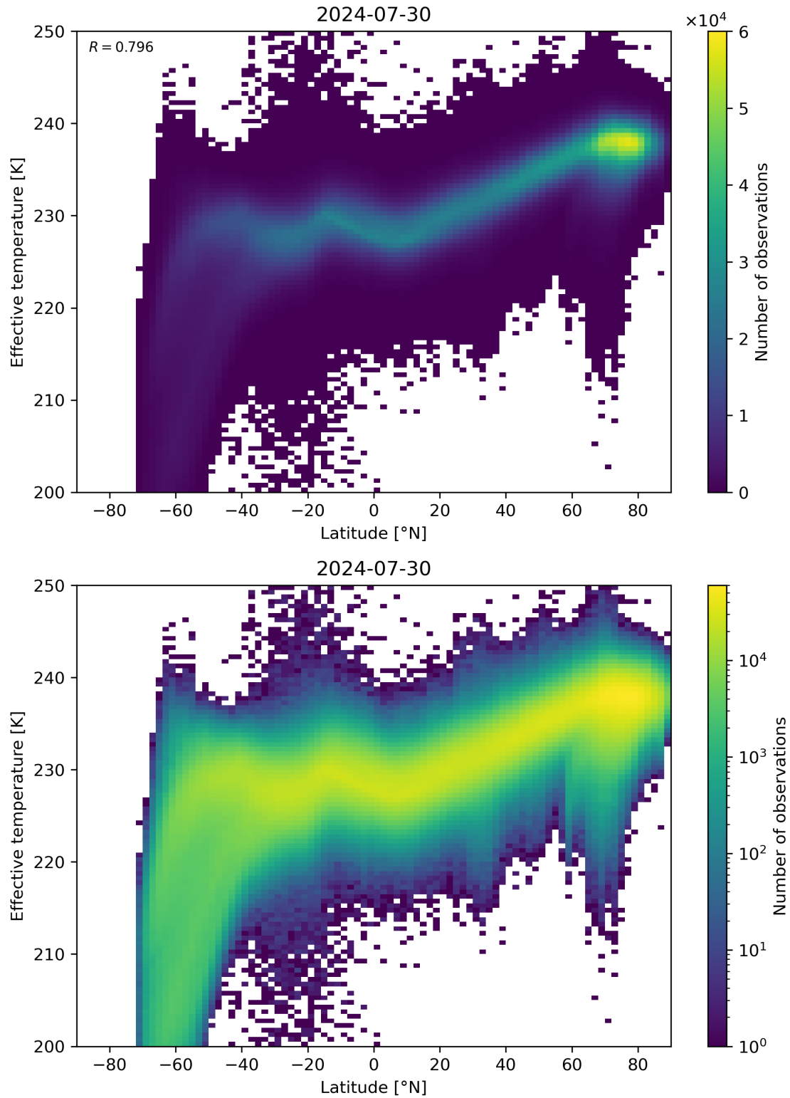
Figure 34: Scatter density plot of “Latitude” against “Effective temperature” for 2024-07-29 to 2024-07-31.
