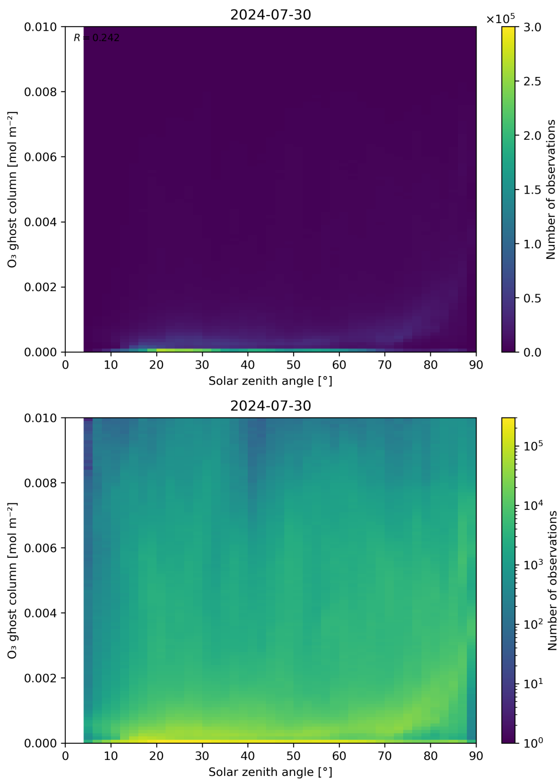
Figure 46: Scatter density plot of “Solar zenith angle” against “O 3 ghost column” for 2024-07-29 to 2024-07-31.
