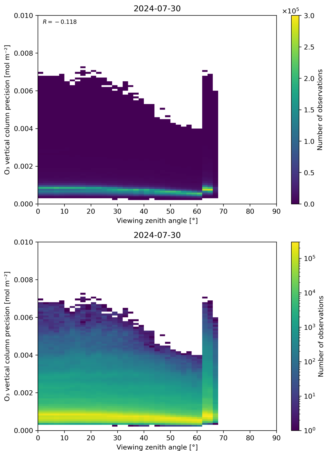
Figure 53: Scatter density plot of “Viewing zenith angle” against “O 3 vertical column precision” for 2024-07-29 to 2024-07-31.
