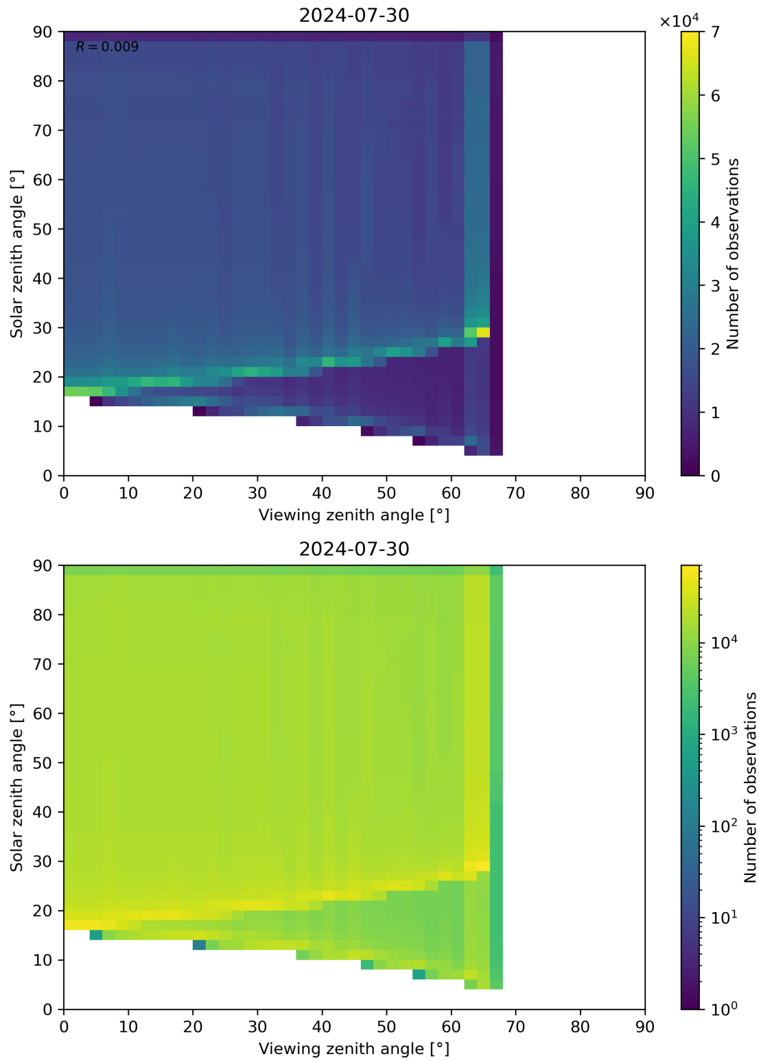
Figure 54: Scatter density plot of “Viewing zenith angle” against “Solar zenith angle” for 2024-07-29 to 2024-07-31.
