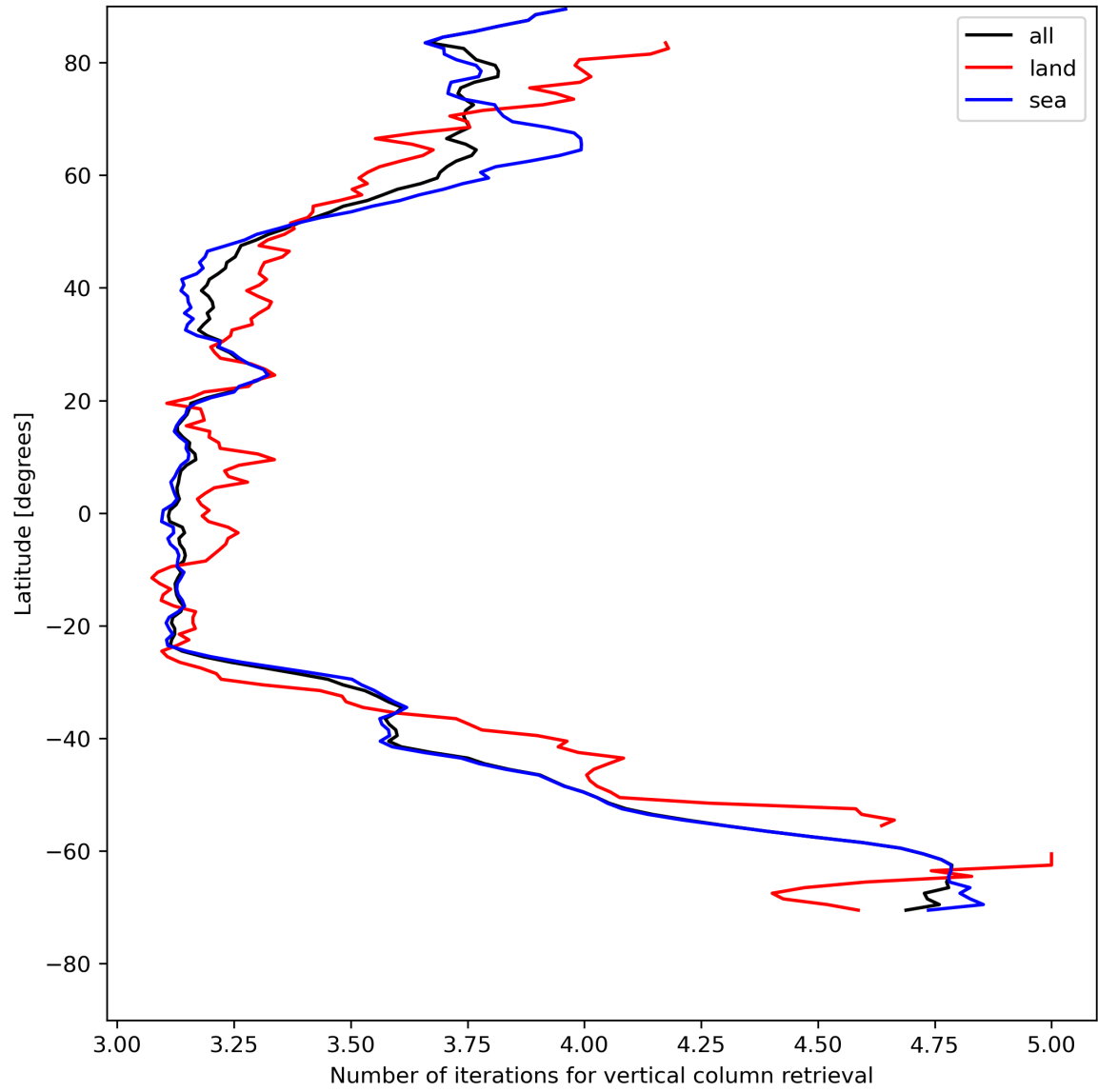
Figure 19: Zonal average of “Number of iterations for vertical column retrieval” for 2024-07-29 to 2024-07-31.
