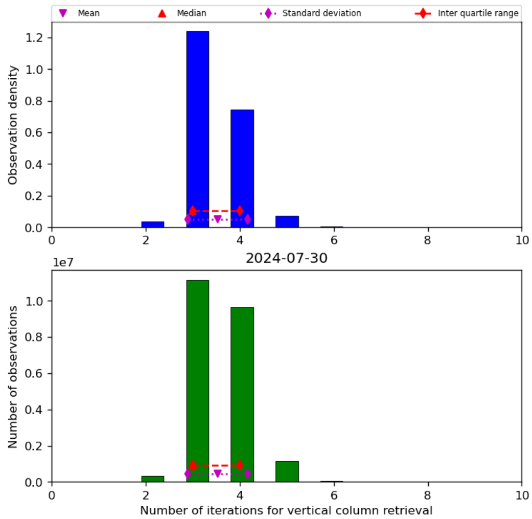
Figure 26: Histogram of “Number of iterations for vertical column retrieval” for 2024-07-29 to 2024-07-31
