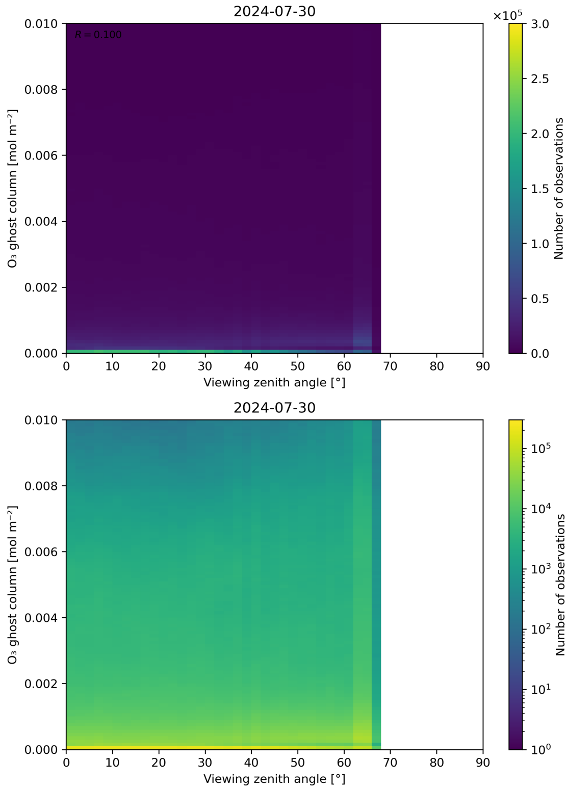
Figure 51: Scatter density plot of “Viewing zenith angle” against “O 3 ghost column” for 2024-07-29 to 2024-07-31.
