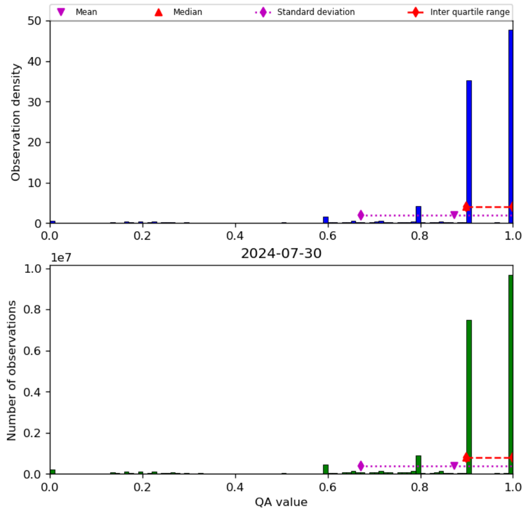
Figure 20: Histogram of “QA value” for 2024-07-29 to 2024-07-31
