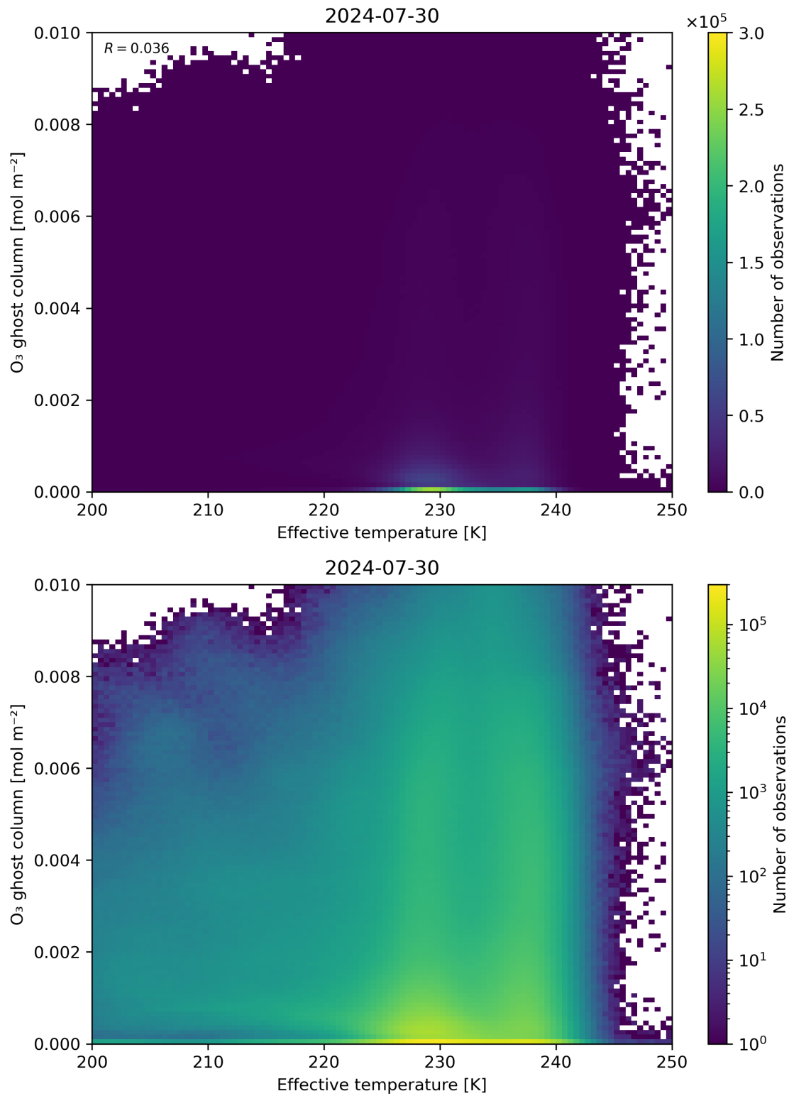
Figure 38: Scatter density plot of “Effective temperature” against “O 3 ghost column” for 2024-07-29 to 2024-07-31.
