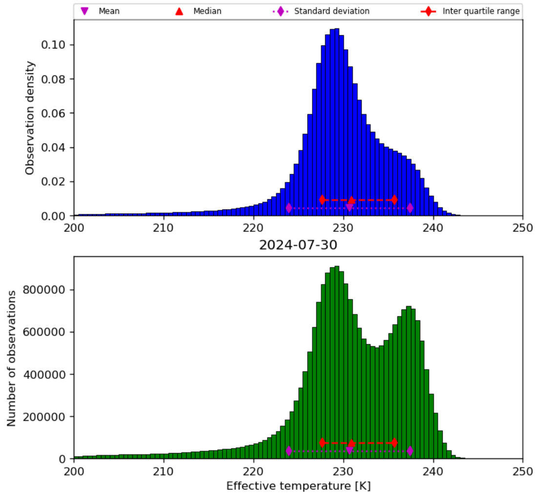
Figure 24: Histogram of “Effective temperature” for 2024-07-29 to 2024-07-31
