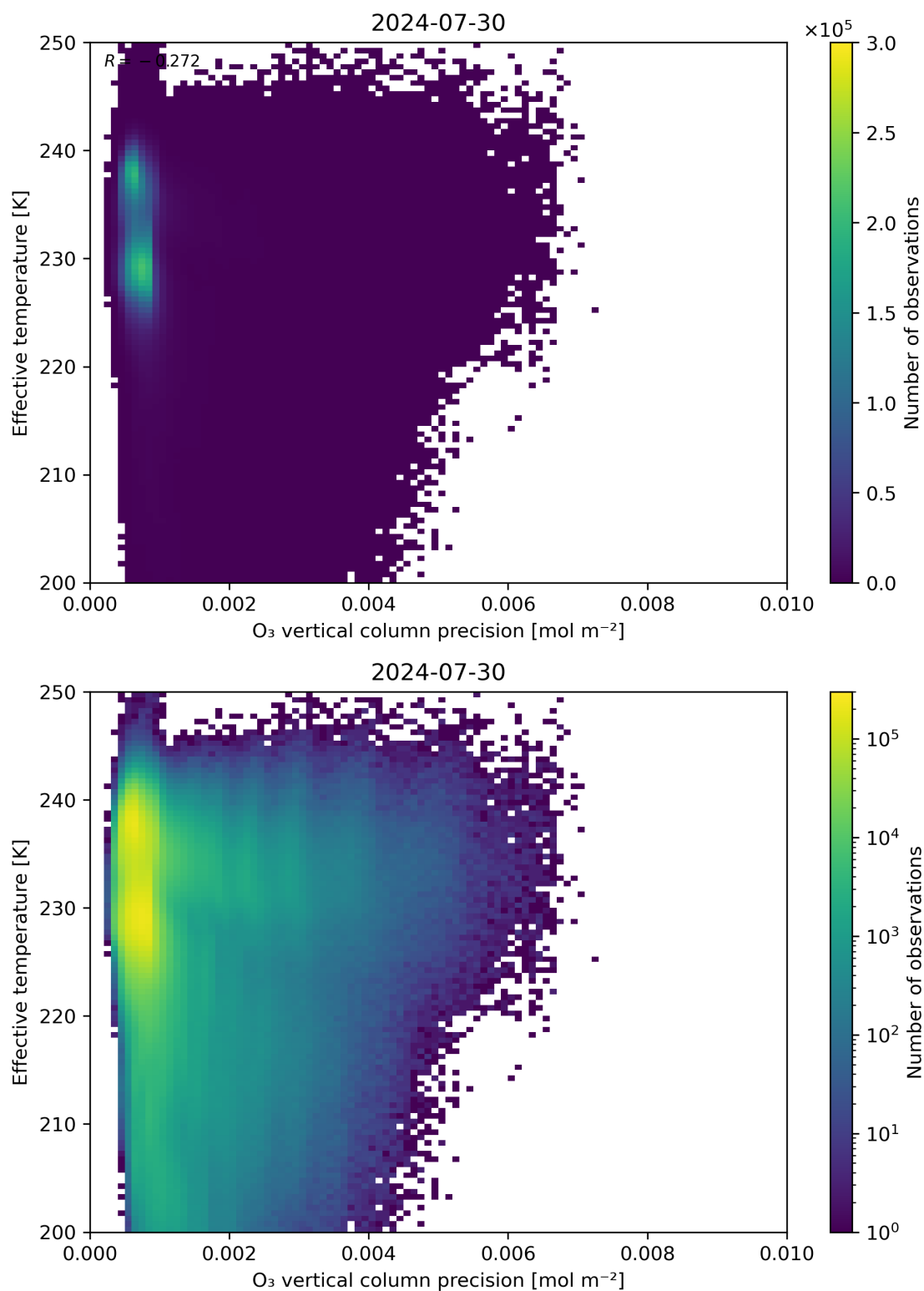
Figure 42: Scatter density plot of “O 3 vertical column precision” against “Effective temperature” for 2024-07-29 to 2024-07-31.
