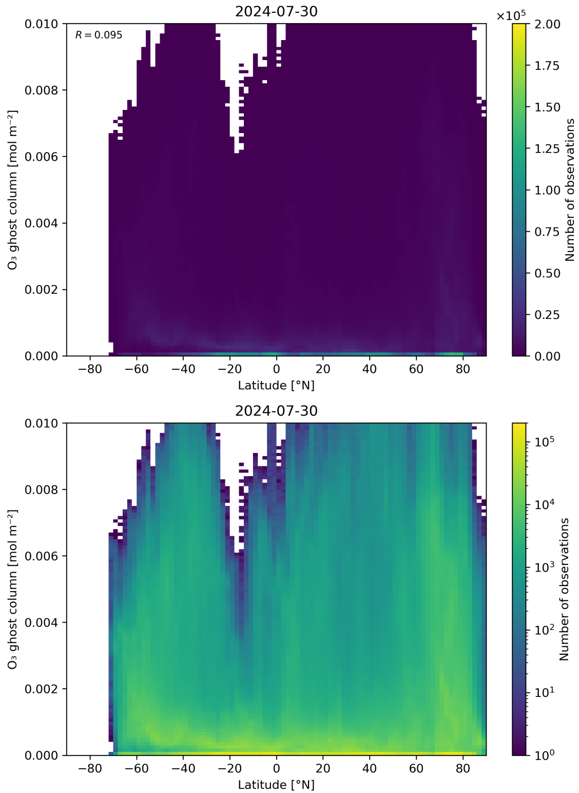
Figure 35: Scatter density plot of “Latitude” against “O 3 ghost column” for 2024-07-29 to 2024-07-31.
