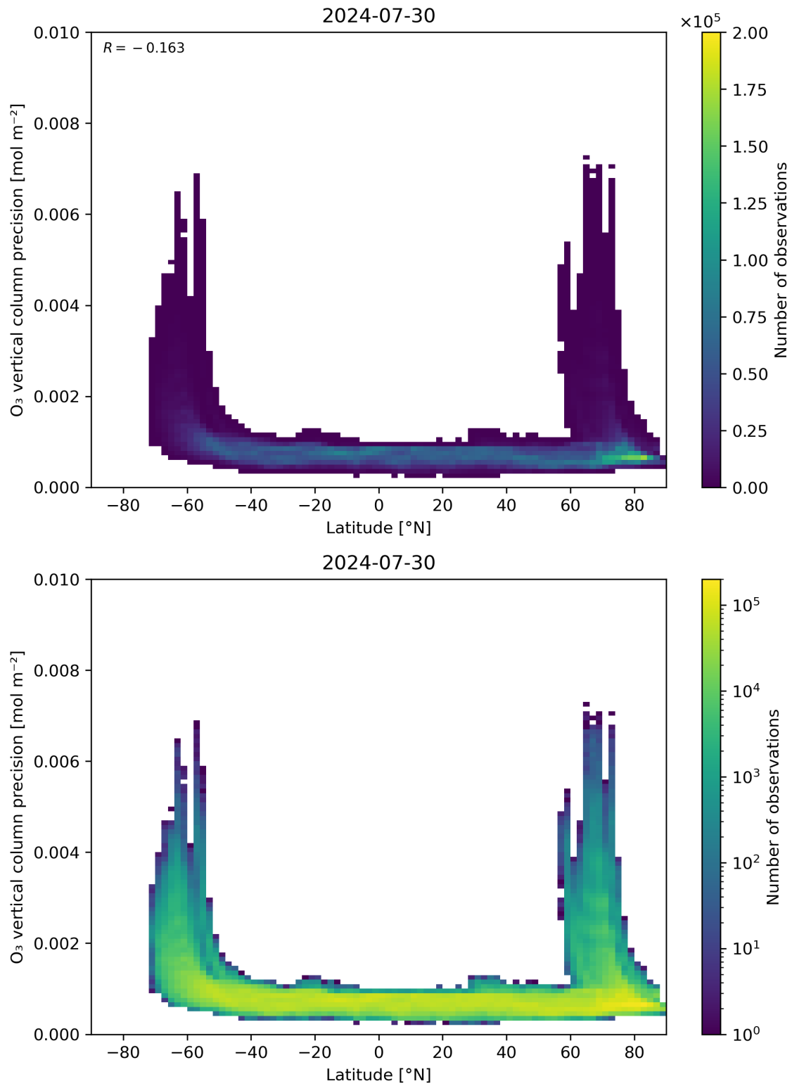
Figure 37: Scatter density plot of “Latitude” against “O 3 vertical column precision” for 2024-07-29 to 2024-07-31.
