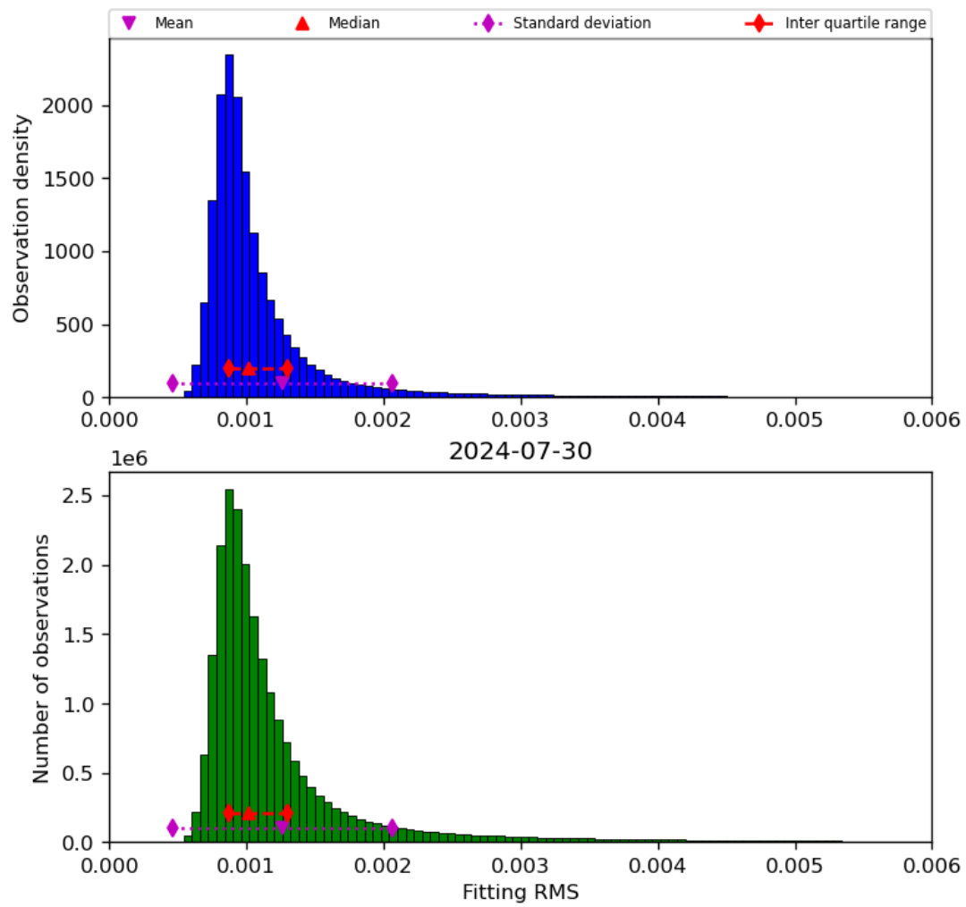
Figure 23: Histogram of “Fitting RMS” for 2024-07-29 to 2024-07-31
