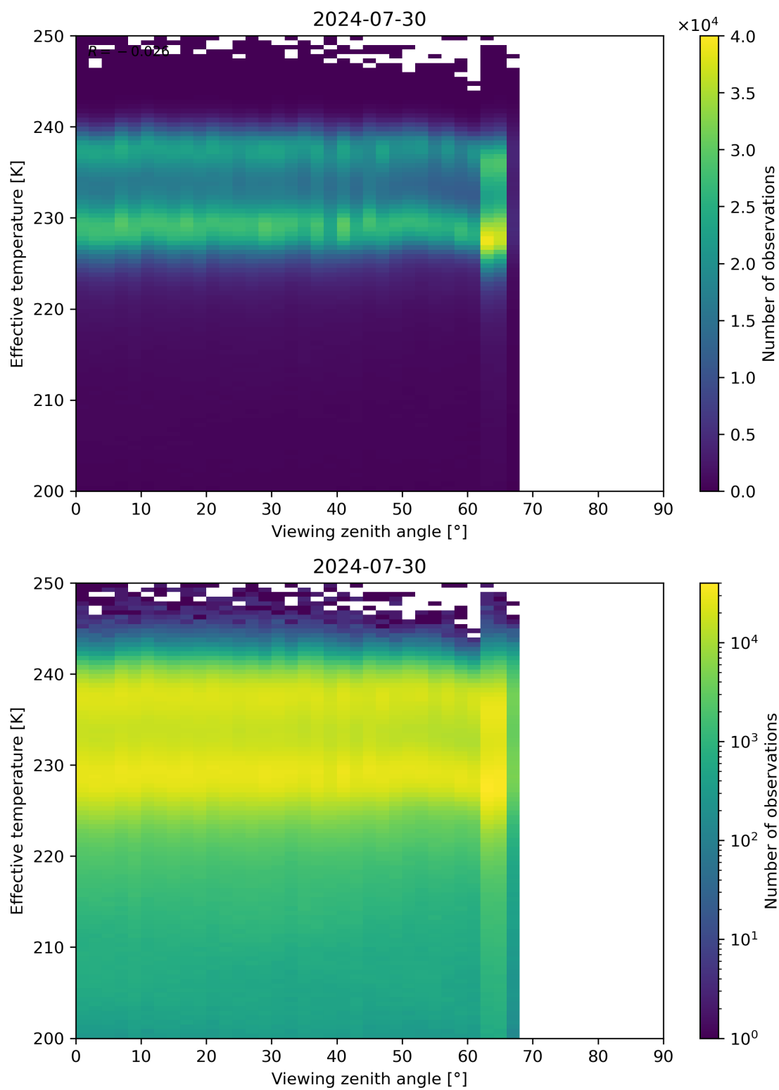
Figure 50: Scatter density plot of “Viewing zenith angle” against “Effective temperature” for 2024-07-29 to 2024-07-31.
