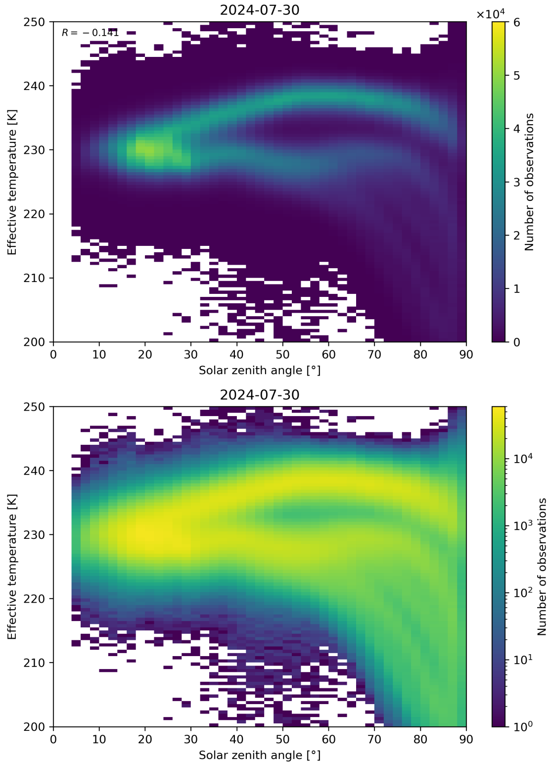
Figure 45: Scatter density plot of “Solar zenith angle” against “Effective temperature” for 2024-07-29 to 2024-07-31.
