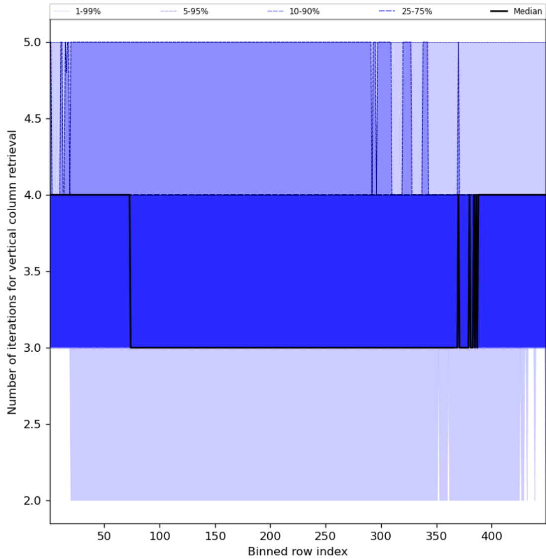
Figure 33: Along track statistics of “Number of iterations for vertical column retrieval” for 2024-07-29 to 2024-07-31
