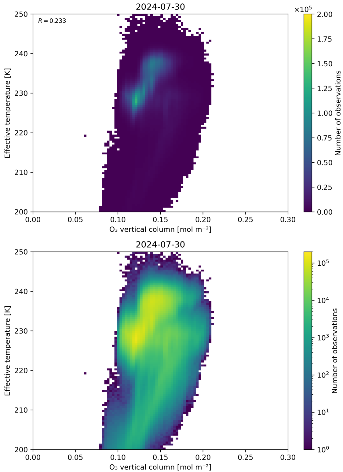
Figure 39: Scatter density plot of “O 3 vertical column” against “Effective temperature” for 2024-07-29 to 2024-07-31.
