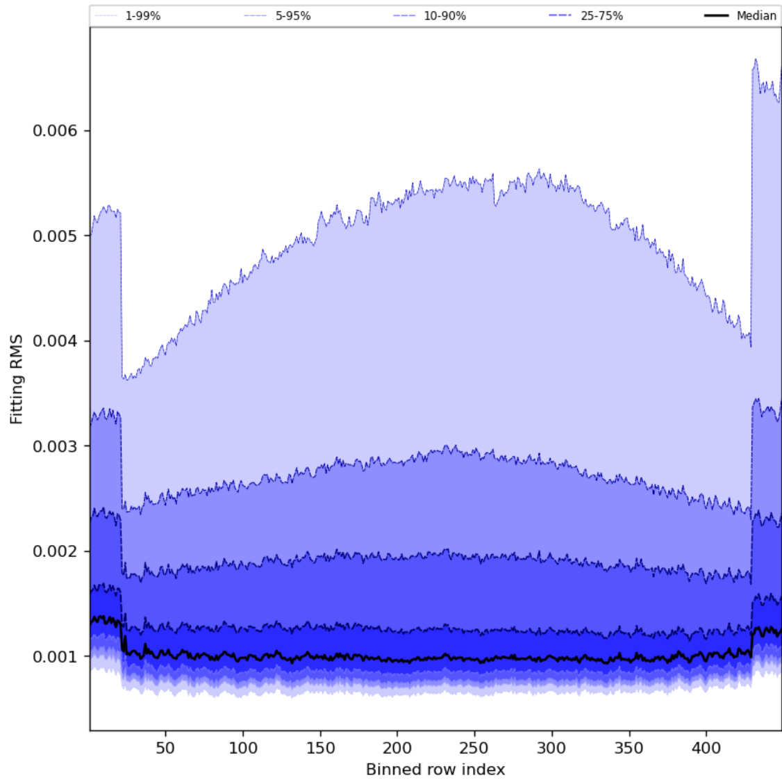
Figure 30: Along track statistics of “Fitting RMS” for 2024-07-29 to 2024-07-31
