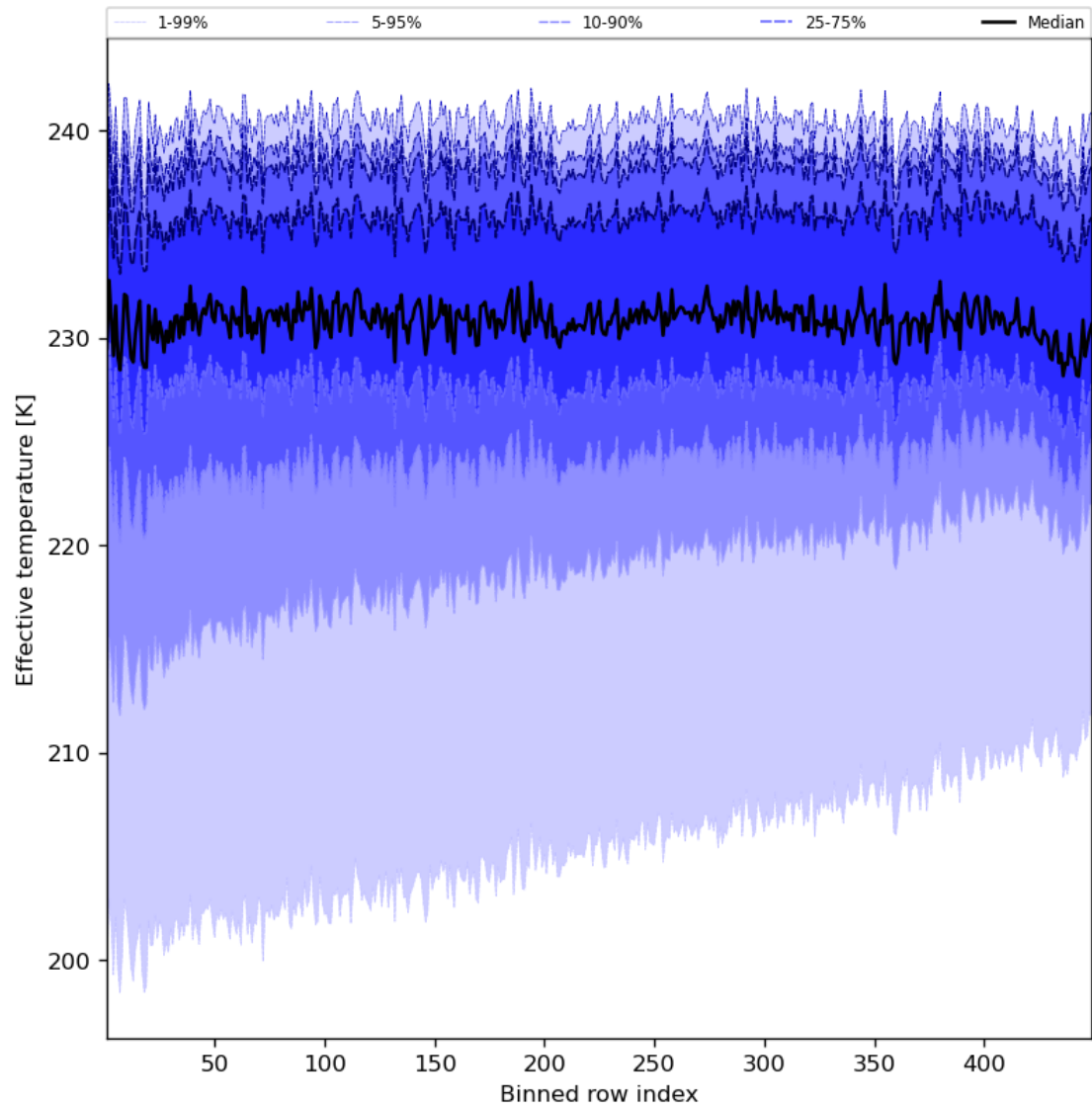
Figure 31: Along track statistics of “Effective temperature” for 2024-07-29 to 2024-07-31
