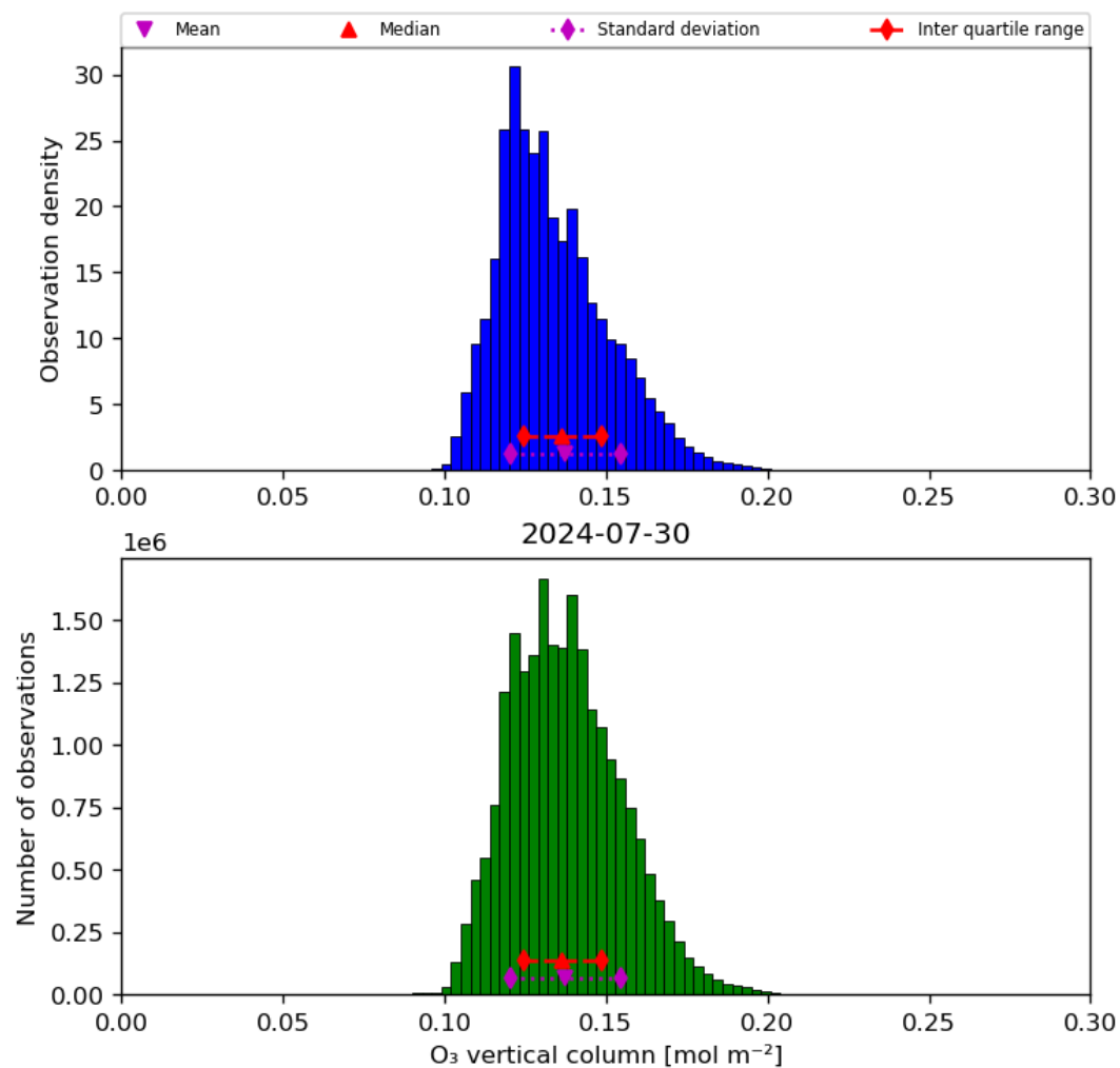
Figure 21: Histogram of “O 3 vertical column” for 2024-07-29 to 2024-07-31
