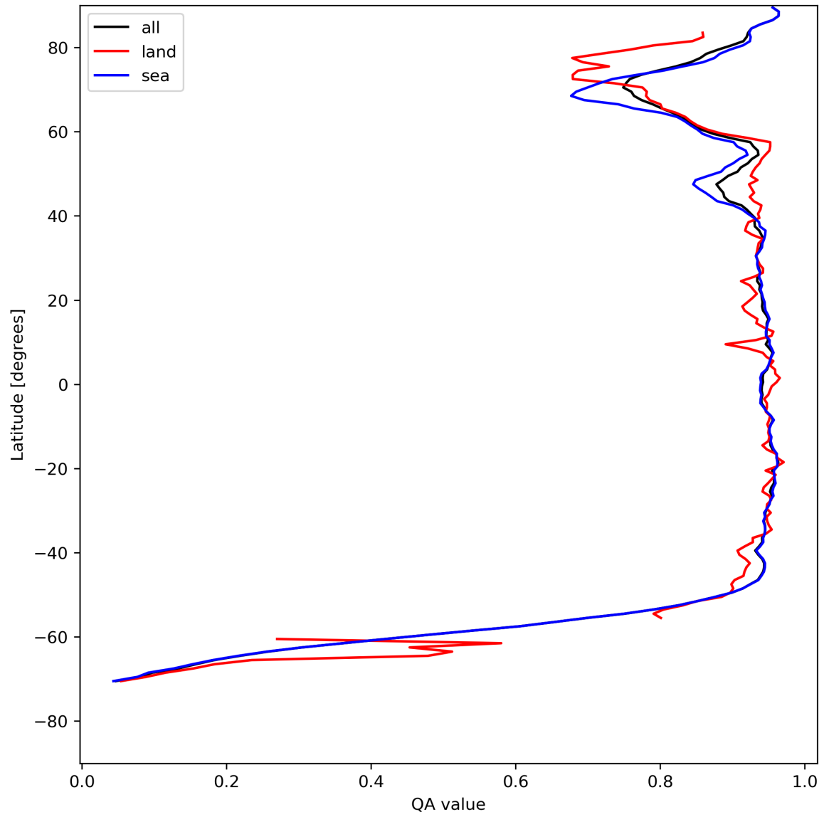
Figure 13: Zonal average of “QA value” for 2024-07-29 to 2024-07-31.
