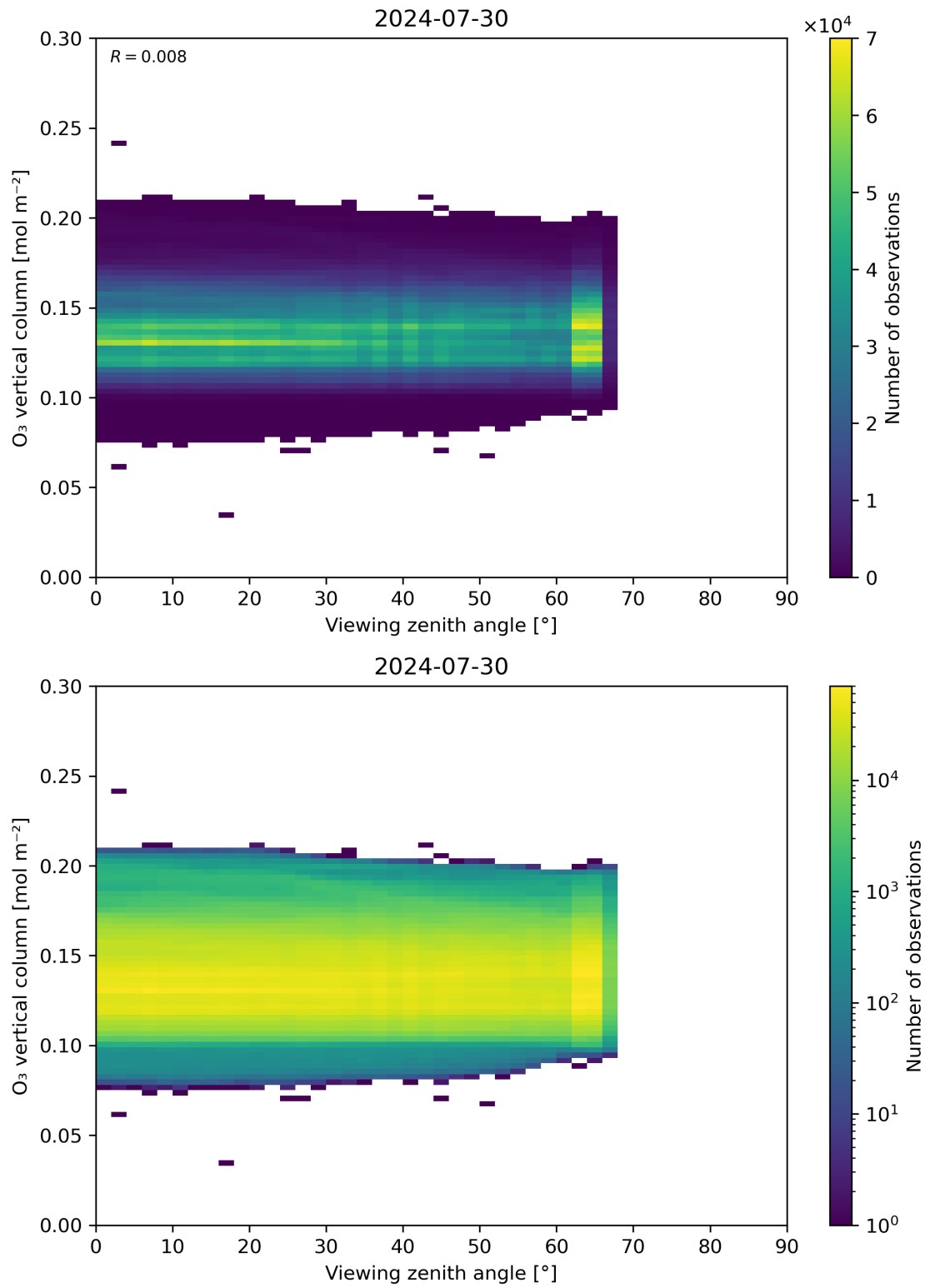
Figure 52: Scatter density plot of “Viewing zenith angle” against “O 3 vertical column” for 2024-07-29 to 2024-07-31.
