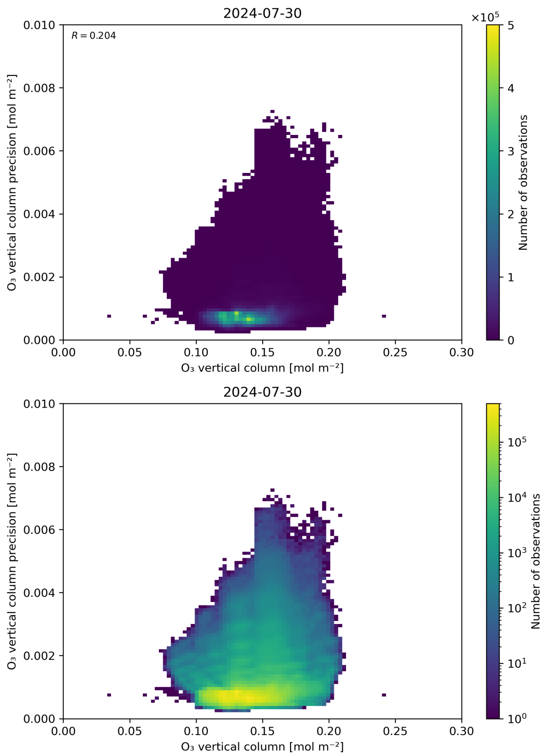
Figure 41: Scatter density plot of “O 3 vertical column” against “O 3 vertical column precision” for 2024-07-29 to 2024-07-31.
