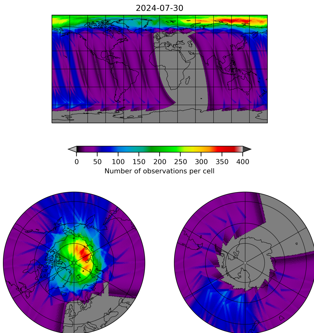
Figure 12: Map of the number of observations for 2024-07-29 to 2024-07-31
