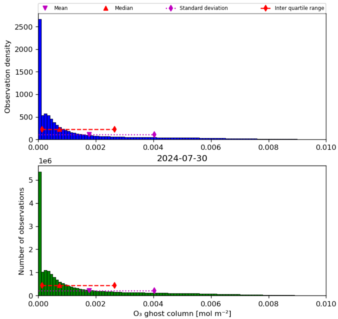
Figure 25: Histogram of “O 3 ghost column” for 2024-07-29 to 2024-07-31
