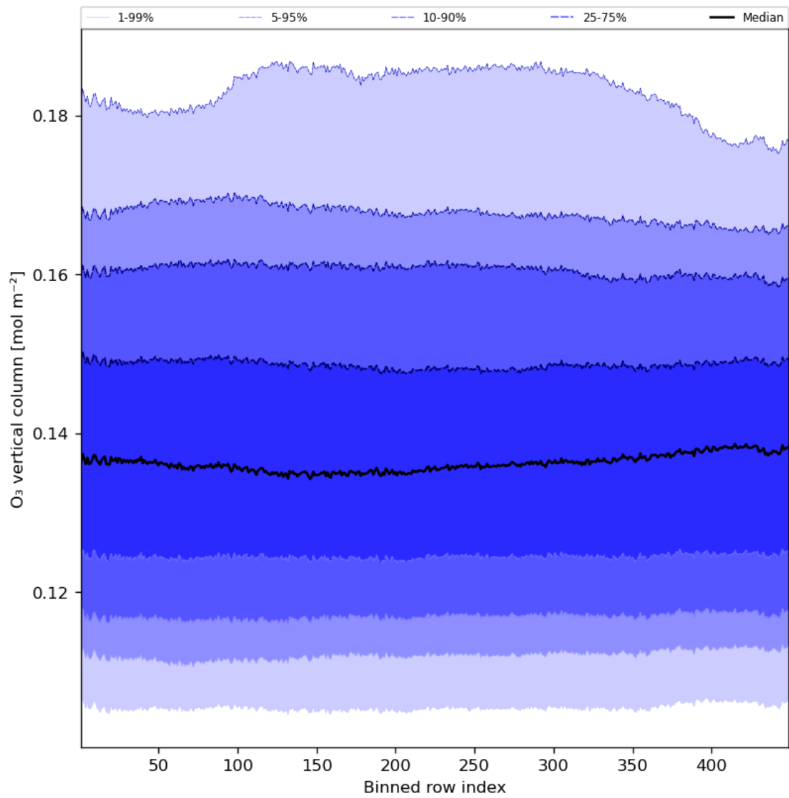
Figure 28: Along track statistics of “O 3 vertical column” for 2024-07-29 to 2024-07-31
