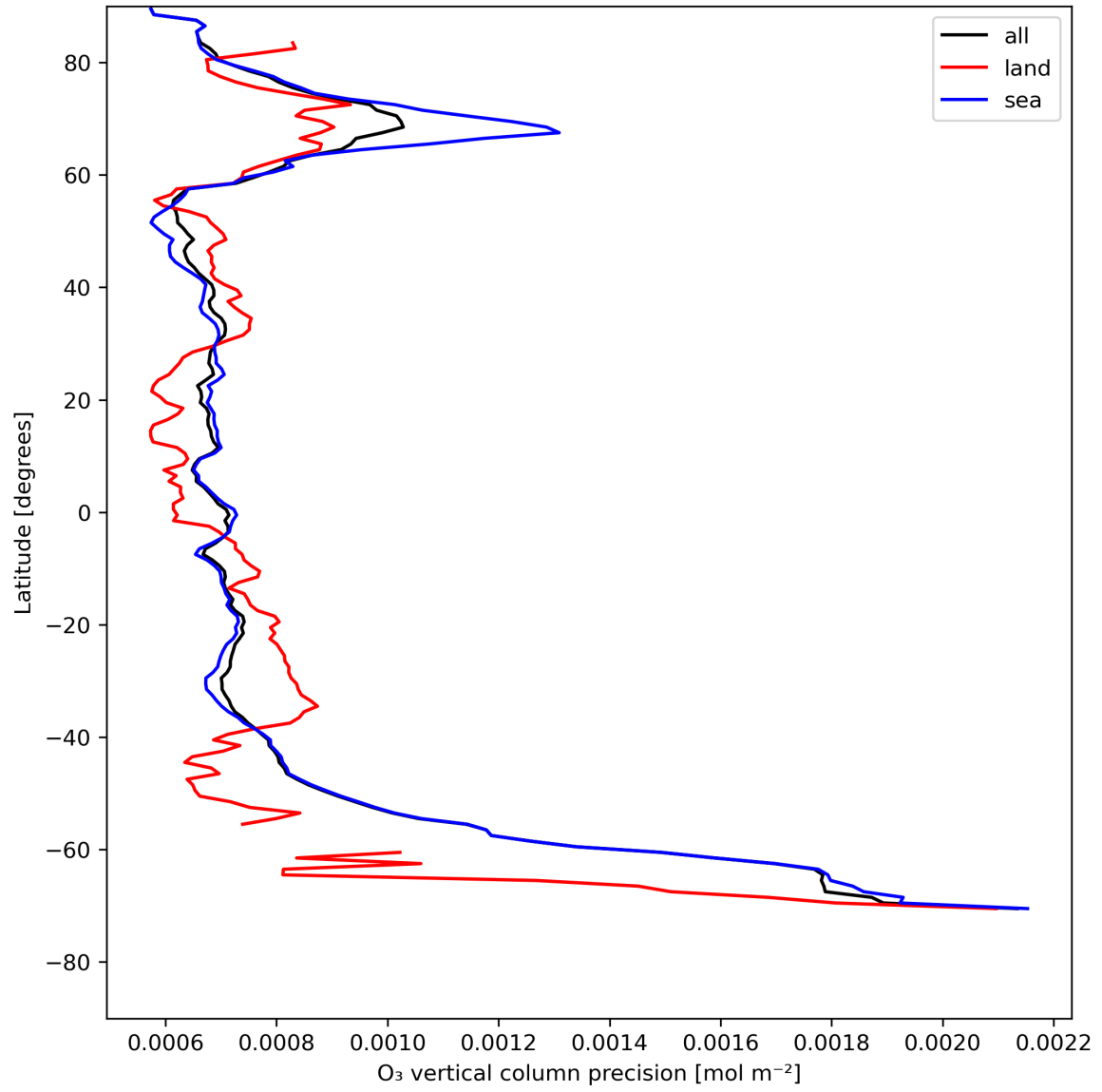
Figure 15: Zonal average of “O 3 vertical column precision” for 2024-07-29 to 2024-07-31.
