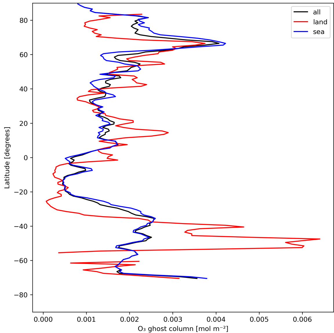
Figure 18: Zonal average of “O 3 ghost column” for 2024-07-29 to 2024-07-31.
