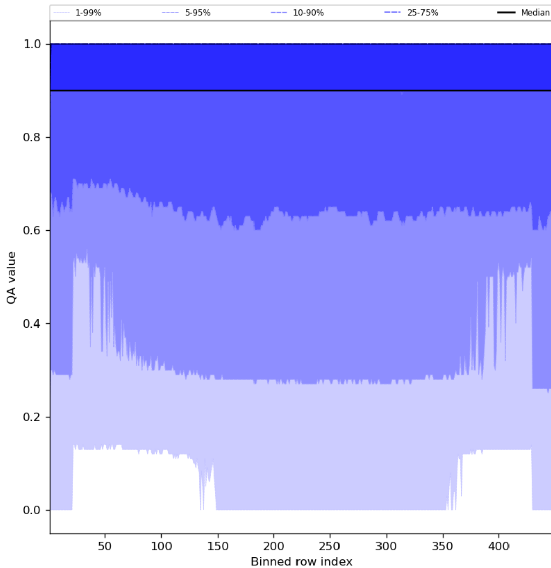
Figure 27: Along track statistics of “QA value” for 2024-07-29 to 2024-07-31
