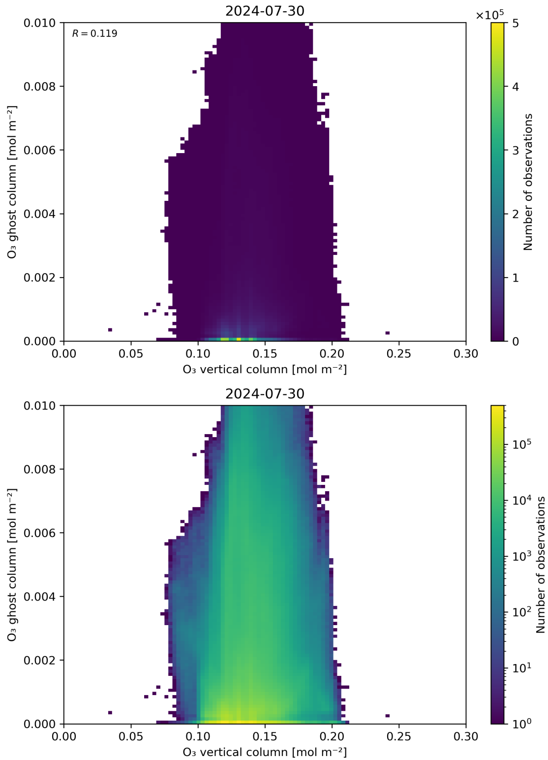
Figure 40: Scatter density plot of “O 3 vertical column” against “O 3 ghost column” for 2024-07-29 to 2024-07-31.
