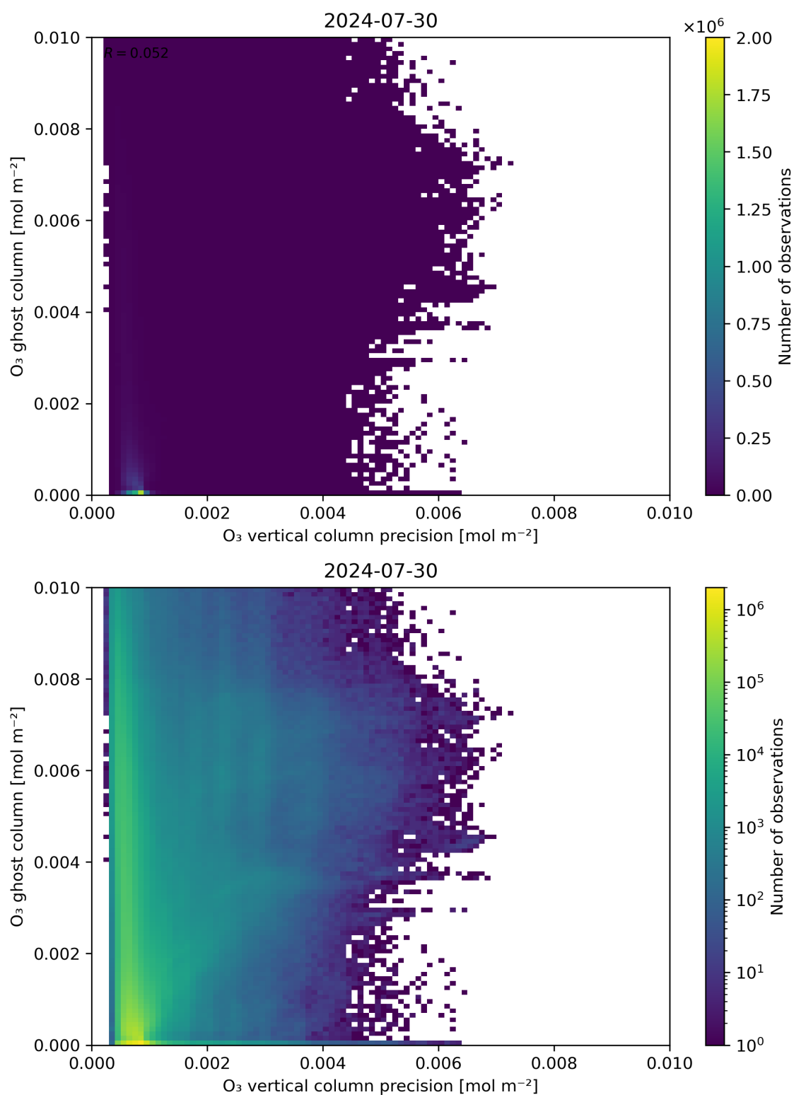
Figure 43: Scatter density plot of “ O_3 vertical column precision” against “ O_3 ghost column” for 2024-07-29 to 2024-07-31.
