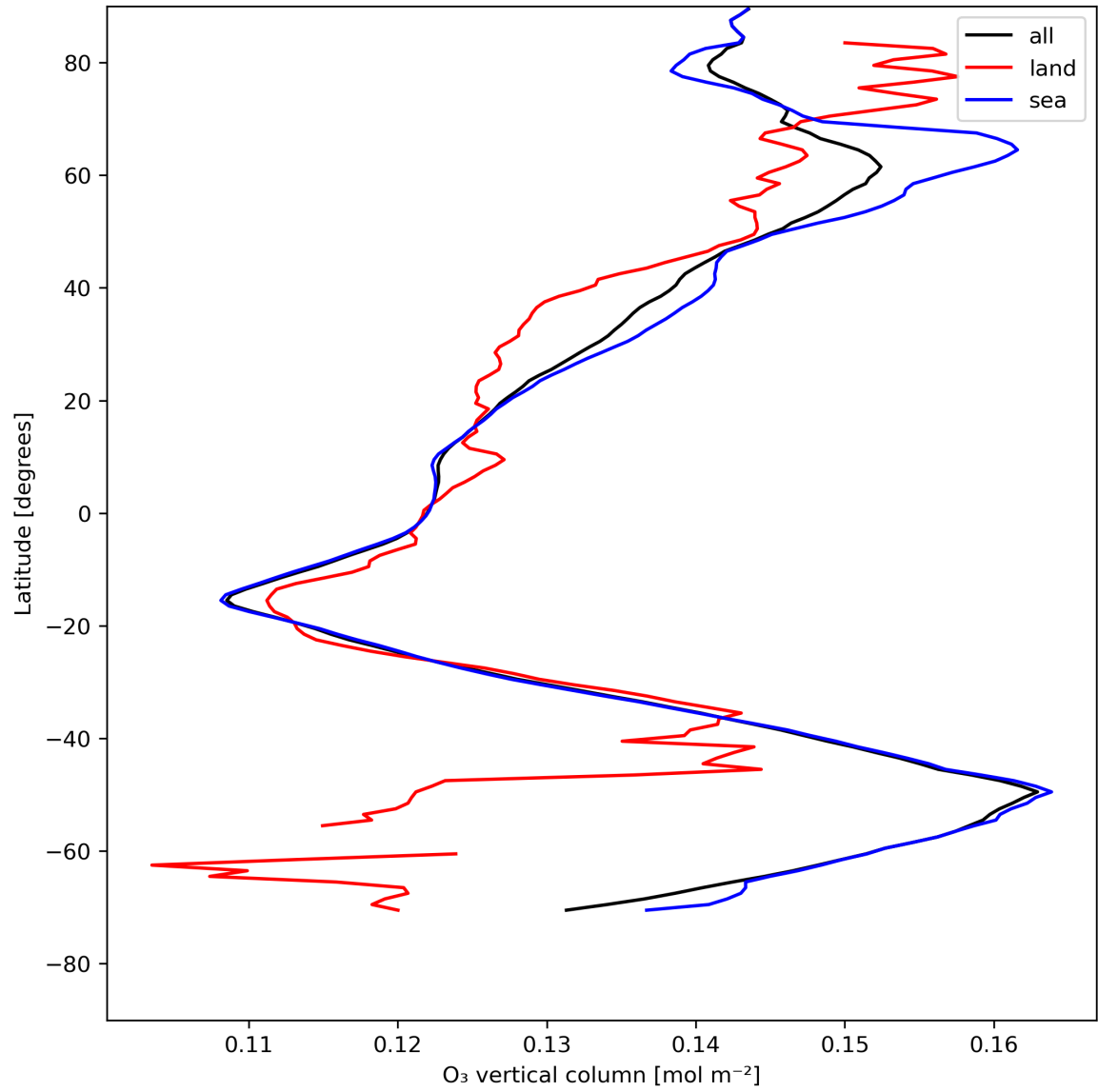
Figure 14: Zonal average of “O 3 vertical column” for 2024-07-29 to 2024-07-31.
