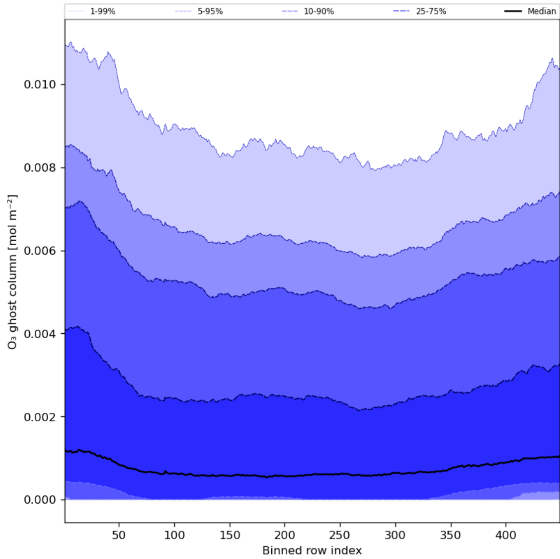
Figure 32: Along track statistics of “O 3 ghost column” for 2024-07-29 to 2024-07-31
