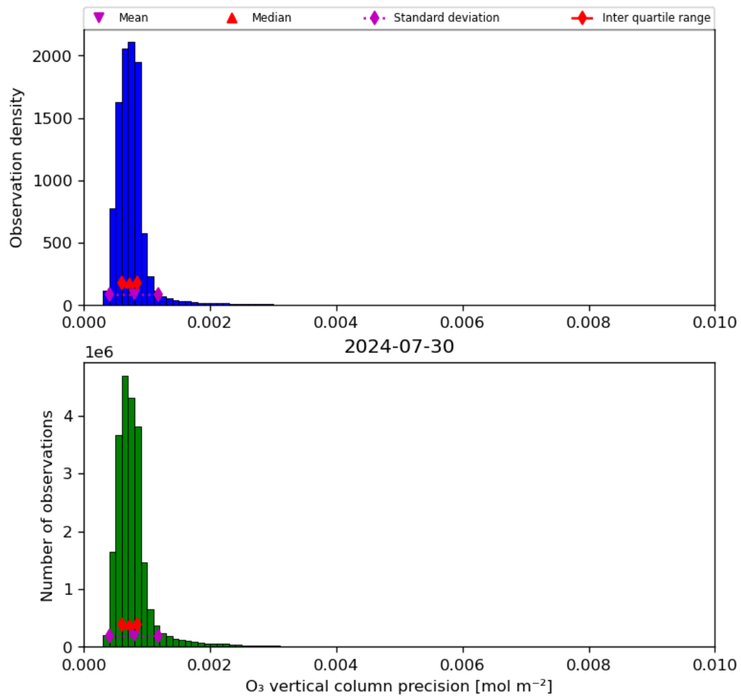
Figure 22: Histogram of “O 3 vertical column precision” for 2024-07-29 to 2024-07-31
