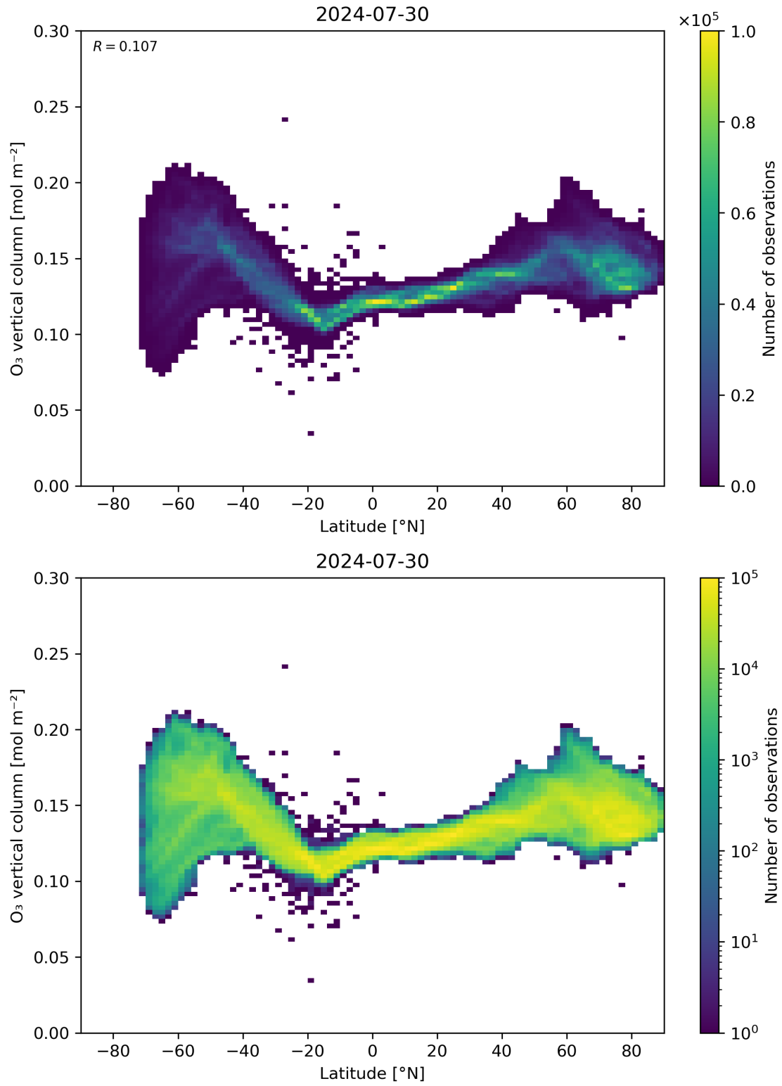
Figure 36: Scatter density plot of “Latitude” against “O 3 vertical column” for 2024-07-29 to 2024-07-31.
