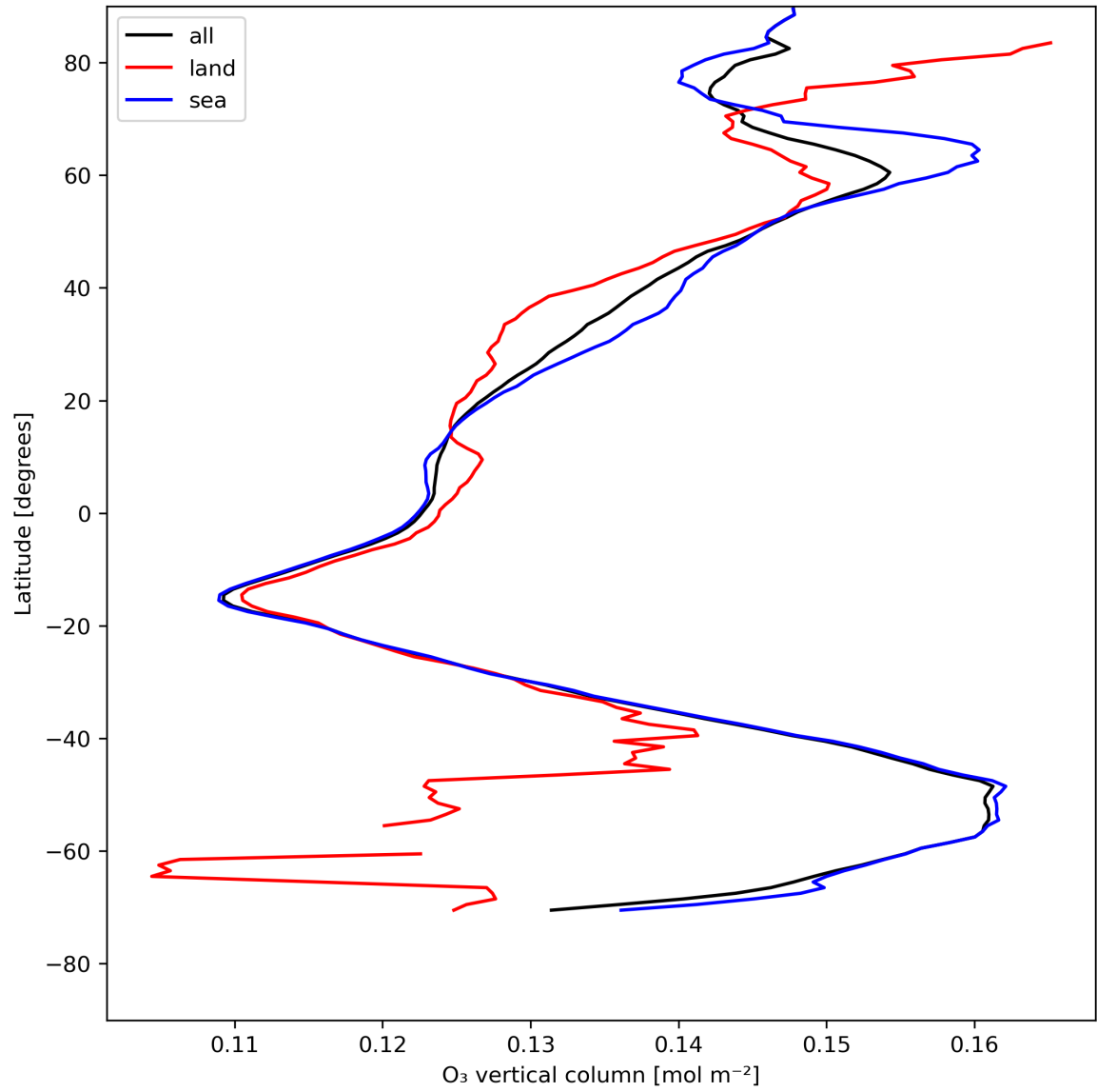
Figure 14: Zonal average of “O 3 vertical column” for 2024-07-31 to 2024-08-01.
