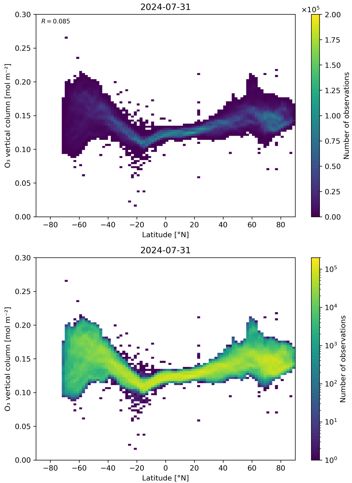
Figure 36: Scatter density plot of “Latitude” against “O 3 vertical column” for 2024-07-31 to 2024-08-01.
