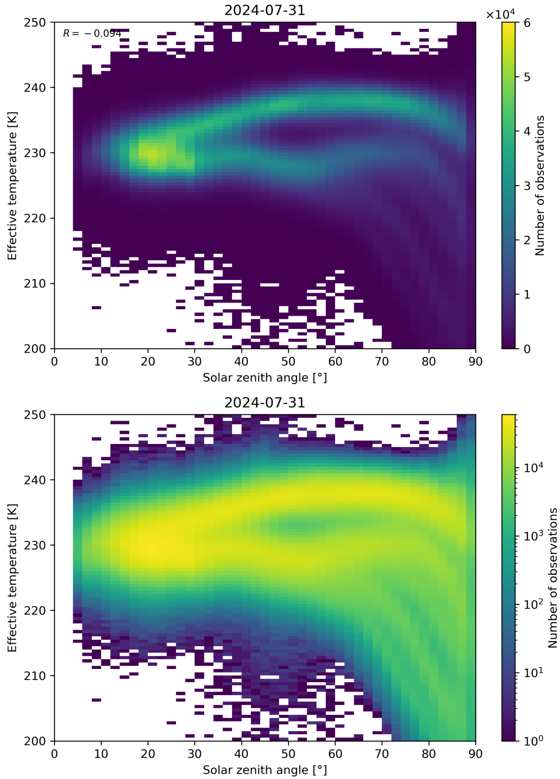
Figure 45: Scatter density plot of “Solar zenith angle” against “Effective temperature” for 2024-07-31 to 2024-08-01.
