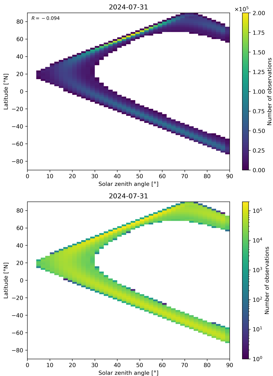
Figure 44: Scatter density plot of “Solar zenith angle” against “Latitude” for 2024-07-31 to 2024-08-01.
