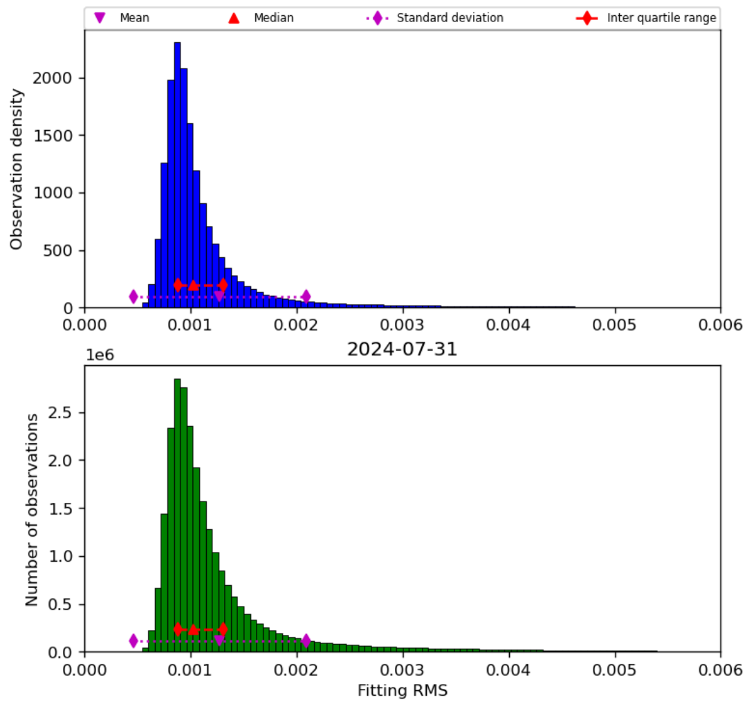
Figure 23: Histogram of “Fitting RMS” for 2024-07-31 to 2024-08-01
