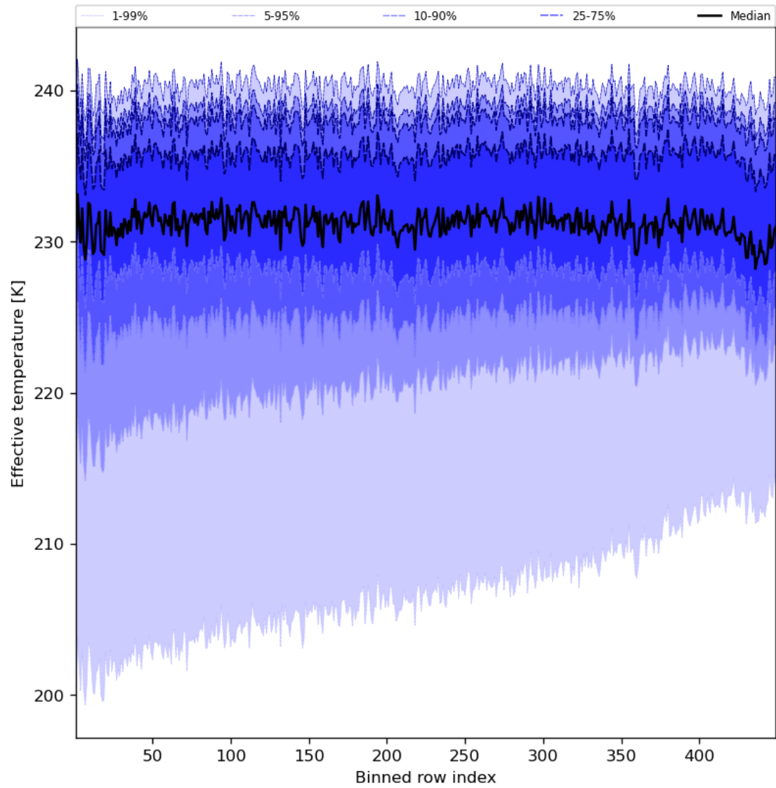
Figure 31: Along track statistics of “Effective temperature” for 2024-07-31 to 2024-08-01
