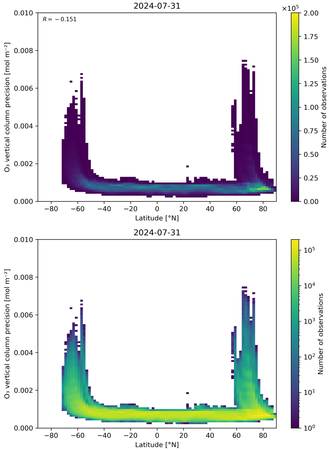
Figure 37: Scatter density plot of “Latitude” against “O 3 vertical column precision” for 2024-07-31 to 2024-08-01.
