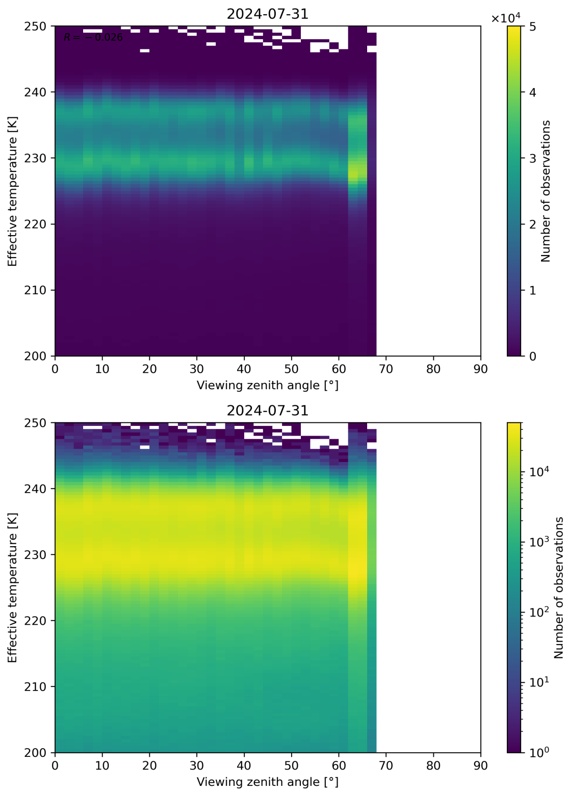
Figure 50: Scatter density plot of “Viewing zenith angle” against “Effective temperature” for 2024-07-31 to 2024-08-01.
