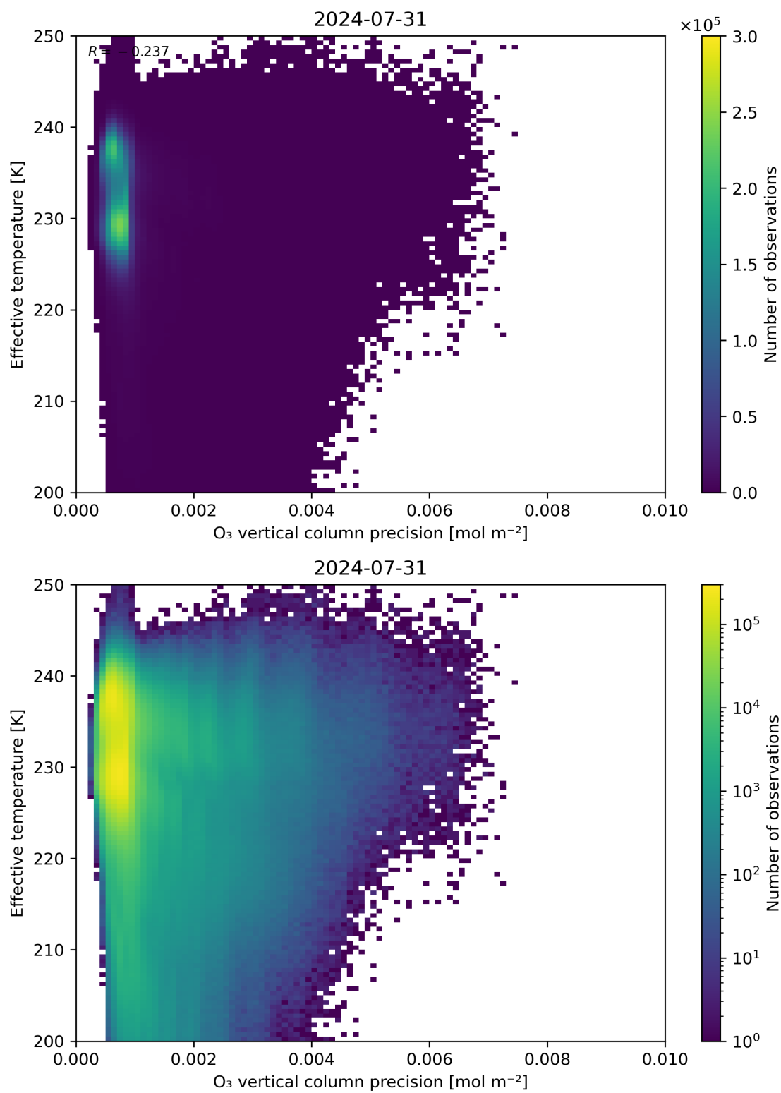
Figure 42: Scatter density plot of “O 3 vertical column precision” against “Effective temperature” for 2024-07-31 to 2024-08-01.
