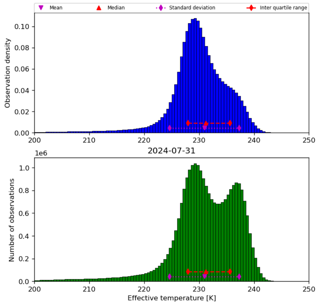
Figure 24: Histogram of “Effective temperature” for 2024-07-31 to 2024-08-01
