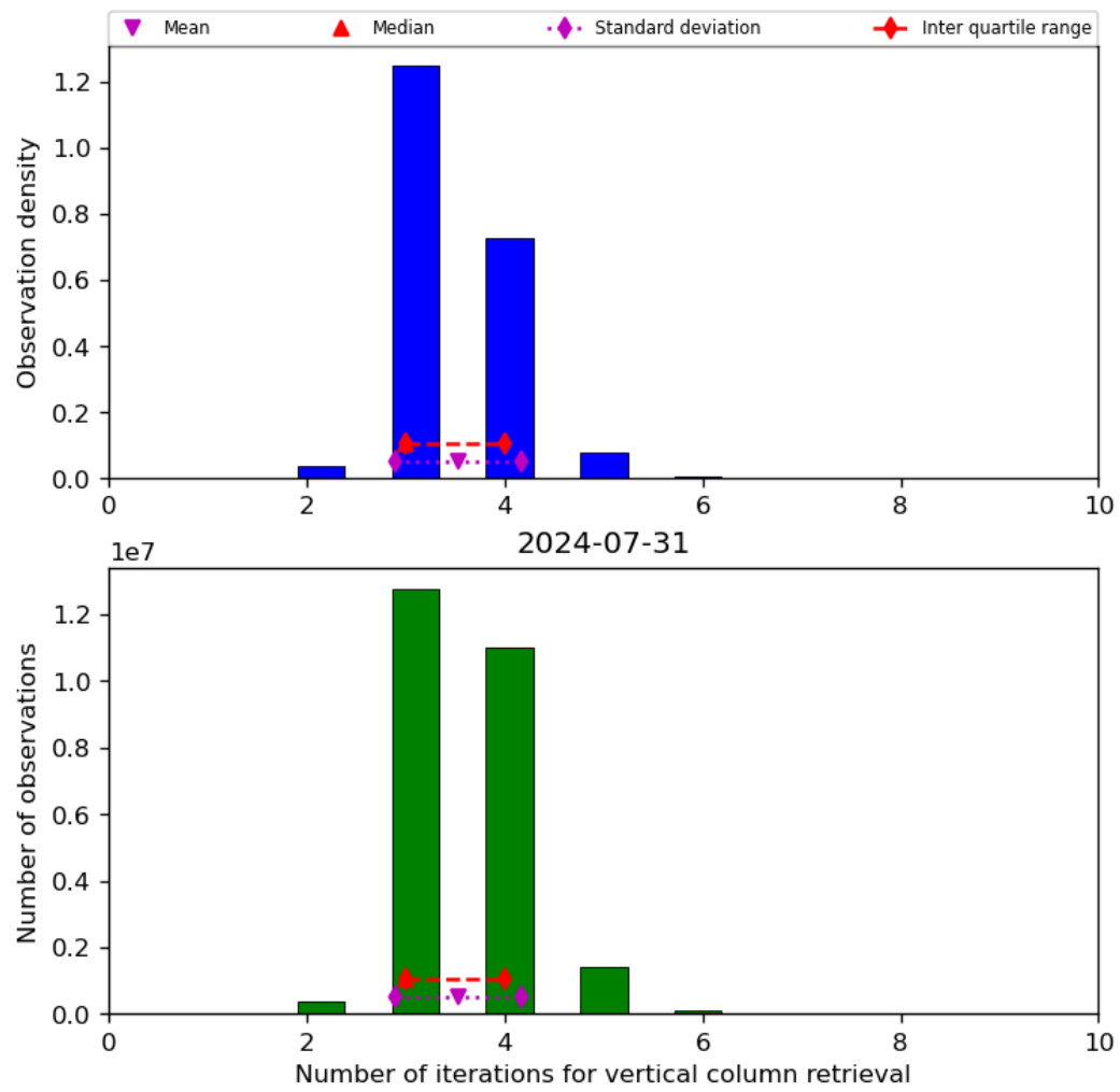
Figure 26: Histogram of “Number of iterations for vertical column retrieval” for 2024-07-31 to 2024-08-01
