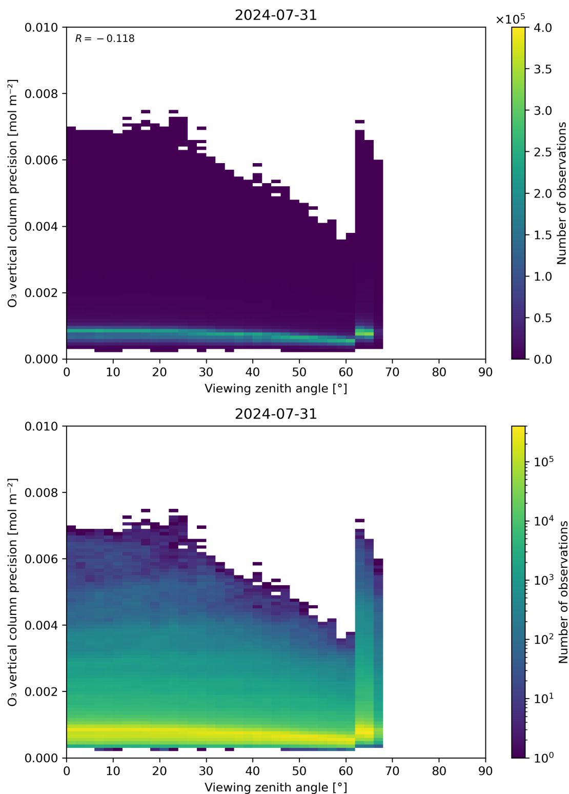
Figure 53: Scatter density plot of “Viewing zenith angle” against “O 3 vertical column precision” for 2024-07-31 to 2024-08-01.
