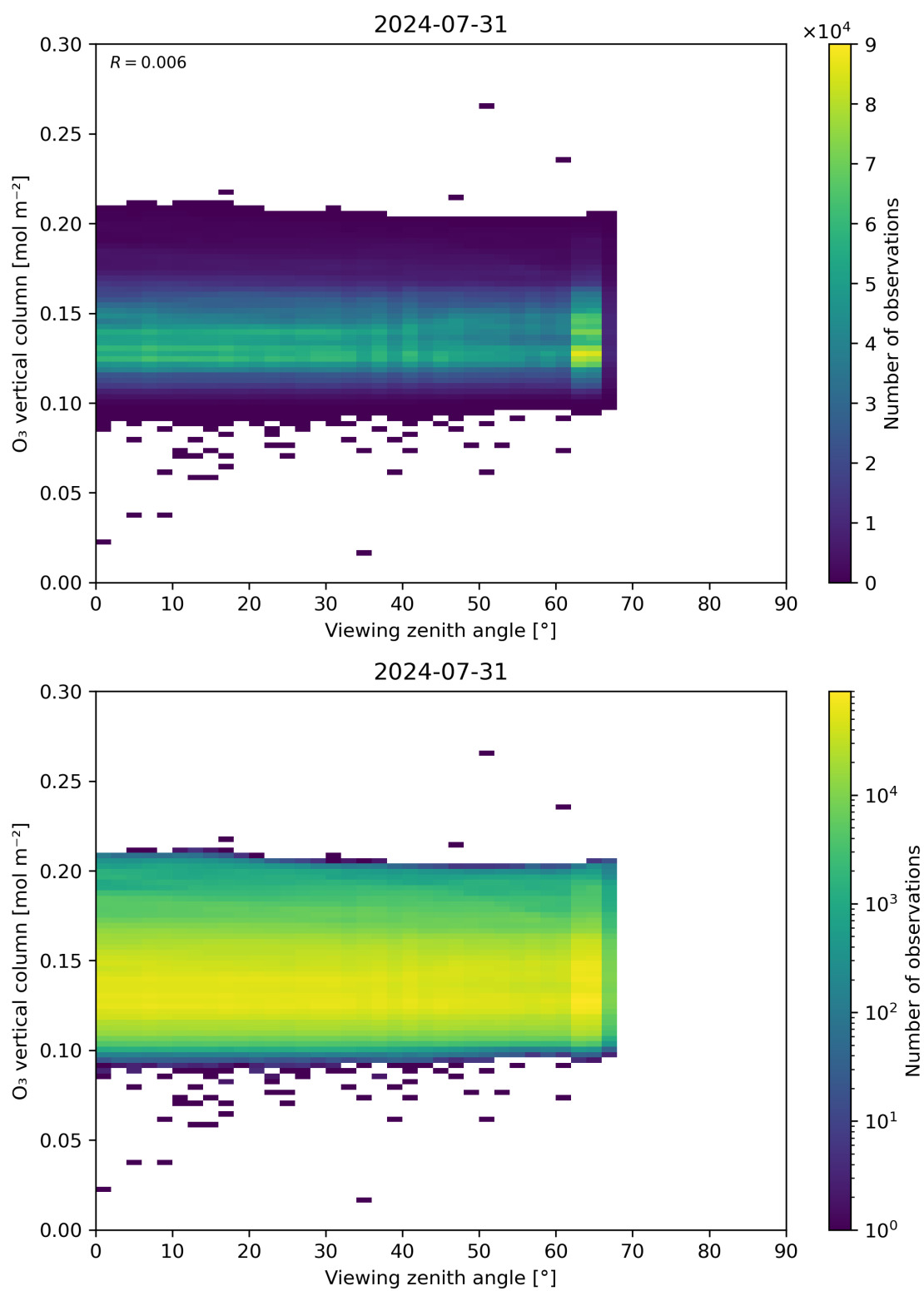
Figure 52: Scatter density plot of “Viewing zenith angle” against “O 3 vertical column” for 2024-07-31 to 2024-08-01.
