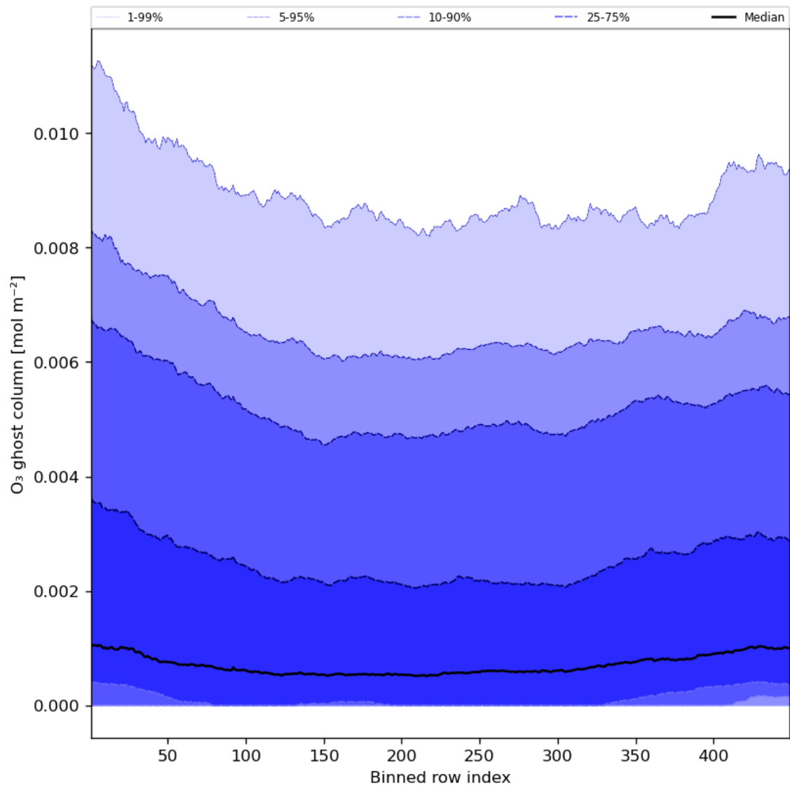
Figure 32: Along track statistics of “O 3 ghost column” for 2024-07-31 to 2024-08-01
