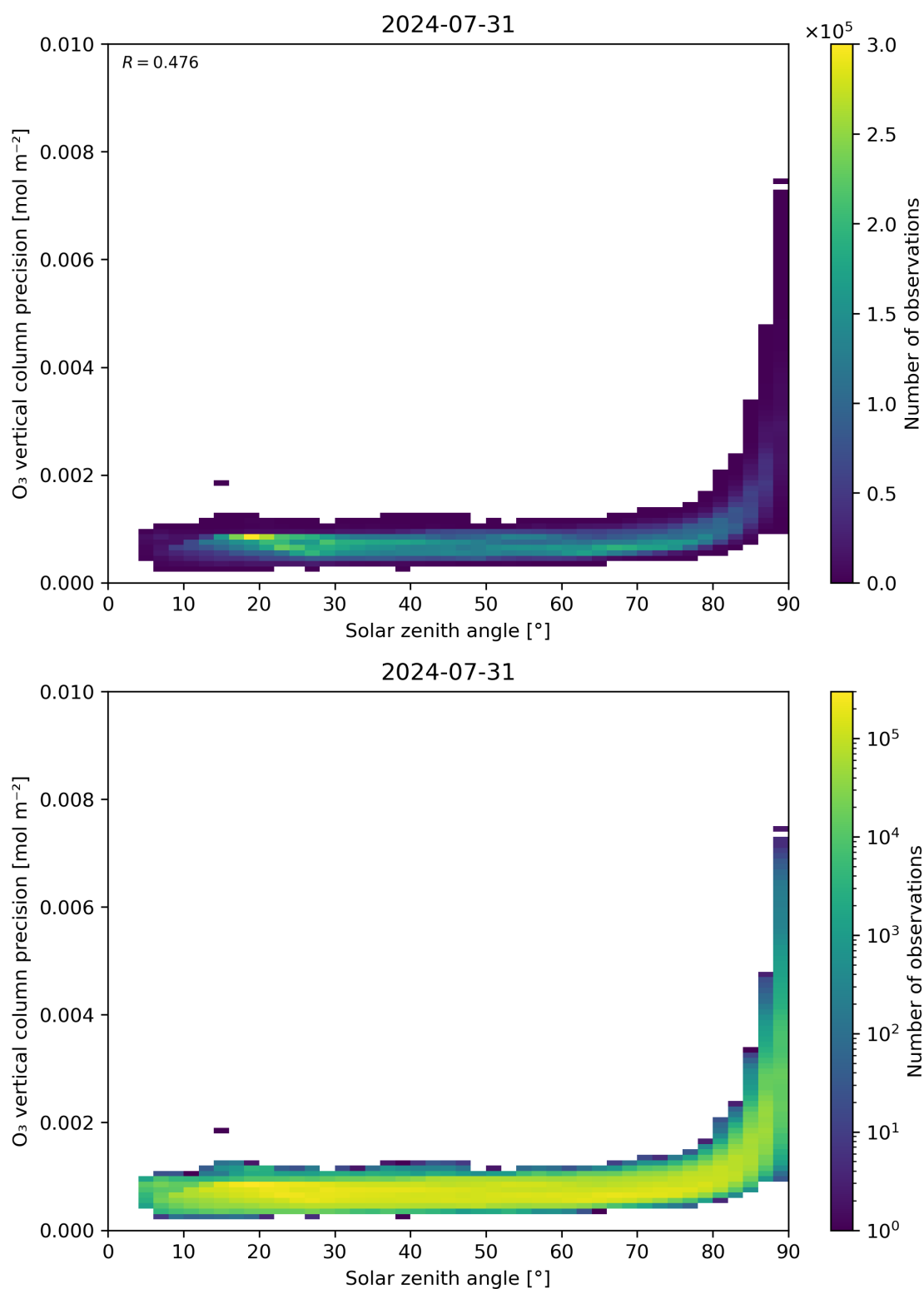
Figure 48: Scatter density plot of “Solar zenith angle” against “O 3 vertical column precision” for 2024-07-31 to 2024-08-01.
