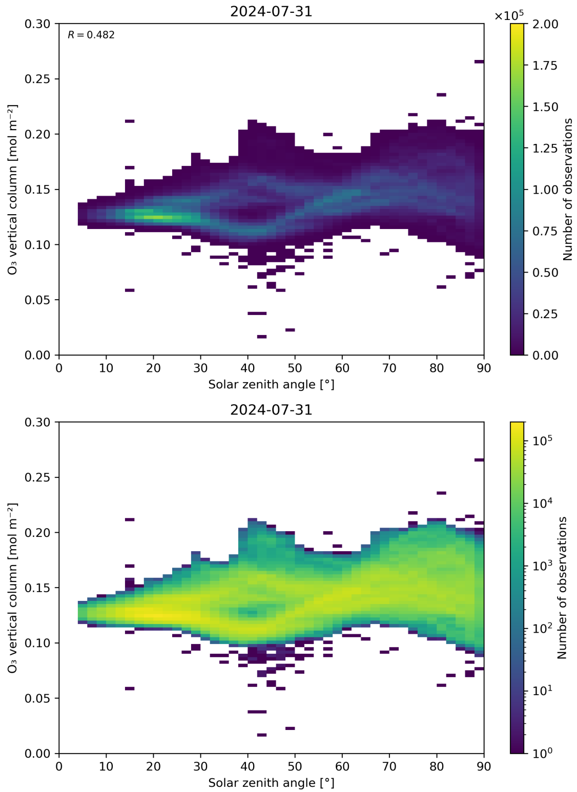
Figure 47: Scatter density plot of “Solar zenith angle” against “O 3 vertical column” for 2024-07-31 to 2024-08-01.
