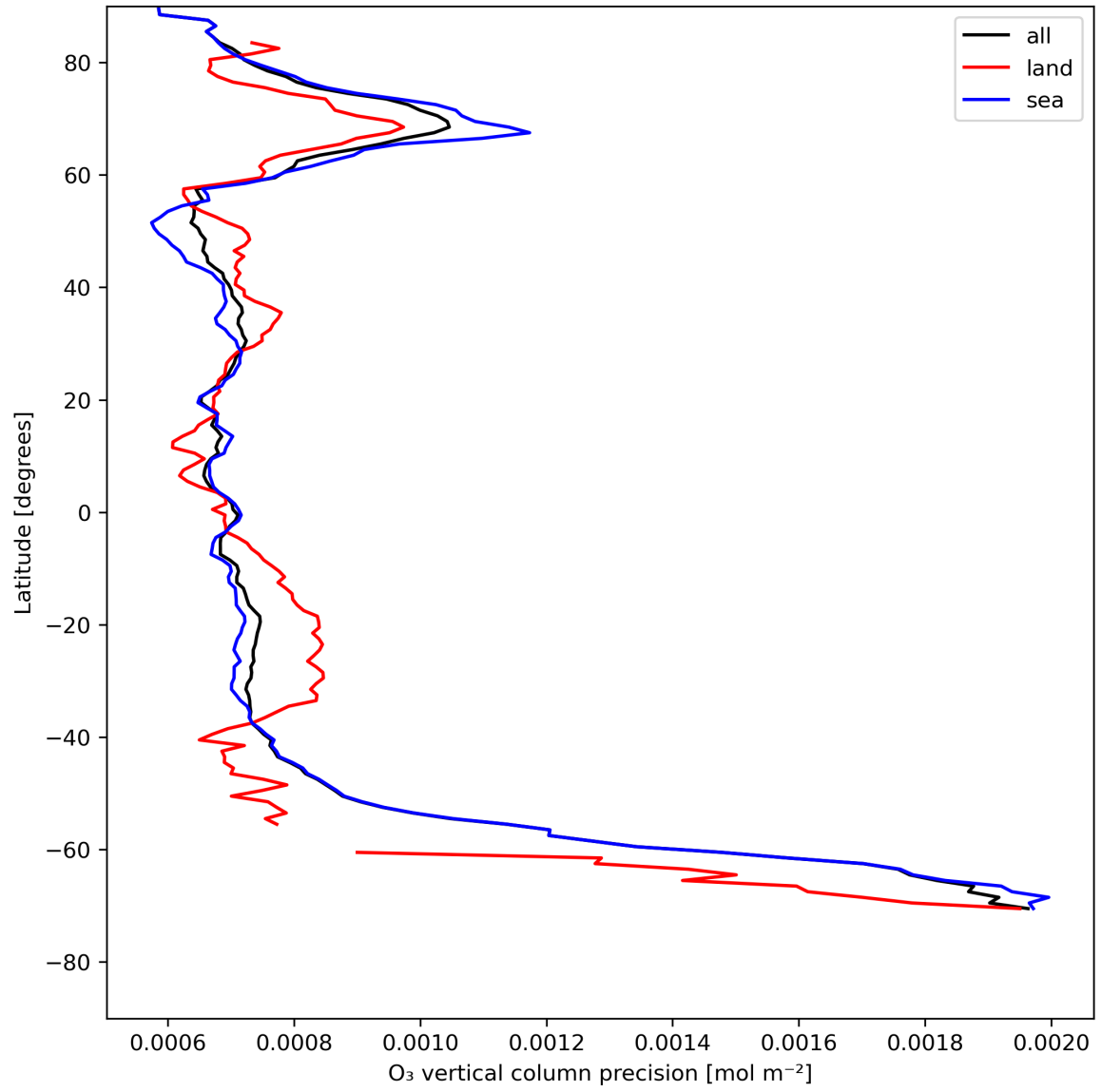
Figure 15: Zonal average of “O 3 vertical column precision” for 2024-07-31 to 2024-08-01.
