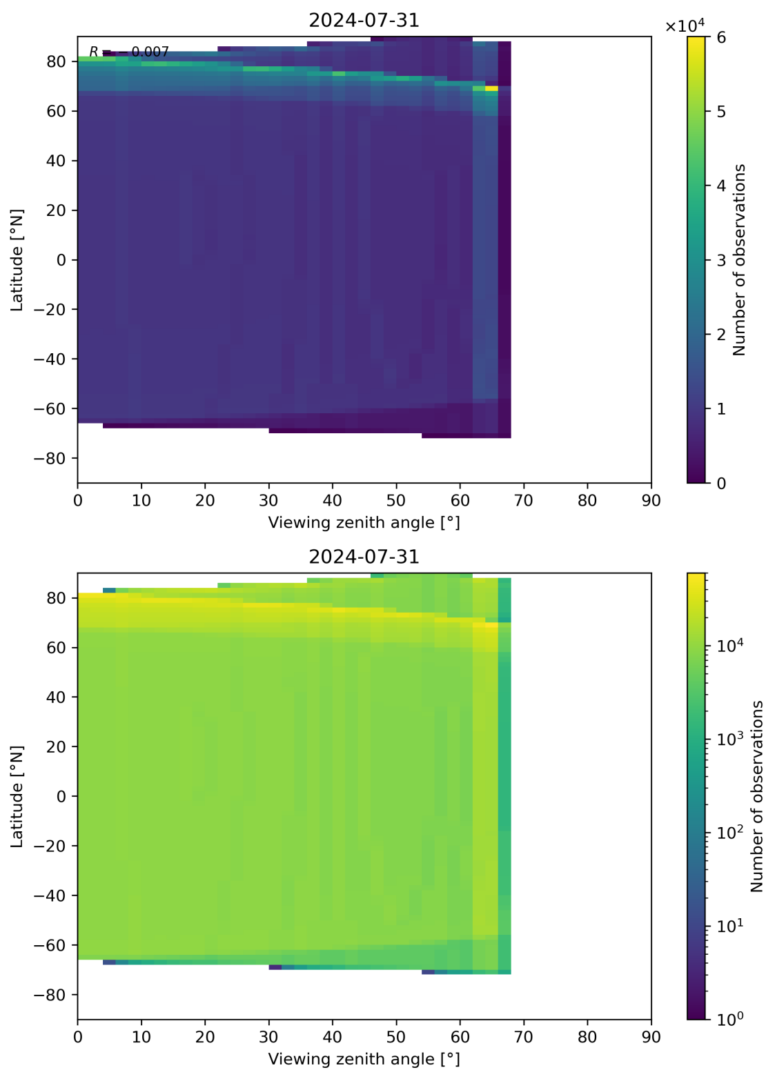
Figure 49: Scatter density plot of “Viewing zenith angle” against “Latitude” for 2024-07-31 to 2024-08-01.
