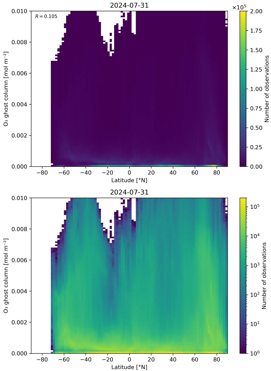
Figure 35: Scatter density plot of “Latitude” against “O 3 ghost column” for 2024-07-31 to 2024-08-01.
