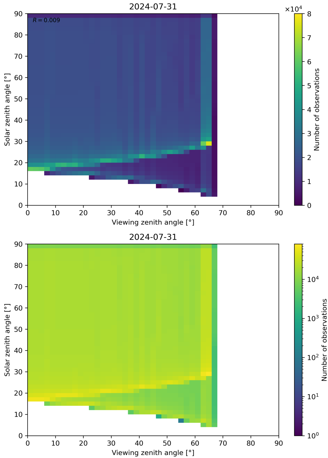
Figure 54: Scatter density plot of “Viewing zenith angle” against “Solar zenith angle” for 2024-07-31 to 2024-08-01.
