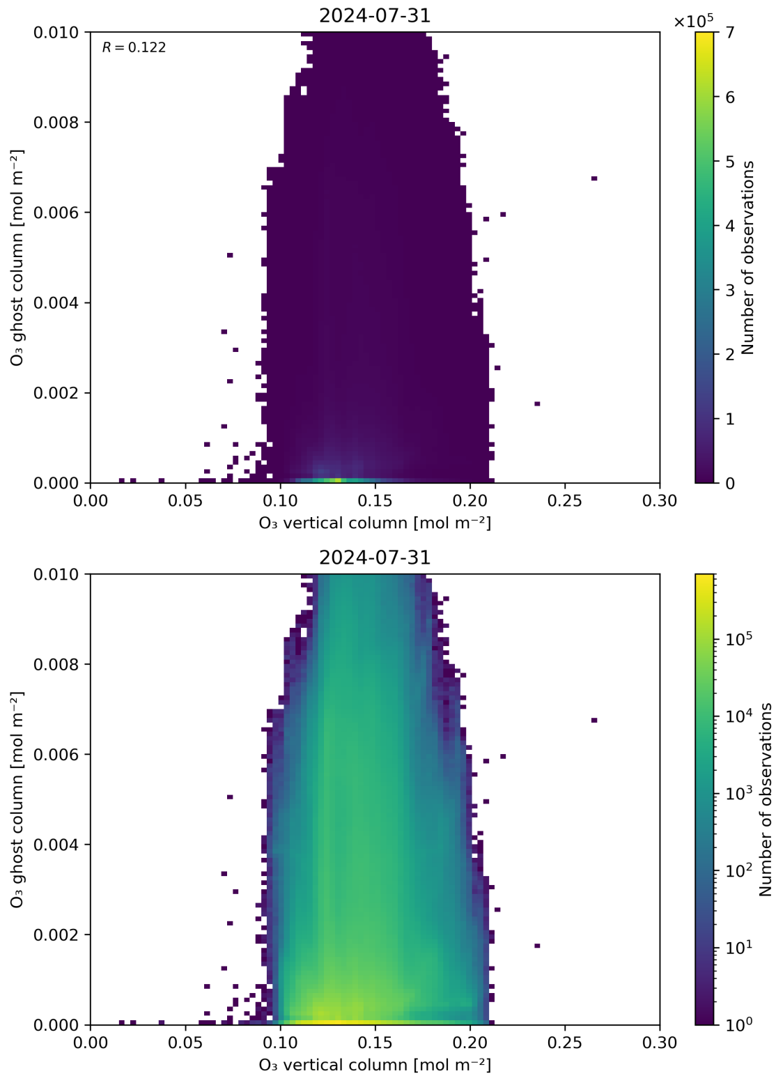
Figure 40: Scatter density plot of “O 3 vertical column” against “O 3 ghost column” for 2024-07-31 to 2024-08-01.
