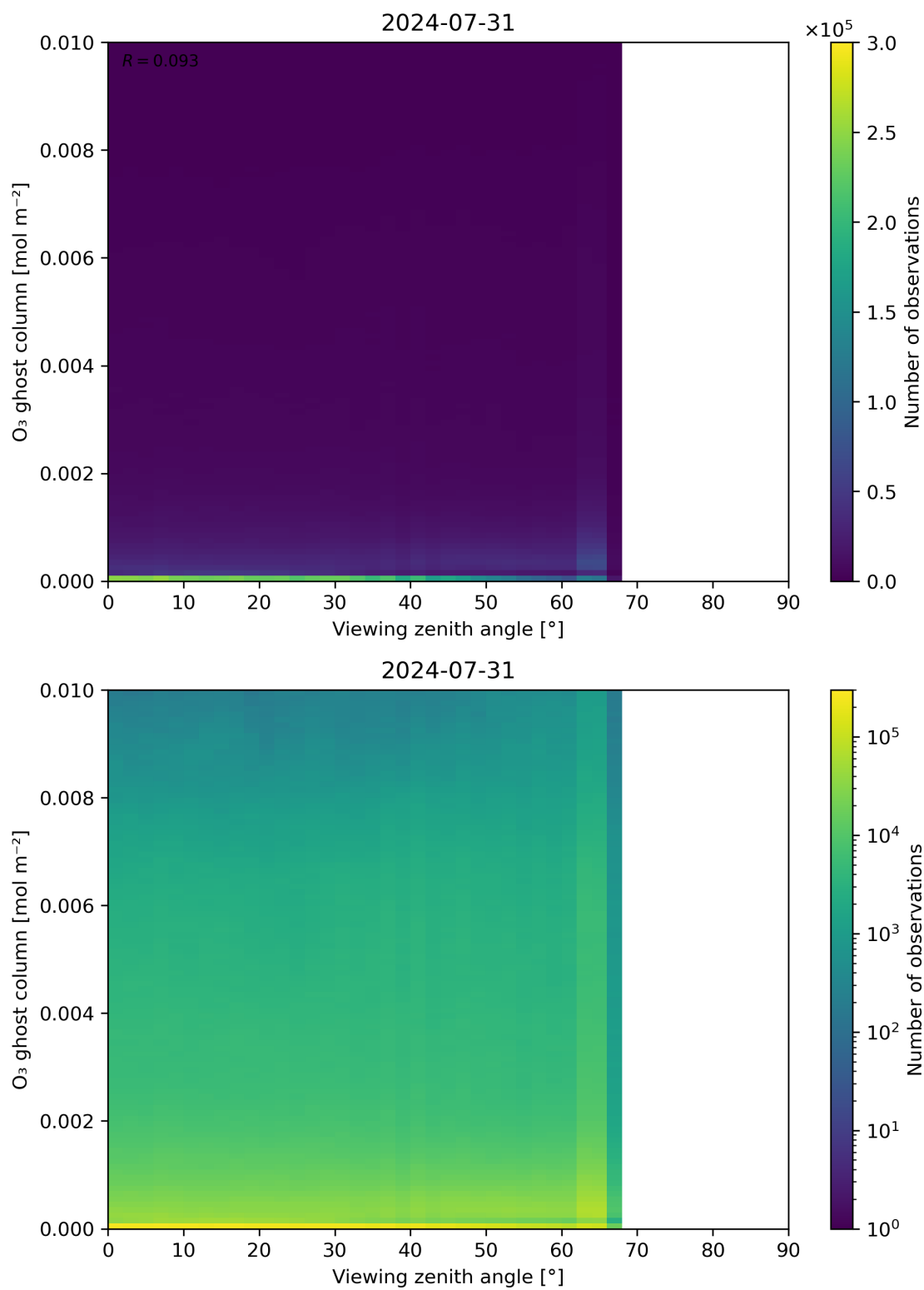
Figure 51: Scatter density plot of “Viewing zenith angle” against “O 3 ghost column” for 2024-07-31 to 2024-08-01.
