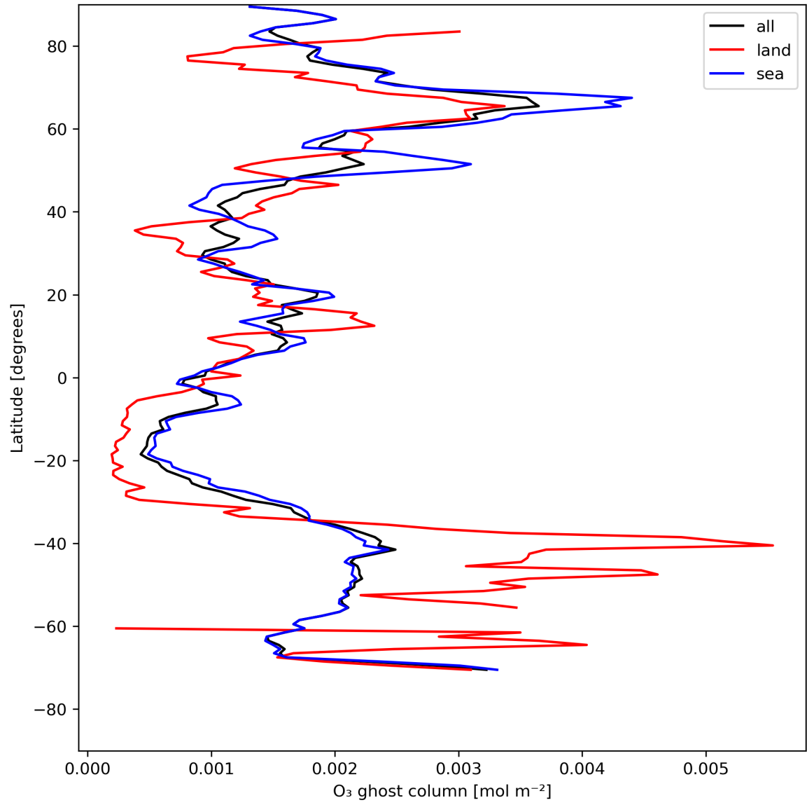
Figure 18: Zonal average of "O 3 ghost column" for 2024-07-31 to 2024-08-01.
