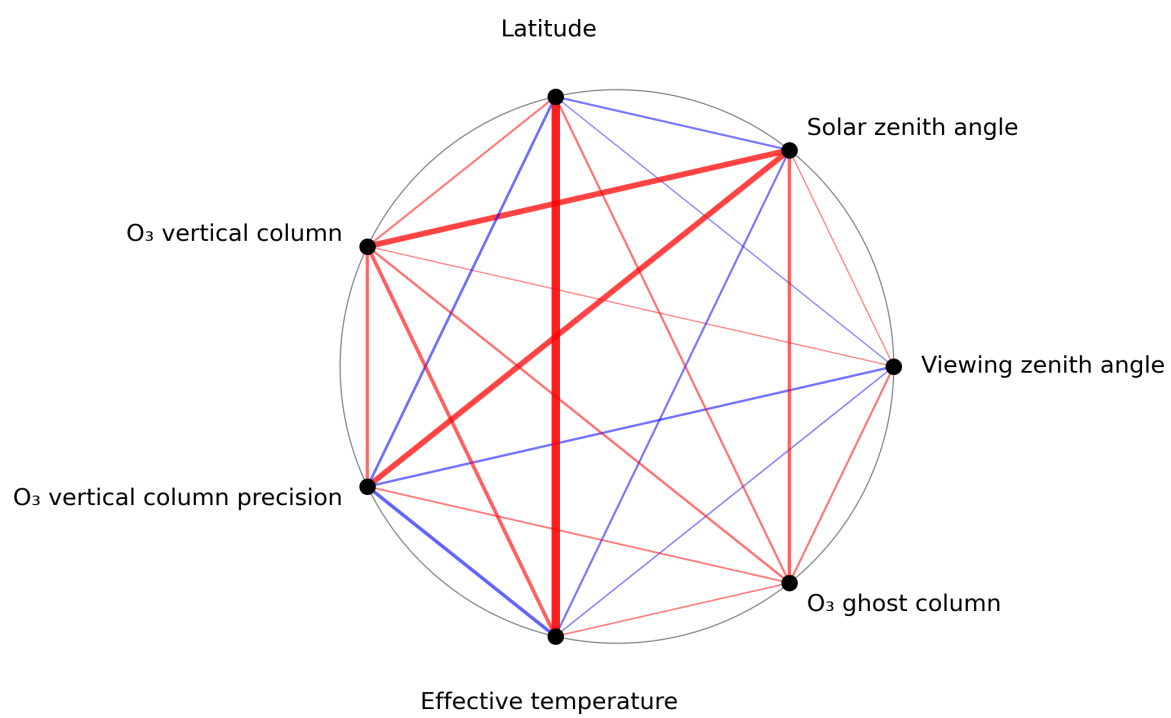
Figure 1: Map of correlation graph for 2024-07-31 to 2024-08-01.
