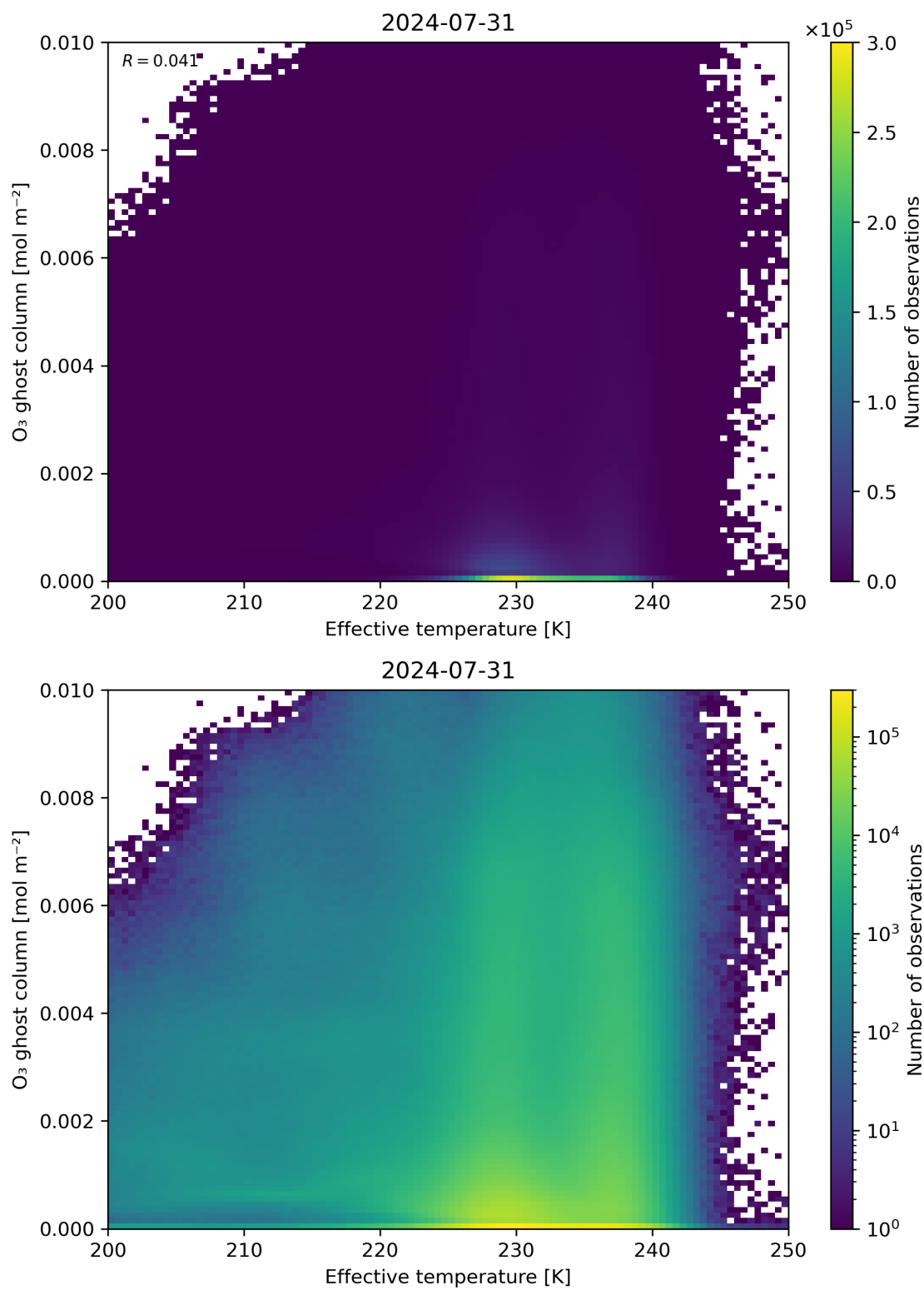
Figure 38: Scatter density plot of “Effective temperature” against “O 3 ghost column” for 2024-07-31 to 2024-08-01.
