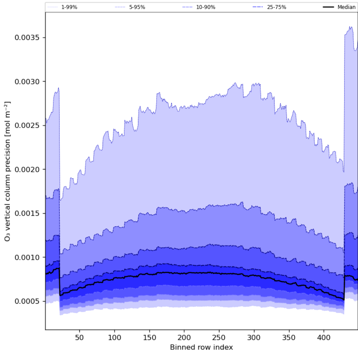
Figure 29: Along track statistics of “O 3 vertical column precision” for 2024-07-31 to 2024-08-01
