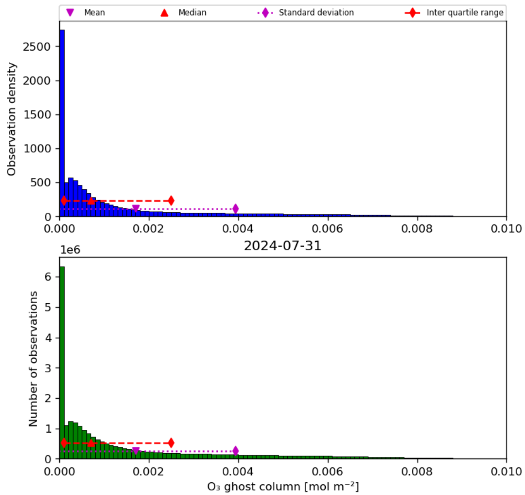
Figure 25: Histogram of “O 3 ghost column” for 2024-07-31 to 2024-08-01
