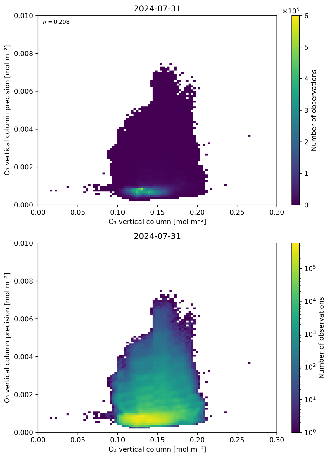
Figure 41: Scatter density plot of “O 3 vertical column” against “O 3 vertical column precision” for 2024-07-31 to 2024-08-01.
