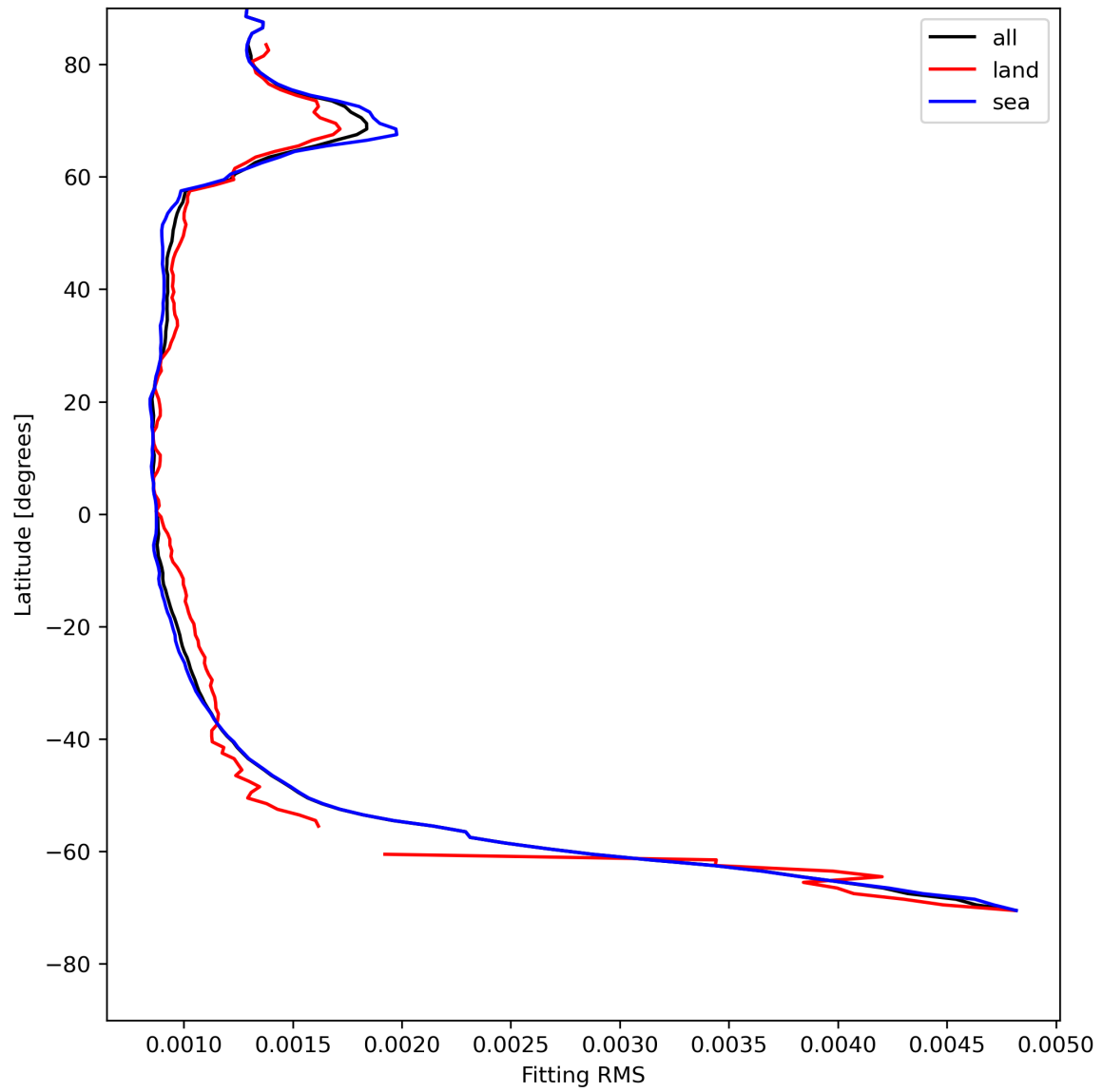
Figure 16: Zonal average of “Fitting RMS” for 2024-07-31 to 2024-08-01.
