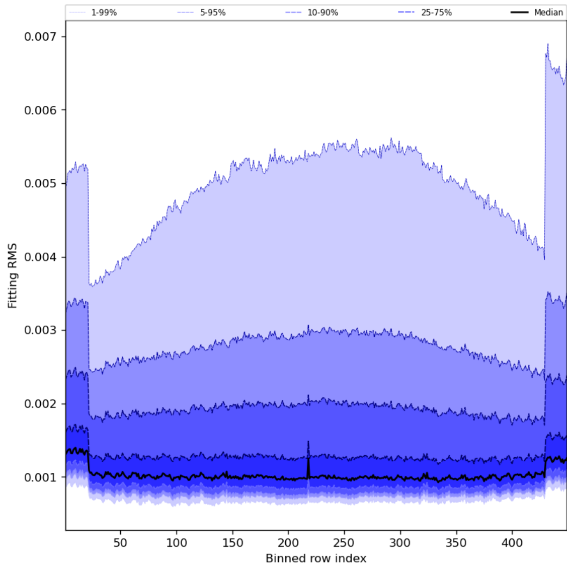
Figure 30: Along track statistics of “Fitting RMS” for 2024-07-31 to 2024-08-01
