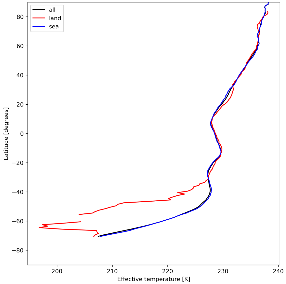
Figure 17: Zonal average of "Effective temperature" for 2024-07-31 to 2024-08-01.
