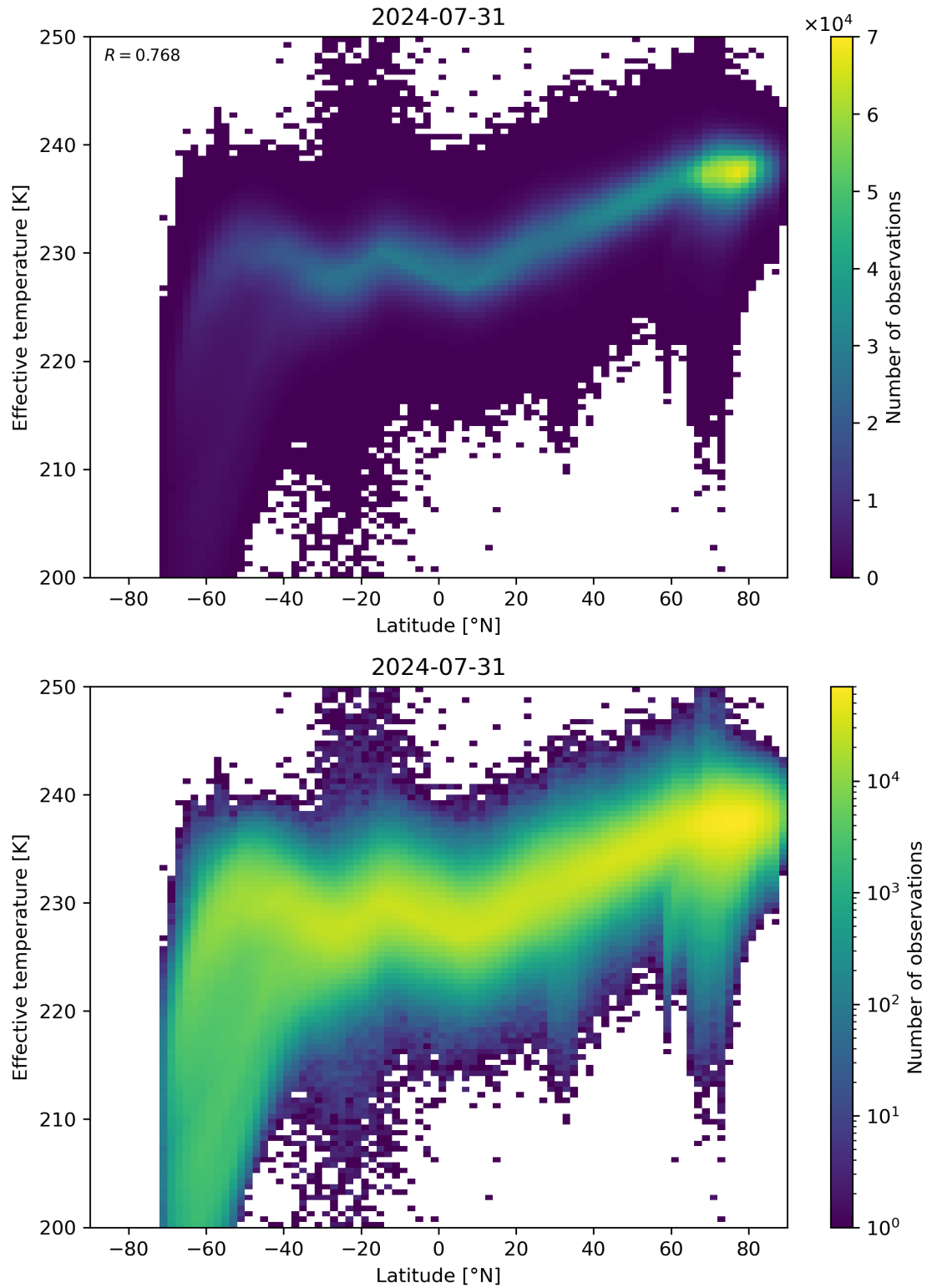
Figure 34: Scatter density plot of “Latitude” against “Effective temperature” for 2024-07-31 to 2024-08-01.
