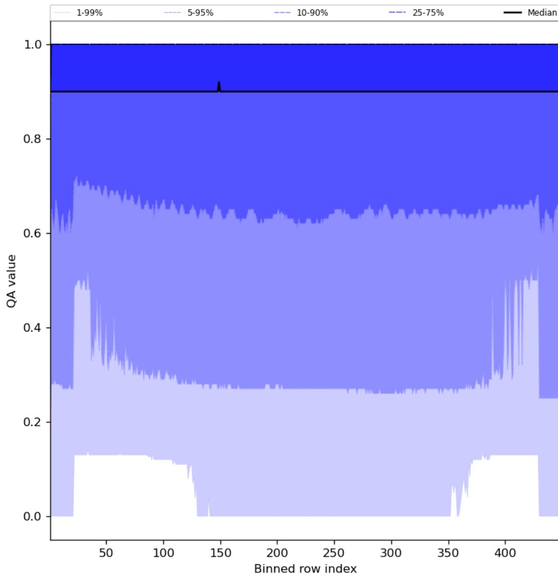
Figure 27: Along track statistics of “QA value” for 2024-07-31 to 2024-08-01
