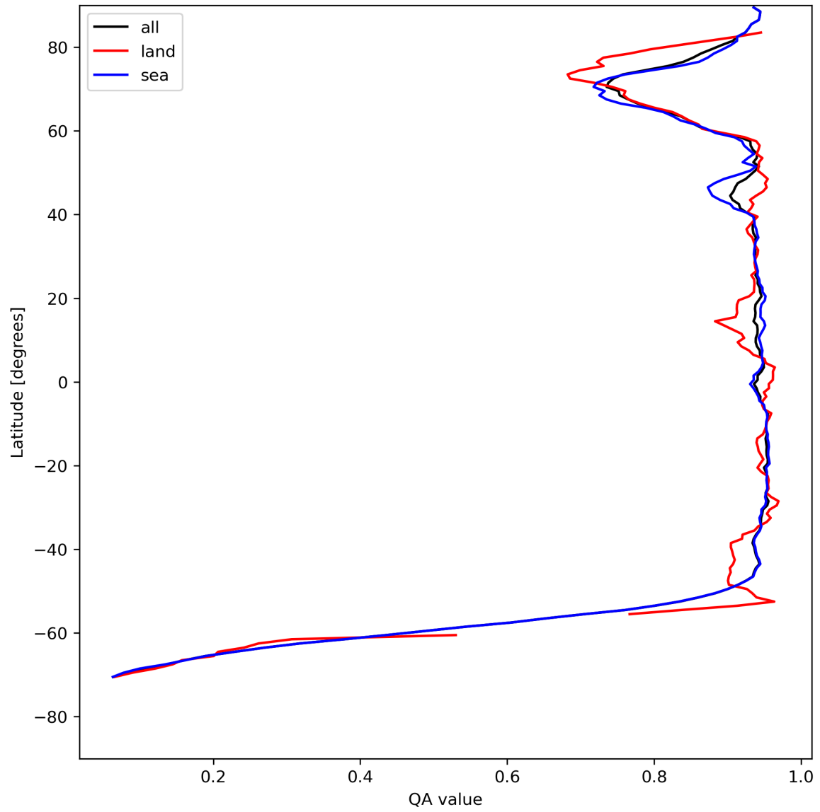
Figure 13: Zonal average of “QA value” for 2024-07-31 to 2024-08-01.
