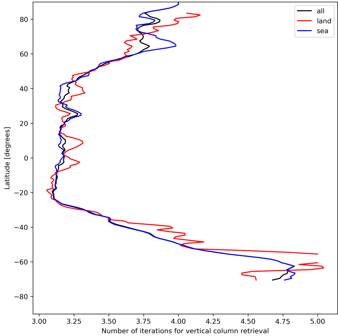
Figure 19: Zonal average of “Number of iterations for vertical column retrieval” for 2024-07-31 to 2024-08-01.
