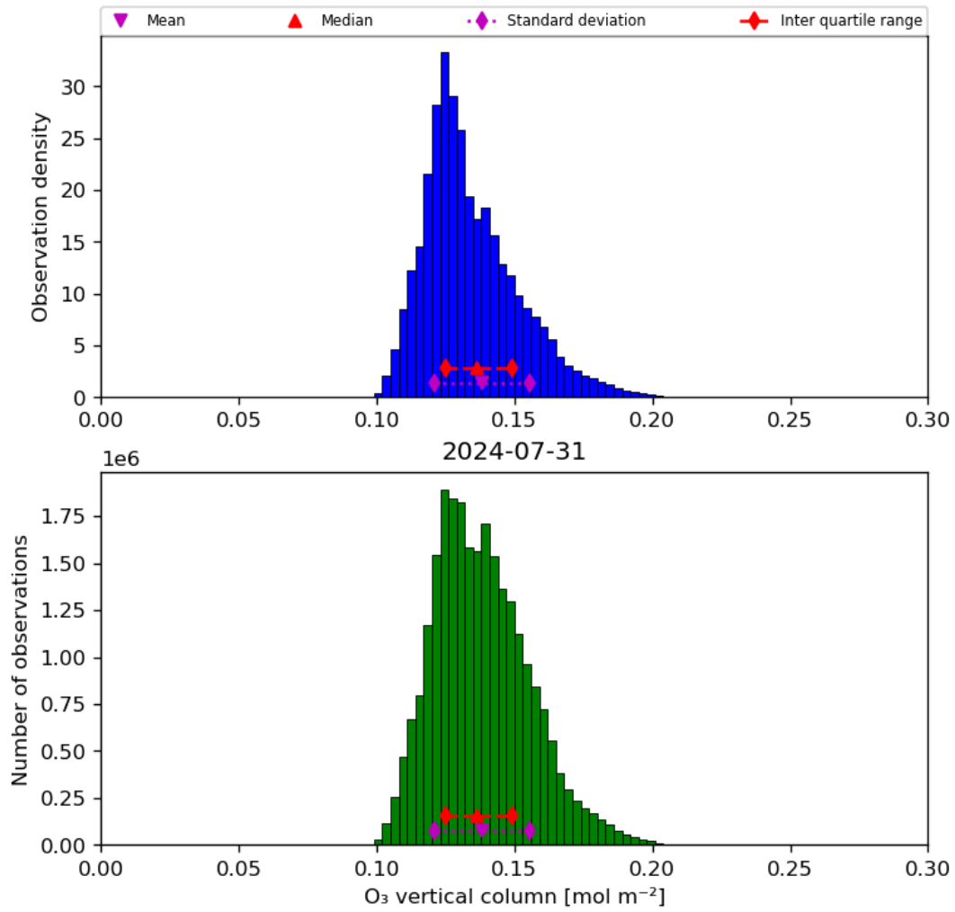
Figure 21: Histogram of “O 3 vertical column” for 2024-07-31 to 2024-08-01
