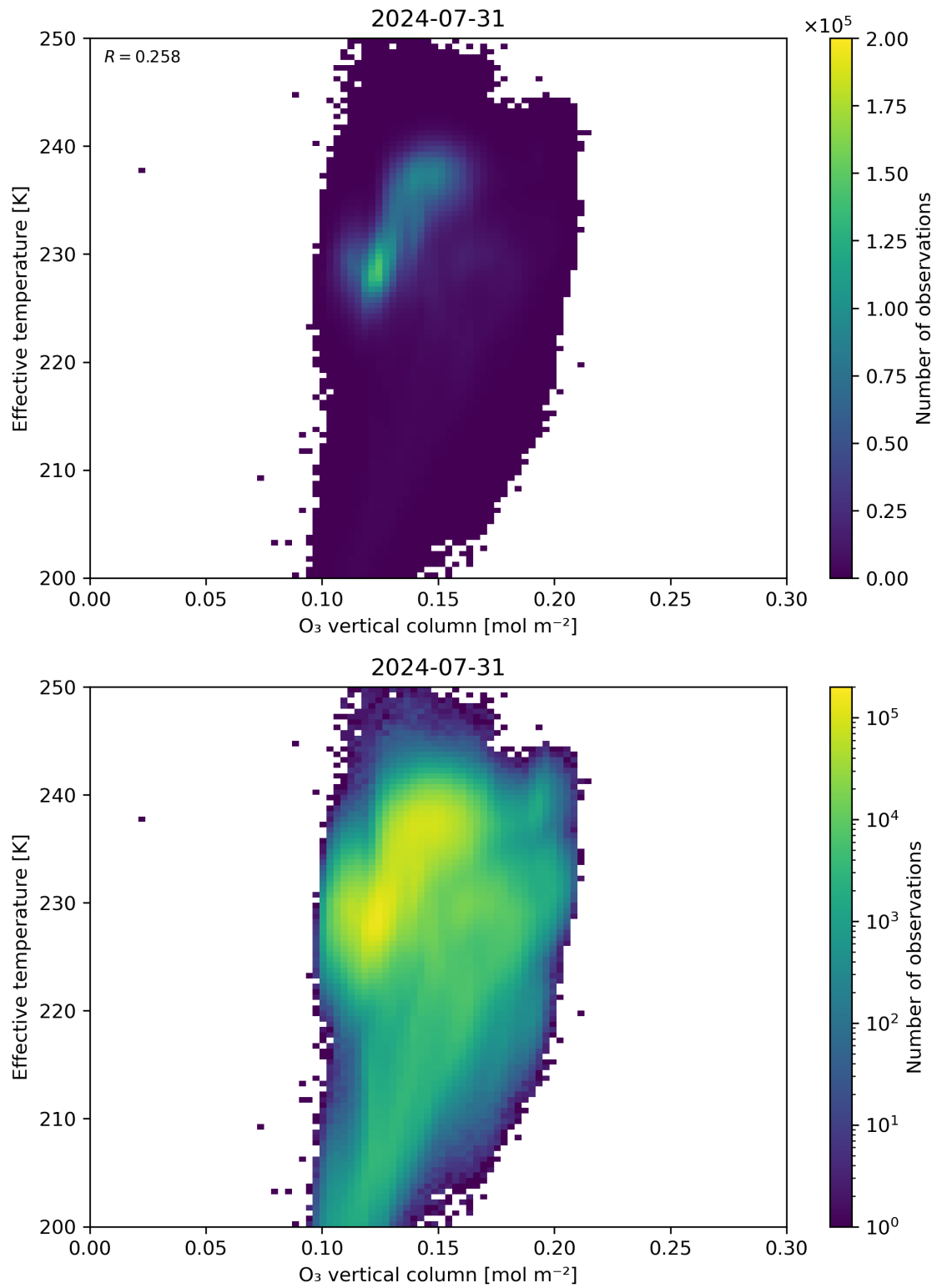
Figure 39: Scatter density plot of “O 3 vertical column” against “Effective temperature” for 2024-07-31 to 2024-08-01.
