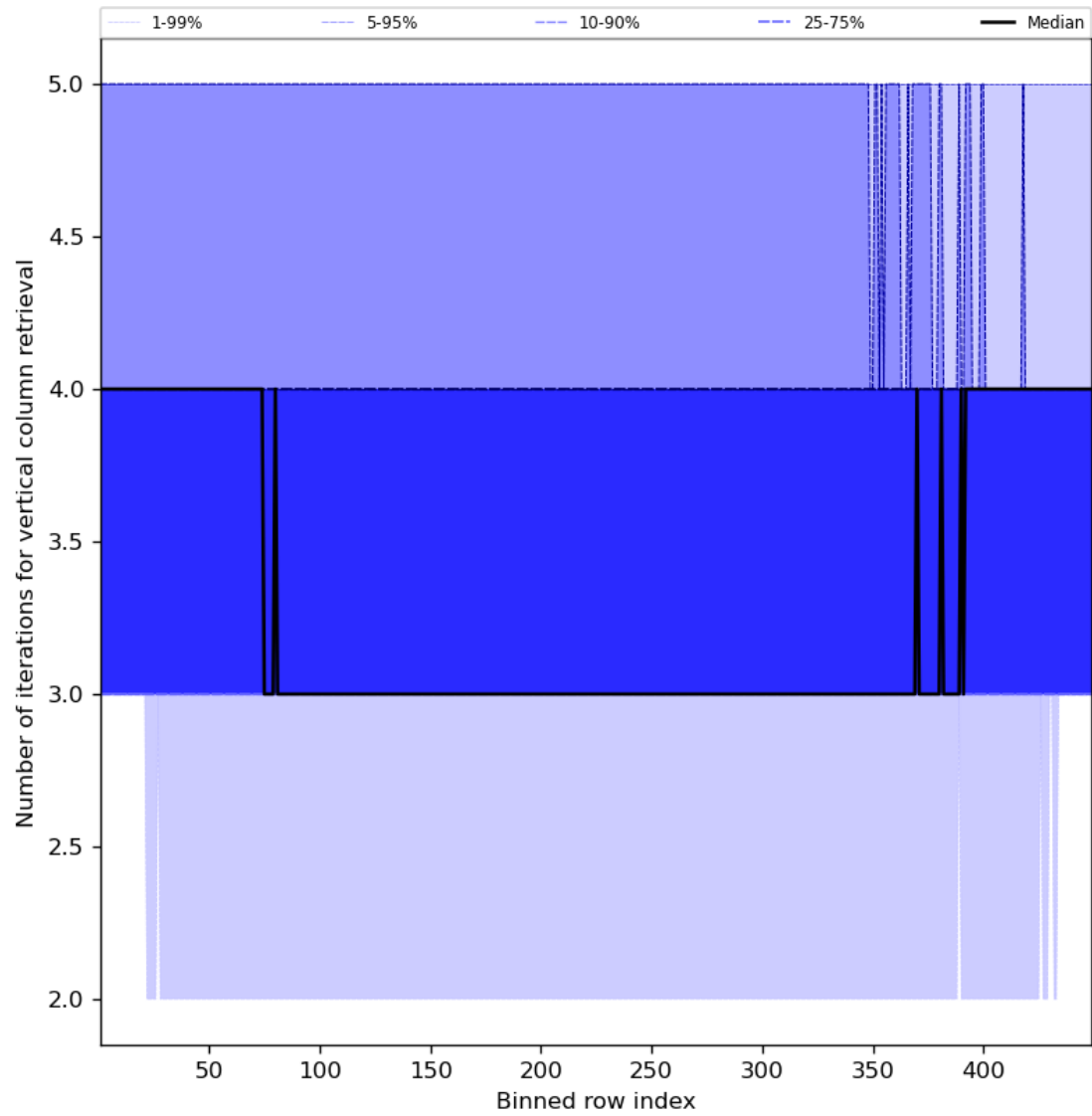
Figure 33: Along track statistics of “Number of iterations for vertical column retrieval” for 2024-07-31 to 2024-08-01
