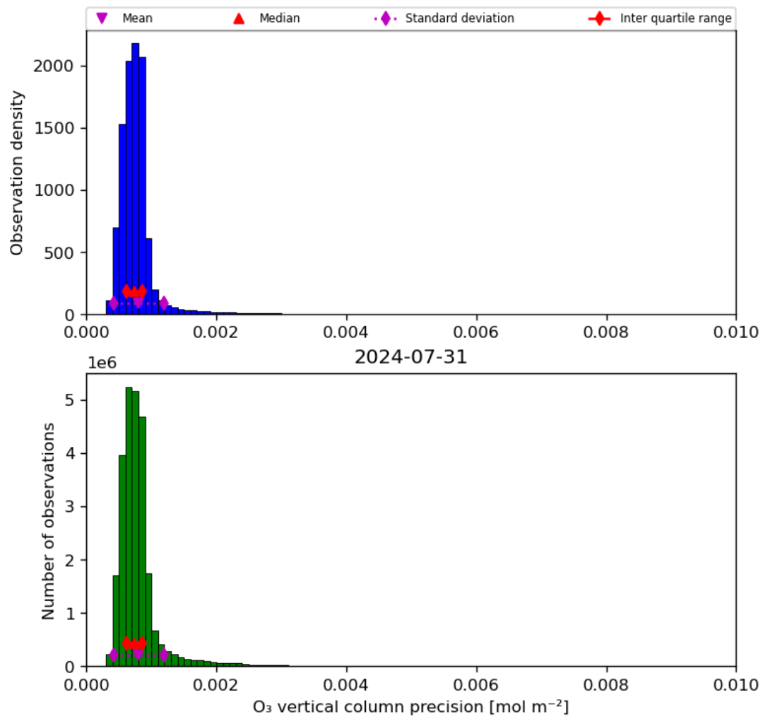
Figure 22: Histogram of “O 3 vertical column precision” for 2024-07-31 to 2024-08-01
