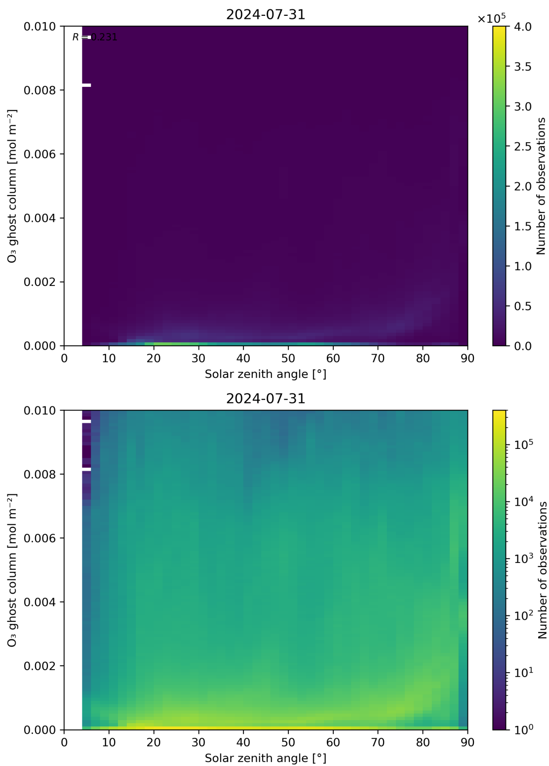
Figure 46: Scatter density plot of “Solar zenith angle” against “O 3 ghost column” for 2024-07-31 to 2024-08-01.
