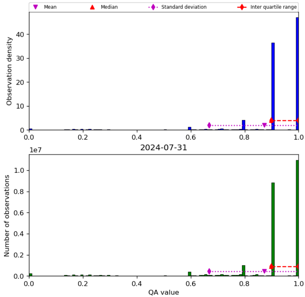
Figure 20: Histogram of “QA value” for 2024-07-31 to 2024-08-01
