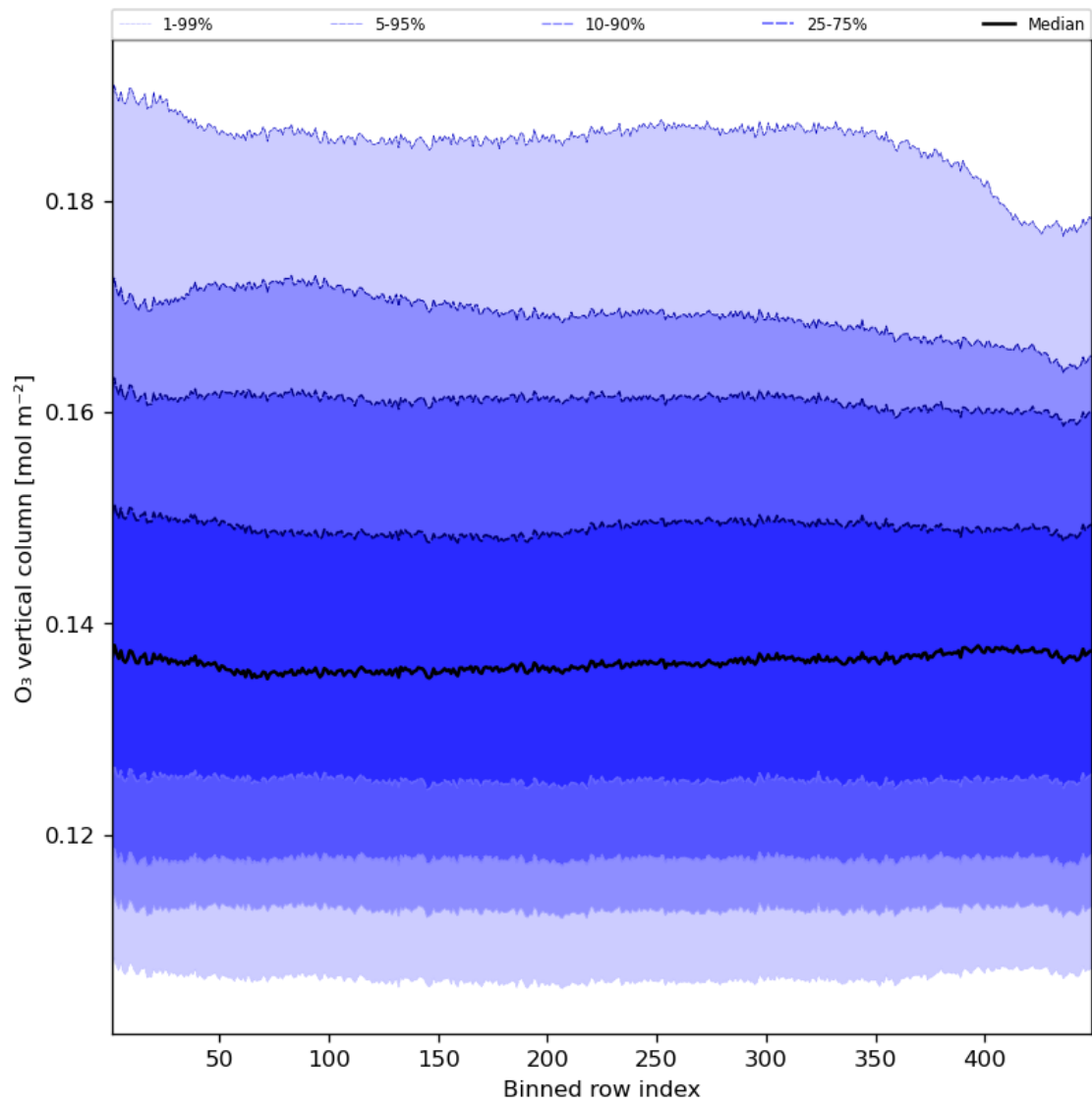
Figure 28: Along track statistics of “O 3 vertical column” for 2024-07-31 to 2024-08-01
