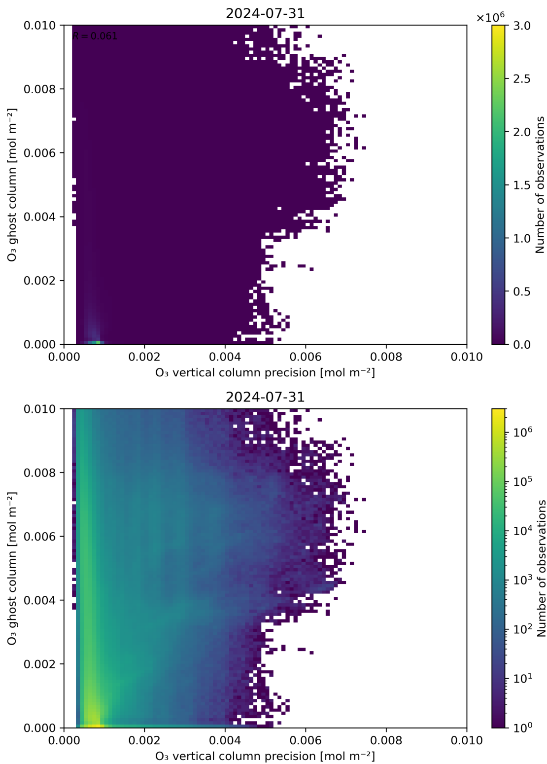
Figure 43: Scatter density plot of “O 3 vertical column precision” against “O 3 ghost column” for 2024-07-31 to 2024-08-01.
