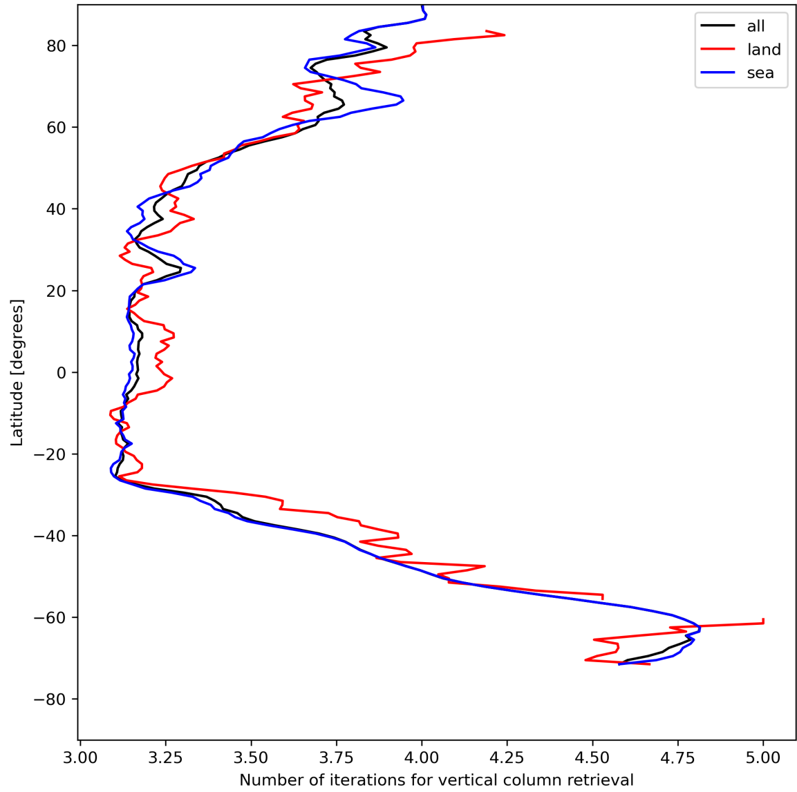
Figure 19: Zonal average of “Number of iterations for vertical column retrieval” for 2024-07-31 to 2024-08-02.
