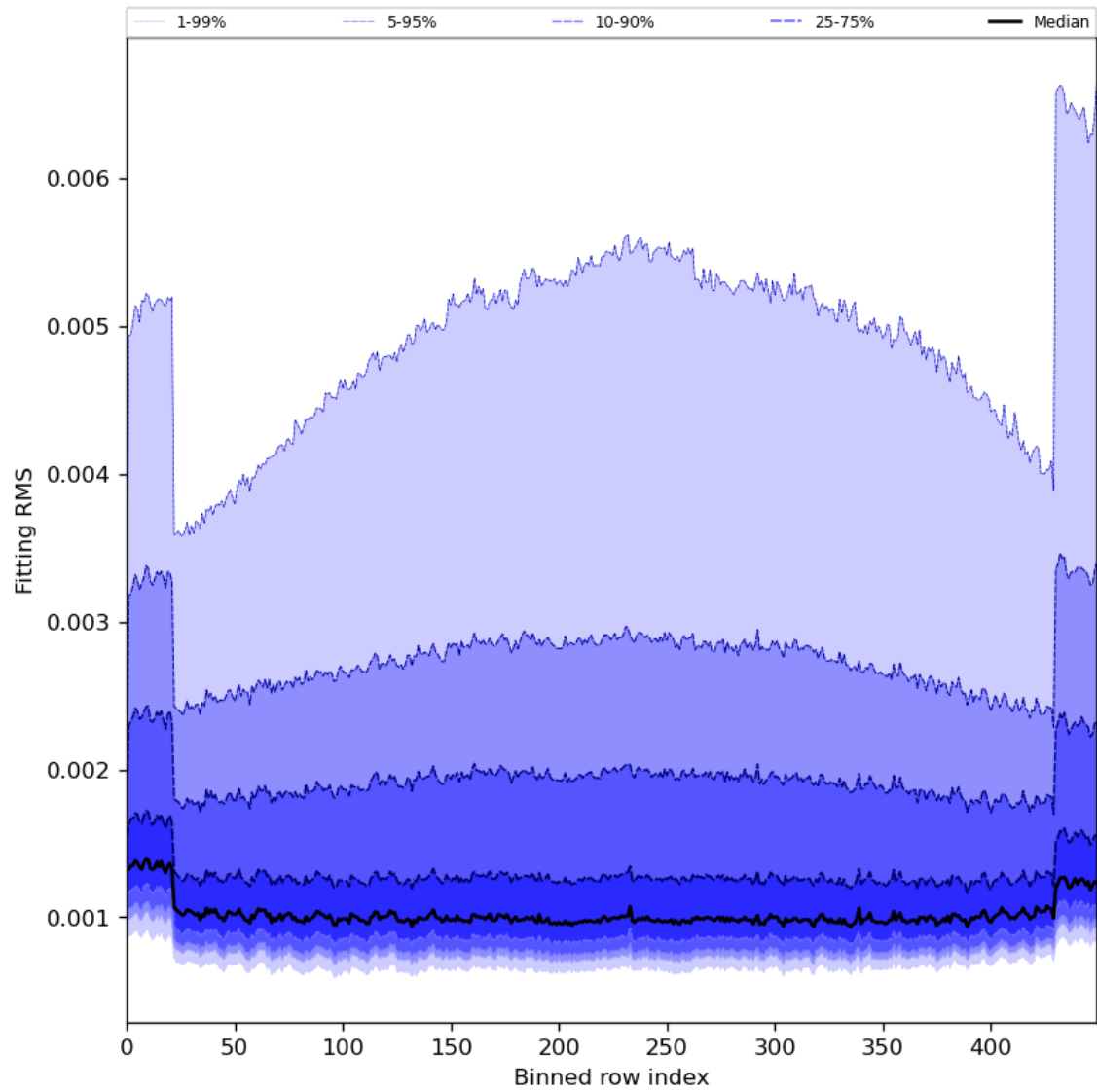
Figure 30: Along track statistics of “Fitting RMS” for 2024-07-31 to 2024-08-02
