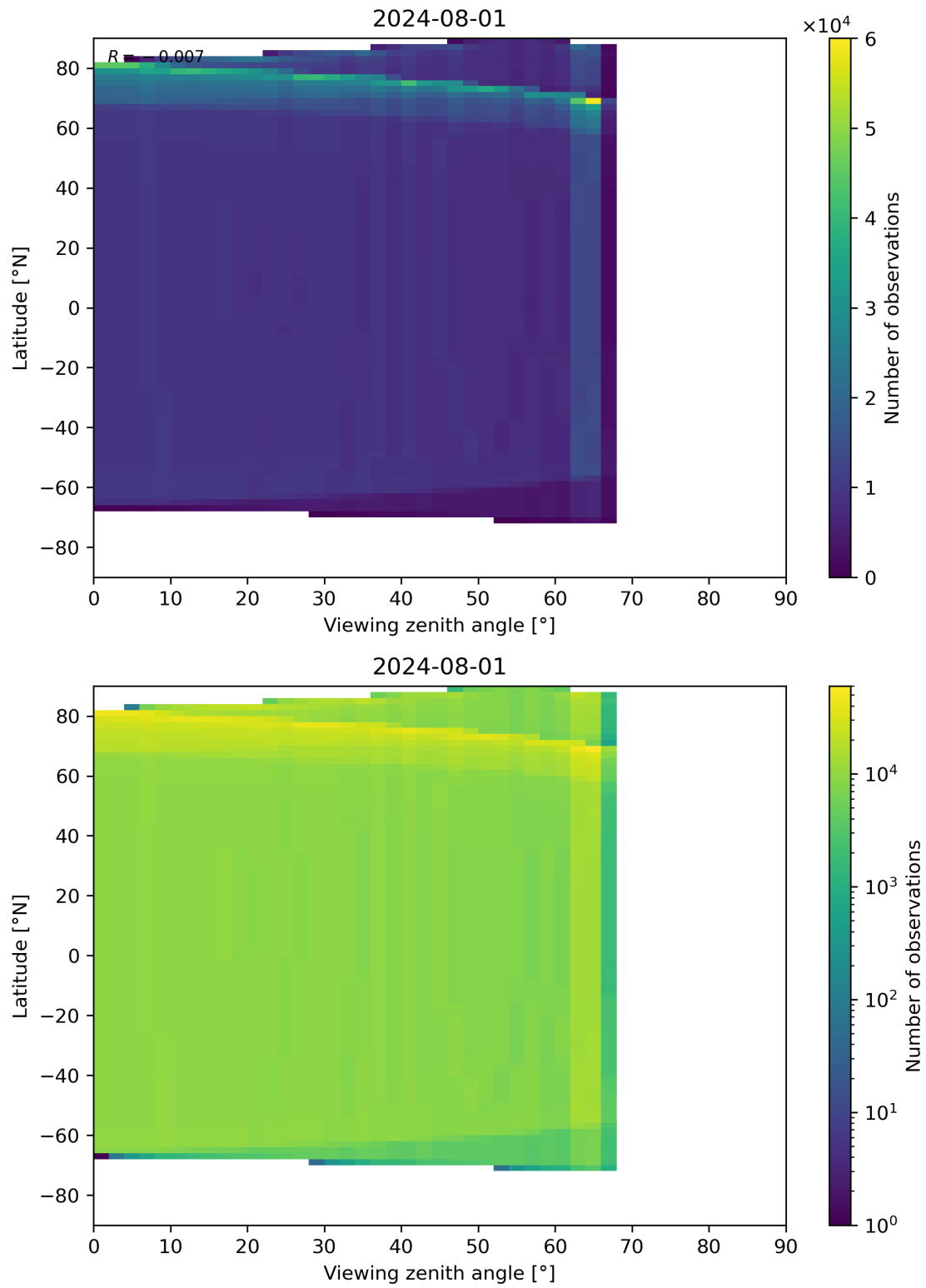
Figure 49: Scatter density plot of “Viewing zenith angle” against “Latitude” for 2024-07-31 to 2024-08-02.
