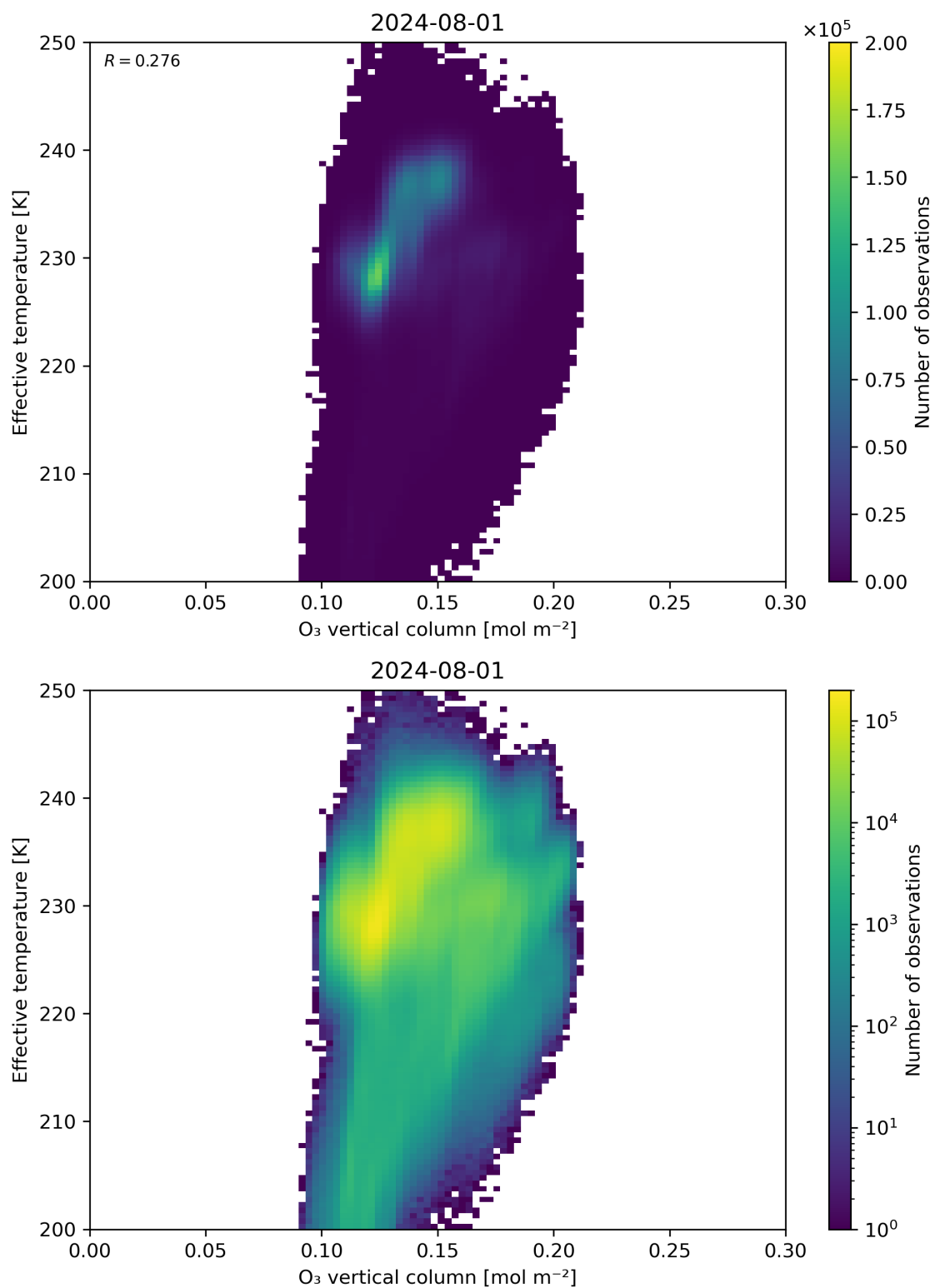
Figure 39: Scatter density plot of “O 3 vertical column” against “Effective temperature” for 2024-07-31 to 2024-08-02.
