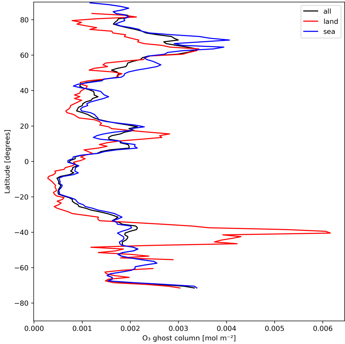
Figure 18: Zonal average of “O 3 ghost column” for 2024-07-31 to 2024-08-02.
