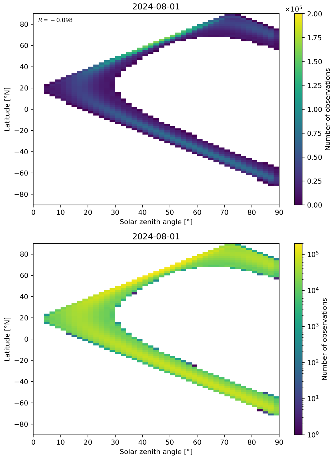
Figure 44: Scatter density plot of “Solar zenith angle” against “Latitude” for 2024-07-31 to 2024-08-02.
