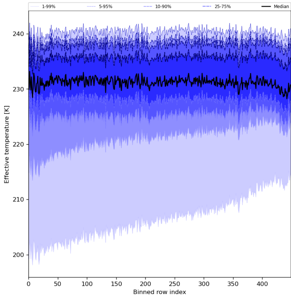
Figure 31: Along track statistics of “Effective temperature” for 2024-07-31 to 2024-08-02
