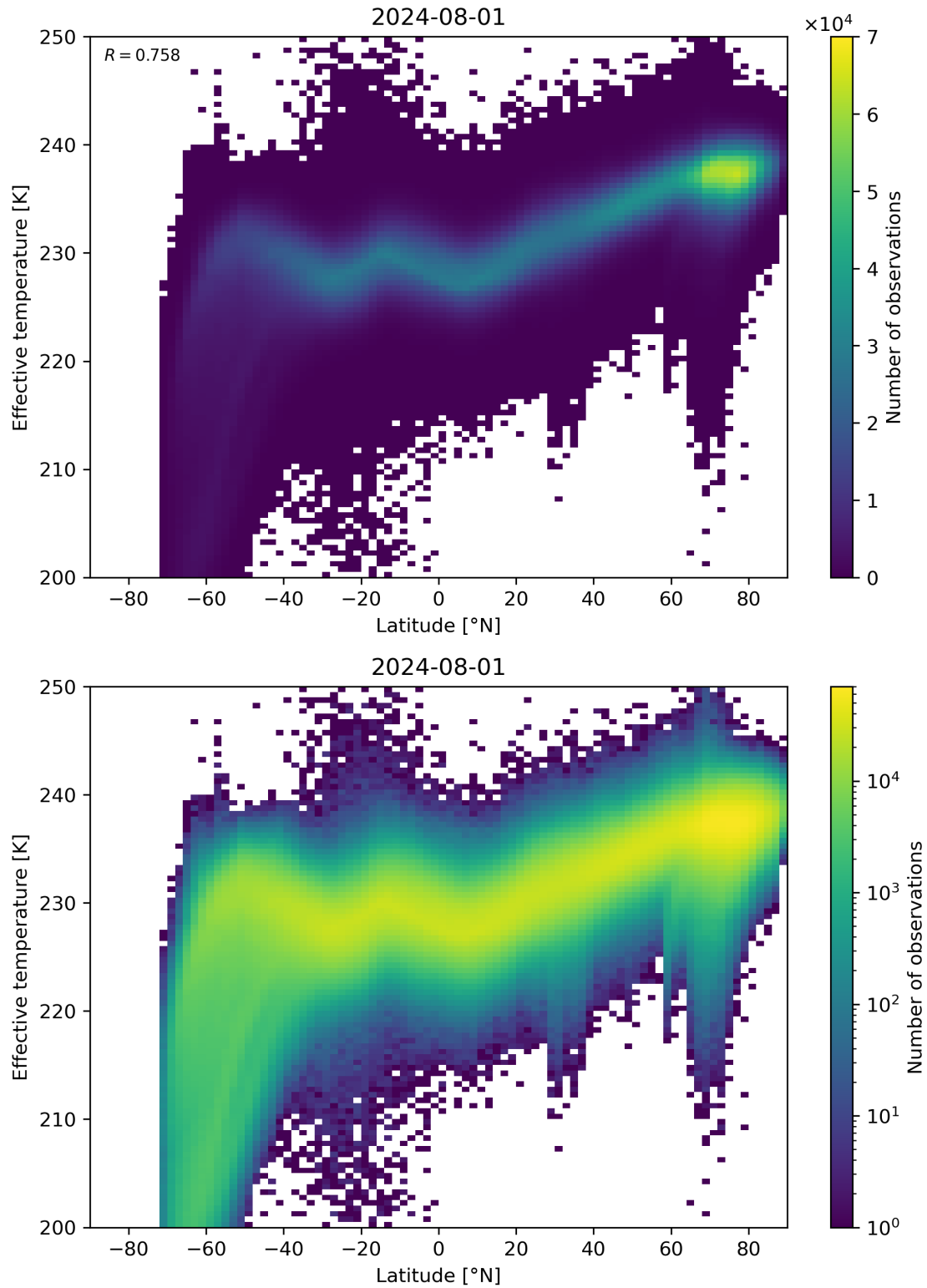
Figure 34: Scatter density plot of “Latitude” against “Effective temperature” for 2024-07-31 to 2024-08-02.
