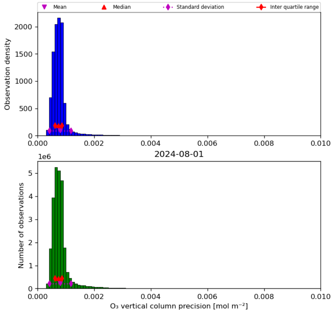
Figure 22: Histogram of “O 3 vertical column precision” for 2024-07-31 to 2024-08-02
