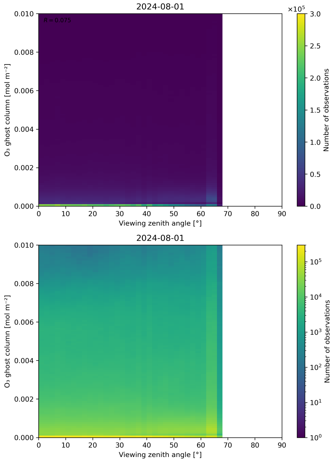
Figure 51: Scatter density plot of “Viewing zenith angle” against “O 3 ghost column” for 2024-07-31 to 2024-08-02.
