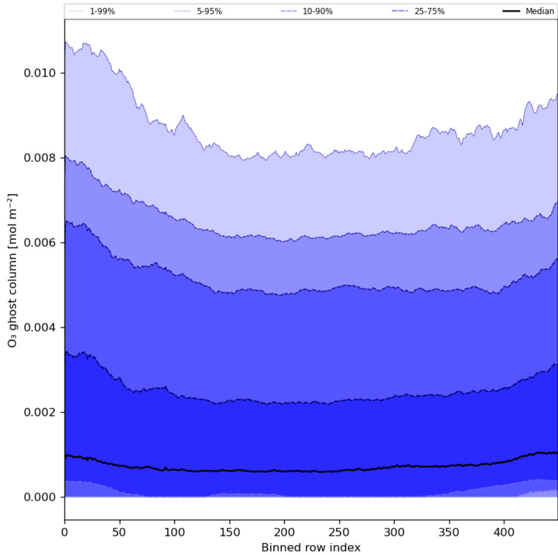
Figure 32: Along track statistics of “O 3 ghost column” for 2024-07-31 to 2024-08-02
