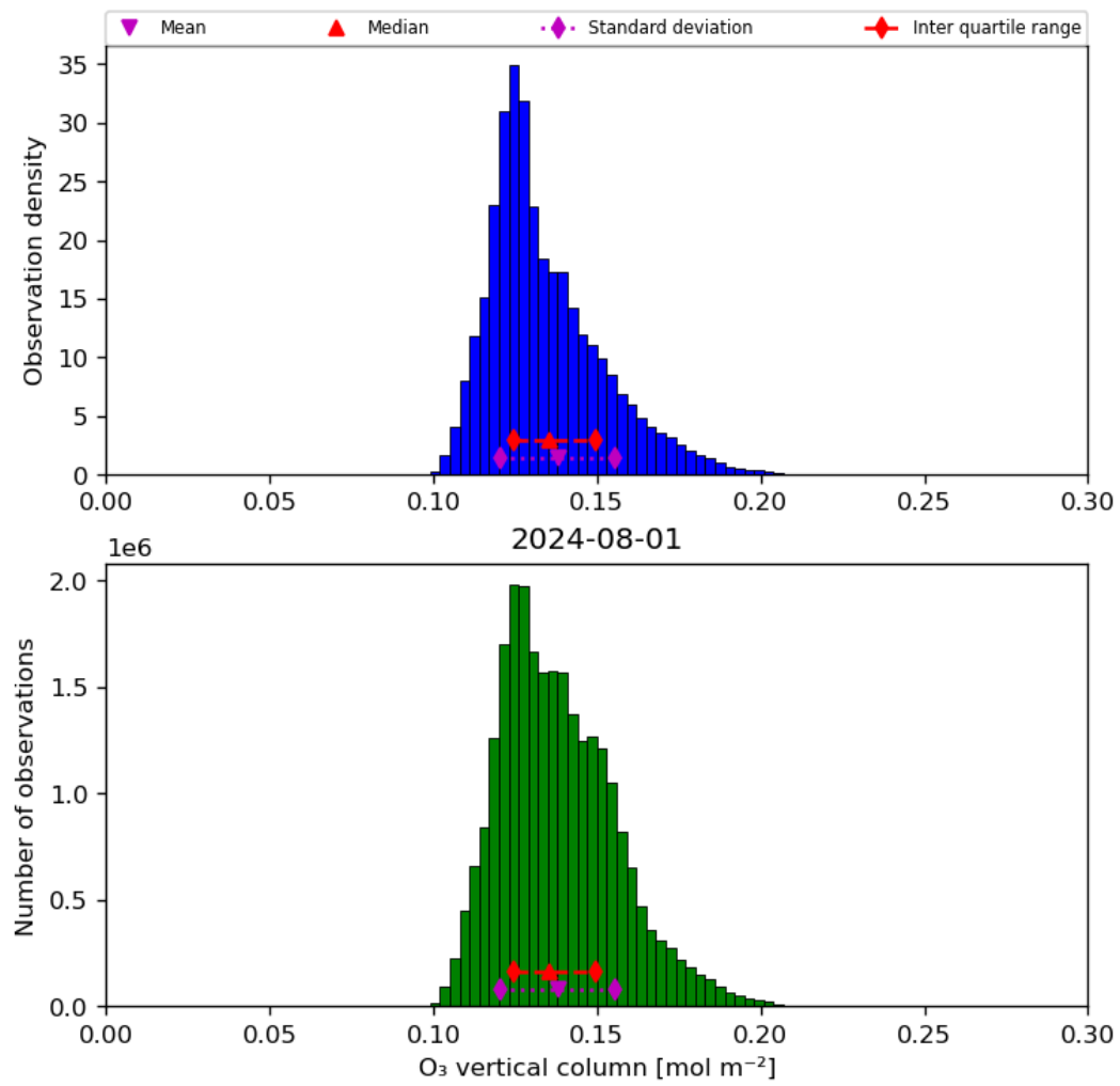
Figure 21: Histogram of “O 3 vertical column” for 2024-07-31 to 2024-08-02
