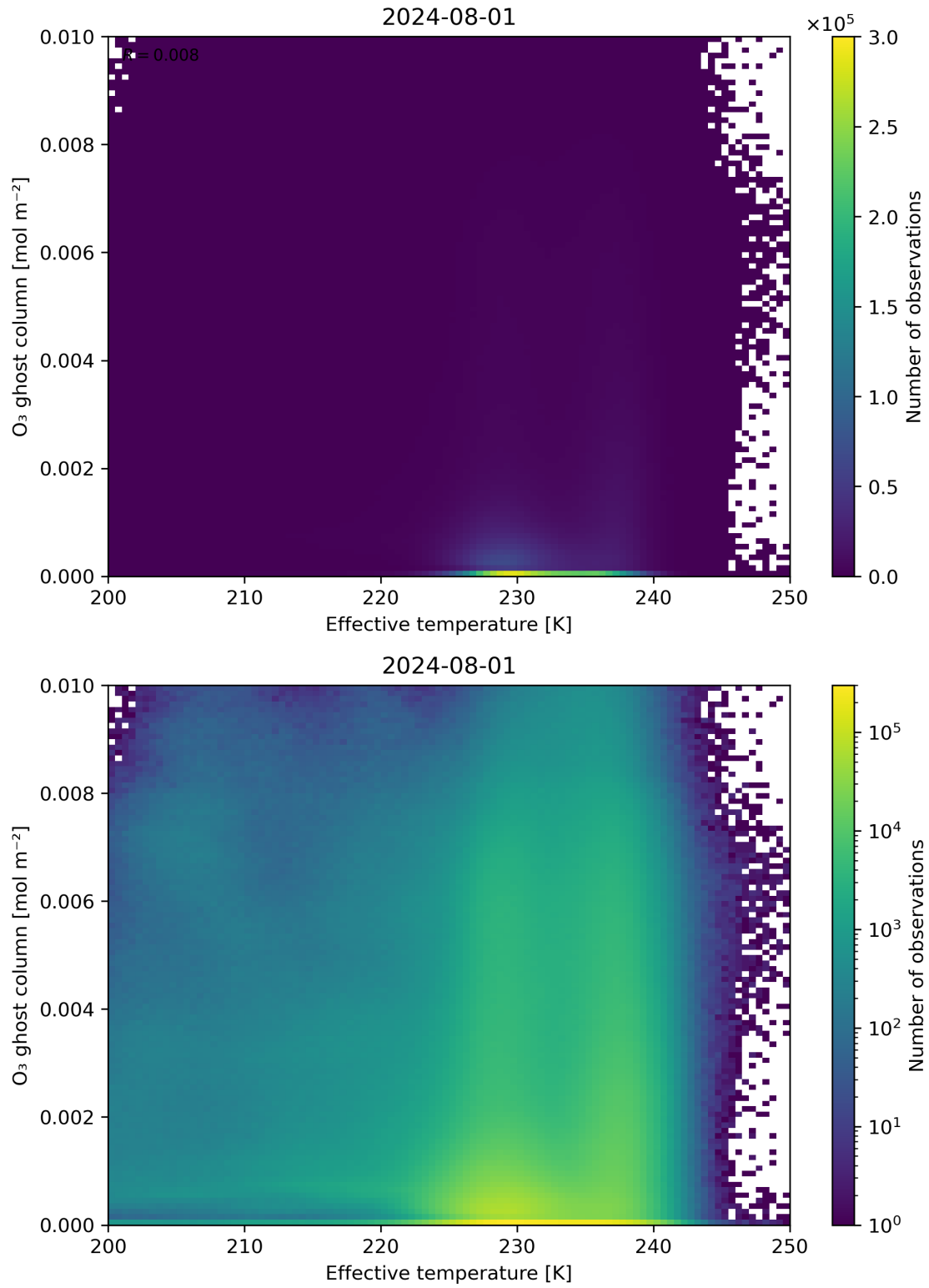
Figure 38: Scatter density plot of “Effective temperature” against “O 3 ghost column” for 2024-07-31 to 2024-08-02.
