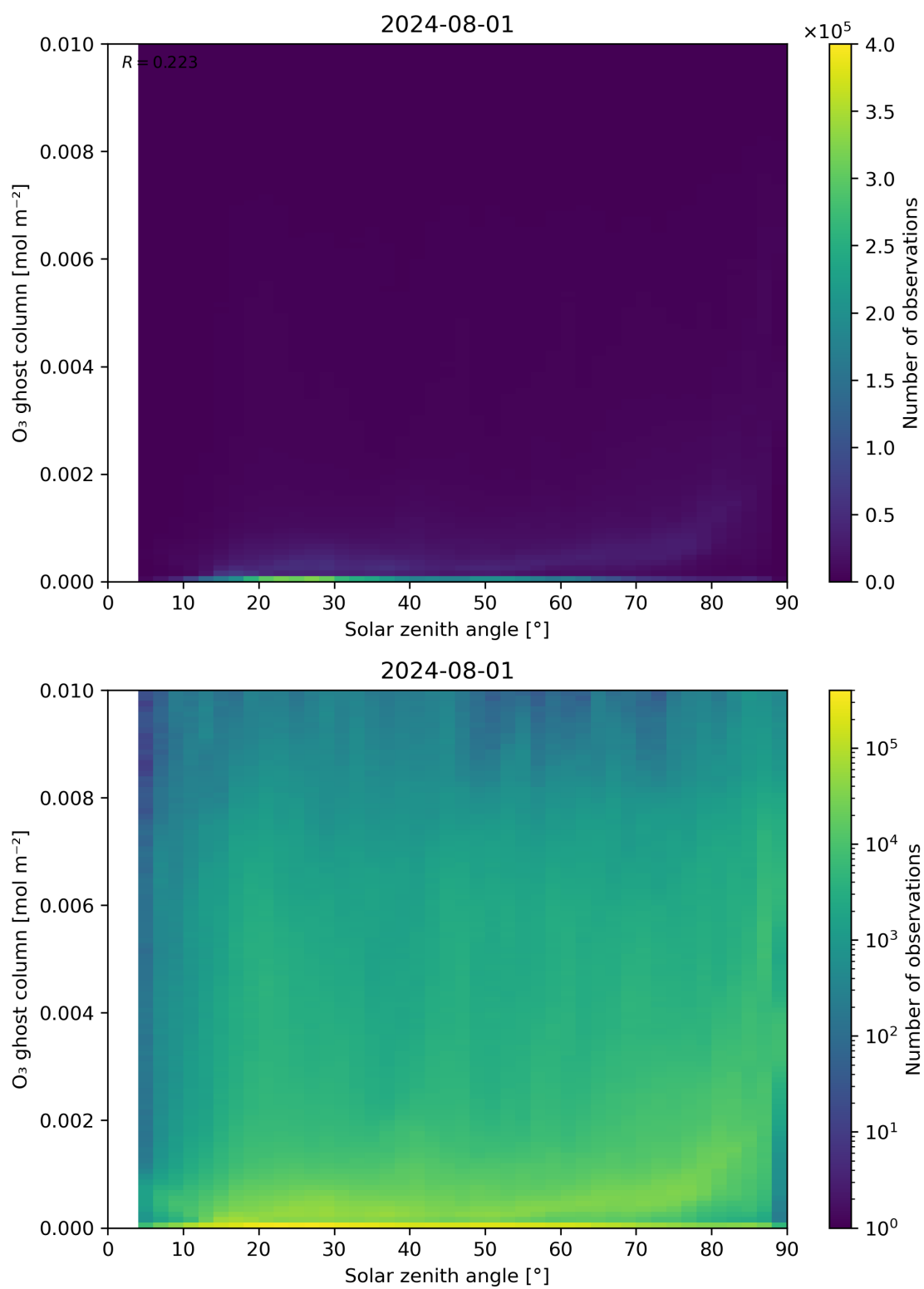
Figure 46: Scatter density plot of “Solar zenith angle” against “O 3 ghost column” for 2024-07-31 to 2024-08-02.
