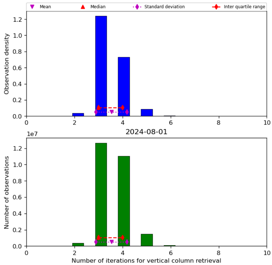
Figure 26: Histogram of “Number of iterations for vertical column retrieval” for 2024-07-31 to 2024-08-02
