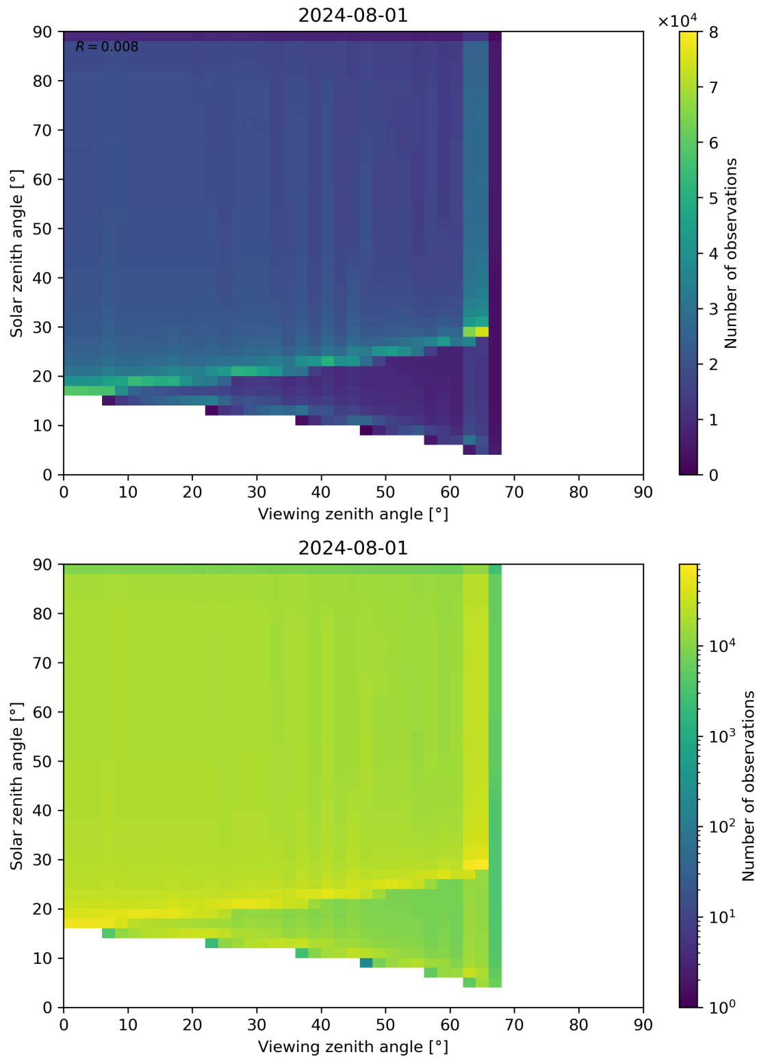
Figure 54: Scatter density plot of “Viewing zenith angle” against “Solar zenith angle” for 2024-07-31 to 2024-08-02.
