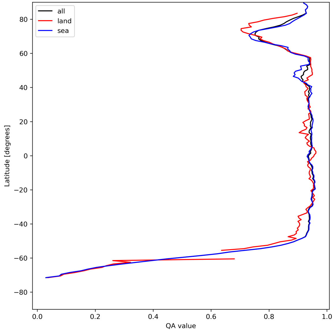
Figure 13: Zonal average of “QA value” for 2024-07-31 to 2024-08-02.
