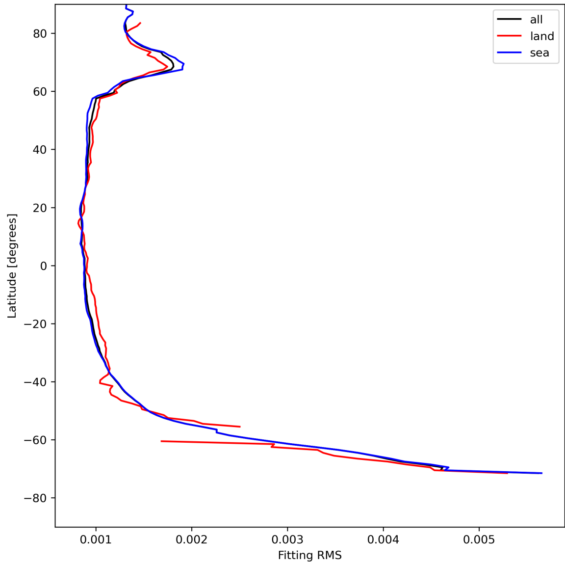
Figure 16: Zonal average of “Fitting RMS” for 2024-07-31 to 2024-08-02.
