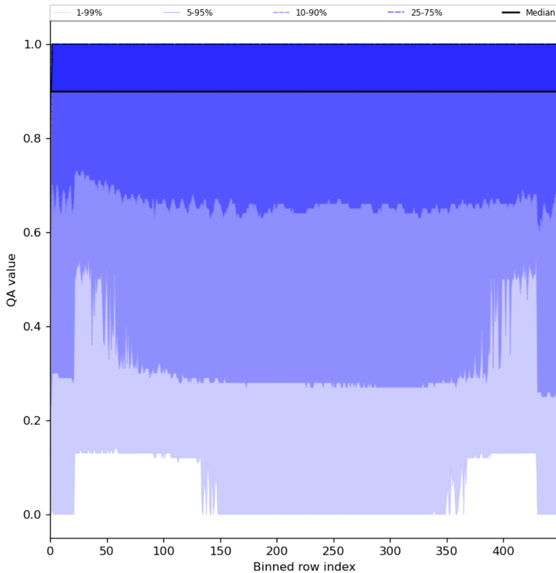
Figure 27: Along track statistics of “QA value” for 2024-07-31 to 2024-08-02
