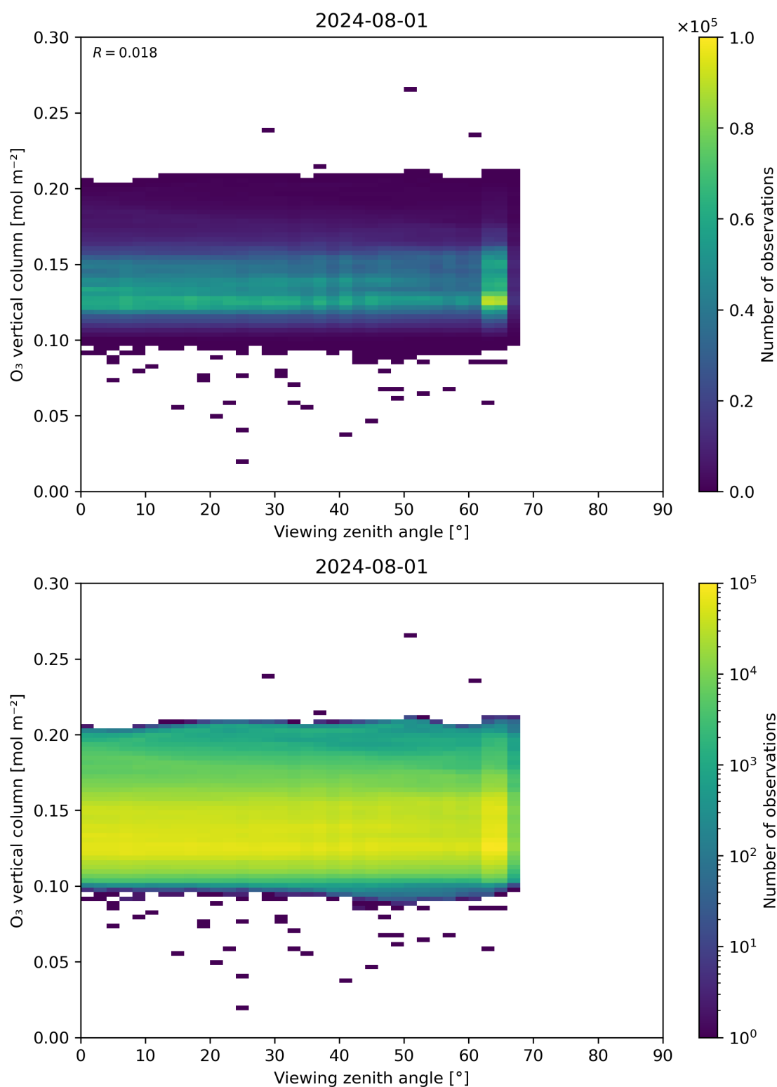
Figure 52: Scatter density plot of “Viewing zenith angle” against “O 3 vertical column” for 2024-07-31 to 2024-08-02.
