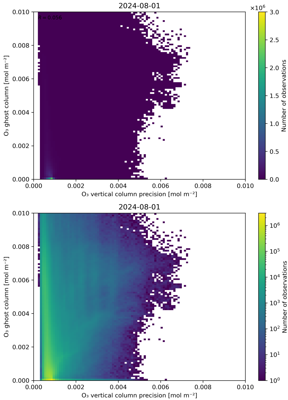
Figure 43: Scatter density plot of “ O_3 vertical column precision” against “ O_3 ghost column” for 2024-07-31 to 2024-08-02.
