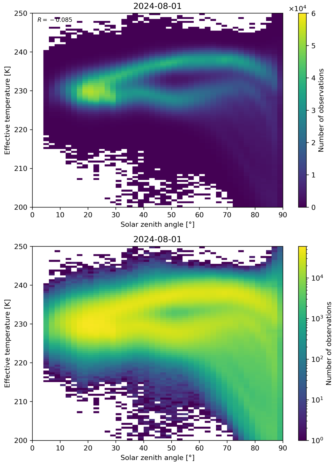
Figure 45: Scatter density plot of “Solar zenith angle” against “Effective temperature” for 2024-07-31 to 2024-08-02.
