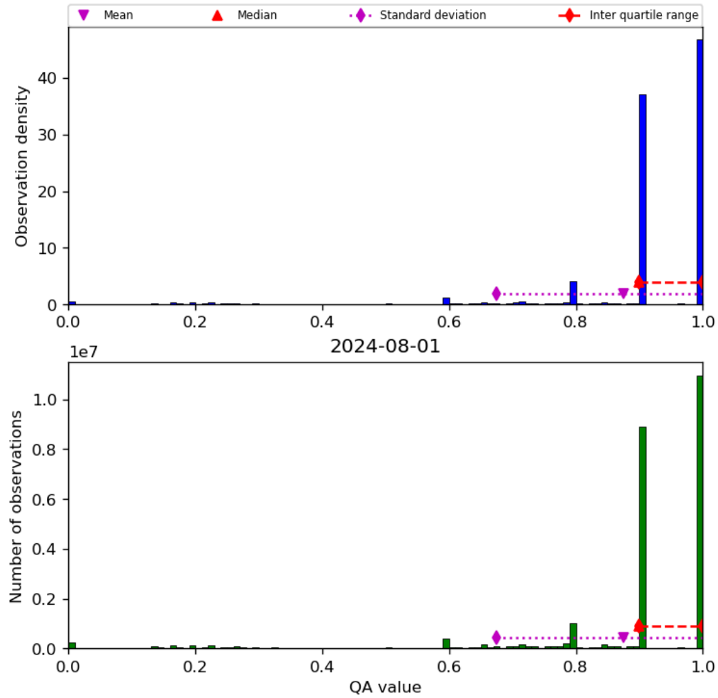
Figure 20: Histogram of “QA value” for 2024-07-31 to 2024-08-02
