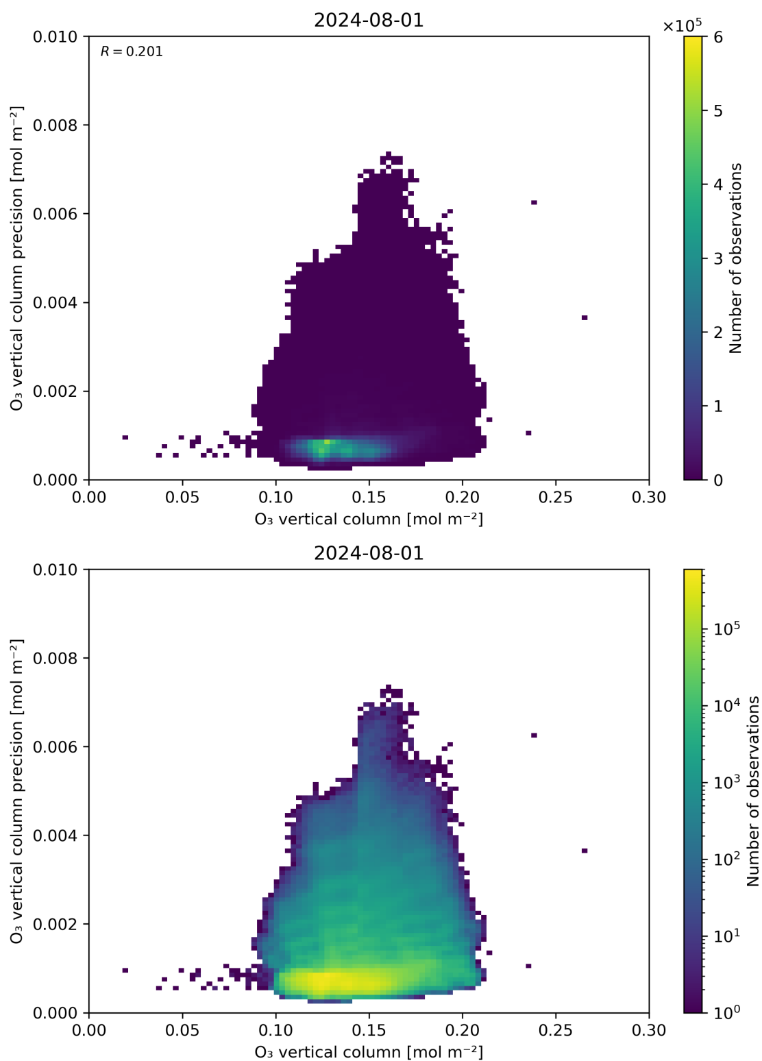
Figure 41: Scatter density plot of “O 3 vertical column” against “O 3 vertical column precision” for 2024-07-31 to 2024-08-02.
