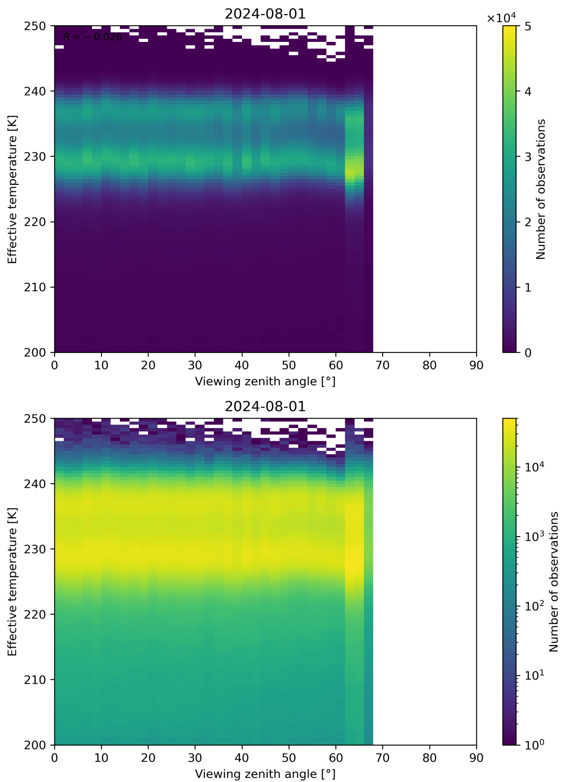
Figure 50: Scatter density plot of “Viewing zenith angle” against “Effective temperature” for 2024-07-31 to 2024-08-02.
