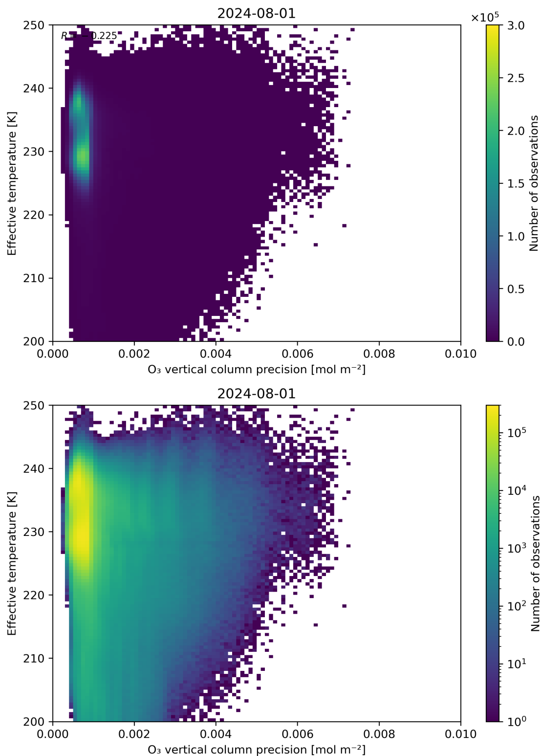
Figure 42: Scatter density plot of “O 3 vertical column precision” against “Effective temperature” for 2024-07-31 to 2024-08-02.
