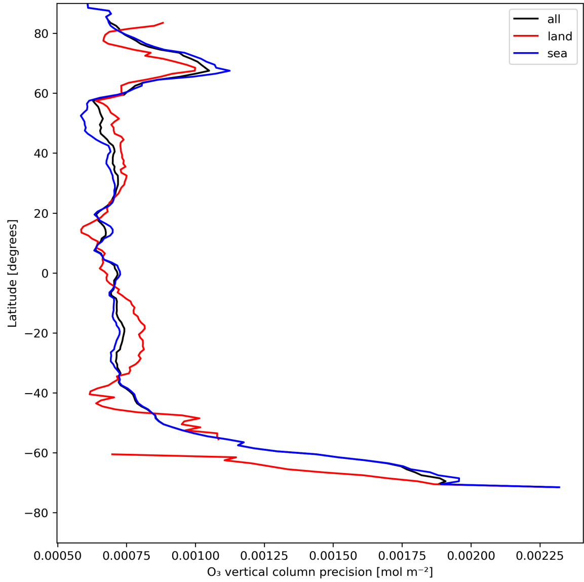
Figure 15: Zonal average of "O 3 vertical column precision" for 2024-07-31 to 2024-08-02.
