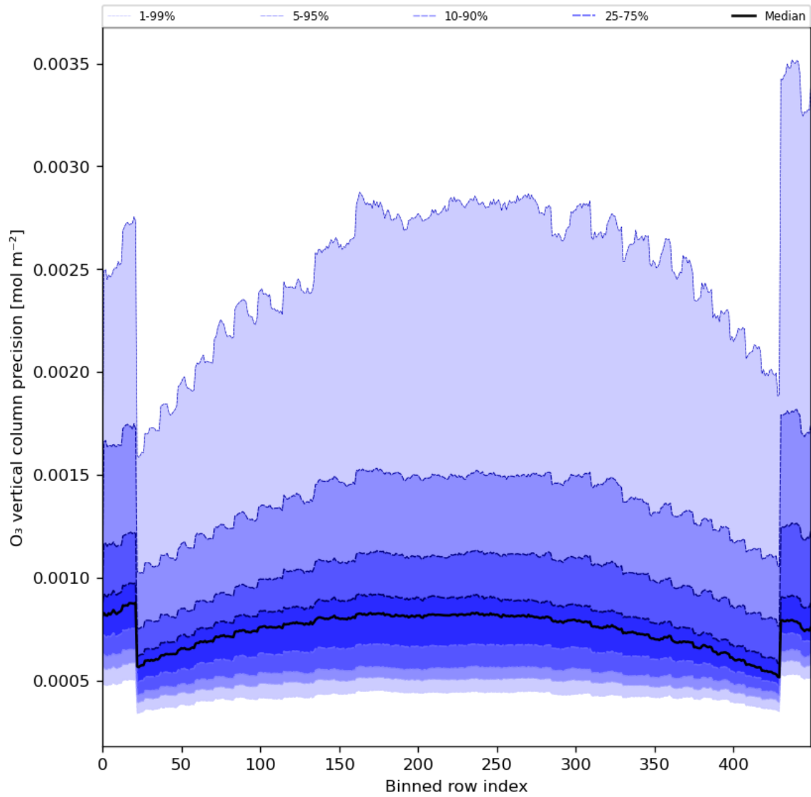
Figure 29: Along track statistics of “O 3 vertical column precision” for 2024-07-31 to 2024-08-02
