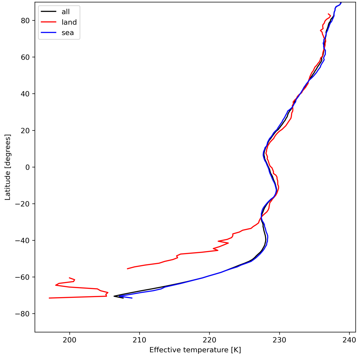
Figure 17: Zonal average of "Effective temperature" for 2024-07-31 to 2024-08-02.
