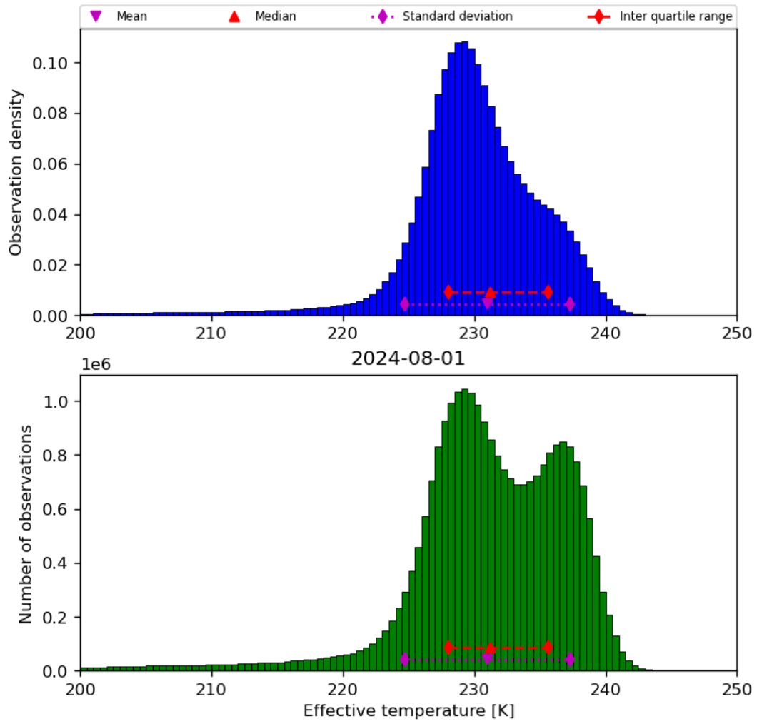
Figure 24: Histogram of “Effective temperature” for 2024-07-31 to 2024-08-02
