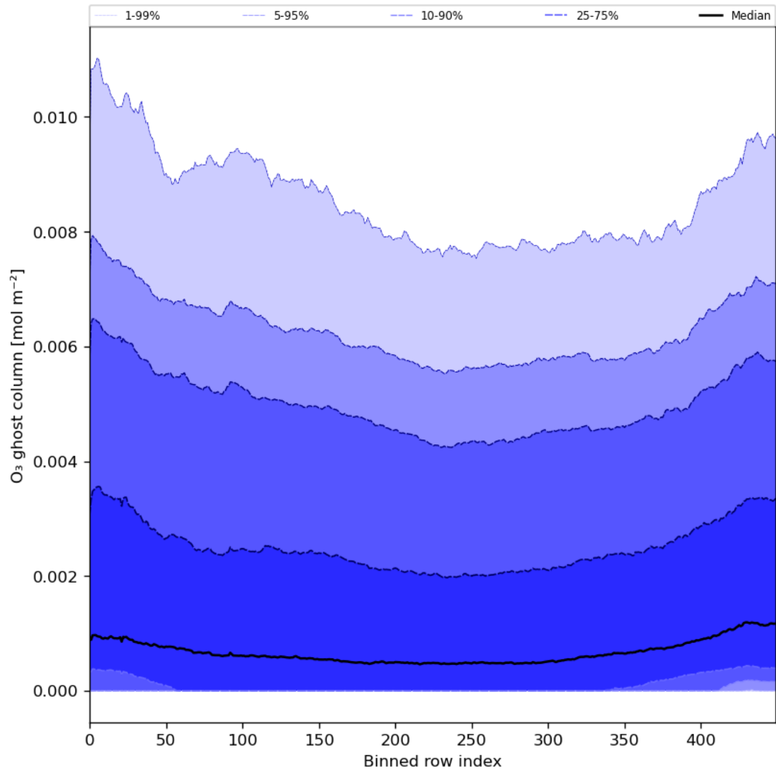
Figure 32: Along track statistics of “O 3 ghost column” for 2024-08-02 to 2024-08-04
