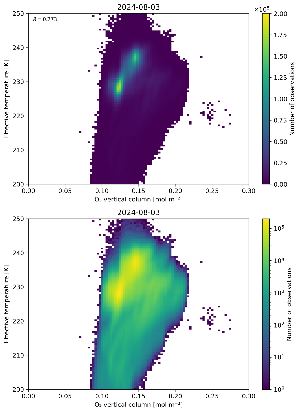
Figure 39: Scatter density plot of “O 3 vertical column” against “Effective temperature” for 2024-08-02 to 2024-08-04.
