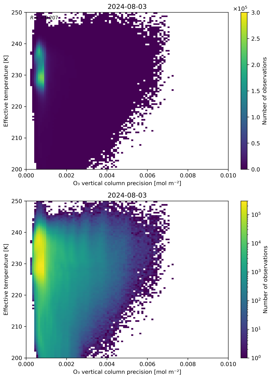
Figure 42: Scatter density plot of “O 3 vertical column precision” against “Effective temperature” for 2024-08-02 to 2024-08-04.
