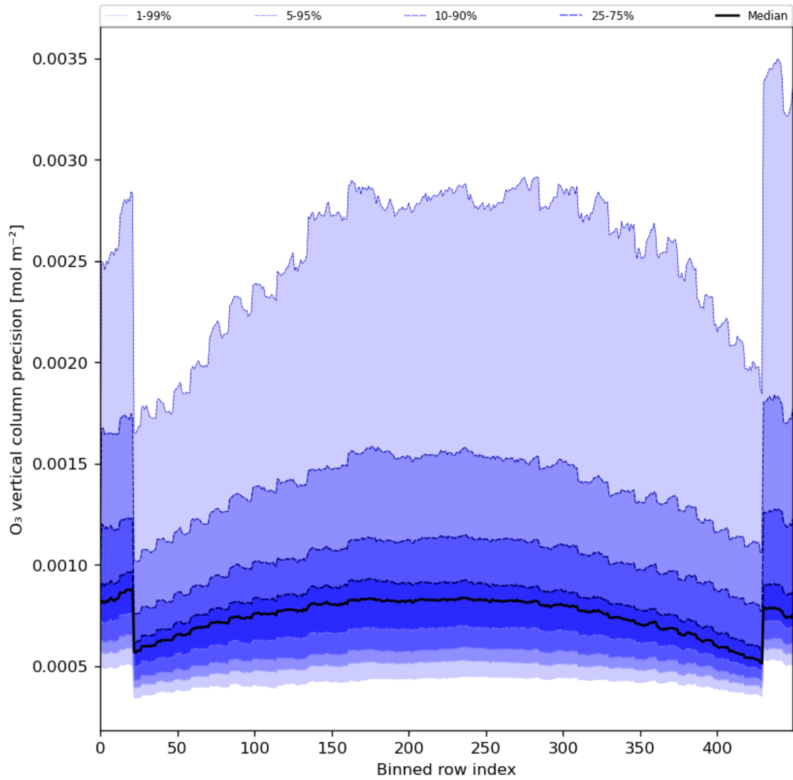
Figure 29: Along track statistics of “O 3 vertical column precision” for 2024-08-02 to 2024-08-04
