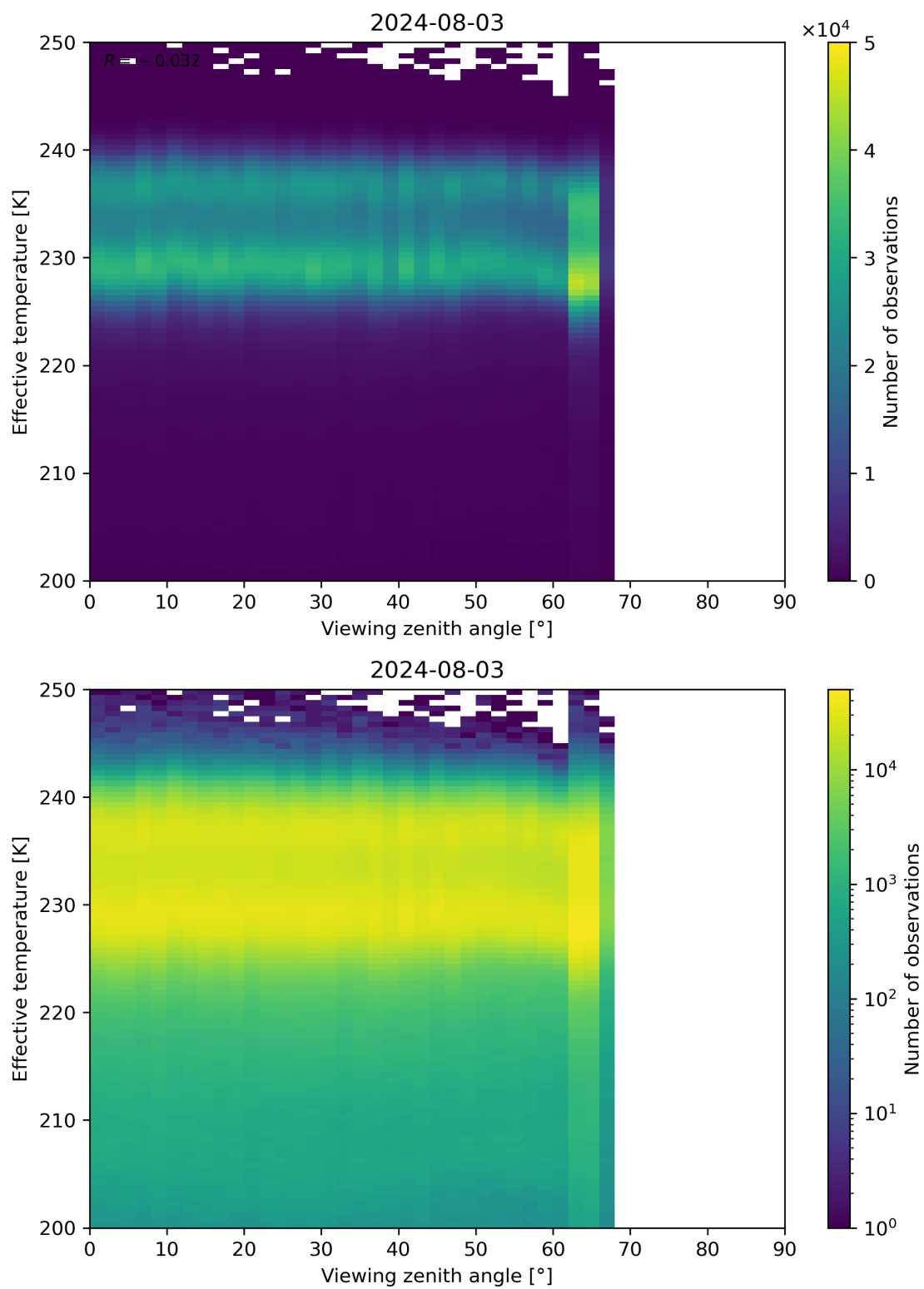
Figure 50: Scatter density plot of “Viewing zenith angle” against “Effective temperature” for 2024-08-02 to 2024-08-04.
