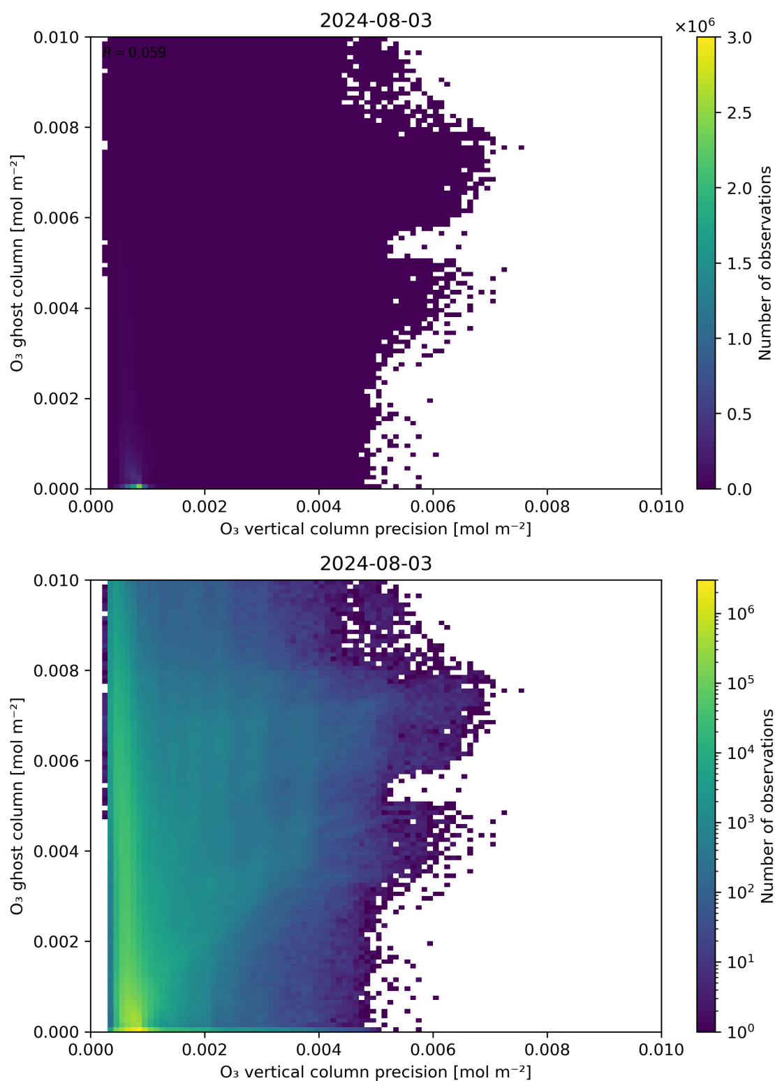
Figure 43: Scatter density plot of “ \text{O}_3 vertical column precision” against “ \text{O}_3 ghost column” for 2024-08-02 to 2024-08-04.
