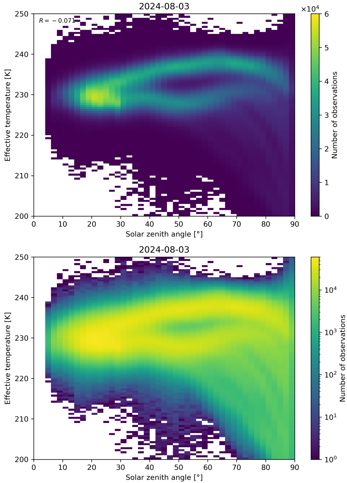
Figure 45: Scatter density plot of “Solar zenith angle” against “Effective temperature” for 2024-08-02 to 2024-08-04.
