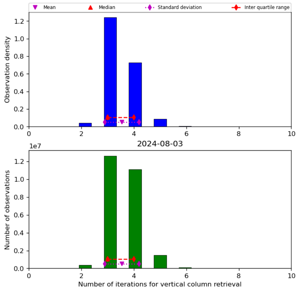
Figure 26: Histogram of “Number of iterations for vertical column retrieval” for 2024-08-02 to 2024-08-04
