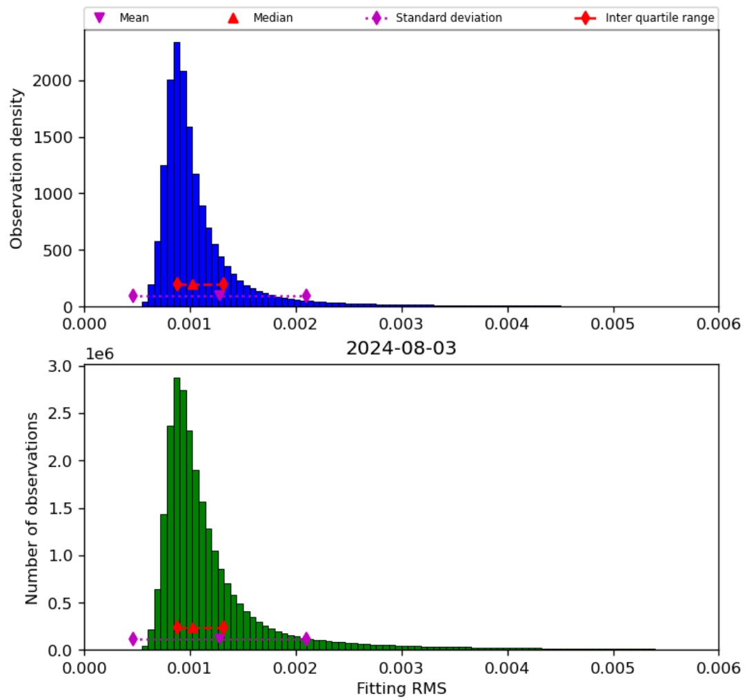
Figure 23: Histogram of “Fitting RMS” for 2024-08-02 to 2024-08-04
