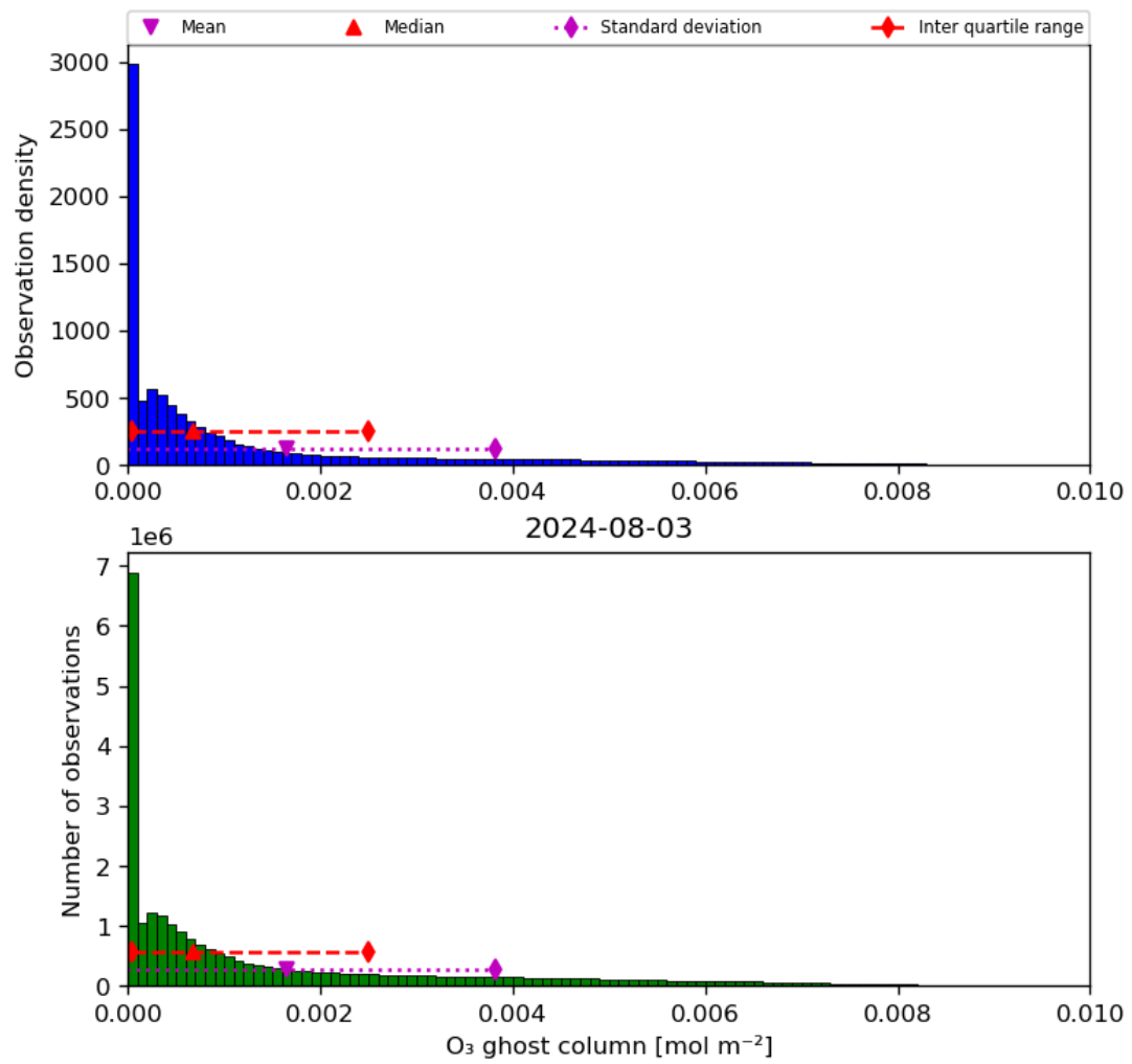
Figure 25: Histogram of “O 3 ghost column” for 2024-08-02 to 2024-08-04
