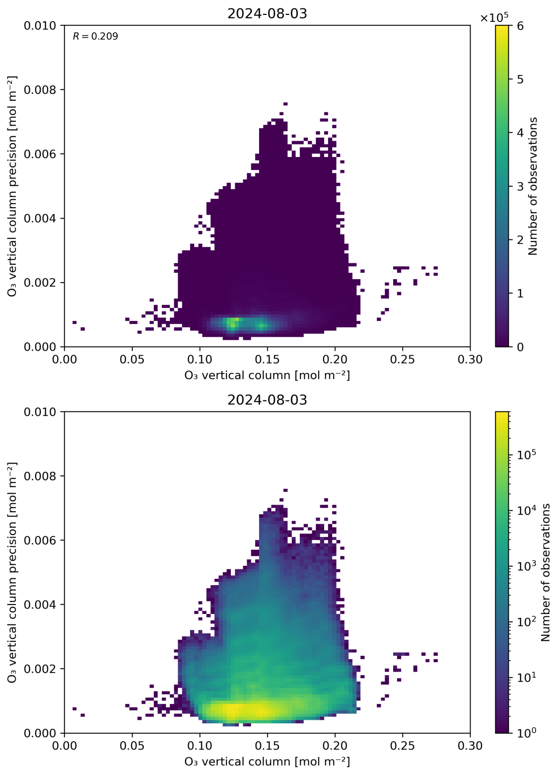
Figure 41: Scatter density plot of “O 3 vertical column” against “O 3 vertical column precision” for 2024-08-02 to 2024-08-04.
