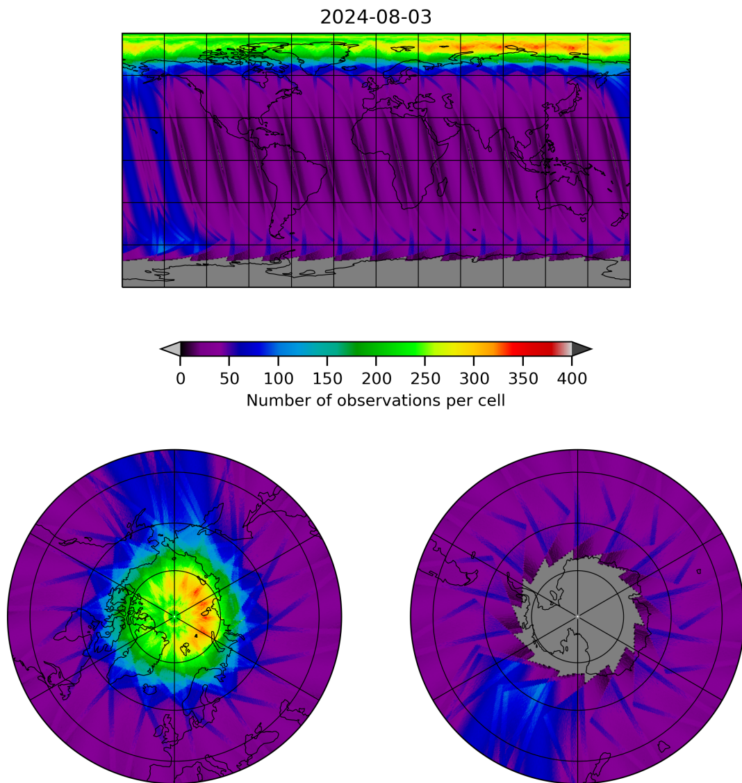
Figure 12: Map of the number of observations for 2024-08-02 to 2024-08-04
