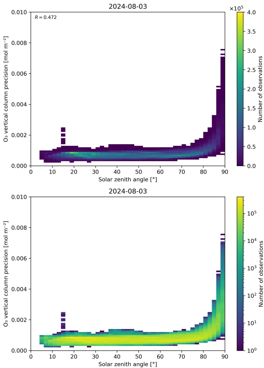
Figure 48: Scatter density plot of “Solar zenith angle” against “O 3 vertical column precision” for 2024-08-02 to 2024-08-04.
