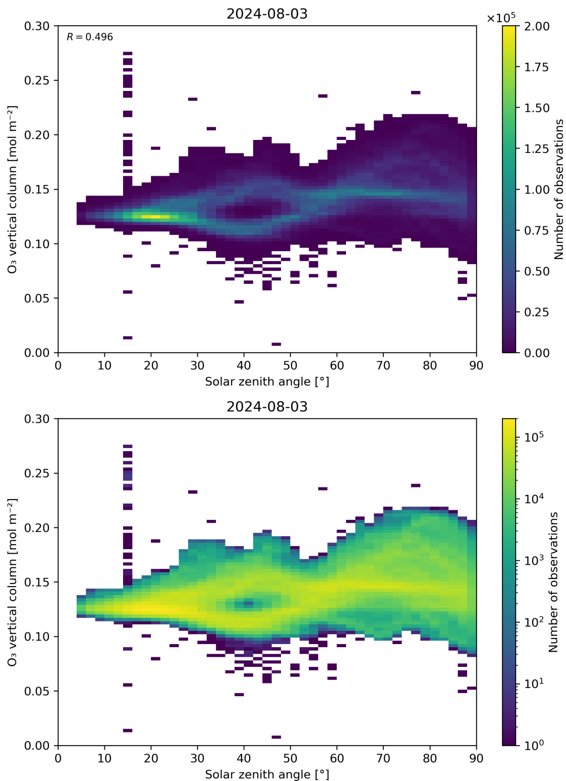
Figure 47: Scatter density plot of “Solar zenith angle” against “O 3 vertical column” for 2024-08-02 to 2024-08-04.
