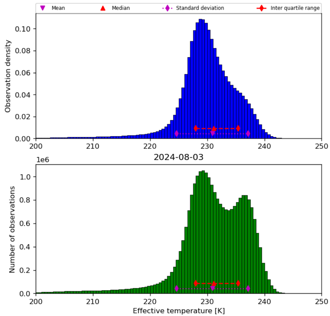
Figure 24: Histogram of “Effective temperature” for 2024-08-02 to 2024-08-04
