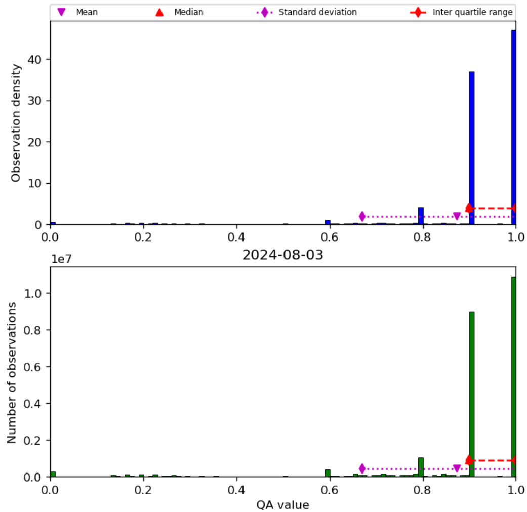
Figure 20: Histogram of “QA value” for 2024-08-02 to 2024-08-04
