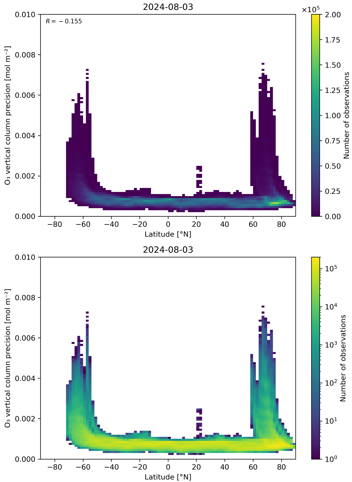
Figure 37: Scatter density plot of “Latitude” against “O 3 vertical column precision” for 2024-08-02 to 2024-08-04.
