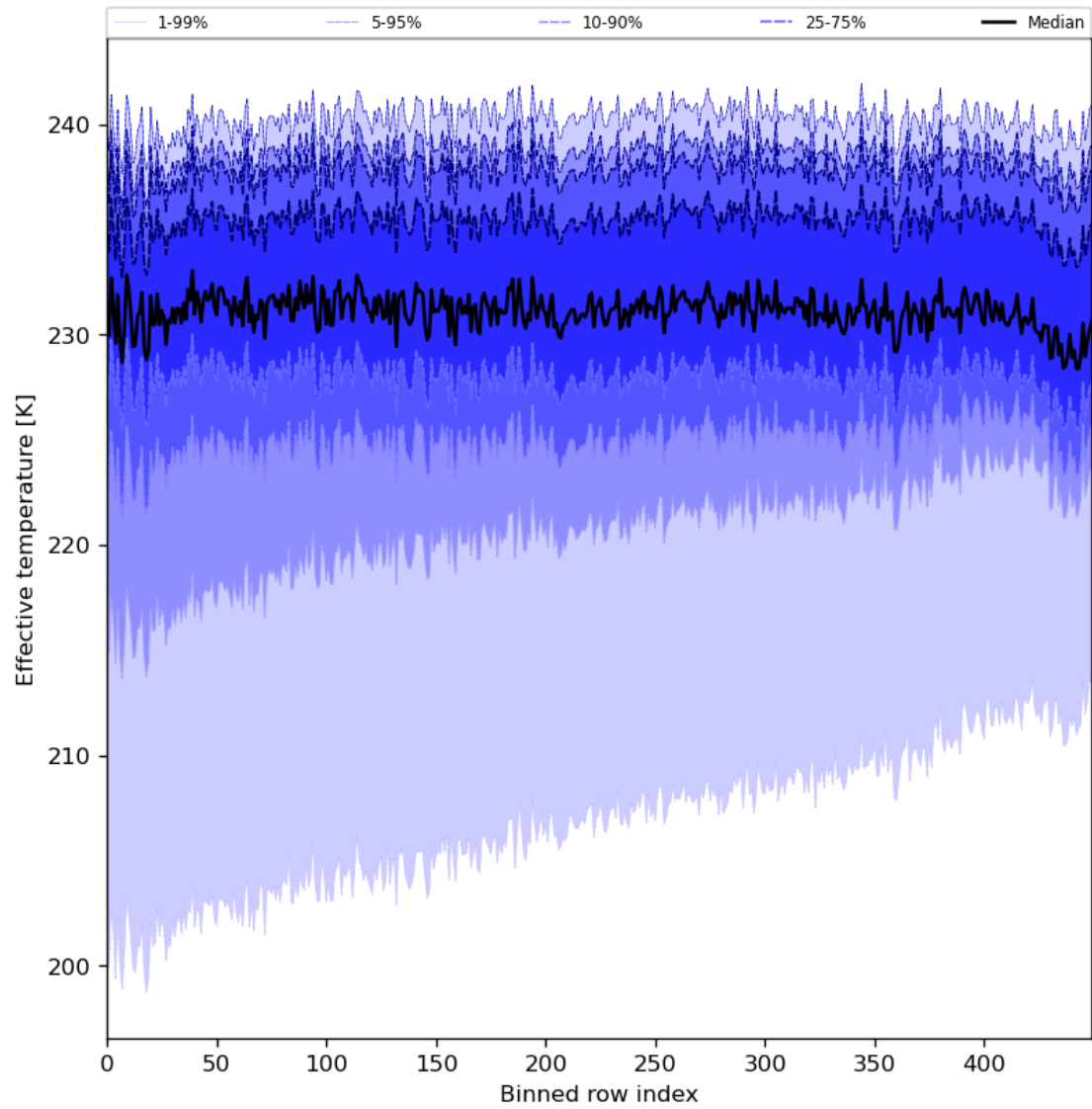
Figure 31: Along track statistics of “Effective temperature” for 2024-08-02 to 2024-08-04
