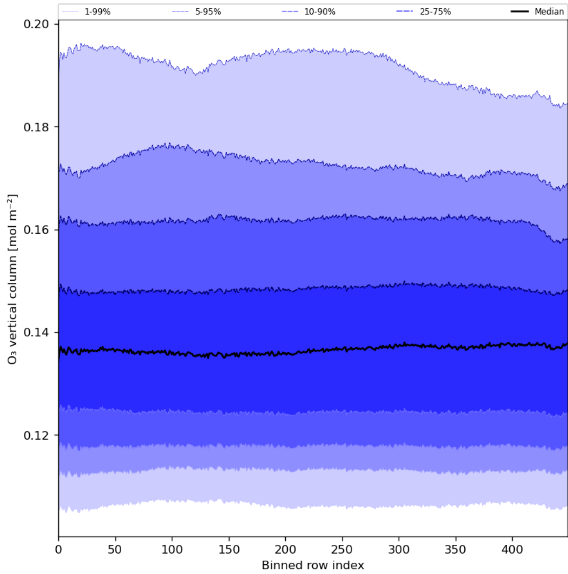
Figure 28: Along track statistics of “O 3 vertical column” for 2024-08-02 to 2024-08-04
