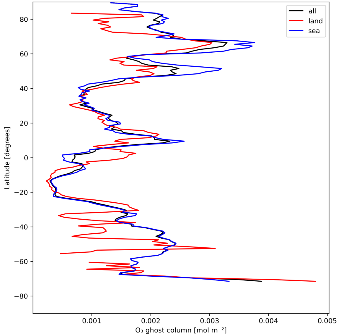
Figure 18: Zonal average of "O 3 ghost column" for 2024-08-02 to 2024-08-04.
