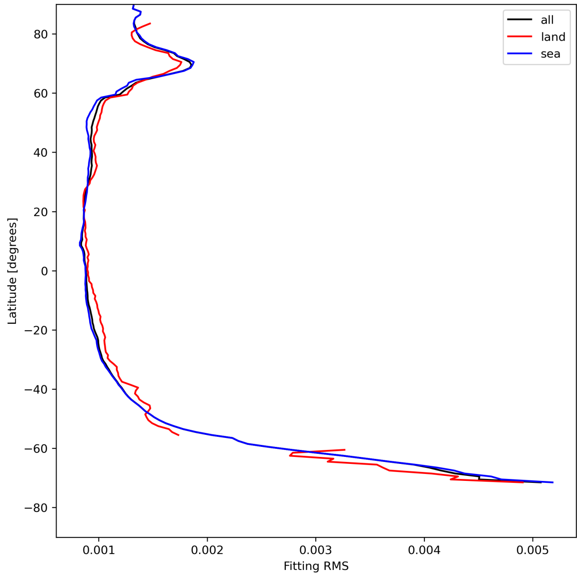
Figure 16: Zonal average of “Fitting RMS” for 2024-08-02 to 2024-08-04.
