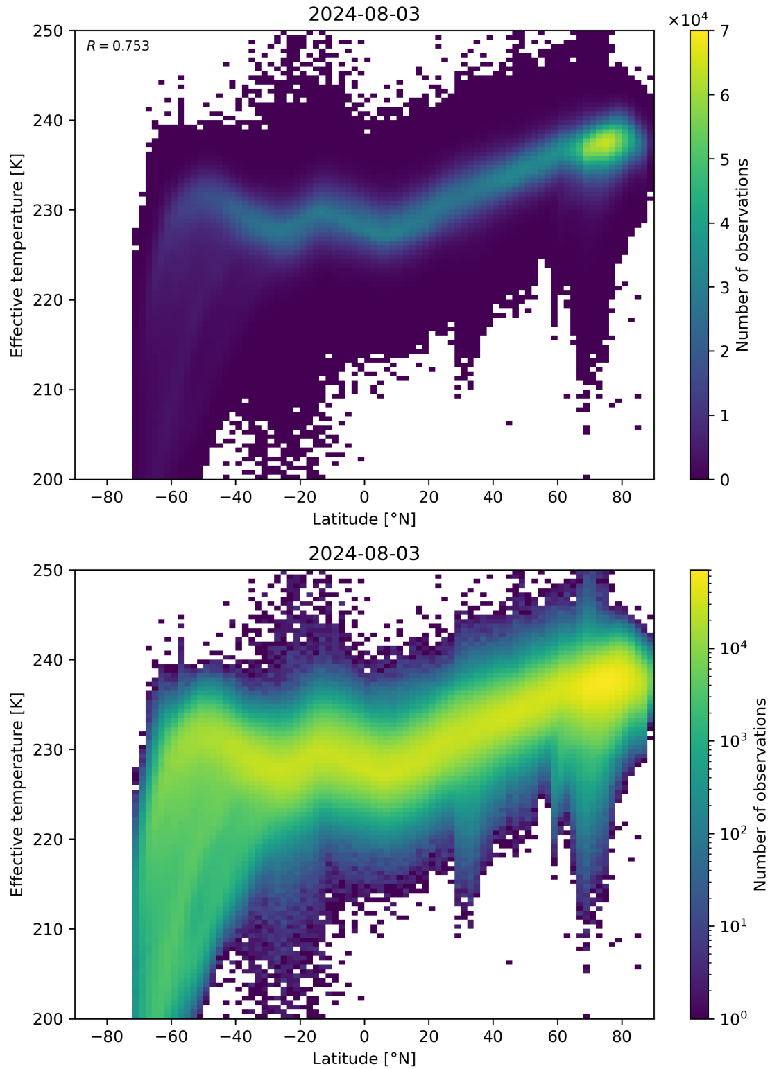
Figure 34: Scatter density plot of “Latitude” against “Effective temperature” for 2024-08-02 to 2024-08-04.
