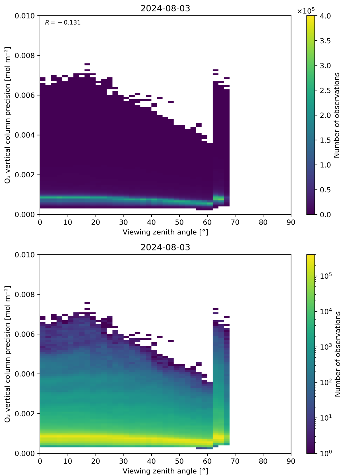
Figure 53: Scatter density plot of “Viewing zenith angle” against “O 3 vertical column precision” for 2024-08-02 to 2024-08-04.
