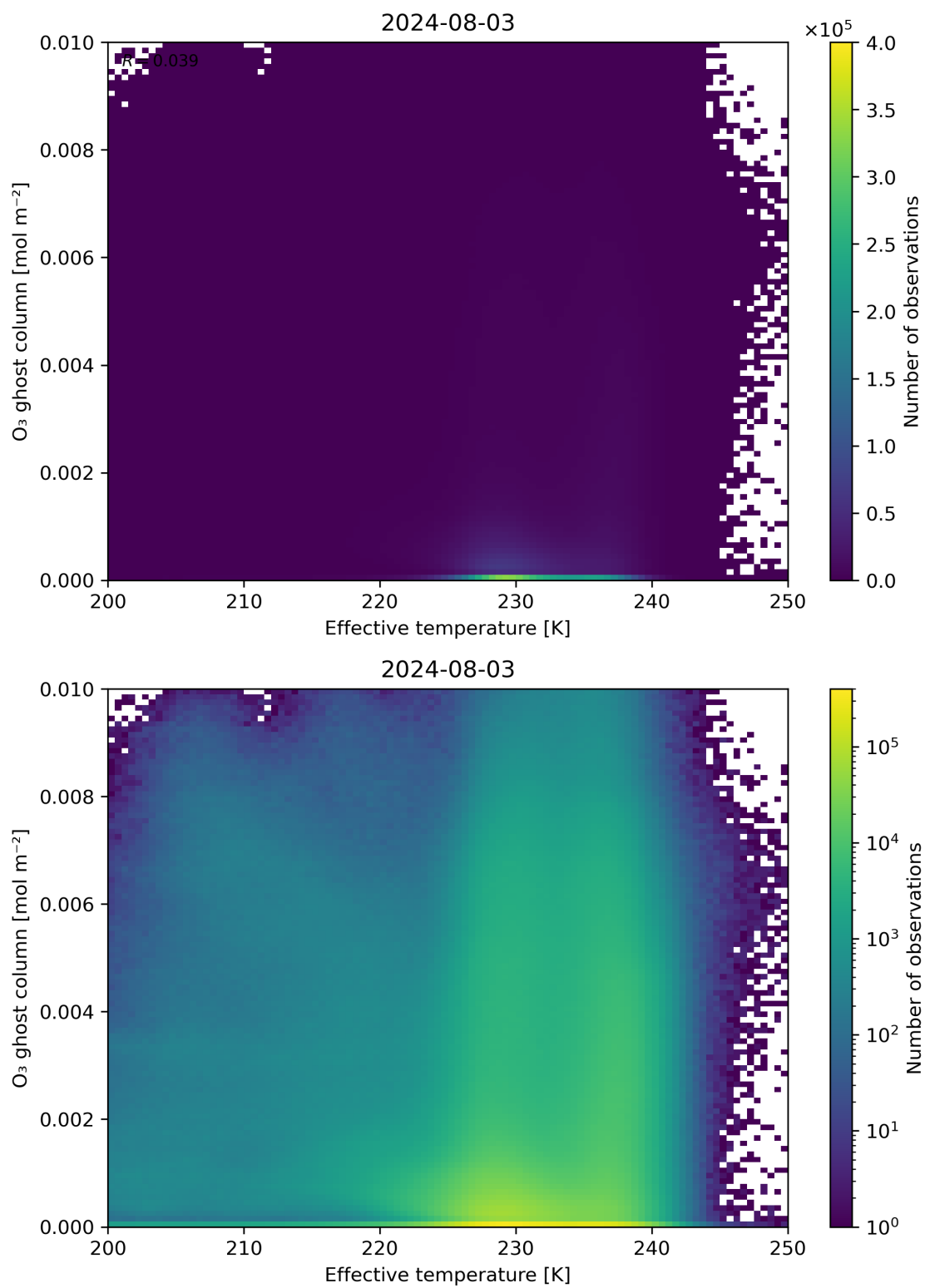
Figure 38: Scatter density plot of “Effective temperature” against “O 3 ghost column” for 2024-08-02 to 2024-08-04.
