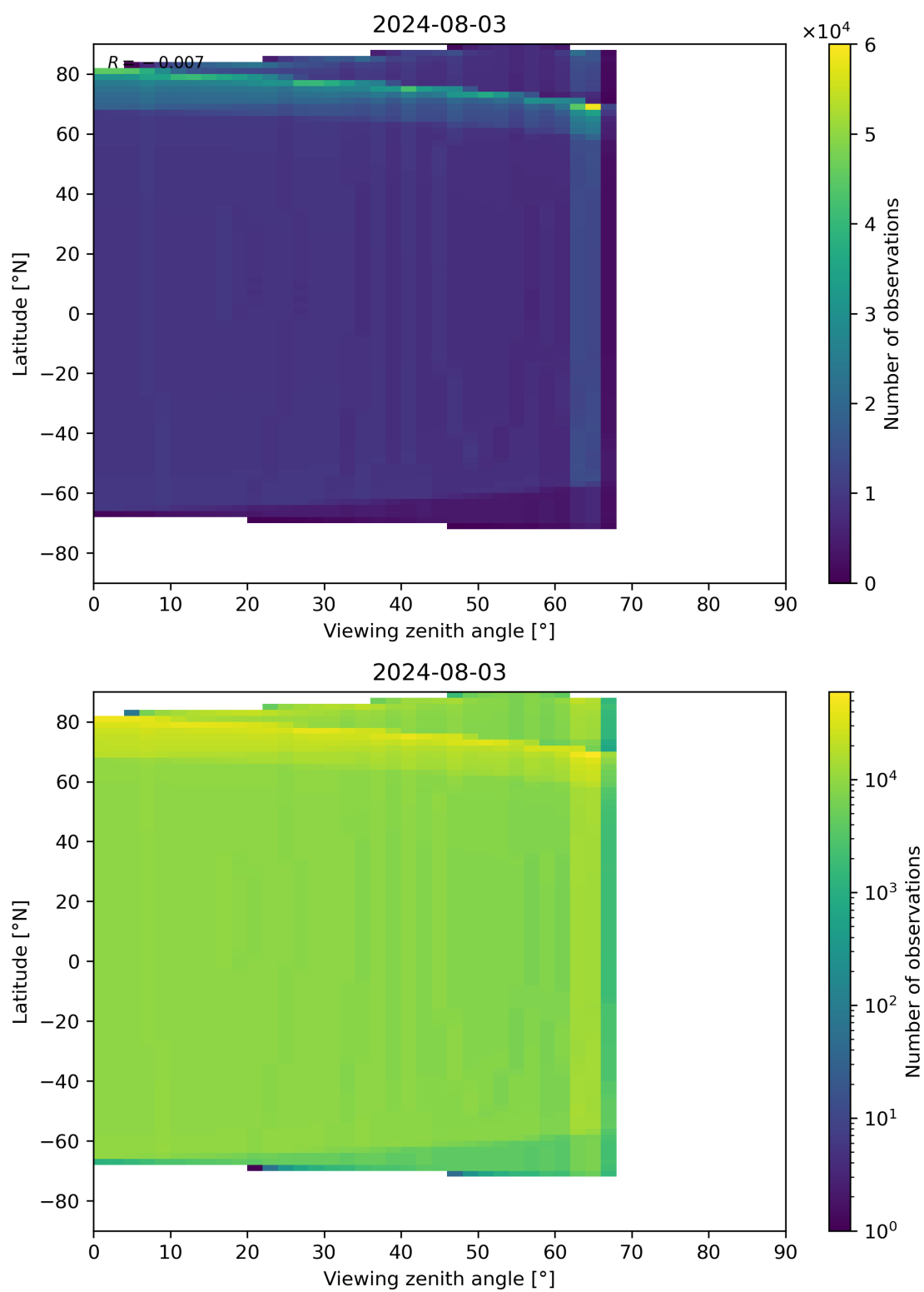
Figure 49: Scatter density plot of “Viewing zenith angle” against “Latitude” for 2024-08-02 to 2024-08-04.
