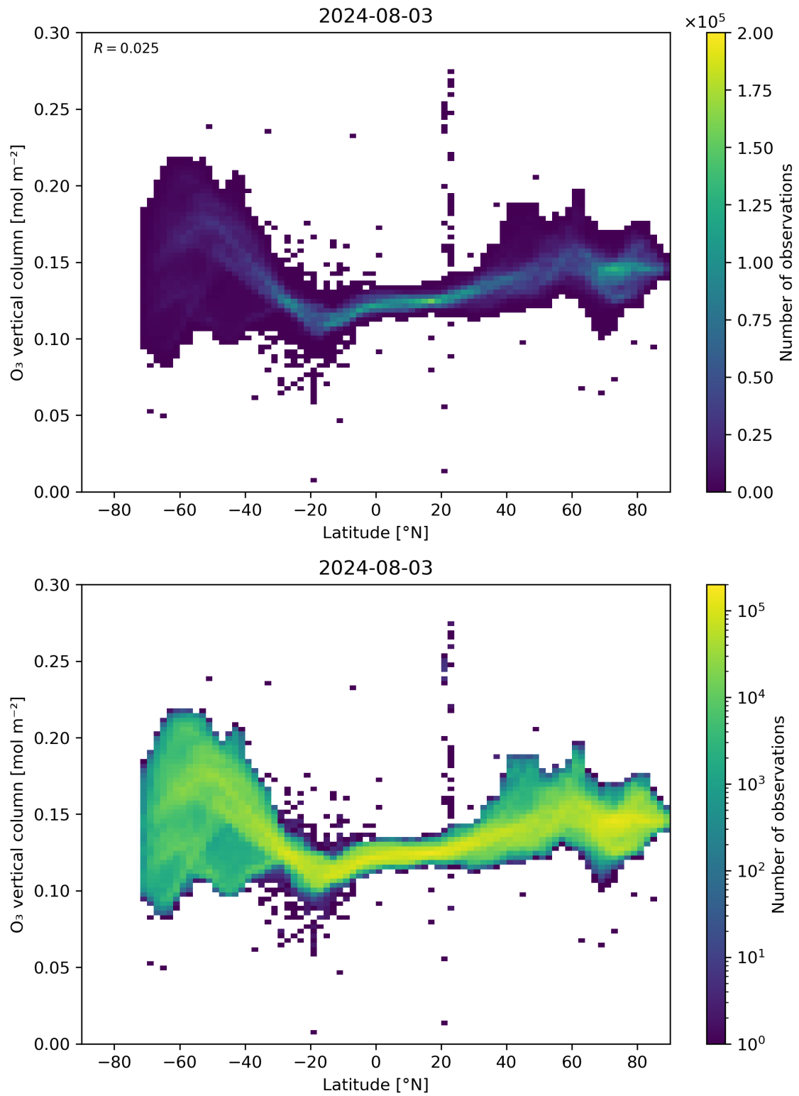
Figure 36: Scatter density plot of “Latitude” against “O 3 vertical column” for 2024-08-02 to 2024-08-04.
