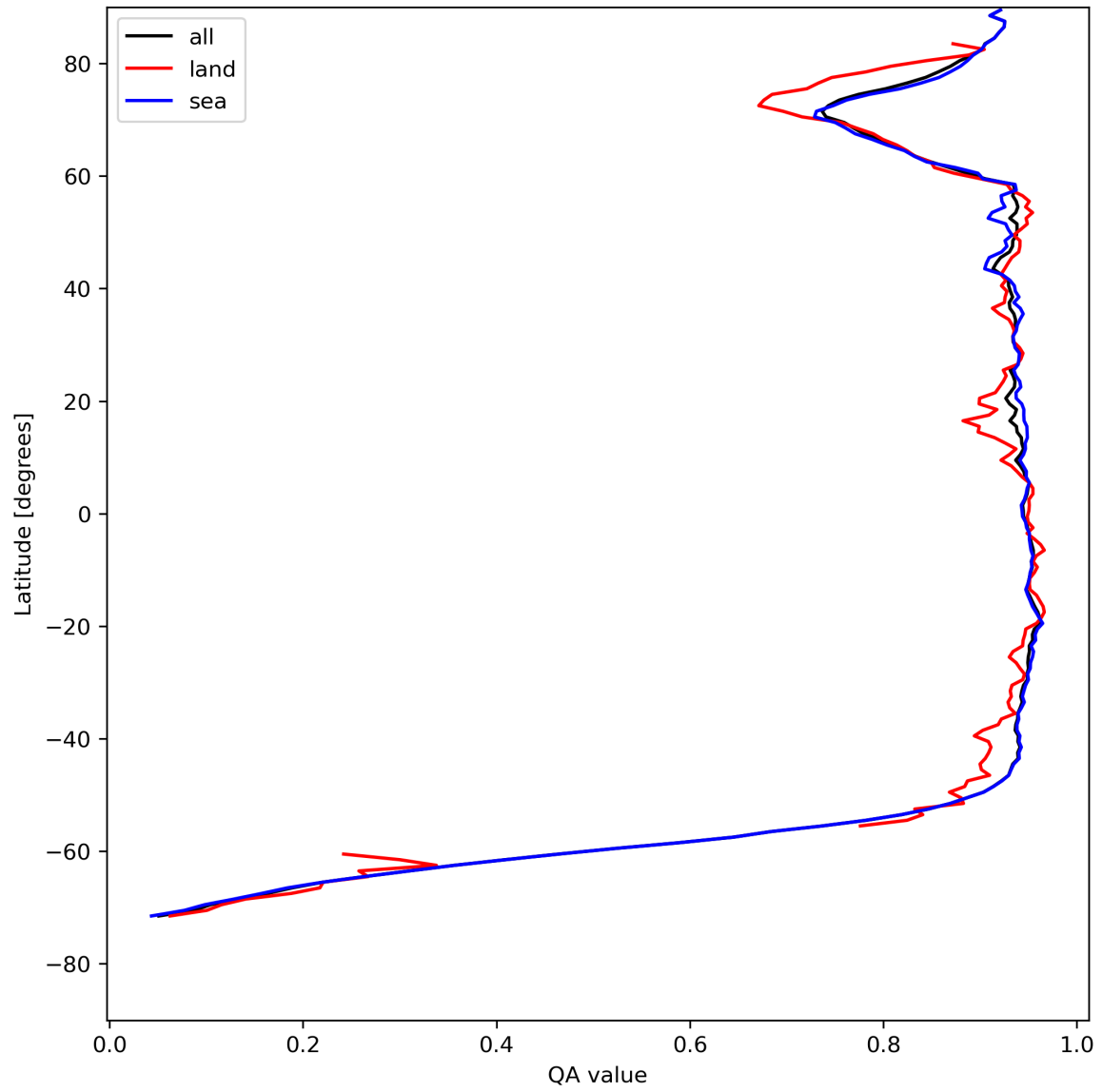
Figure 13: Zonal average of “QA value” for 2024-08-02 to 2024-08-04.
