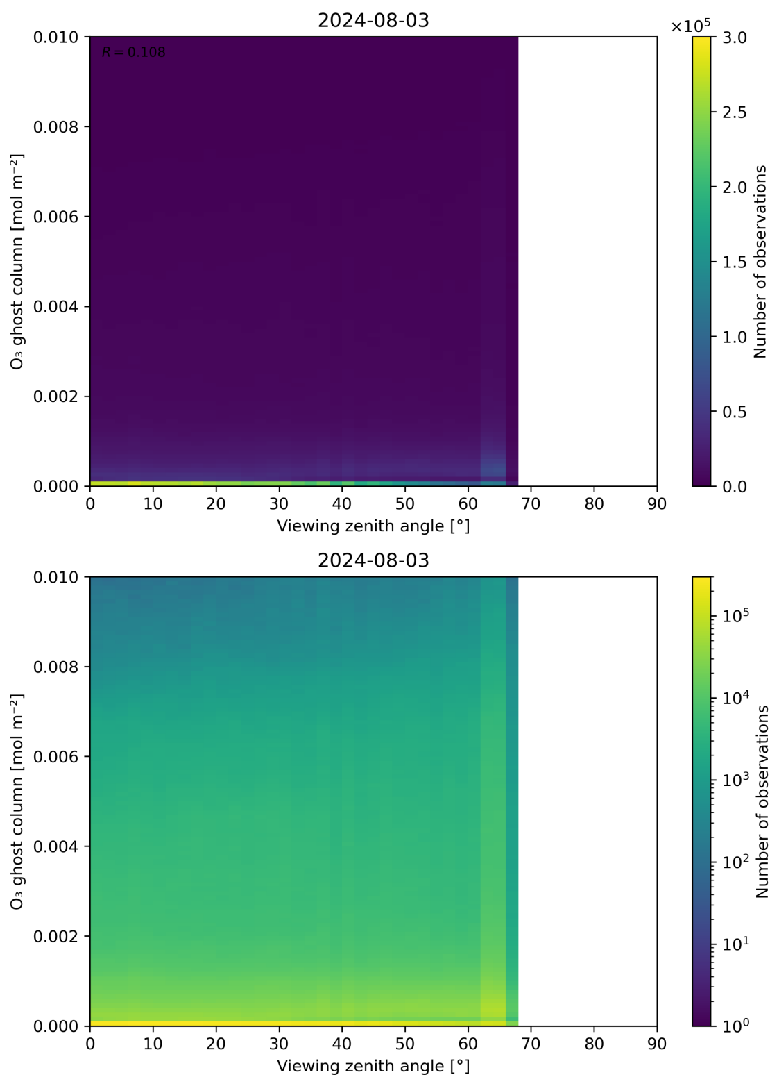
Figure 51: Scatter density plot of “Viewing zenith angle” against “O 3 ghost column” for 2024-08-02 to 2024-08-04.
