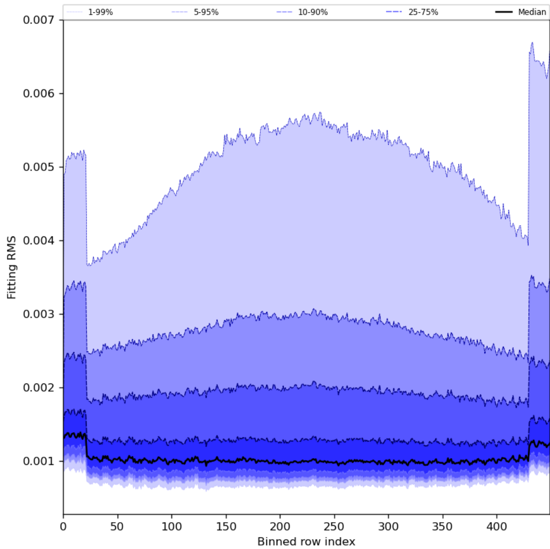
Figure 30: Along track statistics of “Fitting RMS” for 2024-08-02 to 2024-08-04
