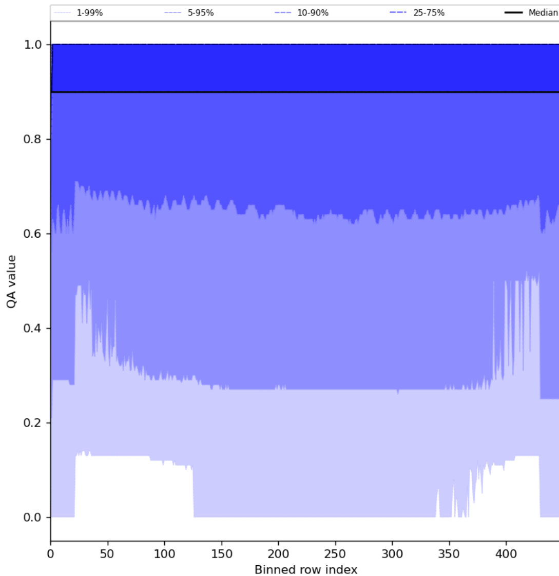
Figure 27: Along track statistics of “QA value” for 2024-08-02 to 2024-08-04
