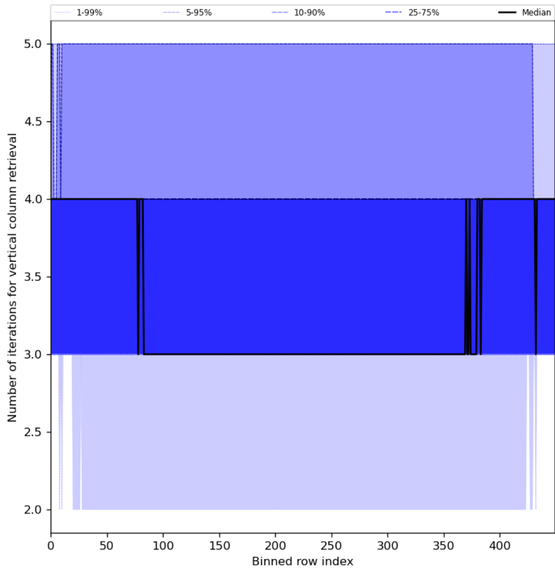
Figure 33: Along track statistics of “Number of iterations for vertical column retrieval” for 2024-08-02 to 2024-08-04
