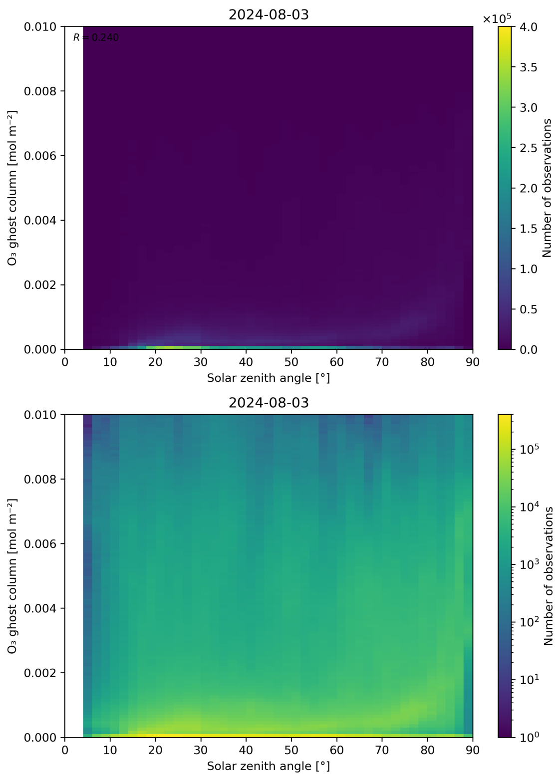
Figure 46: Scatter density plot of “Solar zenith angle” against “O 3 ghost column” for 2024-08-02 to 2024-08-04.
