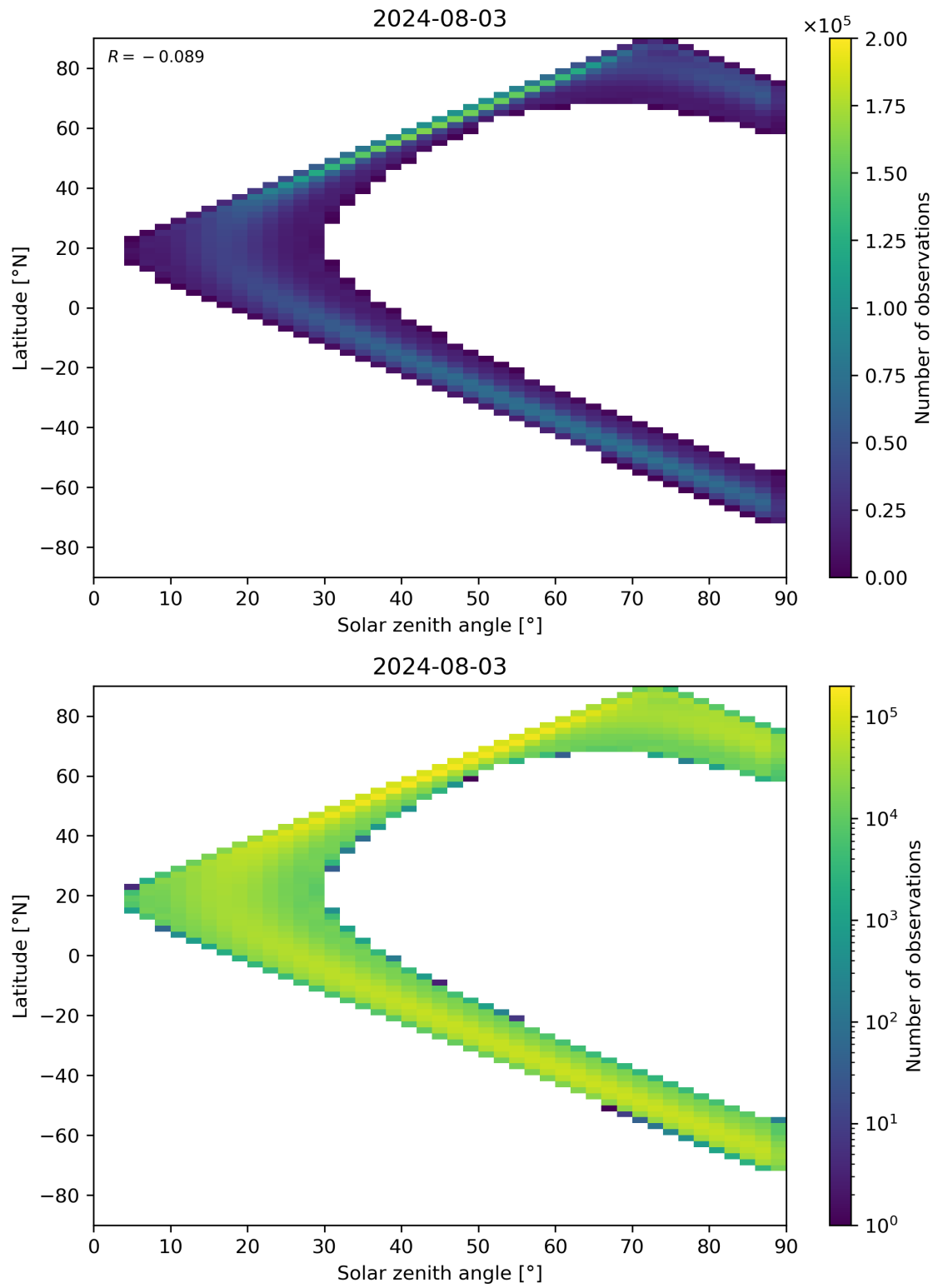
Figure 44: Scatter density plot of “Solar zenith angle” against “Latitude” for 2024-08-02 to 2024-08-04.
