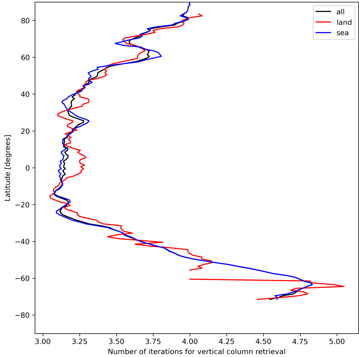
Figure 19: Zonal average of “Number of iterations for vertical column retrieval” for 2024-08-02 to 2024-08-04.
