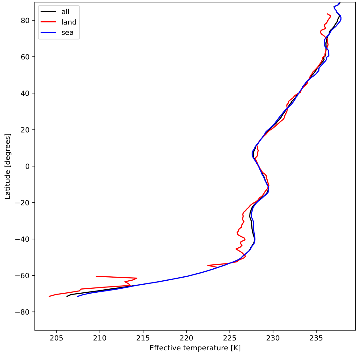
Figure 17: Zonal average of "Effective temperature" for 2024-08-02 to 2024-08-04.
