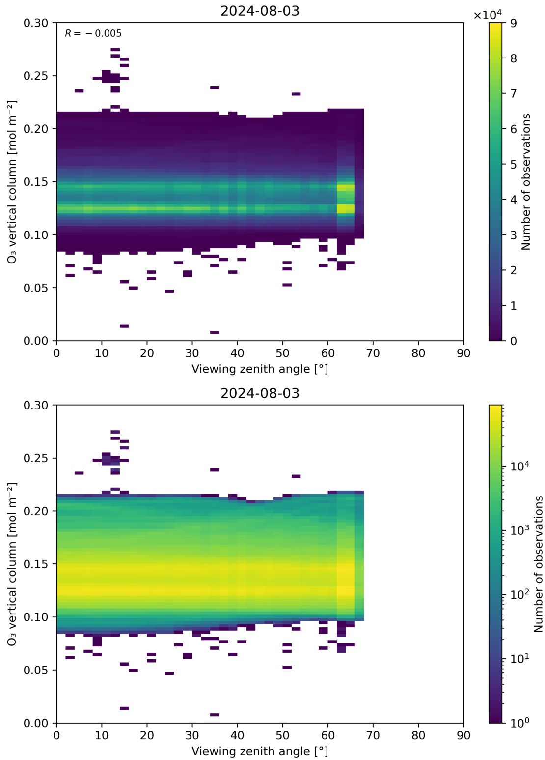
Figure 52: Scatter density plot of “Viewing zenith angle” against “O 3 vertical column” for 2024-08-02 to 2024-08-04.
