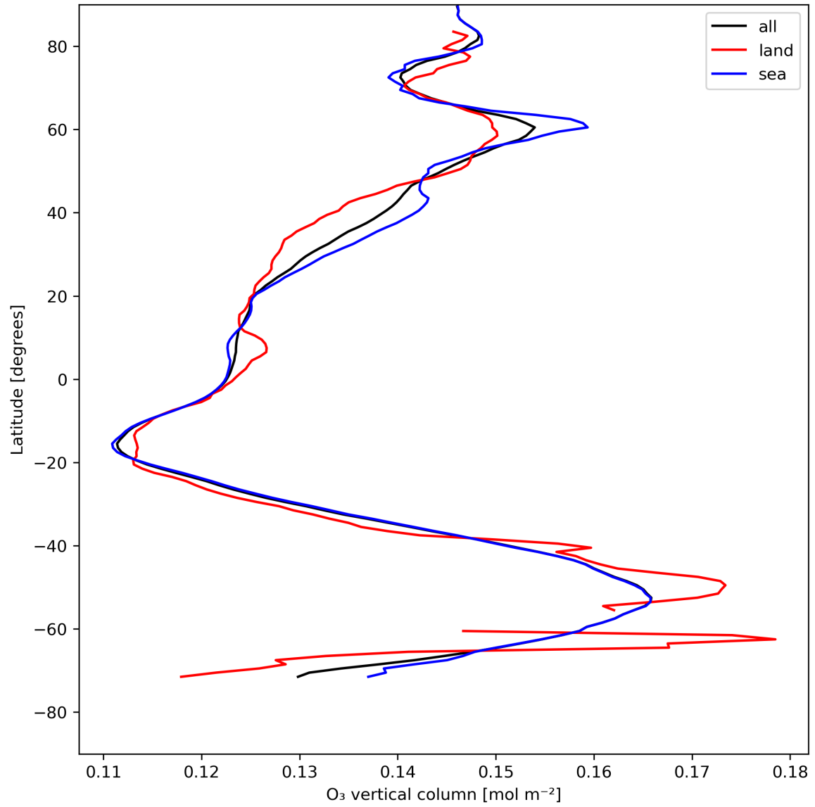
Figure 14: Zonal average of “O 3 vertical column” for 2024-08-02 to 2024-08-04.
