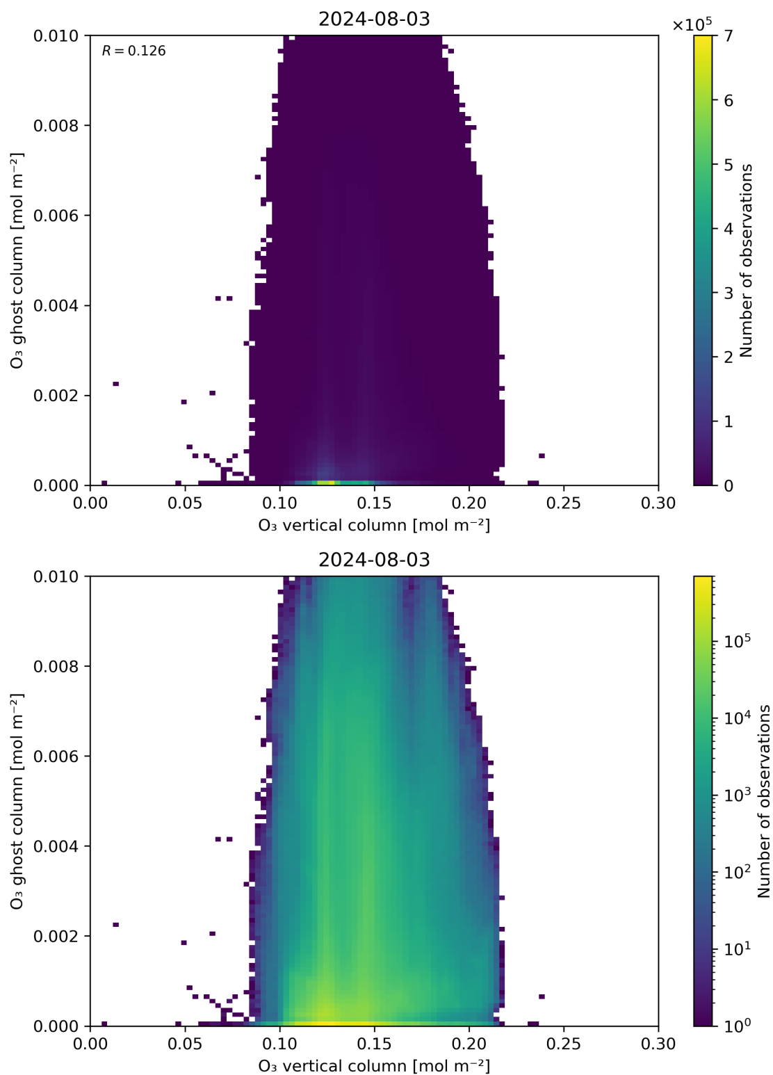
Figure 40: Scatter density plot of “O 3 vertical column” against “O 3 ghost column” for 2024-08-02 to 2024-08-04.
