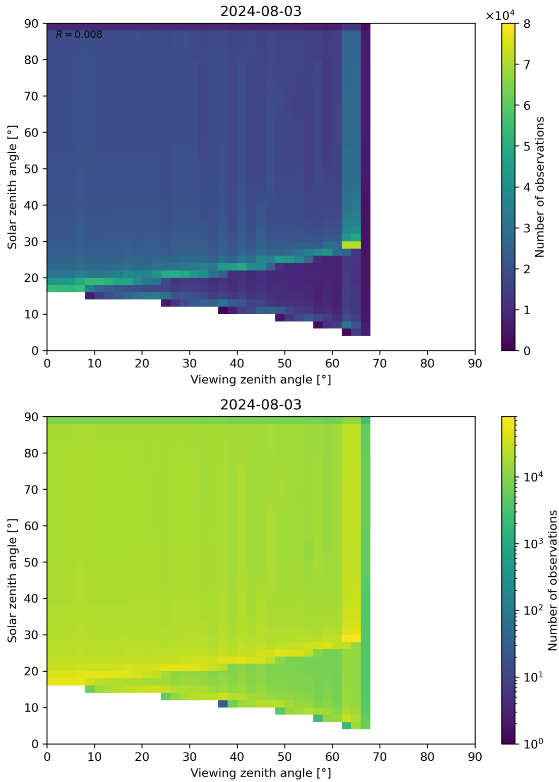
Figure 54: Scatter density plot of “Viewing zenith angle” against “Solar zenith angle” for 2024-08-02 to 2024-08-04.
