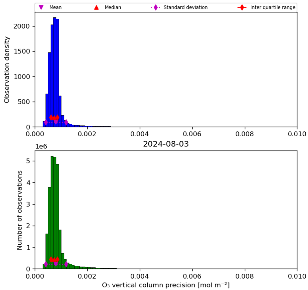
Figure 22: Histogram of “O 3 vertical column precision” for 2024-08-02 to 2024-08-04
