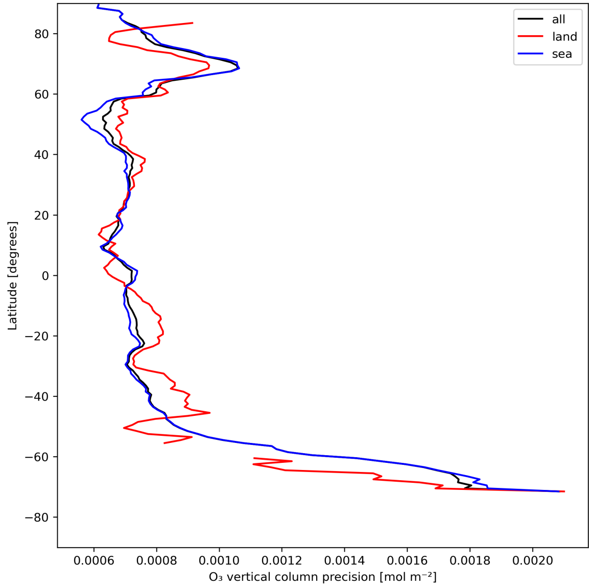
Figure 15: Zonal average of “O 3 vertical column precision” for 2024-08-02 to 2024-08-04.
