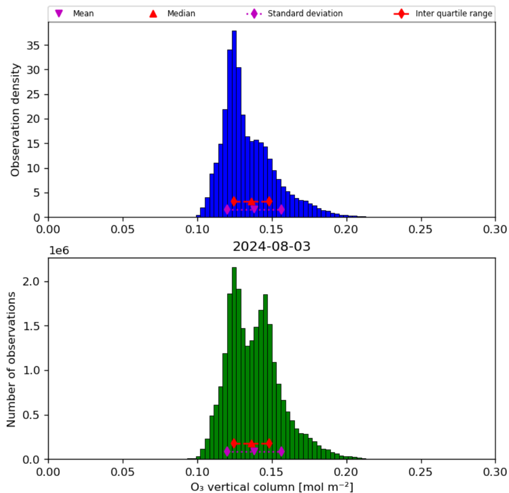
Figure 21: Histogram of “O 3 vertical column” for 2024-08-02 to 2024-08-04
