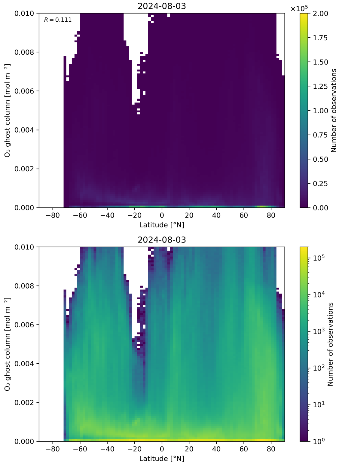
Figure 35: Scatter density plot of “Latitude” against “O 3 ghost column” for 2024-08-02 to 2024-08-04.
