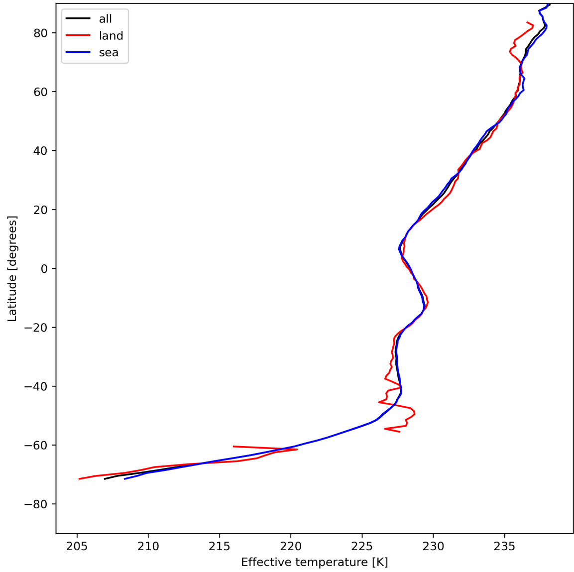
Figure 17: Zonal average of "Effective temperature" for 2024-08-03 to 2024-08-05.
