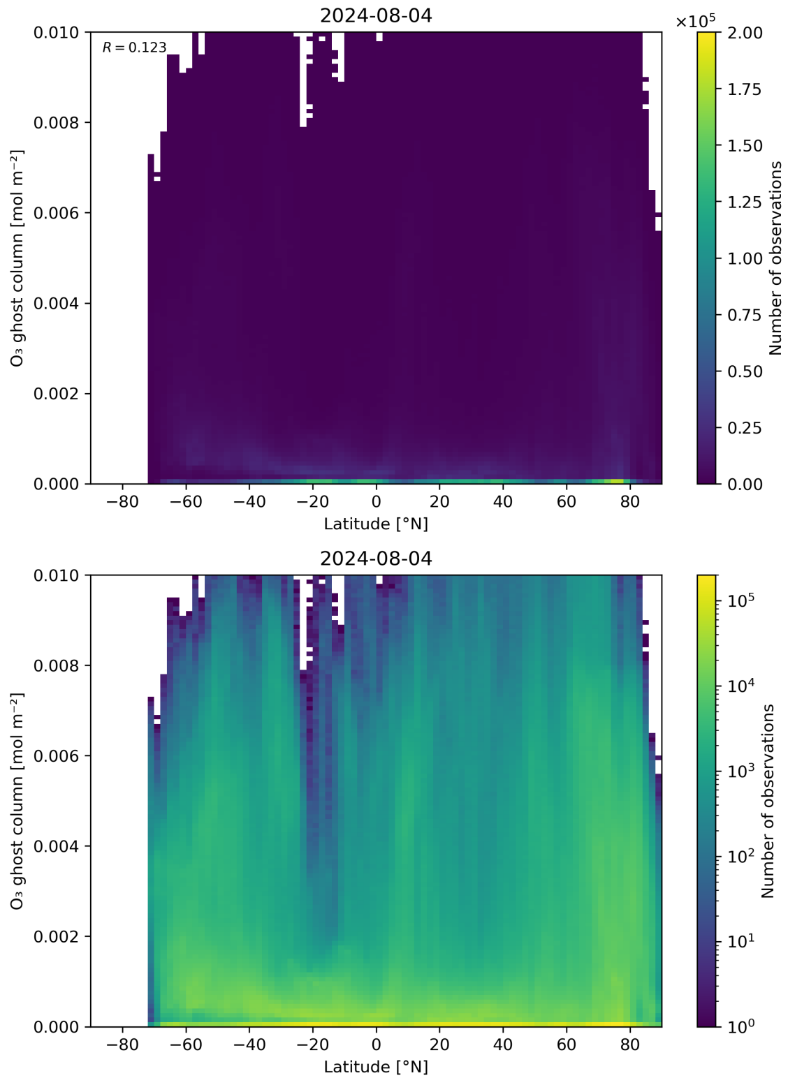
Figure 35: Scatter density plot of “Latitude” against “O 3 ghost column” for 2024-08-03 to 2024-08-05.
