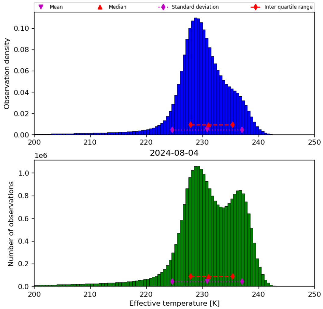
Figure 24: Histogram of “Effective temperature” for 2024-08-03 to 2024-08-05
