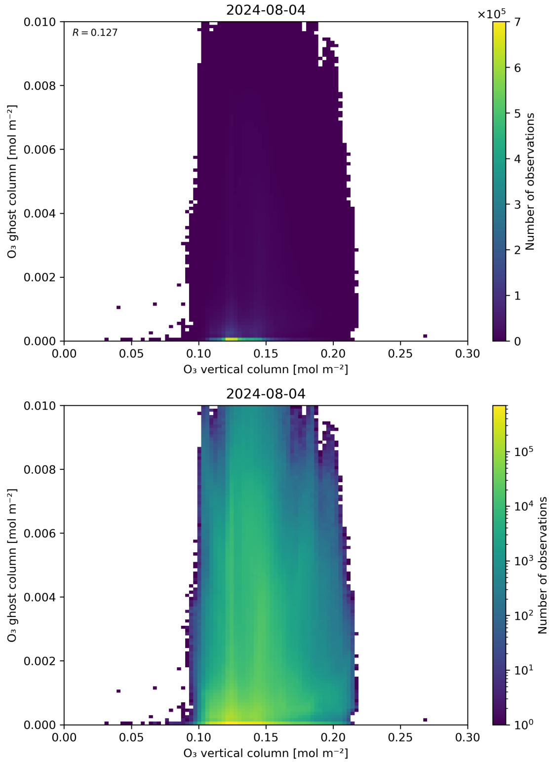
Figure 40: Scatter density plot of “O 3 vertical column” against “O 3 ghost column” for 2024-08-03 to 2024-08-05.
