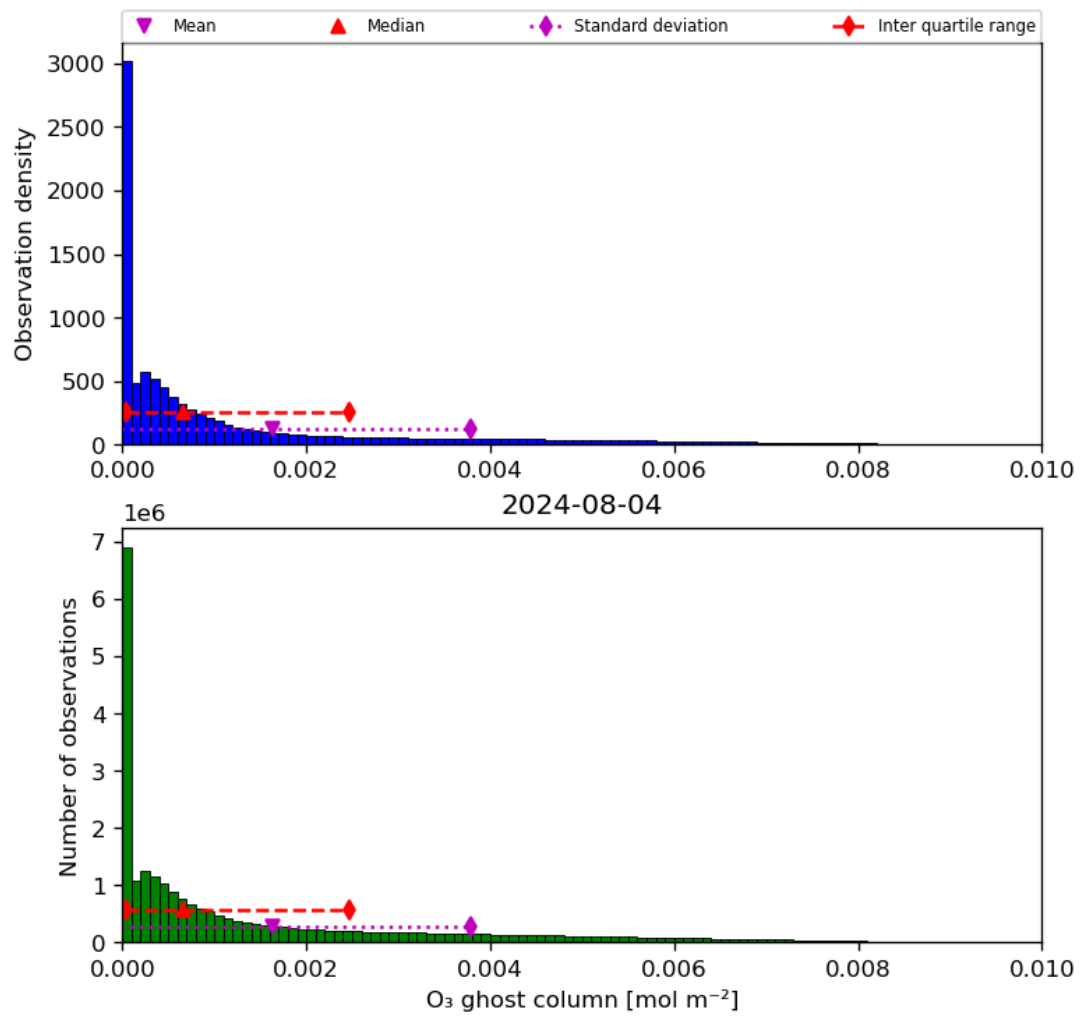
Figure 25: Histogram of “O 3 ghost column” for 2024-08-03 to 2024-08-05
