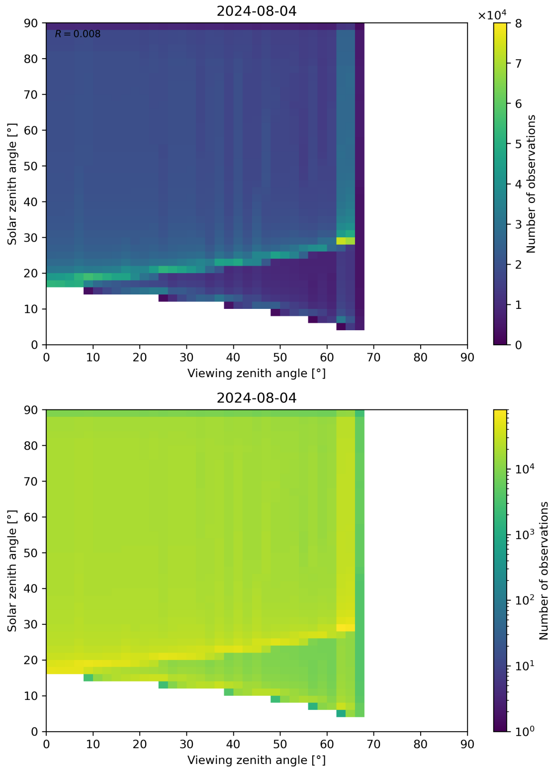
Figure 54: Scatter density plot of “Viewing zenith angle” against “Solar zenith angle” for 2024-08-03 to 2024-08-05.
