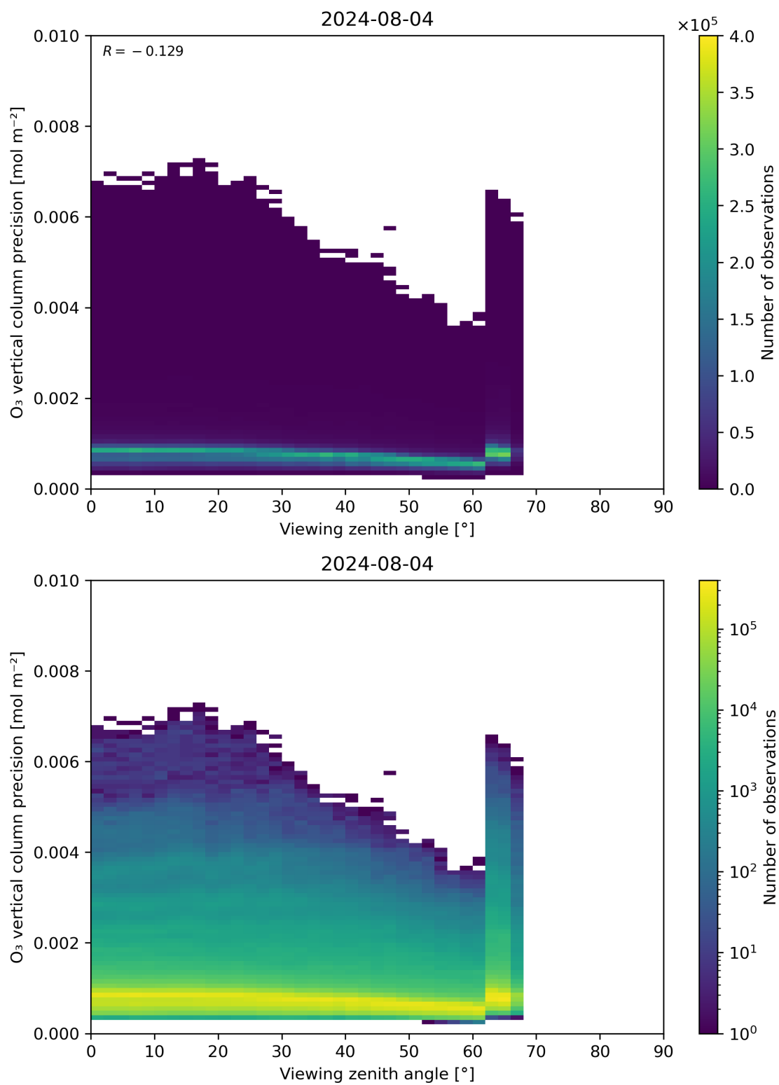
Figure 53: Scatter density plot of “Viewing zenith angle” against “O 3 vertical column precision” for 2024-08-03 to 2024-08-05.
