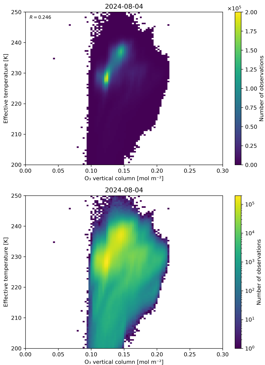
Figure 39: Scatter density plot of “O 3 vertical column” against “Effective temperature” for 2024-08-03 to 2024-08-05.
