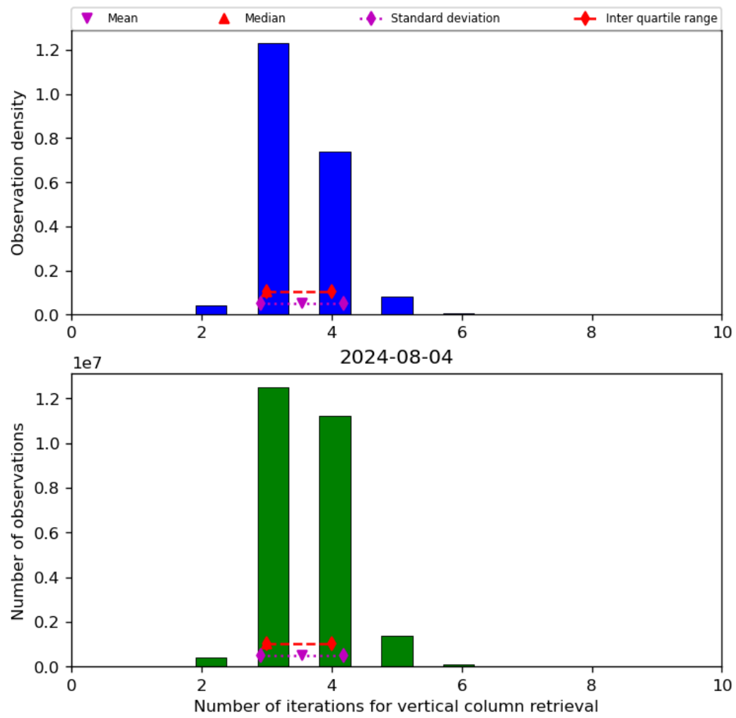
Figure 26: Histogram of “Number of iterations for vertical column retrieval” for 2024-08-03 to 2024-08-05
