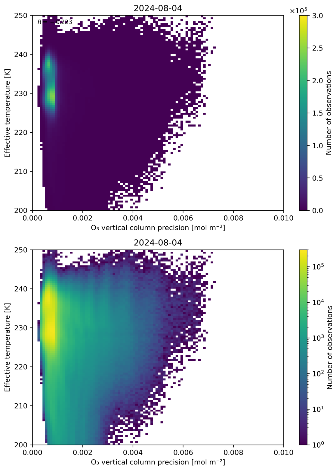
Figure 42: Scatter density plot of “O 3 vertical column precision” against “Effective temperature” for 2024-08-03 to 2024-08-05.
