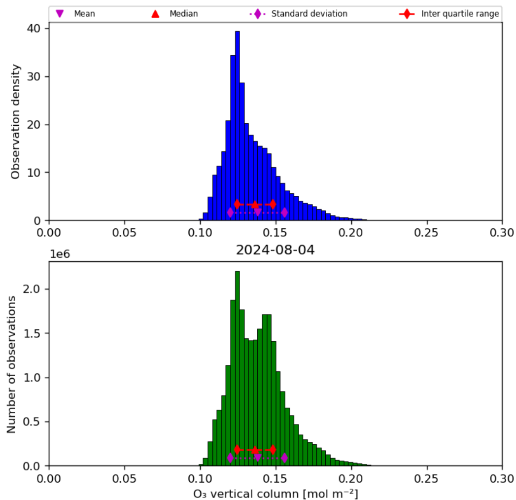
Figure 21: Histogram of “O 3 vertical column” for 2024-08-03 to 2024-08-05
