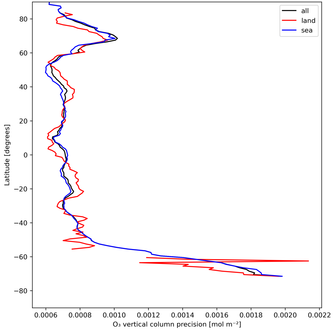
Figure 15: Zonal average of “O 3 vertical column precision” for 2024-08-03 to 2024-08-05.
