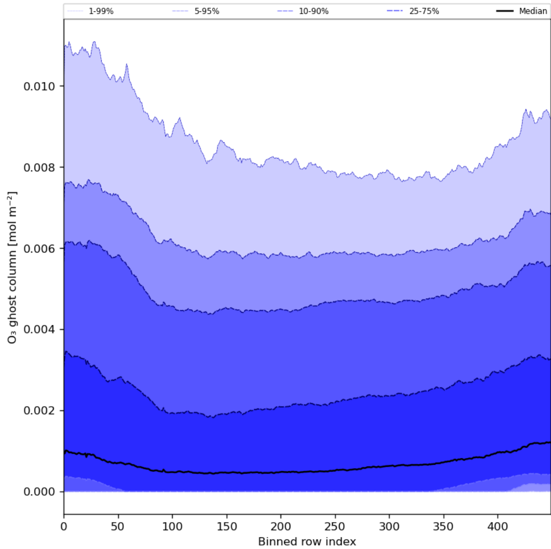
Figure 32: Along track statistics of “O 3 ghost column” for 2024-08-03 to 2024-08-05
