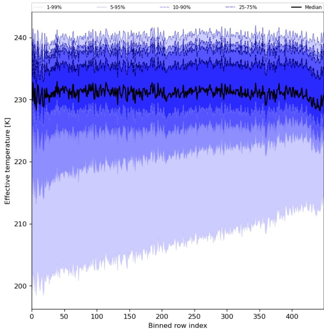
Figure 31: Along track statistics of “Effective temperature” for 2024-08-03 to 2024-08-05
