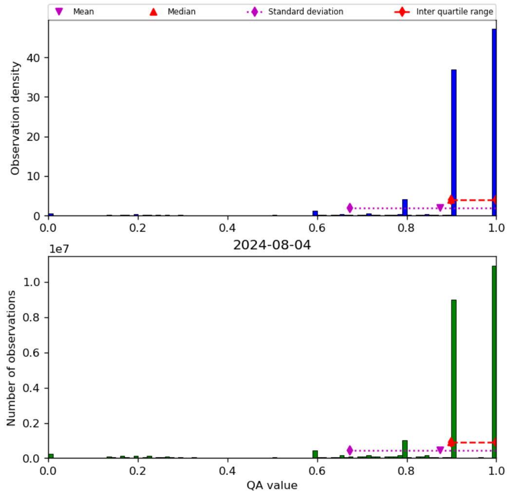
Figure 20: Histogram of “QA value” for 2024-08-03 to 2024-08-05
