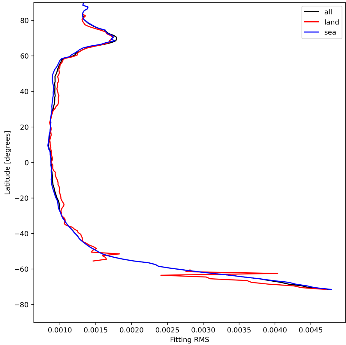
Figure 16: Zonal average of “Fitting RMS” for 2024-08-03 to 2024-08-05.
