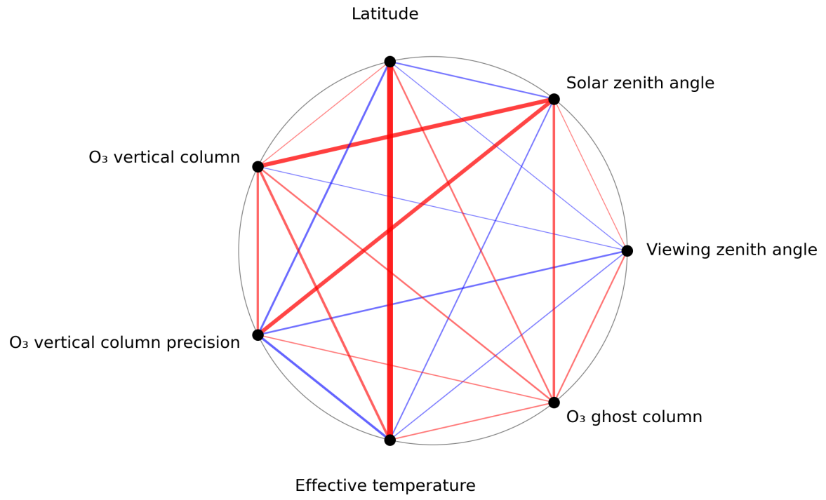
Figure 1: Map of correlation graph for 2024-08-03 to 2024-08-05.
