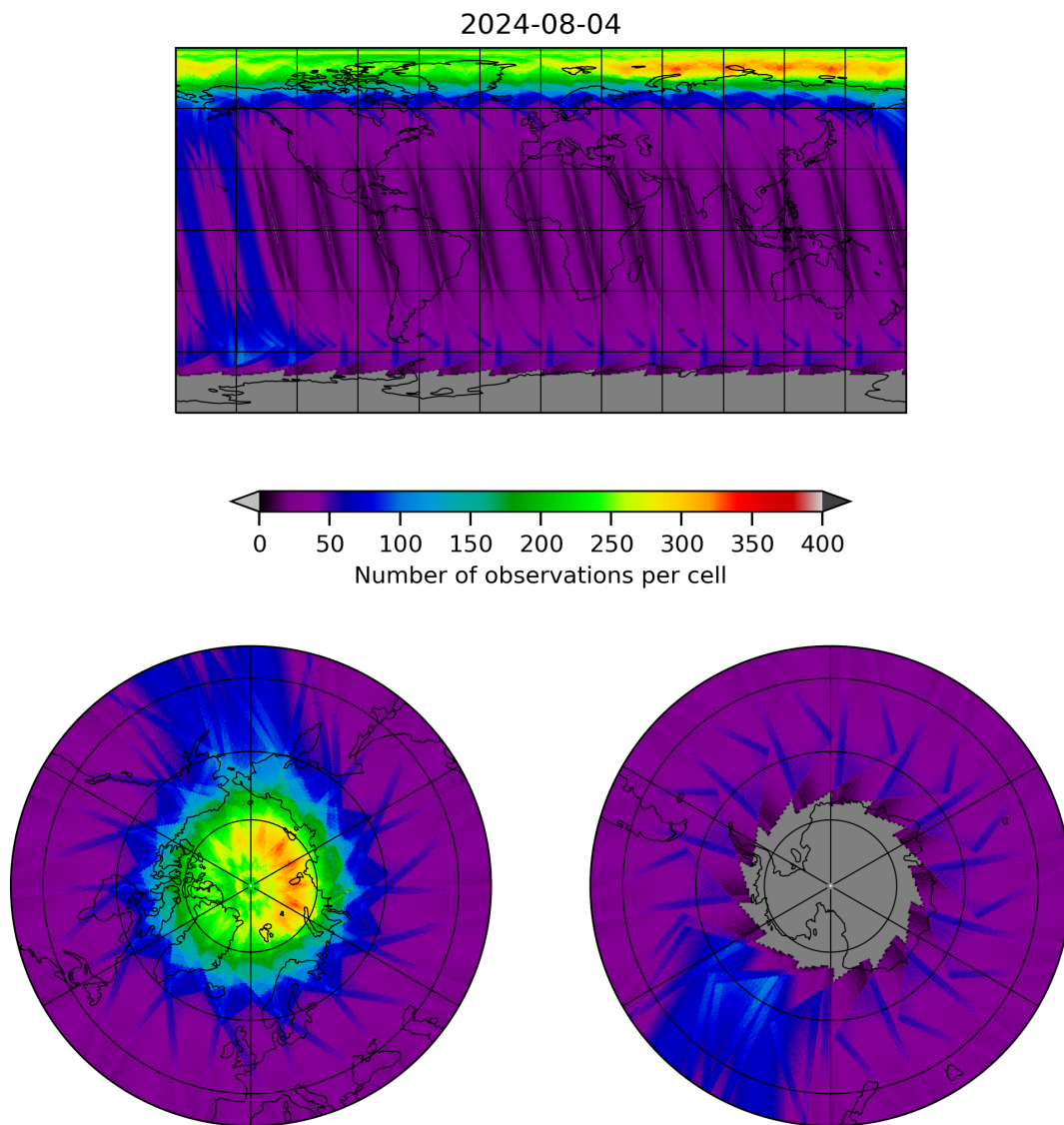
Figure 12: Map of the number of observations for 2024-08-03 to 2024-08-05
