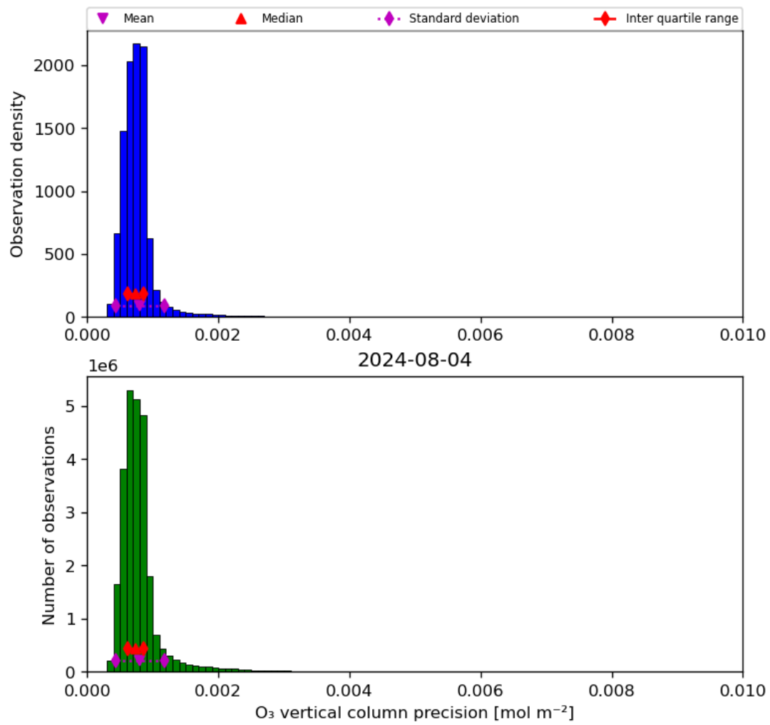
Figure 22: Histogram of “O 3 vertical column precision” for 2024-08-03 to 2024-08-05
