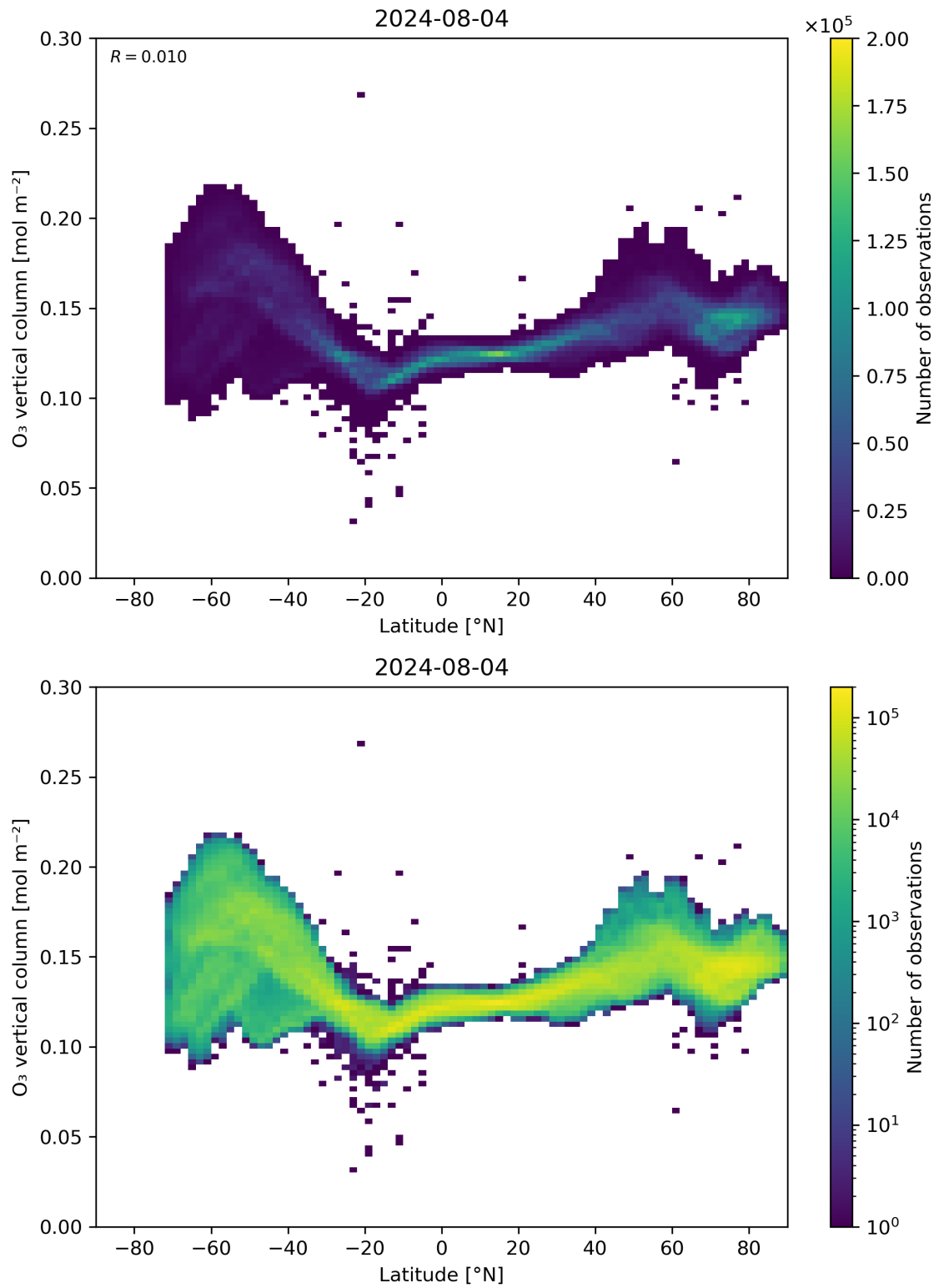
Figure 36: Scatter density plot of “Latitude” against “O 3 vertical column” for 2024-08-03 to 2024-08-05.
