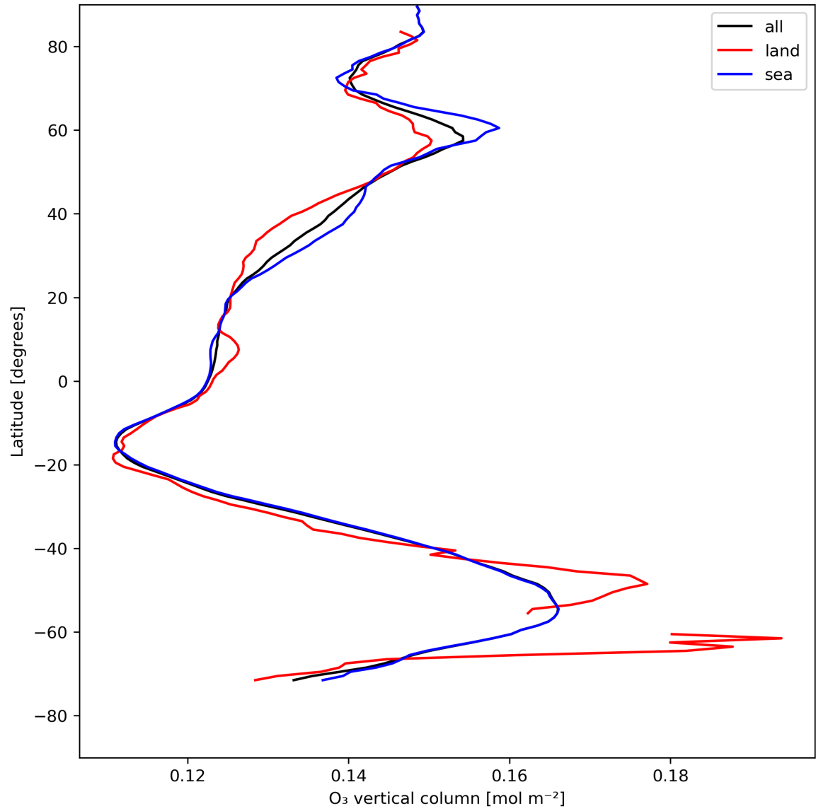
Figure 14: Zonal average of “O 3 vertical column” for 2024-08-03 to 2024-08-05.
