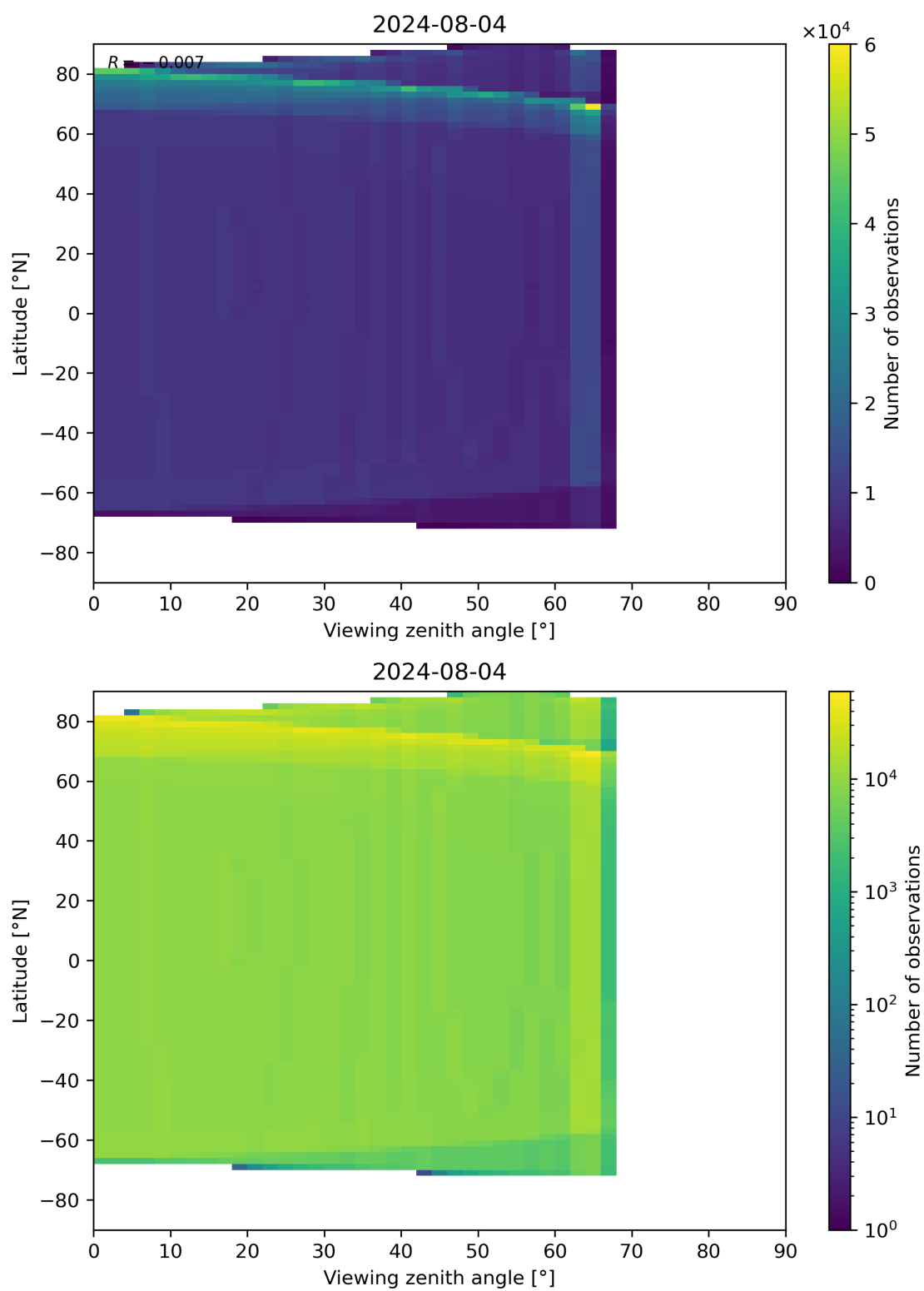
Figure 49: Scatter density plot of “Viewing zenith angle” against “Latitude” for 2024-08-03 to 2024-08-05.
