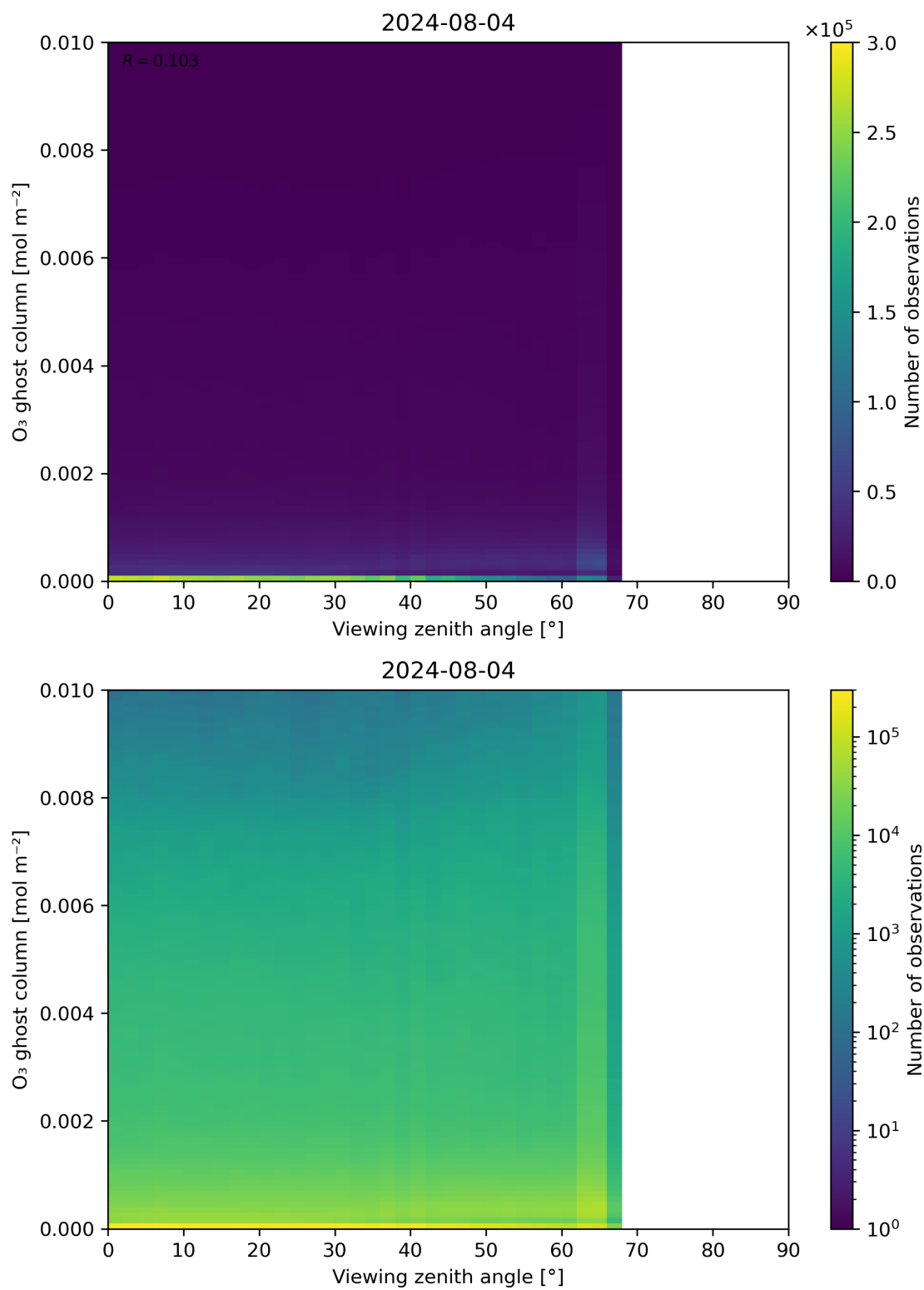
Figure 51: Scatter density plot of “Viewing zenith angle” against “O 3 ghost column” for 2024-08-03 to 2024-08-05.
