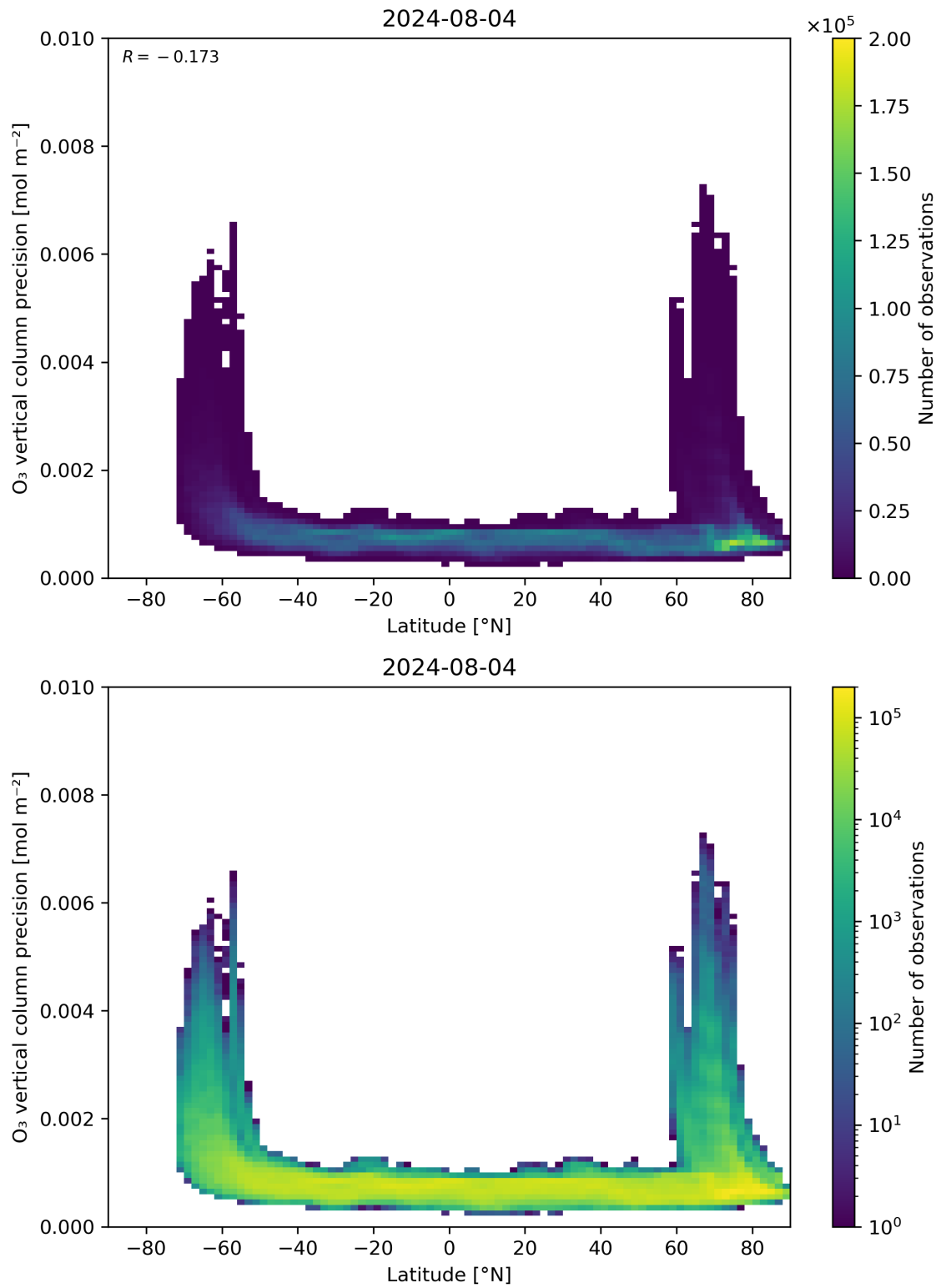
Figure 37: Scatter density plot of “Latitude” against “O 3 vertical column precision” for 2024-08-03 to 2024-08-05.
