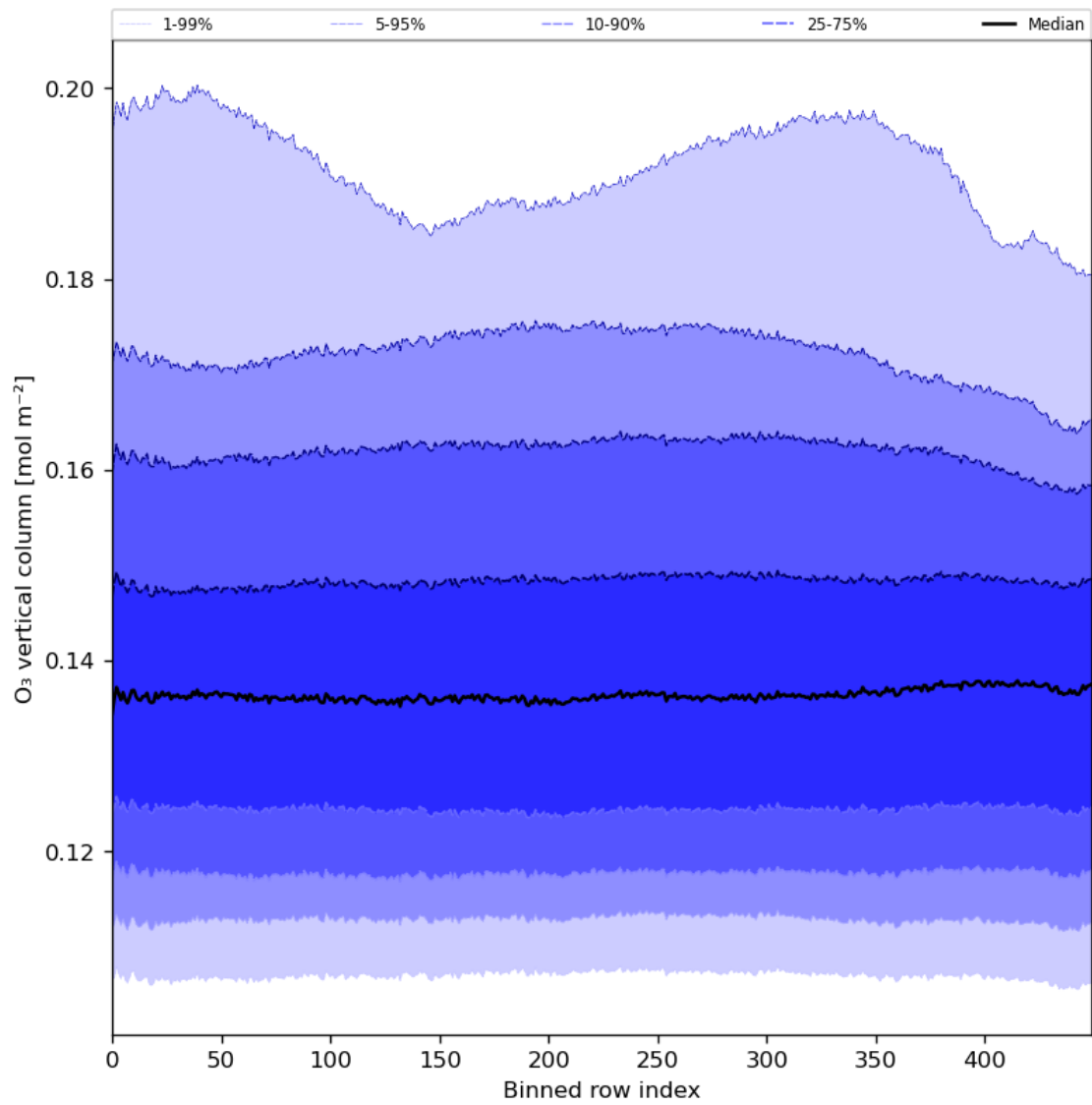
Figure 28: Along track statistics of “O 3 vertical column” for 2024-08-03 to 2024-08-05
