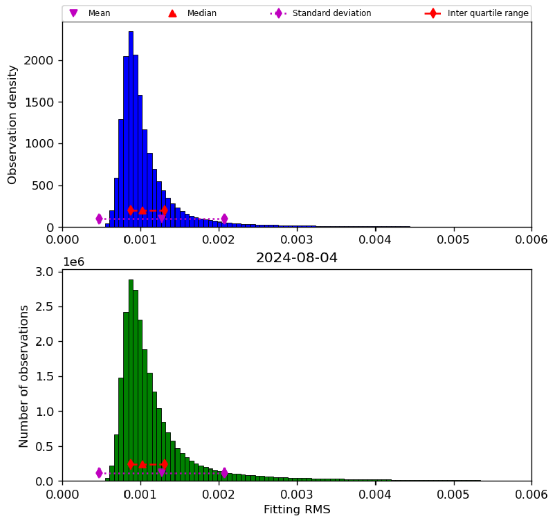
Figure 23: Histogram of “Fitting RMS” for 2024-08-03 to 2024-08-05
