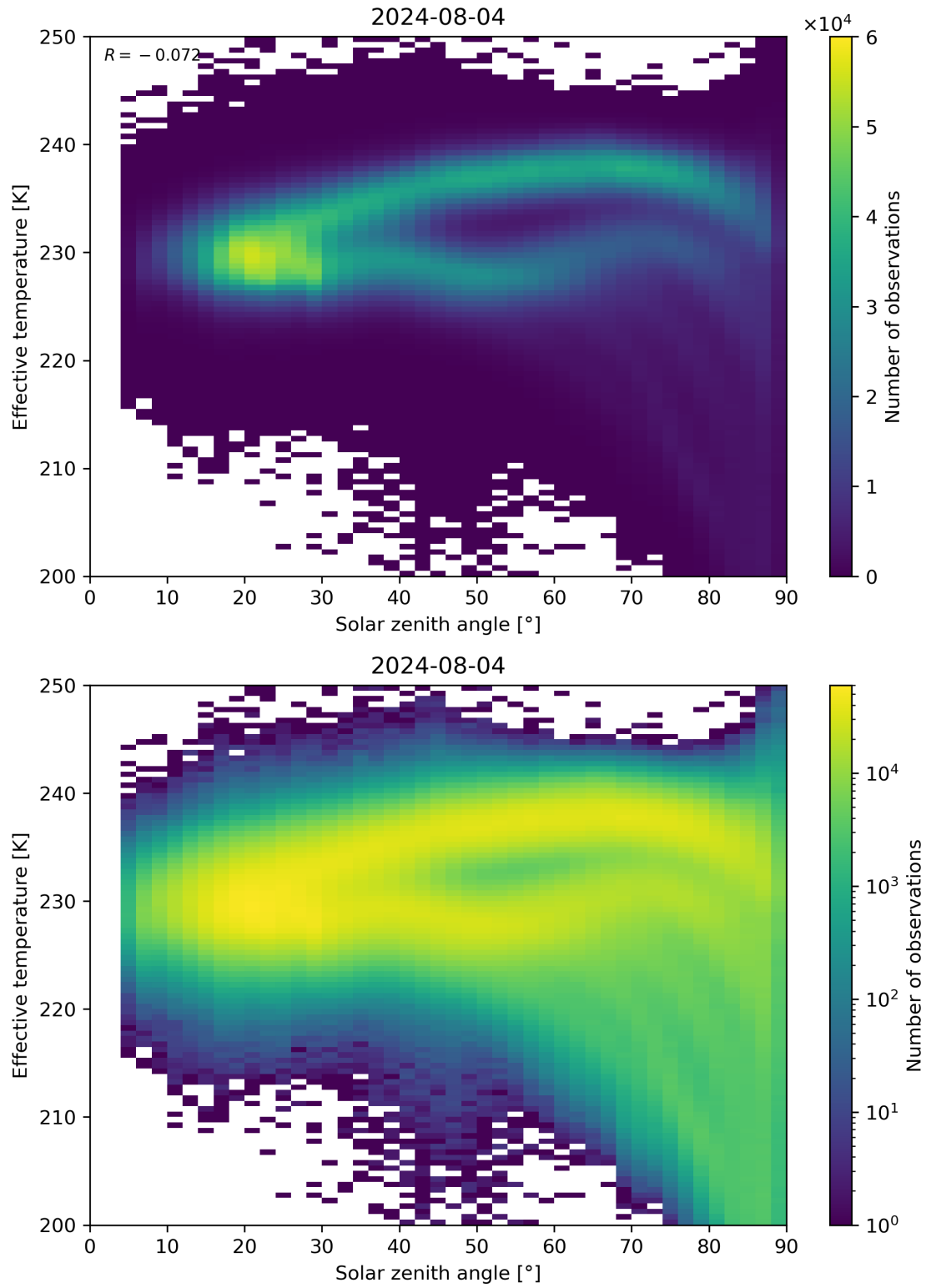
Figure 45: Scatter density plot of “Solar zenith angle” against “Effective temperature” for 2024-08-03 to 2024-08-05.
