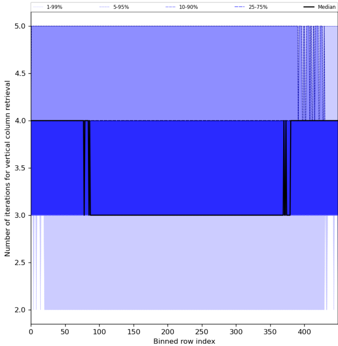
Figure 33: Along track statistics of “Number of iterations for vertical column retrieval” for 2024-08-03 to 2024-08-05
