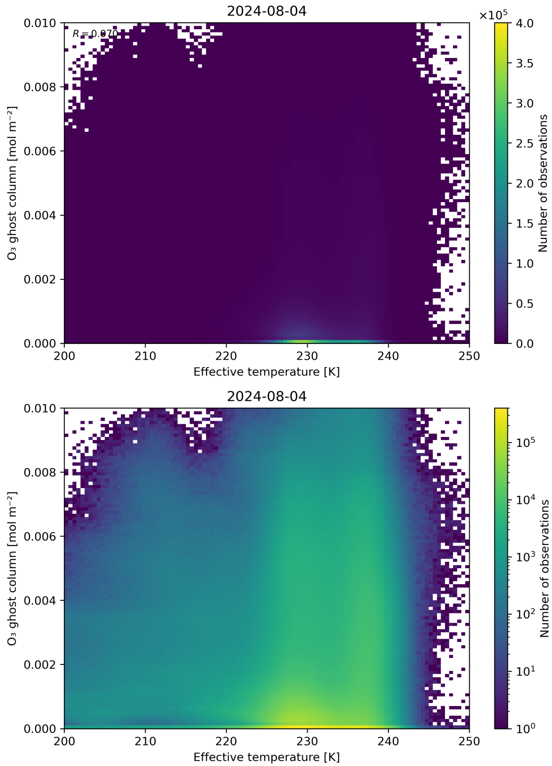
Figure 38: Scatter density plot of “Effective temperature” against “O 3 ghost column” for 2024-08-03 to 2024-08-05.
