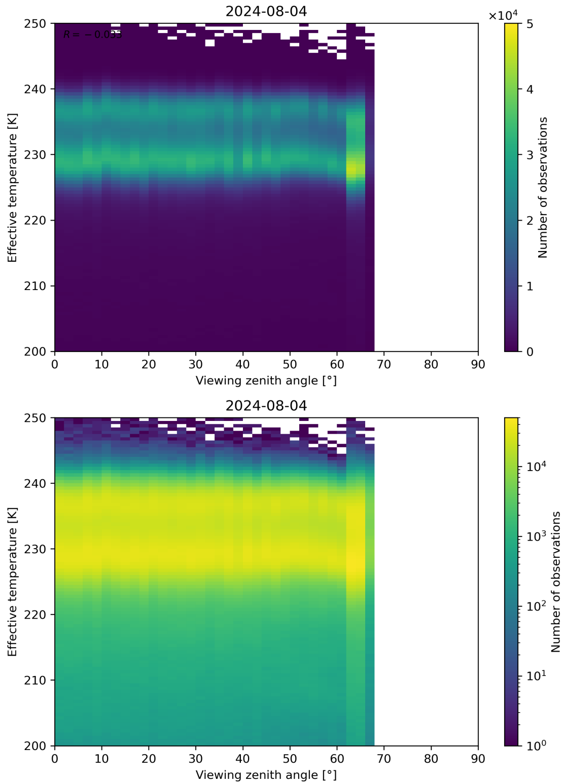
Figure 50: Scatter density plot of “Viewing zenith angle” against “Effective temperature” for 2024-08-03 to 2024-08-05.
