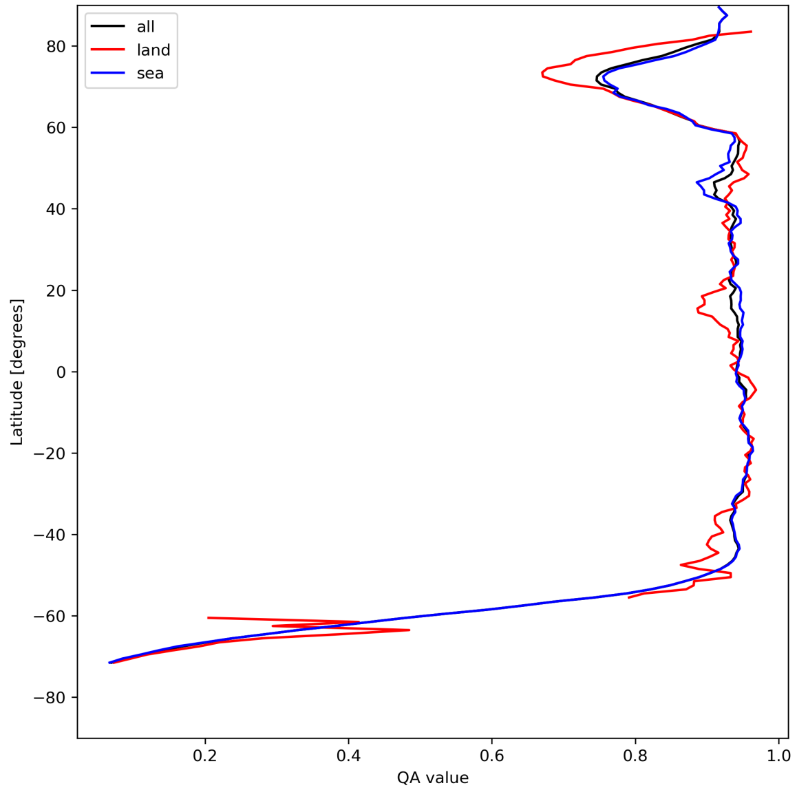
Figure 13: Zonal average of “QA value” for 2024-08-03 to 2024-08-05.
