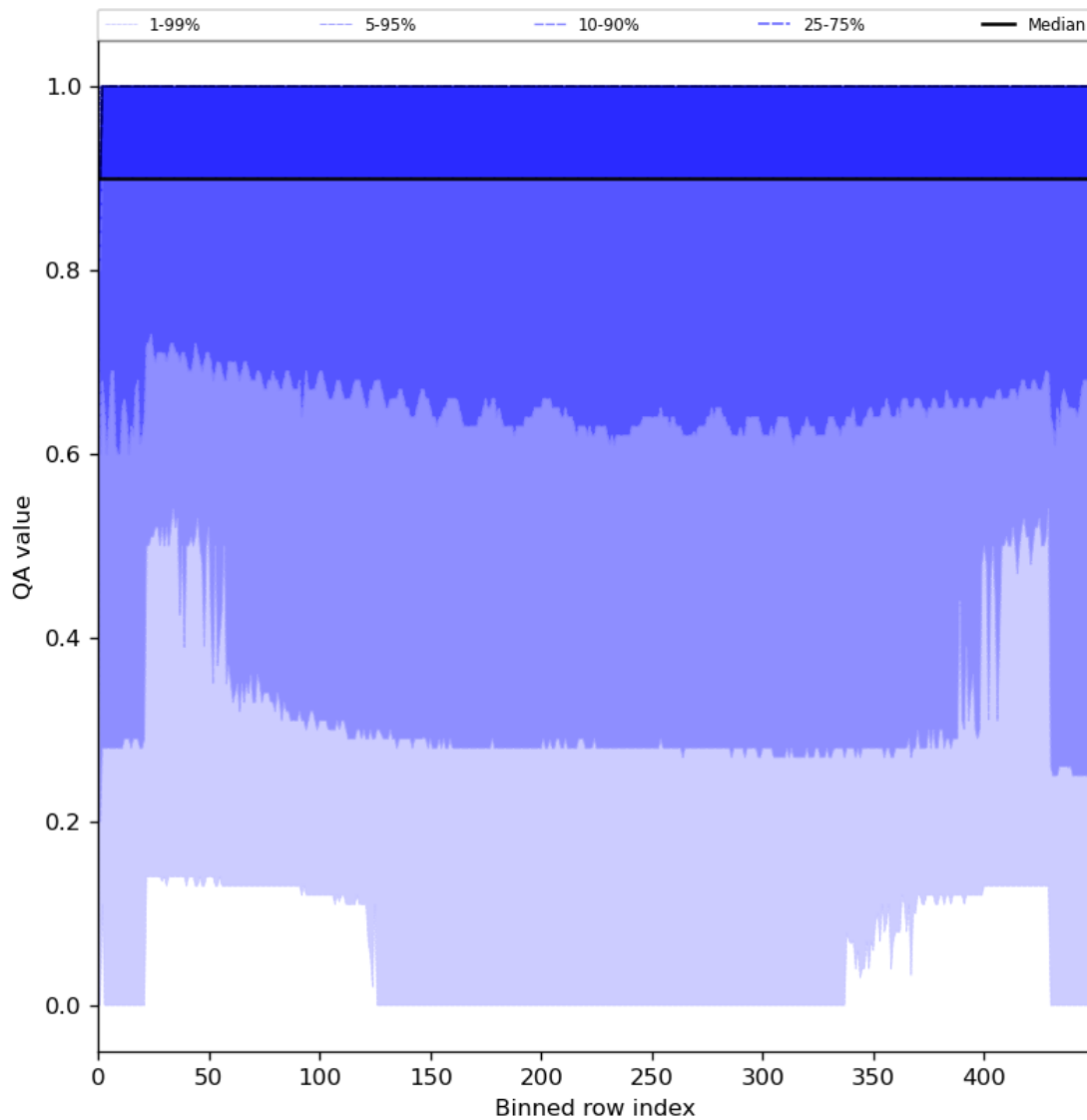
Figure 27: Along track statistics of “QA value” for 2024-08-03 to 2024-08-05
