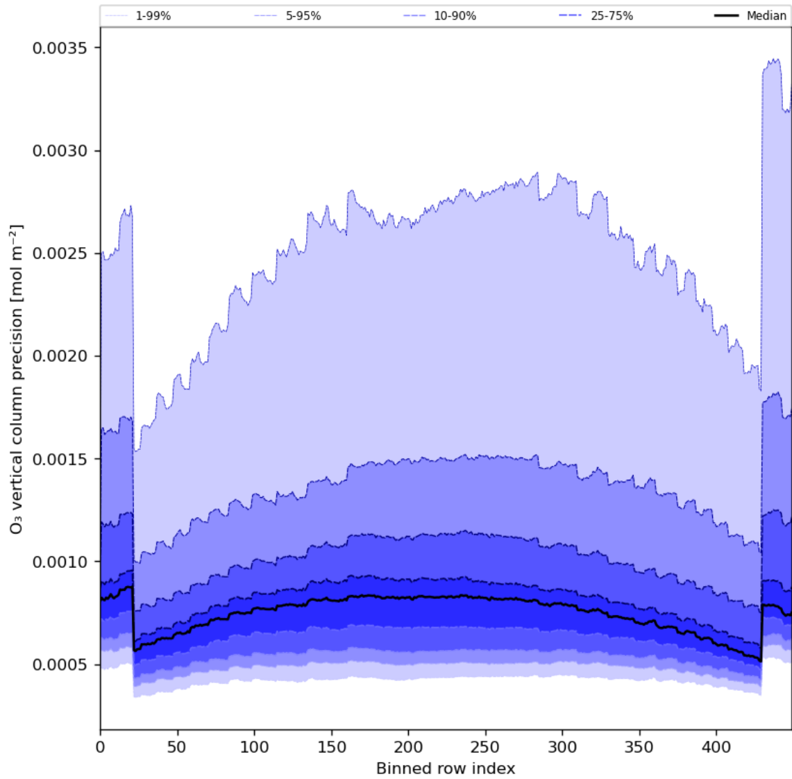
Figure 29: Along track statistics of “O 3 vertical column precision” for 2024-08-03 to 2024-08-05
