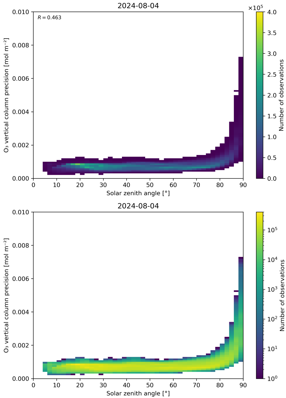
Figure 48: Scatter density plot of “Solar zenith angle” against “O 3 vertical column precision” for 2024-08-03 to 2024-08-05.
