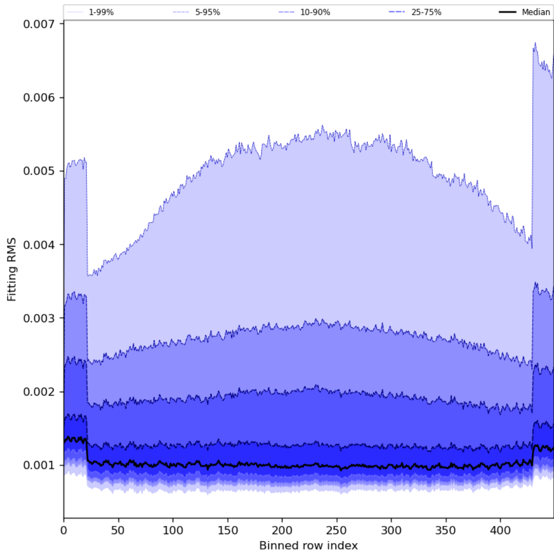
Figure 30: Along track statistics of “Fitting RMS” for 2024-08-03 to 2024-08-05
