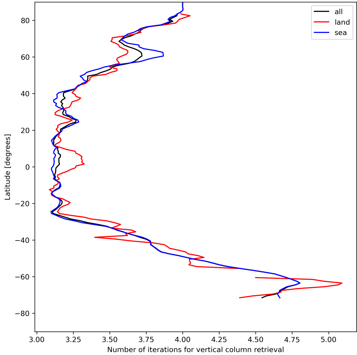
Figure 19: Zonal average of “Number of iterations for vertical column retrieval” for 2024-08-03 to 2024-08-05.
