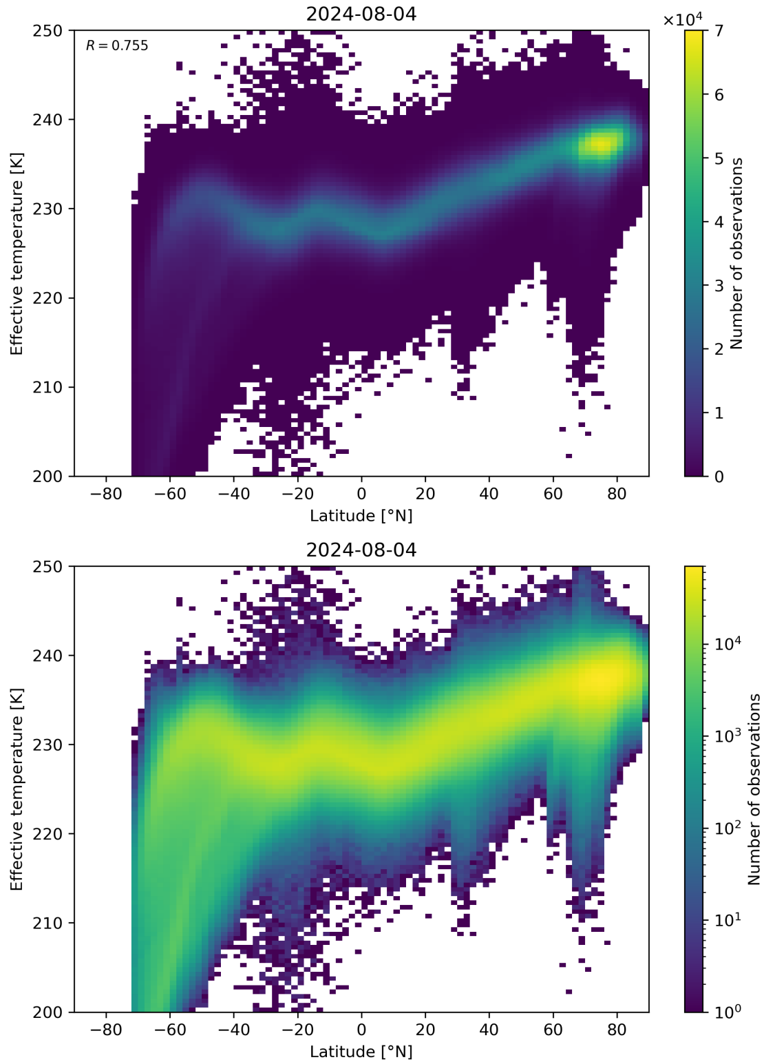
Figure 34: Scatter density plot of “Latitude” against “Effective temperature” for 2024-08-03 to 2024-08-05.
