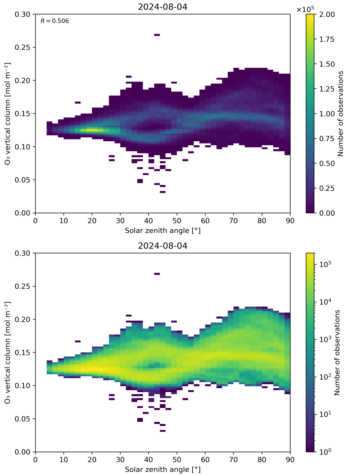
Figure 47: Scatter density plot of “Solar zenith angle” against “O 3 vertical column” for 2024-08-03 to 2024-08-05.
