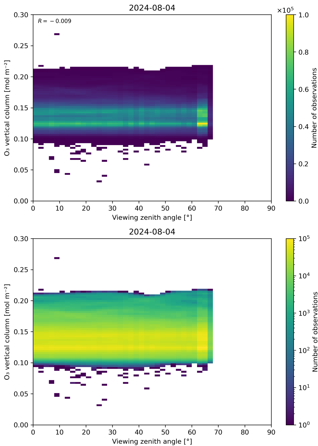
Figure 52: Scatter density plot of “Viewing zenith angle” against “O 3 vertical column” for 2024-08-03 to 2024-08-05.
