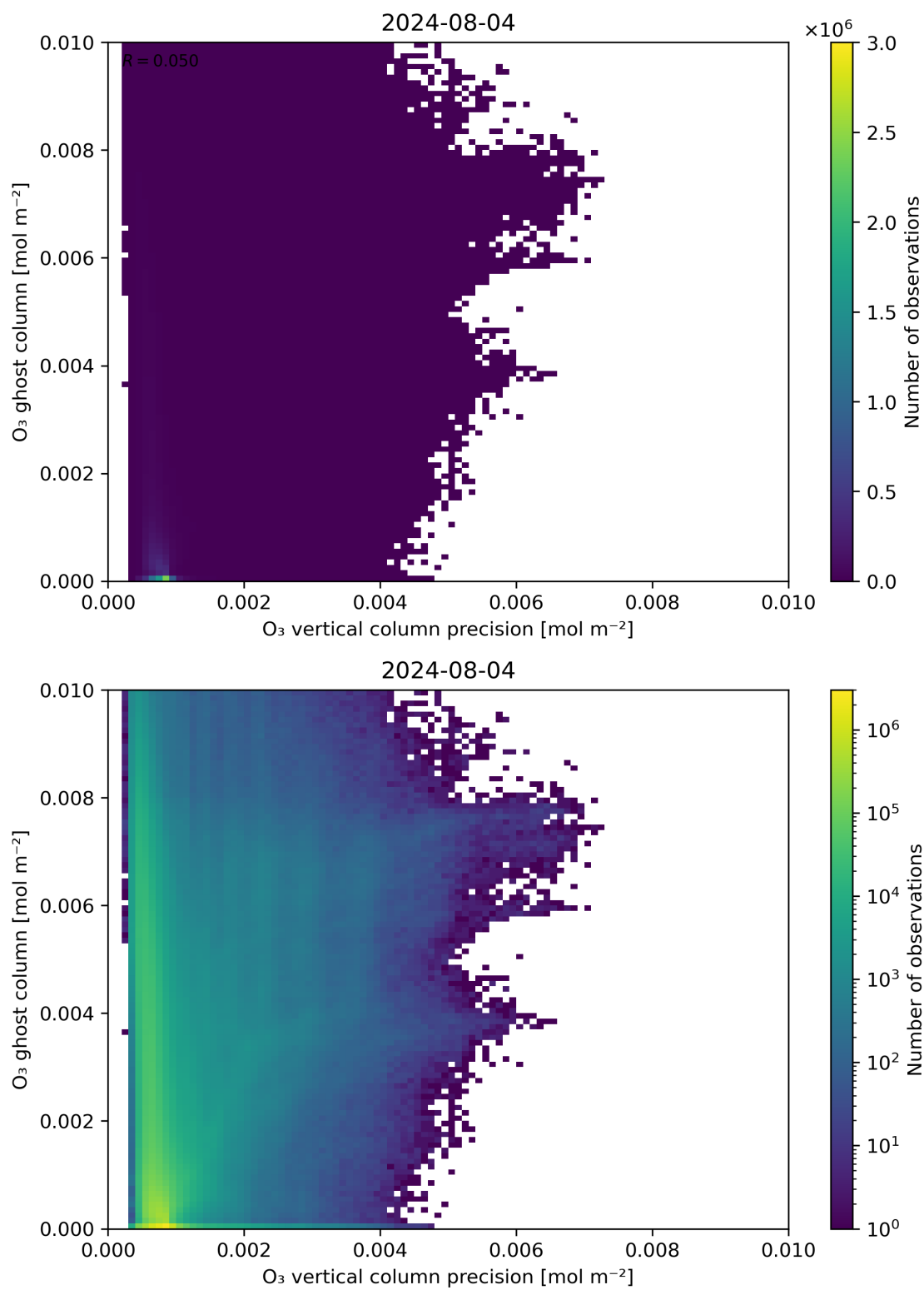
Figure 43: Scatter density plot of “ \text{O}_3 vertical column precision” against “ \text{O}_3 ghost column” for 2024-08-03 to 2024-08-05.
