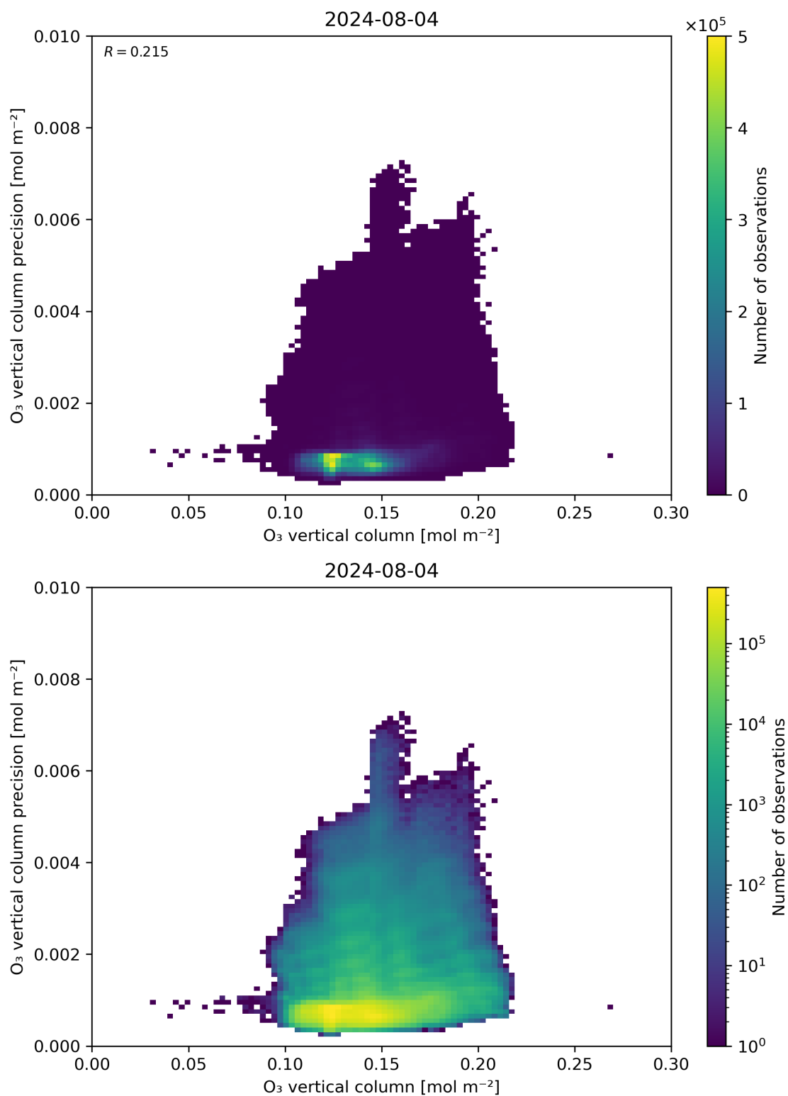
Figure 41: Scatter density plot of “O 3 vertical column” against “O 3 vertical column precision” for 2024-08-03 to 2024-08-05.
