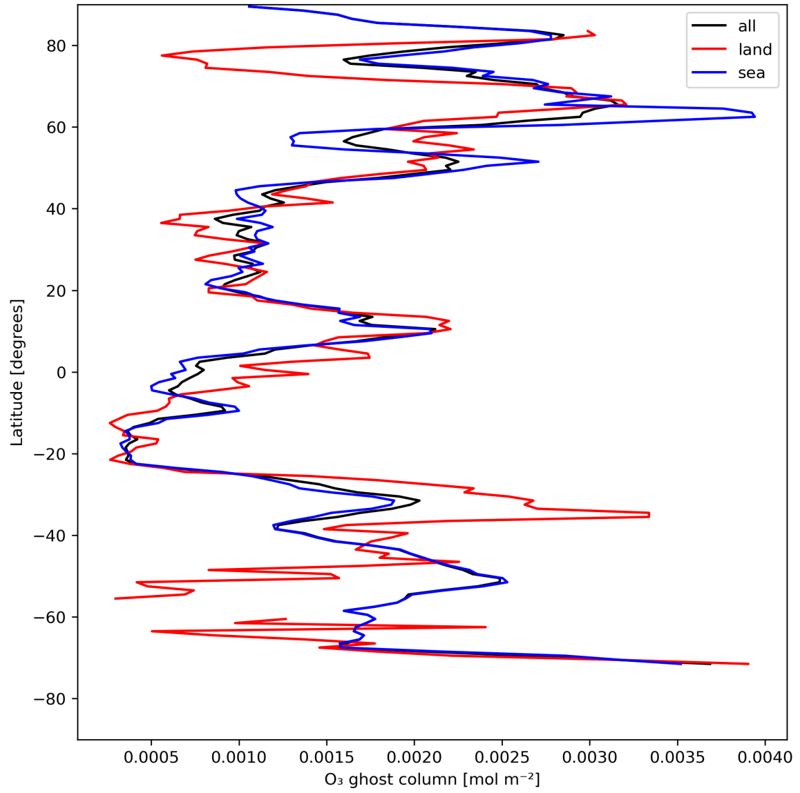
Figure 18: Zonal average of “O 3 ghost column” for 2024-08-03 to 2024-08-05.
