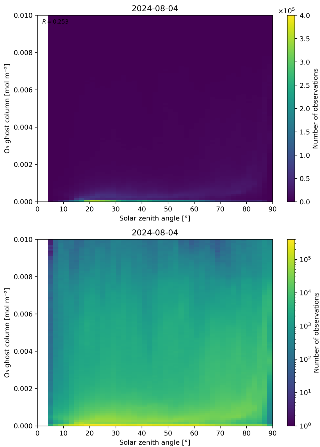
Figure 46: Scatter density plot of “Solar zenith angle” against “O 3 ghost column” for 2024-08-03 to 2024-08-05.
