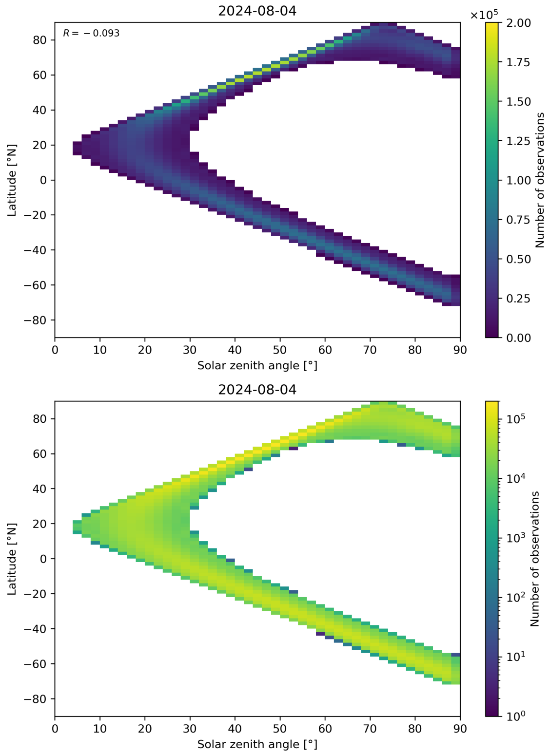
Figure 44: Scatter density plot of “Solar zenith angle” against “Latitude” for 2024-08-03 to 2024-08-05.
