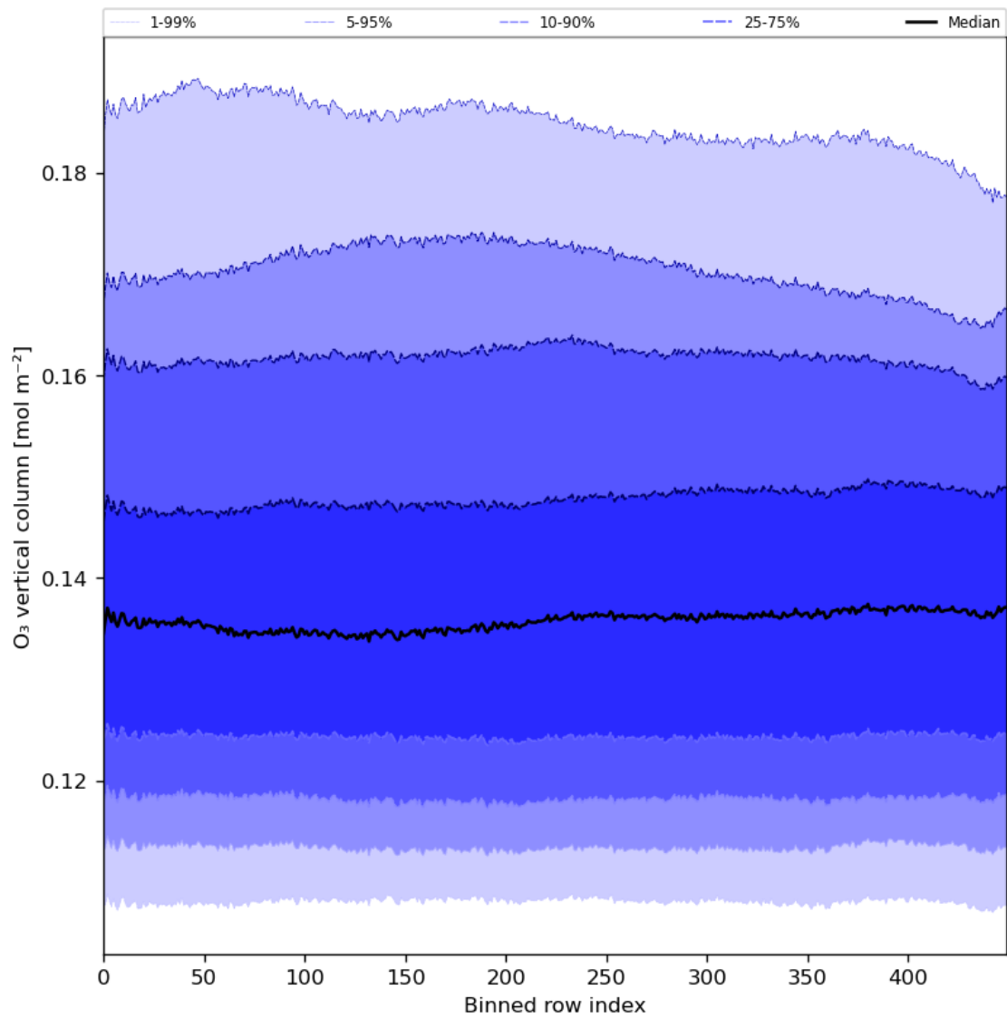
Figure 28: Along track statistics of “O 3 vertical column” for 2024-08-04 to 2024-08-06
