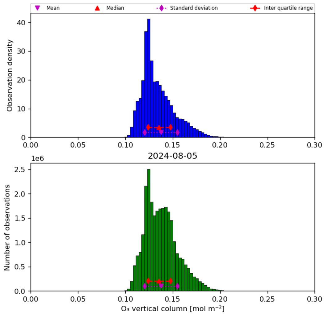
Figure 21: Histogram of “O 3 vertical column” for 2024-08-04 to 2024-08-06
