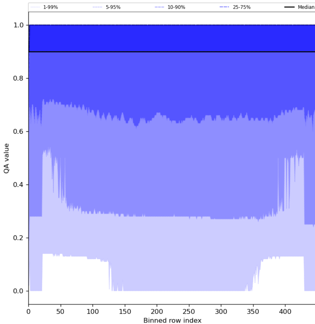
Figure 27: Along track statistics of “QA value” for 2024-08-04 to 2024-08-06
