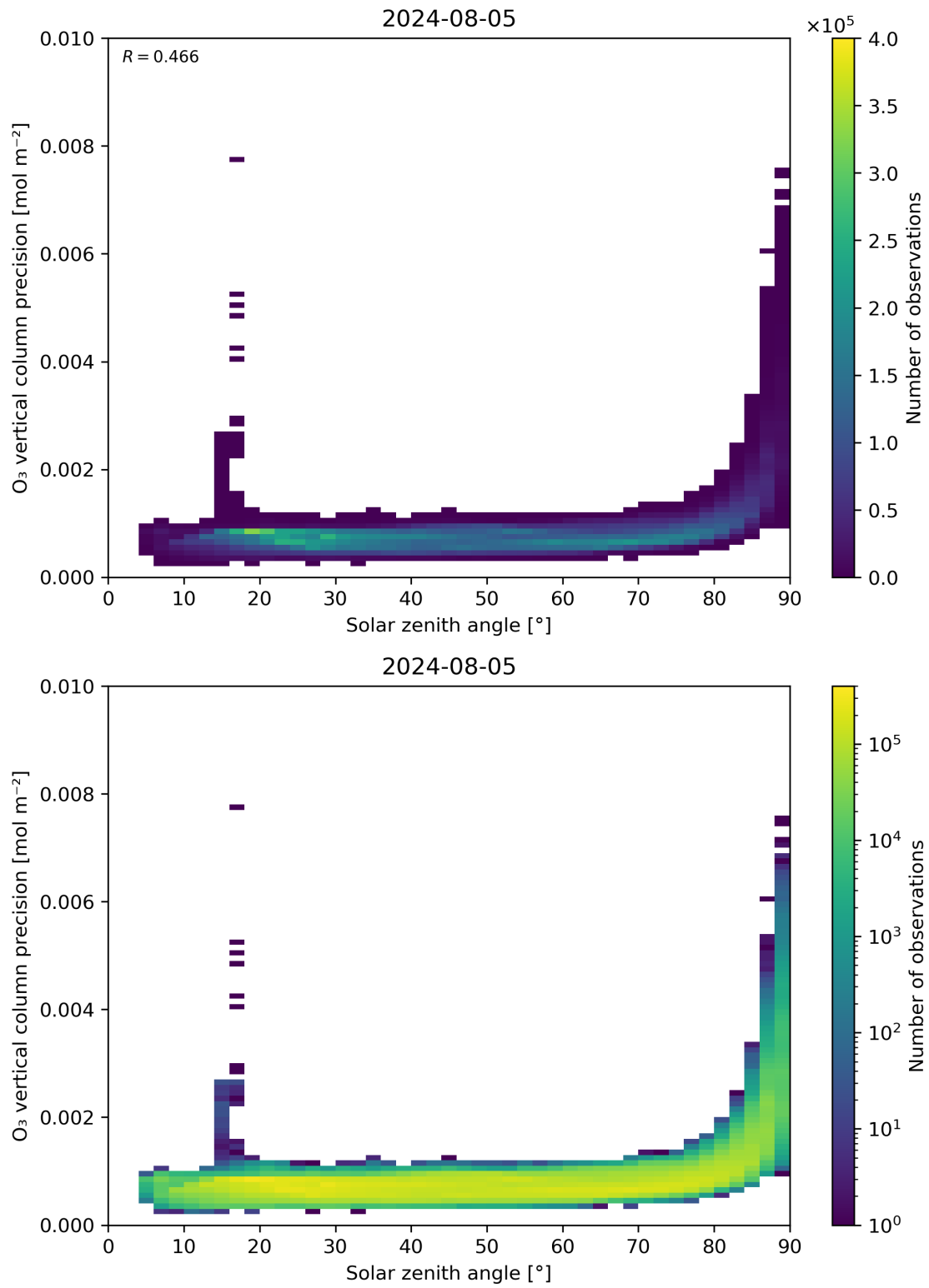
Figure 48: Scatter density plot of “Solar zenith angle” against “O 3 vertical column precision” for 2024-08-04 to 2024-08-06.
