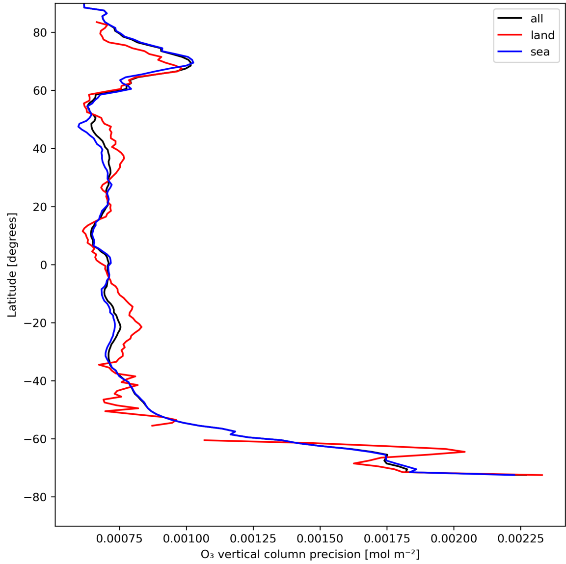
Figure 15: Zonal average of "O 3 vertical column precision" for 2024-08-04 to 2024-08-06.
