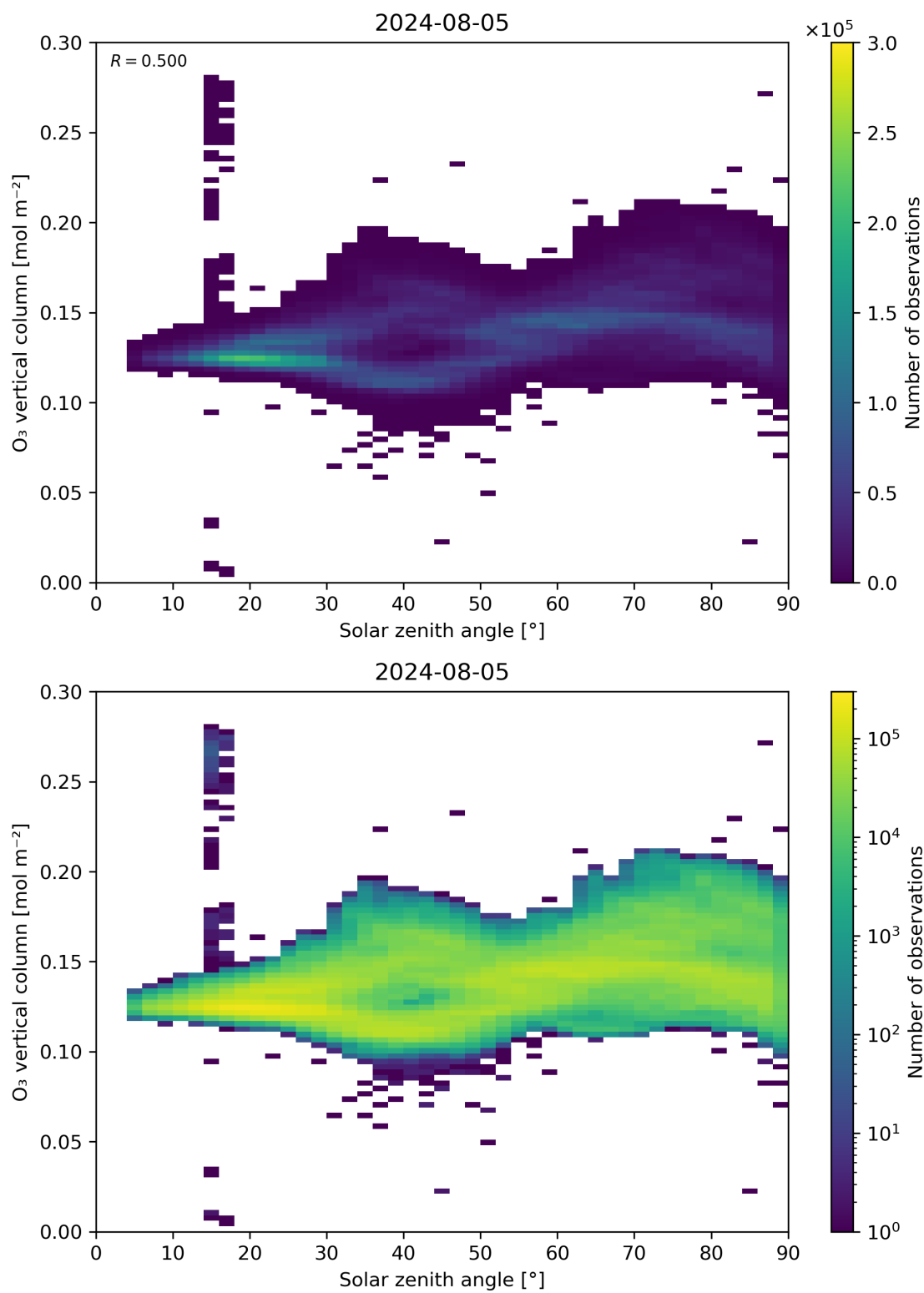
Figure 47: Scatter density plot of “Solar zenith angle” against “O 3 vertical column” for 2024-08-04 to 2024-08-06.
