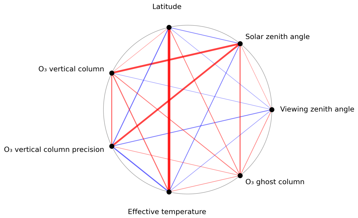
Figure 1: Map of correlation graph for 2024-08-04 to 2024-08-06.
