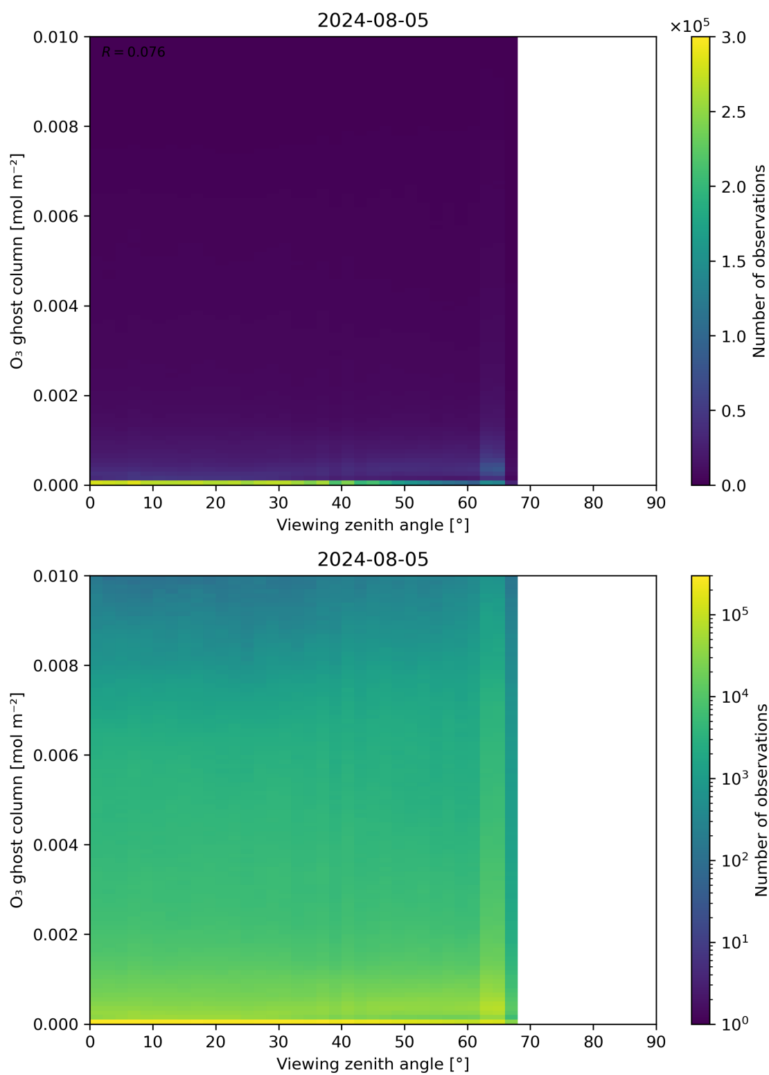
Figure 51: Scatter density plot of “Viewing zenith angle” against “O 3 ghost column” for 2024-08-04 to 2024-08-06.
