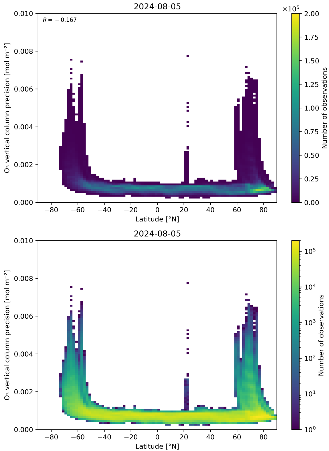
Figure 37: Scatter density plot of “Latitude” against “O 3 vertical column precision” for 2024-08-04 to 2024-08-06.
