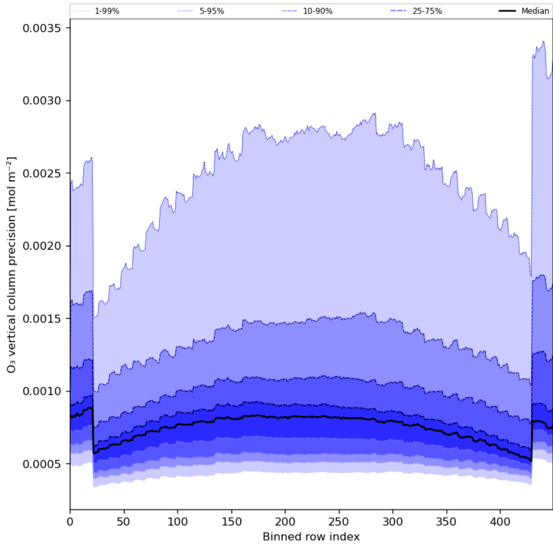
Figure 29: Along track statistics of “O 3 vertical column precision” for 2024-08-04 to 2024-08-06
