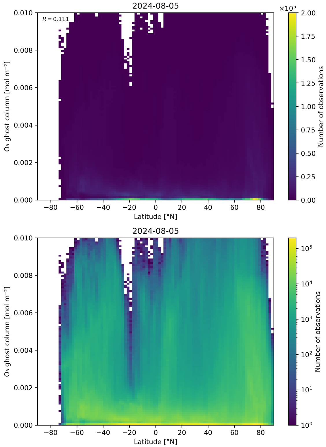
Figure 35: Scatter density plot of “Latitude” against “O 3 ghost column” for 2024-08-04 to 2024-08-06.
