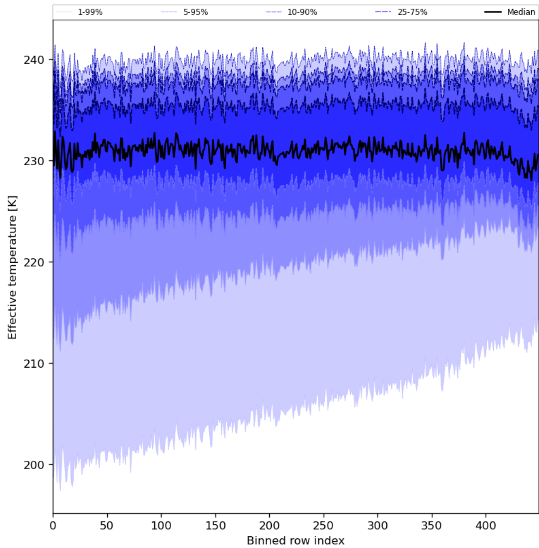
Figure 31: Along track statistics of “Effective temperature” for 2024-08-04 to 2024-08-06
