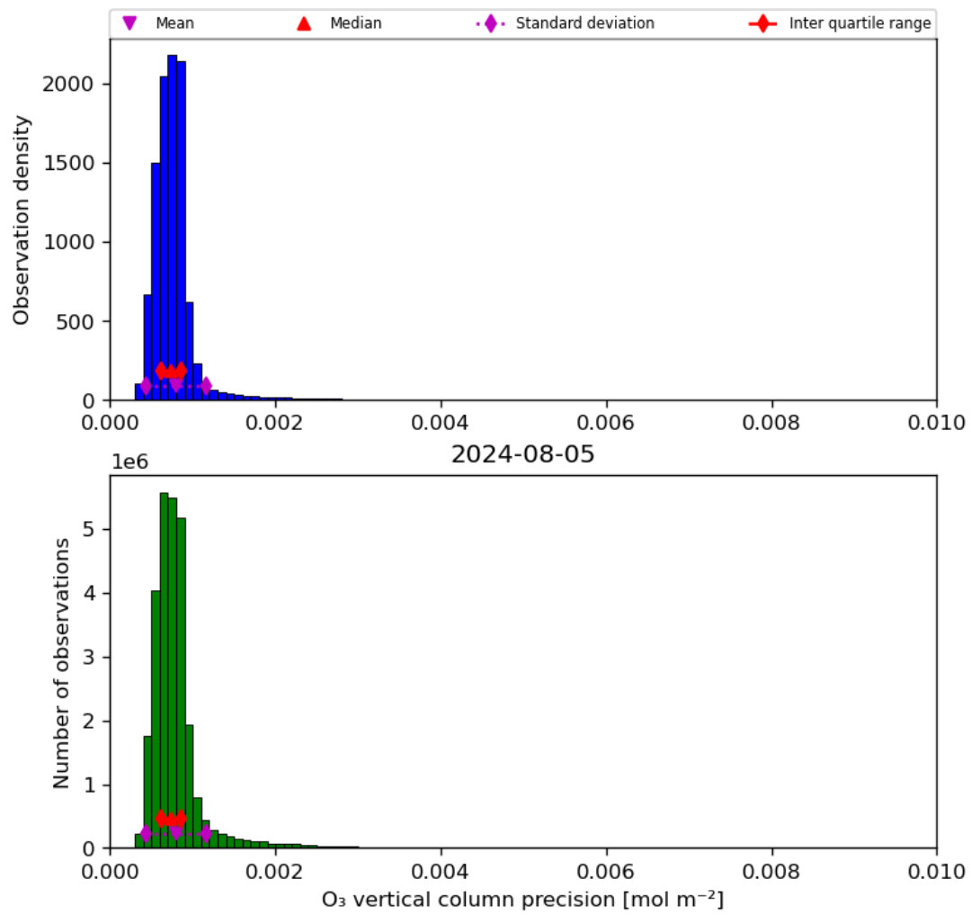
Figure 22: Histogram of “O 3 vertical column precision” for 2024-08-04 to 2024-08-06
