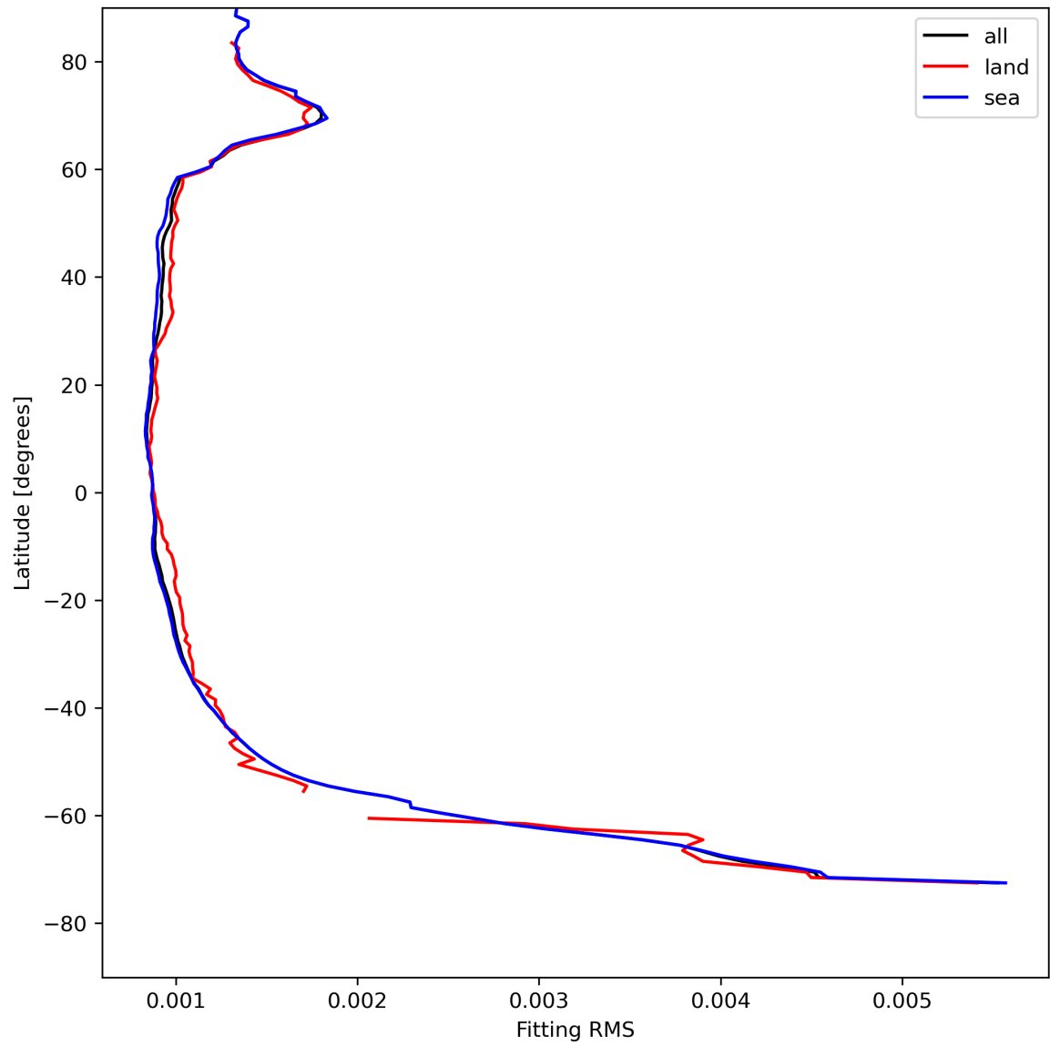
Figure 16: Zonal average of “Fitting RMS” for 2024-08-04 to 2024-08-06.
