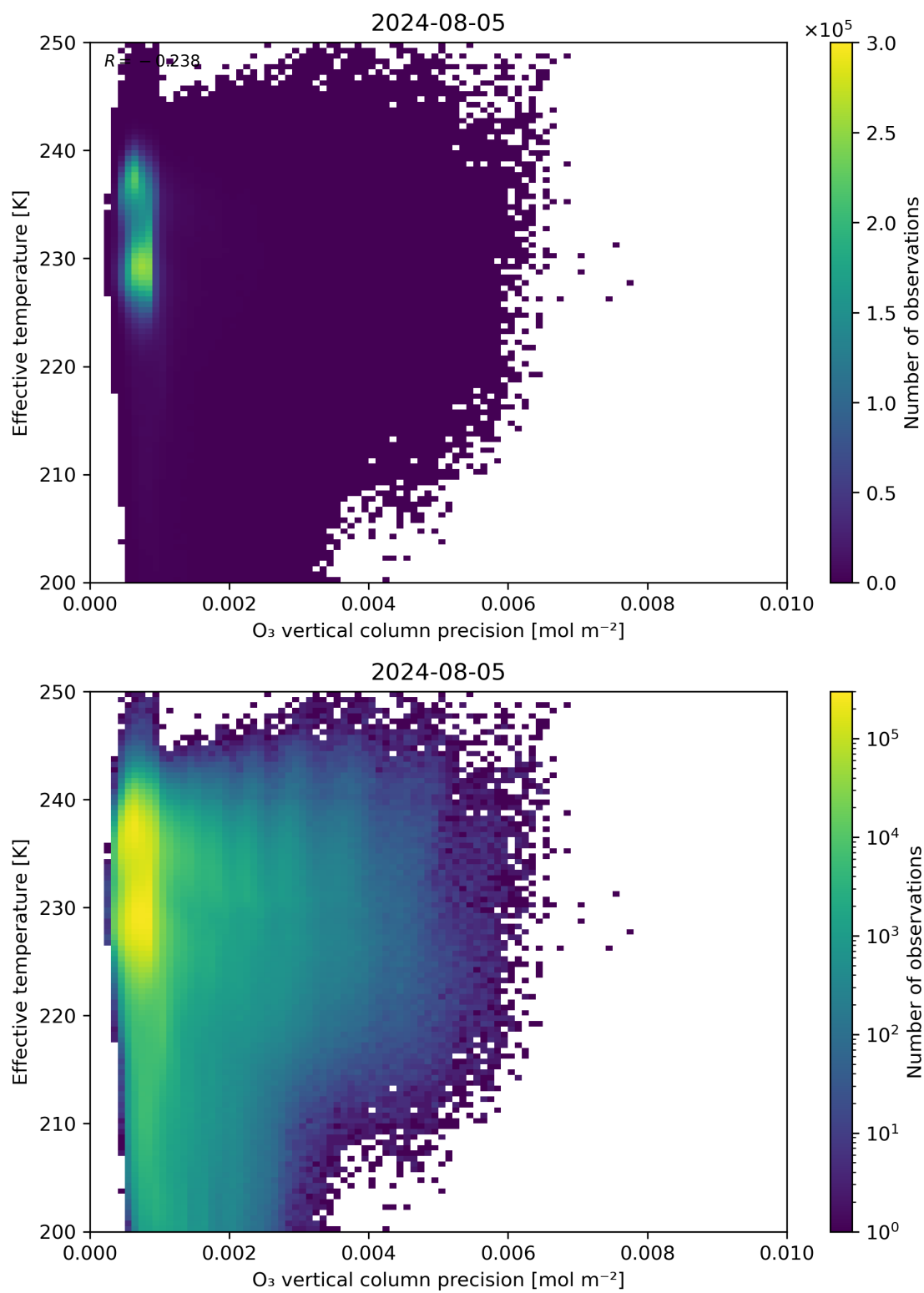
Figure 42: Scatter density plot of “O 3 vertical column precision” against “Effective temperature” for 2024-08-04 to 2024-08-06.
