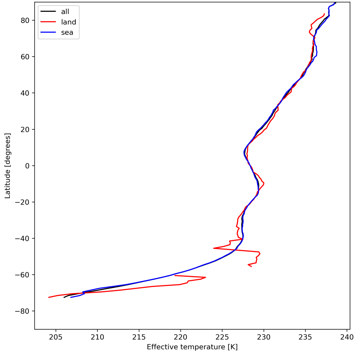
Figure 17: Zonal average of “Effective temperature” for 2024-08-04 to 2024-08-06.
