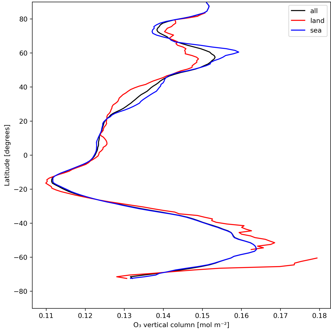
Figure 14: Zonal average of “O 3 vertical column” for 2024-08-04 to 2024-08-06.
