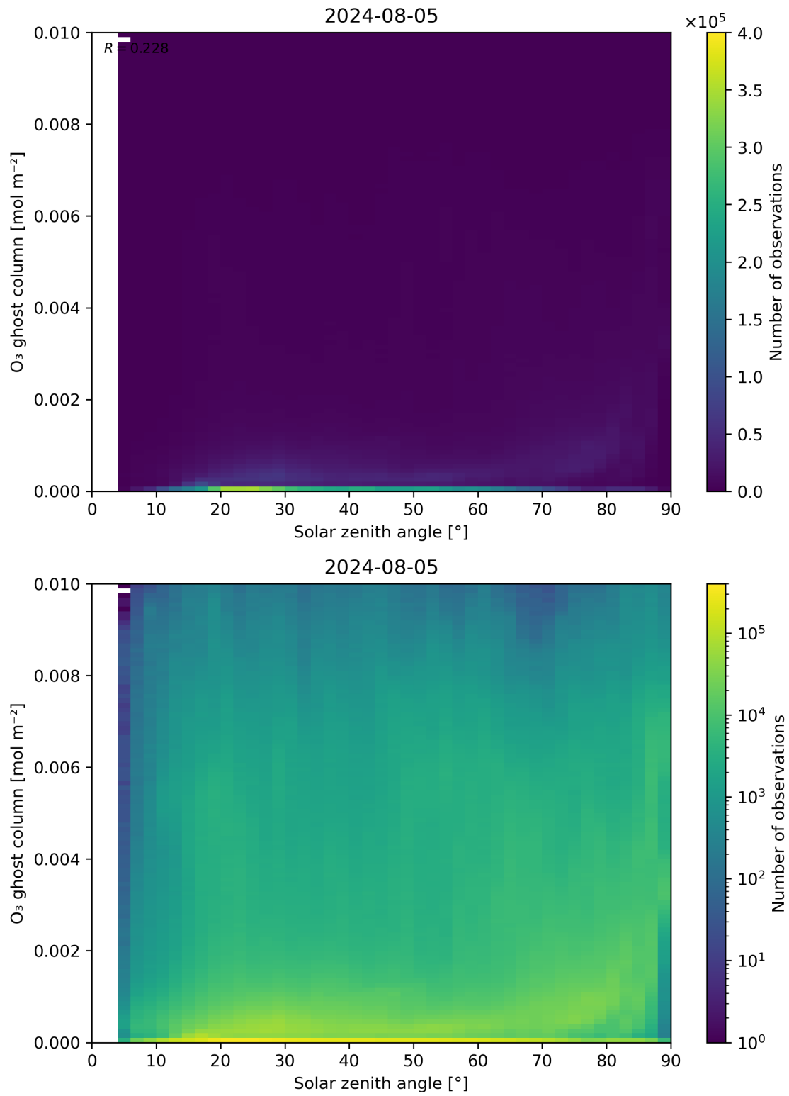
Figure 46: Scatter density plot of “Solar zenith angle” against “O 3 ghost column” for 2024-08-04 to 2024-08-06.
