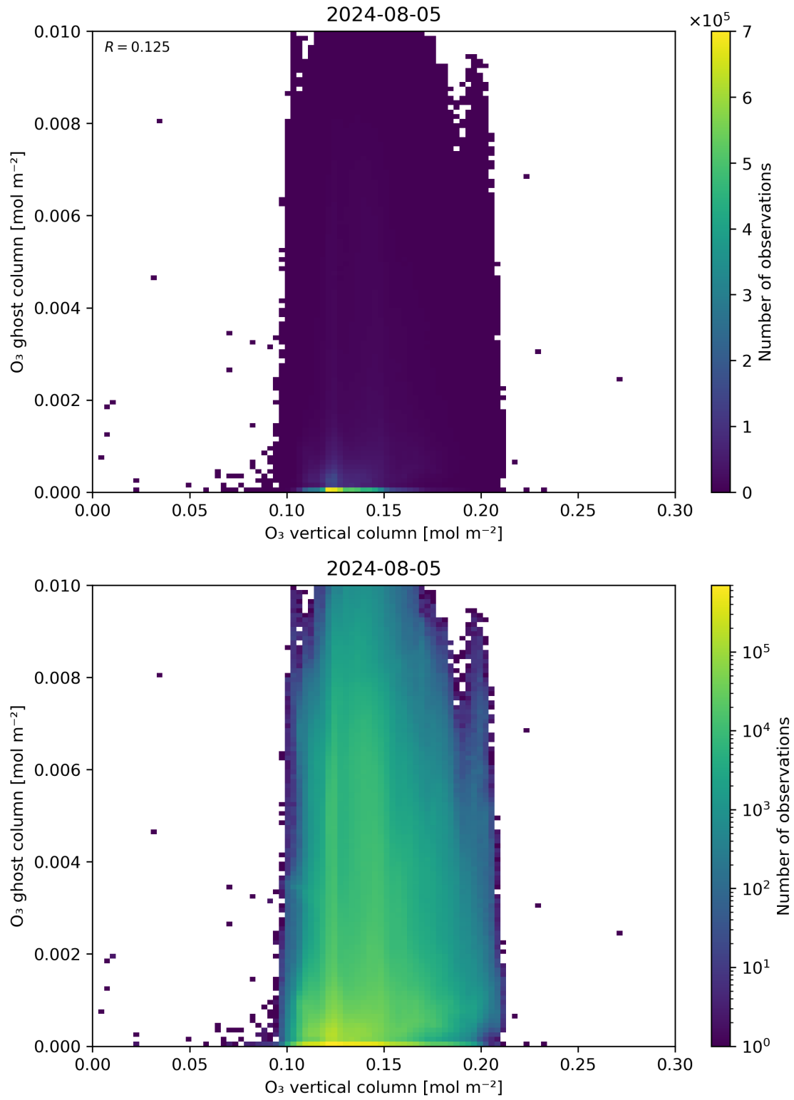
Figure 40: Scatter density plot of “O 3 vertical column” against “O 3 ghost column” for 2024-08-04 to 2024-08-06.
