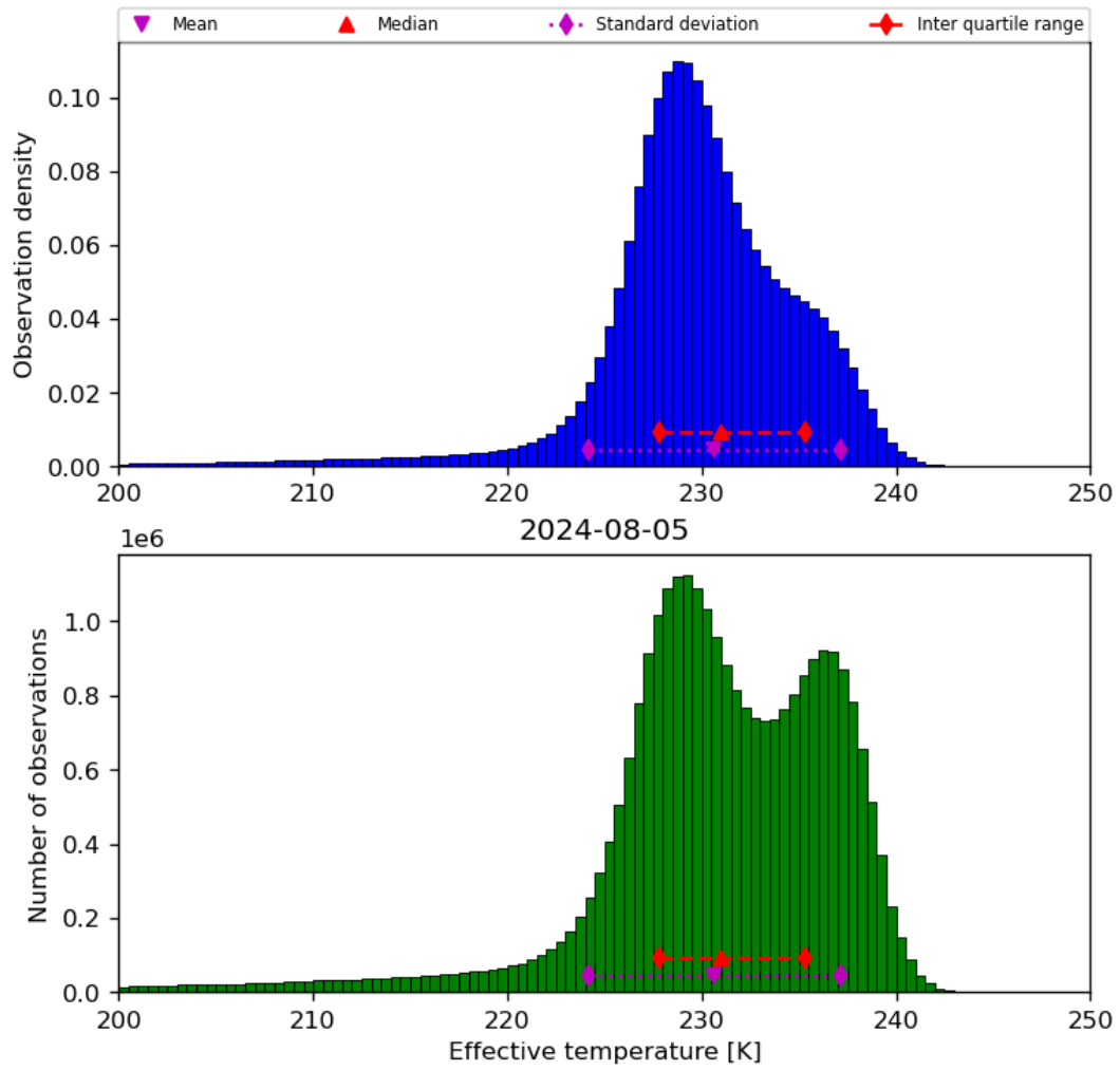
Figure 24: Histogram of “Effective temperature” for 2024-08-04 to 2024-08-06
