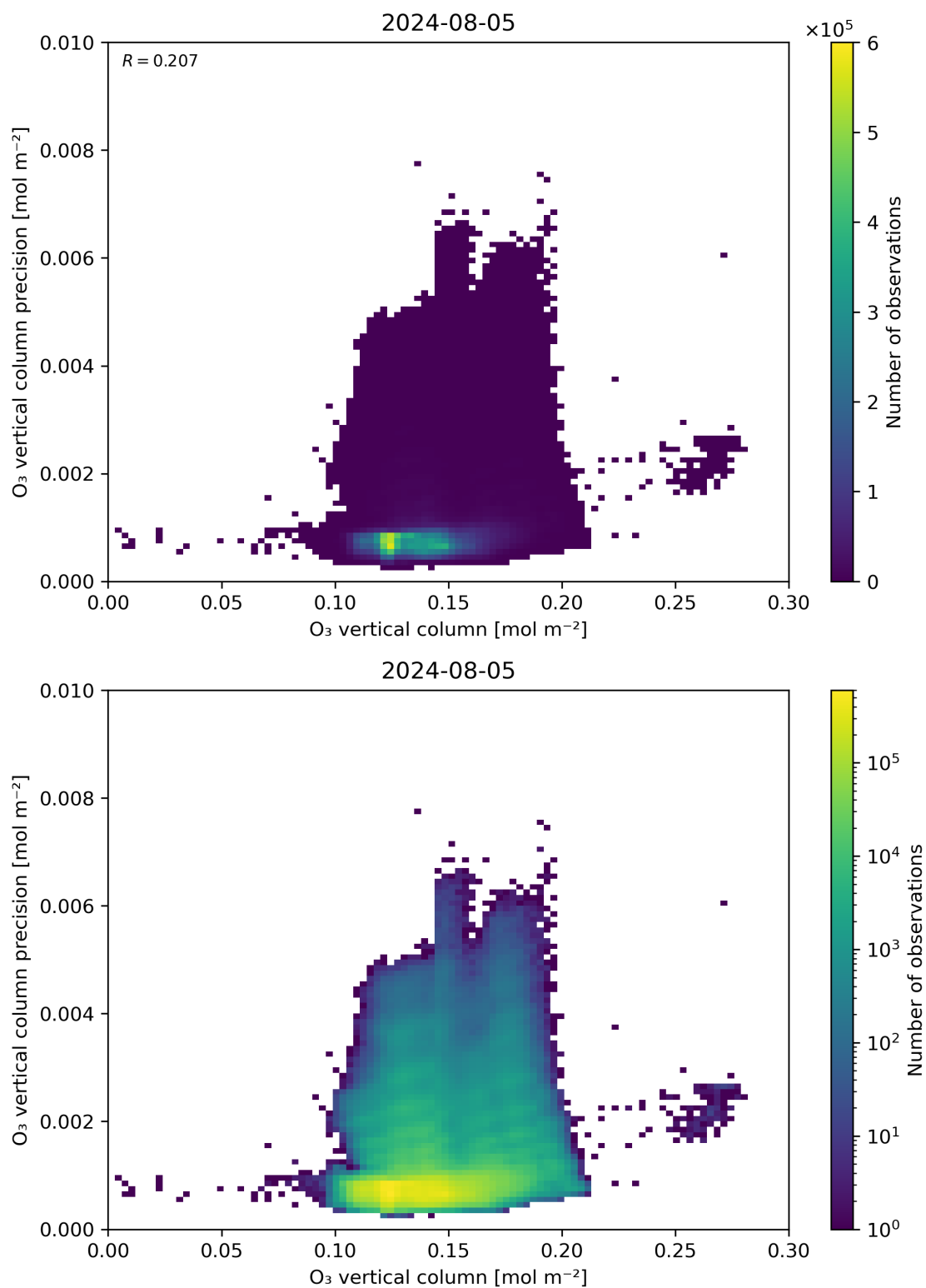
Figure 41: Scatter density plot of “O 3 vertical column” against “O 3 vertical column precision” for 2024-08-04 to 2024-08-06.
