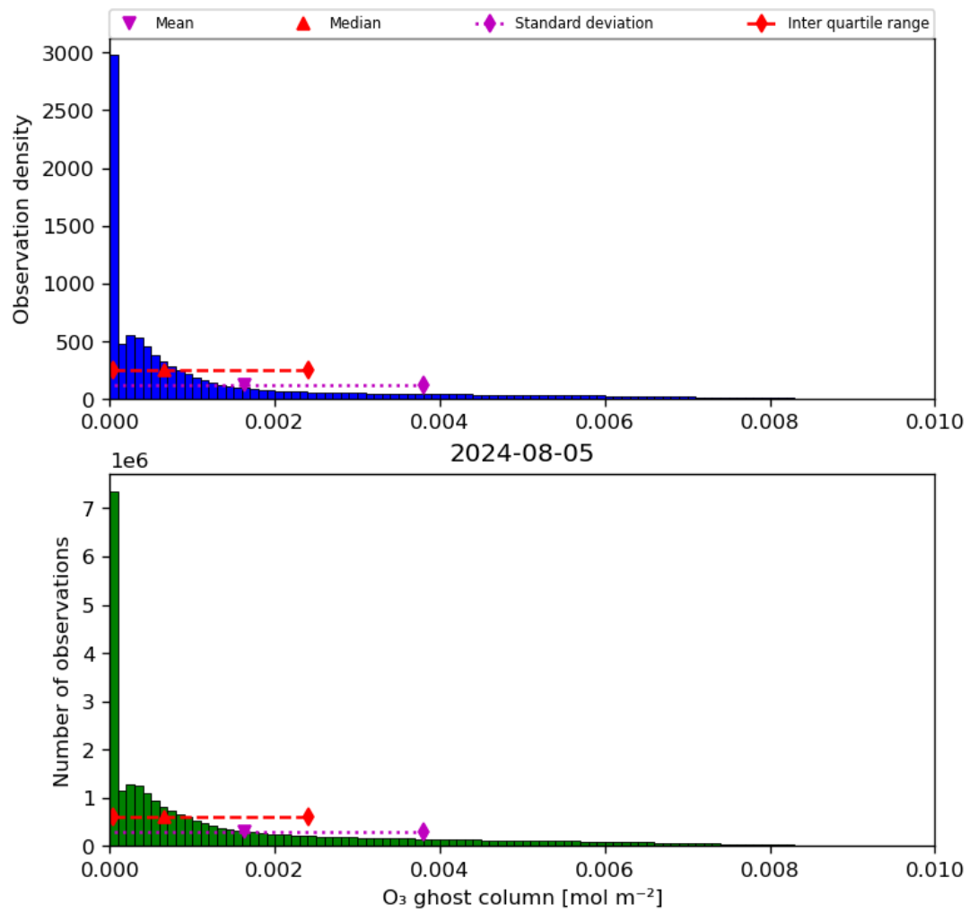
Figure 25: Histogram of “O 3 ghost column” for 2024-08-04 to 2024-08-06
