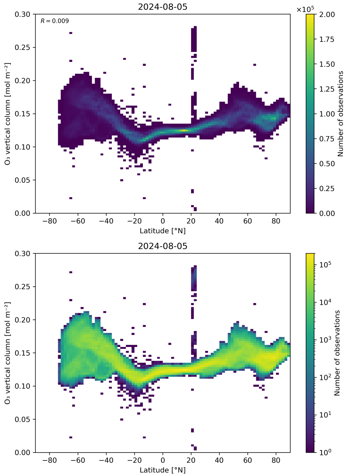
Figure 36: Scatter density plot of “Latitude” against “O 3 vertical column” for 2024-08-04 to 2024-08-06.
