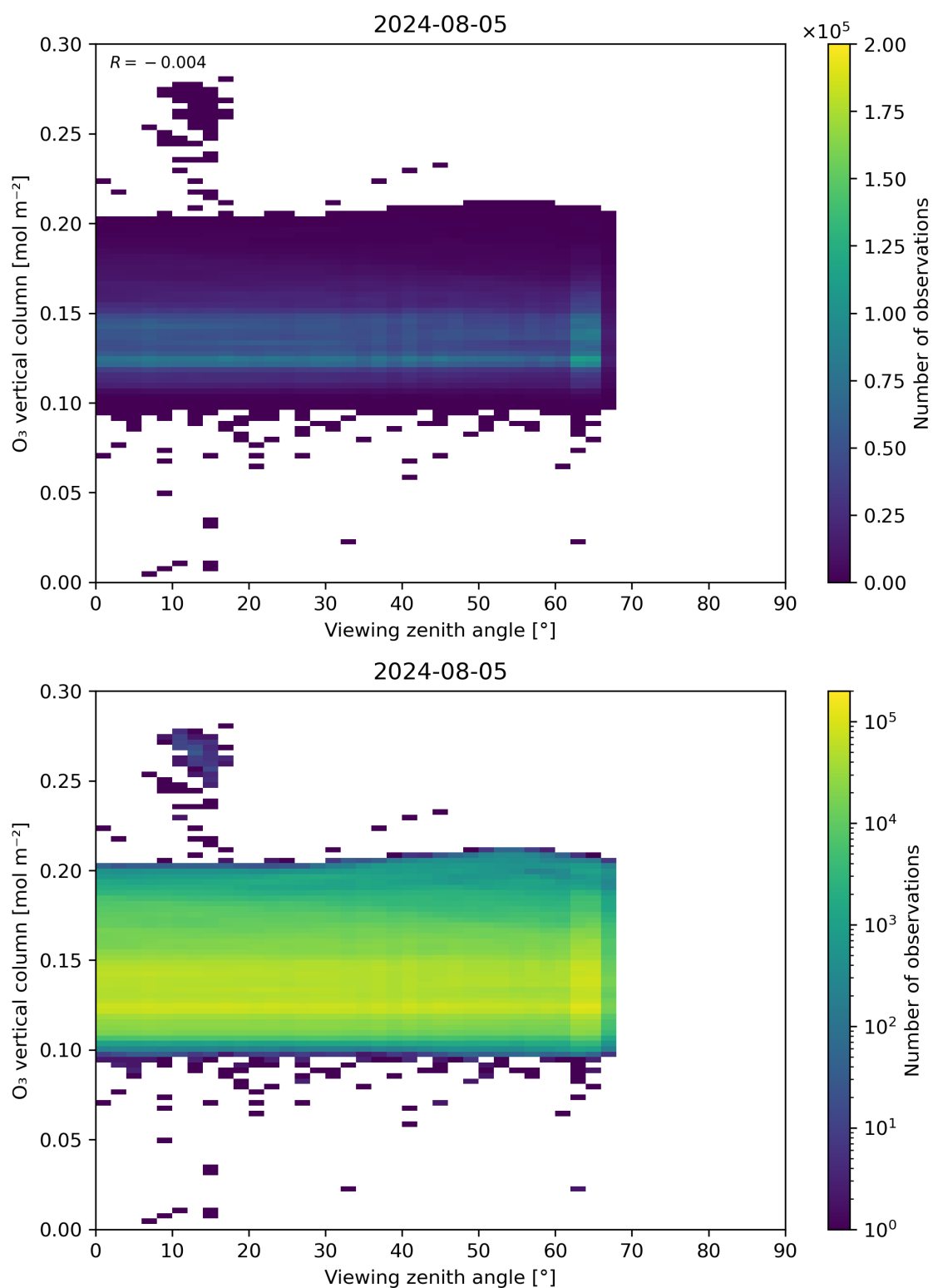
Figure 52: Scatter density plot of “Viewing zenith angle” against “O 3 vertical column” for 2024-08-04 to 2024-08-06.
