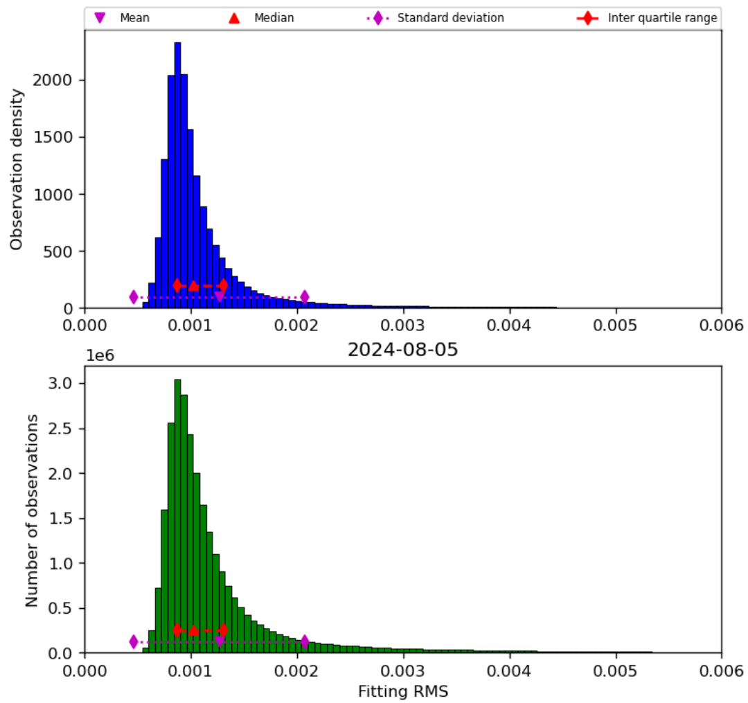
Figure 23: Histogram of “Fitting RMS” for 2024-08-04 to 2024-08-06
