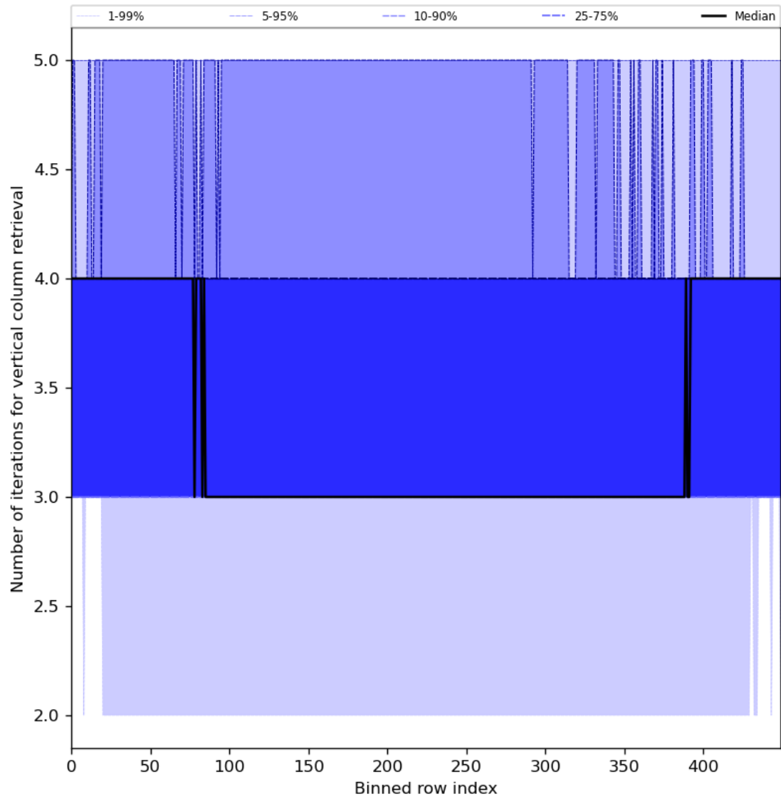
Figure 33: Along track statistics of “Number of iterations for vertical column retrieval” for 2024-08-04 to 2024-08-06
