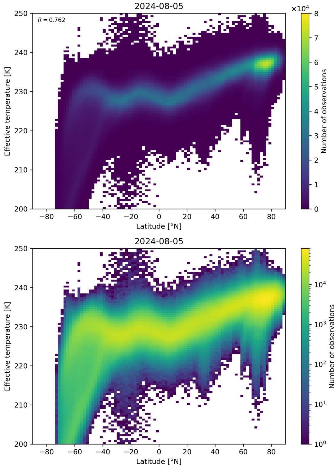
Figure 34: Scatter density plot of “Latitude” against “Effective temperature” for 2024-08-04 to 2024-08-06.
