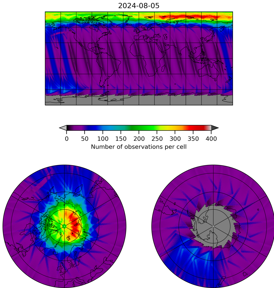
Figure 12: Map of the number of observations for 2024-08-04 to 2024-08-06
