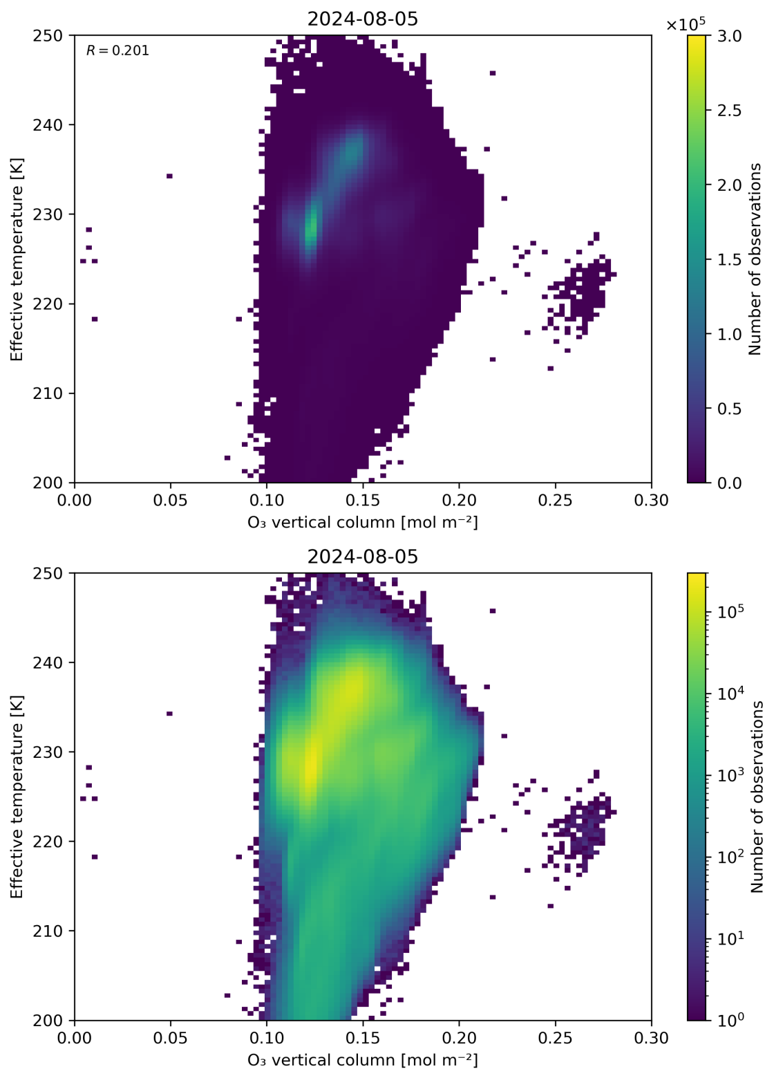
Figure 39: Scatter density plot of “O 3 vertical column” against “Effective temperature” for 2024-08-04 to 2024-08-06.
