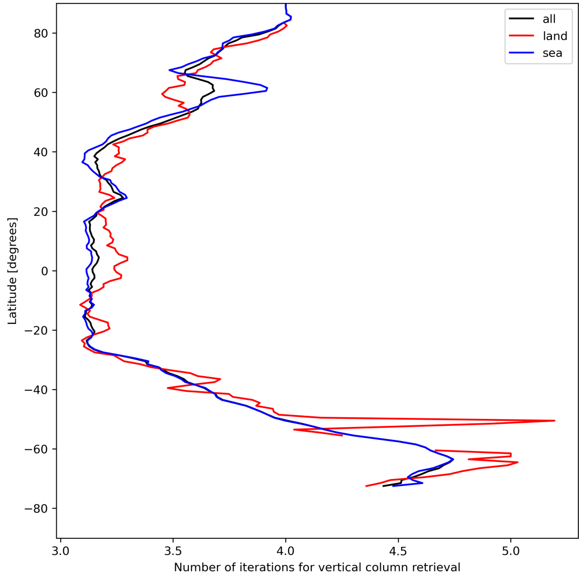
Figure 19: Zonal average of “Number of iterations for vertical column retrieval” for 2024-08-04 to 2024-08-06.
