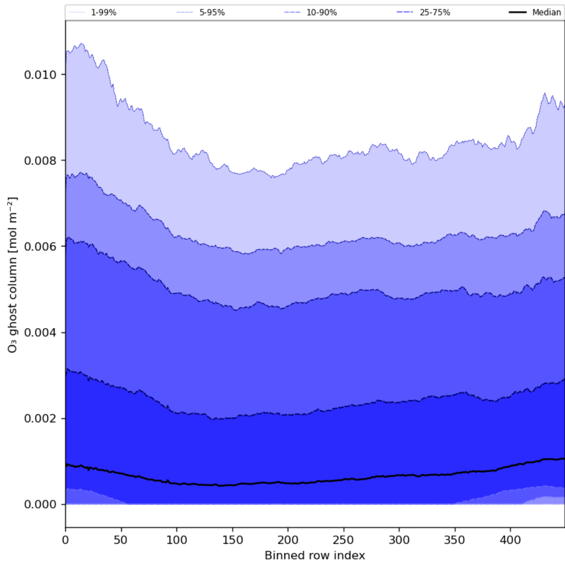
Figure 32: Along track statistics of “O 3 ghost column” for 2024-08-04 to 2024-08-06
