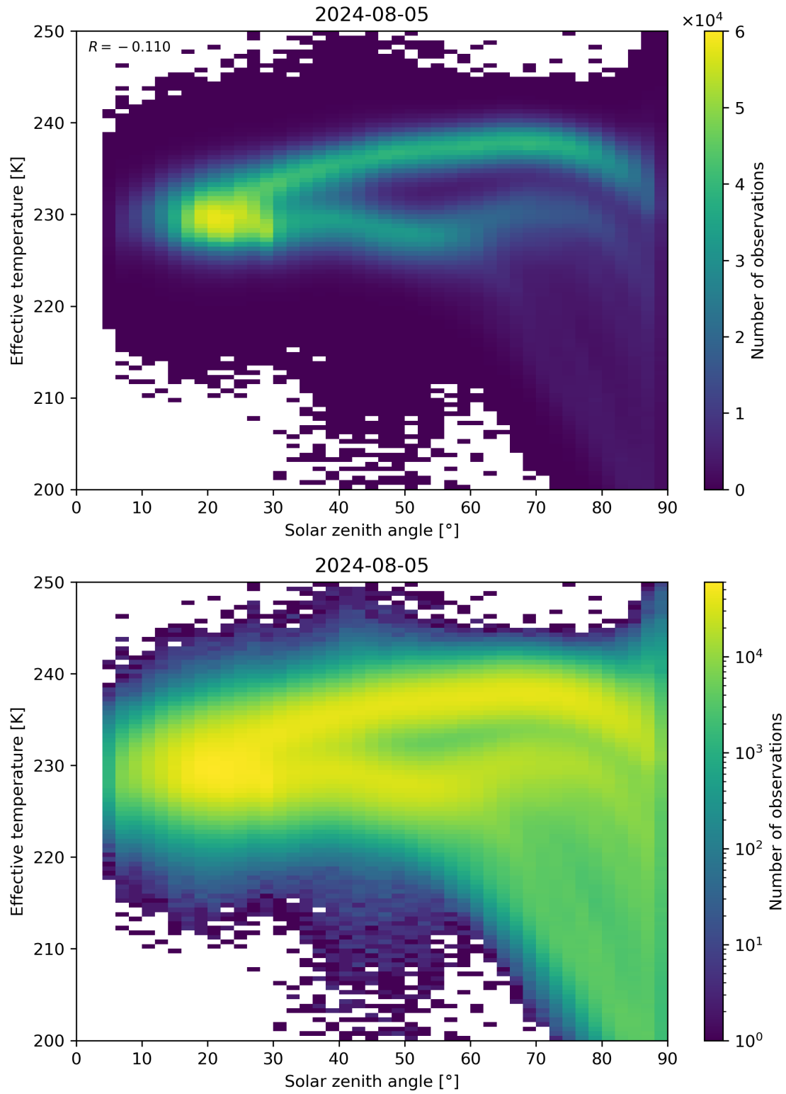
Figure 45: Scatter density plot of “Solar zenith angle” against “Effective temperature” for 2024-08-04 to 2024-08-06.
