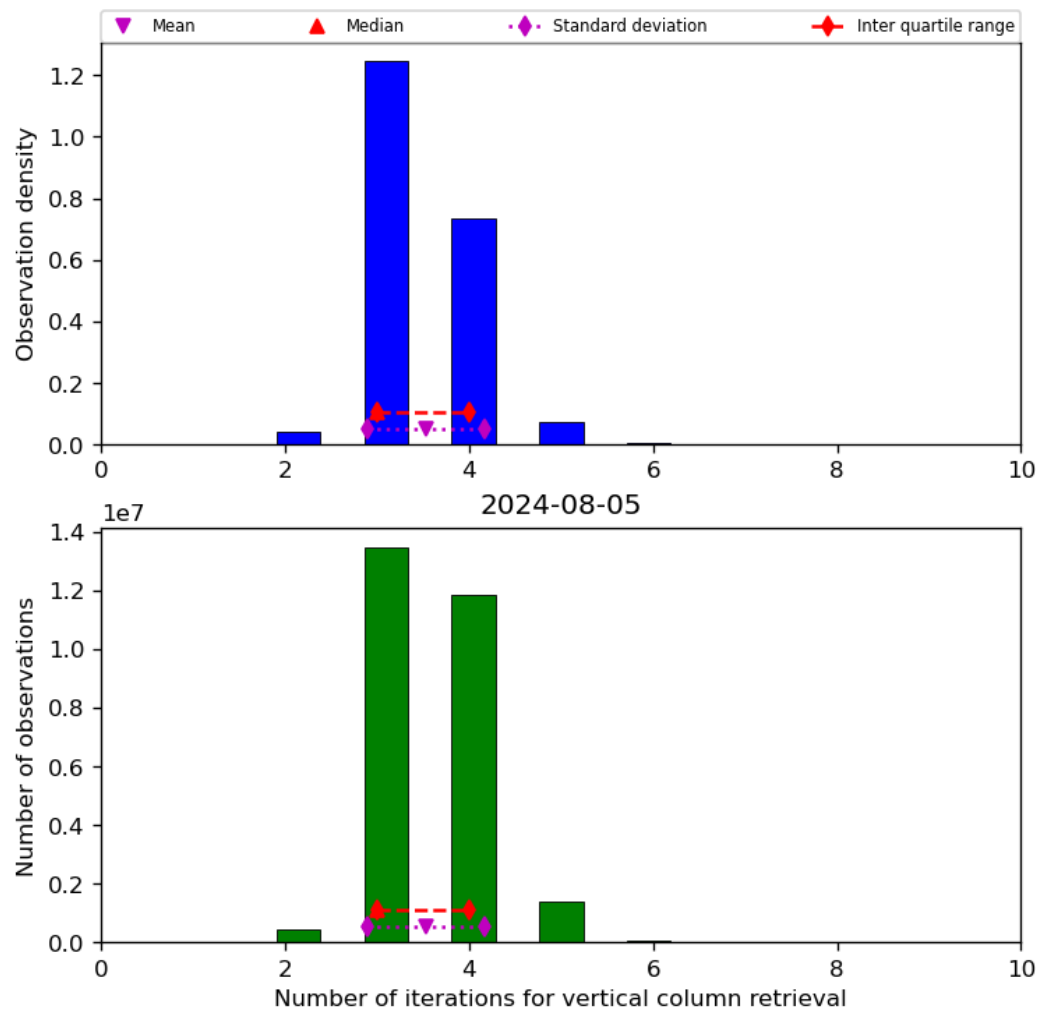
Figure 26: Histogram of “Number of iterations for vertical column retrieval” for 2024-08-04 to 2024-08-06
