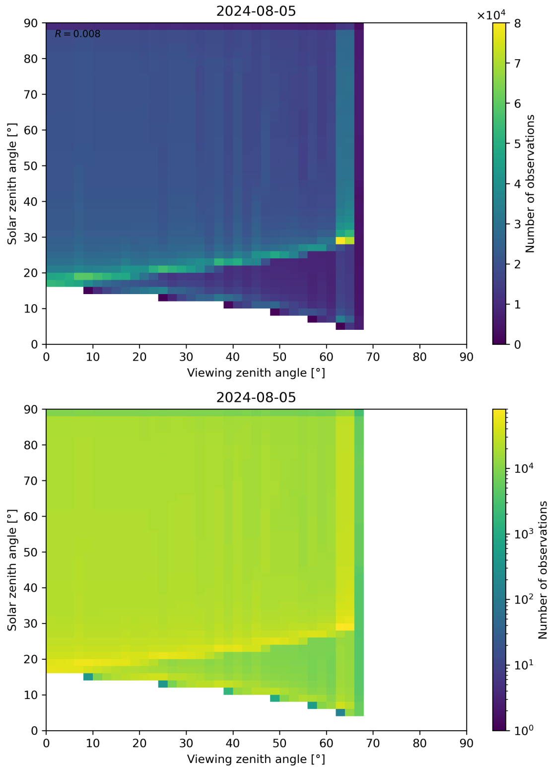
Figure 54: Scatter density plot of “Viewing zenith angle” against “Solar zenith angle” for 2024-08-04 to 2024-08-06.
