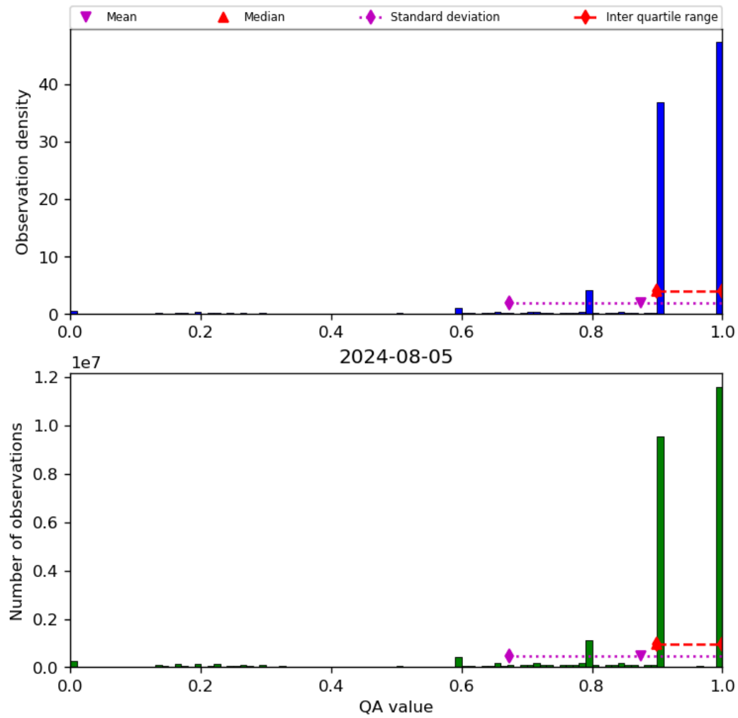
Figure 20: Histogram of “QA value” for 2024-08-04 to 2024-08-06
