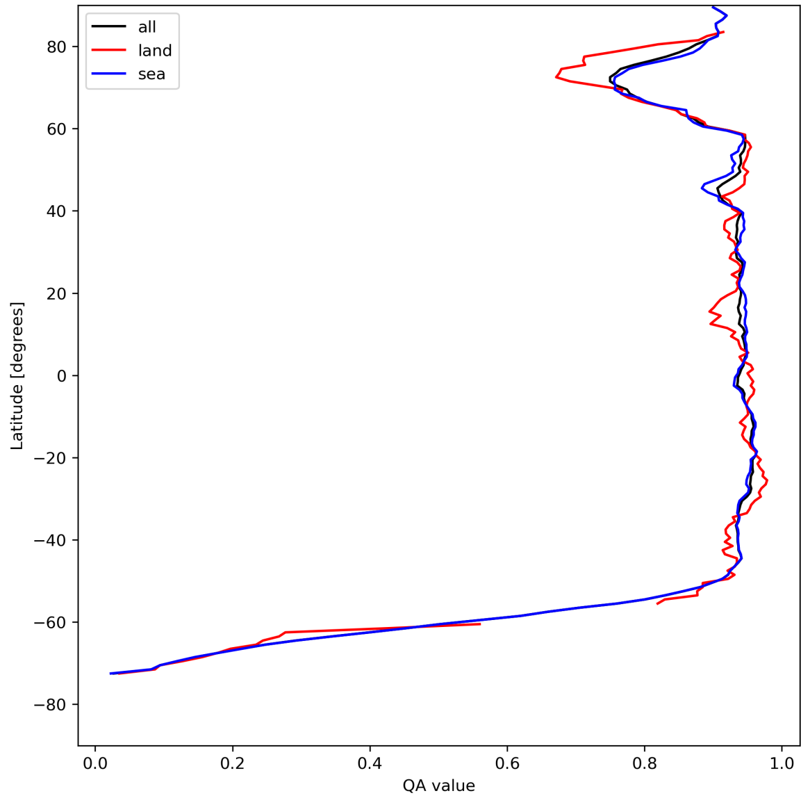
Figure 13: Zonal average of “QA value” for 2024-08-04 to 2024-08-06.
