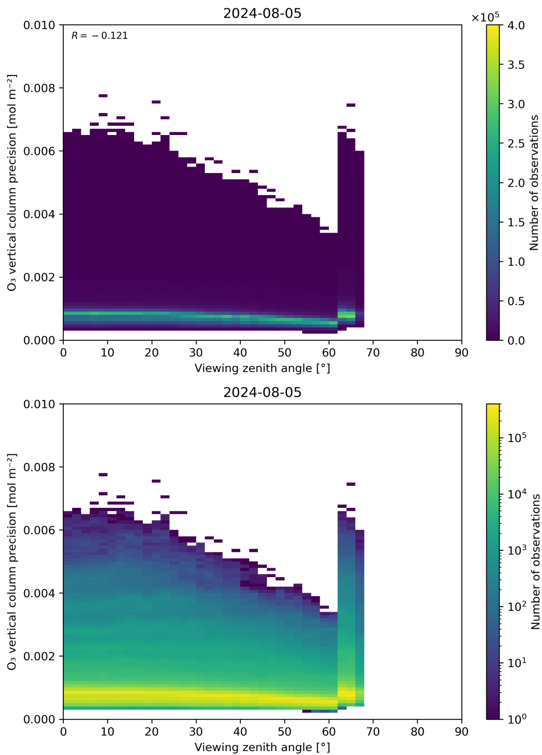
Figure 53: Scatter density plot of “Viewing zenith angle” against “O 3 vertical column precision” for 2024-08-04 to 2024-08-06.
