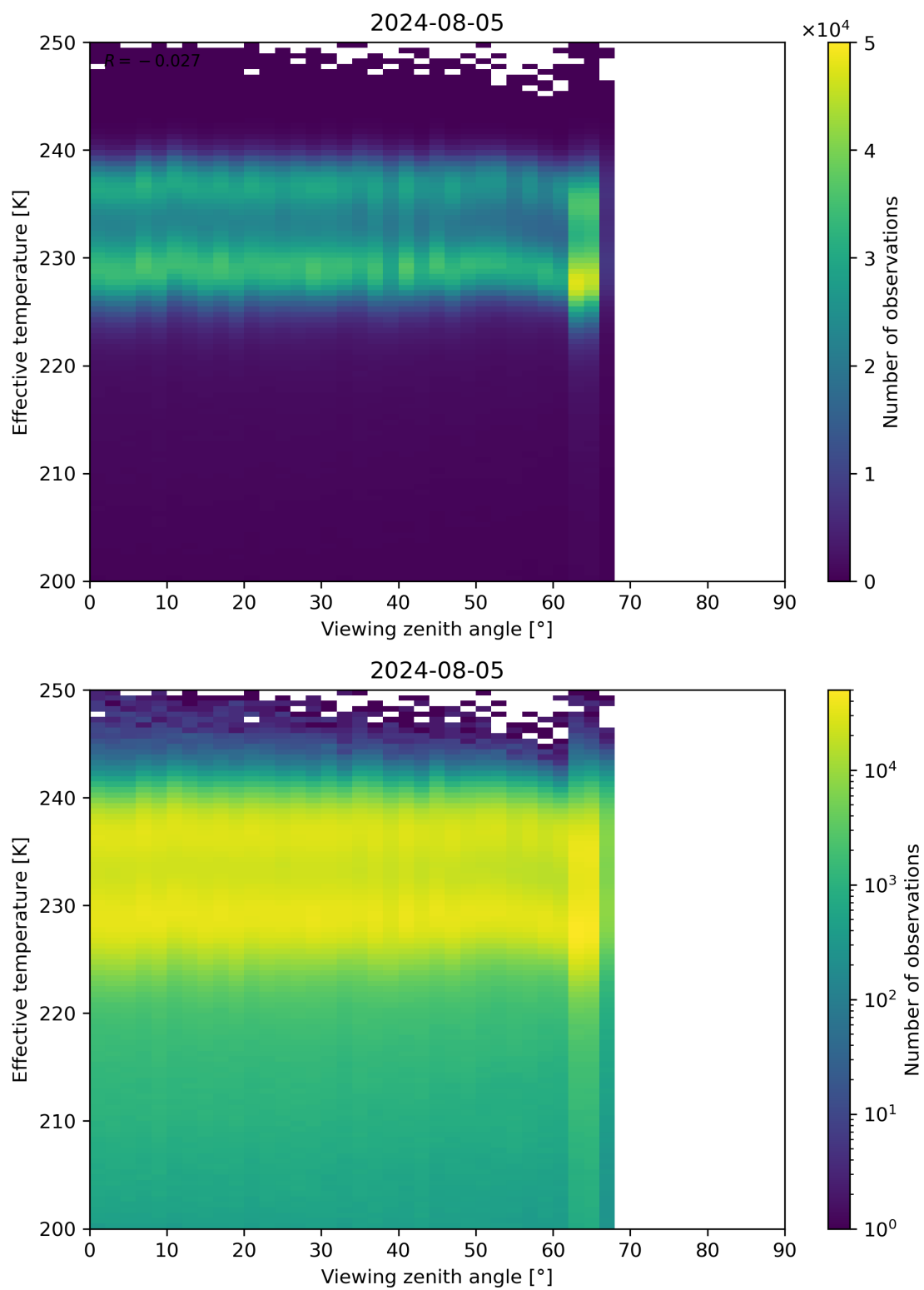
Figure 50: Scatter density plot of “Viewing zenith angle” against “Effective temperature” for 2024-08-04 to 2024-08-06.
