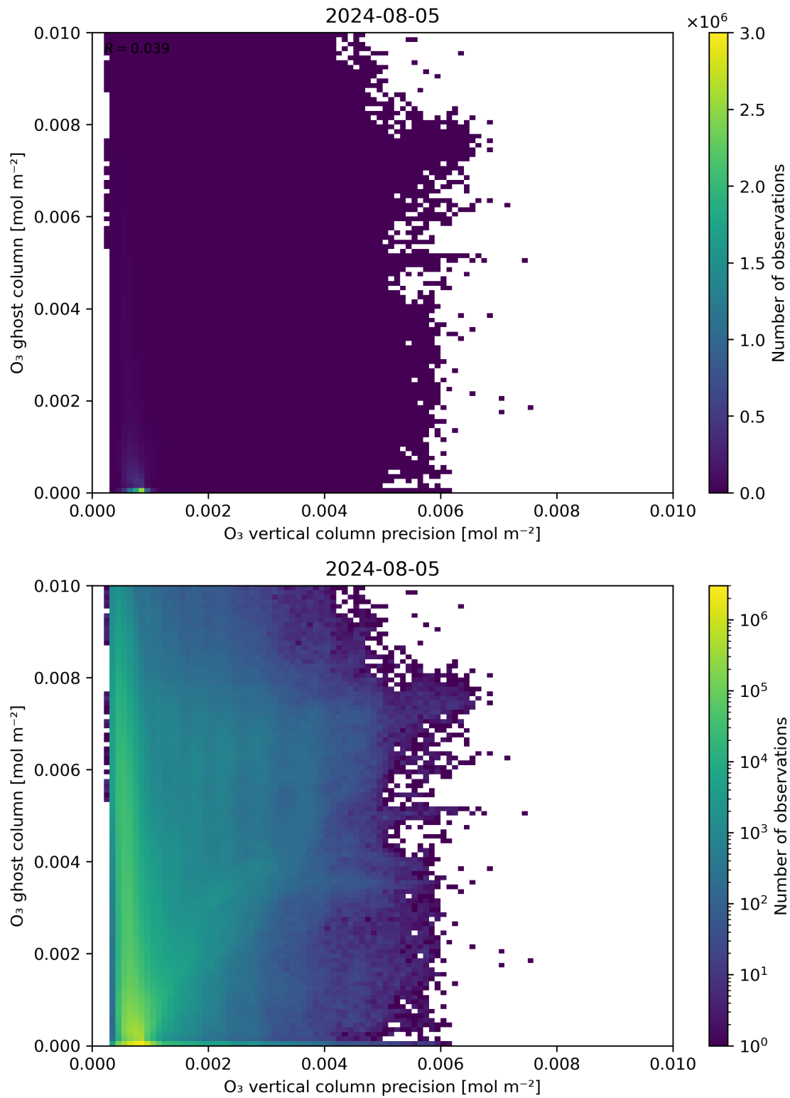
Figure 43: Scatter density plot of “ \text{O}_3 vertical column precision” against “ \text{O}_3 ghost column” for 2024-08-04 to 2024-08-06.
