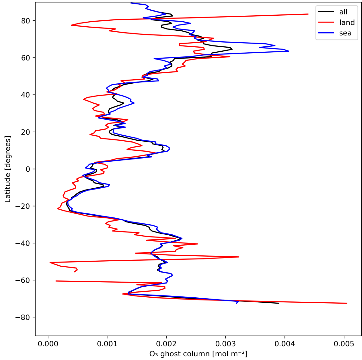
Figure 18: Zonal average of "O 3 ghost column" for 2024-08-04 to 2024-08-06.
