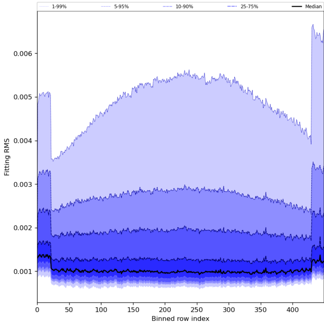
Figure 30: Along track statistics of “Fitting RMS” for 2024-08-04 to 2024-08-06
