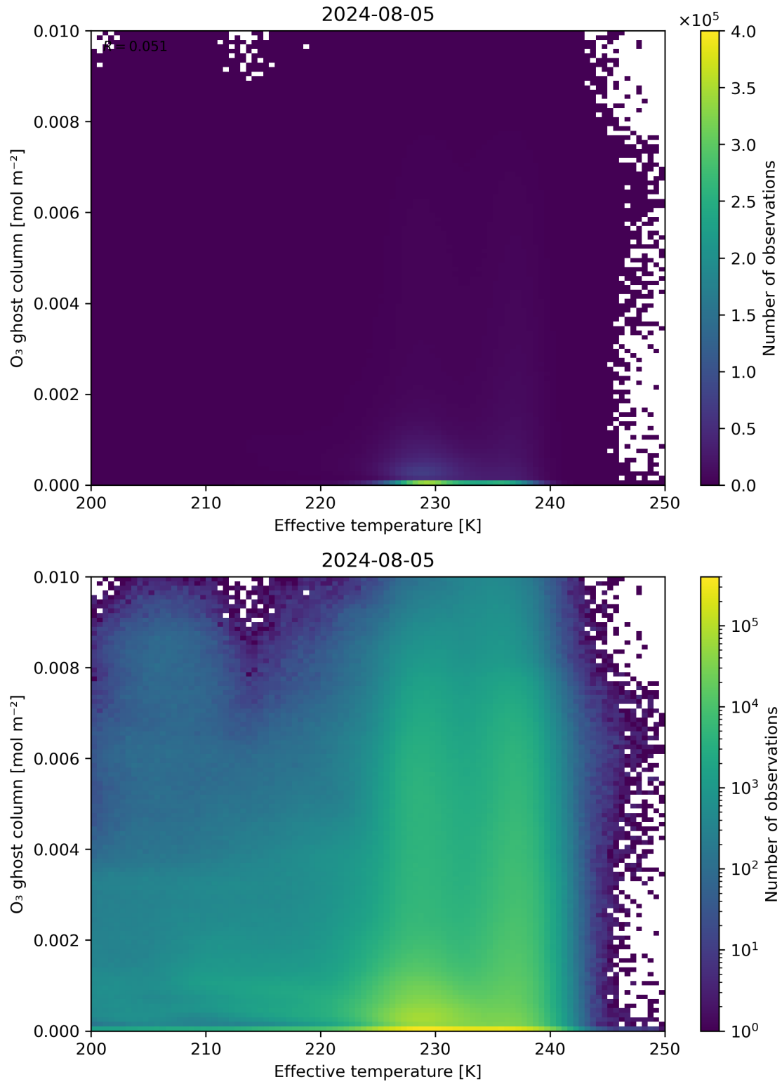
Figure 38: Scatter density plot of “Effective temperature” against “O 3 ghost column” for 2024-08-04 to 2024-08-06.
