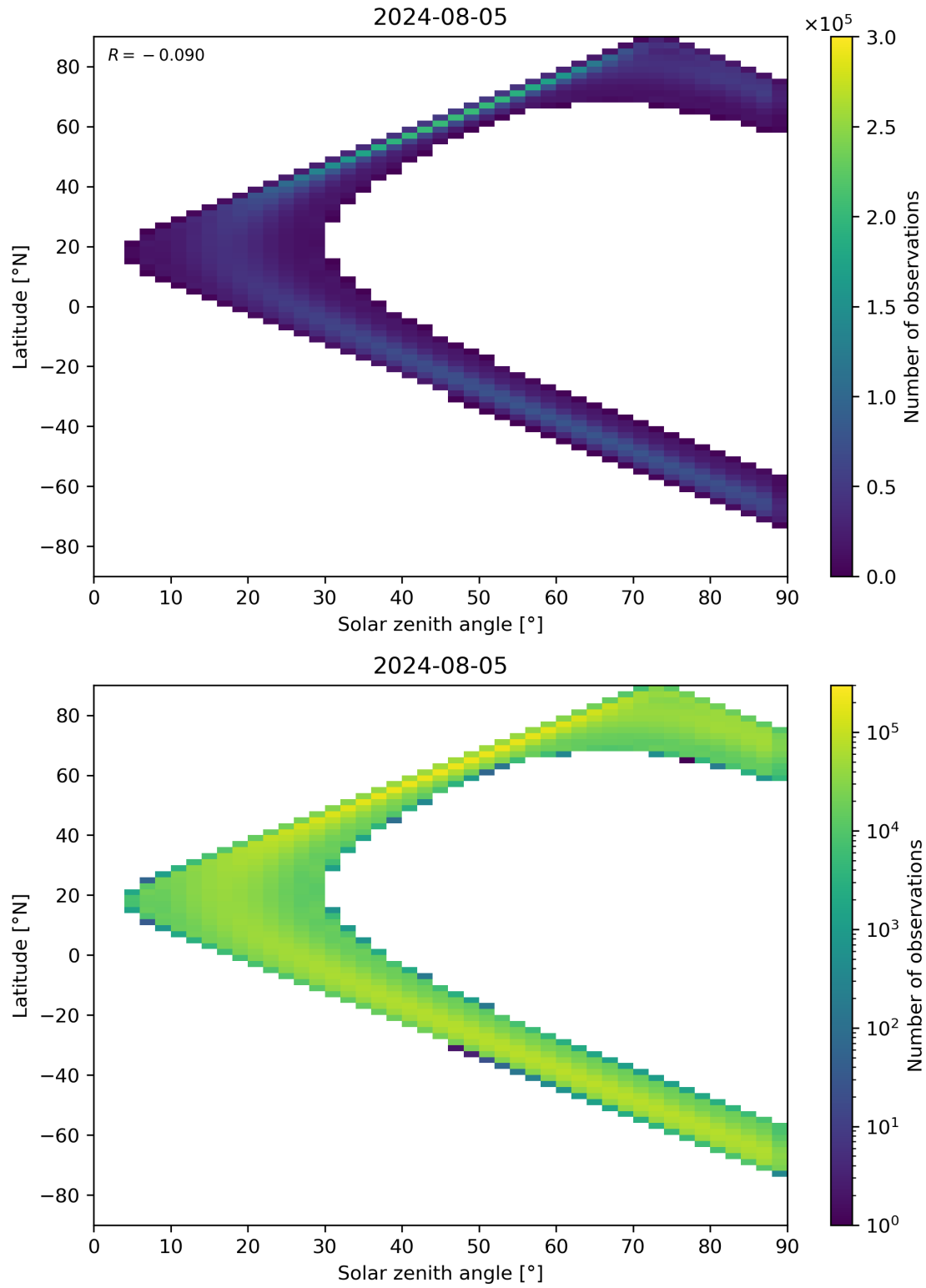
Figure 44: Scatter density plot of “Solar zenith angle” against “Latitude” for 2024-08-04 to 2024-08-06.
