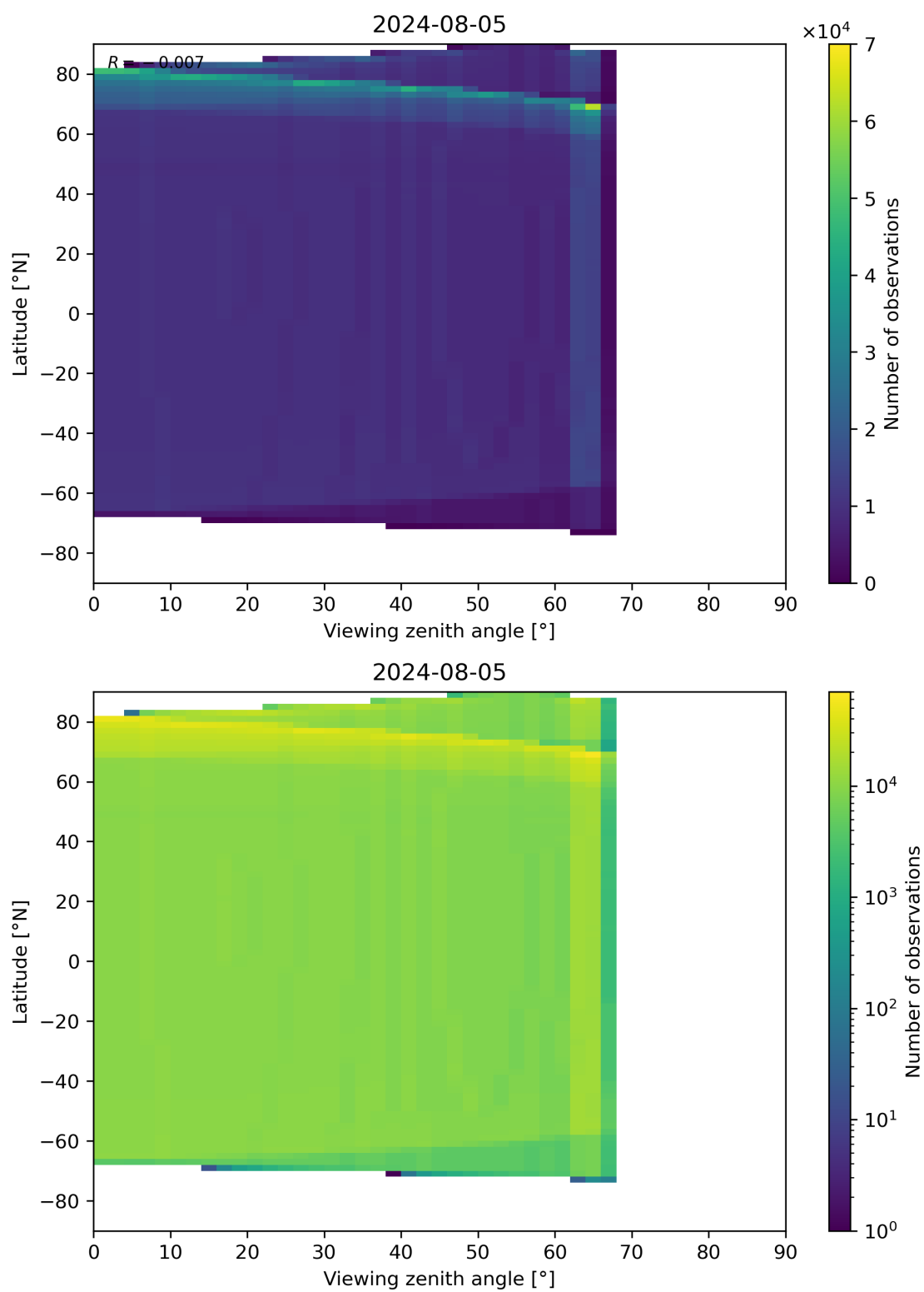
Figure 49: Scatter density plot of “Viewing zenith angle” against “Latitude” for 2024-08-04 to 2024-08-06.
