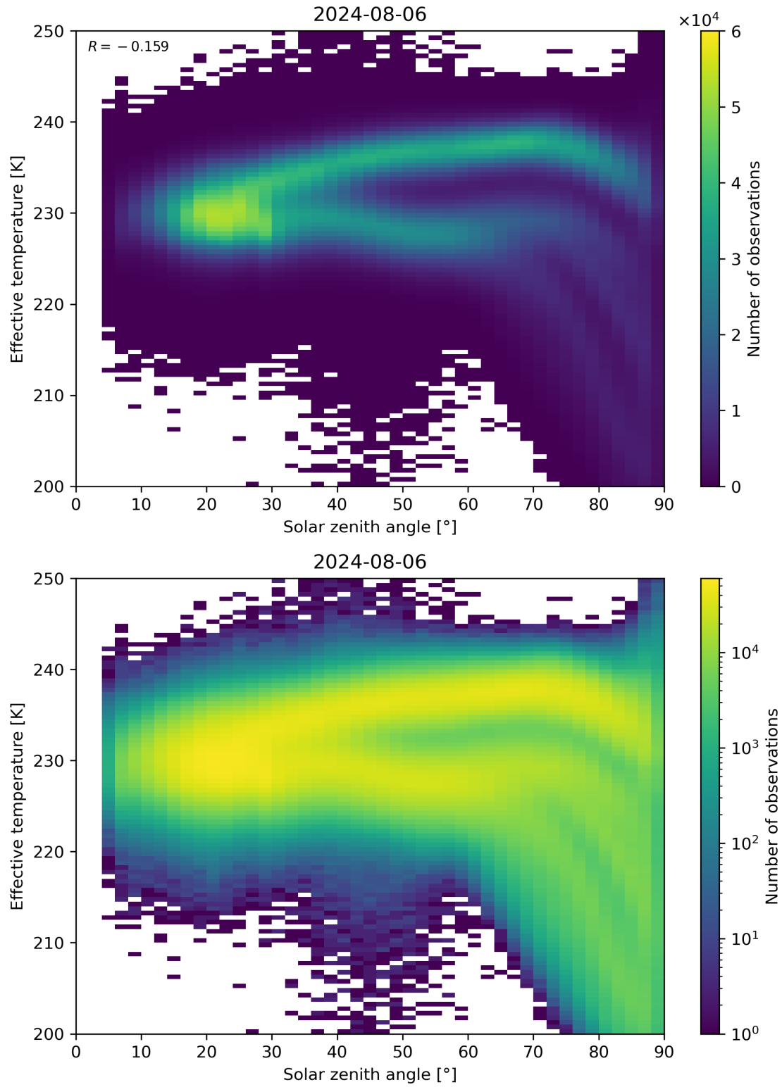
Figure 45: Scatter density plot of “Solar zenith angle” against “Effective temperature” for 2024-08-06 to 2024-08-07.
