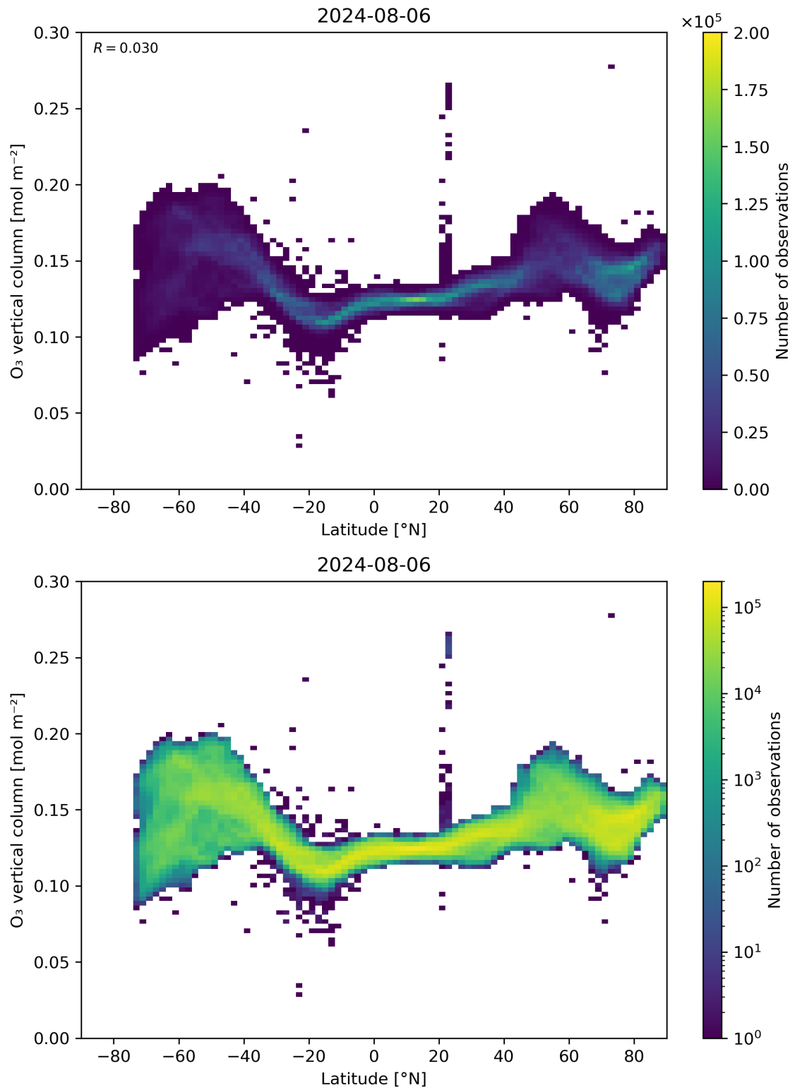
Figure 36: Scatter density plot of “Latitude” against “O 3 vertical column” for 2024-08-06 to 2024-08-07.
