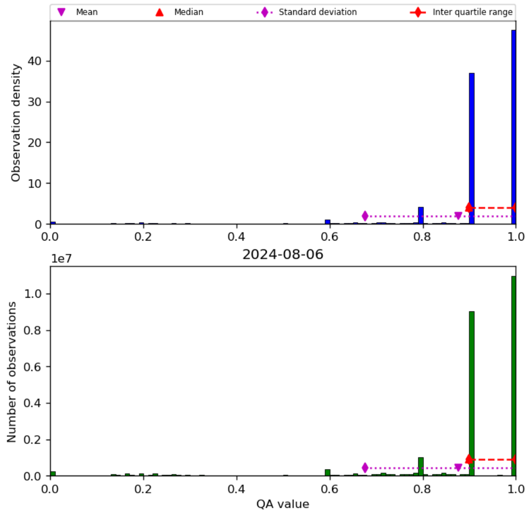
Figure 20: Histogram of “QA value” for 2024-08-06 to 2024-08-07
