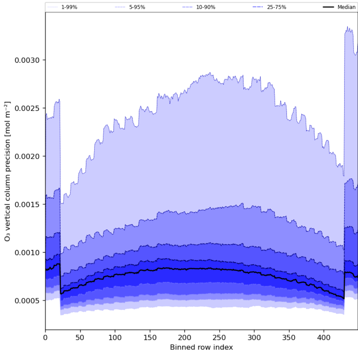
Figure 29: Along track statistics of “O 3 vertical column precision” for 2024-08-06 to 2024-08-07
