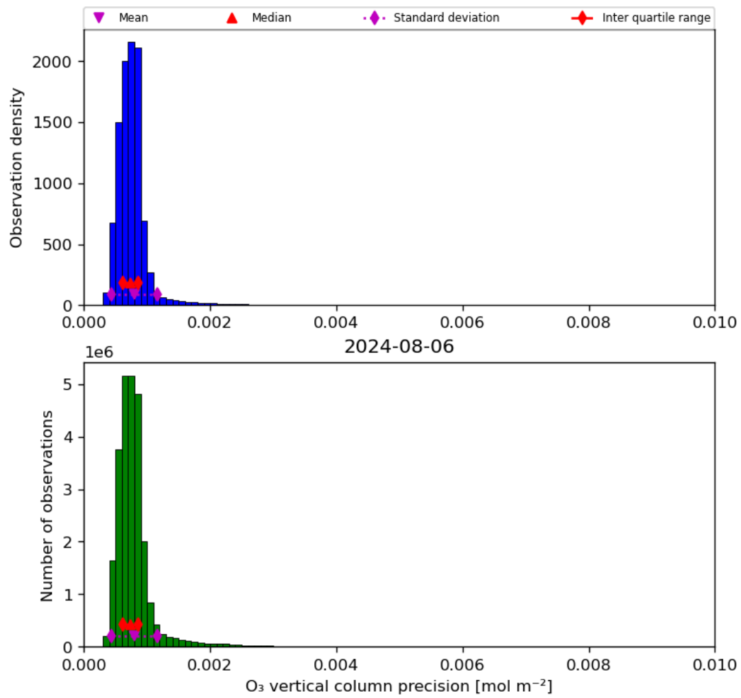
Figure 22: Histogram of “O 3 vertical column precision” for 2024-08-06 to 2024-08-07
