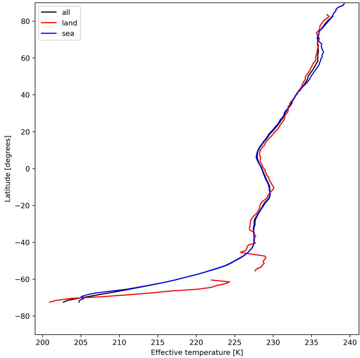
Figure 17: Zonal average of "Effective temperature" for 2024-08-06 to 2024-08-07.
