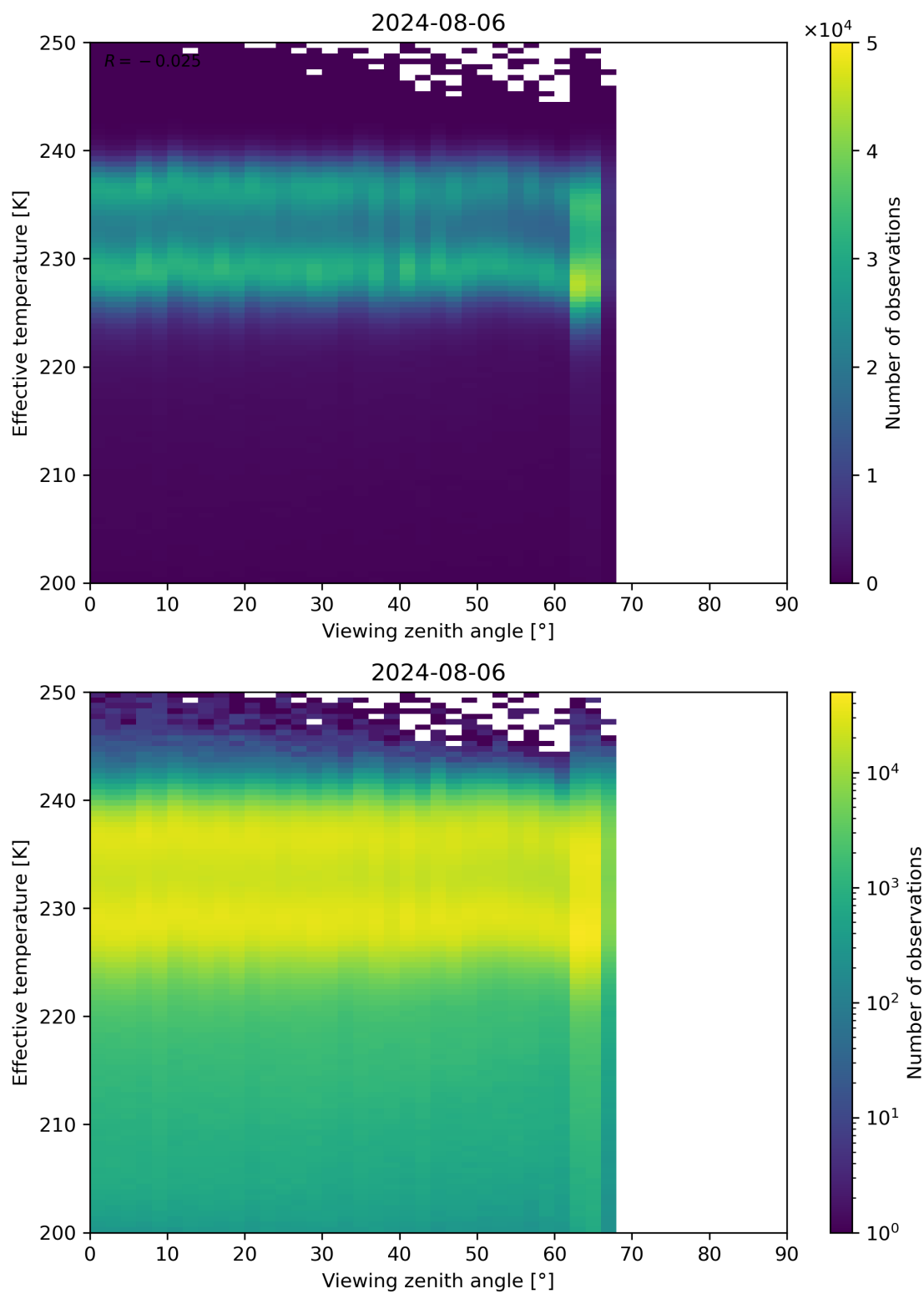
Figure 50: Scatter density plot of “Viewing zenith angle” against “Effective temperature” for 2024-08-06 to 2024-08-07.
