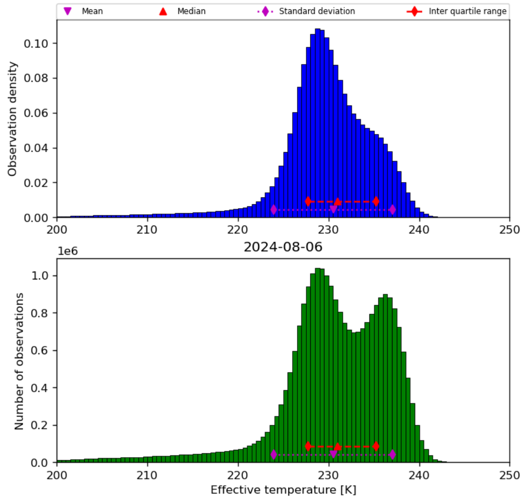
Figure 24: Histogram of “Effective temperature” for 2024-08-06 to 2024-08-07
