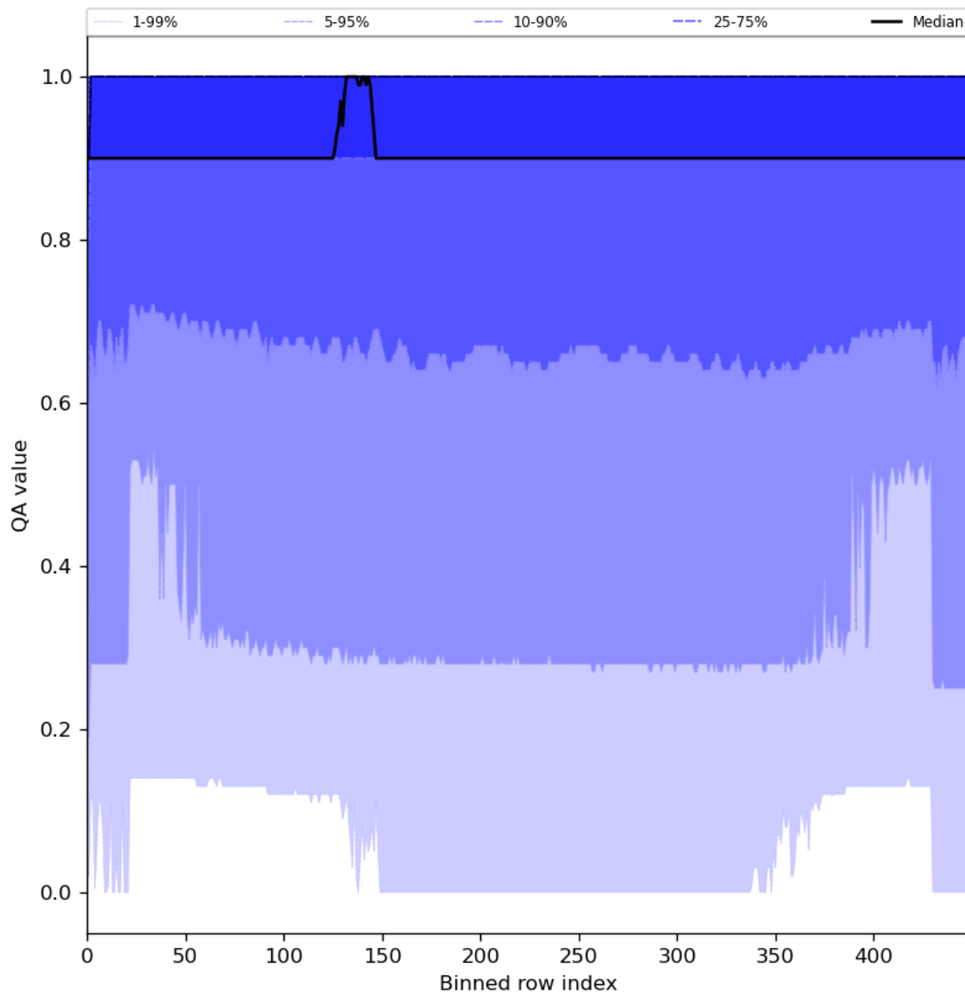
Figure 27: Along track statistics of “QA value” for 2024-08-06 to 2024-08-07
