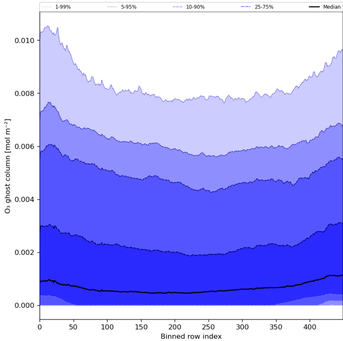
Figure 32: Along track statistics of "O 3 ghost column" for 2024-08-06 to 2024-08-07
