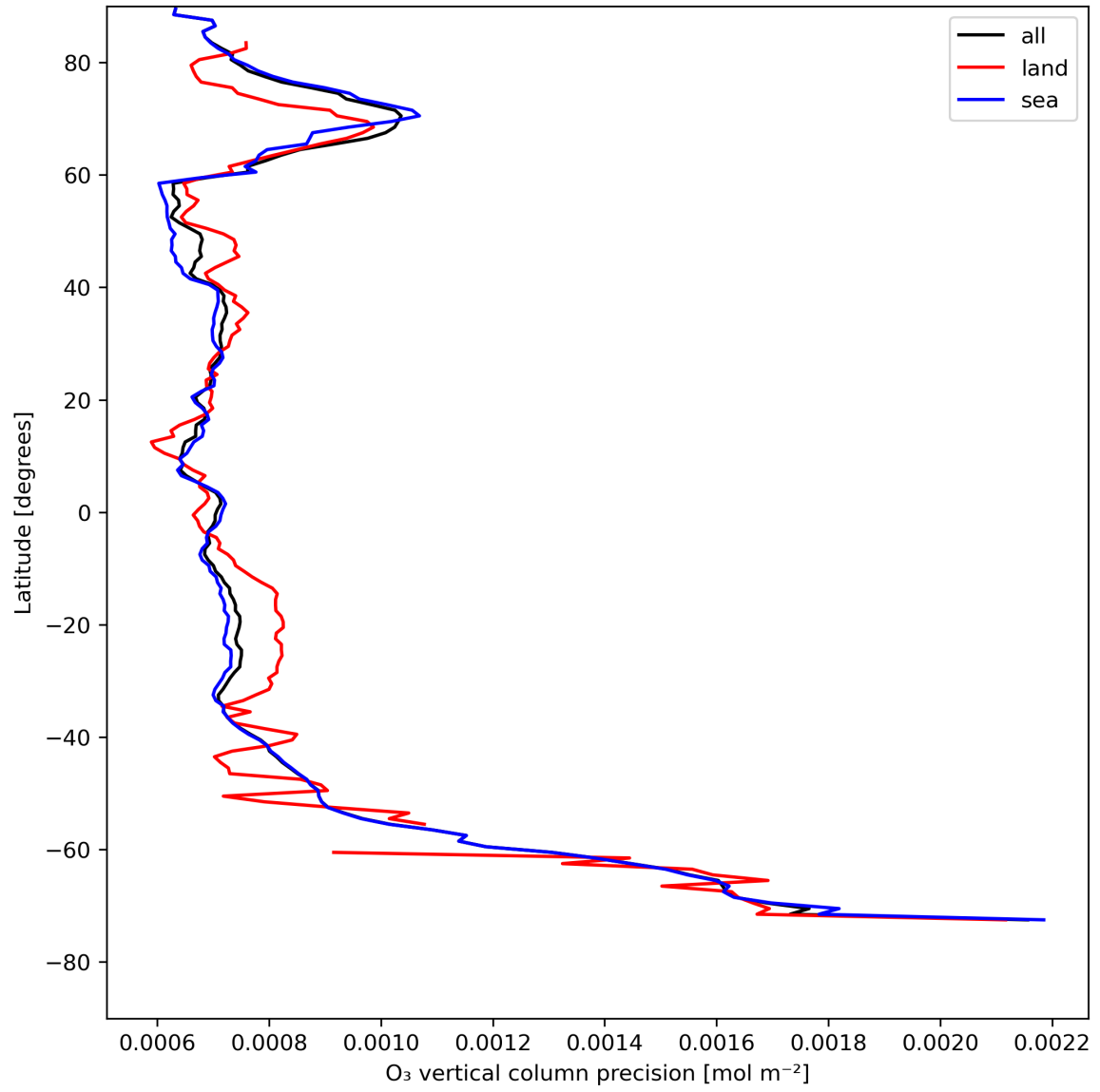
Figure 15: Zonal average of “O 3 vertical column precision” for 2024-08-06 to 2024-08-07.
