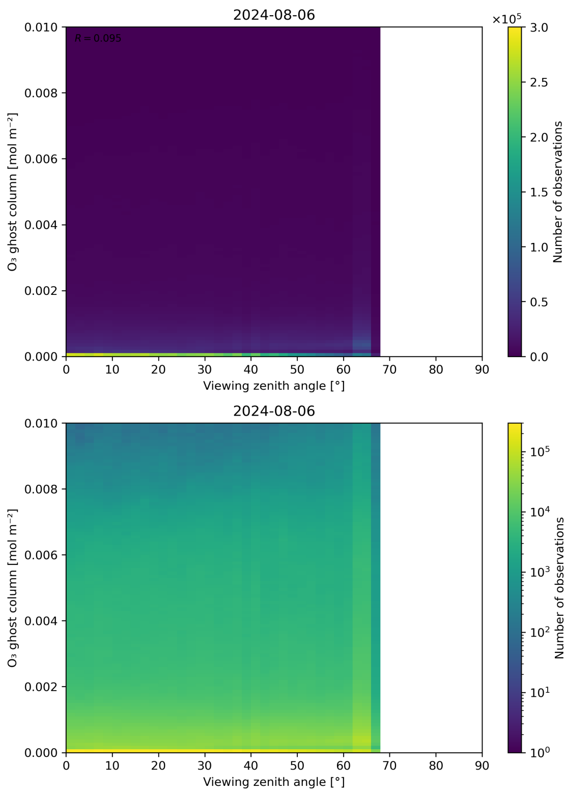
Figure 51: Scatter density plot of “Viewing zenith angle” against “O 3 ghost column” for 2024-08-06 to 2024-08-07.
