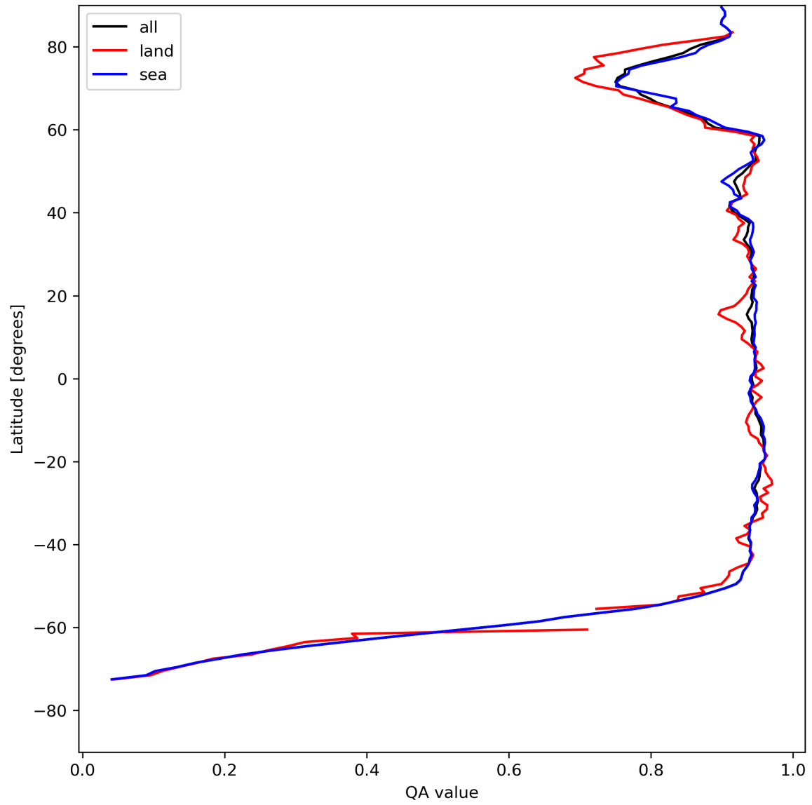
Figure 13: Zonal average of “QA value” for 2024-08-06 to 2024-08-07.
