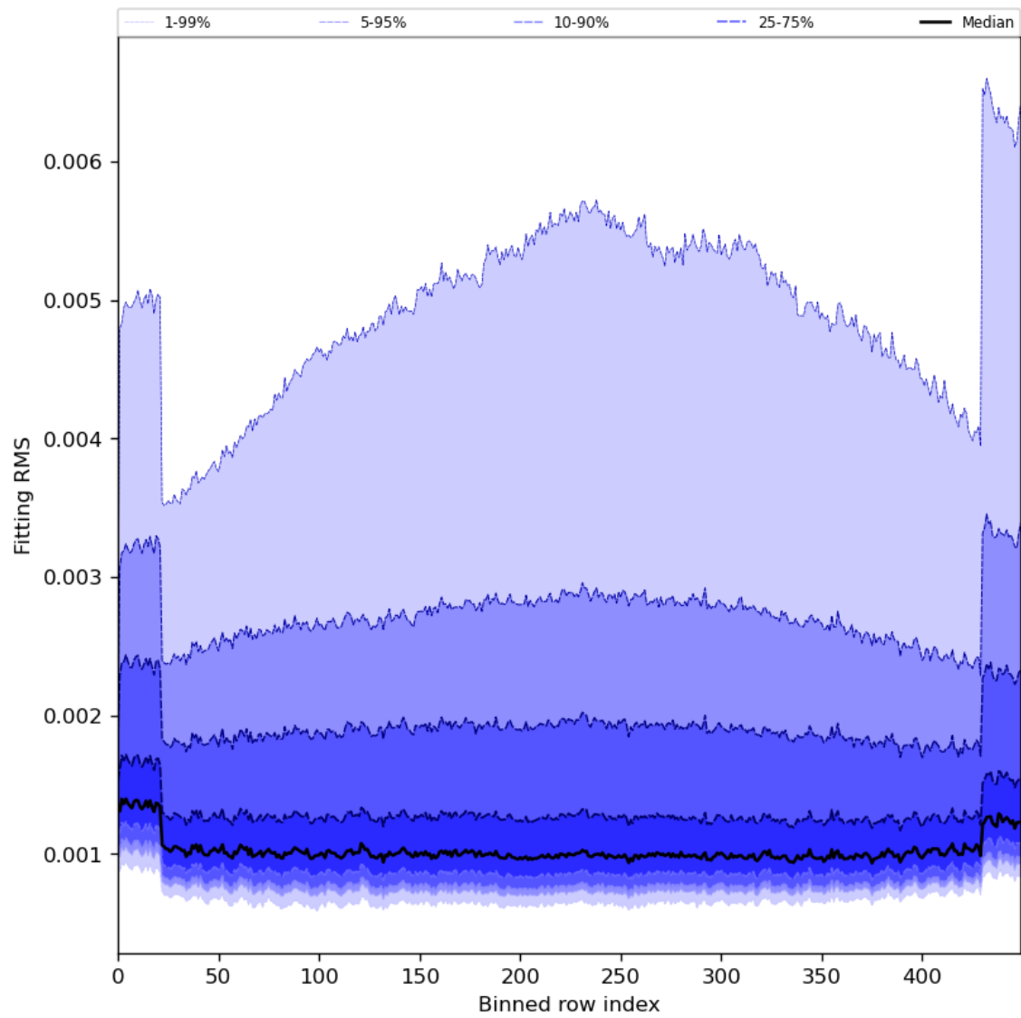
Figure 30: Along track statistics of “Fitting RMS” for 2024-08-06 to 2024-08-07
