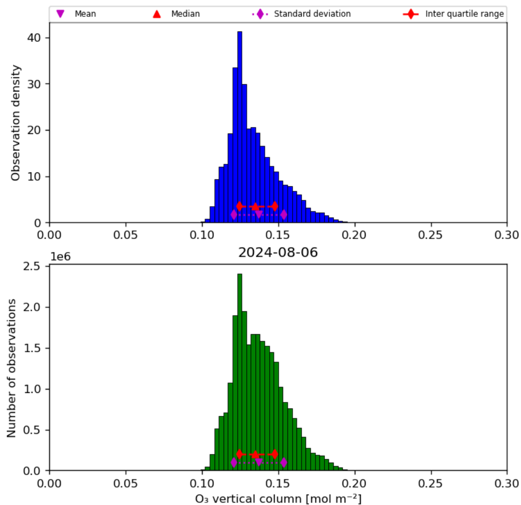
Figure 21: Histogram of “O 3 vertical column” for 2024-08-06 to 2024-08-07
