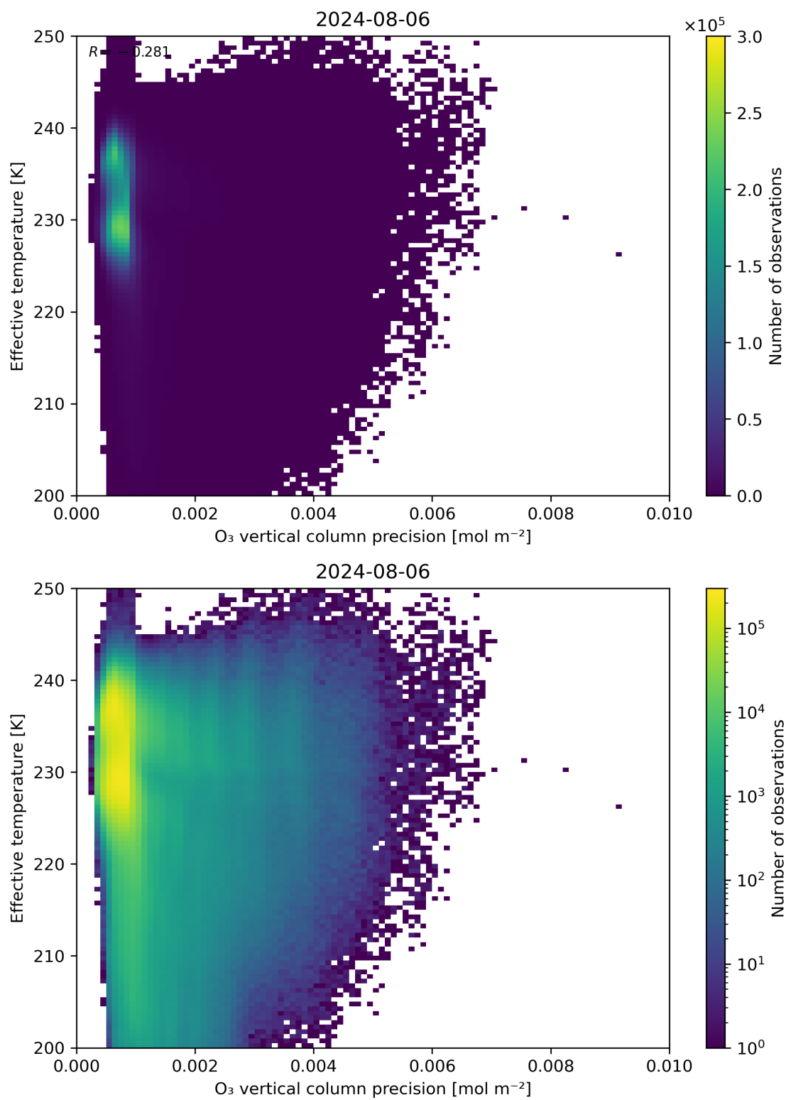
Figure 42: Scatter density plot of “O 3 vertical column precision” against “Effective temperature” for 2024-08-06 to 2024-08-07.
