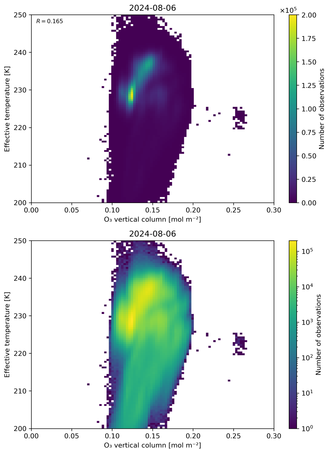
Figure 39: Scatter density plot of “O 3 vertical column” against “Effective temperature” for 2024-08-06 to 2024-08-07.
