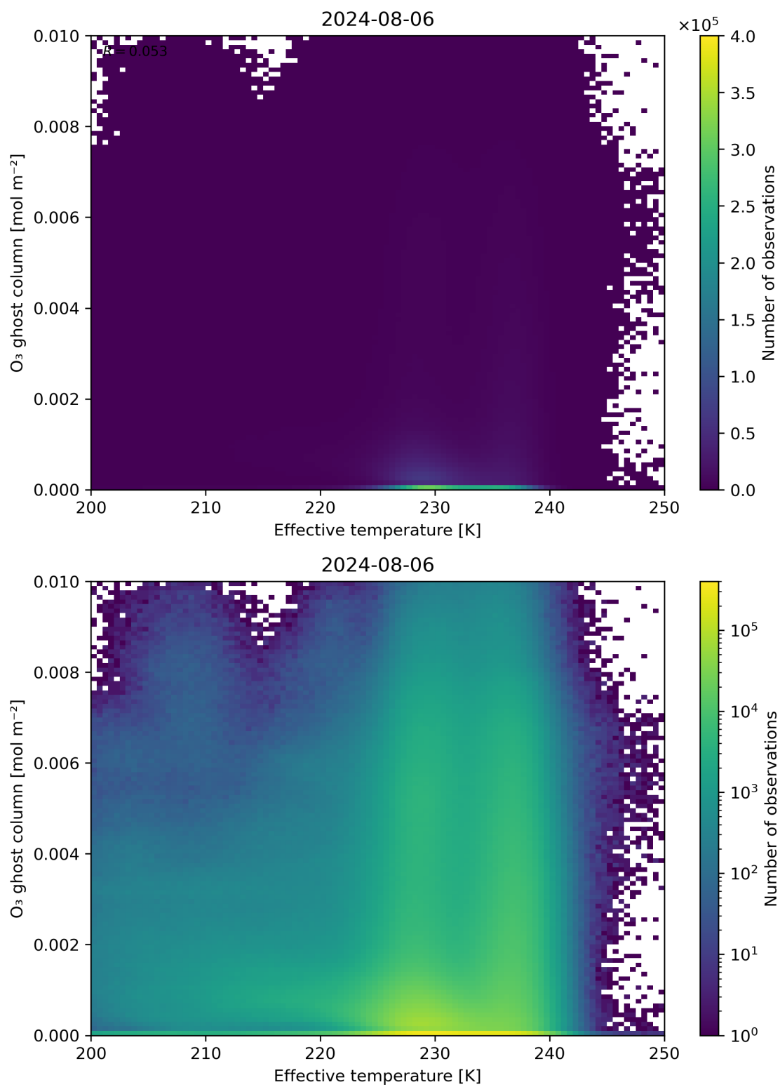
Figure 38: Scatter density plot of “Effective temperature” against “O 3 ghost column” for 2024-08-06 to 2024-08-07.
