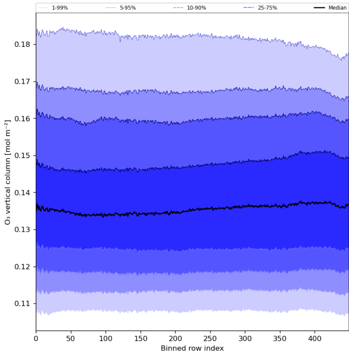
Figure 28: Along track statistics of “O 3 vertical column” for 2024-08-06 to 2024-08-07
