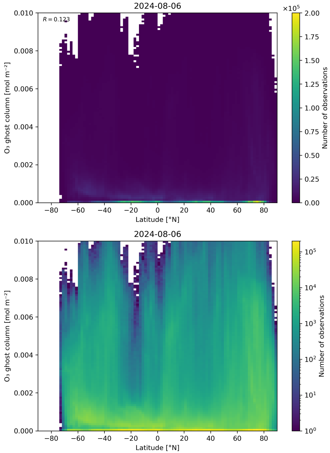
Figure 35: Scatter density plot of “Latitude” against “O 3 ghost column” for 2024-08-06 to 2024-08-07.
