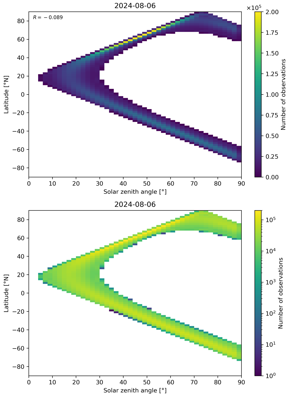
Figure 44: Scatter density plot of “Solar zenith angle” against “Latitude” for 2024-08-06 to 2024-08-07.
