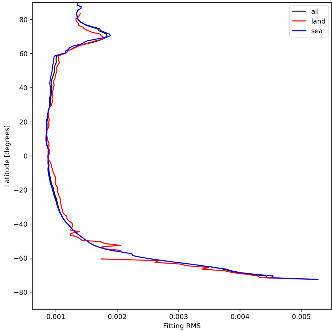
Figure 16: Zonal average of “Fitting RMS” for 2024-08-06 to 2024-08-07.
