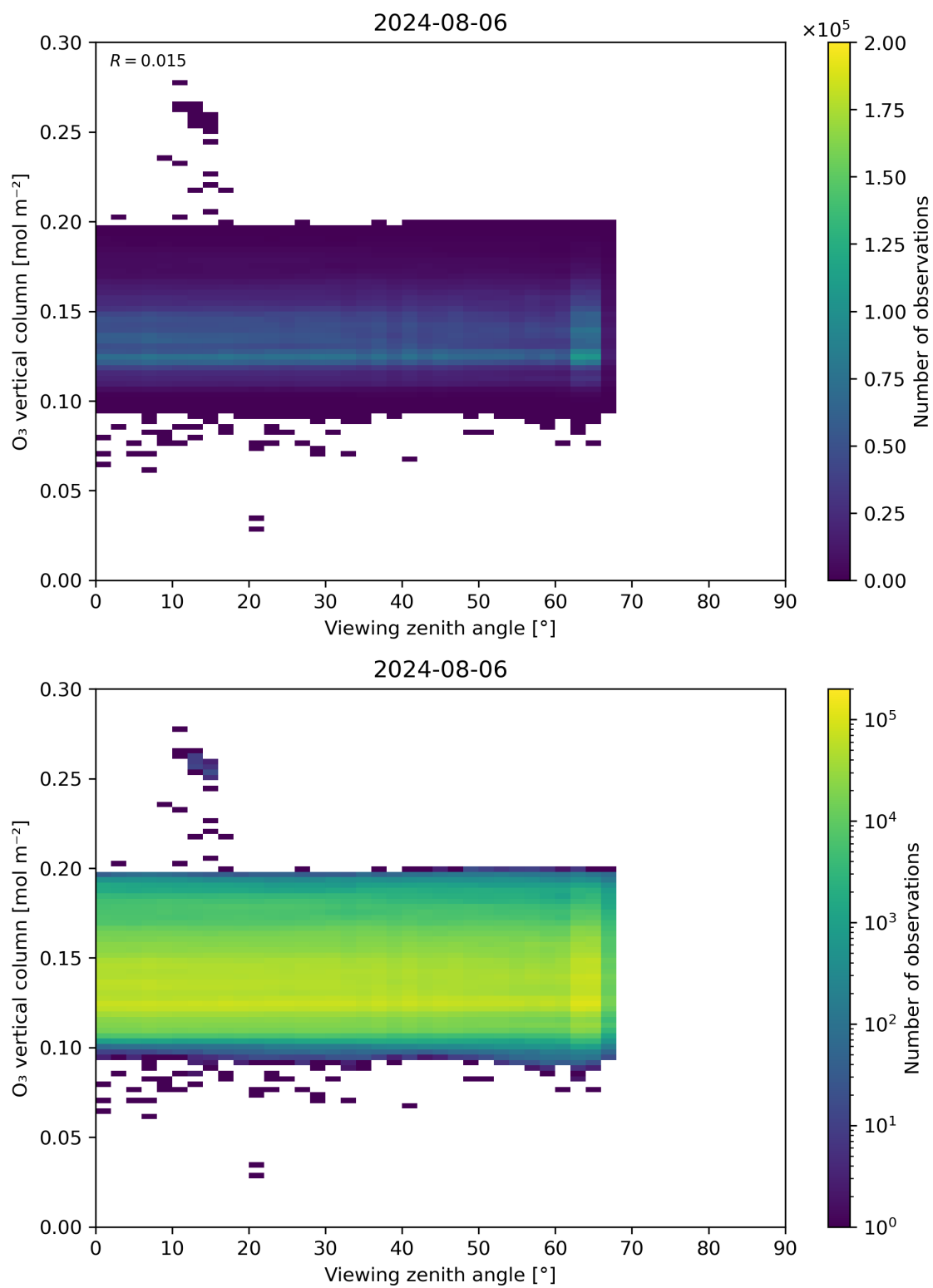
Figure 52: Scatter density plot of “Viewing zenith angle” against “O 3 vertical column” for 2024-08-06 to 2024-08-07.
