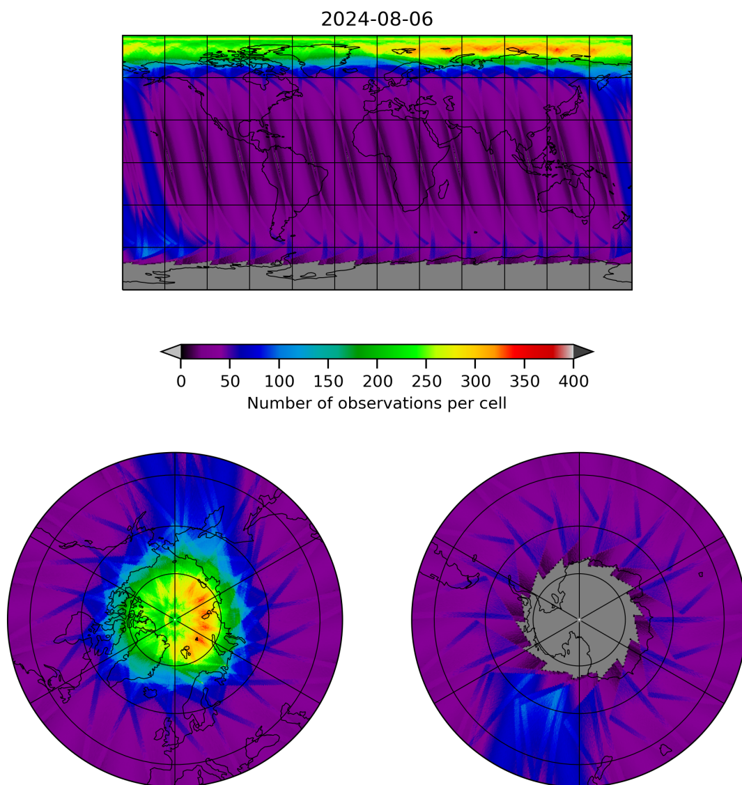
Figure 12: Map of the number of observations for 2024-08-06 to 2024-08-07
