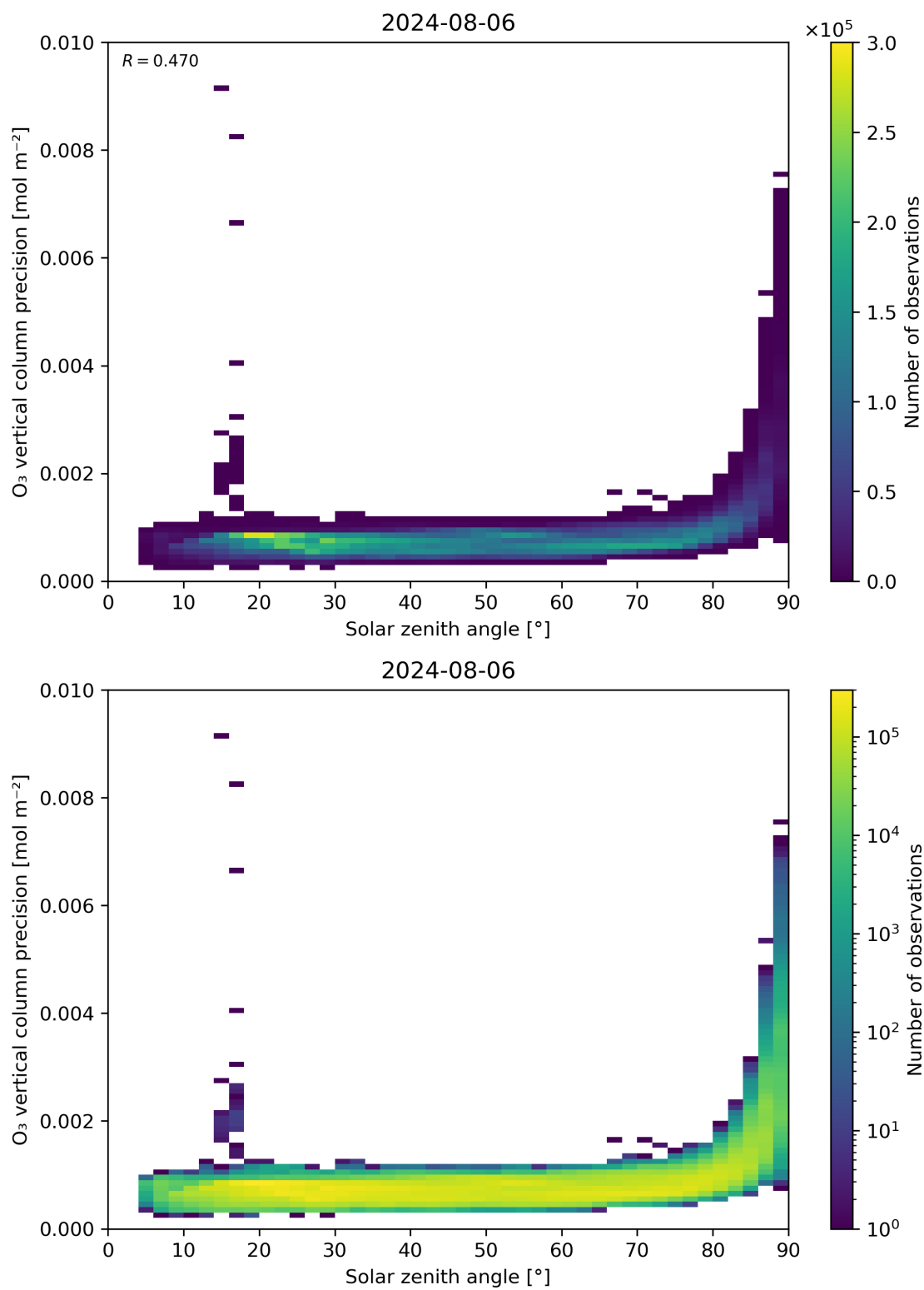
Figure 48: Scatter density plot of “Solar zenith angle” against “O 3 vertical column precision” for 2024-08-06 to 2024-08-07.
