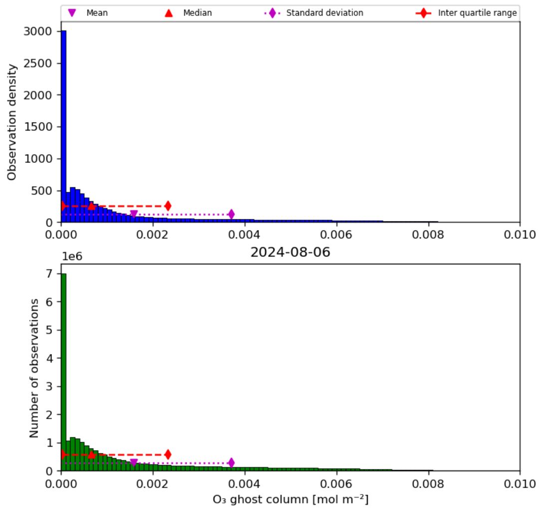
Figure 25: Histogram of “O 3 ghost column” for 2024-08-06 to 2024-08-07
