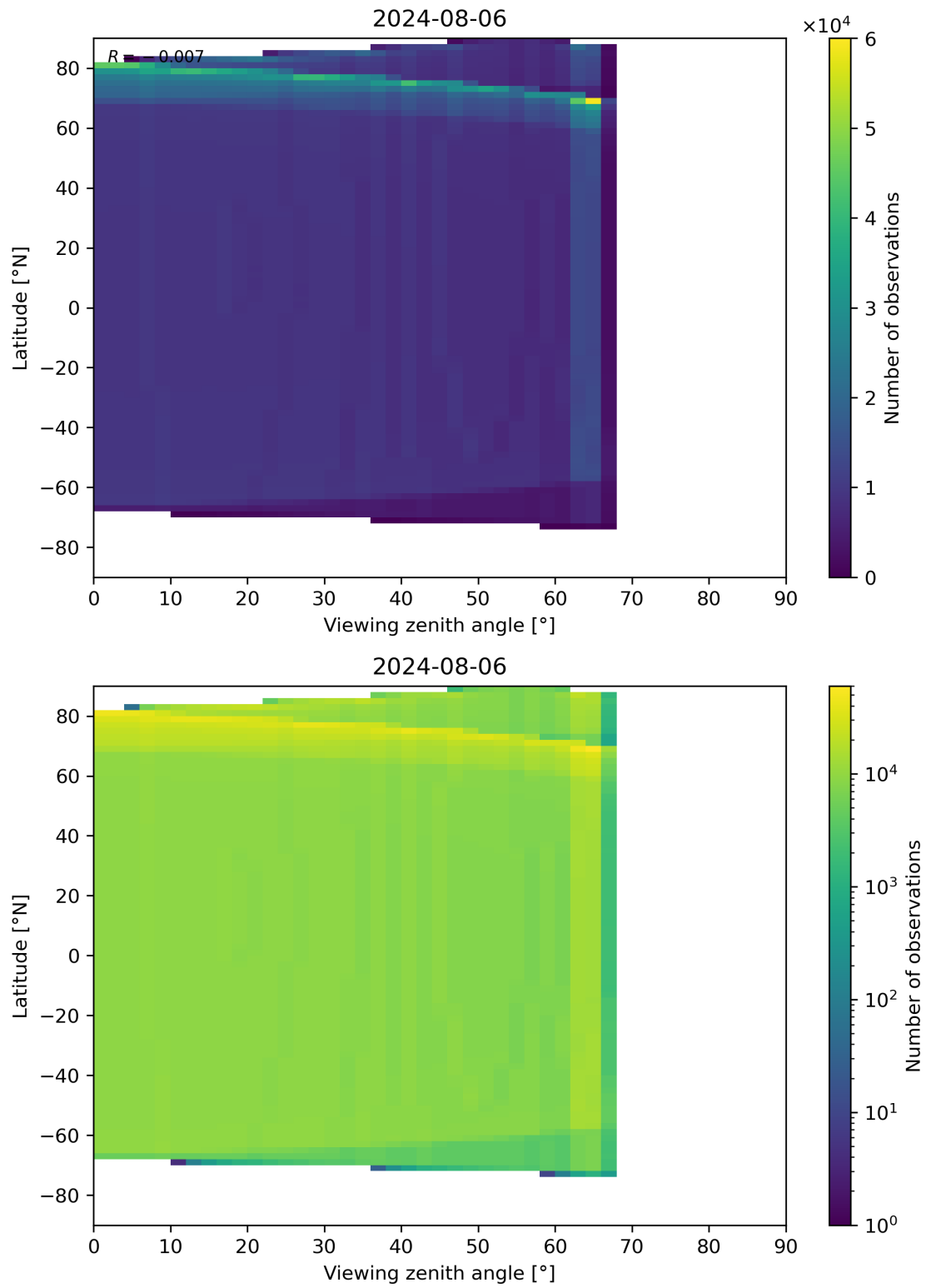
Figure 49: Scatter density plot of “Viewing zenith angle” against “Latitude” for 2024-08-06 to 2024-08-07.
