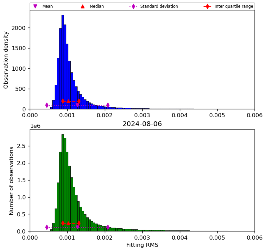
Figure 23: Histogram of “Fitting RMS” for 2024-08-06 to 2024-08-07
