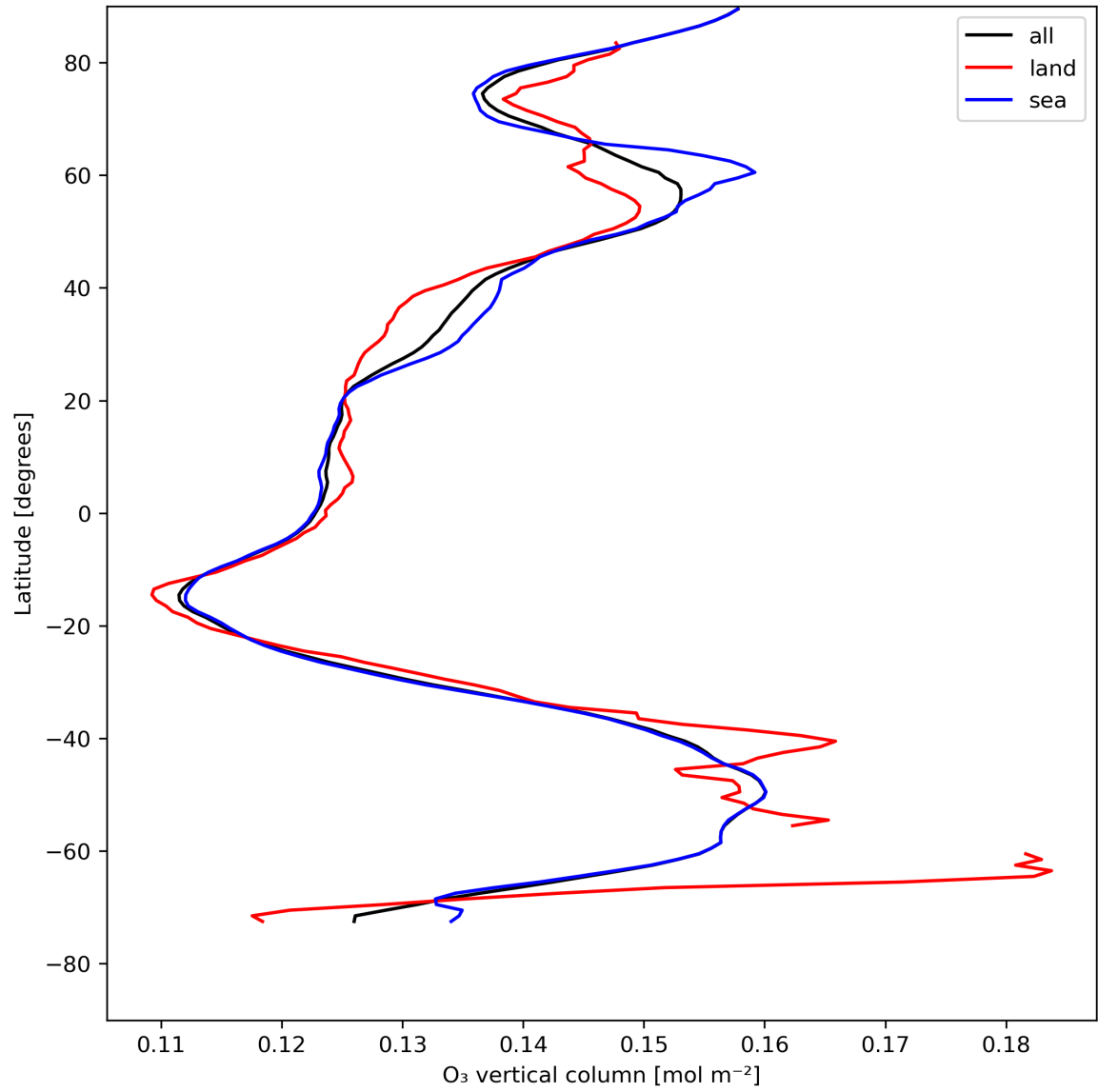
Figure 14: Zonal average of “O 3 vertical column” for 2024-08-06 to 2024-08-07.
