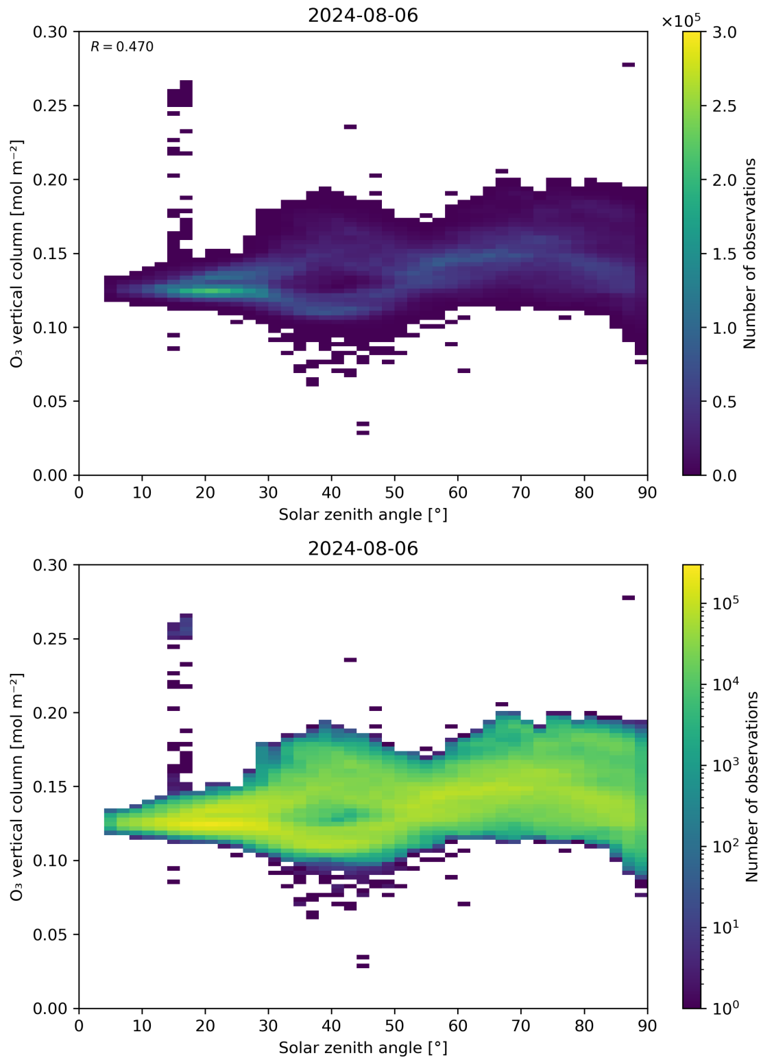
Figure 47: Scatter density plot of “Solar zenith angle” against “O 3 vertical column” for 2024-08-06 to 2024-08-07.
