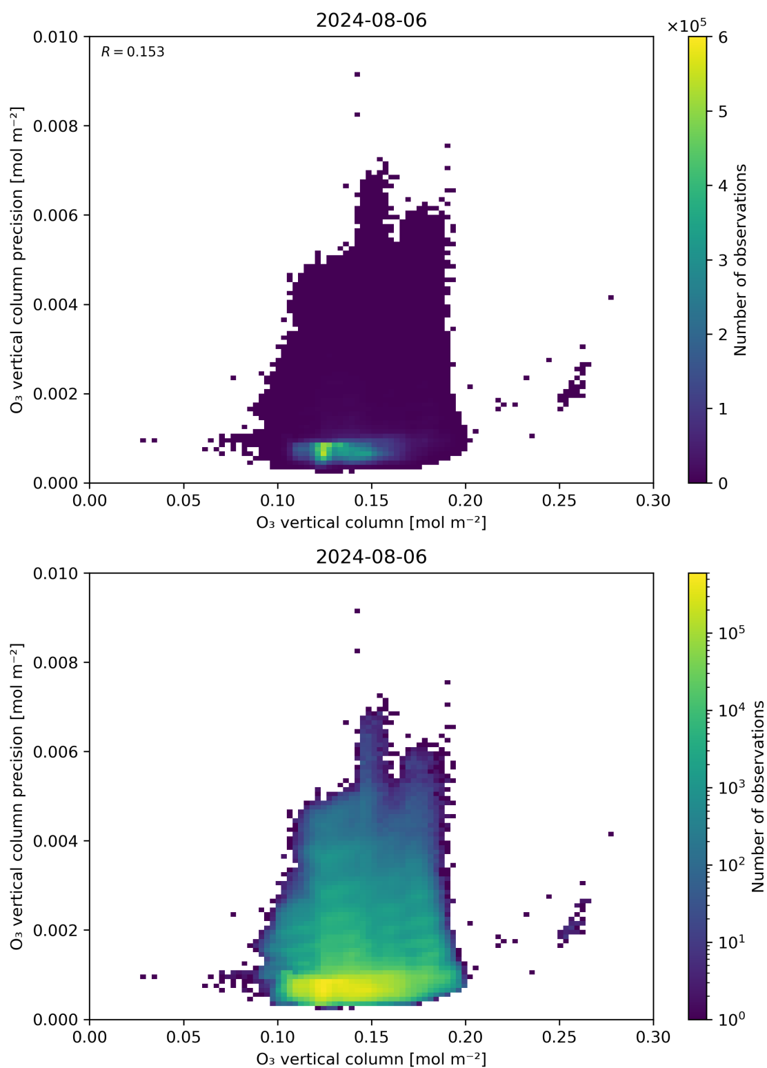
Figure 41: Scatter density plot of “O 3 vertical column” against “O 3 vertical column precision” for 2024-08-06 to 2024-08-07.
