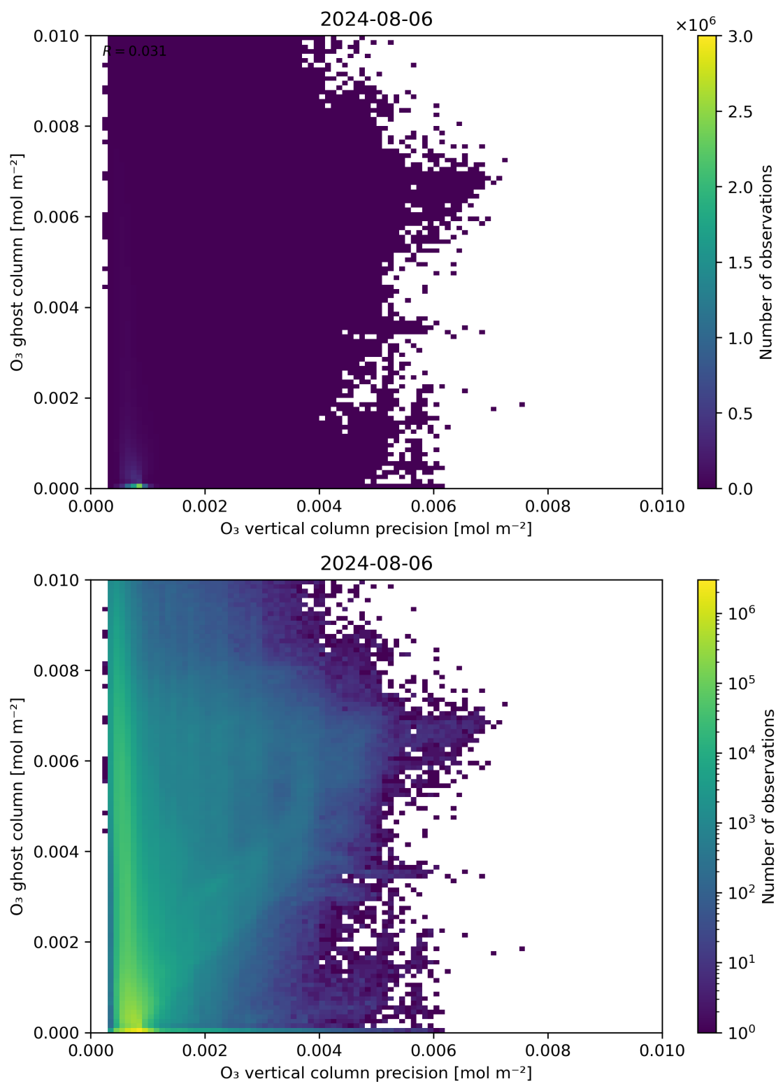
Figure 43: Scatter density plot of “ \text{O}_3 vertical column precision” against “ \text{O}_3 ghost column” for 2024-08-06 to 2024-08-07.
