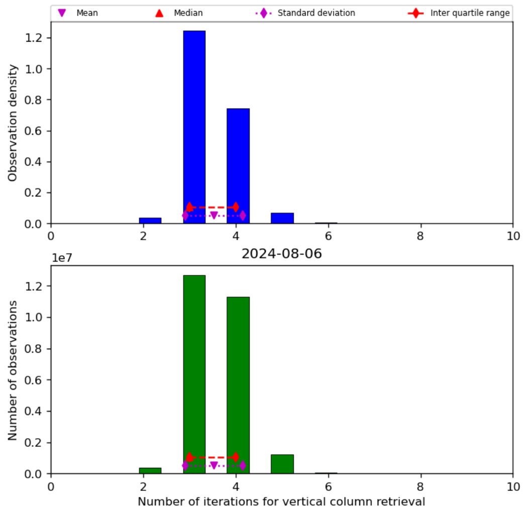
Figure 26: Histogram of “Number of iterations for vertical column retrieval” for 2024-08-06 to 2024-08-07
