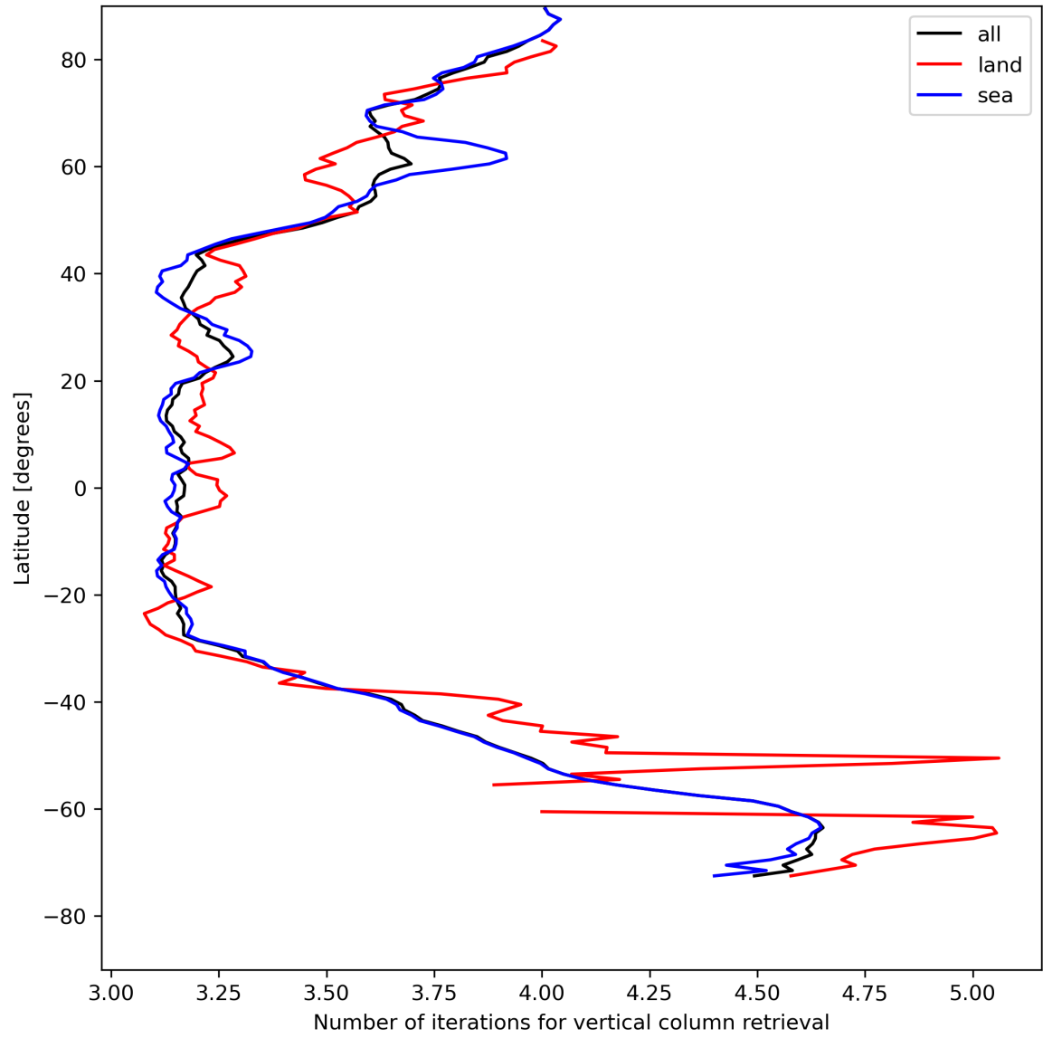
Figure 19: Zonal average of “Number of iterations for vertical column retrieval” for 2024-08-06 to 2024-08-07.
