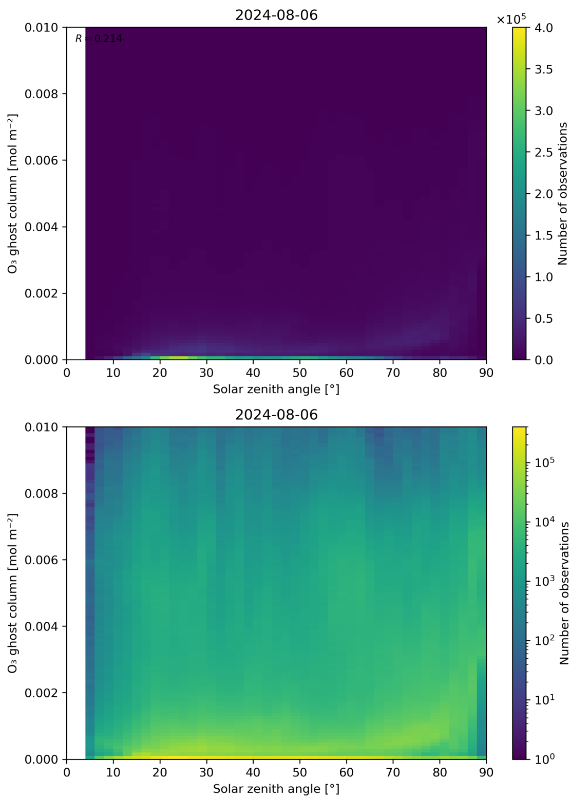
Figure 46: Scatter density plot of “Solar zenith angle” against “O 3 ghost column” for 2024-08-06 to 2024-08-07.
