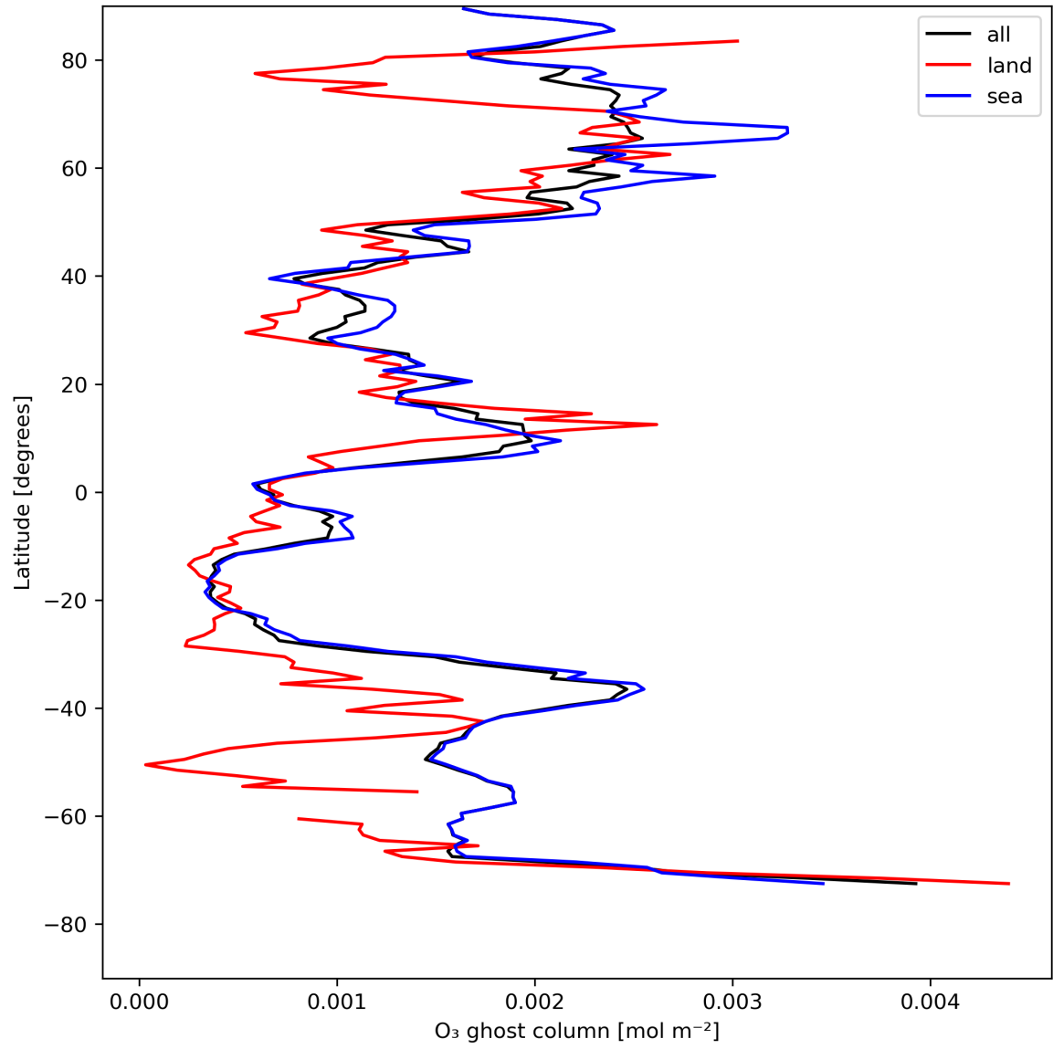
Figure 18: Zonal average of "O 3 ghost column" for 2024-08-06 to 2024-08-07.
