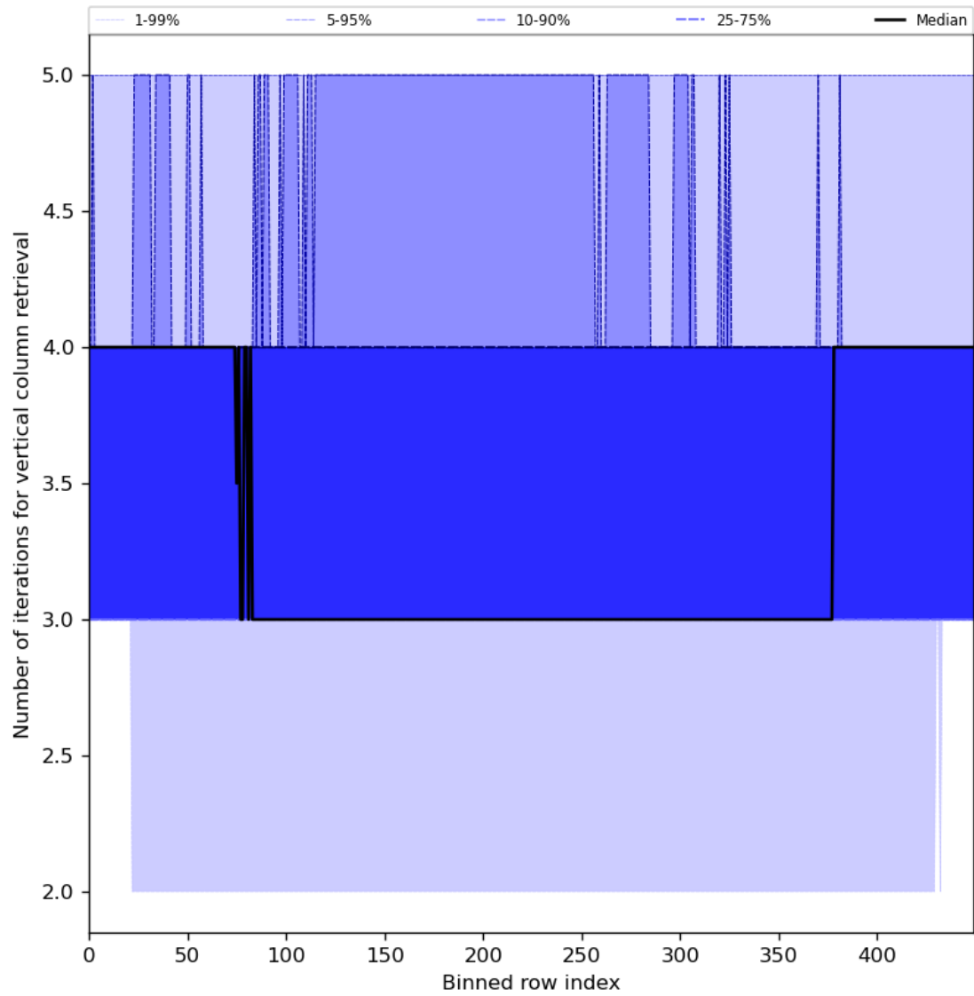
Figure 33: Along track statistics of “Number of iterations for vertical column retrieval” for 2024-08-06 to 2024-08-07
