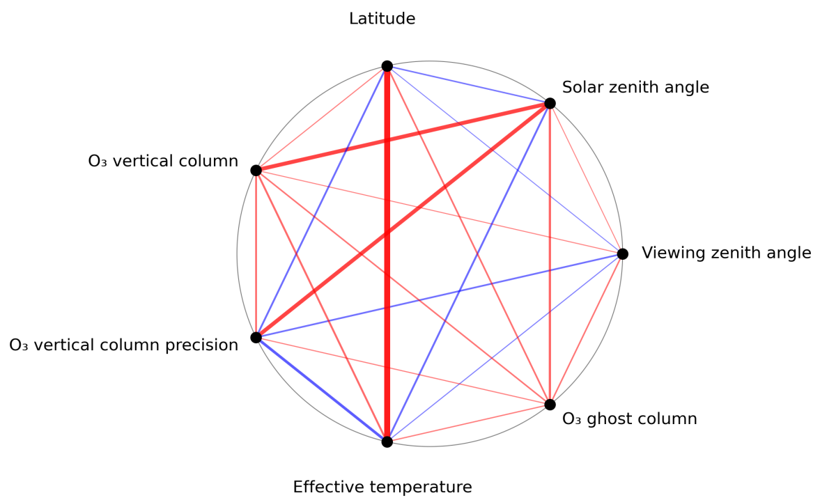
Figure 1: Map of correlation graph for 2024-08-06 to 2024-08-07.
