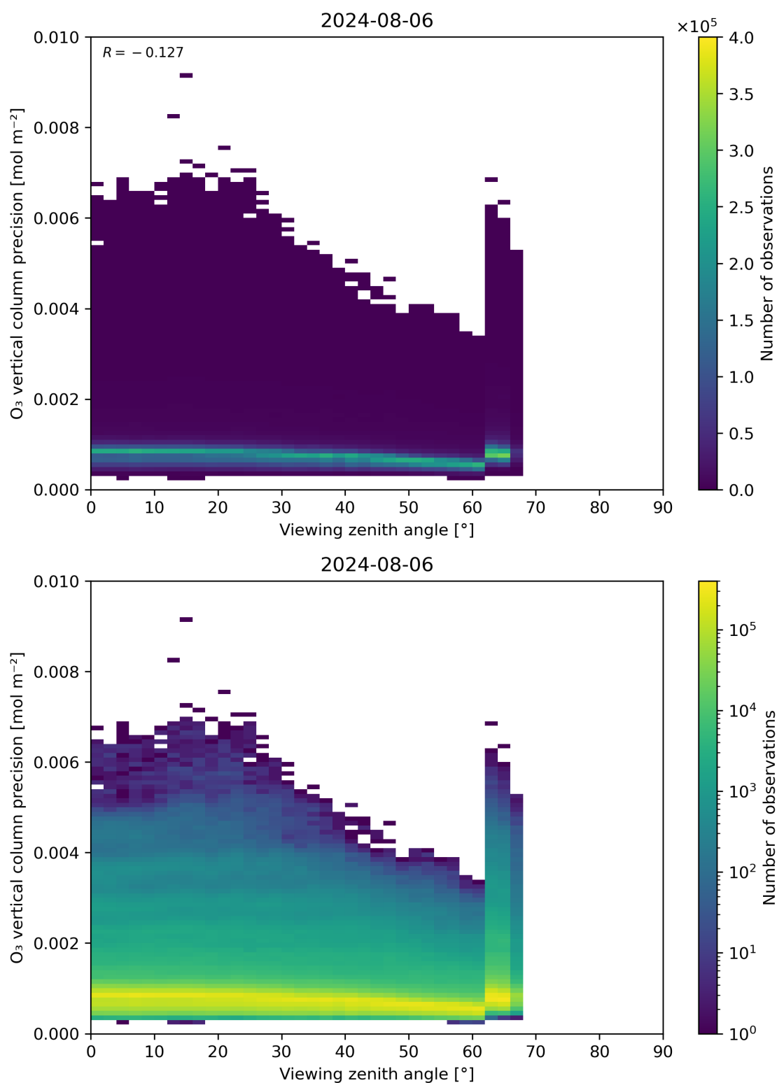
Figure 53: Scatter density plot of “Viewing zenith angle” against “O 3 vertical column precision” for 2024-08-06 to 2024-08-07.
