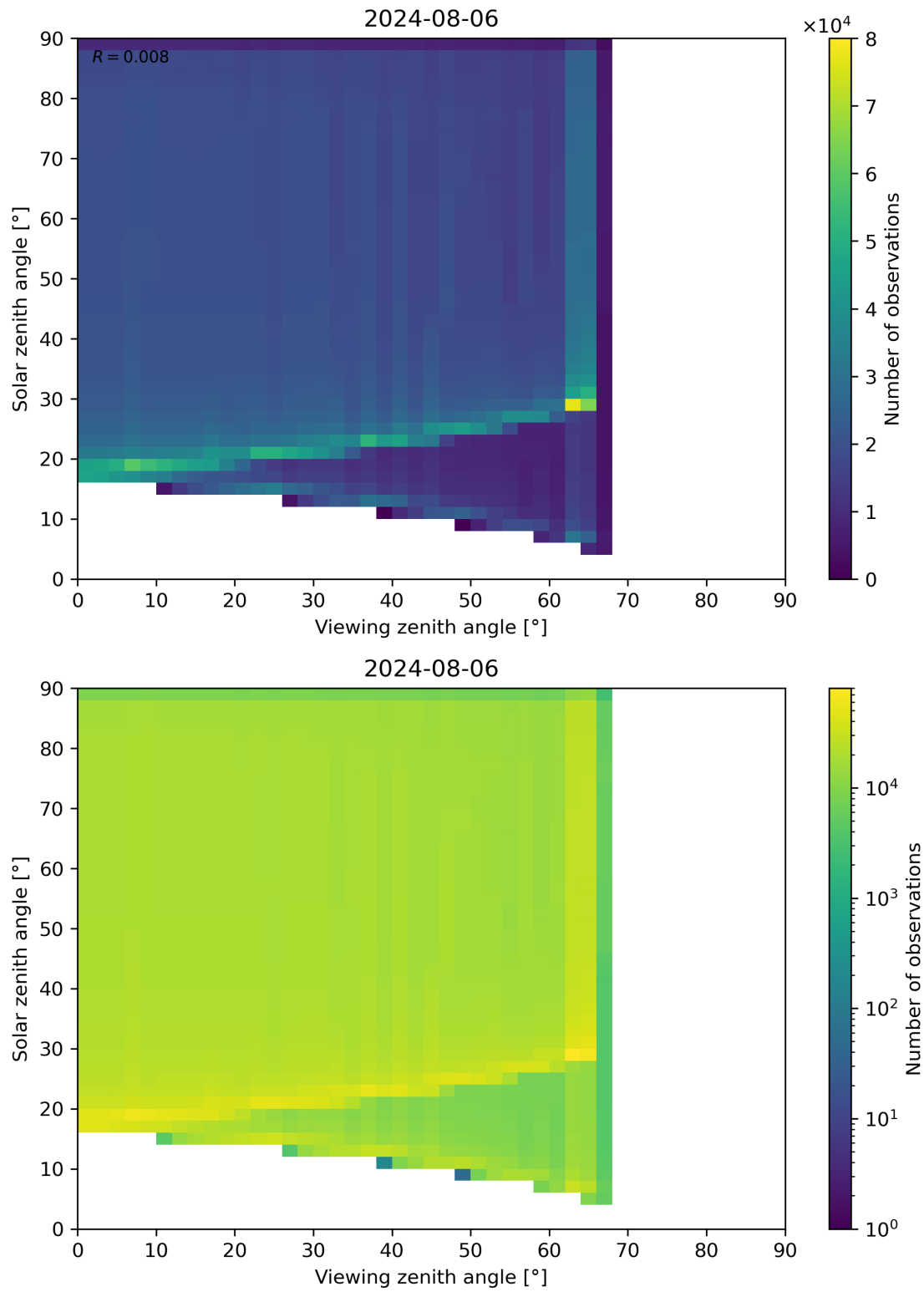
Figure 54: Scatter density plot of “Viewing zenith angle” against “Solar zenith angle” for 2024-08-06 to 2024-08-07.
