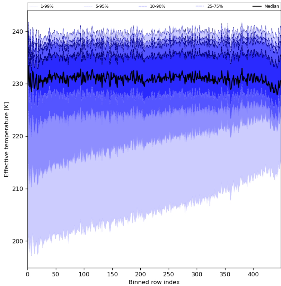
Figure 31: Along track statistics of “Effective temperature” for 2024-08-06 to 2024-08-07
