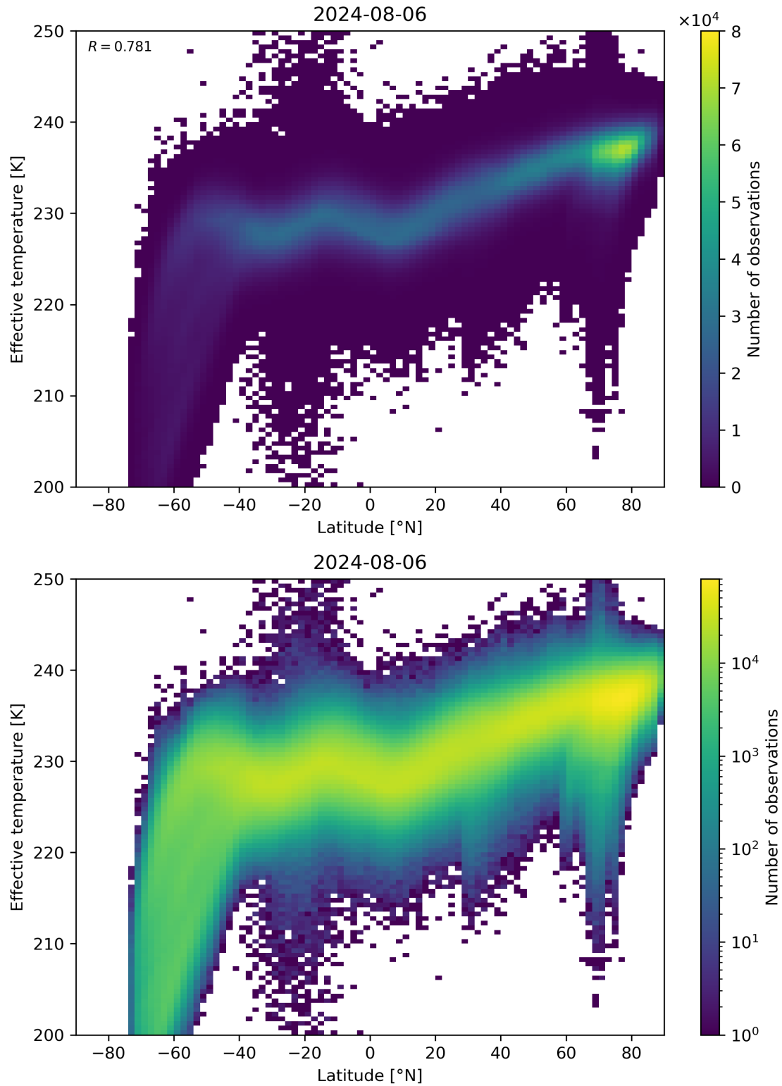
Figure 34: Scatter density plot of “Latitude” against “Effective temperature” for 2024-08-06 to 2024-08-07.
