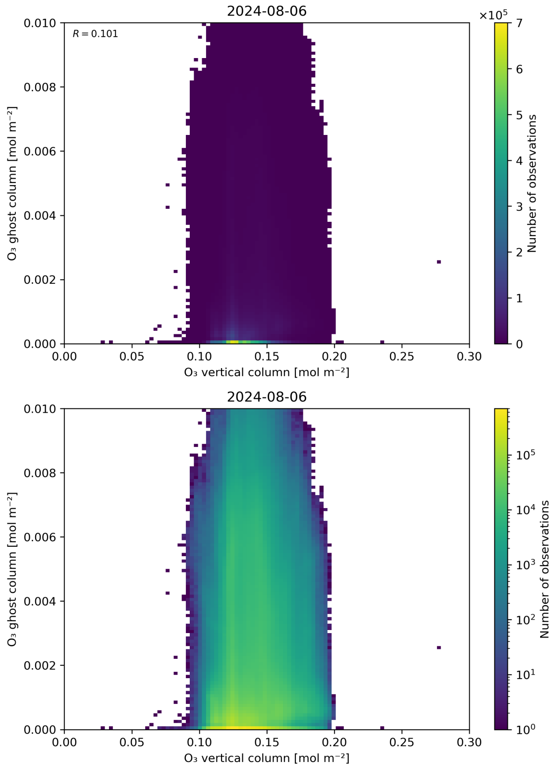
Figure 40: Scatter density plot of “O 3 vertical column” against “O 3 ghost column” for 2024-08-06 to 2024-08-07.
