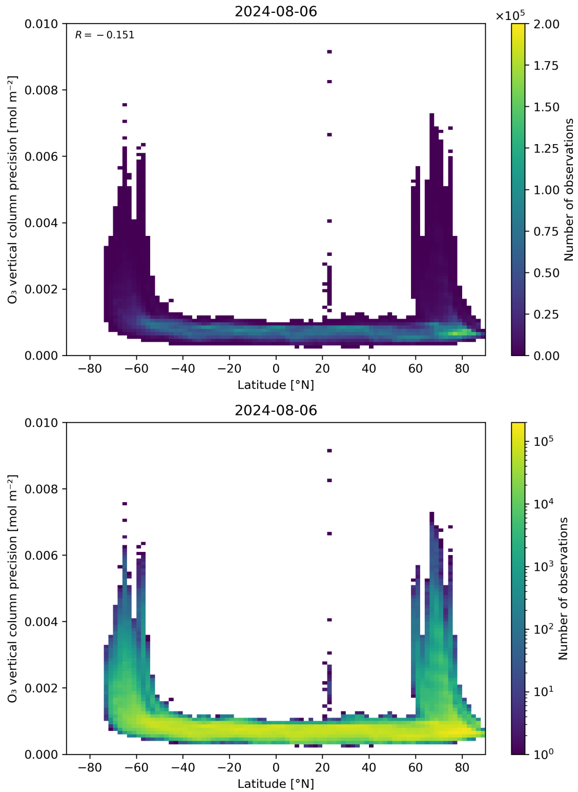
Figure 37: Scatter density plot of “Latitude” against “O 3 vertical column precision” for 2024-08-06 to 2024-08-07.
