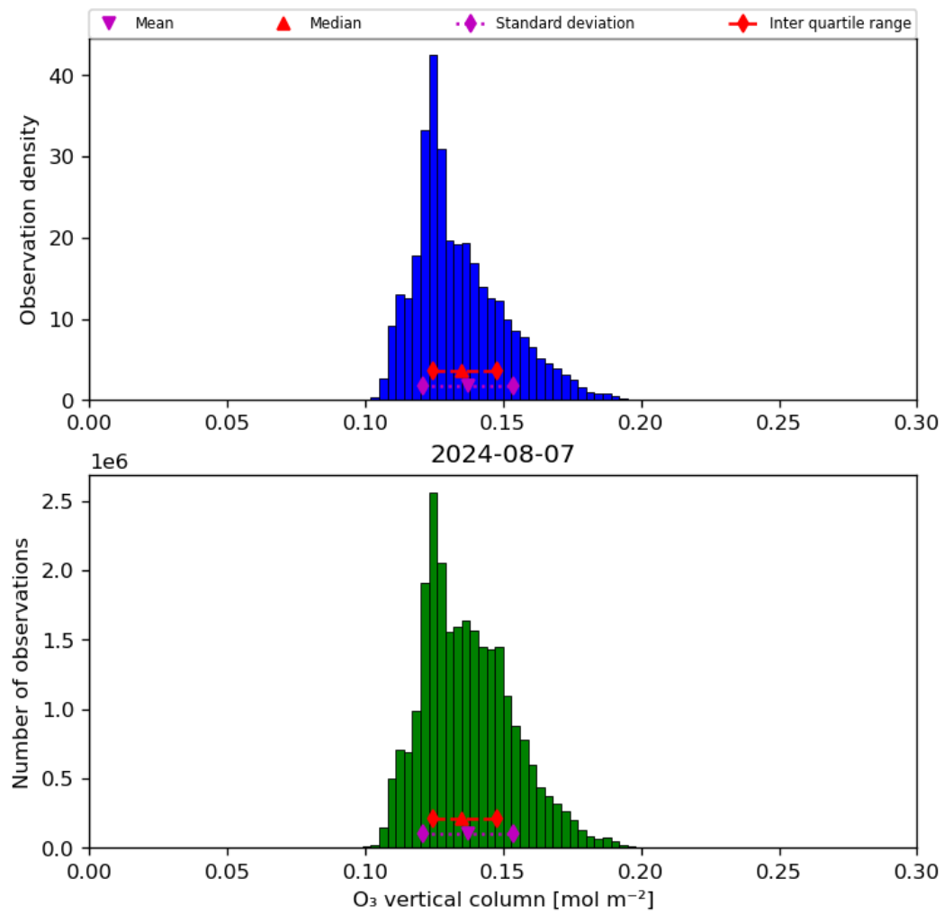
Figure 21: Histogram of “O 3 vertical column” for 2024-08-06 to 2024-08-08
