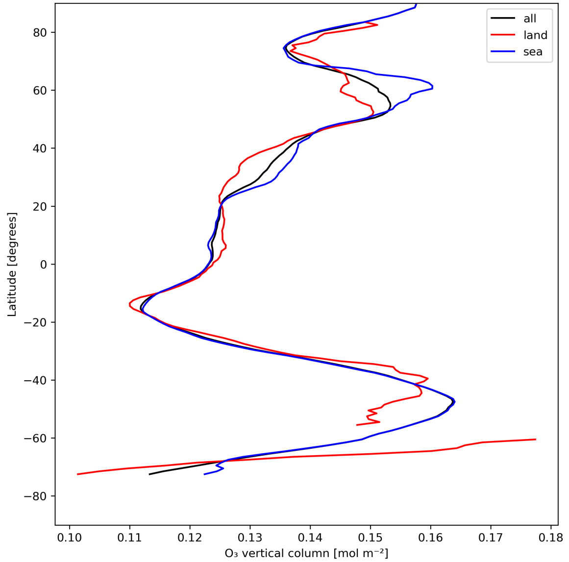
Figure 14: Zonal average of “O 3 vertical column” for 2024-08-06 to 2024-08-08.
