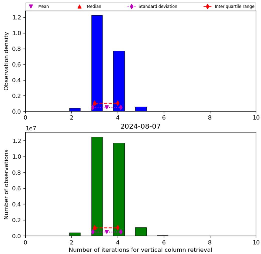
Figure 26: Histogram of “Number of iterations for vertical column retrieval” for 2024-08-06 to 2024-08-08
