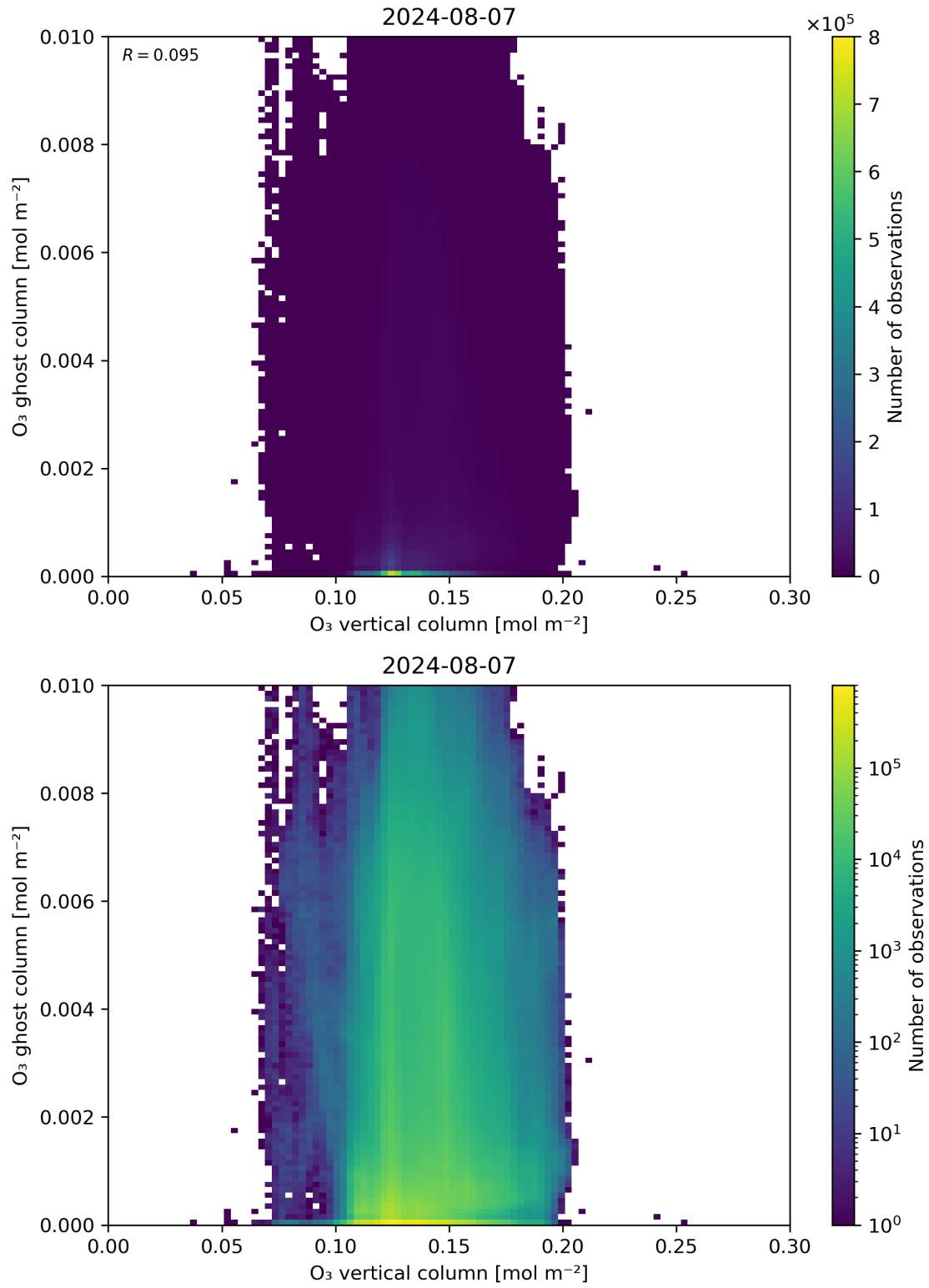
Figure 40: Scatter density plot of “O 3 vertical column” against “O 3 ghost column” for 2024-08-06 to 2024-08-08.
