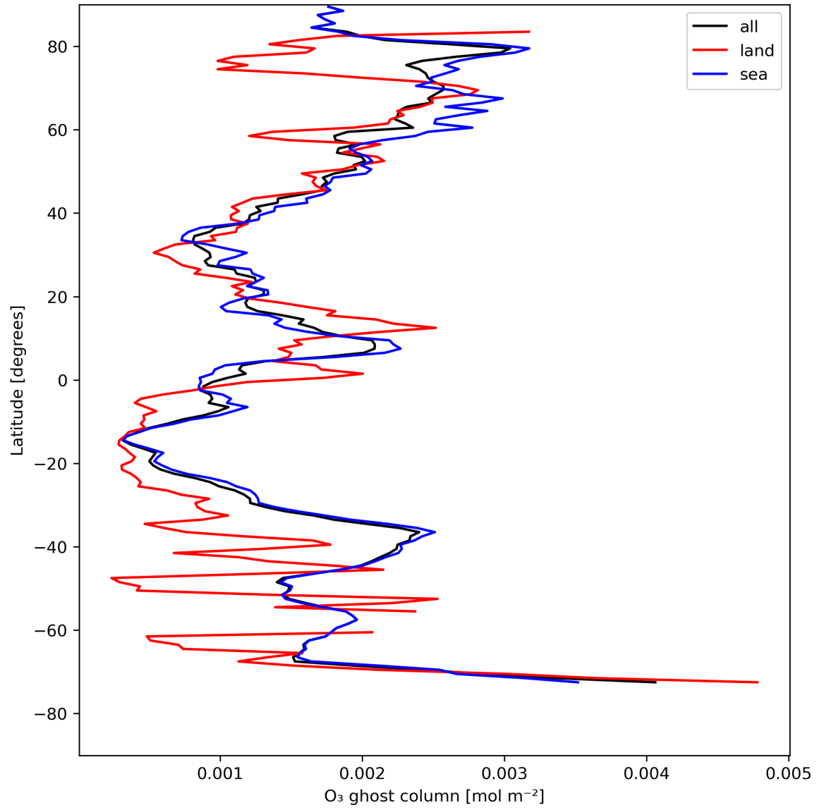
Figure 18: Zonal average of “O 3 ghost column” for 2024-08-06 to 2024-08-08.
