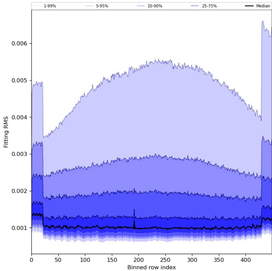
Figure 30: Along track statistics of “Fitting RMS” for 2024-08-06 to 2024-08-08
