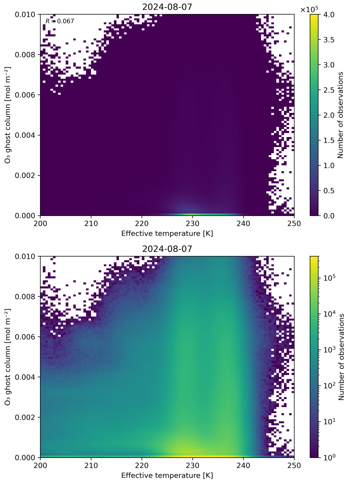
Figure 38: Scatter density plot of “Effective temperature” against “O 3 ghost column” for 2024-08-06 to 2024-08-08.
