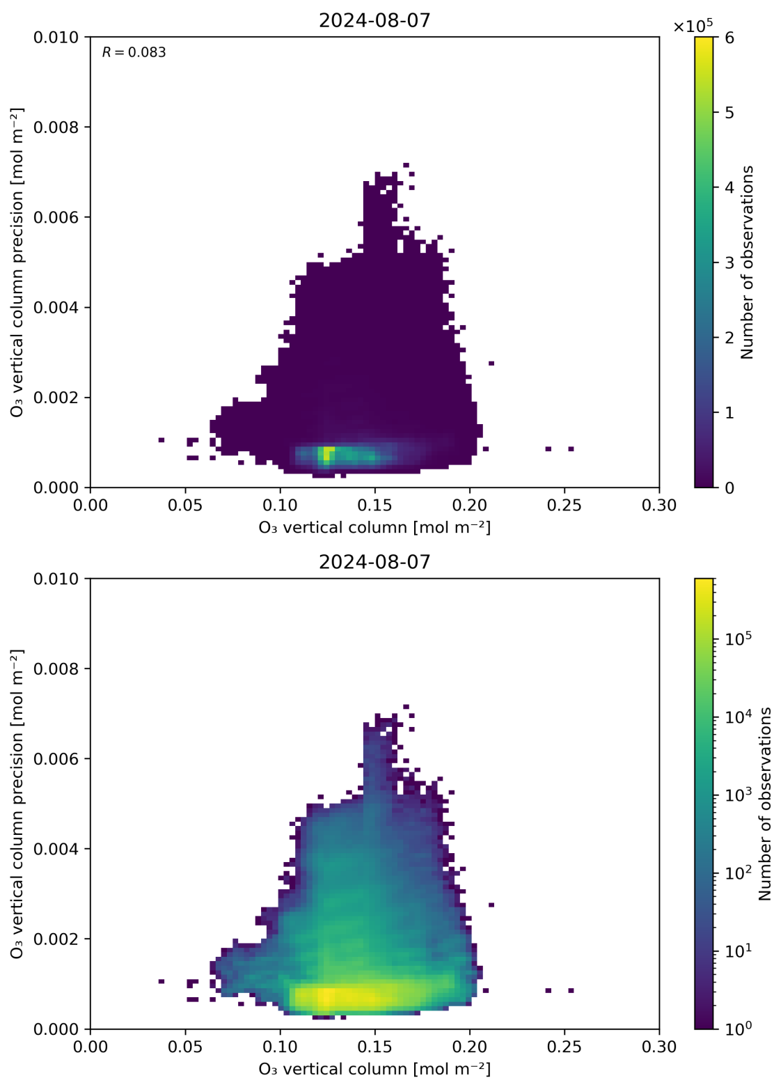
Figure 41: Scatter density plot of “O 3 vertical column” against “O 3 vertical column precision” for 2024-08-06 to 2024-08-08.
