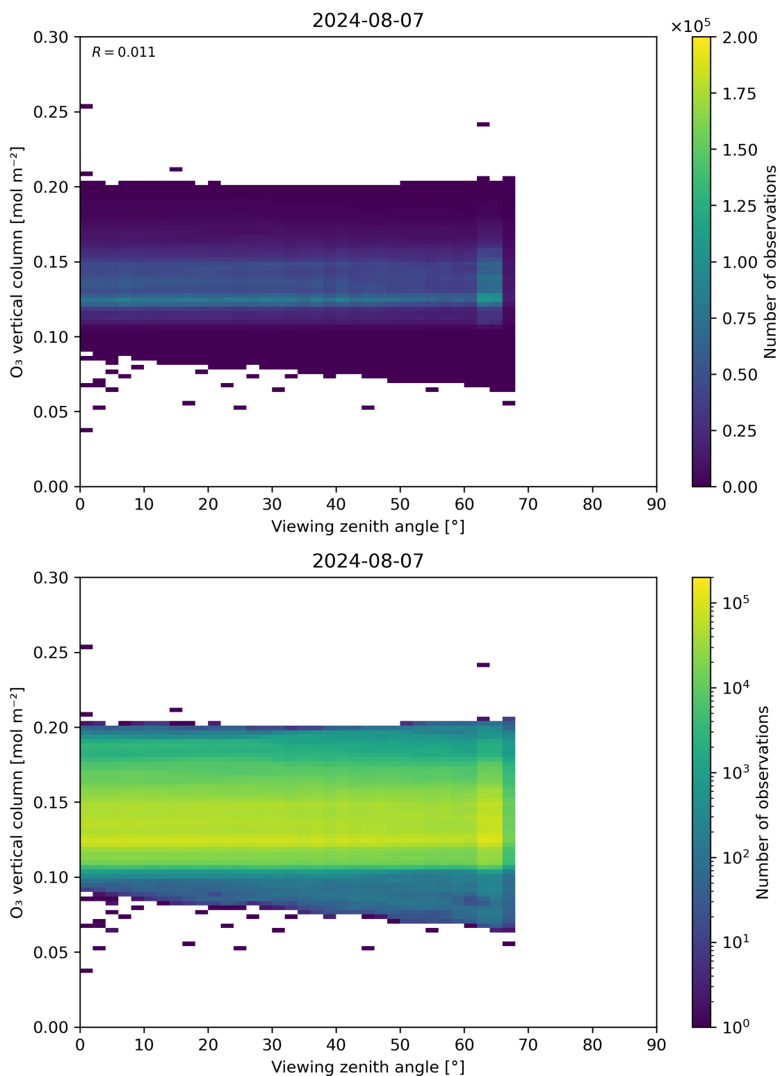
Figure 52: Scatter density plot of “Viewing zenith angle” against “O 3 vertical column” for 2024-08-06 to 2024-08-08.
