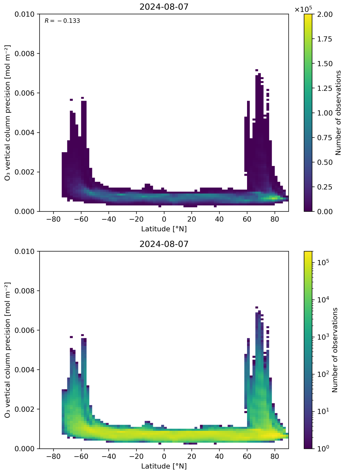
Figure 37: Scatter density plot of “Latitude” against “O 3 vertical column precision” for 2024-08-06 to 2024-08-08.
