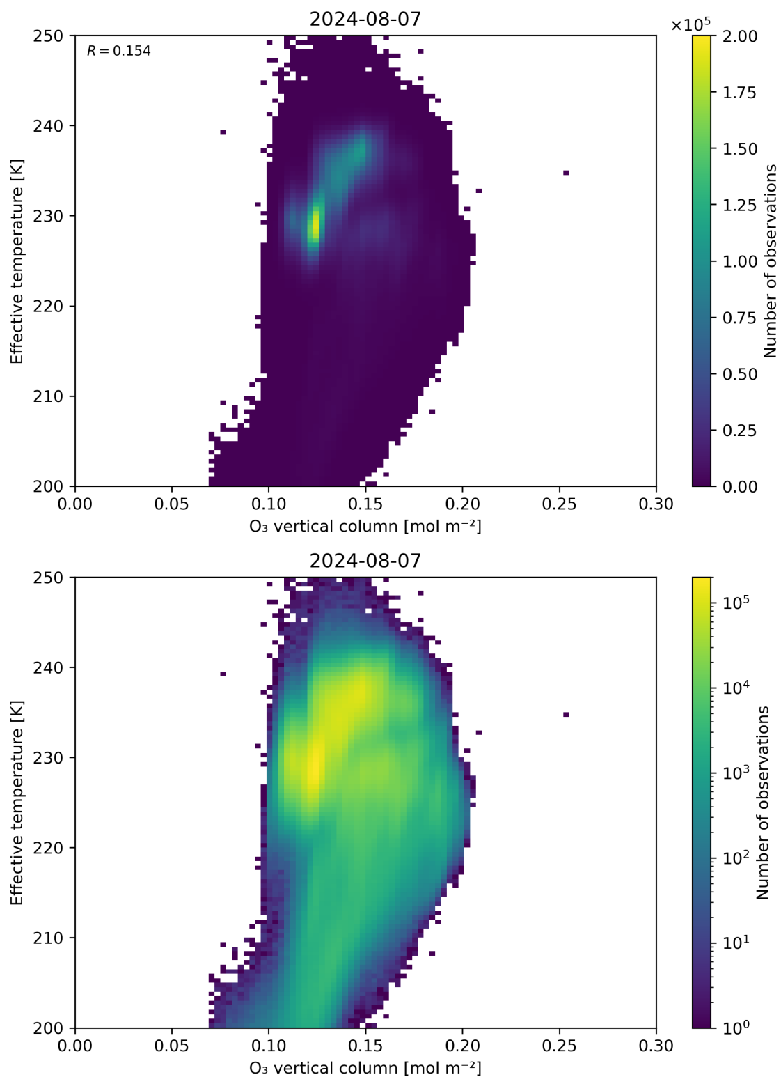
Figure 39: Scatter density plot of “O 3 vertical column” against “Effective temperature” for 2024-08-06 to 2024-08-08.
