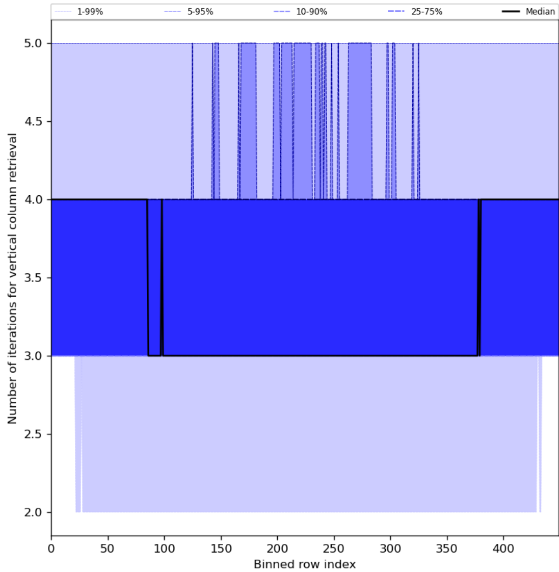
Figure 33: Along track statistics of “Number of iterations for vertical column retrieval” for 2024-08-06 to 2024-08-08
