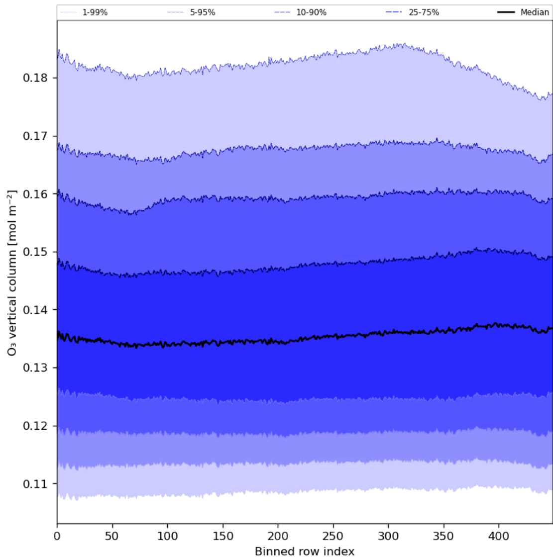
Figure 28: Along track statistics of “O 3 vertical column” for 2024-08-06 to 2024-08-08
