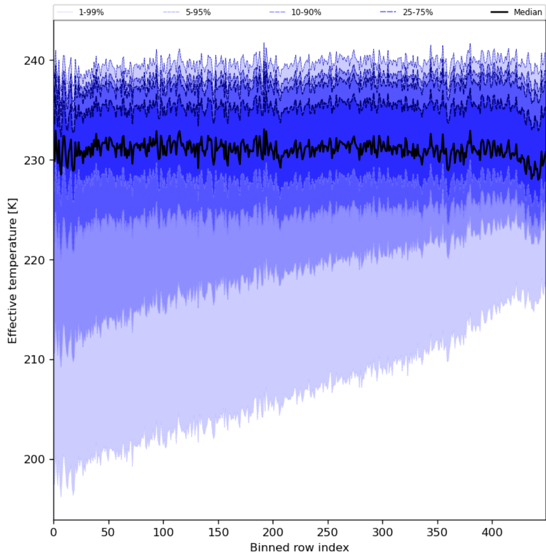
Figure 31: Along track statistics of “Effective temperature” for 2024-08-06 to 2024-08-08
