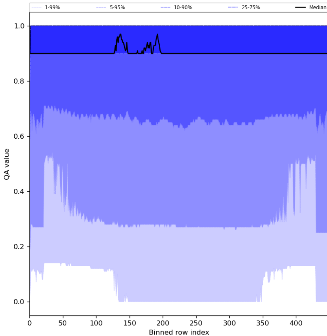
Figure 27: Along track statistics of “QA value” for 2024-08-06 to 2024-08-08
