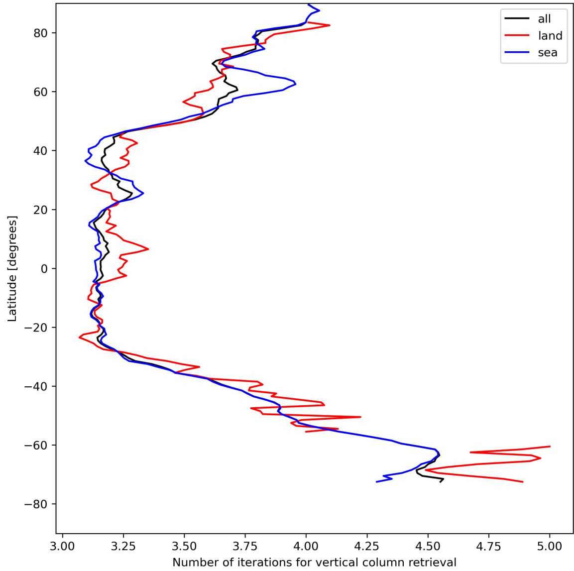
Figure 19: Zonal average of “Number of iterations for vertical column retrieval” for 2024-08-06 to 2024-08-08.
