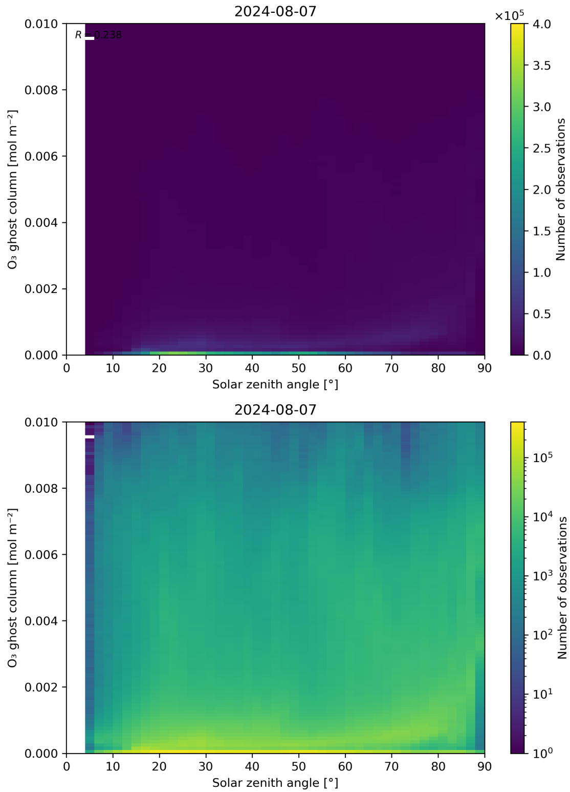
Figure 46: Scatter density plot of “Solar zenith angle” against “O 3 ghost column” for 2024-08-06 to 2024-08-08.
