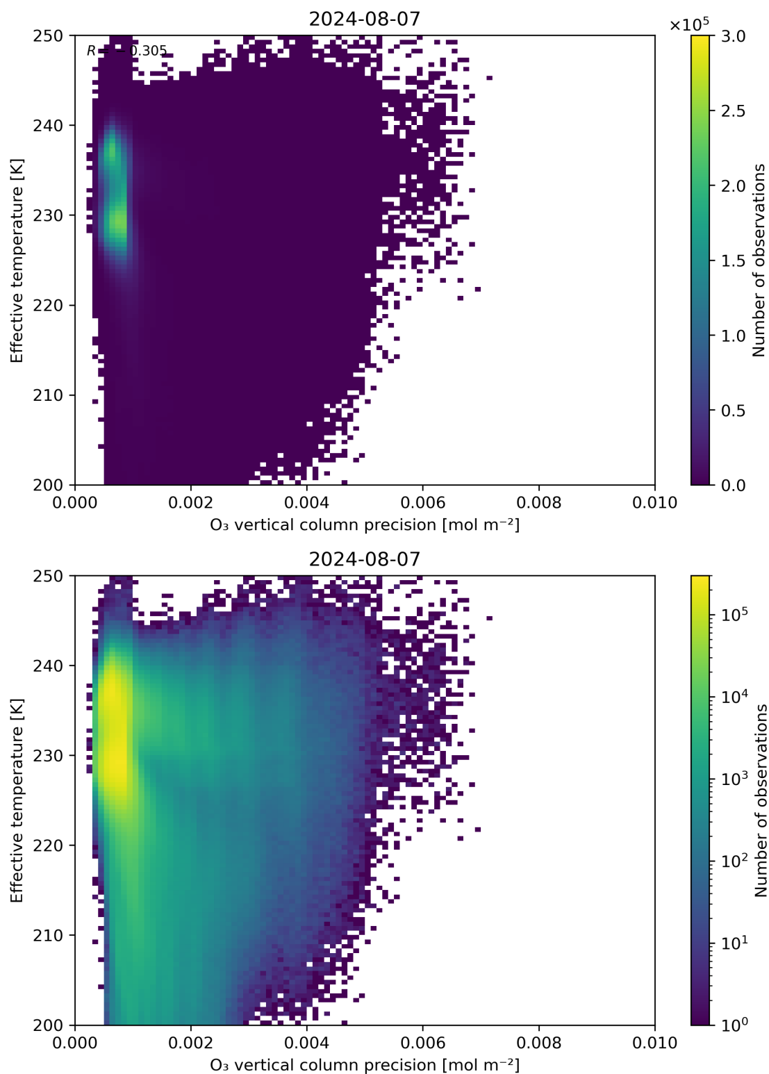
Figure 42: Scatter density plot of “O 3 vertical column precision” against “Effective temperature” for 2024-08-06 to 2024-08-08.
