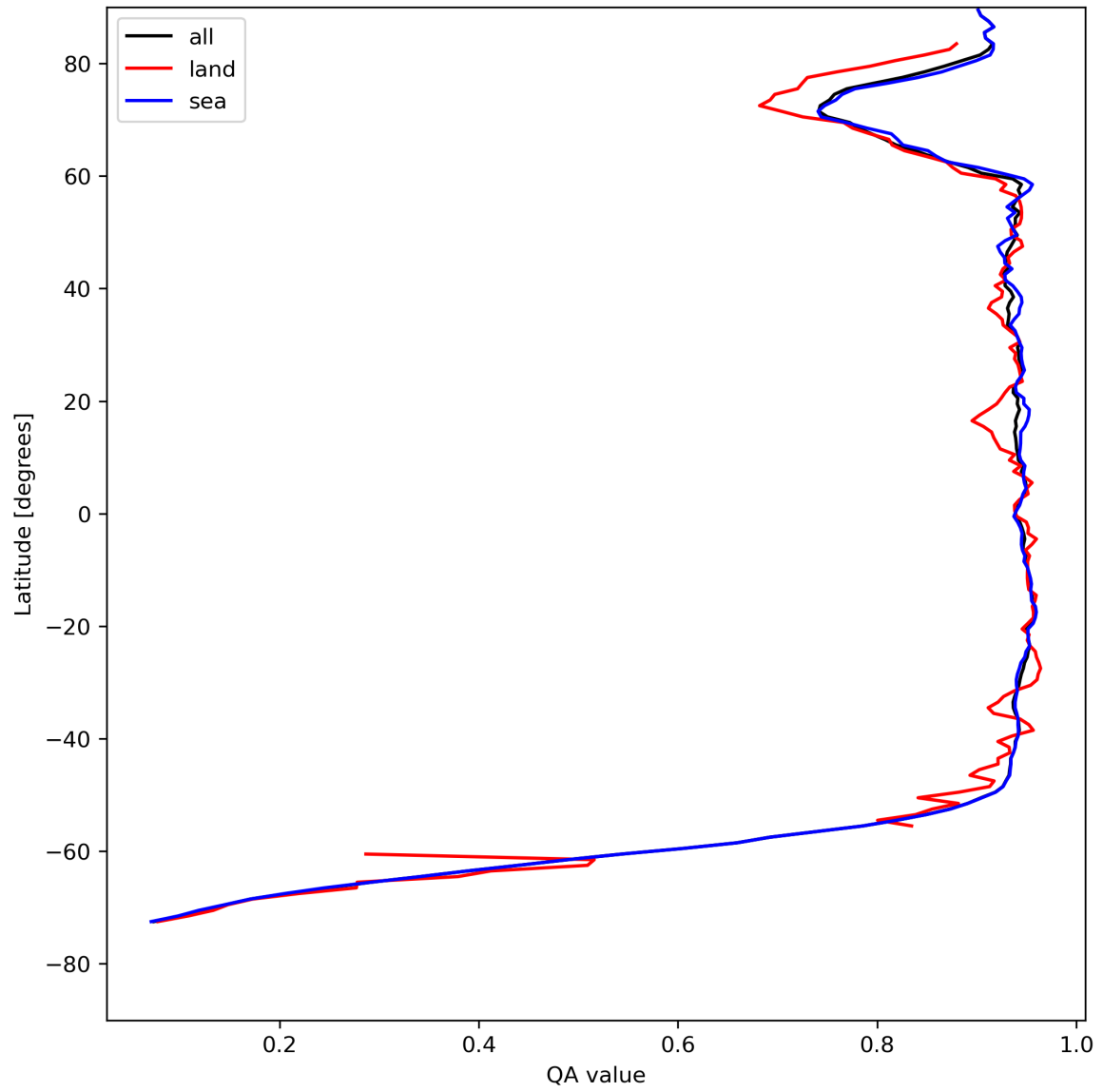
Figure 13: Zonal average of “QA value” for 2024-08-06 to 2024-08-08.
