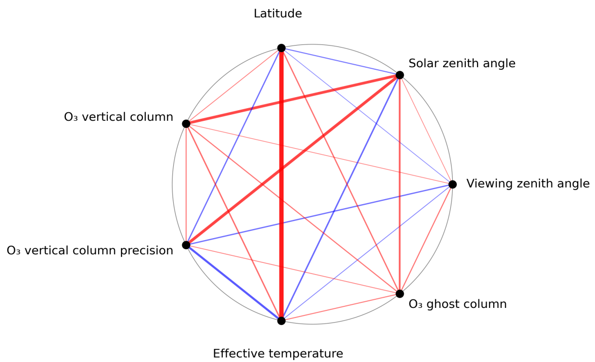
Figure 1: Map of correlation graph for 2024-08-06 to 2024-08-08.
