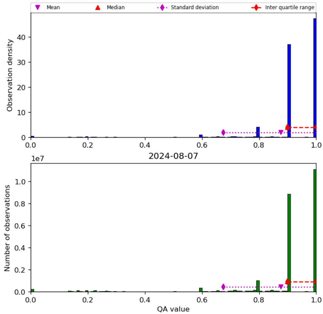
Figure 20: Histogram of “QA value” for 2024-08-06 to 2024-08-08
