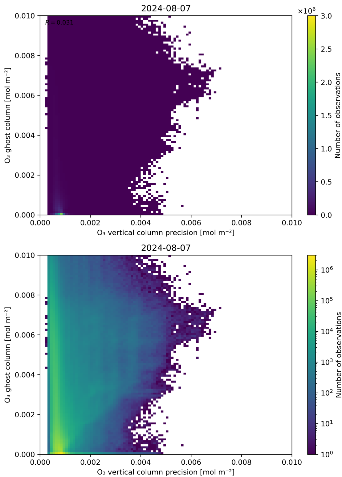
Figure 43: Scatter density plot of “ \text{O}_3 vertical column precision” against “ \text{O}_3 ghost column” for 2024-08-06 to 2024-08-08.
