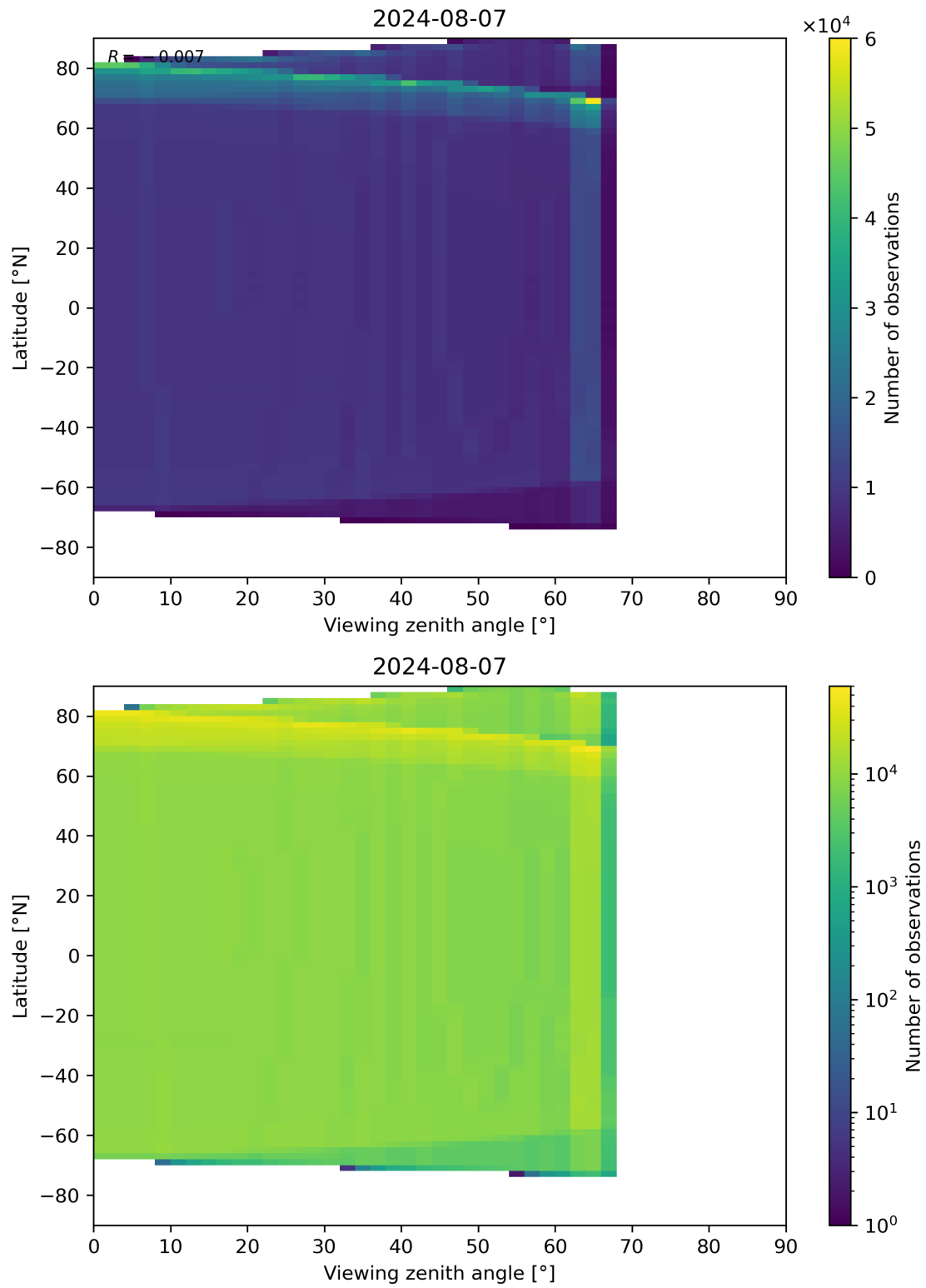
Figure 49: Scatter density plot of “Viewing zenith angle” against “Latitude” for 2024-08-06 to 2024-08-08.
