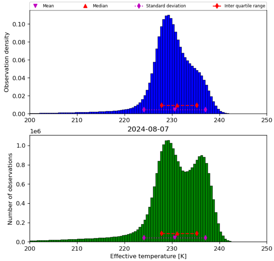
Figure 24: Histogram of “Effective temperature” for 2024-08-06 to 2024-08-08
