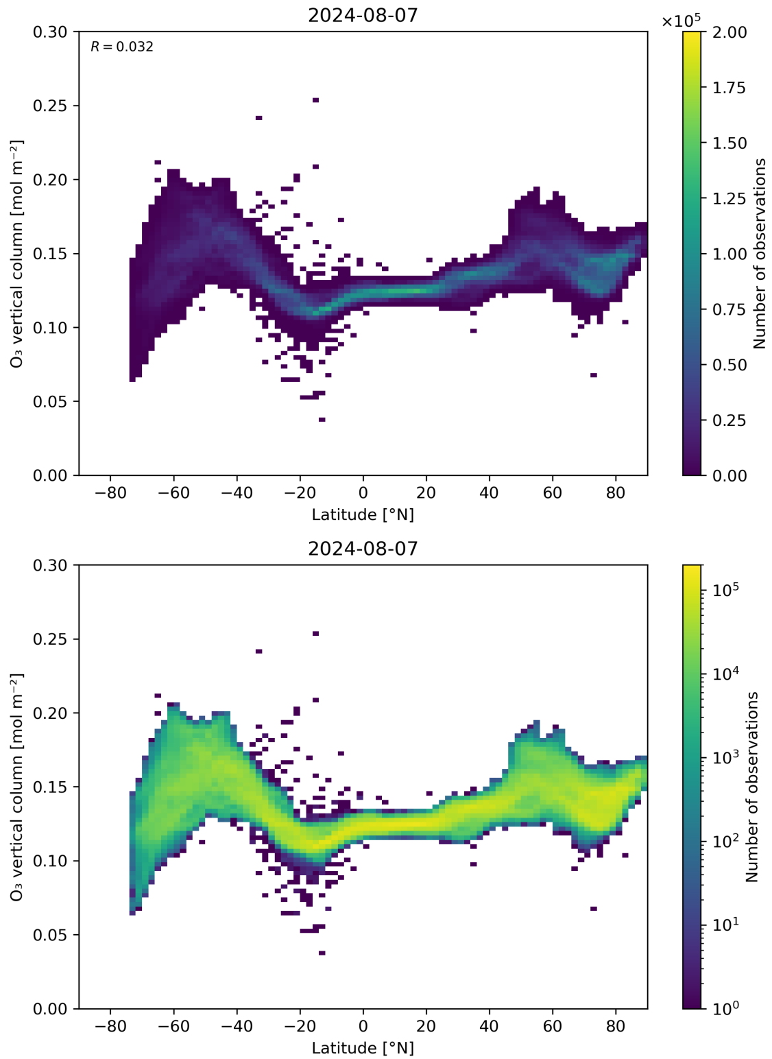
Figure 36: Scatter density plot of “Latitude” against “O 3 vertical column” for 2024-08-06 to 2024-08-08.
