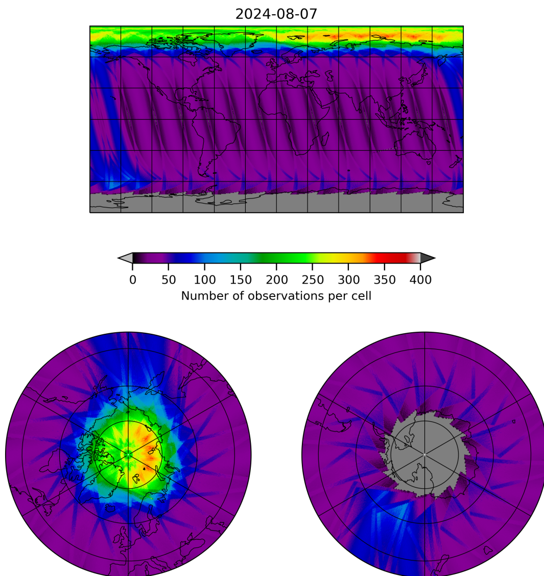
Figure 12: Map of the number of observations for 2024-08-06 to 2024-08-08
