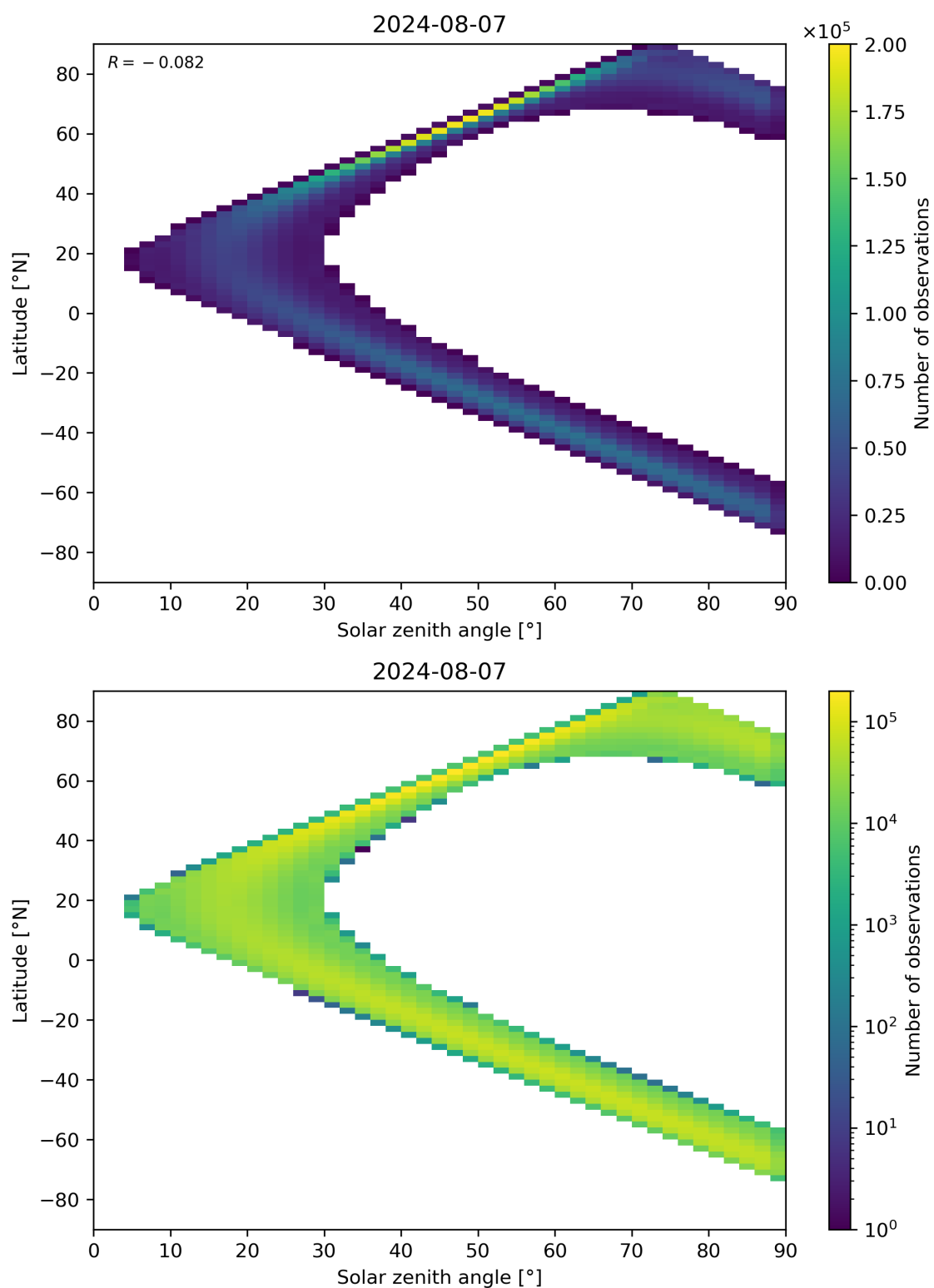
Figure 44: Scatter density plot of “Solar zenith angle” against “Latitude” for 2024-08-06 to 2024-08-08.
