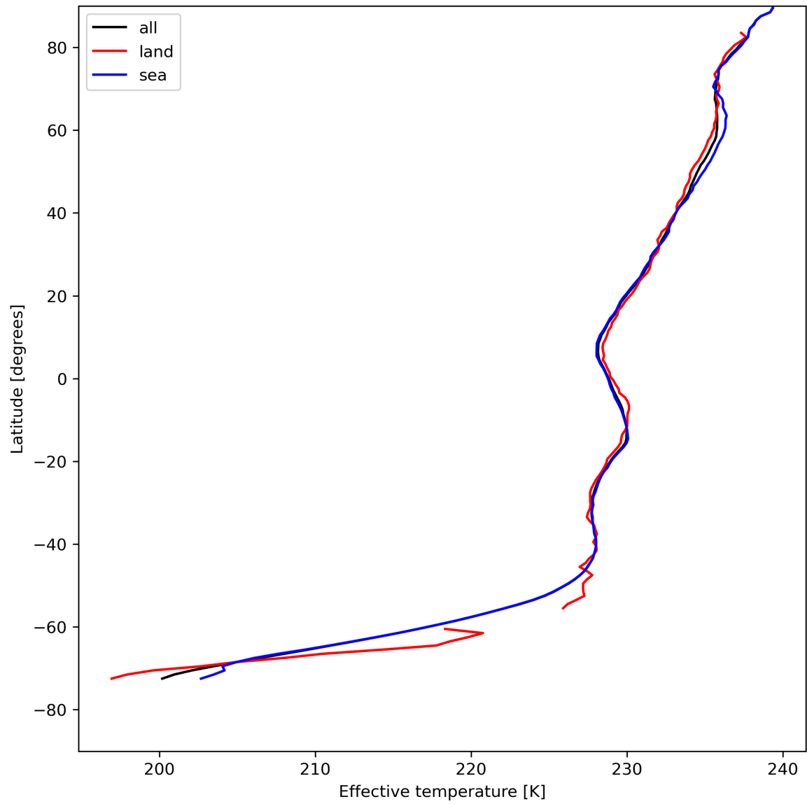
Figure 17: Zonal average of "Effective temperature" for 2024-08-06 to 2024-08-08.
