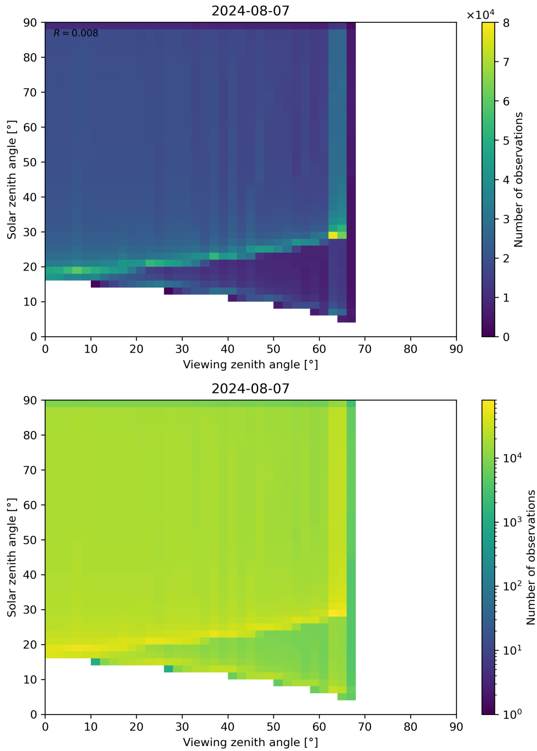
Figure 54: Scatter density plot of “Viewing zenith angle” against “Solar zenith angle” for 2024-08-06 to 2024-08-08.
