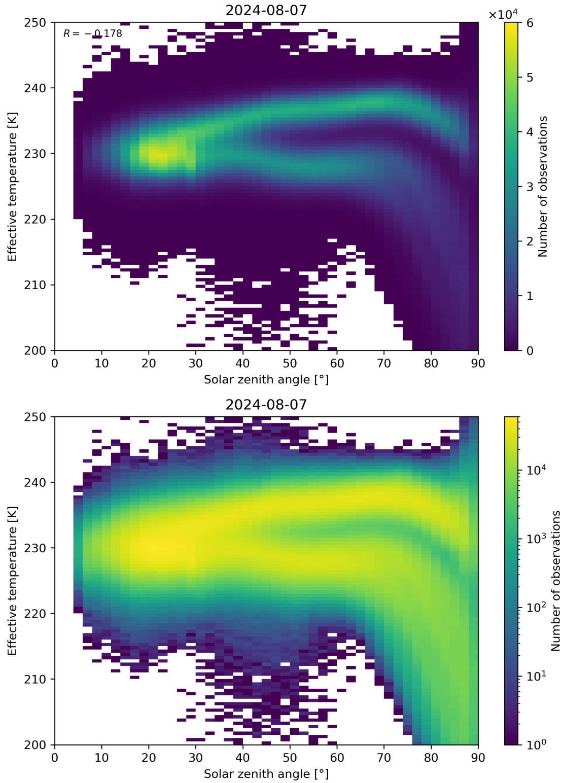
Figure 45: Scatter density plot of “Solar zenith angle” against “Effective temperature” for 2024-08-06 to 2024-08-08.
