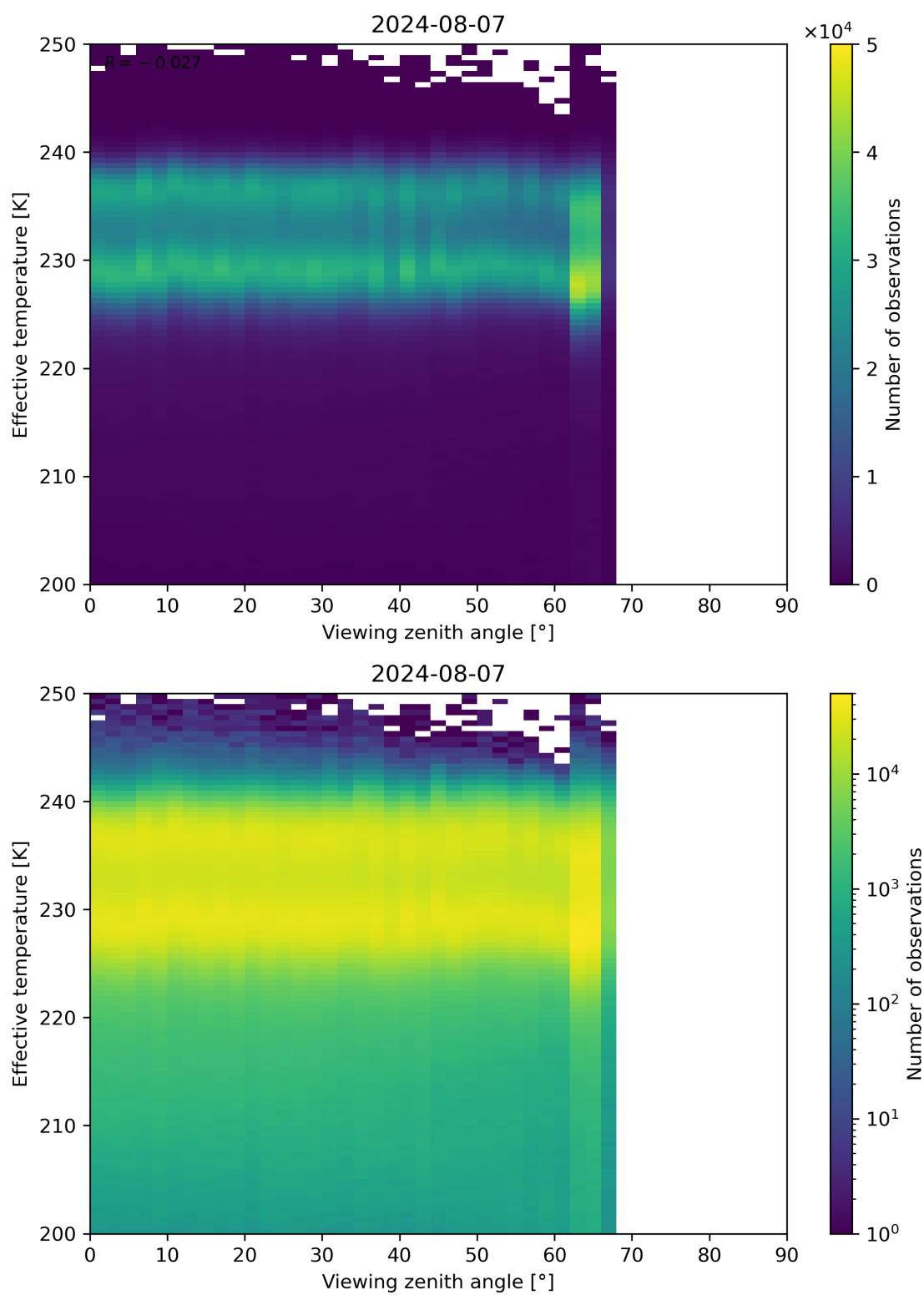
Figure 50: Scatter density plot of “Viewing zenith angle” against “Effective temperature” for 2024-08-06 to 2024-08-08.
