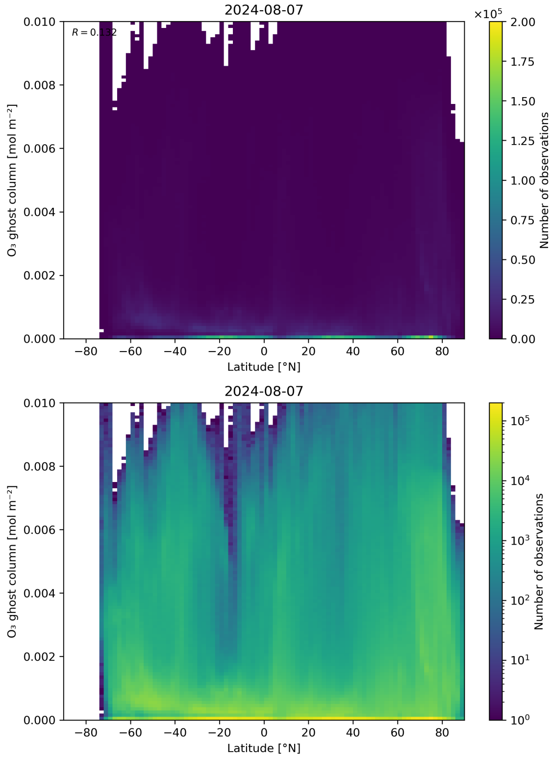
Figure 35: Scatter density plot of “Latitude” against “O 3 ghost column” for 2024-08-06 to 2024-08-08.
