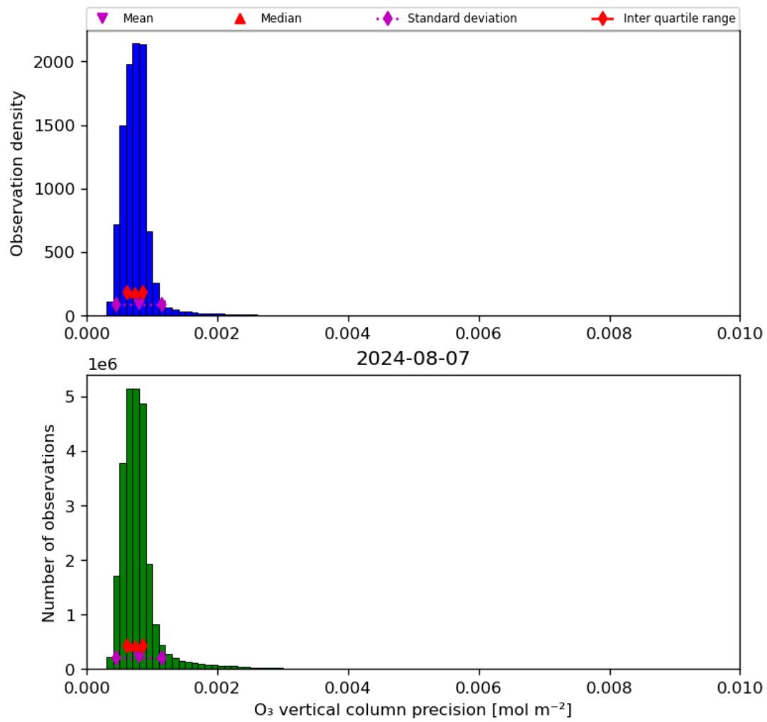
Figure 22: Histogram of “O 3 vertical column precision” for 2024-08-06 to 2024-08-08
