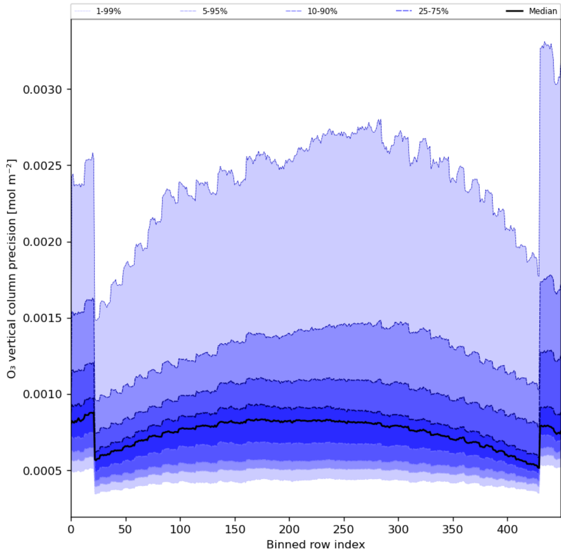
Figure 29: Along track statistics of “O 3 vertical column precision” for 2024-08-06 to 2024-08-08
