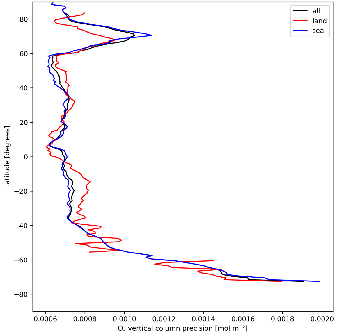
Figure 15: Zonal average of “O 3 vertical column precision” for 2024-08-06 to 2024-08-08.
