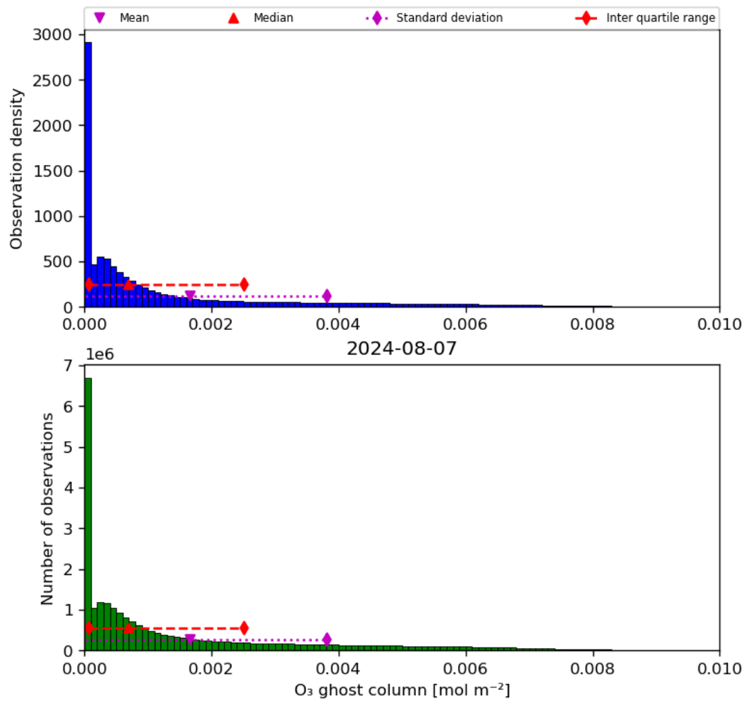
Figure 25: Histogram of “O 3 ghost column” for 2024-08-06 to 2024-08-08
