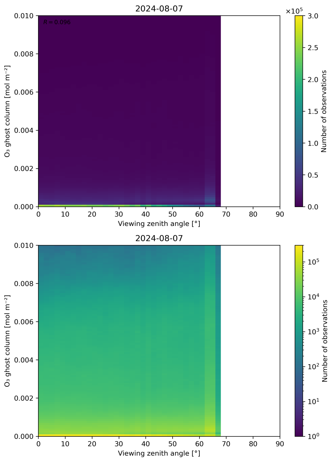
Figure 51: Scatter density plot of “Viewing zenith angle” against “O 3 ghost column” for 2024-08-06 to 2024-08-08.
