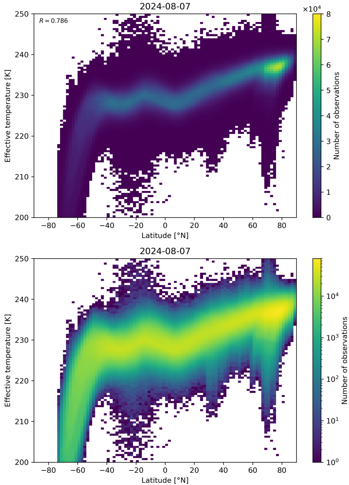
Figure 34: Scatter density plot of “Latitude” against “Effective temperature” for 2024-08-06 to 2024-08-08.
