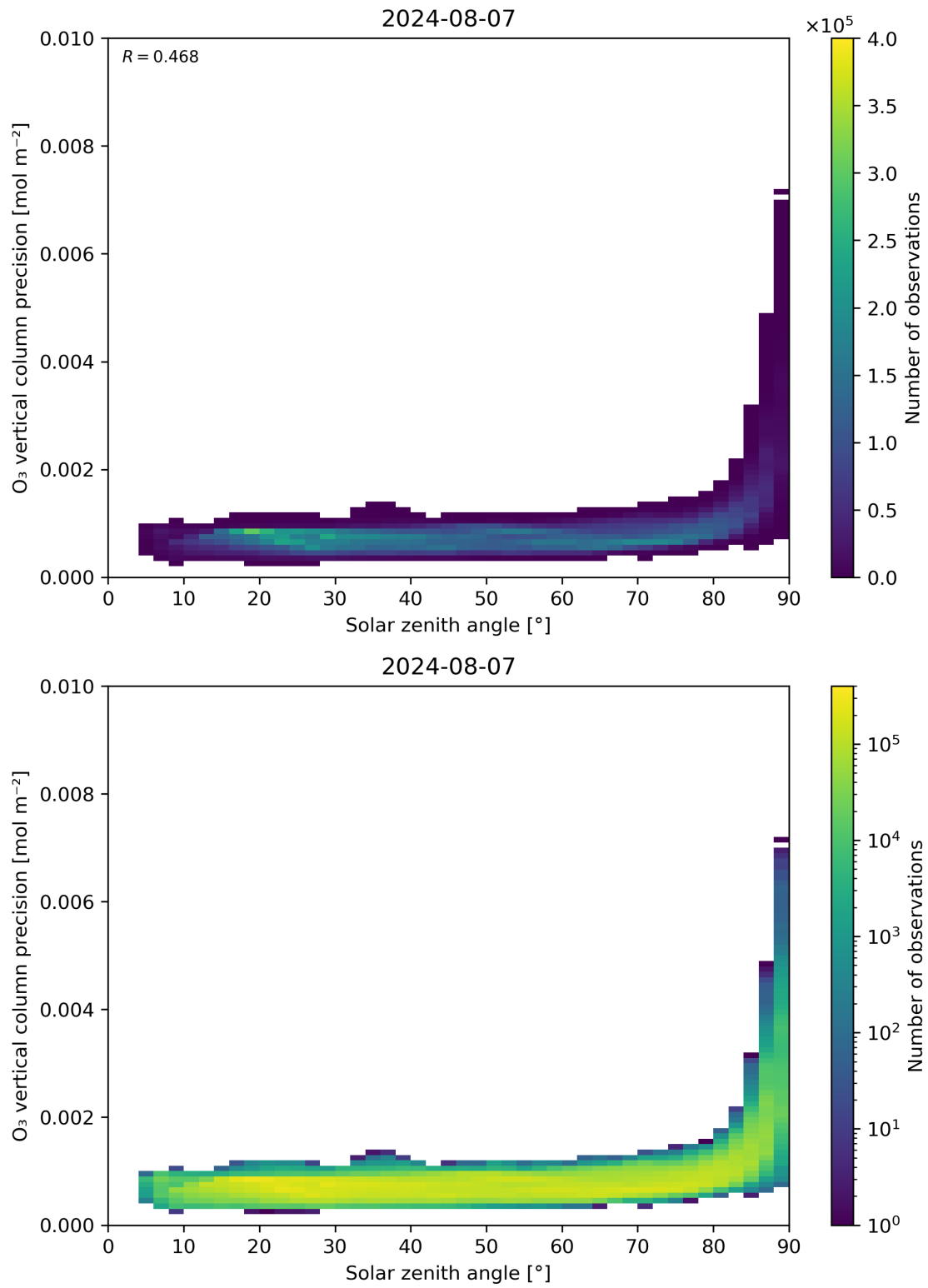
Figure 48: Scatter density plot of “Solar zenith angle” against “O 3 vertical column precision” for 2024-08-06 to 2024-08-08.
