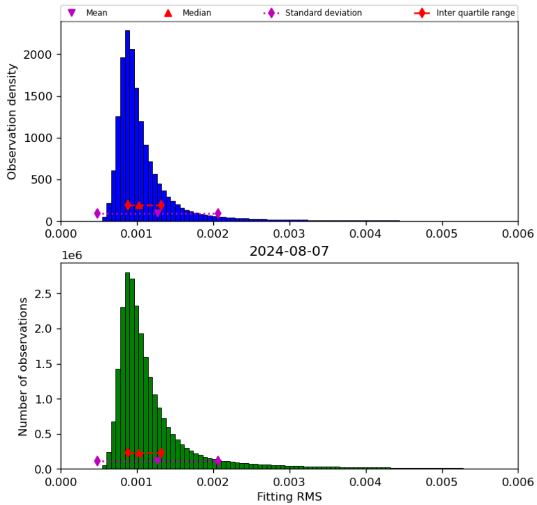
Figure 23: Histogram of “Fitting RMS” for 2024-08-06 to 2024-08-08
