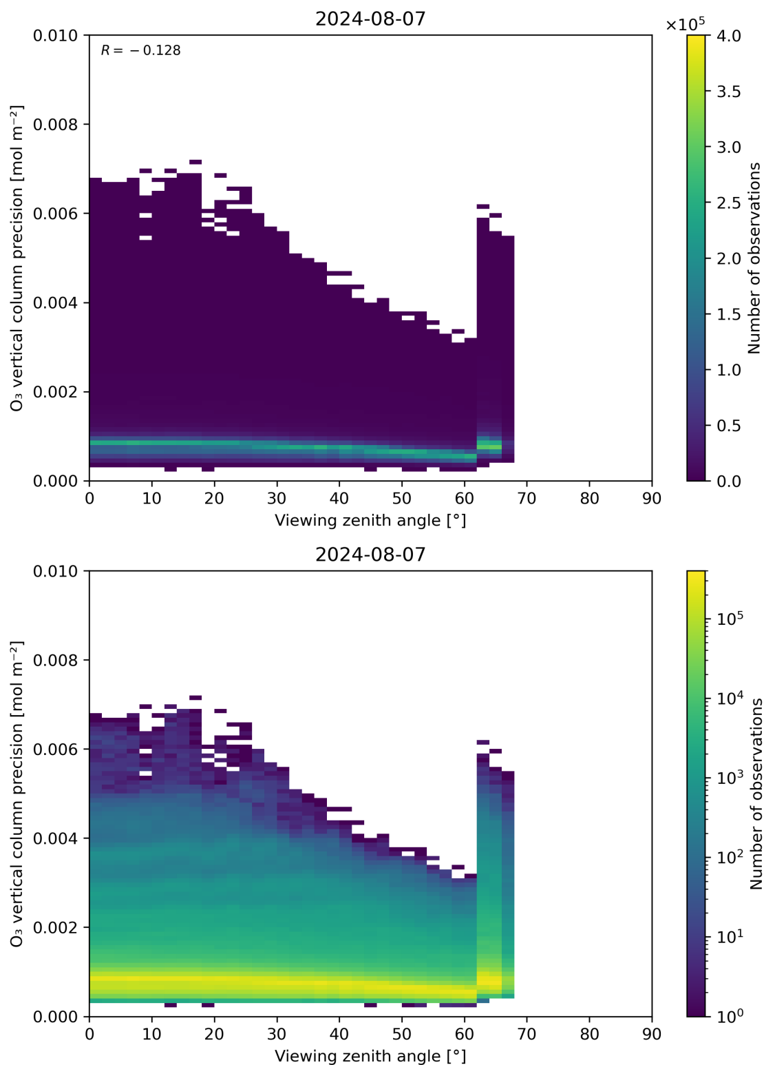
Figure 53: Scatter density plot of “Viewing zenith angle” against “O 3 vertical column precision” for 2024-08-06 to 2024-08-08.
