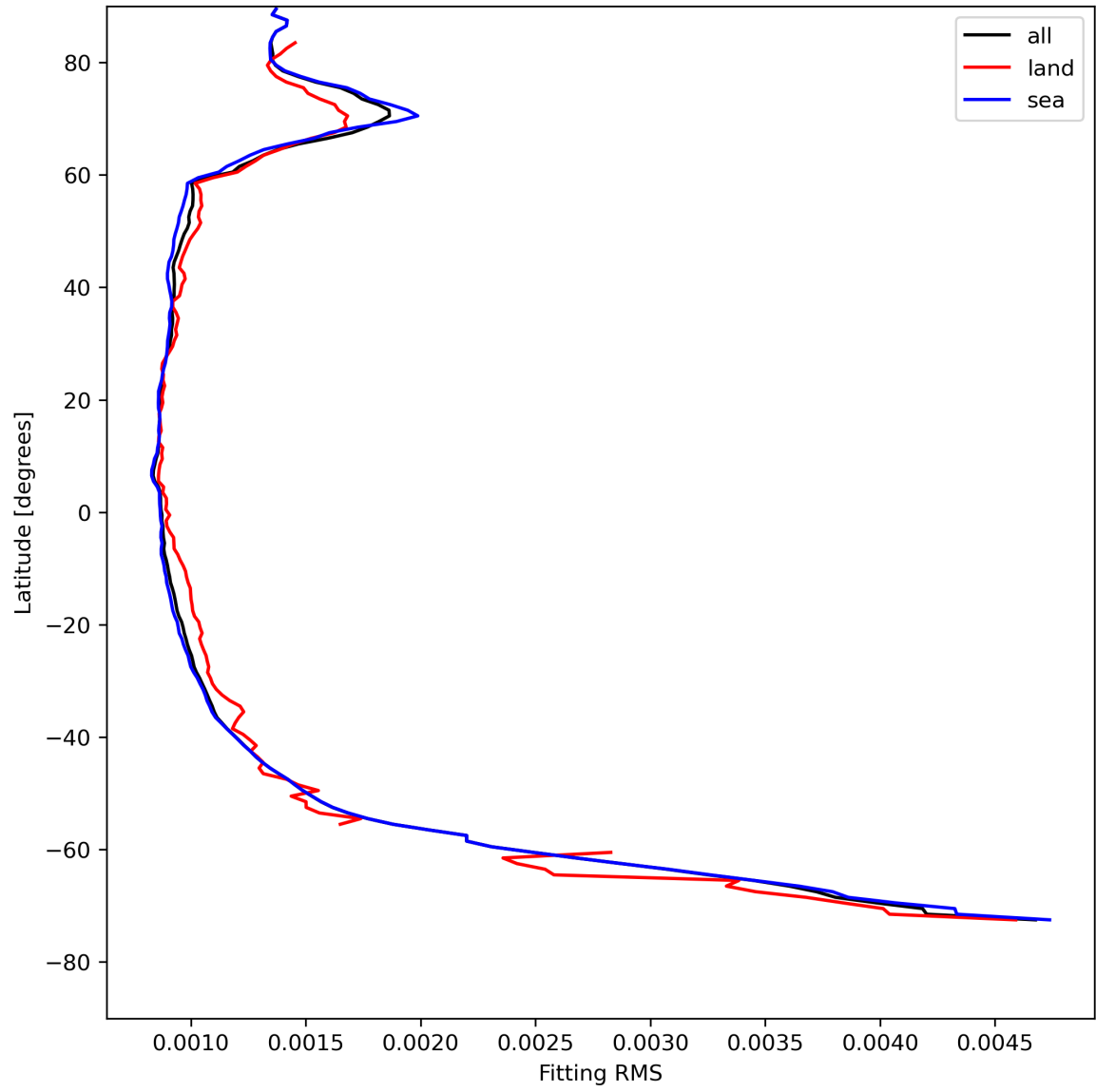
Figure 16: Zonal average of “Fitting RMS” for 2024-08-06 to 2024-08-08.
