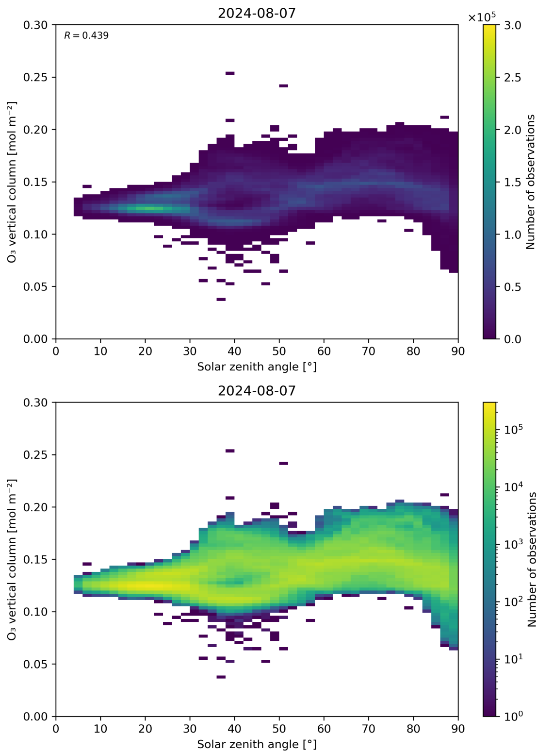
Figure 47: Scatter density plot of “Solar zenith angle” against “O 3 vertical column” for 2024-08-06 to 2024-08-08.
