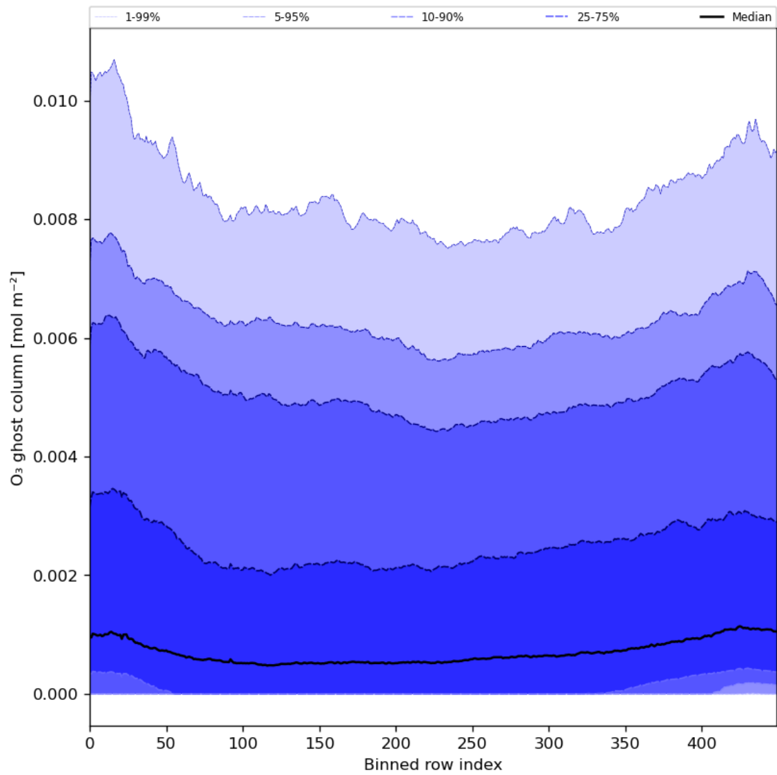
Figure 32: Along track statistics of “O 3 ghost column” for 2024-08-06 to 2024-08-08
