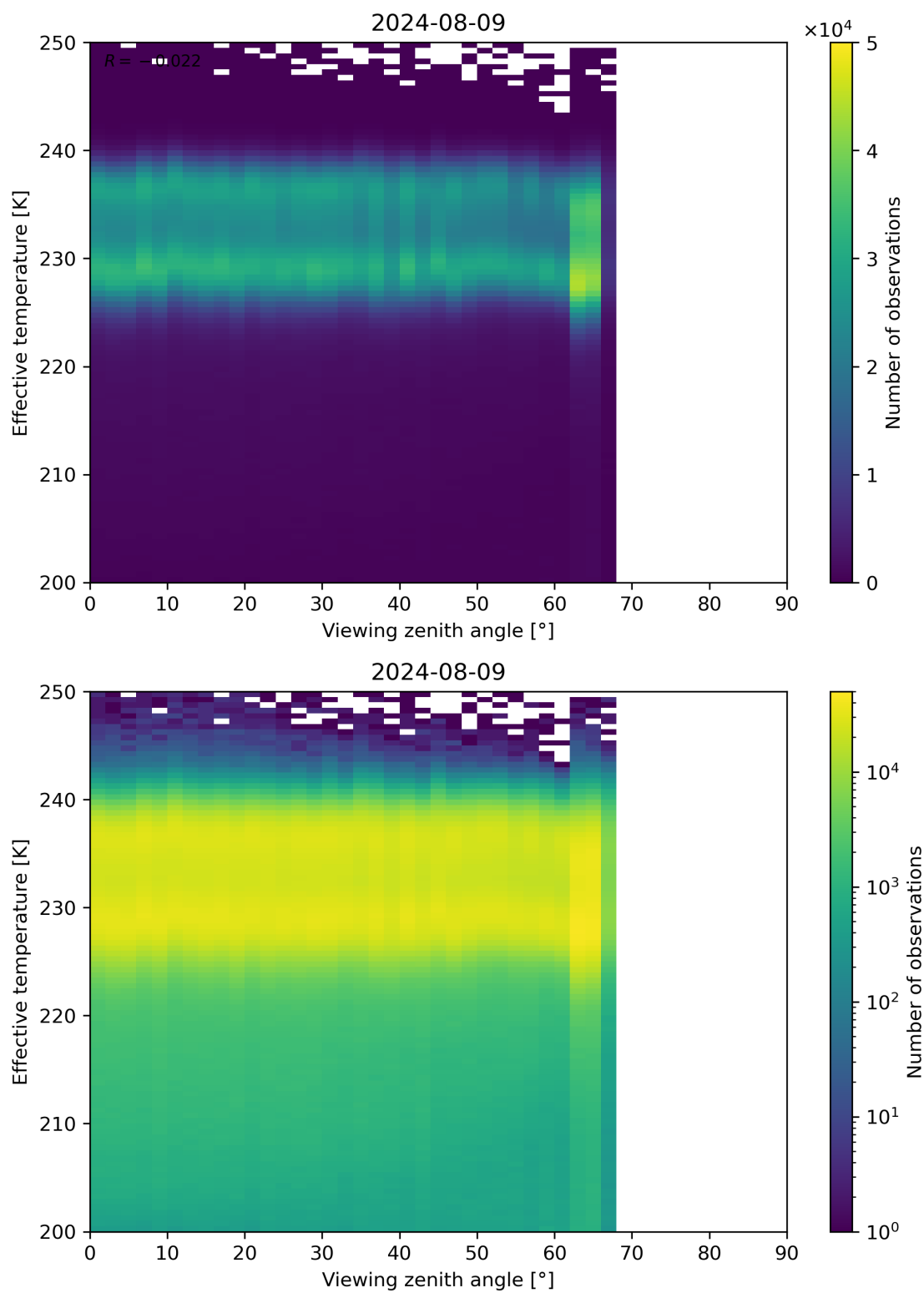
Figure 50: Scatter density plot of “Viewing zenith angle” against “Effective temperature” for 2024-08-08 to 2024-08-10.
