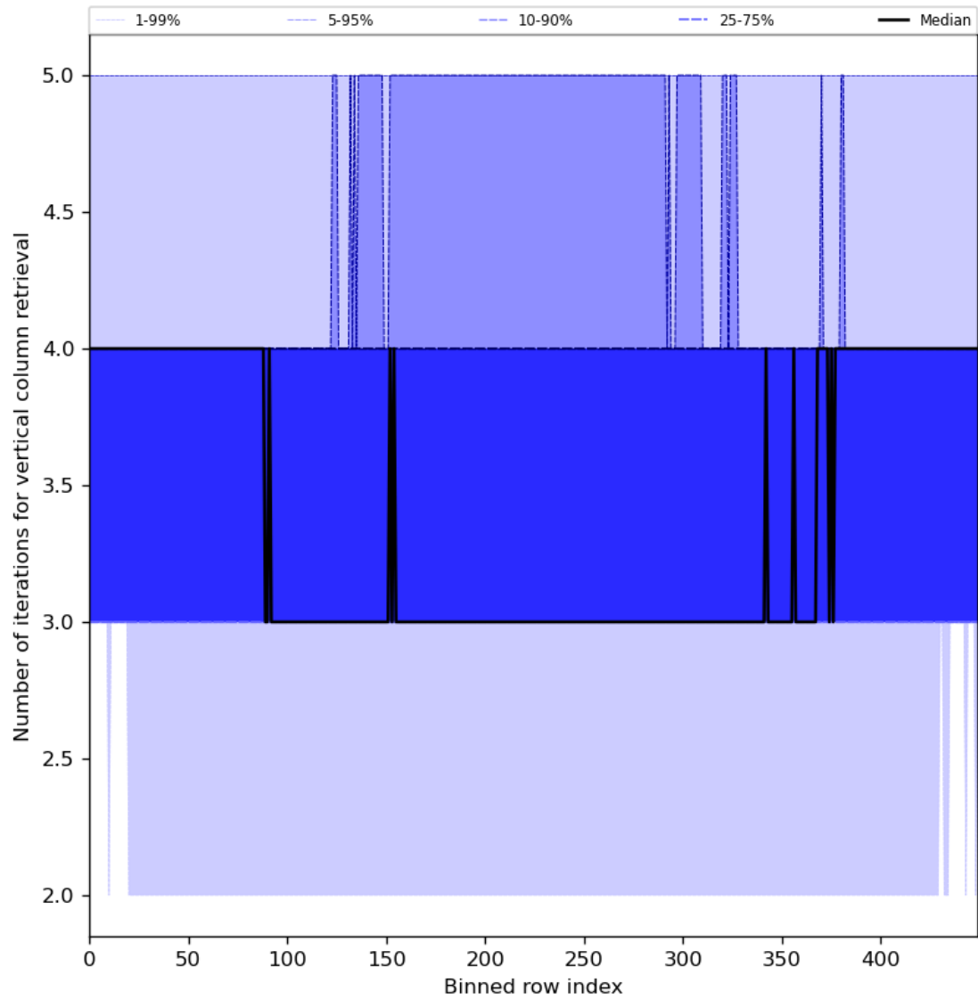
Figure 33: Along track statistics of “Number of iterations for vertical column retrieval” for 2024-08-08 to 2024-08-10
