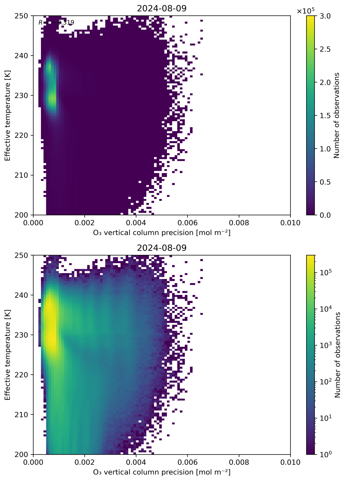
Figure 42: Scatter density plot of “ O_3 vertical column precision” against “Effective temperature” for 2024-08-08 to 2024-08-10.
