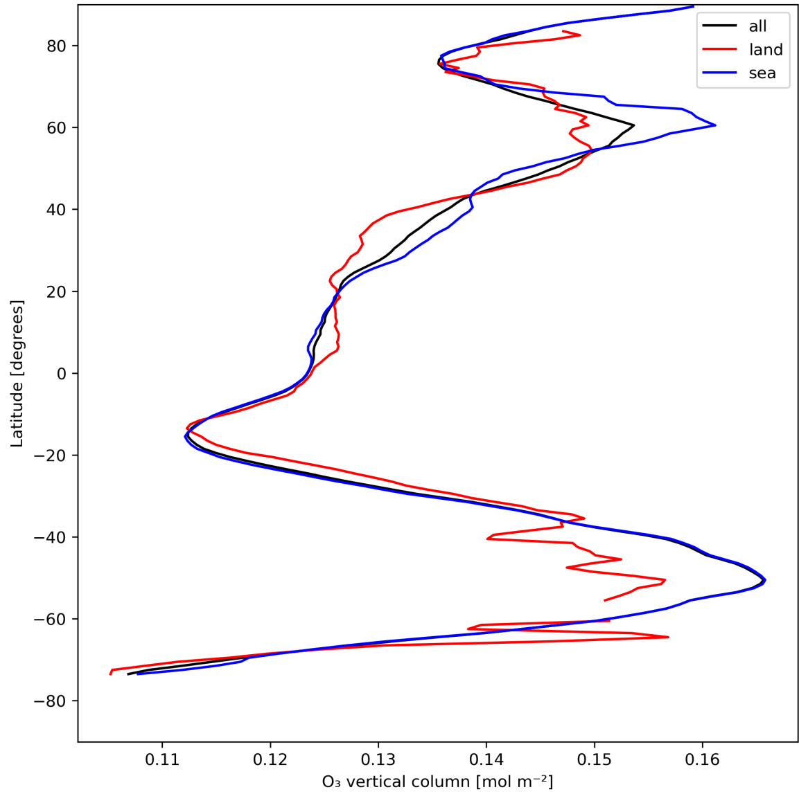
Figure 14: Zonal average of “O 3 vertical column” for 2024-08-08 to 2024-08-10.
