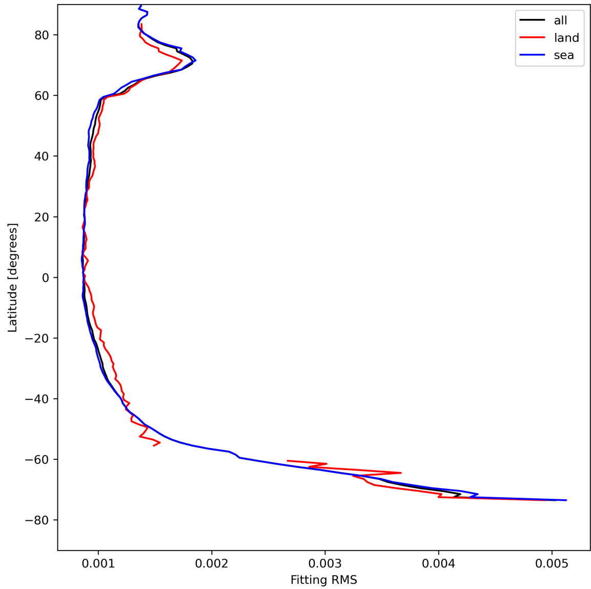
Figure 16: Zonal average of “Fitting RMS” for 2024-08-08 to 2024-08-10.
