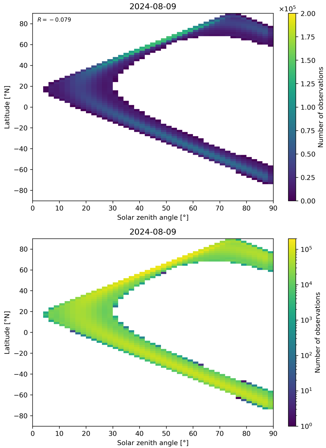
Figure 44: Scatter density plot of “Solar zenith angle” against “Latitude” for 2024-08-08 to 2024-08-10.
