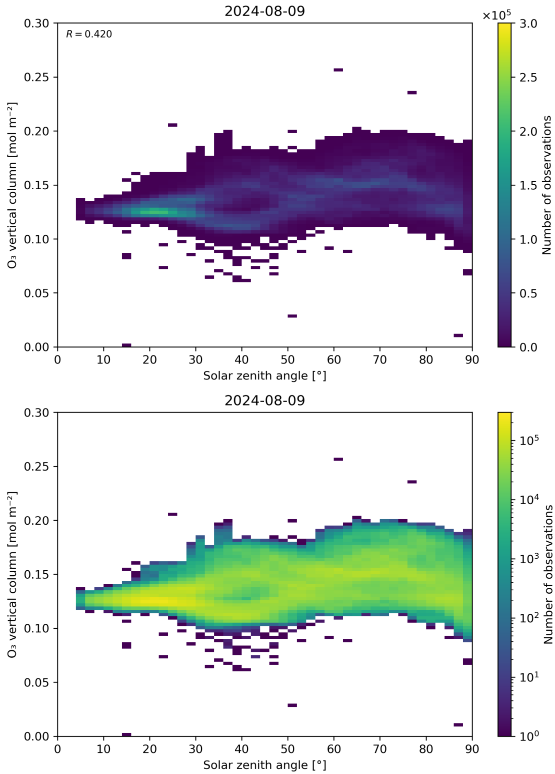
Figure 47: Scatter density plot of “Solar zenith angle” against “O 3 vertical column” for 2024-08-08 to 2024-08-10.
