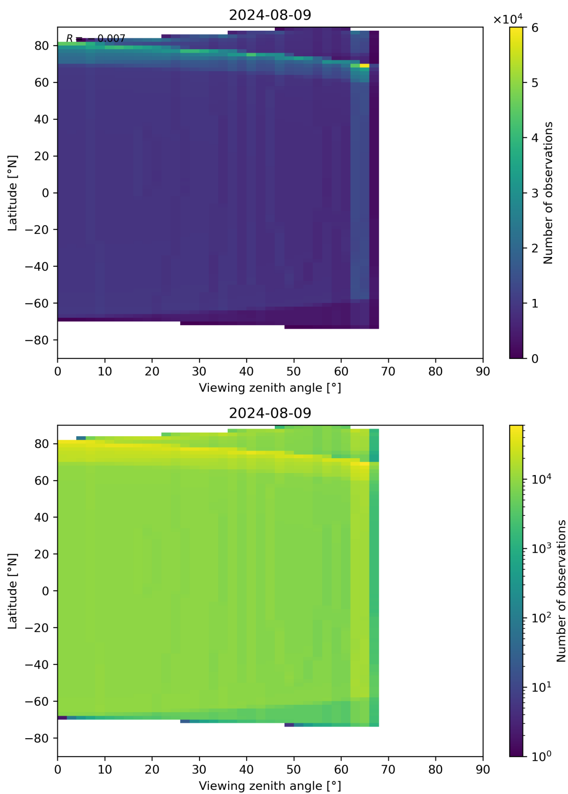
Figure 49: Scatter density plot of “Viewing zenith angle” against “Latitude” for 2024-08-08 to 2024-08-10.
