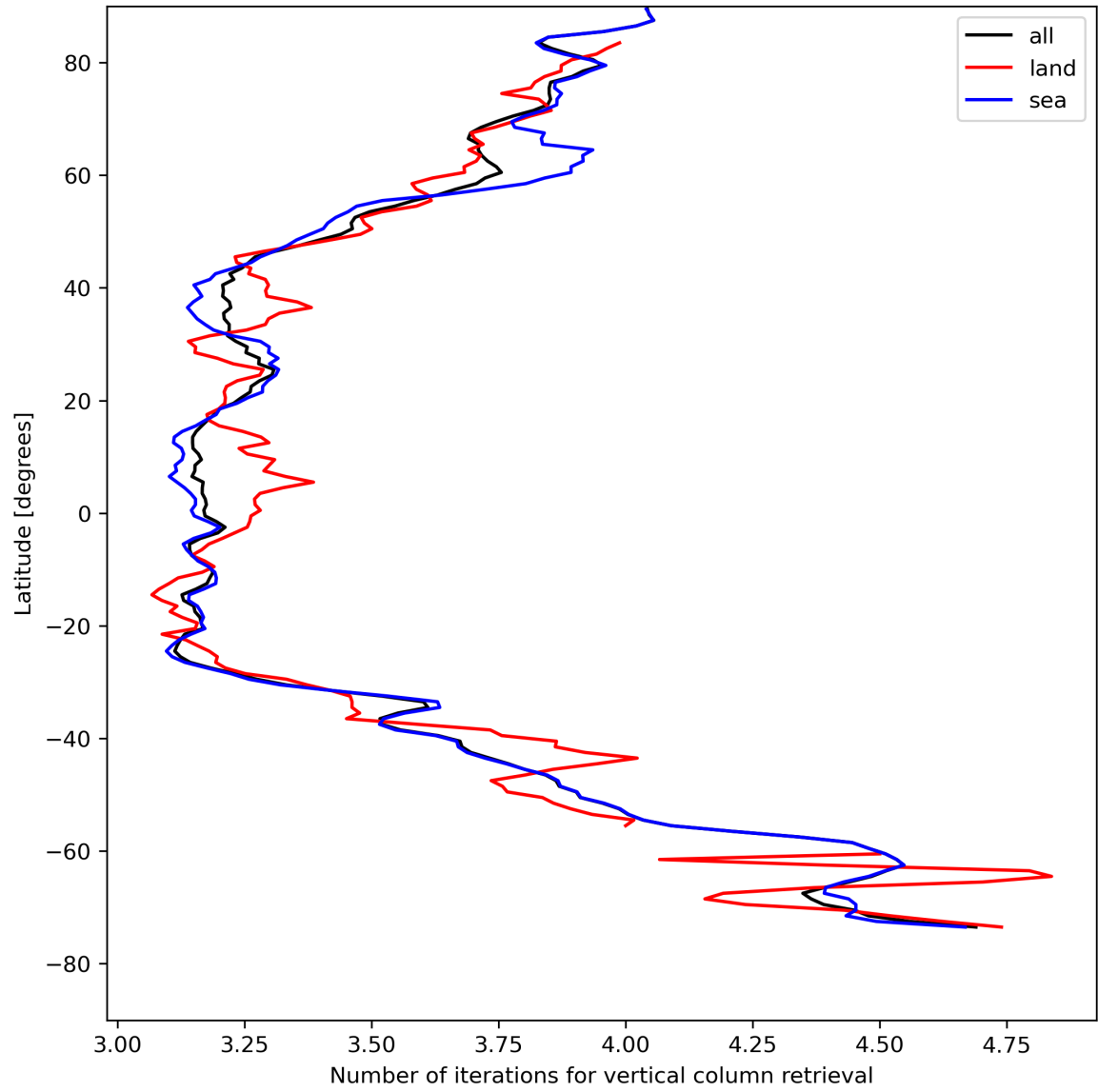
Figure 19: Zonal average of “Number of iterations for vertical column retrieval” for 2024-08-08 to 2024-08-10.
