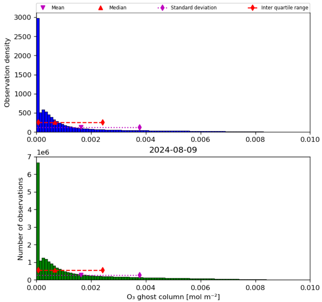
Figure 25: Histogram of “O 3 ghost column” for 2024-08-08 to 2024-08-10
