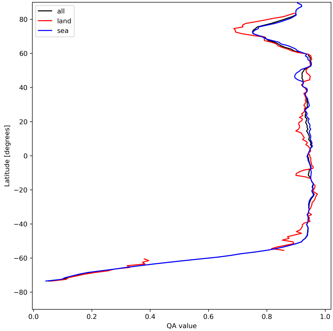
Figure 13: Zonal average of “QA value” for 2024-08-08 to 2024-08-10.
