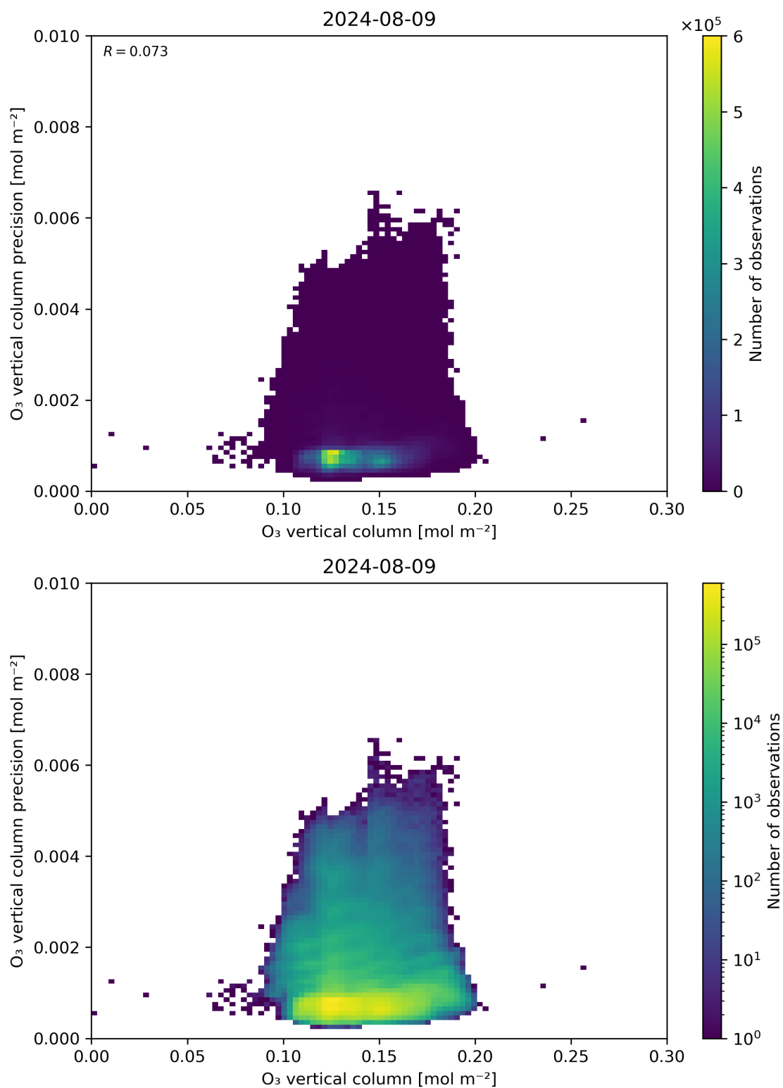
Figure 41: Scatter density plot of “O 3 vertical column” against “O 3 vertical column precision” for 2024-08-08 to 2024-08-10.
