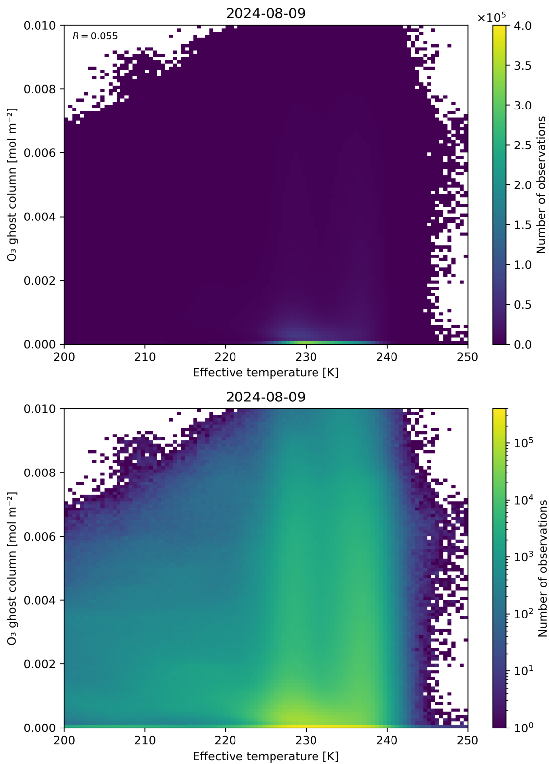
Figure 38: Scatter density plot of “Effective temperature” against “O 3 ghost column” for 2024-08-08 to 2024-08-10.
