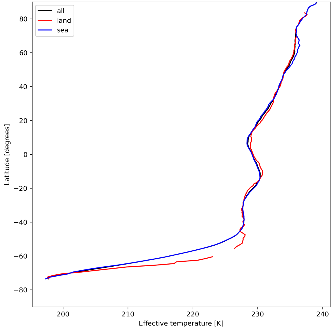
Figure 17: Zonal average of “Effective temperature” for 2024-08-08 to 2024-08-10.
