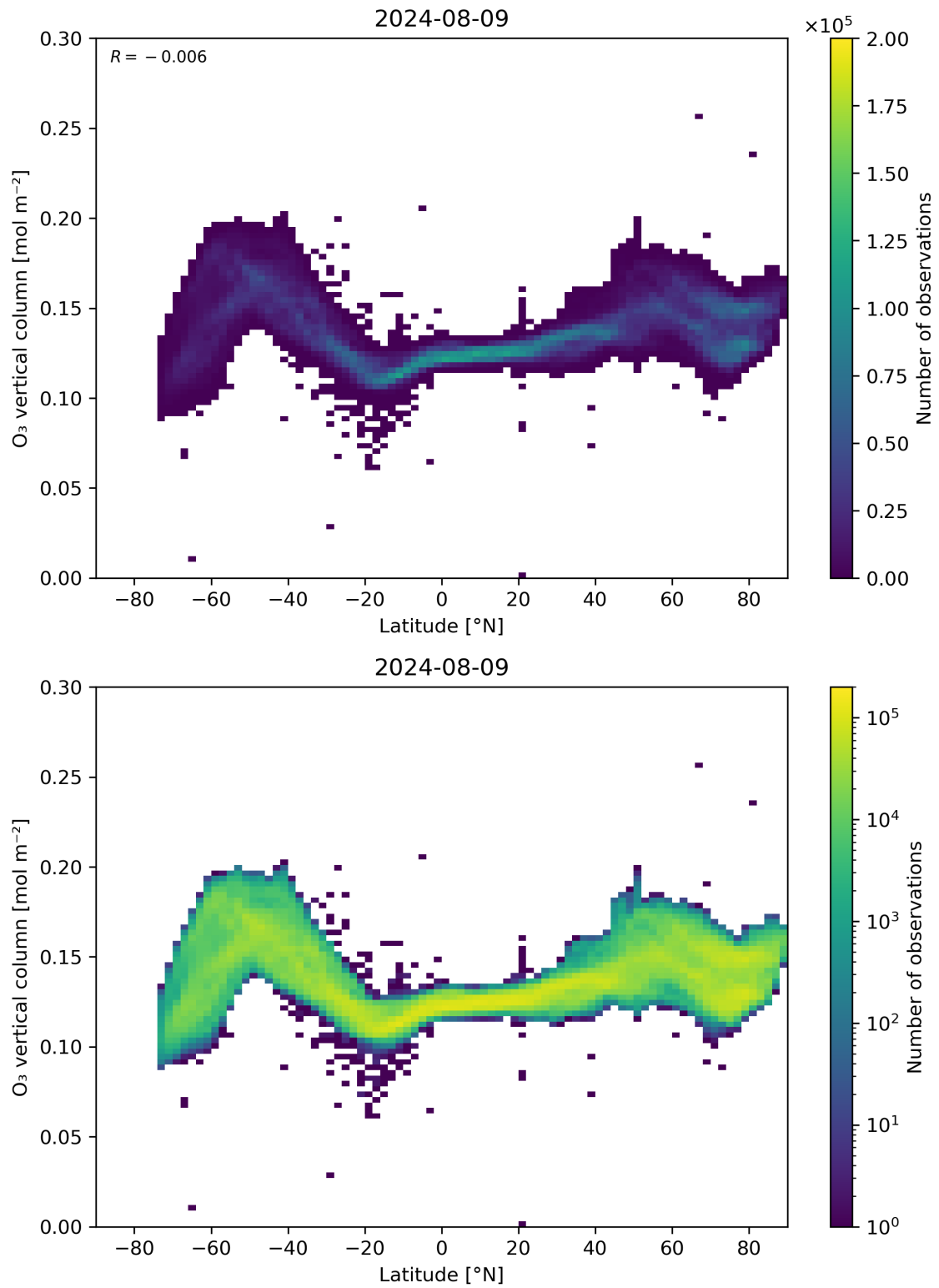
Figure 36: Scatter density plot of “Latitude” against “O 3 vertical column” for 2024-08-08 to 2024-08-10.
