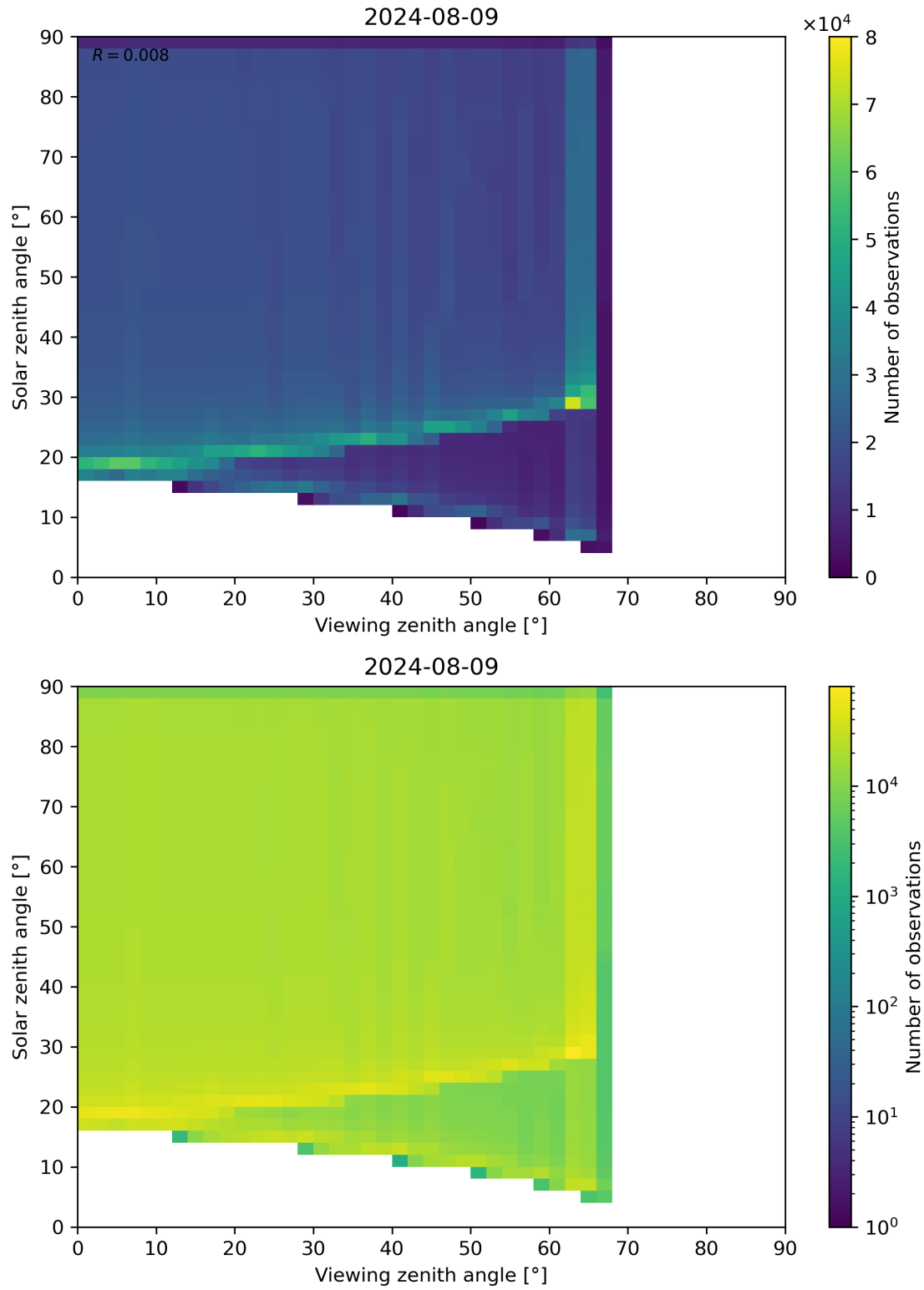
Figure 54: Scatter density plot of “Viewing zenith angle” against “Solar zenith angle” for 2024-08-08 to 2024-08-10.
