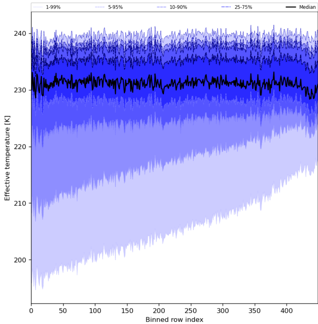
Figure 31: Along track statistics of “Effective temperature” for 2024-08-08 to 2024-08-10
