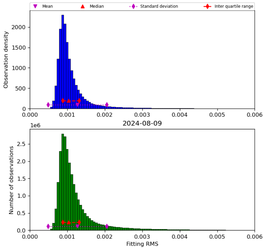
Figure 23: Histogram of “Fitting RMS” for 2024-08-08 to 2024-08-10
