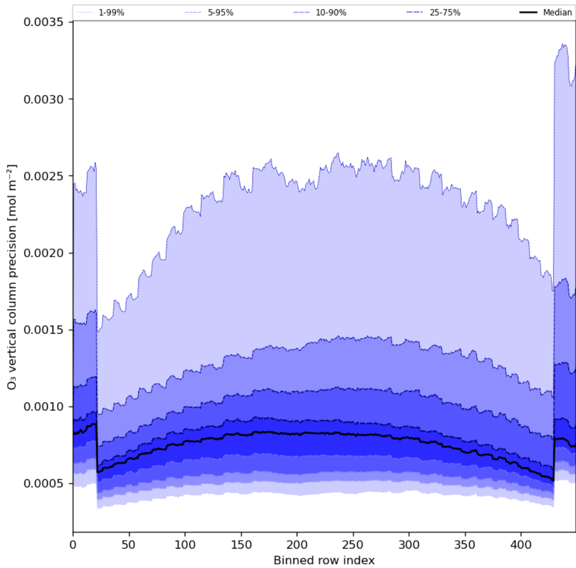
Figure 29: Along track statistics of “O 3 vertical column precision” for 2024-08-08 to 2024-08-10
