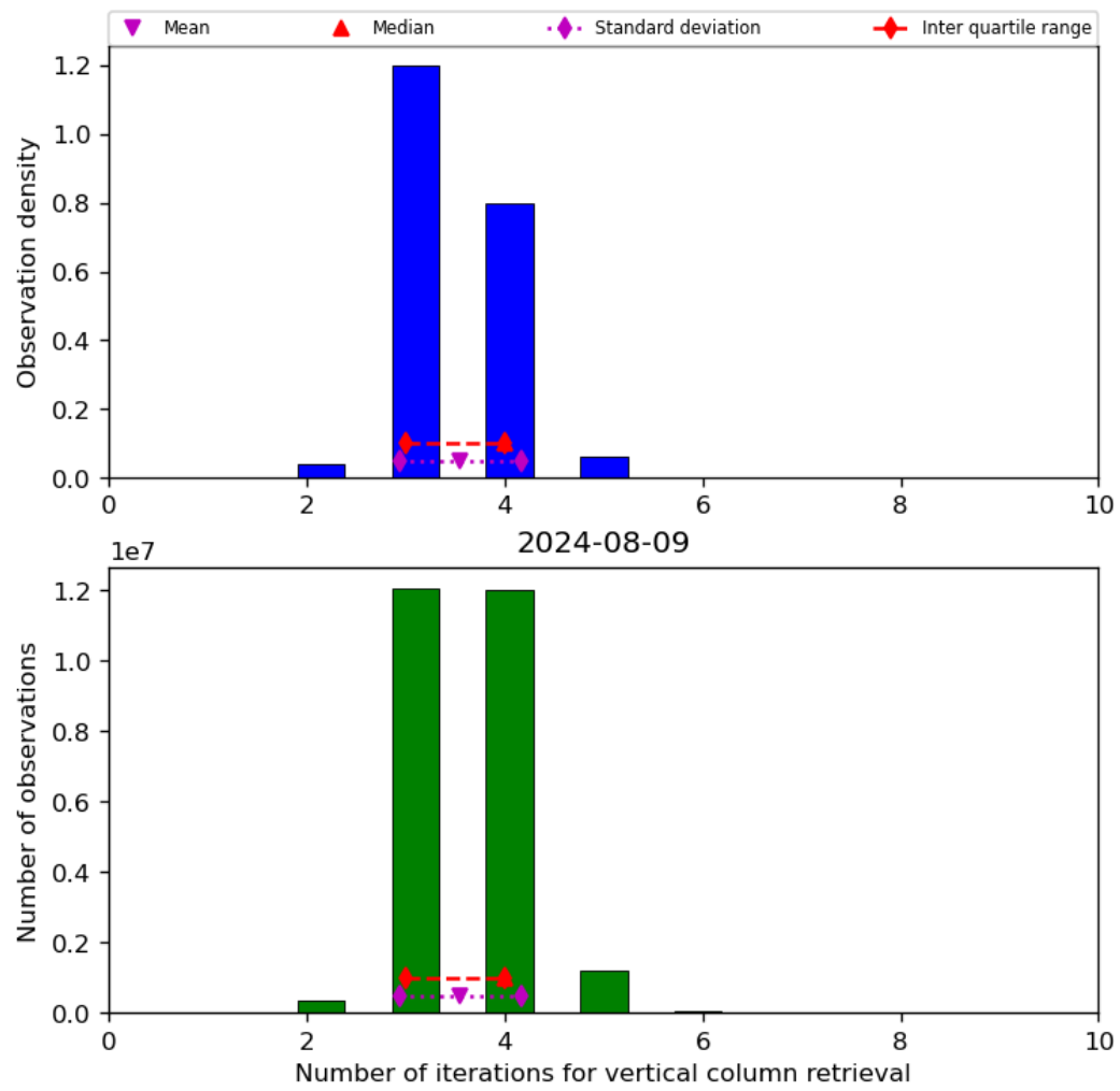
Figure 26: Histogram of “Number of iterations for vertical column retrieval” for 2024-08-08 to 2024-08-10
