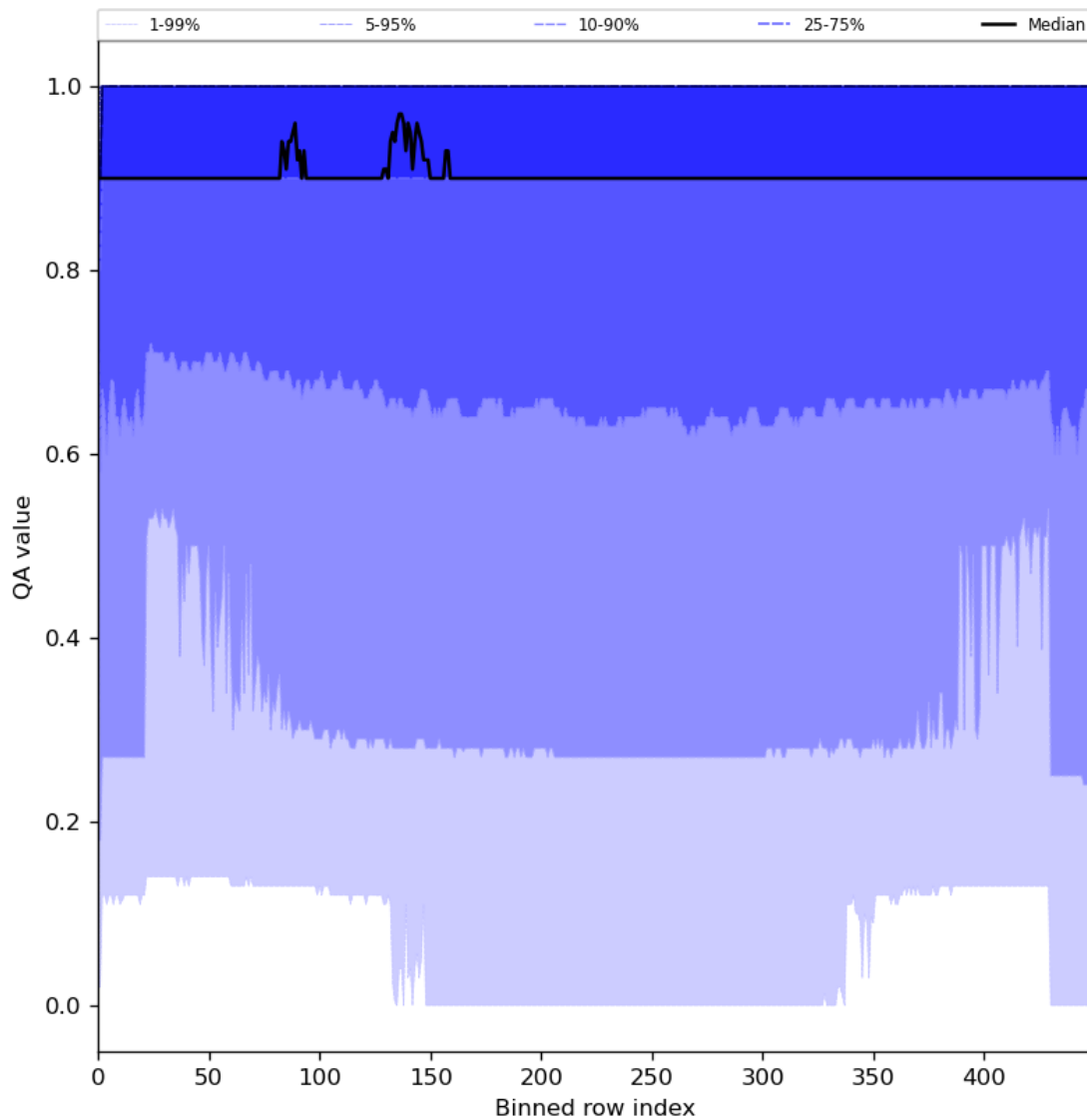
Figure 27: Along track statistics of “QA value” for 2024-08-08 to 2024-08-10
