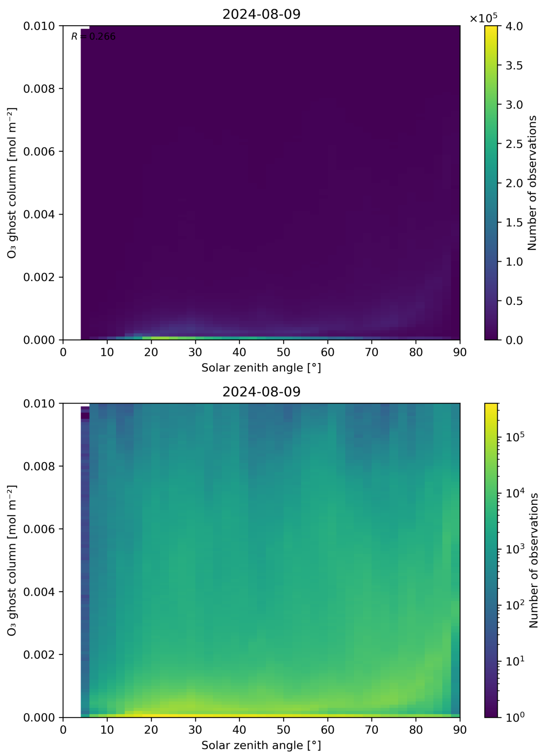
Figure 46: Scatter density plot of “Solar zenith angle” against “O 3 ghost column” for 2024-08-08 to 2024-08-10.
