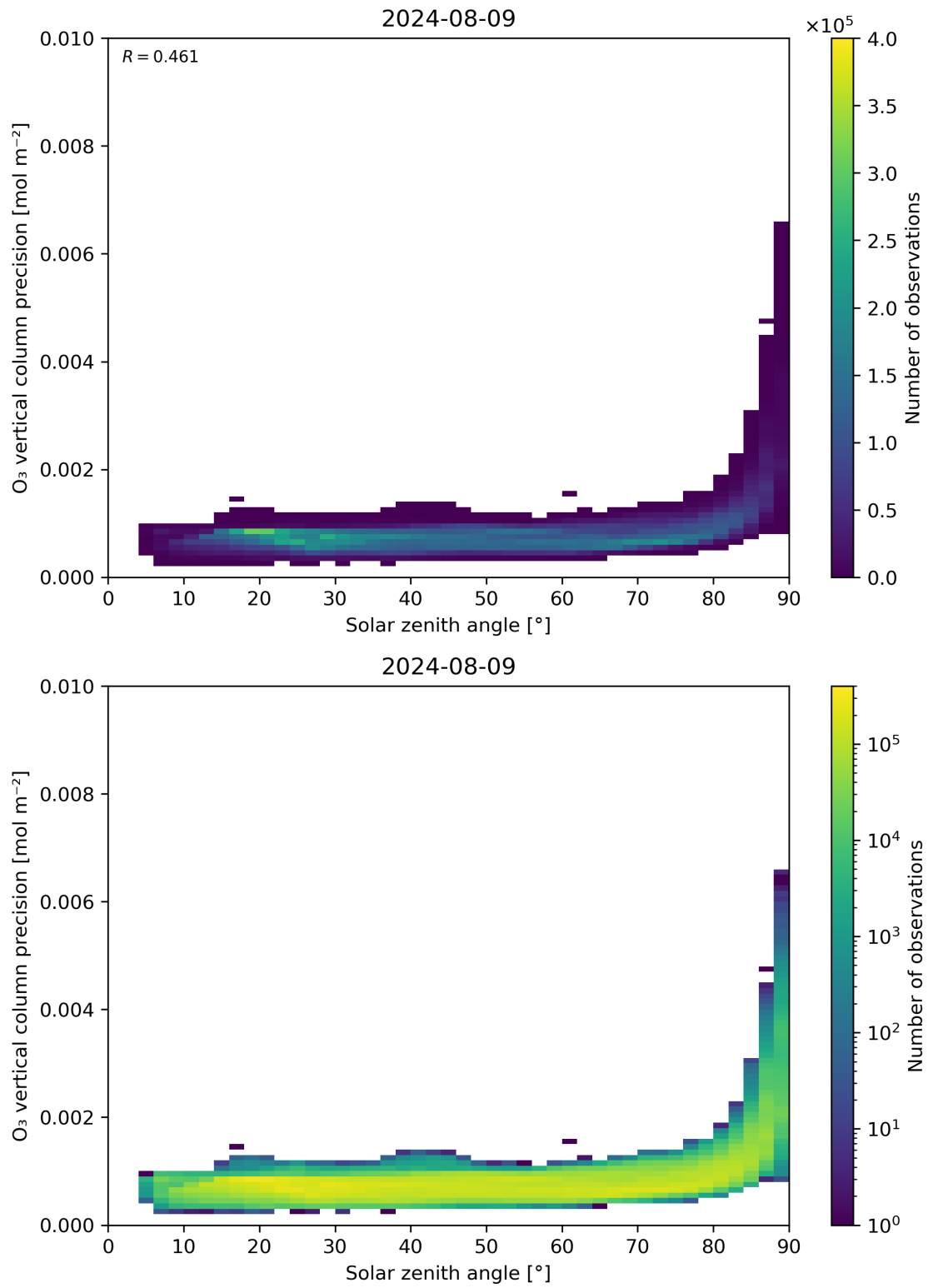
Figure 48: Scatter density plot of “Solar zenith angle” against “O 3 vertical column precision” for 2024-08-08 to 2024-08-10.
