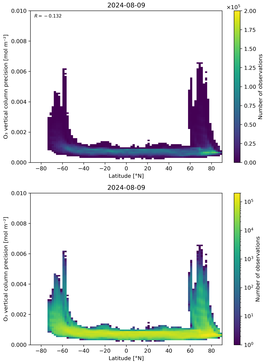
Figure 37: Scatter density plot of “Latitude” against “O 3 vertical column precision” for 2024-08-08 to 2024-08-10.
