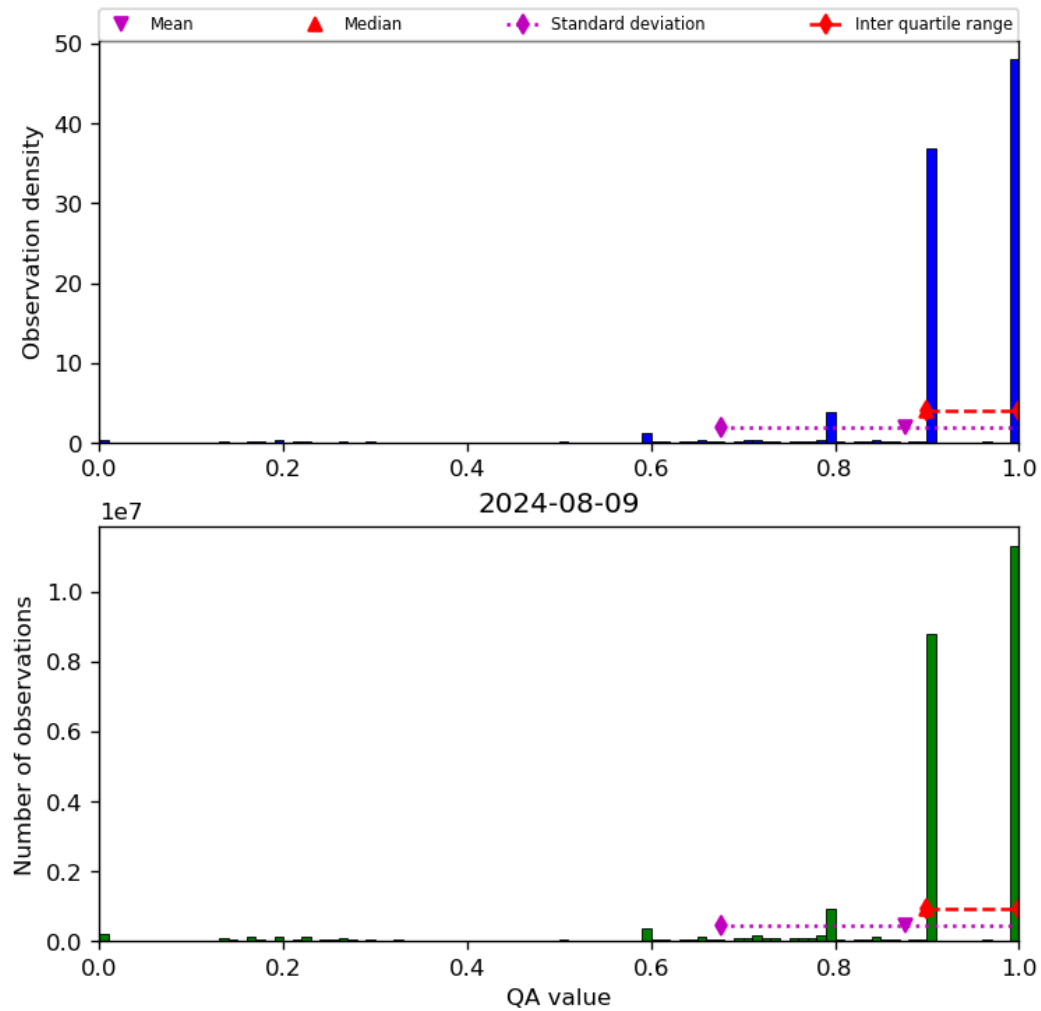
Figure 20: Histogram of “QA value” for 2024-08-08 to 2024-08-10
