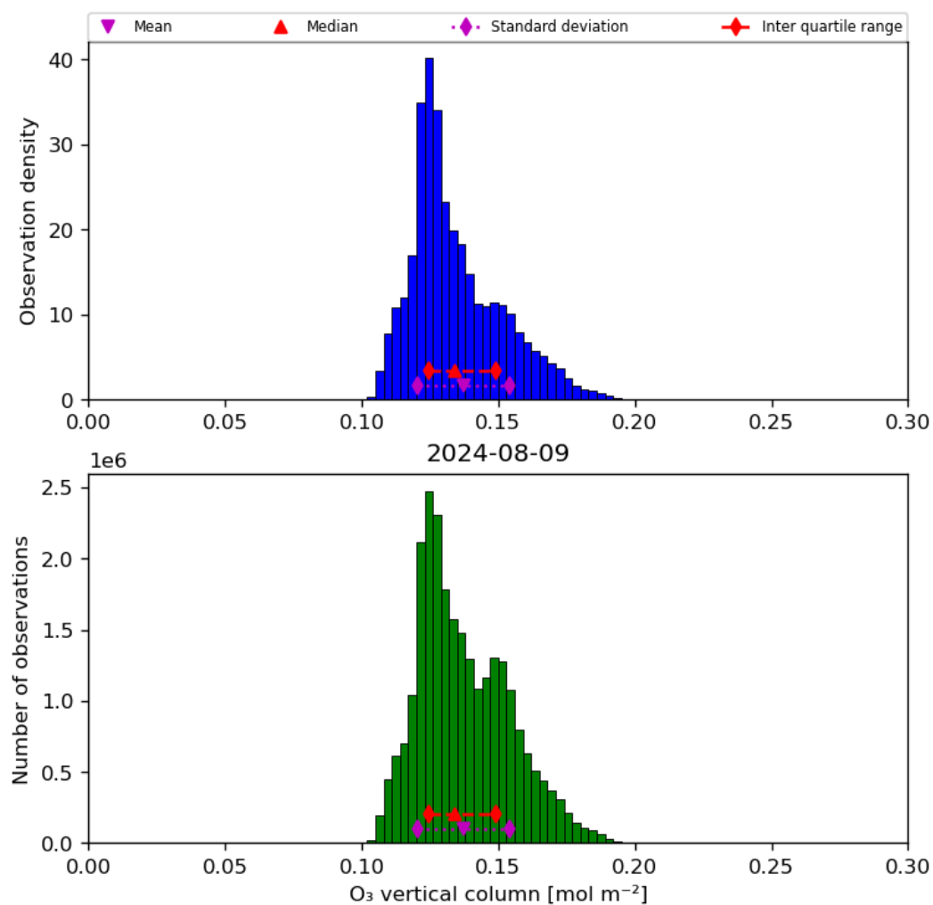
Figure 21: Histogram of “O 3 vertical column” for 2024-08-08 to 2024-08-10
