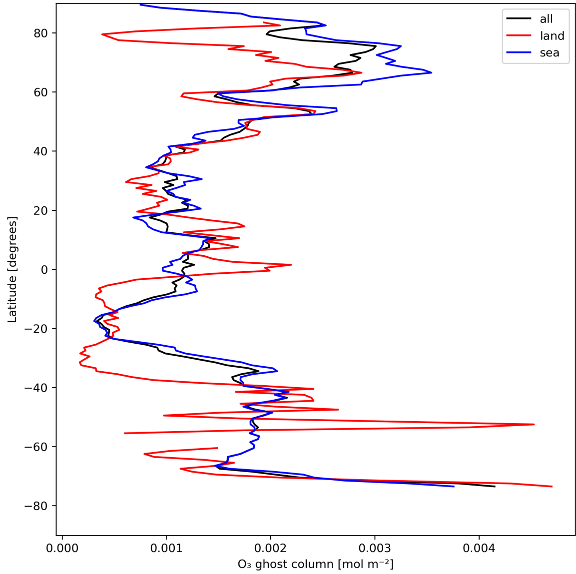
Figure 18: Zonal average of "O 3 ghost column" for 2024-08-08 to 2024-08-10.
