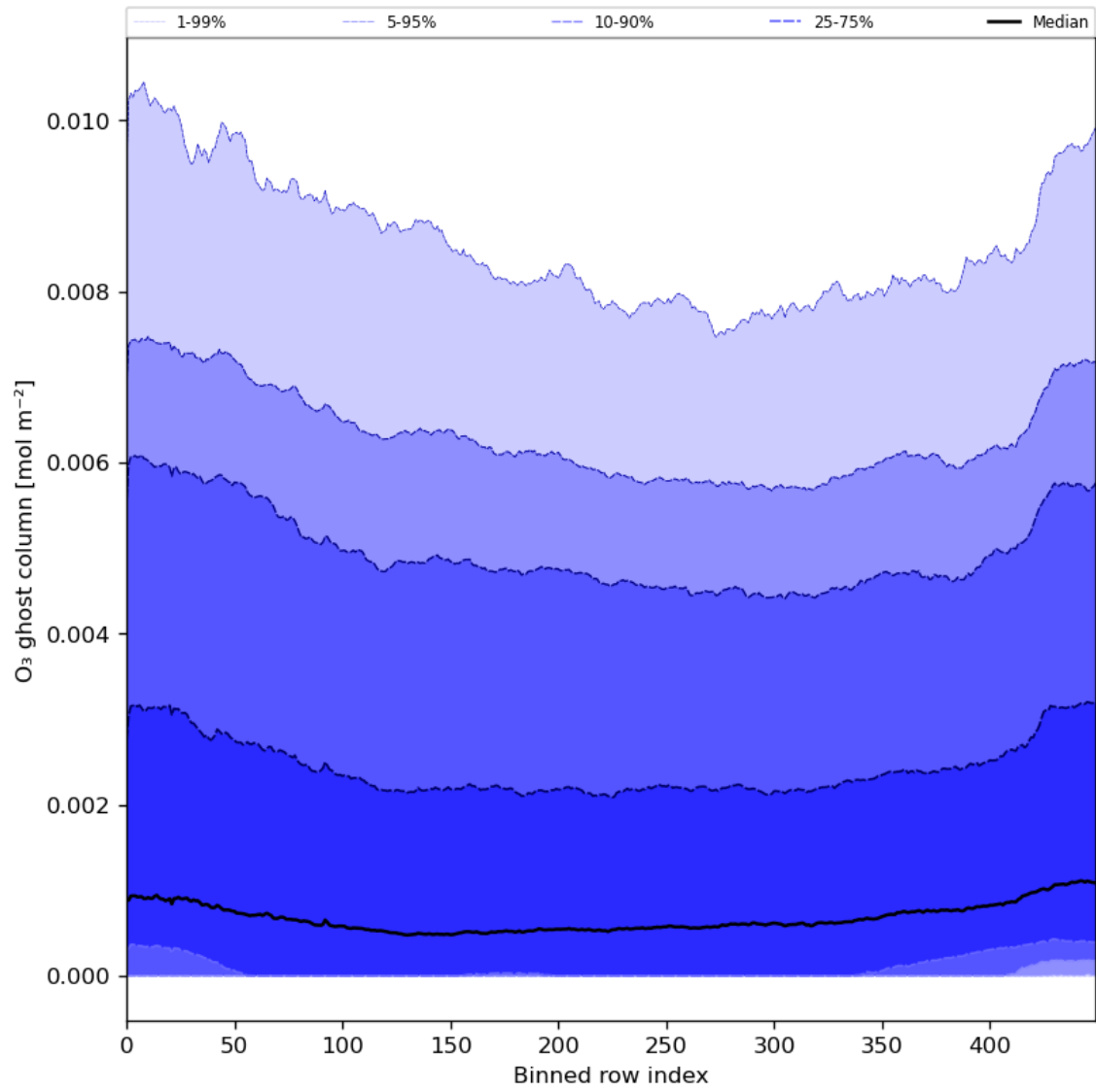
Figure 32: Along track statistics of "O 3 ghost column" for 2024-08-08 to 2024-08-10
