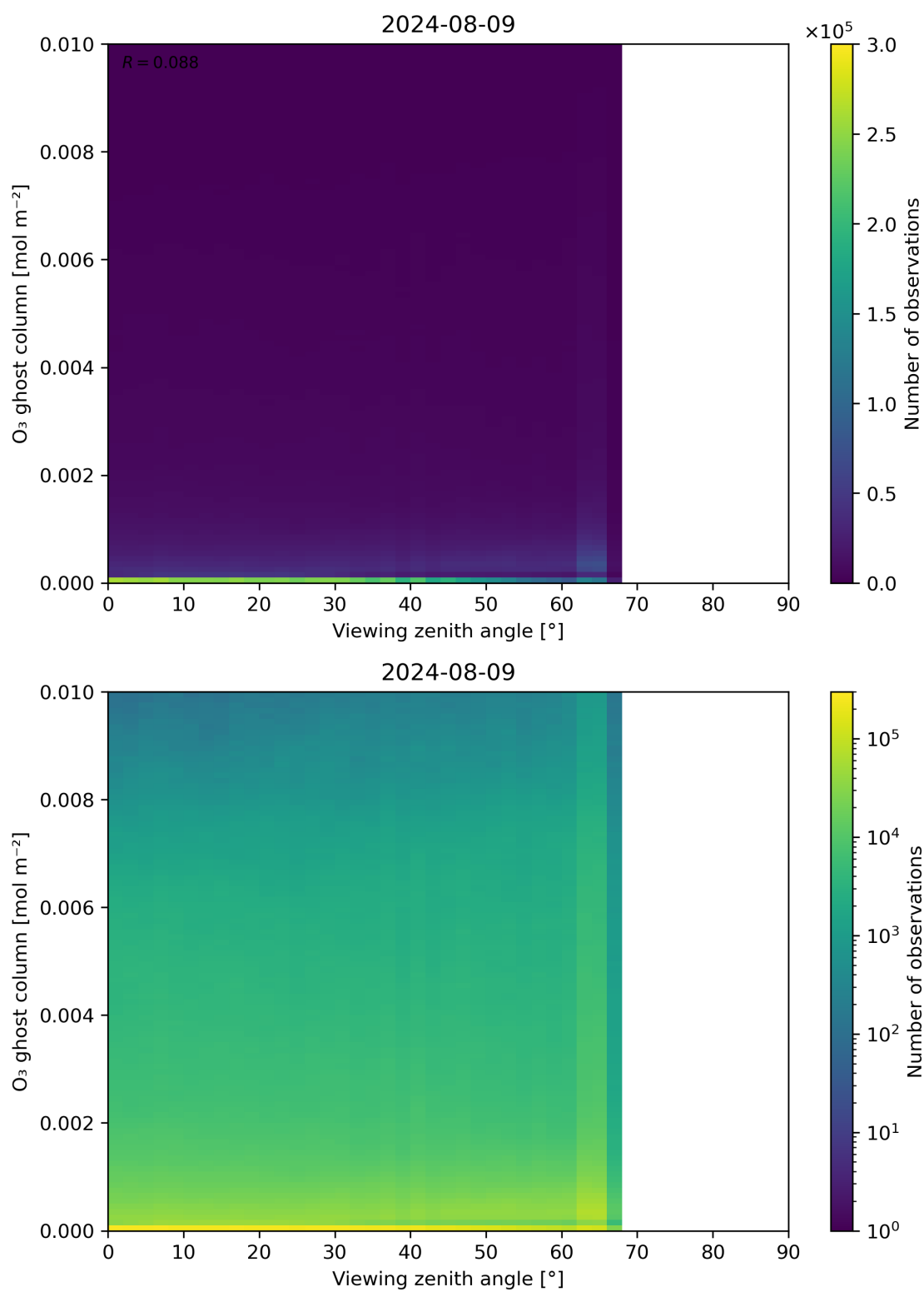
Figure 51: Scatter density plot of “Viewing zenith angle” against “O 3 ghost column” for 2024-08-08 to 2024-08-10.
