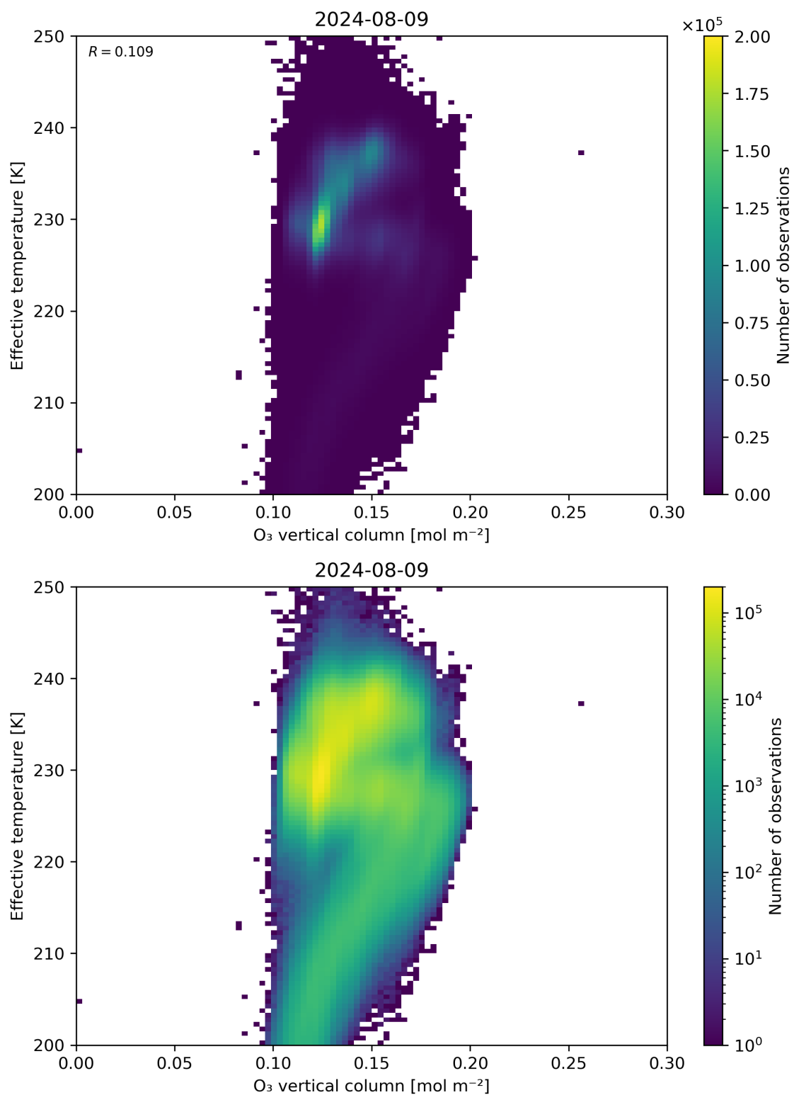
Figure 39: Scatter density plot of “O 3 vertical column” against “Effective temperature” for 2024-08-08 to 2024-08-10.
