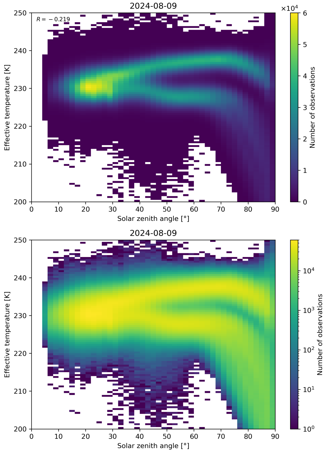
Figure 45: Scatter density plot of “Solar zenith angle” against “Effective temperature” for 2024-08-08 to 2024-08-10.
