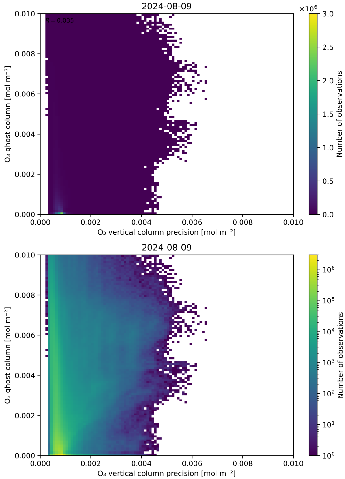
Figure 43: Scatter density plot of “ \text{O}_3 vertical column precision” against “ \text{O}_3 ghost column” for 2024-08-08 to 2024-08-10.
