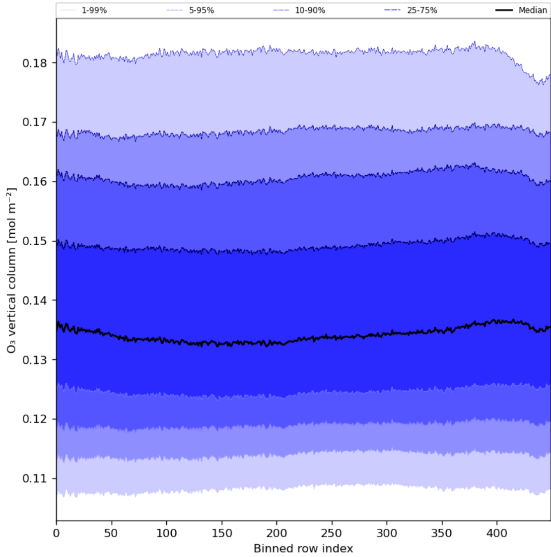
Figure 28: Along track statistics of “O 3 vertical column” for 2024-08-08 to 2024-08-10
