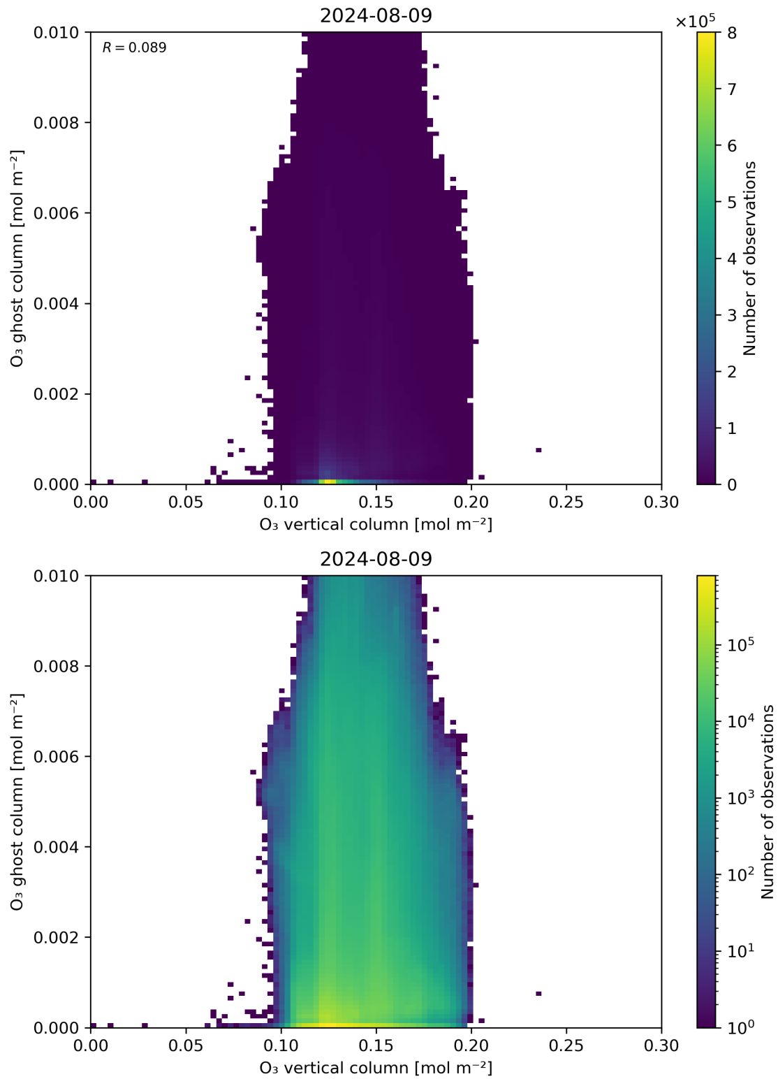
Figure 40: Scatter density plot of “O 3 vertical column” against “O 3 ghost column” for 2024-08-08 to 2024-08-10.
