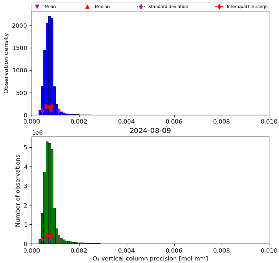
Figure 22: Histogram of “O 3 vertical column precision” for 2024-08-08 to 2024-08-10
