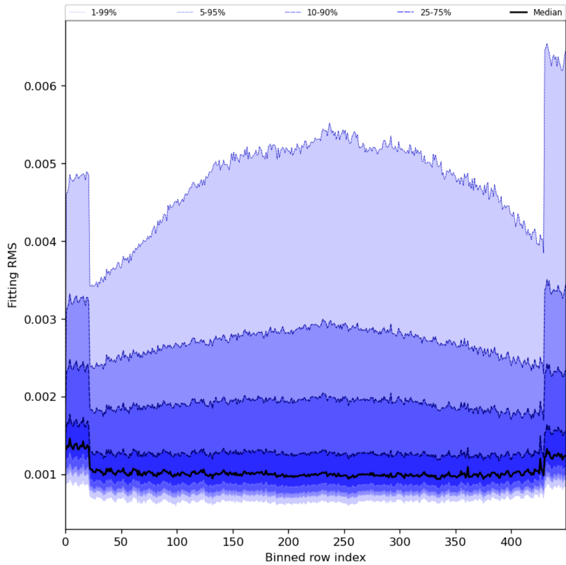
Figure 30: Along track statistics of “Fitting RMS” for 2024-08-08 to 2024-08-10
