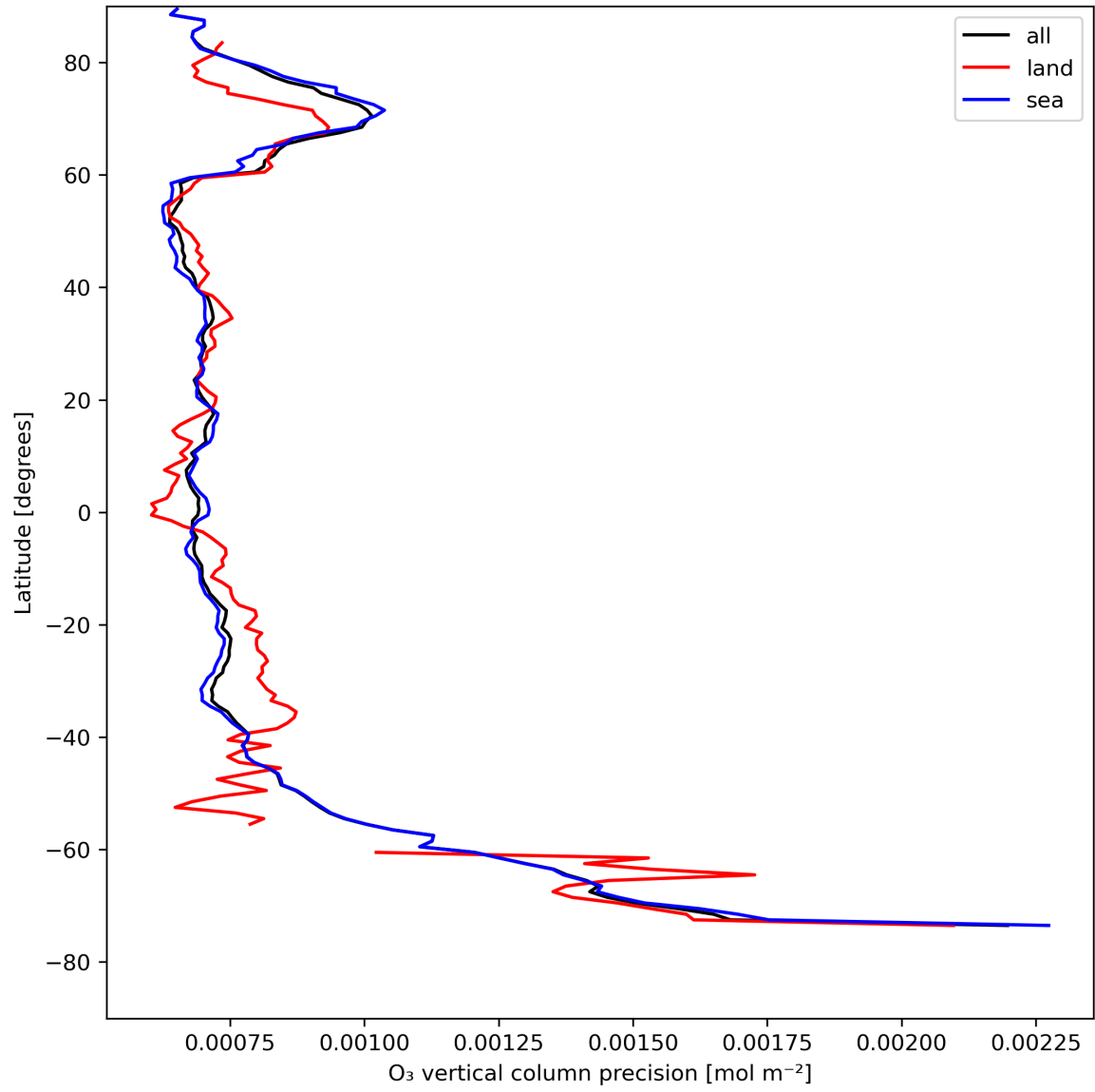
Figure 15: Zonal average of “O 3 vertical column precision” for 2024-08-08 to 2024-08-10.
