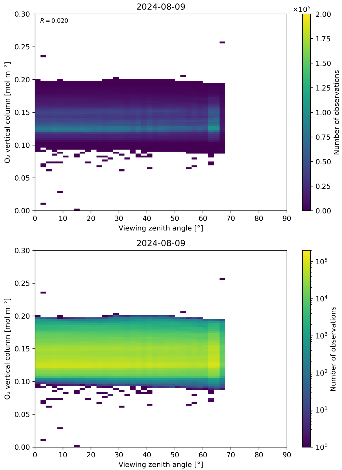
Figure 52: Scatter density plot of “Viewing zenith angle” against “O 3 vertical column” for 2024-08-08 to 2024-08-10.
