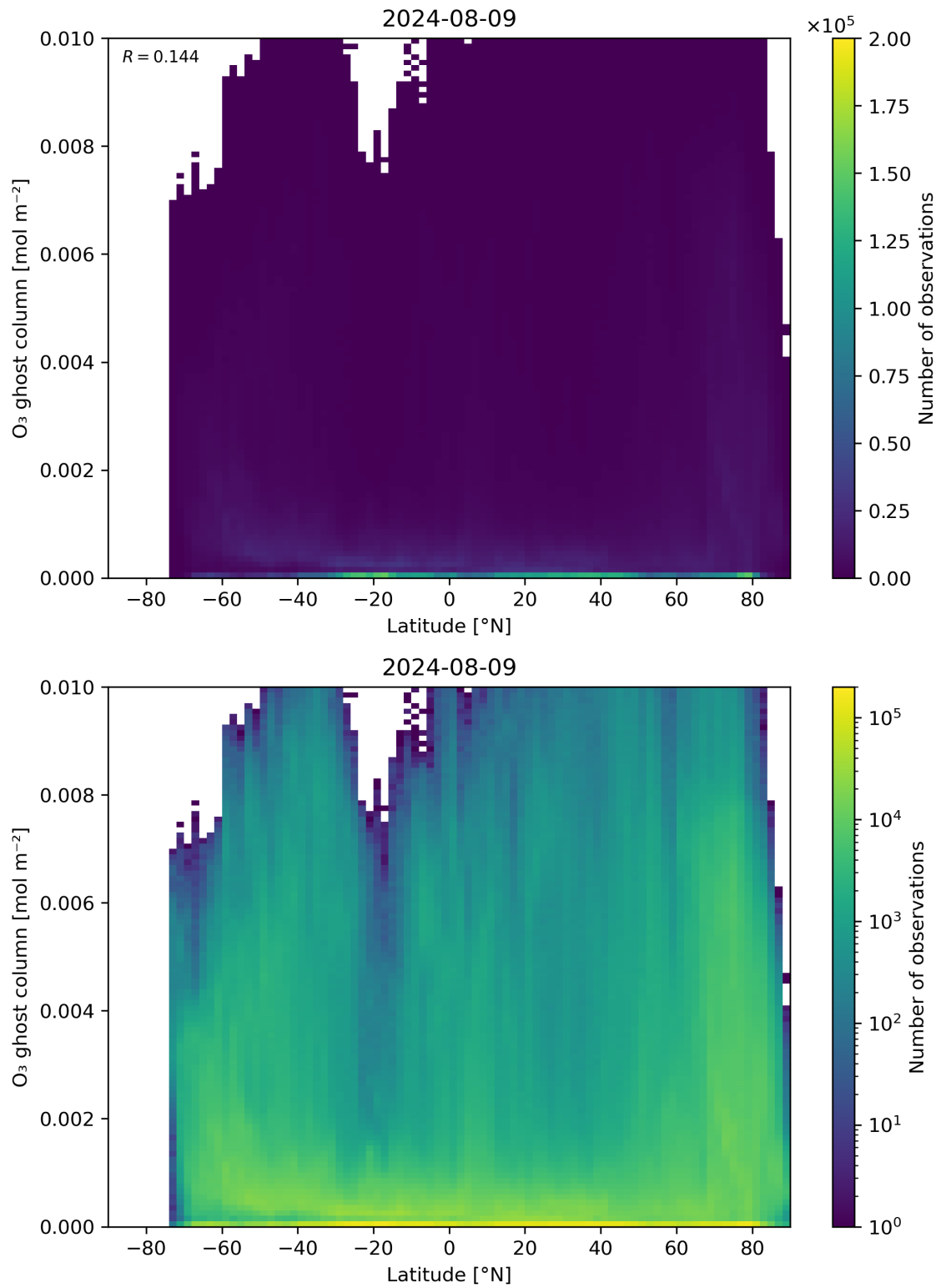
Figure 35: Scatter density plot of “Latitude” against “O 3 ghost column” for 2024-08-08 to 2024-08-10.
