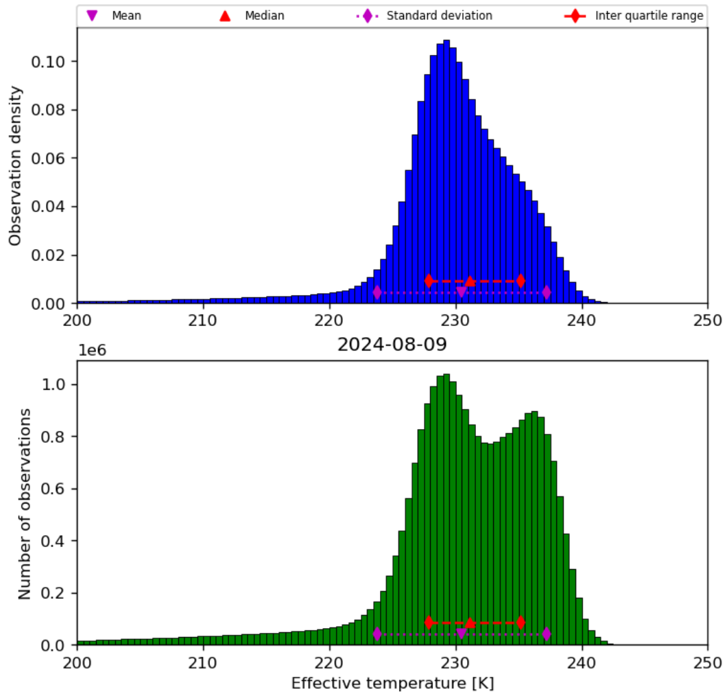
Figure 24: Histogram of “Effective temperature” for 2024-08-08 to 2024-08-10
