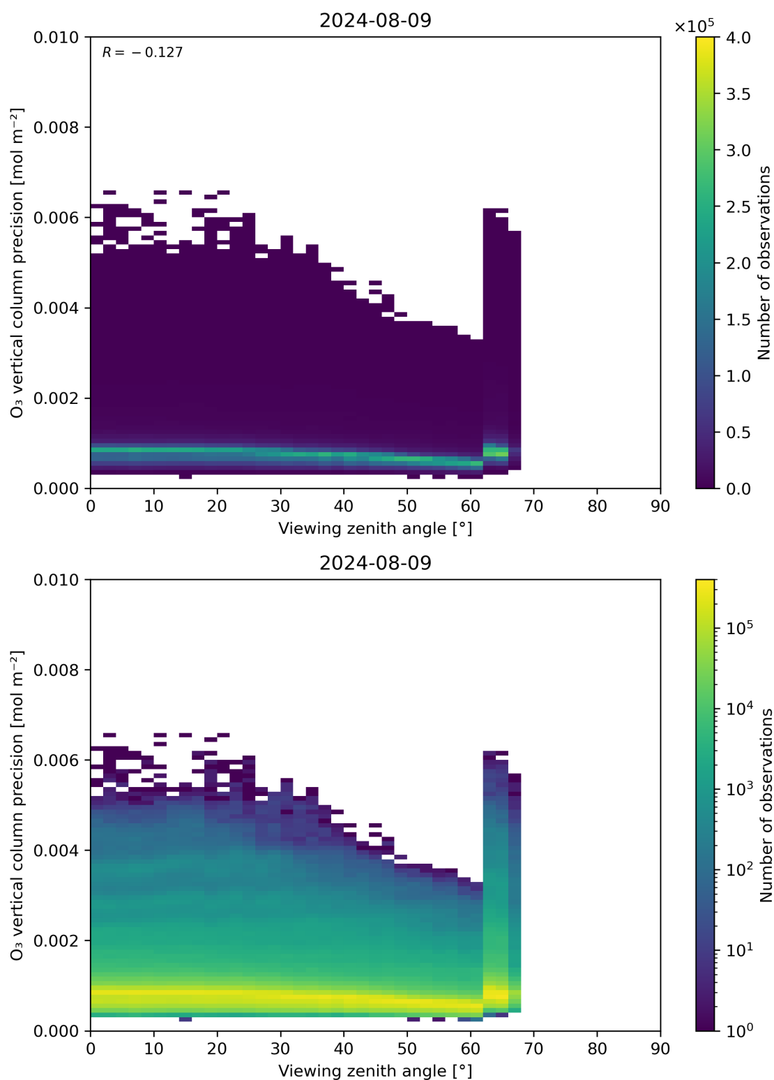
Figure 53: Scatter density plot of “Viewing zenith angle” against “O 3 vertical column precision” for 2024-08-08 to 2024-08-10.
