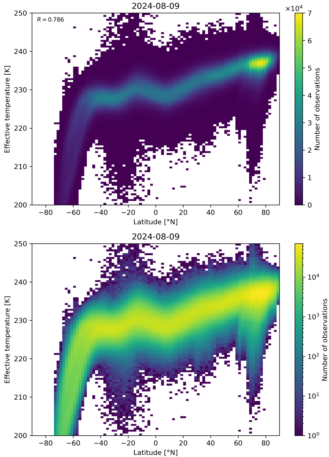
Figure 34: Scatter density plot of “Latitude” against “Effective temperature” for 2024-08-08 to 2024-08-10.
