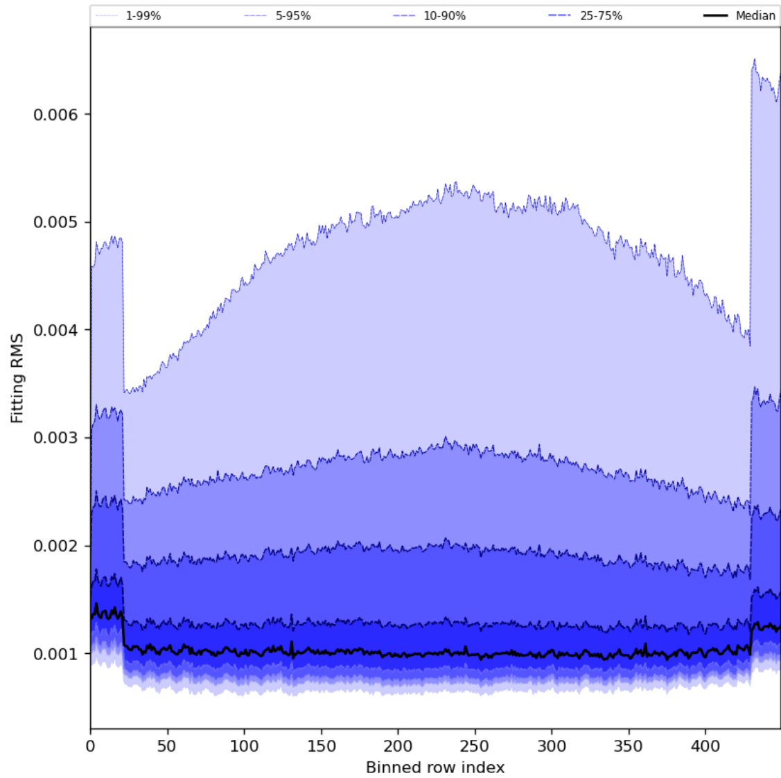
Figure 30: Along track statistics of “Fitting RMS” for 2024-08-09 to 2024-08-11
