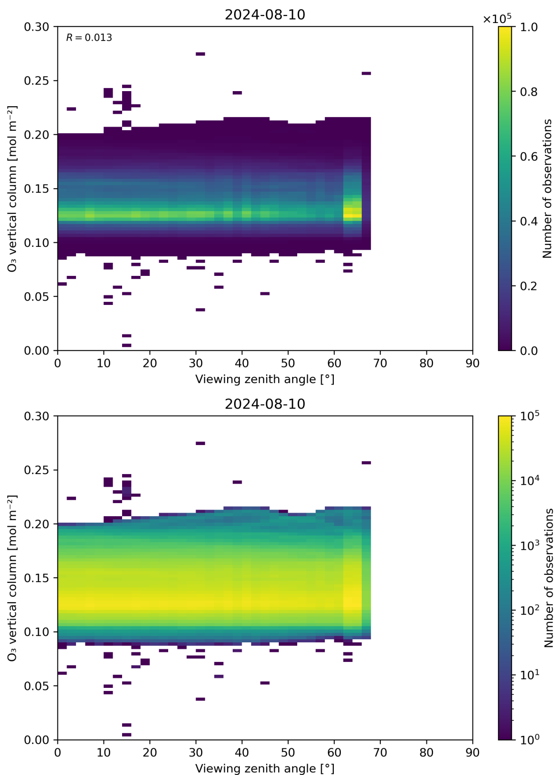
Figure 52: Scatter density plot of “Viewing zenith angle” against “O 3 vertical column” for 2024-08-09 to 2024-08-11.
