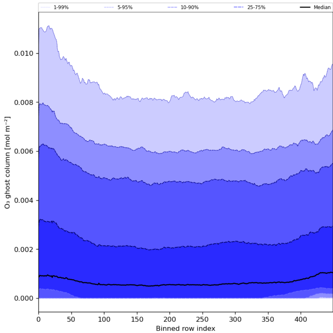
Figure 32: Along track statistics of “O 3 ghost column” for 2024-08-09 to 2024-08-11
