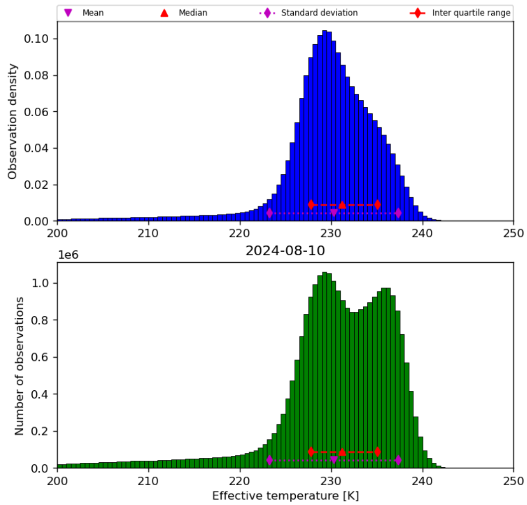
Figure 24: Histogram of “Effective temperature” for 2024-08-09 to 2024-08-11
