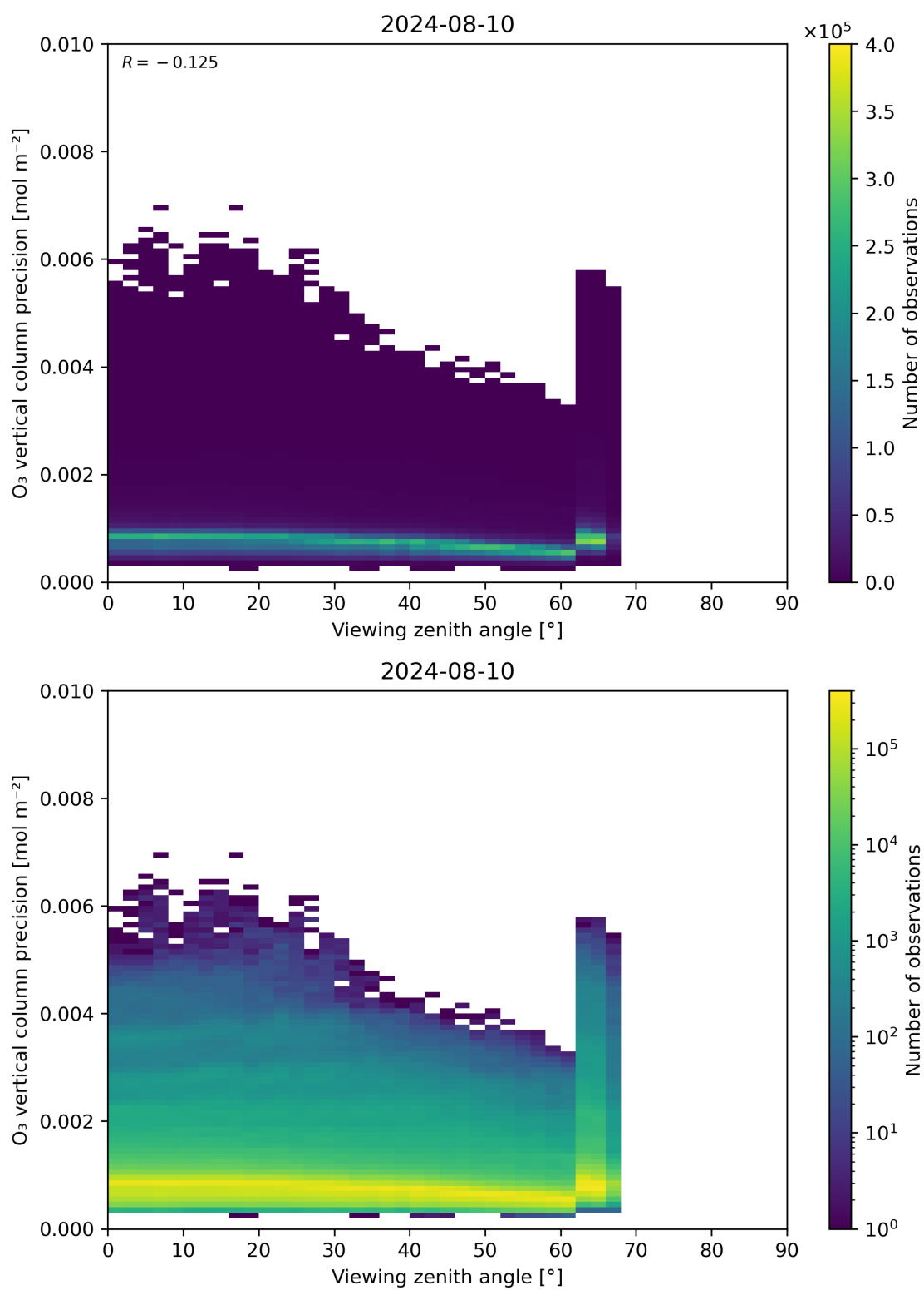
Figure 53: Scatter density plot of “Viewing zenith angle” against “O 3 vertical column precision” for 2024-08-09 to 2024-08-11.
