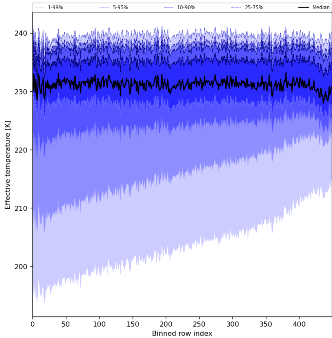
Figure 31: Along track statistics of “Effective temperature” for 2024-08-09 to 2024-08-11
