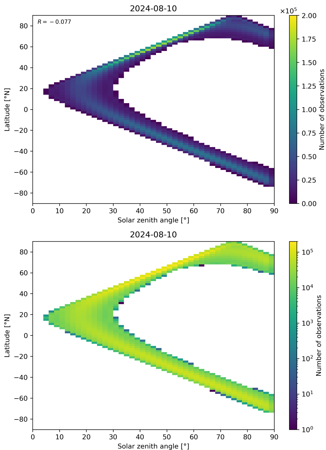
Figure 44: Scatter density plot of “Solar zenith angle” against “Latitude” for 2024-08-09 to 2024-08-11.
