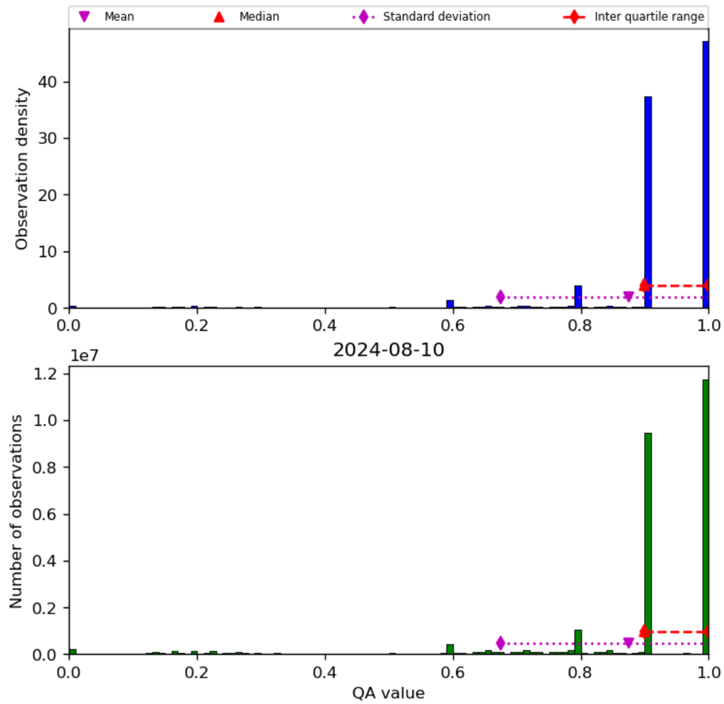
Figure 20: Histogram of “QA value” for 2024-08-09 to 2024-08-11
