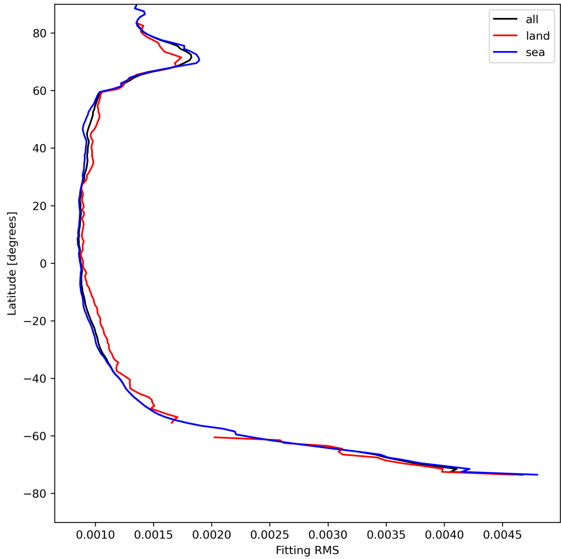
Figure 16: Zonal average of “Fitting RMS” for 2024-08-09 to 2024-08-11.
