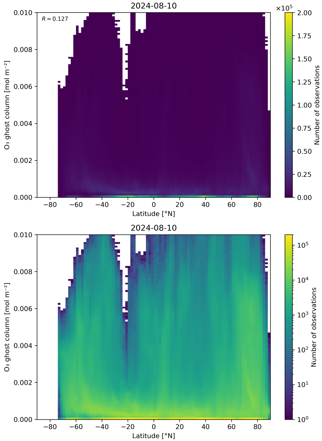
Figure 35: Scatter density plot of “Latitude” against “O 3 ghost column” for 2024-08-09 to 2024-08-11.
