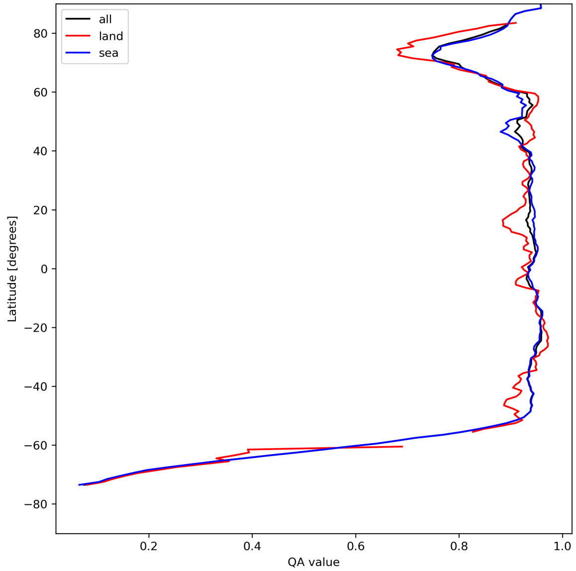
Figure 13: Zonal average of “QA value” for 2024-08-09 to 2024-08-11.
