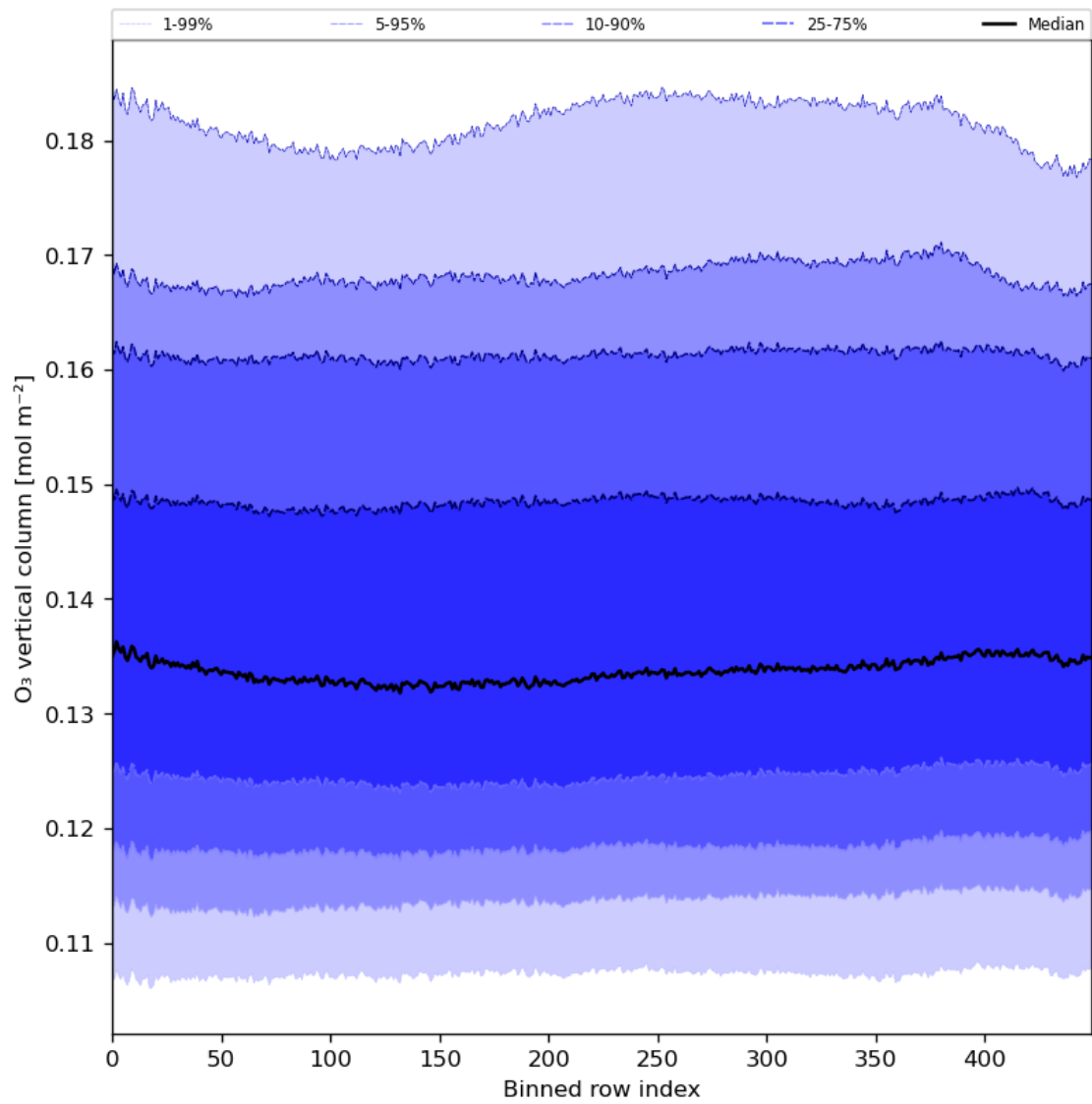
Figure 28: Along track statistics of “O 3 vertical column” for 2024-08-09 to 2024-08-11
