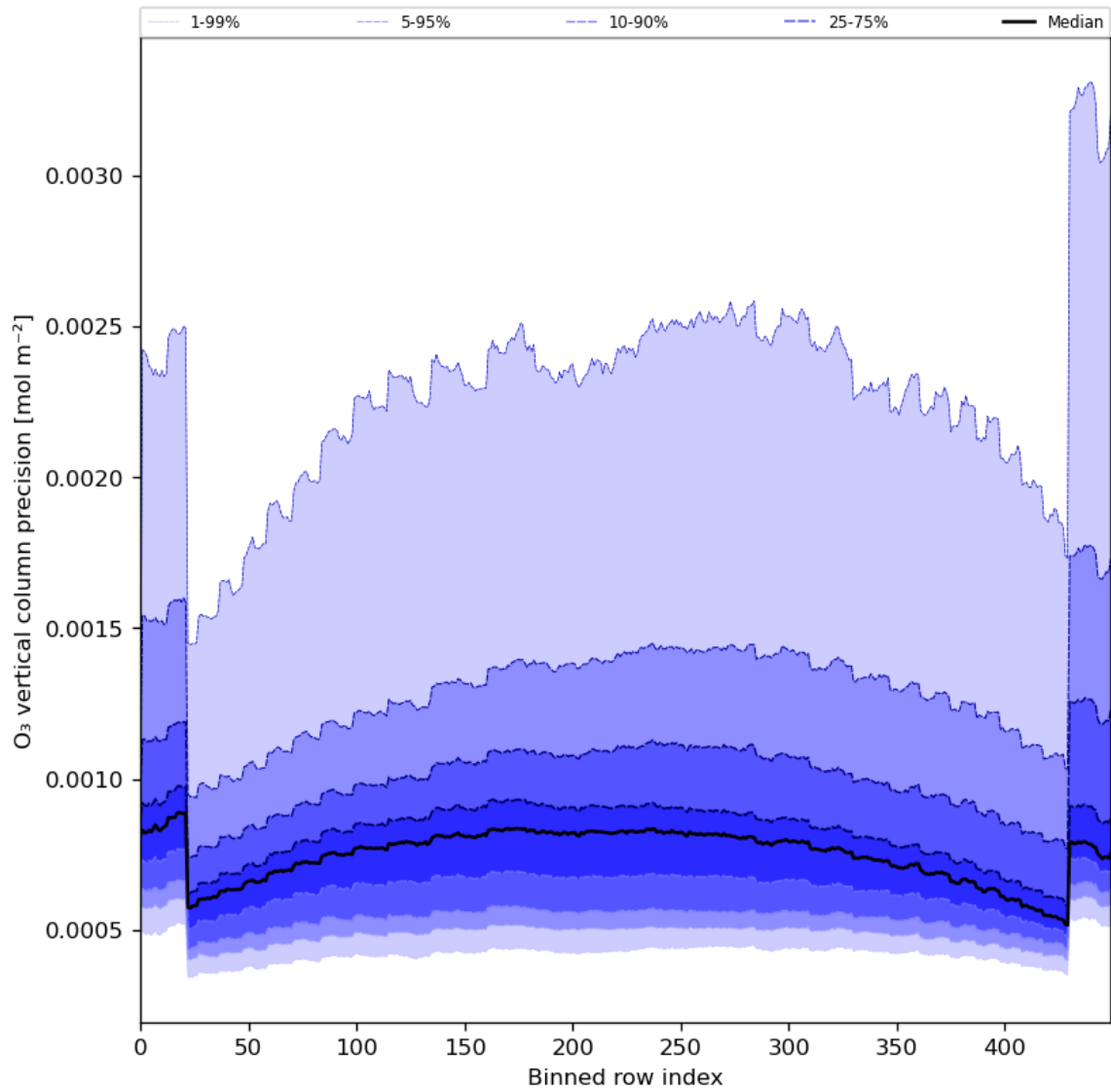
Figure 29: Along track statistics of “O 3 vertical column precision” for 2024-08-09 to 2024-08-11
