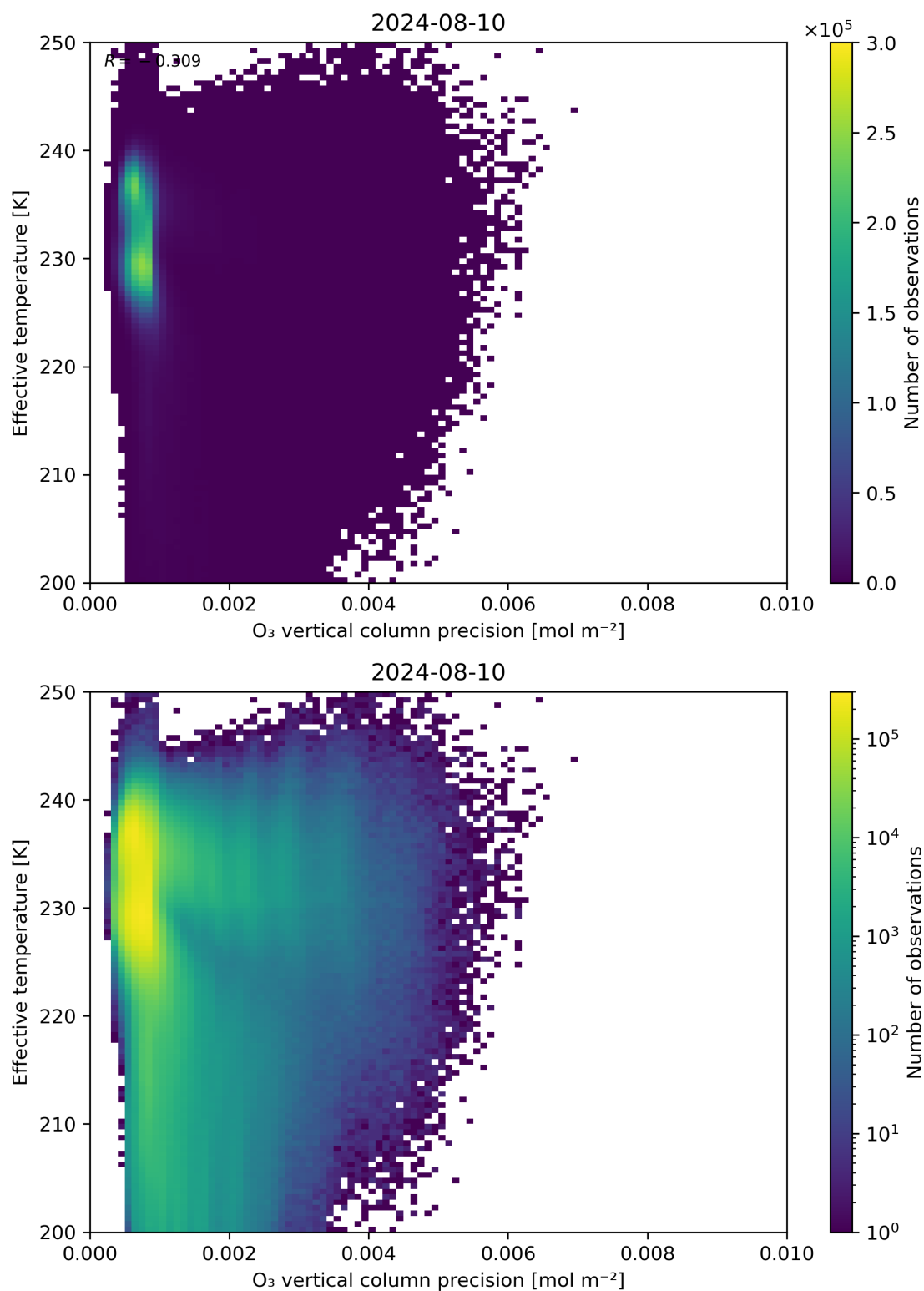
Figure 42: Scatter density plot of “O 3 vertical column precision” against “Effective temperature” for 2024-08-09 to 2024-08-11.
