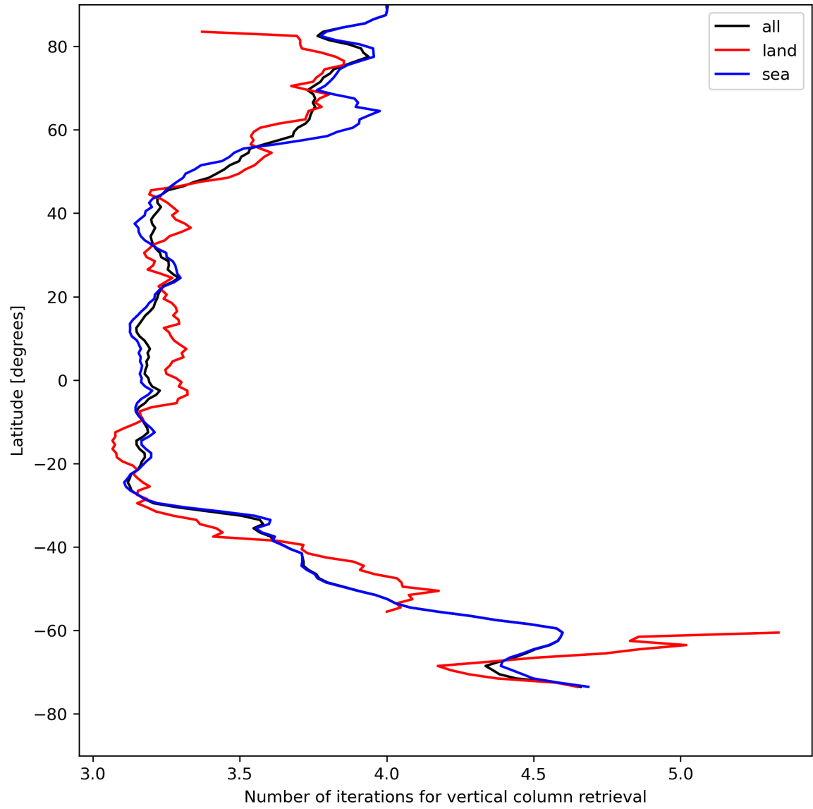
Figure 19: Zonal average of “Number of iterations for vertical column retrieval” for 2024-08-09 to 2024-08-11.
