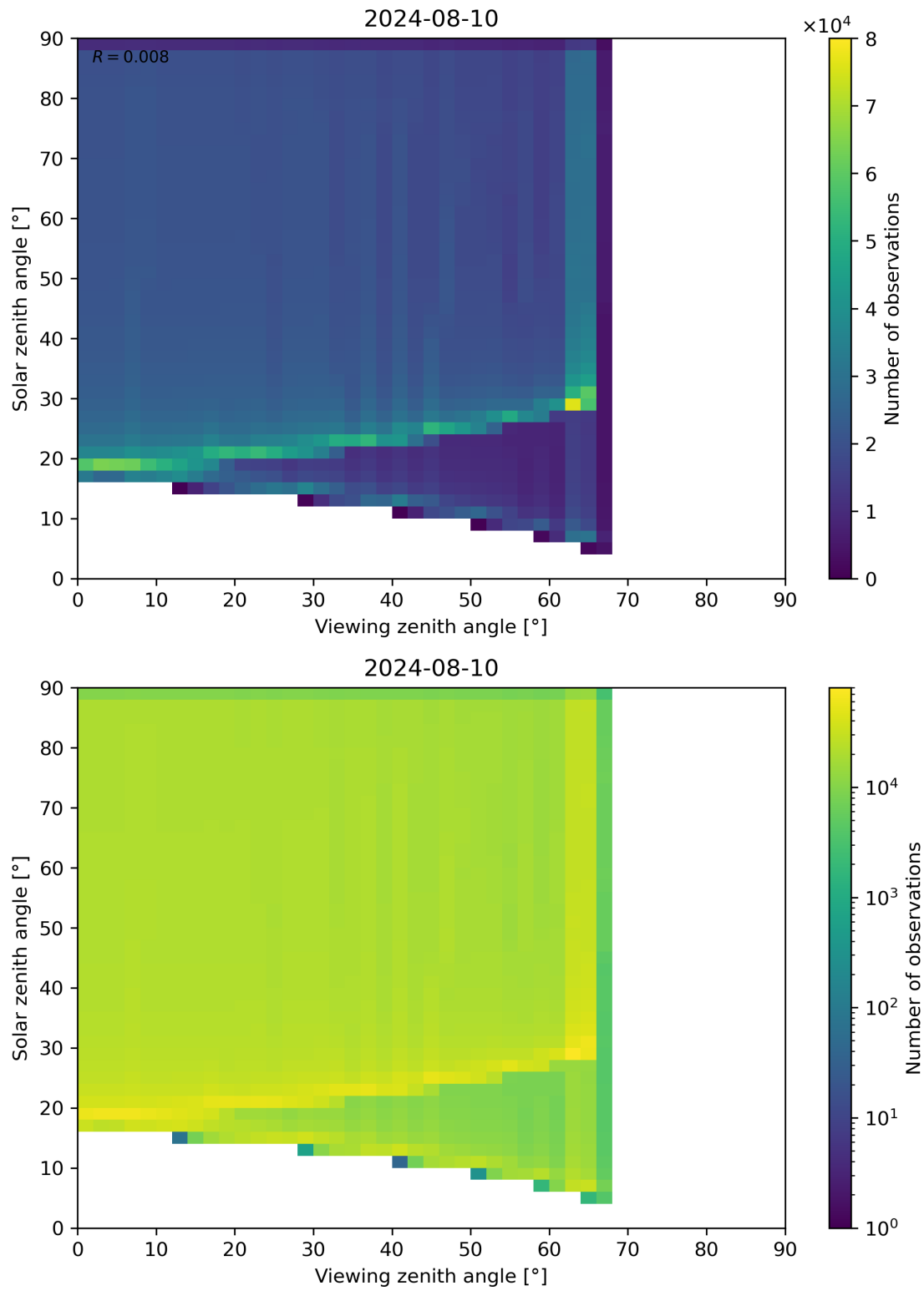
Figure 54: Scatter density plot of “Viewing zenith angle” against “Solar zenith angle” for 2024-08-09 to 2024-08-11.
