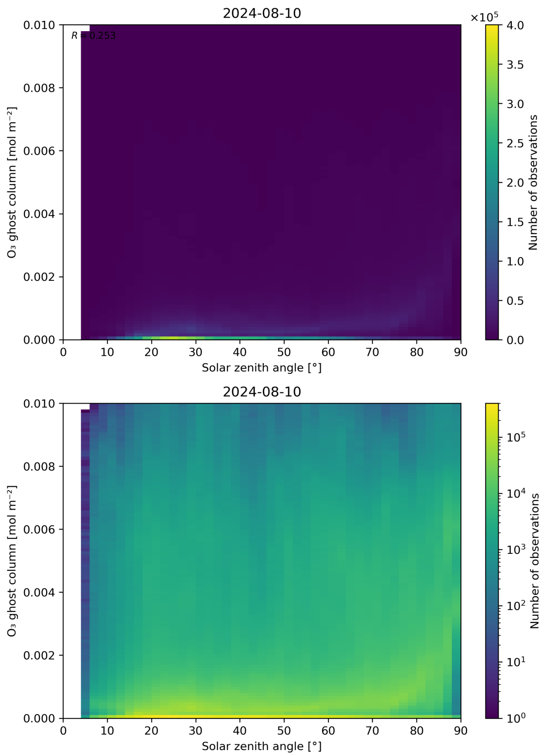
Figure 46: Scatter density plot of “Solar zenith angle” against “O 3 ghost column” for 2024-08-09 to 2024-08-11.
