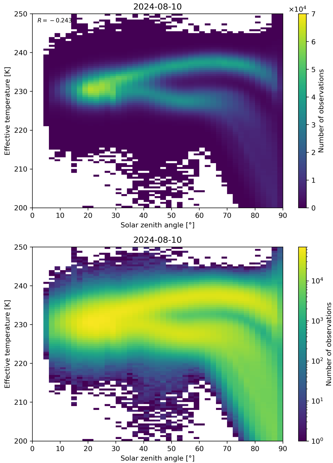
Figure 45: Scatter density plot of “Solar zenith angle” against “Effective temperature” for 2024-08-09 to 2024-08-11.
