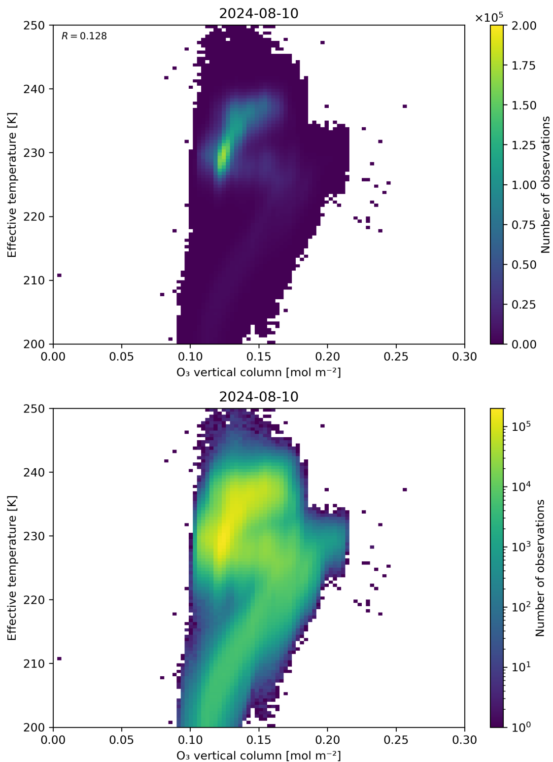
Figure 39: Scatter density plot of “O 3 vertical column” against “Effective temperature” for 2024-08-09 to 2024-08-11.
