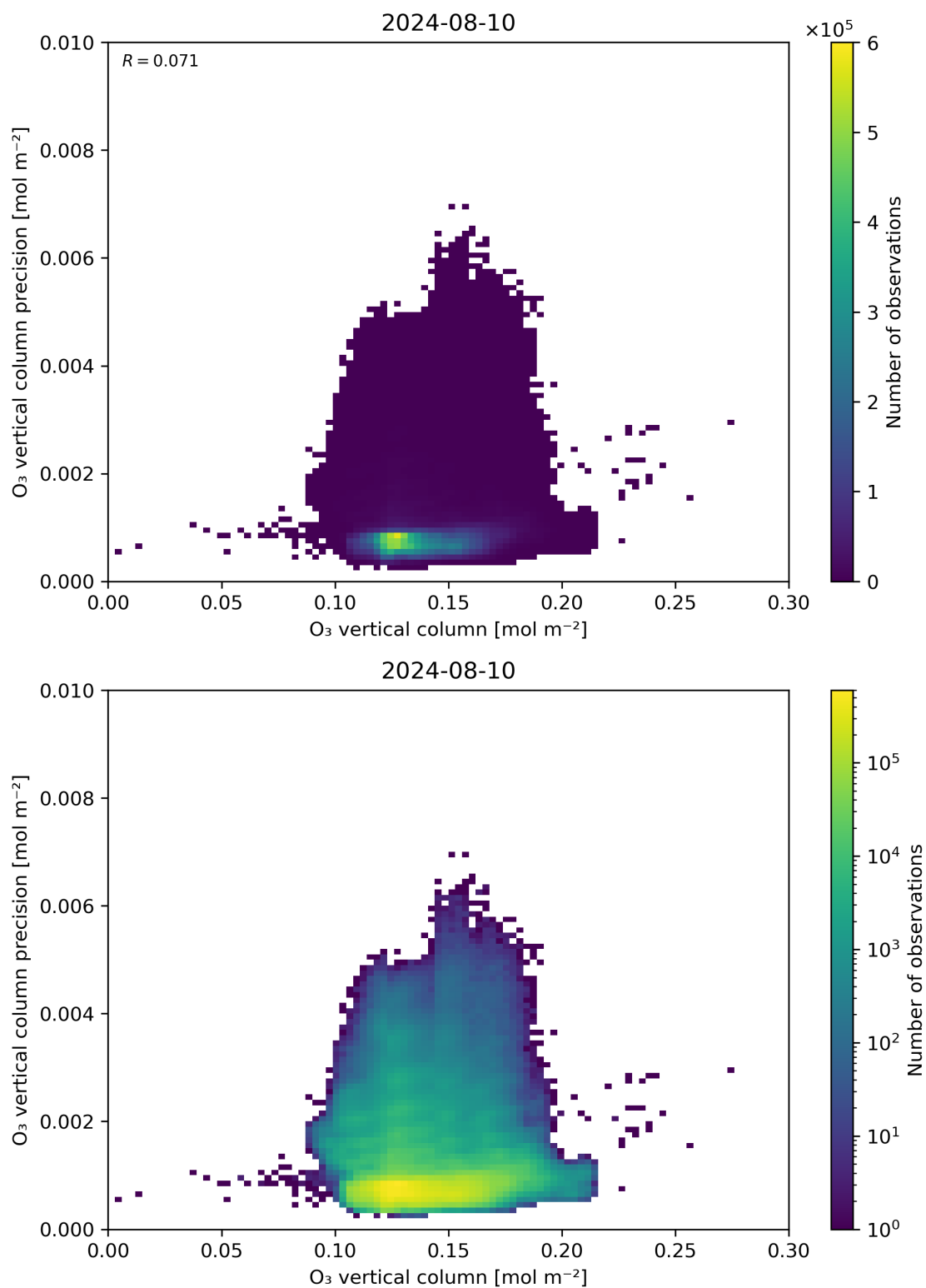
Figure 41: Scatter density plot of “O 3 vertical column” against “O 3 vertical column precision” for 2024-08-09 to 2024-08-11.
