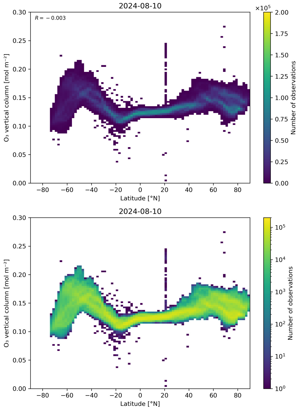
Figure 36: Scatter density plot of “Latitude” against “O 3 vertical column” for 2024-08-09 to 2024-08-11.
