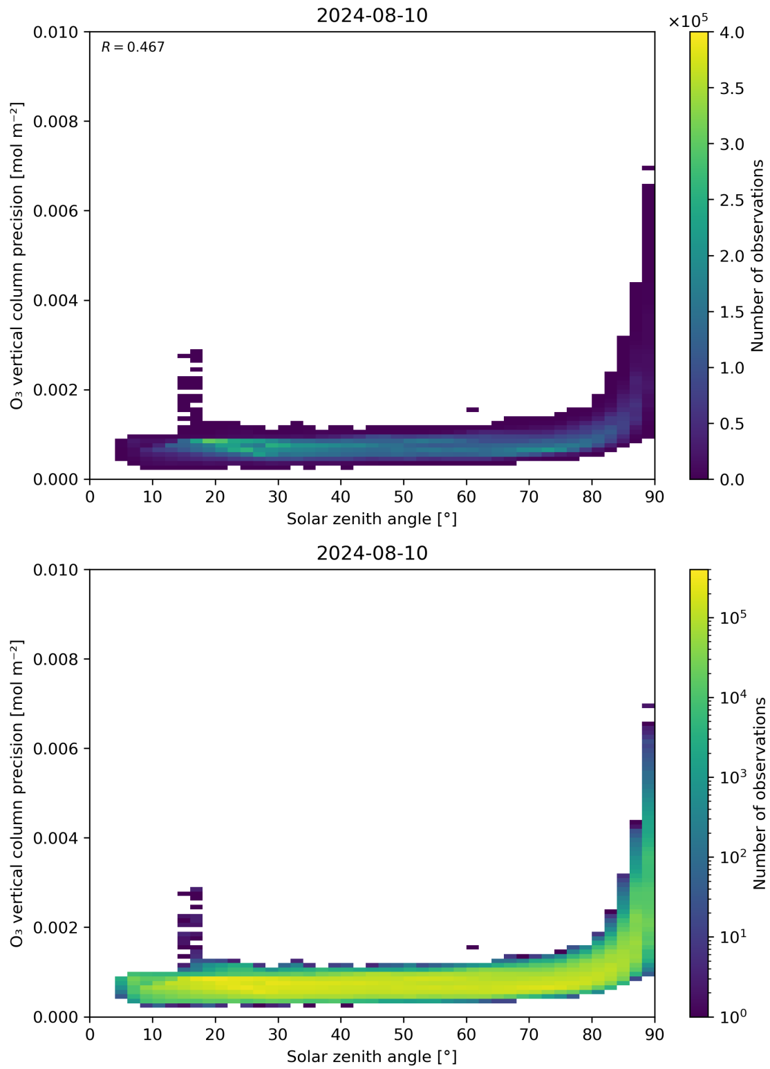
Figure 48: Scatter density plot of “Solar zenith angle” against “O 3 vertical column precision” for 2024-08-09 to 2024-08-11.
