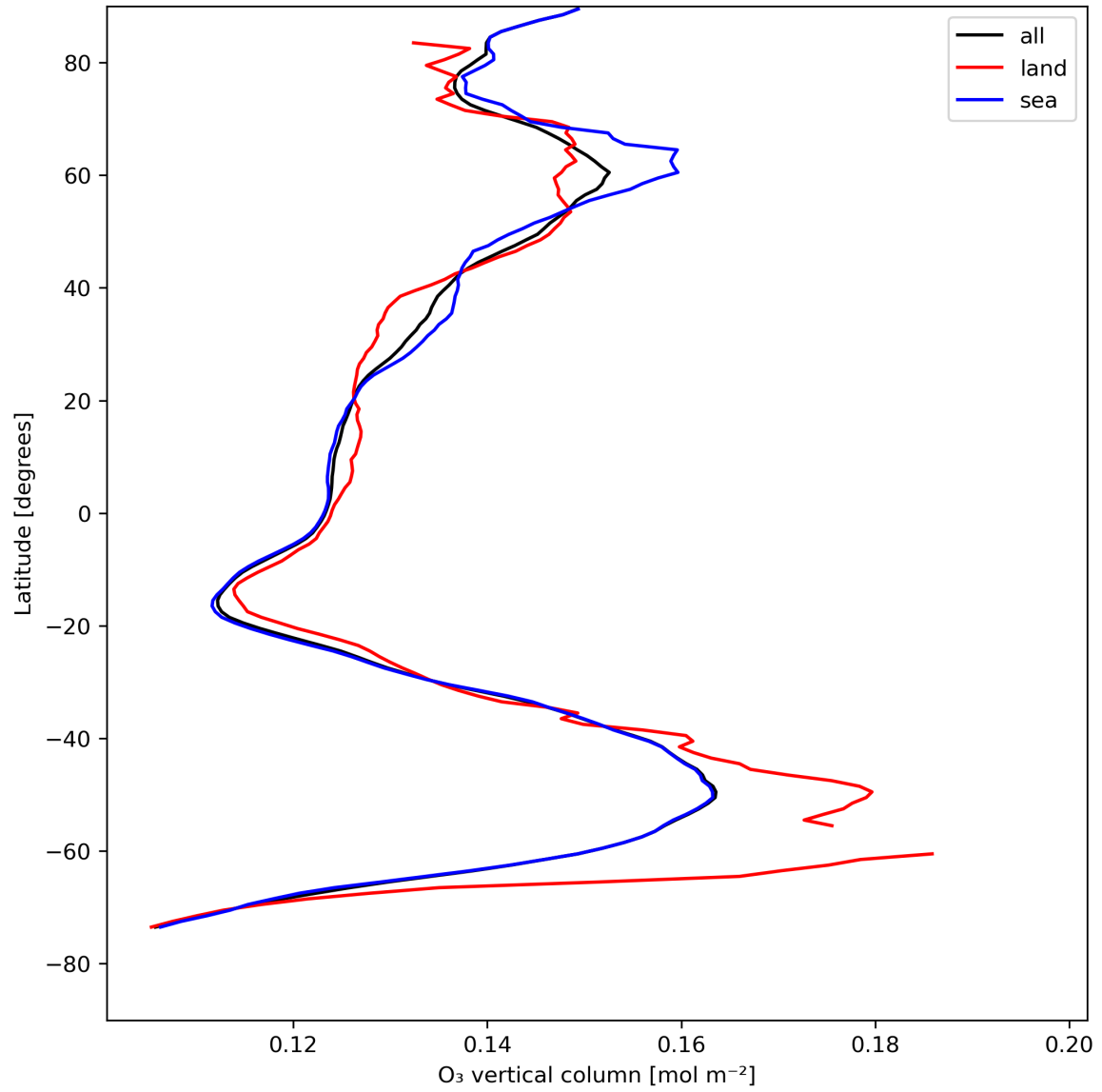
Figure 14: Zonal average of “O 3 vertical column” for 2024-08-09 to 2024-08-11.
