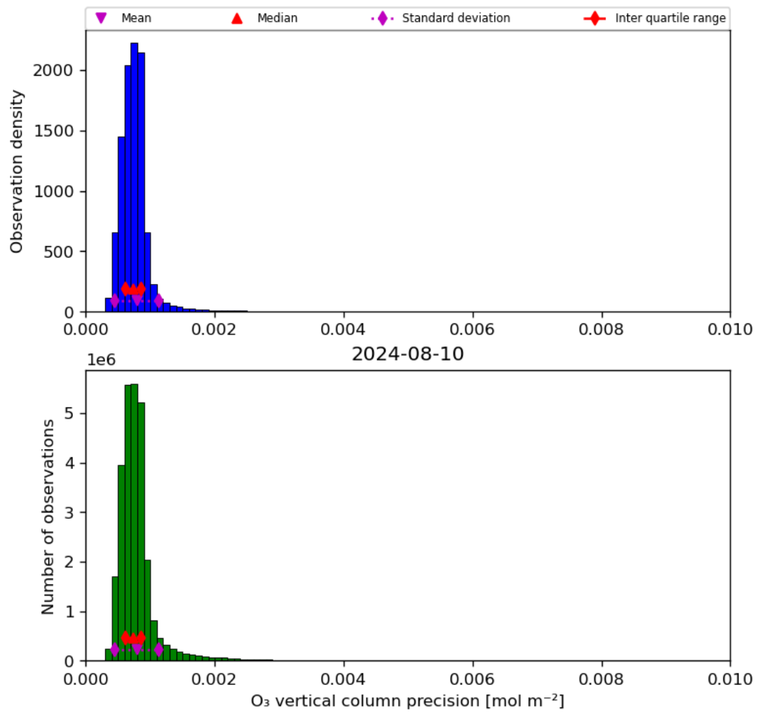
Figure 22: Histogram of “O 3 vertical column precision” for 2024-08-09 to 2024-08-11
