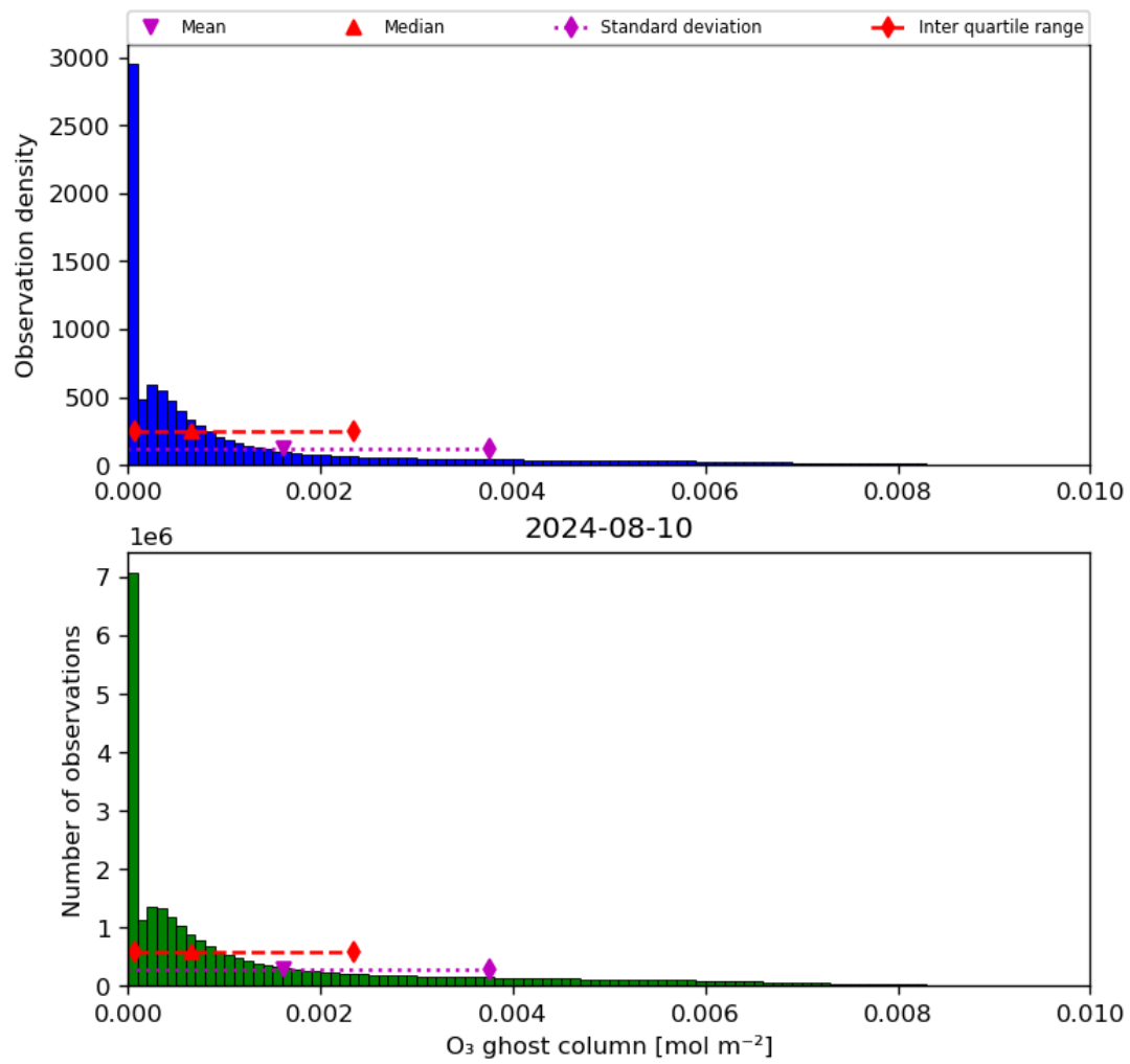
Figure 25: Histogram of “O 3 ghost column” for 2024-08-09 to 2024-08-11
