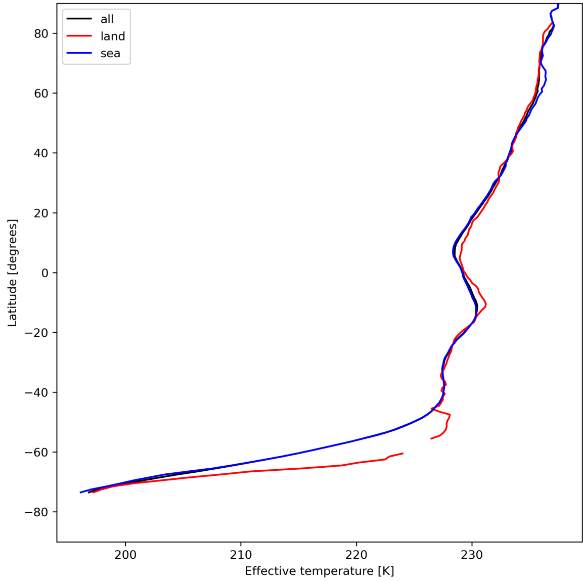
Figure 17: Zonal average of "Effective temperature" for 2024-08-09 to 2024-08-11.
