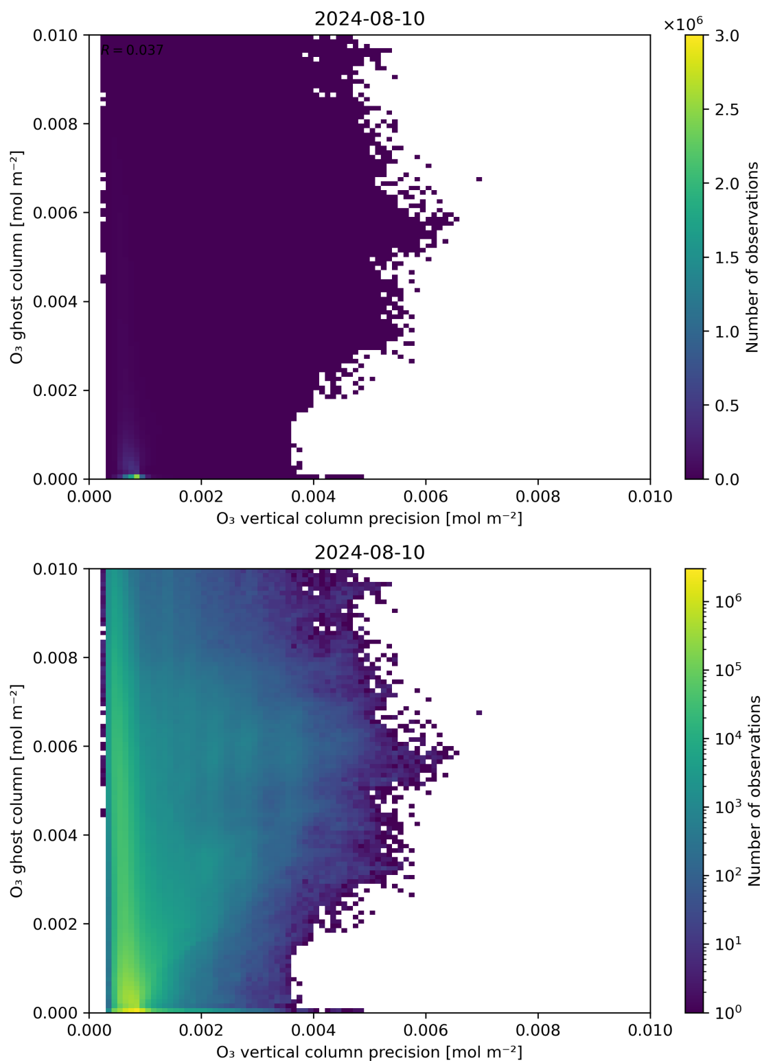
Figure 43: Scatter density plot of “ \text{O}_3 vertical column precision” against “ \text{O}_3 ghost column” for 2024-08-09 to 2024-08-11.
