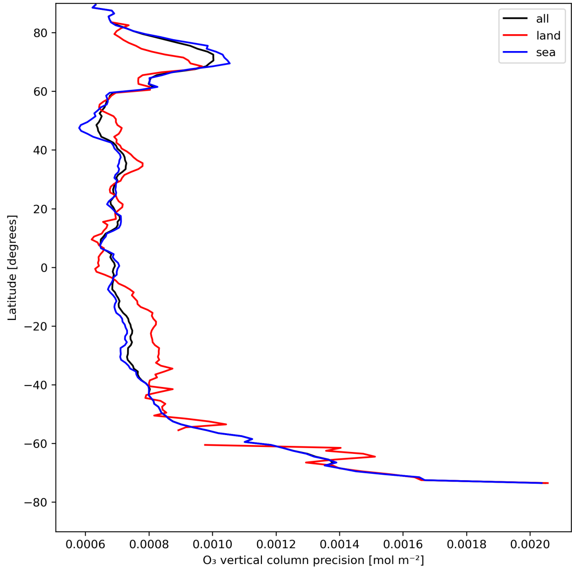
Figure 15: Zonal average of "O 3 vertical column precision" for 2024-08-09 to 2024-08-11.
