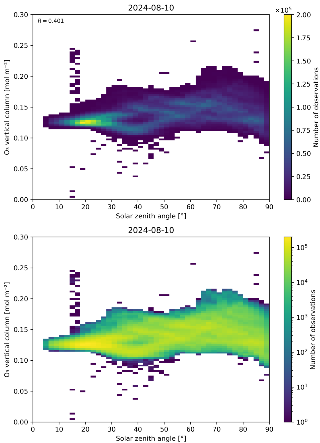
Figure 47: Scatter density plot of “Solar zenith angle” against “O 3 vertical column” for 2024-08-09 to 2024-08-11.
