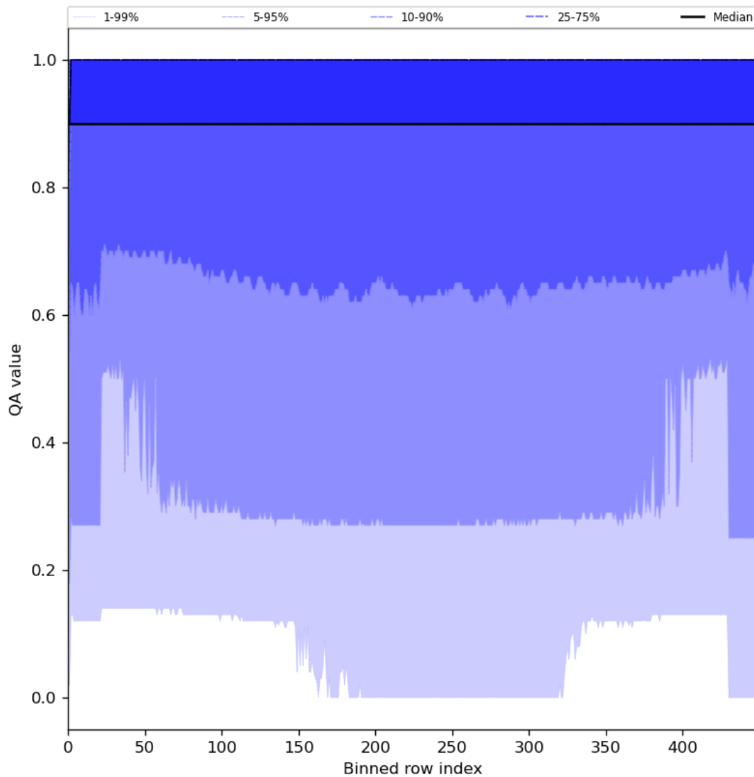
Figure 27: Along track statistics of “QA value” for 2024-08-09 to 2024-08-11
