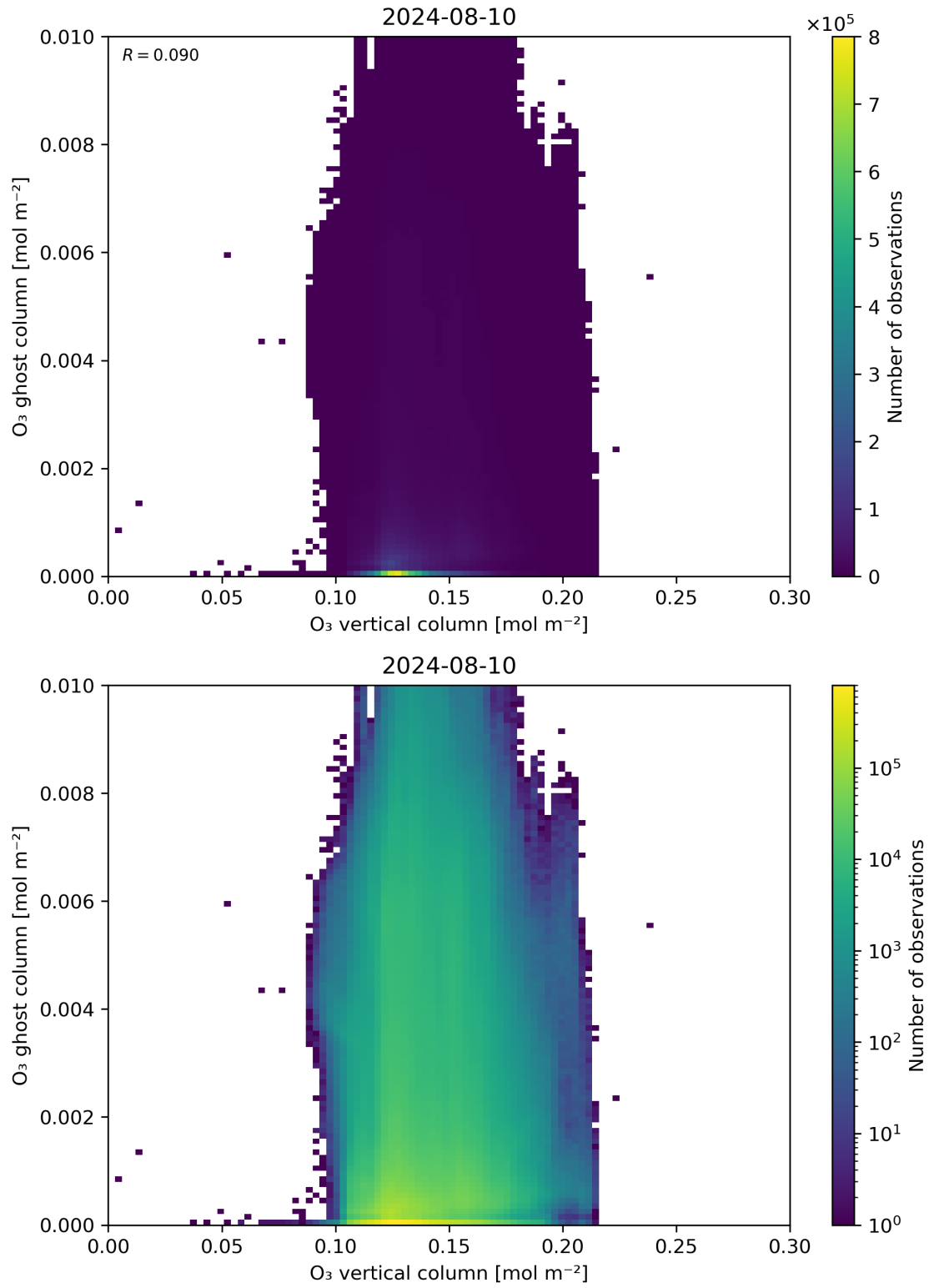
Figure 40: Scatter density plot of “O 3 vertical column” against “O 3 ghost column” for 2024-08-09 to 2024-08-11.
