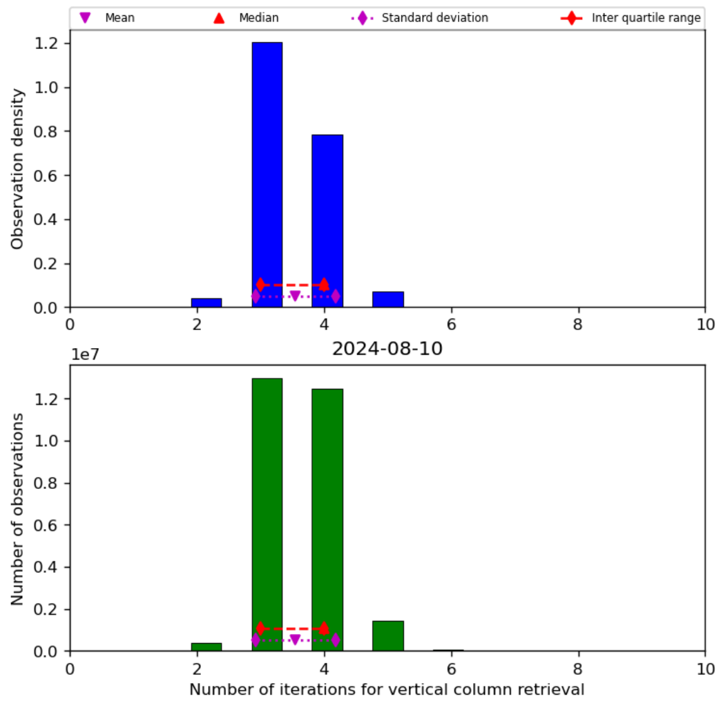
Figure 26: Histogram of “Number of iterations for vertical column retrieval” for 2024-08-09 to 2024-08-11
