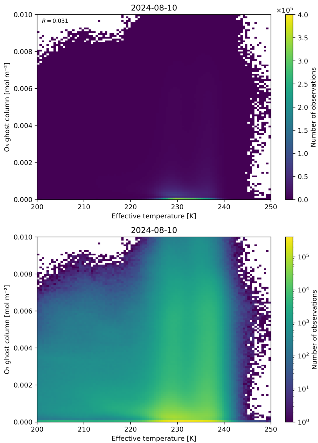
Figure 38: Scatter density plot of “Effective temperature” against “O 3 ghost column” for 2024-08-09 to 2024-08-11.
