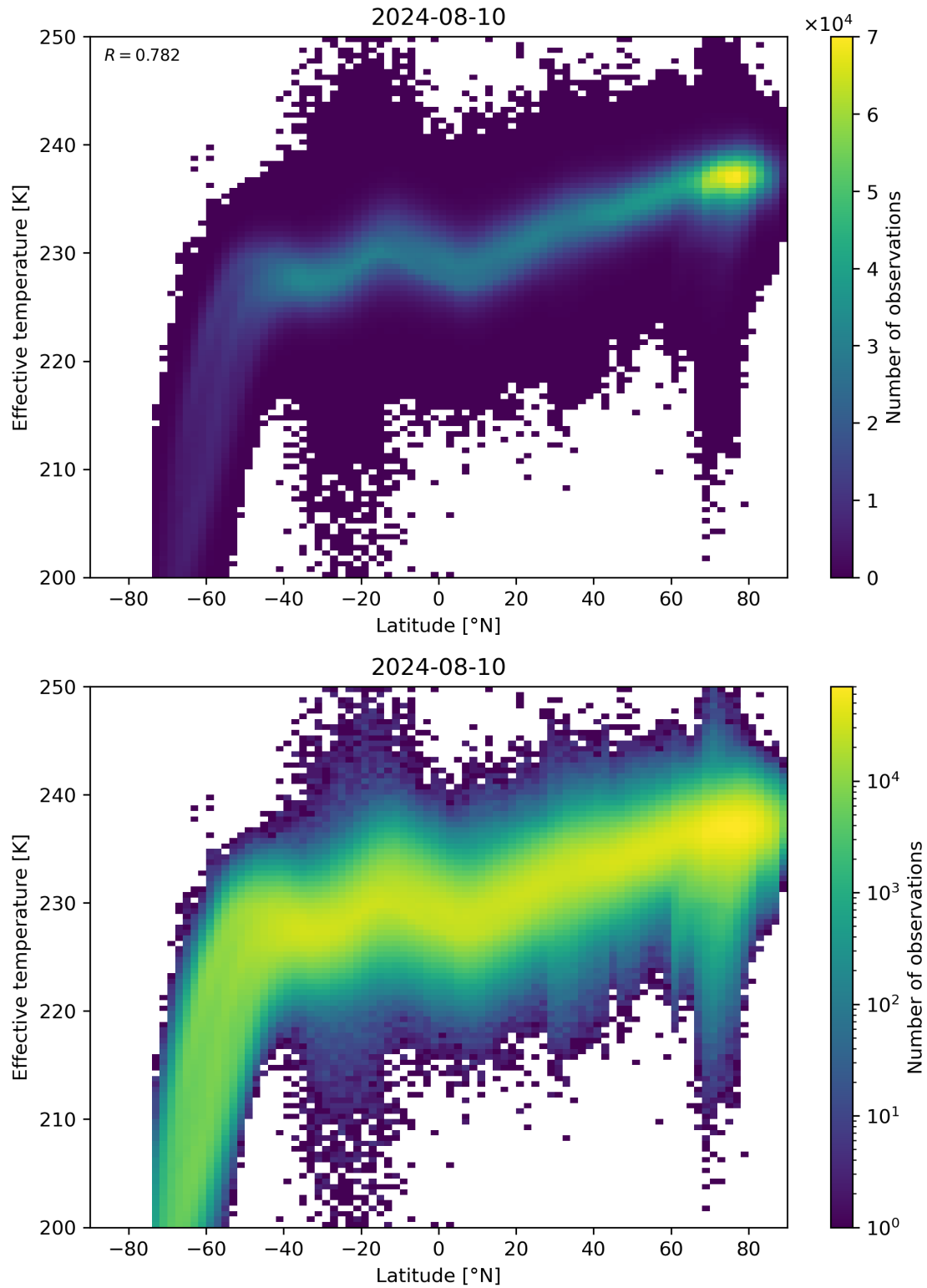
Figure 34: Scatter density plot of “Latitude” against “Effective temperature” for 2024-08-09 to 2024-08-11.
