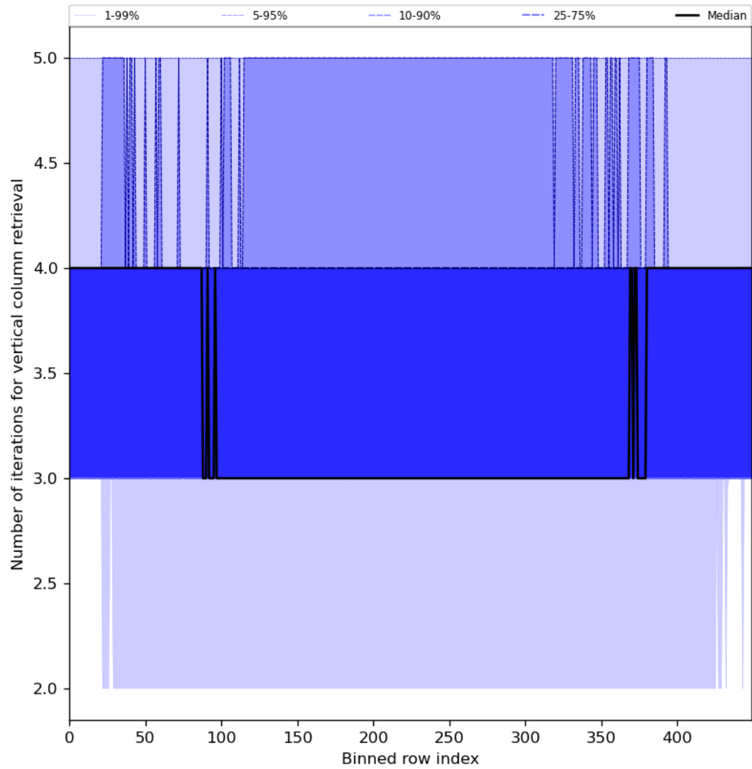
Figure 33: Along track statistics of “Number of iterations for vertical column retrieval” for 2024-08-09 to 2024-08-11
