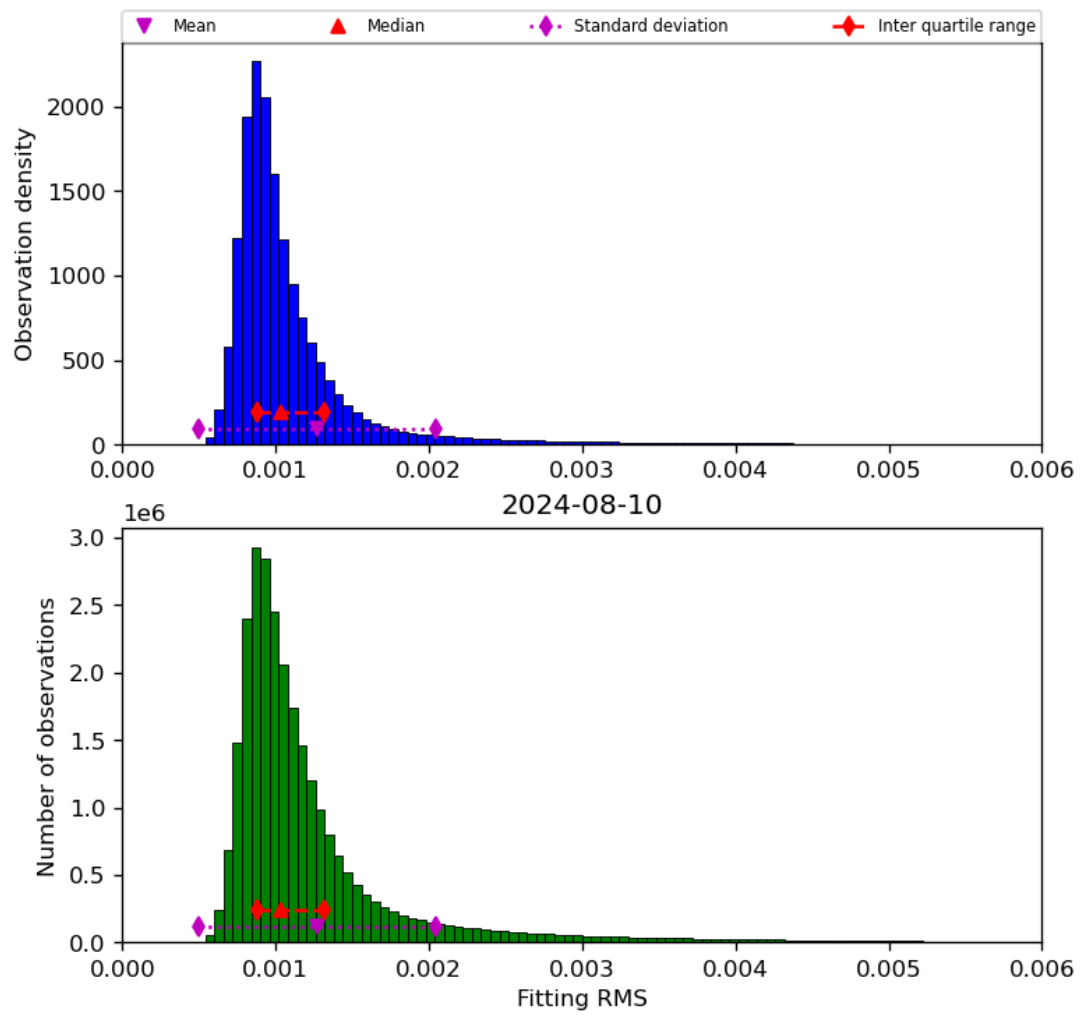
Figure 23: Histogram of “Fitting RMS” for 2024-08-09 to 2024-08-11
