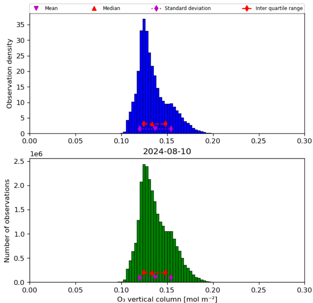
Figure 21: Histogram of “O 3 vertical column” for 2024-08-09 to 2024-08-11
