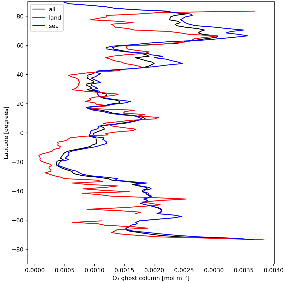
Figure 18: Zonal average of "O 3 ghost column" for 2024-08-09 to 2024-08-11.
