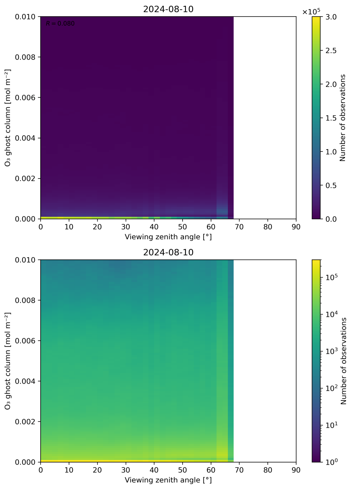
Figure 51: Scatter density plot of “Viewing zenith angle” against “O 3 ghost column” for 2024-08-09 to 2024-08-11.
