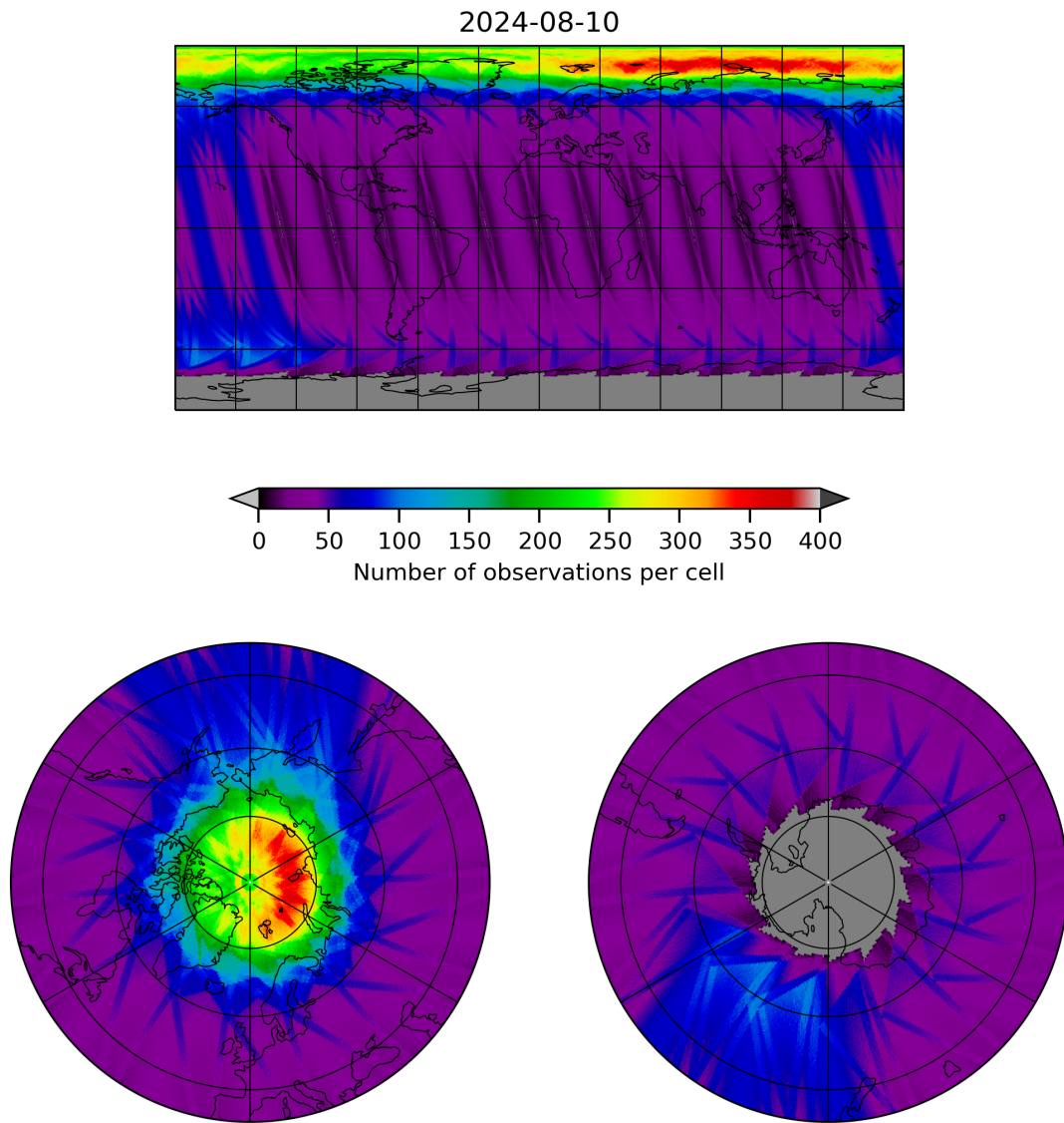
Figure 12: Map of the number of observations for 2024-08-09 to 2024-08-11
