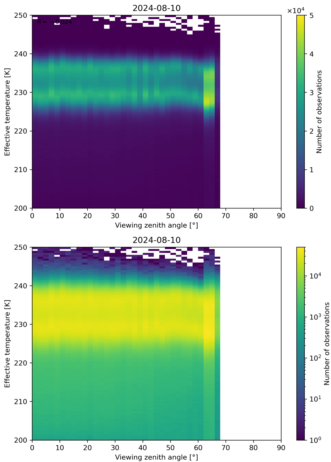
Figure 50: Scatter density plot of “Viewing zenith angle” against “Effective temperature” for 2024-08-09 to 2024-08-11.
