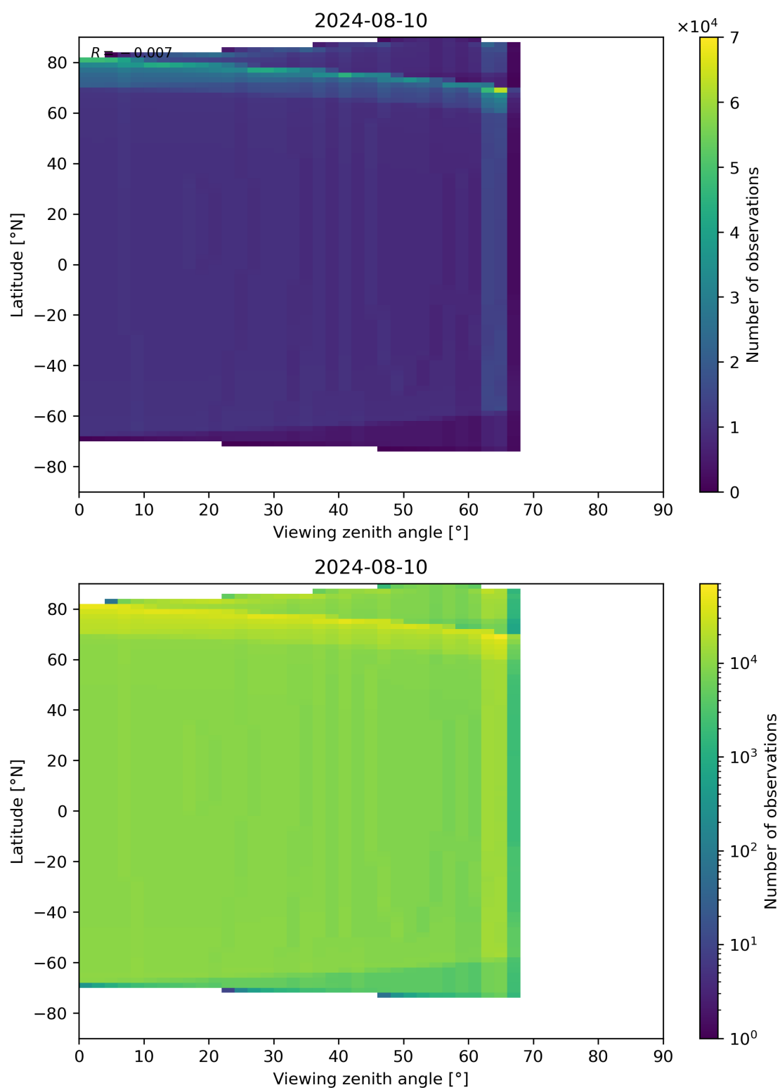
Figure 49: Scatter density plot of “Viewing zenith angle” against “Latitude” for 2024-08-09 to 2024-08-11.
