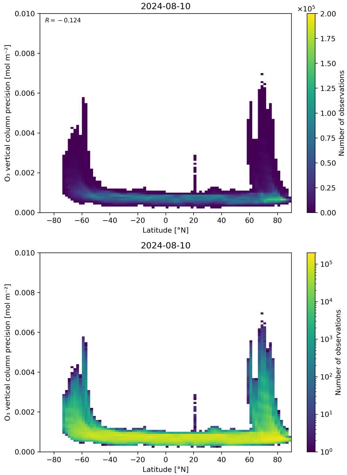
Figure 37: Scatter density plot of “Latitude” against “O 3 vertical column precision” for 2024-08-09 to 2024-08-11.
