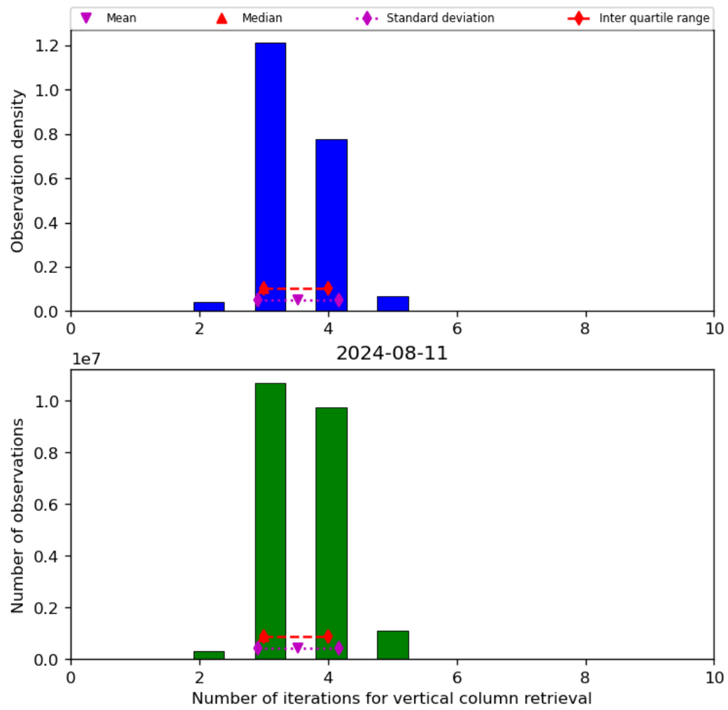
Figure 26: Histogram of “Number of iterations for vertical column retrieval” for 2024-08-11 to 2024-08-11
