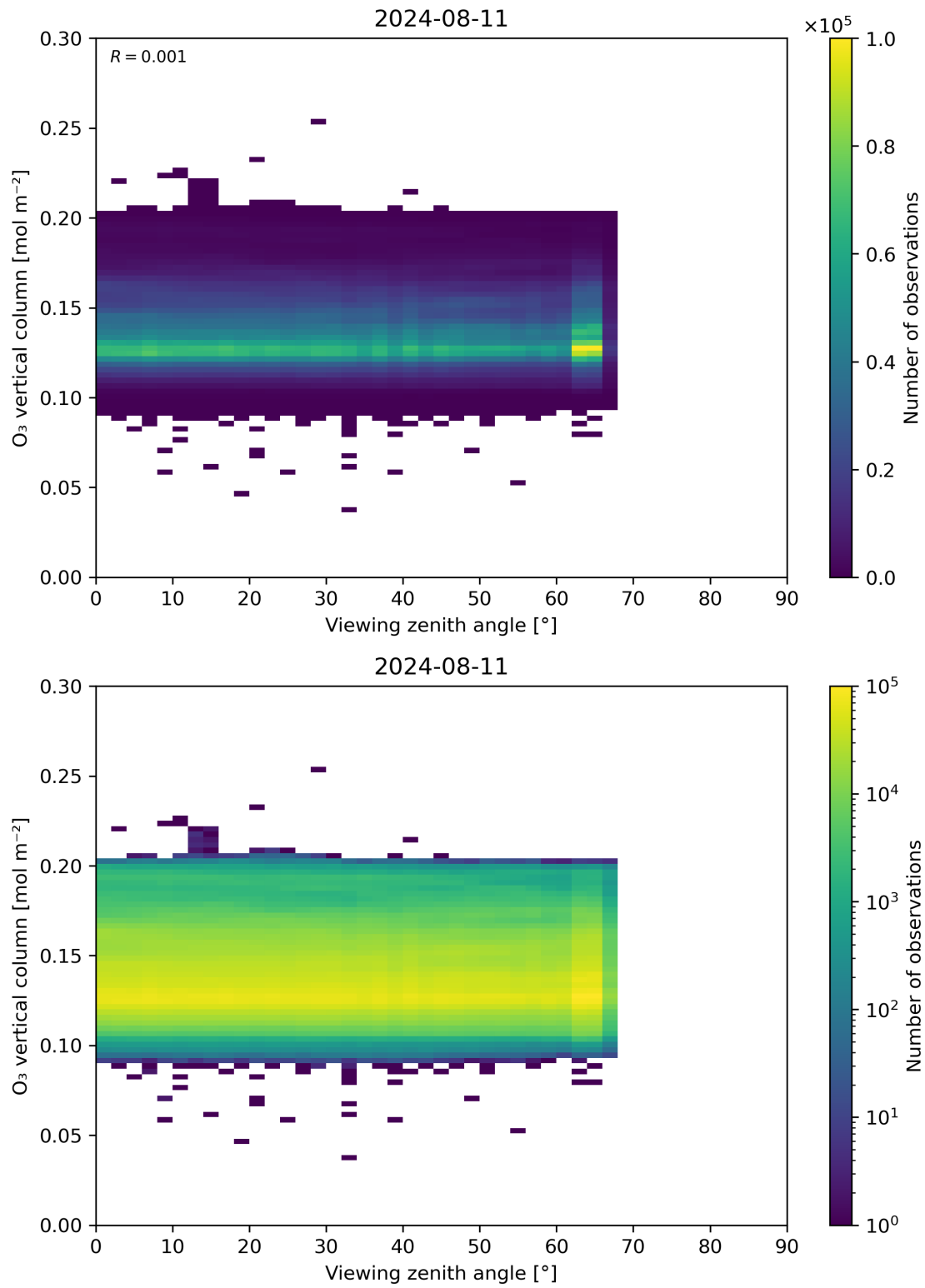
Figure 52: Scatter density plot of “Viewing zenith angle” against “O 3 vertical column” for 2024-08-11 to 2024-08-11.
