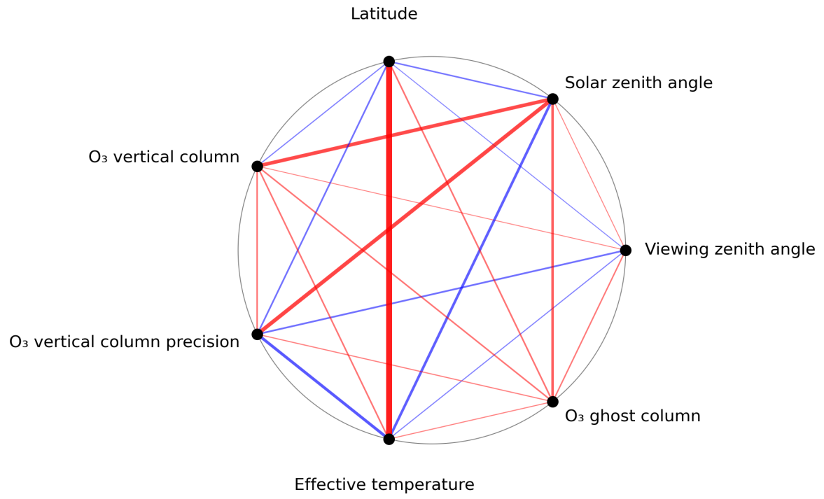
Figure 1: Map of correlation graph for 2024-08-11 to 2024-08-11.
