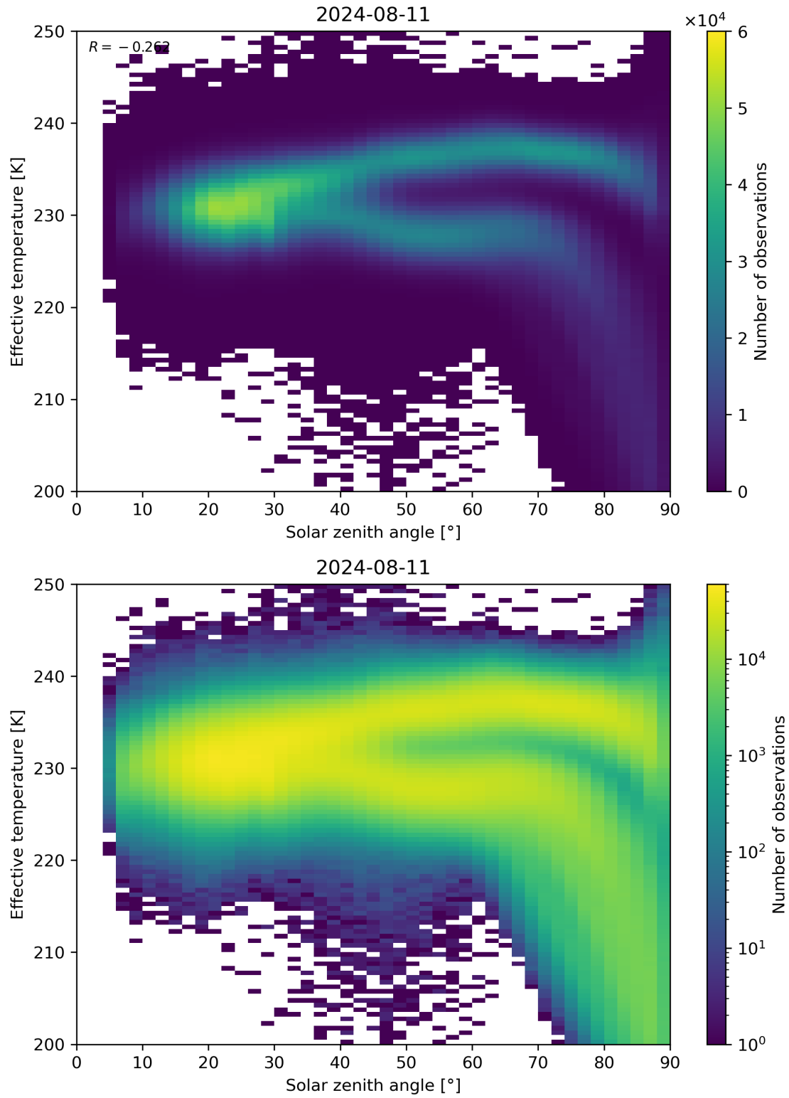
Figure 45: Scatter density plot of “Solar zenith angle” against “Effective temperature” for 2024-08-11 to 2024-08-11.
