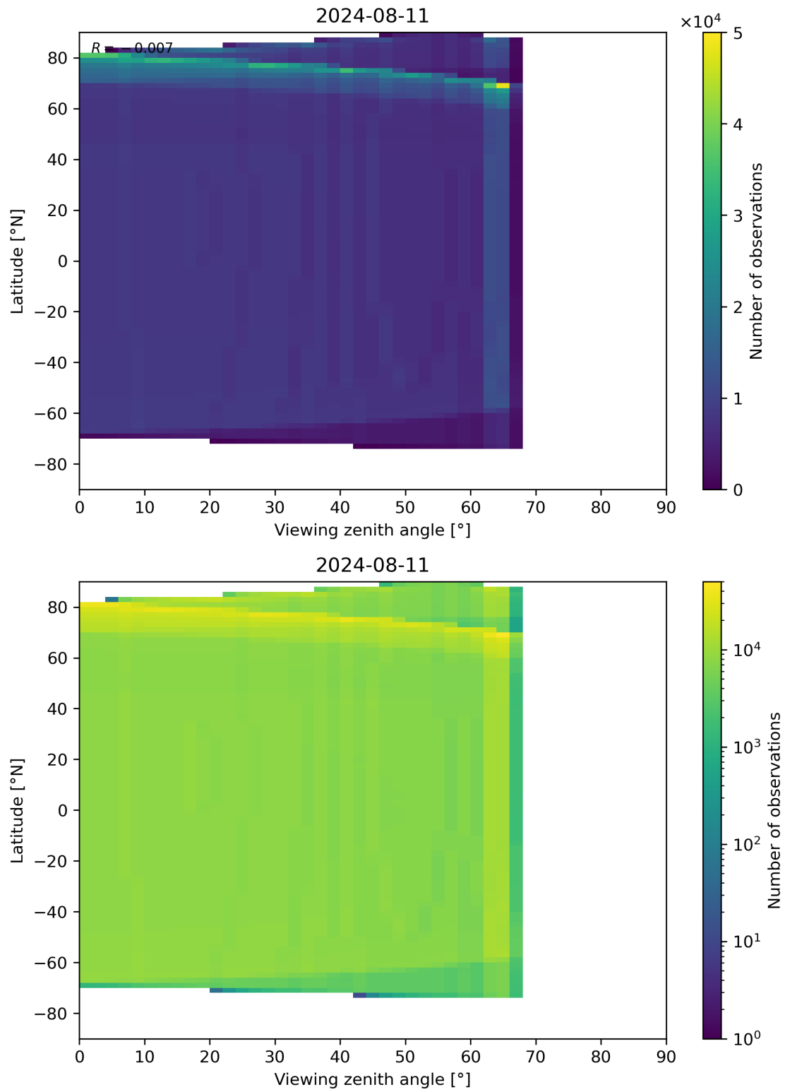
Figure 49: Scatter density plot of “Viewing zenith angle” against “Latitude” for 2024-08-11 to 2024-08-11.
