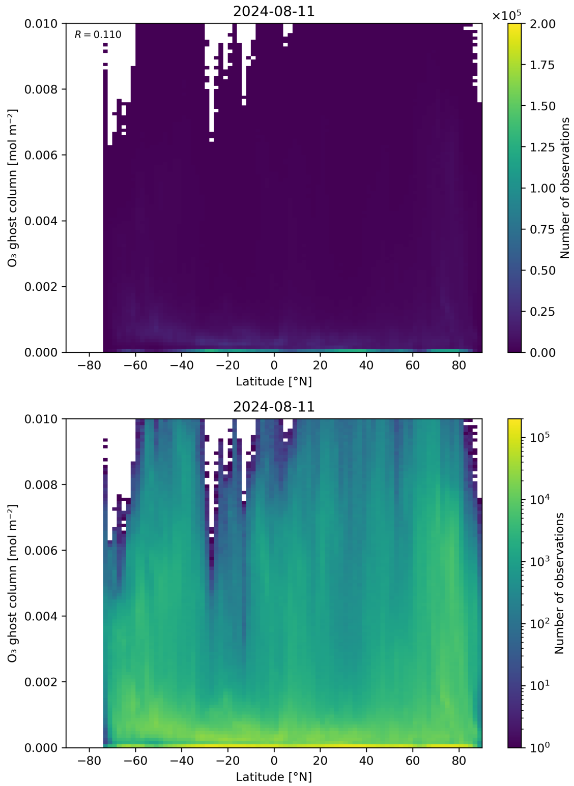
Figure 35: Scatter density plot of “Latitude” against “O 3 ghost column” for 2024-08-11 to 2024-08-11.
