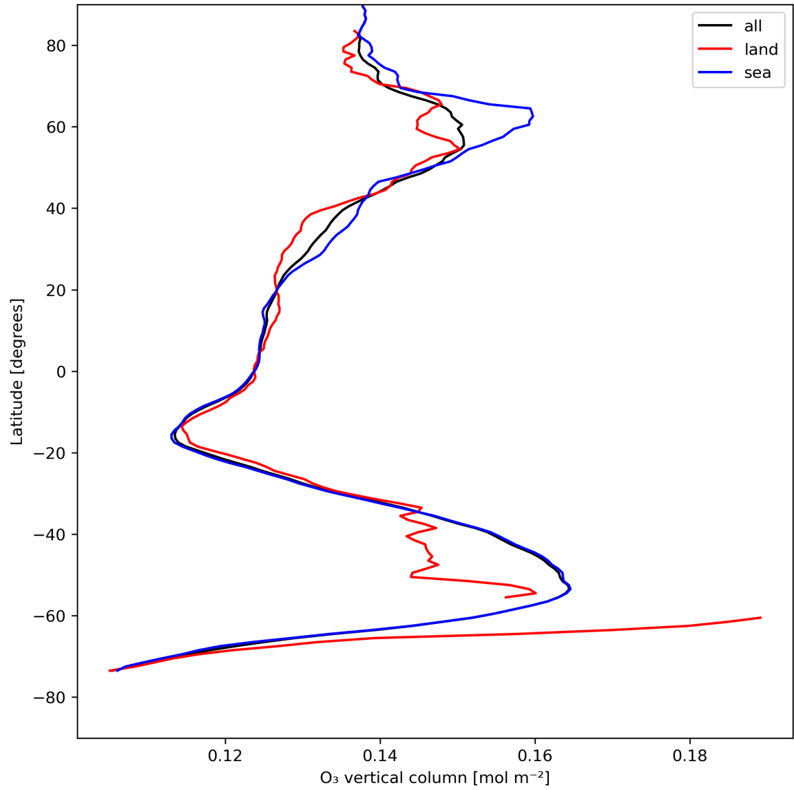
Figure 14: Zonal average of “O 3 vertical column” for 2024-08-11 to 2024-08-11.
