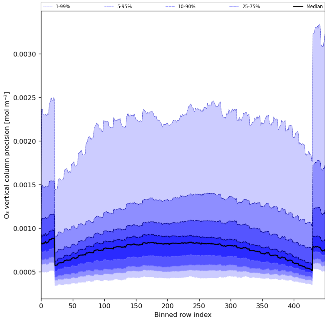
Figure 29: Along track statistics of “O 3 vertical column precision” for 2024-08-11 to 2024-08-11
