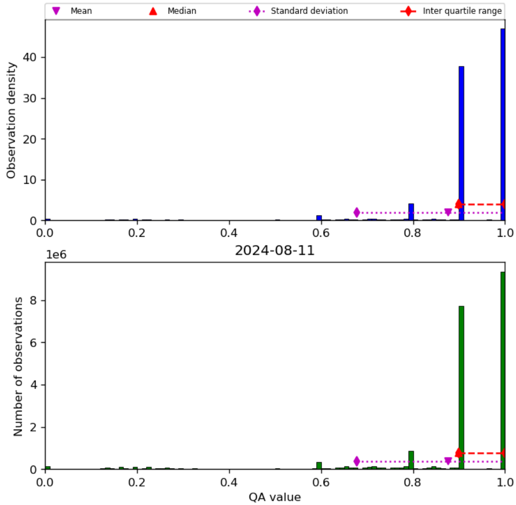
Figure 20: Histogram of “QA value” for 2024-08-11 to 2024-08-11
