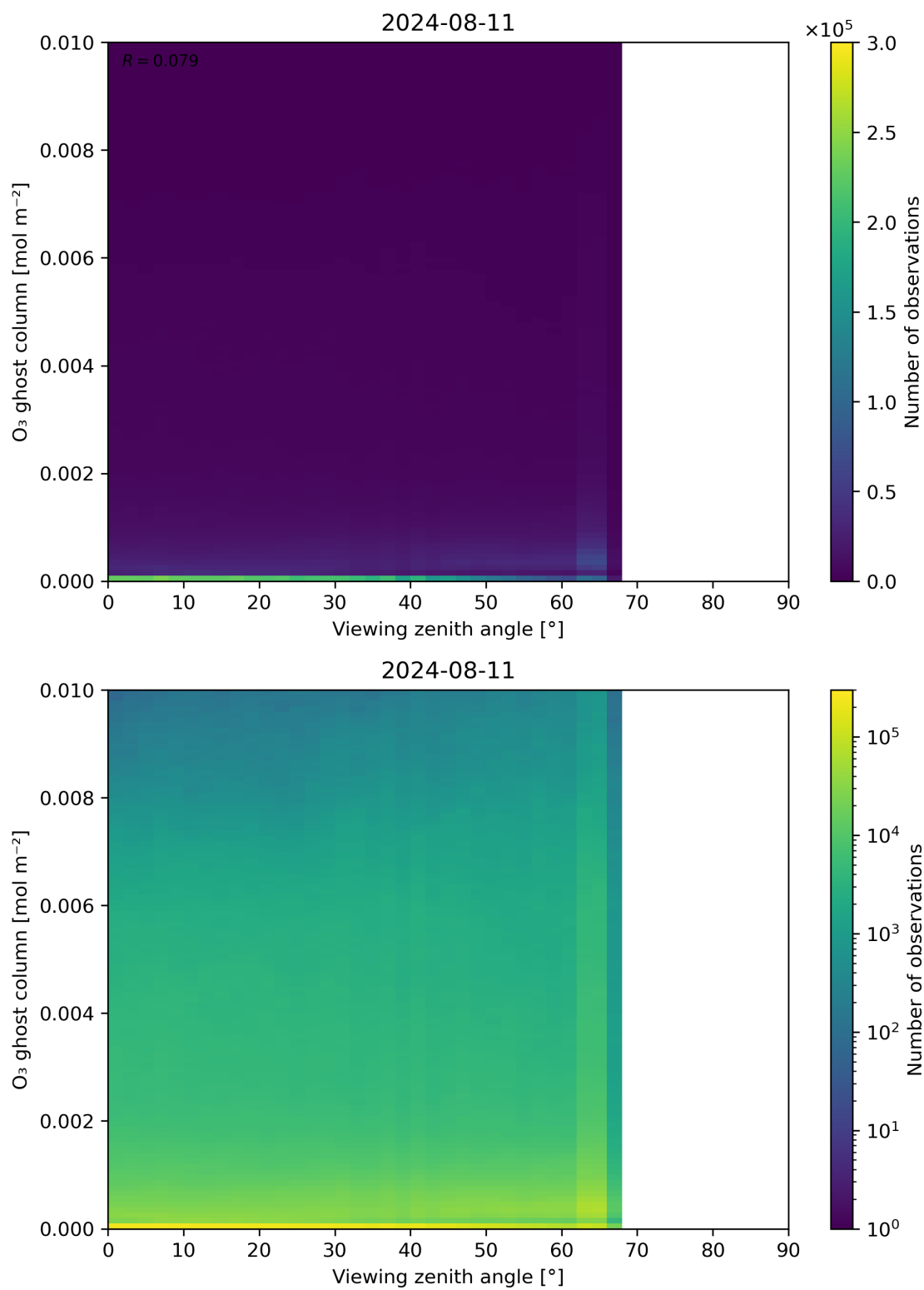
Figure 51: Scatter density plot of “Viewing zenith angle” against “O 3 ghost column” for 2024-08-11 to 2024-08-11.
