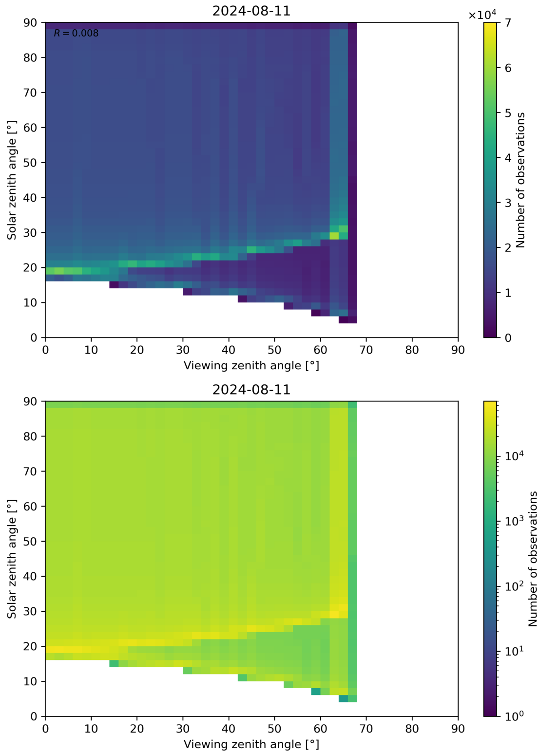
Figure 54: Scatter density plot of “Viewing zenith angle” against “Solar zenith angle” for 2024-08-11 to 2024-08-11.
