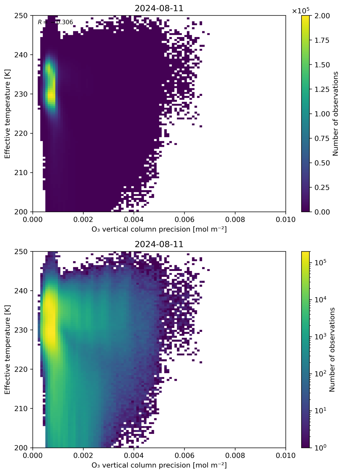
Figure 42: Scatter density plot of “O 3 vertical column precision” against “Effective temperature” for 2024-08-11 to 2024-08-11.
