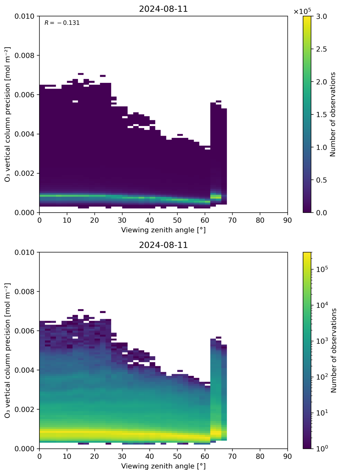
Figure 53: Scatter density plot of “Viewing zenith angle” against “O 3 vertical column precision” for 2024-08-11 to 2024-08-11.
