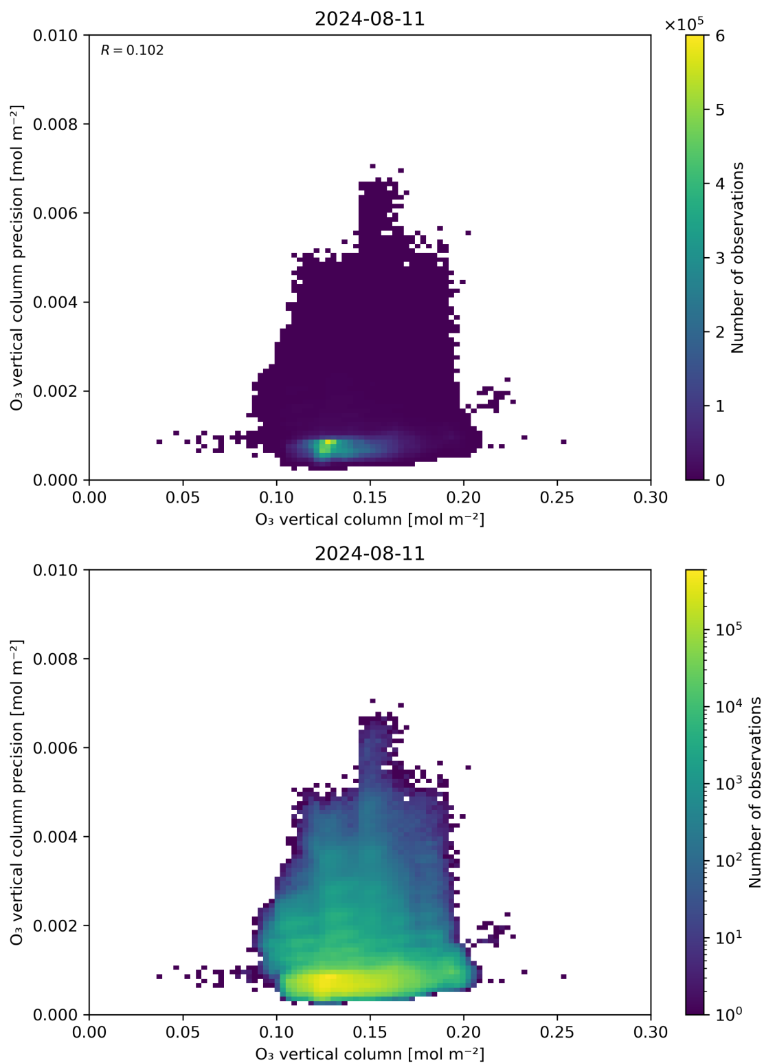
Figure 41: Scatter density plot of “O 3 vertical column” against “O 3 vertical column precision” for 2024-08-11 to 2024-08-11.
