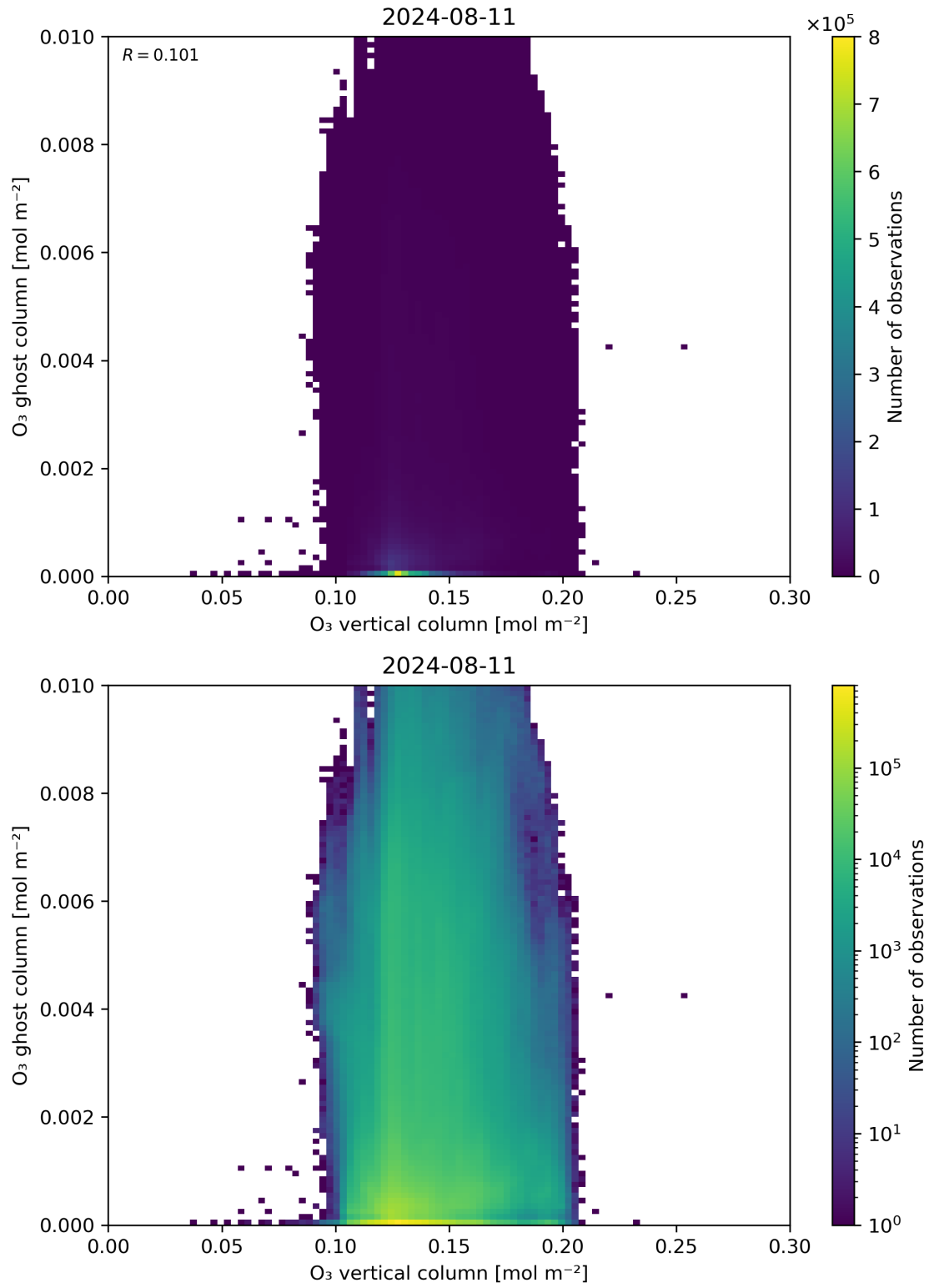
Figure 40: Scatter density plot of “O 3 vertical column” against “O 3 ghost column” for 2024-08-11 to 2024-08-11.
