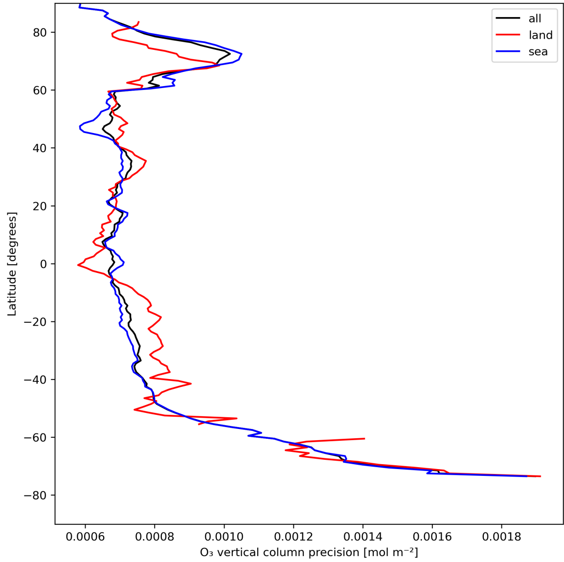
Figure 15: Zonal average of “O 3 vertical column precision” for 2024-08-11 to 2024-08-11.
