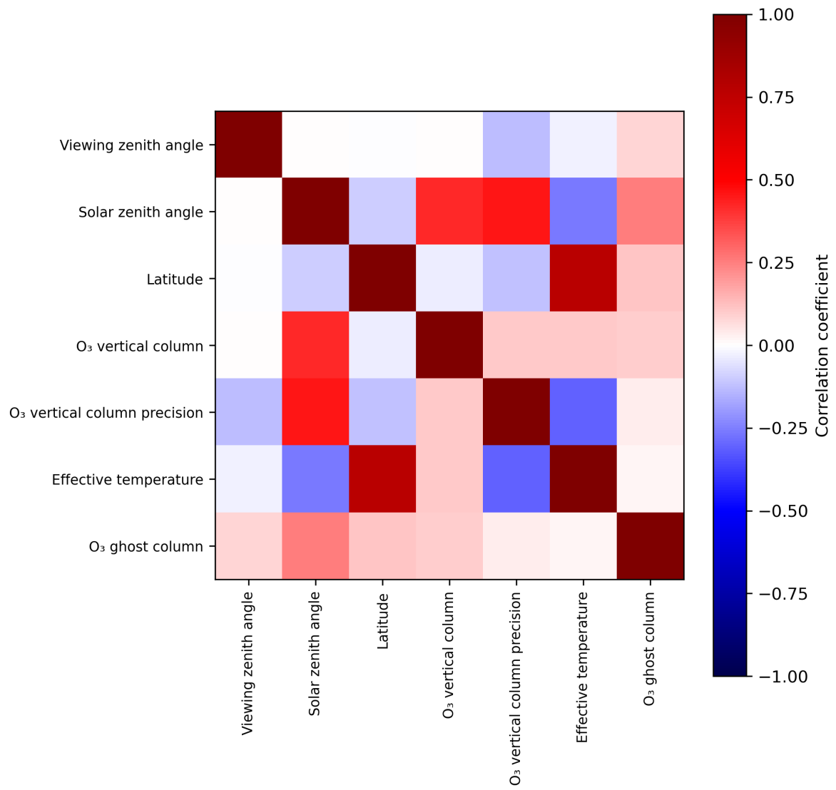
Figure 2: Map of correlation matrix for 2024-08-11 to 2024-08-11.
