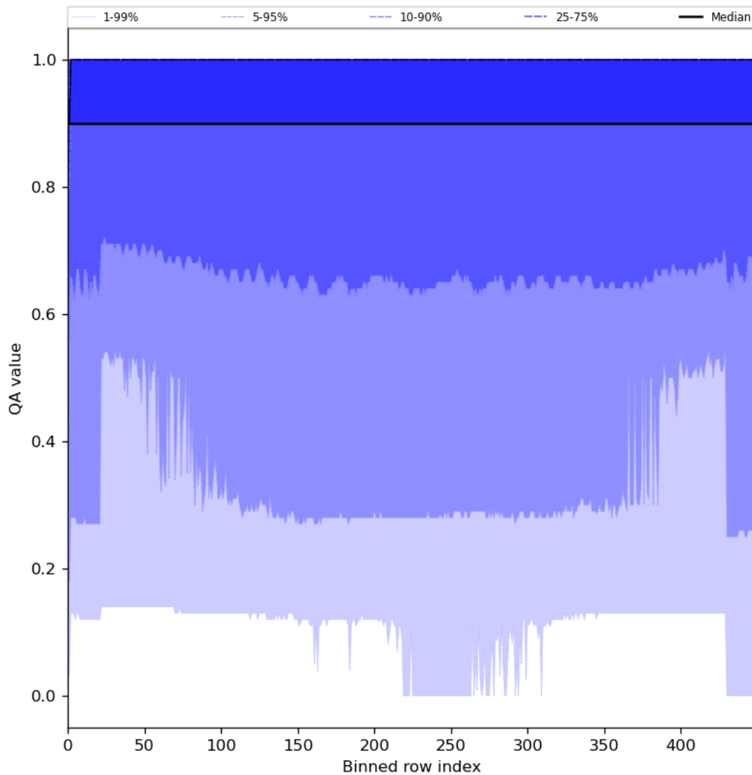
Figure 27: Along track statistics of “QA value” for 2024-08-11 to 2024-08-11
