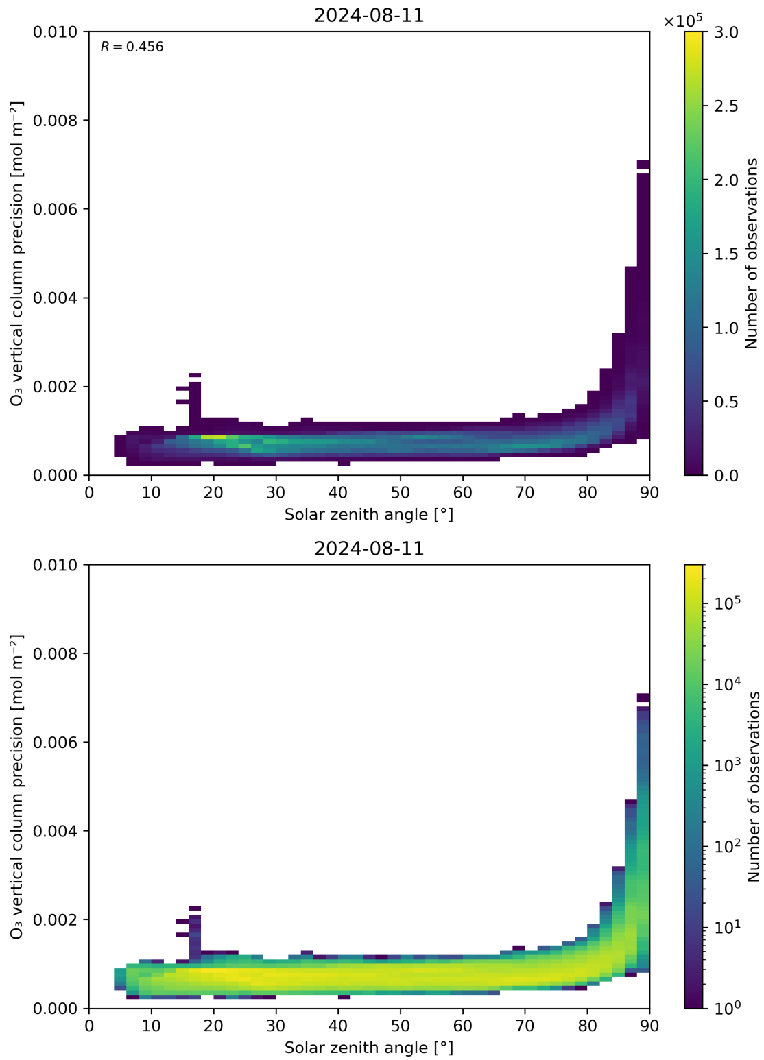
Figure 48: Scatter density plot of “Solar zenith angle” against “O 3 vertical column precision” for 2024-08-11 to 2024-08-11.
