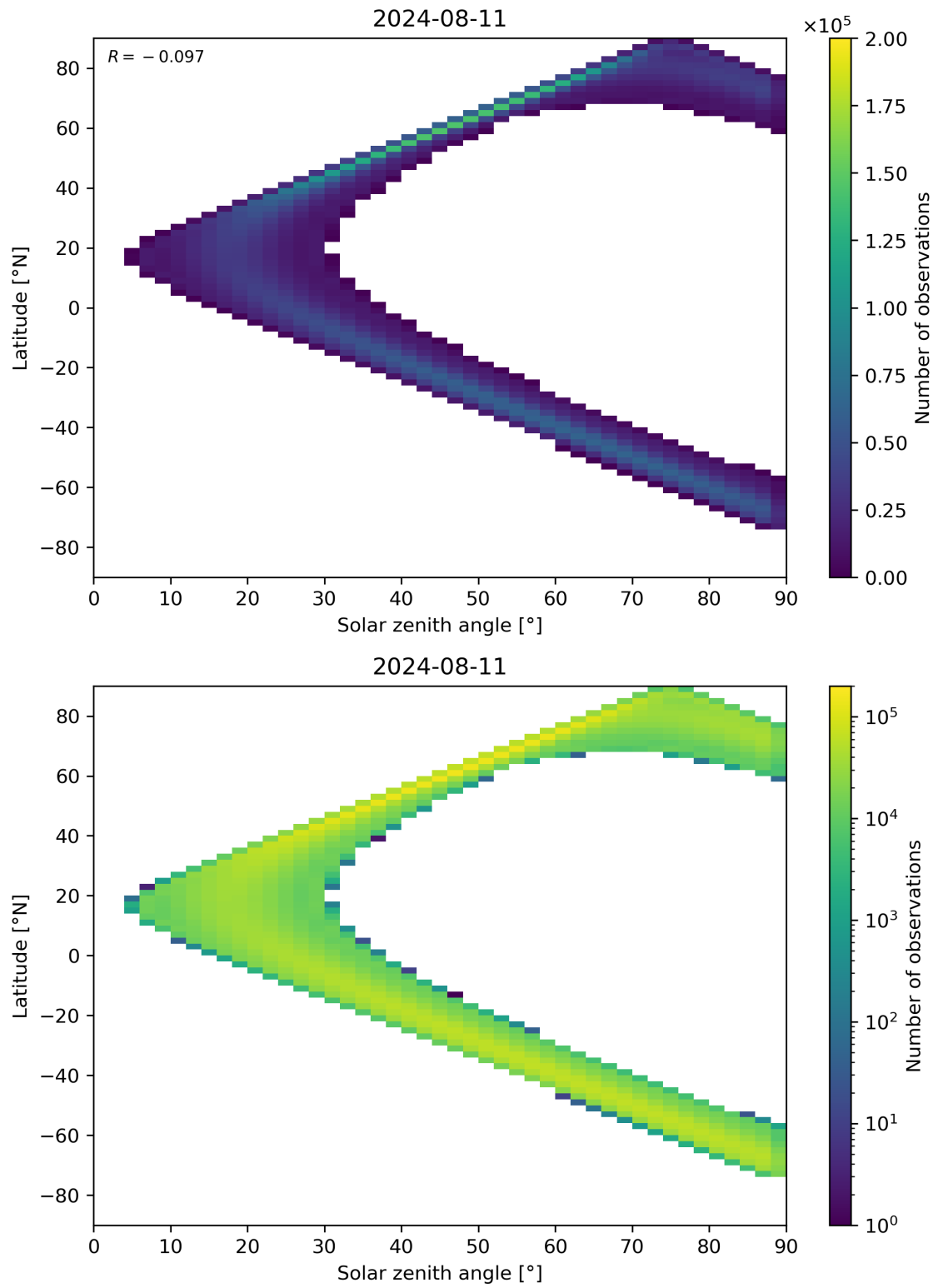
Figure 44: Scatter density plot of “Solar zenith angle” against “Latitude” for 2024-08-11 to 2024-08-11.
