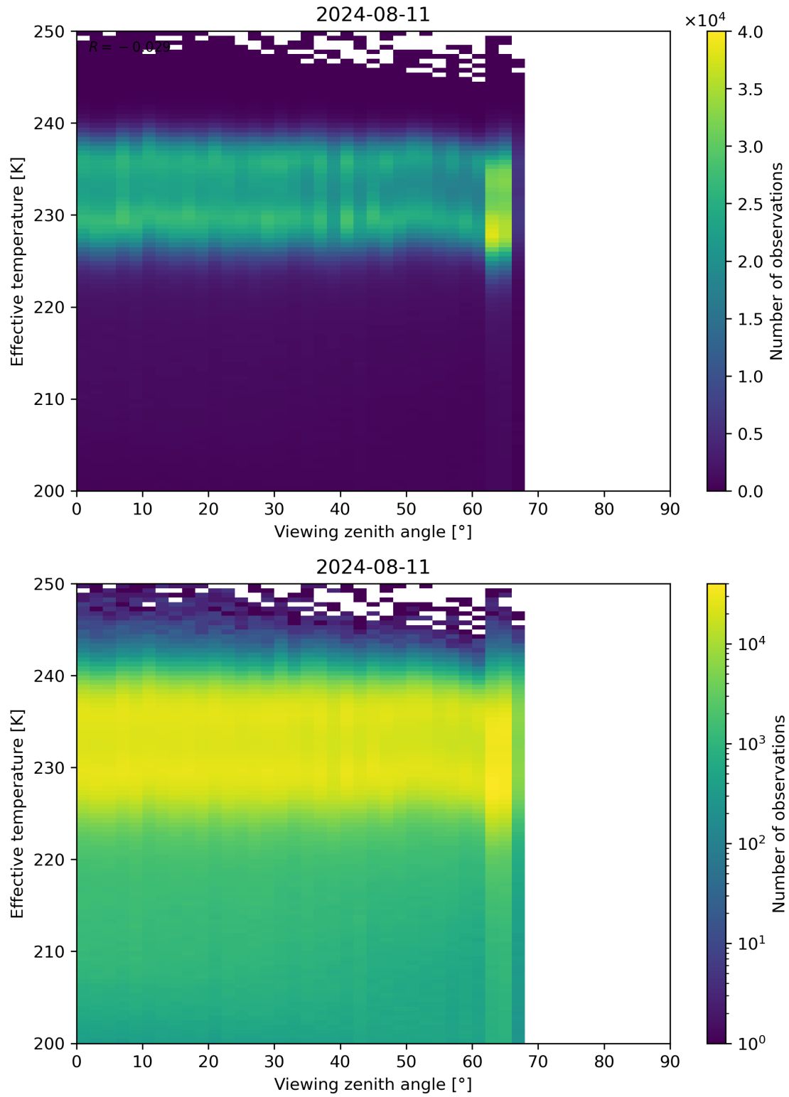
Figure 50: Scatter density plot of “Viewing zenith angle” against “Effective temperature” for 2024-08-11 to 2024-08-11.
