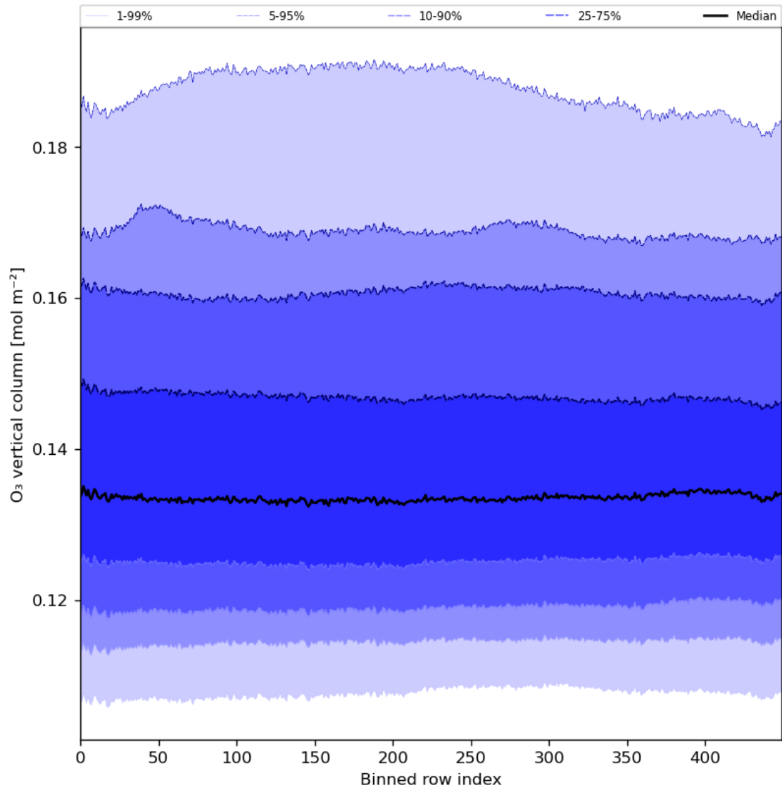
Figure 28: Along track statistics of “O 3 vertical column” for 2024-08-11 to 2024-08-11
