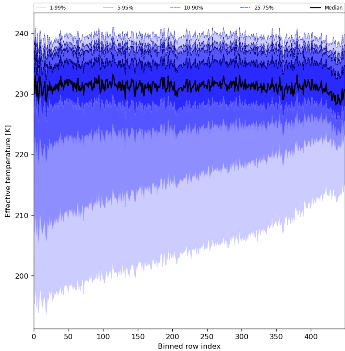
Figure 31: Along track statistics of “Effective temperature” for 2024-08-11 to 2024-08-11
