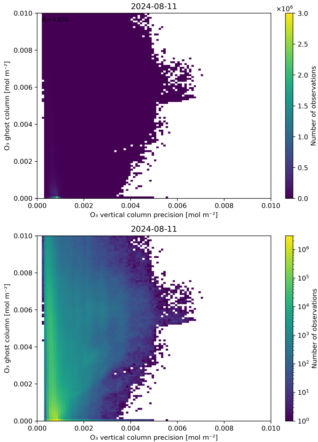
Figure 43: Scatter density plot of “ \text{O}_3 vertical column precision” against “ \text{O}_3 ghost column” for 2024-08-11 to 2024-08-11.
