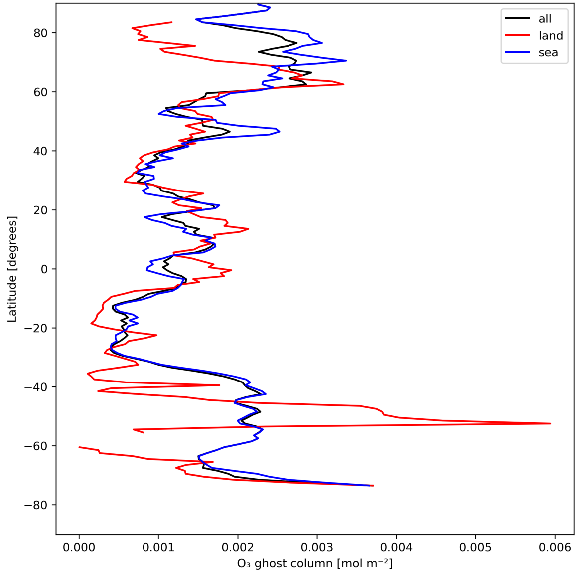
Figure 18: Zonal average of "O 3 ghost column" for 2024-08-11 to 2024-08-11.
