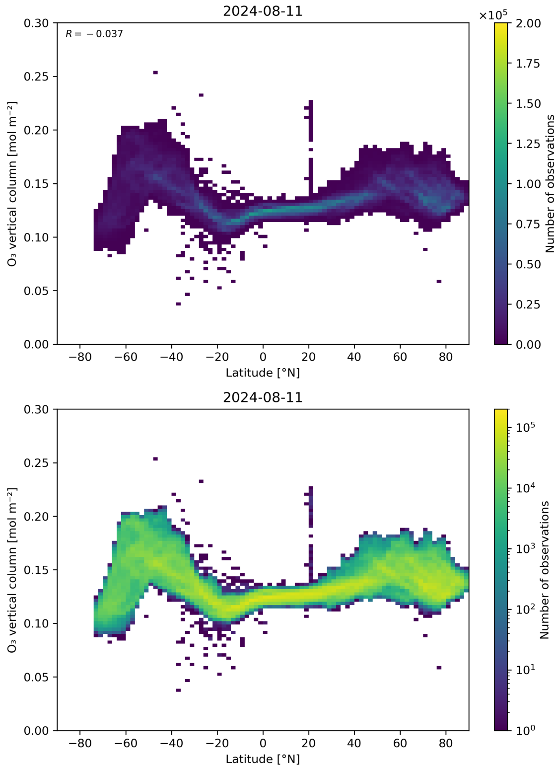
Figure 36: Scatter density plot of “Latitude” against “O 3 vertical column” for 2024-08-11 to 2024-08-11.
