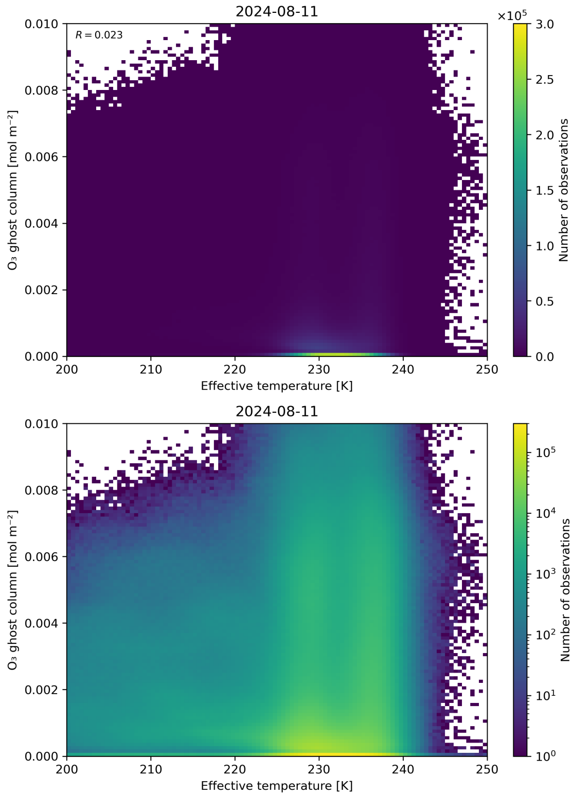
Figure 38: Scatter density plot of “Effective temperature” against “O 3 ghost column” for 2024-08-11 to 2024-08-11.
