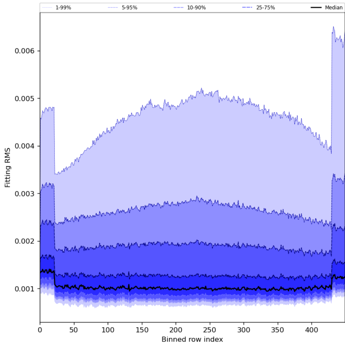
Figure 30: Along track statistics of “Fitting RMS” for 2024-08-11 to 2024-08-11
