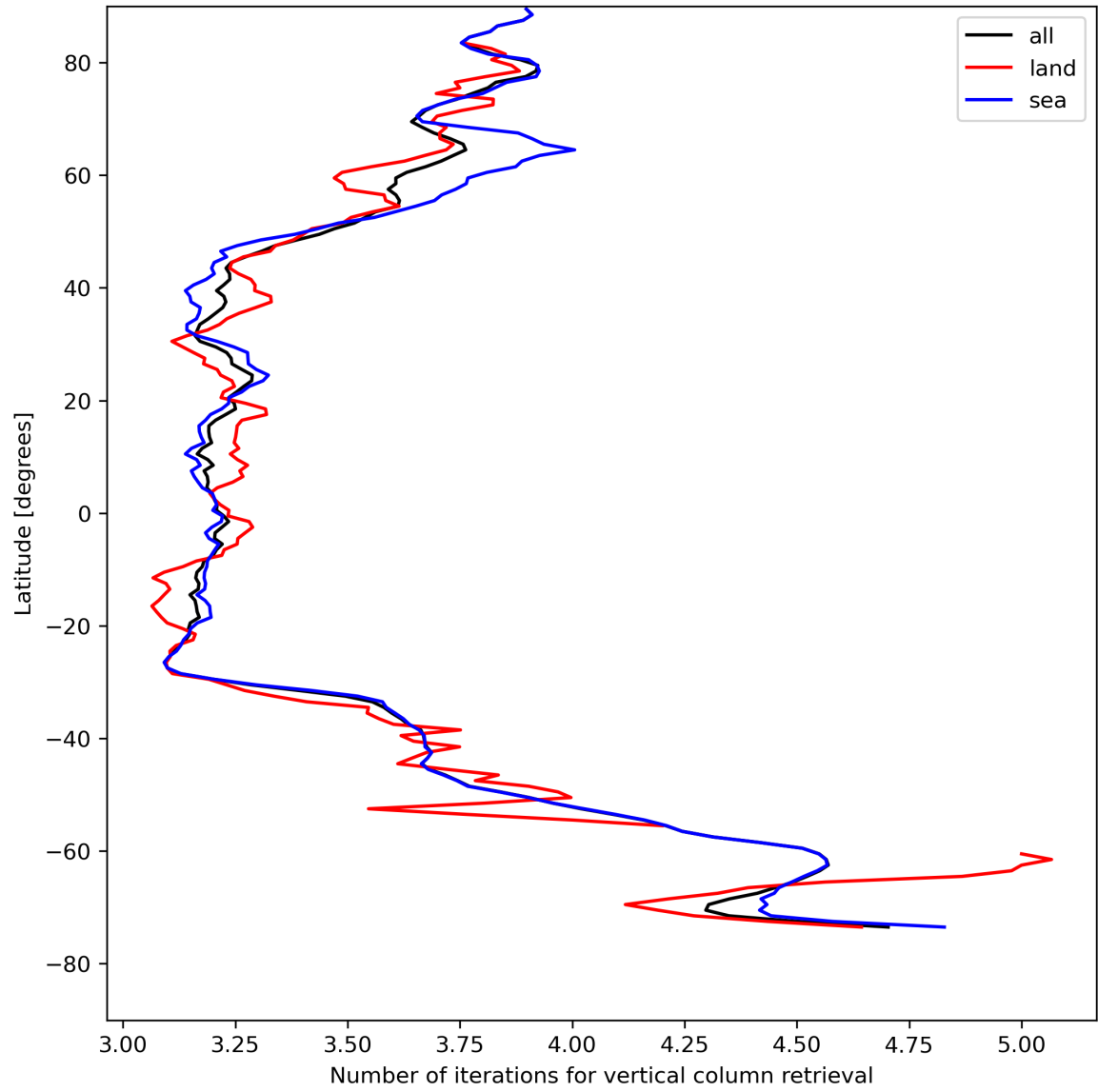
Figure 19: Zonal average of “Number of iterations for vertical column retrieval” for 2024-08-11 to 2024-08-11.
