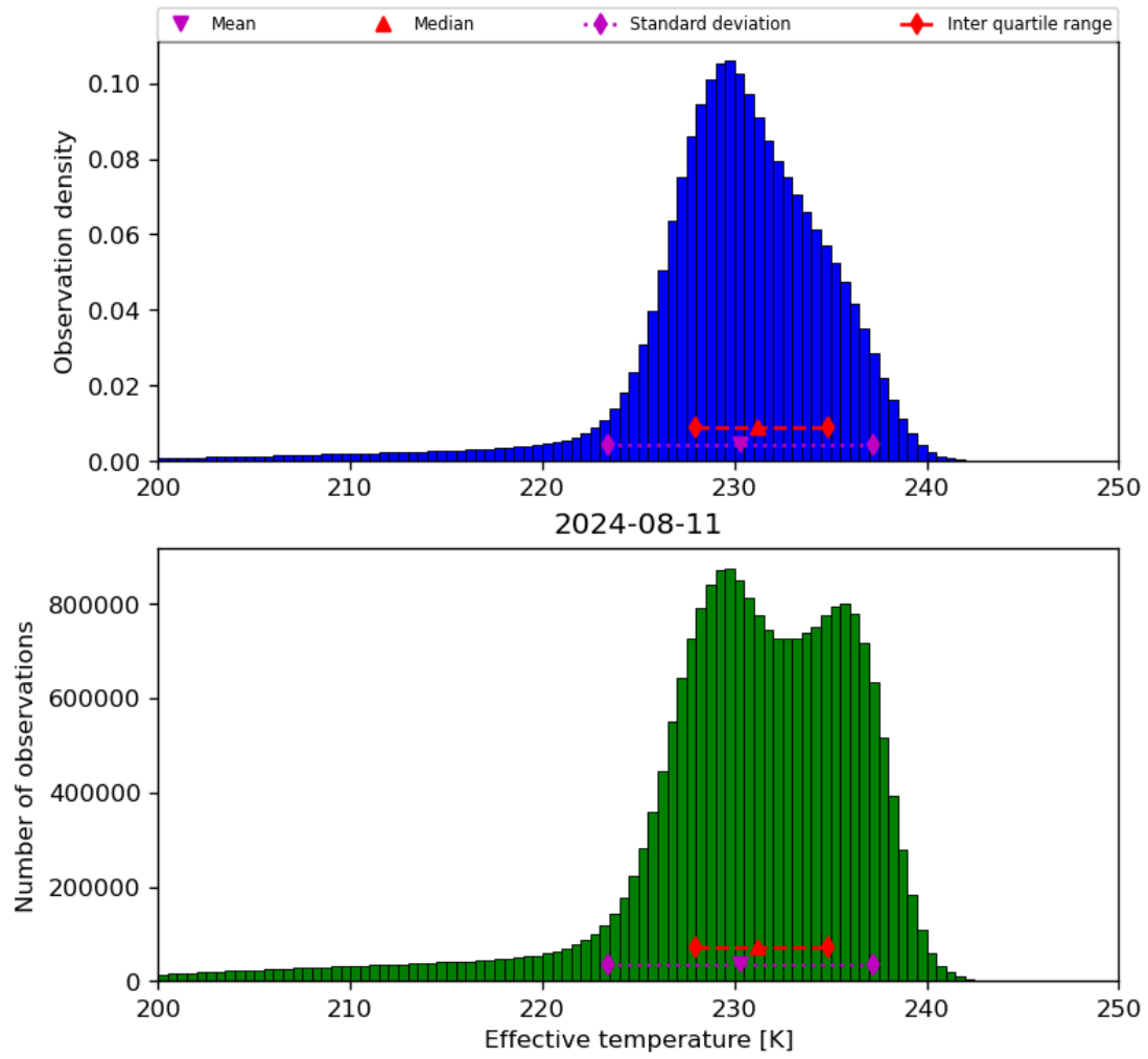
Figure 24: Histogram of “Effective temperature” for 2024-08-11 to 2024-08-11
