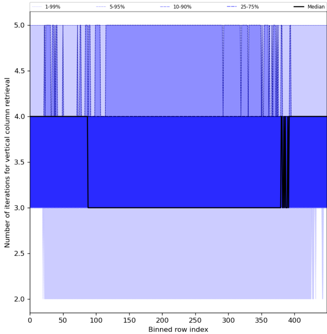
Figure 33: Along track statistics of “Number of iterations for vertical column retrieval” for 2024-08-11 to 2024-08-11
