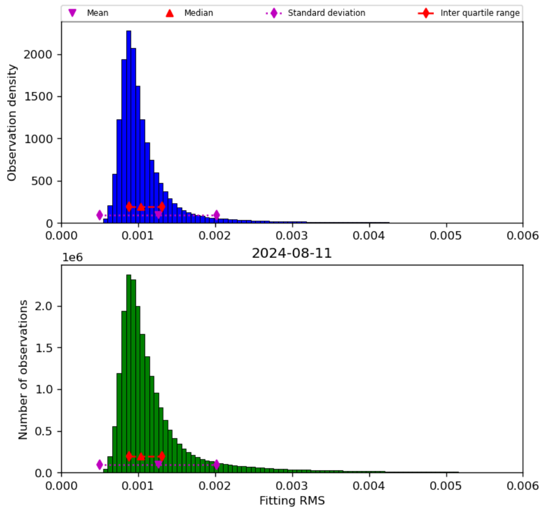
Figure 23: Histogram of “Fitting RMS” for 2024-08-11 to 2024-08-11
