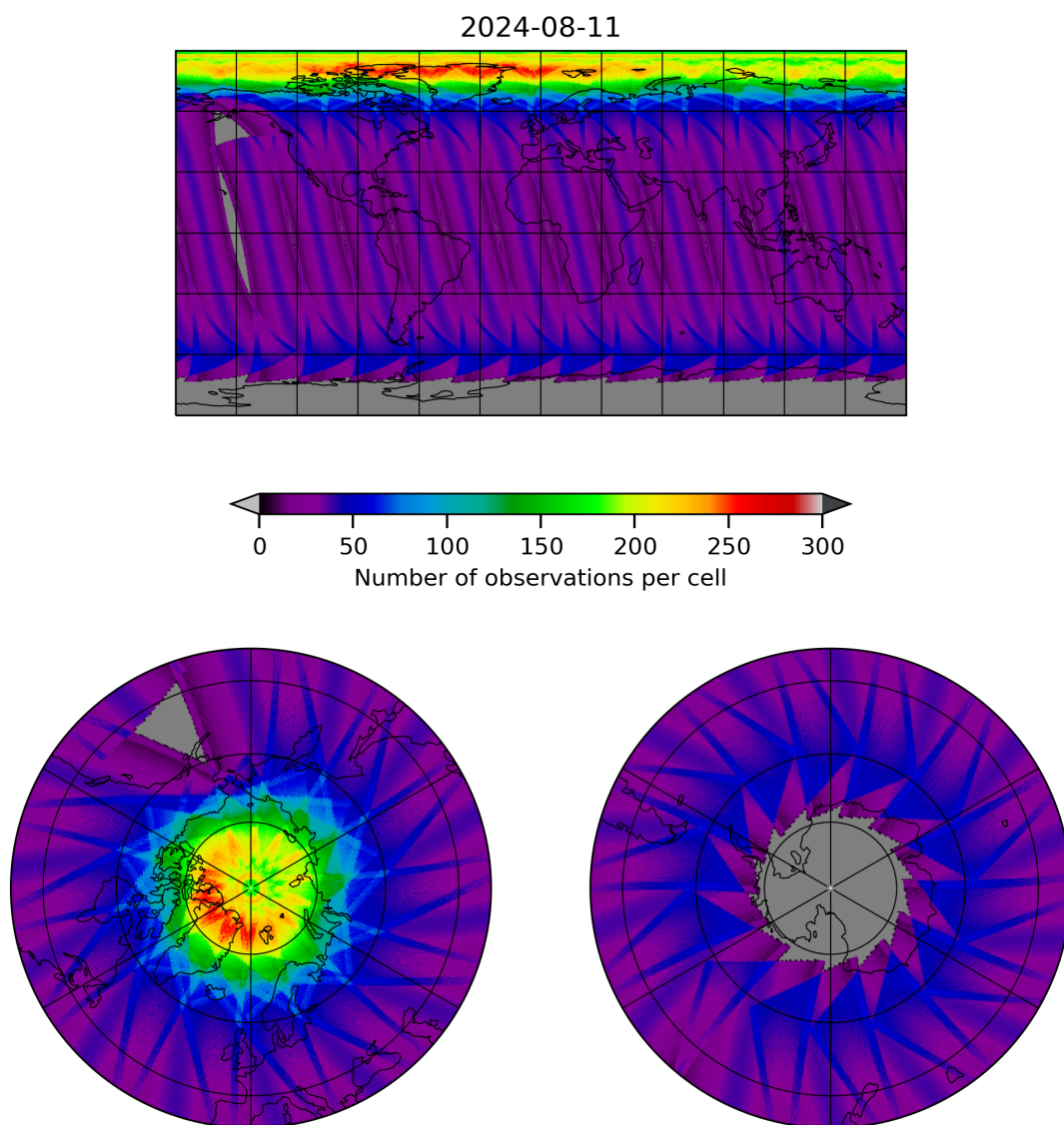
Figure 12: Map of the number of observations for 2024-08-11 to 2024-08-11
