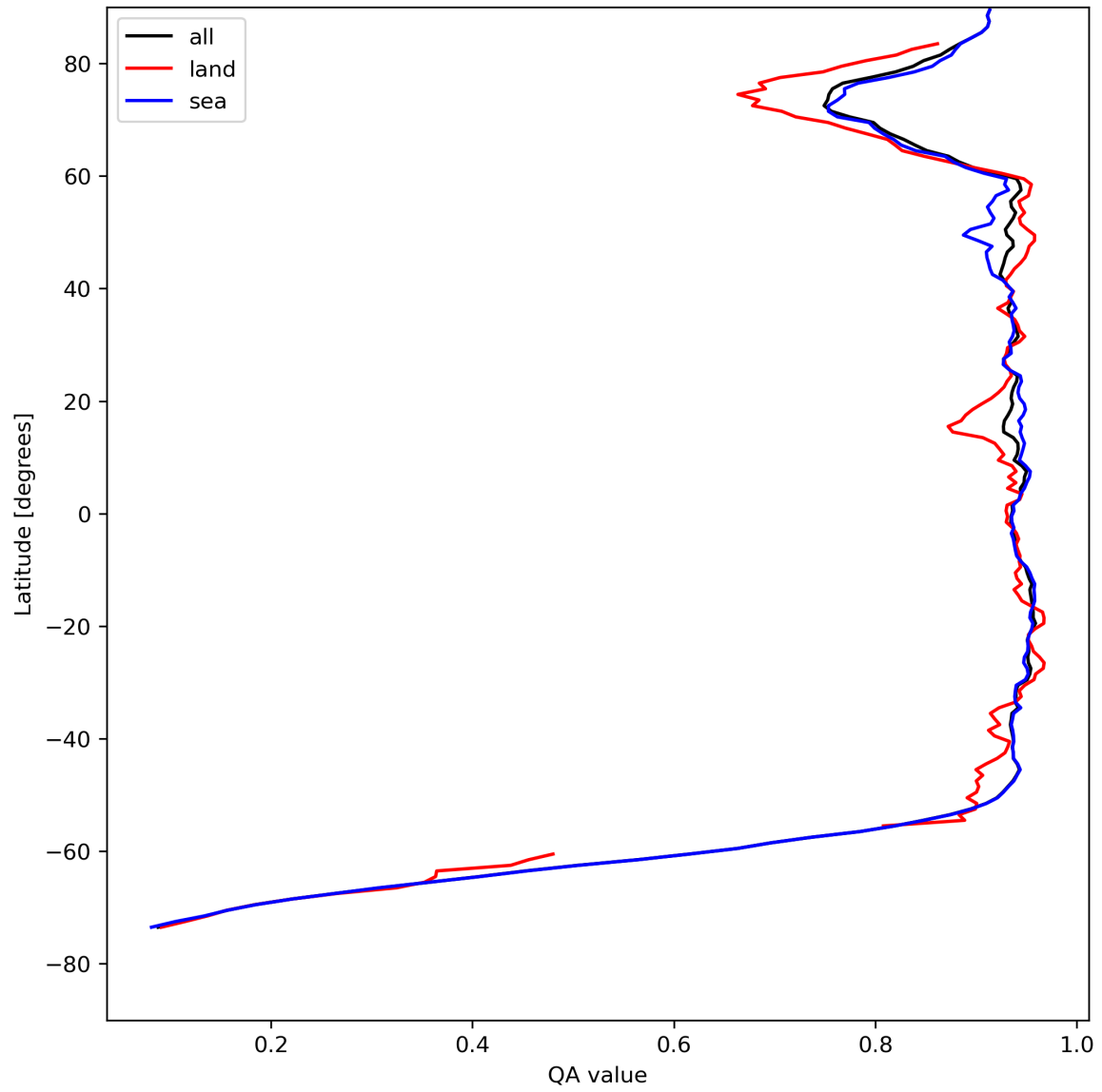
Figure 13: Zonal average of “QA value” for 2024-08-11 to 2024-08-11.
