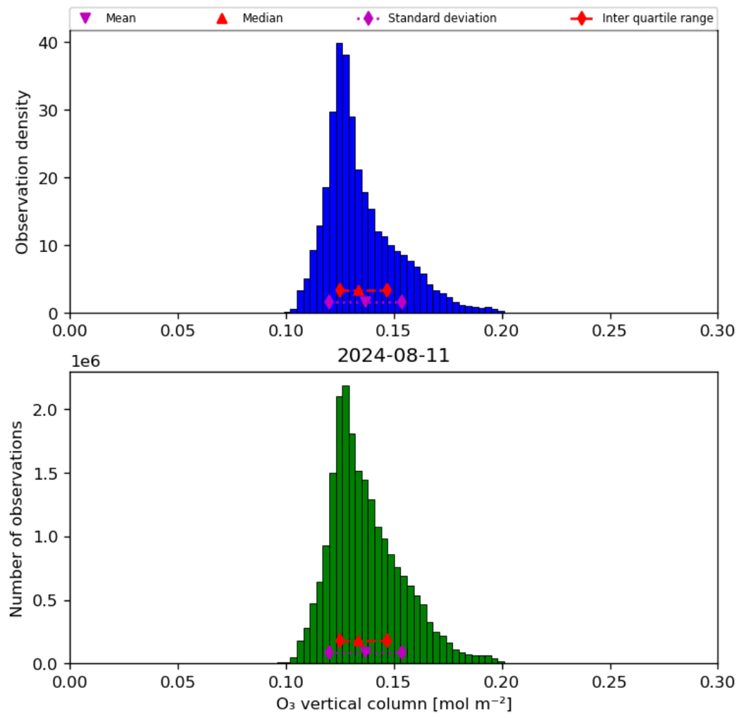
Figure 21: Histogram of “O 3 vertical column” for 2024-08-11 to 2024-08-11
