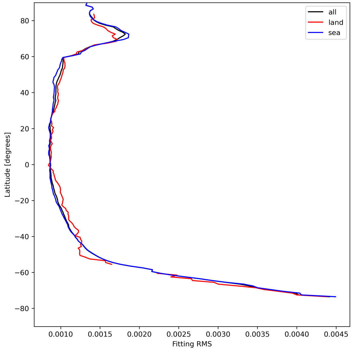
Figure 16: Zonal average of “Fitting RMS” for 2024-08-11 to 2024-08-11.
