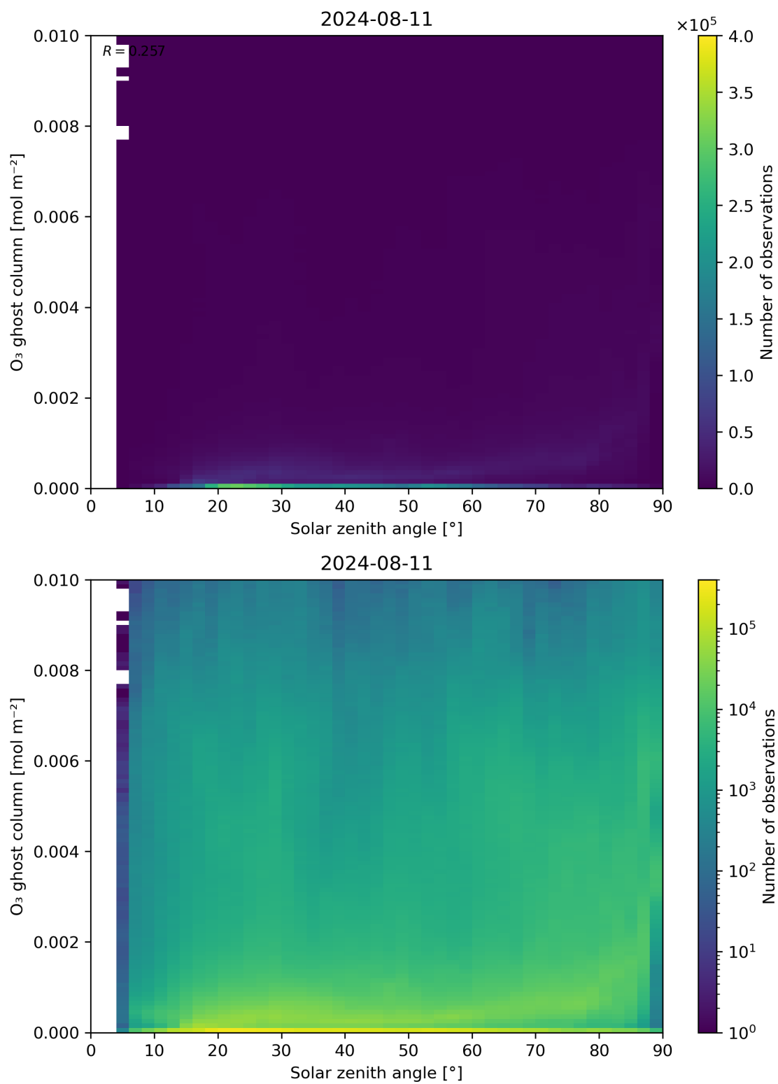
Figure 46: Scatter density plot of “Solar zenith angle” against “O 3 ghost column” for 2024-08-11 to 2024-08-11.
