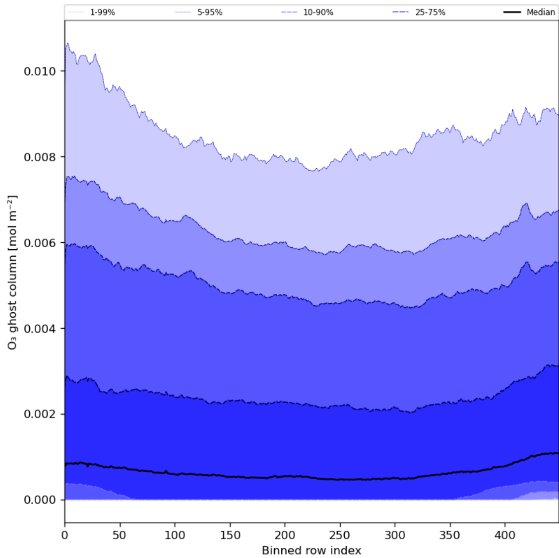
Figure 32: Along track statistics of “O 3 ghost column” for 2024-08-11 to 2024-08-11
