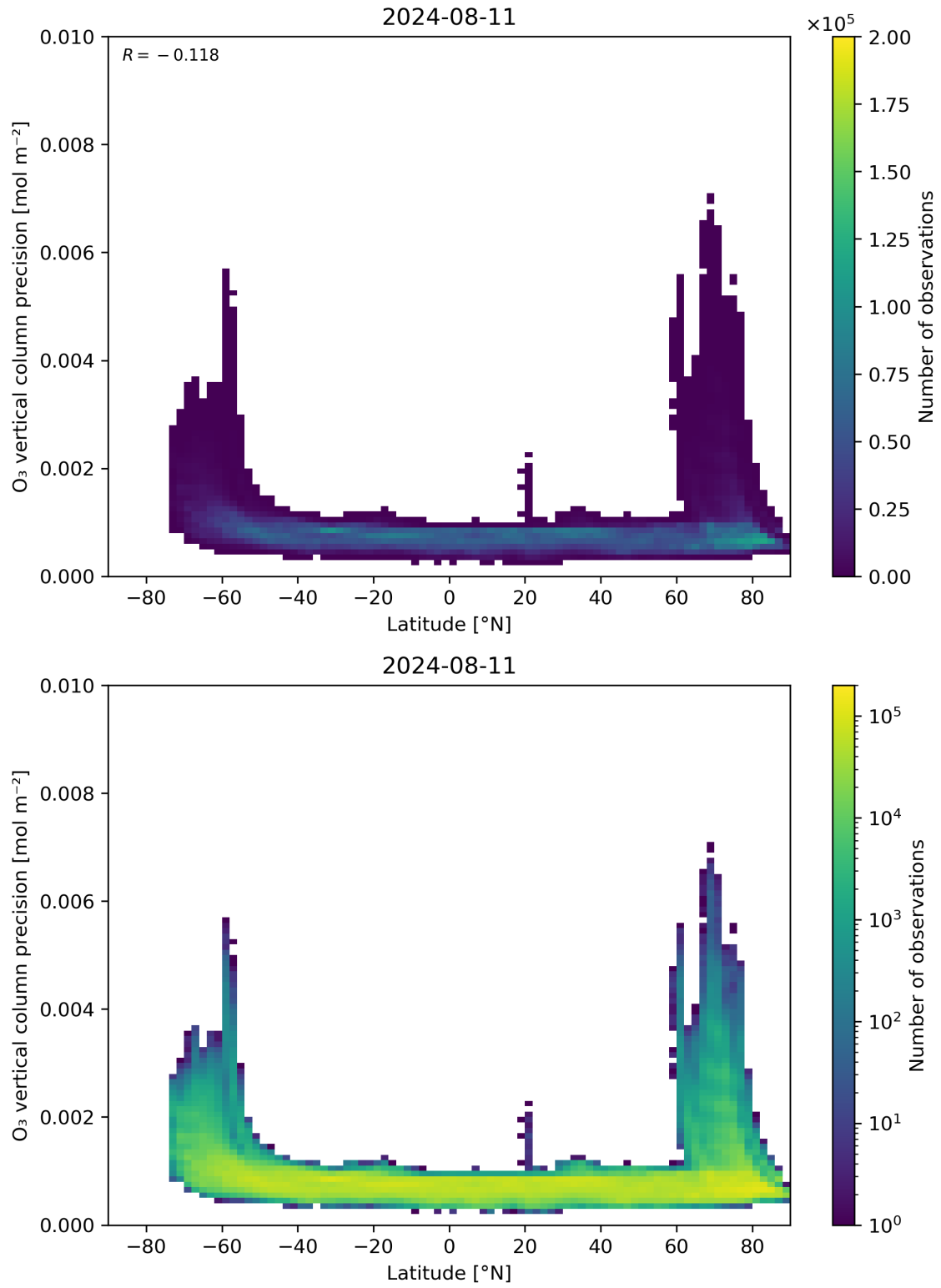
Figure 37: Scatter density plot of “Latitude” against “O 3 vertical column precision” for 2024-08-11 to 2024-08-11.
