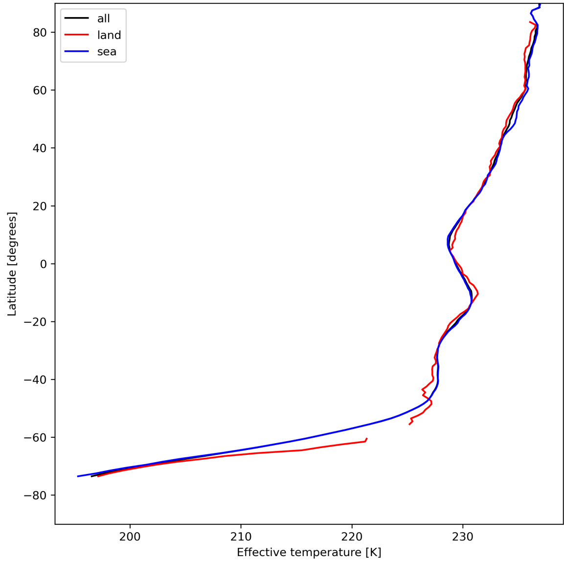
Figure 17: Zonal average of "Effective temperature" for 2024-08-11 to 2024-08-11.
