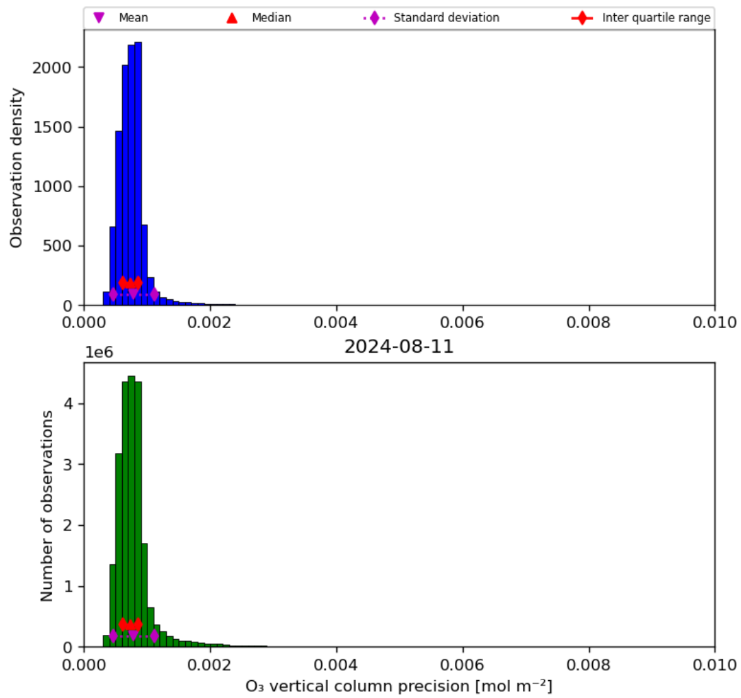
Figure 22: Histogram of “O 3 vertical column precision” for 2024-08-11 to 2024-08-11
