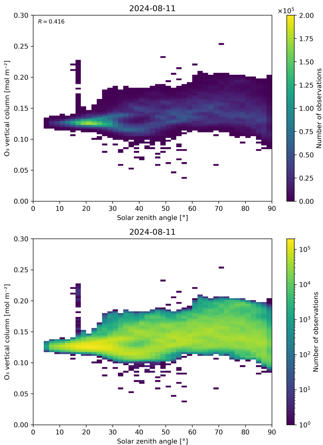
Figure 47: Scatter density plot of “Solar zenith angle” against “O 3 vertical column” for 2024-08-11 to 2024-08-11.
