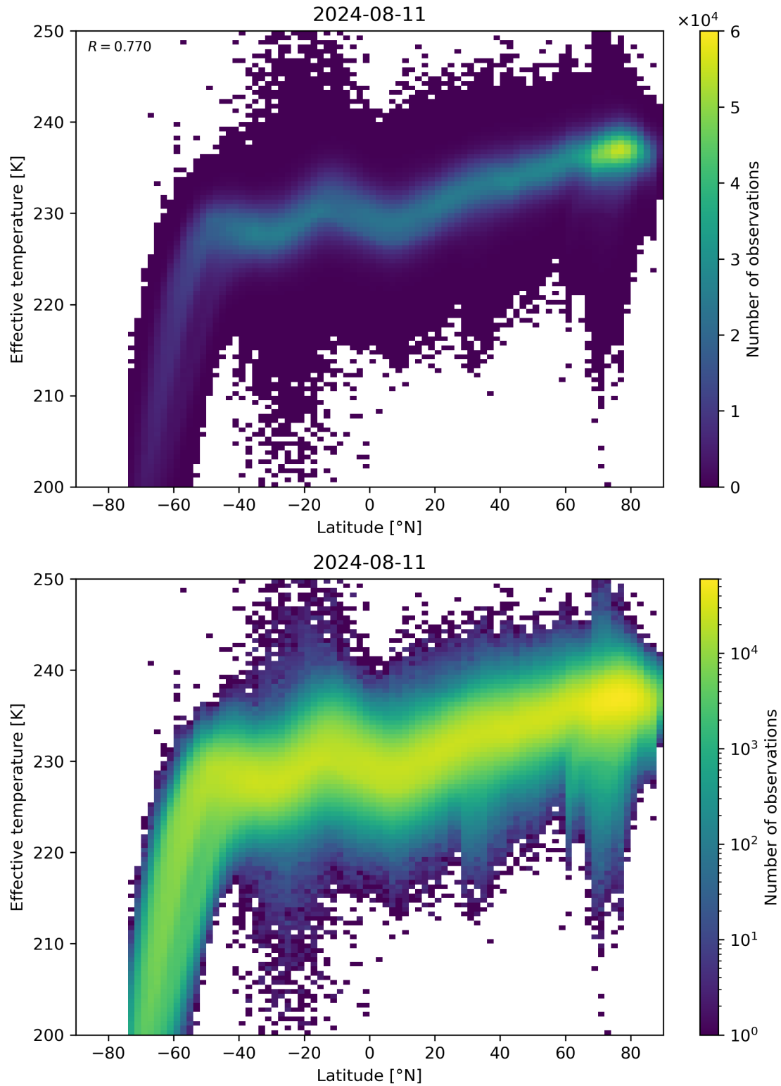
Figure 34: Scatter density plot of “Latitude” against “Effective temperature” for 2024-08-11 to 2024-08-11.
