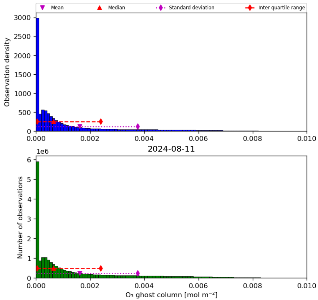
Figure 25: Histogram of “O 3 ghost column” for 2024-08-11 to 2024-08-11
