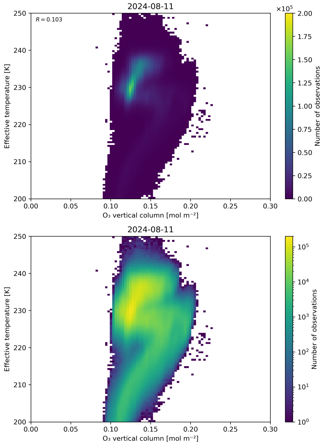
Figure 39: Scatter density plot of “O 3 vertical column” against “Effective temperature” for 2024-08-11 to 2024-08-11.
