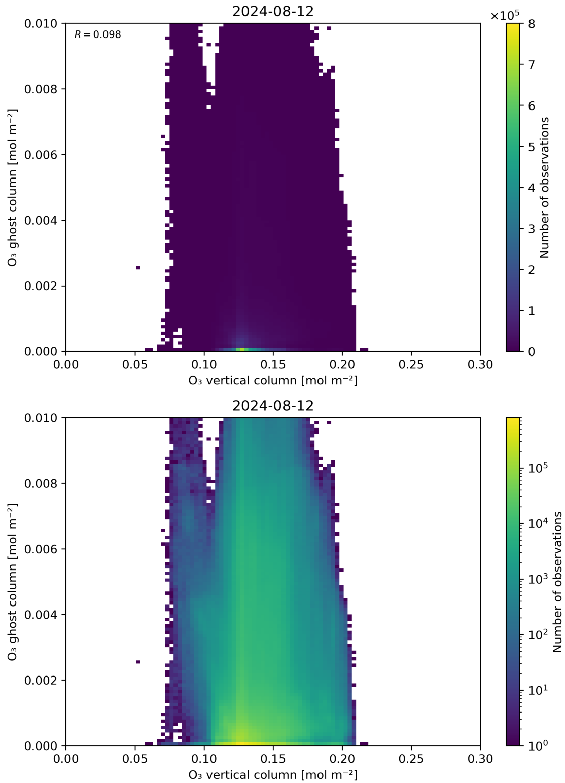
Figure 40: Scatter density plot of “O 3 vertical column” against “O 3 ghost column” for 2024-08-12 to 2024-08-13.
