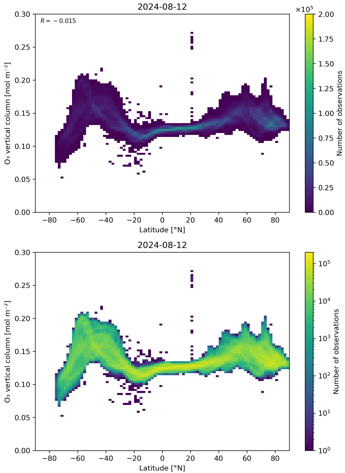
Figure 36: Scatter density plot of “Latitude” against “O 3 vertical column” for 2024-08-12 to 2024-08-13.
