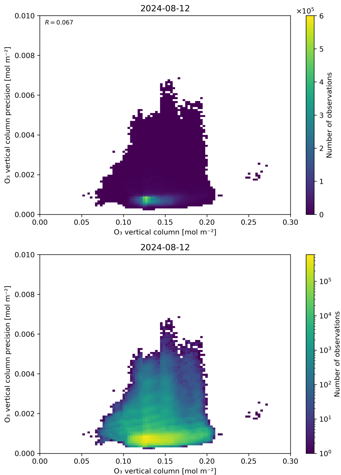
Figure 41: Scatter density plot of “O 3 vertical column” against “O 3 vertical column precision” for 2024-08-12 to 2024-08-13.
