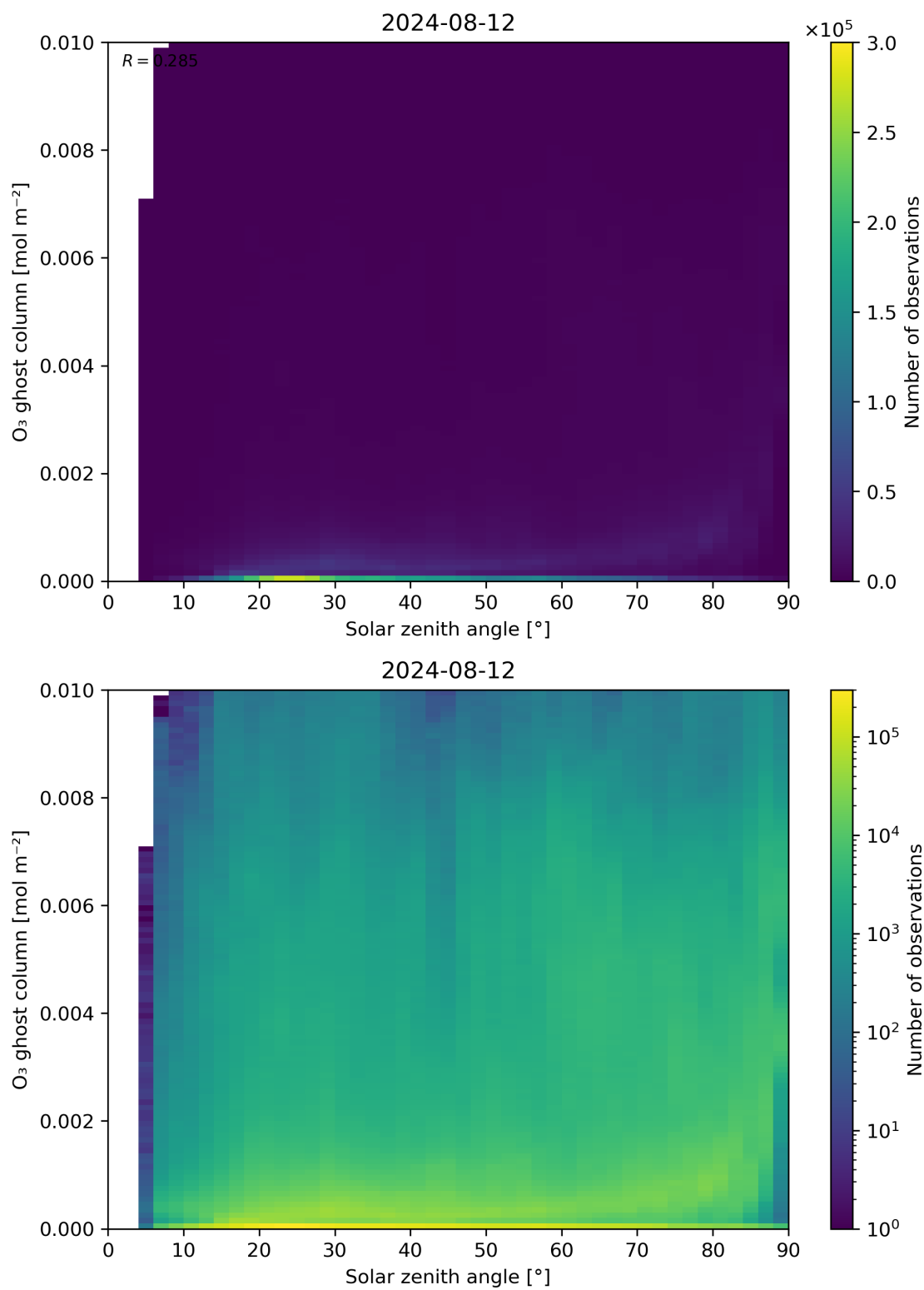
Figure 46: Scatter density plot of “Solar zenith angle” against “O 3 ghost column” for 2024-08-12 to 2024-08-13.
