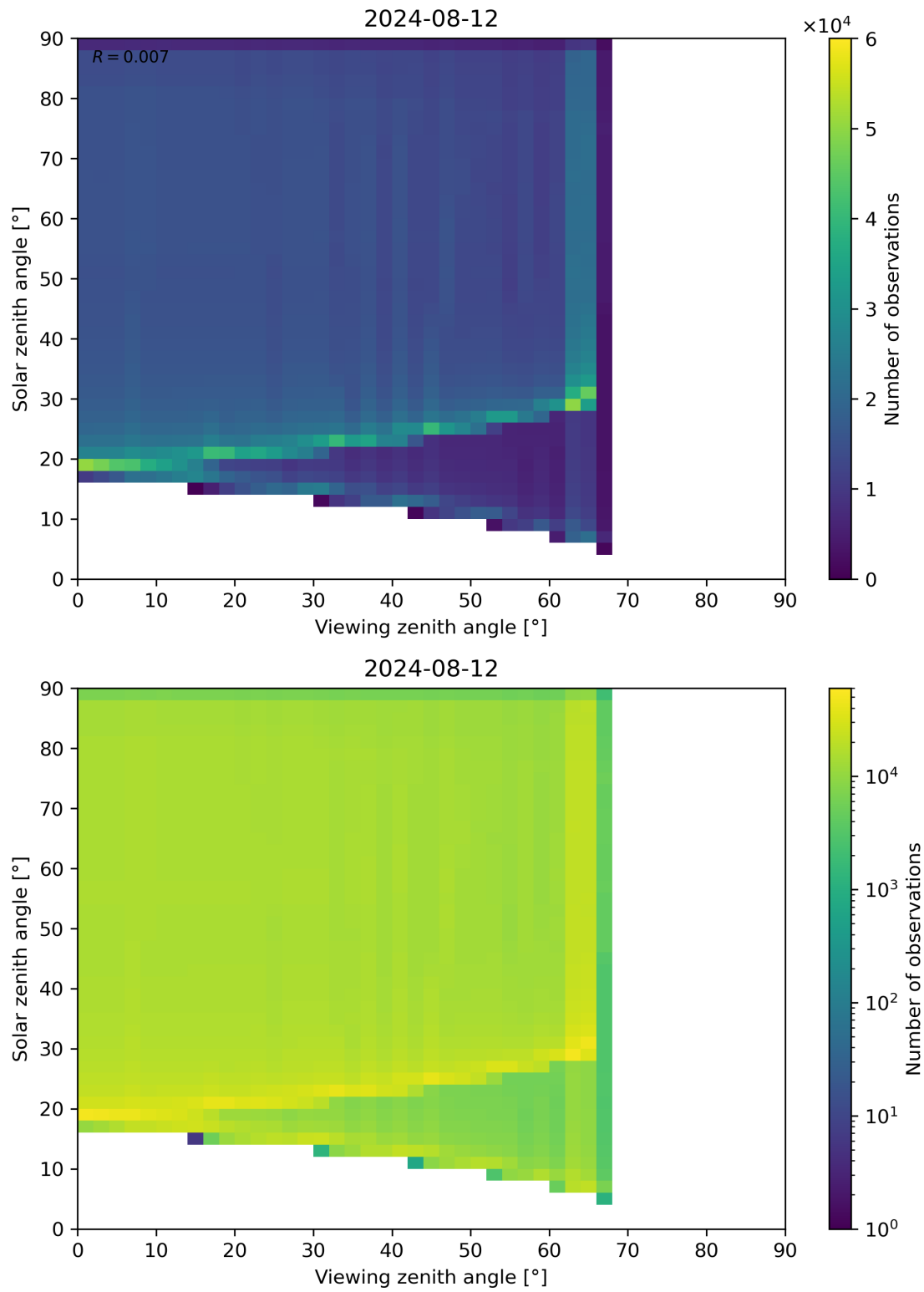
Figure 54: Scatter density plot of “Viewing zenith angle” against “Solar zenith angle” for 2024-08-12 to 2024-08-13.
