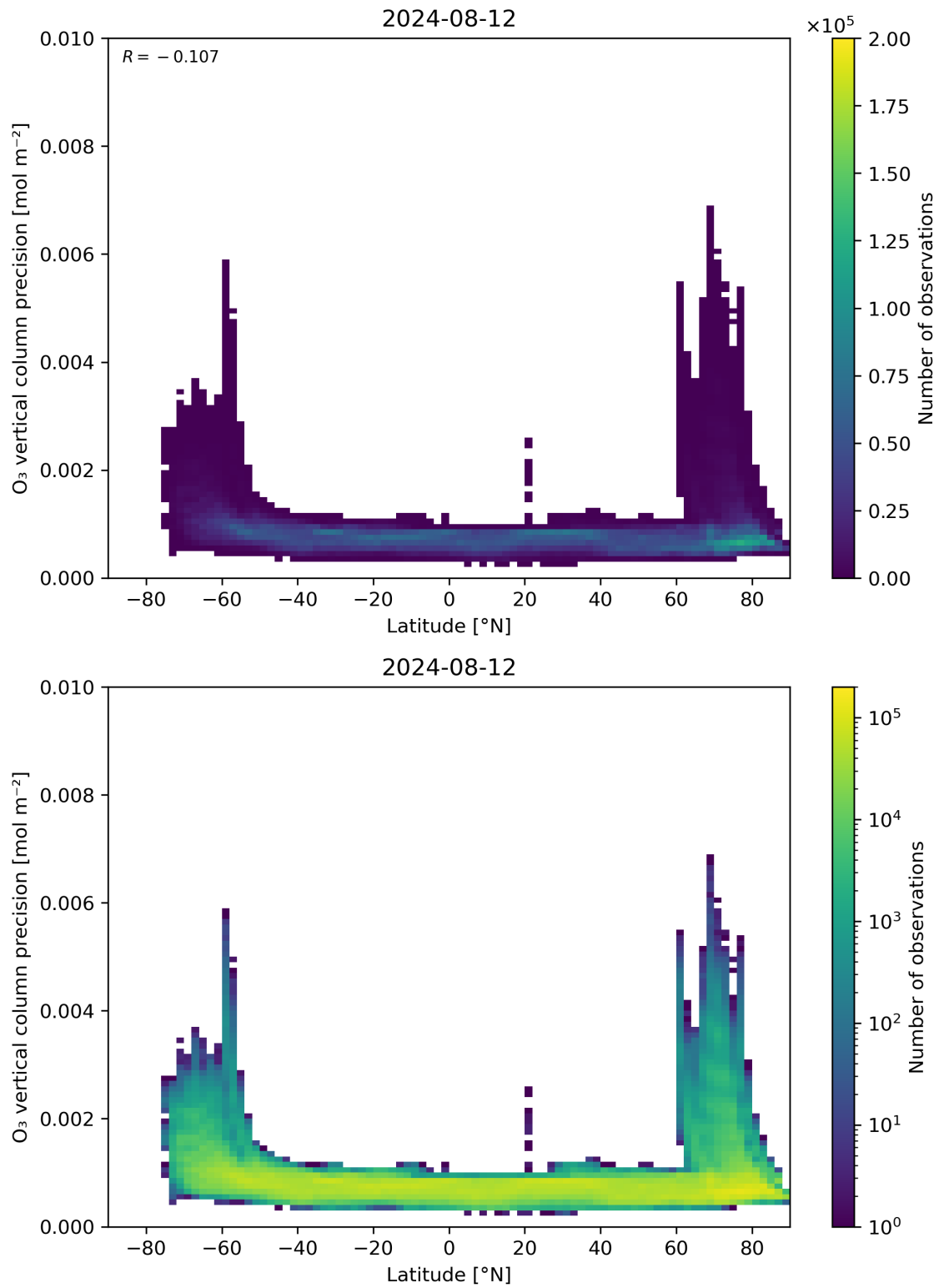
Figure 37: Scatter density plot of “Latitude” against “O 3 vertical column precision” for 2024-08-12 to 2024-08-13.
