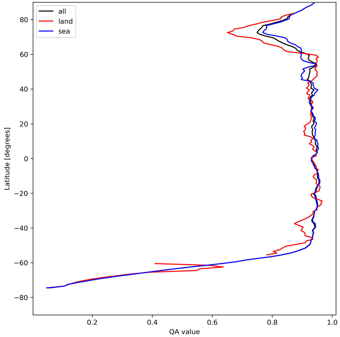
Figure 13: Zonal average of “QA value” for 2024-08-12 to 2024-08-13.
