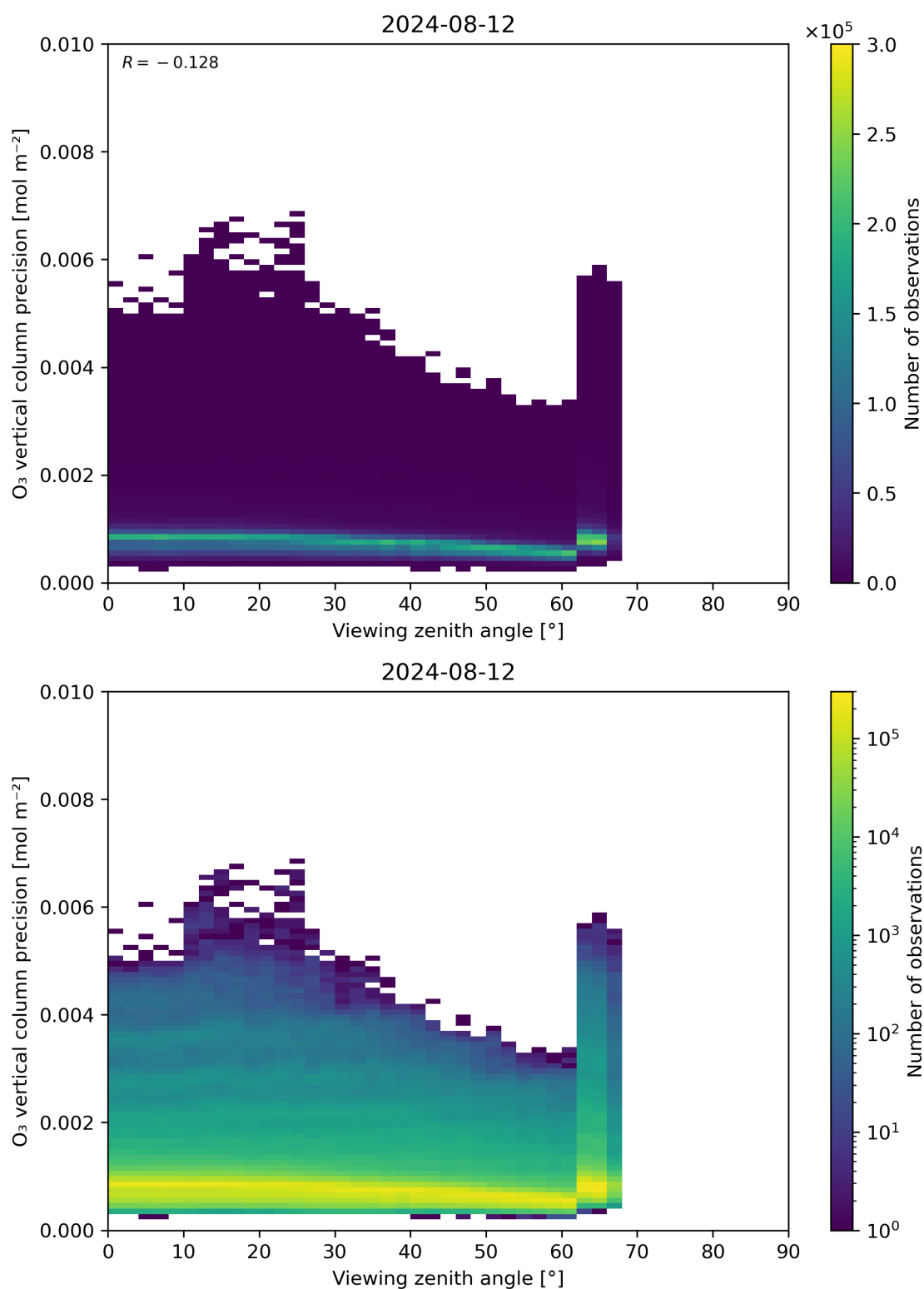
Figure 53: Scatter density plot of “Viewing zenith angle” against “O 3 vertical column precision” for 2024-08-12 to 2024-08-13.
