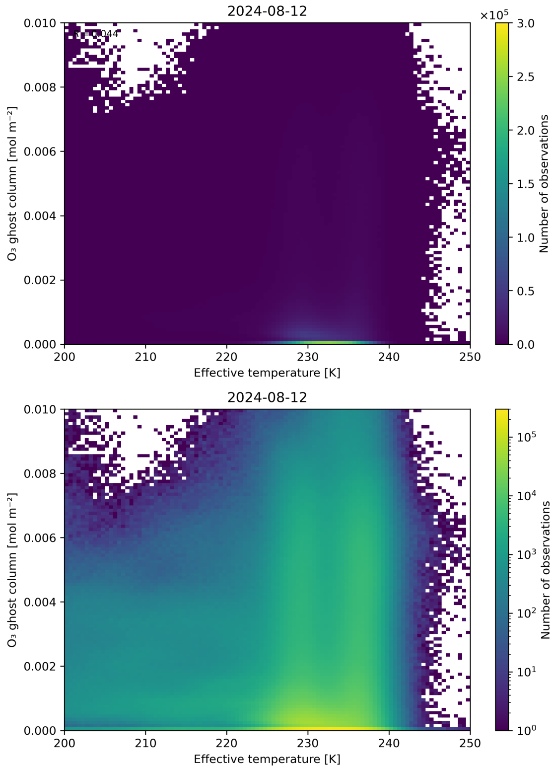
Figure 38: Scatter density plot of “Effective temperature” against “O 3 ghost column” for 2024-08-12 to 2024-08-13.
