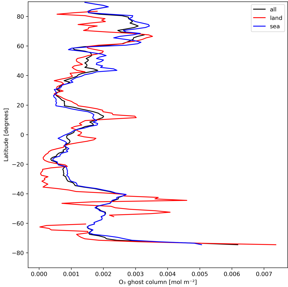
Figure 18: Zonal average of "O 3 ghost column" for 2024-08-12 to 2024-08-13.
