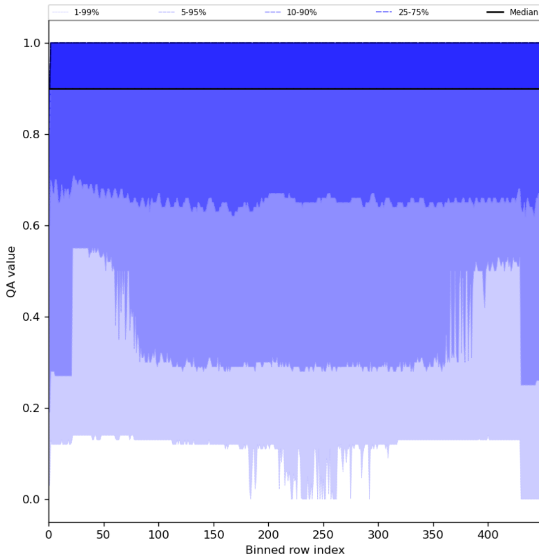
Figure 27: Along track statistics of “QA value” for 2024-08-12 to 2024-08-13
