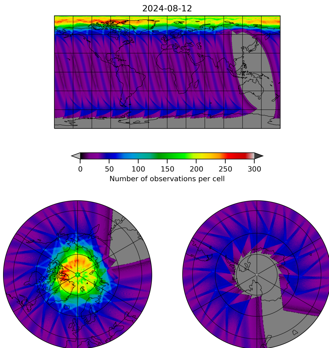
Figure 12: Map of the number of observations for 2024-08-12 to 2024-08-13
