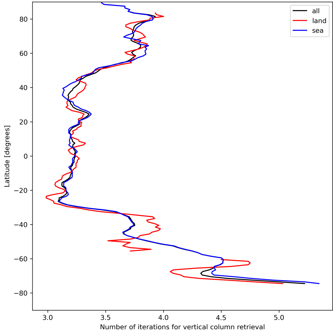
Figure 19: Zonal average of “Number of iterations for vertical column retrieval” for 2024-08-12 to 2024-08-13.
