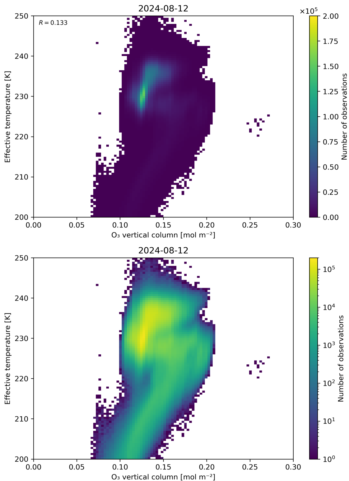
Figure 39: Scatter density plot of “O 3 vertical column” against “Effective temperature” for 2024-08-12 to 2024-08-13.
