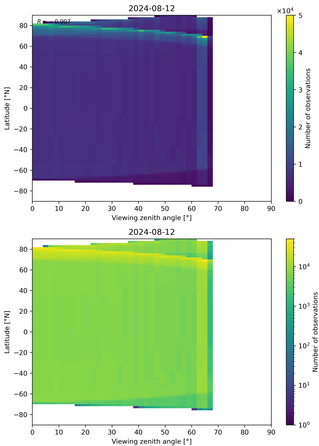
Figure 49: Scatter density plot of “Viewing zenith angle” against “Latitude” for 2024-08-12 to 2024-08-13.
