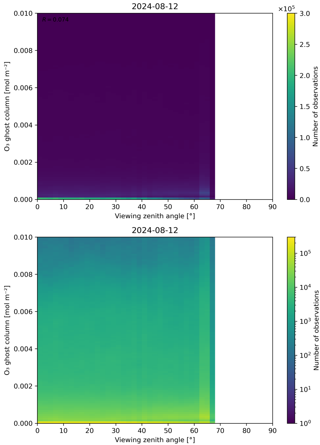
Figure 51: Scatter density plot of “Viewing zenith angle” against “O 3 ghost column” for 2024-08-12 to 2024-08-13.
