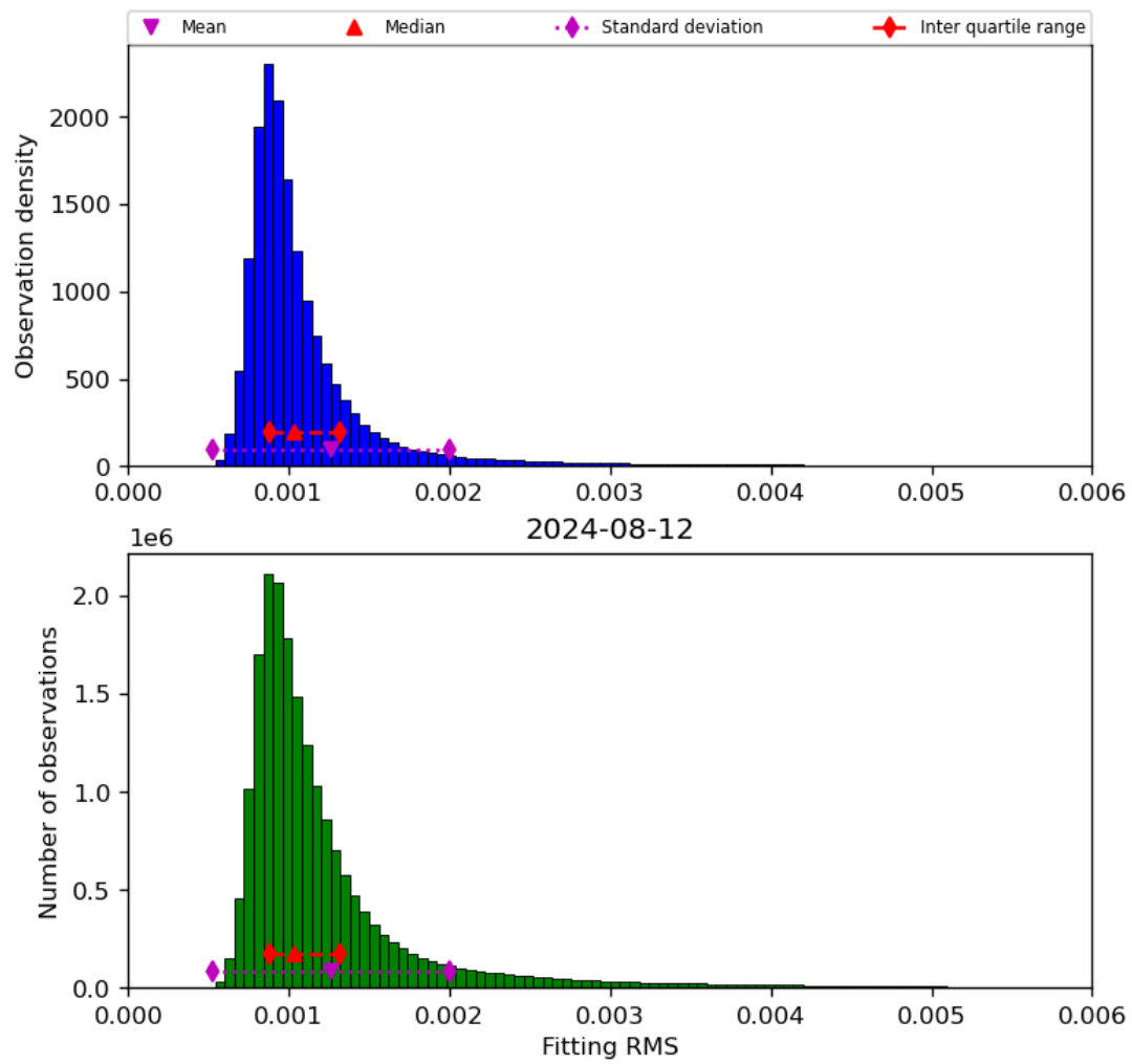
Figure 23: Histogram of “Fitting RMS” for 2024-08-12 to 2024-08-13
