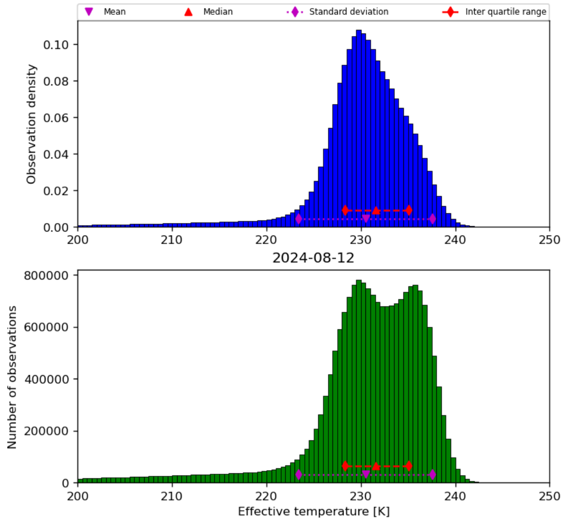
Figure 24: Histogram of “Effective temperature” for 2024-08-12 to 2024-08-13
