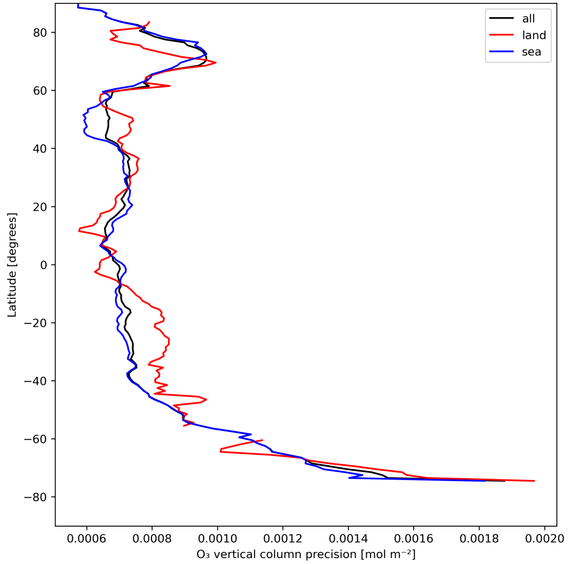
Figure 15: Zonal average of “O 3 vertical column precision” for 2024-08-12 to 2024-08-13.
