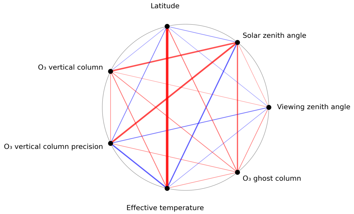
Figure 1: Map of correlation graph for 2024-08-12 to 2024-08-13.
