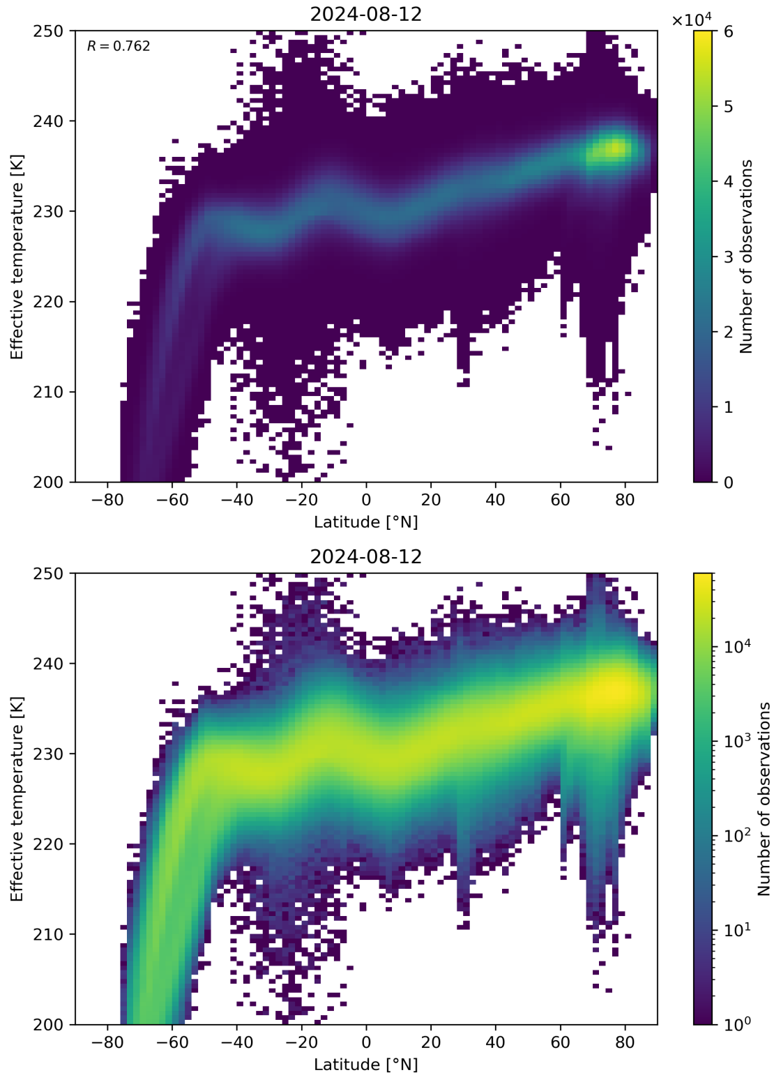
Figure 34: Scatter density plot of “Latitude” against “Effective temperature” for 2024-08-12 to 2024-08-13.
