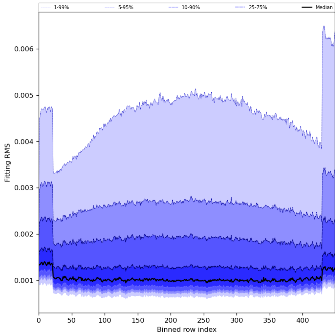
Figure 30: Along track statistics of “Fitting RMS” for 2024-08-12 to 2024-08-13
