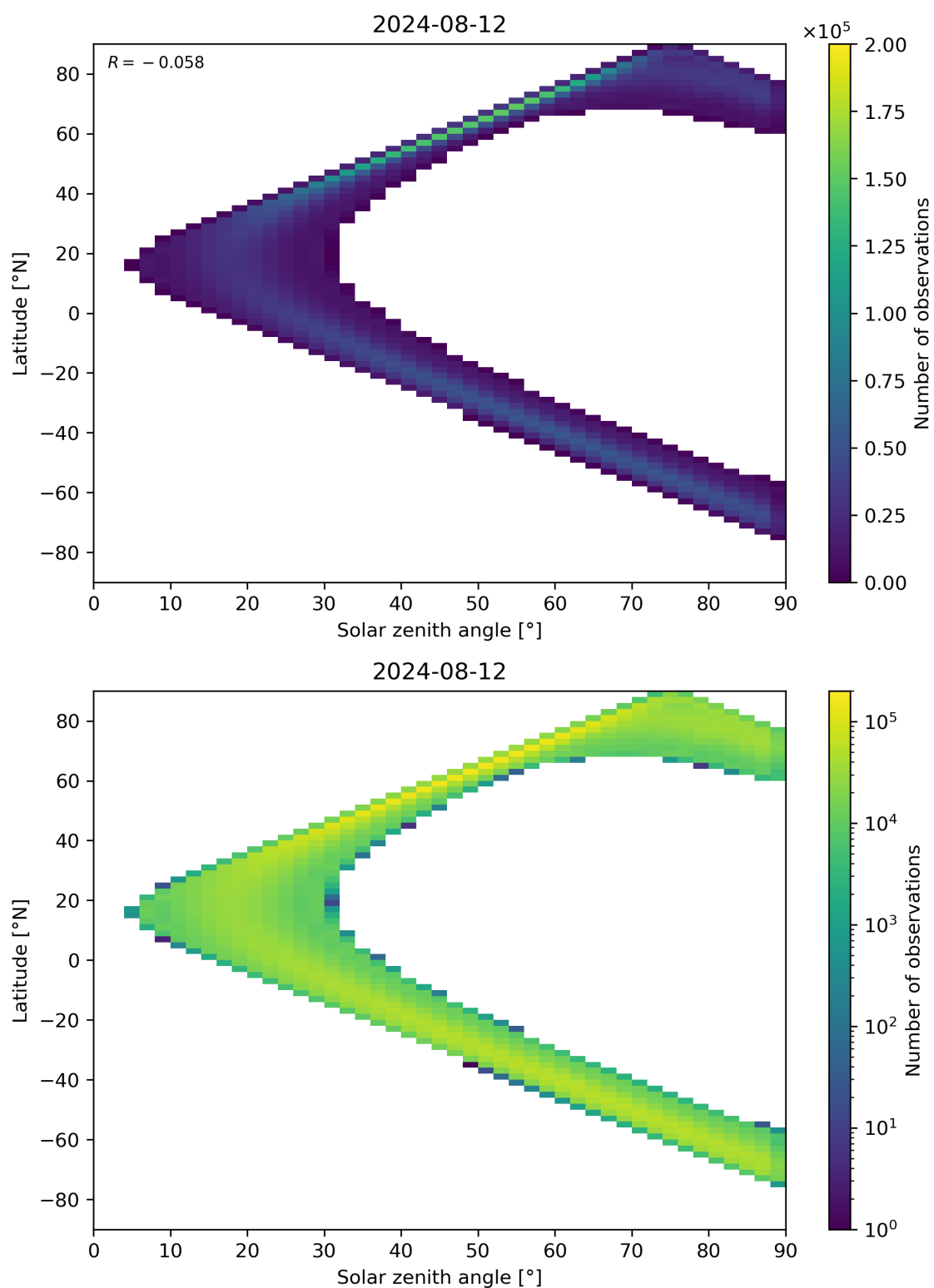
Figure 44: Scatter density plot of “Solar zenith angle” against “Latitude” for 2024-08-12 to 2024-08-13.
