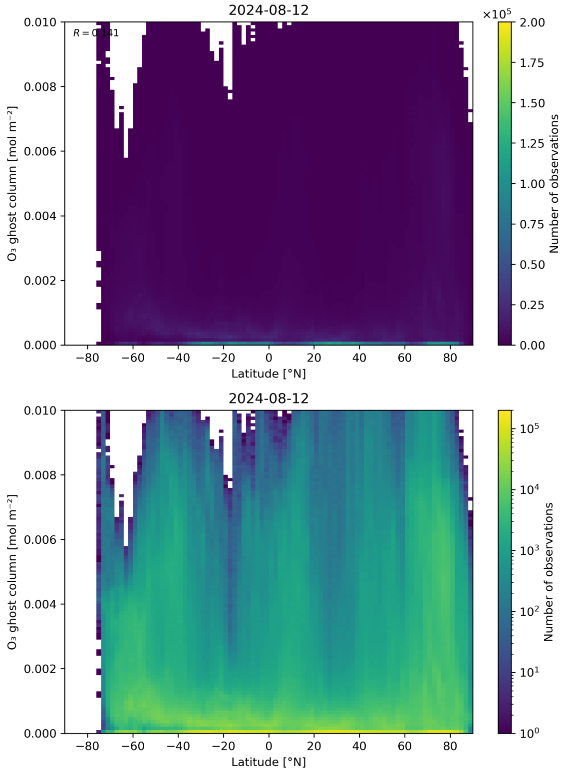
Figure 35: Scatter density plot of “Latitude” against “O 3 ghost column” for 2024-08-12 to 2024-08-13.
