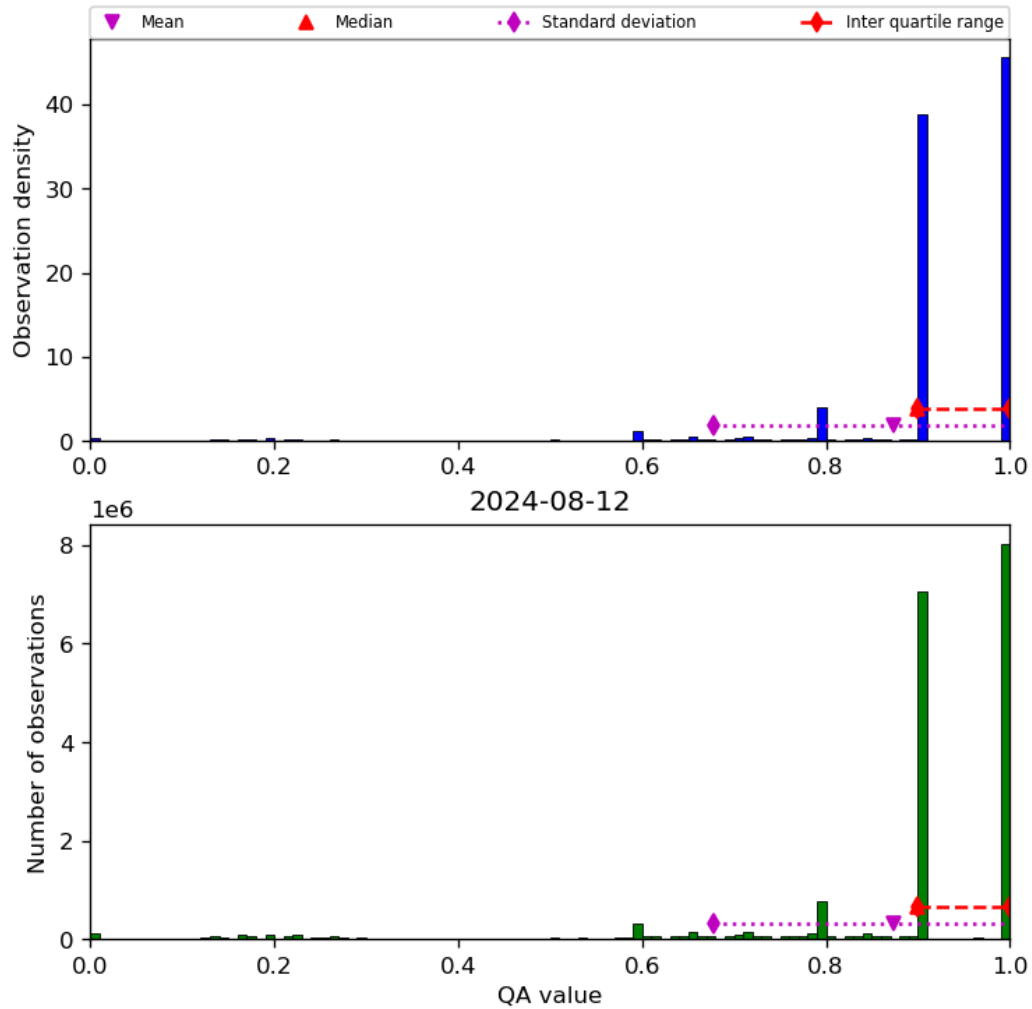
Figure 20: Histogram of “QA value” for 2024-08-12 to 2024-08-13
