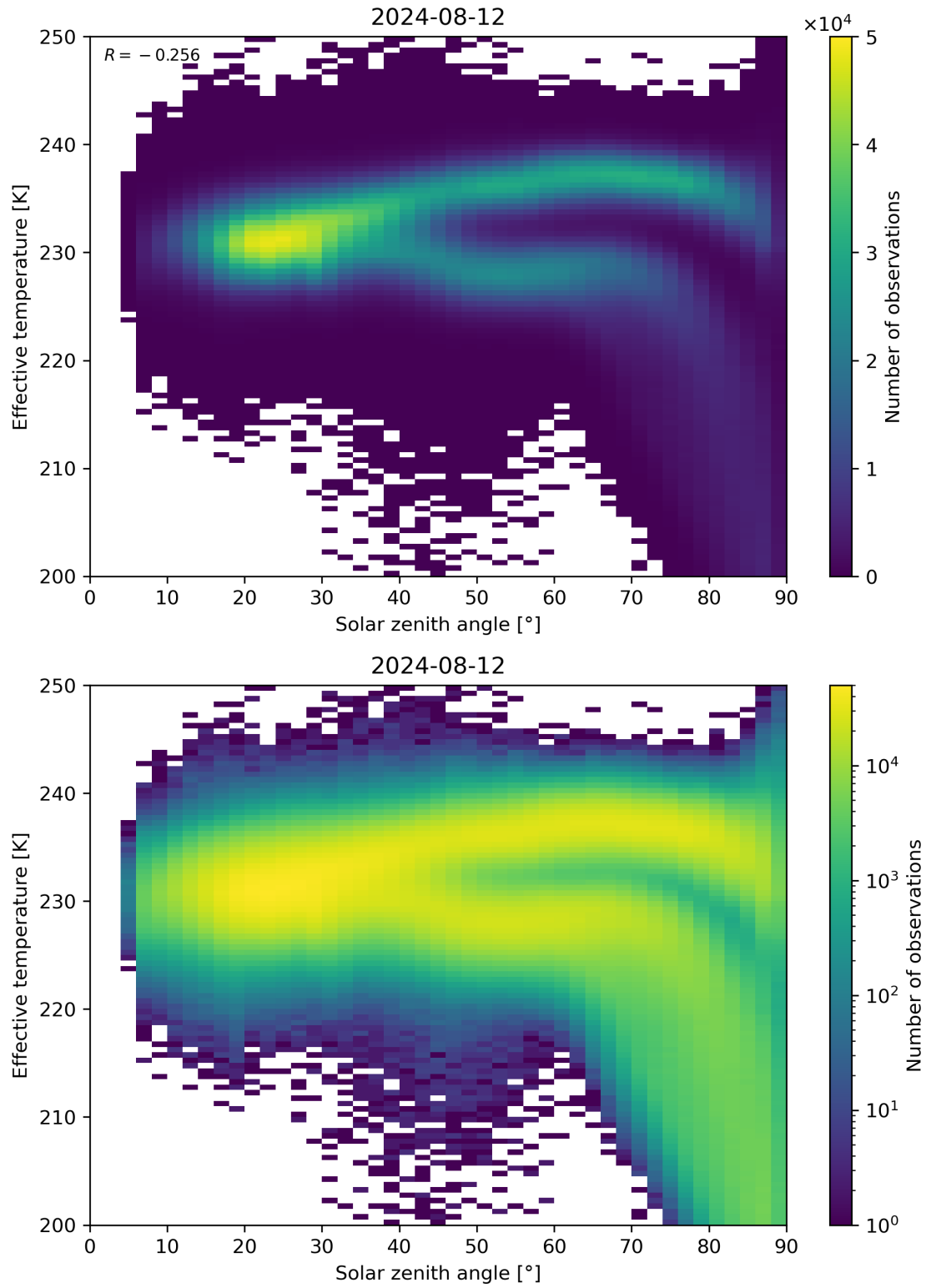
Figure 45: Scatter density plot of “Solar zenith angle” against “Effective temperature” for 2024-08-12 to 2024-08-13.
