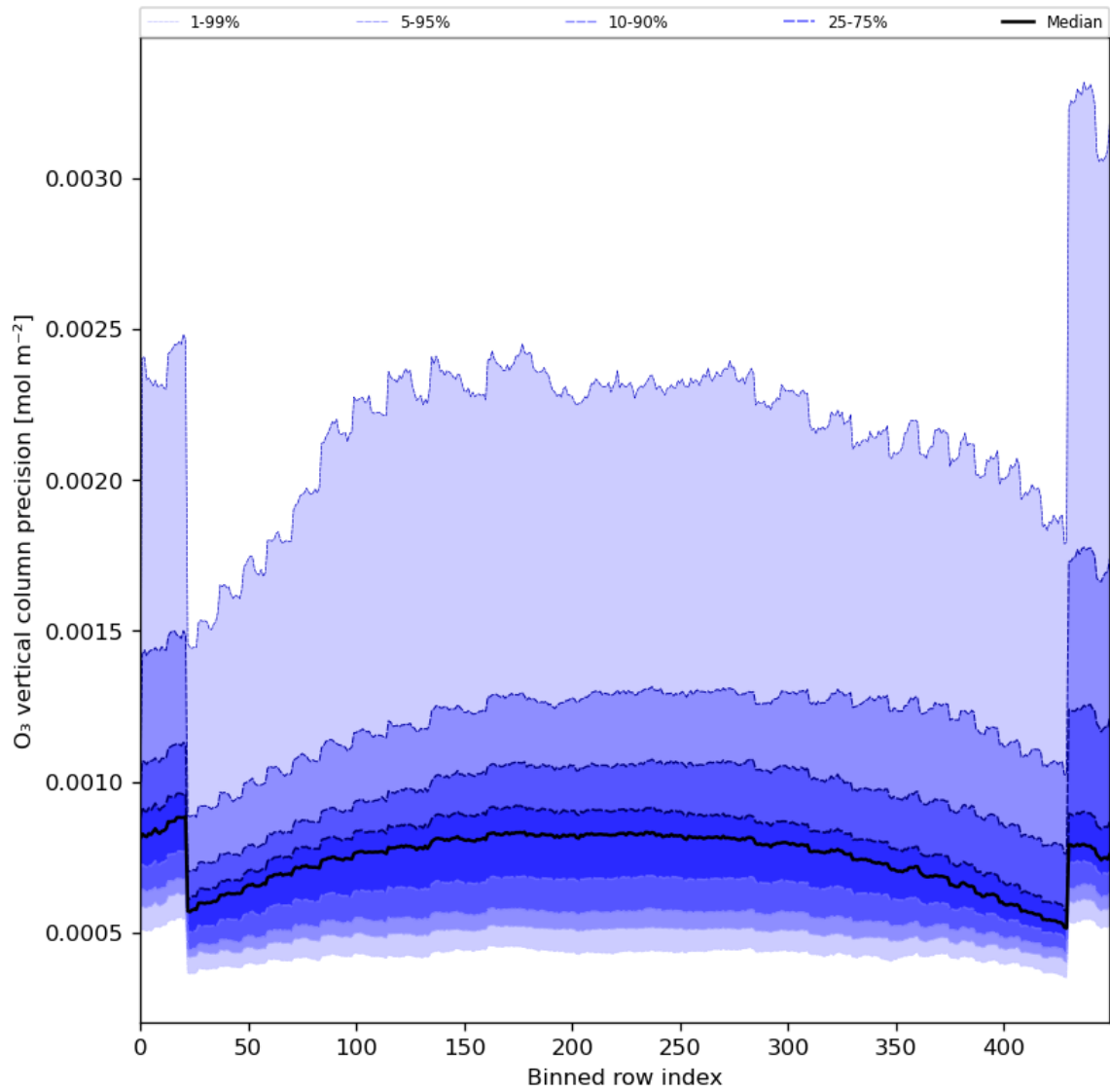
Figure 29: Along track statistics of “O 3 vertical column precision” for 2024-08-12 to 2024-08-13
