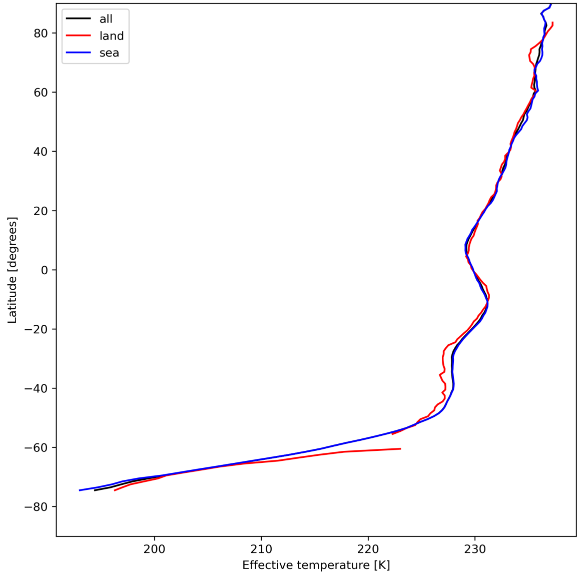
Figure 17: Zonal average of "Effective temperature" for 2024-08-12 to 2024-08-13.
