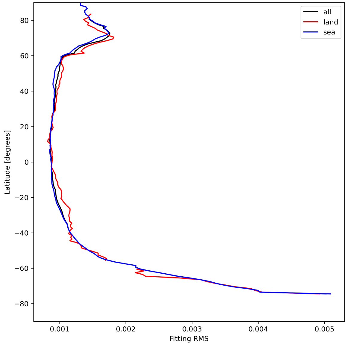
Figure 16: Zonal average of “Fitting RMS” for 2024-08-12 to 2024-08-13.
