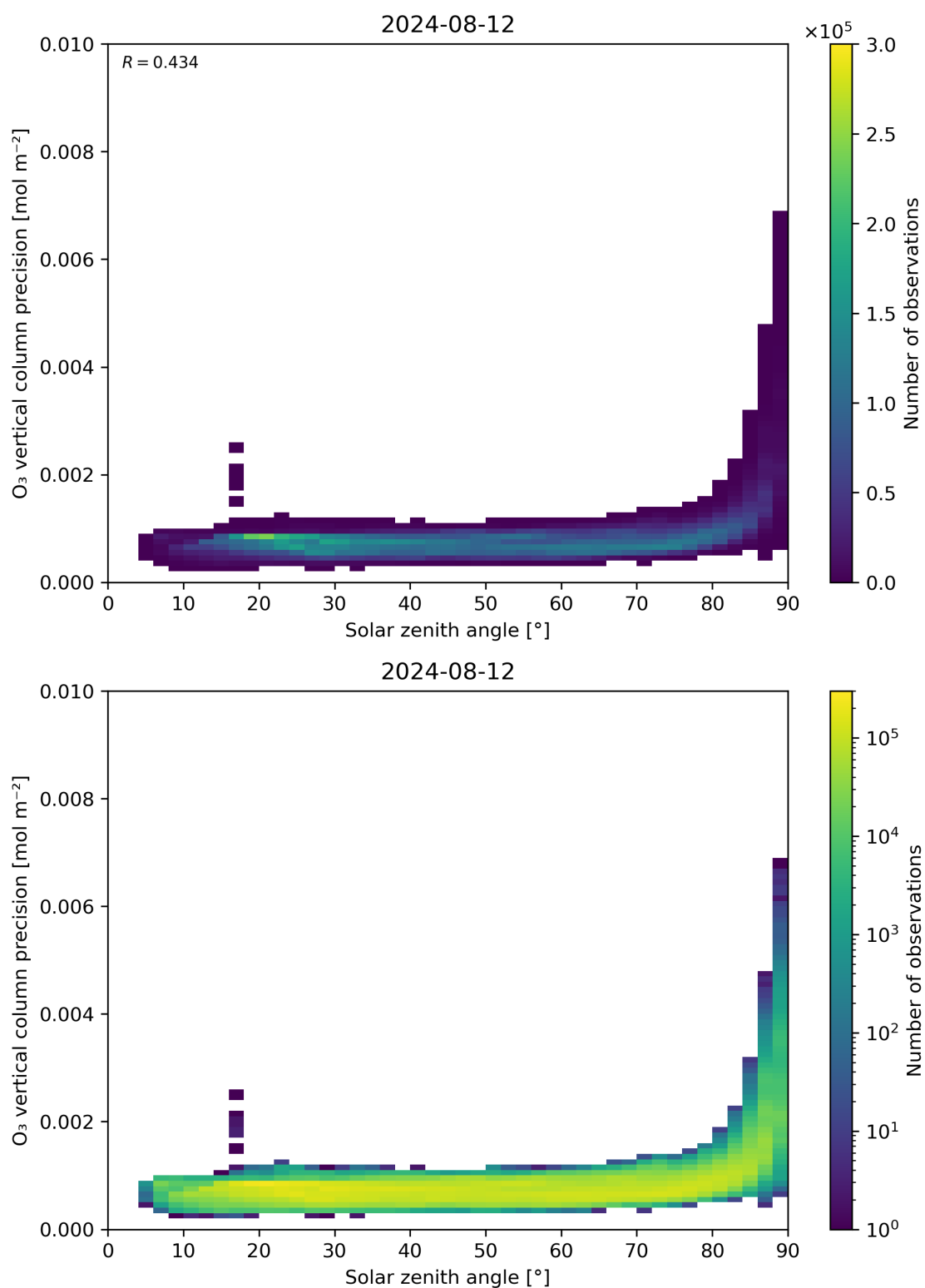
Figure 48: Scatter density plot of “Solar zenith angle” against “O 3 vertical column precision” for 2024-08-12 to 2024-08-13.
