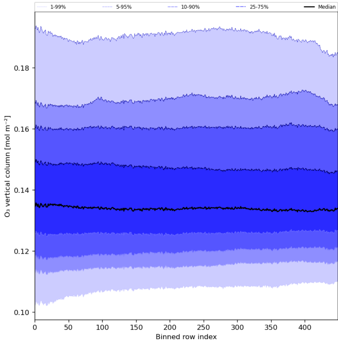
Figure 28: Along track statistics of “O 3 vertical column” for 2024-08-12 to 2024-08-13
