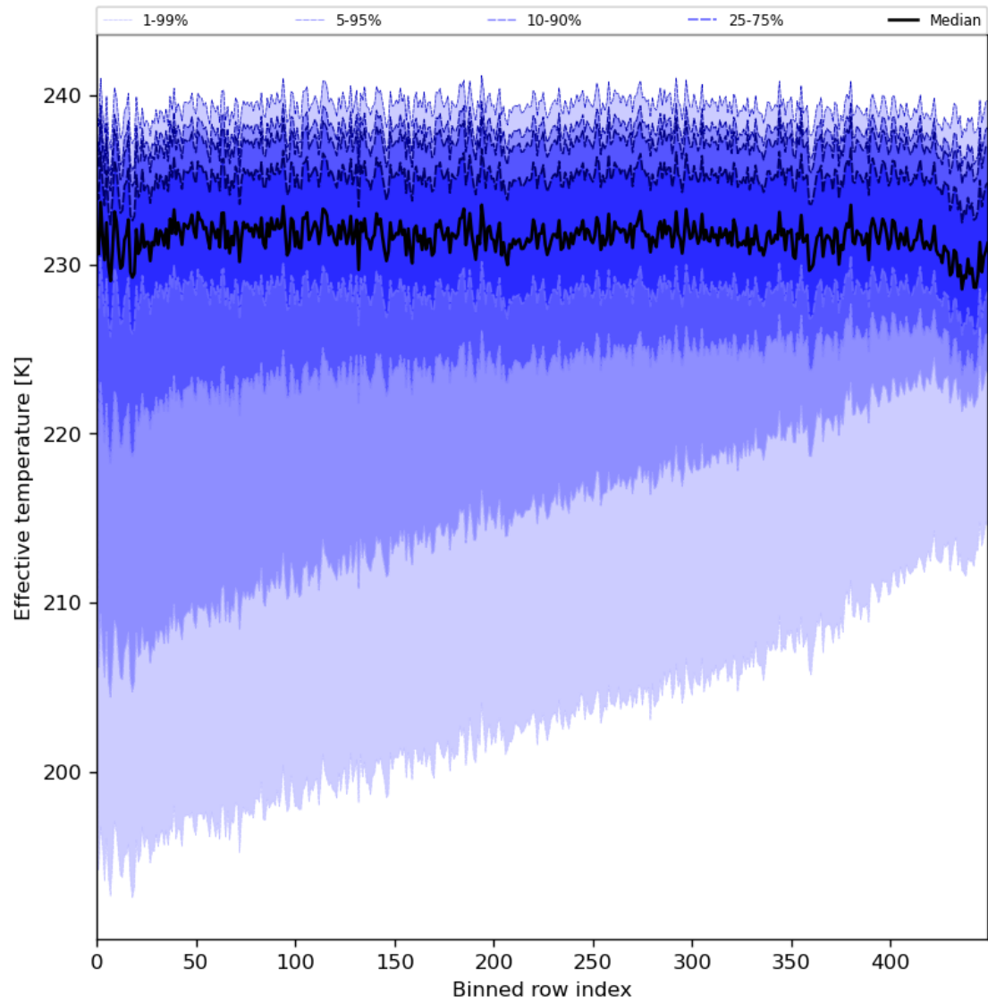
Figure 31: Along track statistics of “Effective temperature” for 2024-08-12 to 2024-08-13
