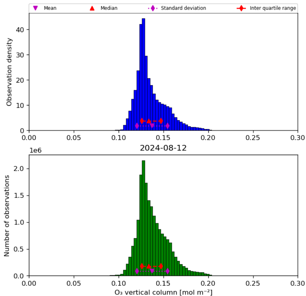
Figure 21: Histogram of “O 3 vertical column” for 2024-08-12 to 2024-08-13
