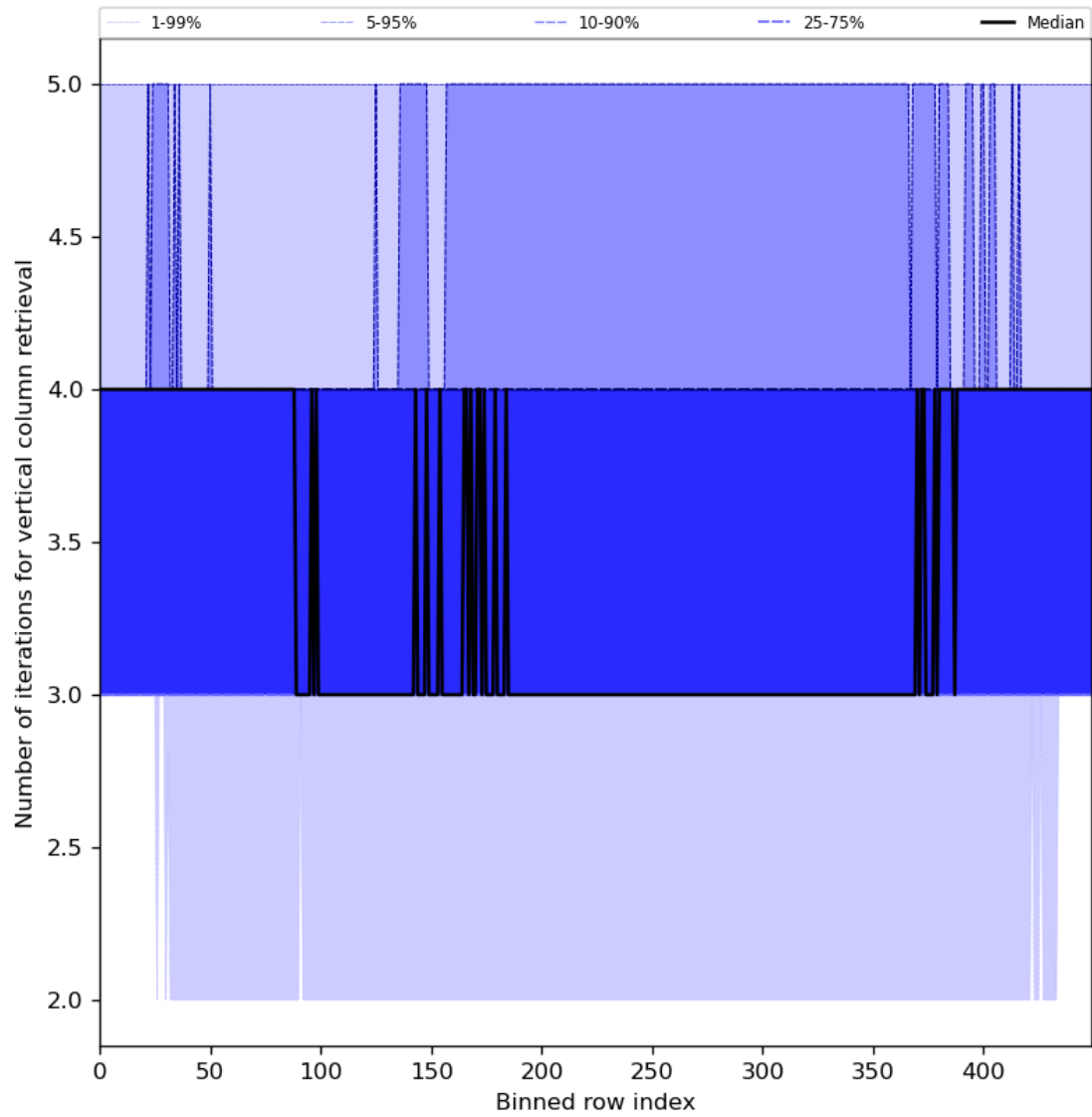
Figure 33: Along track statistics of “Number of iterations for vertical column retrieval” for 2024-08-12 to 2024-08-13
