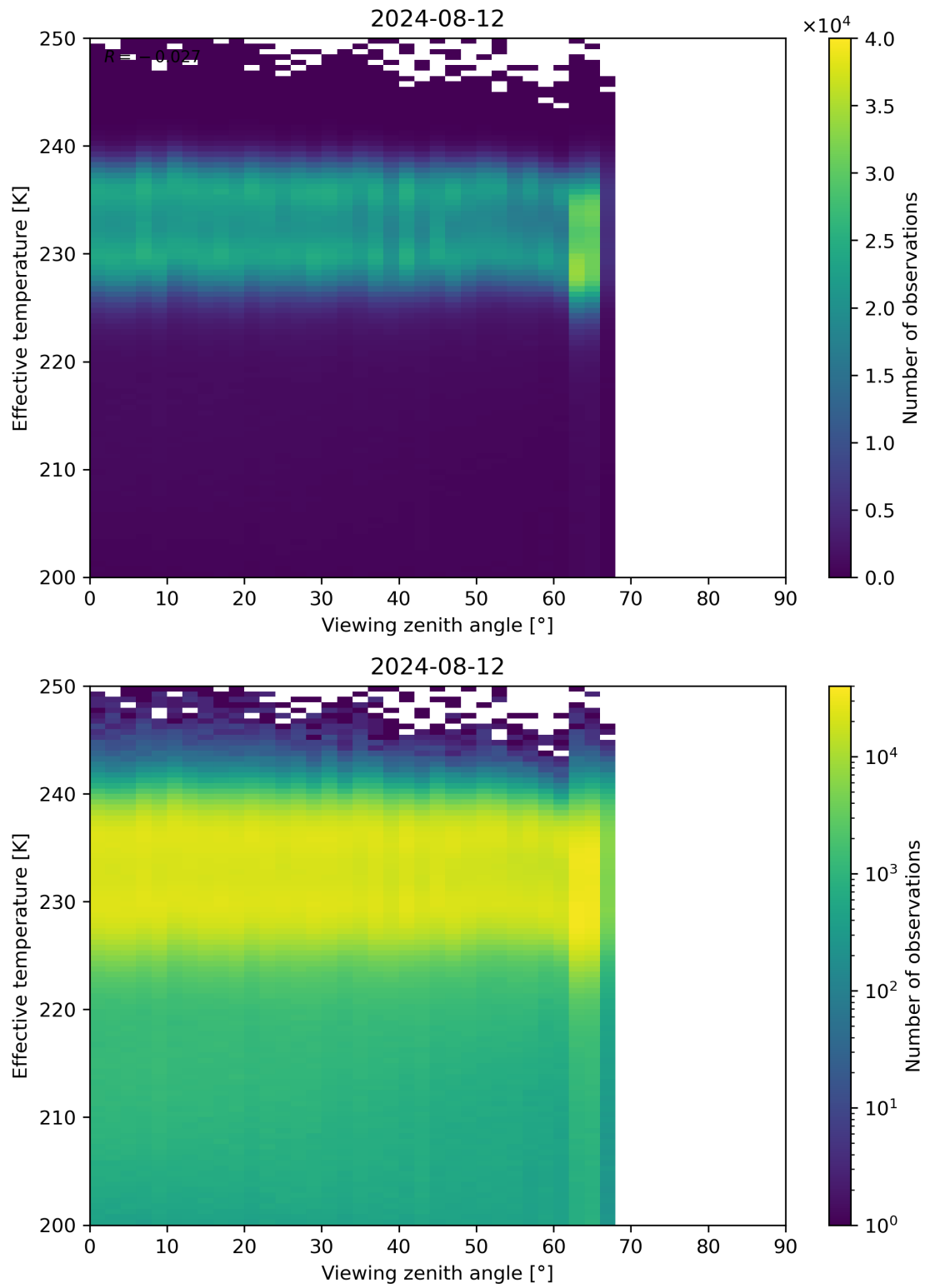
Figure 50: Scatter density plot of “Viewing zenith angle” against “Effective temperature” for 2024-08-12 to 2024-08-13.
