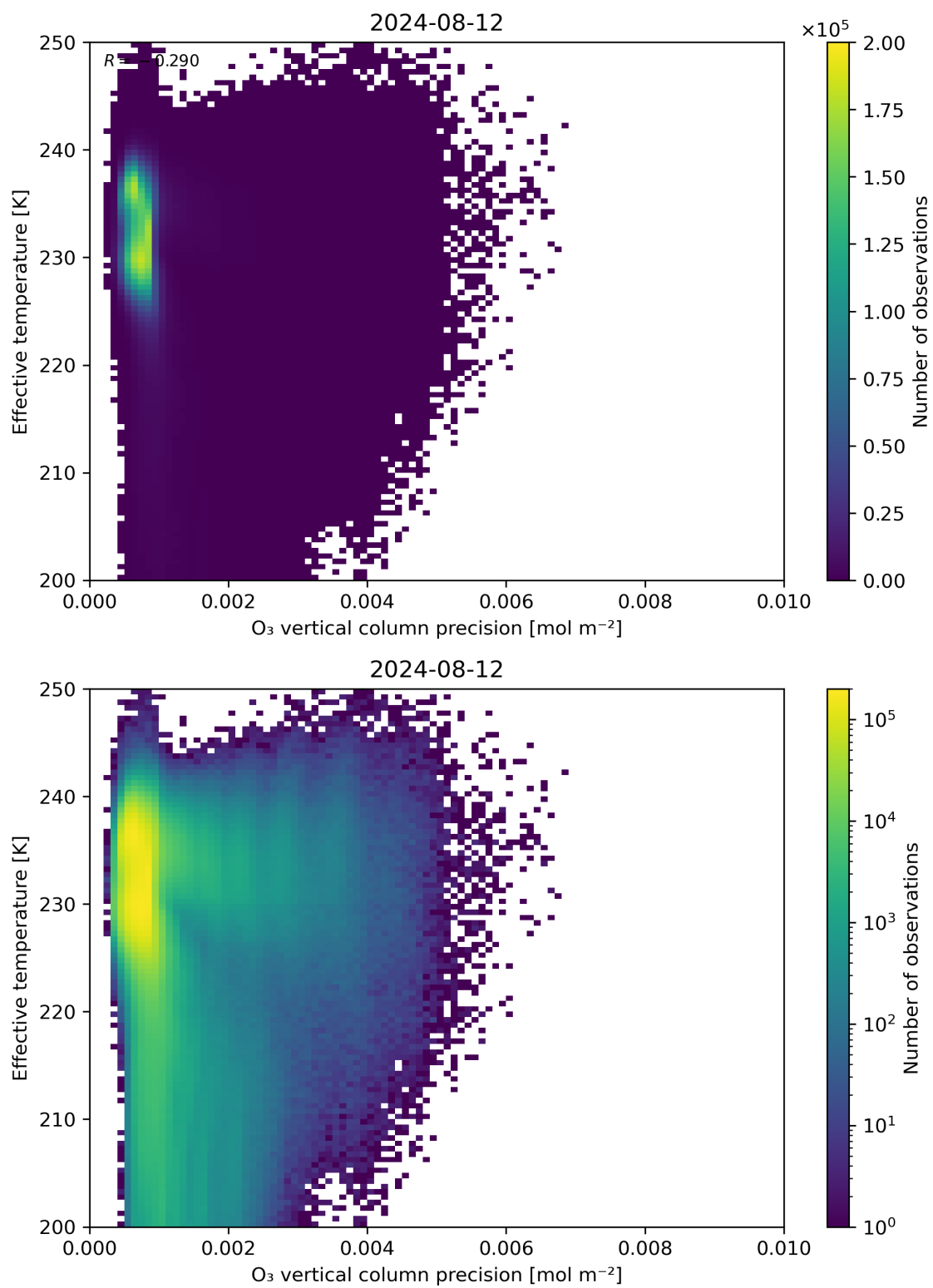
Figure 42: Scatter density plot of “O 3 vertical column precision” against “Effective temperature” for 2024-08-12 to 2024-08-13.
