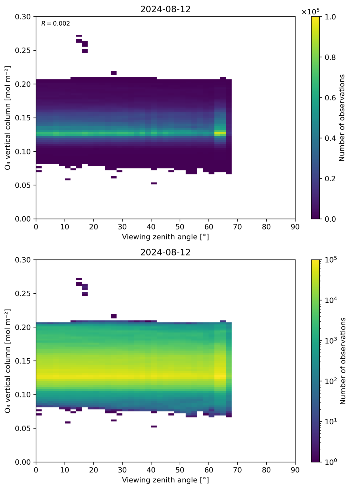
Figure 52: Scatter density plot of “Viewing zenith angle” against “O 3 vertical column” for 2024-08-12 to 2024-08-13.
