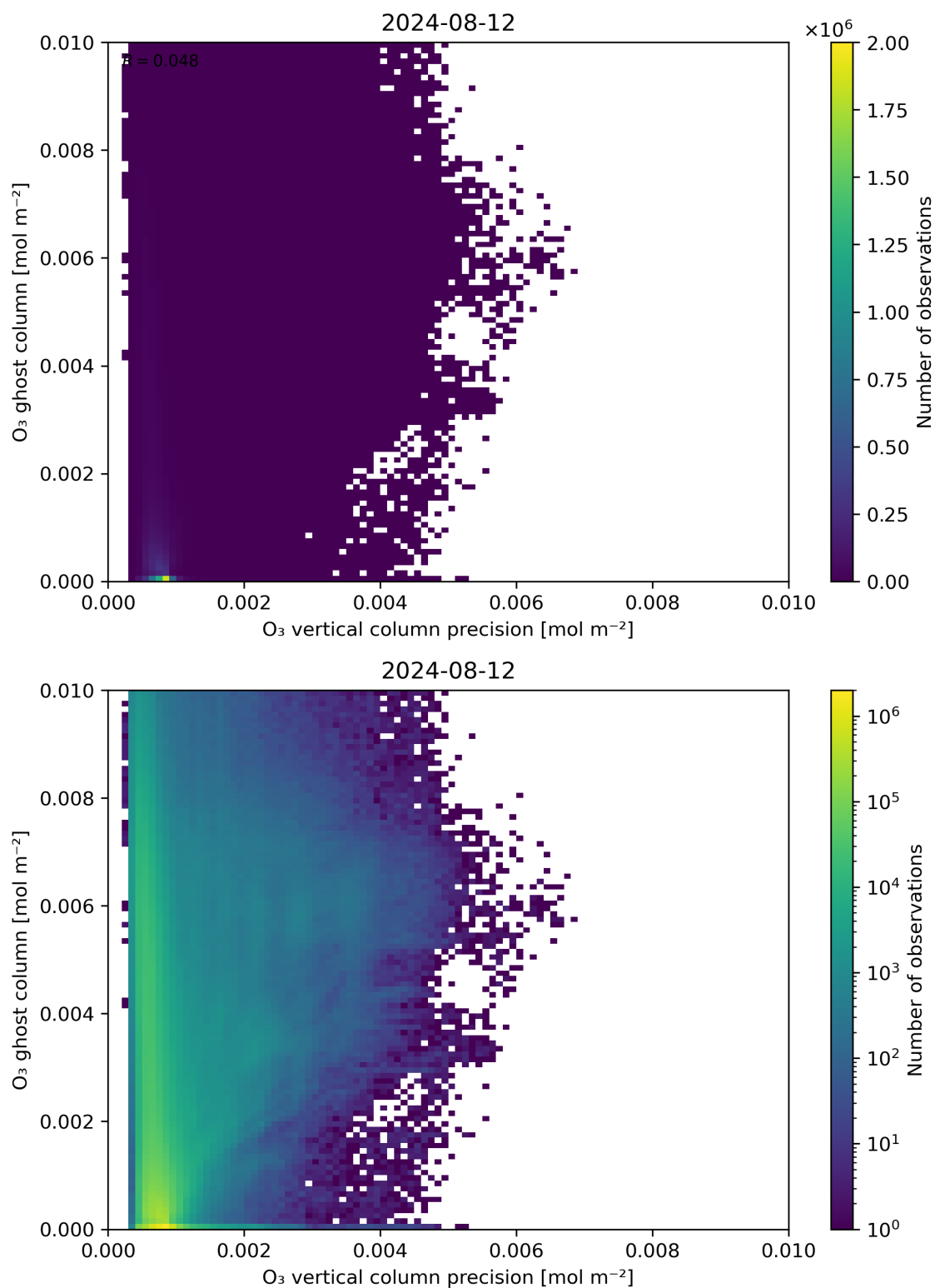
Figure 43: Scatter density plot of “O 3 vertical column precision” against “O 3 ghost column” for 2024-08-12 to 2024-08-13.
