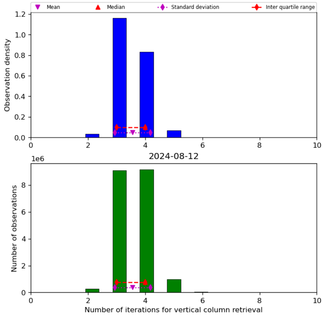
Figure 26: Histogram of “Number of iterations for vertical column retrieval” for 2024-08-12 to 2024-08-13
