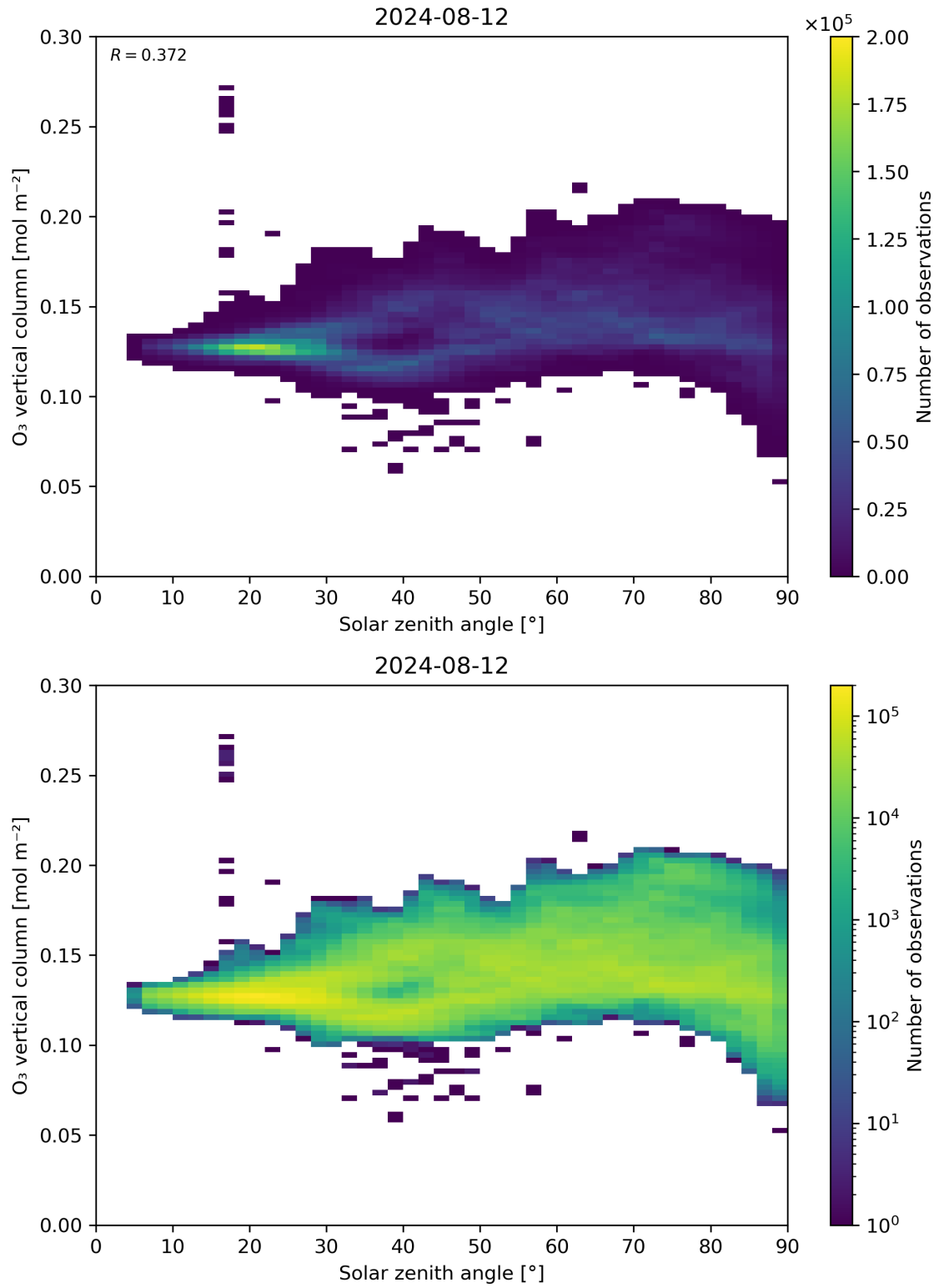
Figure 47: Scatter density plot of “Solar zenith angle” against “O 3 vertical column” for 2024-08-12 to 2024-08-13.
