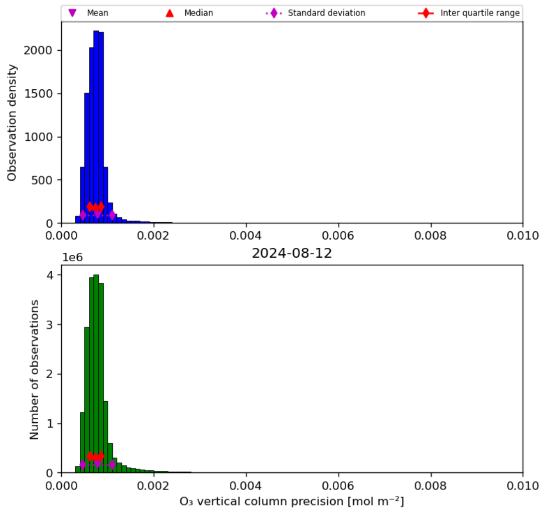
Figure 22: Histogram of “O 3 vertical column precision” for 2024-08-12 to 2024-08-13
