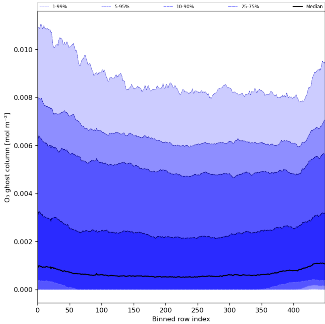
Figure 32: Along track statistics of “O 3 ghost column” for 2024-08-12 to 2024-08-13
