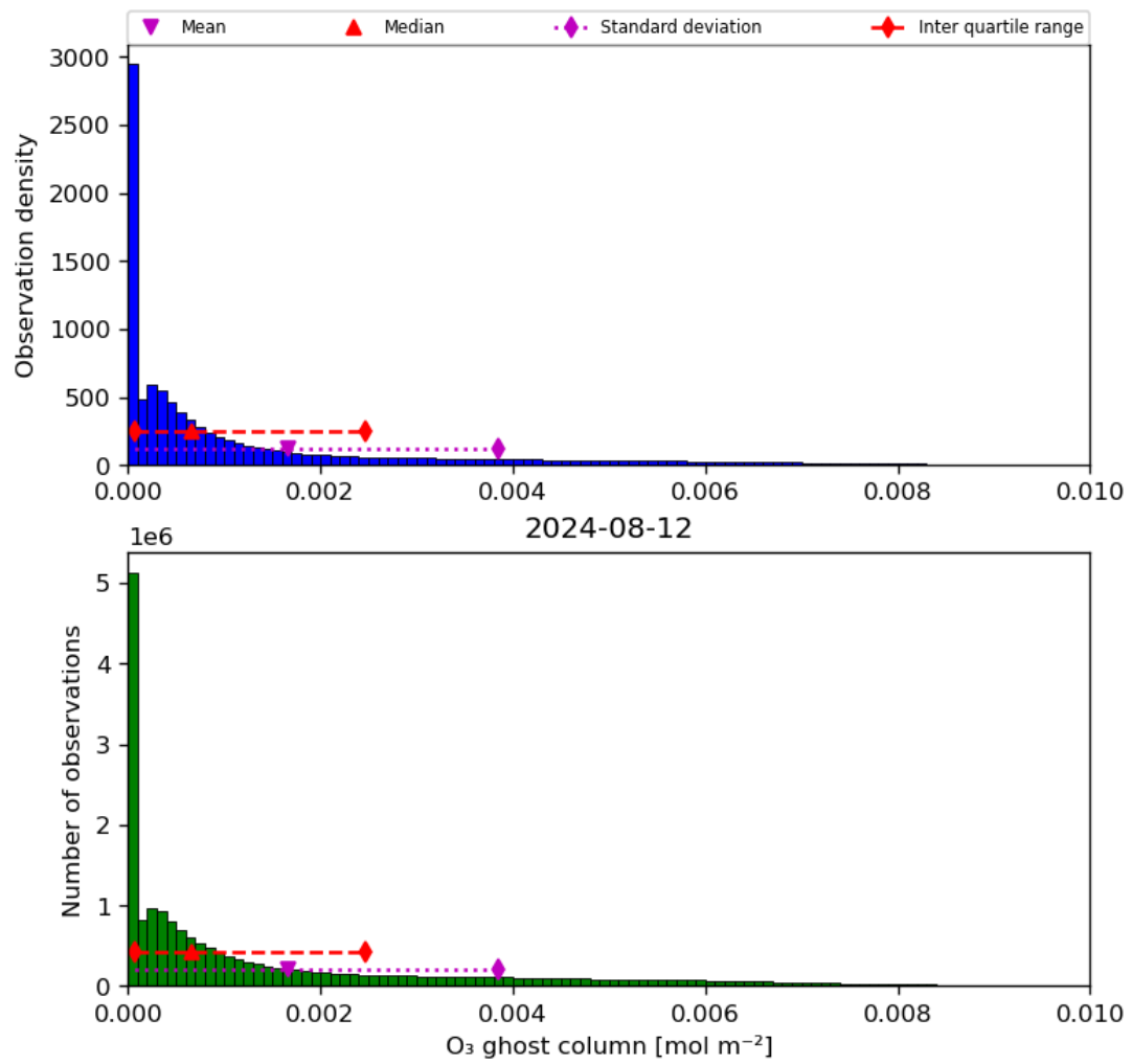
Figure 25: Histogram of “O 3 ghost column” for 2024-08-12 to 2024-08-13
