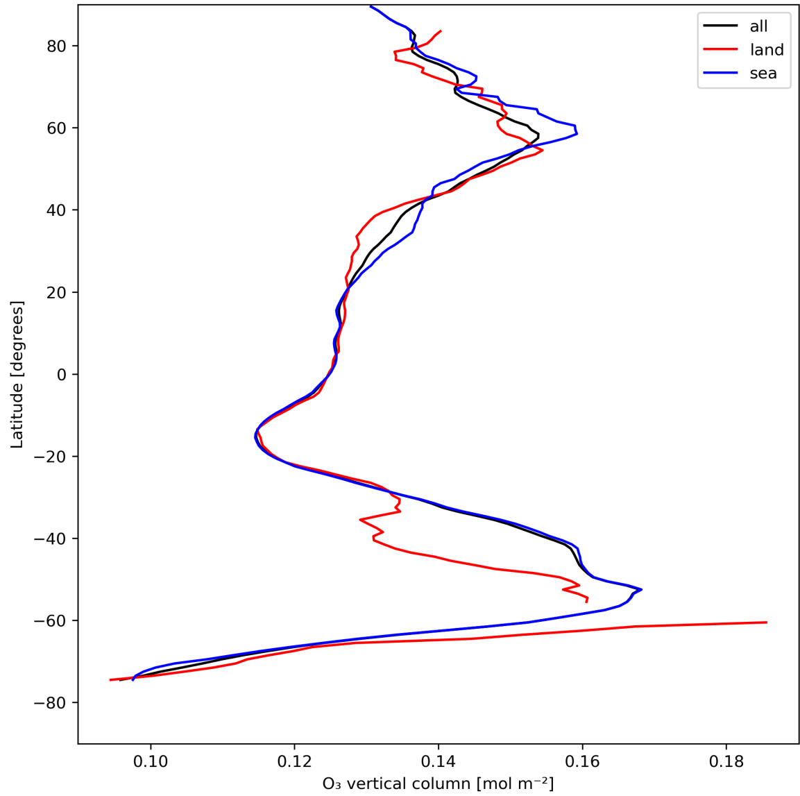
Figure 14: Zonal average of “O 3 vertical column” for 2024-08-12 to 2024-08-13.
