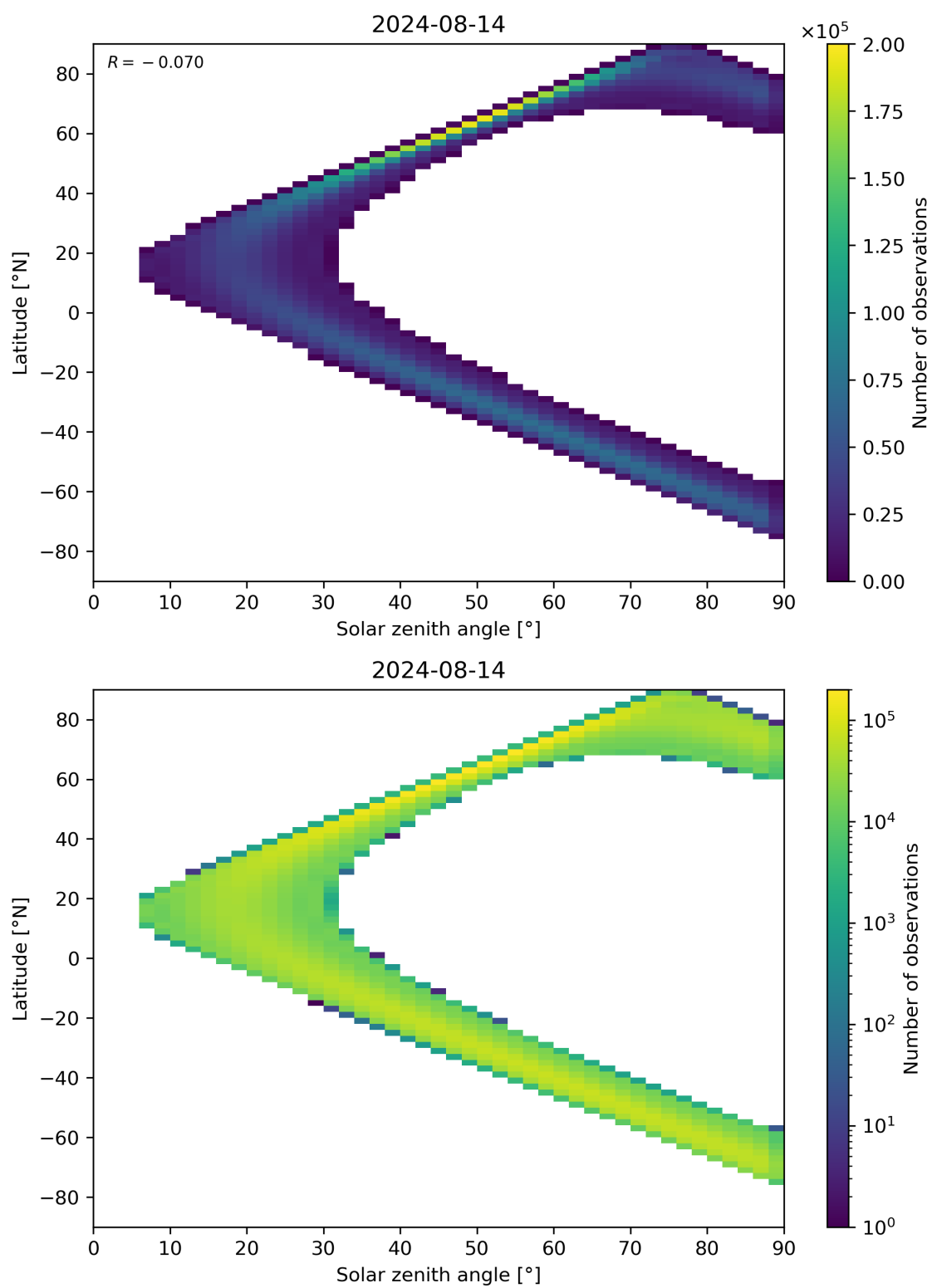
Figure 44: Scatter density plot of “Solar zenith angle” against “Latitude” for 2024-08-13 to 2024-08-15.
