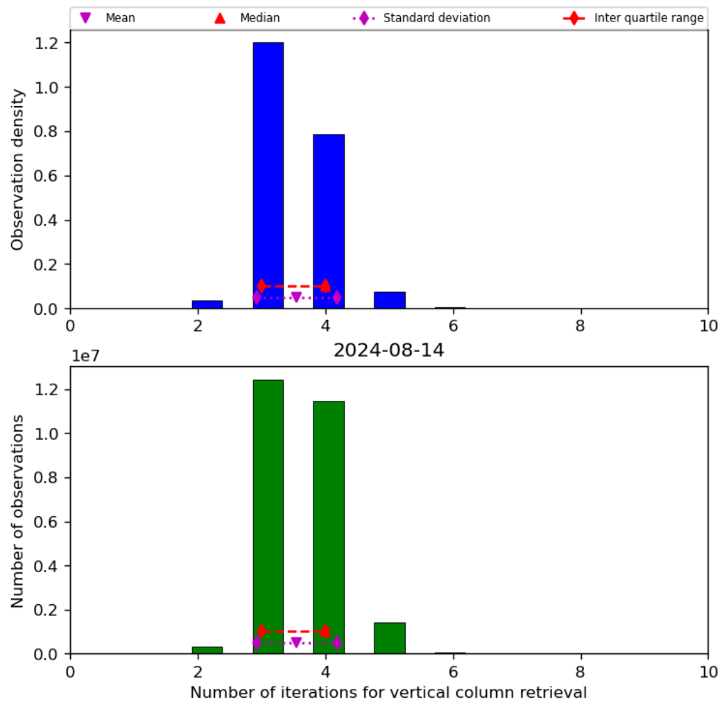
Figure 26: Histogram of “Number of iterations for vertical column retrieval” for 2024-08-13 to 2024-08-15
