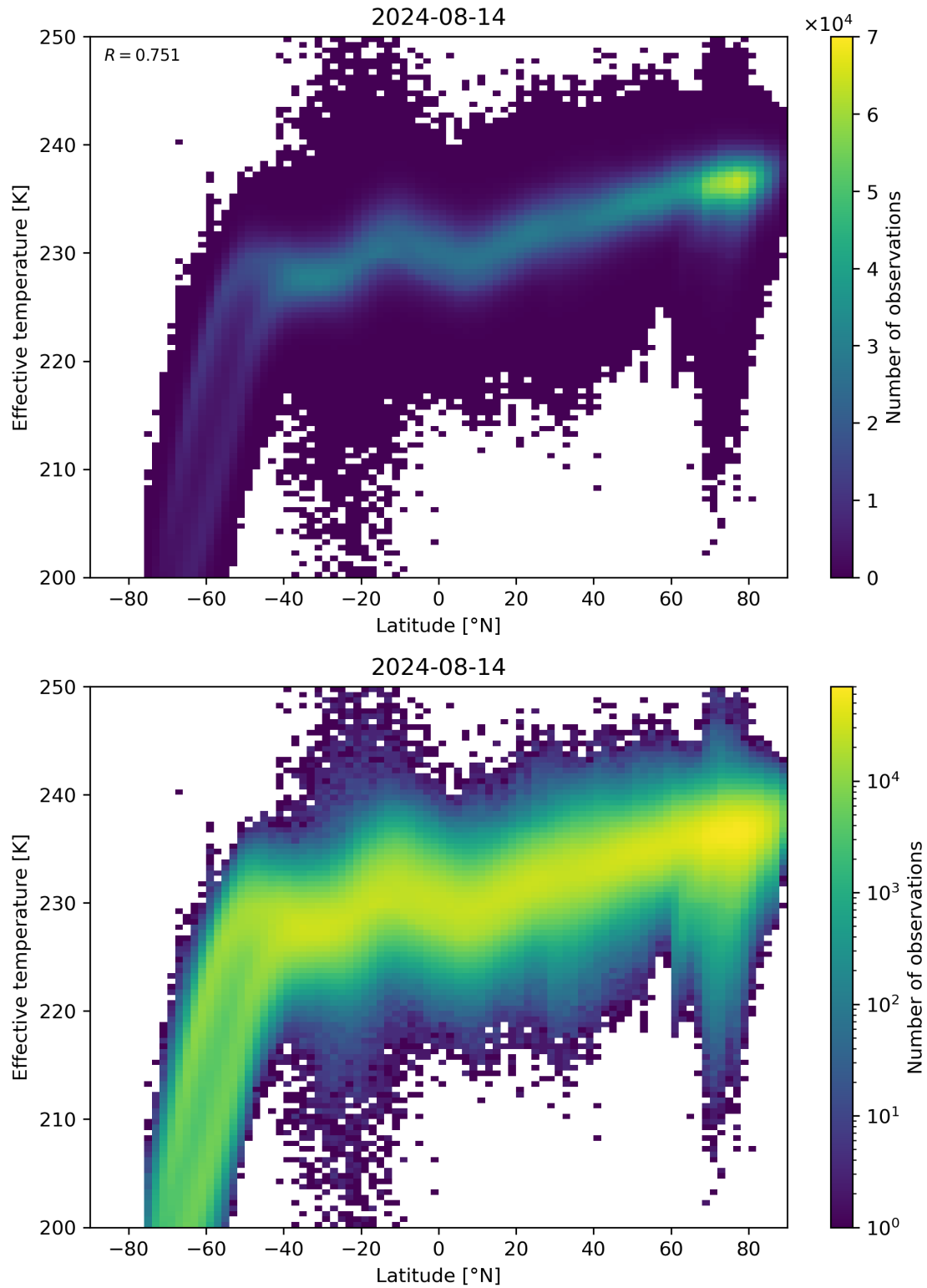
Figure 34: Scatter density plot of “Latitude” against “Effective temperature” for 2024-08-13 to 2024-08-15.
