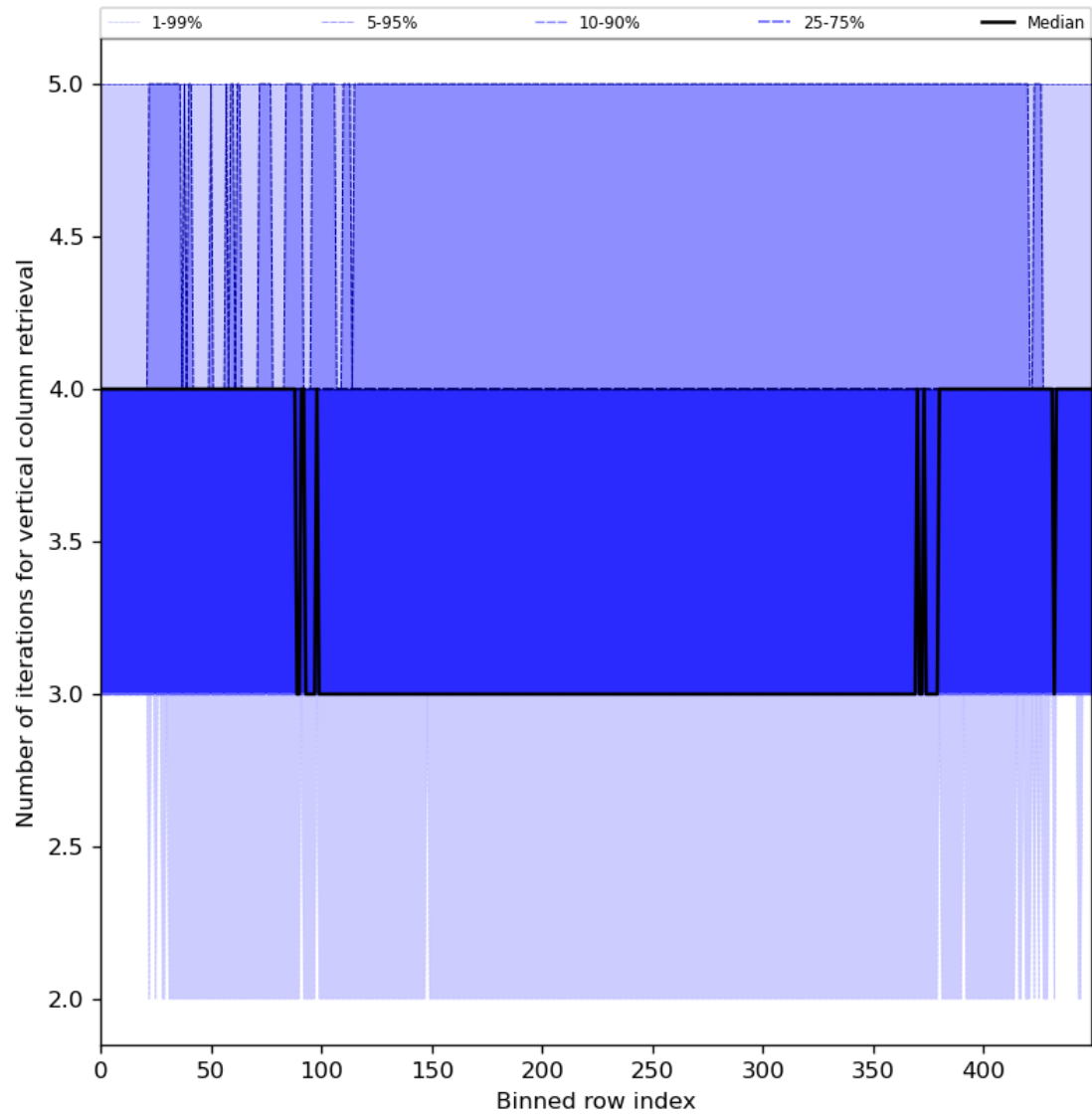
Figure 33: Along track statistics of “Number of iterations for vertical column retrieval” for 2024-08-13 to 2024-08-15
