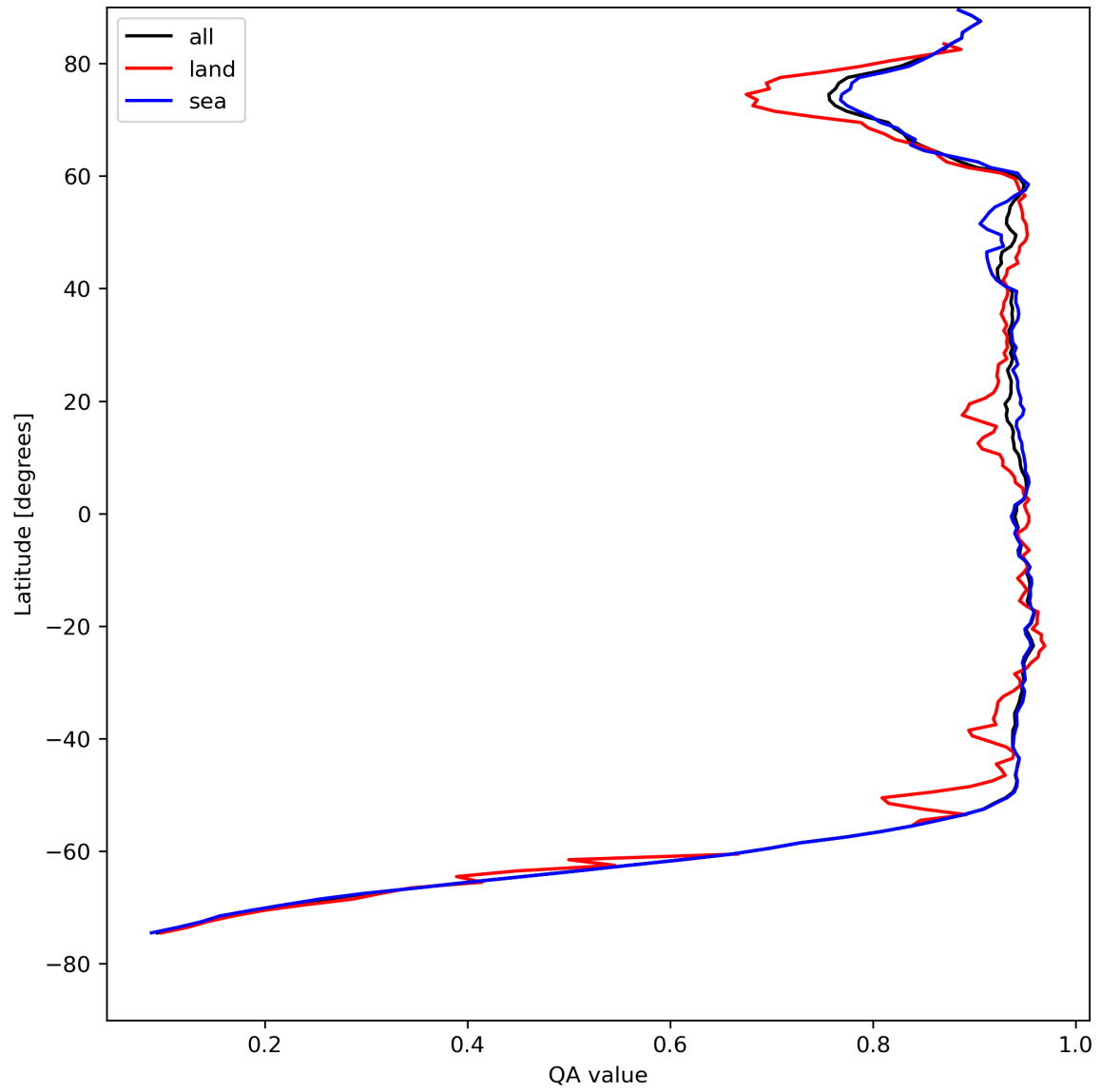
Figure 13: Zonal average of “QA value” for 2024-08-13 to 2024-08-15.
