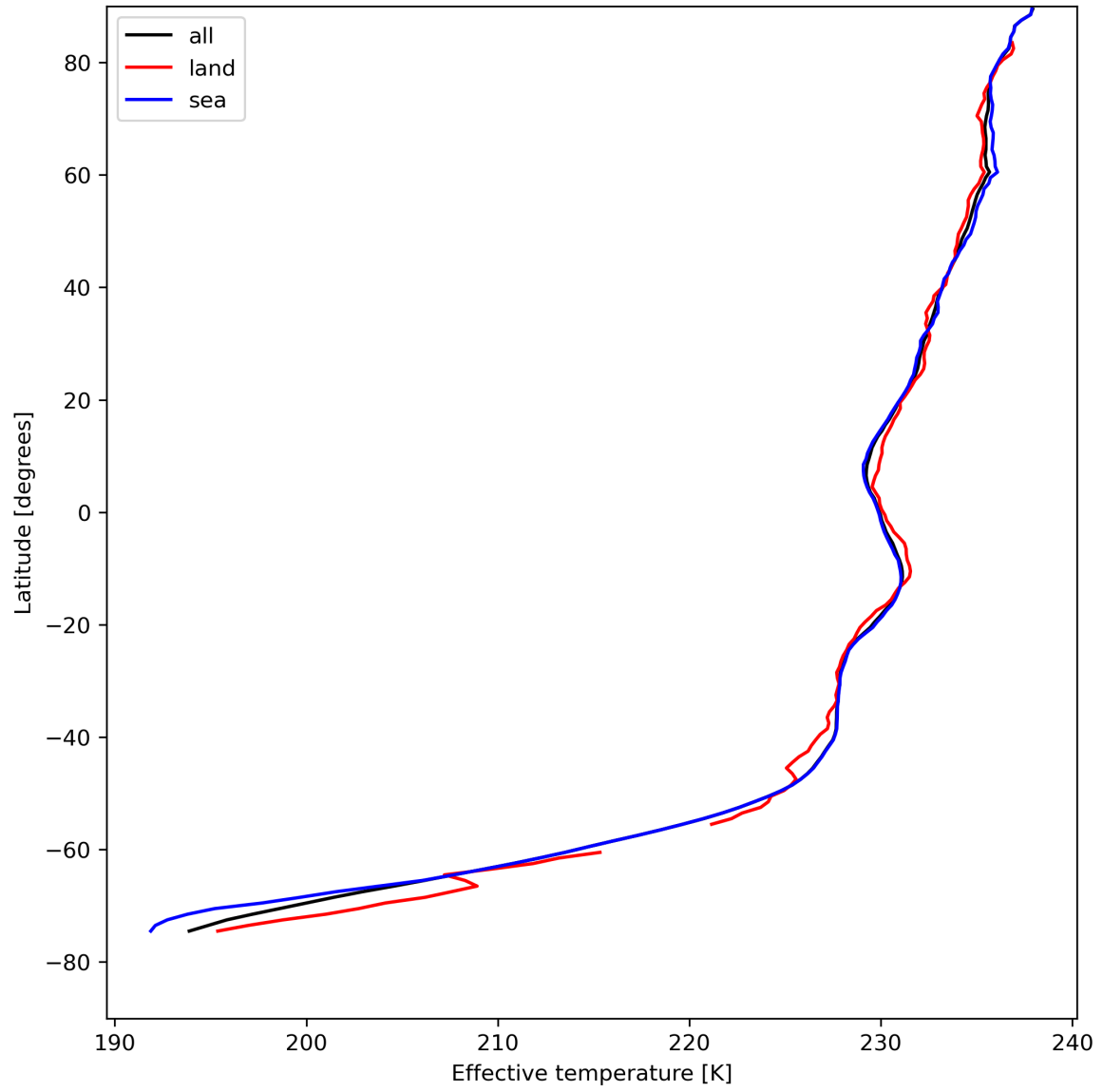
Figure 17: Zonal average of “Effective temperature” for 2024-08-13 to 2024-08-15.
