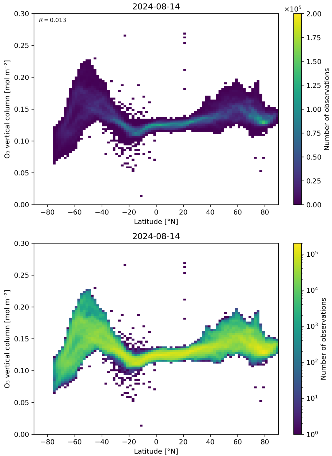
Figure 36: Scatter density plot of “Latitude” against “O 3 vertical column” for 2024-08-13 to 2024-08-15.
