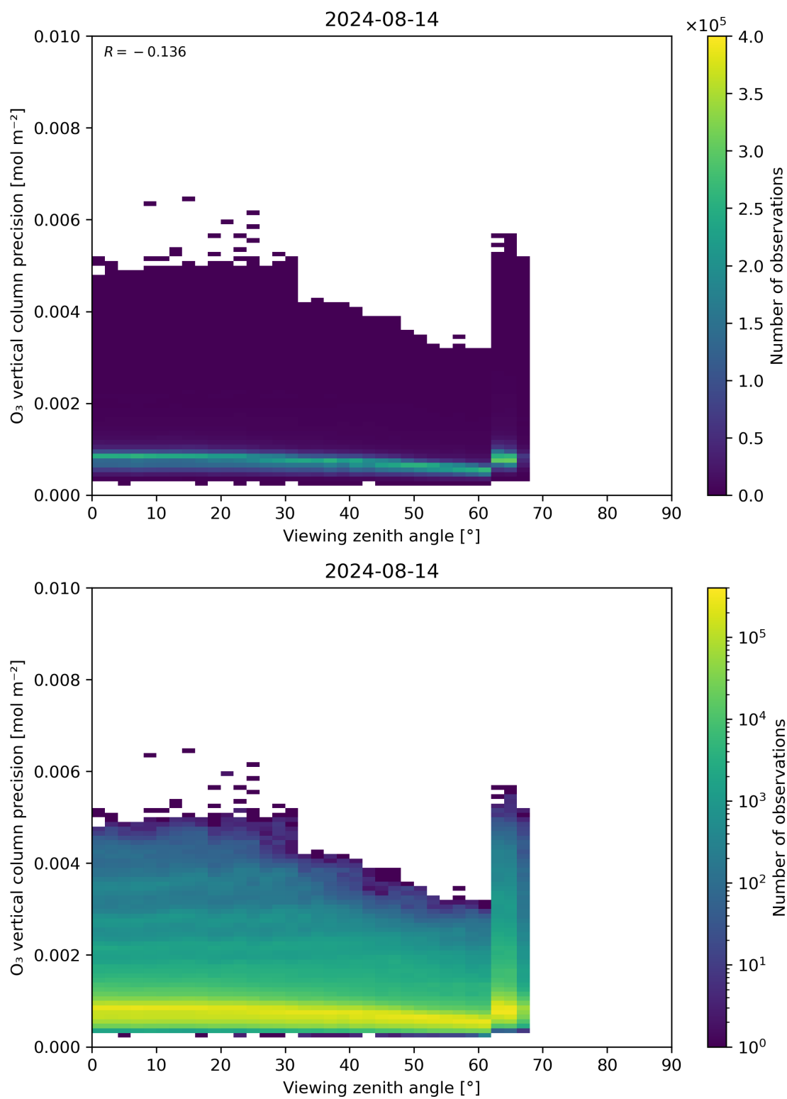
Figure 53: Scatter density plot of “Viewing zenith angle” against “O 3 vertical column precision” for 2024-08-13 to 2024-08-15.
