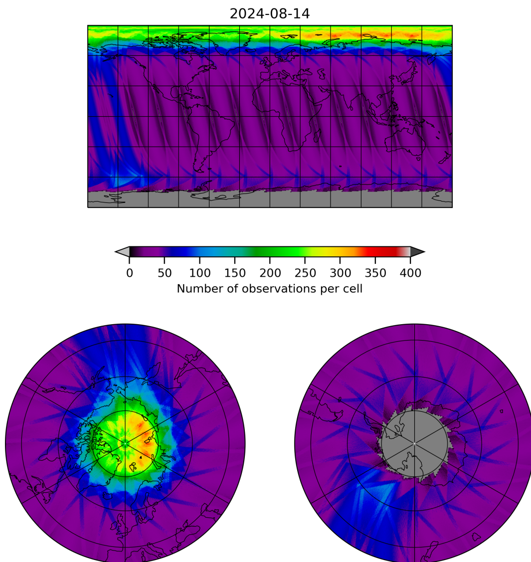
Figure 12: Map of the number of observations for 2024-08-13 to 2024-08-15
