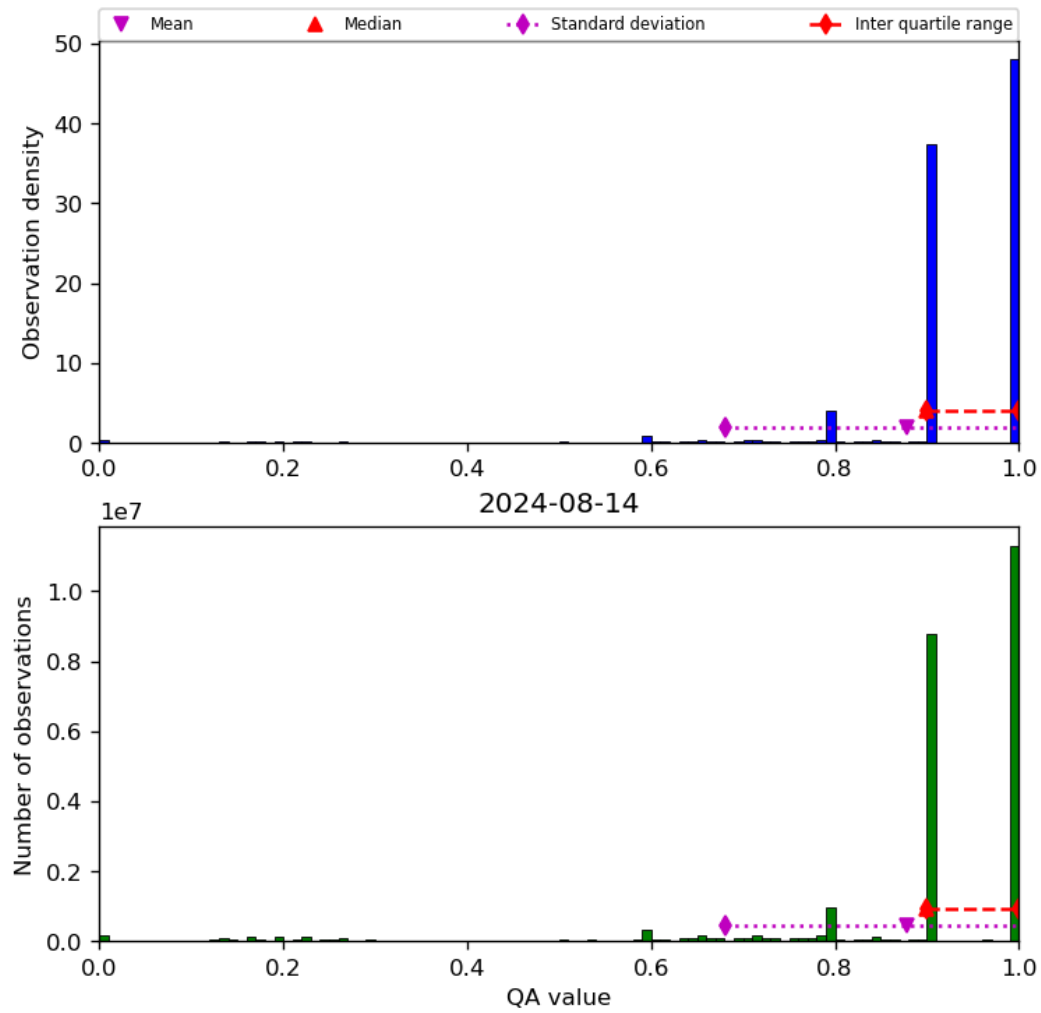
Figure 20: Histogram of “QA value” for 2024-08-13 to 2024-08-15
