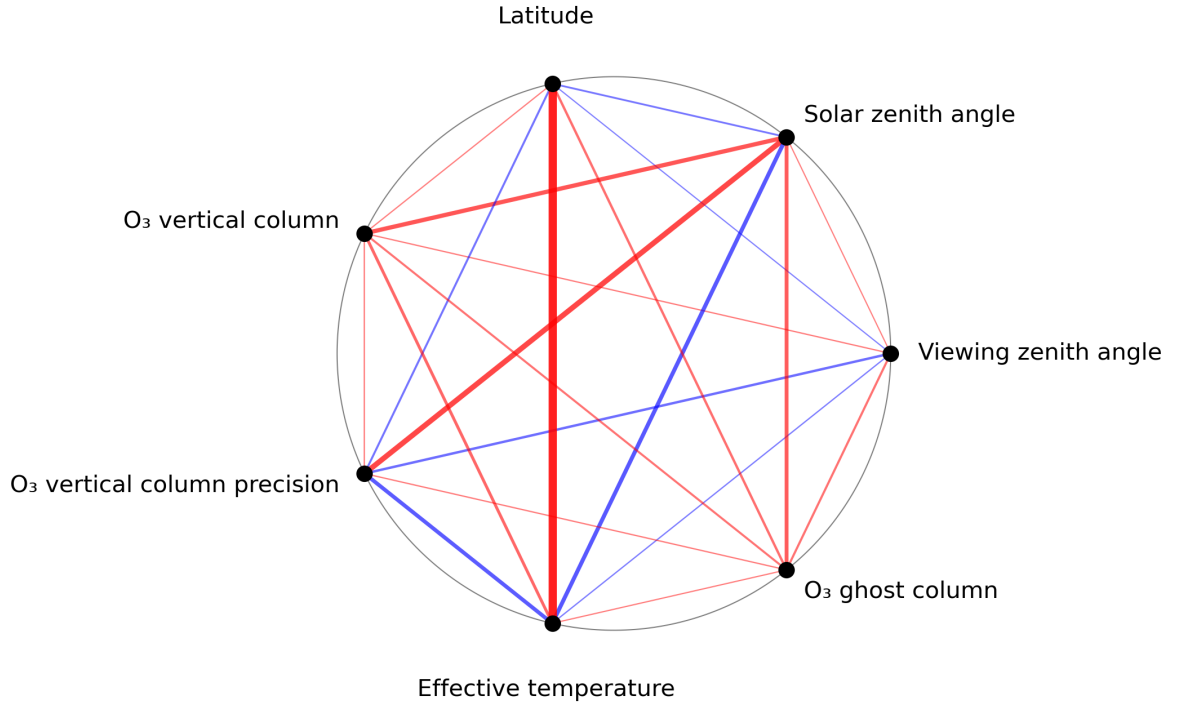
Figure 1: Map of correlation graph for 2024-08-13 to 2024-08-15.
