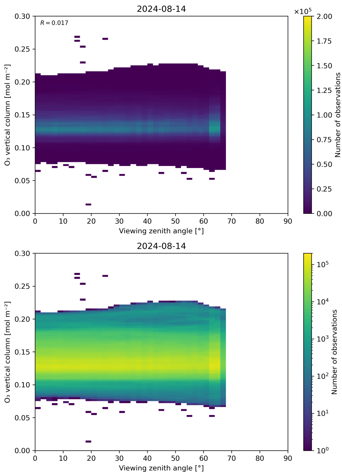
Figure 52: Scatter density plot of “Viewing zenith angle” against “O 3 vertical column” for 2024-08-13 to 2024-08-15.
