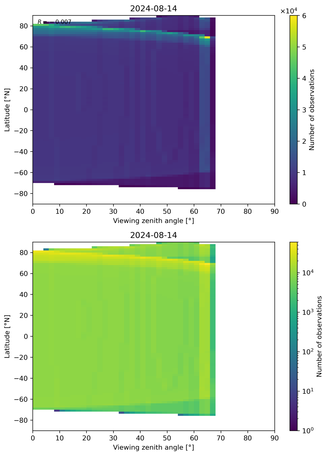
Figure 49: Scatter density plot of “Viewing zenith angle” against “Latitude” for 2024-08-13 to 2024-08-15.
