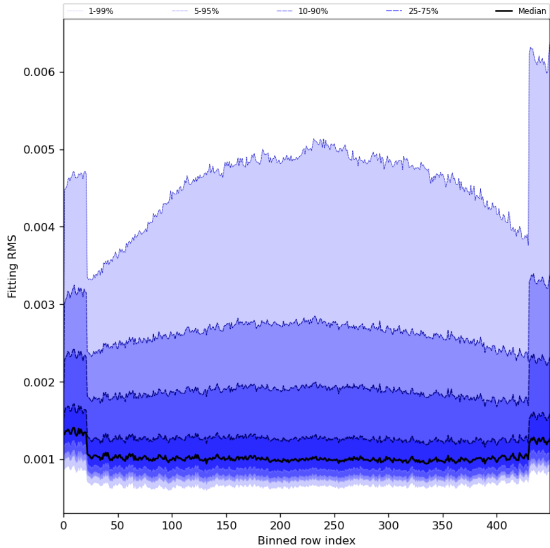
Figure 30: Along track statistics of “Fitting RMS” for 2024-08-13 to 2024-08-15
