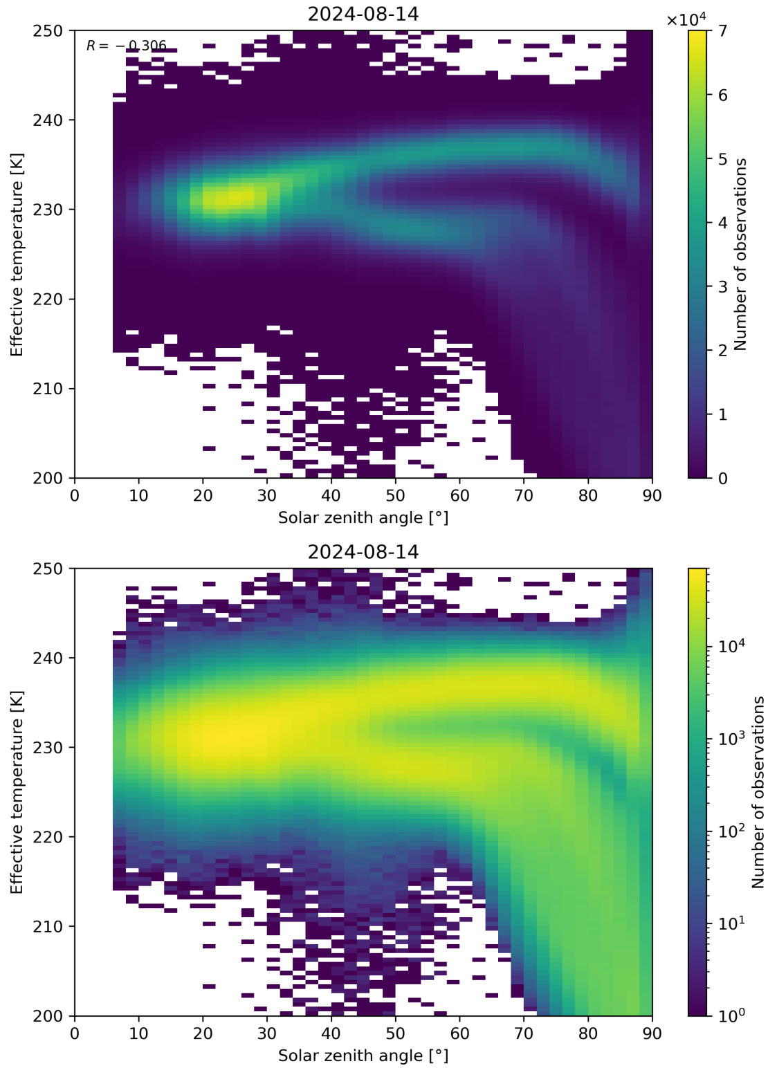
Figure 45: Scatter density plot of “Solar zenith angle” against “Effective temperature” for 2024-08-13 to 2024-08-15.
