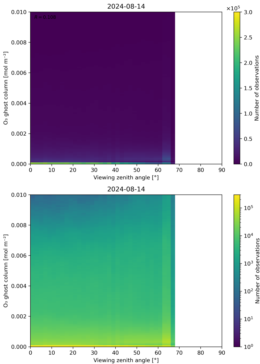
Figure 51: Scatter density plot of “Viewing zenith angle” against “O 3 ghost column” for 2024-08-13 to 2024-08-15.
