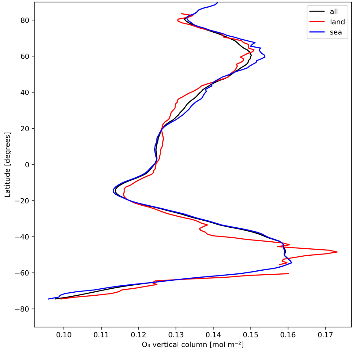
Figure 14: Zonal average of “O 3 vertical column” for 2024-08-13 to 2024-08-15.
