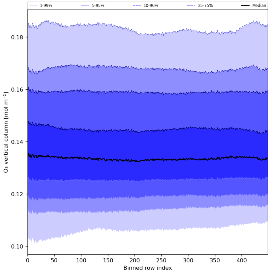
Figure 28: Along track statistics of “O 3 vertical column” for 2024-08-13 to 2024-08-15
