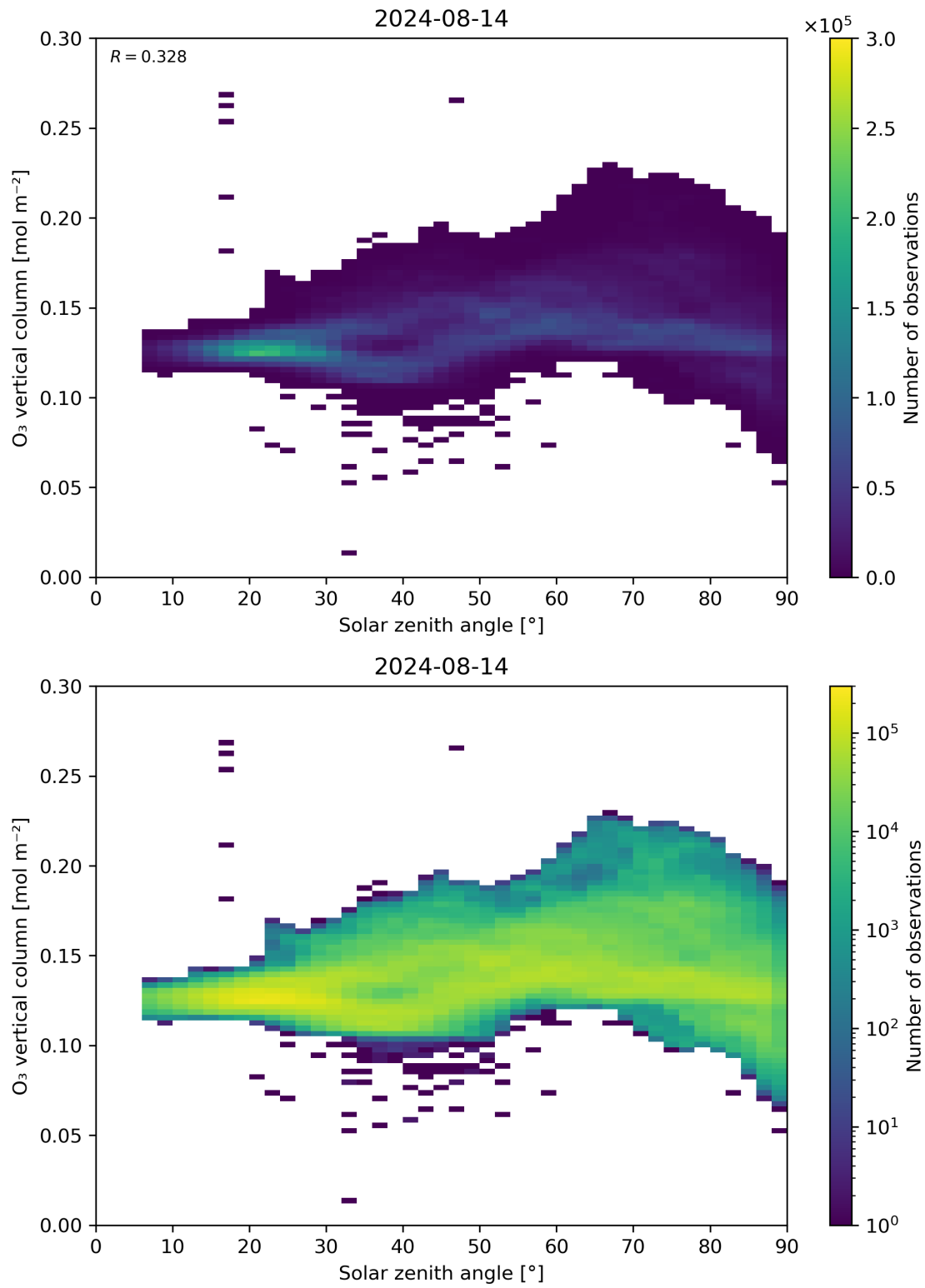
Figure 47: Scatter density plot of “Solar zenith angle” against “O 3 vertical column” for 2024-08-13 to 2024-08-15.
