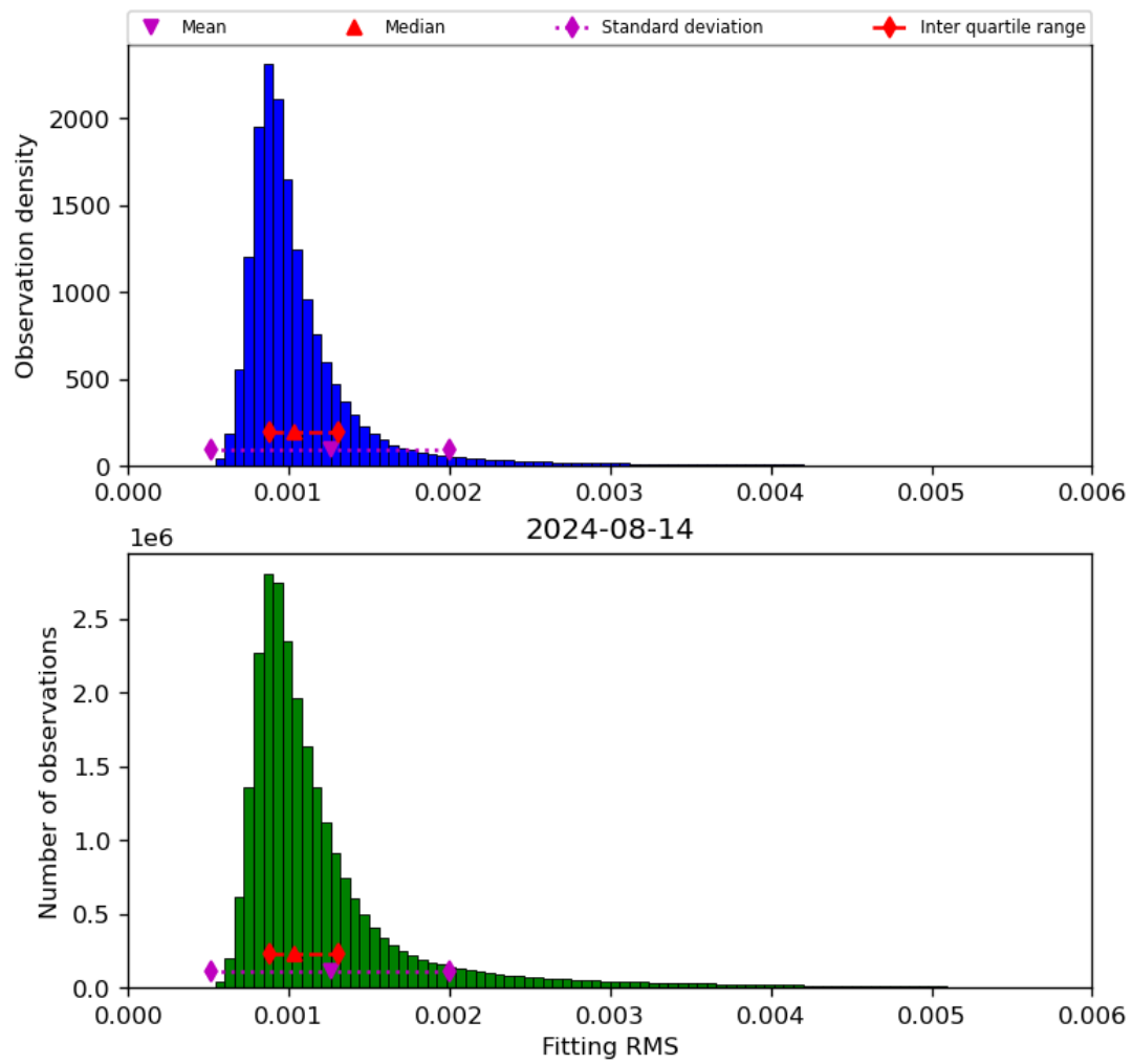
Figure 23: Histogram of “Fitting RMS” for 2024-08-13 to 2024-08-15
