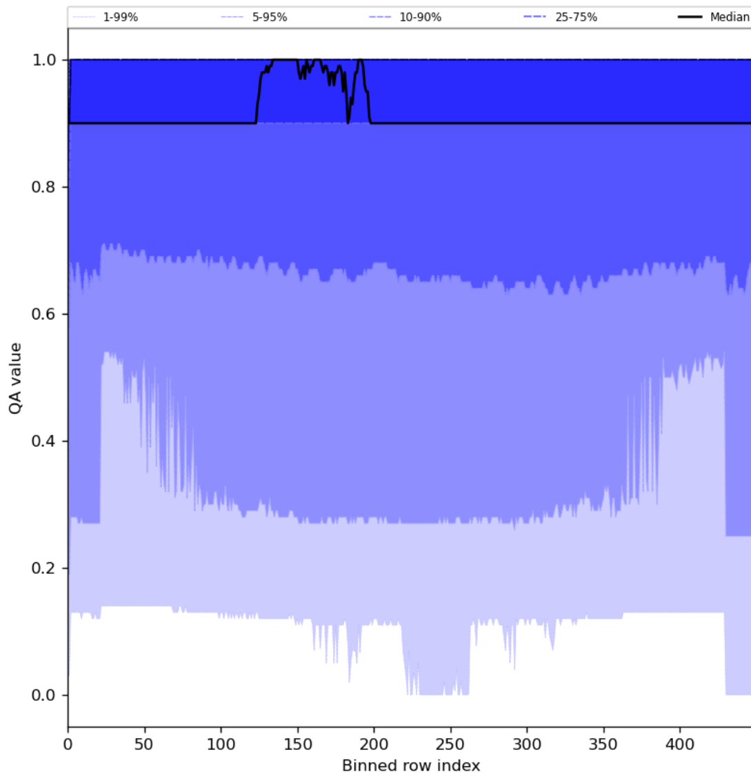
Figure 27: Along track statistics of “QA value” for 2024-08-13 to 2024-08-15
