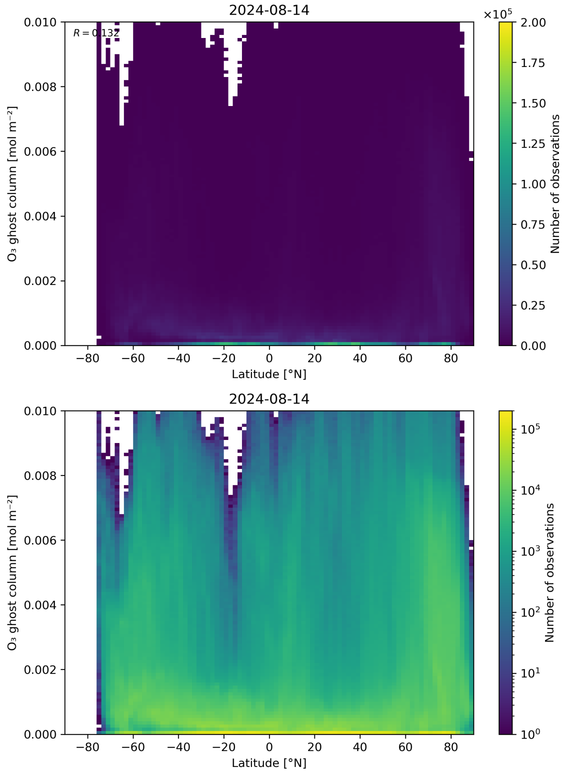
Figure 35: Scatter density plot of “Latitude” against “O 3 ghost column” for 2024-08-13 to 2024-08-15.
