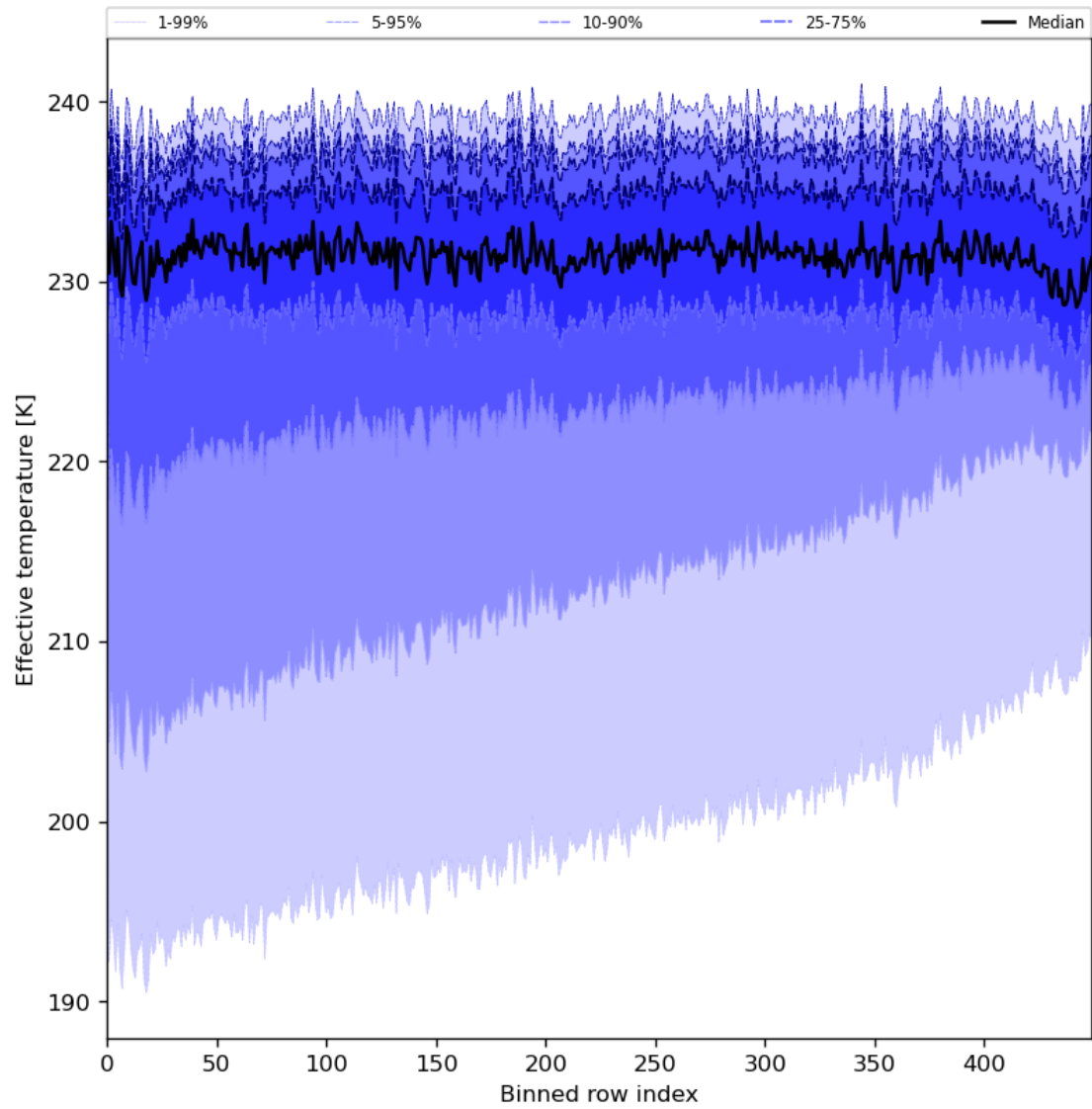
Figure 31: Along track statistics of “Effective temperature” for 2024-08-13 to 2024-08-15
