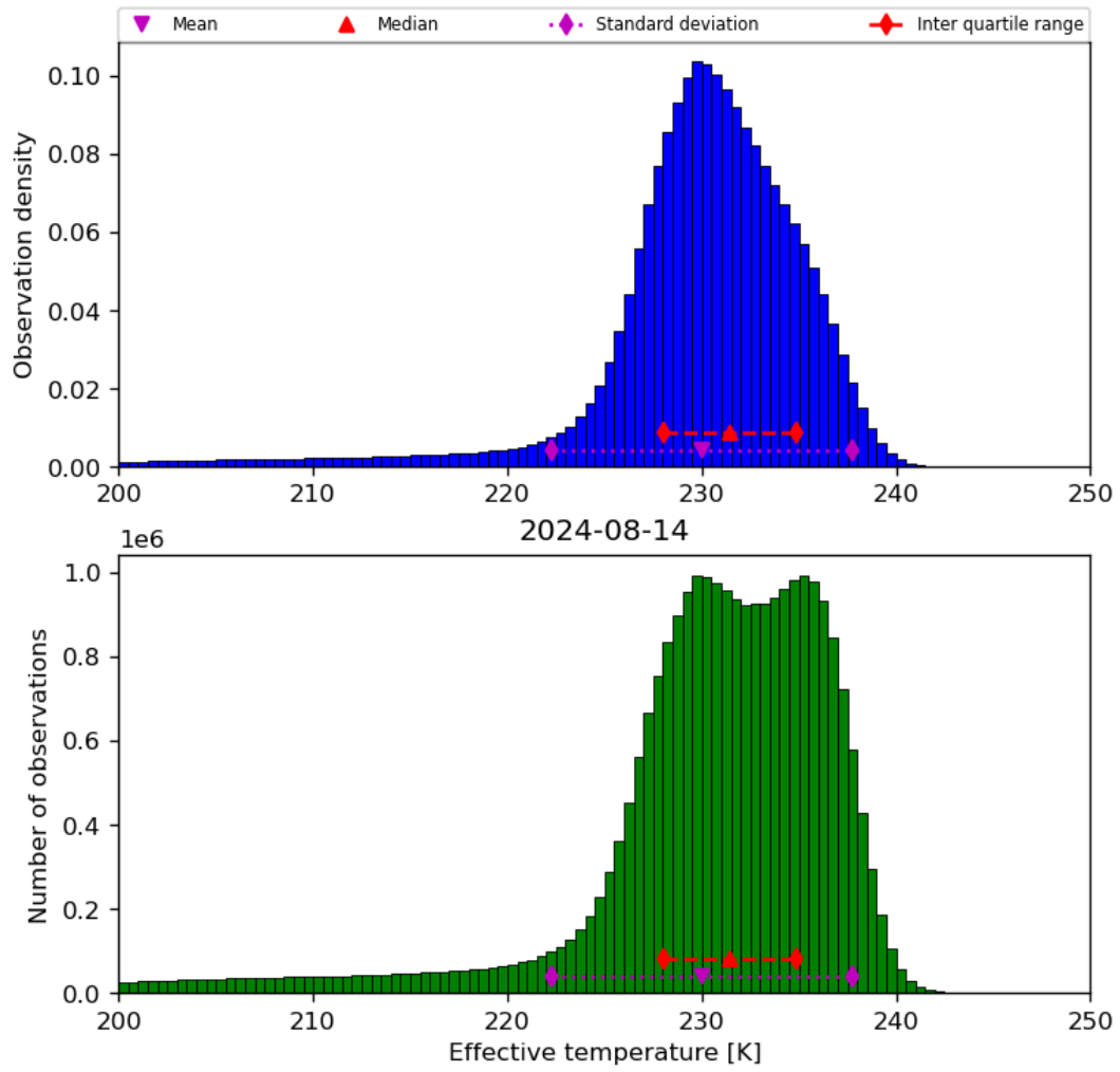
Figure 24: Histogram of “Effective temperature” for 2024-08-13 to 2024-08-15
