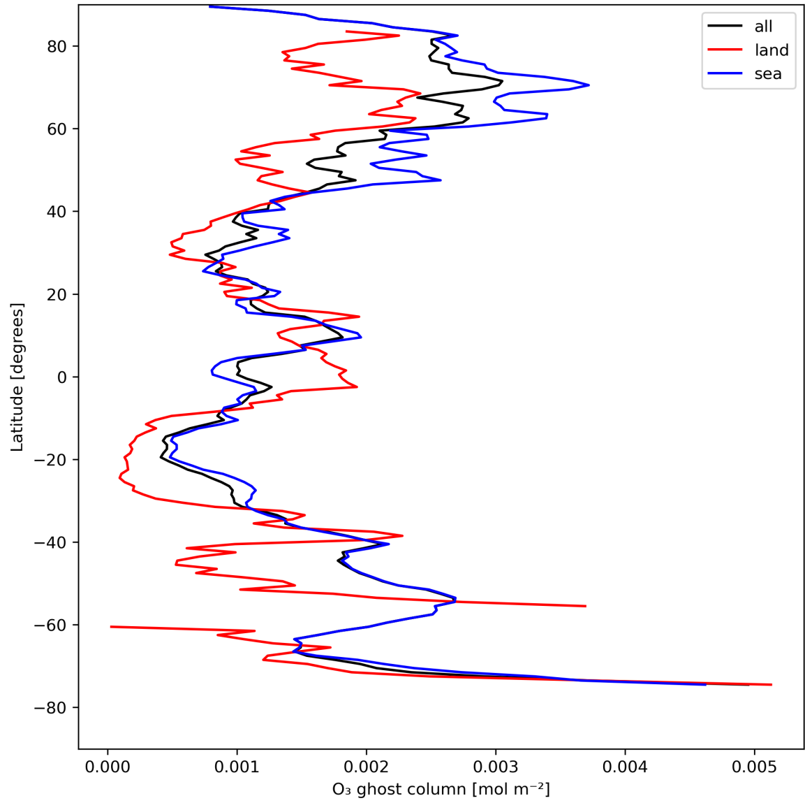
Figure 18: Zonal average of "O 3 ghost column" for 2024-08-13 to 2024-08-15.
