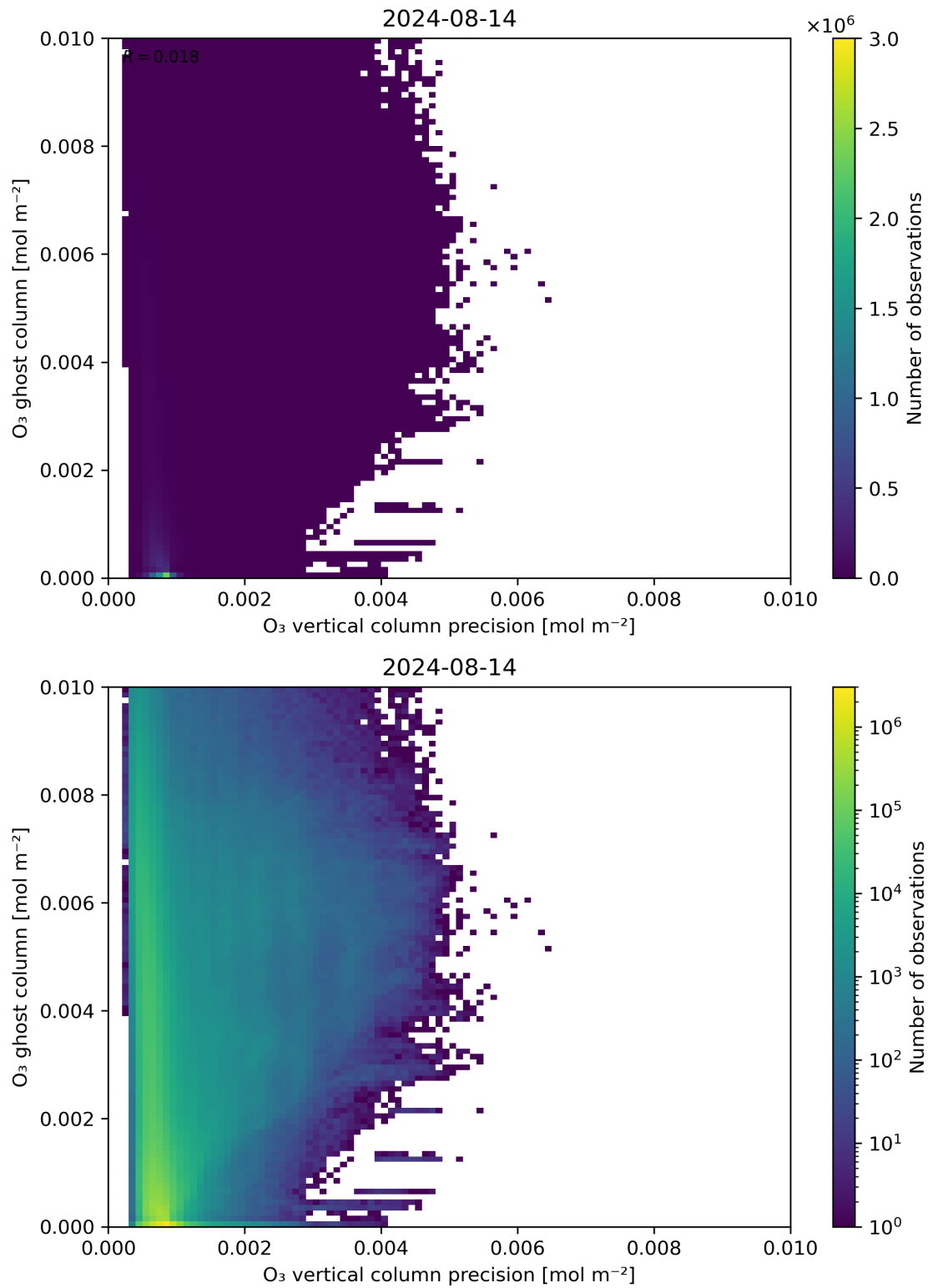
Figure 43: Scatter density plot of “O 3 vertical column precision” against “O 3 ghost column” for 2024-08-13 to 2024-08-15.
