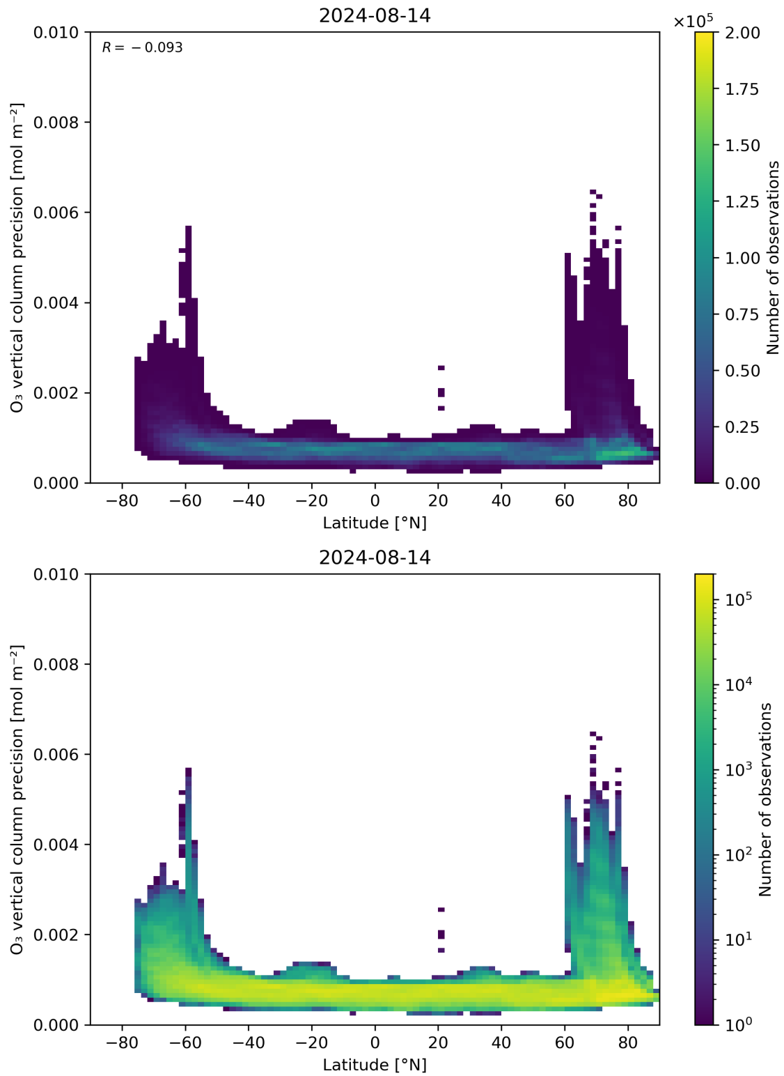
Figure 37: Scatter density plot of “Latitude” against “O 3 vertical column precision” for 2024-08-13 to 2024-08-15.
