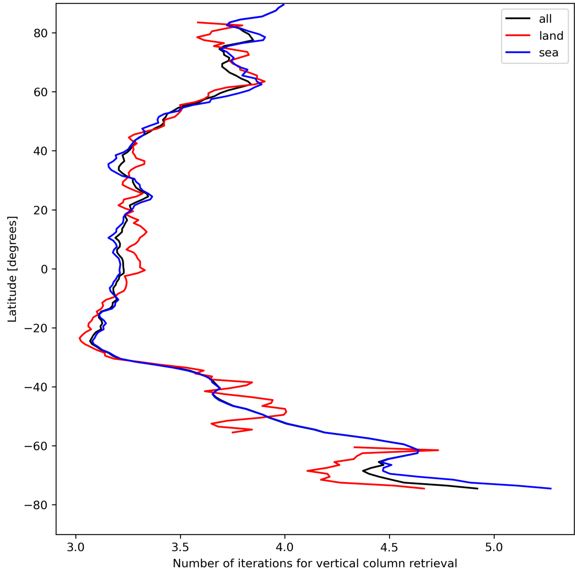
Figure 19: Zonal average of “Number of iterations for vertical column retrieval” for 2024-08-13 to 2024-08-15.
