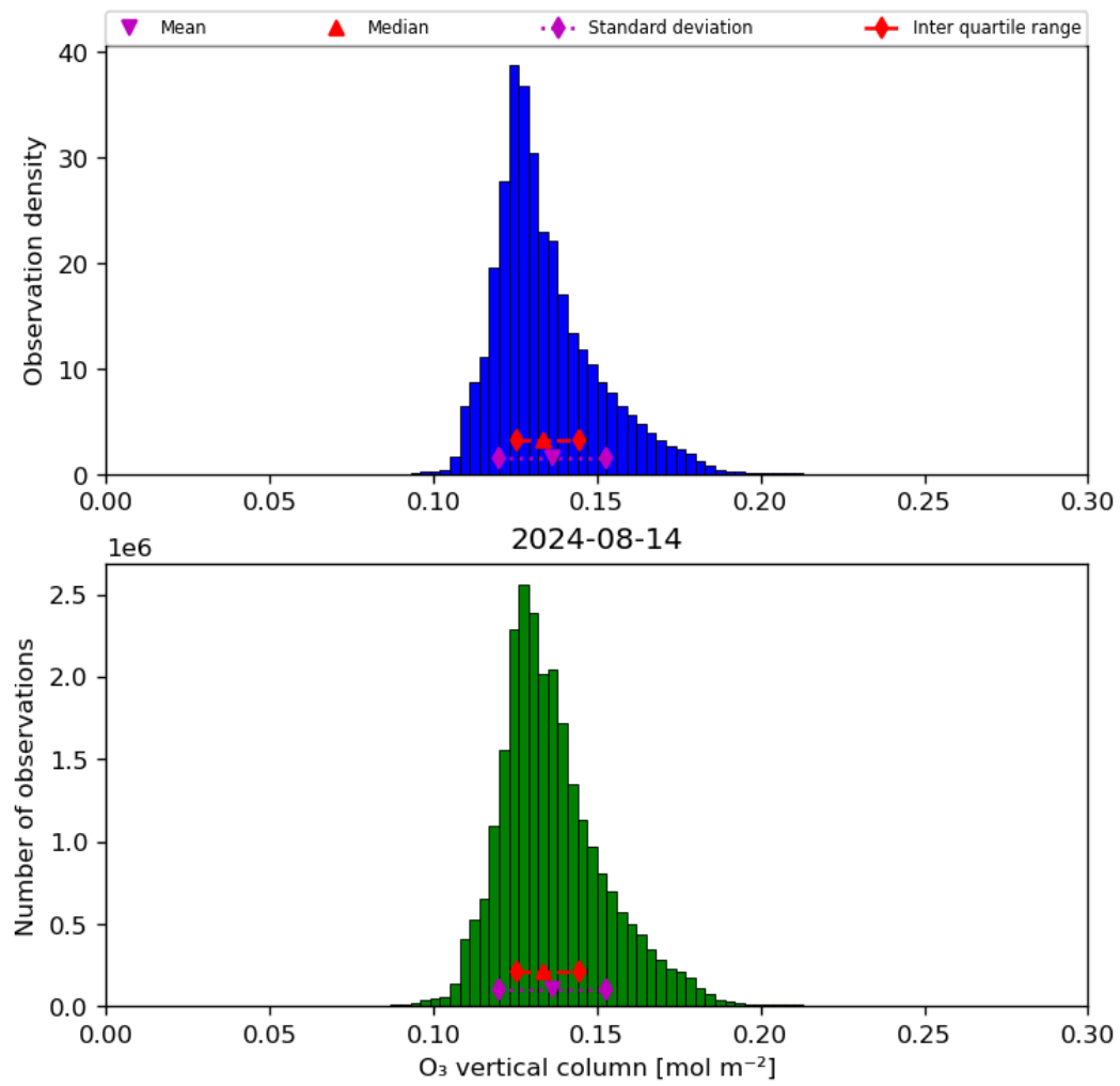
Figure 21: Histogram of “O 3 vertical column” for 2024-08-13 to 2024-08-15
