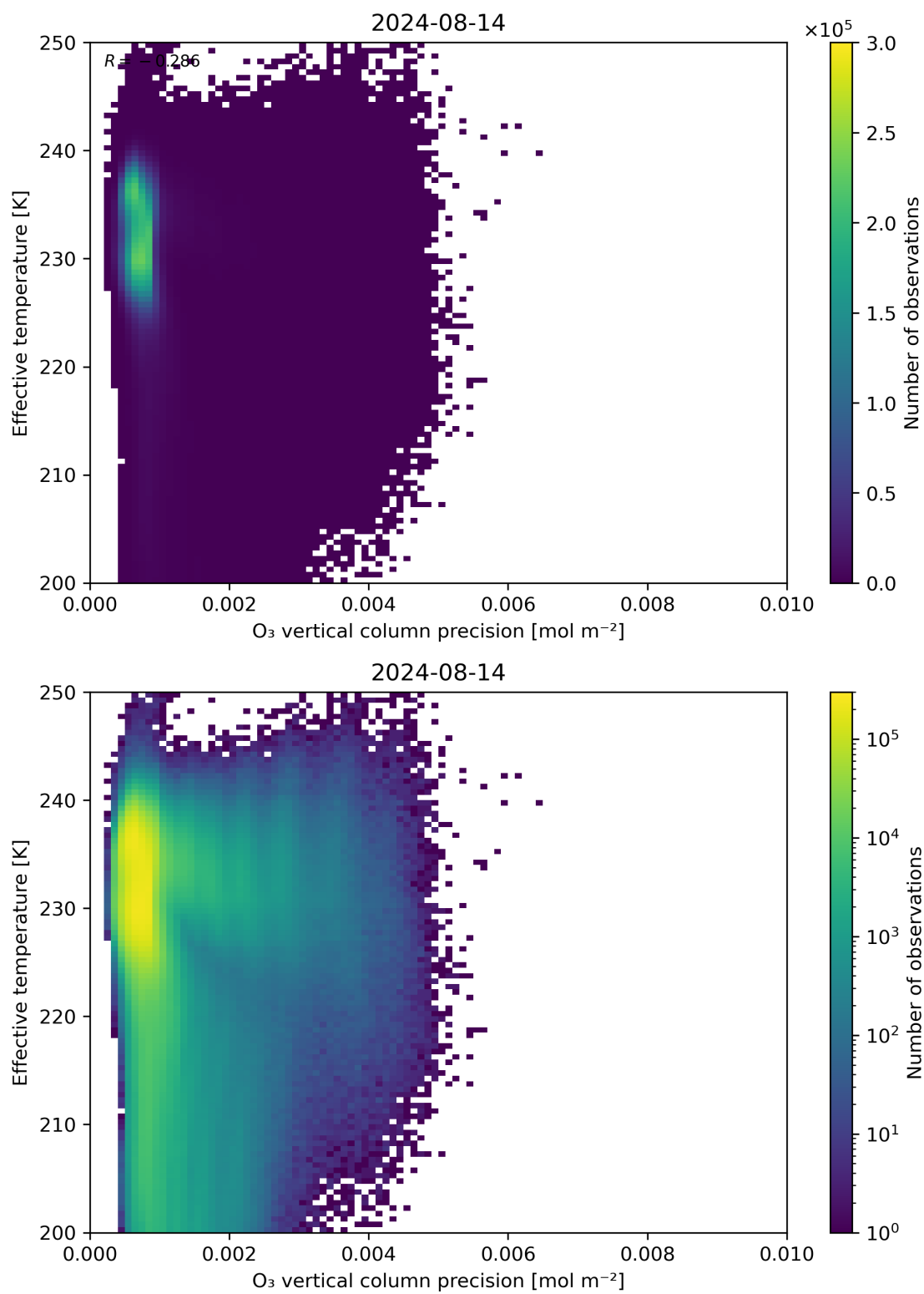
Figure 42: Scatter density plot of “O 3 vertical column precision” against “Effective temperature” for 2024-08-13 to 2024-08-15.
