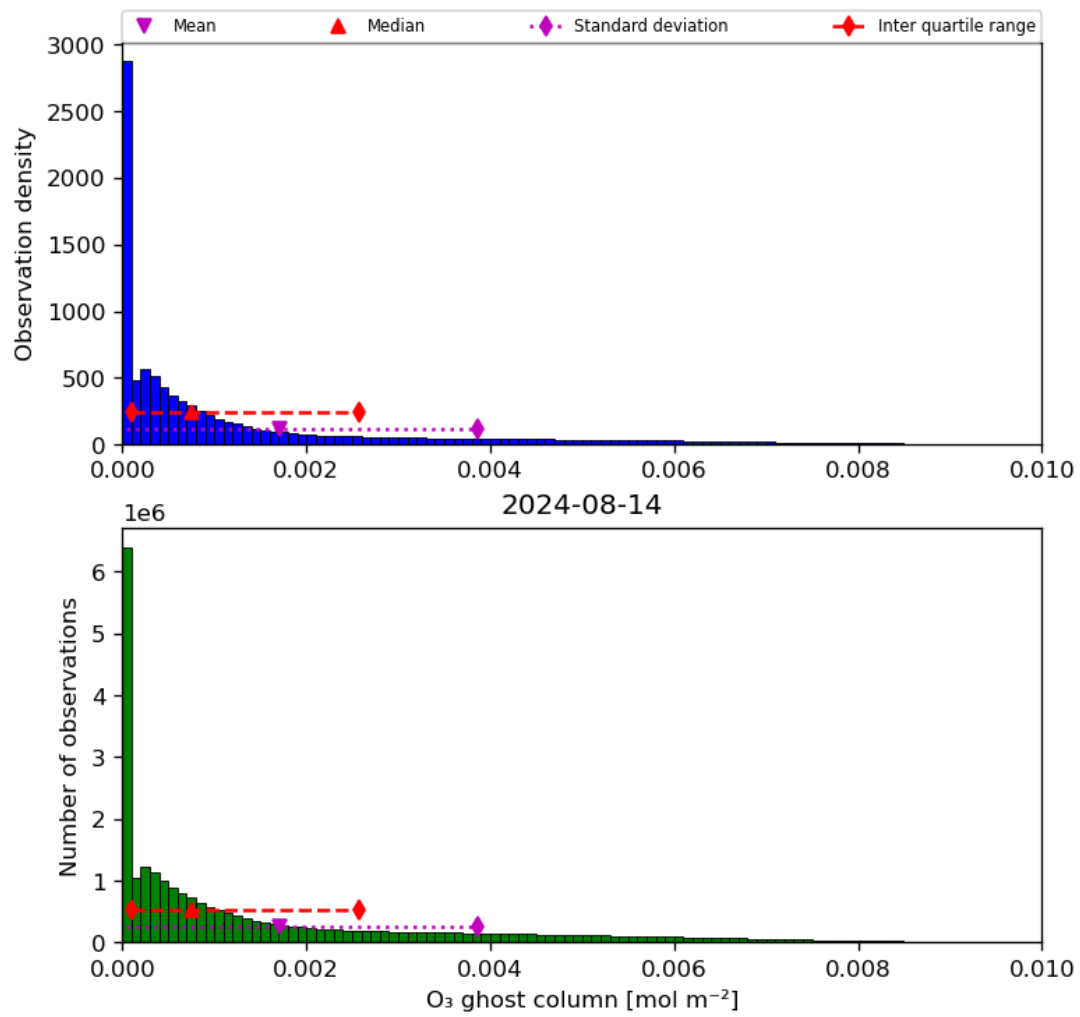
Figure 25: Histogram of "O 3 ghost column" for 2024-08-13 to 2024-08-15
