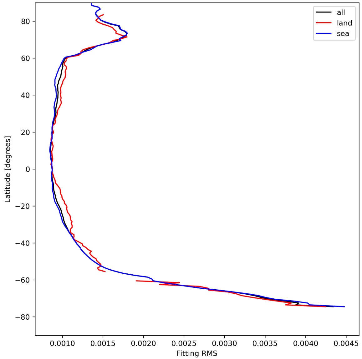
Figure 16: Zonal average of “Fitting RMS” for 2024-08-13 to 2024-08-15.
