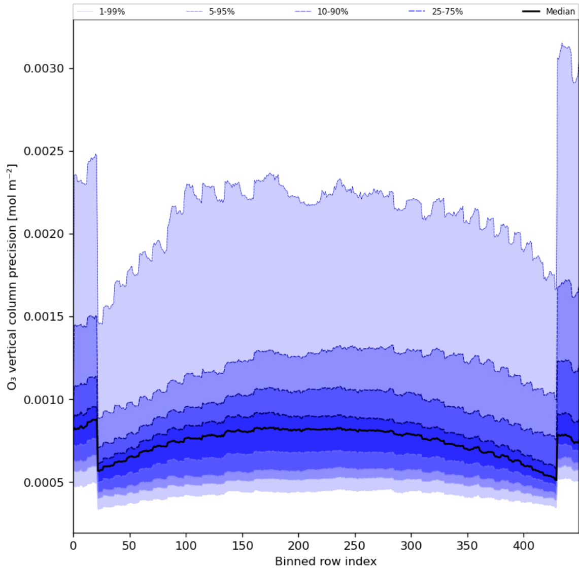
Figure 29: Along track statistics of “O 3 vertical column precision” for 2024-08-13 to 2024-08-15
