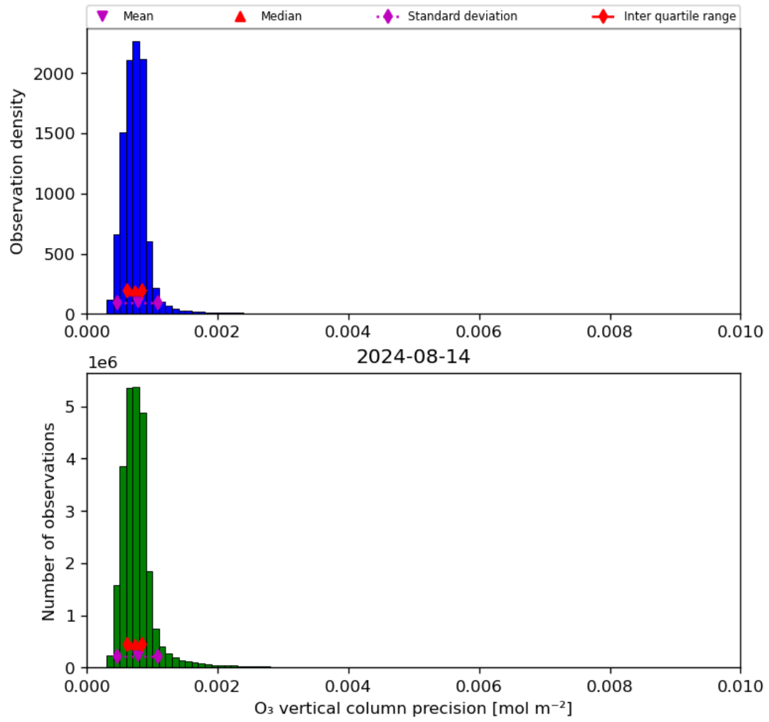
Figure 22: Histogram of “O 3 vertical column precision” for 2024-08-13 to 2024-08-15
