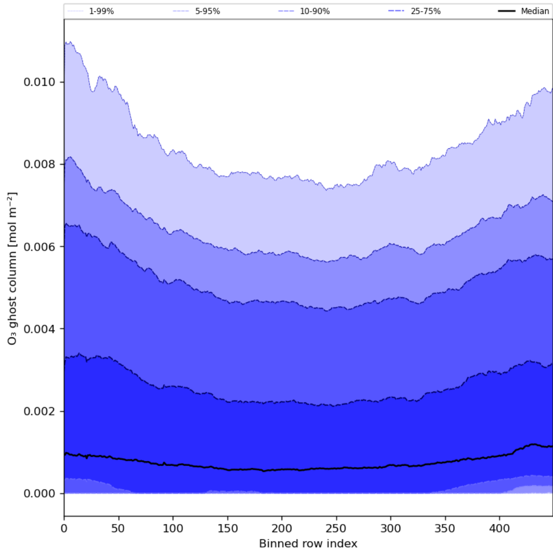
Figure 32: Along track statistics of “O 3 ghost column” for 2024-08-13 to 2024-08-15
