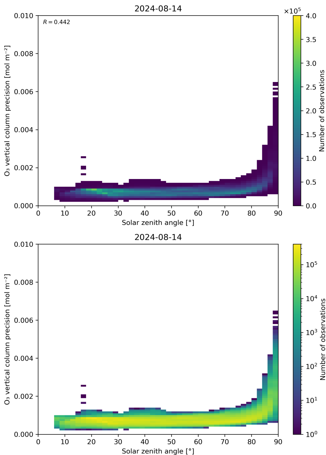
Figure 48: Scatter density plot of “Solar zenith angle” against “O 3 vertical column precision” for 2024-08-13 to 2024-08-15.
