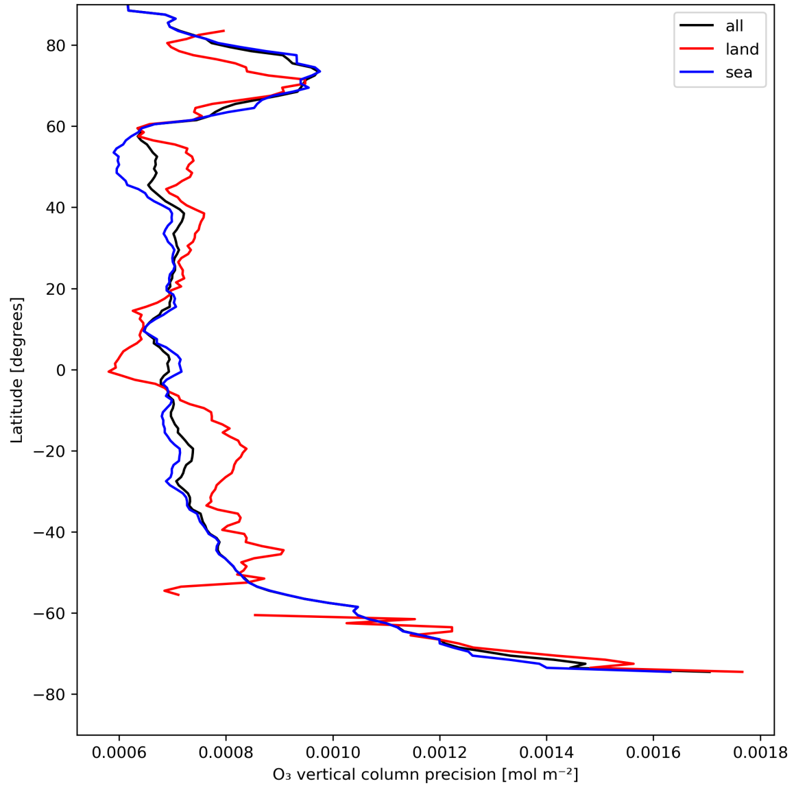
Figure 15: Zonal average of "O 3 vertical column precision" for 2024-08-13 to 2024-08-15.
