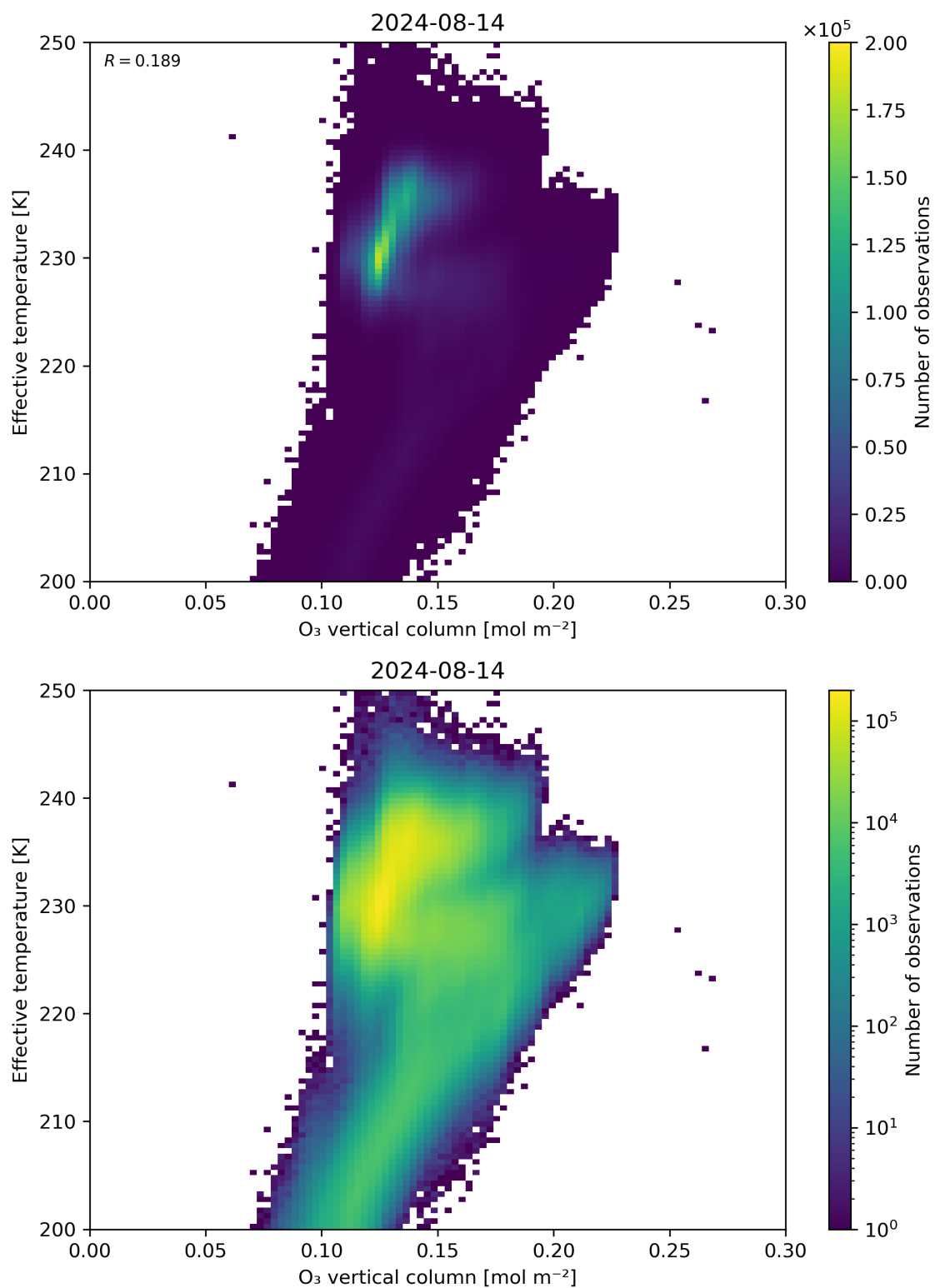
Figure 39: Scatter density plot of “O 3 vertical column” against “Effective temperature” for 2024-08-13 to 2024-08-15.
