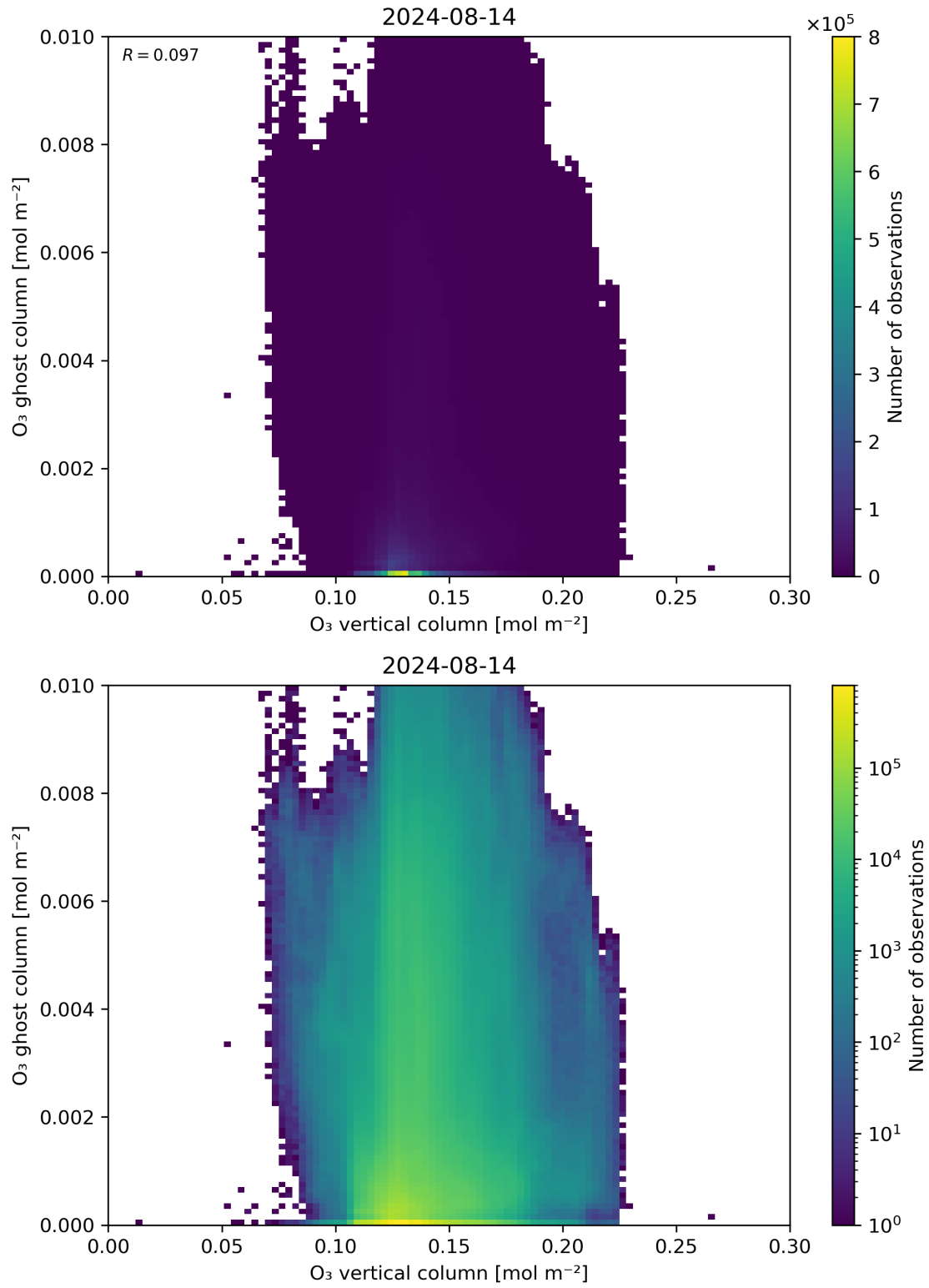
Figure 40: Scatter density plot of “O 3 vertical column” against “O 3 ghost column” for 2024-08-13 to 2024-08-15.
