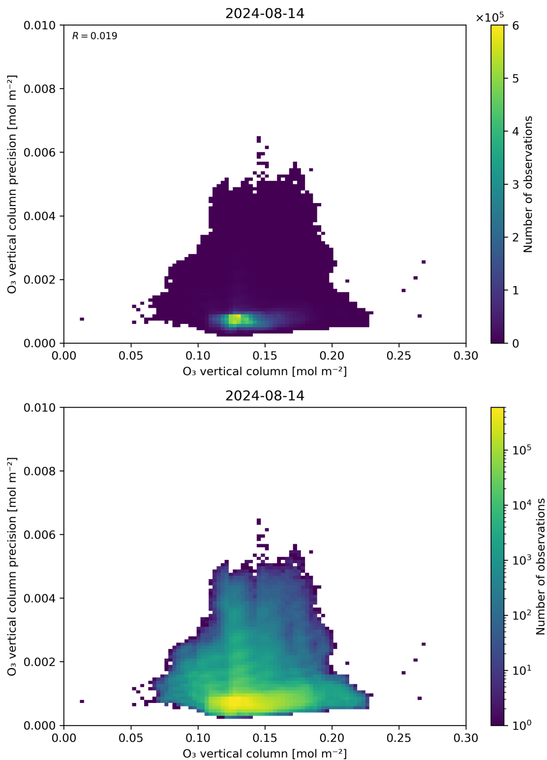
Figure 41: Scatter density plot of “O 3 vertical column” against “O 3 vertical column precision” for 2024-08-13 to 2024-08-15.
