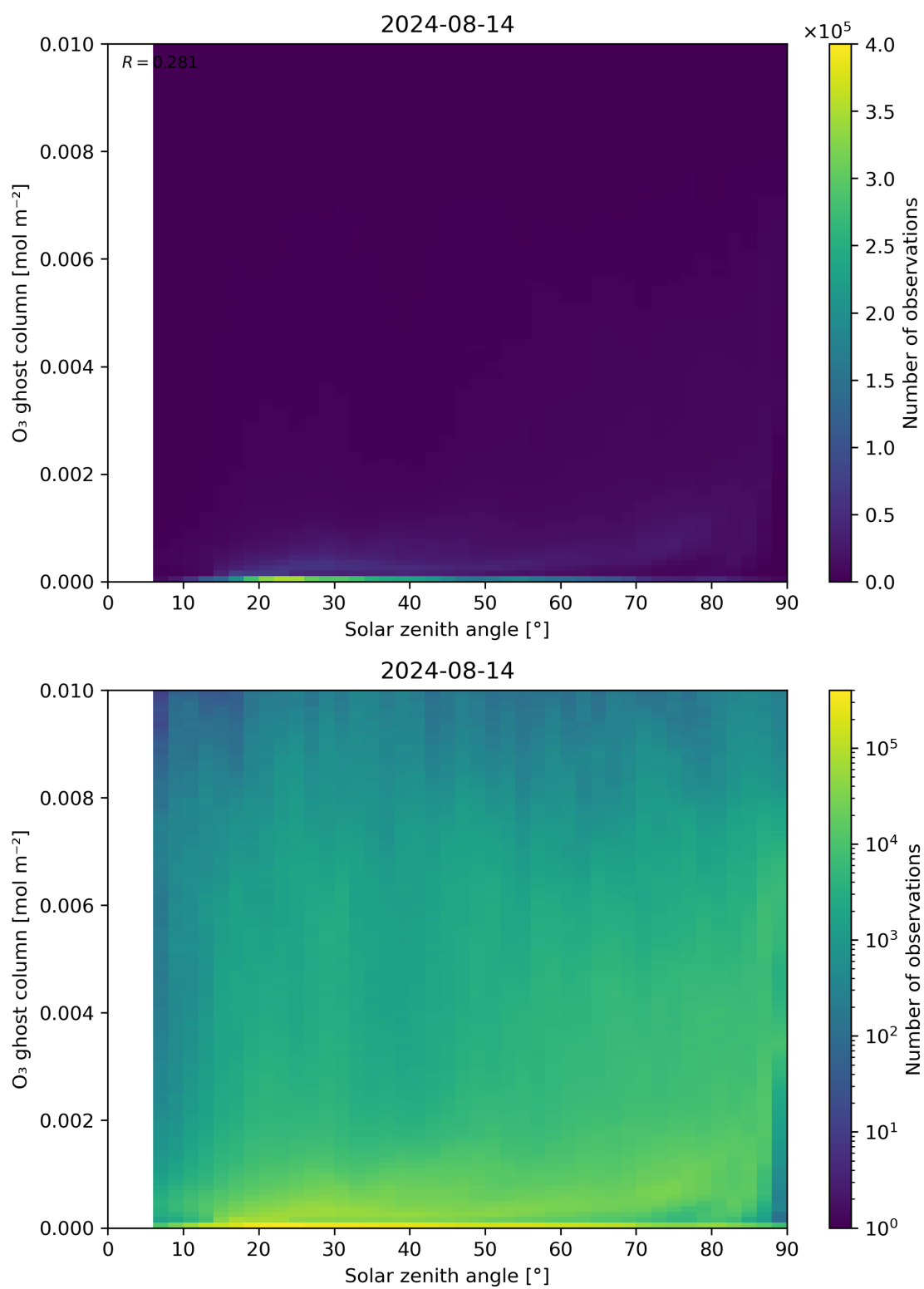
Figure 46: Scatter density plot of “Solar zenith angle” against “O 3 ghost column” for 2024-08-13 to 2024-08-15.
