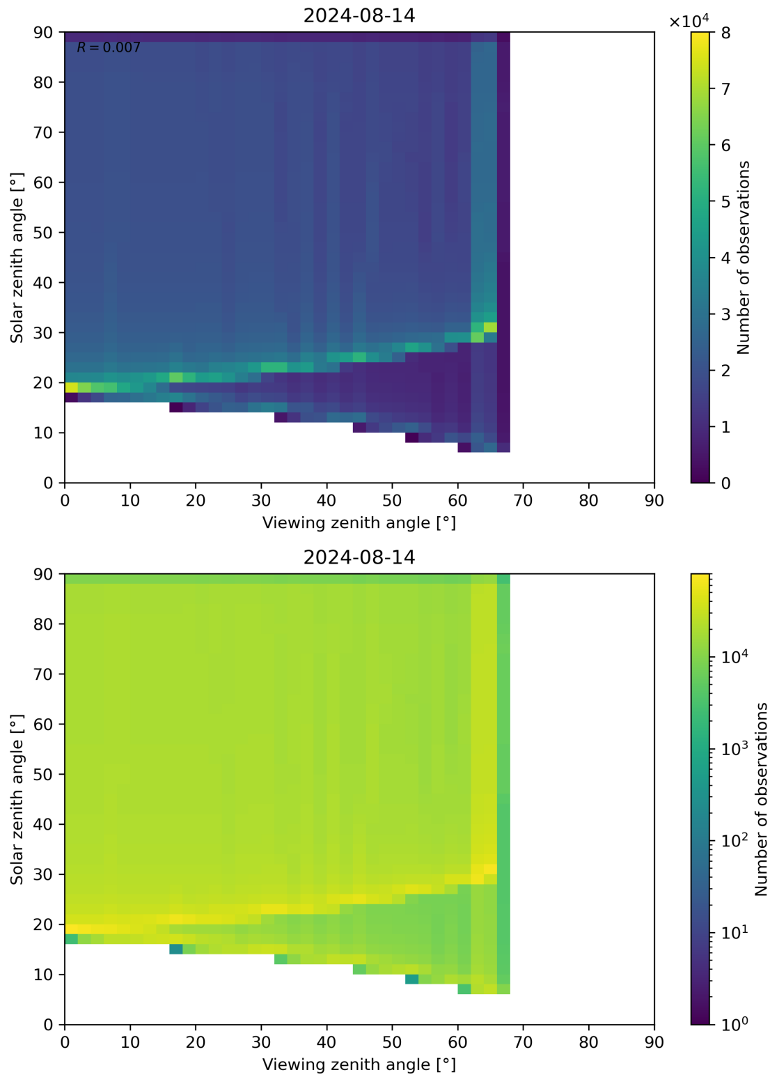
Figure 54: Scatter density plot of “Viewing zenith angle” against “Solar zenith angle” for 2024-08-13 to 2024-08-15.
