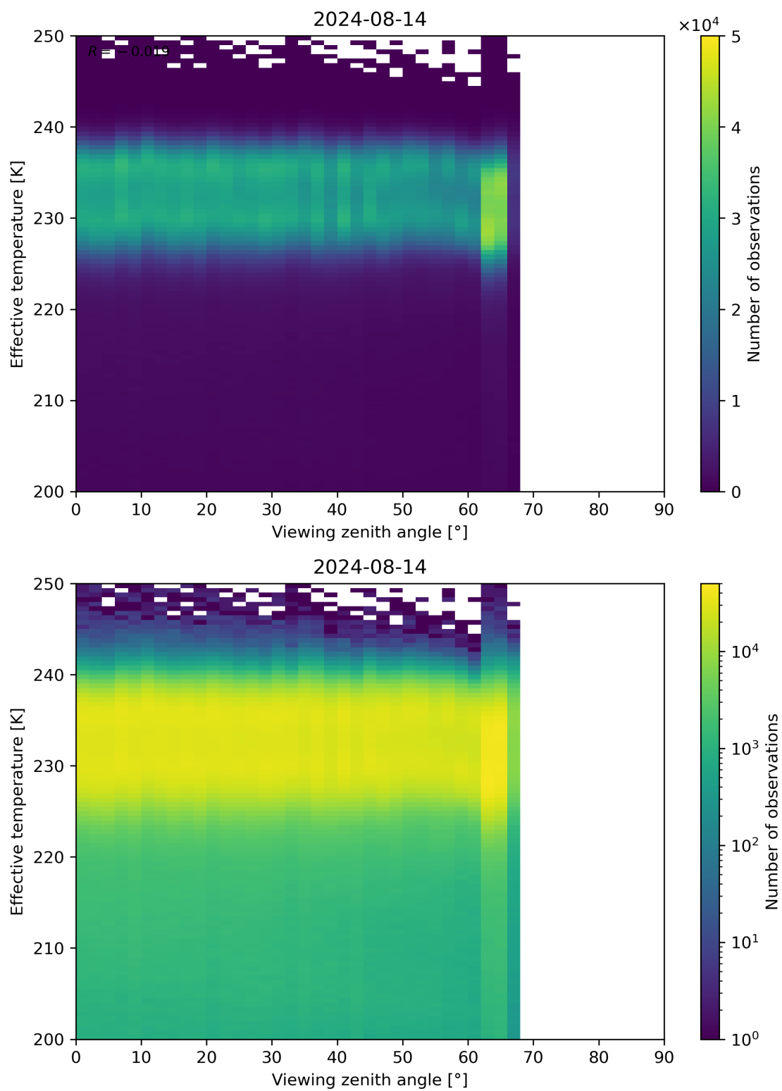
Figure 50: Scatter density plot of “Viewing zenith angle” against “Effective temperature” for 2024-08-13 to 2024-08-15.
