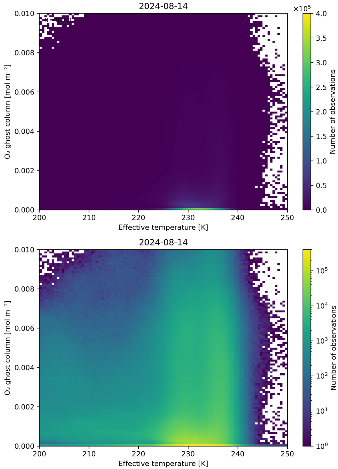
Figure 38: Scatter density plot of “Effective temperature” against “O 3 ghost column” for 2024-08-13 to 2024-08-15.
