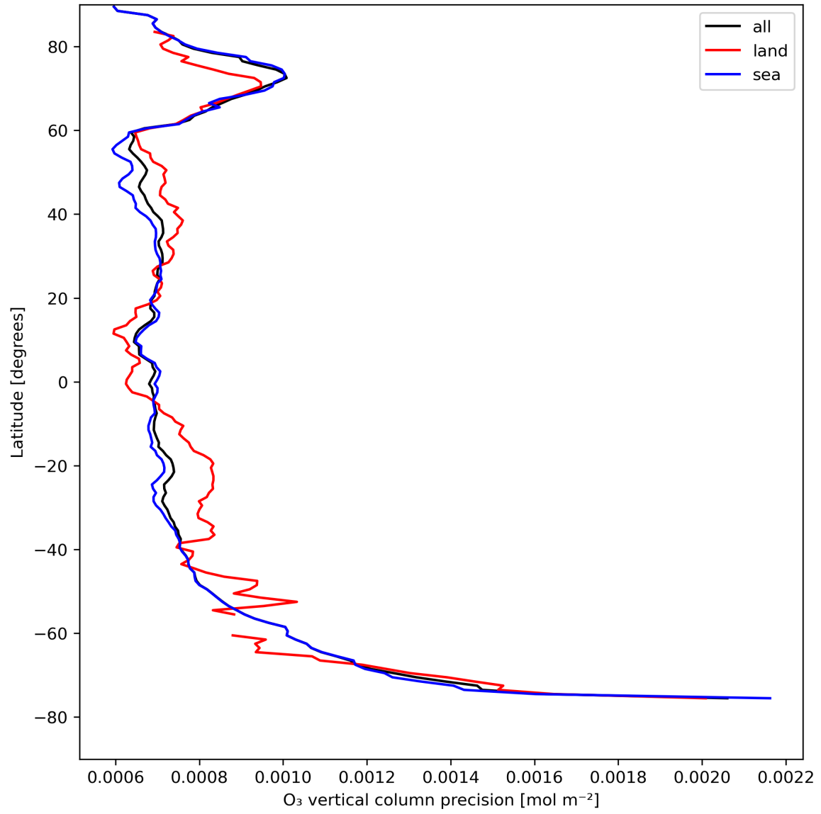
Figure 15: Zonal average of “O 3 vertical column precision” for 2024-08-14 to 2024-08-16.
