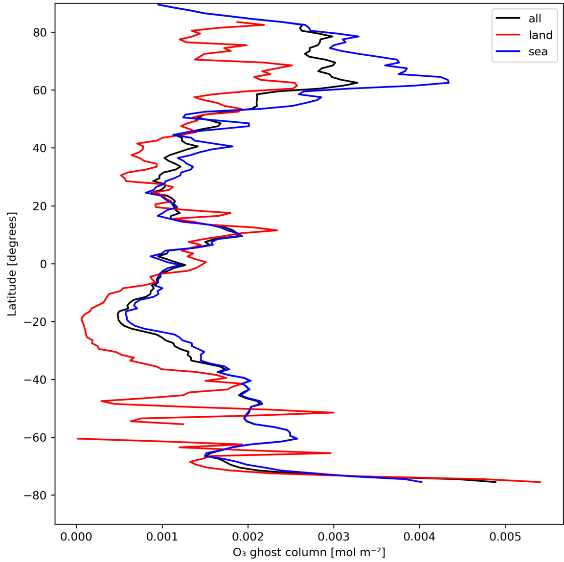
Figure 18: Zonal average of "O 3 ghost column" for 2024-08-14 to 2024-08-16.
