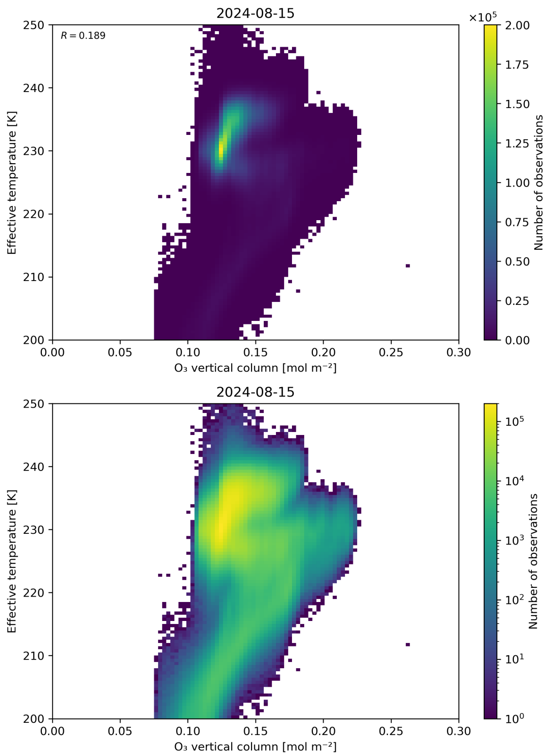
Figure 39: Scatter density plot of “O 3 vertical column” against “Effective temperature” for 2024-08-14 to 2024-08-16.
