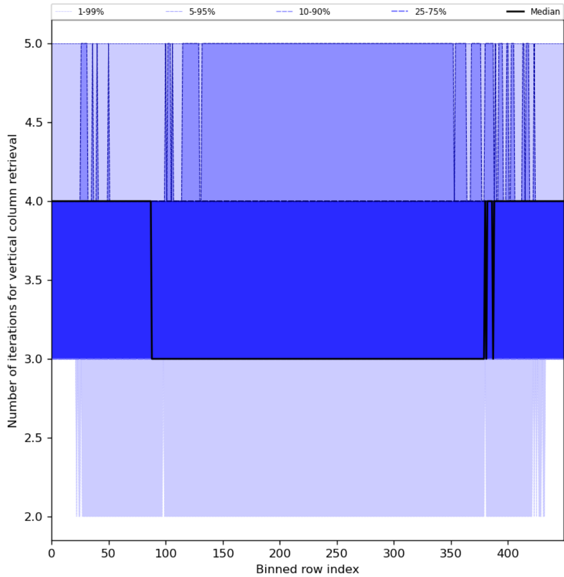
Figure 33: Along track statistics of “Number of iterations for vertical column retrieval” for 2024-08-14 to 2024-08-16
