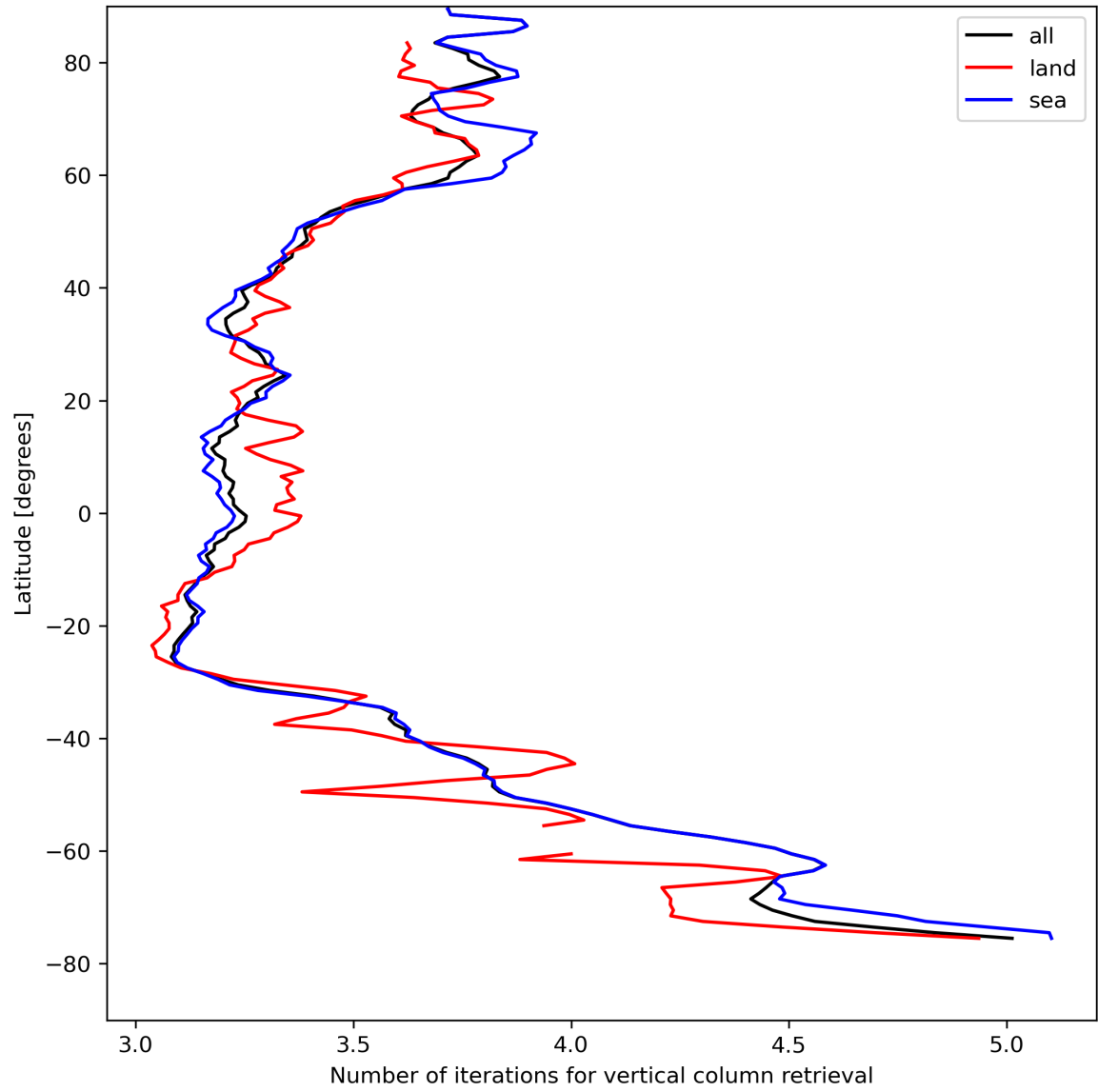
Figure 19: Zonal average of “Number of iterations for vertical column retrieval” for 2024-08-14 to 2024-08-16.
