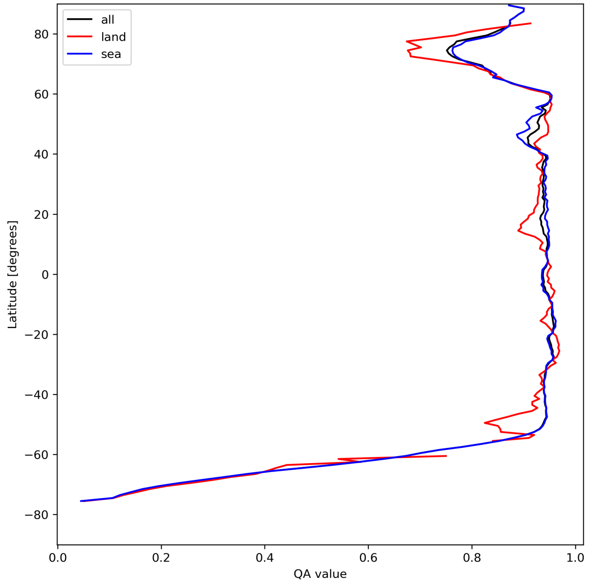
Figure 13: Zonal average of “QA value” for 2024-08-14 to 2024-08-16.
