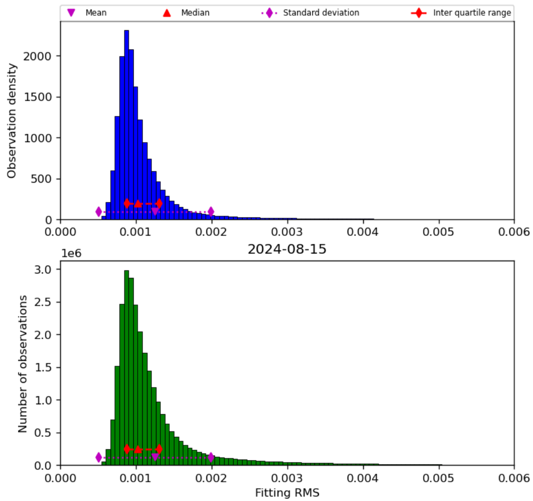
Figure 23: Histogram of “Fitting RMS” for 2024-08-14 to 2024-08-16
