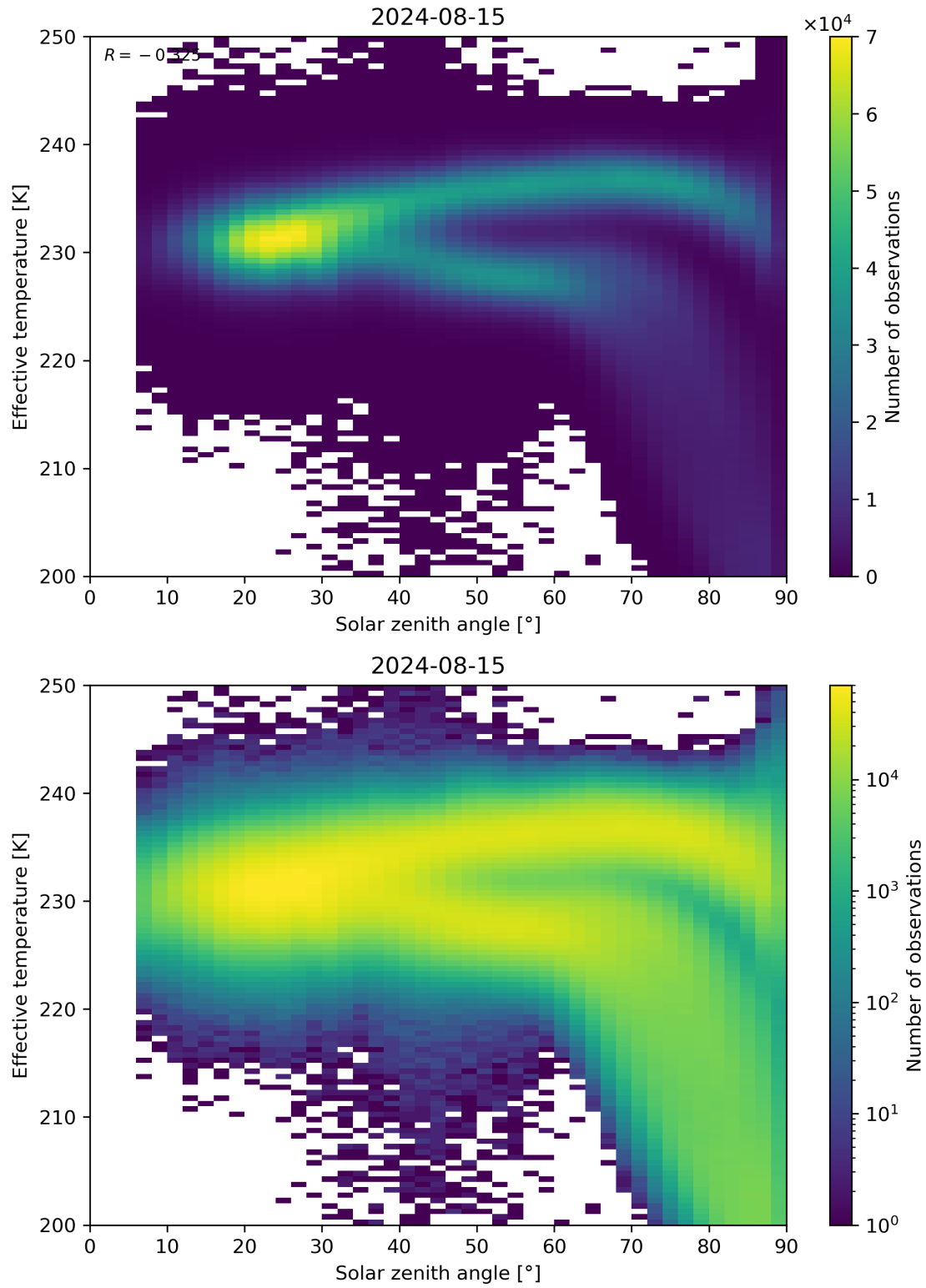
Figure 45: Scatter density plot of “Solar zenith angle” against “Effective temperature” for 2024-08-14 to 2024-08-16.
