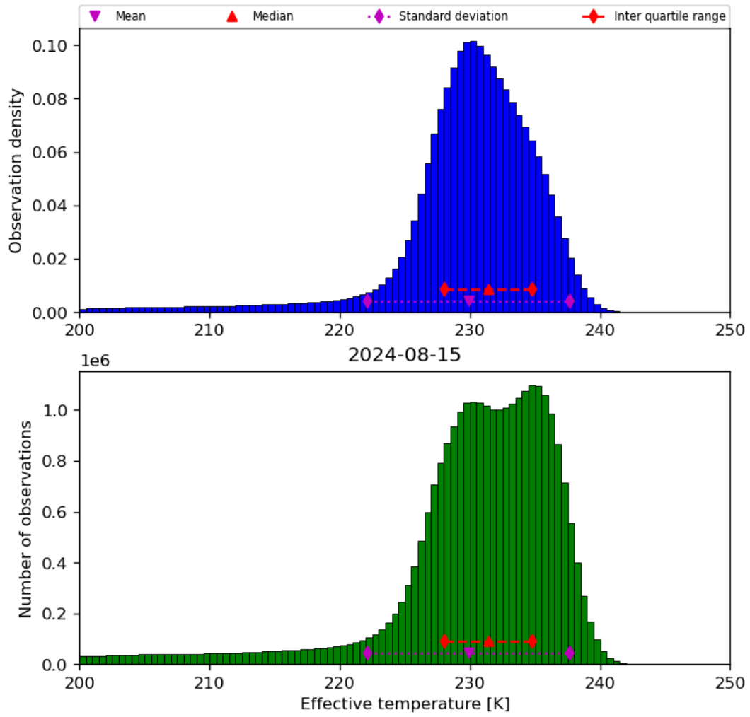
Figure 24: Histogram of “Effective temperature” for 2024-08-14 to 2024-08-16
