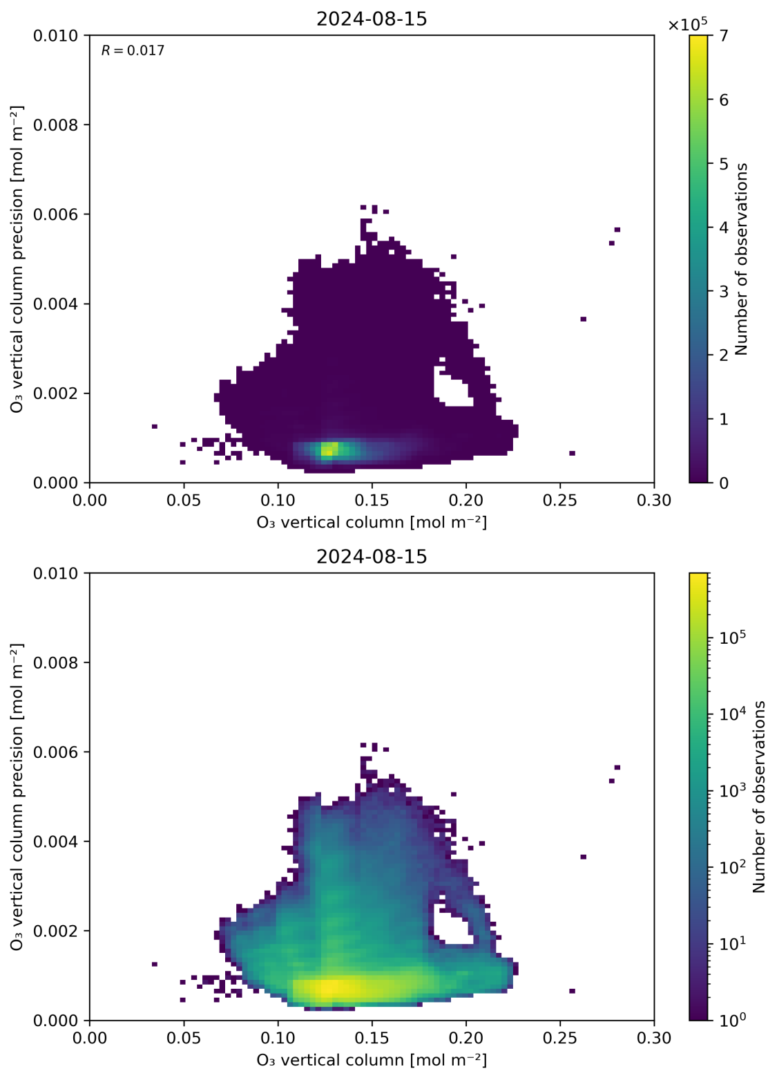
Figure 41: Scatter density plot of “O 3 vertical column” against “O 3 vertical column precision” for 2024-08-14 to 2024-08-16.
