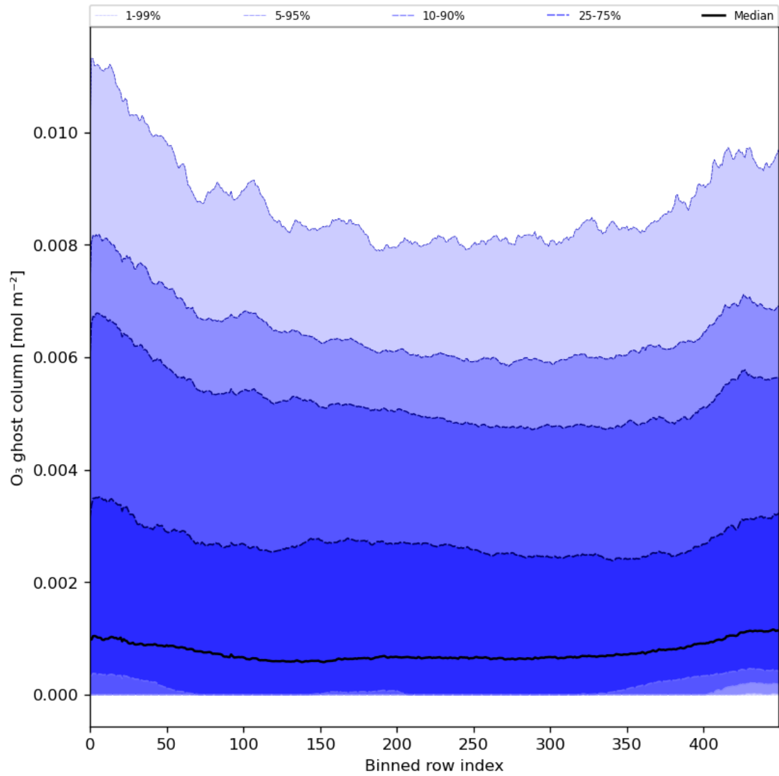
Figure 32: Along track statistics of “O 3 ghost column” for 2024-08-14 to 2024-08-16
