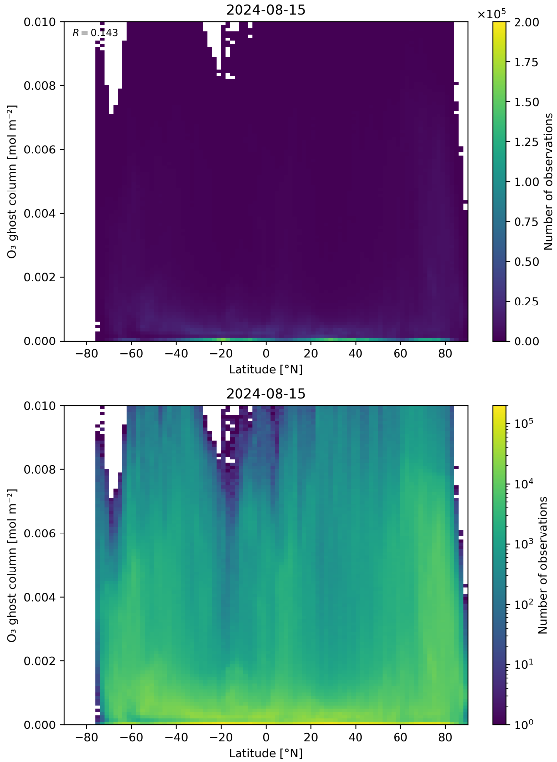
Figure 35: Scatter density plot of “Latitude” against “O 3 ghost column” for 2024-08-14 to 2024-08-16.
