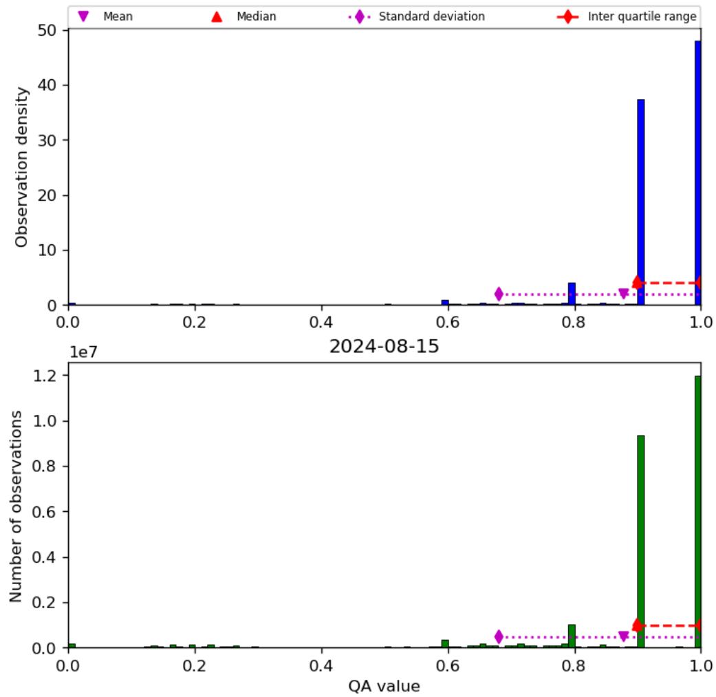
Figure 20: Histogram of “QA value” for 2024-08-14 to 2024-08-16
