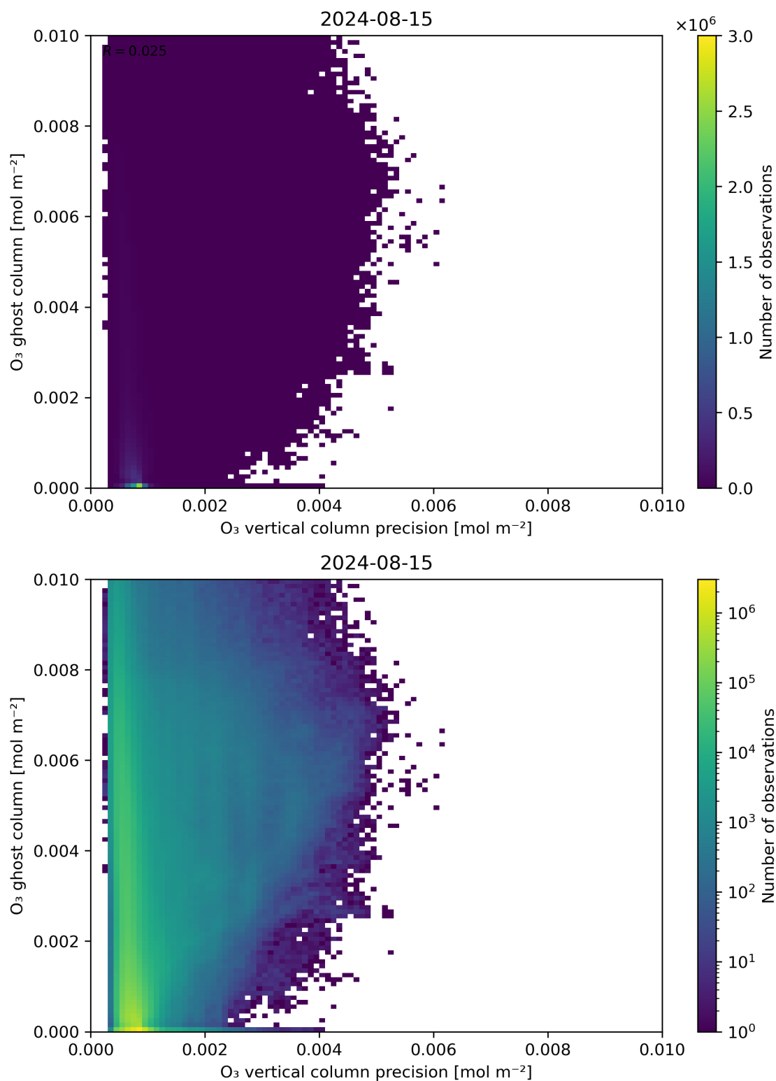
Figure 43: Scatter density plot of “O 3 vertical column precision” against “O 3 ghost column” for 2024-08-14 to 2024-08-16.
