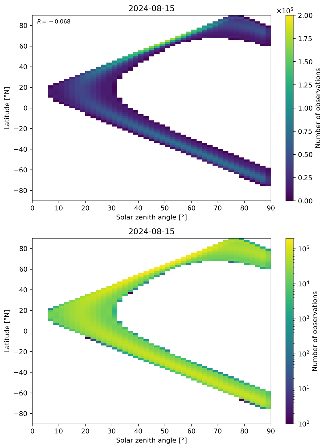
Figure 44: Scatter density plot of “Solar zenith angle” against “Latitude” for 2024-08-14 to 2024-08-16.
