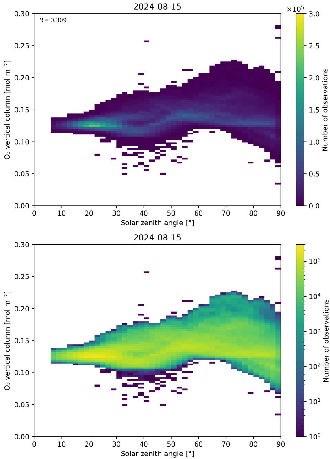
Figure 47: Scatter density plot of “Solar zenith angle” against “O 3 vertical column” for 2024-08-14 to 2024-08-16.
