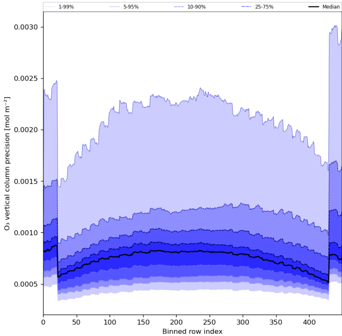
Figure 29: Along track statistics of “O 3 vertical column precision” for 2024-08-14 to 2024-08-16
