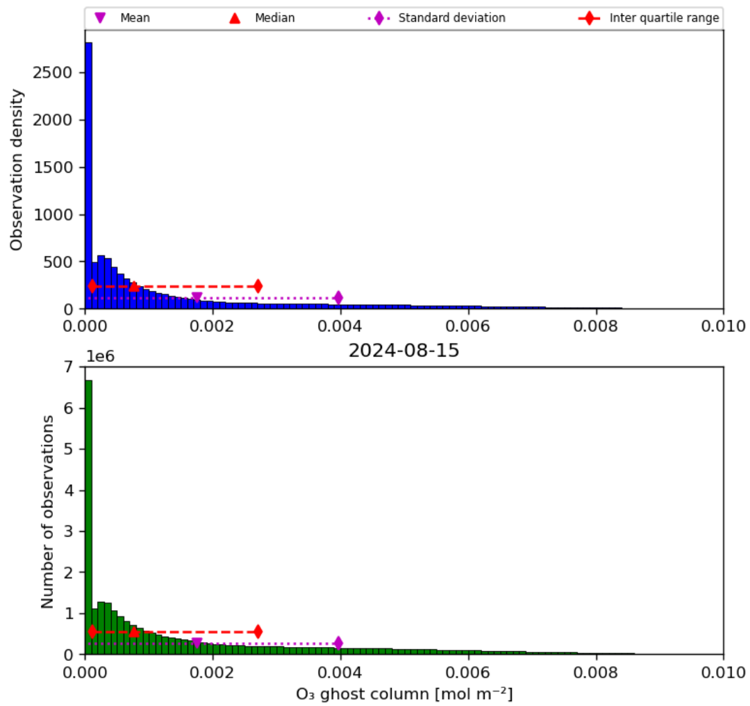
Figure 25: Histogram of “O 3 ghost column” for 2024-08-14 to 2024-08-16
