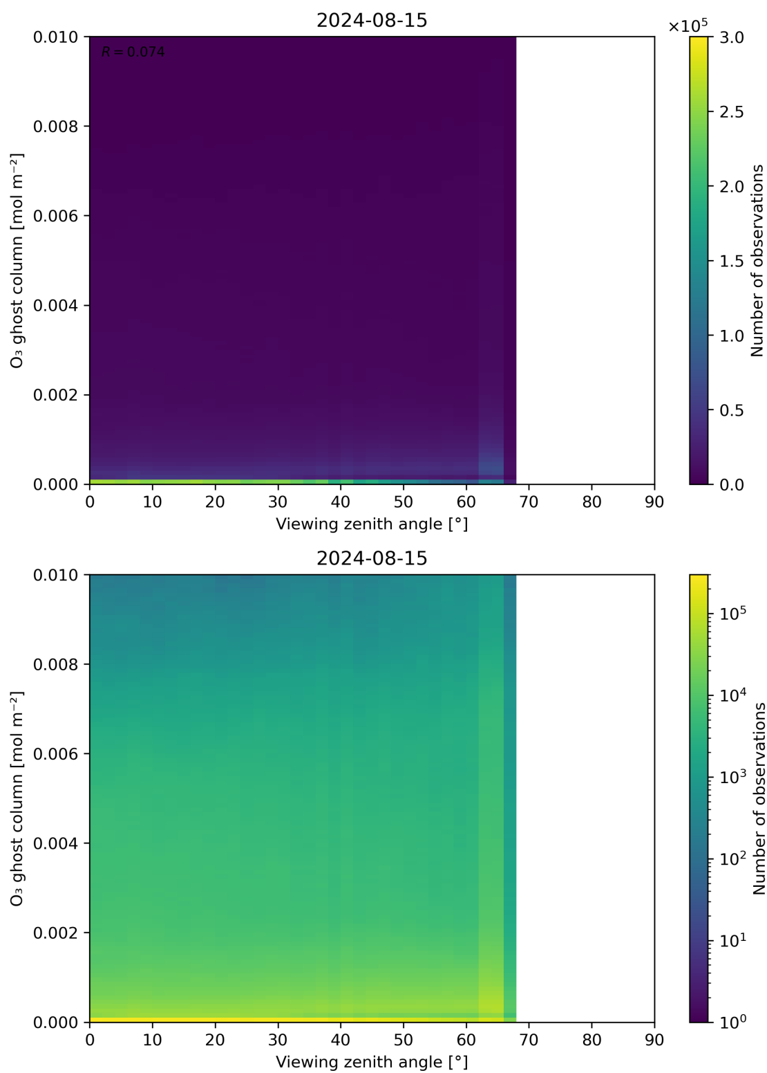
Figure 51: Scatter density plot of “Viewing zenith angle” against “O 3 ghost column” for 2024-08-14 to 2024-08-16.
