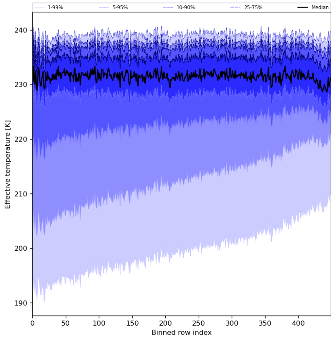
Figure 31: Along track statistics of “Effective temperature” for 2024-08-14 to 2024-08-16
