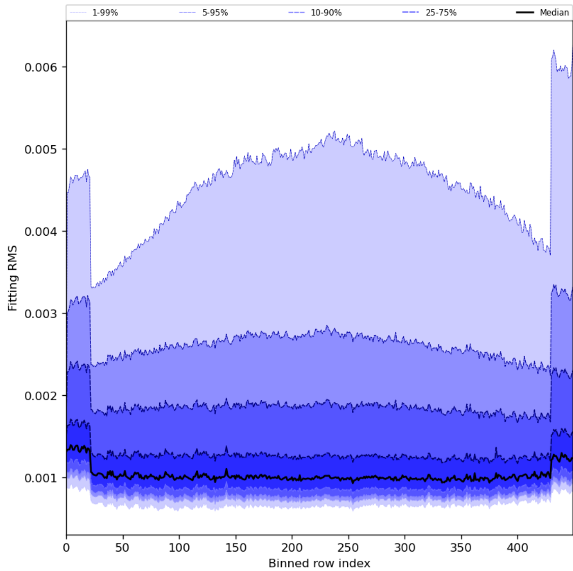
Figure 30: Along track statistics of “Fitting RMS” for 2024-08-14 to 2024-08-16
