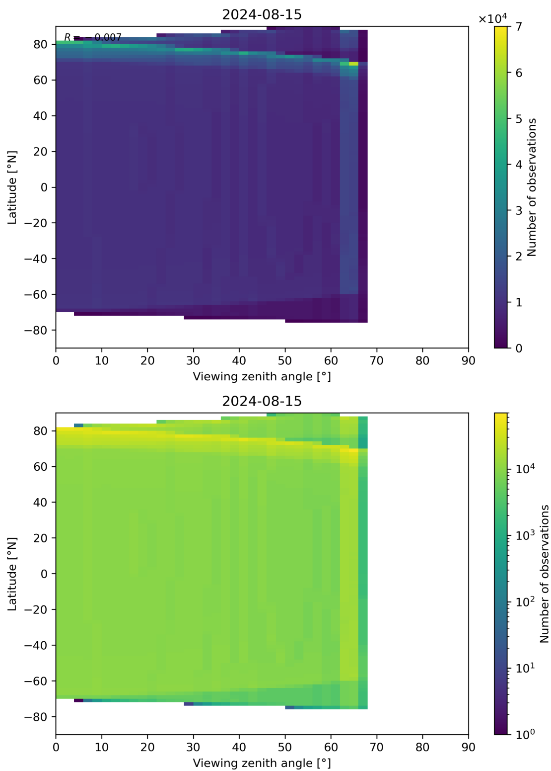
Figure 49: Scatter density plot of “Viewing zenith angle” against “Latitude” for 2024-08-14 to 2024-08-16.
