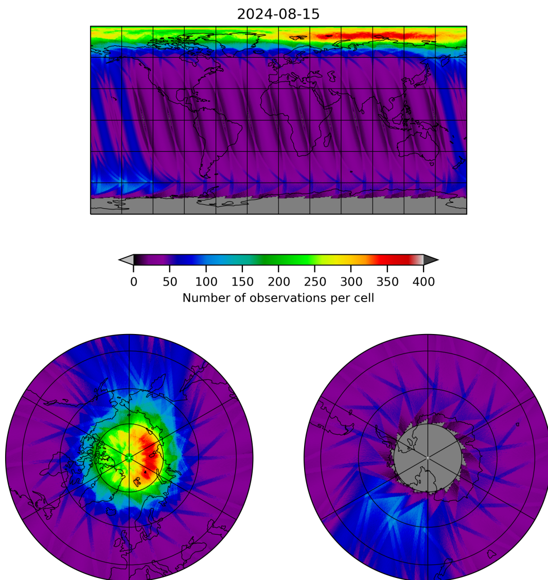
Figure 12: Map of the number of observations for 2024-08-14 to 2024-08-16
