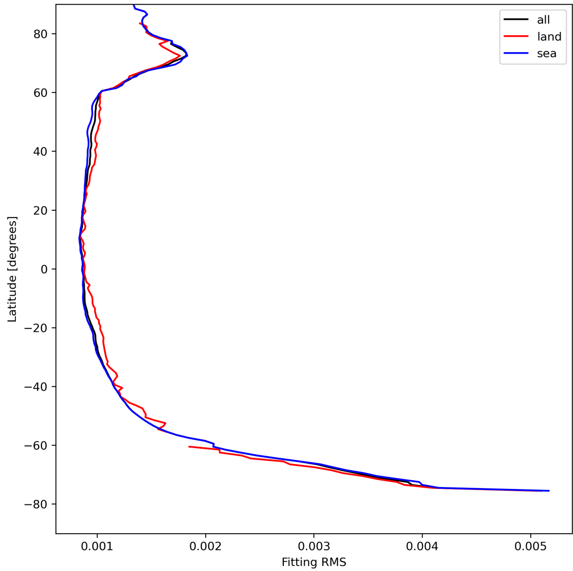
Figure 16: Zonal average of “Fitting RMS” for 2024-08-14 to 2024-08-16.
