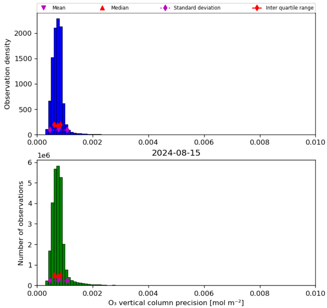
Figure 22: Histogram of “O 3 vertical column precision” for 2024-08-14 to 2024-08-16
