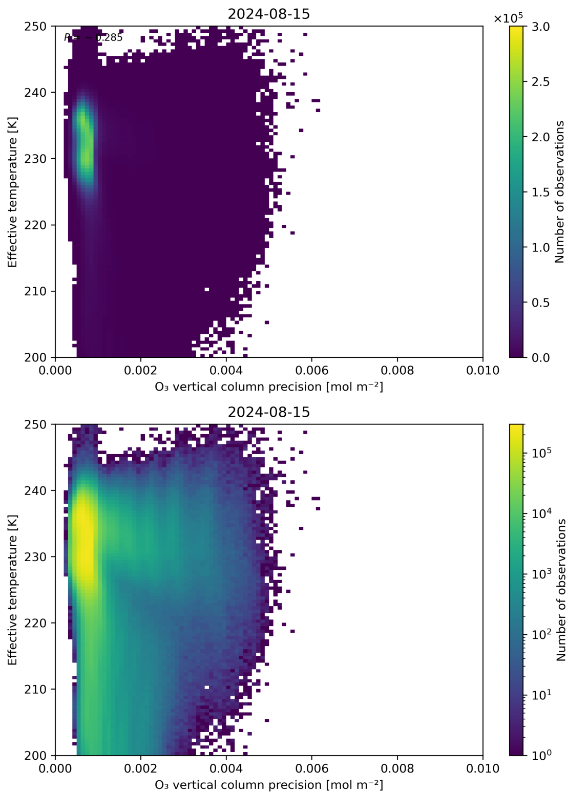
Figure 42: Scatter density plot of “O 3 vertical column precision” against “Effective temperature” for 2024-08-14 to 2024-08-16.
