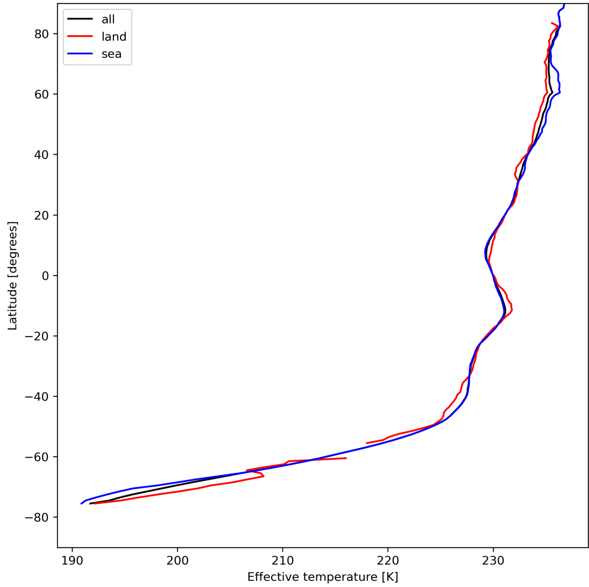
Figure 17: Zonal average of “Effective temperature” for 2024-08-14 to 2024-08-16.
