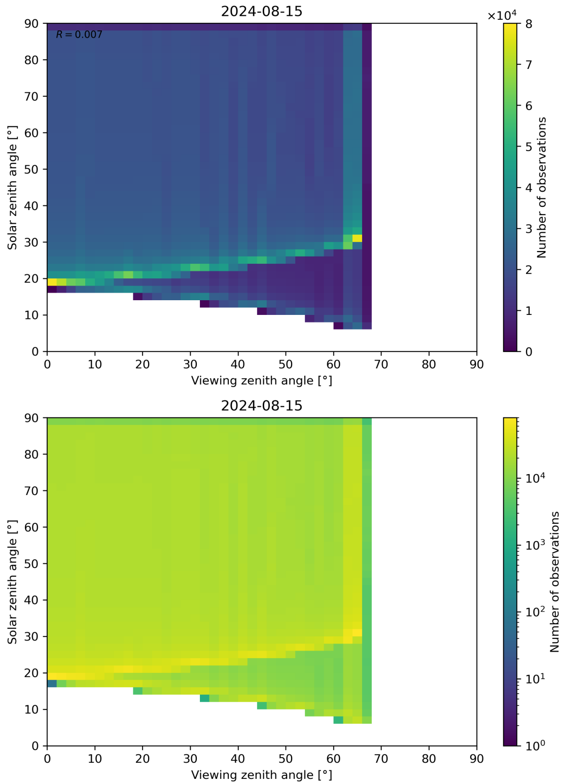
Figure 54: Scatter density plot of “Viewing zenith angle” against “Solar zenith angle” for 2024-08-14 to 2024-08-16.
