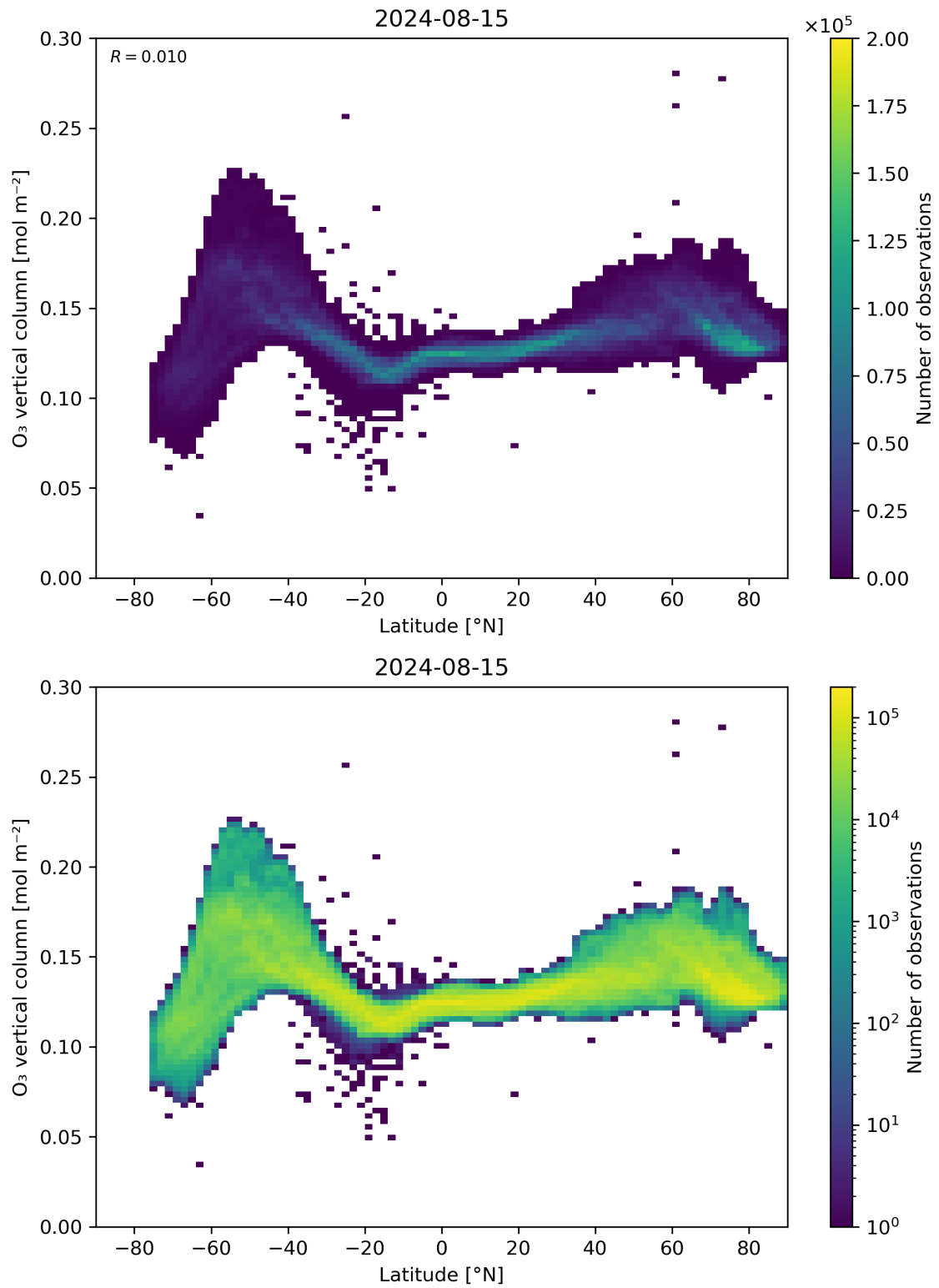
Figure 36: Scatter density plot of “Latitude” against “O 3 vertical column” for 2024-08-14 to 2024-08-16.
