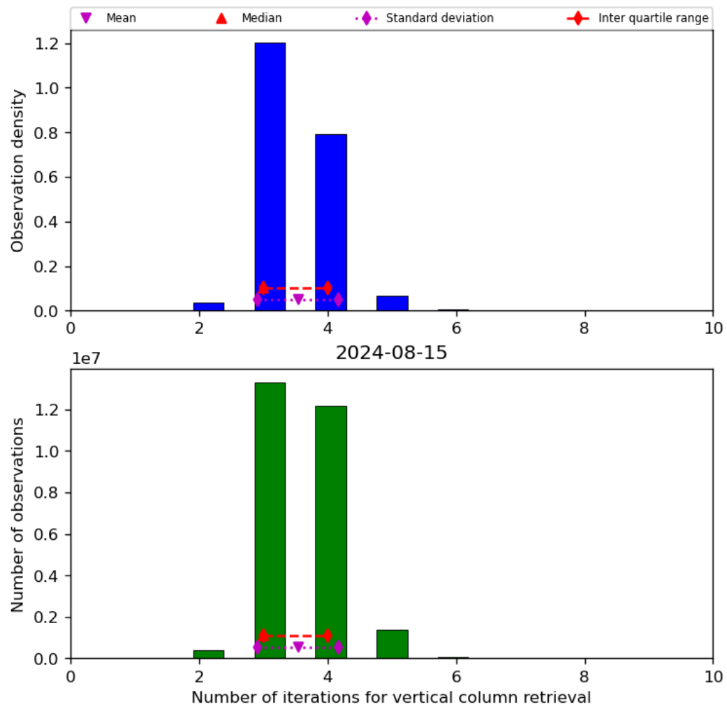
Figure 26: Histogram of “Number of iterations for vertical column retrieval” for 2024-08-14 to 2024-08-16
