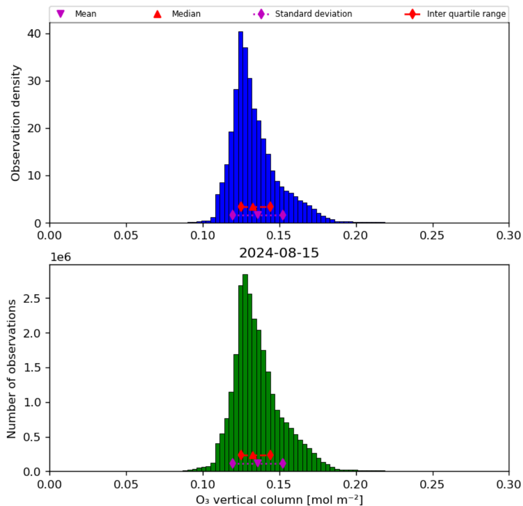
Figure 21: Histogram of “O 3 vertical column” for 2024-08-14 to 2024-08-16
