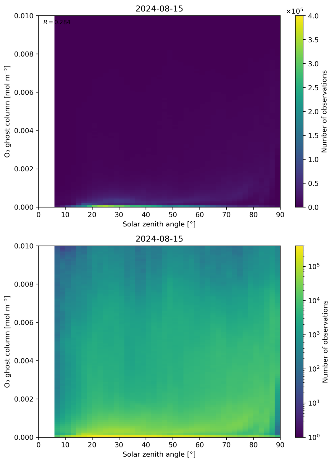
Figure 46: Scatter density plot of “Solar zenith angle” against “O 3 ghost column” for 2024-08-14 to 2024-08-16.
