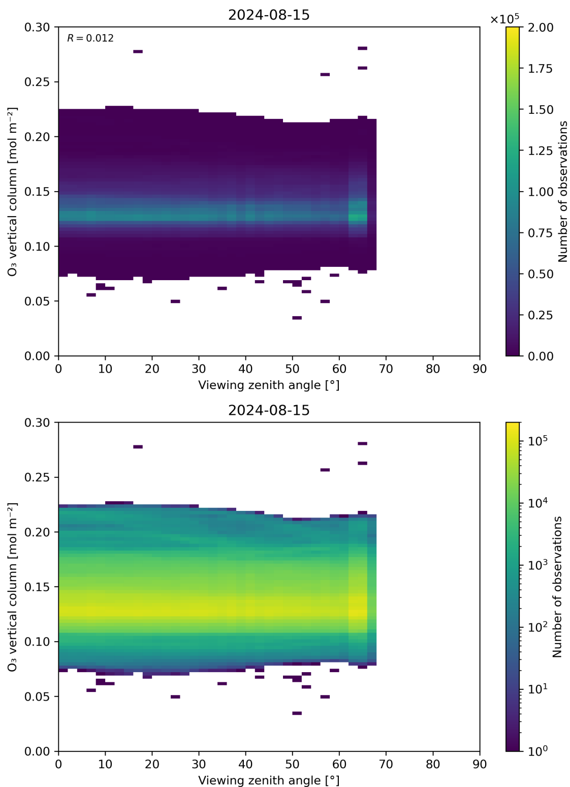
Figure 52: Scatter density plot of “Viewing zenith angle” against “O 3 vertical column” for 2024-08-14 to 2024-08-16.
