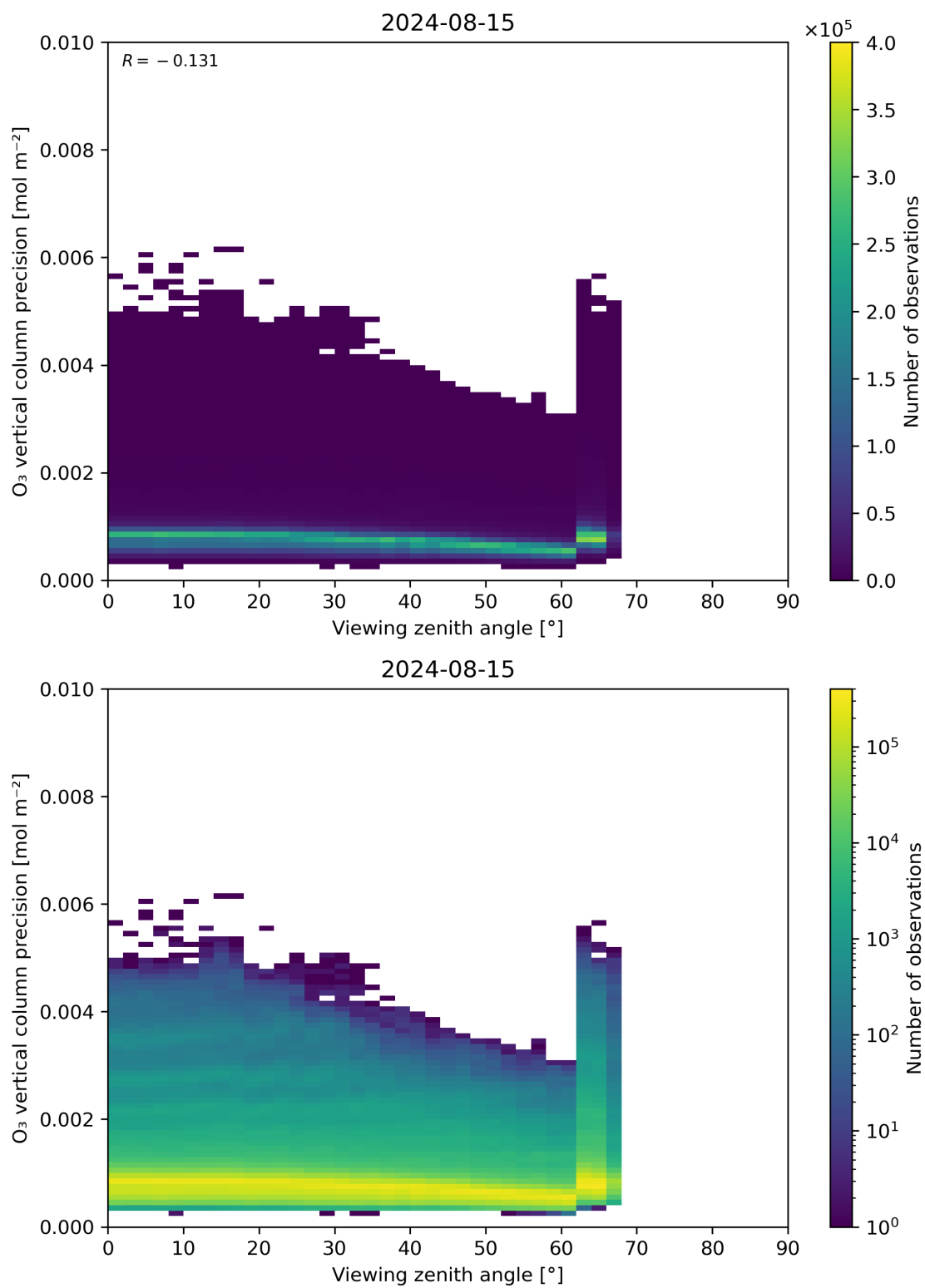
Figure 53: Scatter density plot of “Viewing zenith angle” against “O 3 vertical column precision” for 2024-08-14 to 2024-08-16.
