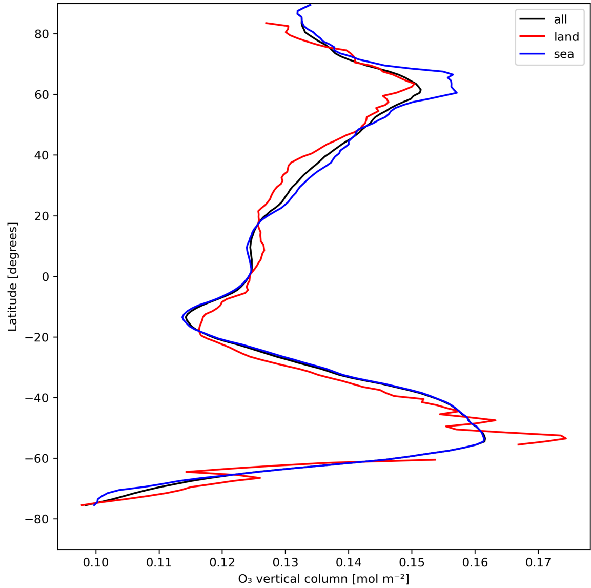
Figure 14: Zonal average of “O 3 vertical column” for 2024-08-14 to 2024-08-16.
