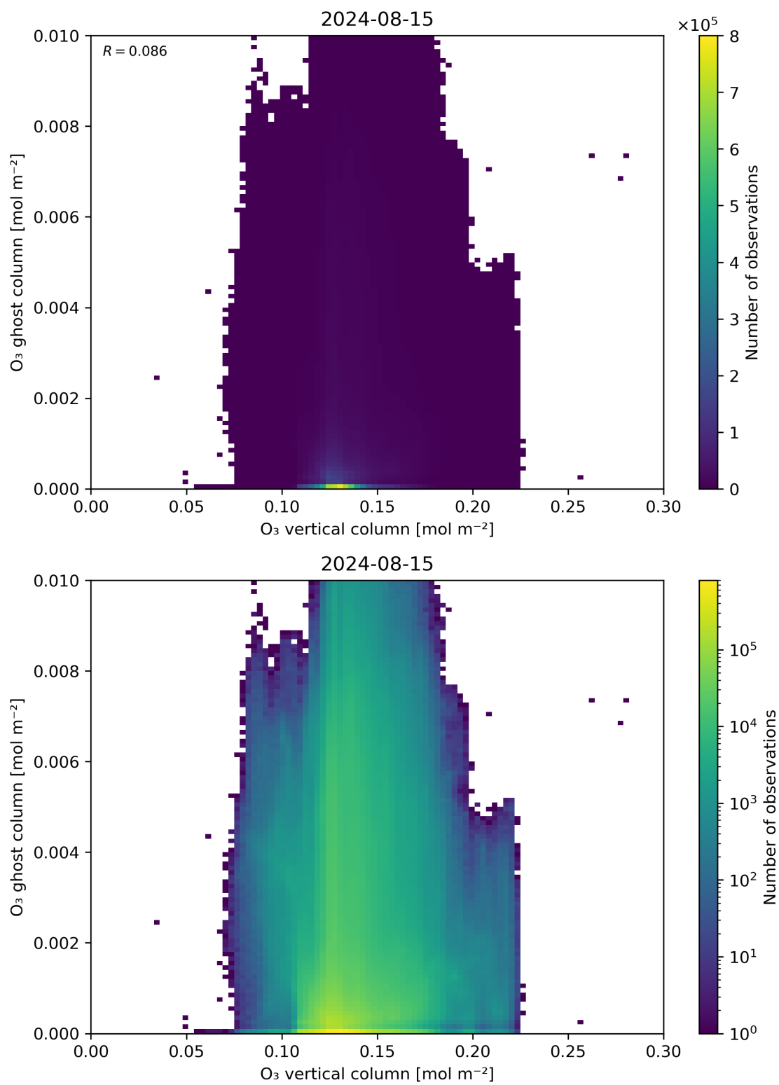
Figure 40: Scatter density plot of “O 3 vertical column” against “O 3 ghost column” for 2024-08-14 to 2024-08-16.
