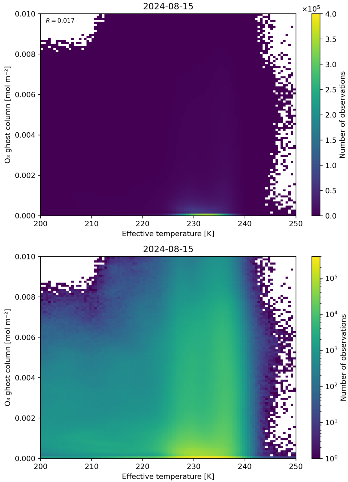
Figure 38: Scatter density plot of “Effective temperature” against “O 3 ghost column” for 2024-08-14 to 2024-08-16.
