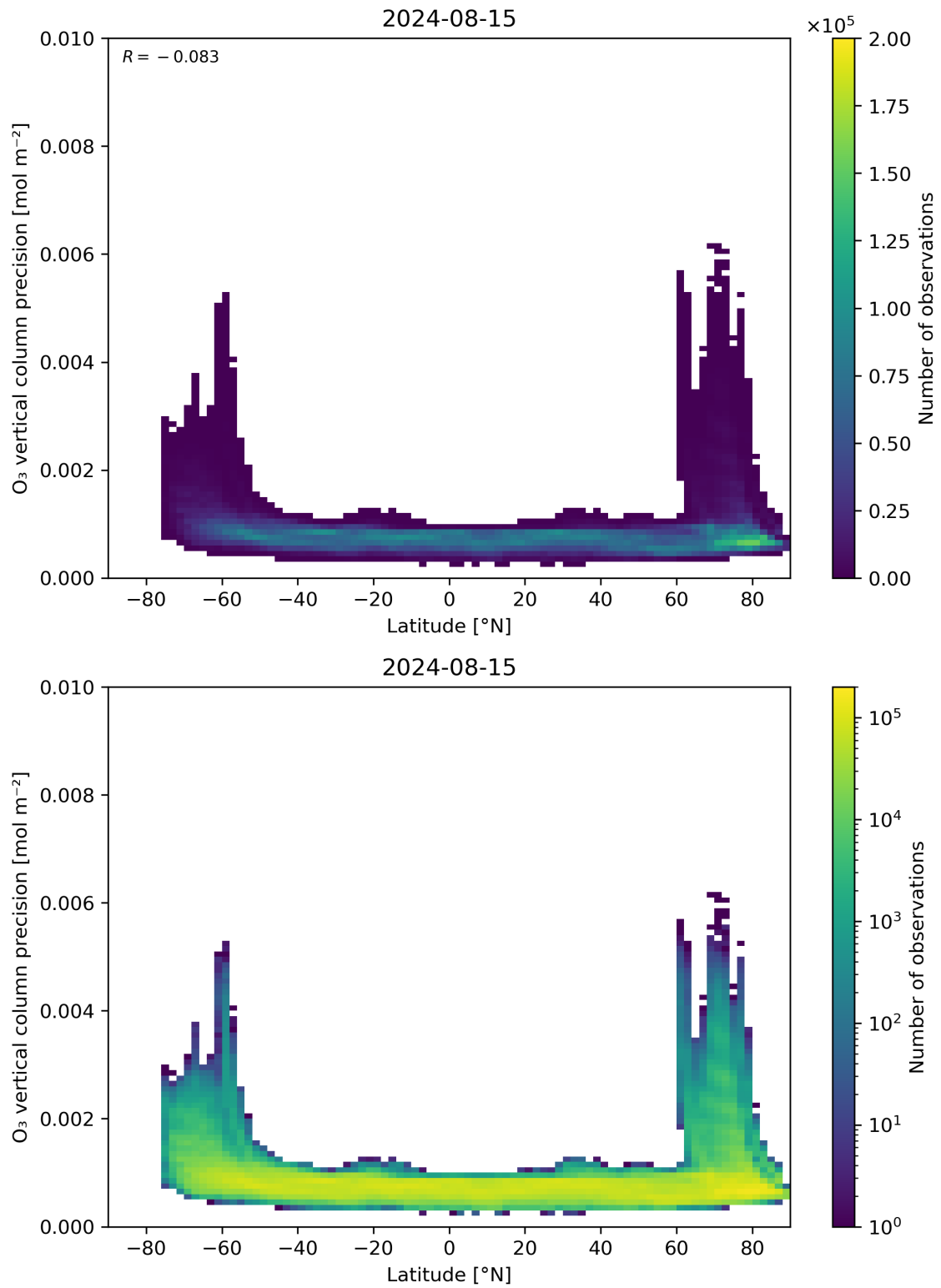
Figure 37: Scatter density plot of “Latitude” against “O 3 vertical column precision” for 2024-08-14 to 2024-08-16.
