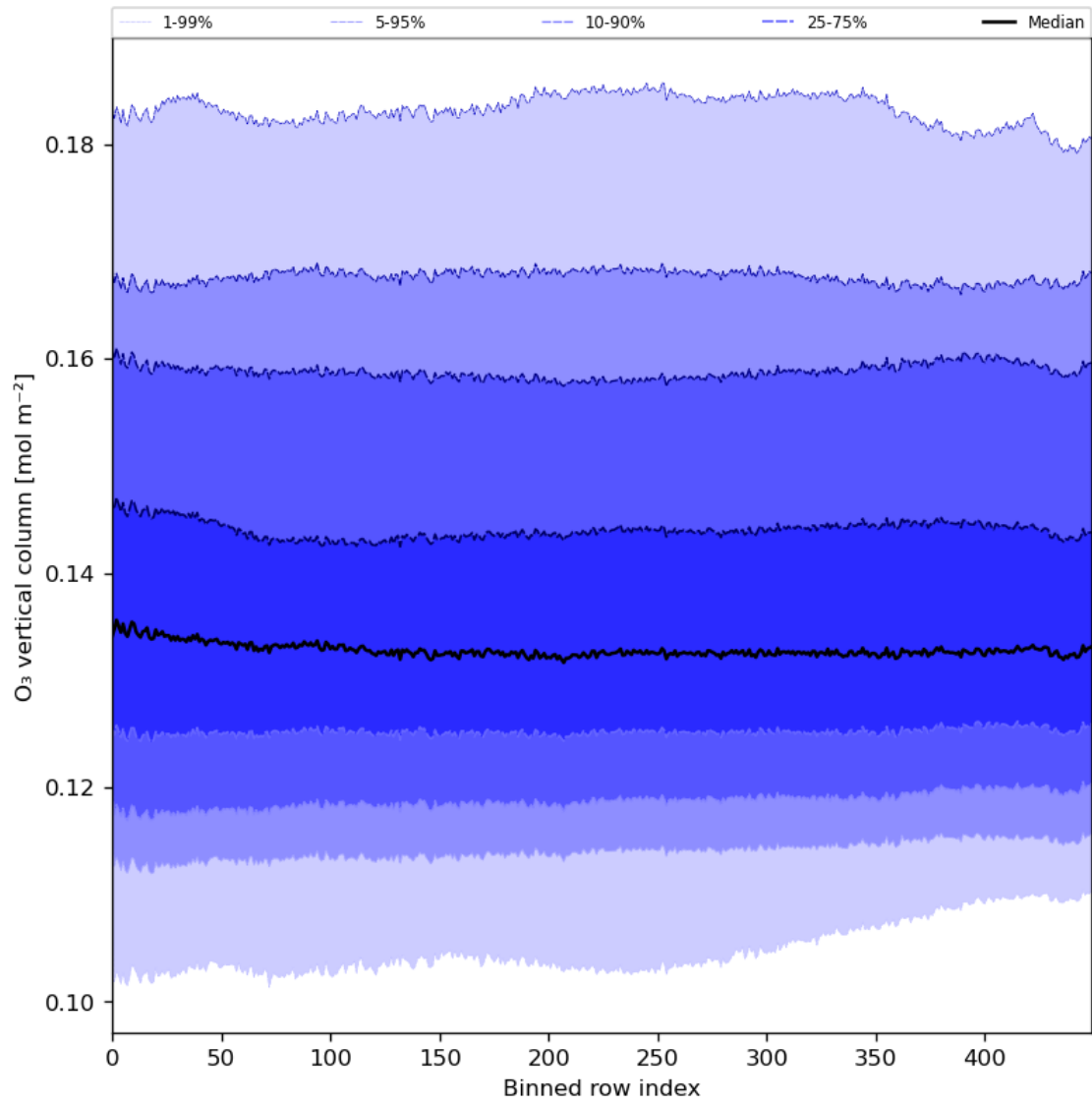
Figure 28: Along track statistics of “O 3 vertical column” for 2024-08-14 to 2024-08-16
