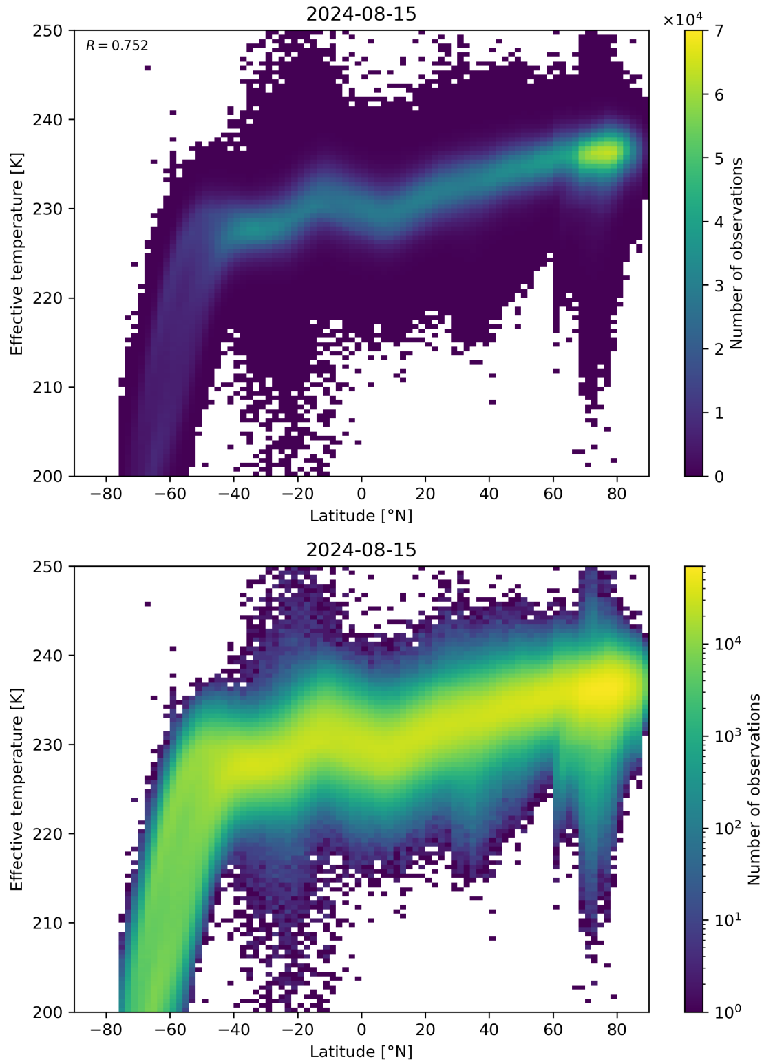
Figure 34: Scatter density plot of “Latitude” against “Effective temperature” for 2024-08-14 to 2024-08-16.
