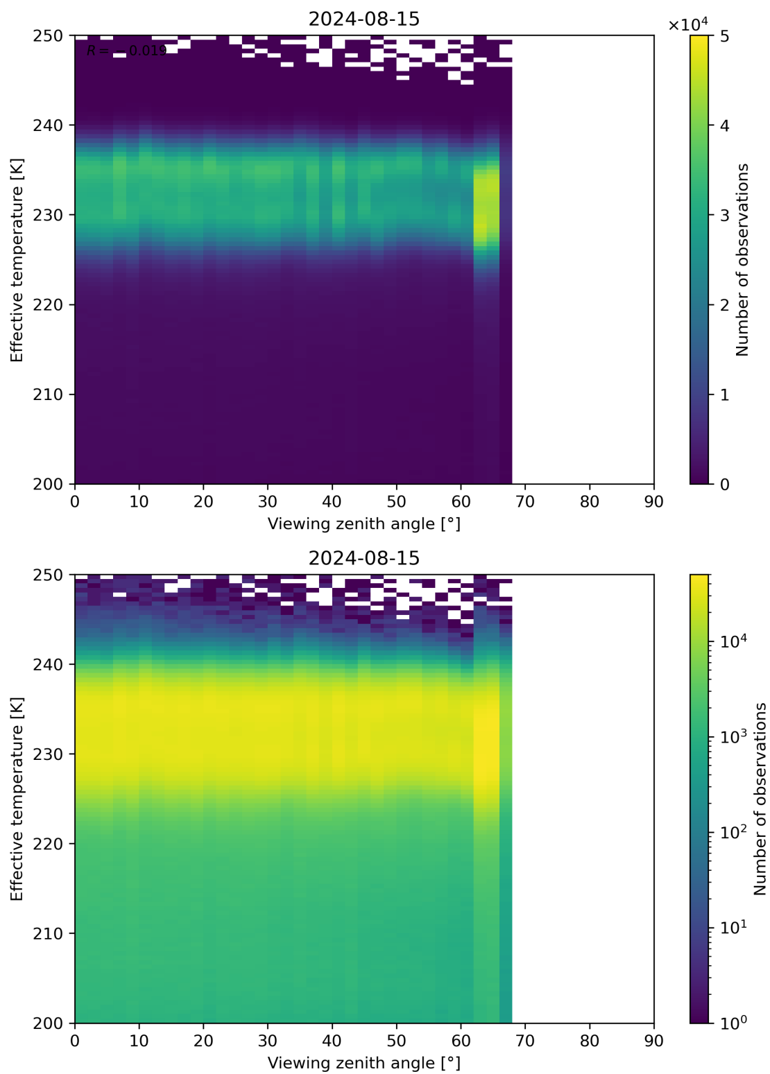
Figure 50: Scatter density plot of “Viewing zenith angle” against “Effective temperature” for 2024-08-14 to 2024-08-16.
