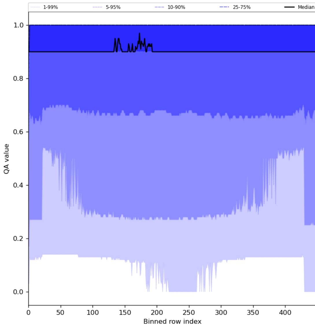
Figure 27: Along track statistics of “QA value” for 2024-08-14 to 2024-08-16
