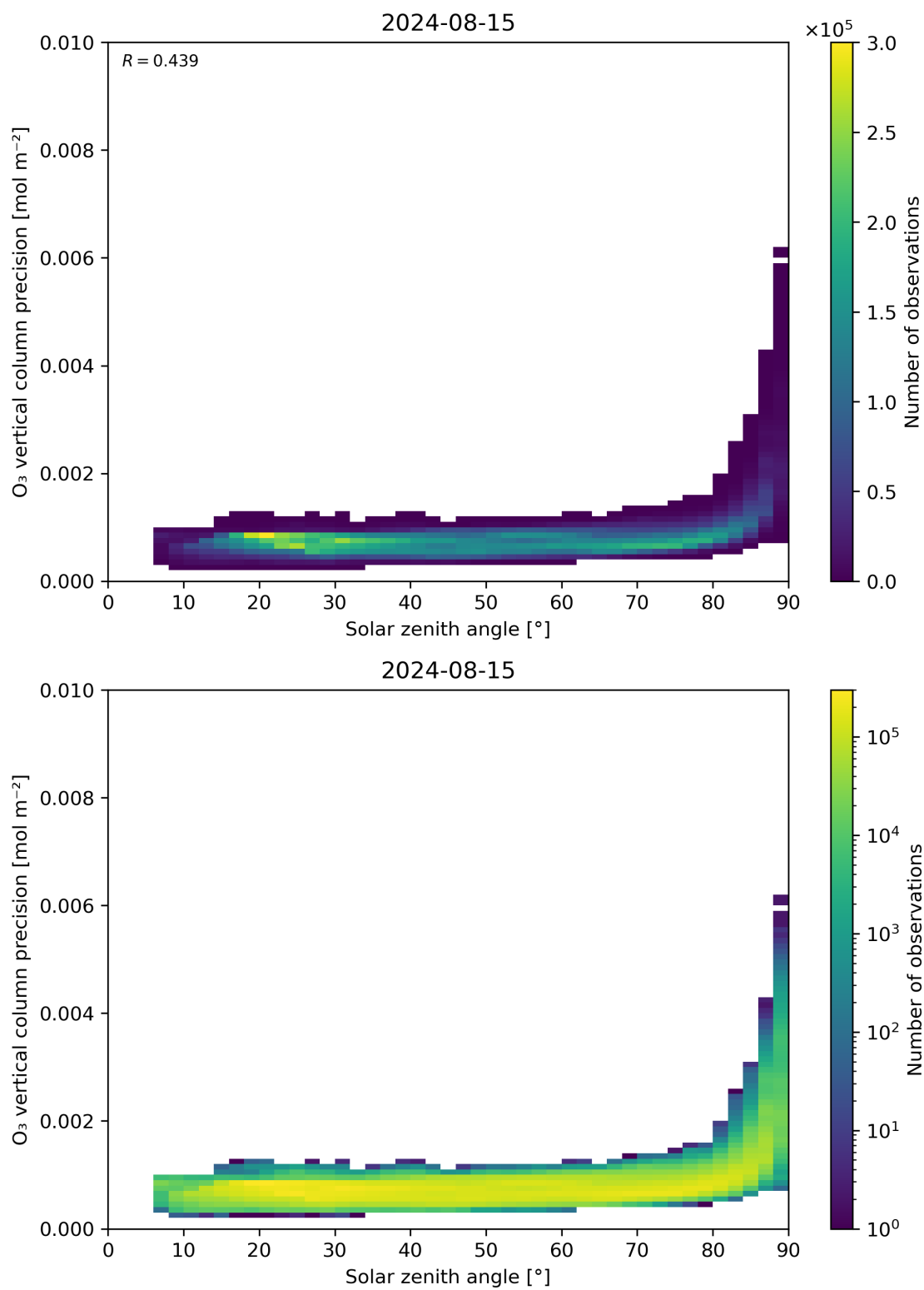
Figure 48: Scatter density plot of “Solar zenith angle” against “O 3 vertical column precision” for 2024-08-14 to 2024-08-16.
