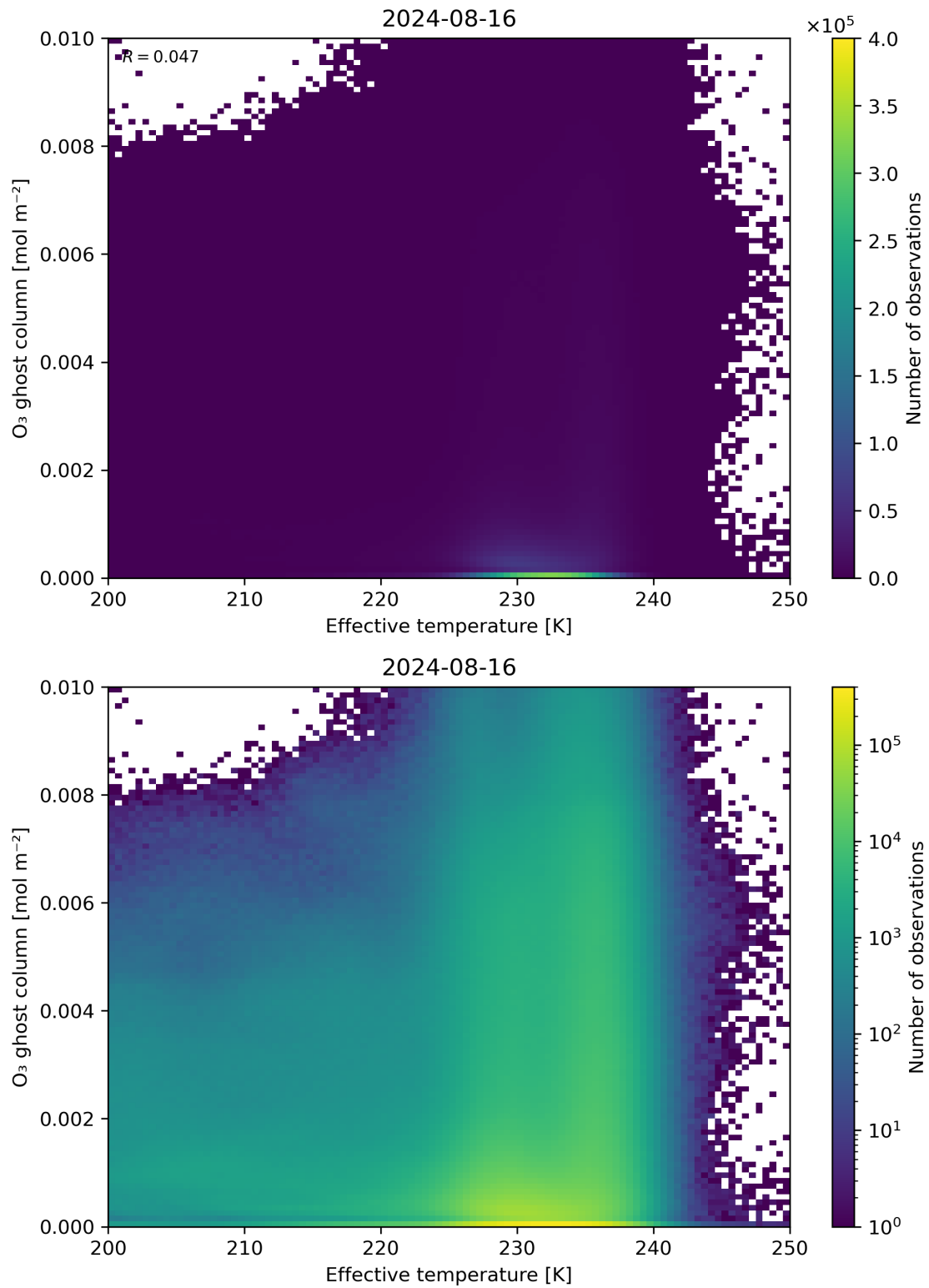
Figure 38: Scatter density plot of “Effective temperature” against “O 3 ghost column” for 2024-08-16 to 2024-08-17.
