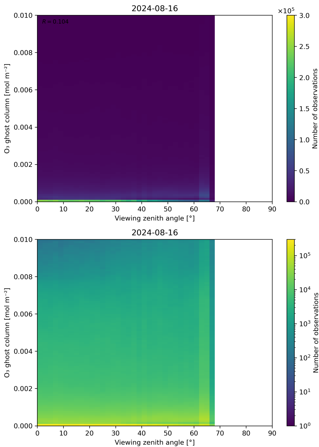
Figure 51: Scatter density plot of “Viewing zenith angle” against “O 3 ghost column” for 2024-08-16 to 2024-08-17.
