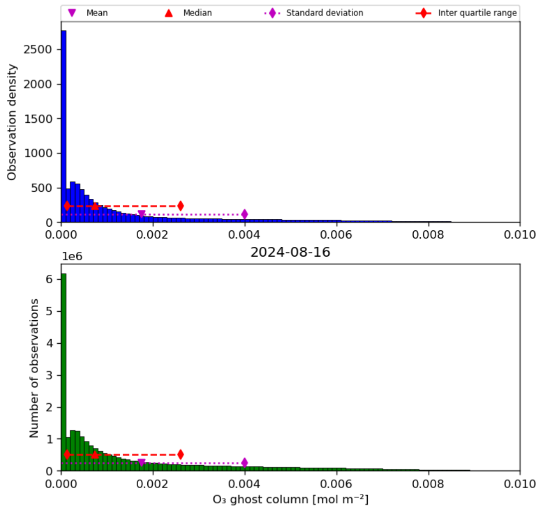
Figure 25: Histogram of “O 3 ghost column” for 2024-08-16 to 2024-08-17
