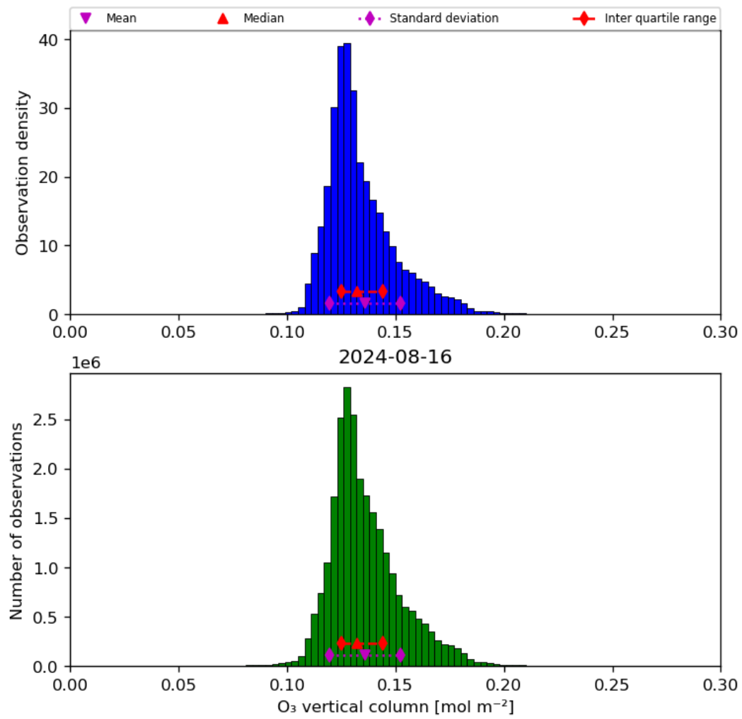
Figure 21: Histogram of “O 3 vertical column” for 2024-08-16 to 2024-08-17
