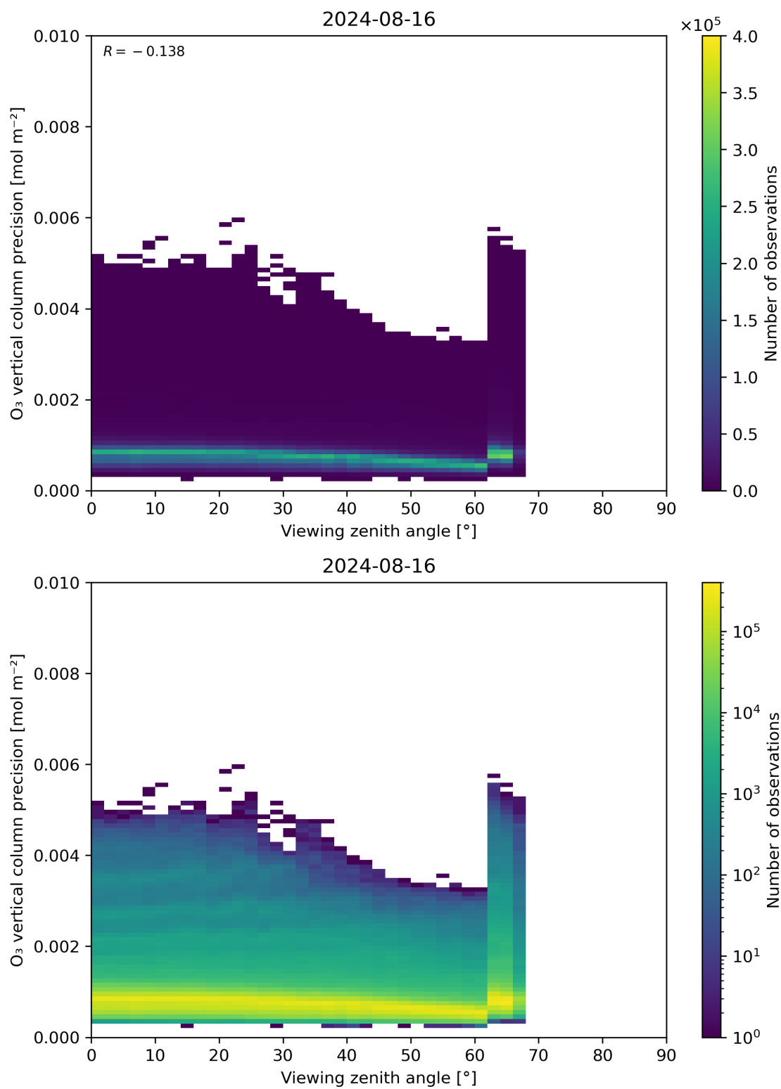
Figure 53: Scatter density plot of “Viewing zenith angle” against “O 3 vertical column precision” for 2024-08-16 to 2024-08-17.
