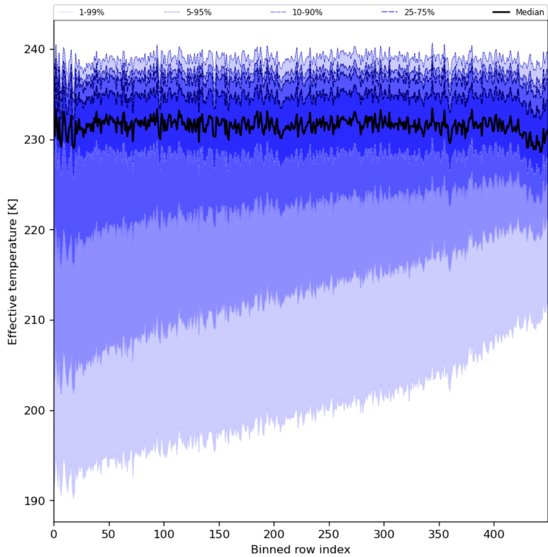
Figure 31: Along track statistics of “Effective temperature” for 2024-08-16 to 2024-08-17
