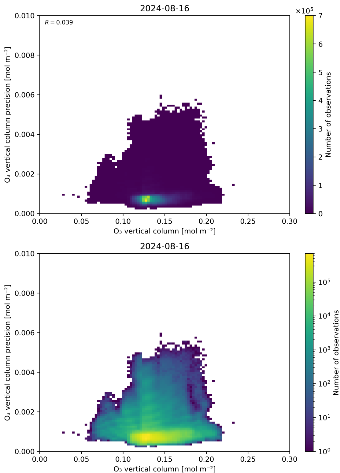
Figure 41: Scatter density plot of “O 3 vertical column” against “O 3 vertical column precision” for 2024-08-16 to 2024-08-17.
