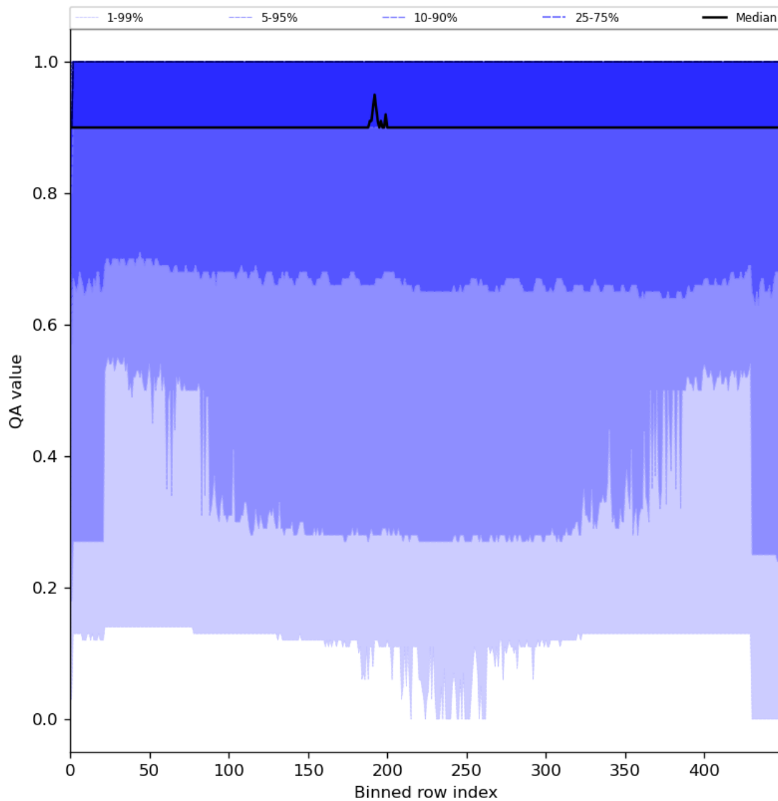
Figure 27: Along track statistics of “QA value” for 2024-08-16 to 2024-08-17
