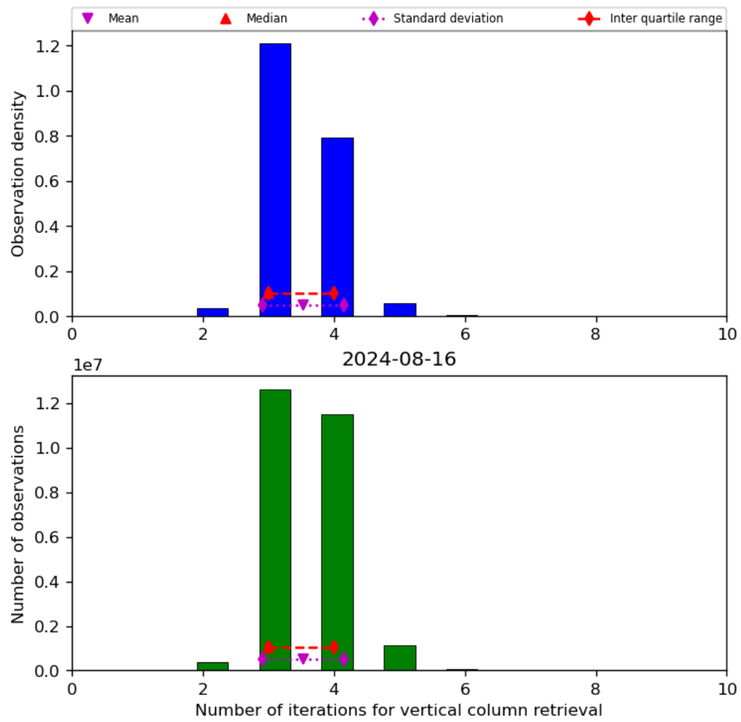
Figure 26: Histogram of “Number of iterations for vertical column retrieval” for 2024-08-16 to 2024-08-17
