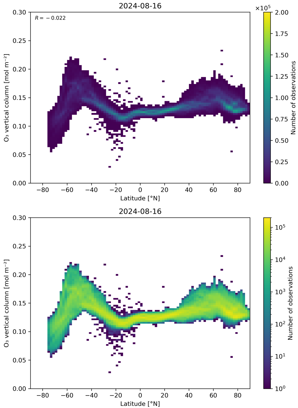
Figure 36: Scatter density plot of “Latitude” against “O 3 vertical column” for 2024-08-16 to 2024-08-17.
