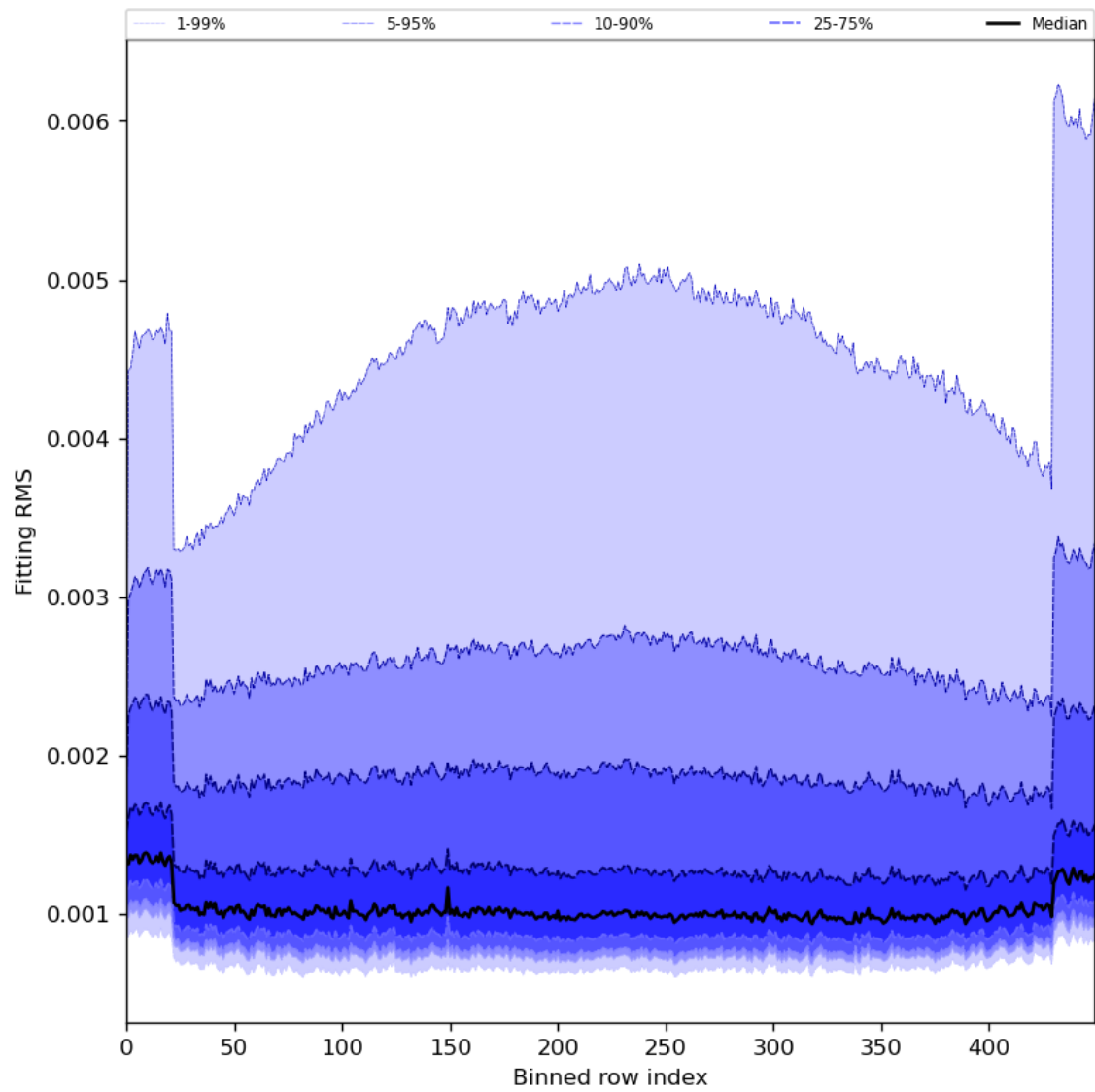
Figure 30: Along track statistics of “Fitting RMS” for 2024-08-16 to 2024-08-17
