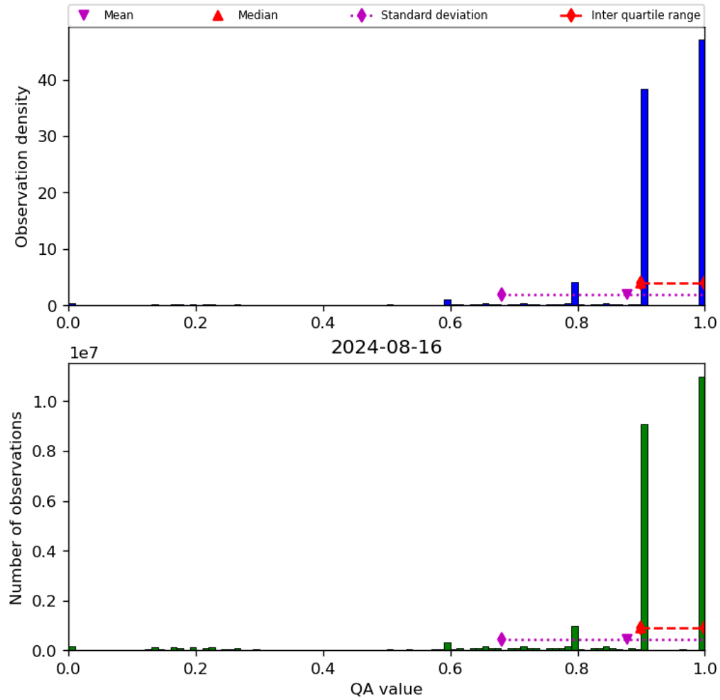
Figure 20: Histogram of “QA value” for 2024-08-16 to 2024-08-17
