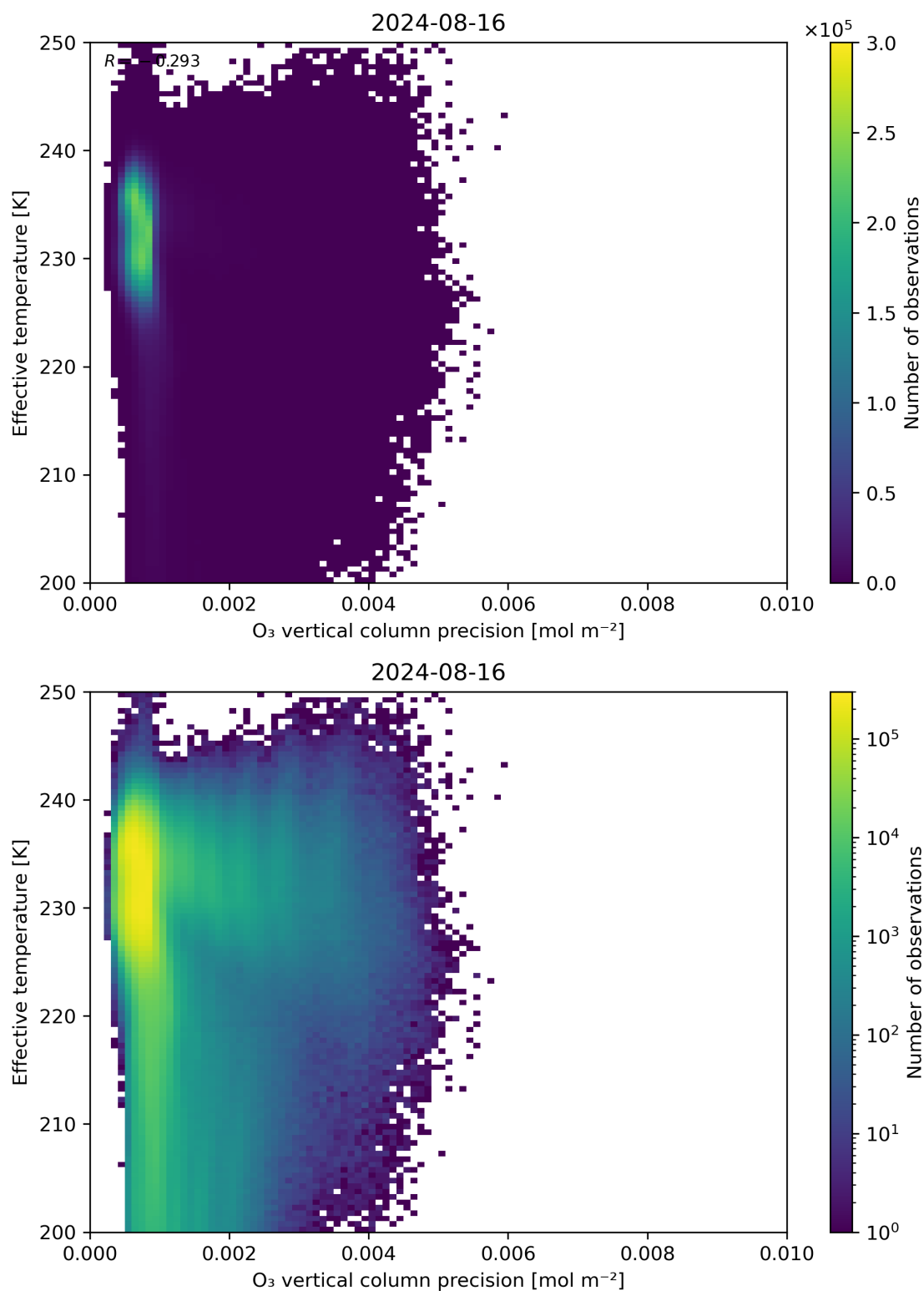
Figure 42: Scatter density plot of “O 3 vertical column precision” against “Effective temperature” for 2024-08-16 to 2024-08-17.
