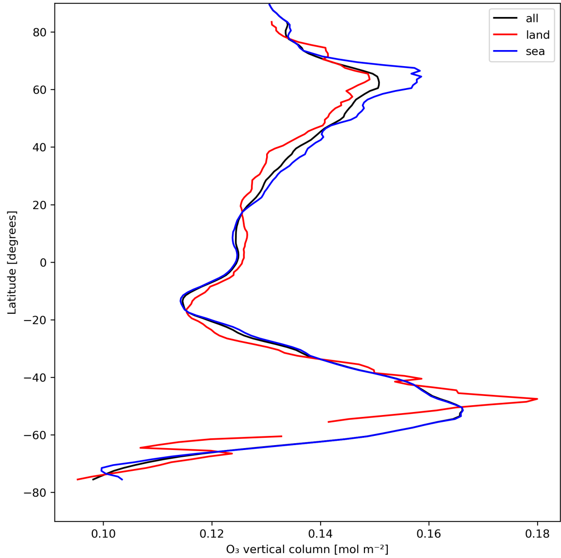
Figure 14: Zonal average of “O 3 vertical column” for 2024-08-16 to 2024-08-17.
