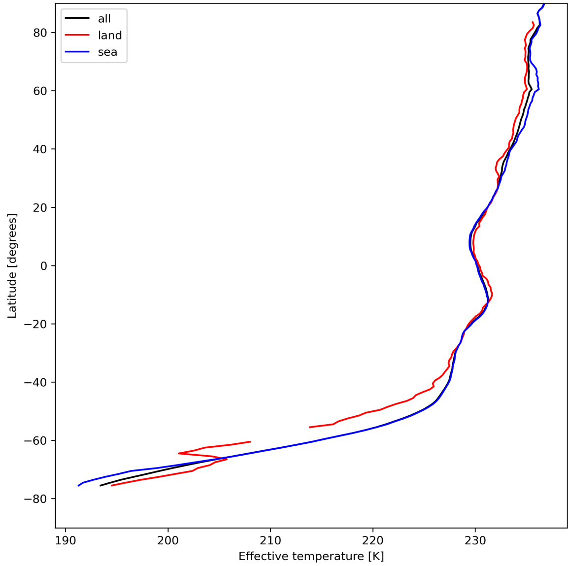
Figure 17: Zonal average of "Effective temperature" for 2024-08-16 to 2024-08-17.
