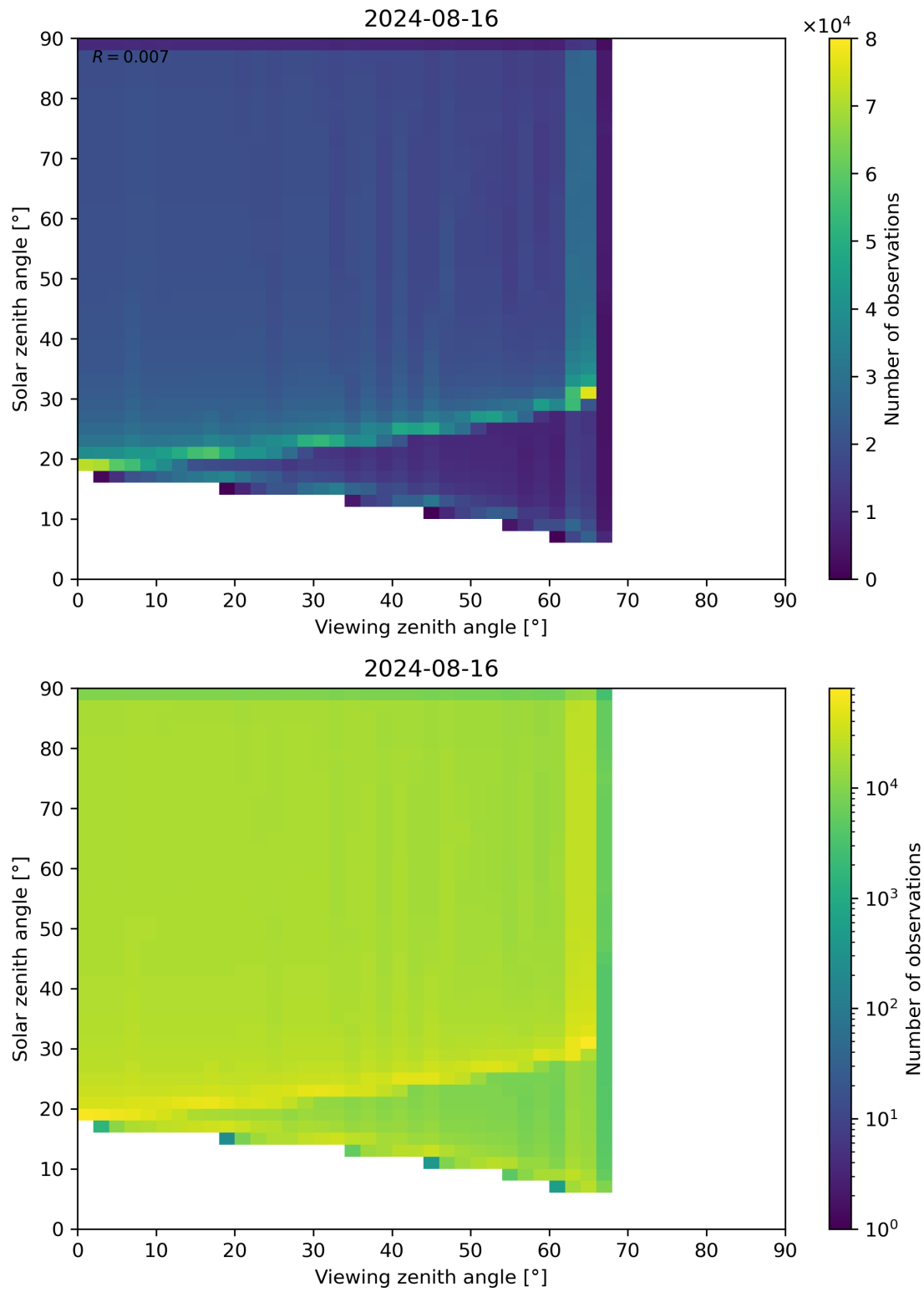
Figure 54: Scatter density plot of “Viewing zenith angle” against “Solar zenith angle” for 2024-08-16 to 2024-08-17.
