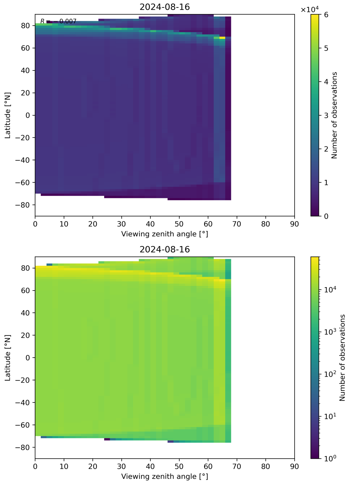
Figure 49: Scatter density plot of “Viewing zenith angle” against “Latitude” for 2024-08-16 to 2024-08-17.
