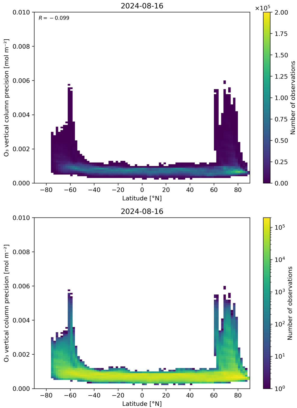
Figure 37: Scatter density plot of “Latitude” against “O 3 vertical column precision” for 2024-08-16 to 2024-08-17.
