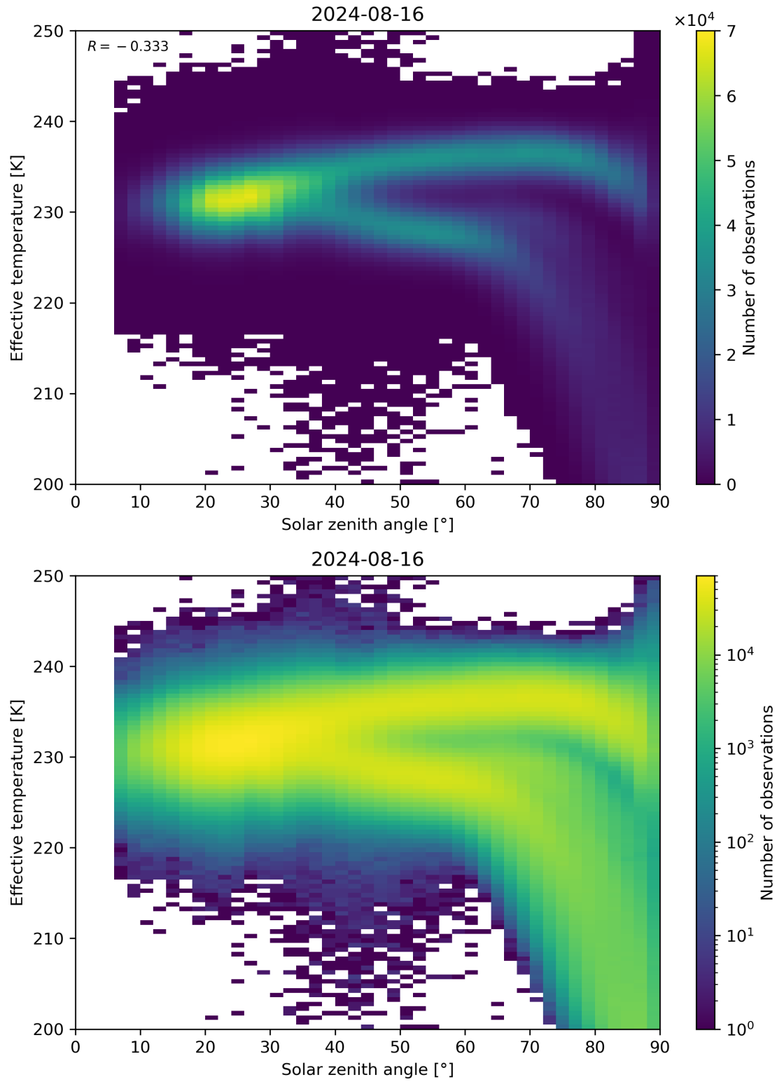
Figure 45: Scatter density plot of “Solar zenith angle” against “Effective temperature” for 2024-08-16 to 2024-08-17.
