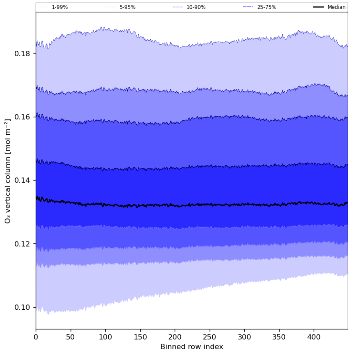
Figure 28: Along track statistics of “O 3 vertical column” for 2024-08-16 to 2024-08-17
