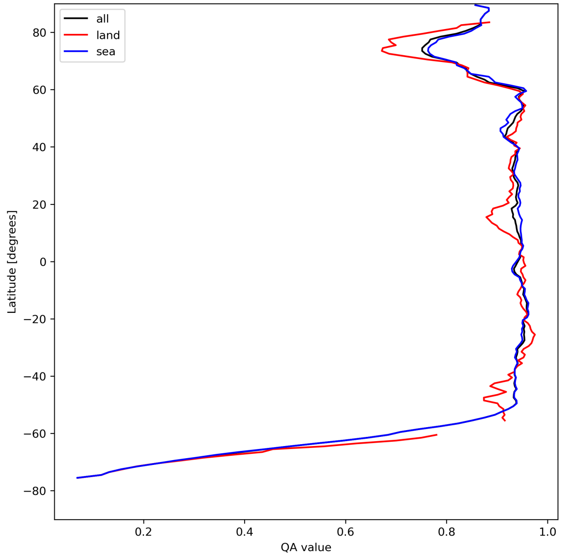
Figure 13: Zonal average of “QA value” for 2024-08-16 to 2024-08-17.
