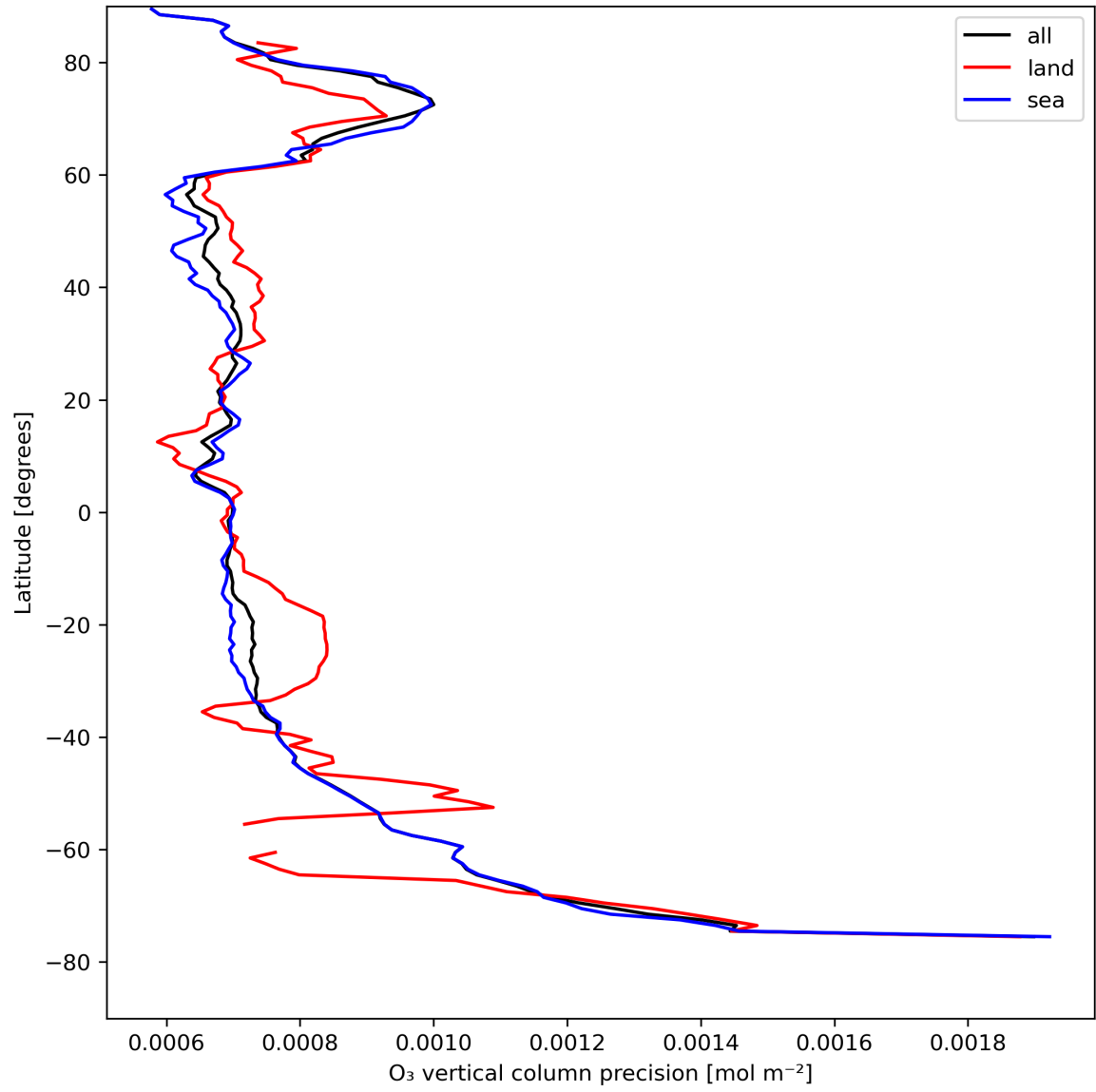
Figure 15: Zonal average of "O 3 vertical column precision" for 2024-08-16 to 2024-08-17.
