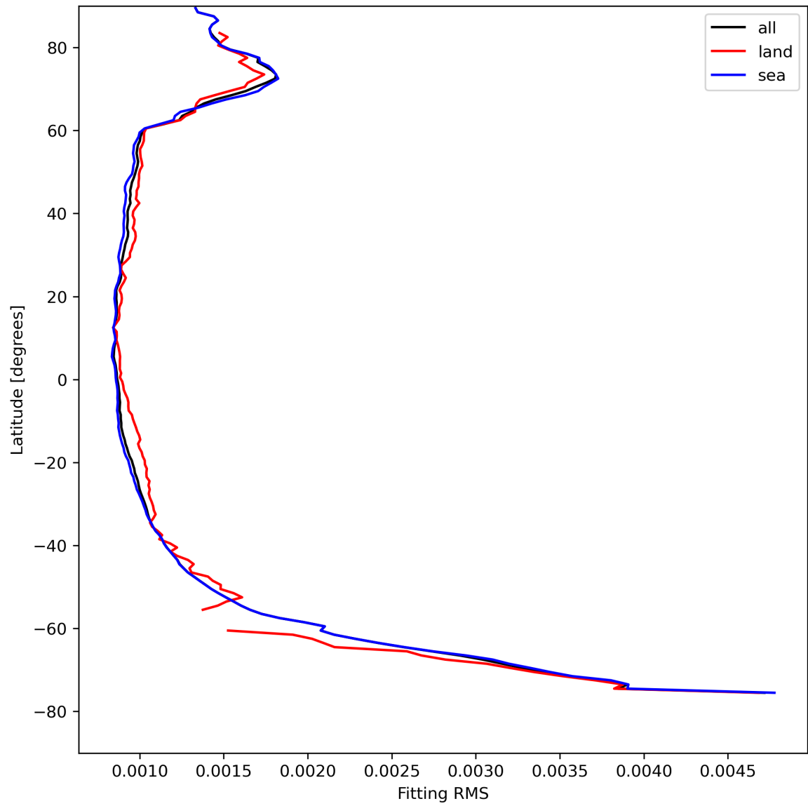
Figure 16: Zonal average of “Fitting RMS” for 2024-08-16 to 2024-08-17.
