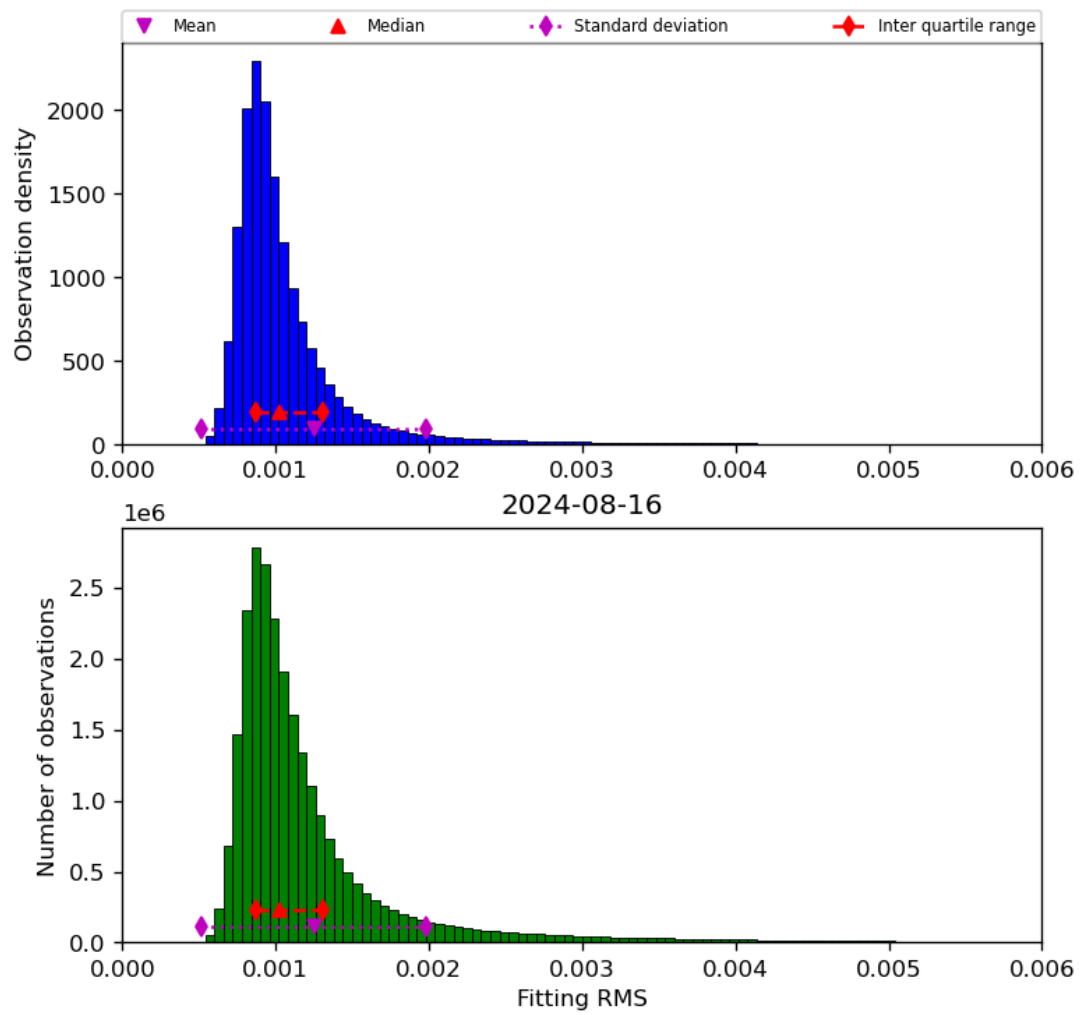
Figure 23: Histogram of “Fitting RMS” for 2024-08-16 to 2024-08-17
