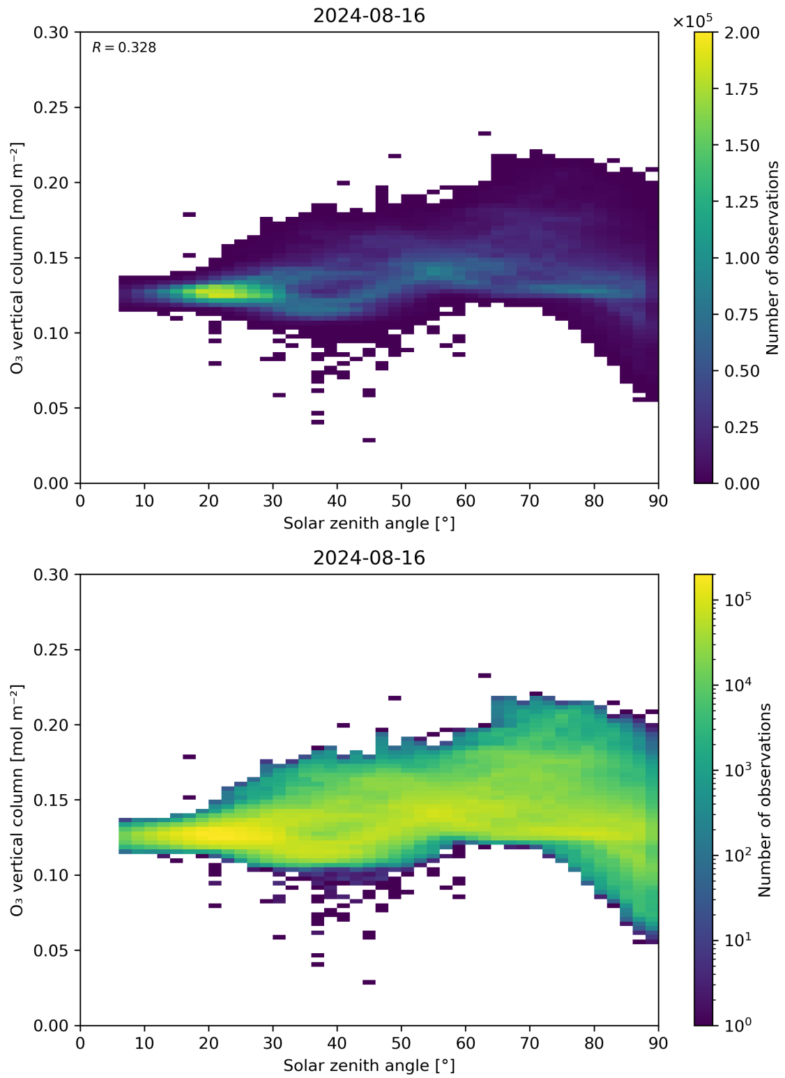
Figure 47: Scatter density plot of “Solar zenith angle” against “O 3 vertical column” for 2024-08-16 to 2024-08-17.
