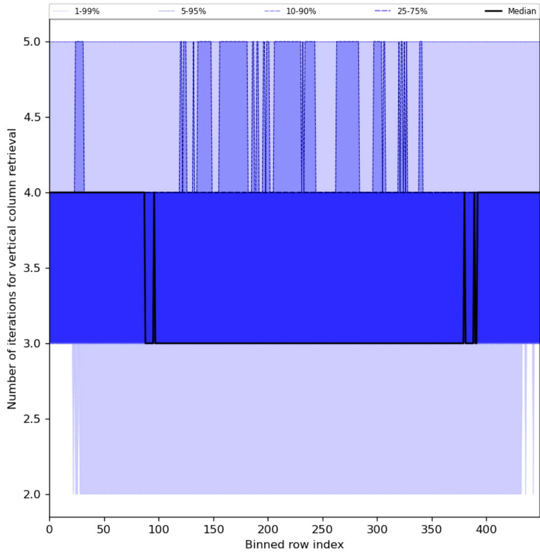
Figure 33: Along track statistics of “Number of iterations for vertical column retrieval” for 2024-08-16 to 2024-08-17
