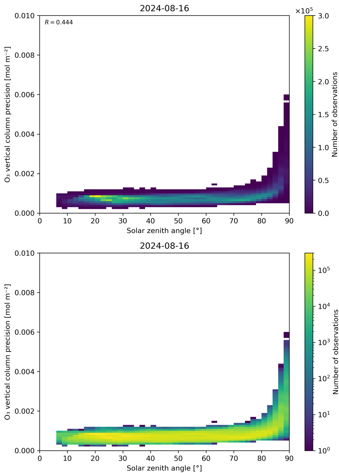
Figure 48: Scatter density plot of “Solar zenith angle” against “O 3 vertical column precision” for 2024-08-16 to 2024-08-17.
