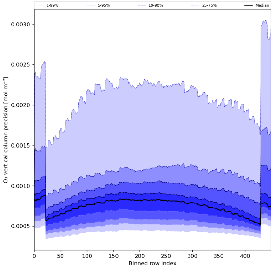
Figure 29: Along track statistics of “O 3 vertical column precision” for 2024-08-16 to 2024-08-17
