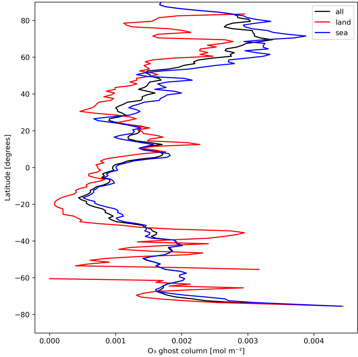
Figure 18: Zonal average of "O 3 ghost column" for 2024-08-16 to 2024-08-17.
