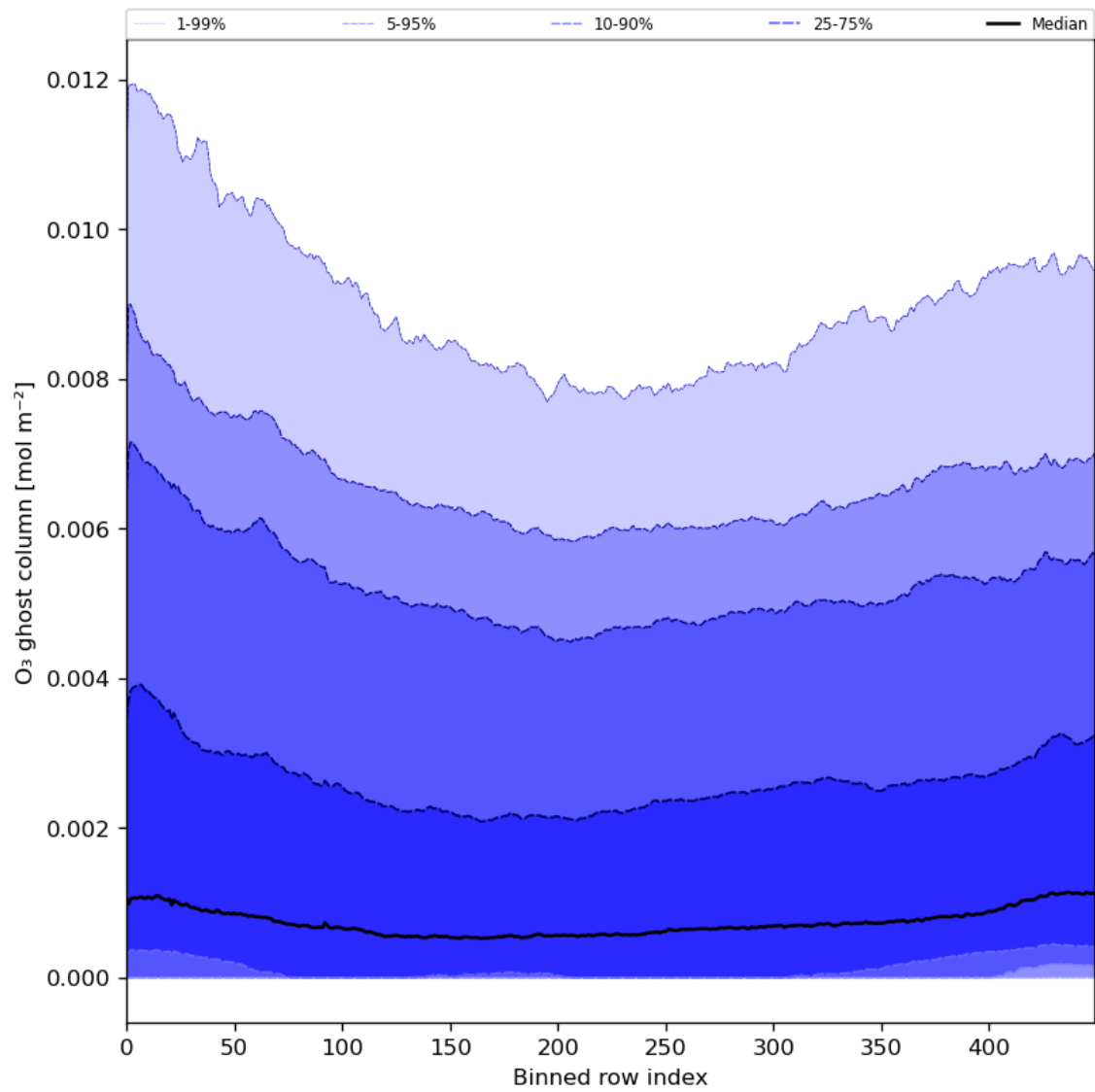
Figure 32: Along track statistics of “O 3 ghost column” for 2024-08-16 to 2024-08-17
