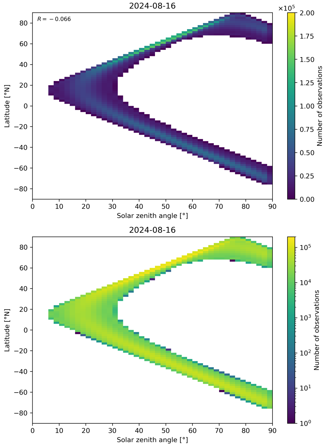
Figure 44: Scatter density plot of “Solar zenith angle” against “Latitude” for 2024-08-16 to 2024-08-17.
