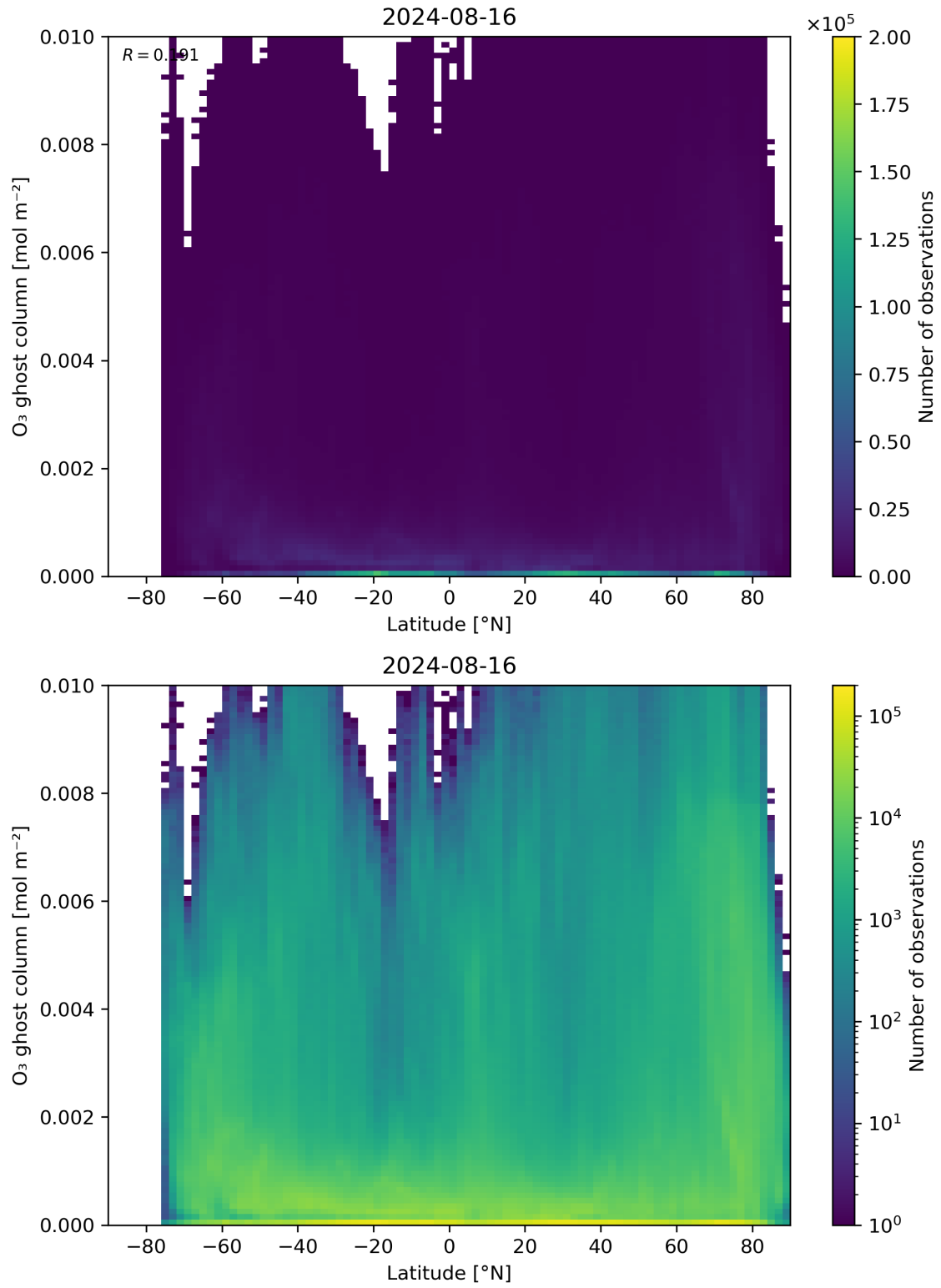
Figure 35: Scatter density plot of “Latitude” against “O 3 ghost column” for 2024-08-16 to 2024-08-17.
