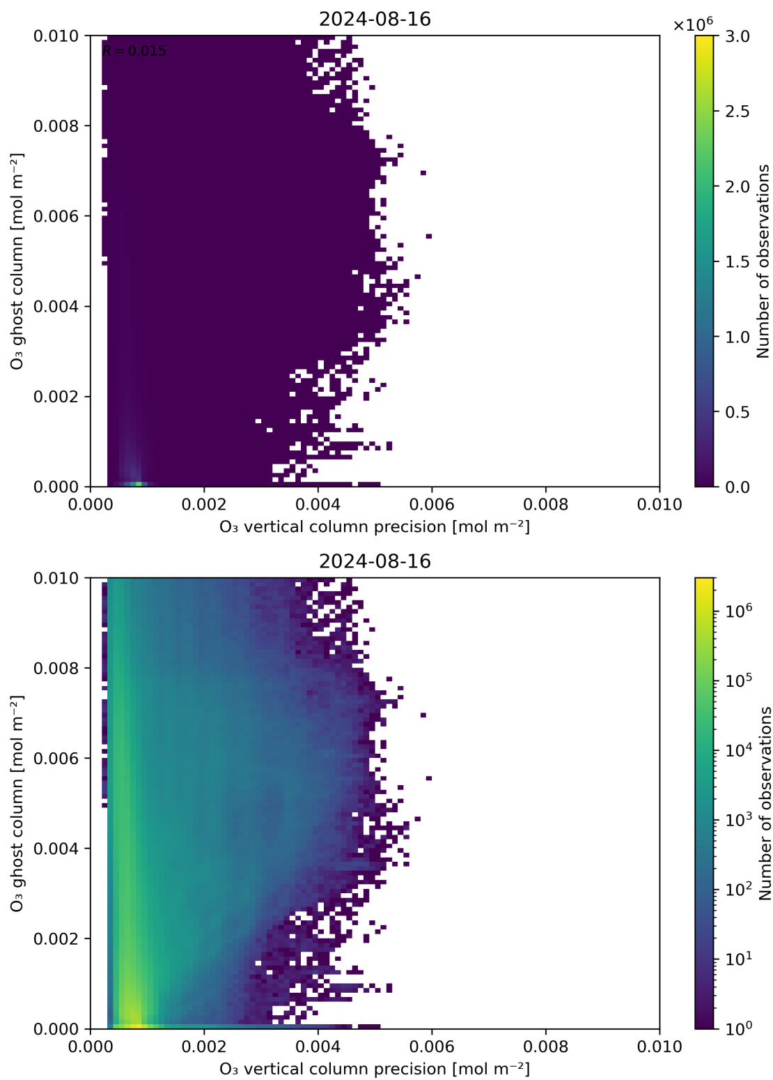
Figure 43: Scatter density plot of “ \text{O}_3 vertical column precision” against “ \text{O}_3 ghost column” for 2024-08-16 to 2024-08-17.
