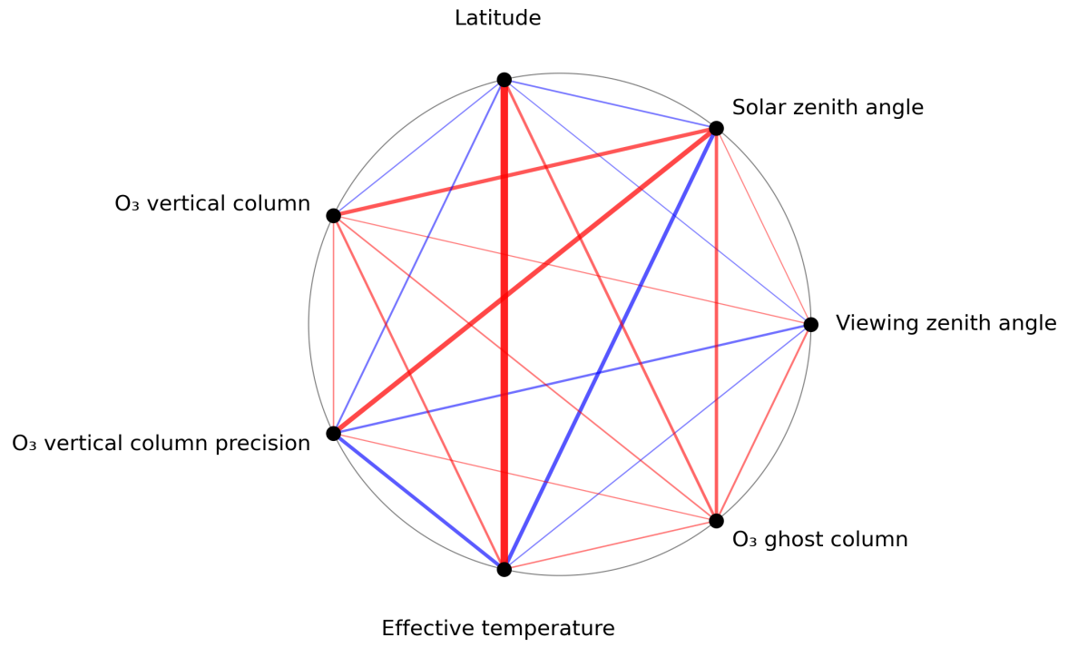
Figure 1: Map of correlation graph for 2024-08-16 to 2024-08-17.
