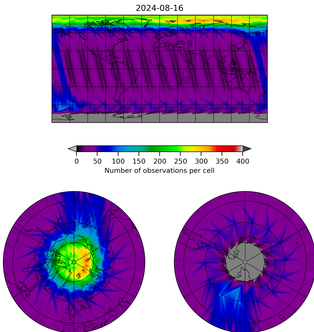
Figure 12: Map of the number of observations for 2024-08-16 to 2024-08-17
