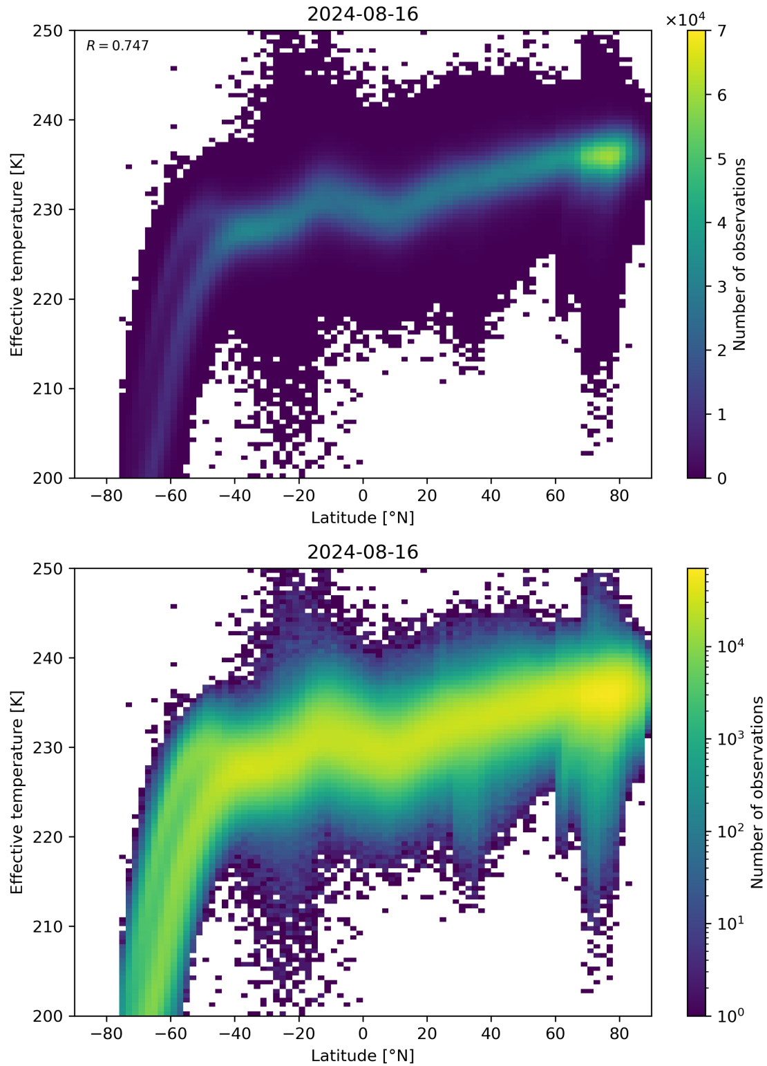
Figure 34: Scatter density plot of “Latitude” against “Effective temperature” for 2024-08-16 to 2024-08-17.
