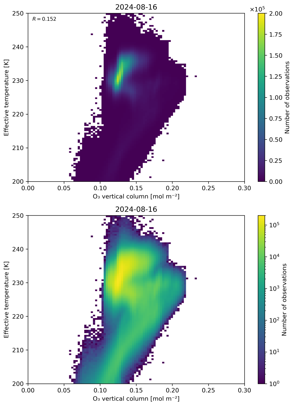
Figure 39: Scatter density plot of “O 3 vertical column” against “Effective temperature” for 2024-08-16 to 2024-08-17.
