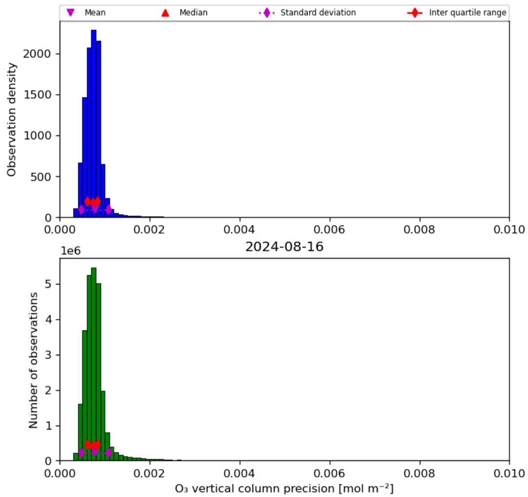
Figure 22: Histogram of “O 3 vertical column precision” for 2024-08-16 to 2024-08-17
