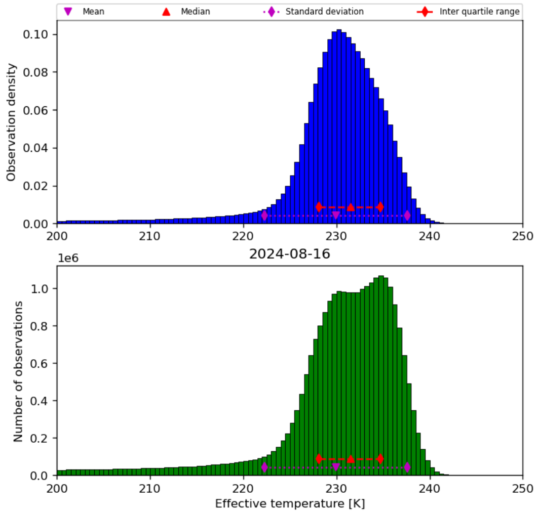
Figure 24: Histogram of “Effective temperature” for 2024-08-16 to 2024-08-17
