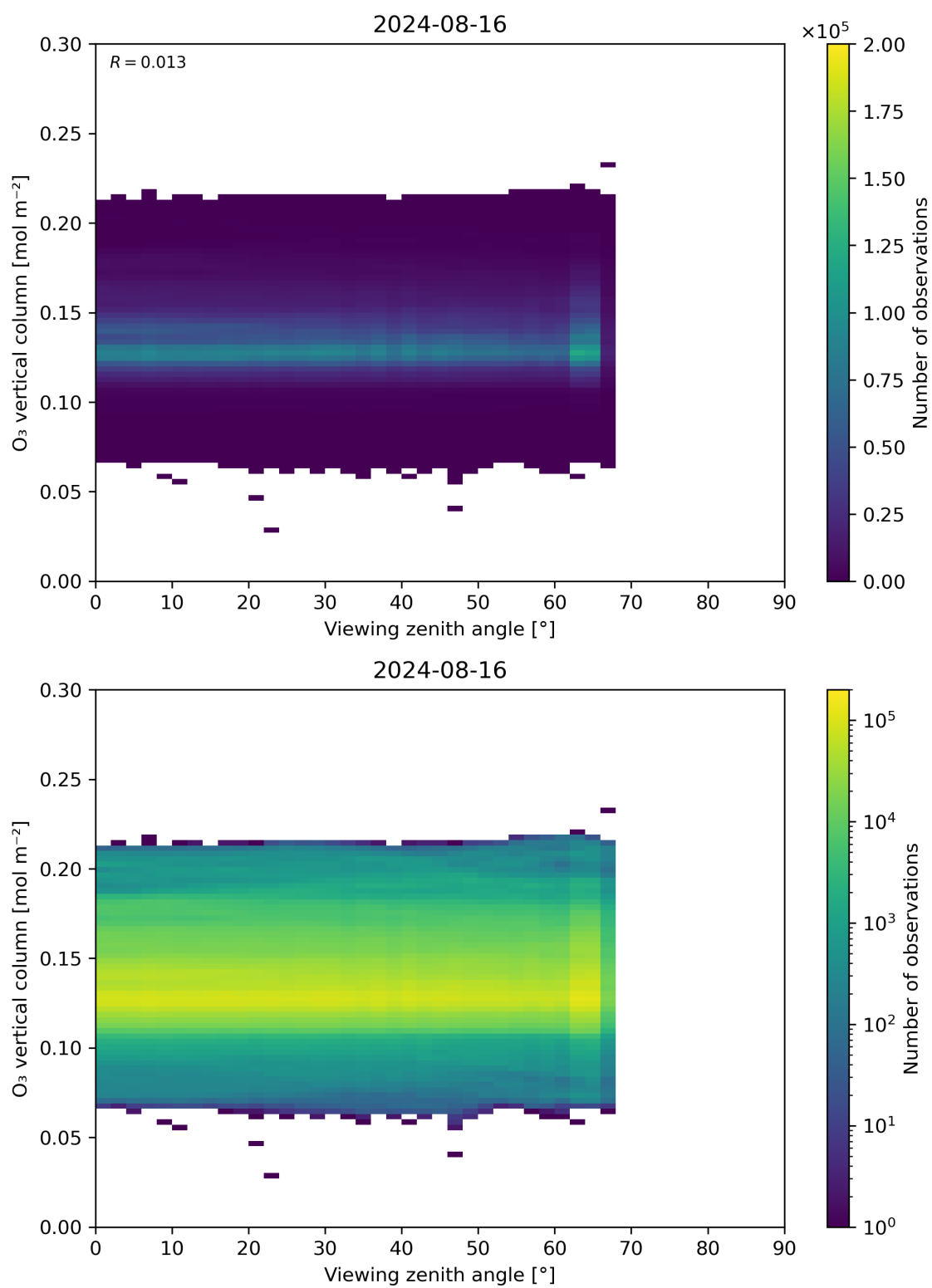
Figure 52: Scatter density plot of “Viewing zenith angle” against “O 3 vertical column” for 2024-08-16 to 2024-08-17.
