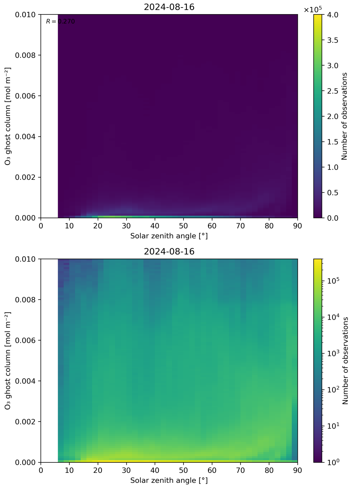
Figure 46: Scatter density plot of “Solar zenith angle” against “O 3 ghost column” for 2024-08-16 to 2024-08-17.
