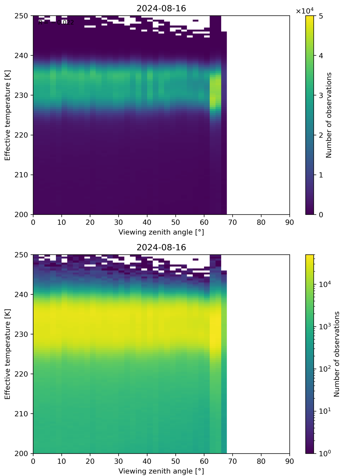
Figure 50: Scatter density plot of “Viewing zenith angle” against “Effective temperature” for 2024-08-16 to 2024-08-17.
