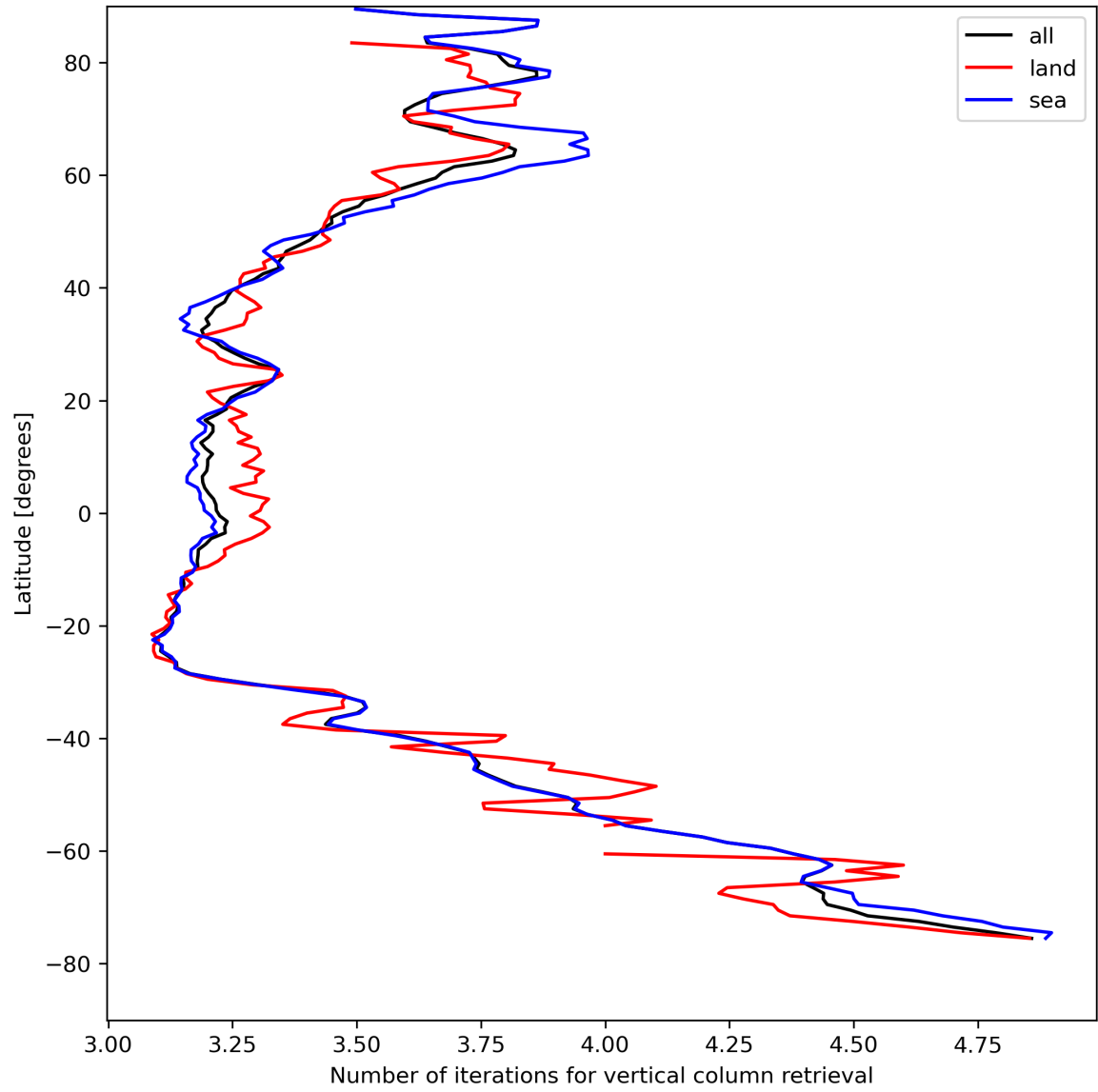
Figure 19: Zonal average of “Number of iterations for vertical column retrieval” for 2024-08-16 to 2024-08-17.
