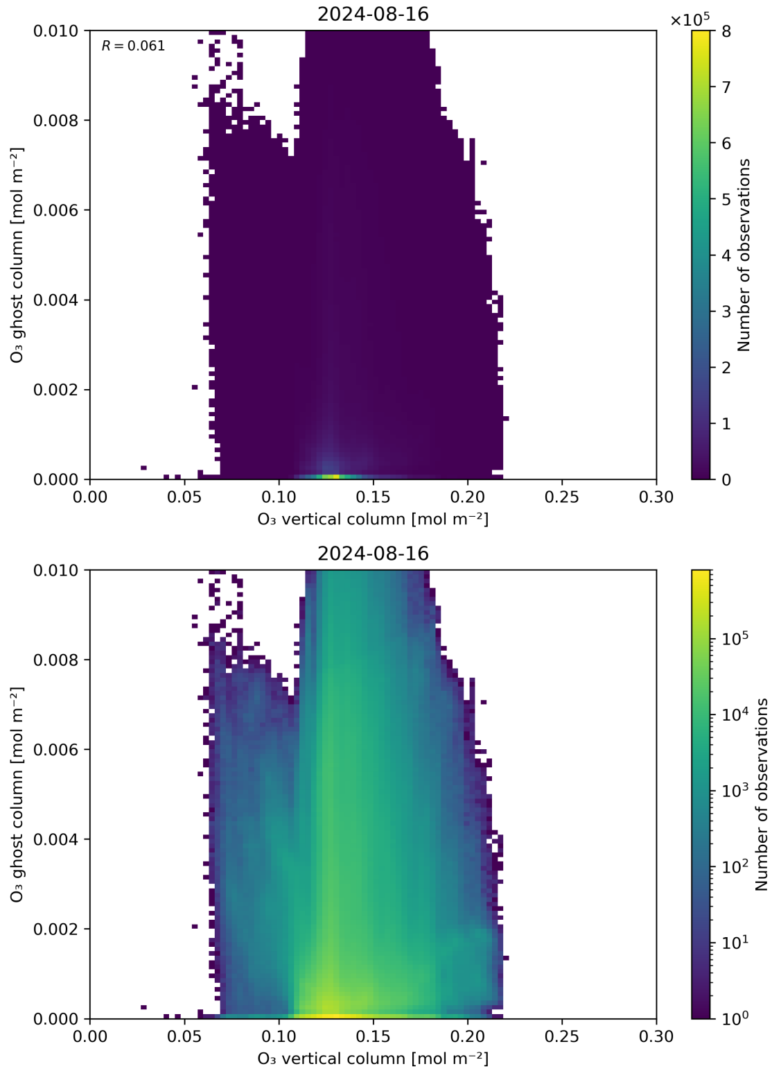
Figure 40: Scatter density plot of “O 3 vertical column” against “O 3 ghost column” for 2024-08-16 to 2024-08-17.
