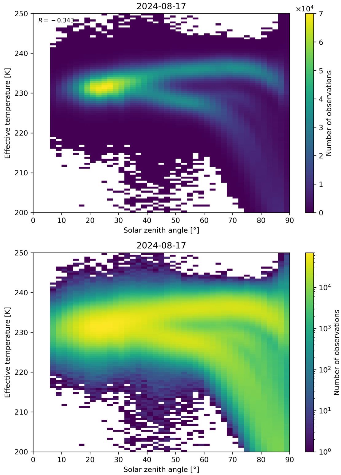
Figure 45: Scatter density plot of “Solar zenith angle” against “Effective temperature” for 2024-08-16 to 2024-08-18.
