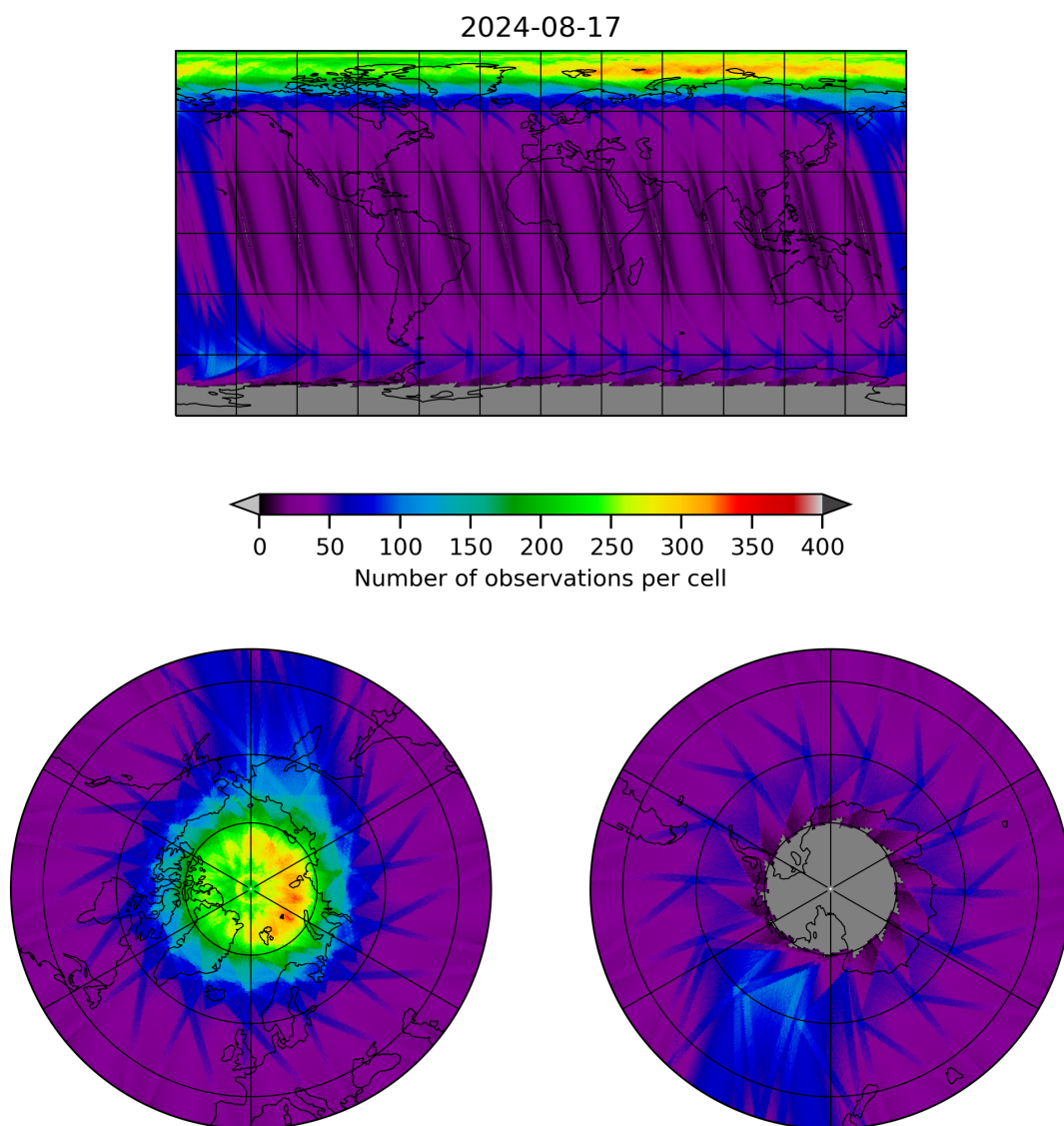
Figure 12: Map of the number of observations for 2024-08-16 to 2024-08-18
