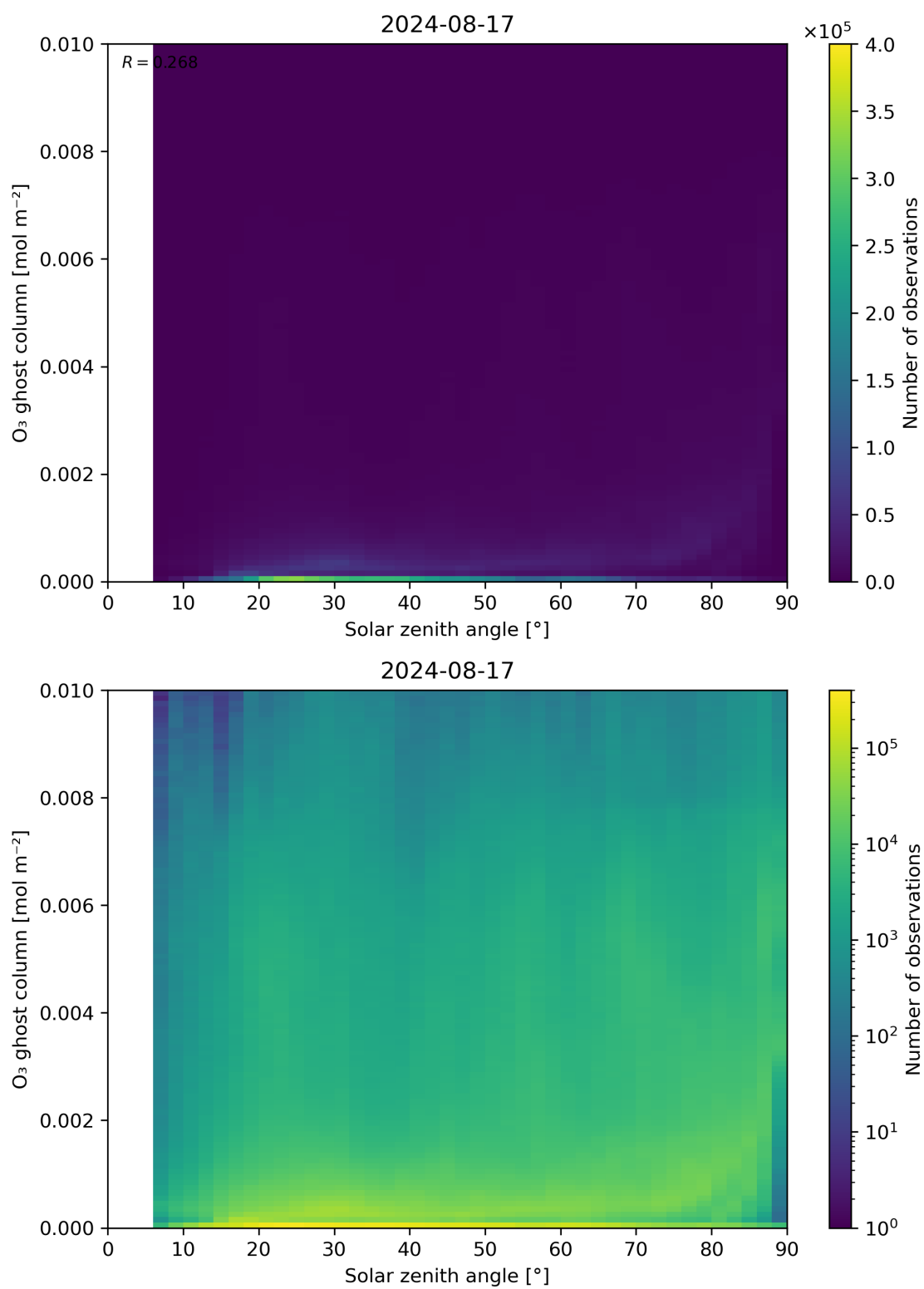
Figure 46: Scatter density plot of “Solar zenith angle” against “O 3 ghost column” for 2024-08-16 to 2024-08-18.
