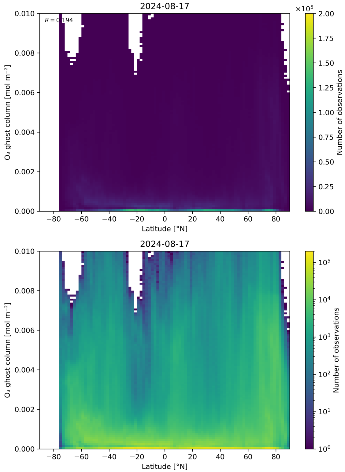
Figure 35: Scatter density plot of “Latitude” against “O 3 ghost column” for 2024-08-16 to 2024-08-18.
