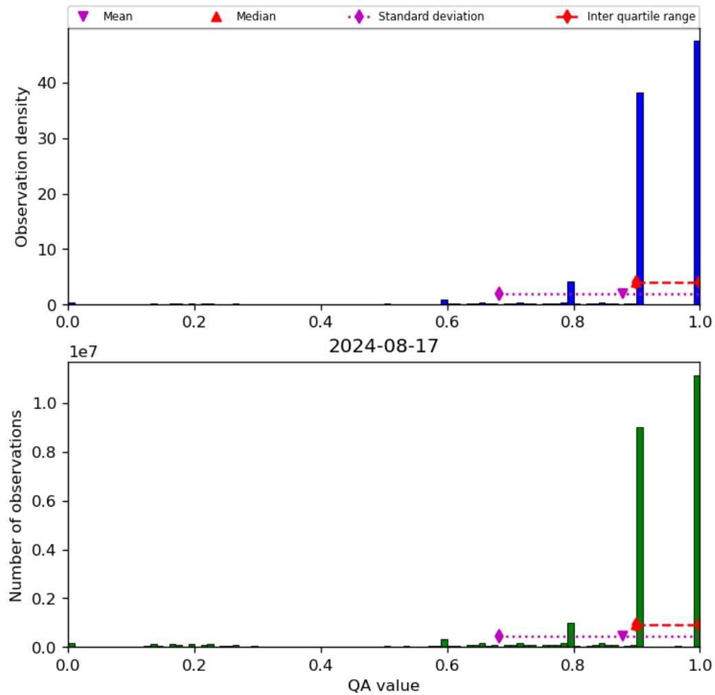
Figure 20: Histogram of “QA value” for 2024-08-16 to 2024-08-18
