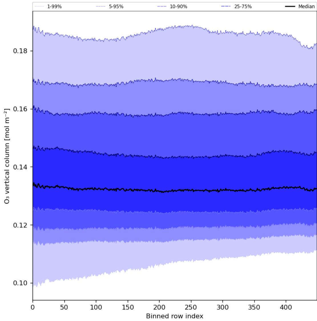
Figure 28: Along track statistics of “O 3 vertical column” for 2024-08-16 to 2024-08-18
