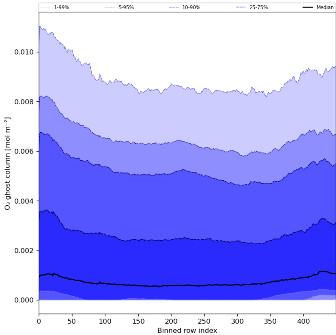
Figure 32: Along track statistics of “O 3 ghost column” for 2024-08-16 to 2024-08-18
