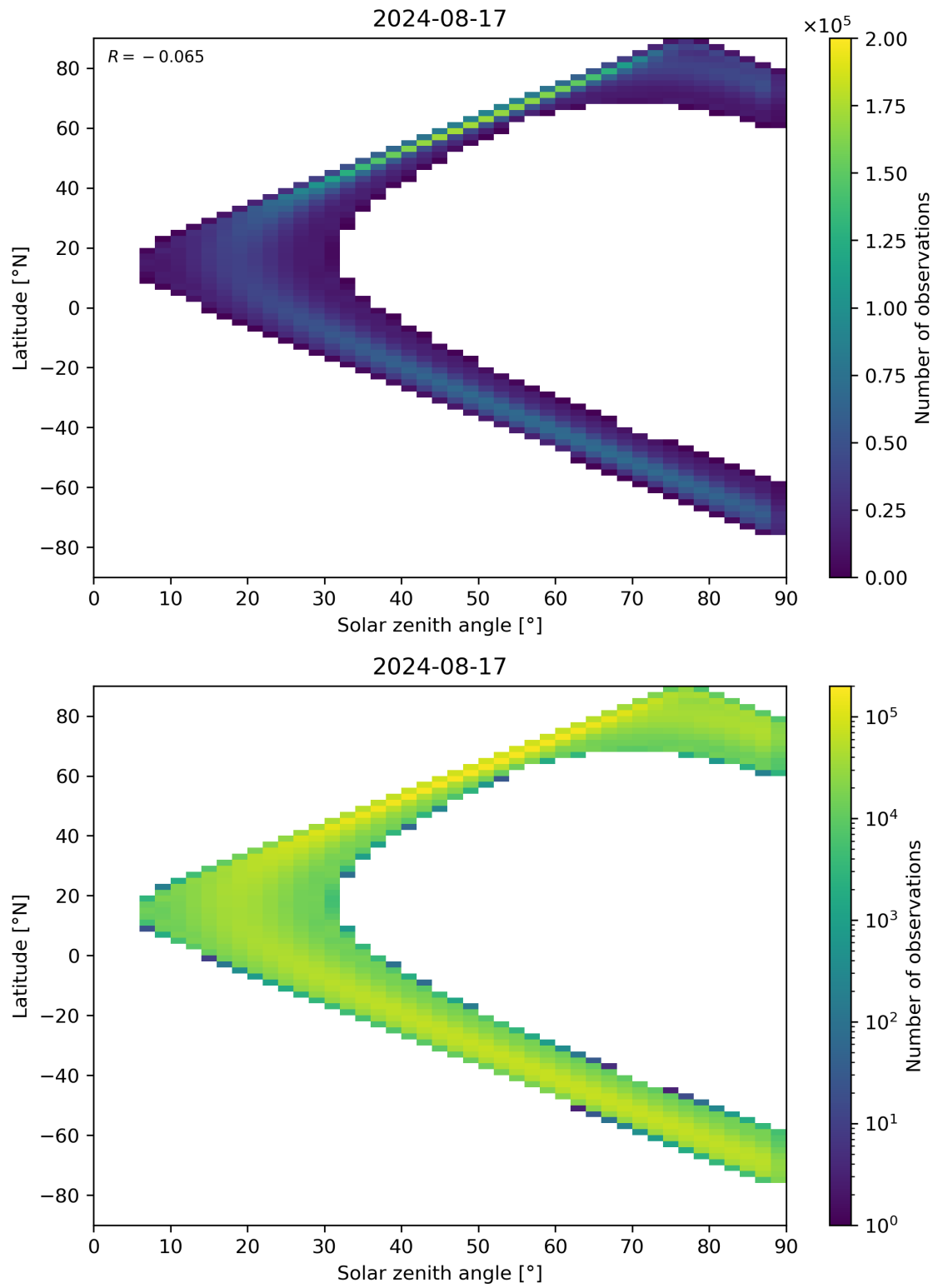
Figure 44: Scatter density plot of “Solar zenith angle” against “Latitude” for 2024-08-16 to 2024-08-18.
