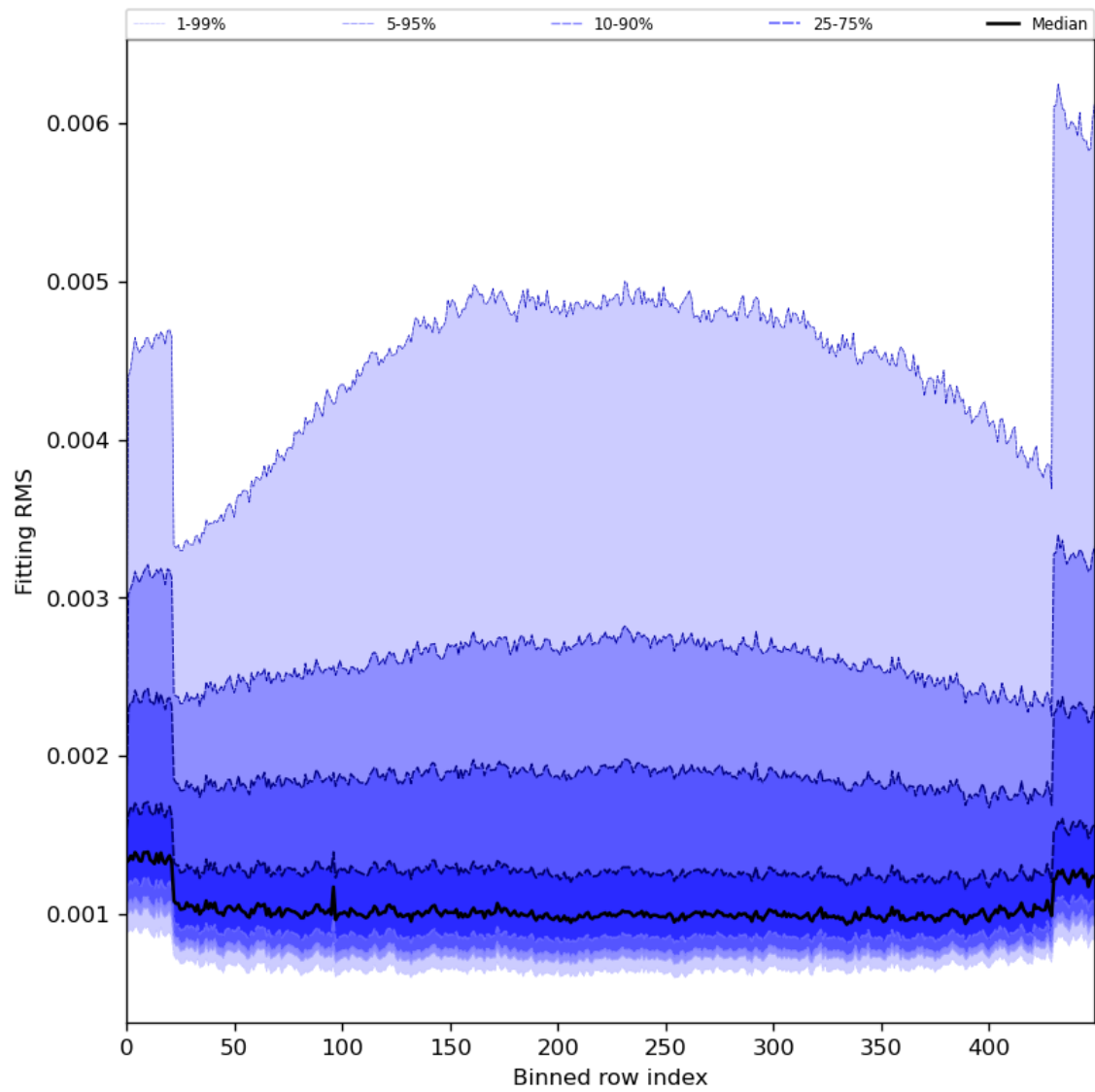
Figure 30: Along track statistics of “Fitting RMS” for 2024-08-16 to 2024-08-18
