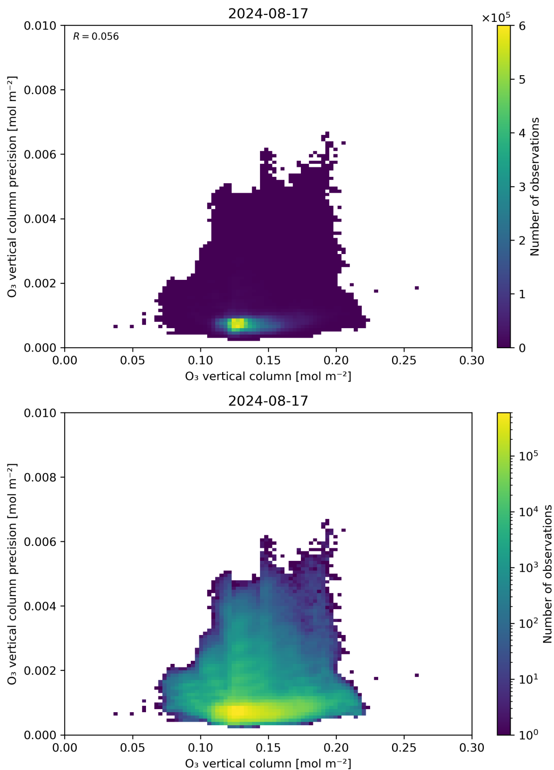
Figure 41: Scatter density plot of “O 3 vertical column” against “O 3 vertical column precision” for 2024-08-16 to 2024-08-18.
