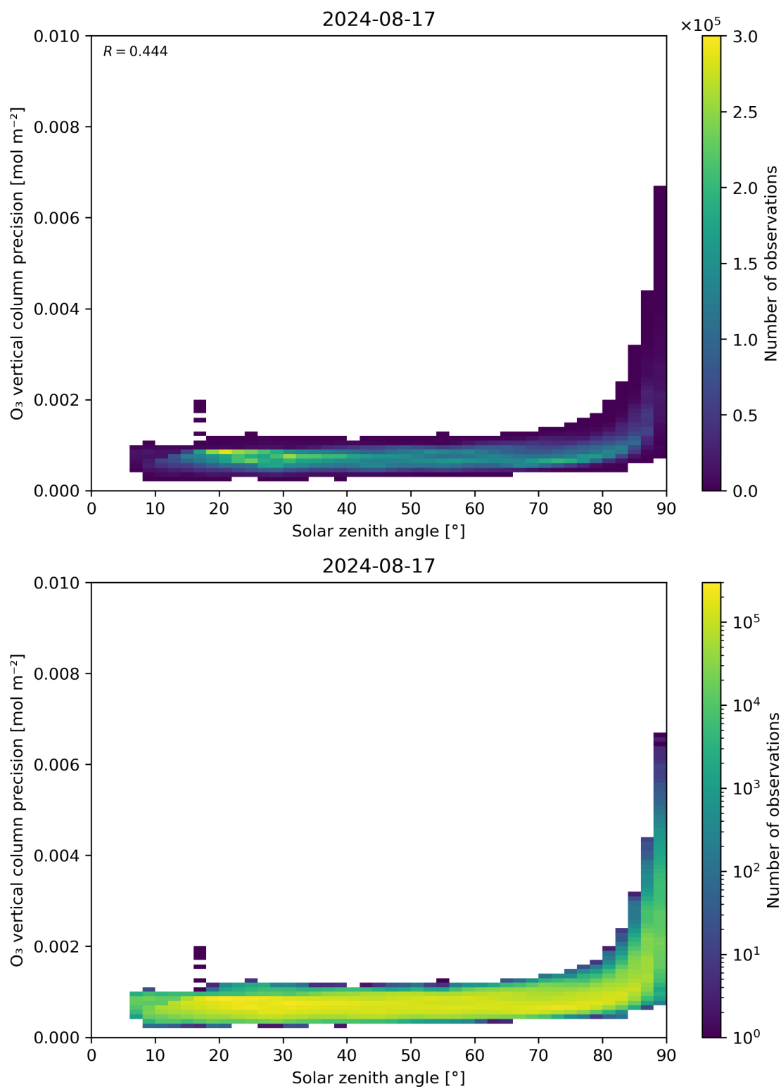
Figure 48: Scatter density plot of “Solar zenith angle” against “O 3 vertical column precision” for 2024-08-16 to 2024-08-18.
