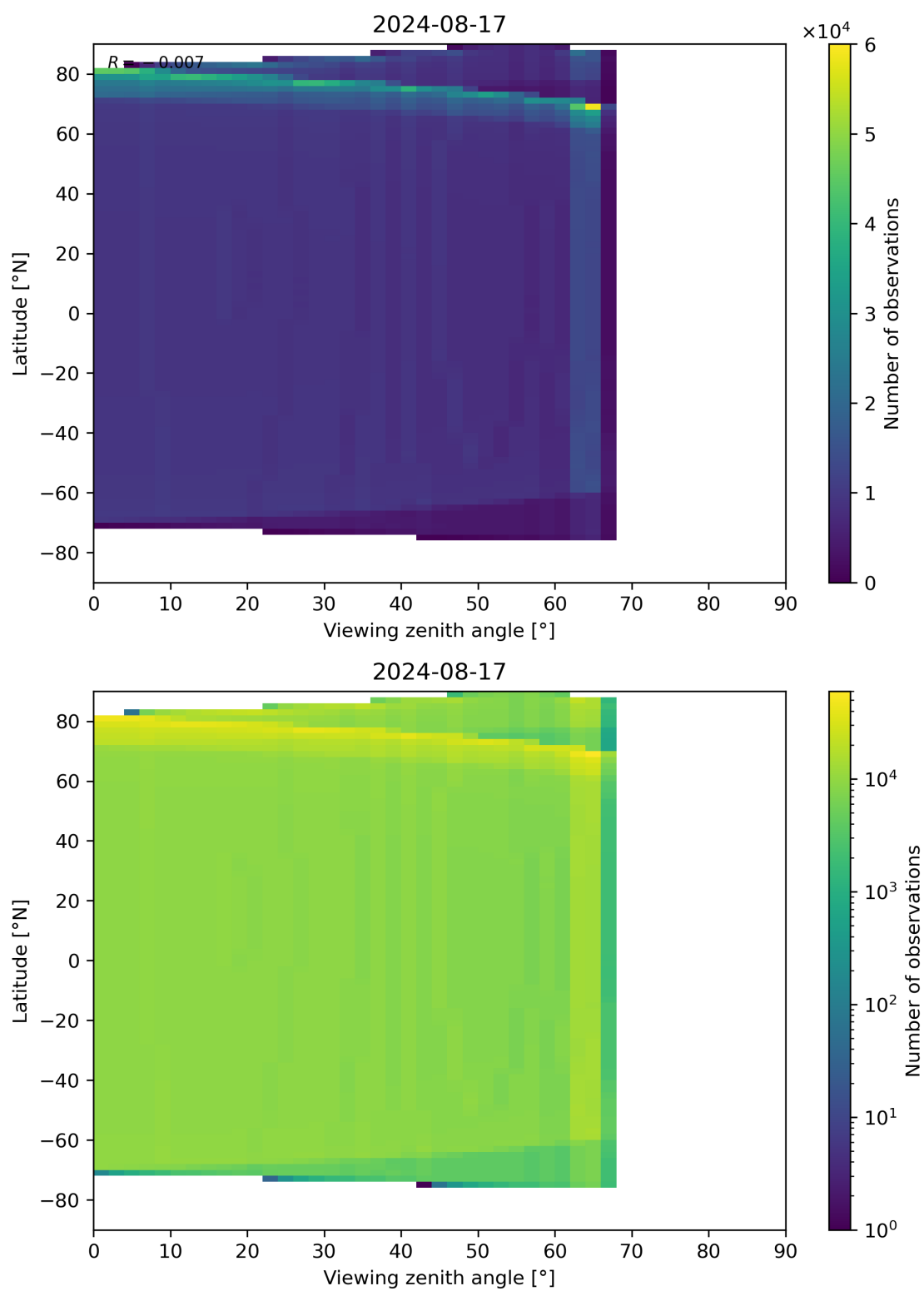
Figure 49: Scatter density plot of “Viewing zenith angle” against “Latitude” for 2024-08-16 to 2024-08-18.
