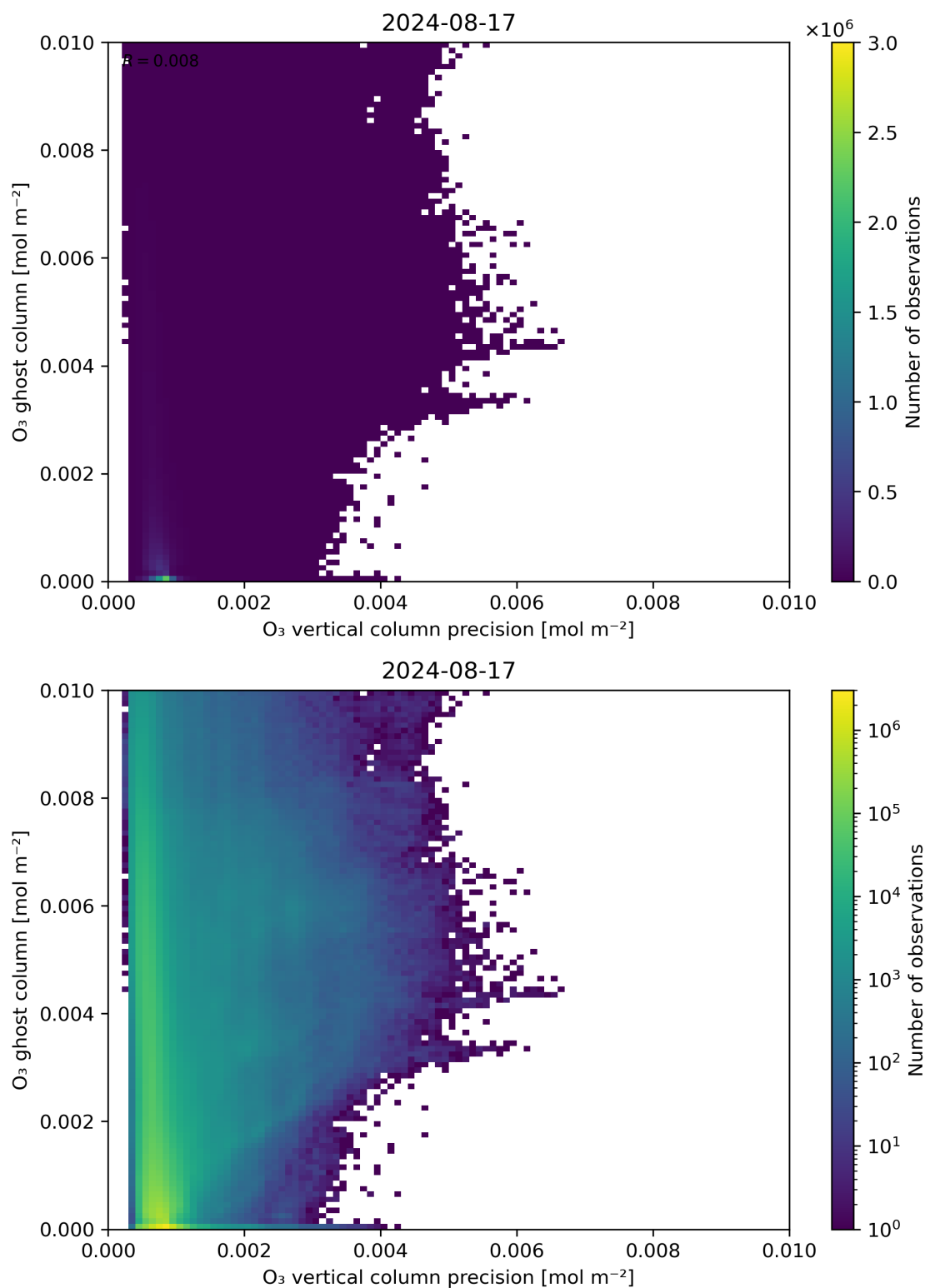
Figure 43: Scatter density plot of “O 3 vertical column precision” against “O 3 ghost column” for 2024-08-16 to 2024-08-18.
