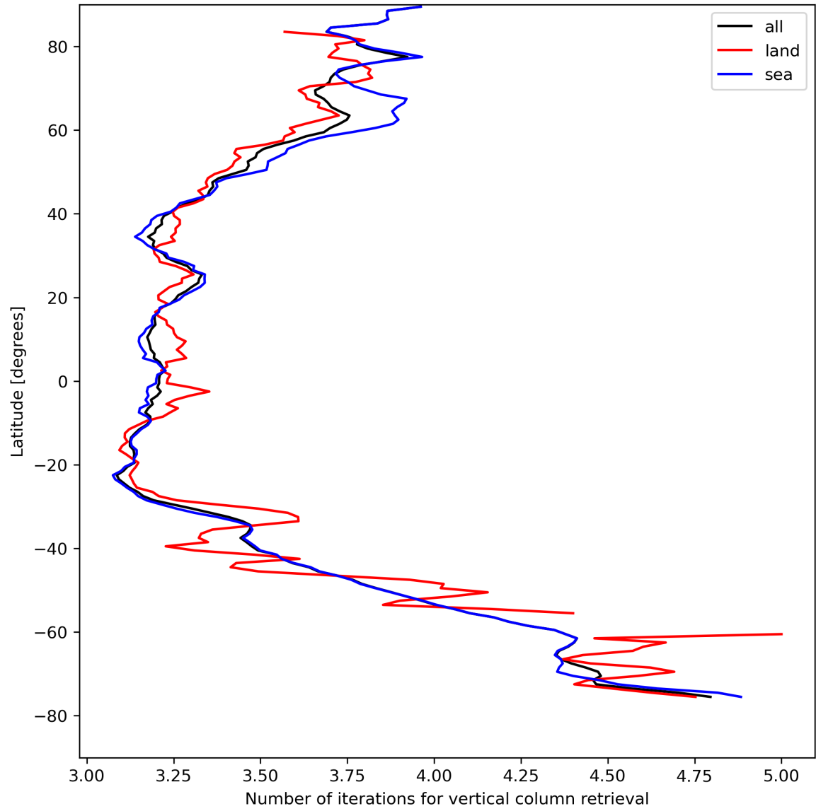
Figure 19: Zonal average of “Number of iterations for vertical column retrieval” for 2024-08-16 to 2024-08-18.
