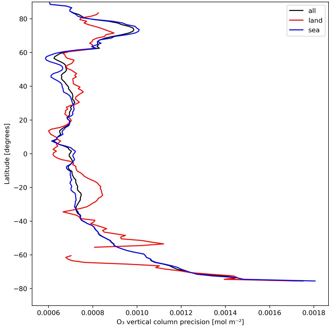
Figure 15: Zonal average of "O 3 vertical column precision" for 2024-08-16 to 2024-08-18.
