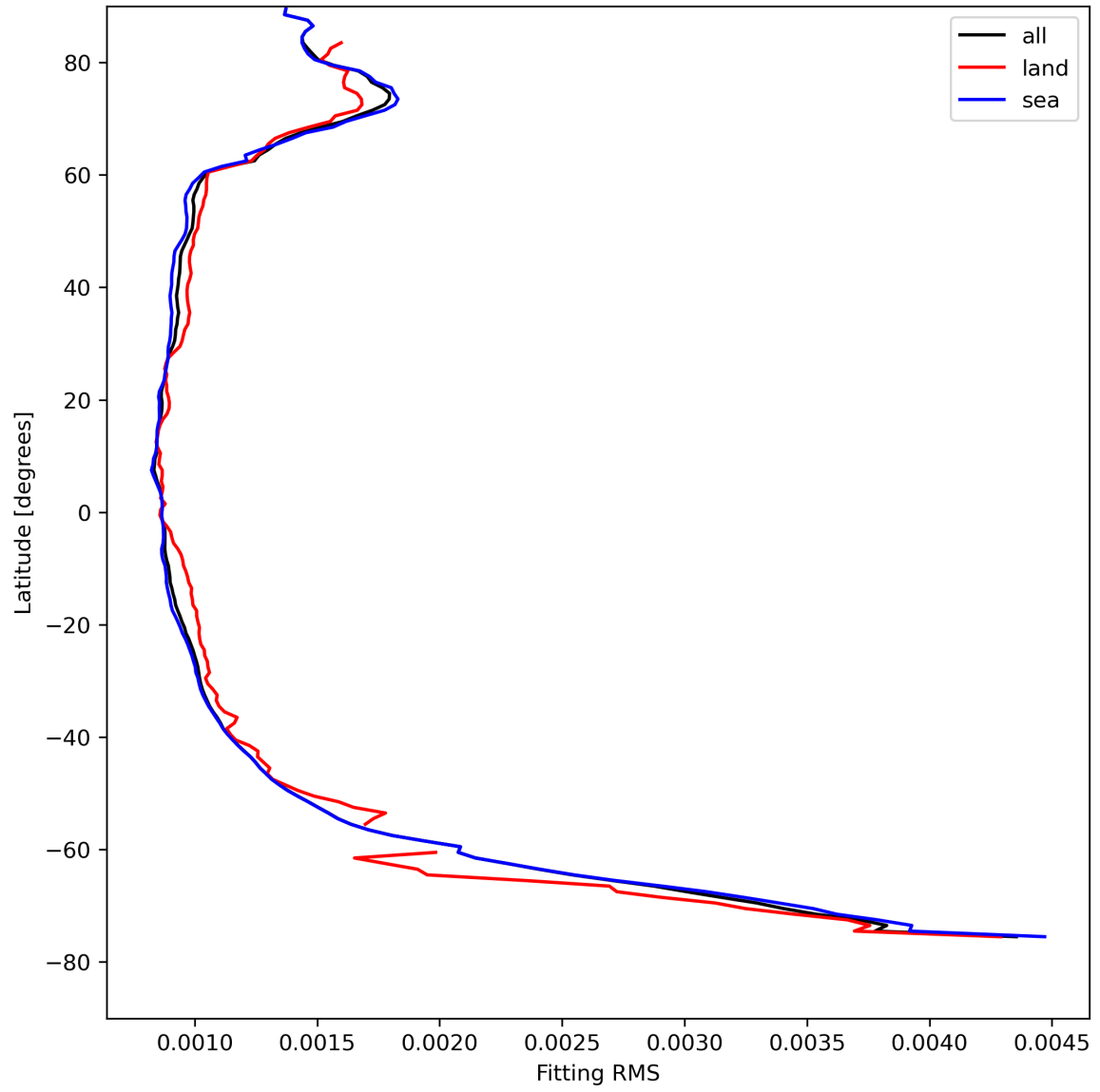
Figure 16: Zonal average of “Fitting RMS” for 2024-08-16 to 2024-08-18.
