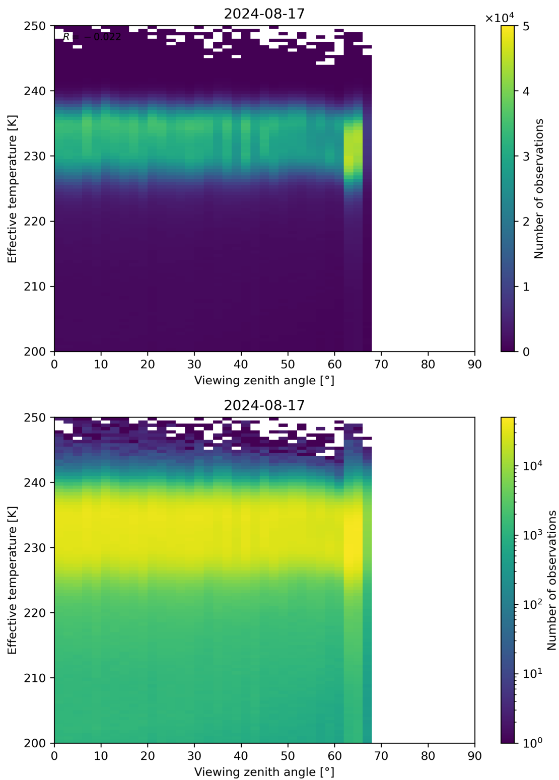
Figure 50: Scatter density plot of “Viewing zenith angle” against “Effective temperature” for 2024-08-16 to 2024-08-18.
