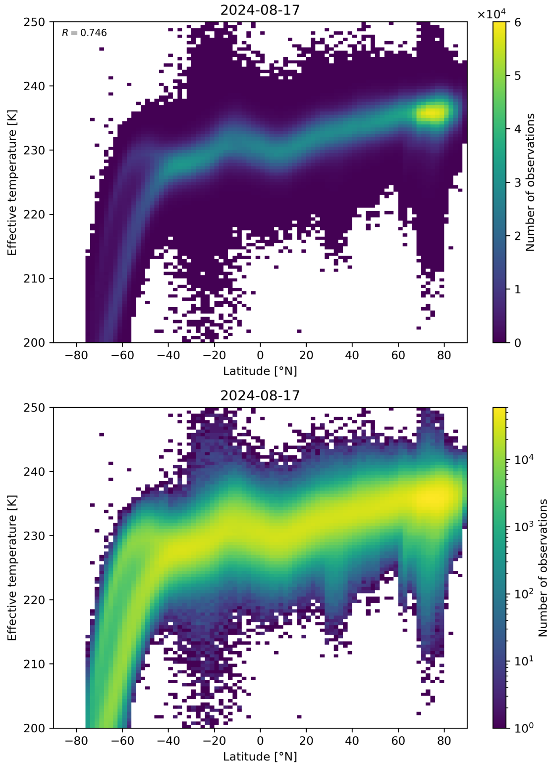
Figure 34: Scatter density plot of “Latitude” against “Effective temperature” for 2024-08-16 to 2024-08-18.
