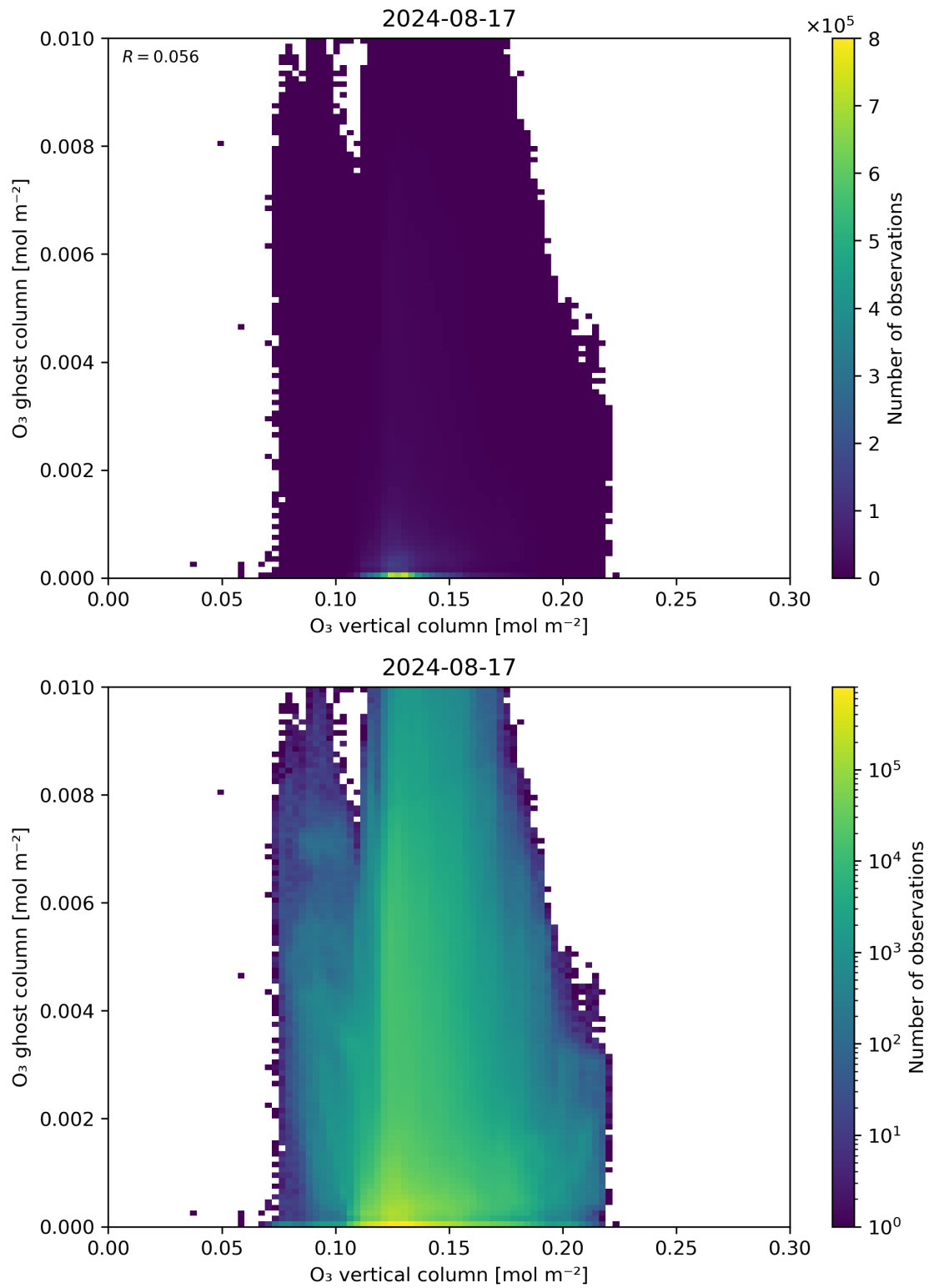
Figure 40: Scatter density plot of “O 3 vertical column” against “O 3 ghost column” for 2024-08-16 to 2024-08-18.
