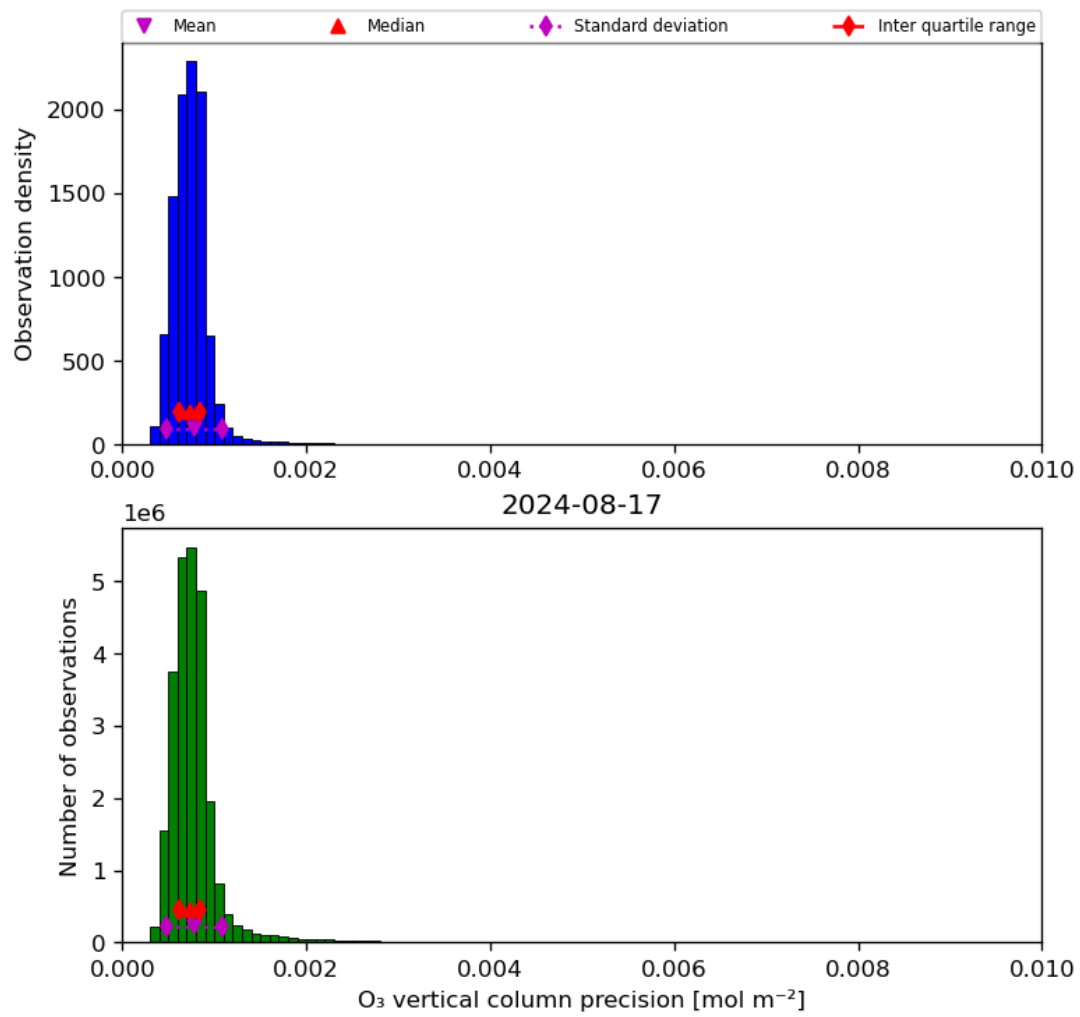
Figure 22: Histogram of “O 3 vertical column precision” for 2024-08-16 to 2024-08-18
