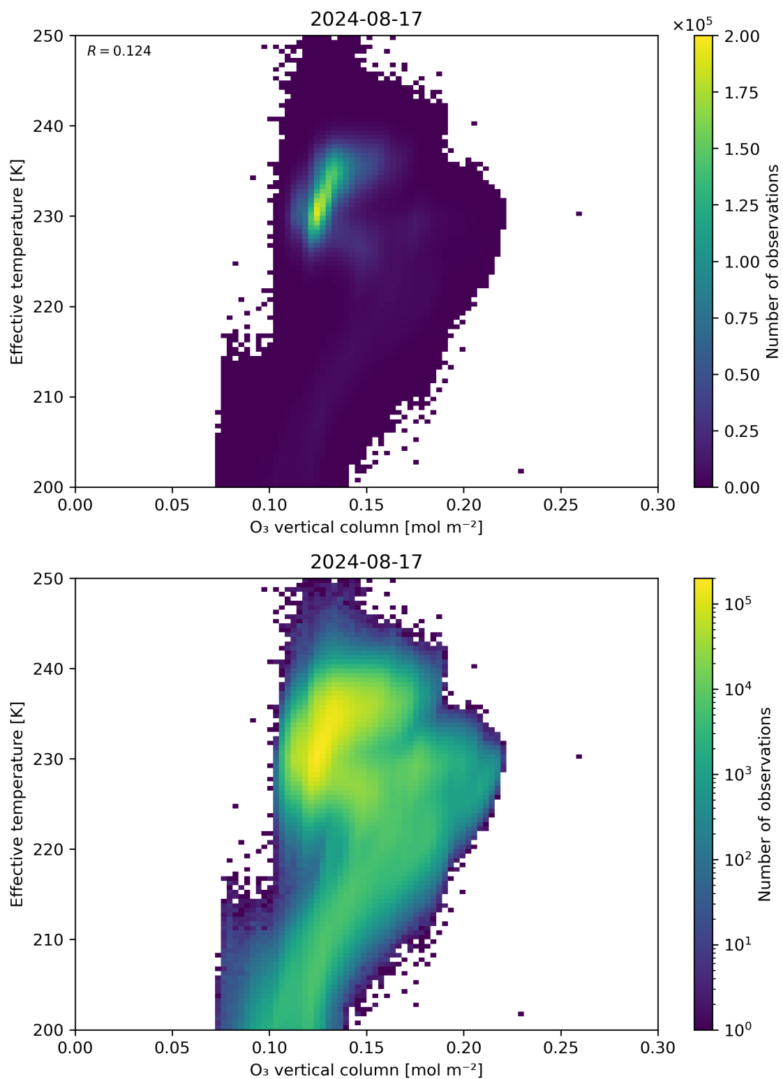
Figure 39: Scatter density plot of “O 3 vertical column” against “Effective temperature” for 2024-08-16 to 2024-08-18.
