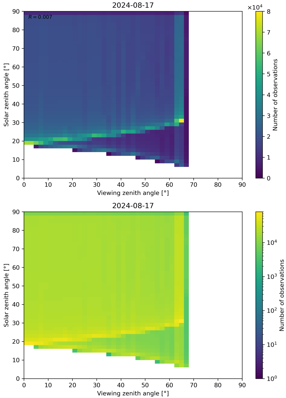
Figure 54: Scatter density plot of “Viewing zenith angle” against “Solar zenith angle” for 2024-08-16 to 2024-08-18.
