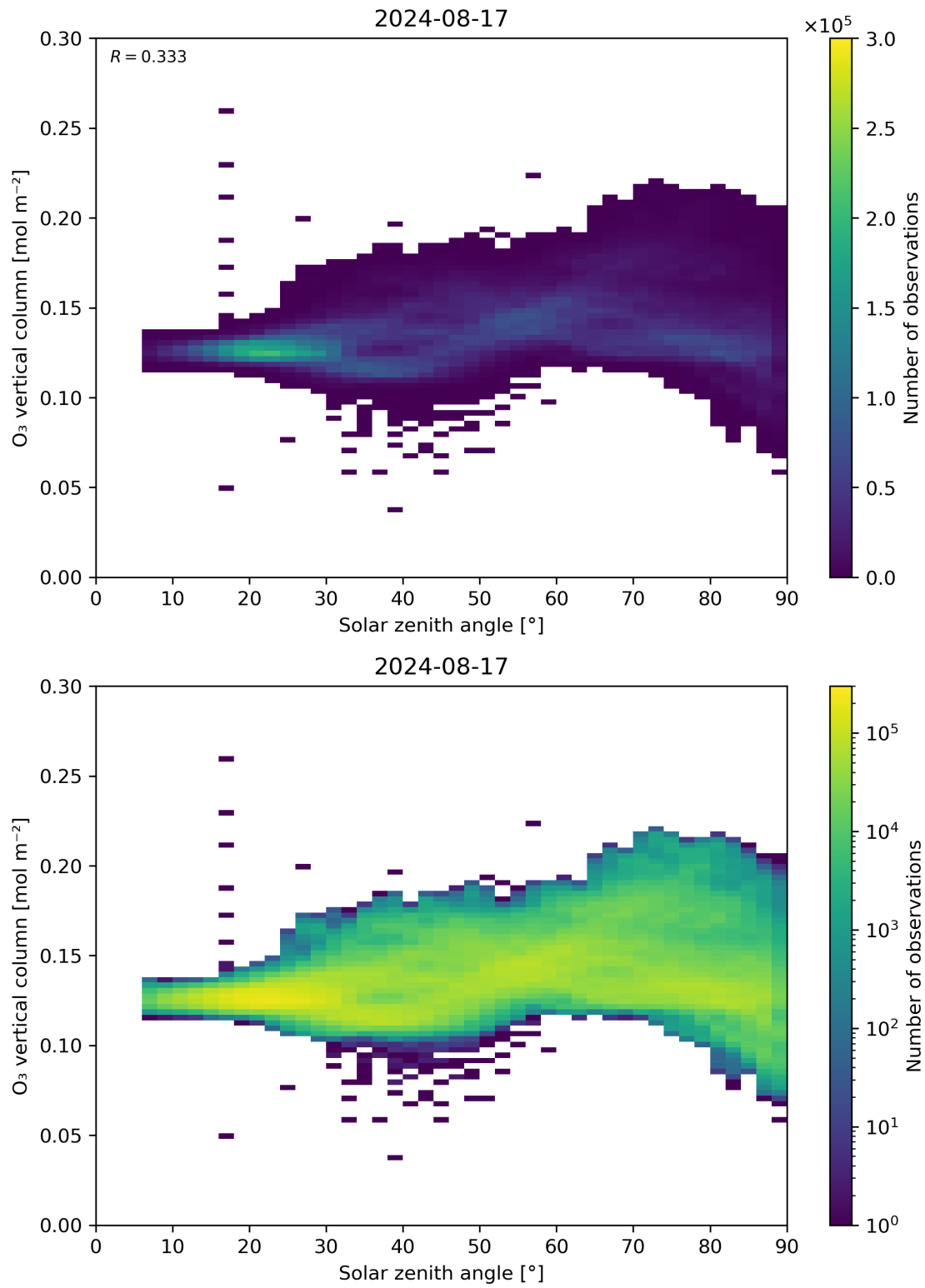
Figure 47: Scatter density plot of “Solar zenith angle” against “O 3 vertical column” for 2024-08-16 to 2024-08-18.
