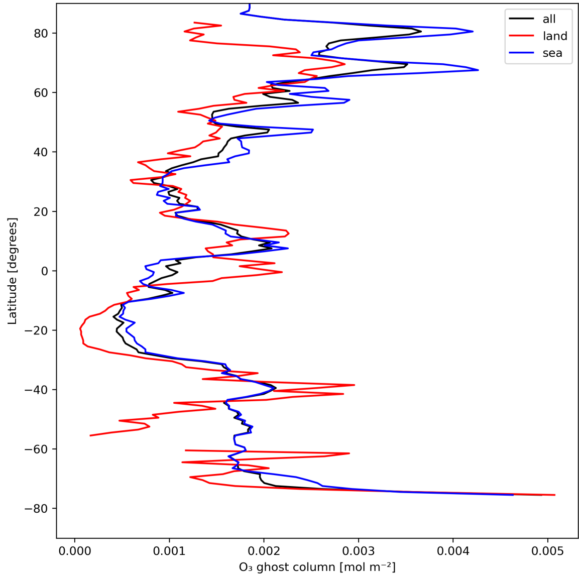
Figure 18: Zonal average of "O 3 ghost column" for 2024-08-16 to 2024-08-18.
