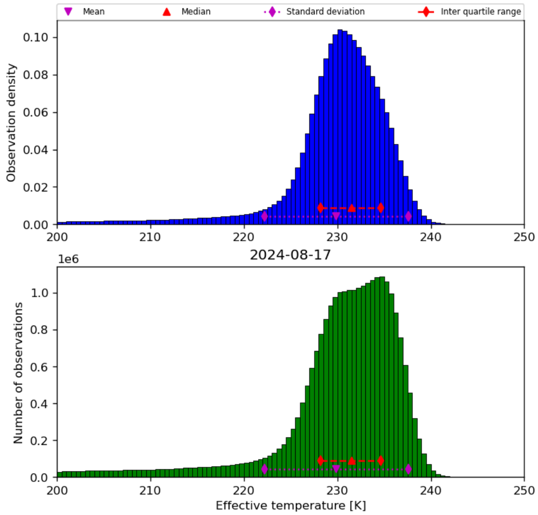
Figure 24: Histogram of “Effective temperature” for 2024-08-16 to 2024-08-18
