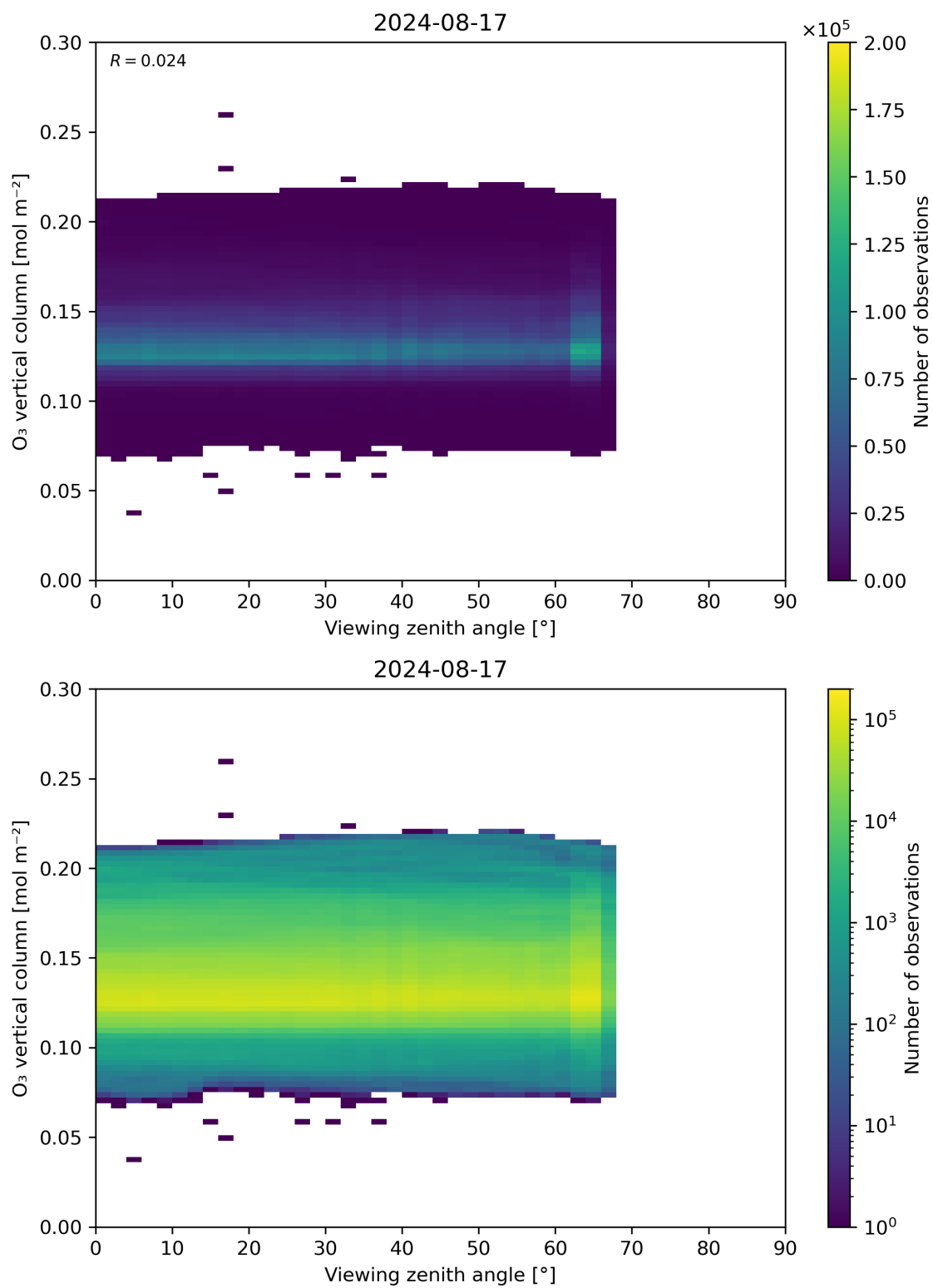
Figure 52: Scatter density plot of “Viewing zenith angle” against “O 3 vertical column” for 2024-08-16 to 2024-08-18.
