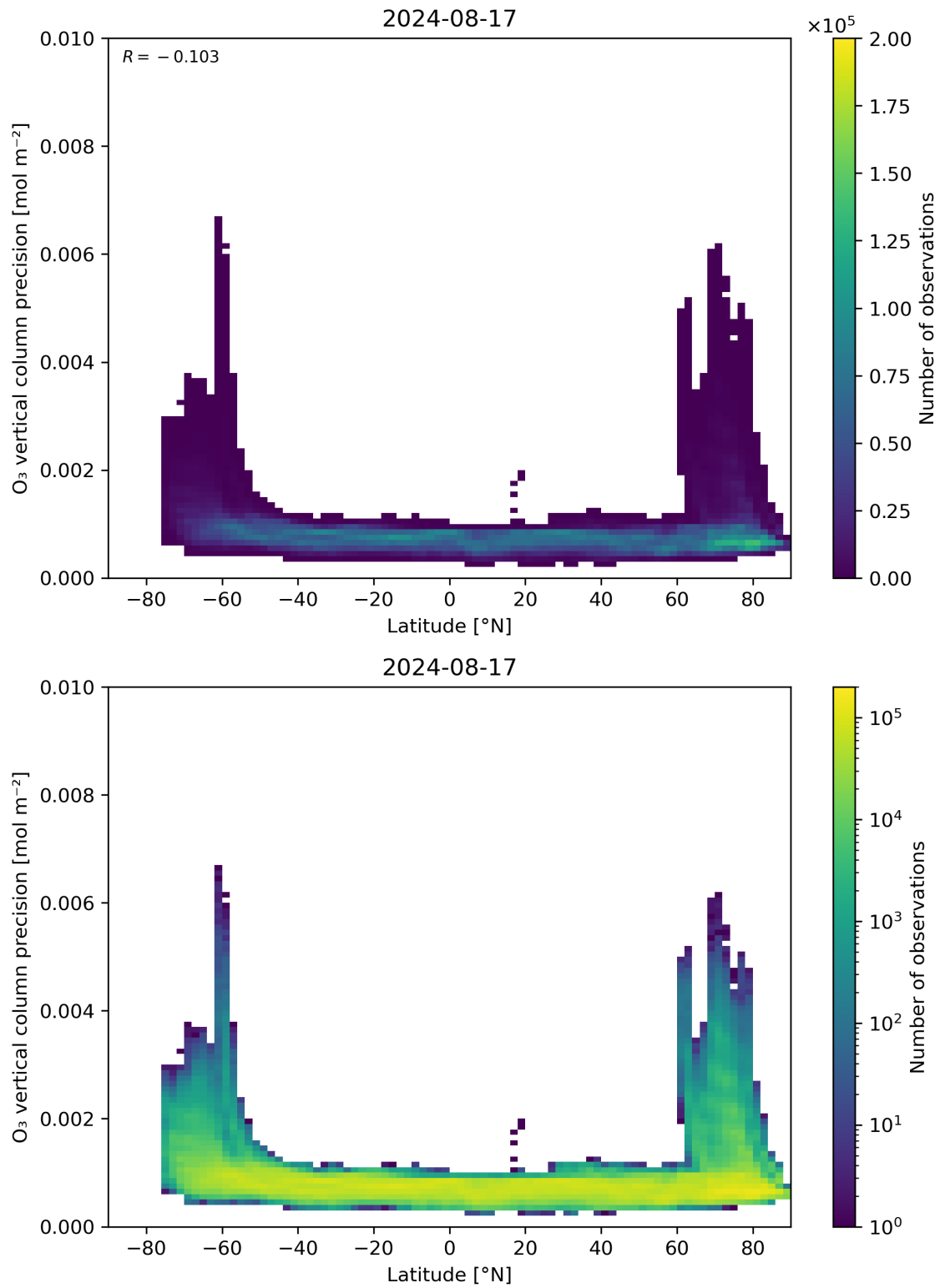
Figure 37: Scatter density plot of “Latitude” against “O 3 vertical column precision” for 2024-08-16 to 2024-08-18.
