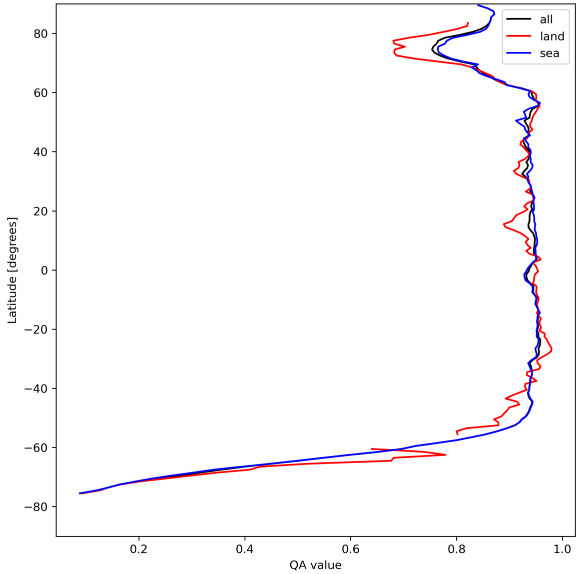
Figure 13: Zonal average of “QA value” for 2024-08-16 to 2024-08-18.
