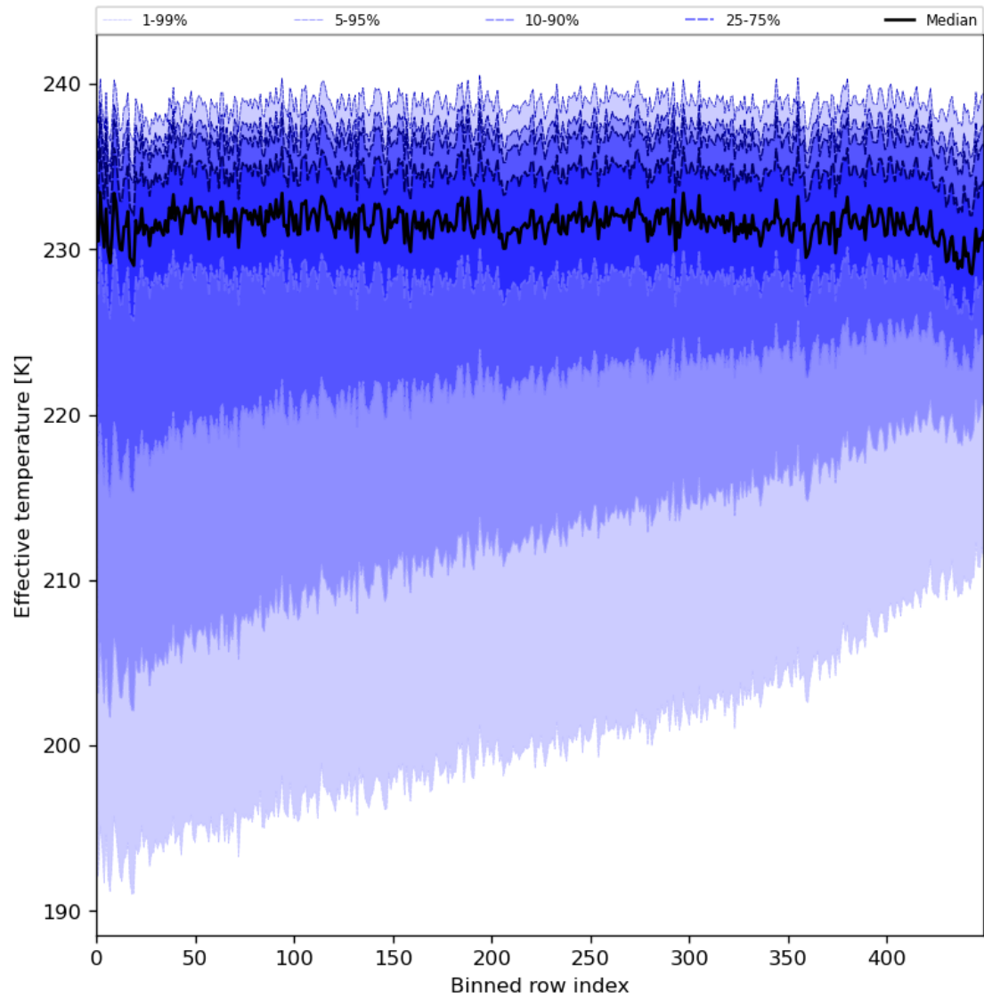
Figure 31: Along track statistics of “Effective temperature” for 2024-08-16 to 2024-08-18
