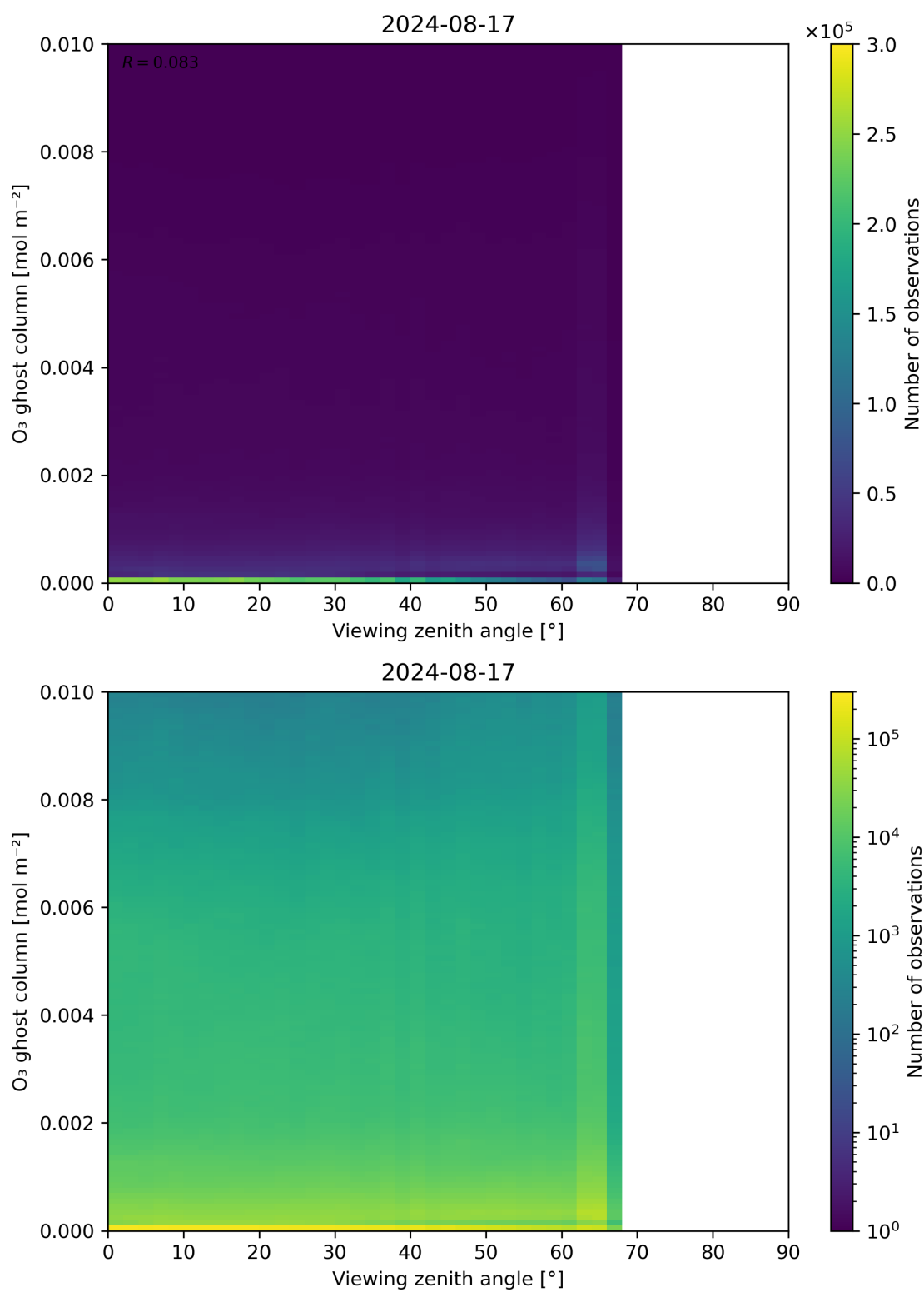
Figure 51: Scatter density plot of “Viewing zenith angle” against “O 3 ghost column” for 2024-08-16 to 2024-08-18.
