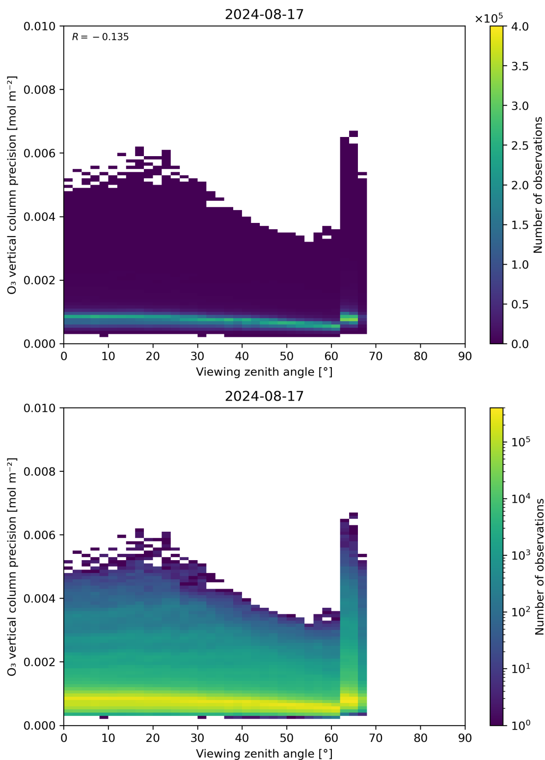
Figure 53: Scatter density plot of “Viewing zenith angle” against “O 3 vertical column precision” for 2024-08-16 to 2024-08-18.
