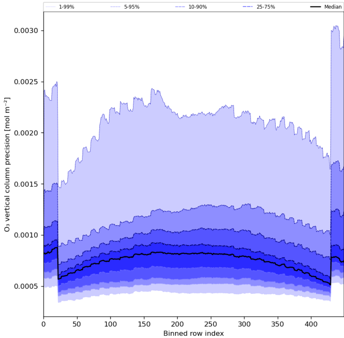
Figure 29: Along track statistics of “O 3 vertical column precision” for 2024-08-16 to 2024-08-18
