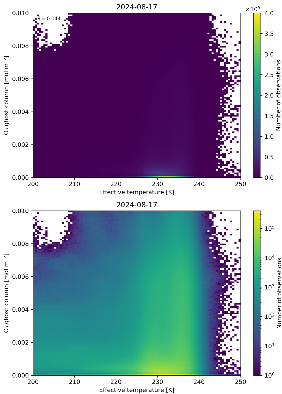
Figure 38: Scatter density plot of “Effective temperature” against “O 3 ghost column” for 2024-08-16 to 2024-08-18.
