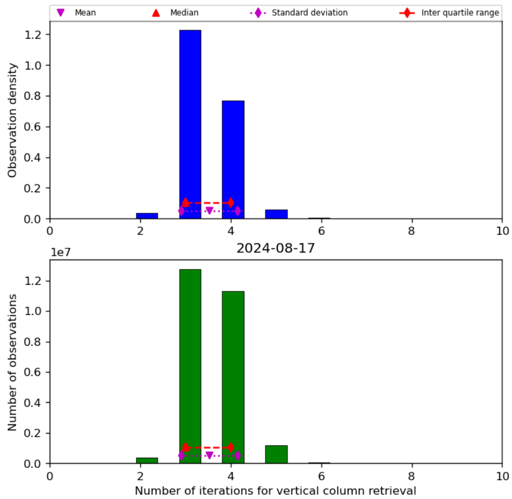
Figure 26: Histogram of “Number of iterations for vertical column retrieval” for 2024-08-16 to 2024-08-18
