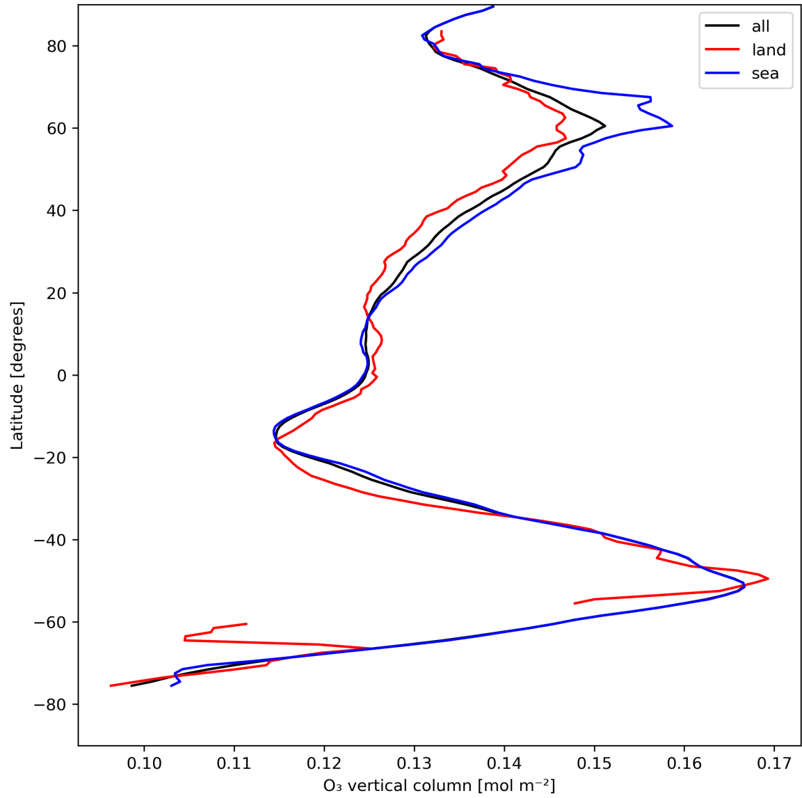
Figure 14: Zonal average of “O 3 vertical column” for 2024-08-16 to 2024-08-18.
