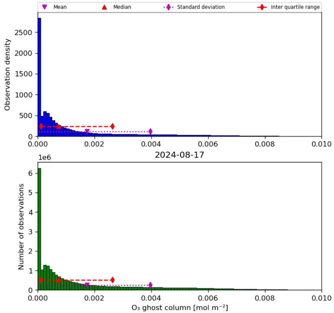
Figure 25: Histogram of “O 3 ghost column” for 2024-08-16 to 2024-08-18
