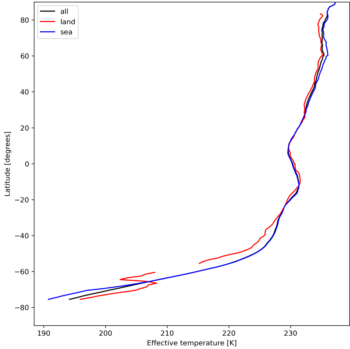
Figure 17: Zonal average of "Effective temperature" for 2024-08-16 to 2024-08-18.
