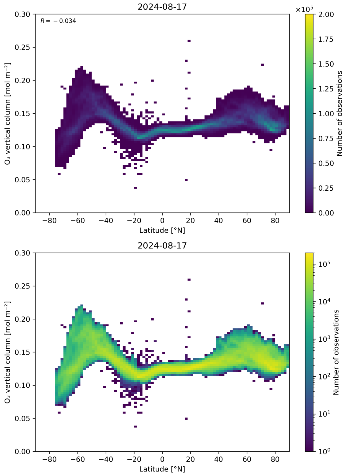
Figure 36: Scatter density plot of “Latitude” against “O 3 vertical column” for 2024-08-16 to 2024-08-18.
