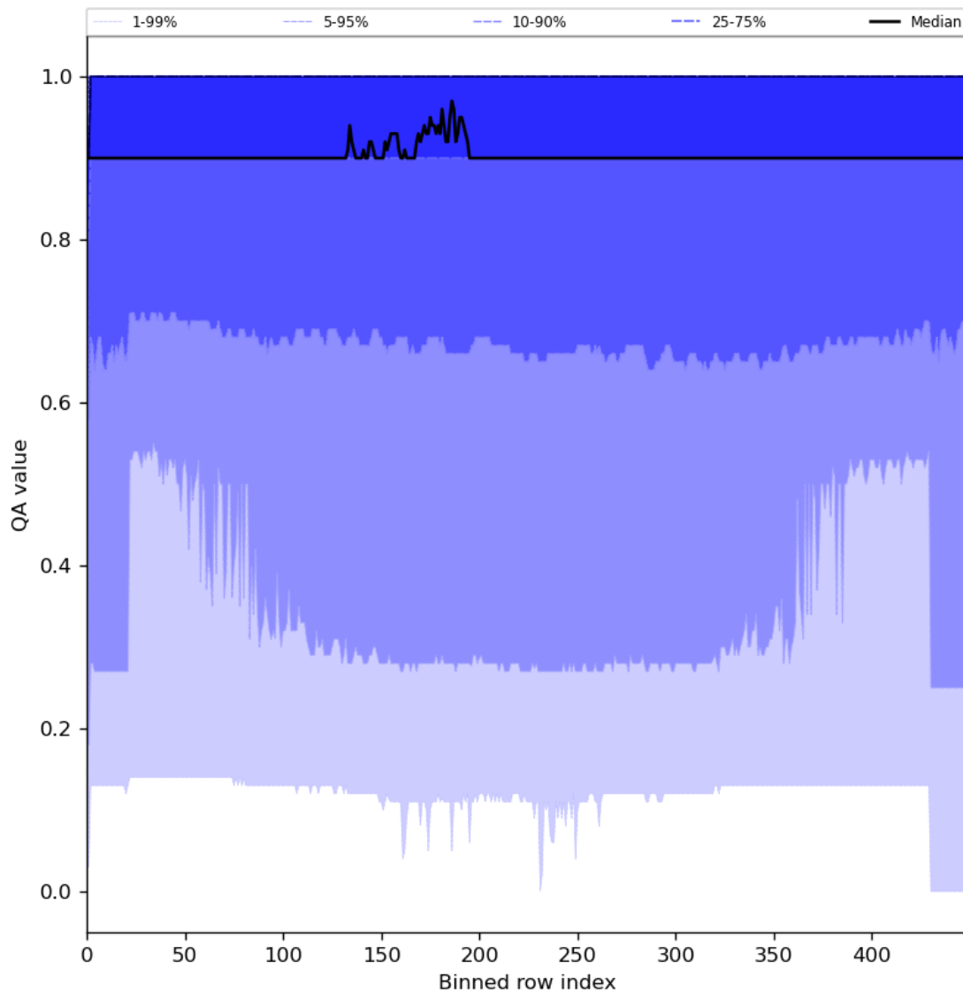
Figure 27: Along track statistics of “QA value” for 2024-08-16 to 2024-08-18
