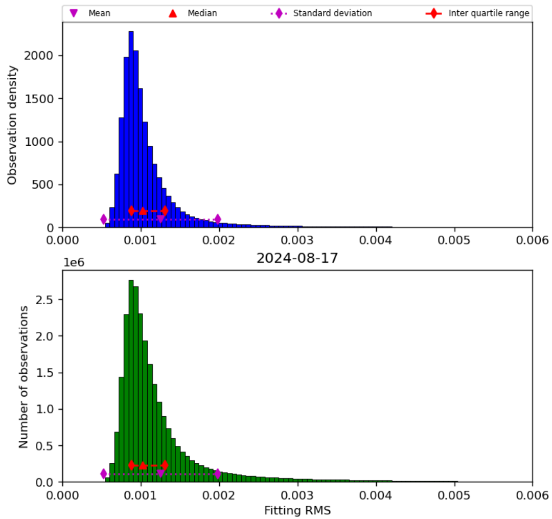
Figure 23: Histogram of “Fitting RMS” for 2024-08-16 to 2024-08-18
