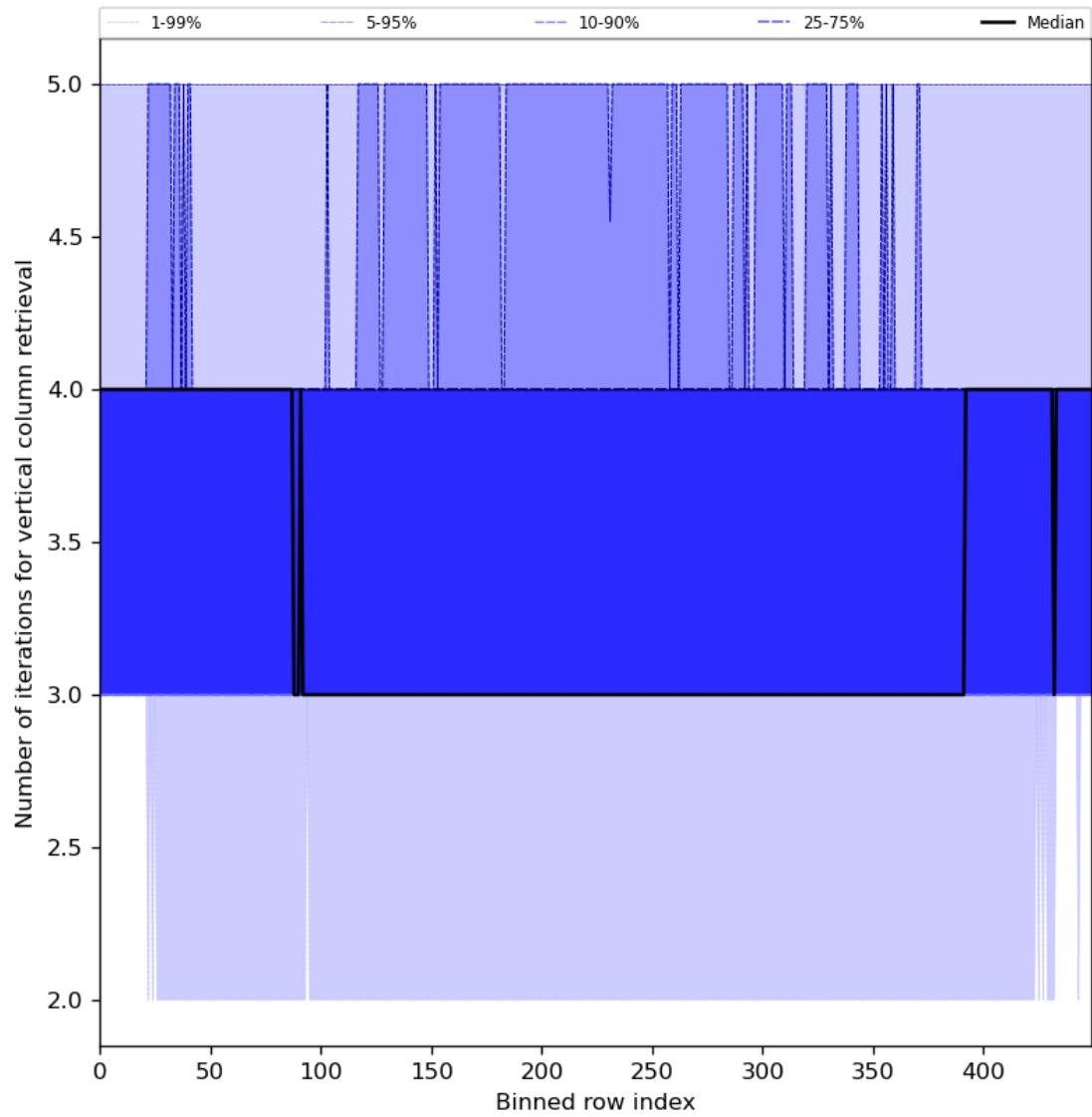
Figure 33: Along track statistics of “Number of iterations for vertical column retrieval” for 2024-08-16 to 2024-08-18
