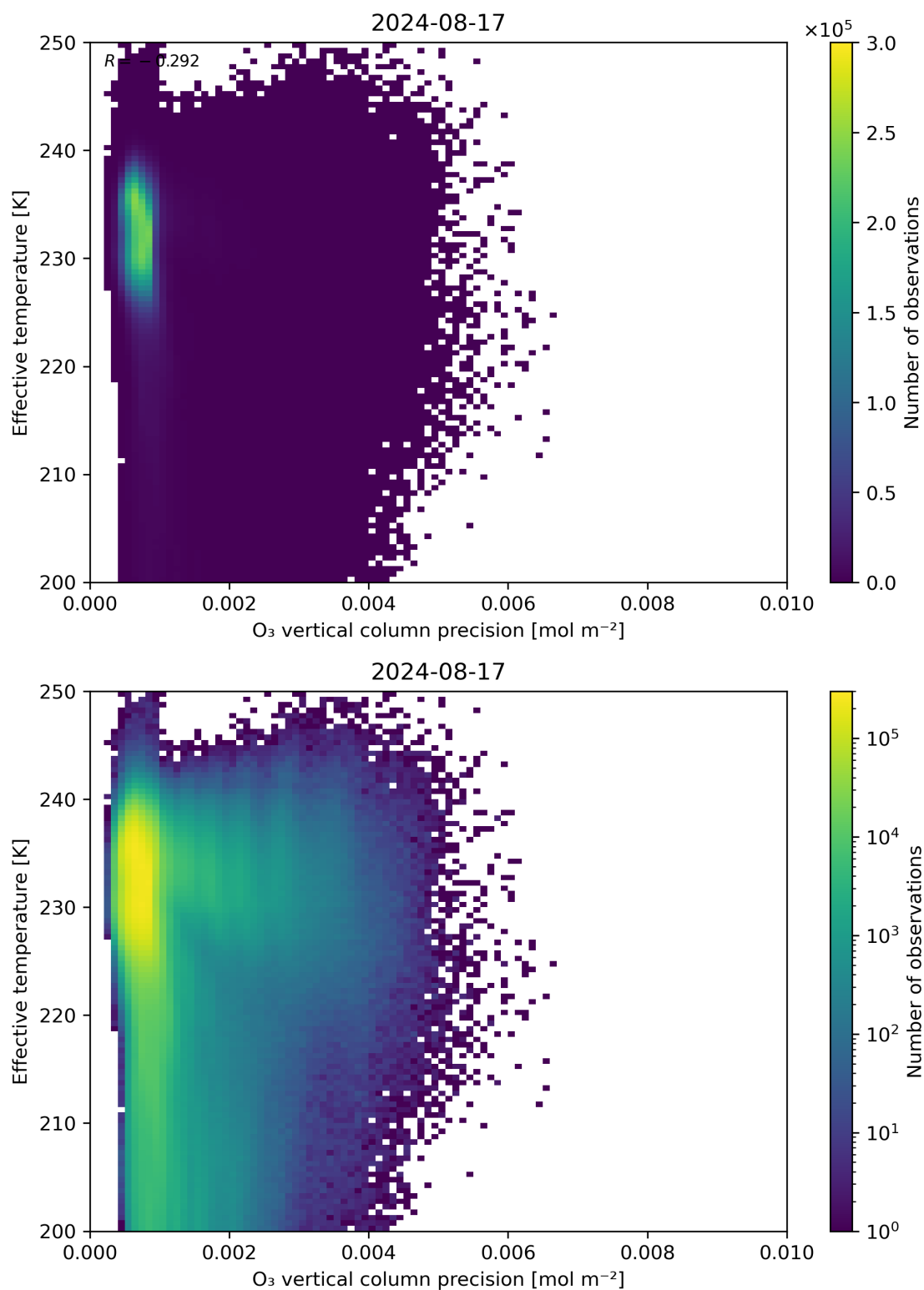
Figure 42: Scatter density plot of “O 3 vertical column precision” against “Effective temperature” for 2024-08-16 to 2024-08-18.
