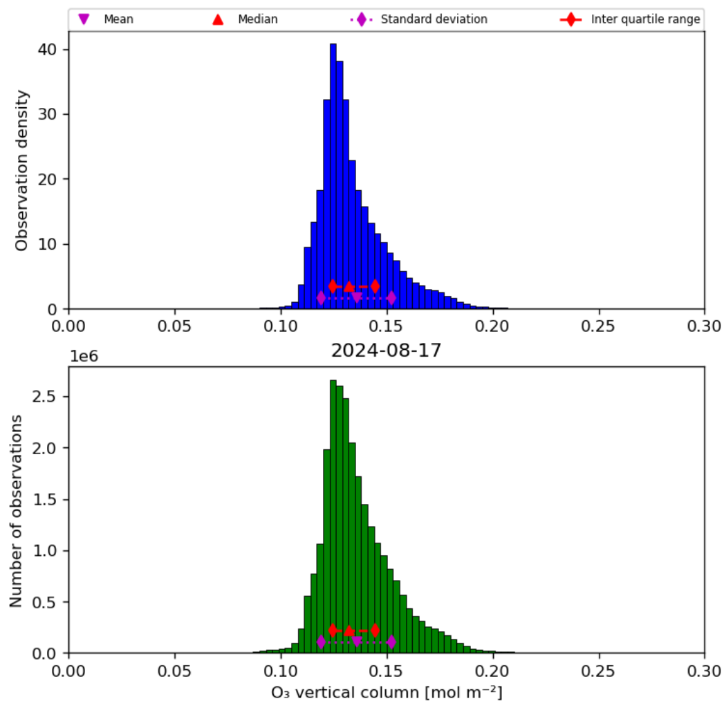
Figure 21: Histogram of “O 3 vertical column” for 2024-08-16 to 2024-08-18
