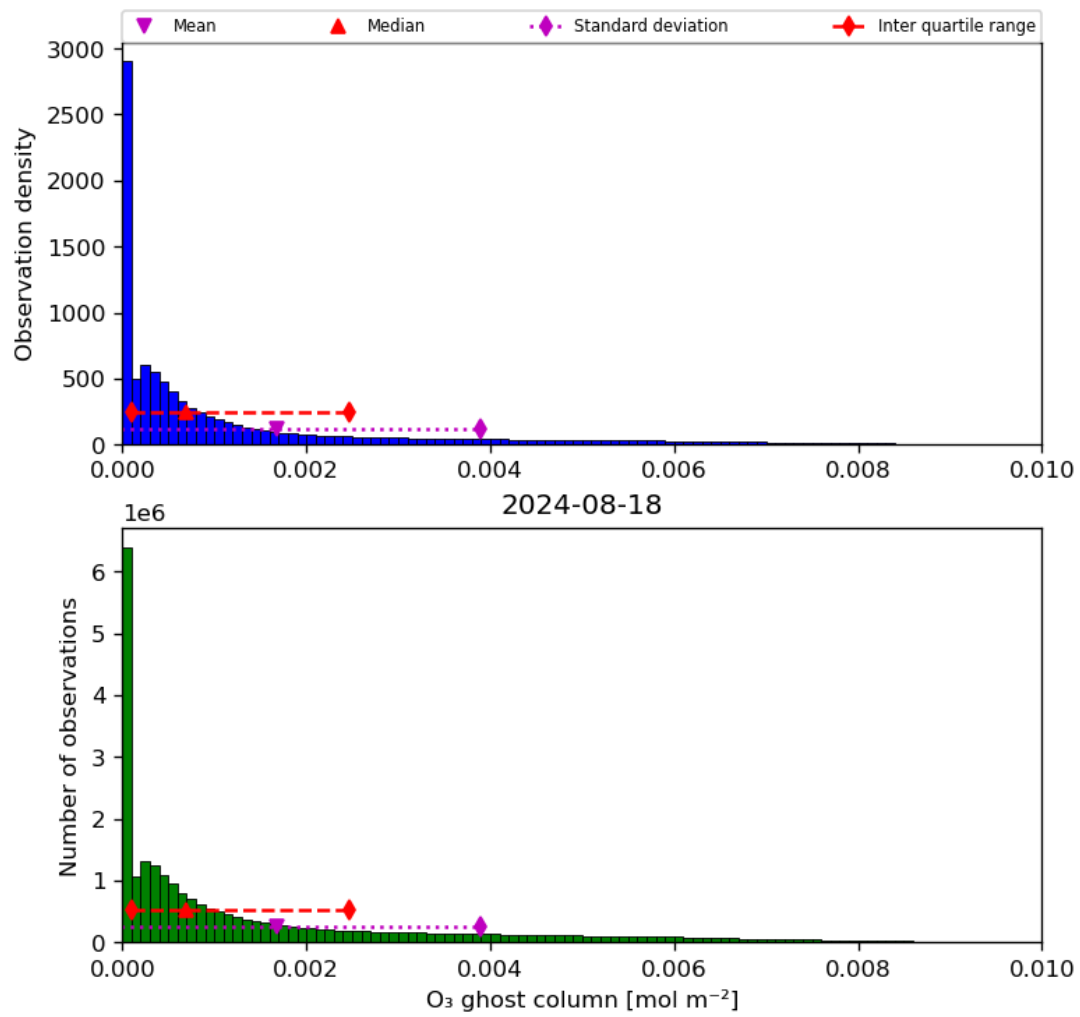
Figure 25: Histogram of “O 3 ghost column” for 2024-08-17 to 2024-08-19
