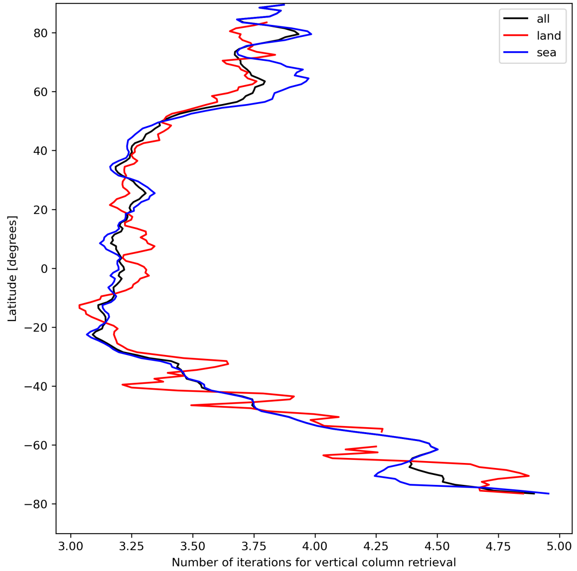
Figure 19: Zonal average of “Number of iterations for vertical column retrieval” for 2024-08-17 to 2024-08-19.
