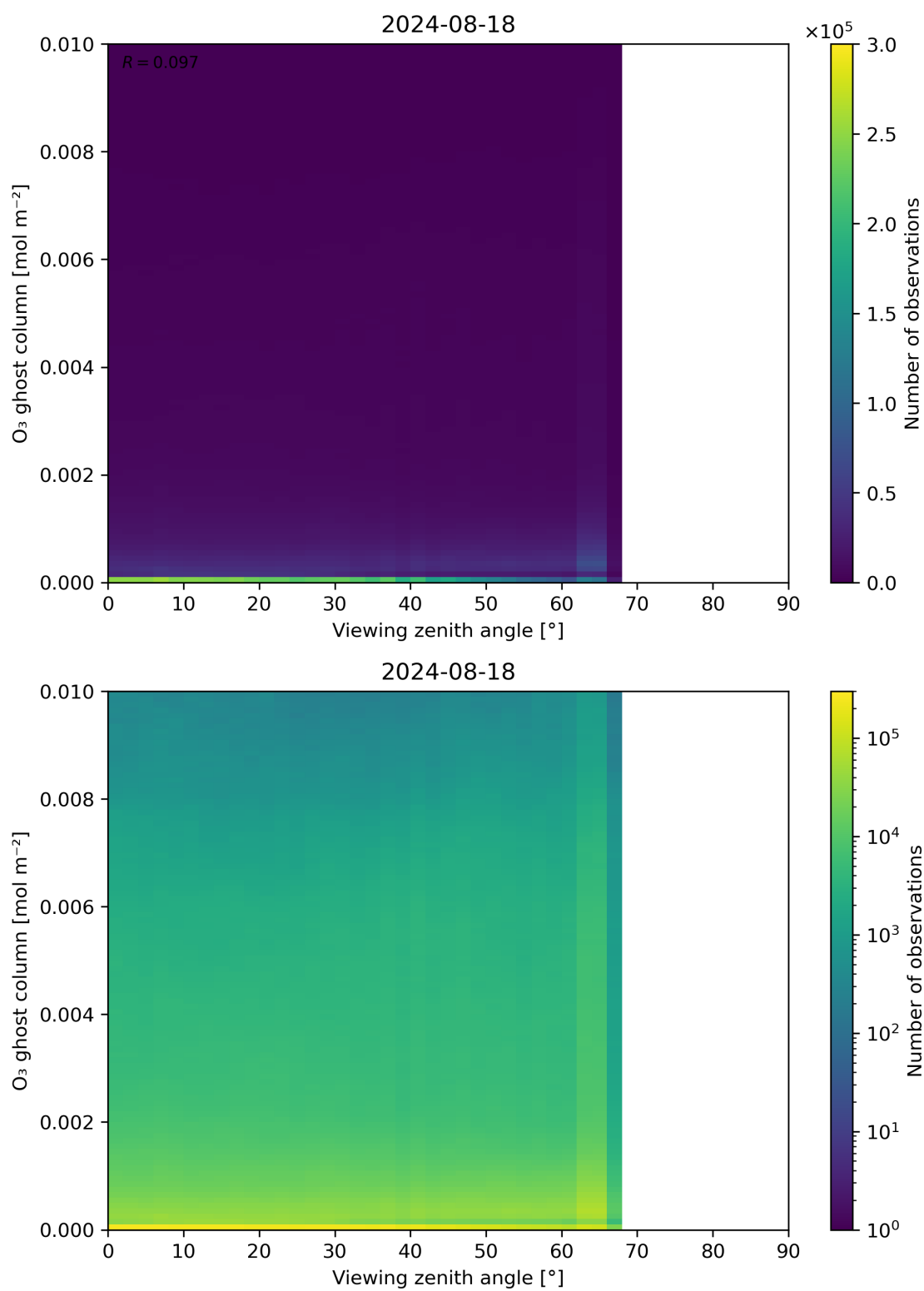
Figure 51: Scatter density plot of “Viewing zenith angle” against “O 3 ghost column” for 2024-08-17 to 2024-08-19.
