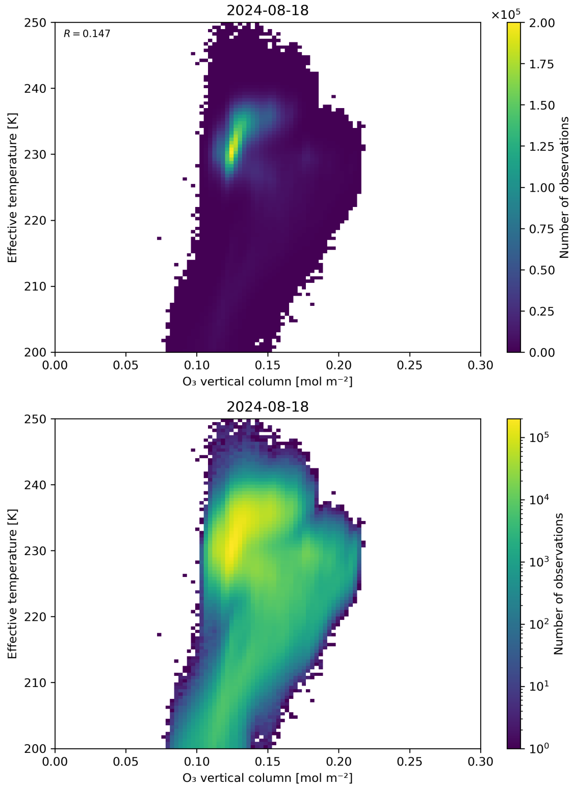
Figure 39: Scatter density plot of “O 3 vertical column” against “Effective temperature” for 2024-08-17 to 2024-08-19.
