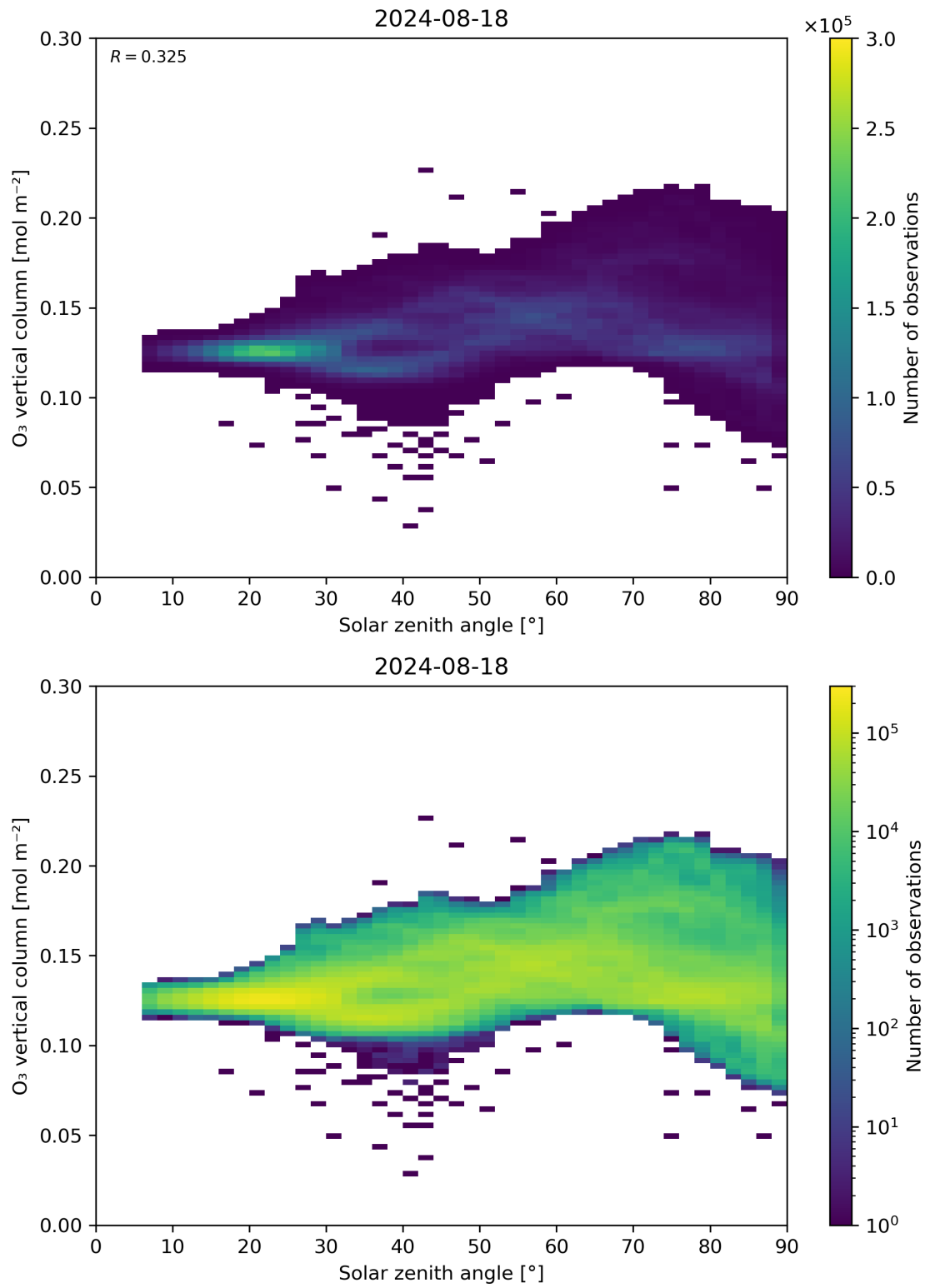
Figure 47: Scatter density plot of “Solar zenith angle” against “O 3 vertical column” for 2024-08-17 to 2024-08-19.
