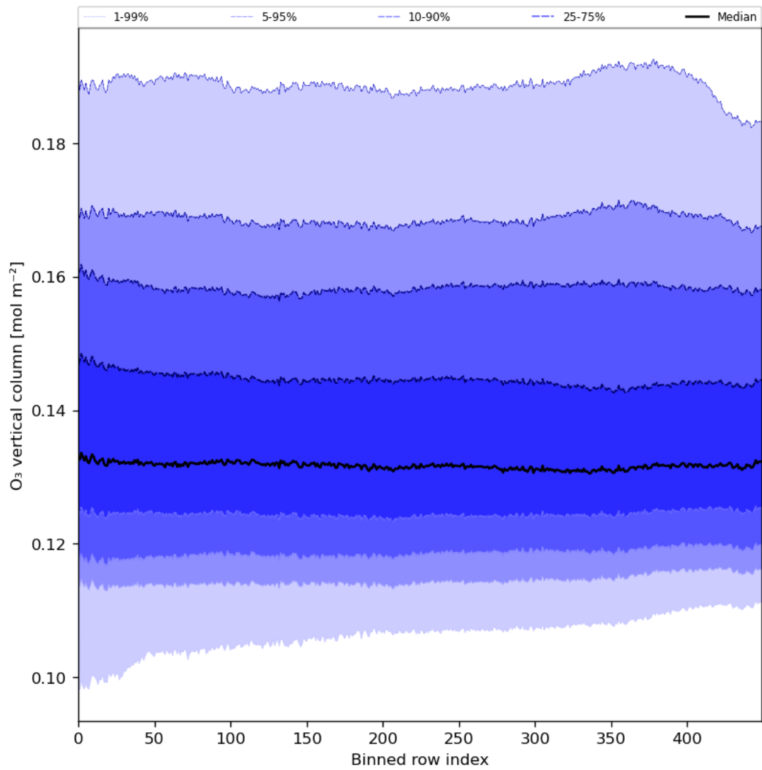
Figure 28: Along track statistics of “O 3 vertical column” for 2024-08-17 to 2024-08-19
