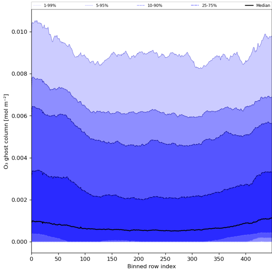
Figure 32: Along track statistics of “O 3 ghost column” for 2024-08-17 to 2024-08-19
