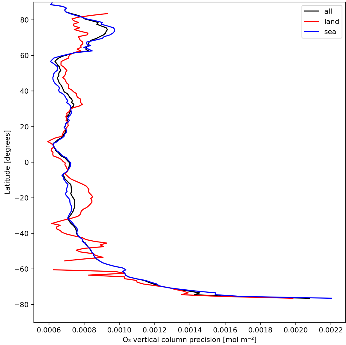
Figure 15: Zonal average of "O 3 vertical column precision" for 2024-08-17 to 2024-08-19.
