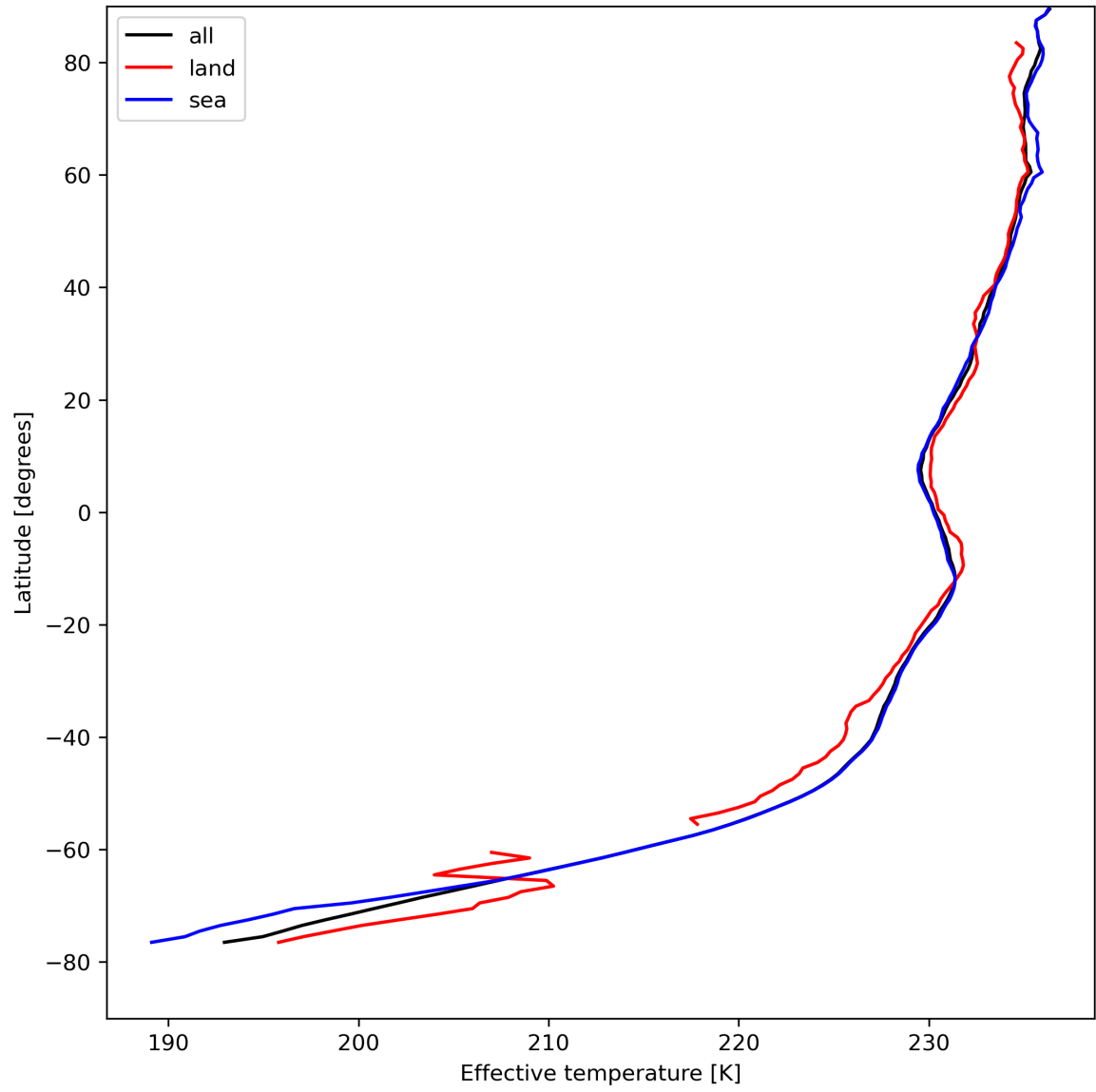
Figure 17: Zonal average of “Effective temperature” for 2024-08-17 to 2024-08-19.
