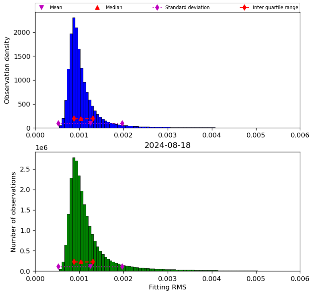
Figure 23: Histogram of “Fitting RMS” for 2024-08-17 to 2024-08-19
