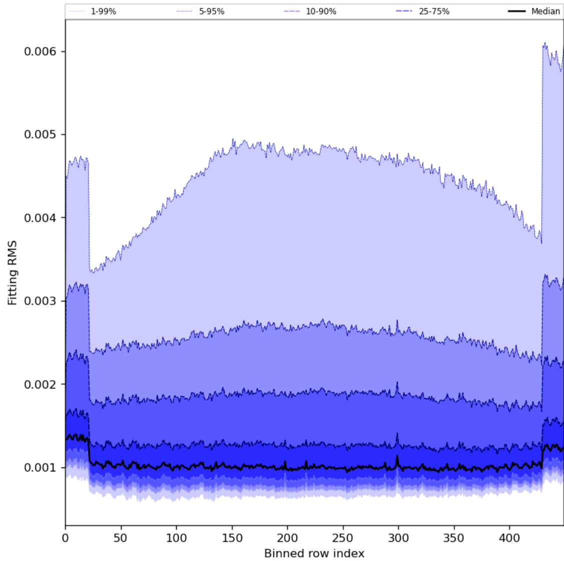
Figure 30: Along track statistics of “Fitting RMS” for 2024-08-17 to 2024-08-19
