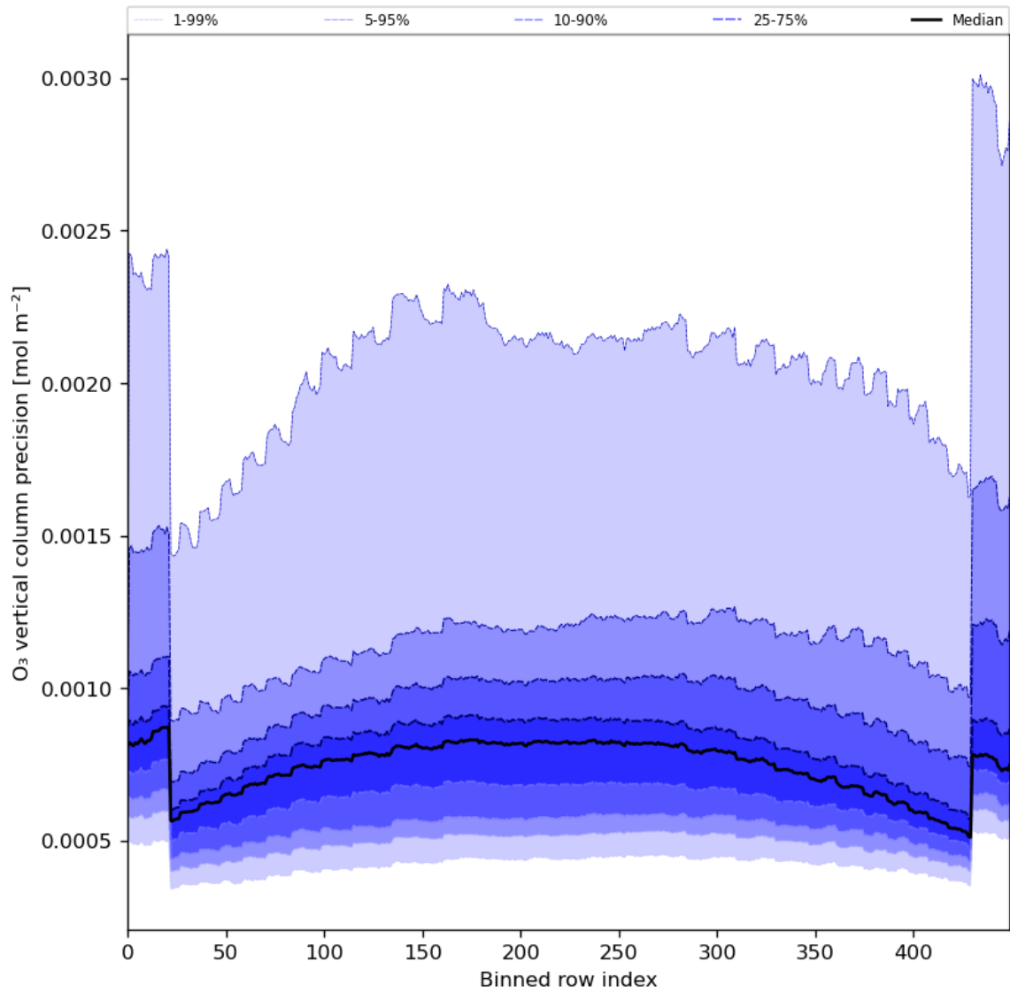
Figure 29: Along track statistics of “O 3 vertical column precision” for 2024-08-17 to 2024-08-19
