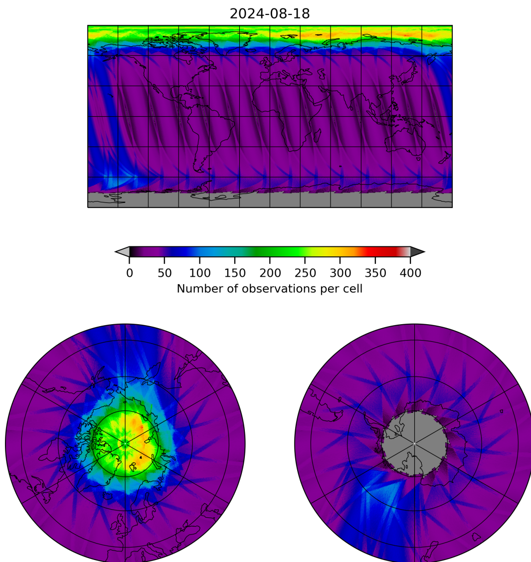
Figure 12: Map of the number of observations for 2024-08-17 to 2024-08-19
