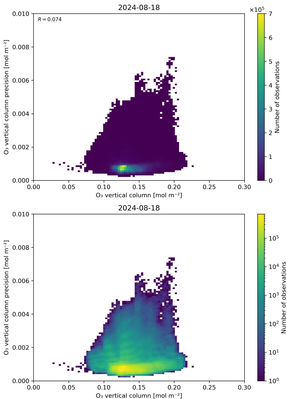
Figure 41: Scatter density plot of “O 3 vertical column” against “O 3 vertical column precision” for 2024-08-17 to 2024-08-19.
