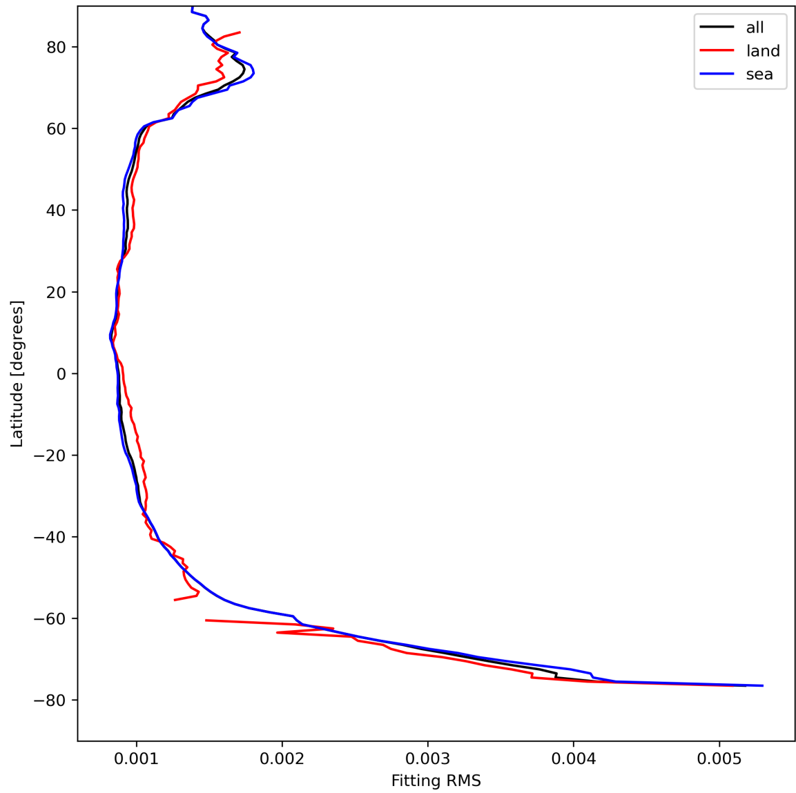
Figure 16: Zonal average of “Fitting RMS” for 2024-08-17 to 2024-08-19.
