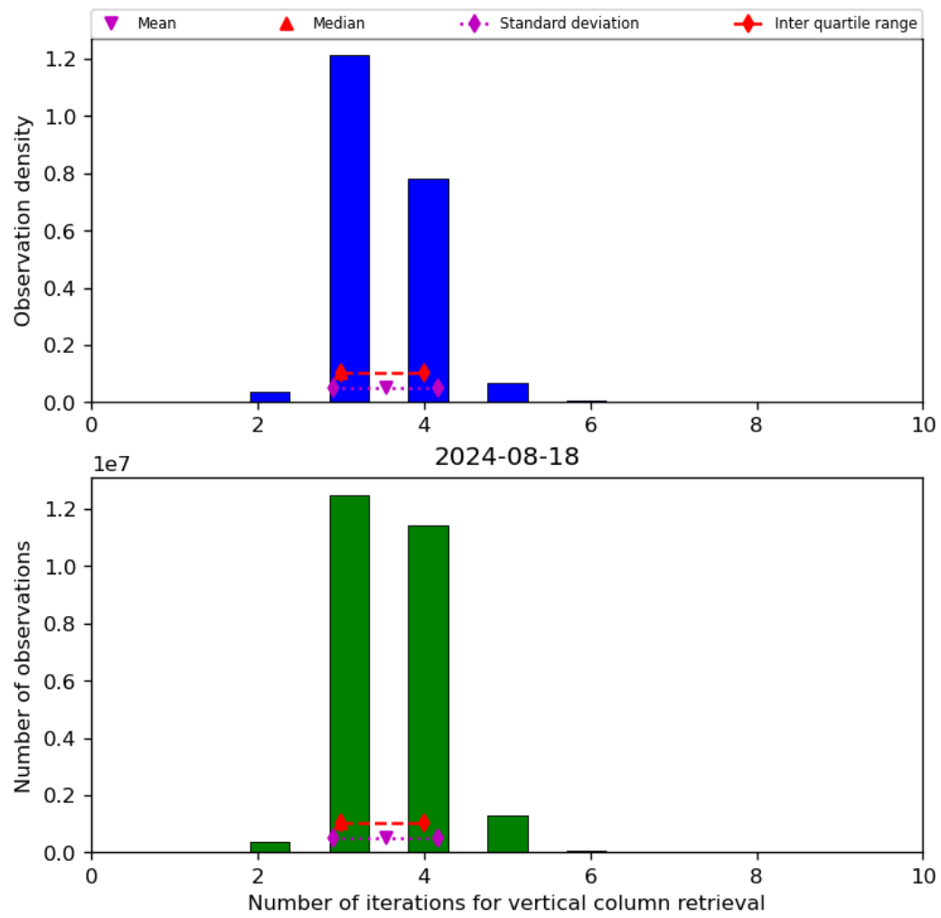
Figure 26: Histogram of “Number of iterations for vertical column retrieval” for 2024-08-17 to 2024-08-19
