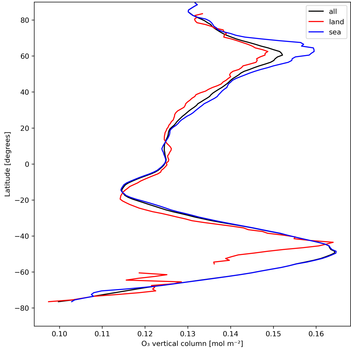
Figure 14: Zonal average of “O 3 vertical column” for 2024-08-17 to 2024-08-19.
