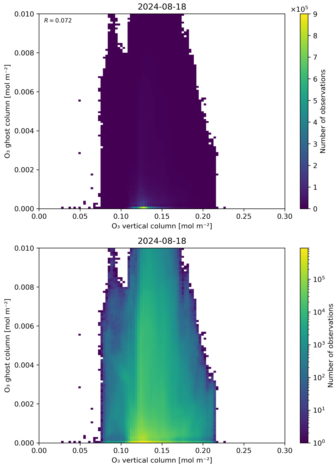
Figure 40: Scatter density plot of “O 3 vertical column” against “O 3 ghost column” for 2024-08-17 to 2024-08-19.
