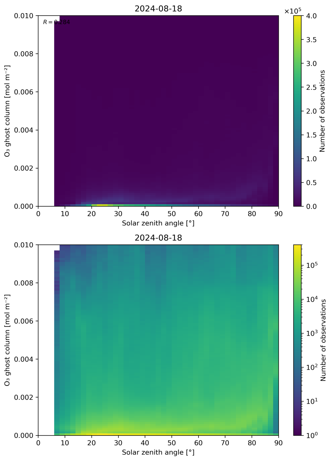
Figure 46: Scatter density plot of “Solar zenith angle” against “O 3 ghost column” for 2024-08-17 to 2024-08-19.
