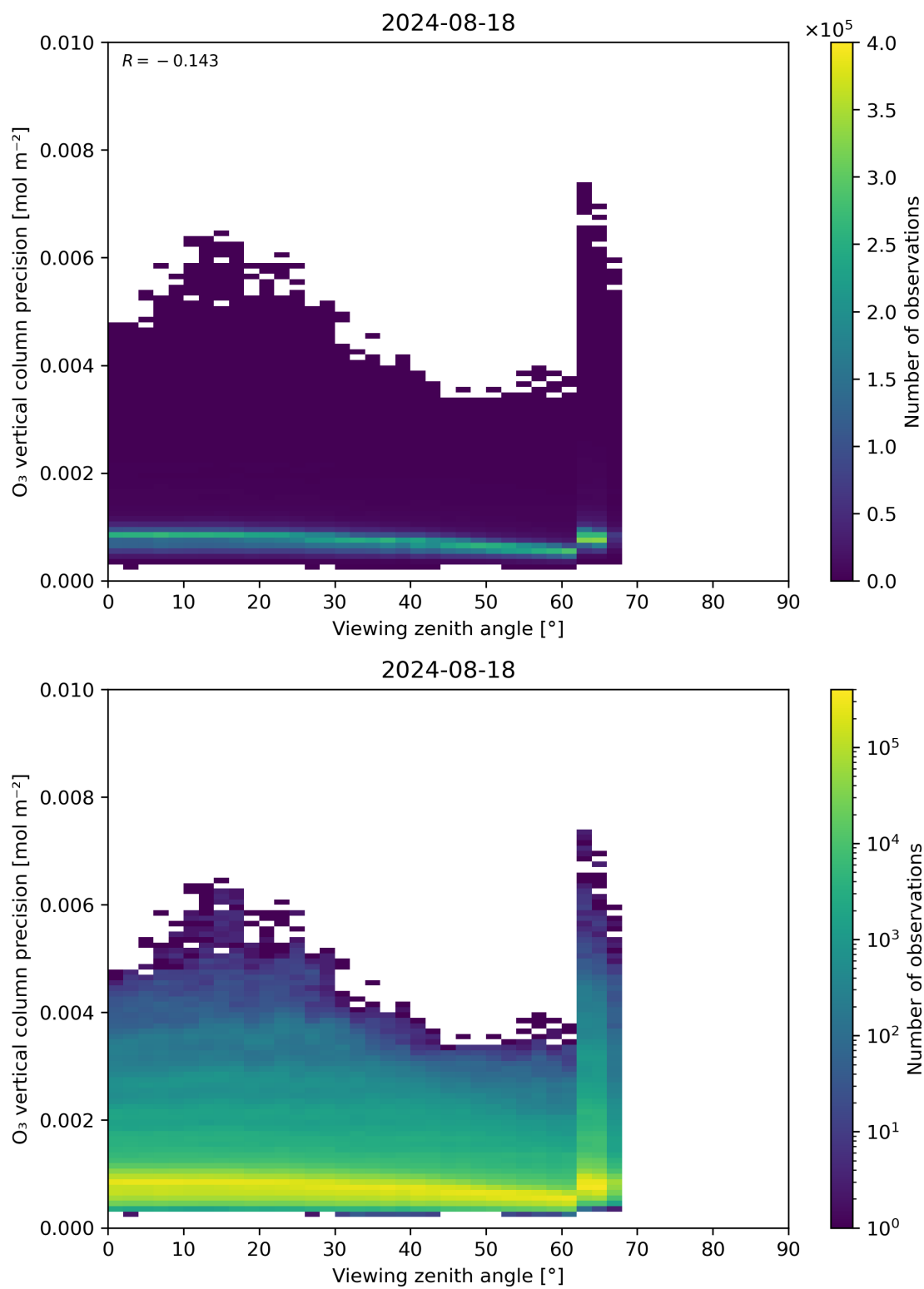
Figure 53: Scatter density plot of “Viewing zenith angle” against “O 3 vertical column precision” for 2024-08-17 to 2024-08-19.
