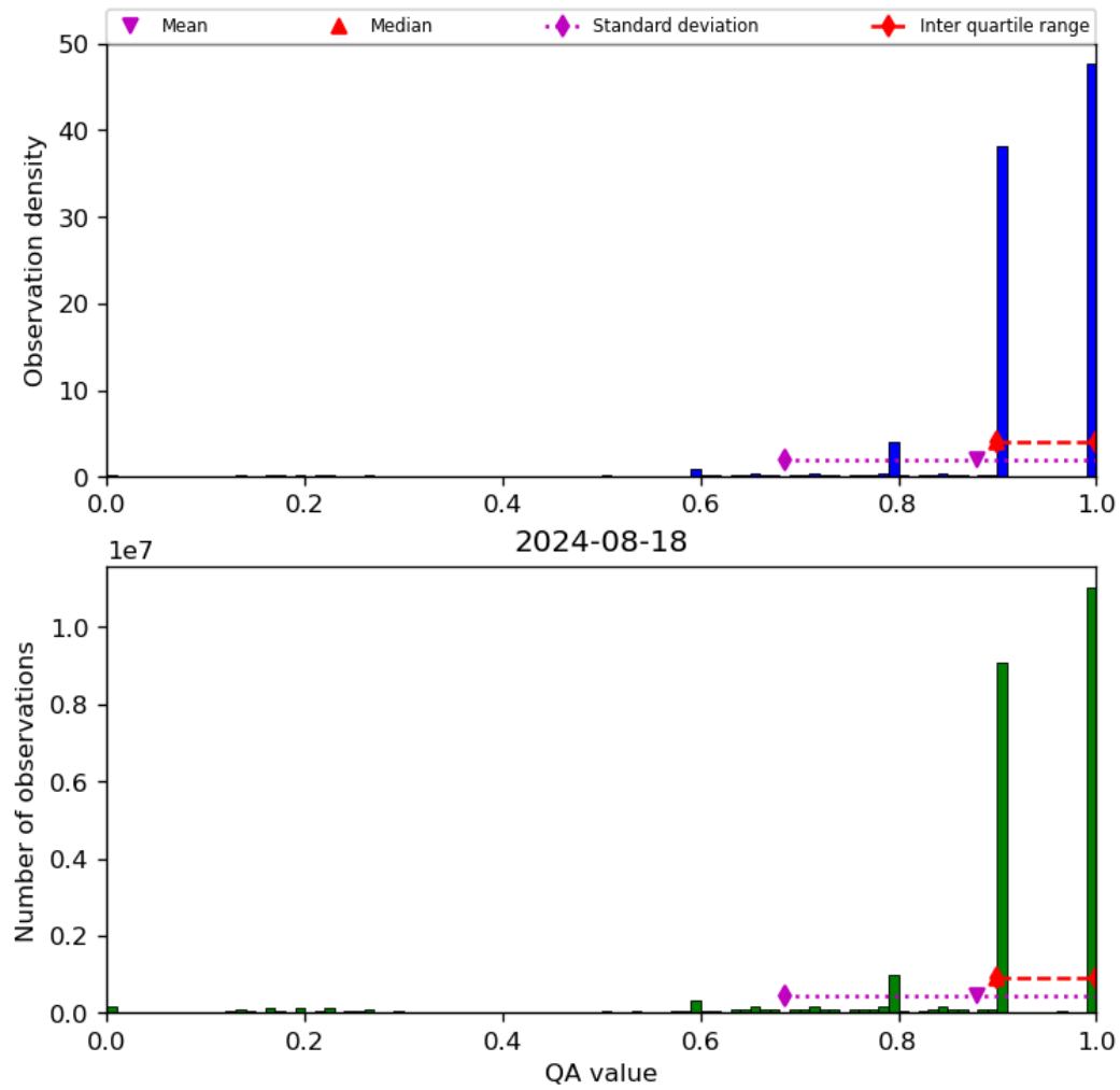
Figure 20: Histogram of “QA value” for 2024-08-17 to 2024-08-19
