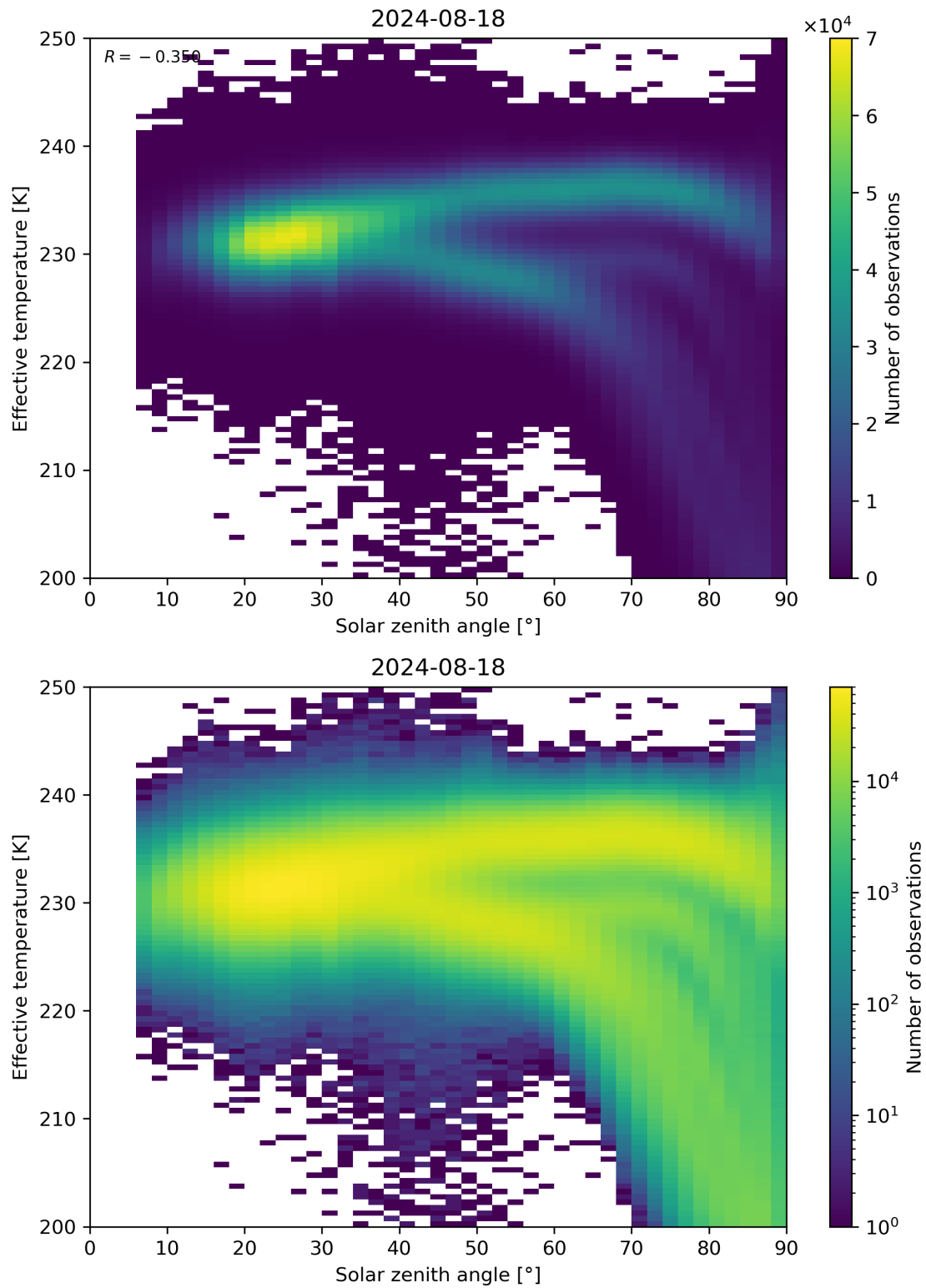
Figure 45: Scatter density plot of “Solar zenith angle” against “Effective temperature” for 2024-08-17 to 2024-08-19.
