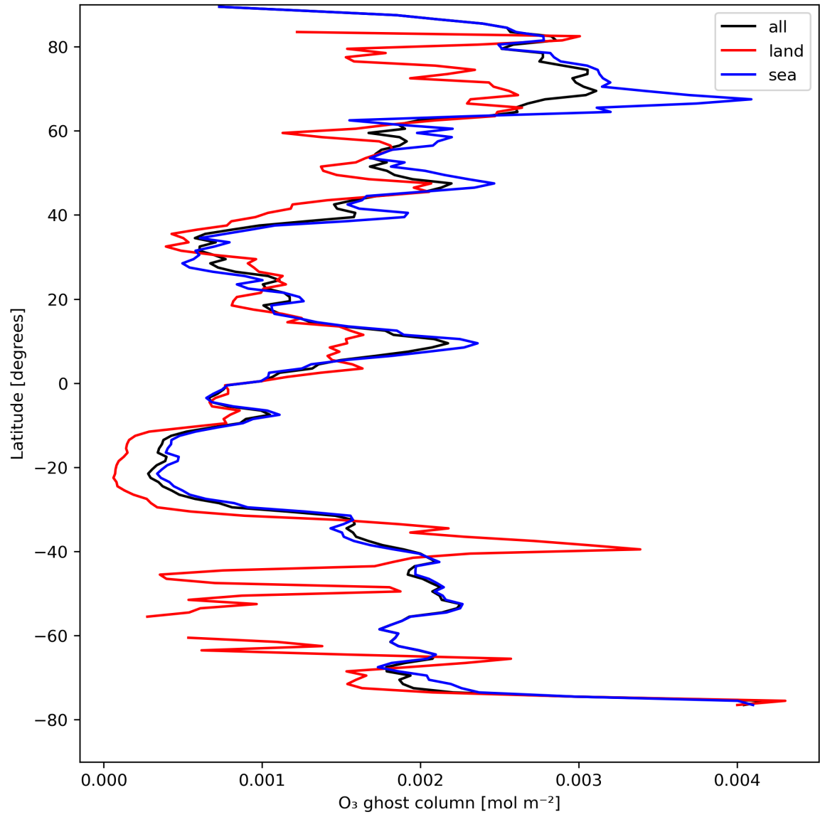
Figure 18: Zonal average of “O 3 ghost column” for 2024-08-17 to 2024-08-19.
