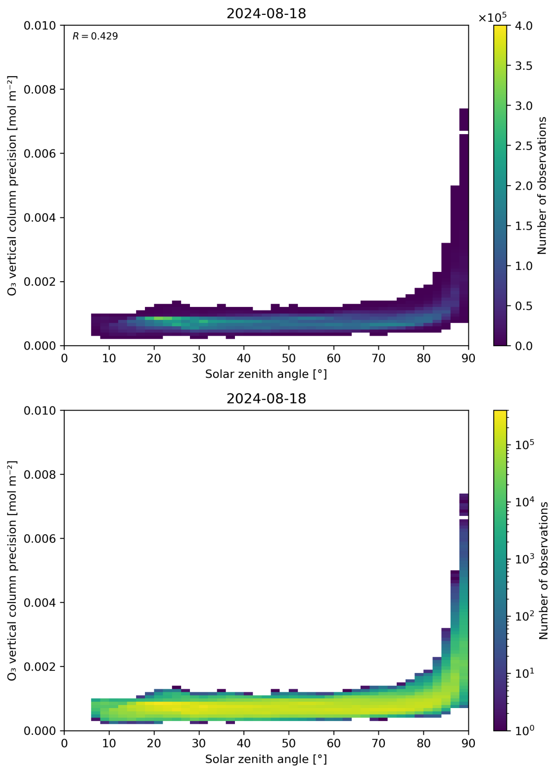
Figure 48: Scatter density plot of “Solar zenith angle” against “O 3 vertical column precision” for 2024-08-17 to 2024-08-19.
