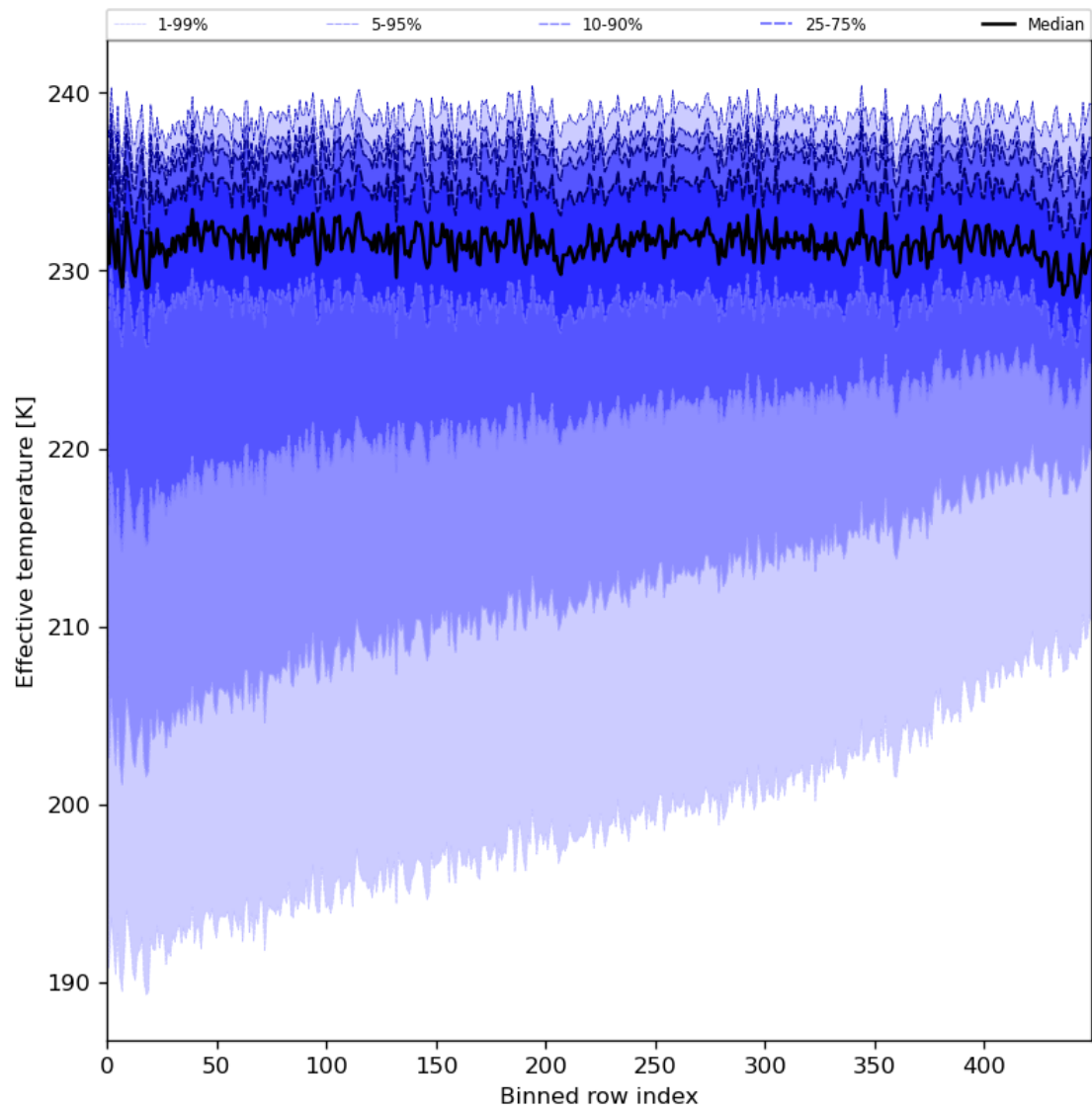
Figure 31: Along track statistics of “Effective temperature” for 2024-08-17 to 2024-08-19
