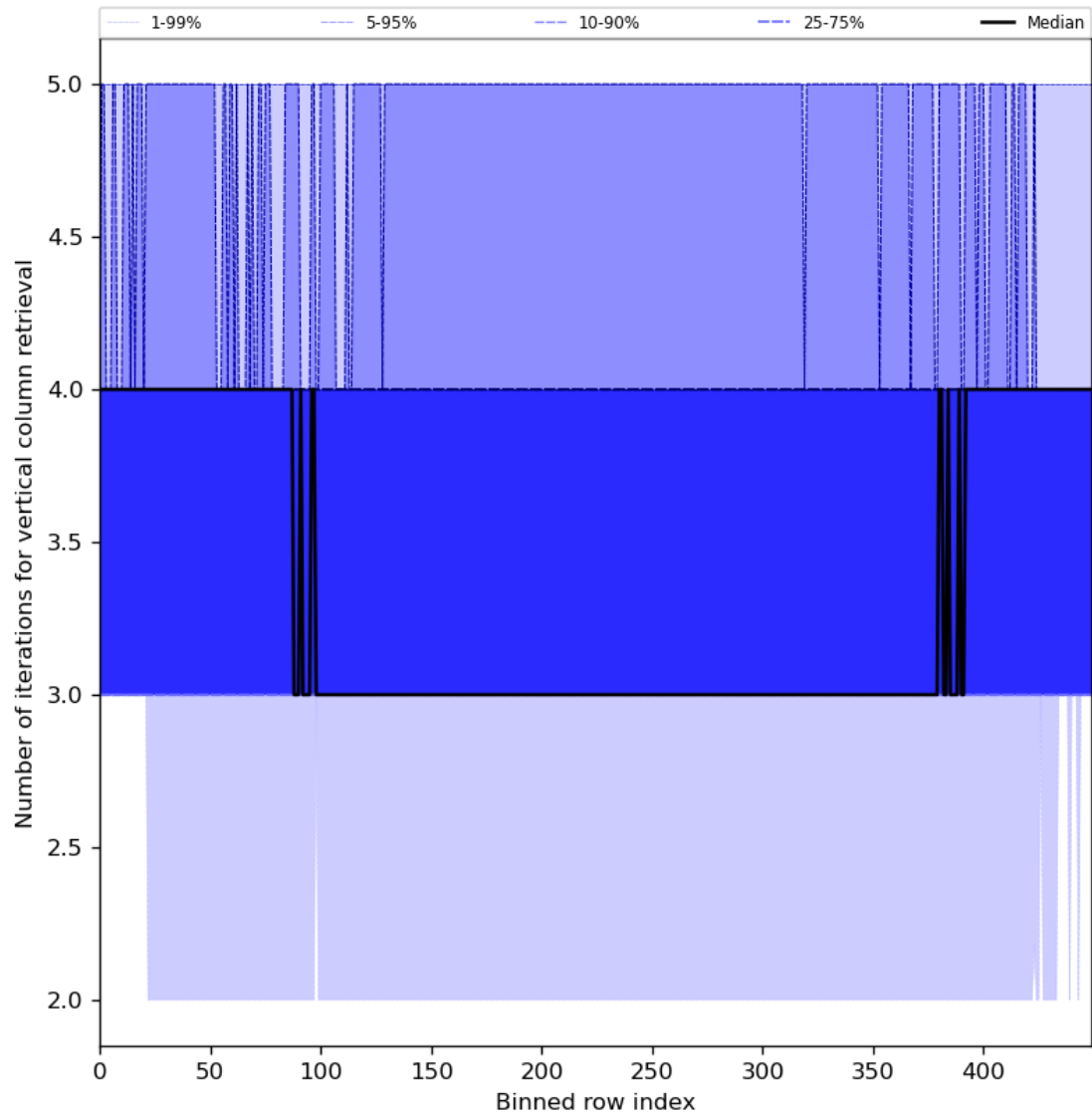
Figure 33: Along track statistics of “Number of iterations for vertical column retrieval” for 2024-08-17 to 2024-08-19
