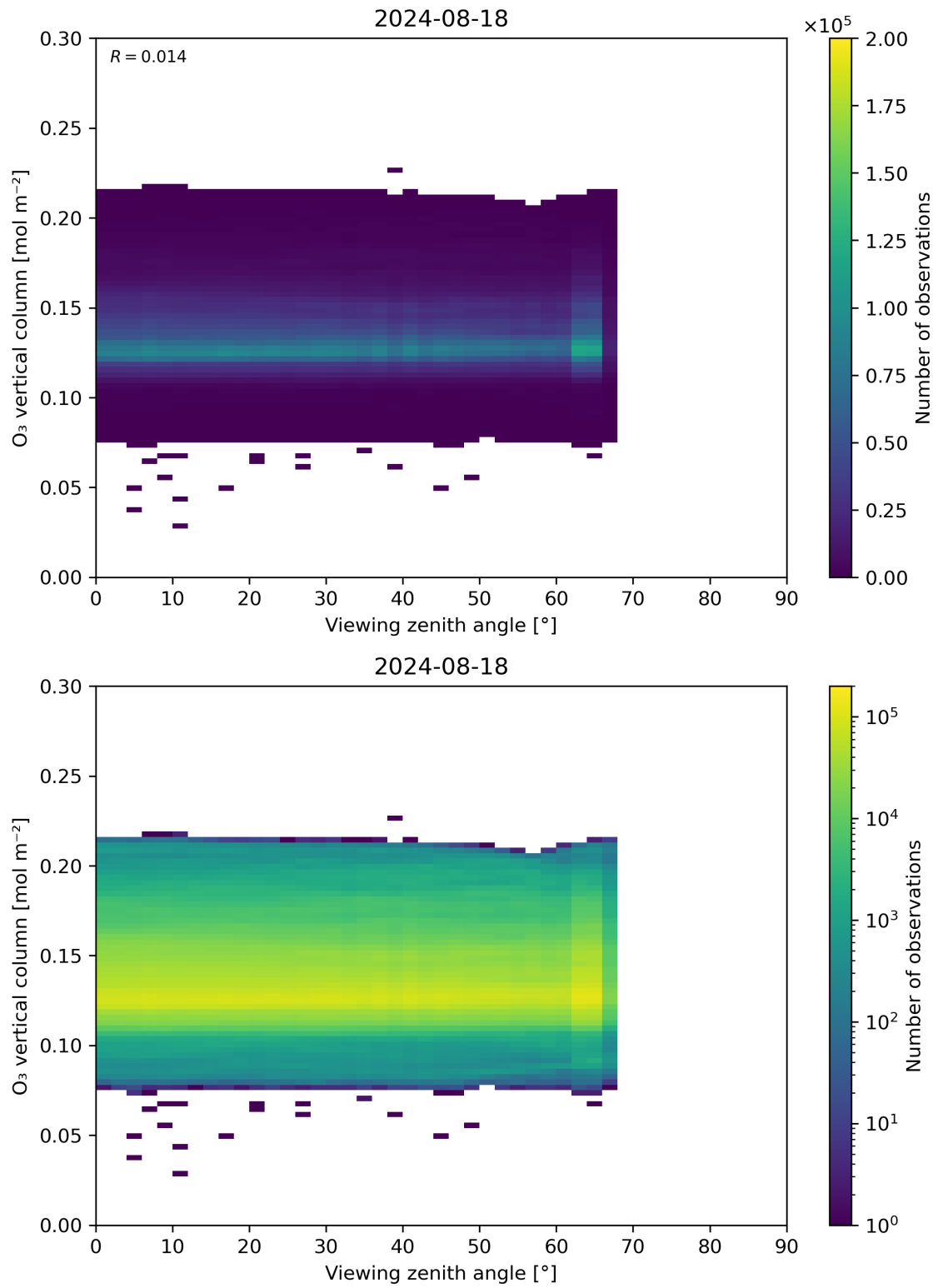
Figure 52: Scatter density plot of “Viewing zenith angle” against “O 3 vertical column” for 2024-08-17 to 2024-08-19.
