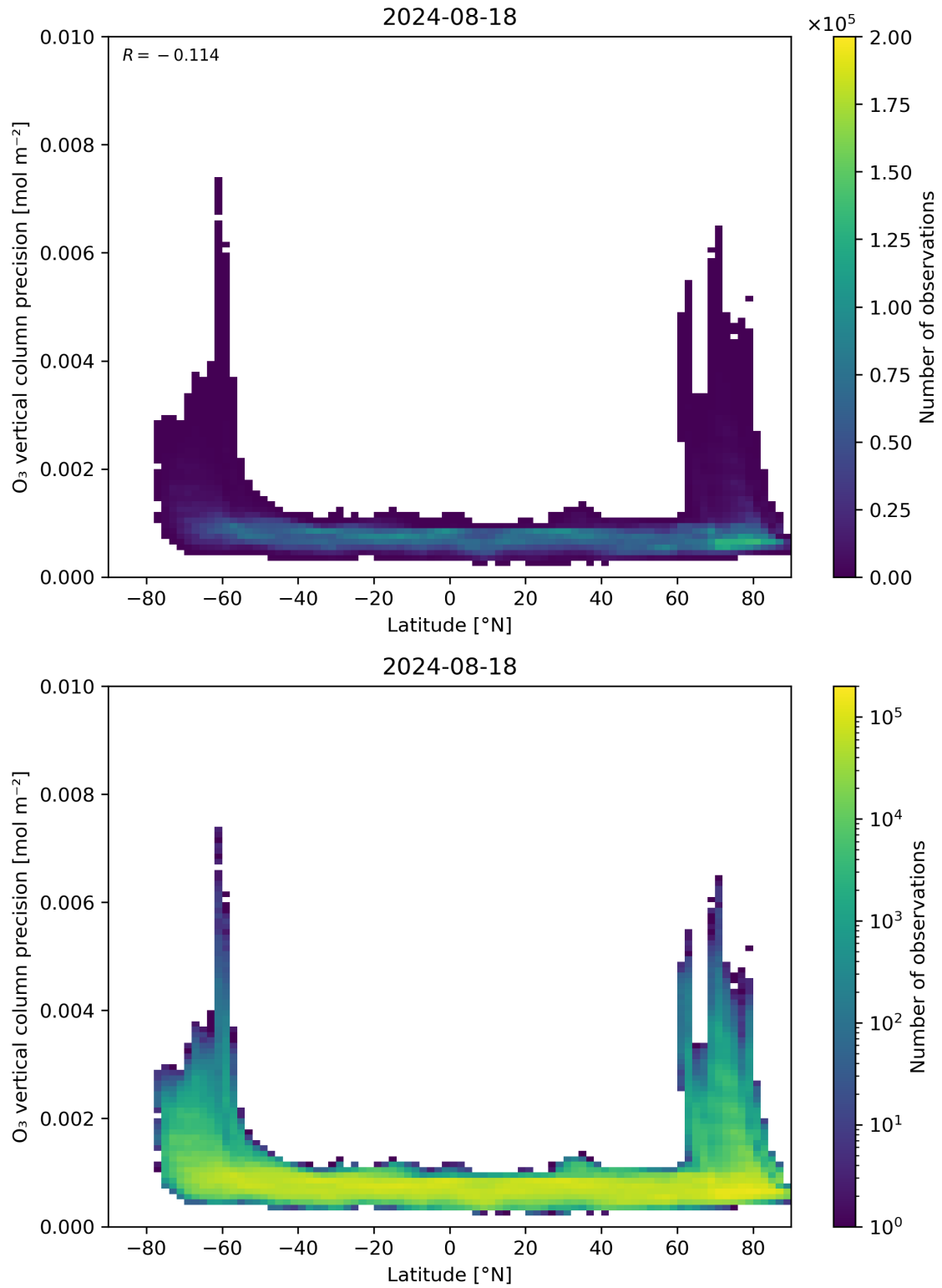
Figure 37: Scatter density plot of “Latitude” against “O 3 vertical column precision” for 2024-08-17 to 2024-08-19.
