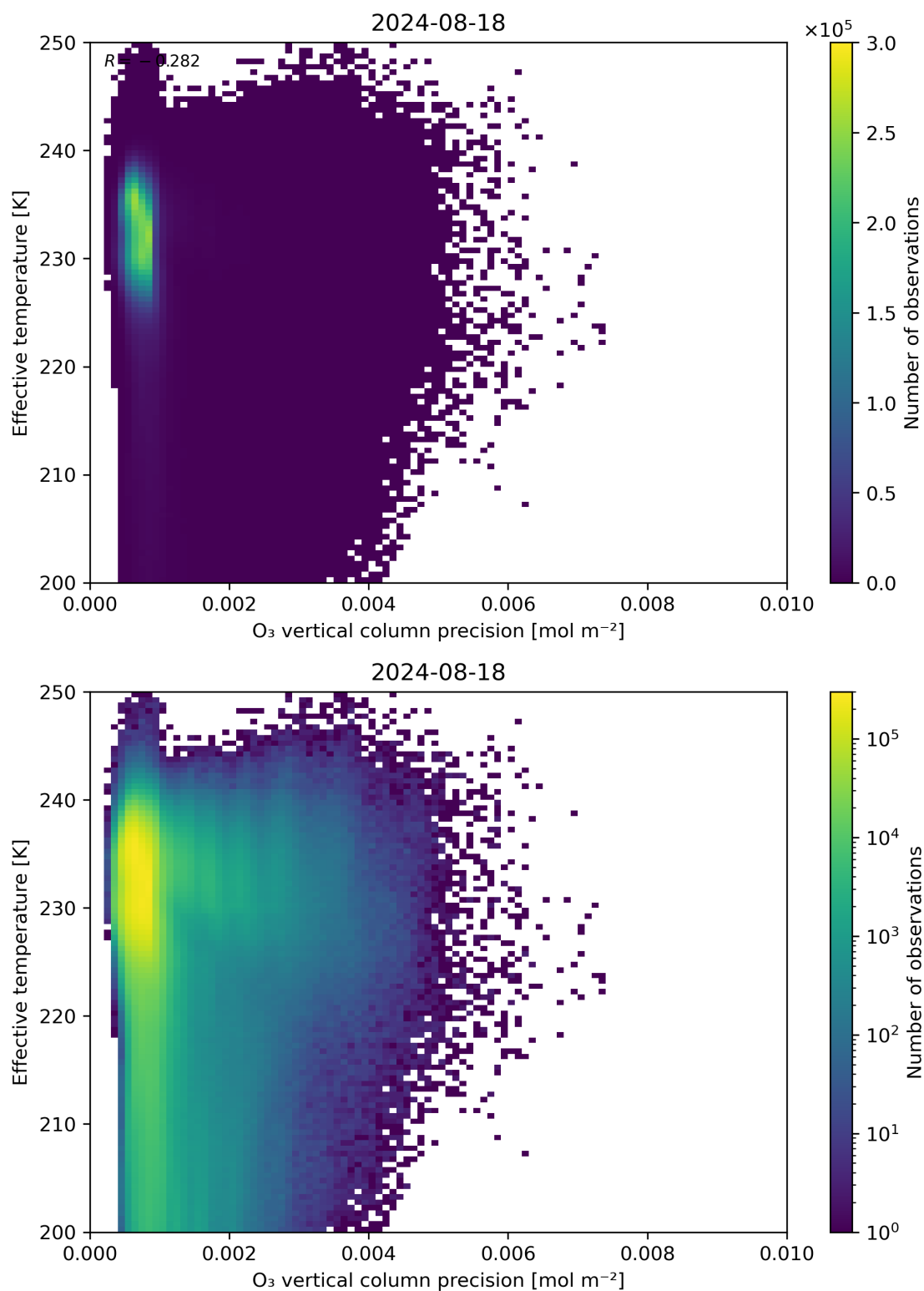
Figure 42: Scatter density plot of “O 3 vertical column precision” against “Effective temperature” for 2024-08-17 to 2024-08-19.
