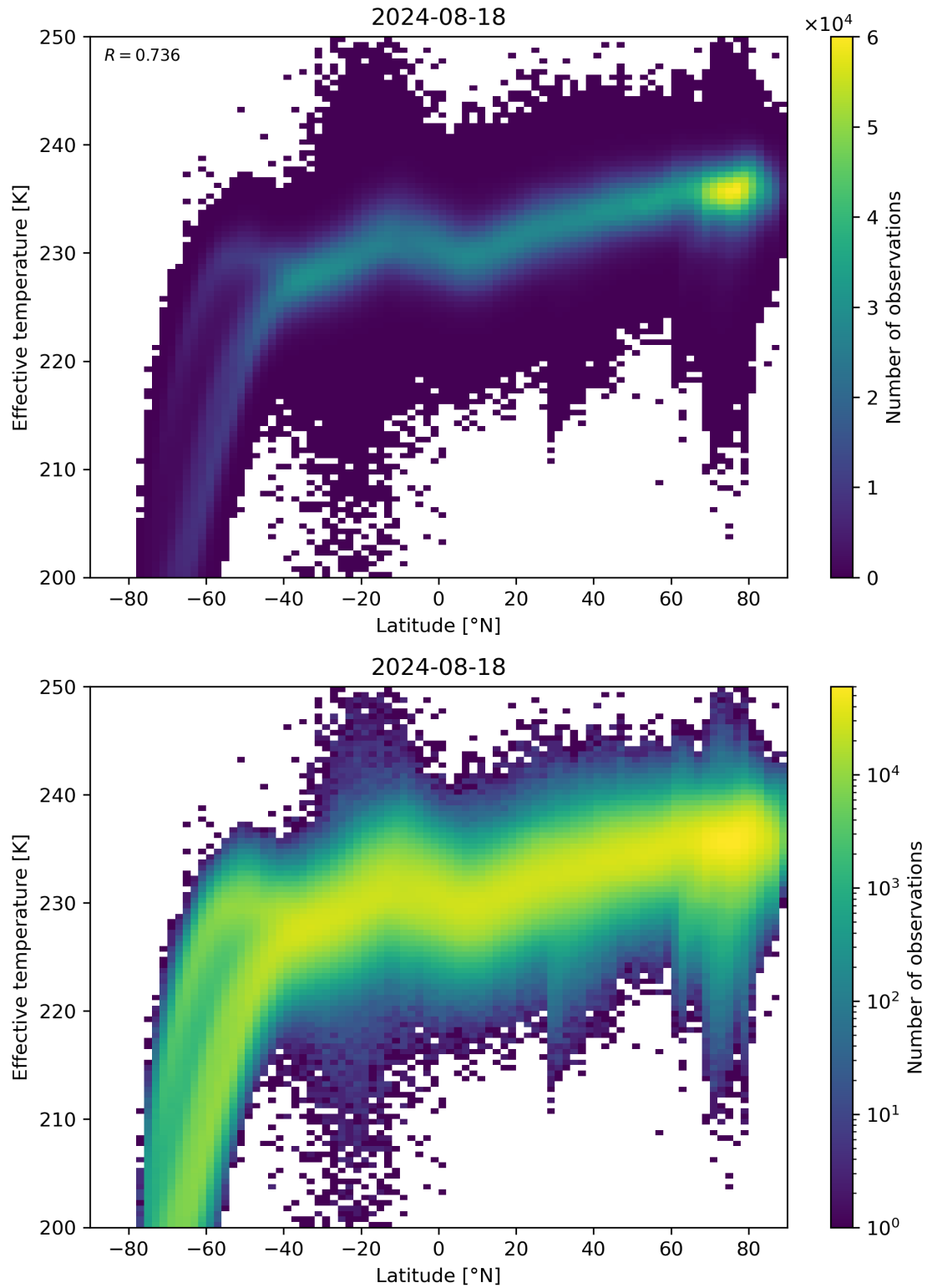
Figure 34: Scatter density plot of “Latitude” against “Effective temperature” for 2024-08-17 to 2024-08-19.
