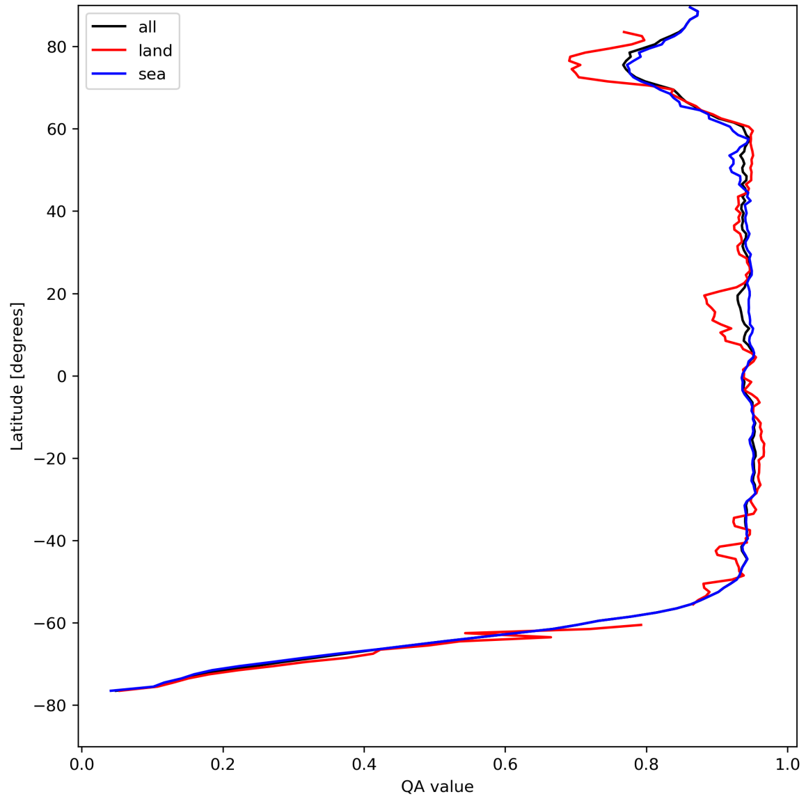
Figure 13: Zonal average of “QA value” for 2024-08-17 to 2024-08-19.
