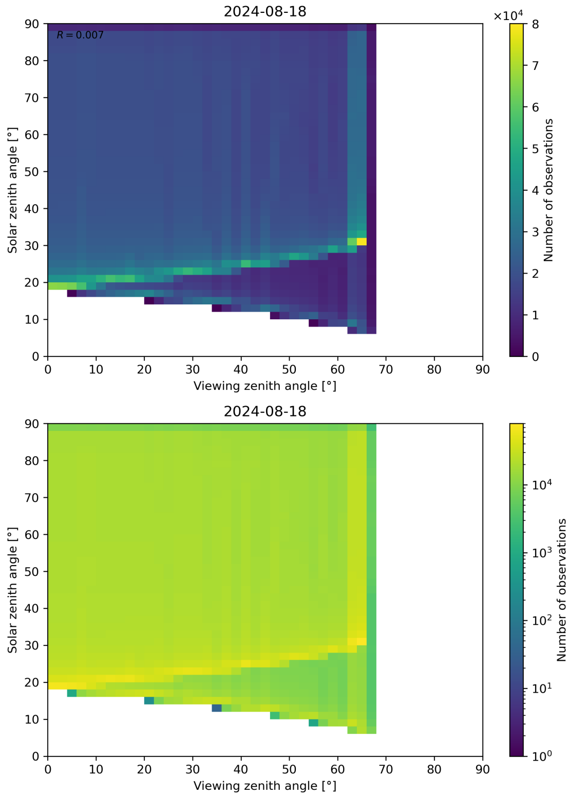
Figure 54: Scatter density plot of “Viewing zenith angle” against “Solar zenith angle” for 2024-08-17 to 2024-08-19.
