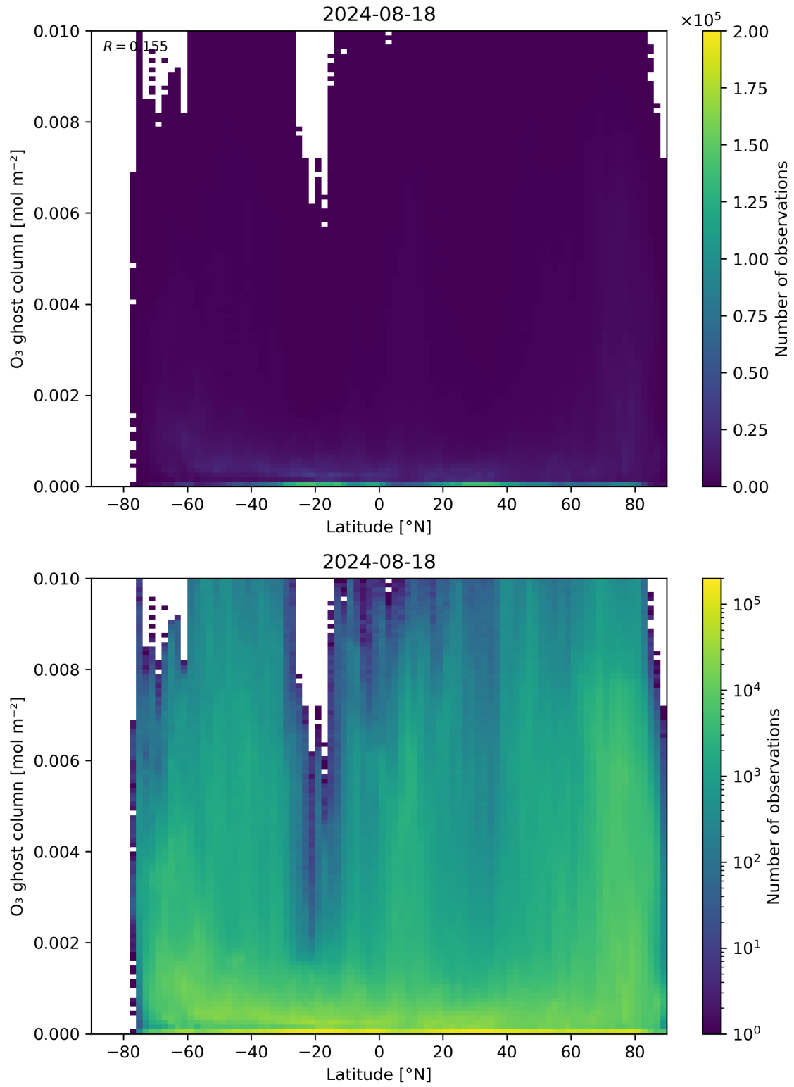
Figure 35: Scatter density plot of “Latitude” against “O 3 ghost column” for 2024-08-17 to 2024-08-19.
