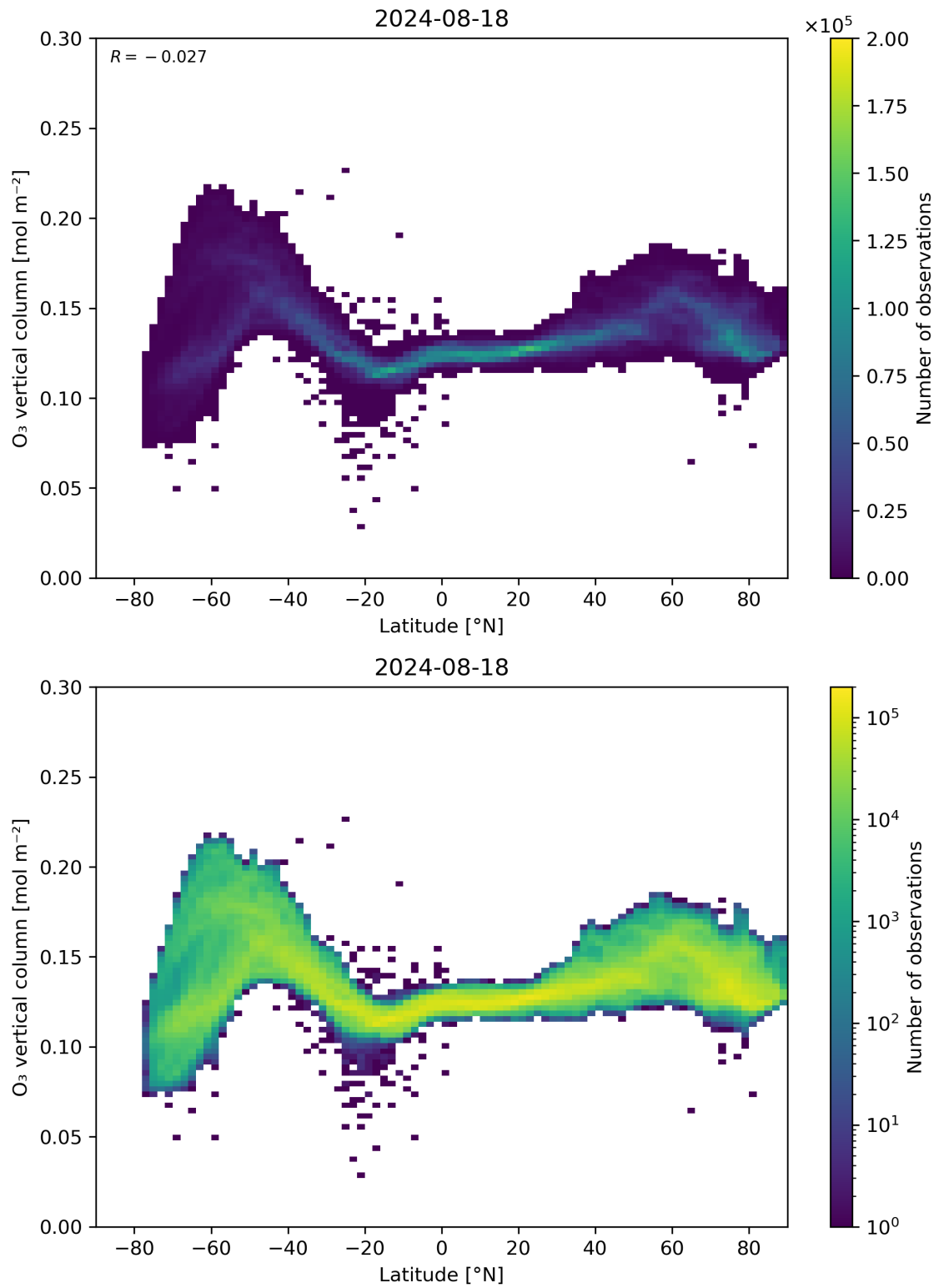
Figure 36: Scatter density plot of “Latitude” against “O 3 vertical column” for 2024-08-17 to 2024-08-19.
