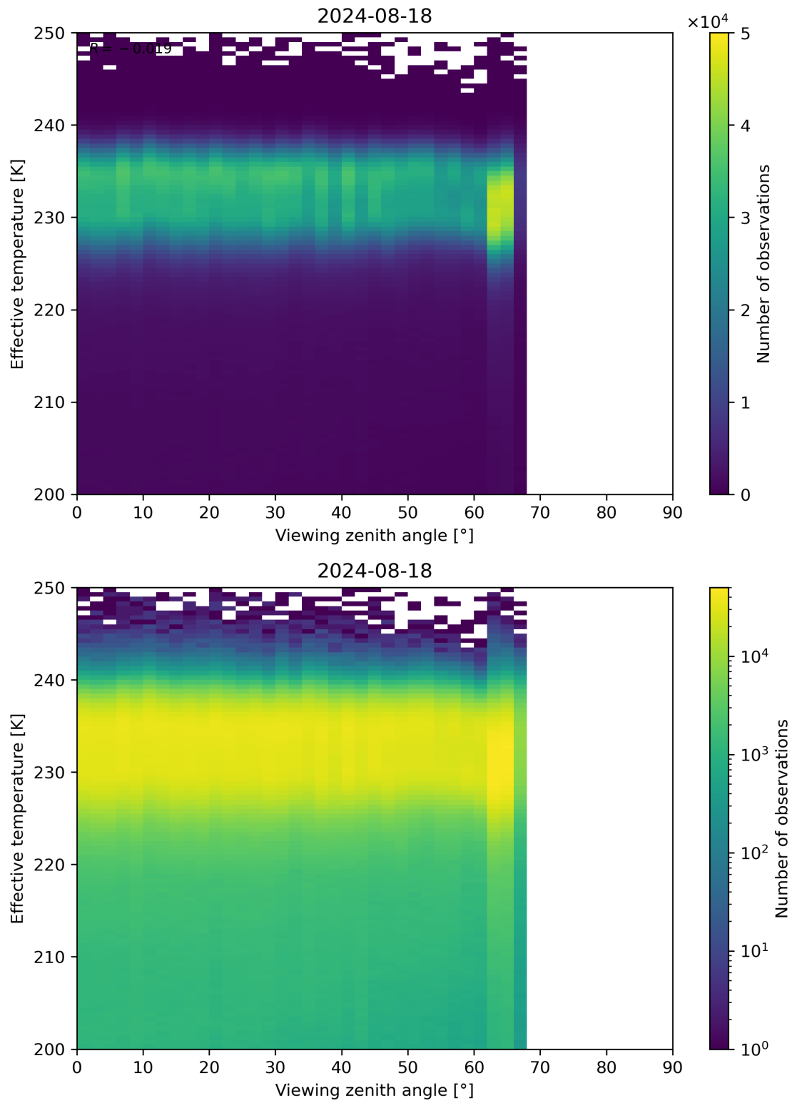
Figure 50: Scatter density plot of “Viewing zenith angle” against “Effective temperature” for 2024-08-17 to 2024-08-19.
