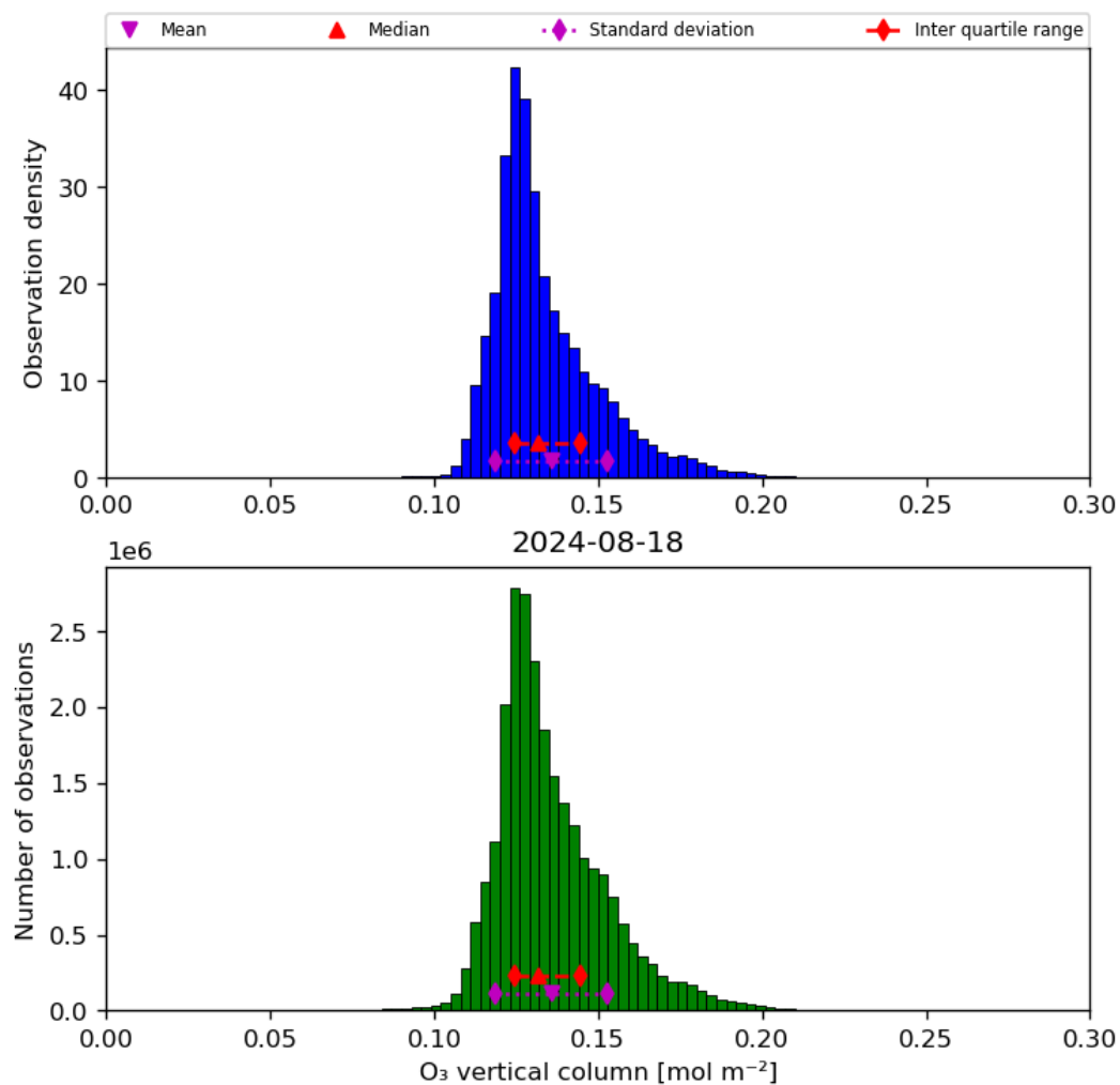
Figure 21: Histogram of “O 3 vertical column” for 2024-08-17 to 2024-08-19
