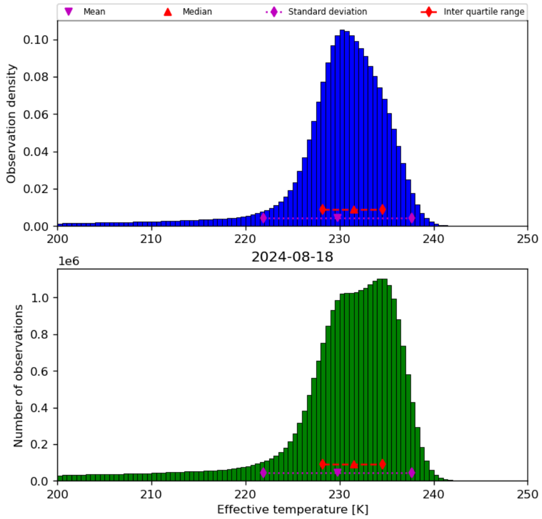
Figure 24: Histogram of “Effective temperature” for 2024-08-17 to 2024-08-19
