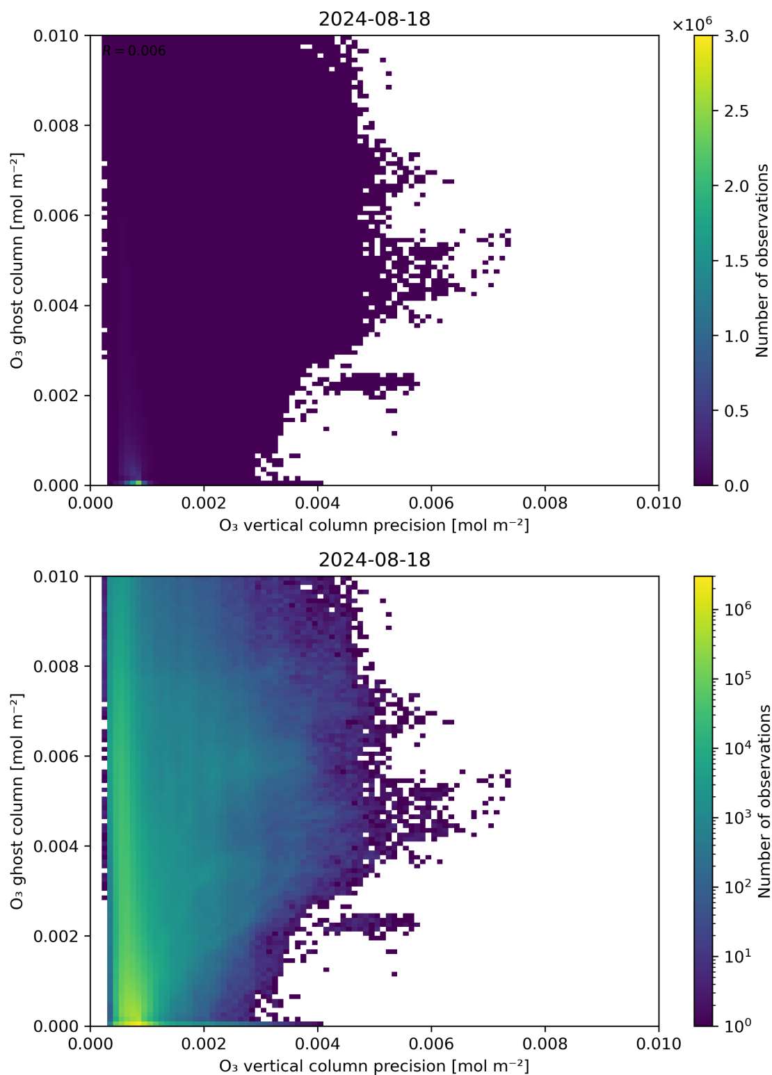
Figure 43: Scatter density plot of “O 3 vertical column precision” against “O 3 ghost column” for 2024-08-17 to 2024-08-19.
