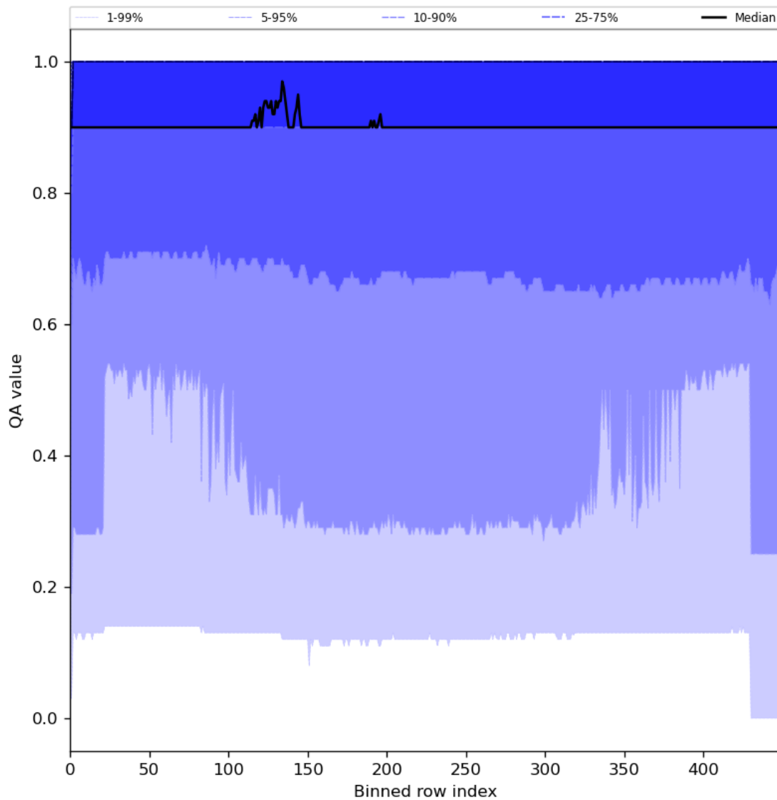
Figure 27: Along track statistics of “QA value” for 2024-08-17 to 2024-08-19
