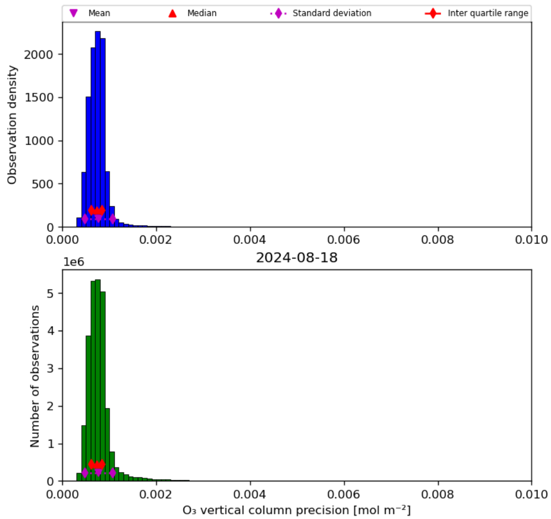
Figure 22: Histogram of “O 3 vertical column precision” for 2024-08-17 to 2024-08-19
