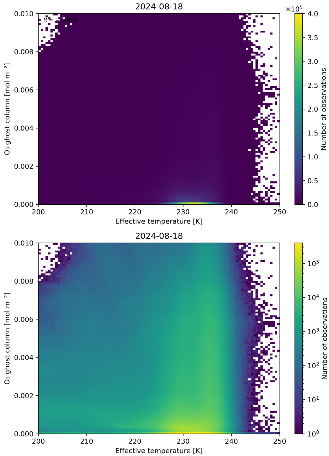
Figure 38: Scatter density plot of “Effective temperature” against “O 3 ghost column” for 2024-08-17 to 2024-08-19.
