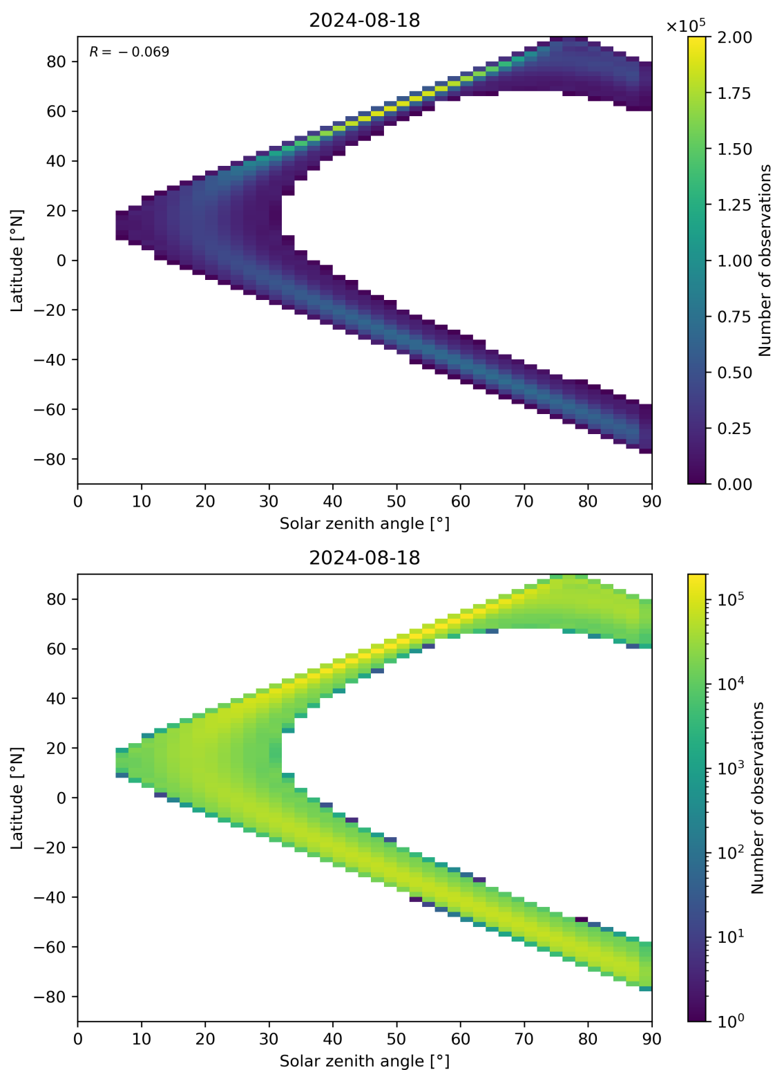
Figure 44: Scatter density plot of “Solar zenith angle” against “Latitude” for 2024-08-17 to 2024-08-19.
