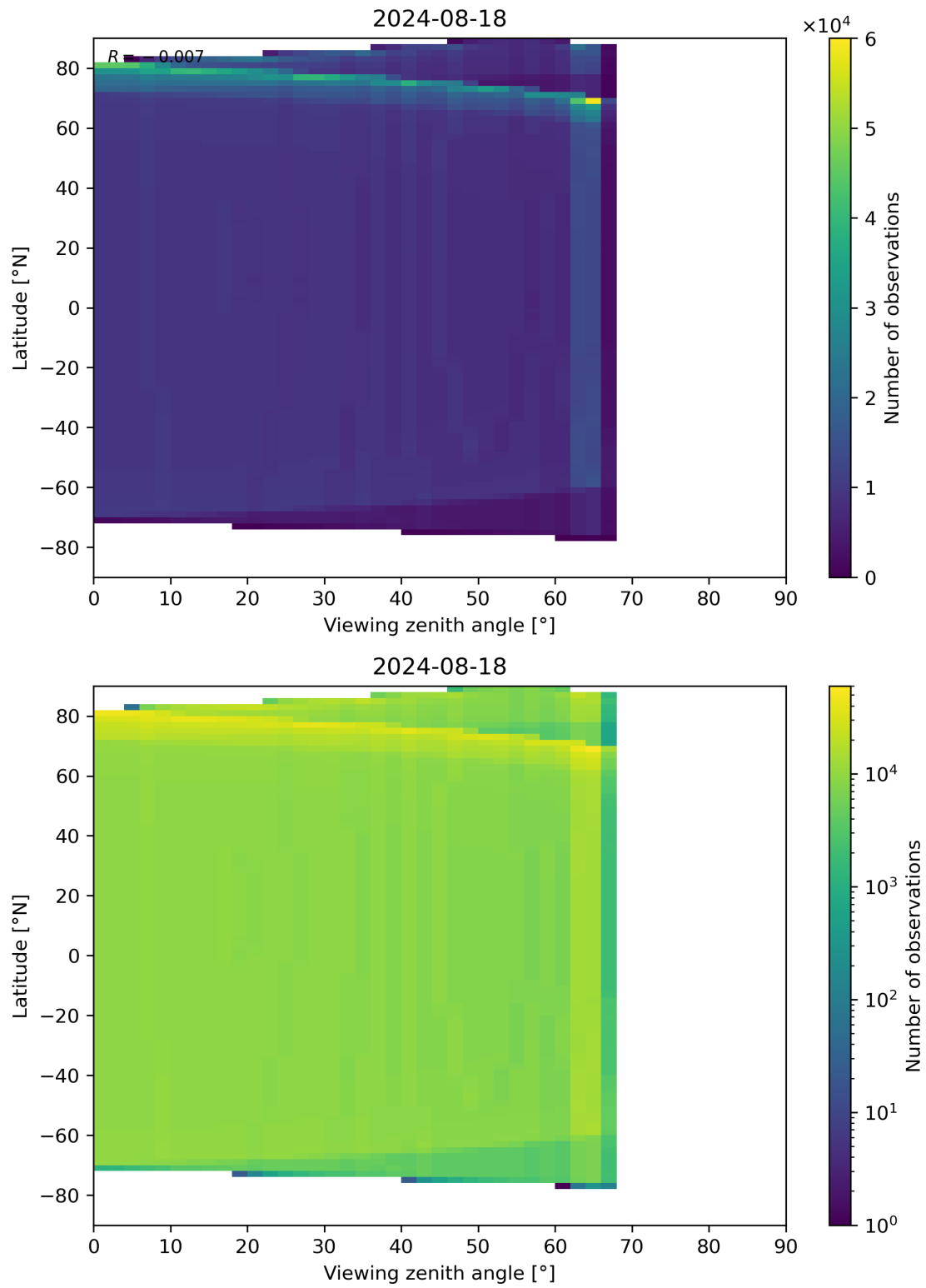
Figure 49: Scatter density plot of “Viewing zenith angle” against “Latitude” for 2024-08-17 to 2024-08-19.
