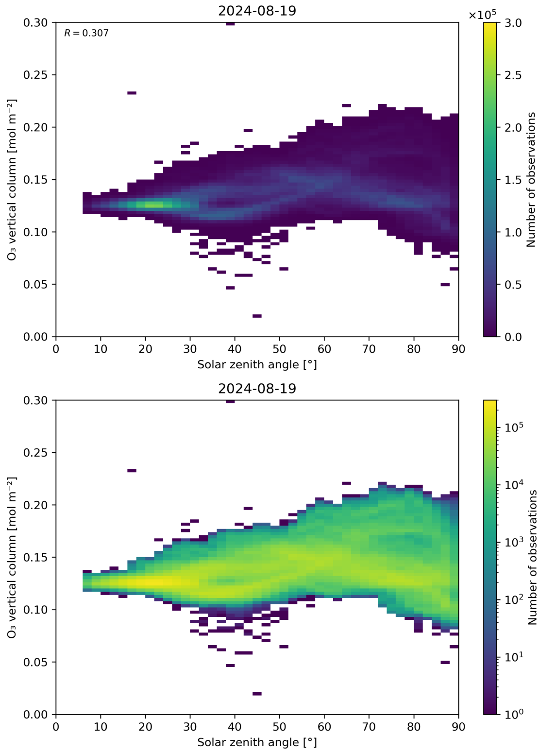
Figure 47: Scatter density plot of “Solar zenith angle” against “O 3 vertical column” for 2024-08-18 to 2024-08-20.
