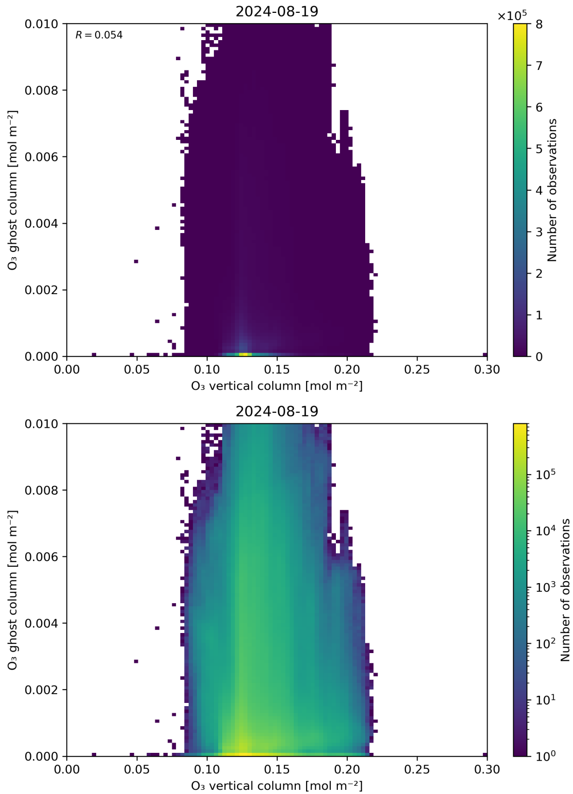
Figure 40: Scatter density plot of “O 3 vertical column” against “O 3 ghost column” for 2024-08-18 to 2024-08-20.
