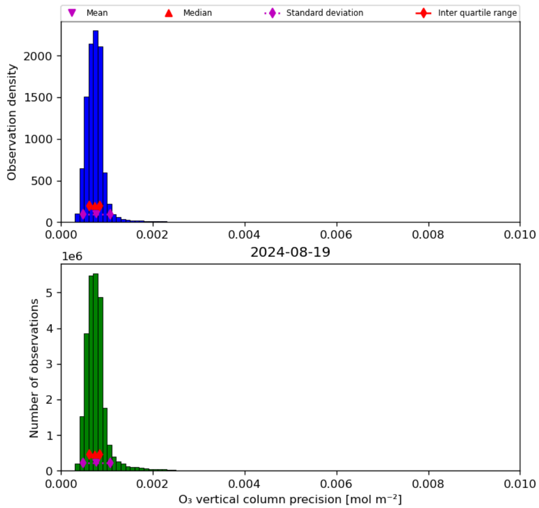
Figure 22: Histogram of “O 3 vertical column precision” for 2024-08-18 to 2024-08-20
