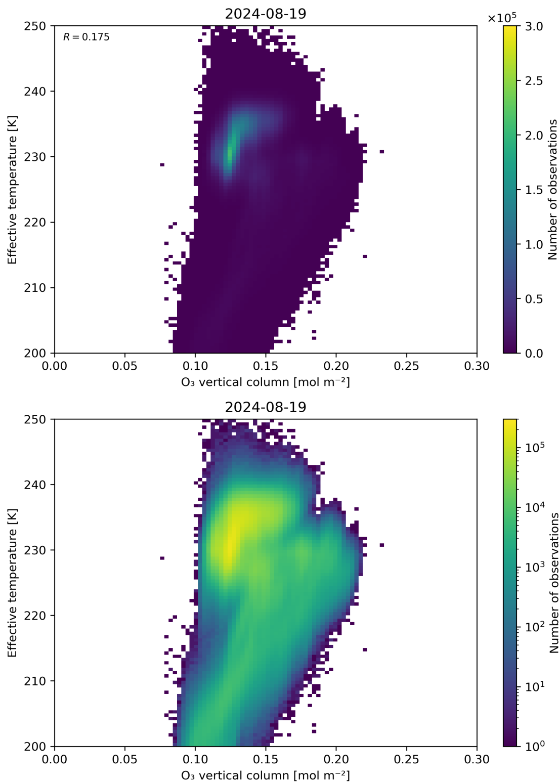
Figure 39: Scatter density plot of “O 3 vertical column” against “Effective temperature” for 2024-08-18 to 2024-08-20.
