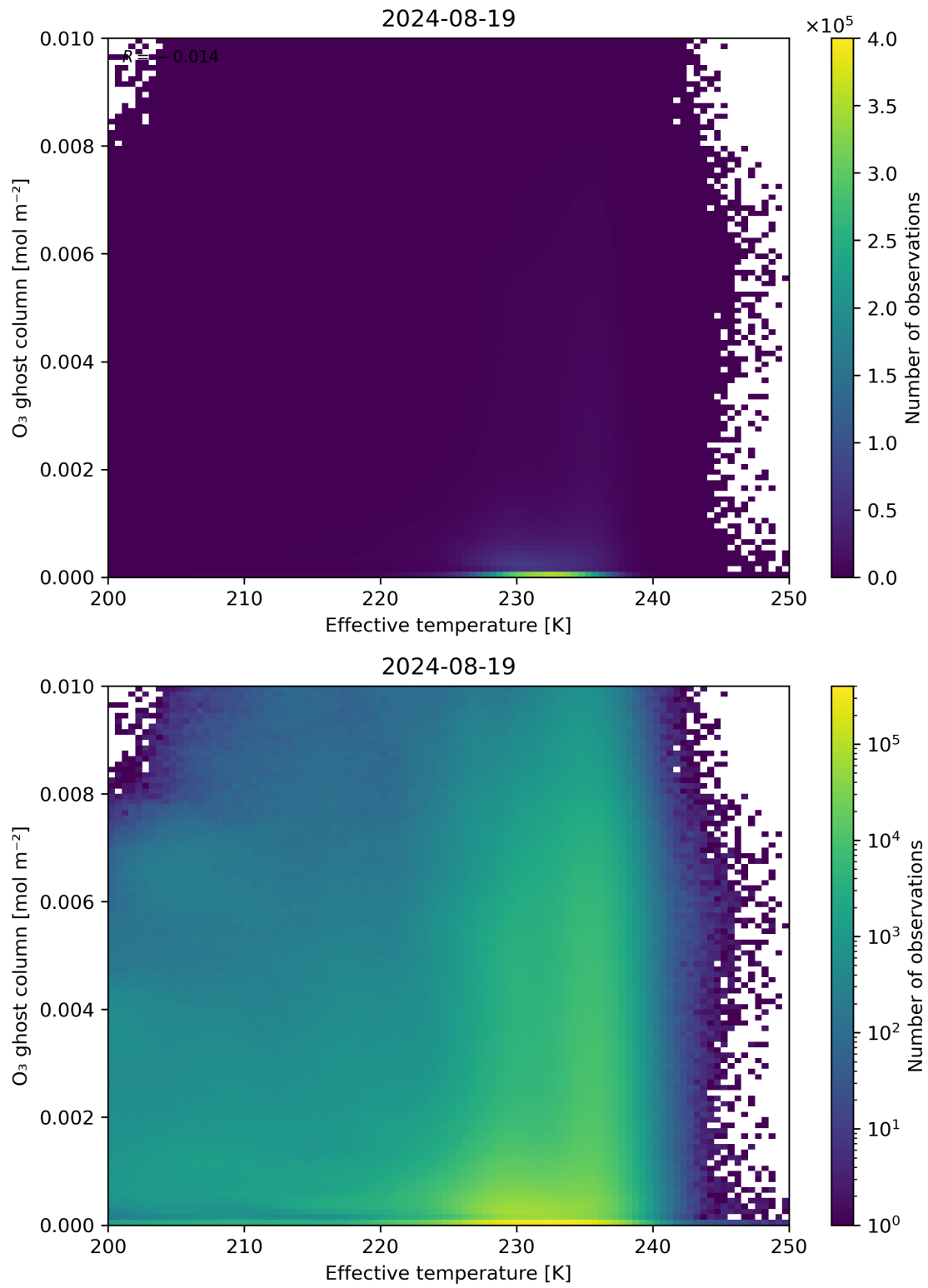
Figure 38: Scatter density plot of “Effective temperature” against “O 3 ghost column” for 2024-08-18 to 2024-08-20.
