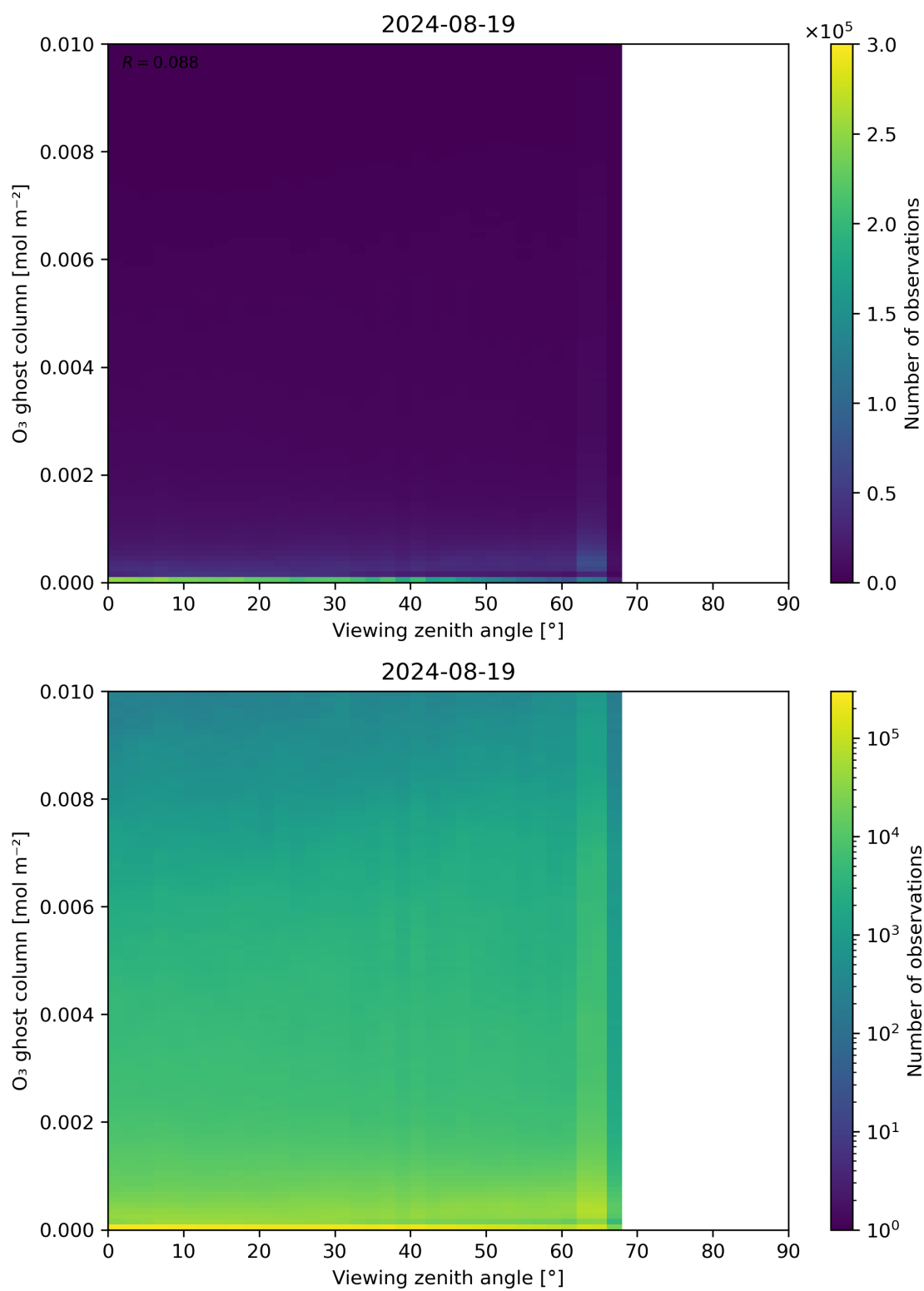
Figure 51: Scatter density plot of “Viewing zenith angle” against “O 3 ghost column” for 2024-08-18 to 2024-08-20.
