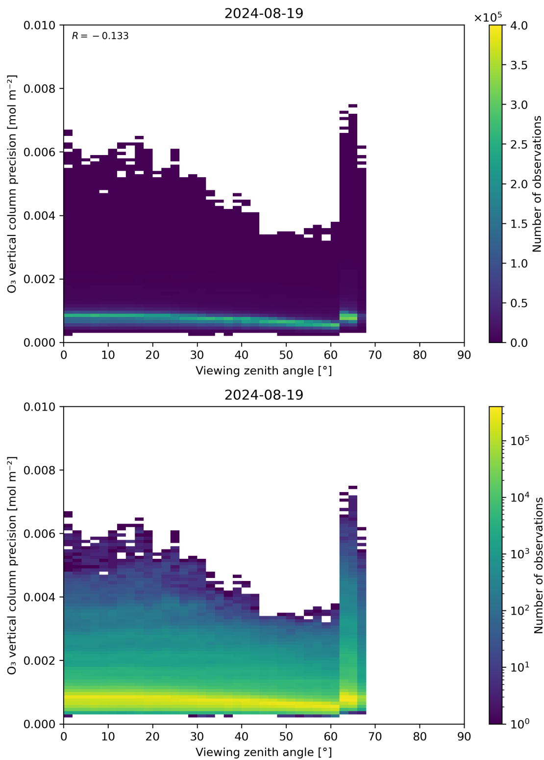
Figure 53: Scatter density plot of “Viewing zenith angle” against “O 3 vertical column precision” for 2024-08-18 to 2024-08-20.
