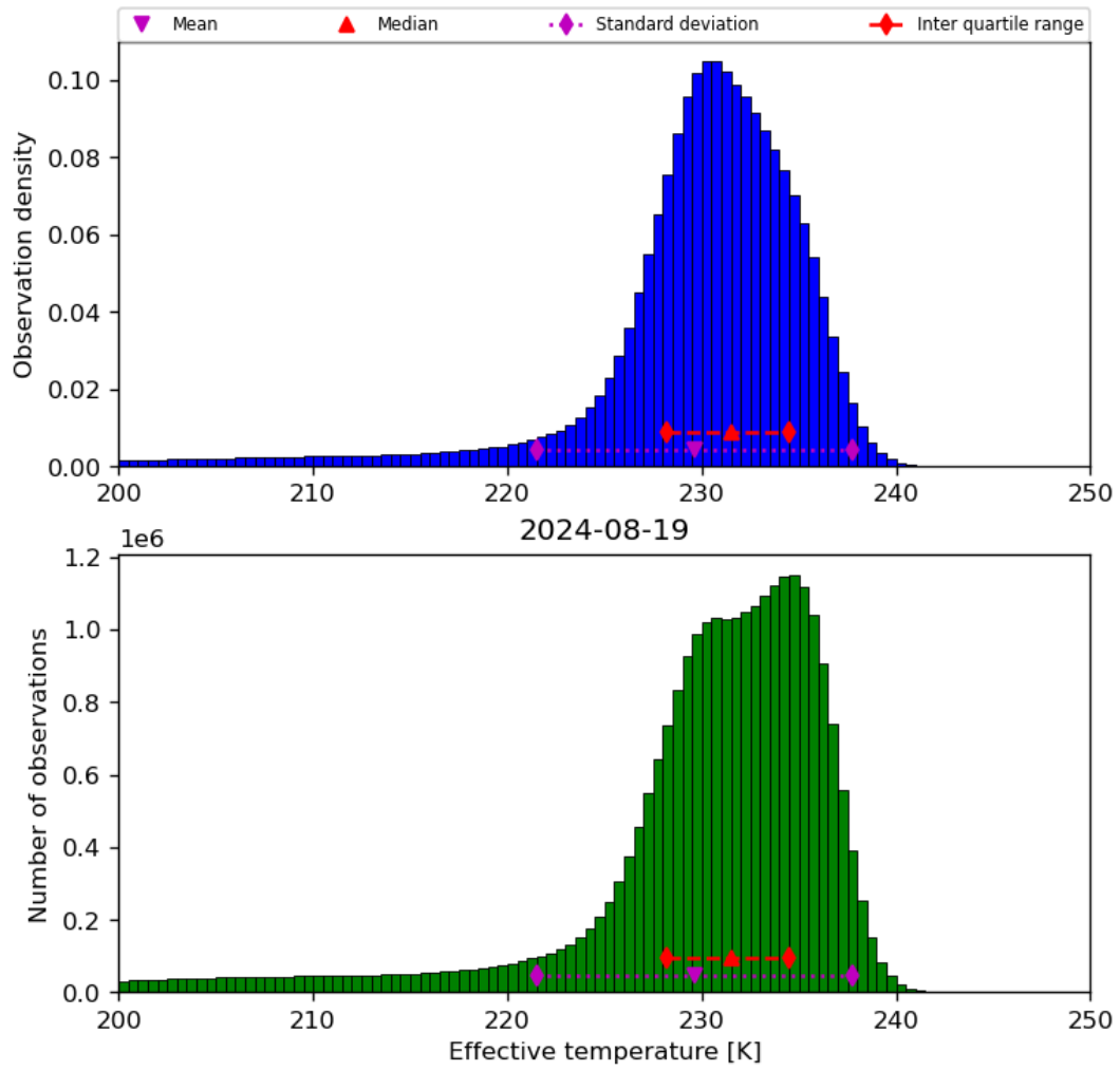
Figure 24: Histogram of “Effective temperature” for 2024-08-18 to 2024-08-20
