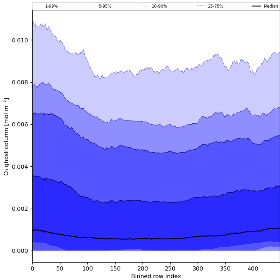
Figure 32: Along track statistics of “O 3 ghost column” for 2024-08-18 to 2024-08-20
