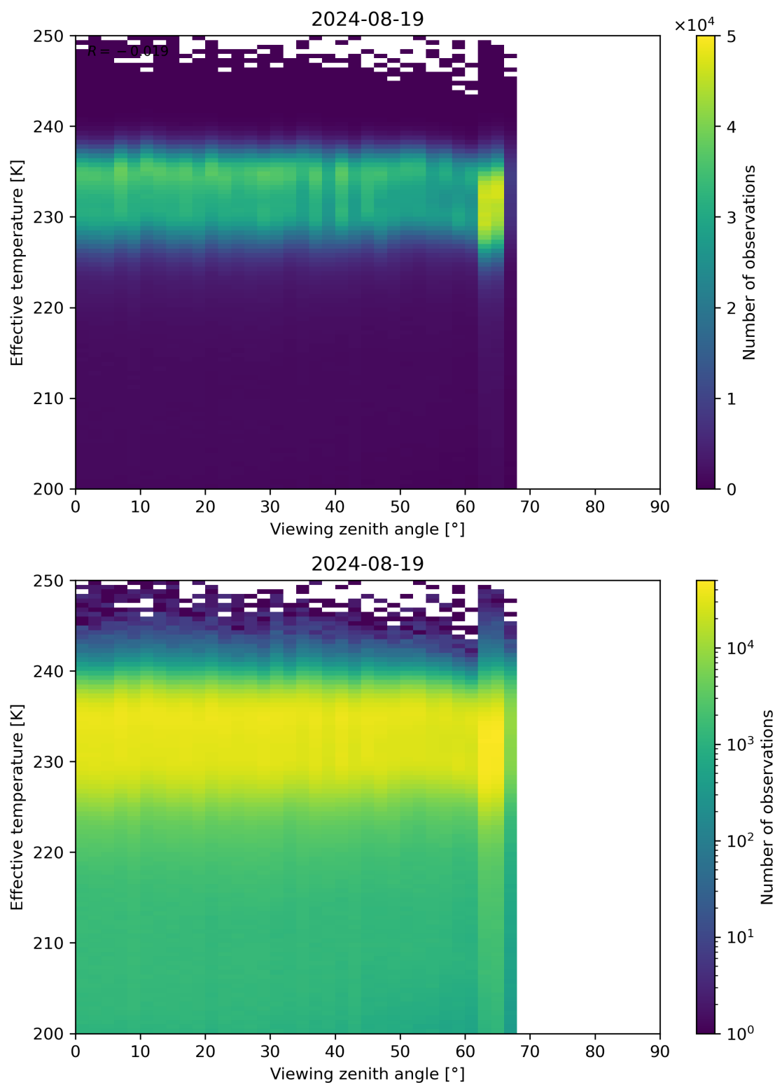
Figure 50: Scatter density plot of “Viewing zenith angle” against “Effective temperature” for 2024-08-18 to 2024-08-20.
