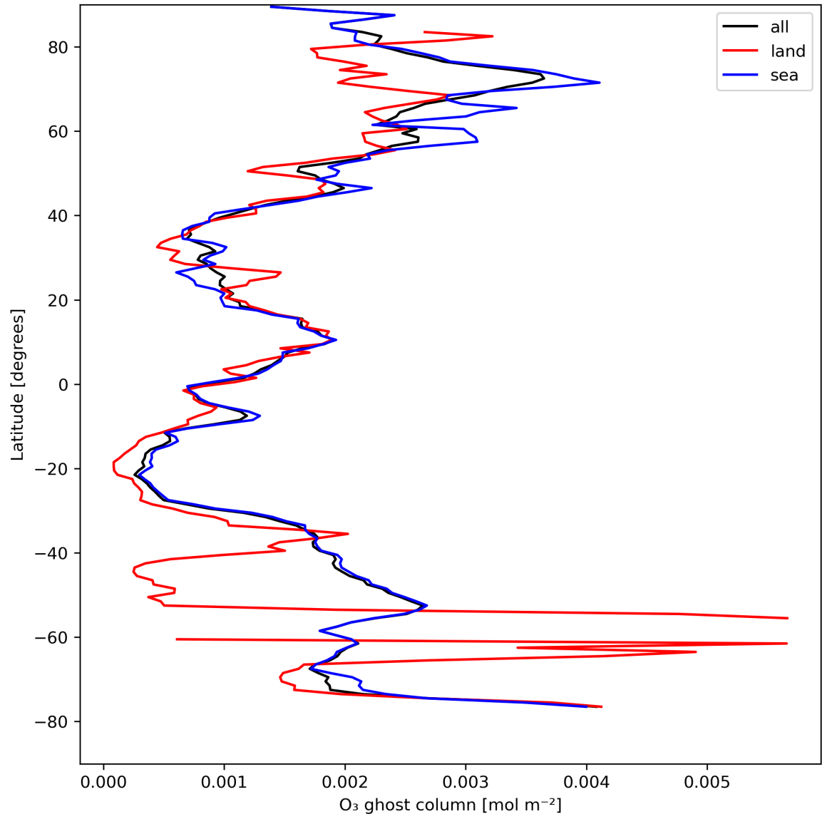
Figure 18: Zonal average of “O 3 ghost column” for 2024-08-18 to 2024-08-20.
