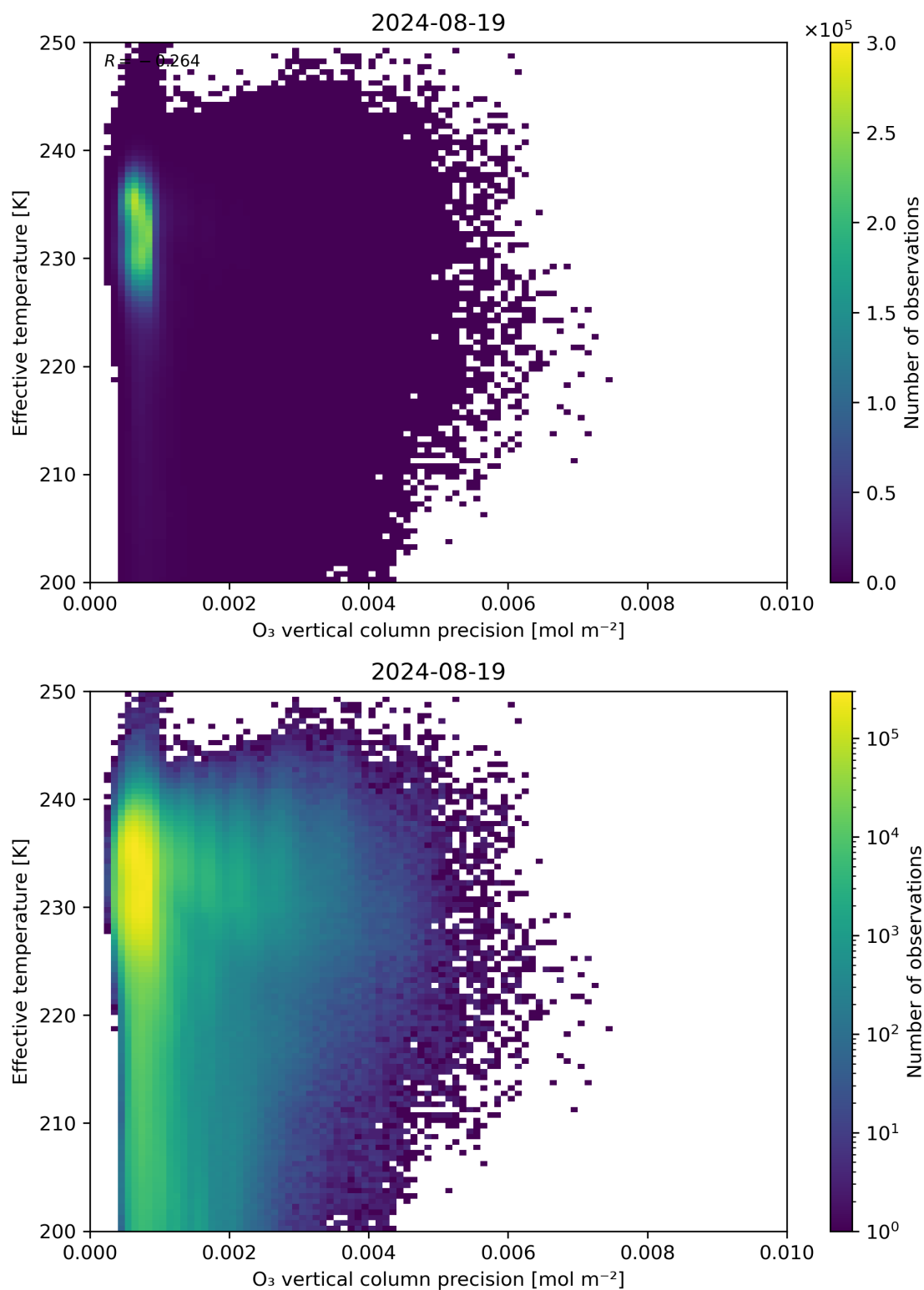
Figure 42: Scatter density plot of “O 3 vertical column precision” against “Effective temperature” for 2024-08-18 to 2024-08-20.
