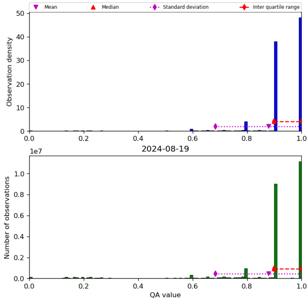
Figure 20: Histogram of “QA value” for 2024-08-18 to 2024-08-20
