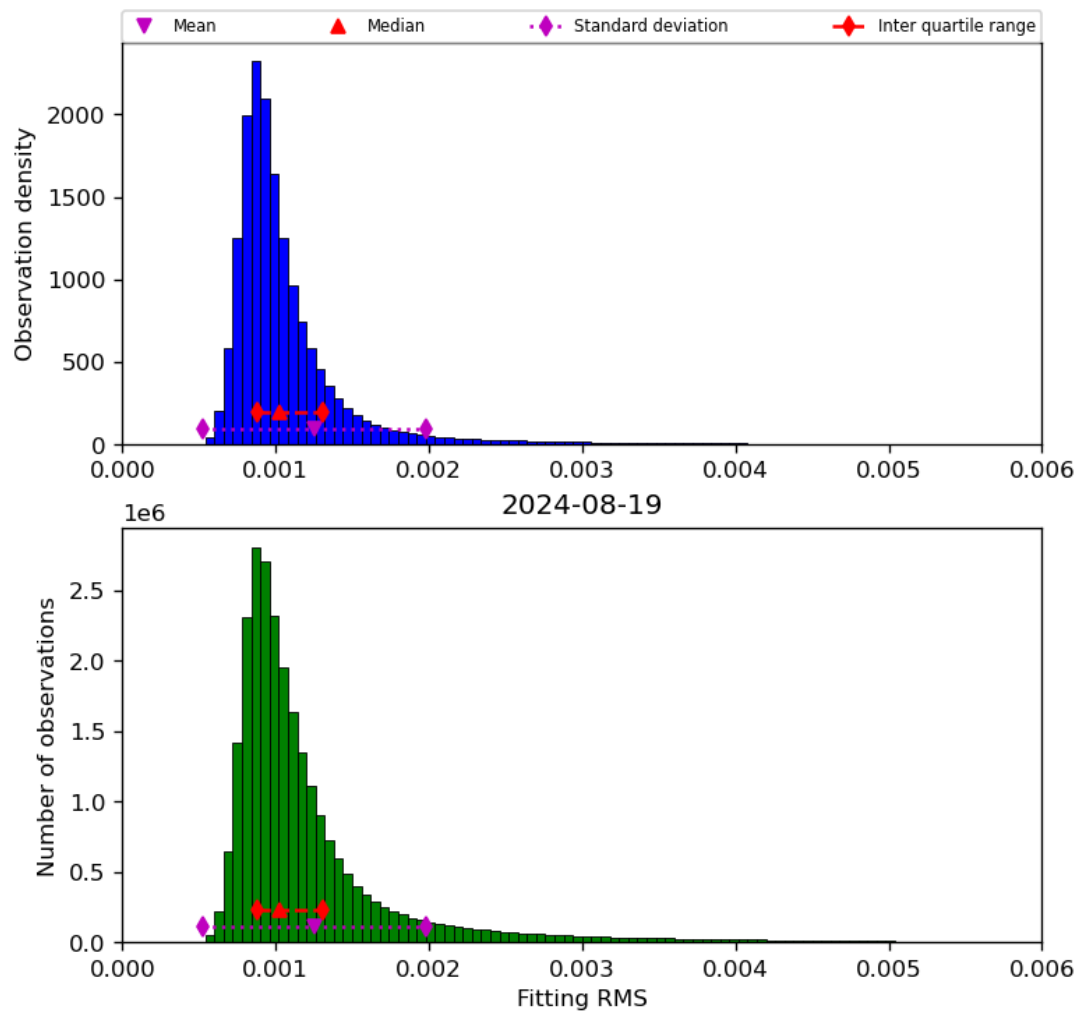
Figure 23: Histogram of “Fitting RMS” for 2024-08-18 to 2024-08-20
