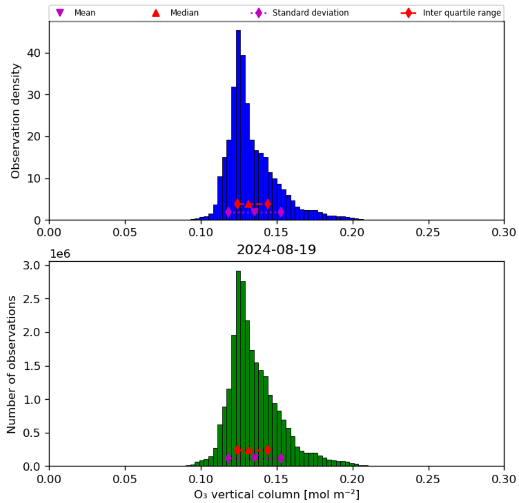
Figure 21: Histogram of “O 3 vertical column” for 2024-08-18 to 2024-08-20
