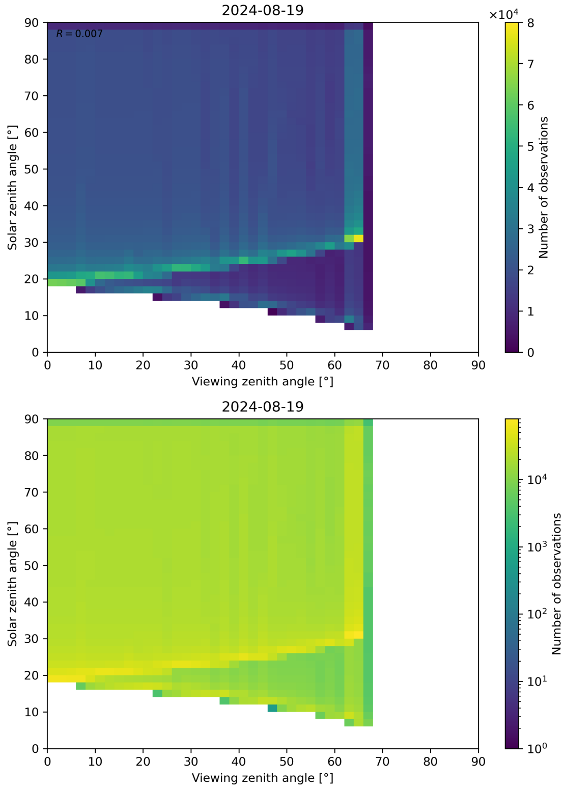
Figure 54: Scatter density plot of “Viewing zenith angle” against “Solar zenith angle” for 2024-08-18 to 2024-08-20.
