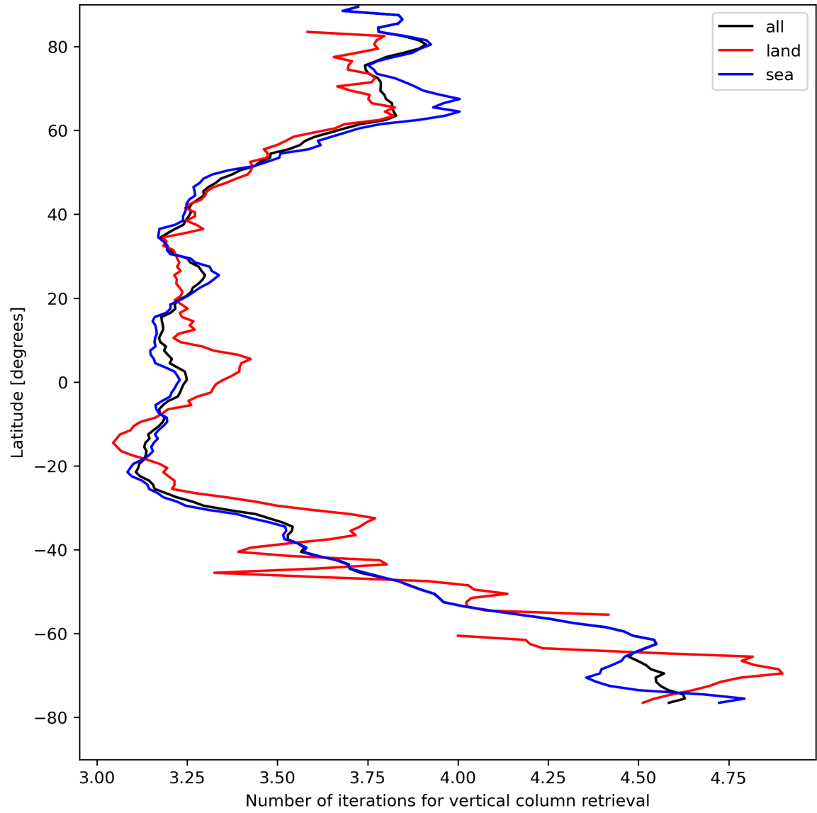
Figure 19: Zonal average of “Number of iterations for vertical column retrieval” for 2024-08-18 to 2024-08-20.
