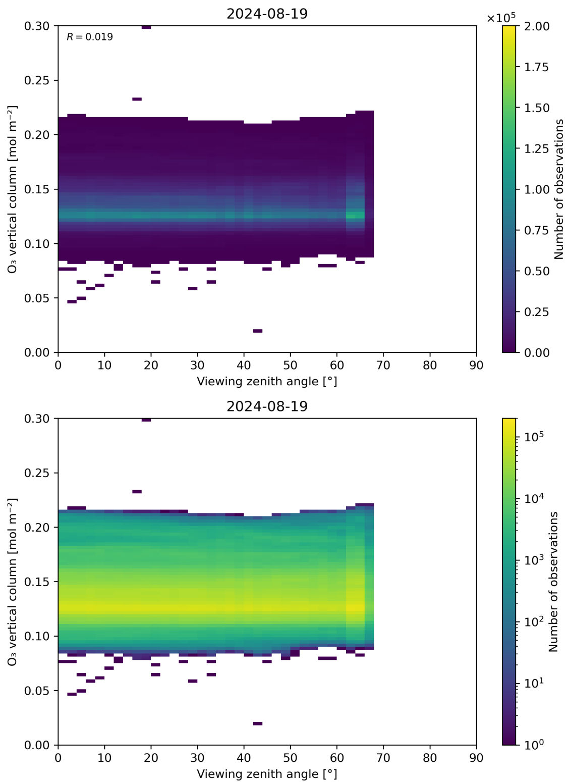
Figure 52: Scatter density plot of “Viewing zenith angle” against “O 3 vertical column” for 2024-08-18 to 2024-08-20.
