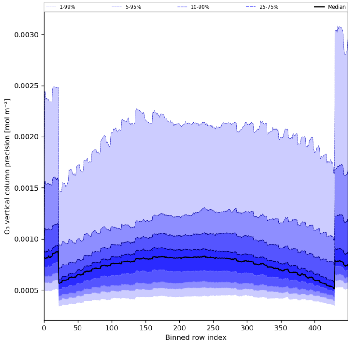
Figure 29: Along track statistics of “O 3 vertical column precision” for 2024-08-18 to 2024-08-20
