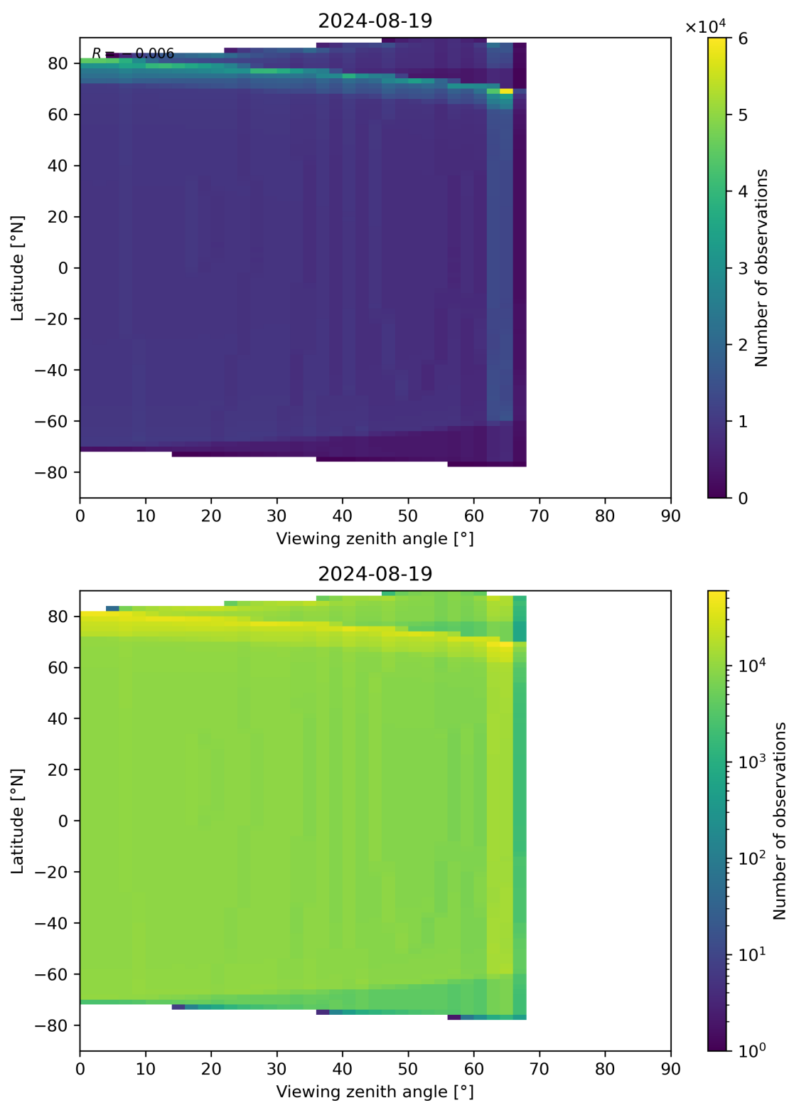
Figure 49: Scatter density plot of “Viewing zenith angle” against “Latitude” for 2024-08-18 to 2024-08-20.
