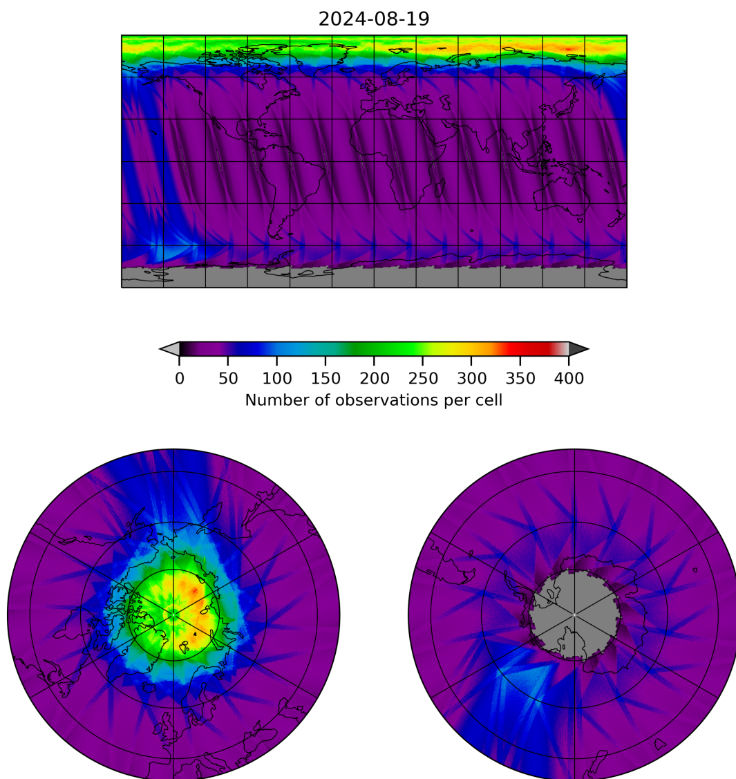
Figure 12: Map of the number of observations for 2024-08-18 to 2024-08-20
