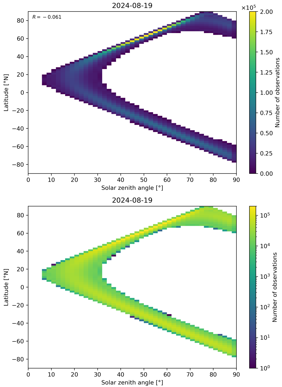
Figure 44: Scatter density plot of “Solar zenith angle” against “Latitude” for 2024-08-18 to 2024-08-20.
