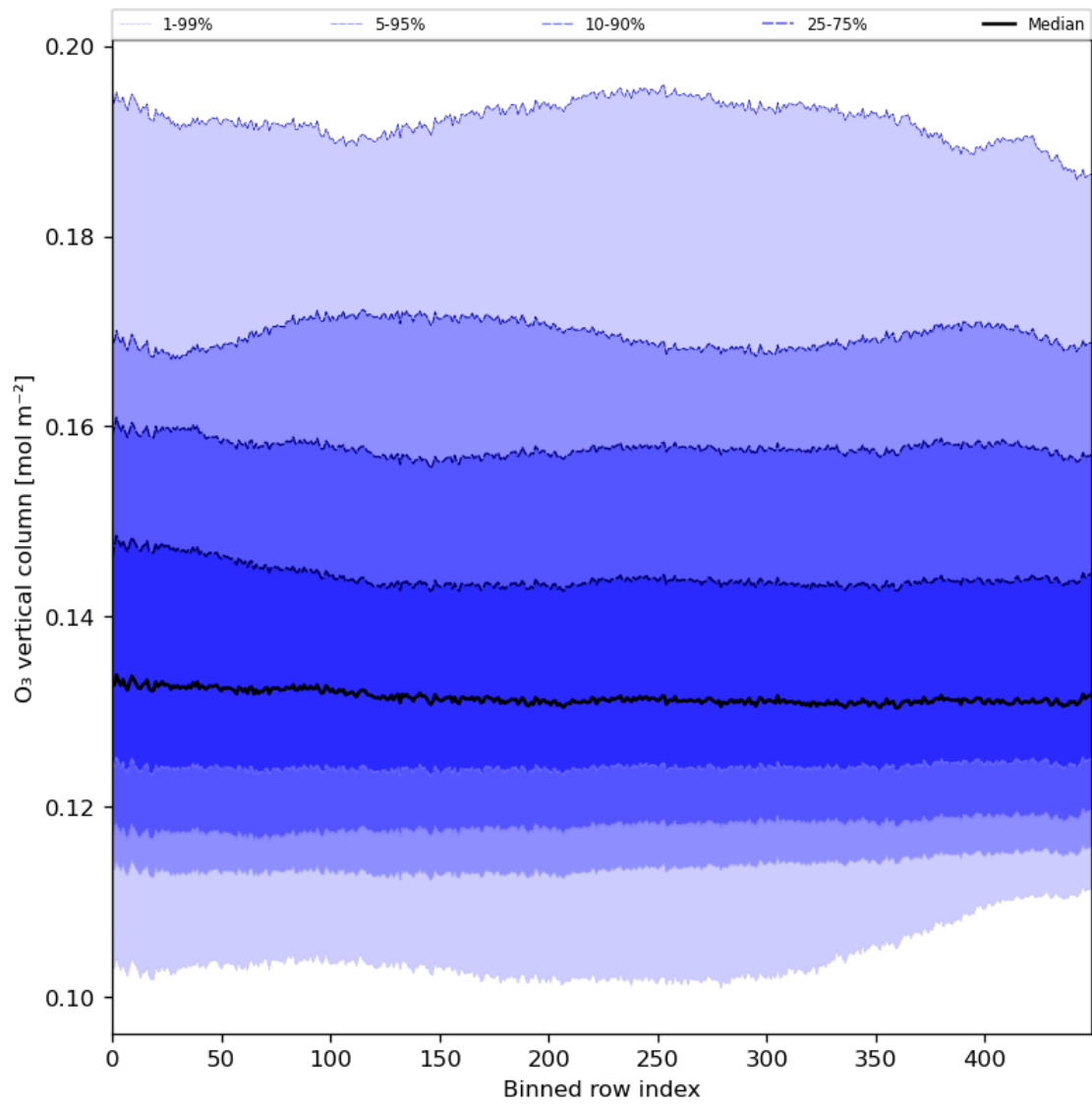
Figure 28: Along track statistics of “O 3 vertical column” for 2024-08-18 to 2024-08-20
