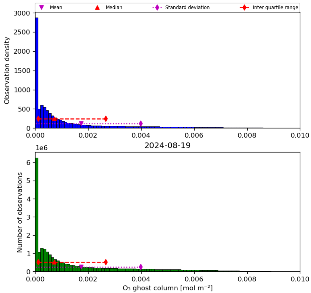
Figure 25: Histogram of “O 3 ghost column” for 2024-08-18 to 2024-08-20
