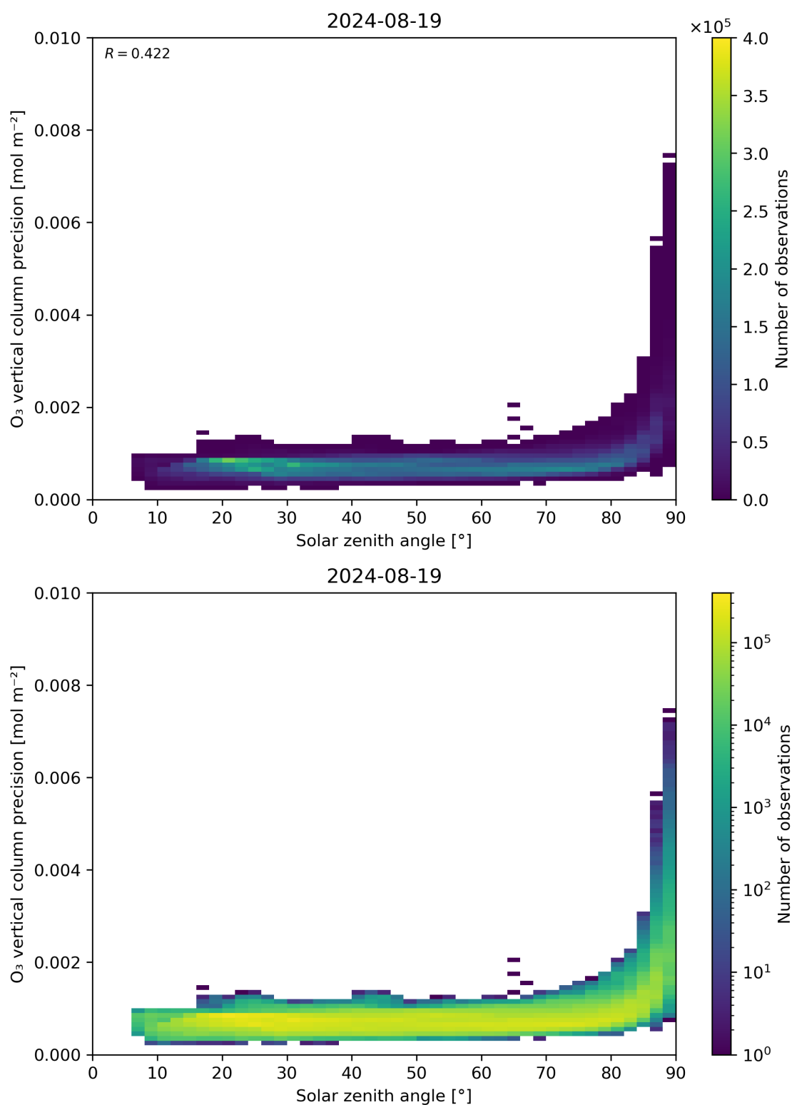
Figure 48: Scatter density plot of “Solar zenith angle” against “O 3 vertical column precision” for 2024-08-18 to 2024-08-20.
