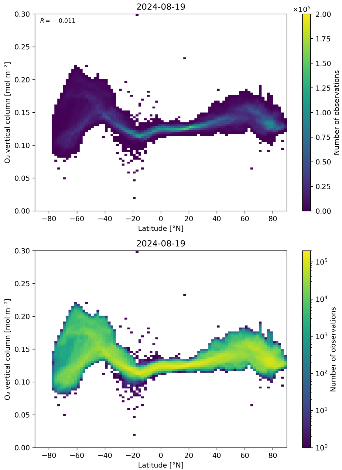
Figure 36: Scatter density plot of “Latitude” against “O 3 vertical column” for 2024-08-18 to 2024-08-20.
