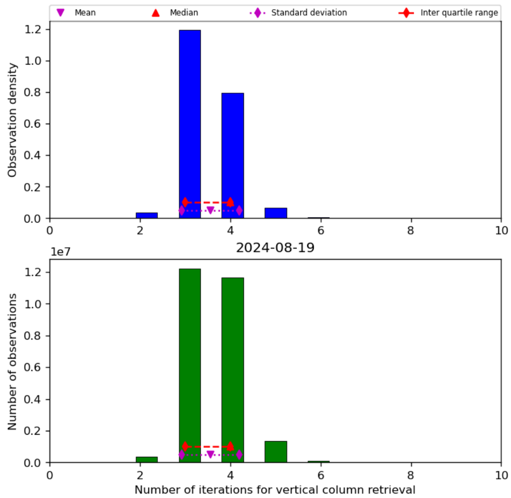
Figure 26: Histogram of “Number of iterations for vertical column retrieval” for 2024-08-18 to 2024-08-20
