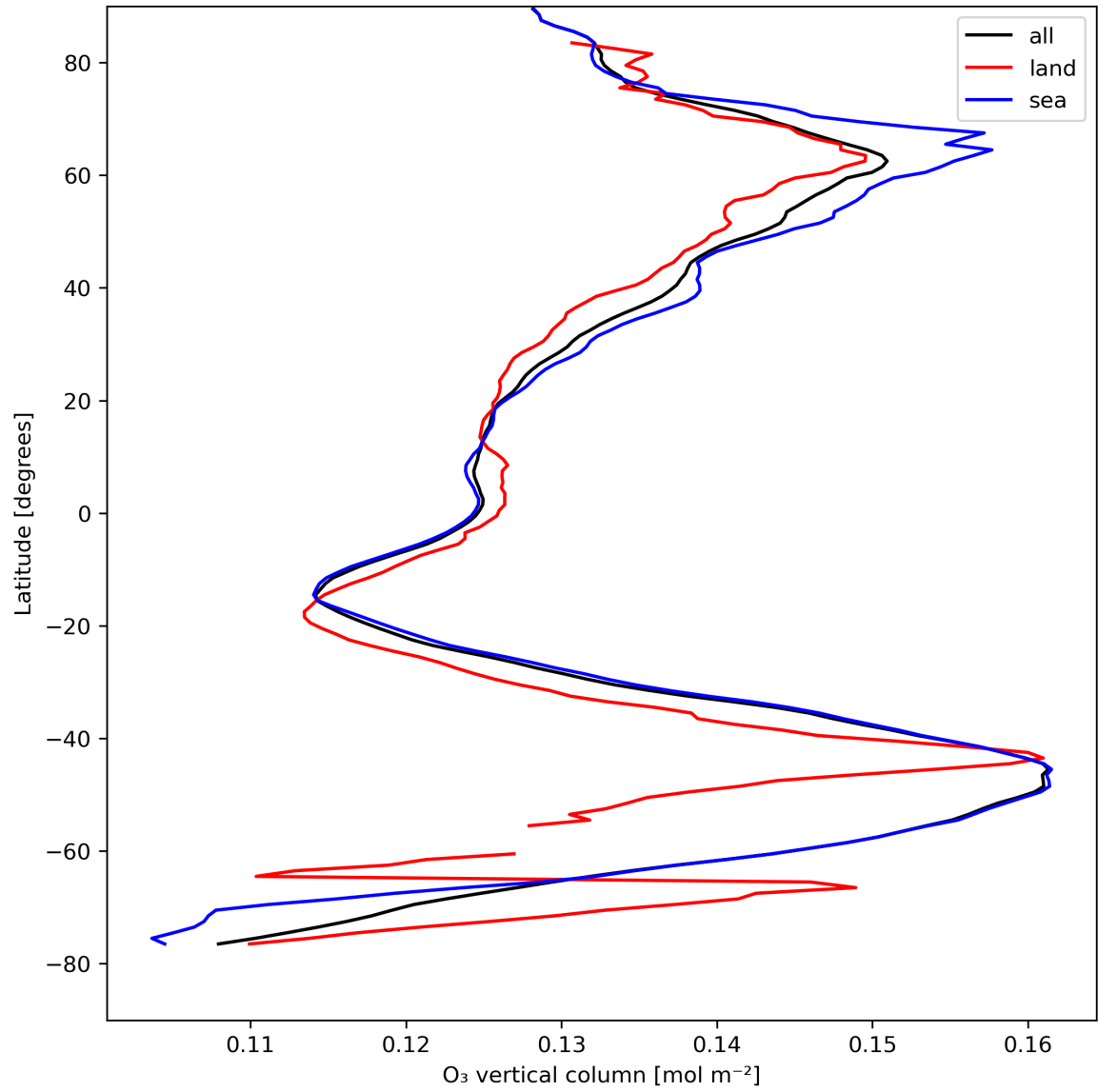
Figure 14: Zonal average of “O 3 vertical column” for 2024-08-18 to 2024-08-20.
