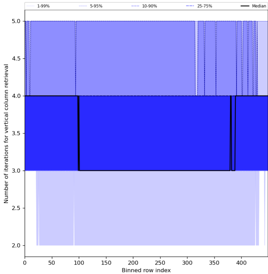
Figure 33: Along track statistics of “Number of iterations for vertical column retrieval” for 2024-08-18 to 2024-08-20
