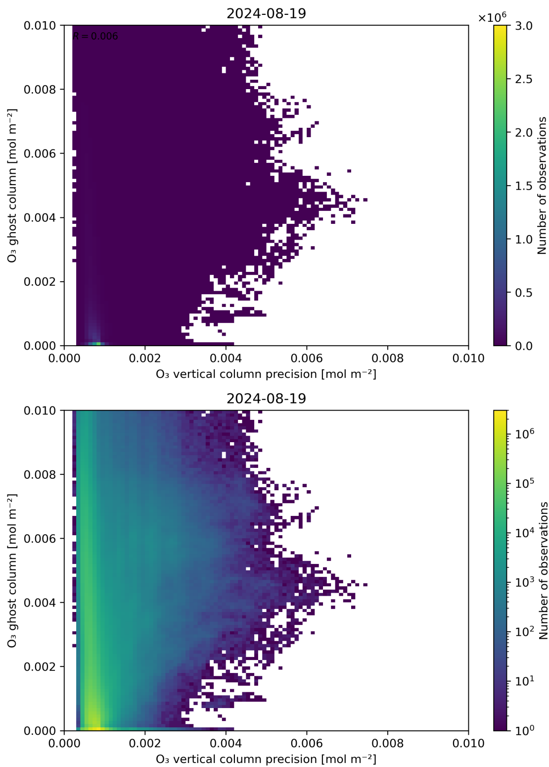
Figure 43: Scatter density plot of “O 3 vertical column precision” against “O 3 ghost column” for 2024-08-18 to 2024-08-20.
