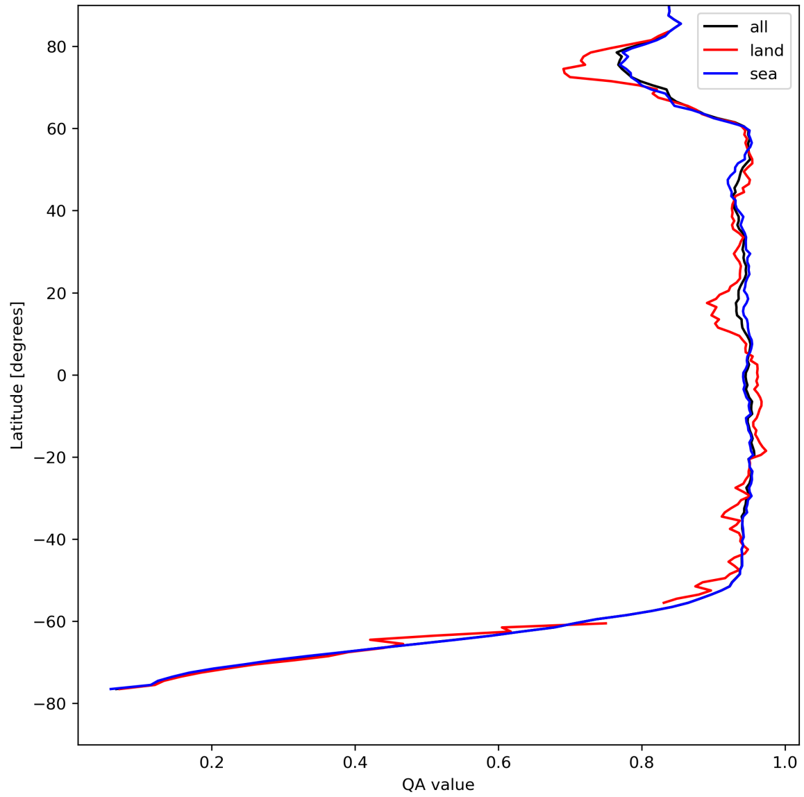
Figure 13: Zonal average of “QA value” for 2024-08-18 to 2024-08-20.
