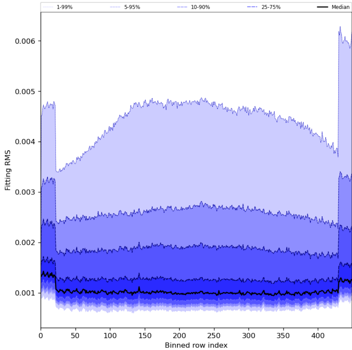
Figure 30: Along track statistics of “Fitting RMS” for 2024-08-18 to 2024-08-20
