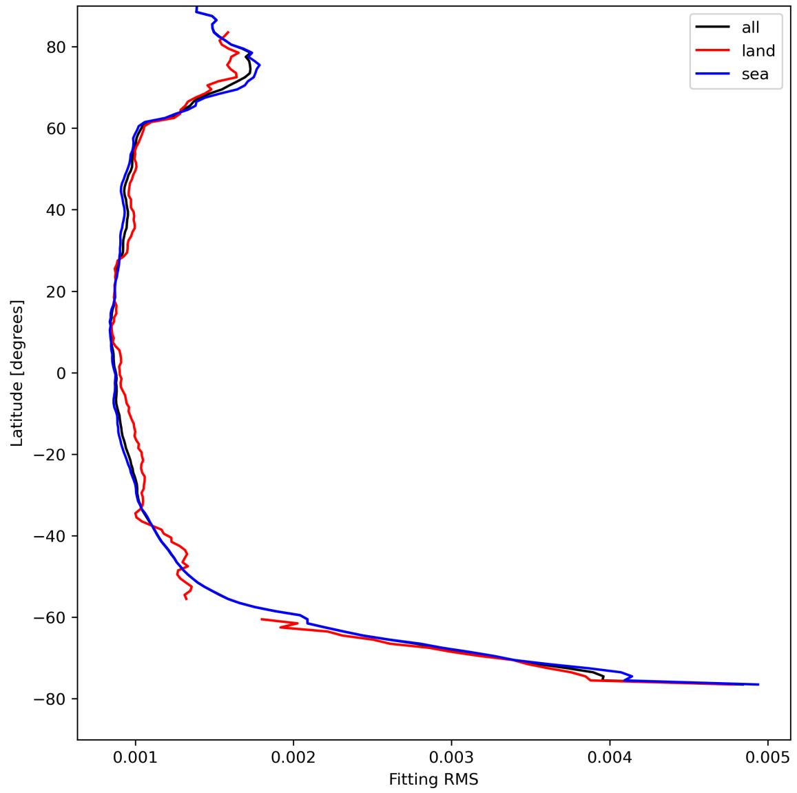
Figure 16: Zonal average of “Fitting RMS” for 2024-08-18 to 2024-08-20.
