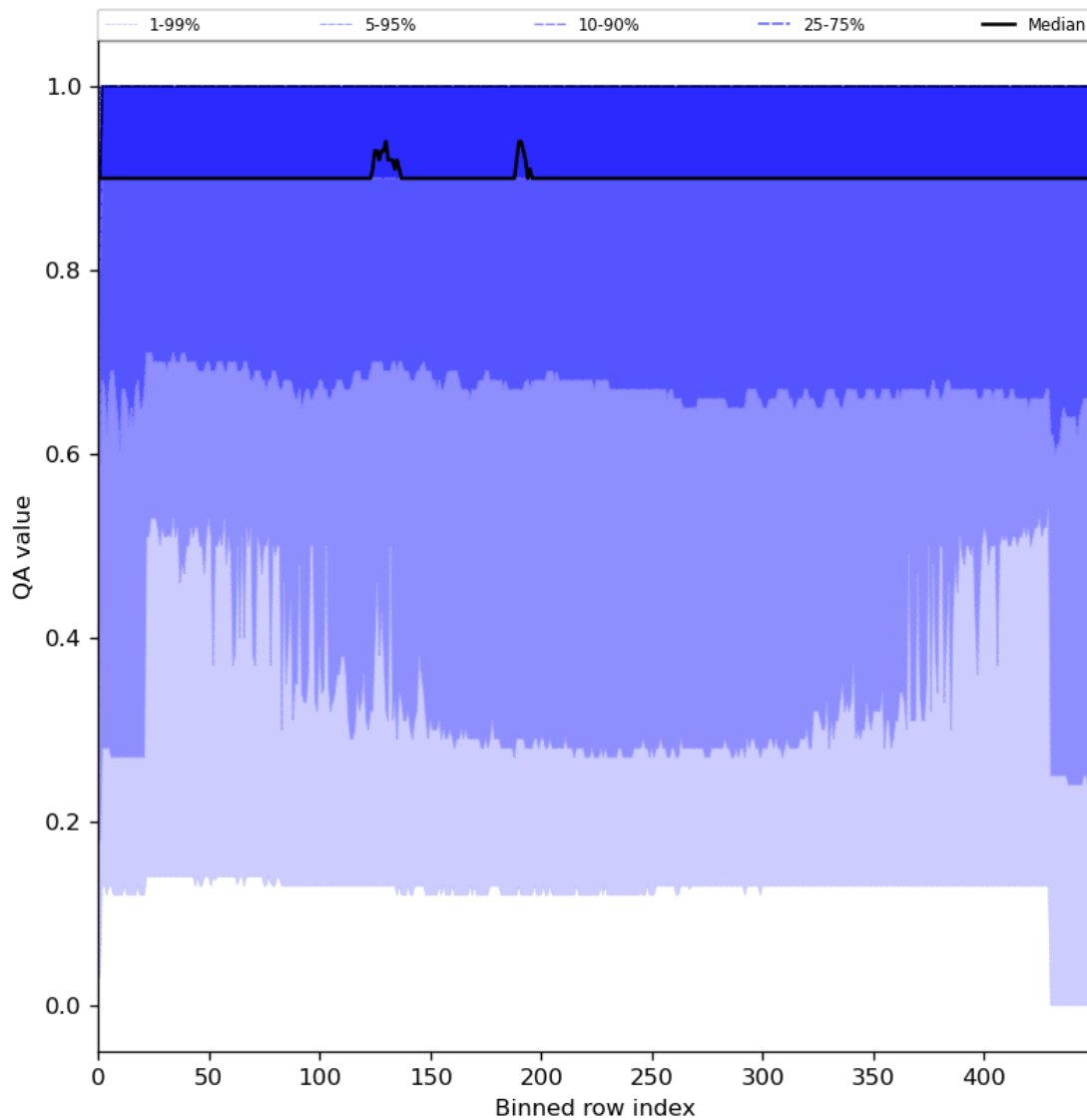
Figure 27: Along track statistics of “QA value” for 2024-08-18 to 2024-08-20
