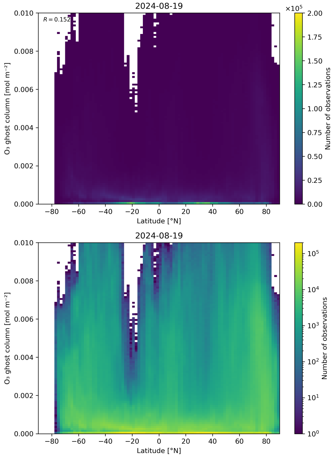
Figure 35: Scatter density plot of “Latitude” against “O 3 ghost column” for 2024-08-18 to 2024-08-20.
