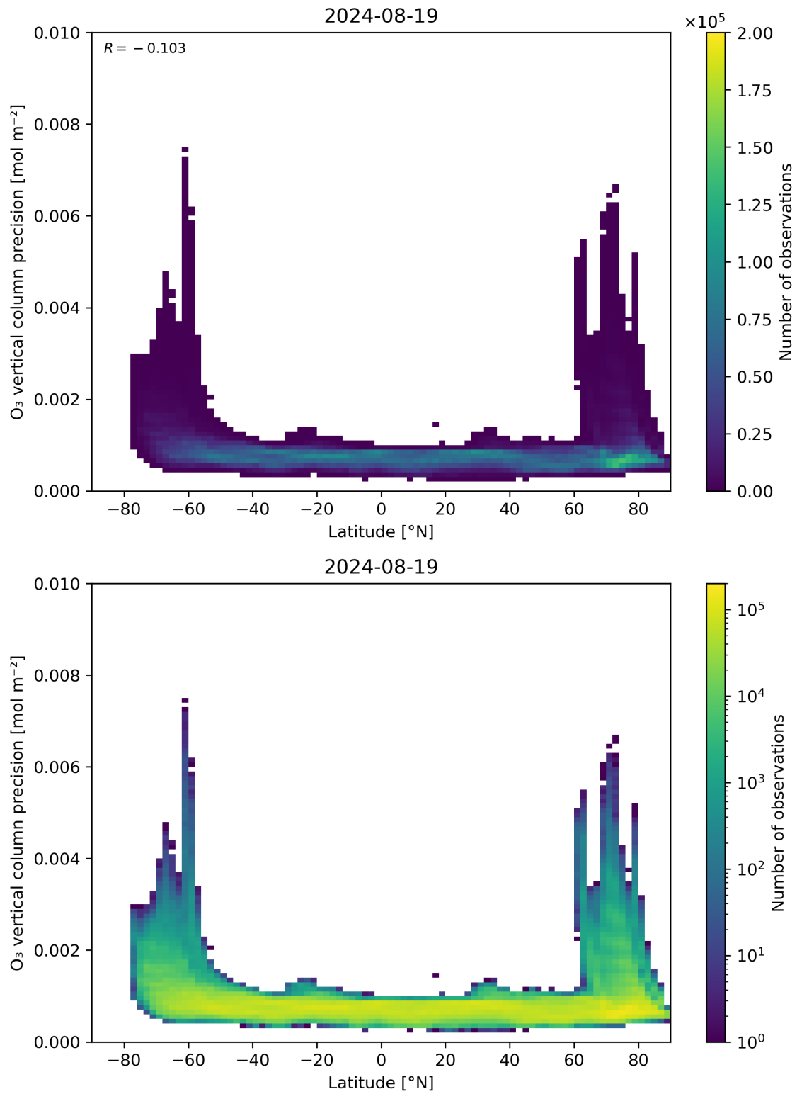
Figure 37: Scatter density plot of “Latitude” against “O 3 vertical column precision” for 2024-08-18 to 2024-08-20.
