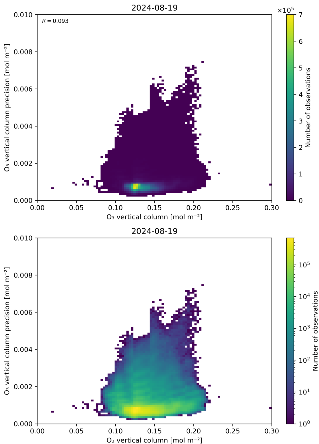
Figure 41: Scatter density plot of “O 3 vertical column” against “O 3 vertical column precision” for 2024-08-18 to 2024-08-20.
