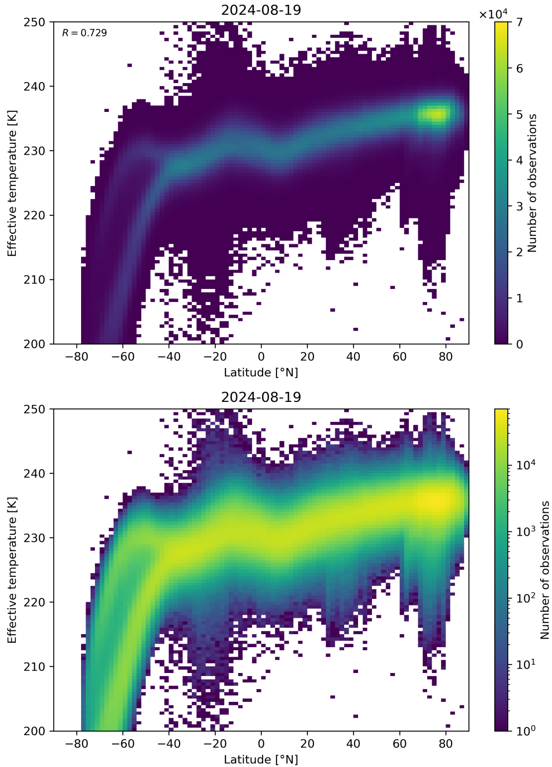
Figure 34: Scatter density plot of “Latitude” against “Effective temperature” for 2024-08-18 to 2024-08-20.
