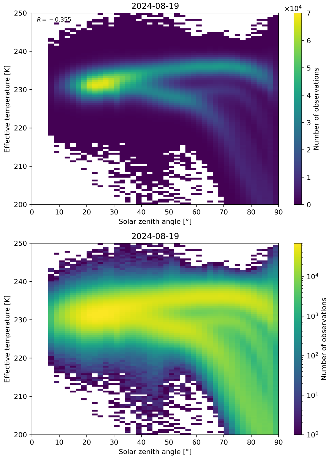
Figure 45: Scatter density plot of “Solar zenith angle” against “Effective temperature” for 2024-08-18 to 2024-08-20.
