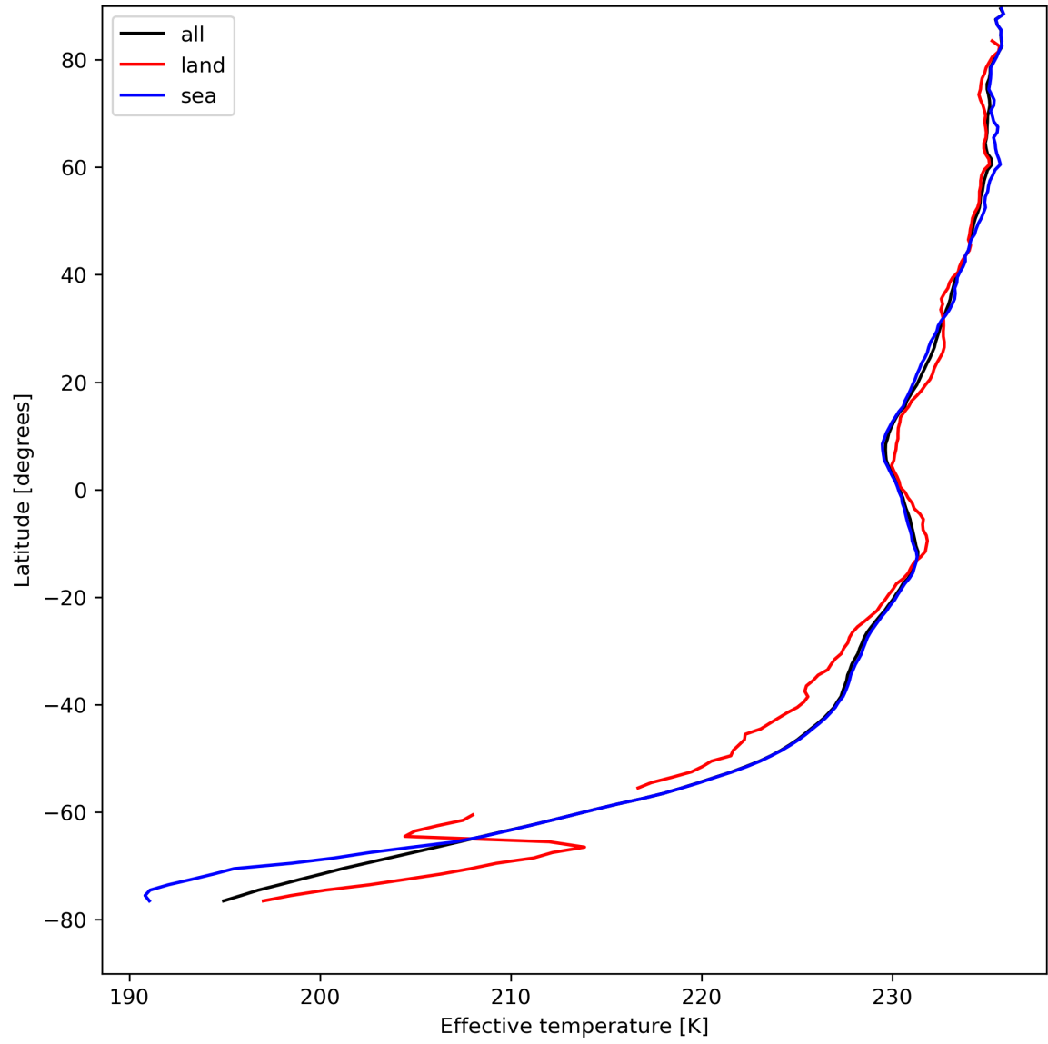
Figure 17: Zonal average of "Effective temperature" for 2024-08-18 to 2024-08-20.
