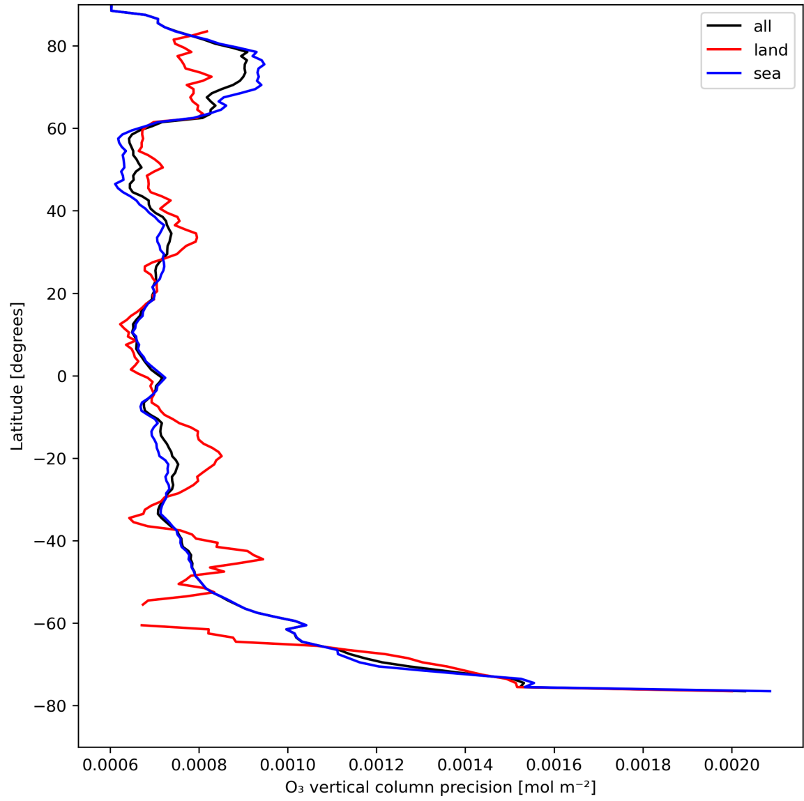
Figure 15: Zonal average of "O 3 vertical column precision" for 2024-08-18 to 2024-08-20.
