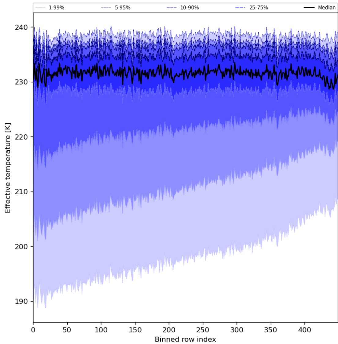
Figure 31: Along track statistics of “Effective temperature” for 2024-08-18 to 2024-08-20
