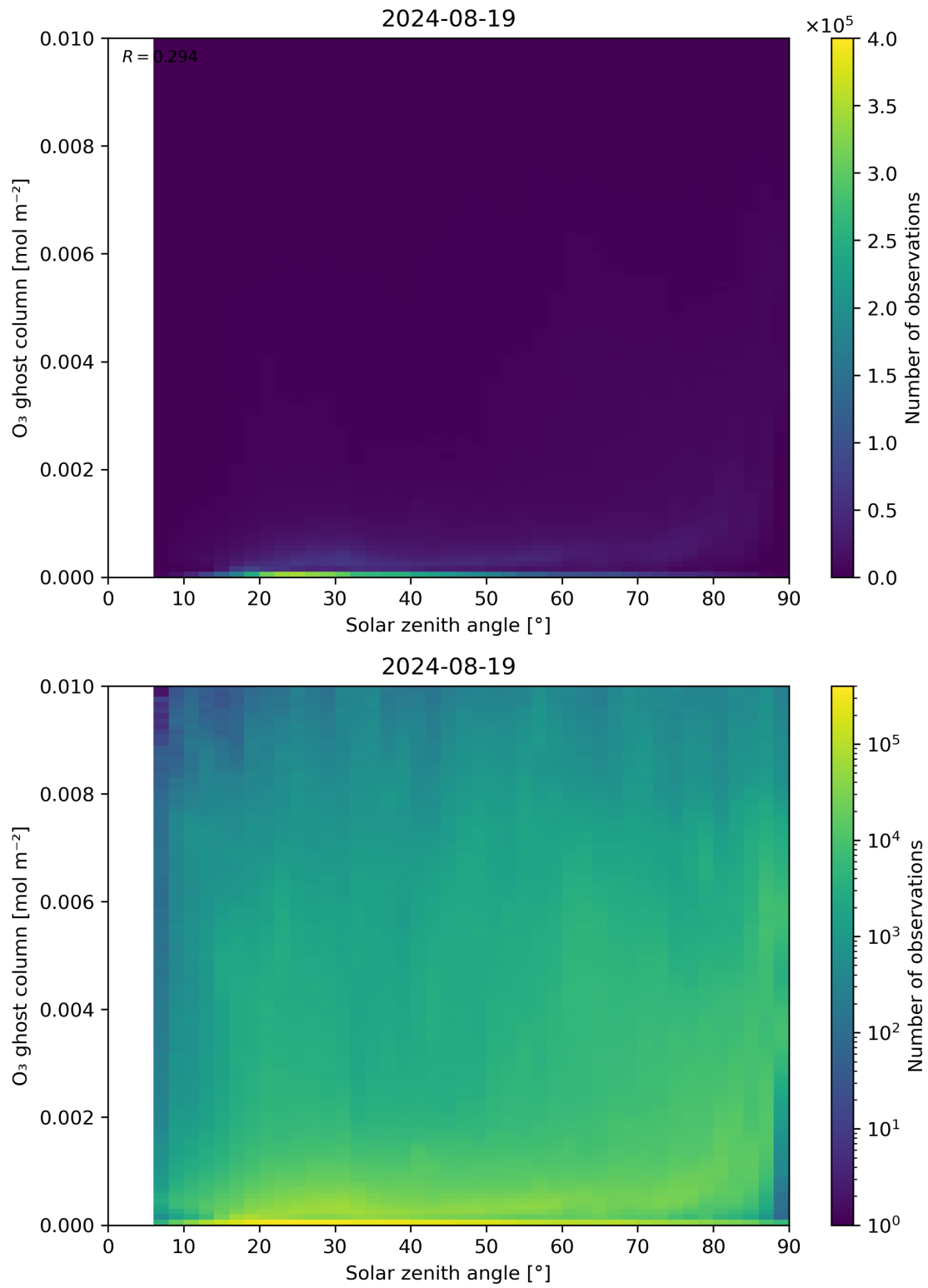
Figure 46: Scatter density plot of “Solar zenith angle” against “O 3 ghost column” for 2024-08-18 to 2024-08-20.
