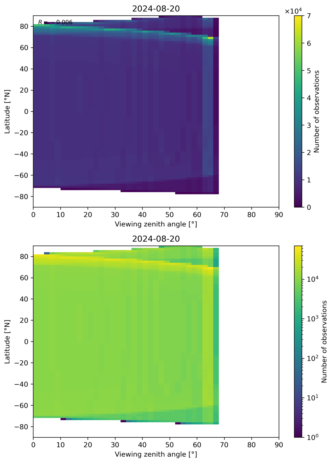
Figure 49: Scatter density plot of “Viewing zenith angle” against “Latitude” for 2024-08-19 to 2024-08-21.
