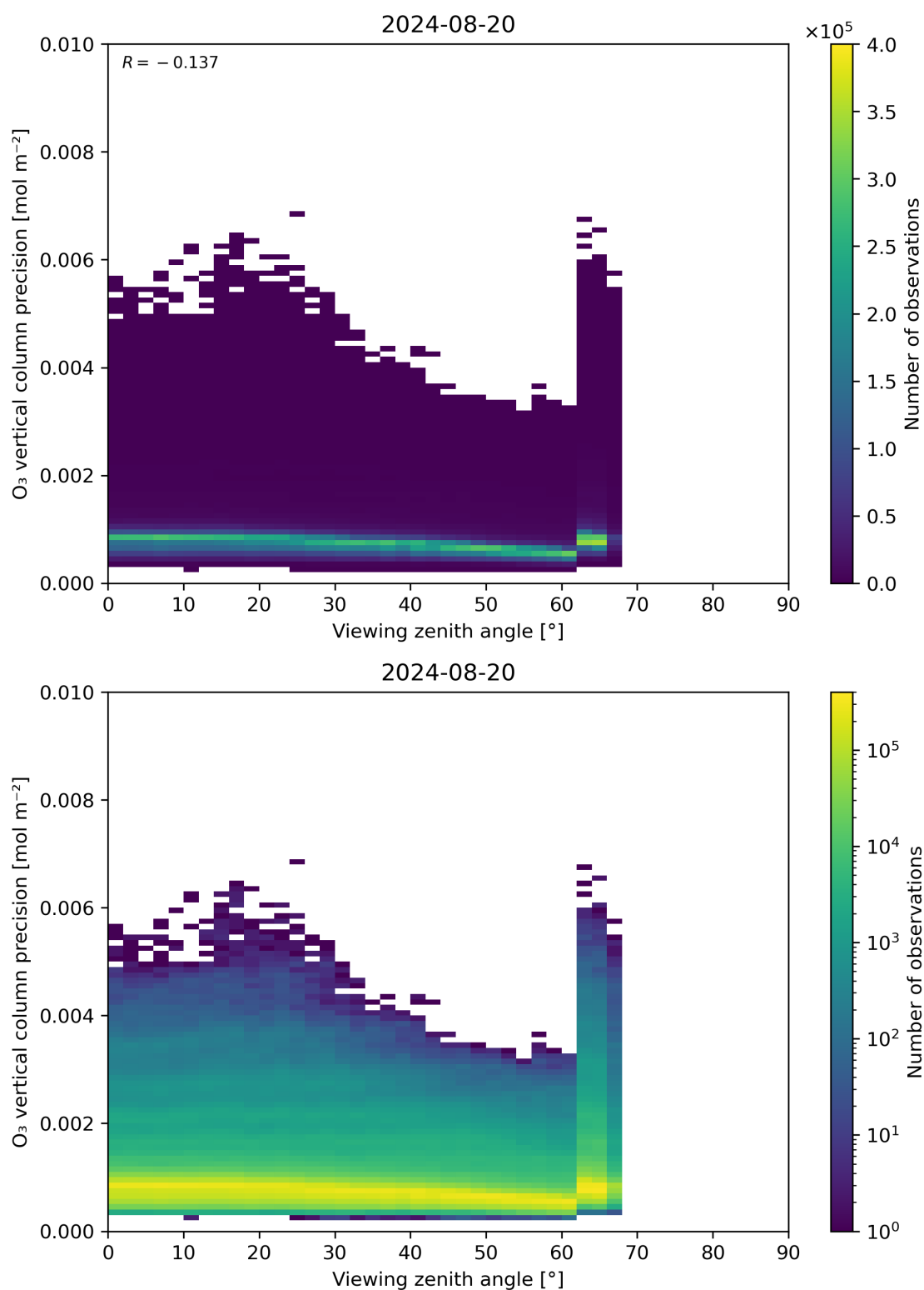
Figure 53: Scatter density plot of “Viewing zenith angle” against “O 3 vertical column precision” for 2024-08-19 to 2024-08-21.
