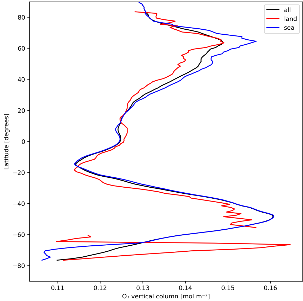
Figure 14: Zonal average of “O 3 vertical column” for 2024-08-19 to 2024-08-21.
