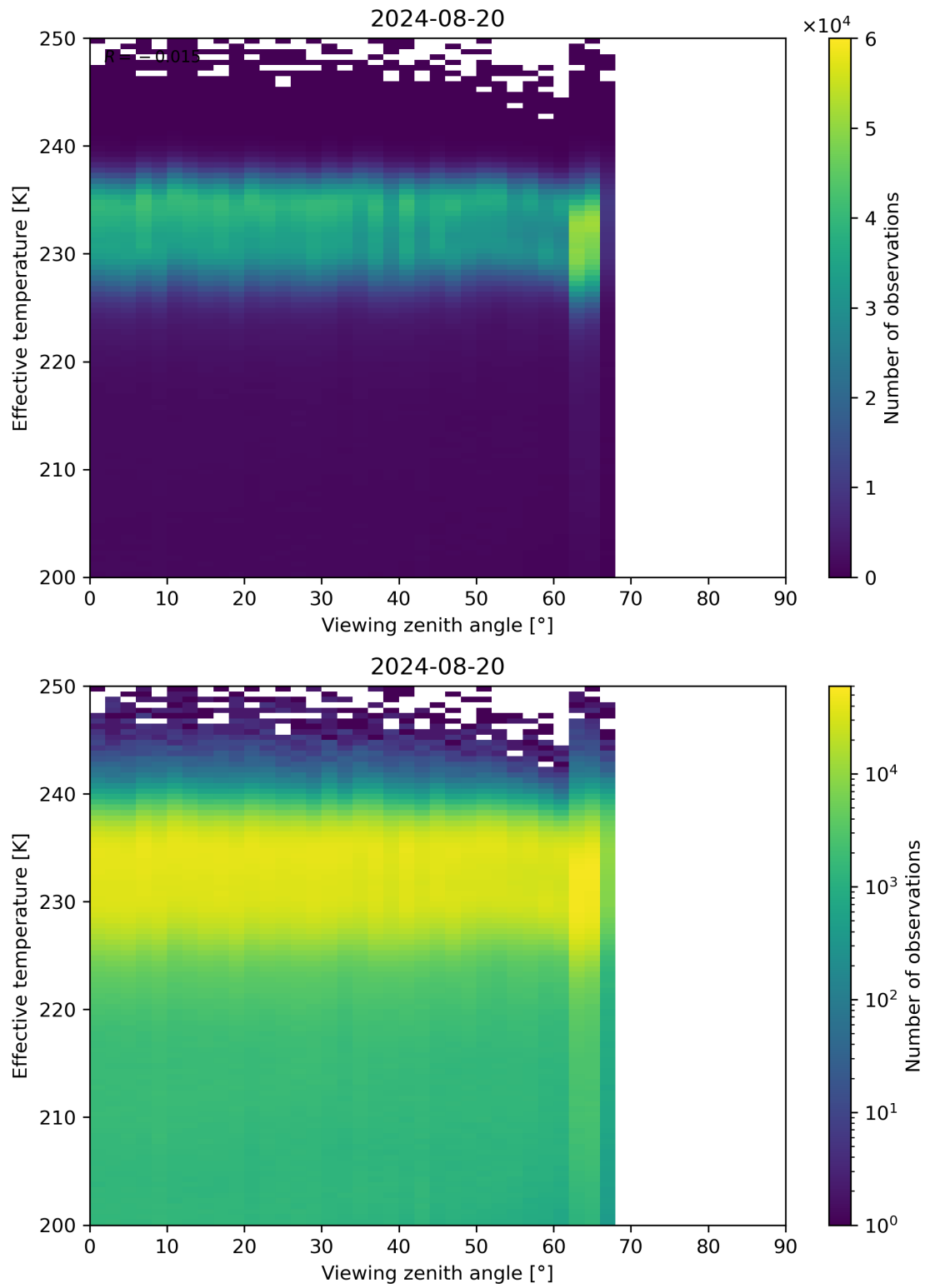
Figure 50: Scatter density plot of “Viewing zenith angle” against “Effective temperature” for 2024-08-19 to 2024-08-21.
