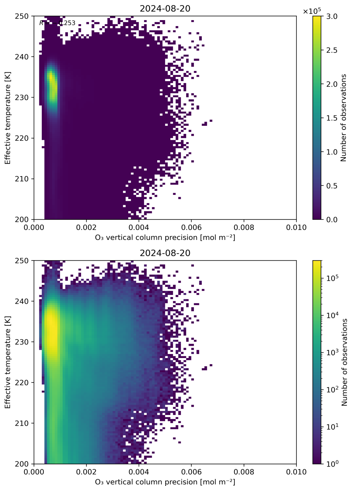
Figure 42: Scatter density plot of “O 3 vertical column precision” against “Effective temperature” for 2024-08-19 to 2024-08-21.
