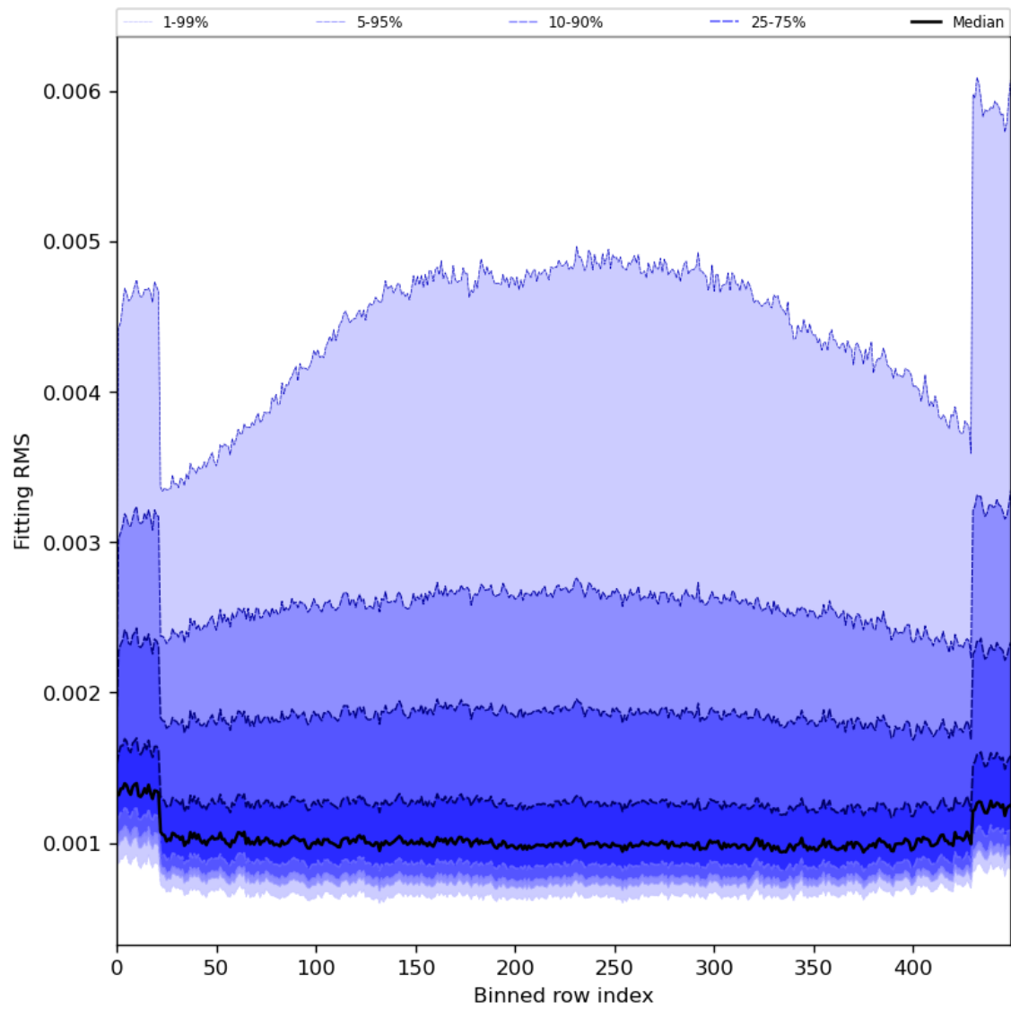
Figure 30: Along track statistics of “Fitting RMS” for 2024-08-19 to 2024-08-21
