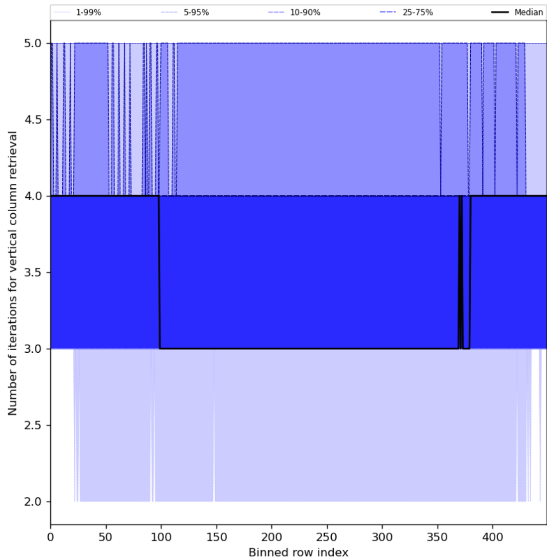
Figure 33: Along track statistics of “Number of iterations for vertical column retrieval” for 2024-08-19 to 2024-08-21
