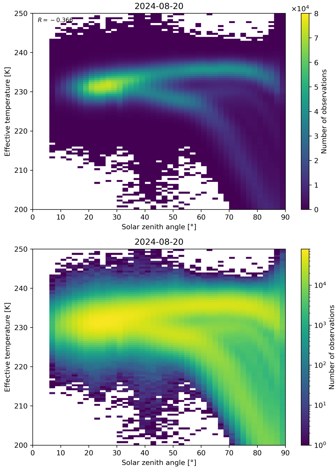
Figure 45: Scatter density plot of “Solar zenith angle” against “Effective temperature” for 2024-08-19 to 2024-08-21.
