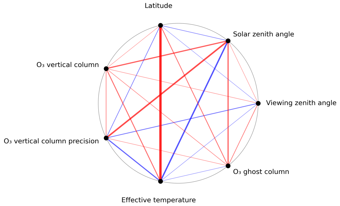
Figure 1: Map of correlation graph for 2024-08-19 to 2024-08-21.
