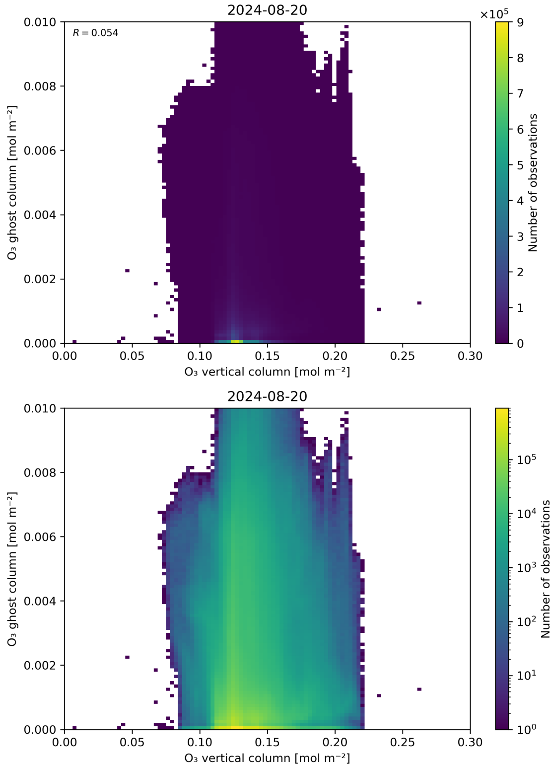
Figure 40: Scatter density plot of “O 3 vertical column” against “O 3 ghost column” for 2024-08-19 to 2024-08-21.
