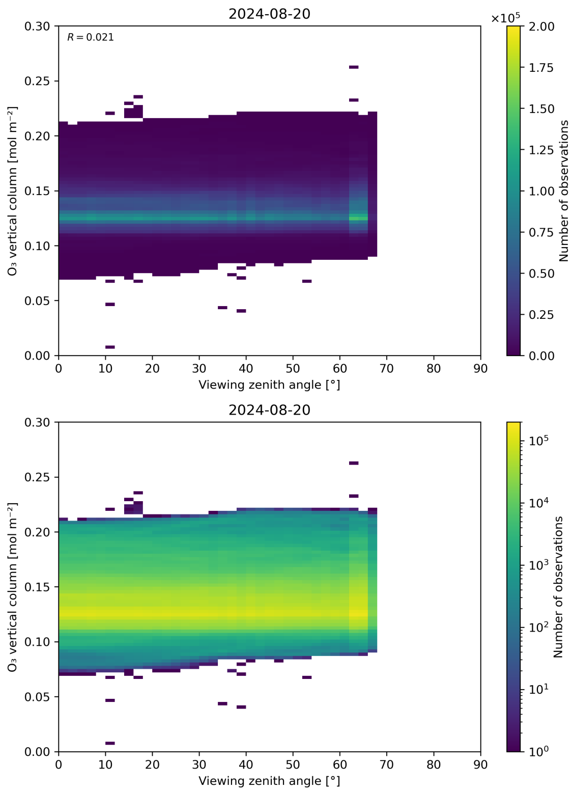
Figure 52: Scatter density plot of “Viewing zenith angle” against “O 3 vertical column” for 2024-08-19 to 2024-08-21.
