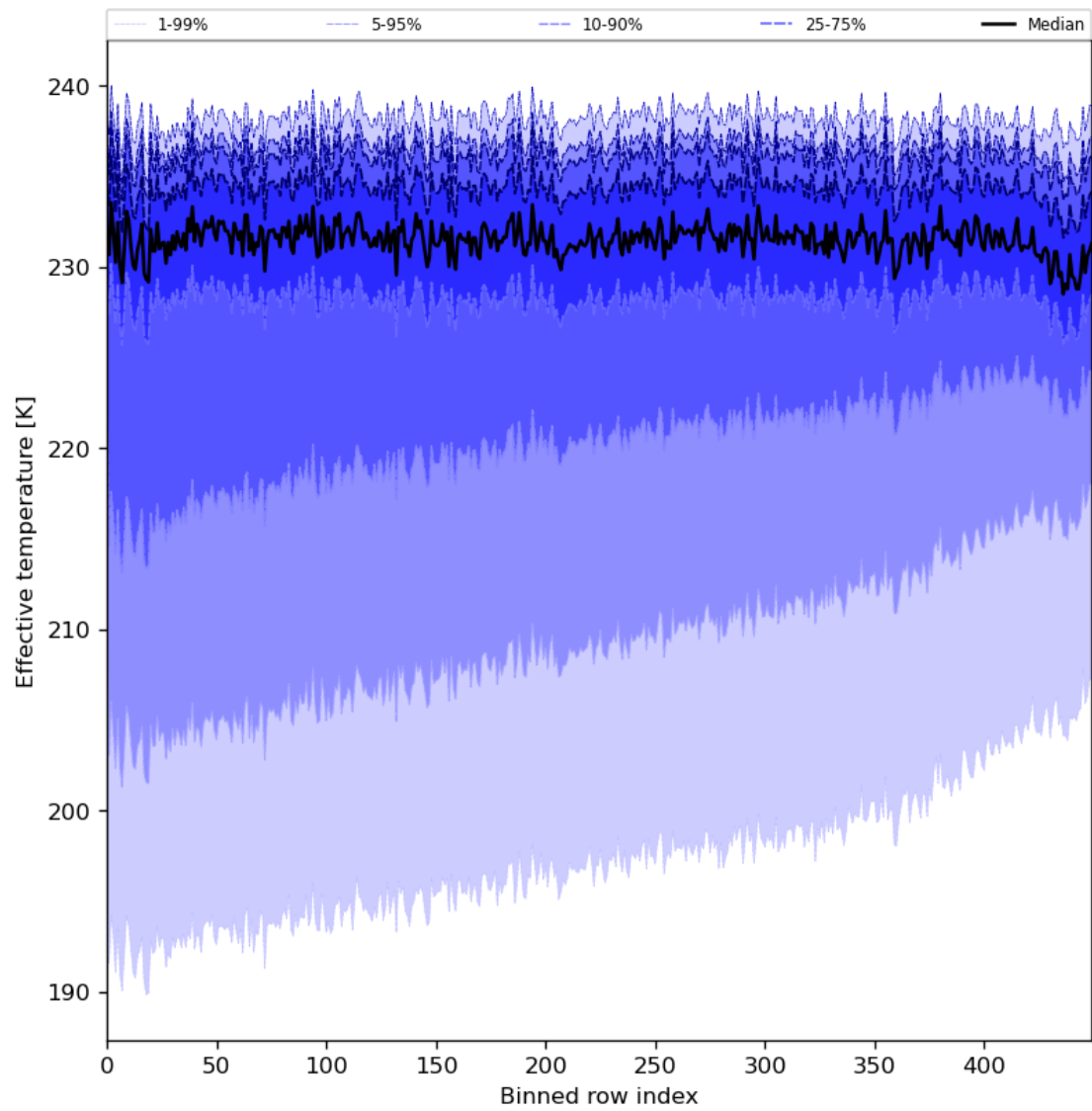
Figure 31: Along track statistics of “Effective temperature” for 2024-08-19 to 2024-08-21
