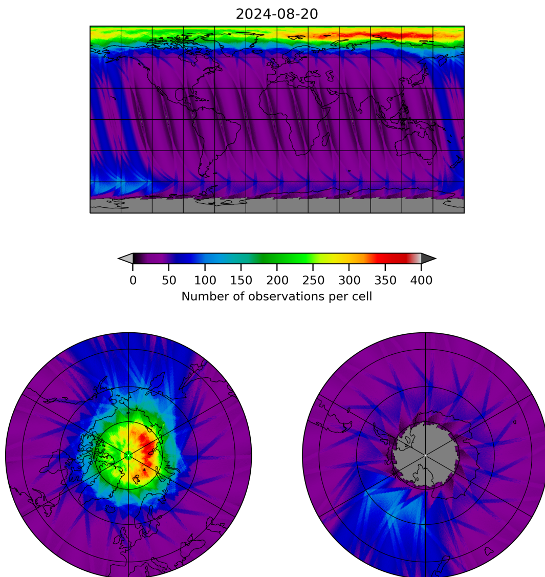
Figure 12: Map of the number of observations for 2024-08-19 to 2024-08-21
