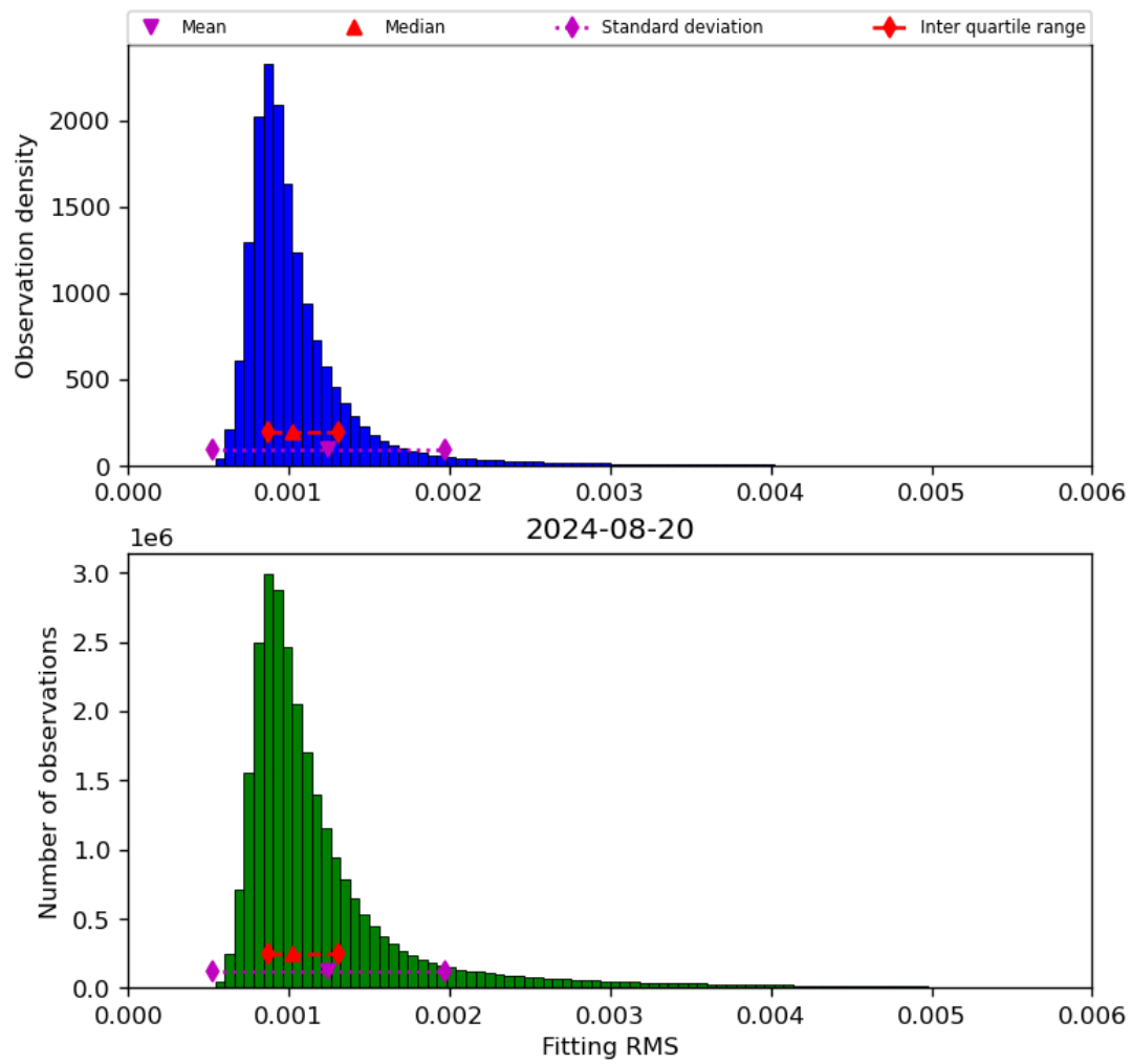
Figure 23: Histogram of “Fitting RMS” for 2024-08-19 to 2024-08-21
