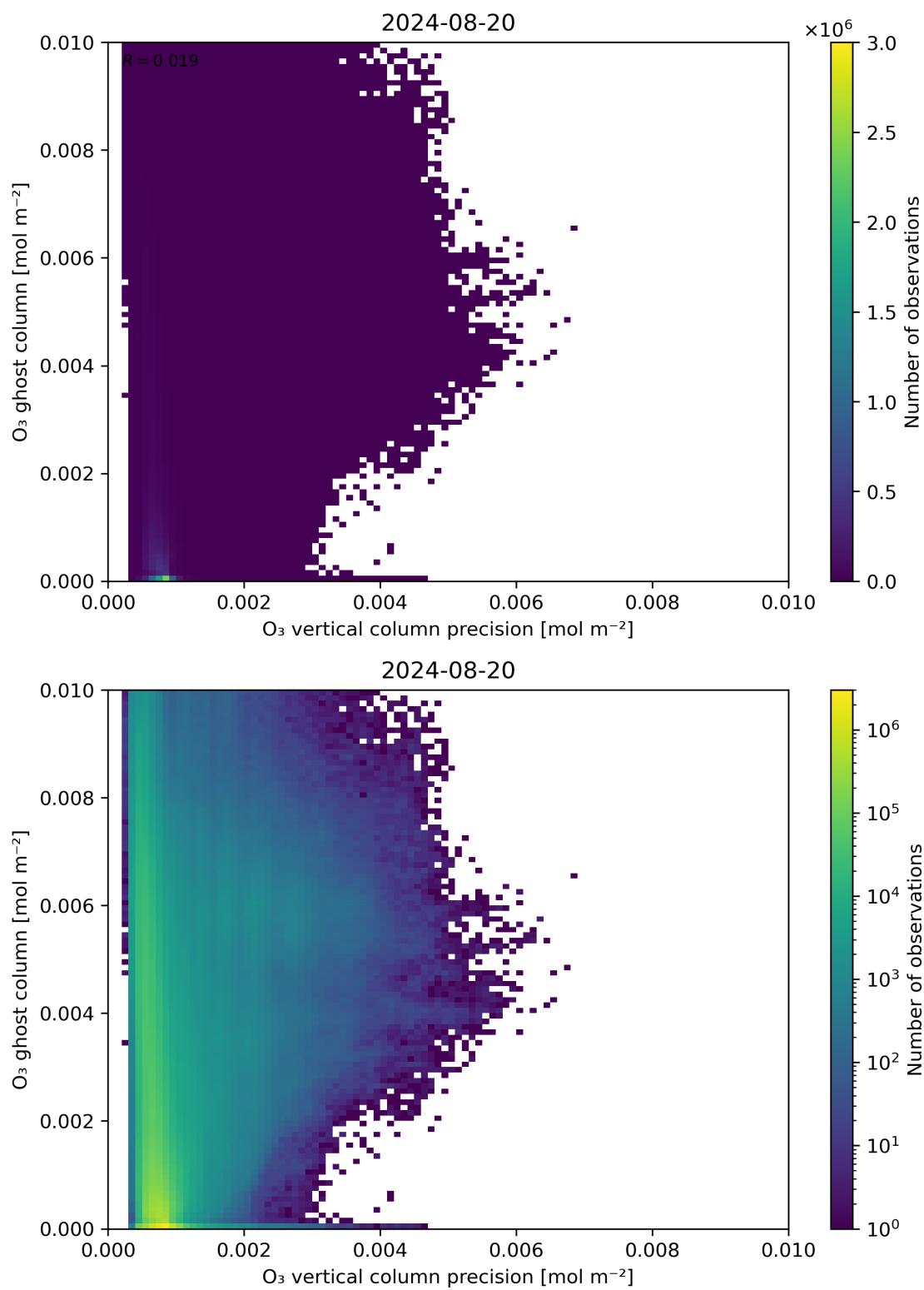
Figure 43: Scatter density plot of “ \text{O}_3 vertical column precision” against “ \text{O}_3 ghost column” for 2024-08-19 to 2024-08-21.
