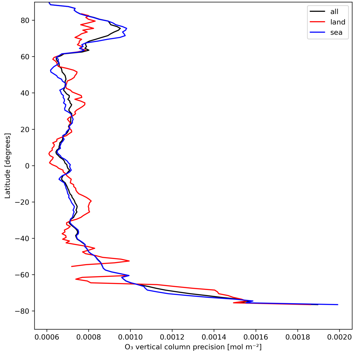
Figure 15: Zonal average of “O 3 vertical column precision” for 2024-08-19 to 2024-08-21.
