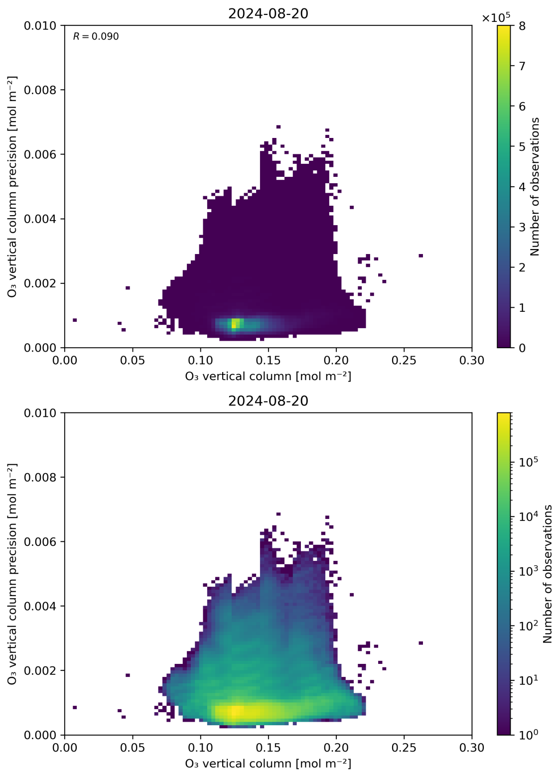
Figure 41: Scatter density plot of “O 3 vertical column” against “O 3 vertical column precision” for 2024-08-19 to 2024-08-21.
