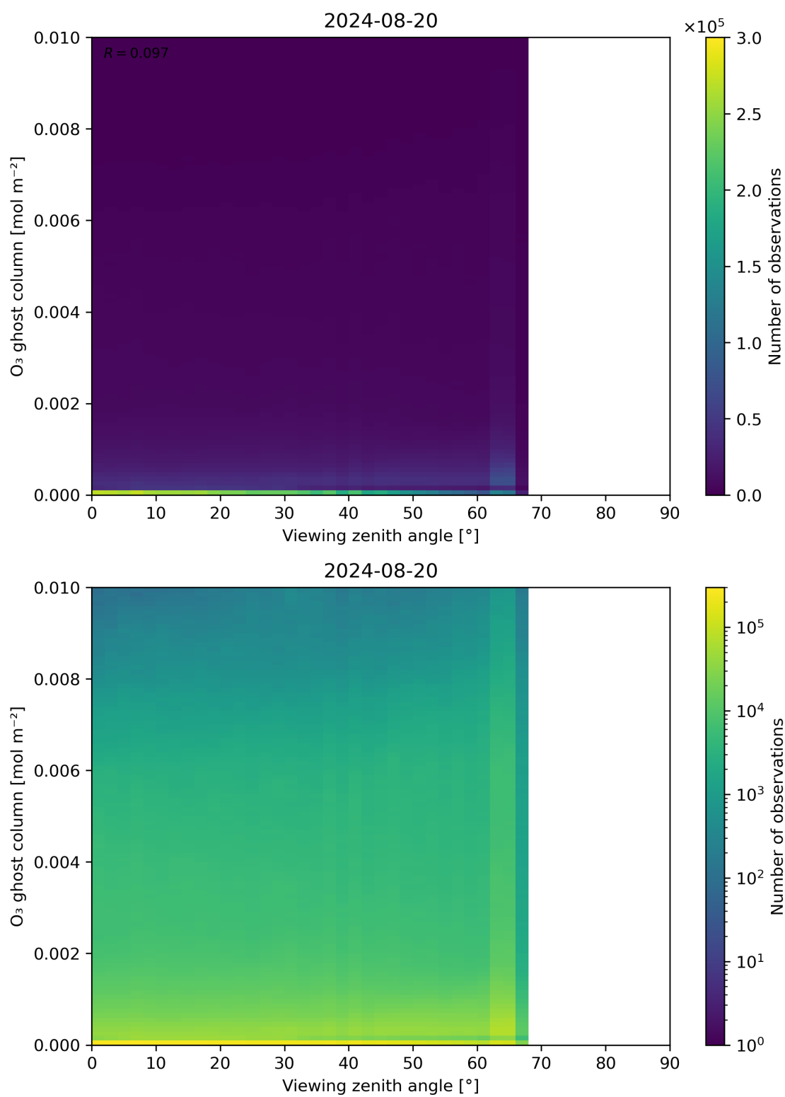
Figure 51: Scatter density plot of “Viewing zenith angle” against “O 3 ghost column” for 2024-08-19 to 2024-08-21.
