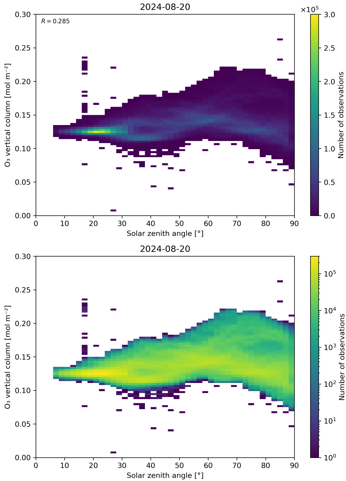
Figure 47: Scatter density plot of “Solar zenith angle” against “O 3 vertical column” for 2024-08-19 to 2024-08-21.
