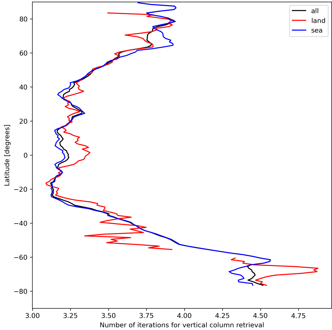
Figure 19: Zonal average of “Number of iterations for vertical column retrieval” for 2024-08-19 to 2024-08-21.
