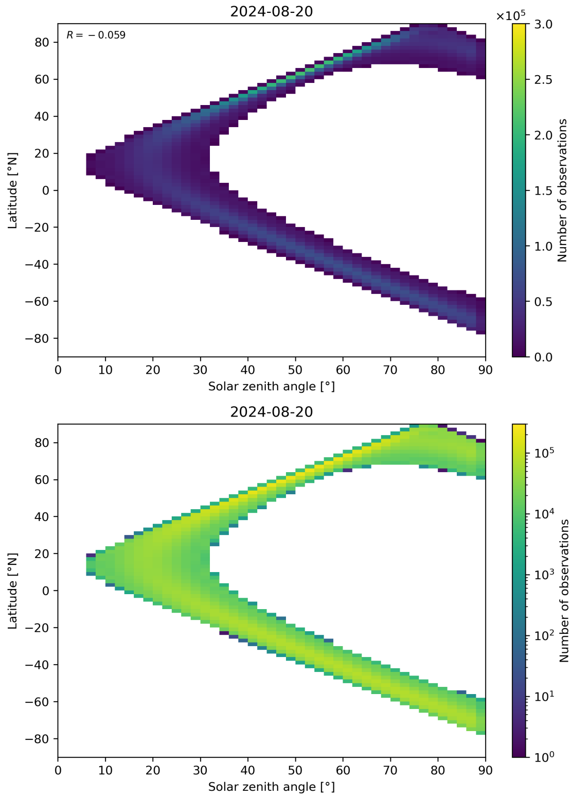
Figure 44: Scatter density plot of “Solar zenith angle” against “Latitude” for 2024-08-19 to 2024-08-21.
