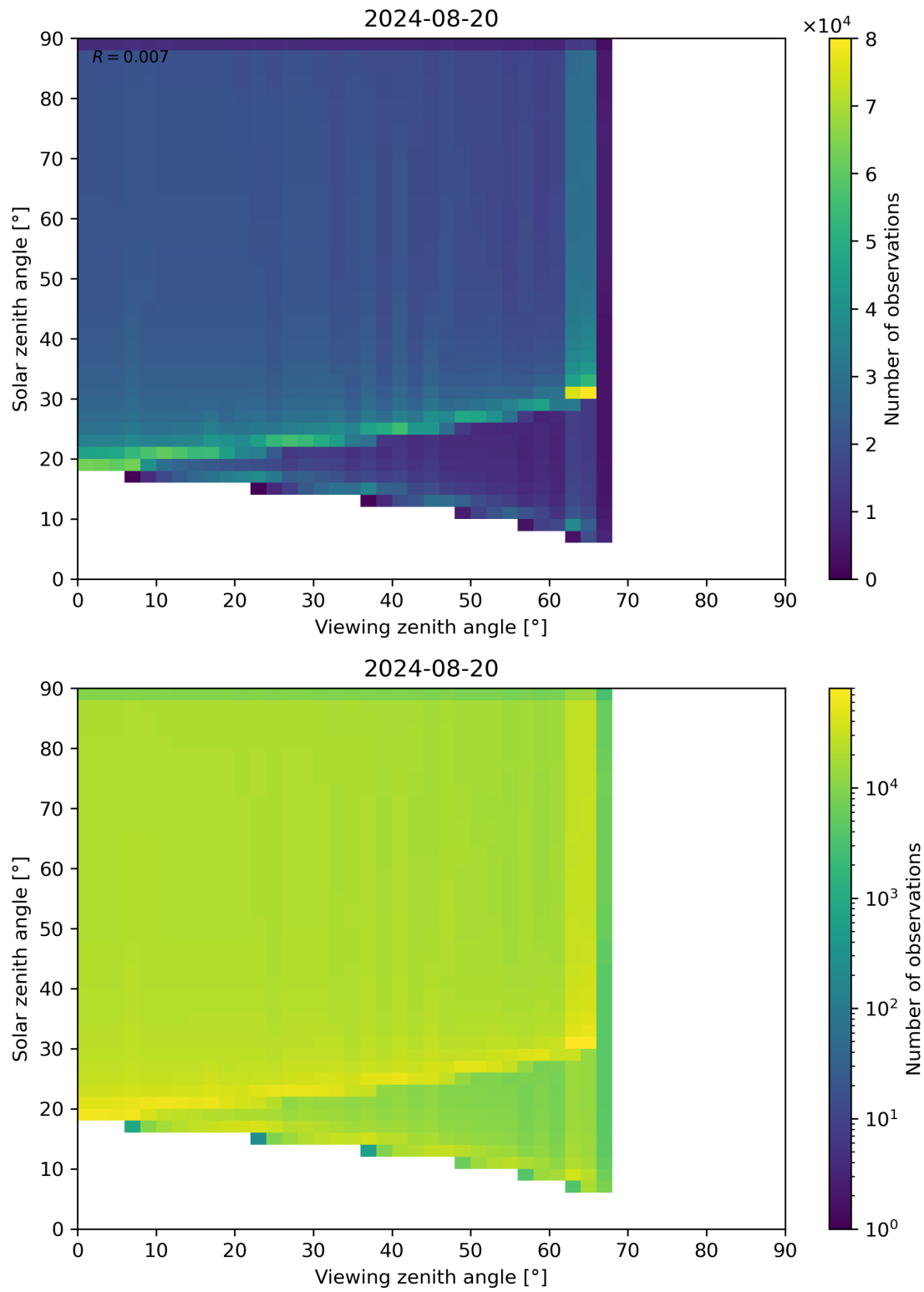
Figure 54: Scatter density plot of “Viewing zenith angle” against “Solar zenith angle” for 2024-08-19 to 2024-08-21.
