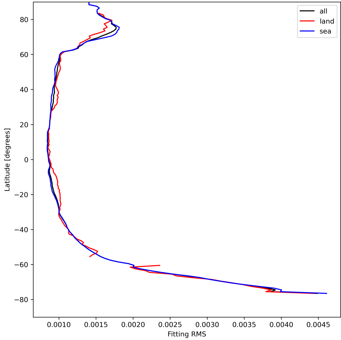
Figure 16: Zonal average of “Fitting RMS” for 2024-08-19 to 2024-08-21.
