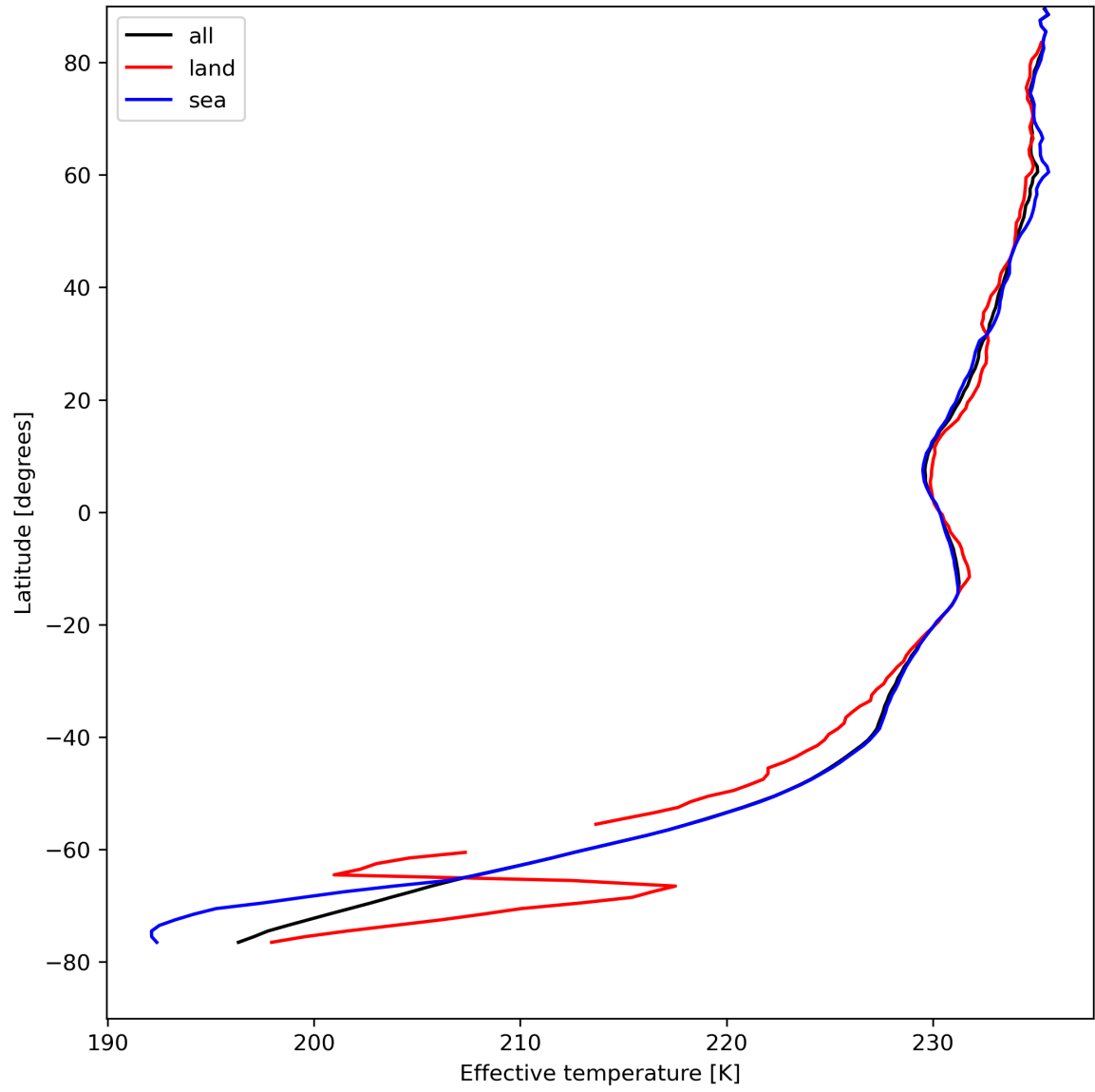
Figure 17: Zonal average of "Effective temperature" for 2024-08-19 to 2024-08-21.
