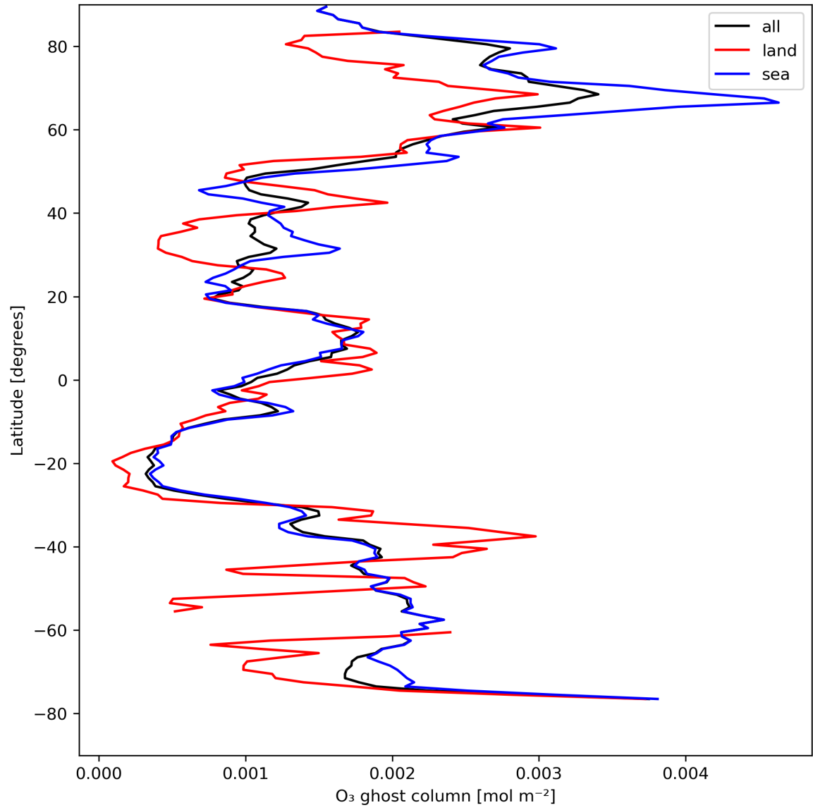
Figure 18: Zonal average of "O 3 ghost column" for 2024-08-19 to 2024-08-21.
