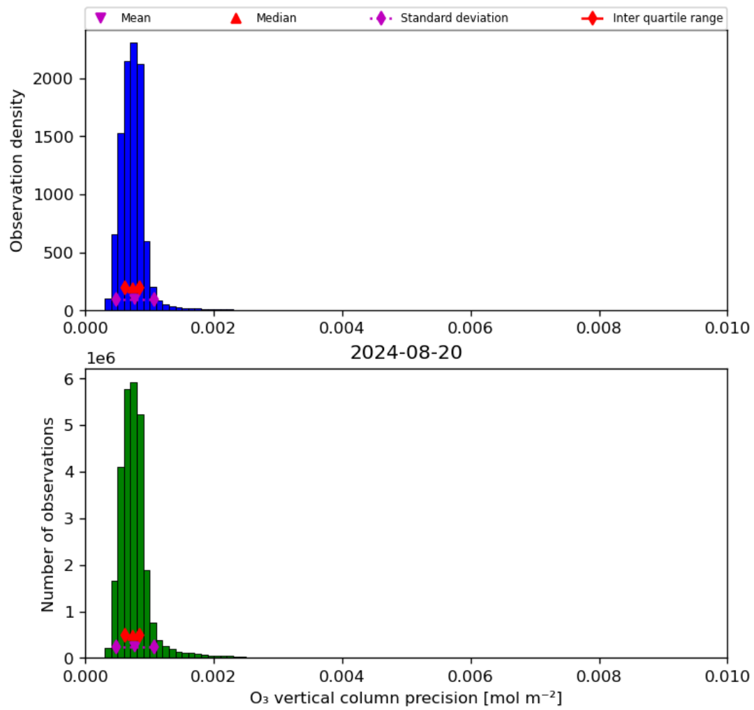
Figure 22: Histogram of “O 3 vertical column precision” for 2024-08-19 to 2024-08-21
