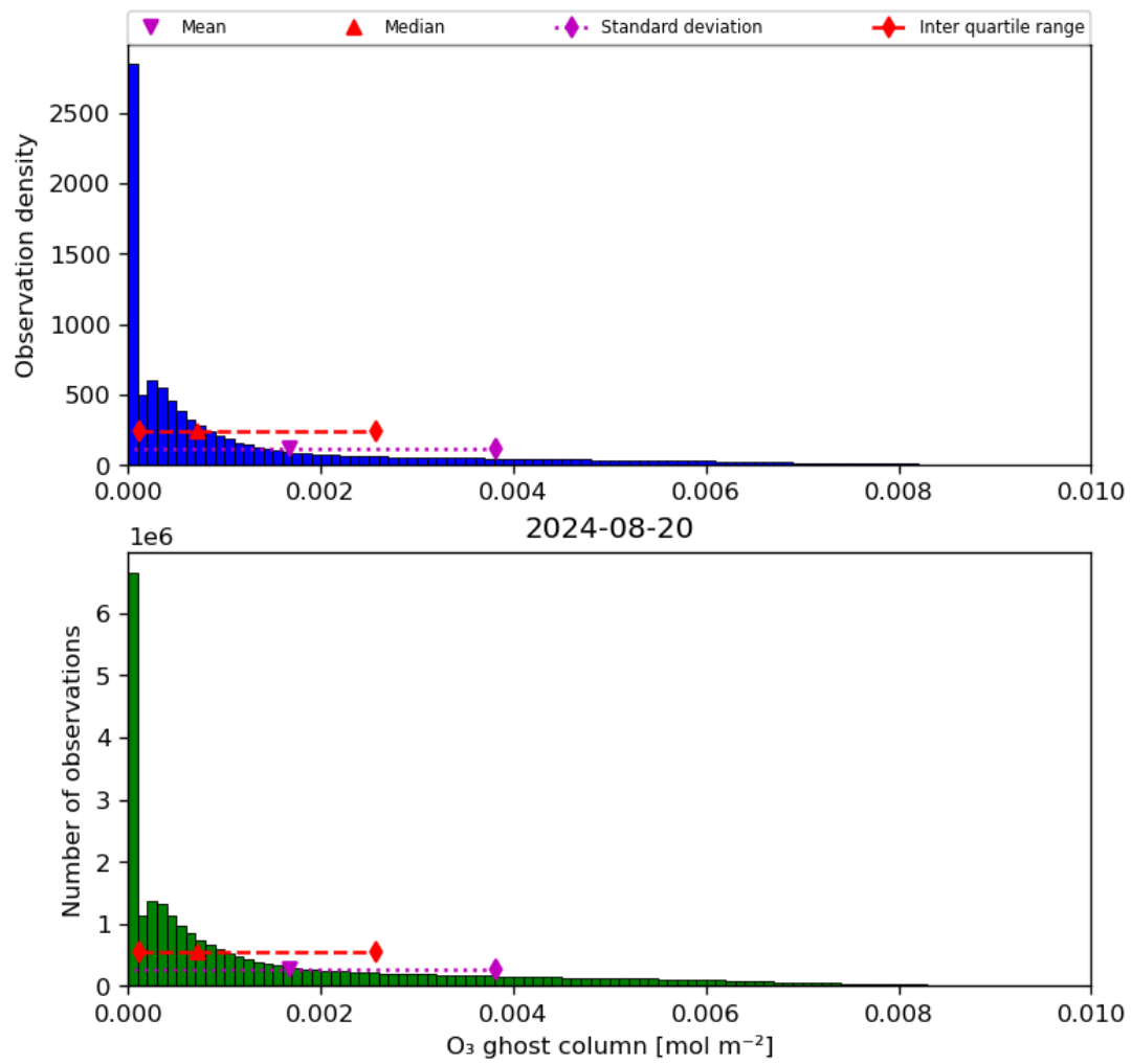
Figure 25: Histogram of “O 3 ghost column” for 2024-08-19 to 2024-08-21
