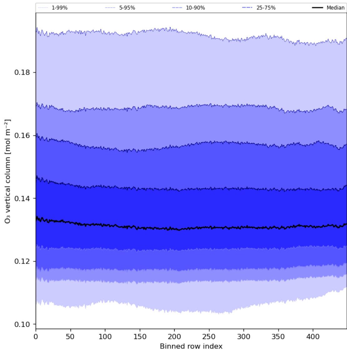
Figure 28: Along track statistics of “O 3 vertical column” for 2024-08-19 to 2024-08-21
