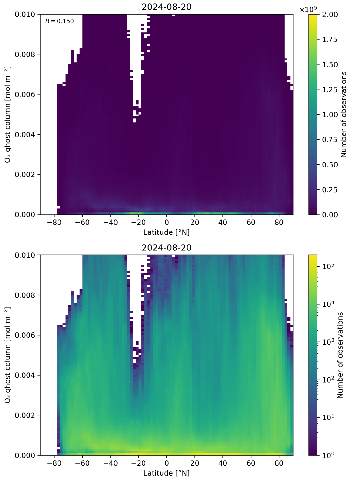
Figure 35: Scatter density plot of “Latitude” against “O 3 ghost column” for 2024-08-19 to 2024-08-21.
