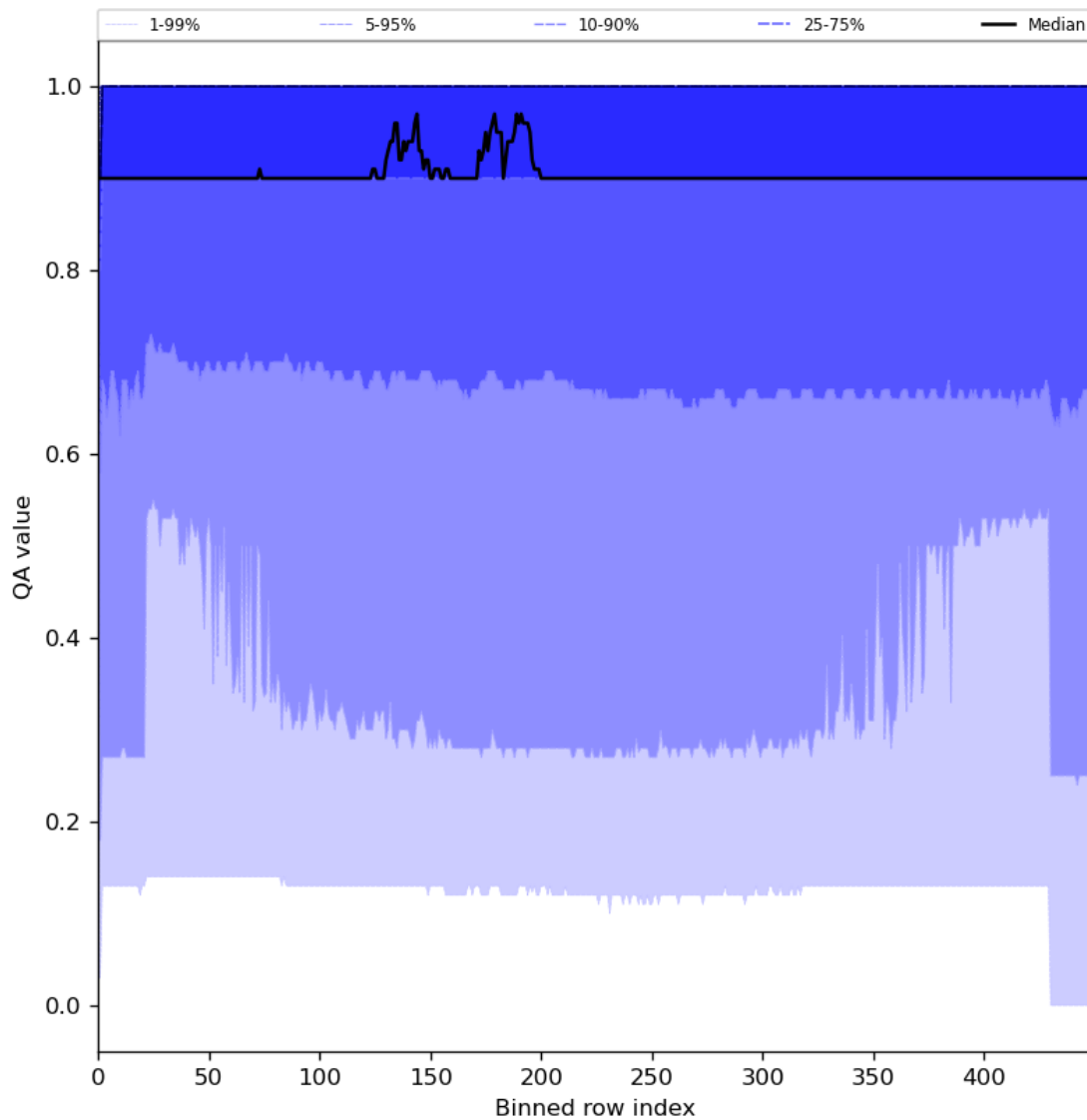
Figure 27: Along track statistics of “QA value” for 2024-08-19 to 2024-08-21
