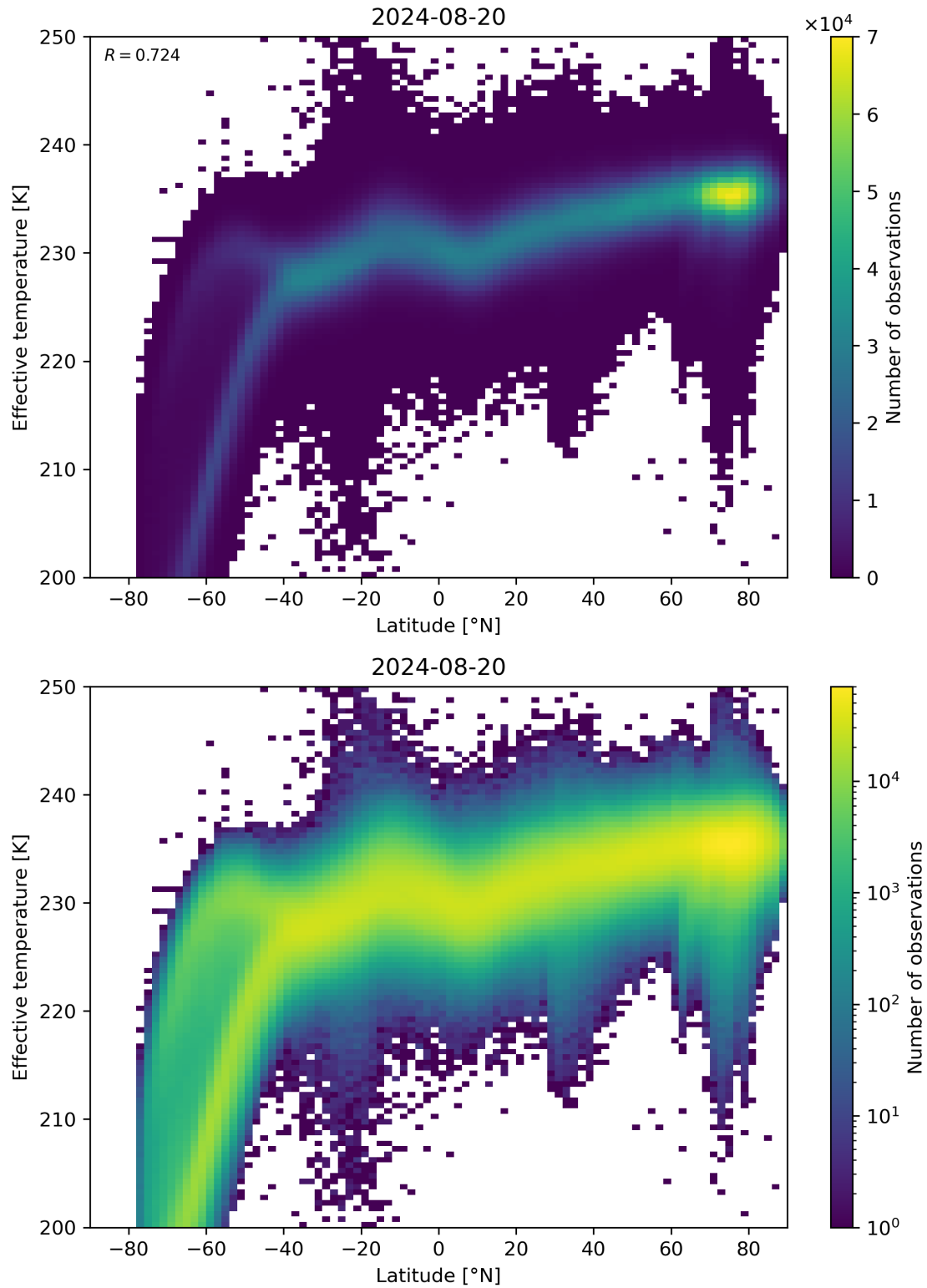
Figure 34: Scatter density plot of “Latitude” against “Effective temperature” for 2024-08-19 to 2024-08-21.
