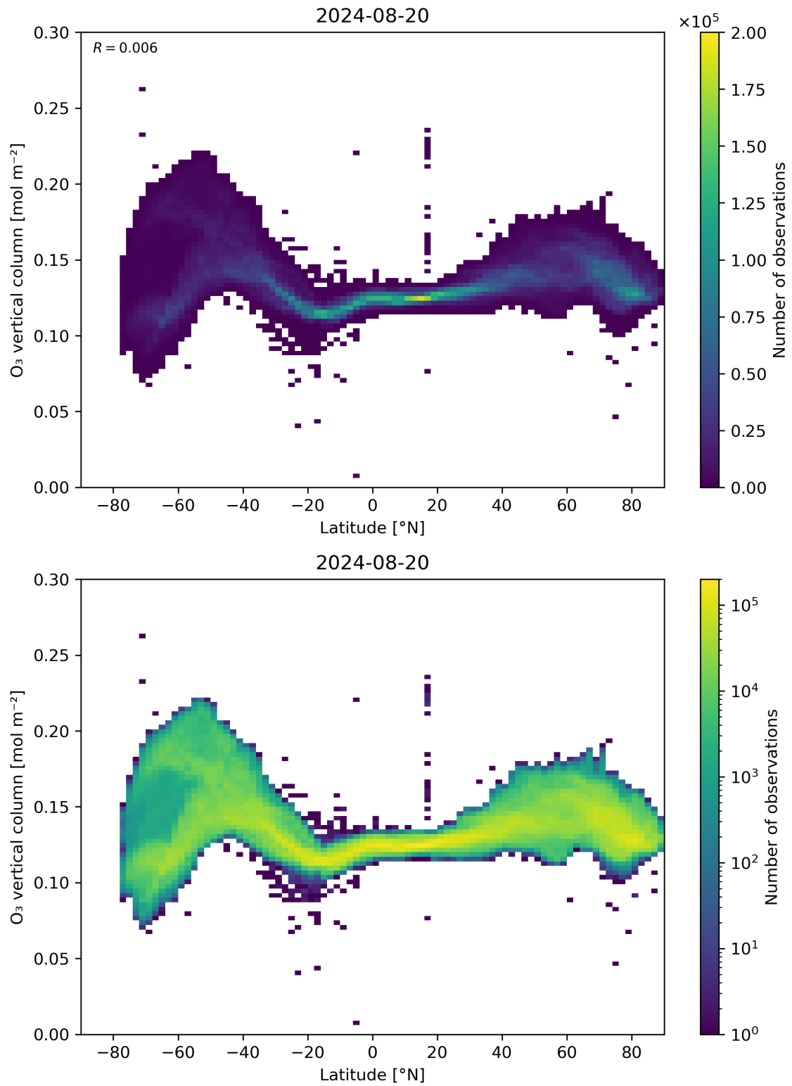
Figure 36: Scatter density plot of “Latitude” against “O 3 vertical column” for 2024-08-19 to 2024-08-21.
