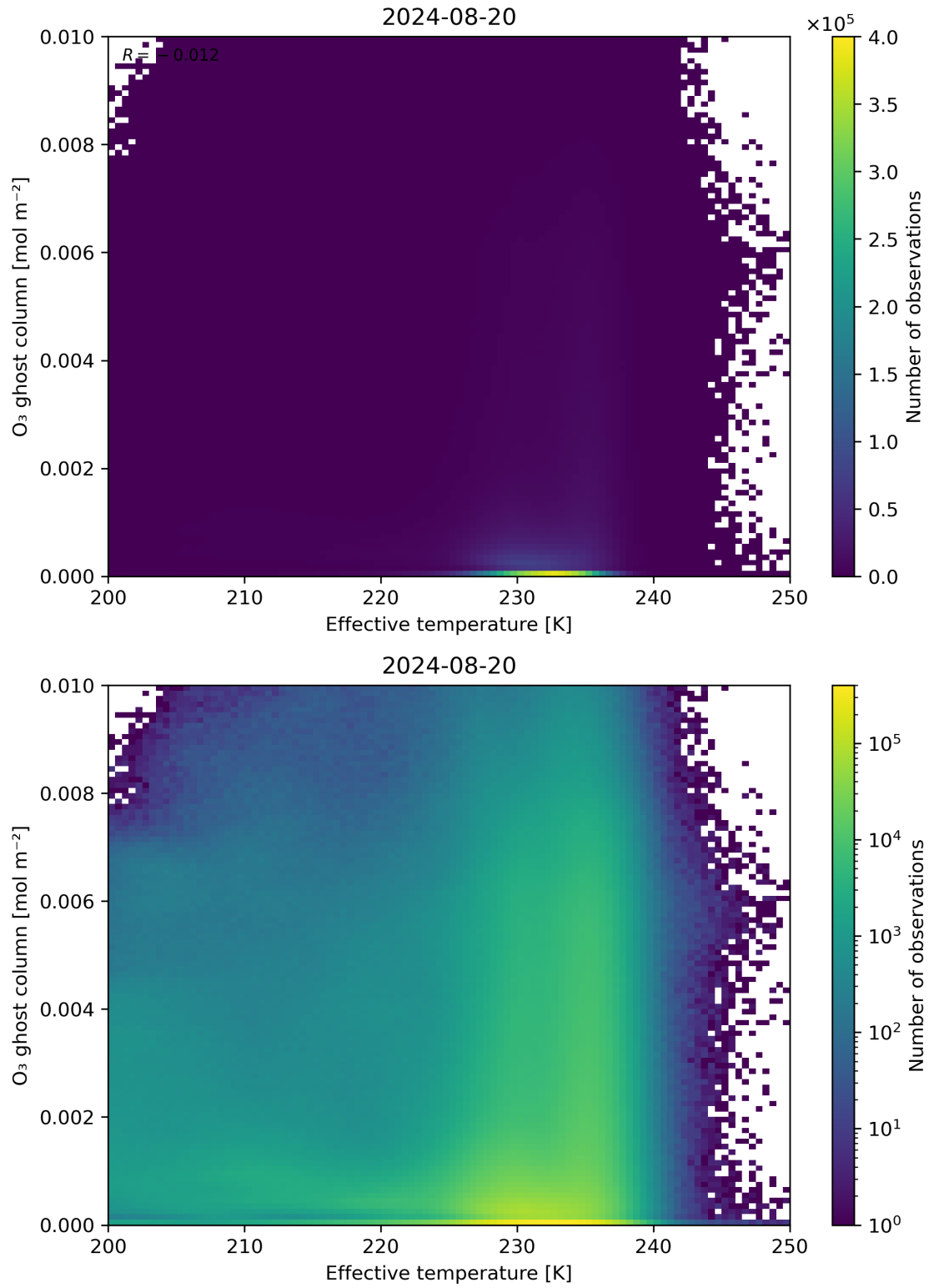
Figure 38: Scatter density plot of “Effective temperature” against “O 3 ghost column” for 2024-08-19 to 2024-08-21.
