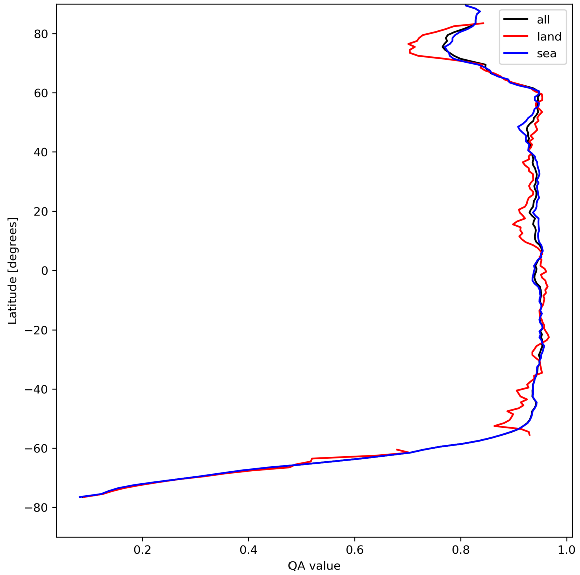
Figure 13: Zonal average of “QA value” for 2024-08-19 to 2024-08-21.
