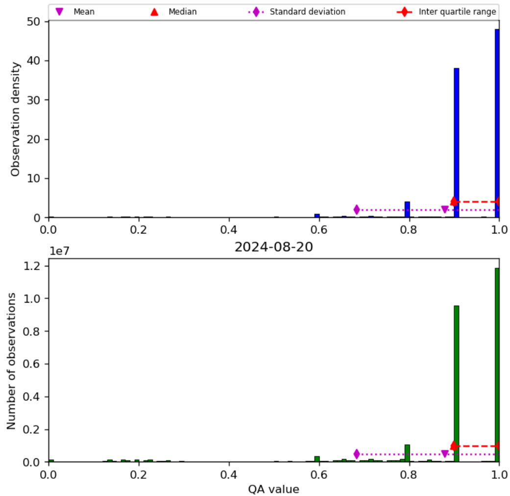
Figure 20: Histogram of “QA value” for 2024-08-19 to 2024-08-21
