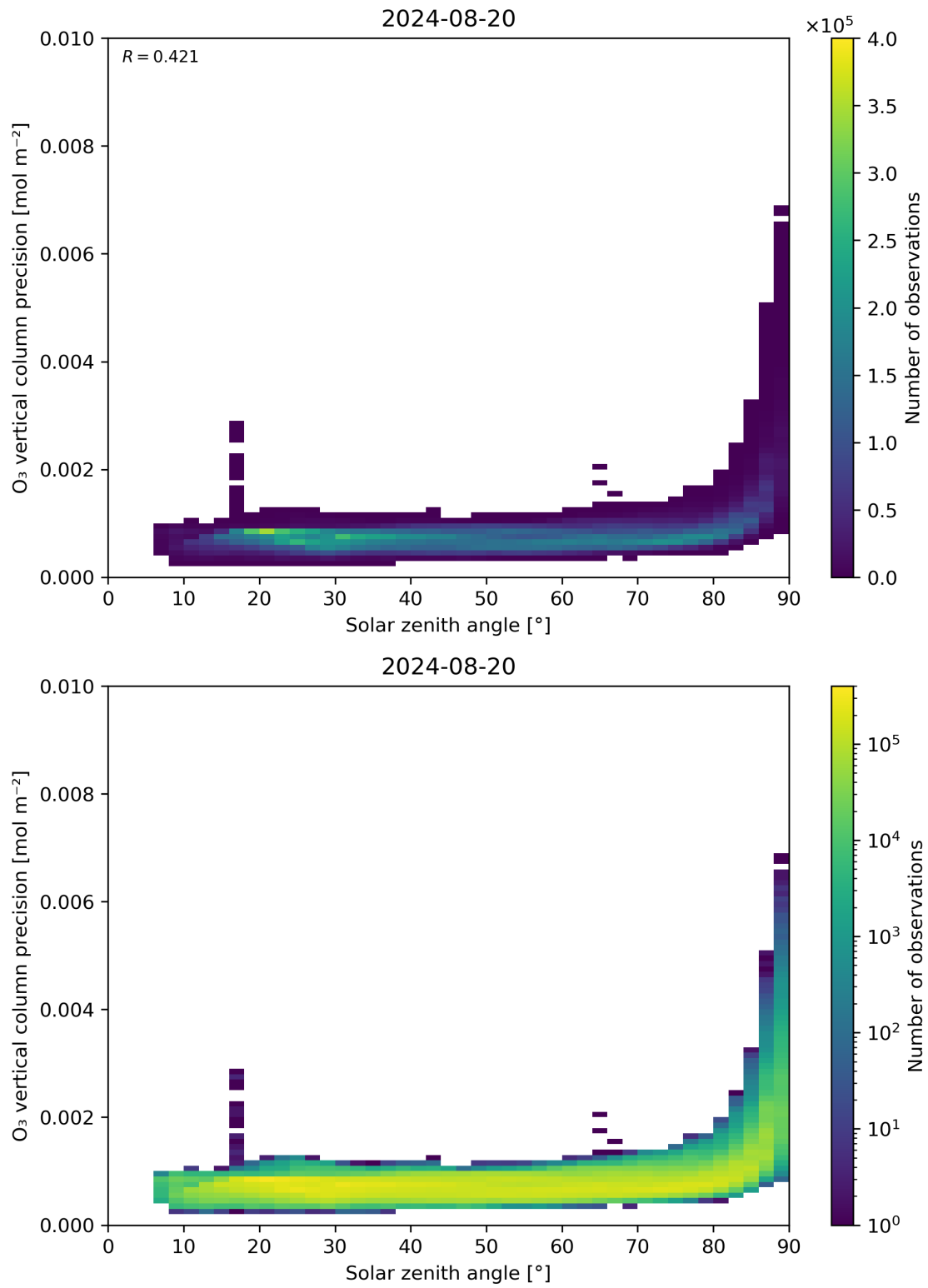
Figure 48: Scatter density plot of “Solar zenith angle” against “O 3 vertical column precision” for 2024-08-19 to 2024-08-21.
