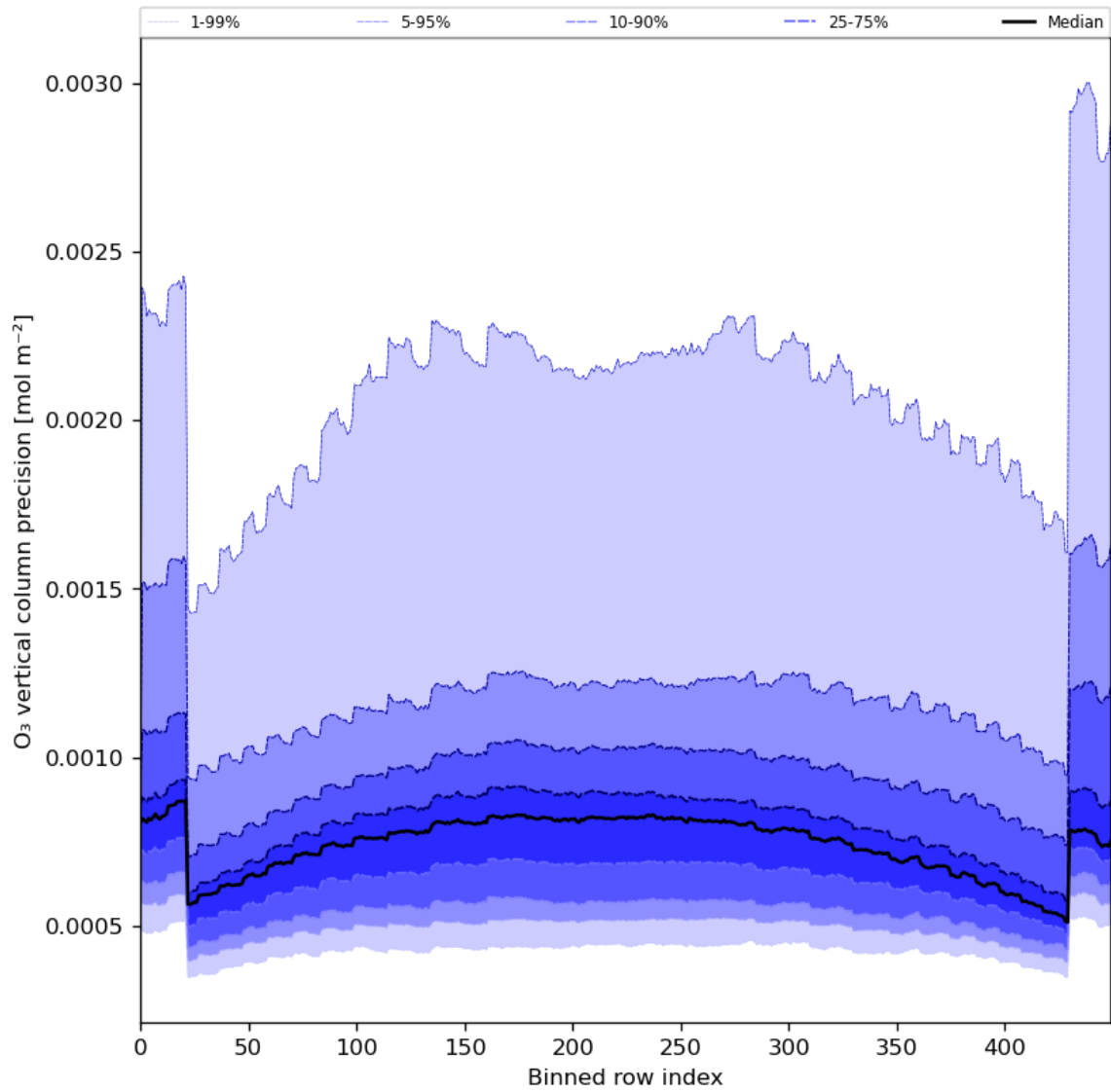
Figure 29: Along track statistics of “O 3 vertical column precision” for 2024-08-19 to 2024-08-21
