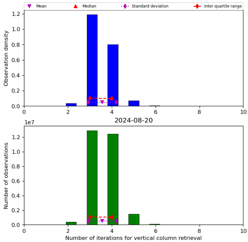
Figure 26: Histogram of “Number of iterations for vertical column retrieval” for 2024-08-19 to 2024-08-21
