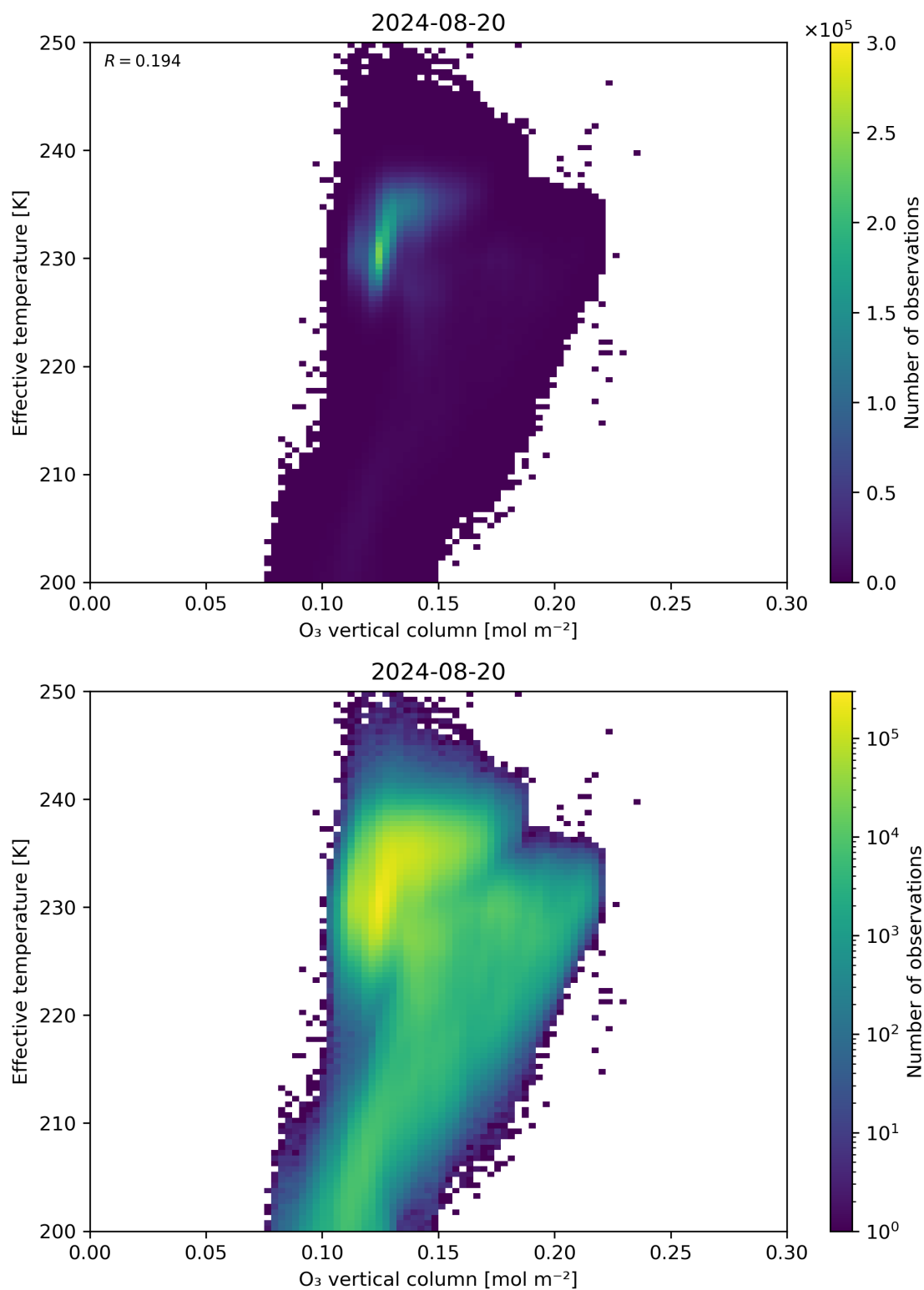
Figure 39: Scatter density plot of “O 3 vertical column” against “Effective temperature” for 2024-08-19 to 2024-08-21.
