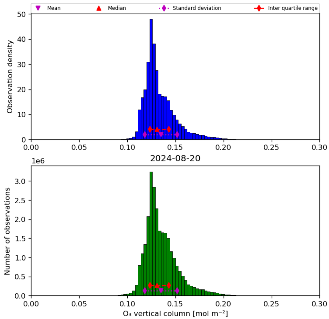
Figure 21: Histogram of “O 3 vertical column” for 2024-08-19 to 2024-08-21
