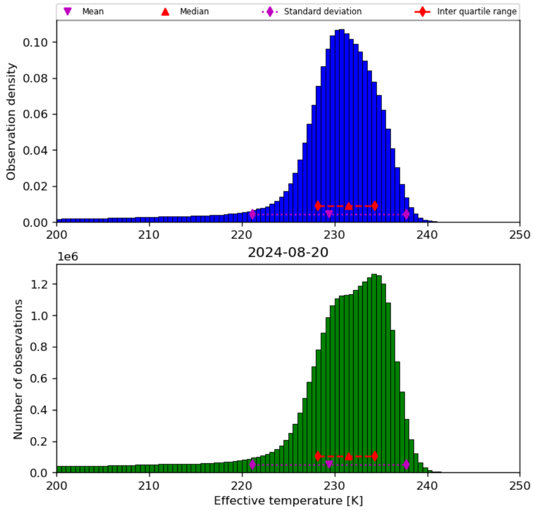
Figure 24: Histogram of “Effective temperature” for 2024-08-19 to 2024-08-21
