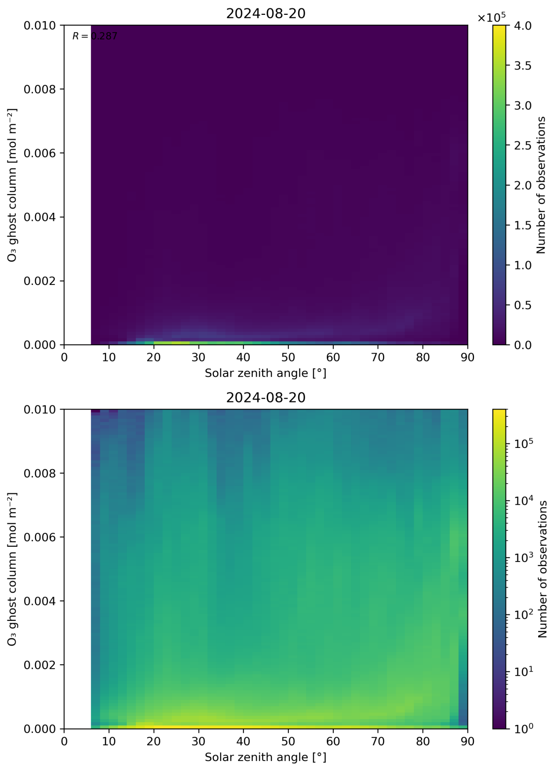
Figure 46: Scatter density plot of “Solar zenith angle” against “O 3 ghost column” for 2024-08-19 to 2024-08-21.
