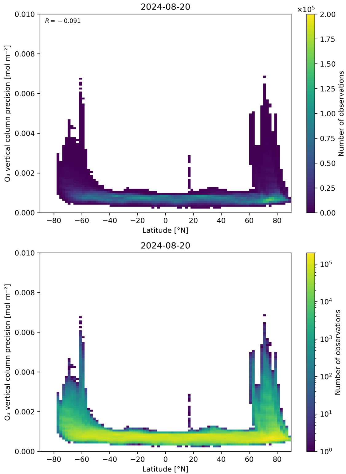
Figure 37: Scatter density plot of “Latitude” against “O 3 vertical column precision” for 2024-08-19 to 2024-08-21.
