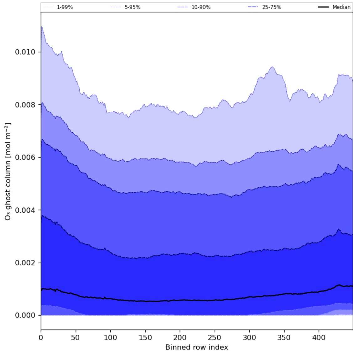
Figure 32: Along track statistics of “O 3 ghost column” for 2024-08-19 to 2024-08-21
